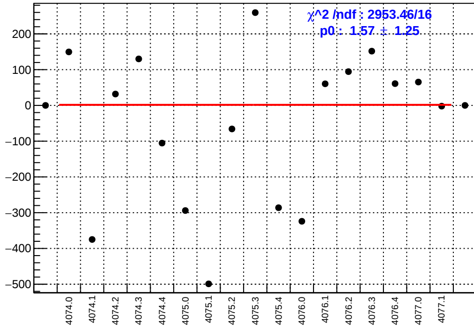
slug43-Left: asym_left_dd.mean/ppb-reg_asym_left_dd.mean/ppb
