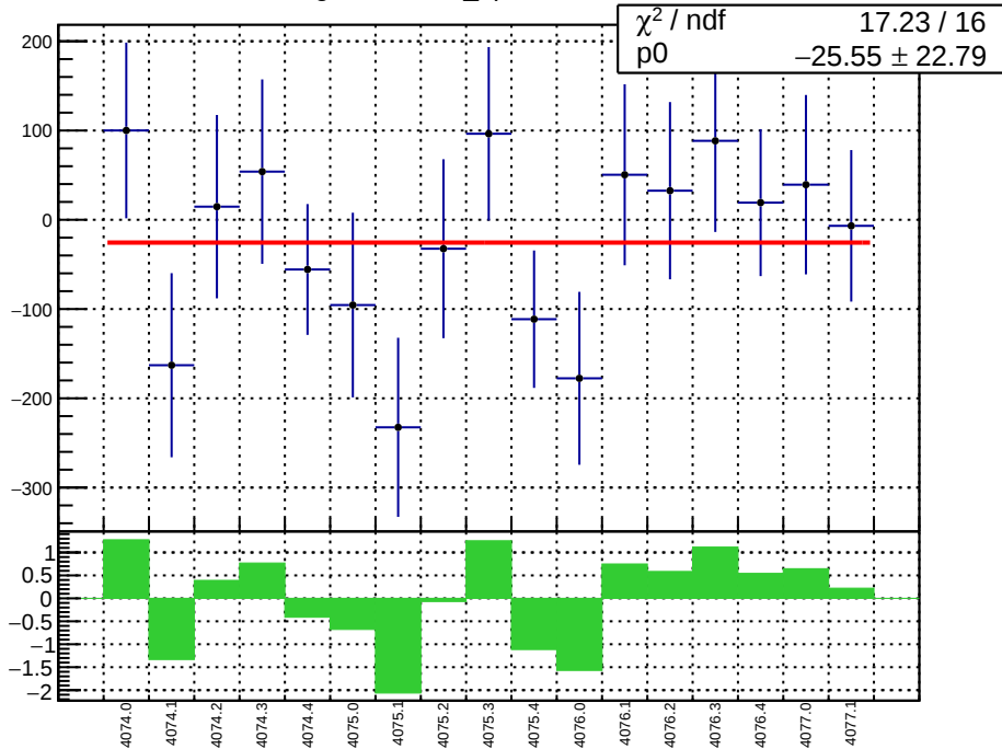
slug43-Left: diff_bpm4eX.mean/nm
