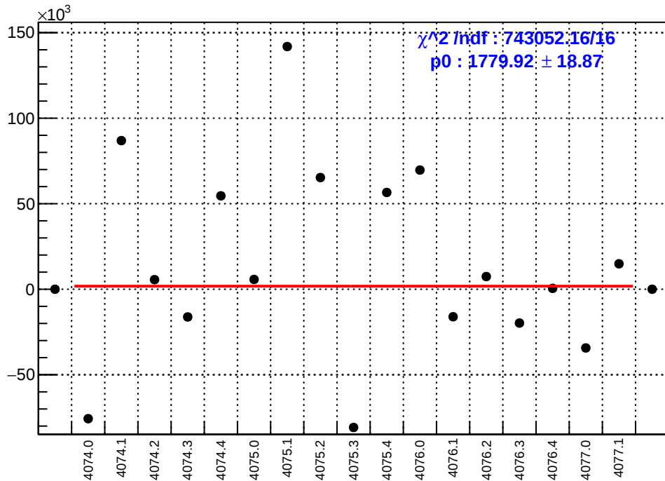
slug43-Left: asym_sam4.mean/ppb-reg_asym_sam4.mean/ppb
