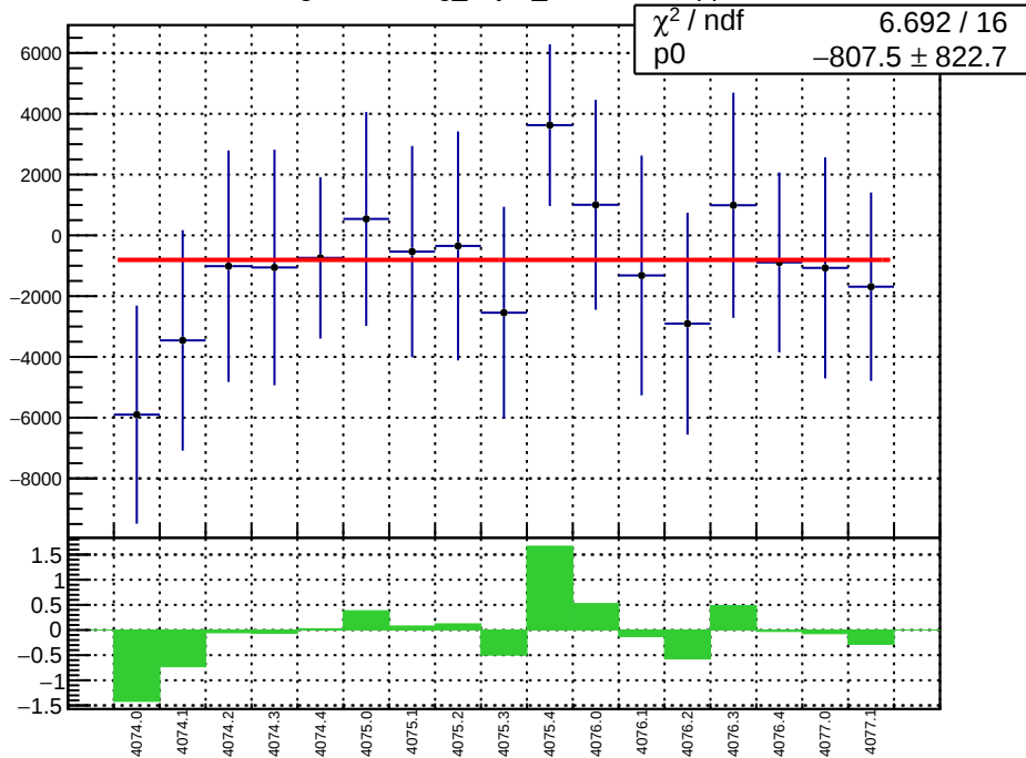
slug43-Left: reg_asym_sam5.mean/ppb
