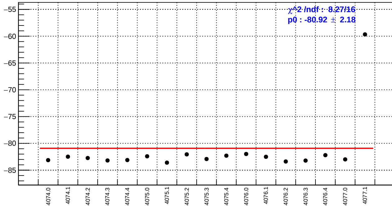
slug43-Left: us_avg_bpm12X/(ppb/nm)
