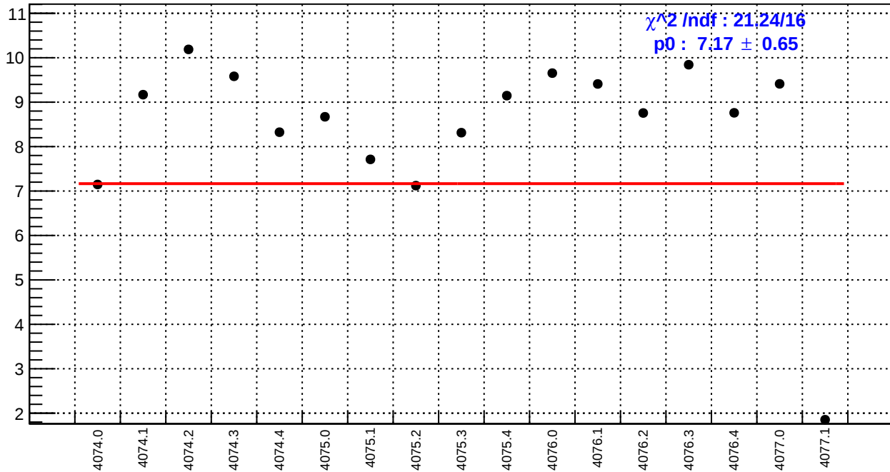
slug43-Left: us_avg_bpm4aY/(ppb/nm)
