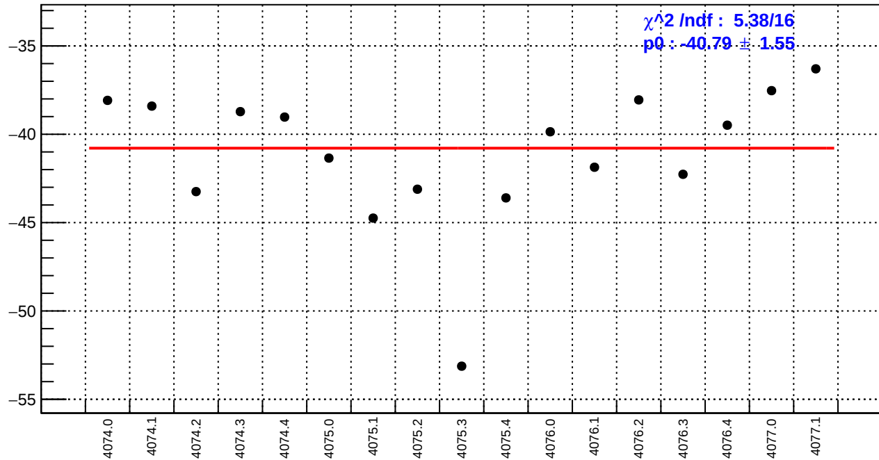
slug43-Left: dsr_bpm4aX/(ppb/nm)
