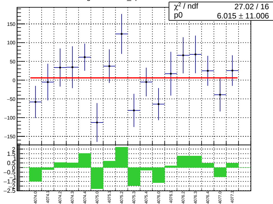
slug43-Left: diff_bpm4eY.mean/nm
