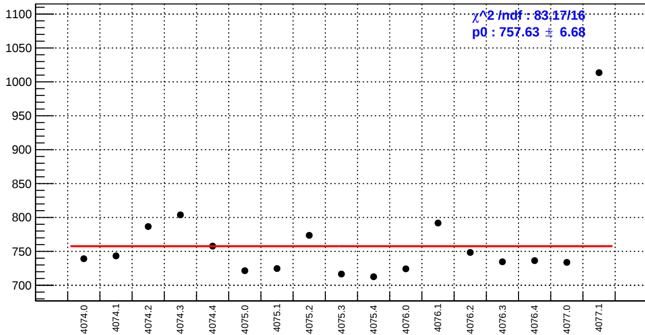
slug43-Left: reg_asym_sam3.rms/ppm
