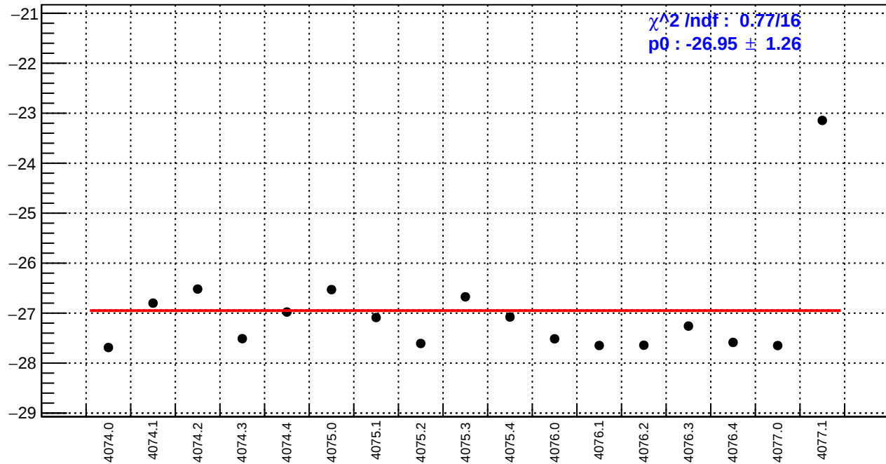
slug43-Left: ds_avg_bpm4eX/(ppb/nm)
