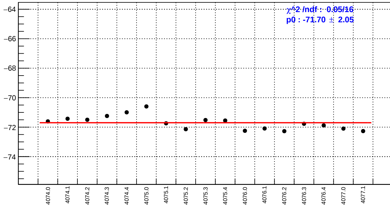
slug43-Left: left_avg_bpm4eX/(ppb/nm)
