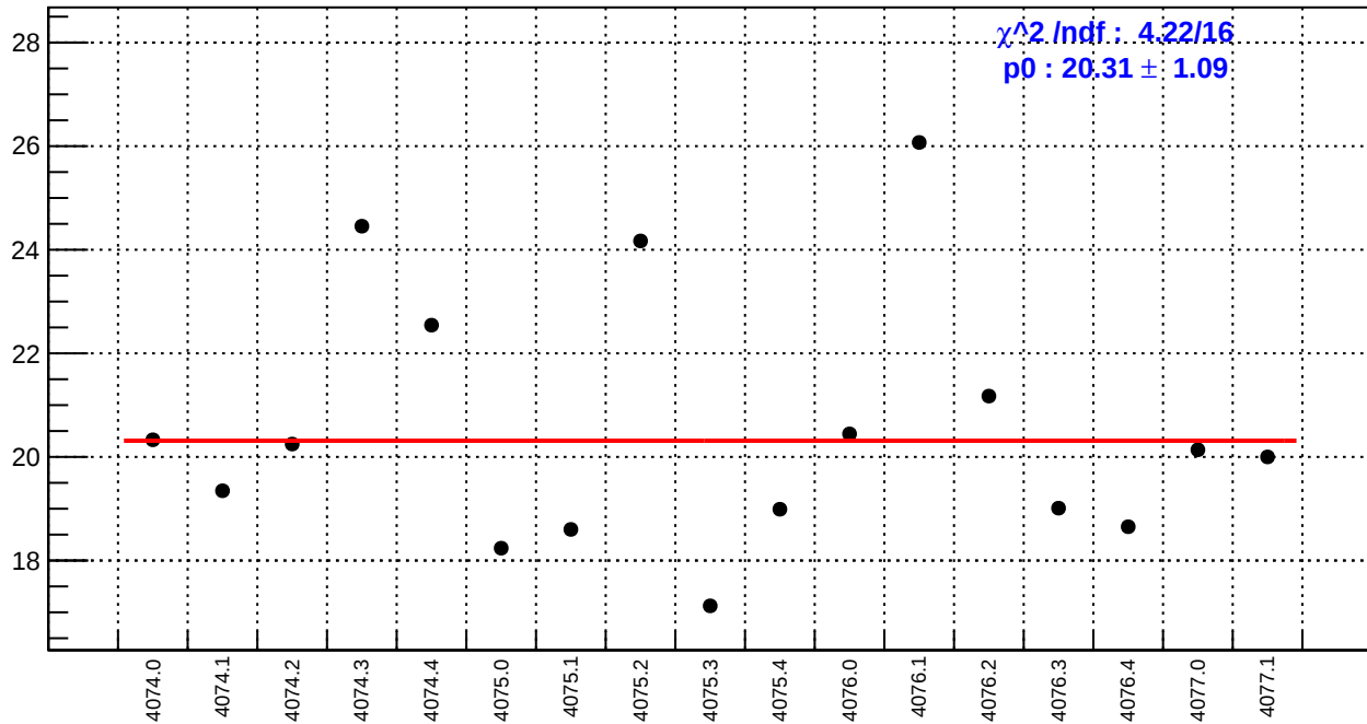
slug43-Left: usl_bpm4aX/(ppb/nm)
