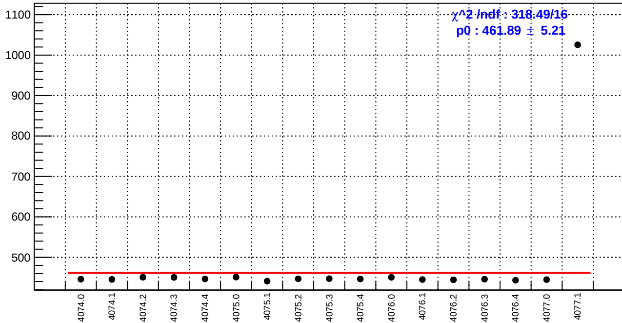
slug43-Left: reg_asym_right_avg.rms/ppm
