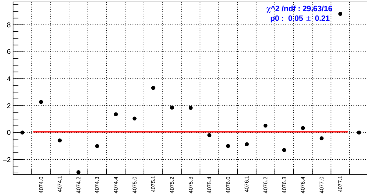
slug43-Left: us_avg_bpm4eY/(ppb/nm)
