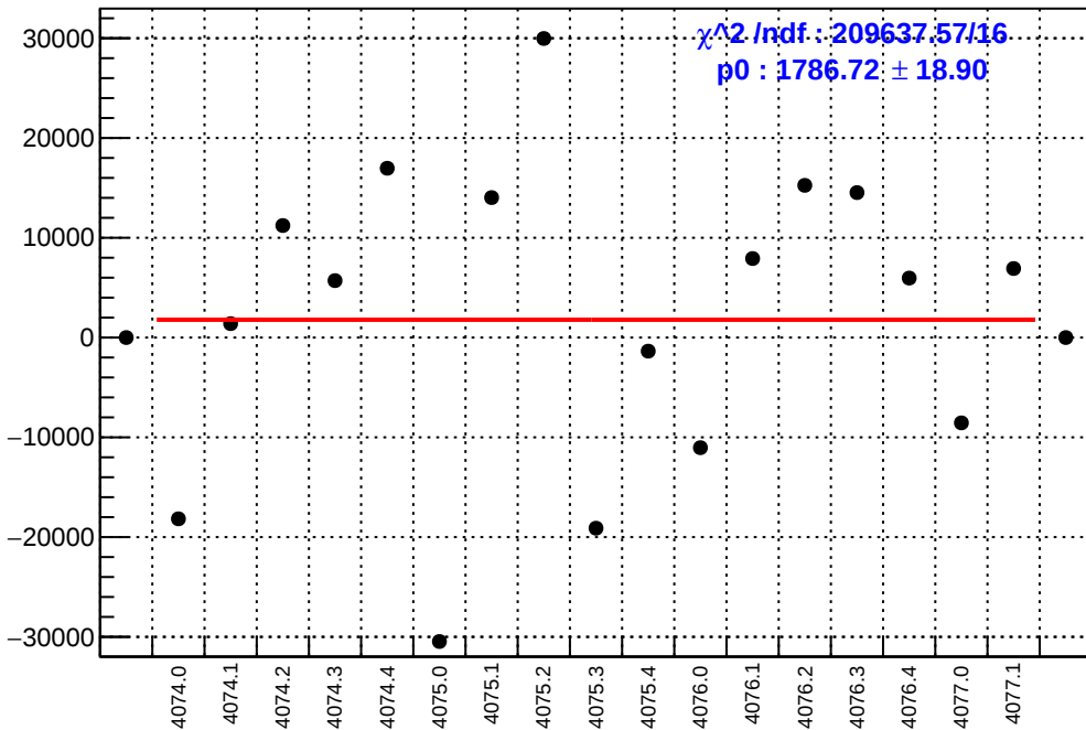
slug43-Left: asym_sam5.mean/ppb-reg_asym_sam5.mean/ppb
