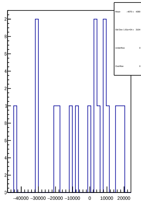
slug43-Left: 1D Corr asym_sam7.mean/ppb-reg_asym_sam7.mean/ppb
