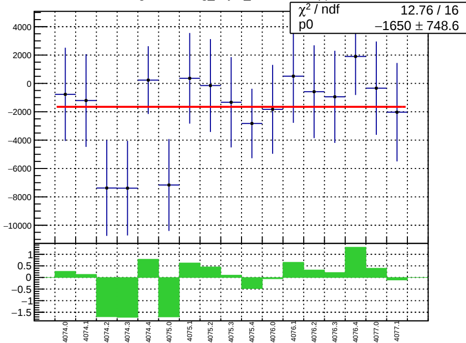
slug43-Left: reg_asym_sam7.mean/ppb
