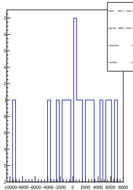
slug43-Left: 1D Corr asym_ds_avg.mean/ppb-reg_asym_ds_avg.mean/ppb
