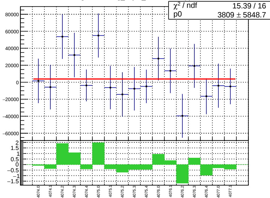
slug43-Left: reg_asym_sam2.mean/ppb
