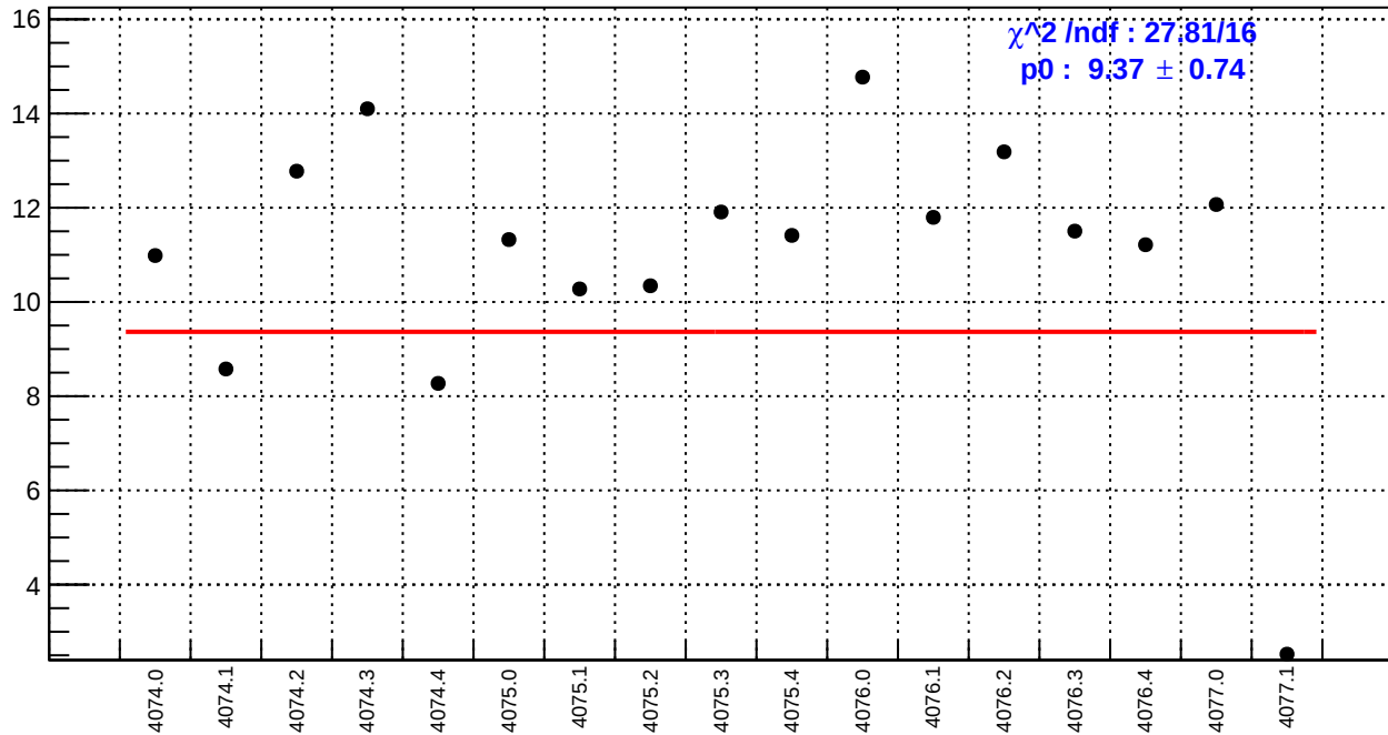
slug43-Left: dsr_bpm4aY/(ppb/nm)
