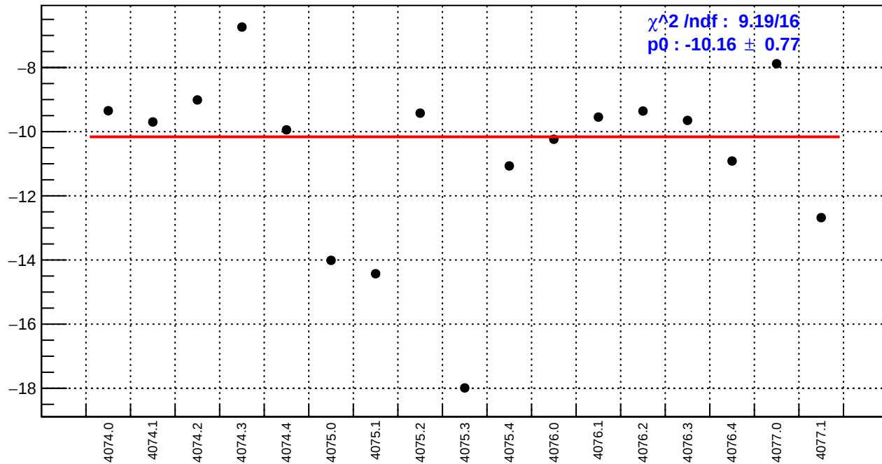
slug43-Left: us_avg_bpm4aX/(ppb/nm)
