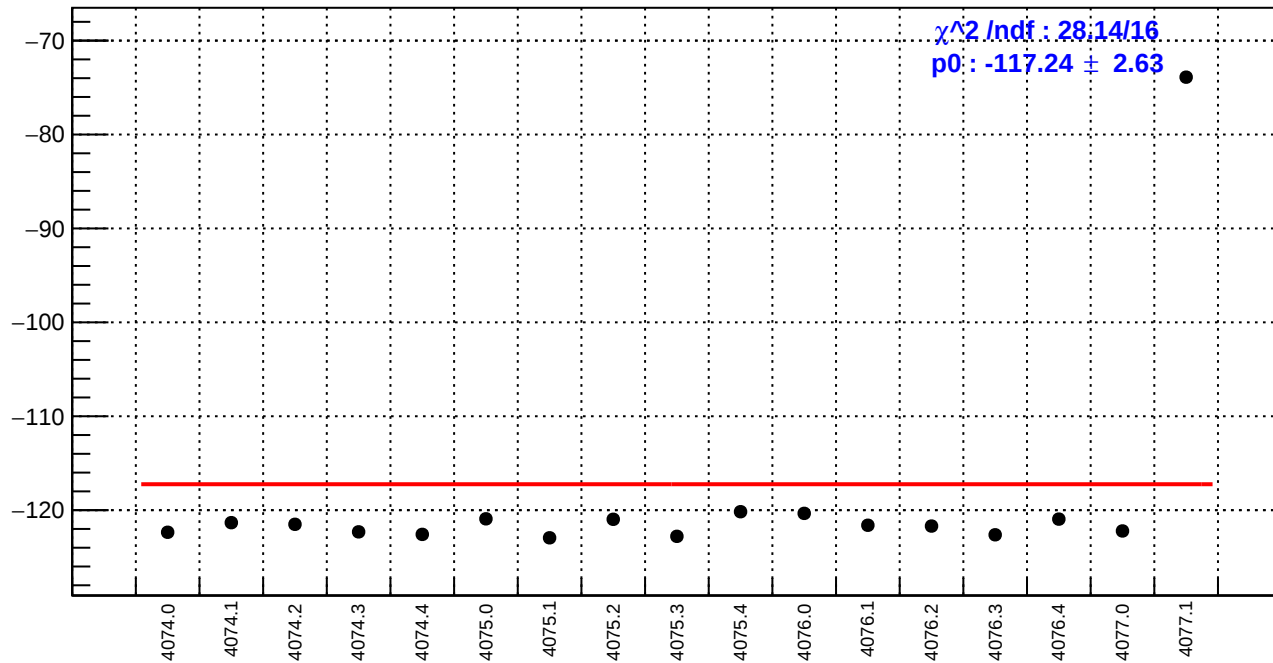
slug43-Left: right_avg_bpm12X/(ppb/nm)
