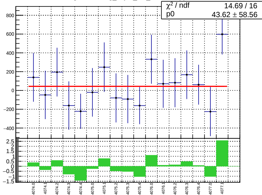
slug43-Left: reg_asym_left_dd.mean/ppb
