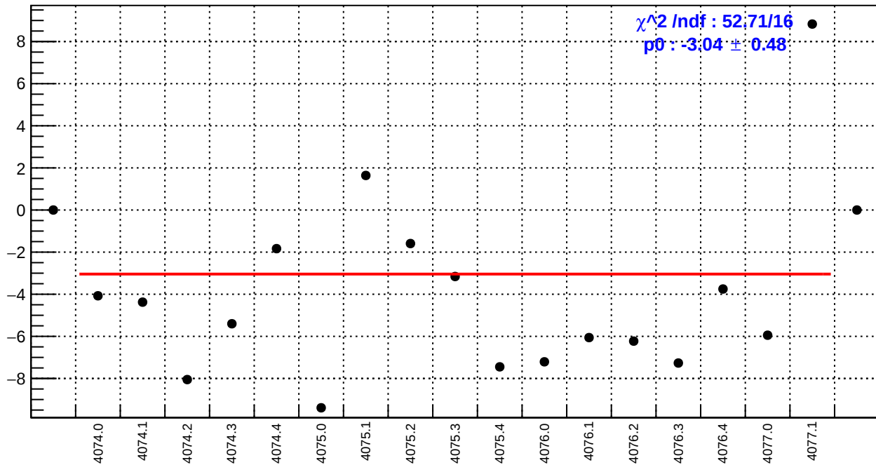
slug43-Left: usr_bpm4eY/(ppb/nm)
