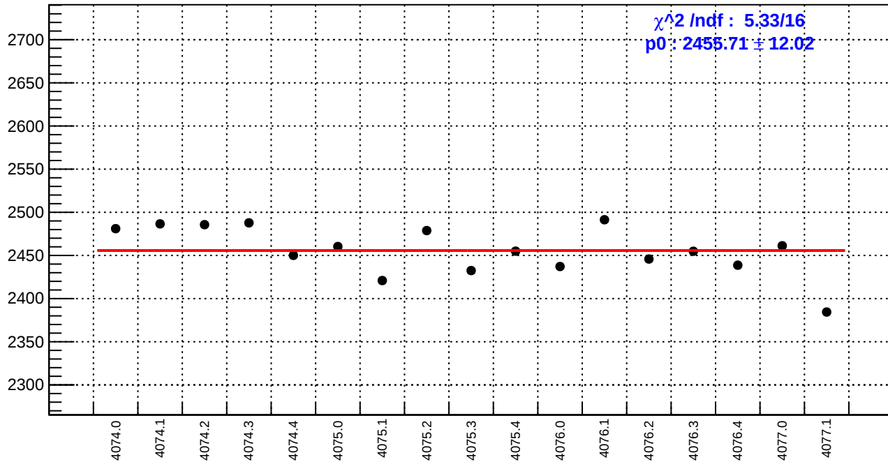
slug43-Left: reg_asym_sam2.rms/ppm
