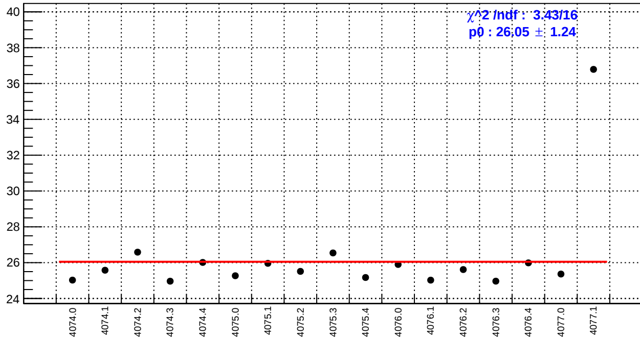
slug43-Left: usr_bpm4eX/(ppb/nm)
