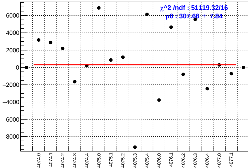
slug43-Left: asym_ds_avg.mean/ppb-reg_asym_ds_avg.mean/ppb
