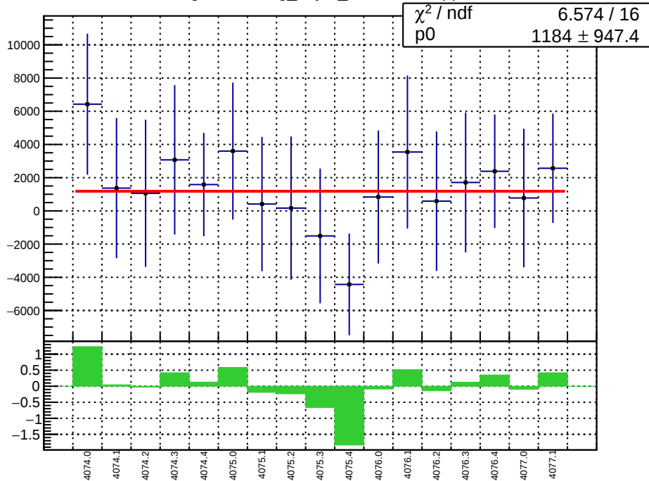
slug43-Left: reg_asym_sam1.mean/ppb
