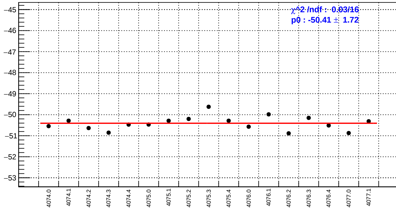
slug43-Left: left_avg_bpm12X/(ppb/nm)
