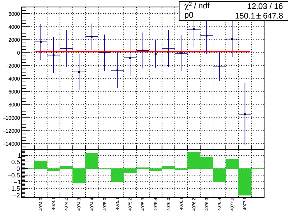
slug43-Left: reg_asym_ds_avg.mean/ppb
