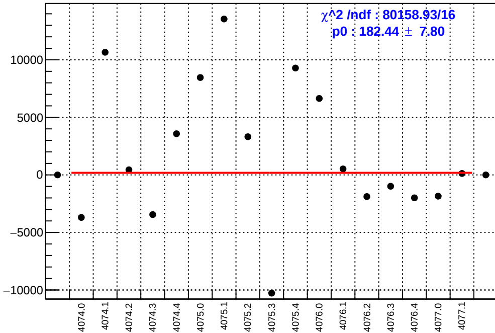
slug43-Left: asym_usl.mean/ppb-reg_asym_usl.mean/ppb
