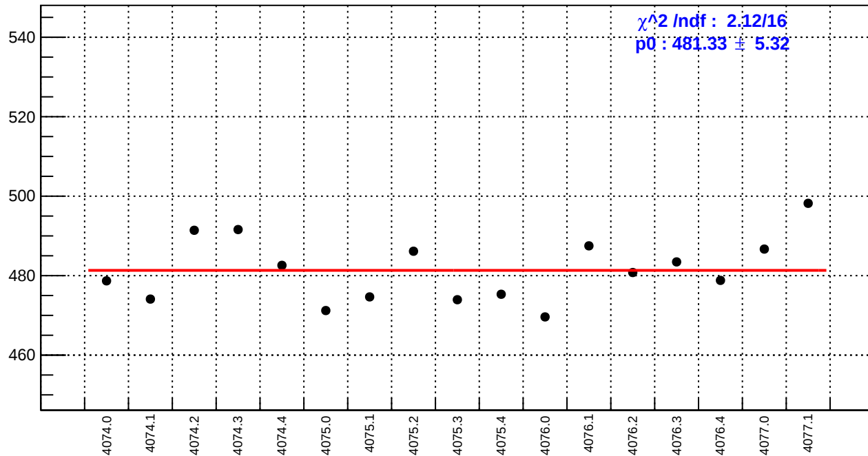
slug43-Left: reg_asym_sam8.rms/ppm
