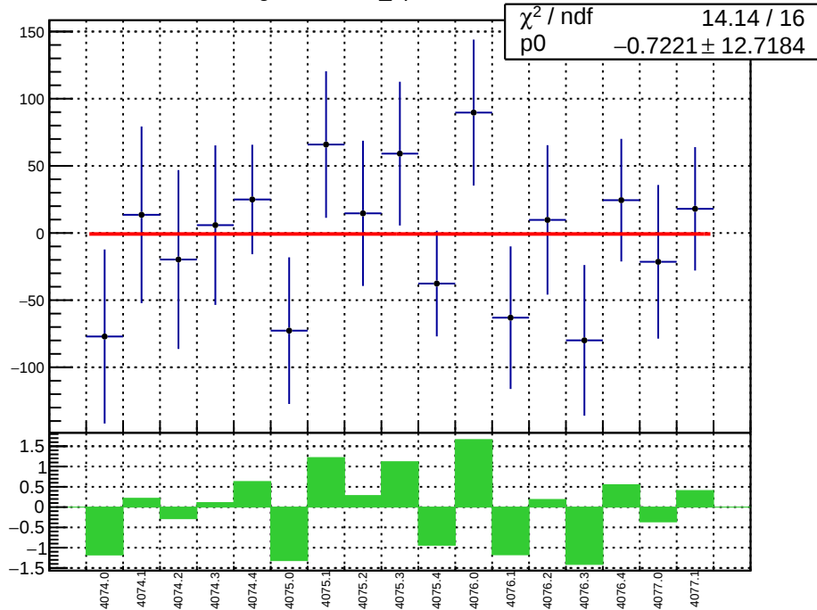
slug43-Left: diff_bpm11X.mean/nm
