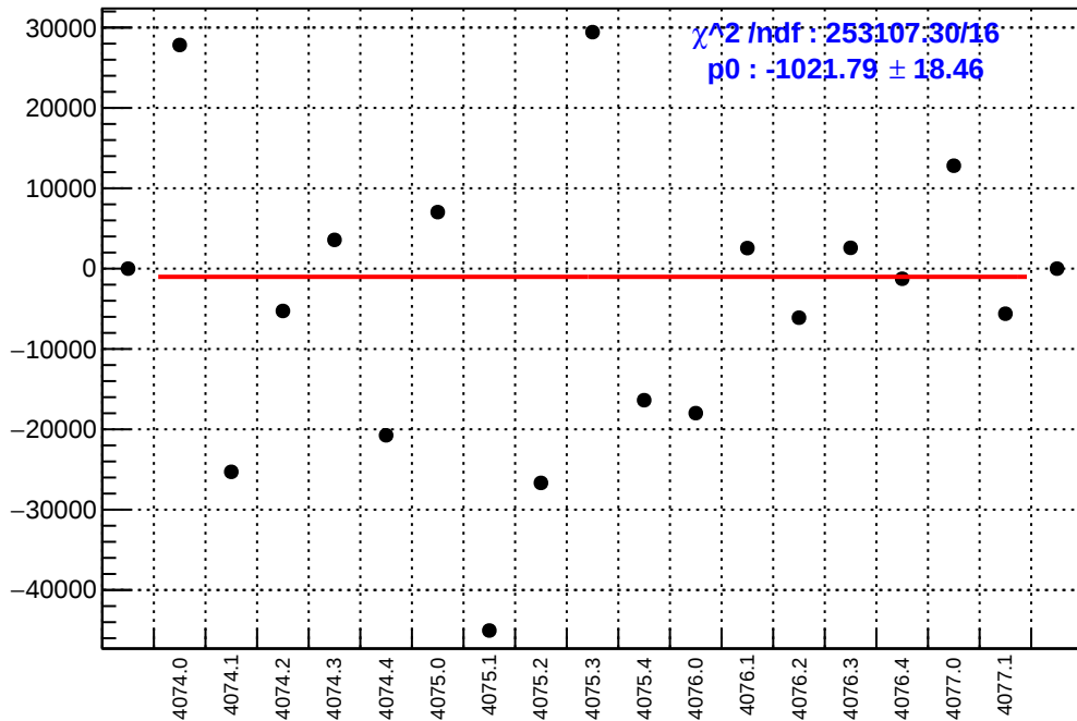
slug43-Left: asym_sam8.mean/ppb-reg_asym_sam8.mean/ppb
