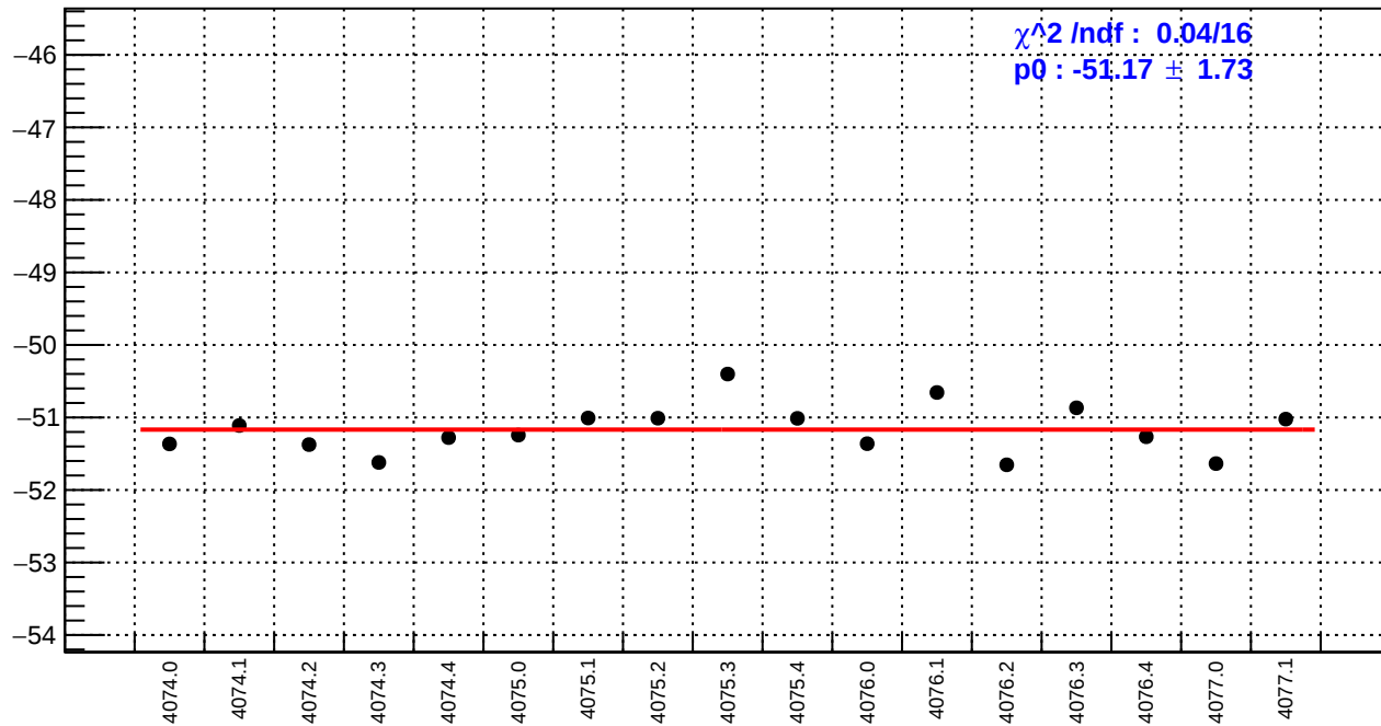
slug43-Left: dsl_bpm12X/(ppb/nm)
