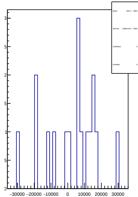
slug43-Left: 1D Corr asym_sam5.mean/ppb-reg_asym_sam5.mean/ppb
