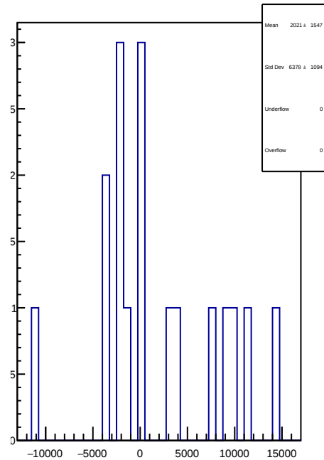
slug43-Left: 1D Corr asym_dsl.mean/ppb-reg_asym_dsl.mean/ppb
