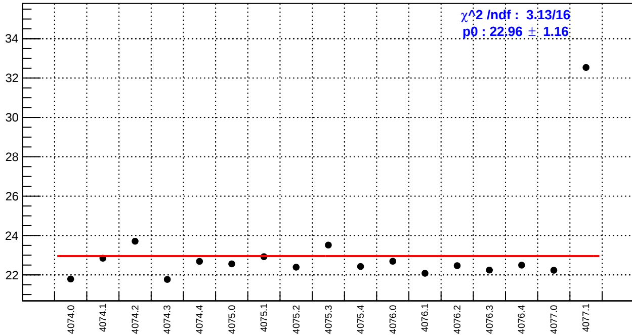
slug43-Left: right_avg_bpm4eX/(ppb/nm)
