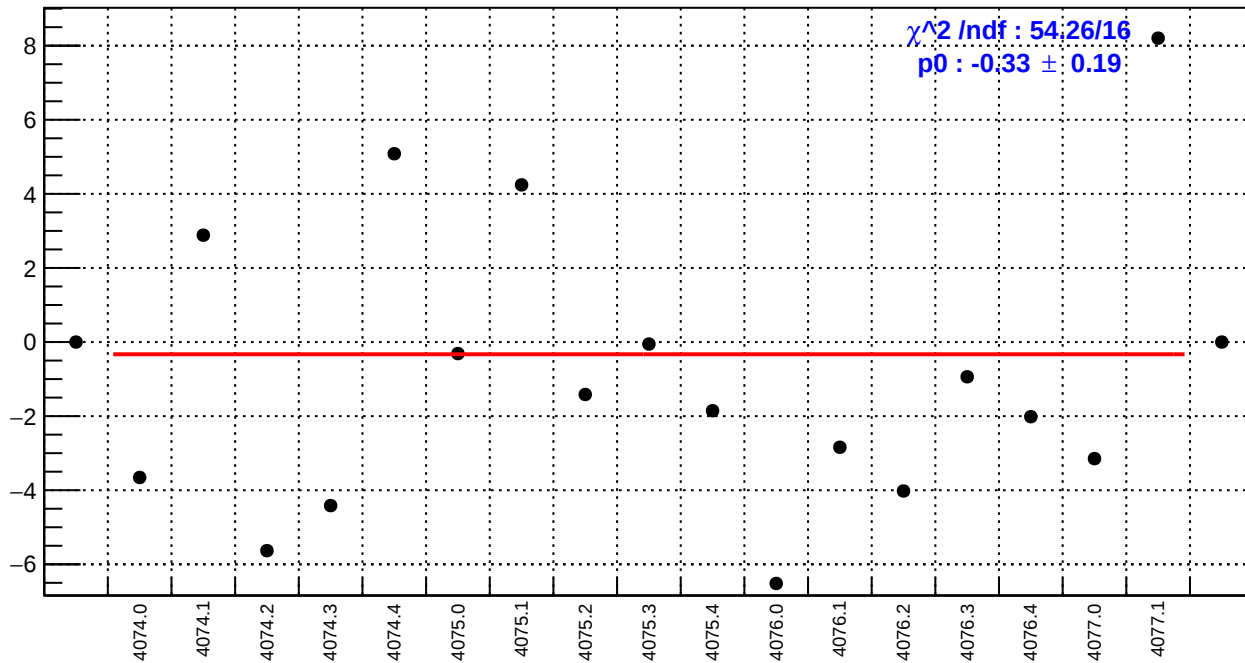
slug43-Left: dsr_bpm4eY/(ppb/nm)
