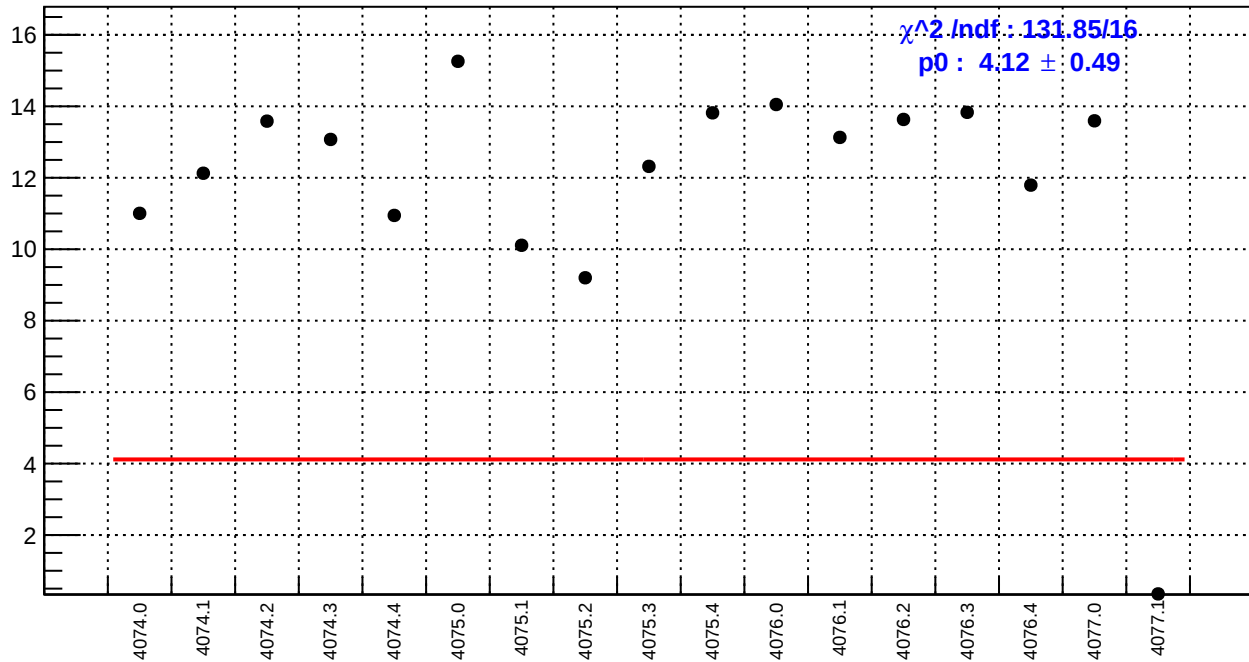
slug43-Left: usr_bpm4aY/(ppb/nm)
