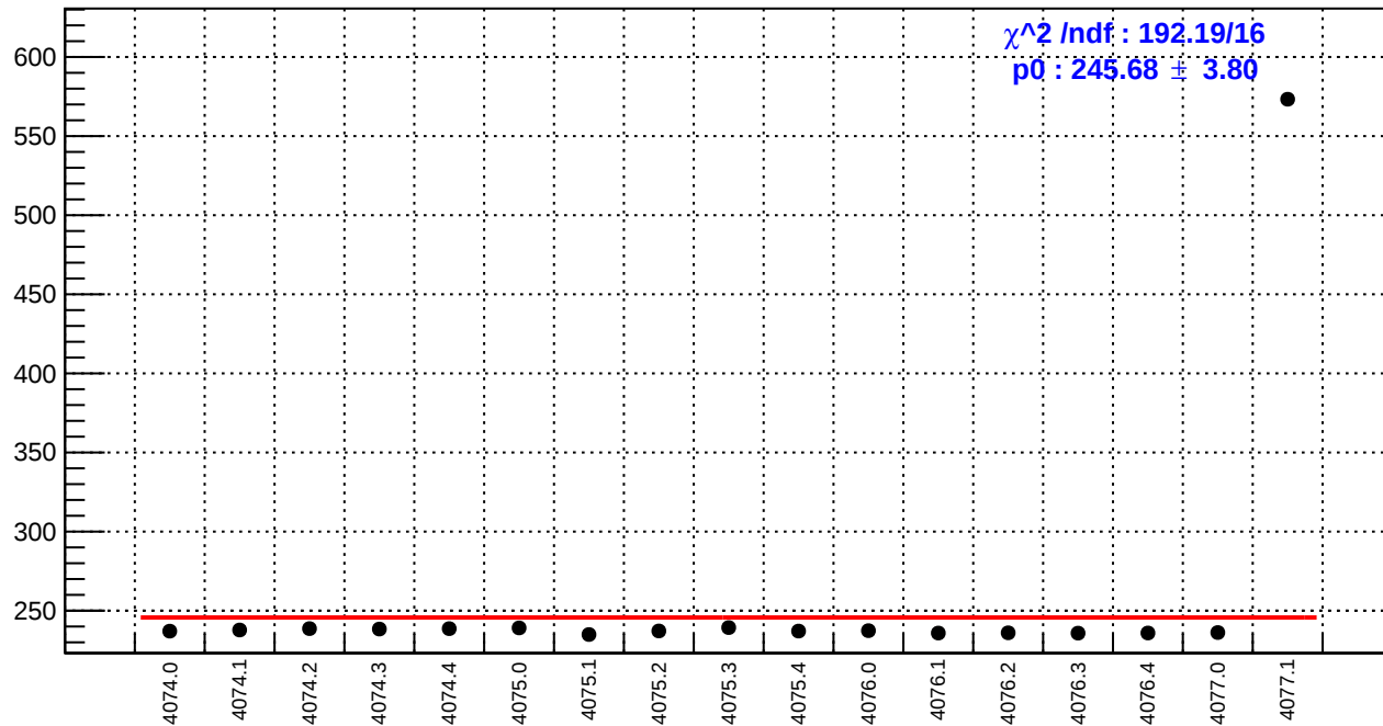
slug43-Left: reg_asym_us_dd.rms/ppm
