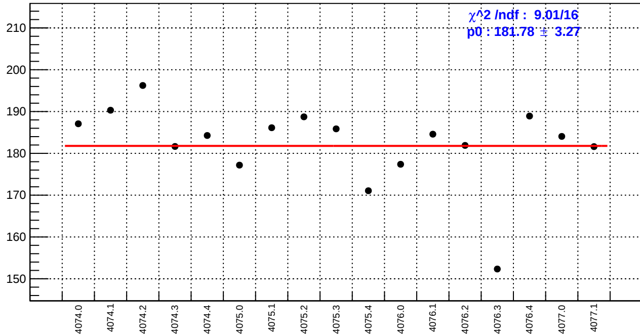
slug43-Left: asym_bcm_an_us.rms/ppm
