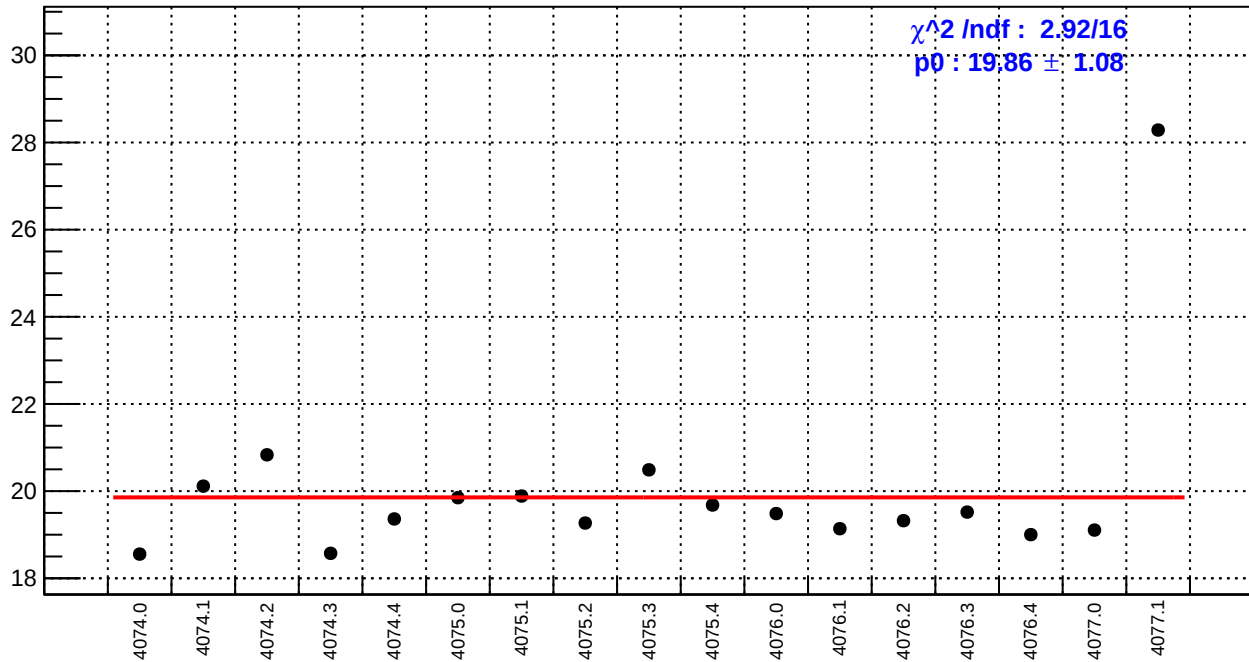
slug43-Left: dsr_bpm4eX/(ppb/nm)
