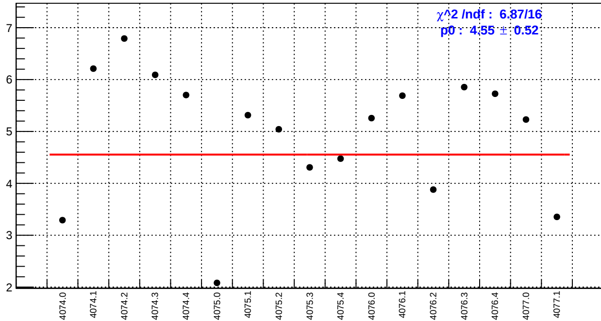
slug43-Left: usl_bpm4aY/(ppb/nm)
