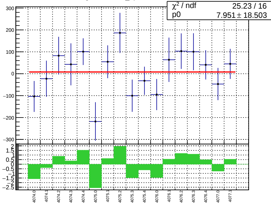
slug43-Left: diff_bpm4aY.mean/nm
