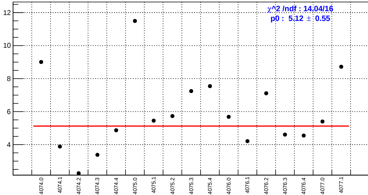
slug43-Left: left_avg_bpm4eY/(ppb/nm)
