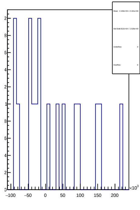
slug43-Left: 1D Corr asym_sam3.mean/ppb-reg_asym_sam3.mean/ppb
