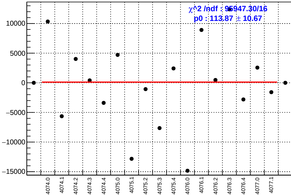
slug43-Left: asym_dsr.mean/ppb-reg_asym_dsr.mean/ppb
