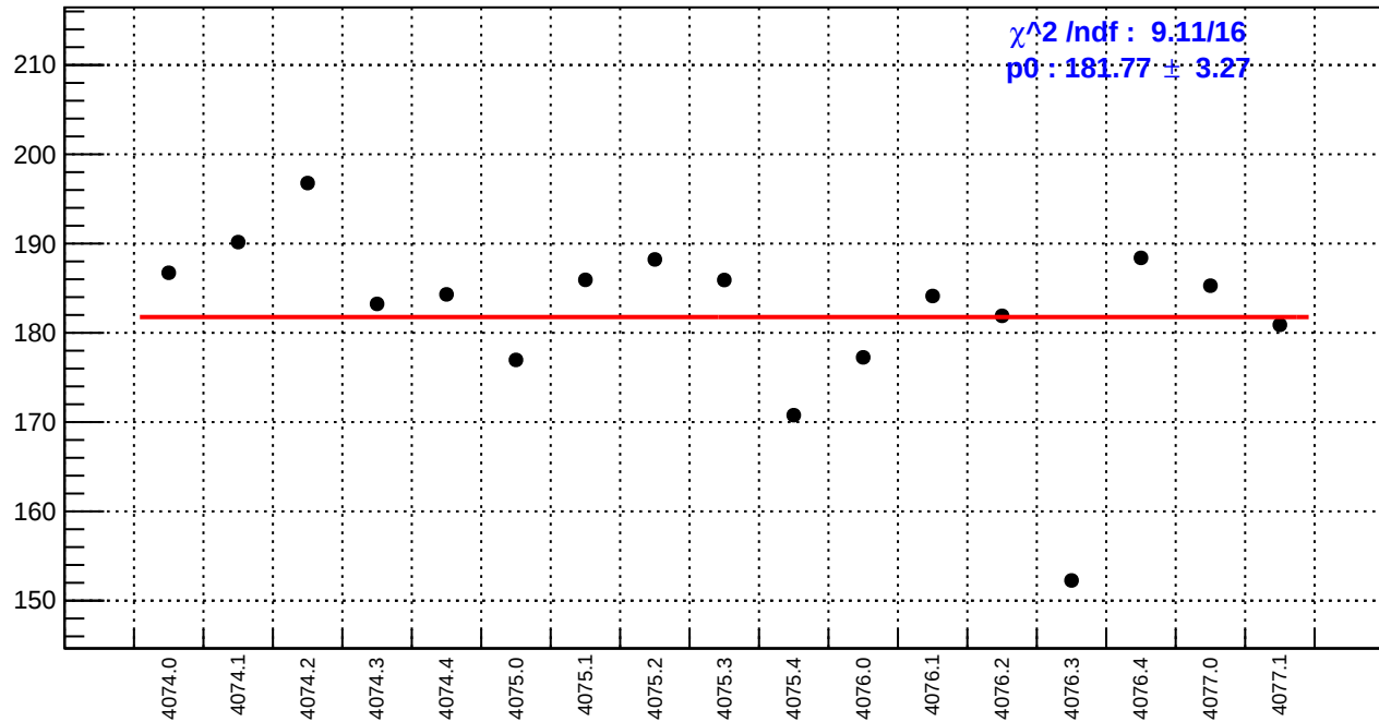
slug43-Left: asym_bcm_an_ds.rms/ppm
