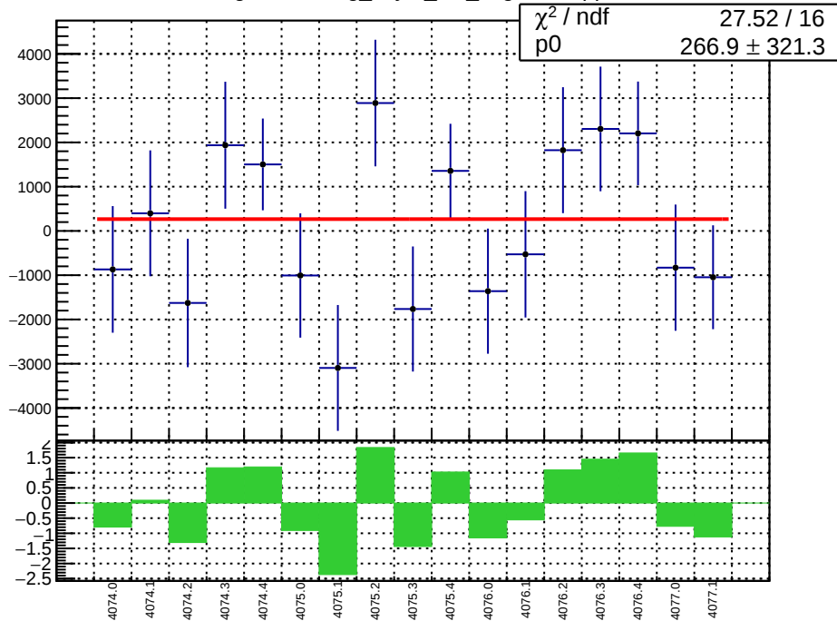
slug43-Left: reg_asym_left_avg.mean/ppb
