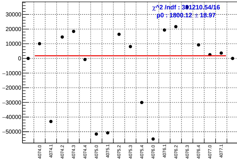
slug43-Left: asym_sam6.mean/ppb-reg_asym_sam6.mean/ppb
