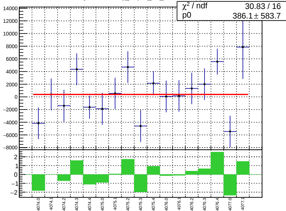
slug43-Left: reg_asym_us_dd.mean/ppb
