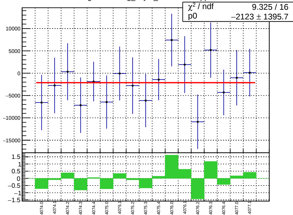
slug43-Left: reg_asym_sam6.mean/ppb
