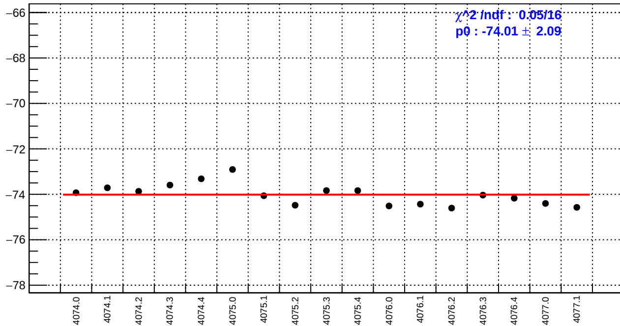
slug43-Left: dsl_bpm4eX/(ppb/nm)
