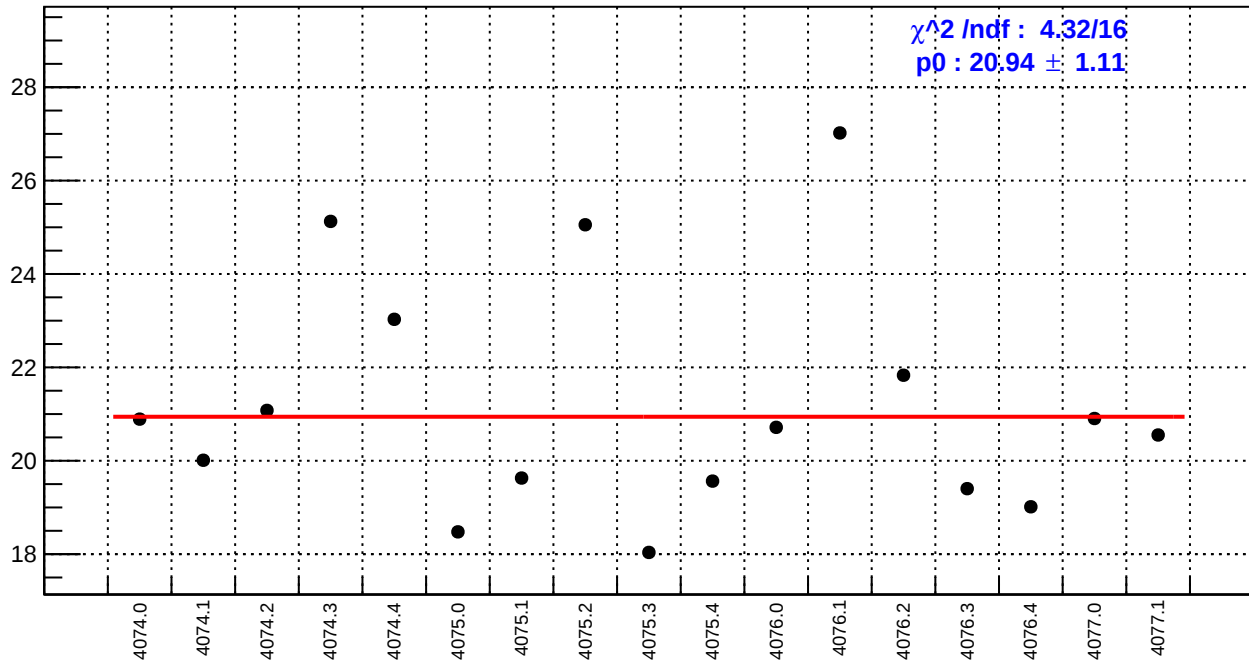
slug43-Left: left_avg_bpm4aX/(ppb/nm)
