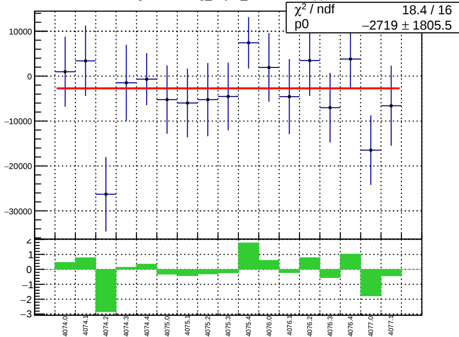
slug43-Left: reg_asym_sam3.mean/ppb
