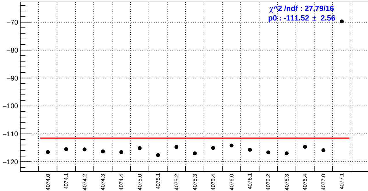
slug43-Left: usr_bpm12X/(ppb/nm)
