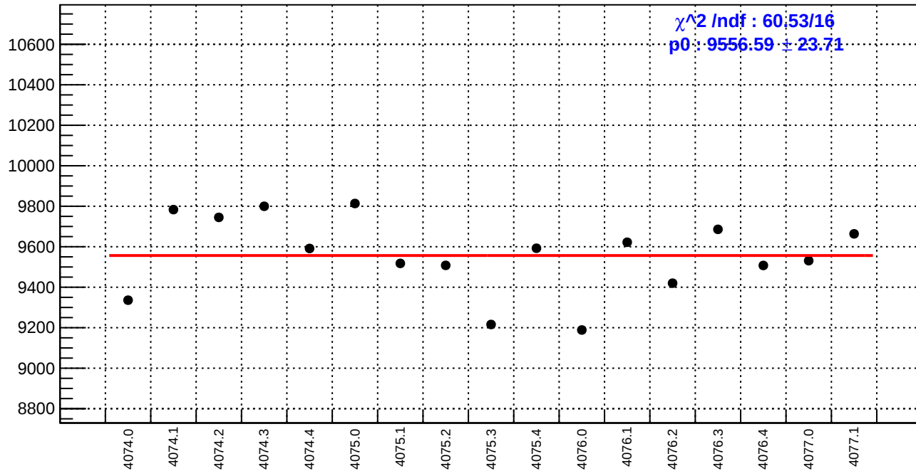
slug43-Left: diff_bpm4eX.rms/nm
