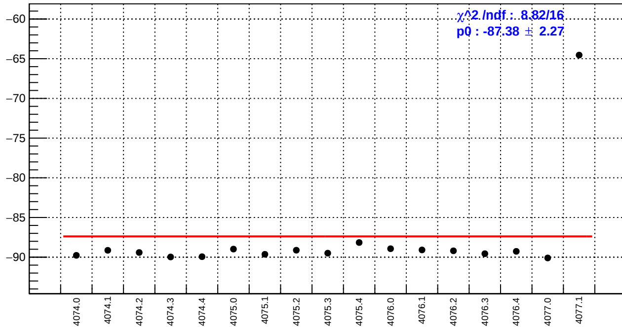
slug43-Left: ds_avg_bpm12X/(ppb/nm)
