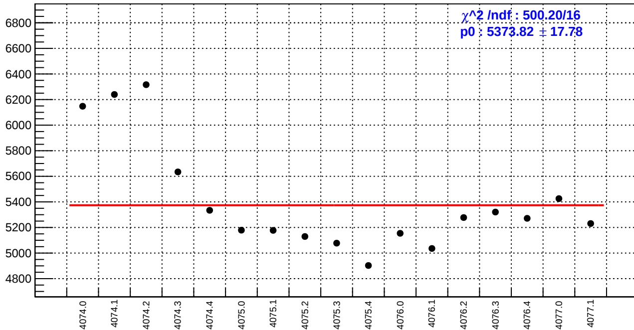
slug43-Left: diff_bpm11X.rms/nm
