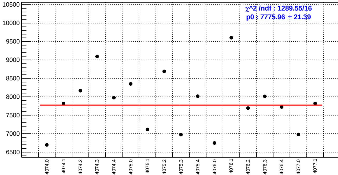
slug43-Left: diff_bpm4aY.rms/nm
