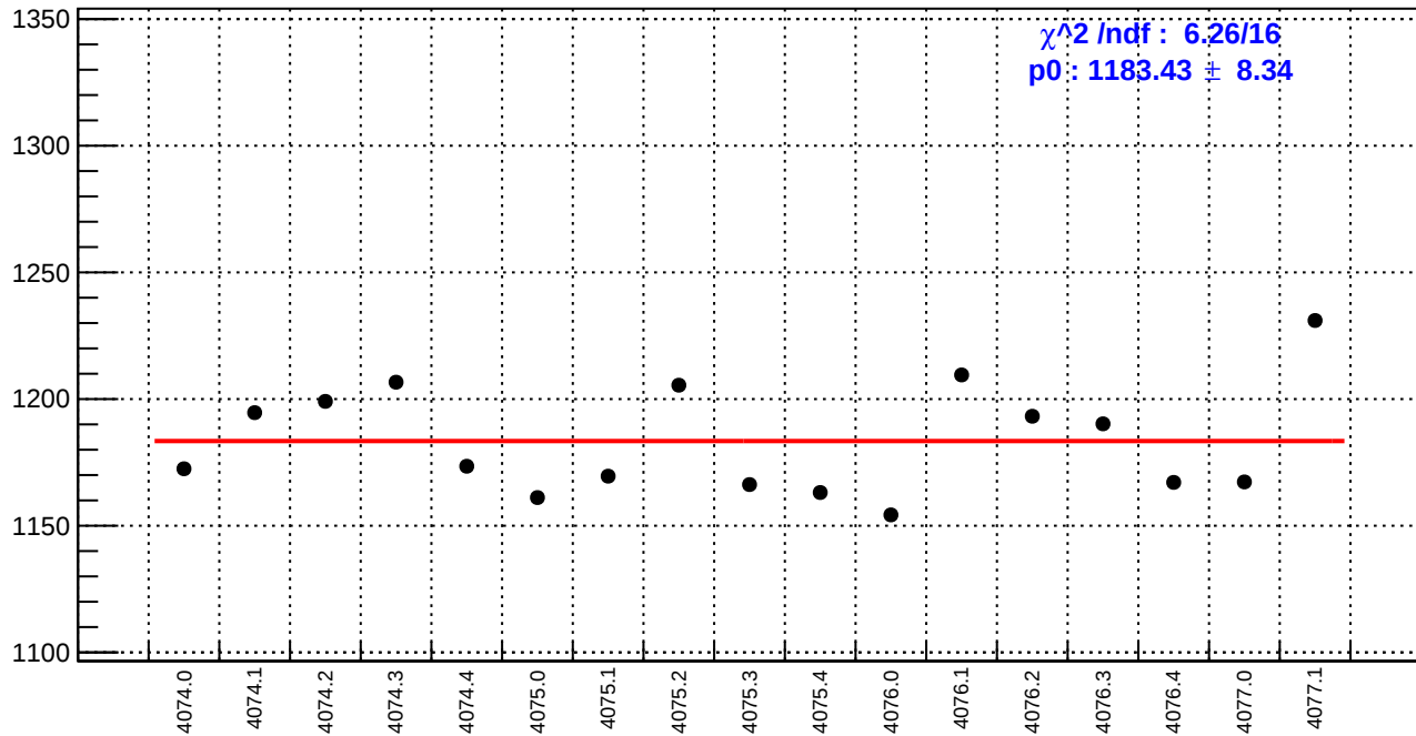
slug43-Left: reg_asym_sam4.rms/ppm
