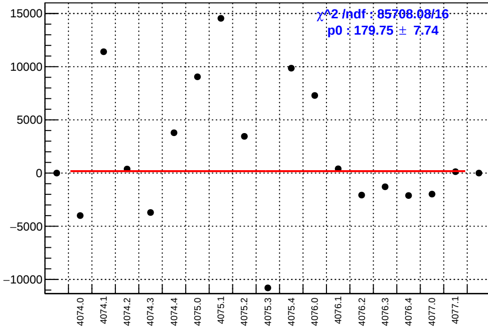
slug43-Left: asym_dsl.mean/ppb-reg_asym_dsl.mean/ppb
