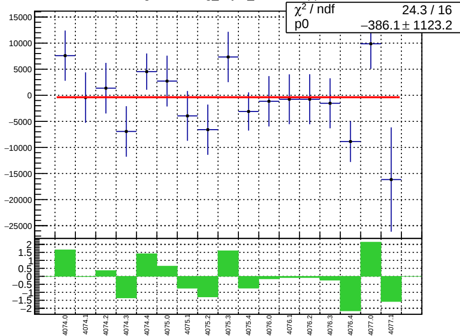
slug43-Left: reg_asym_usr.mean/ppb
