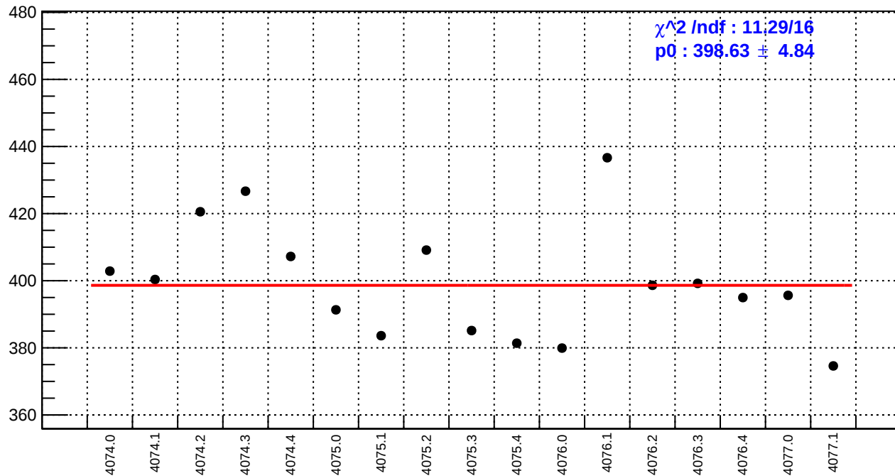
slug43-Left: reg_asym_sam1.rms/ppm
