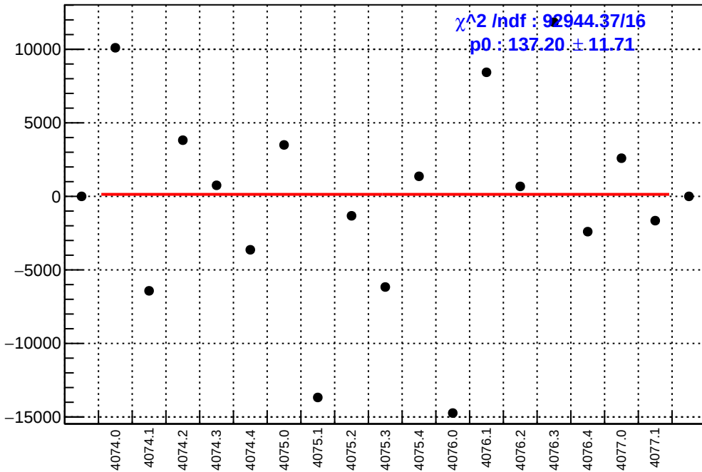
slug43-Left: asym_usr.mean/ppb-reg_asym_usr.mean/ppb
