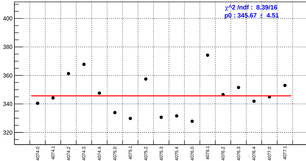
slug43-Left: reg_asym_sam5.rms/ppm
