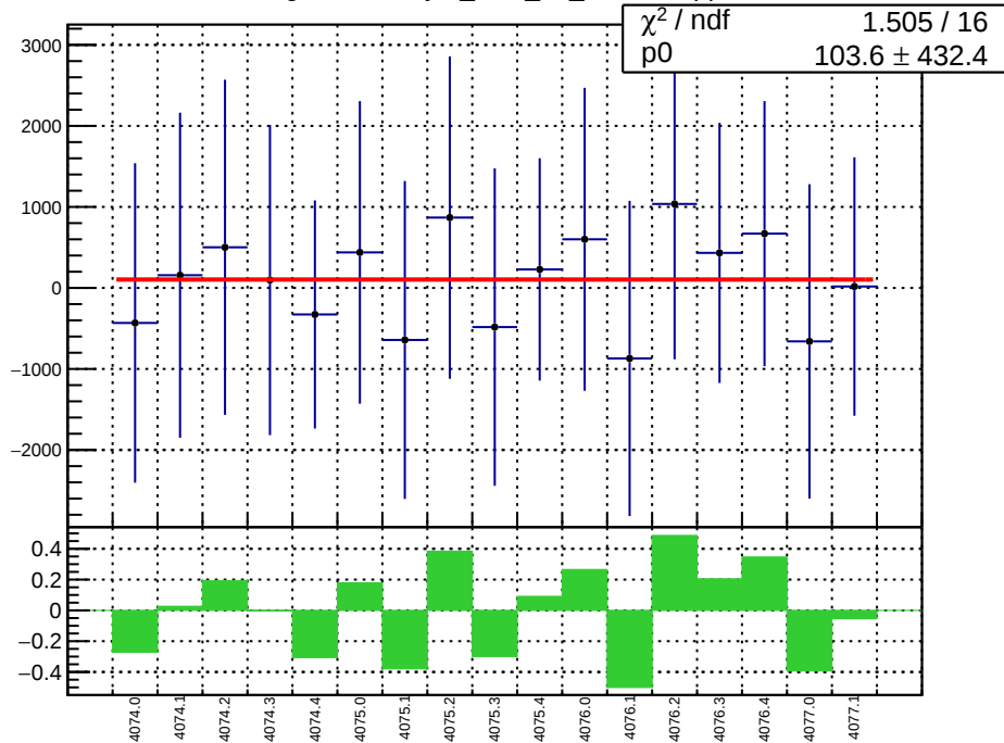
slug43-Left: asym_bcm_an_us.mean/ppb
