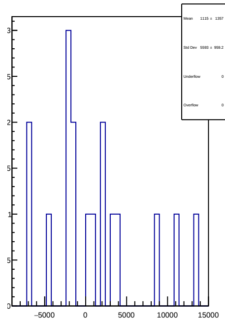
slug43-Left: 1D Corr asym_ds_dd.mean/ppb-reg_asym_ds_dd.mean/ppb
