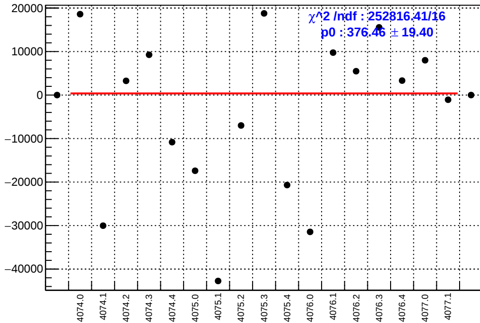
slug43-Left: asym_sam7.mean/ppb-reg_asym_sam7.mean/ppb
