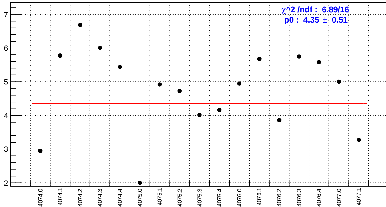
slug43-Left: left_avg_bpm4aY/(ppb/nm)
