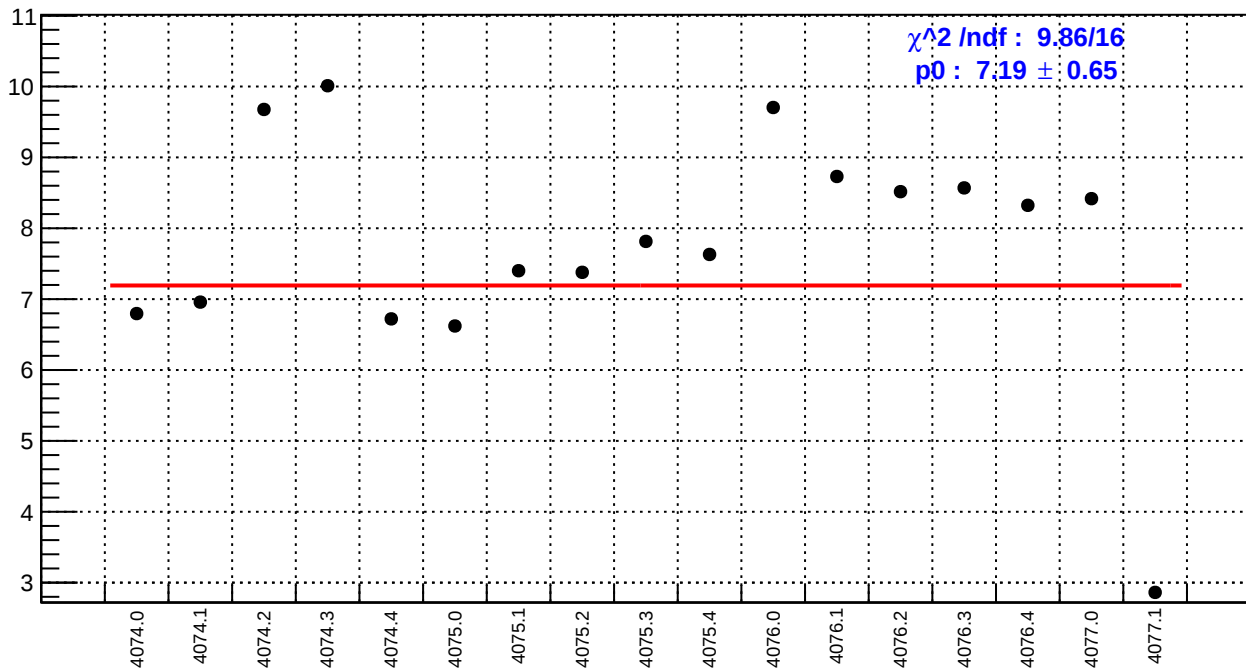
slug43-Left: ds_avg_bpm4aY/(ppb/nm)
