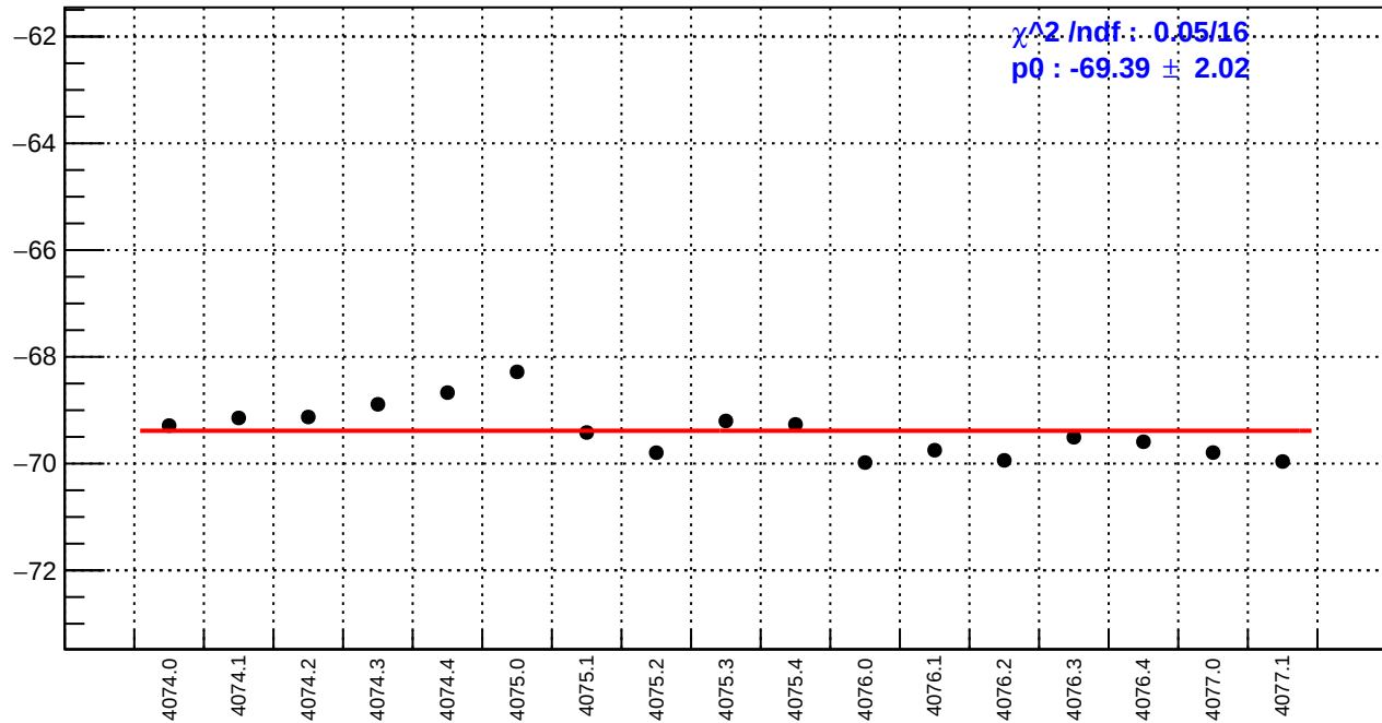
slug43-Left: usl_bpm4eX/(ppb/nm)
