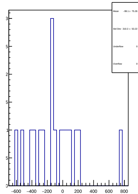
slug43-Left: 1D Corr asym_right_dd.mean/ppb-reg_asym_right_dd.mean/ppb
