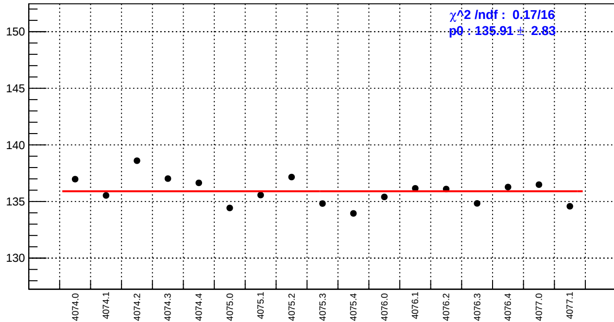
slug43-Left: reg_asym_usl.rms/ppm
