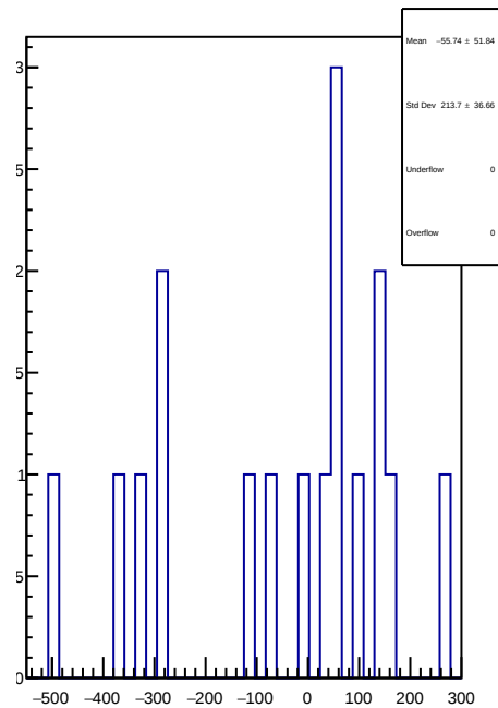
slug43-Left: 1D Corr asym_left_dd.mean/ppb-reg_asym_left_dd.mean/ppb
