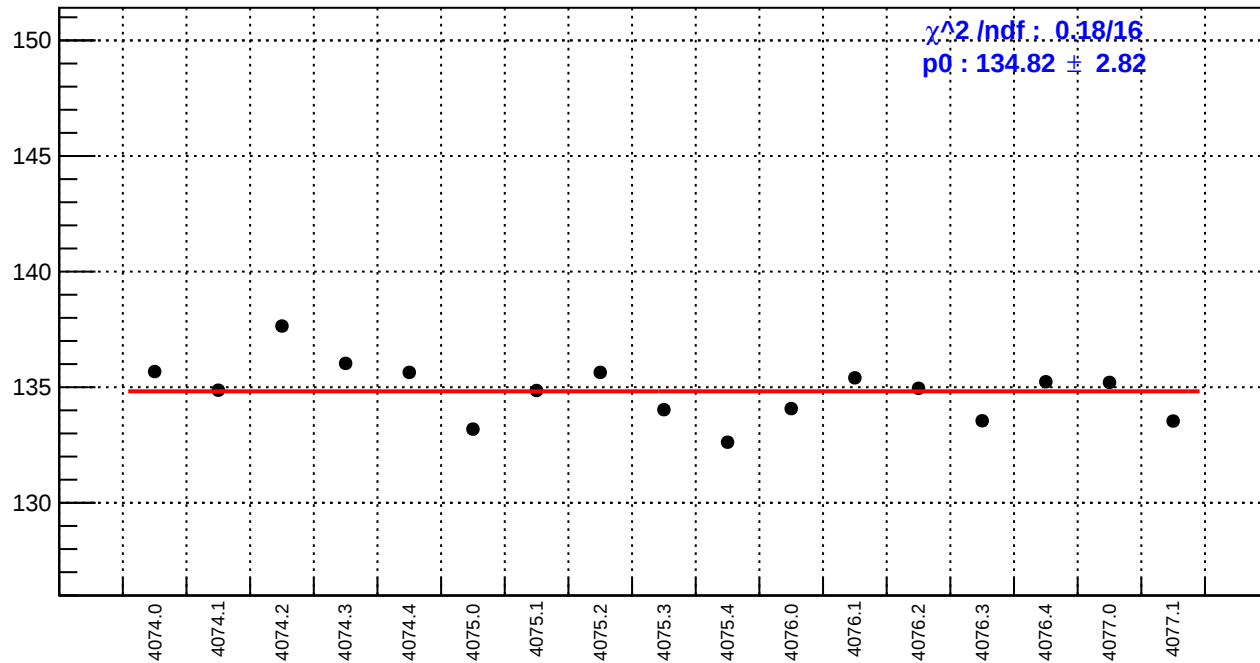
slug43-Left: reg_asym_left_avg.rms/ppm
