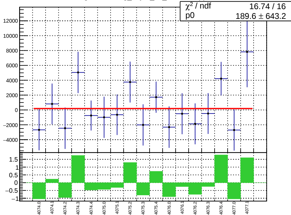
slug43-Left: reg_asym_ds_dd.mean/ppb
