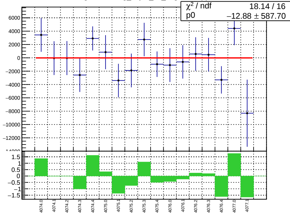
slug43-Left: reg_asym_us_avg.mean/ppb
