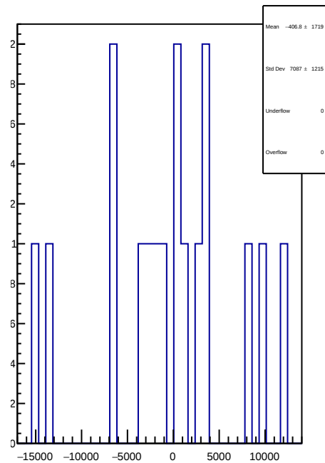
slug43-Left: 1D Corr asym_usr.mean/ppb-reg_asym_usr.mean/ppb
