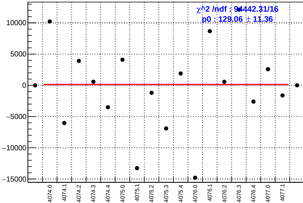
slug43-Left: asym_right_avg.mean/ppb-reg_asym_right_avg.mean/ppb
