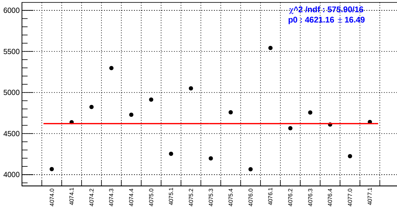
slug43-Left: diff_bpm4eY.rms/nm
