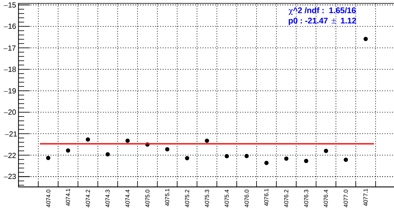
slug43-Left: us_avg_bpm4eX/(ppb/nm)
