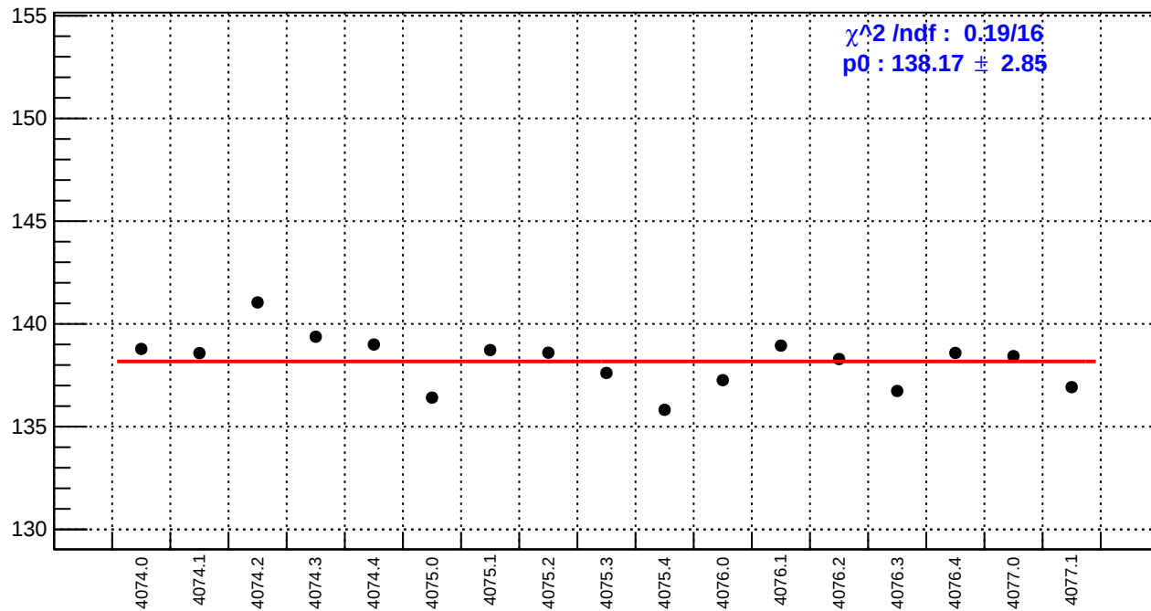
slug43-Left: reg_asym_dsl.rms/ppm
