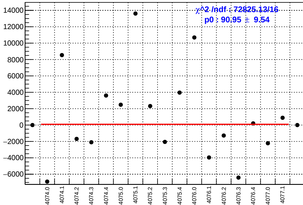
slug43-Left: asym_us_dd.mean/ppb-reg_asym_us_dd.mean/ppb
