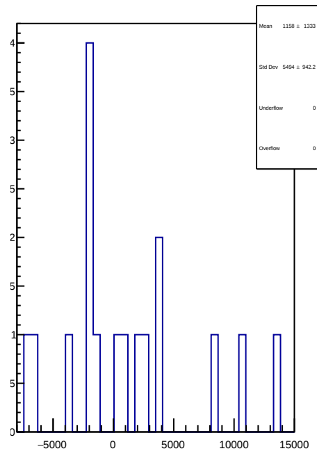
slug43-Left: 1D Corr asym_us_dd.mean/ppb-reg_asym_us_dd.mean/ppb
