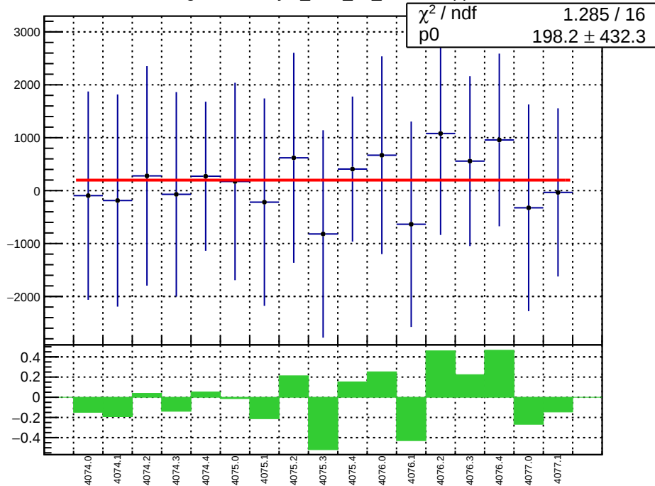
slug43-Left: asym_bcm_an_ds.mean/ppb
