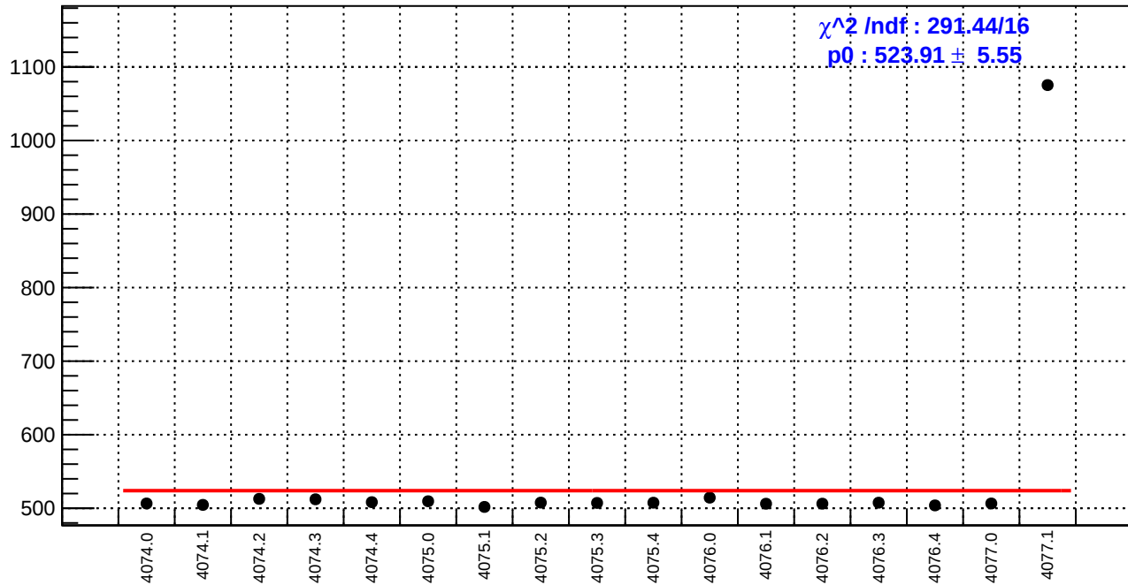
slug43-Left: reg_asym_dsr.rms/ppm
