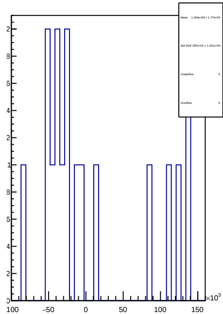
slug43-Left: 1D Corr asym_sam2.mean/ppb-reg_asym_sam2.mean/ppb
