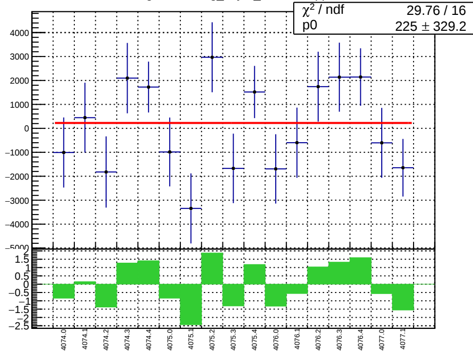
slug43-Left: reg_asym_dsl.mean/ppb
