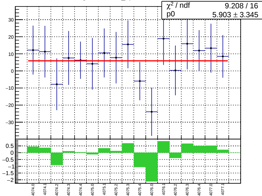
slug43-Left: diff_bpm4aX.mean/nm
