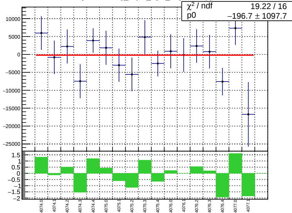
slug43-Left: reg_asym_right_avg.mean/ppb
