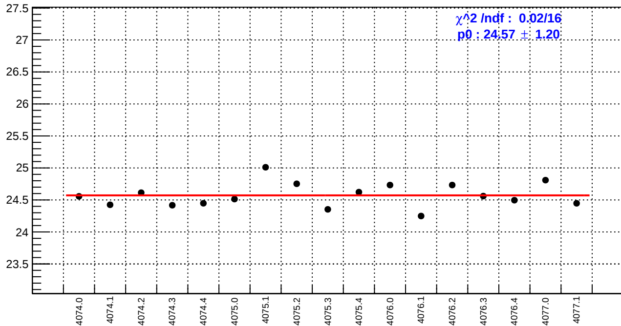
slug43-Left: reg_asym_left_dd.rms/ppm
