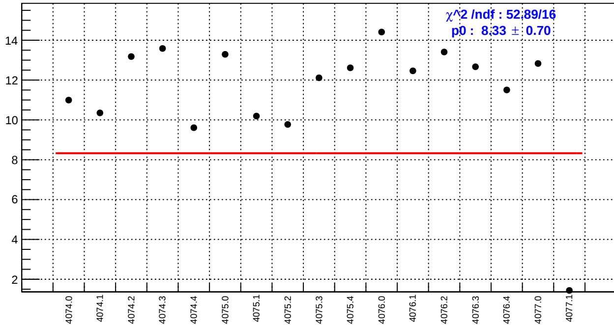
slug43-Left: right_avg_bpm4aY/(ppb/nm)
