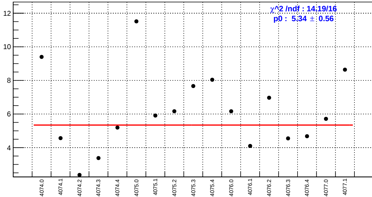
slug43-Left: dsl_bpm4eY/(ppb/nm)
