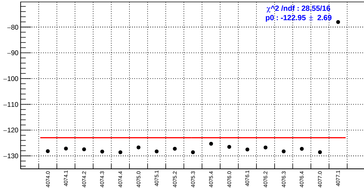
slug43-Left: dsr_bpm12X/(ppb/nm)
