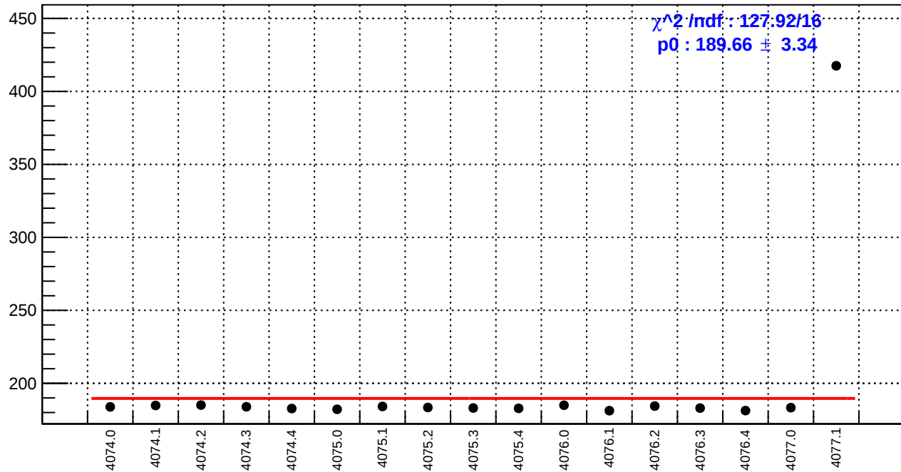
slug43-Left: reg_asym_right_dd.rms/ppm
