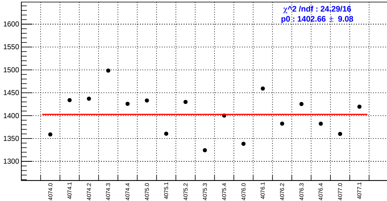
slug43-Left: diff_bpm4aX.rms/nm
