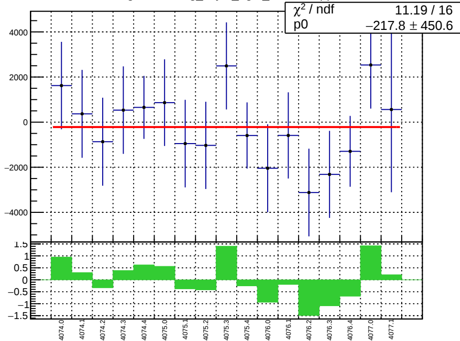
slug43-Left: reg_asym_right_dd.mean/ppb
