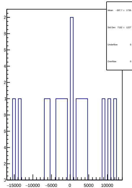
slug43-Left: 1D Corr asym_right_avg.mean/ppb-reg_asym_right_avg.mean/ppb
