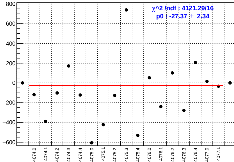
slug43-Left: asym_right_dd.mean/ppb-reg_asym_right_dd.mean/ppb
