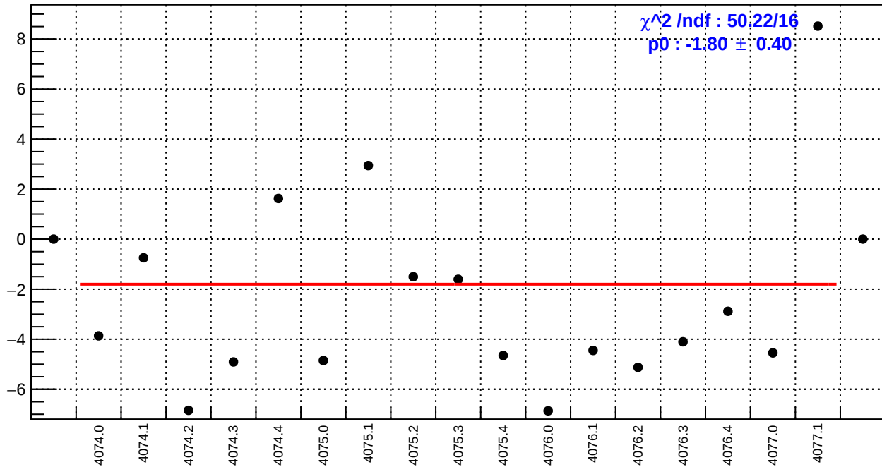
slug43-Left: right_avg_bpm4eY/(ppb/nm)
