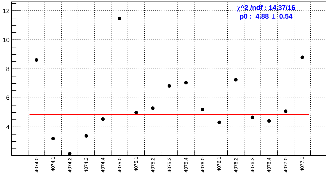
slug43-Left: usl_bpm4eY/(ppb/nm)
