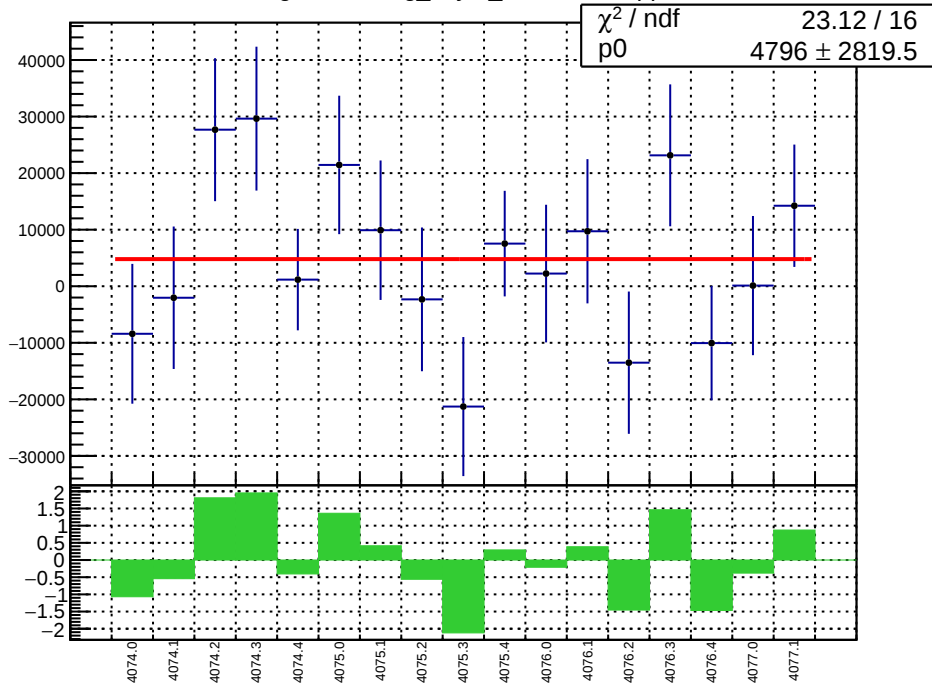
slug43-Left: reg_asym_sam4.mean/ppb
