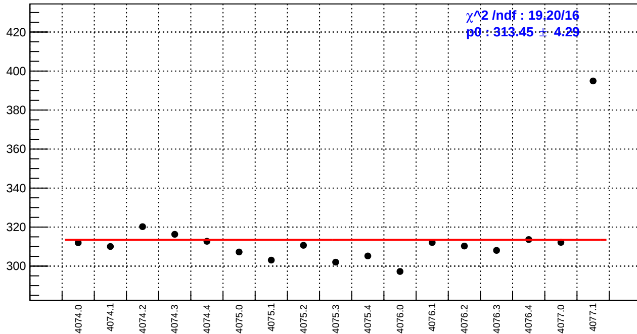
slug43-Left: reg_asym_sam7.rms/ppm
