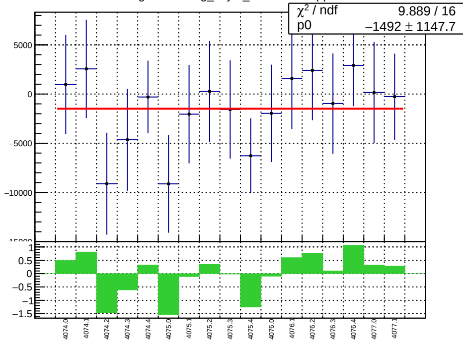
slug43-Left: reg_asym_sam8.mean/ppb
