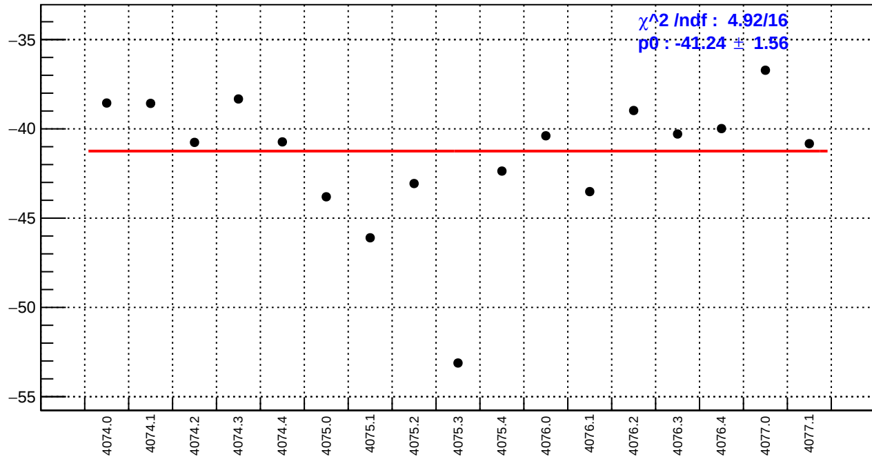
slug43-Left: right_avg_bpm4aX/(ppb/nm)
