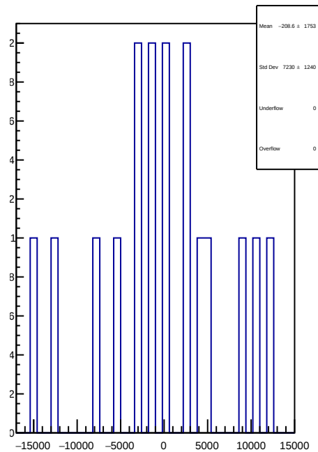
slug43-Left: 1D Corr asym_dsr.mean/ppb-reg_asym_dsr.mean/ppb
