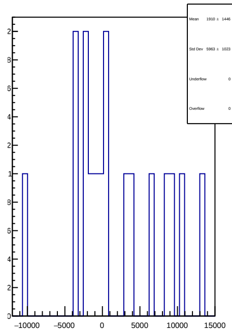
slug43-Left: 1D Corr asym_usl.mean/ppb-reg_asym_usl.mean/ppb
