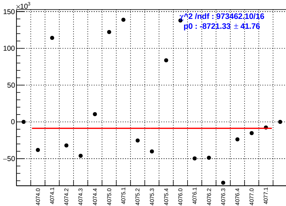
slug43-Left: asym_sam2.mean/ppb-reg_asym_sam2.mean/ppb
