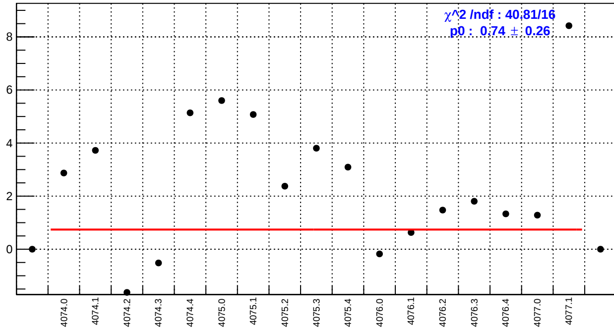
slug43-Left: ds_avg_bpm4eY/(ppb/nm)
