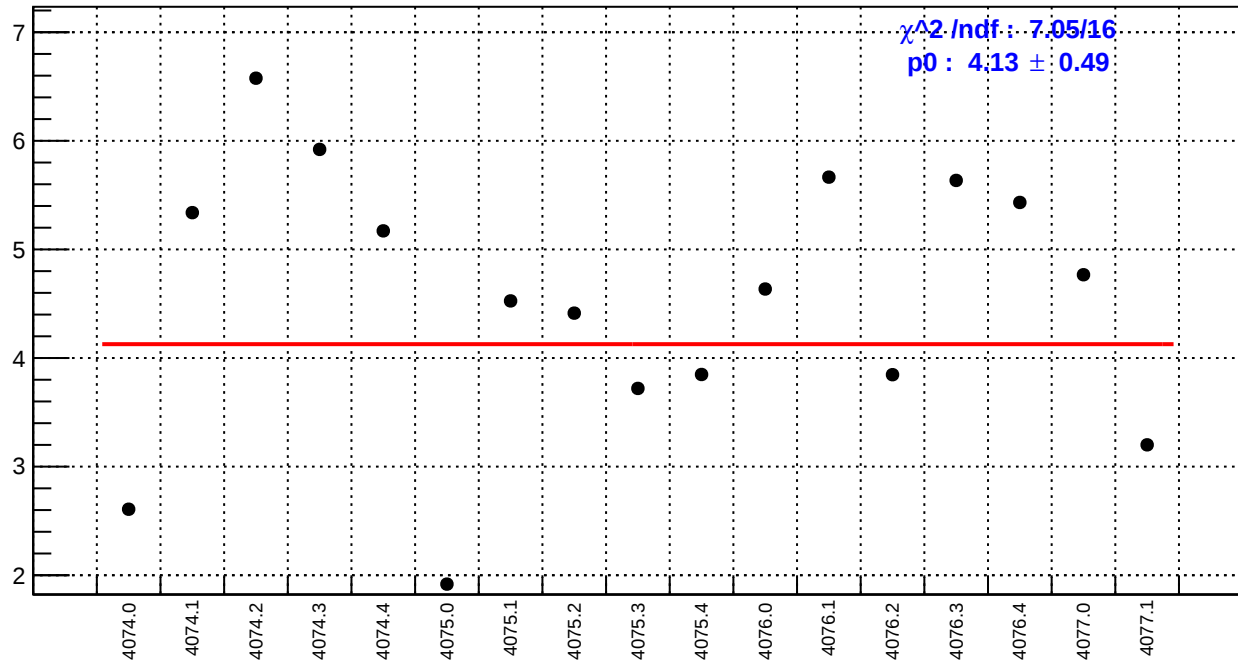
slug43-Left: dsl_bpm4aY/(ppb/nm)
