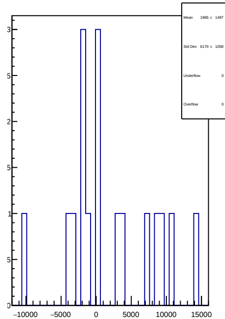
slug43-Left: 1D Corr asym_left_avg.mean/ppb-reg_asym_left_avg.mean/ppb
