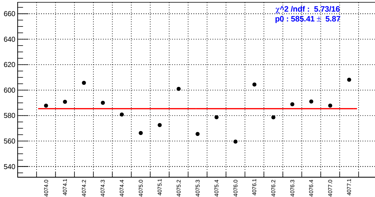
slug43-Left: reg_asym_sam6.rms/ppm
