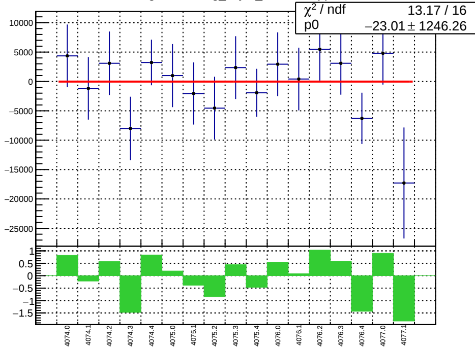
slug43-Left: reg_asym_dsr.mean/ppb
