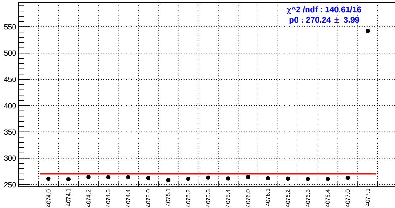
slug43-Left: reg_asym_ds_dd.rms/ppm
