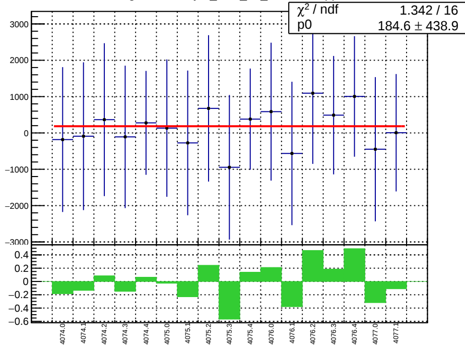
slug43-Left: asym_bcm_an_ds3.mean/ppb
