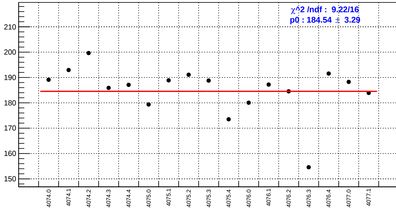
slug43-Left: asym_bcm_an_ds3.rms/ppm
