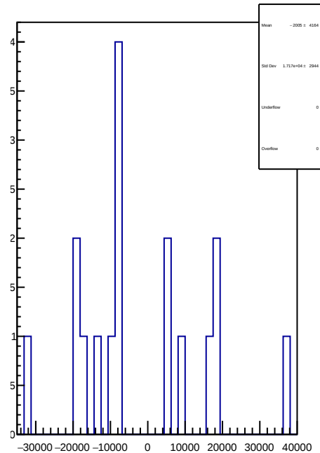
slug43-Left: 1D Corr asym_sam1.mean/ppb-reg_asym_sam1.mean/ppb
