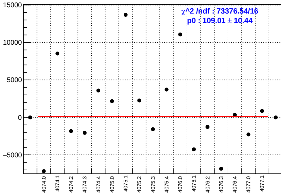
slug43-Left: asym_ds_dd.mean/ppb-reg_asym_ds_dd.mean/ppb
