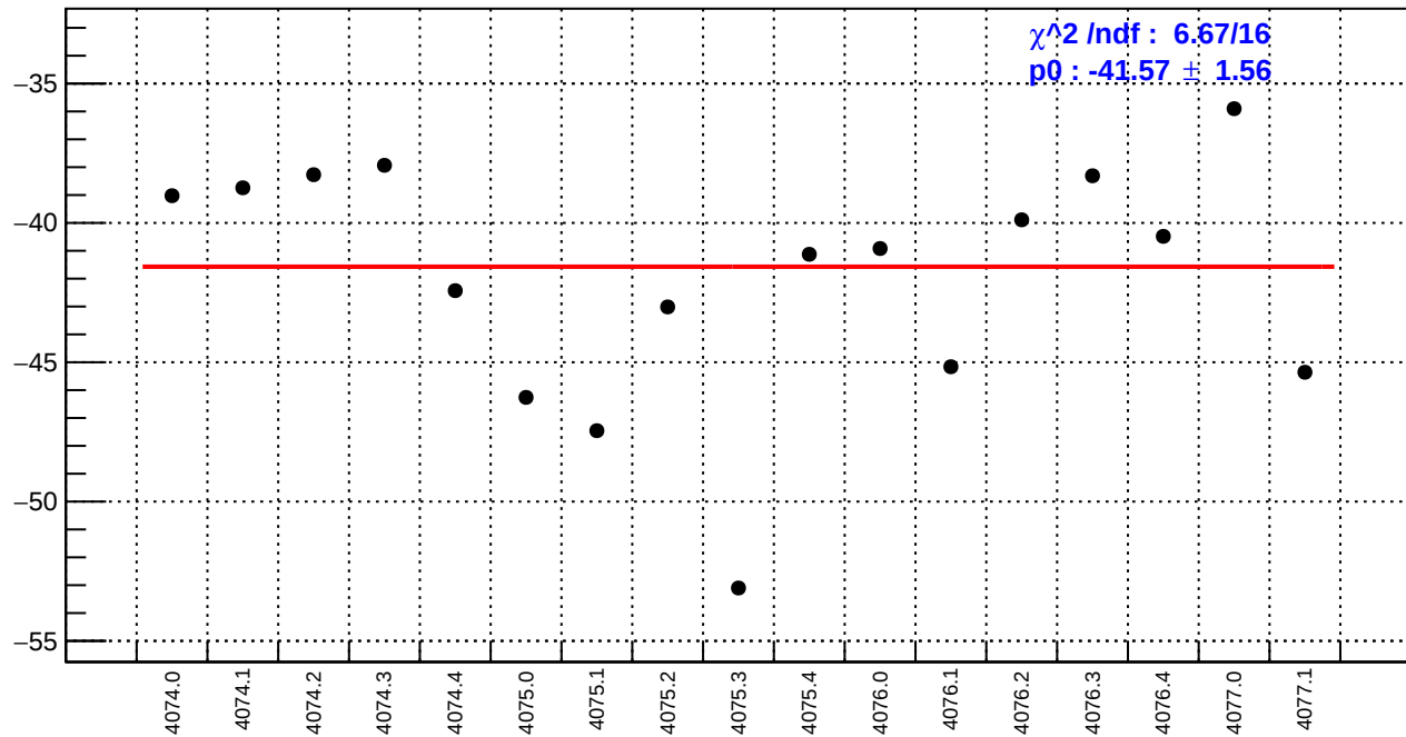
slug43-Left: usr_bpm4aX/(ppb/nm)
