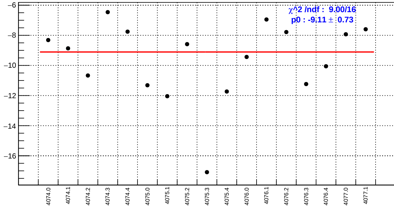
slug43-Left: ds_avg_bpm4aX/(ppb/nm)
