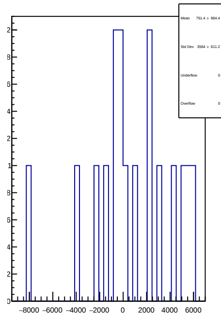
slug43-Left: 1D Corr asym_us_avg.mean/ppb-reg_asym_us_avg.mean/ppb
