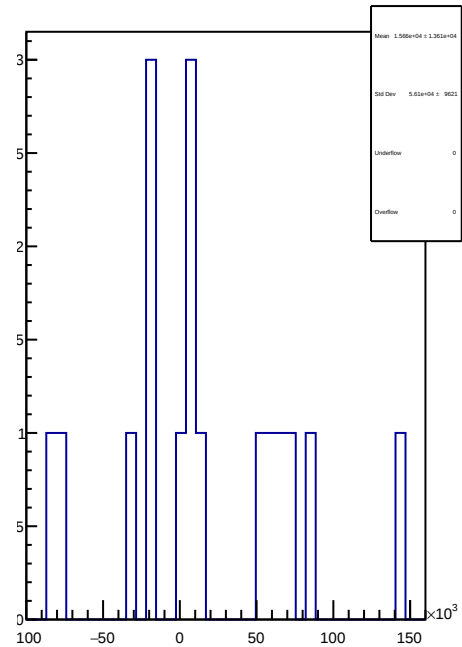
slug43-Left: 1D Corr asym_sam4.mean/ppb-reg_asym_sam4.mean/ppb
