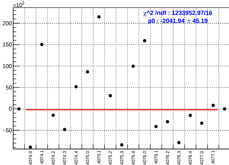
slug43-Left: asym_sam3.mean/ppb-reg_asym_sam3.mean/ppb
