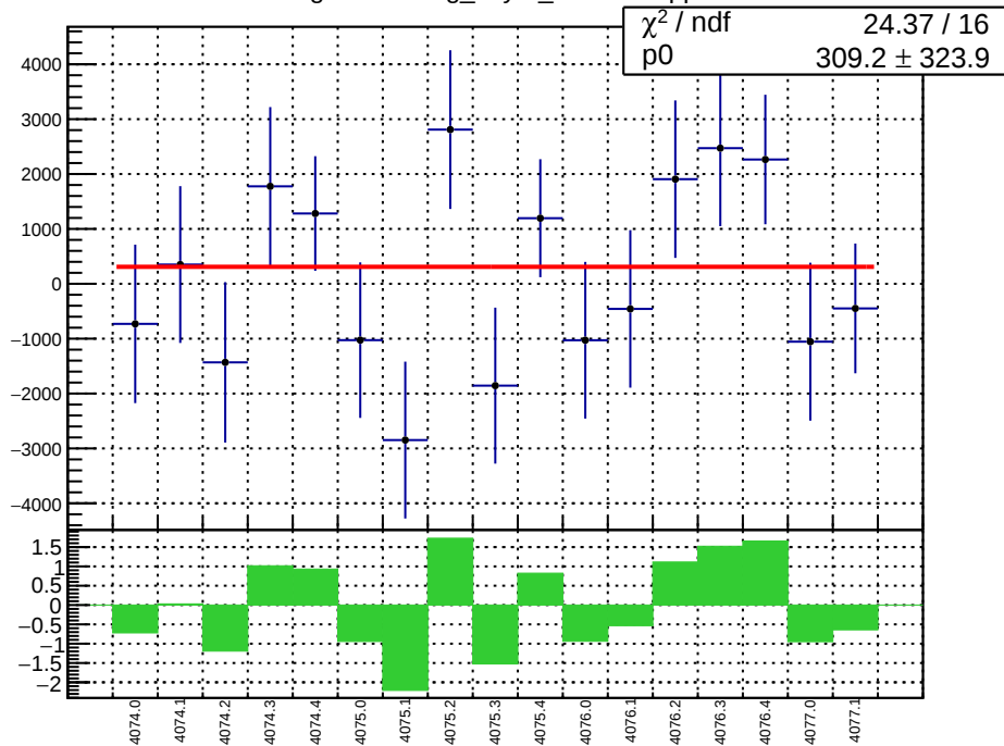
slug43-Left: reg_asym_usl.mean/ppb
