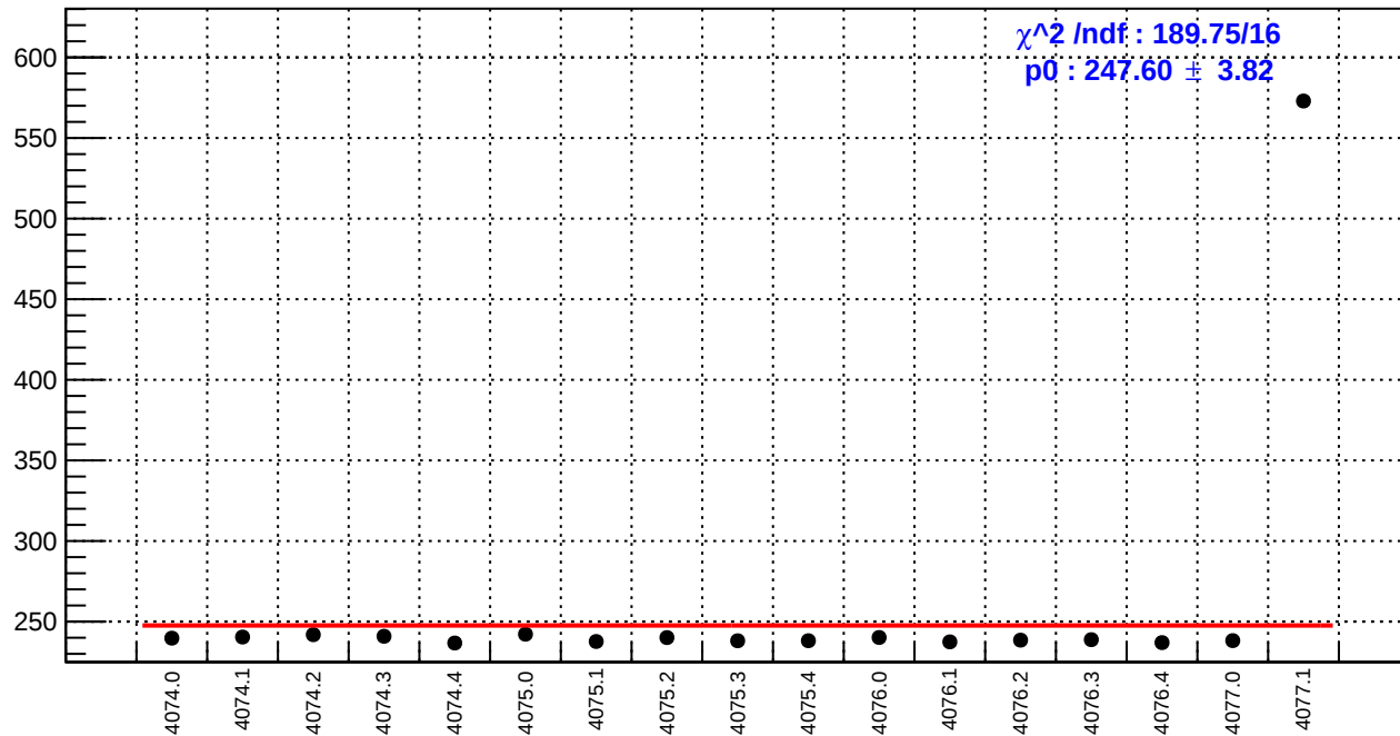
slug43-Left: reg_asym_us_avg.rms/ppm
