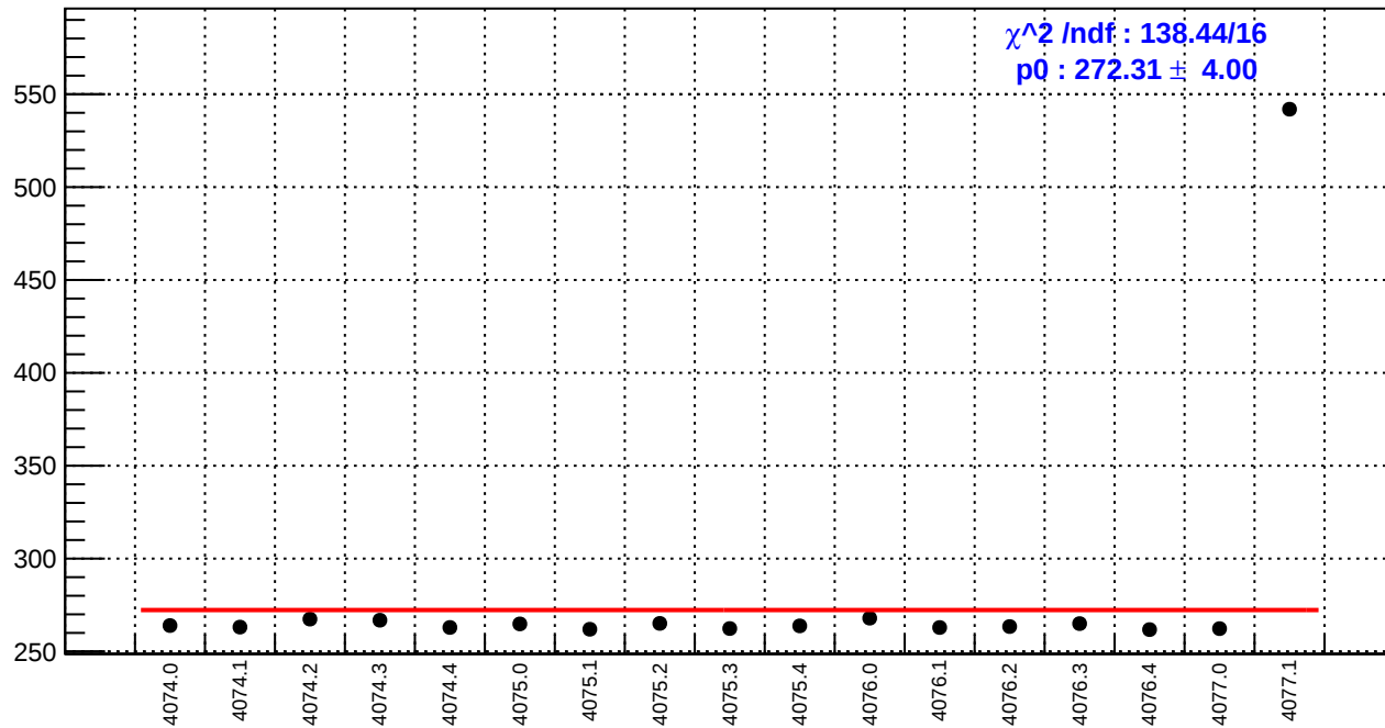
slug43-Left: reg_asym_ds_avg.rms/ppm
