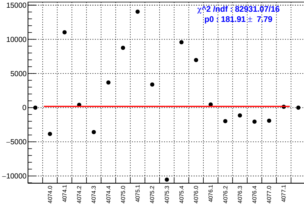
slug43-Left: asym_left_avg.mean/ppb-reg_asym_left_avg.mean/ppb
