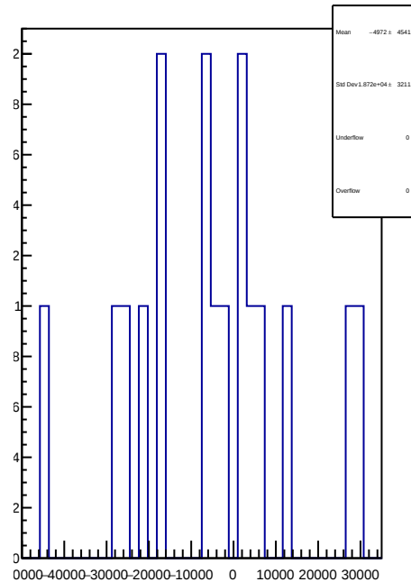
slug43-Left: 1D Corr asym_sam8.mean/ppb-reg_asym_sam8.mean/ppb
