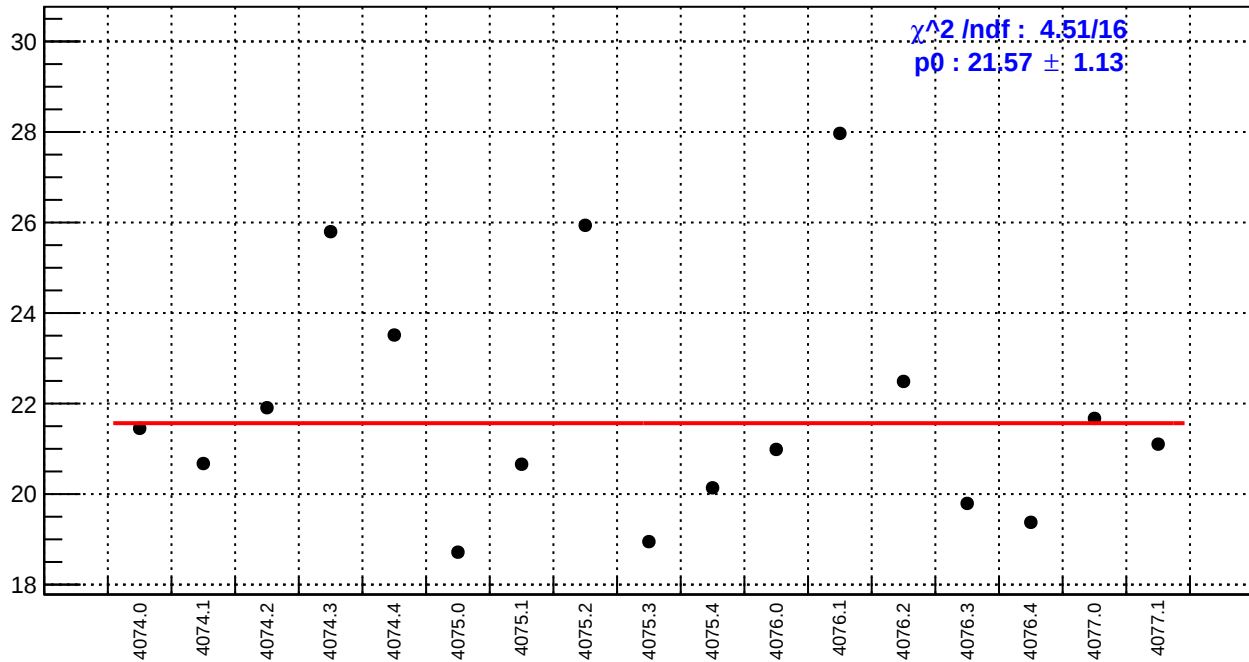
slug43-Left: dsl_bpm4aX/(ppb/nm)
