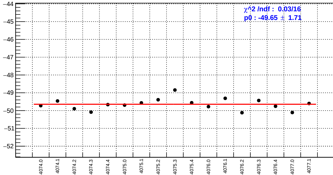
slug43-Left: usl_bpm12X/(ppb/nm)
