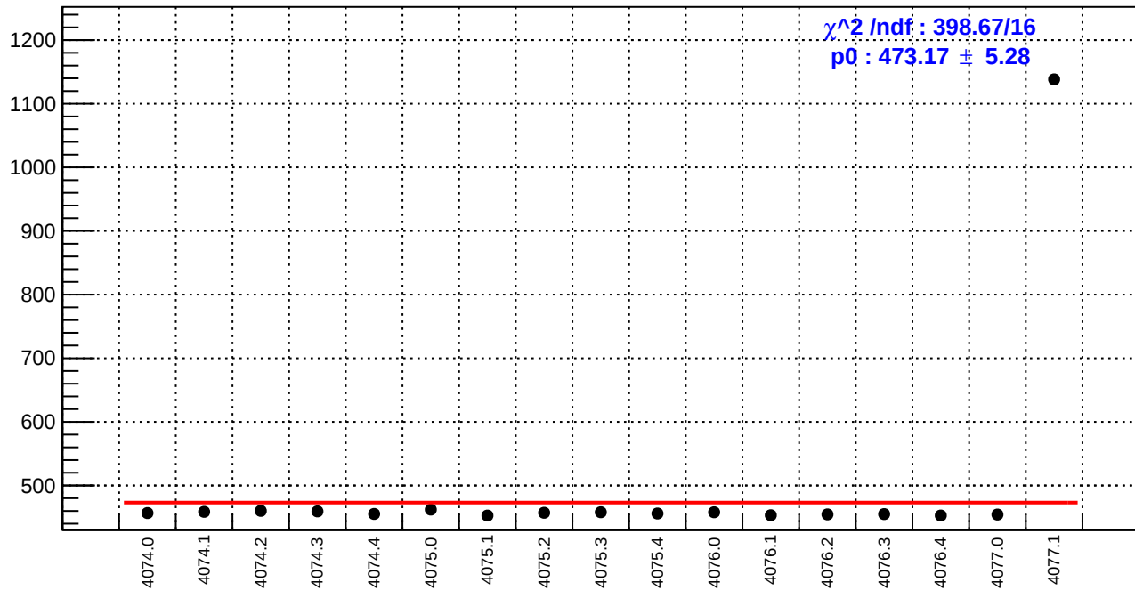
slug43-Left: reg_asym_usr.rms/ppm
