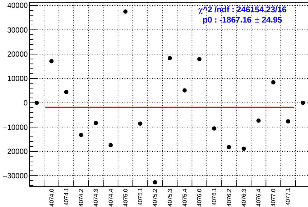
slug43-Left: asym_sam1.mean/ppb-reg_asym_sam1.mean/ppb
