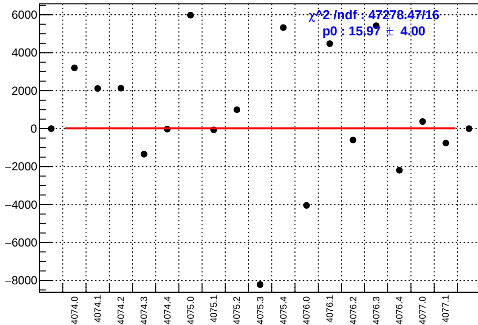
slug43-Left: asym_us_avg.mean/ppb-reg_asym_us_avg.mean/ppb
