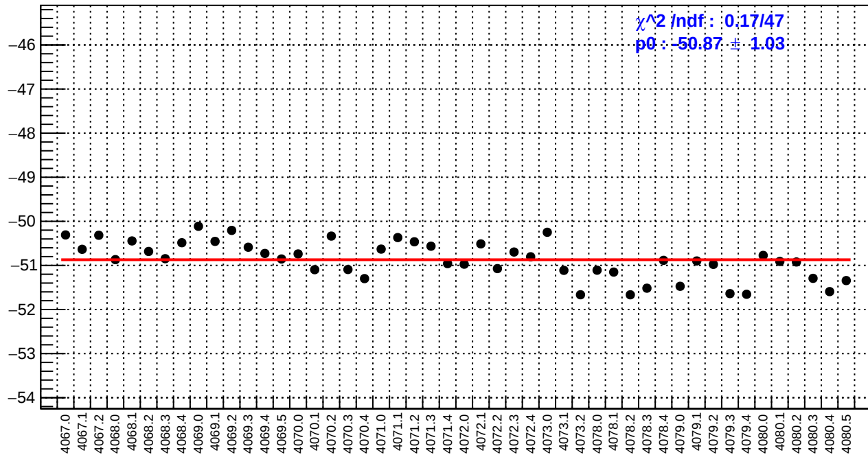
slug43: dsl_bpm12X/(ppb/nm)
