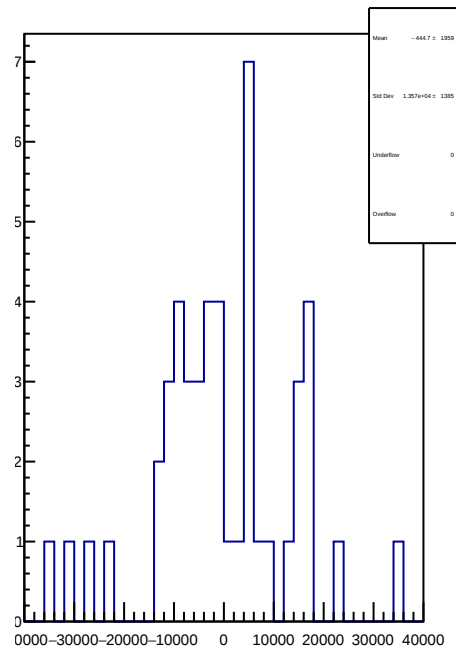
slug43: 1D Corr asym_sam1.mean/ppb-reg_asym_sam1.mean/ppb
