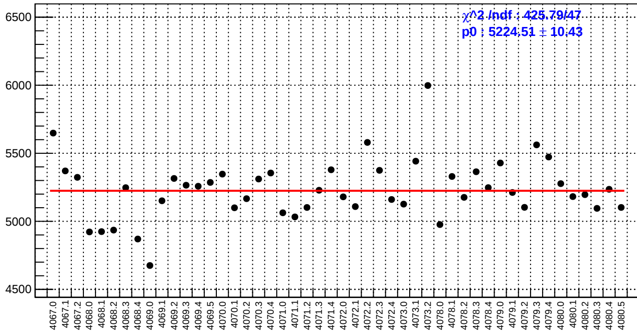
slug43: diff_bpm11X.rms/nm
