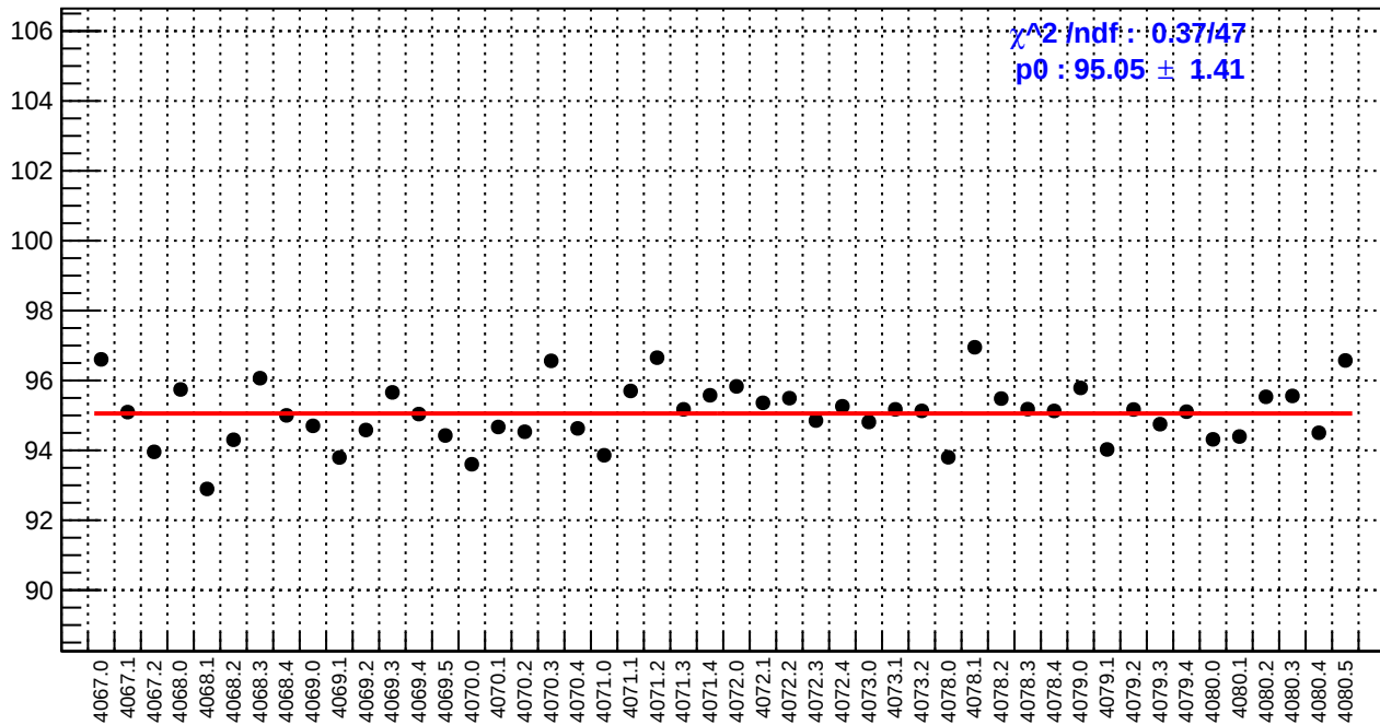
slug43: reg_asym_us_avg.rms/ppm
