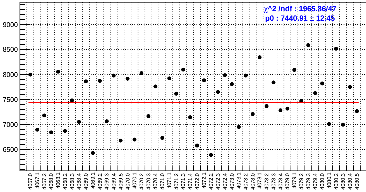
slug43: diff_bpm4aY.rms/nm
