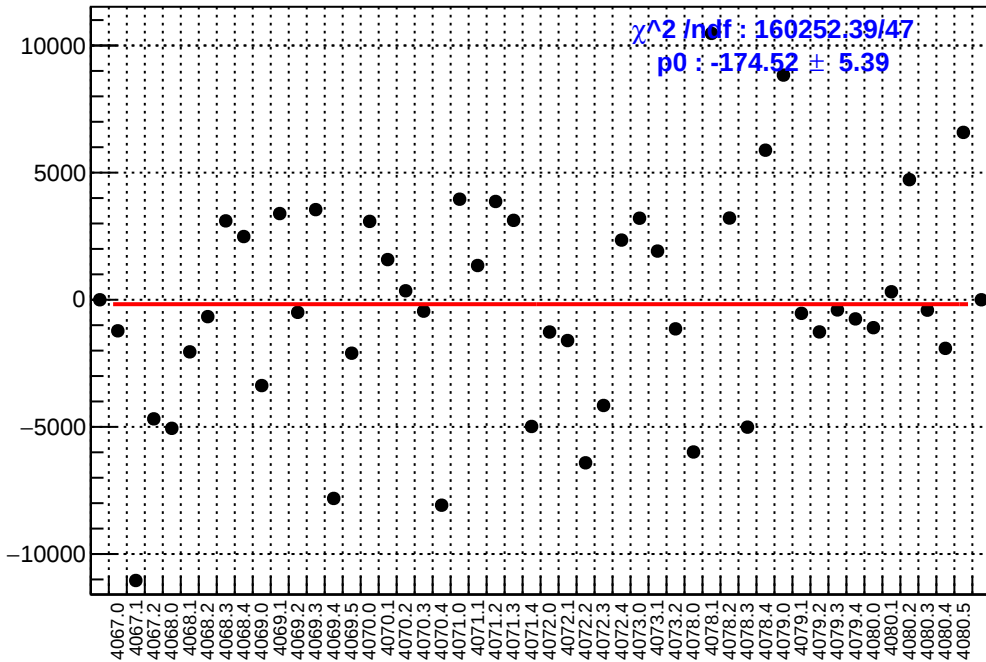
slug43: asym_usr.mean/ppb-reg_asym_usr.mean/ppb
