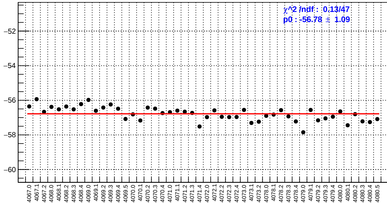
slug43: right_avg_bpm12X/(ppb/nm)
