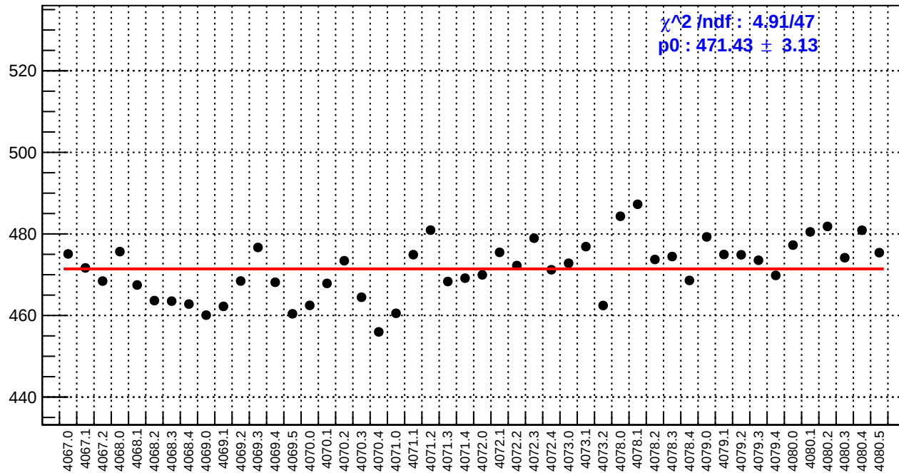
slug43: reg_asym_sam8.rms/ppm
