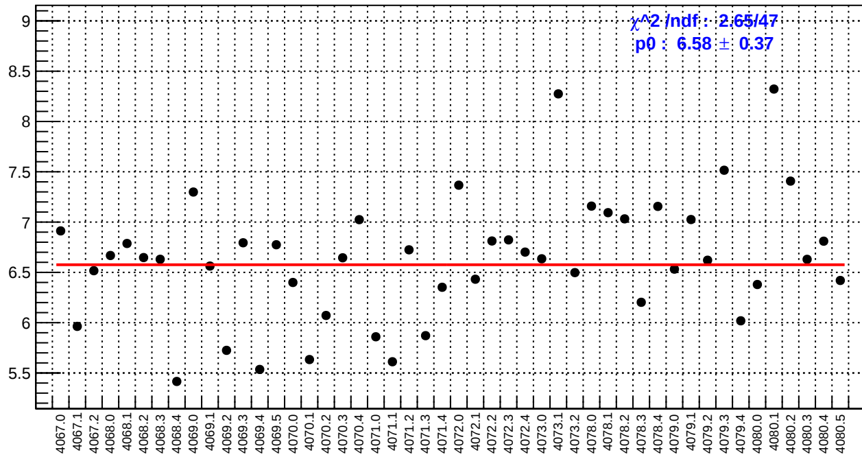
slug43: us_avg_bpm4aY/(ppb/nm)
