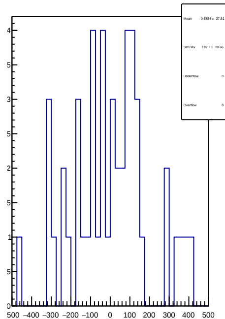
slug43: 1D Corr asym_left_dd.mean/ppb-reg_asym_left_dd.mean/ppb
