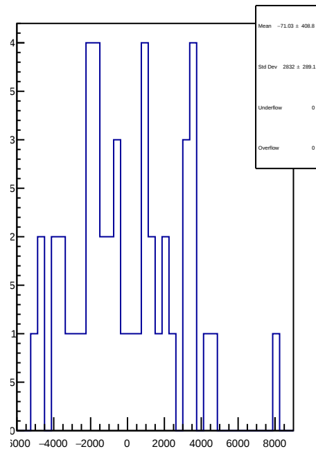
slug43: 1D Corr asym_us_avg.mean/ppb-reg_asym_us_avg.mean/ppb
