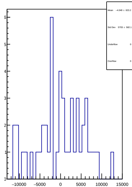
slug43: 1D Corr asym_usl.mean/ppb-reg_asym_usl.mean/ppb
