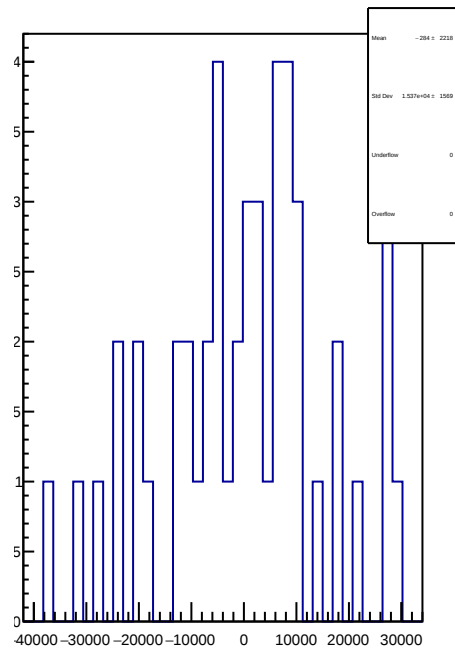
slug43: 1D Corr asym_sam7.mean/ppb-reg_asym_sam7.mean/ppb
