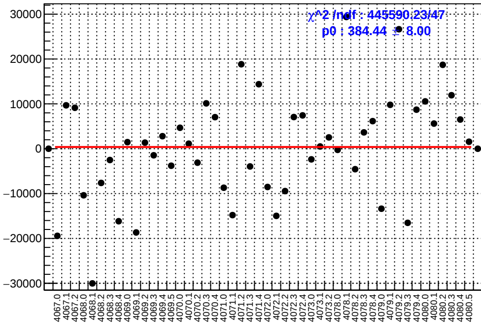
slug43: asym_sam5.mean/ppb-reg_asym_sam5.mean/ppb
