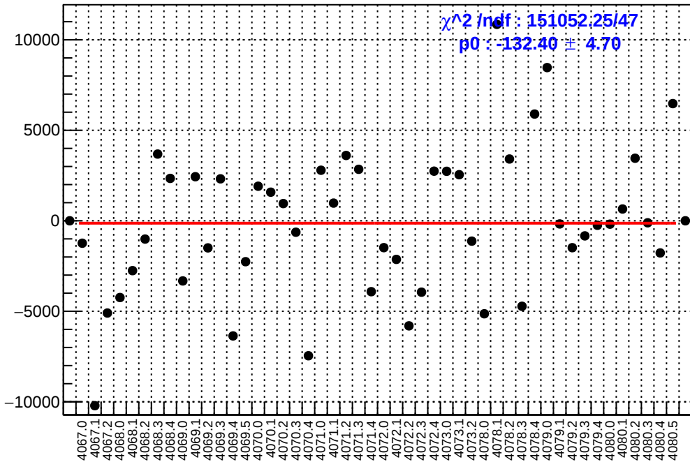
slug43: asym_dsr.mean/ppb-reg_asym_dsr.mean/ppb
