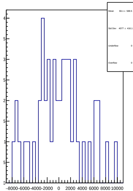
slug43: 1D Corr asym_ds_dd.mean/ppb-reg_asym_ds_dd.mean/ppb
