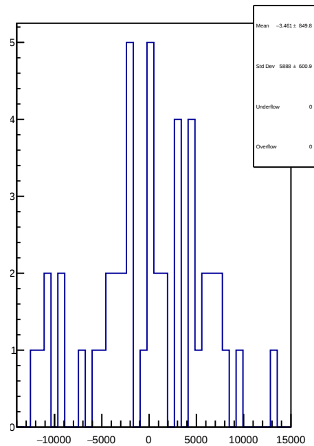
slug43: 1D Corr asym_left_avg.mean/ppb-reg_asym_left_avg.mean/ppb
