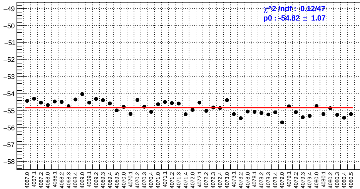
slug43: ds_avg_bpm12X/(ppb/nm)
