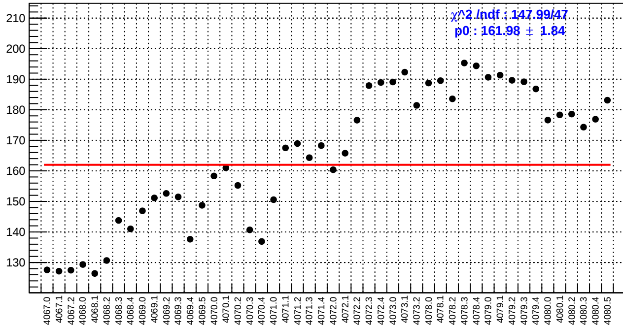
slug43: asym_bcm_an_us.rms/ppm
