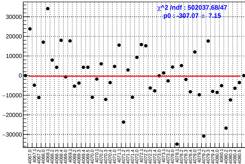
slug43: asym_sam1.mean/ppb-reg_asym_sam1.mean/ppb
