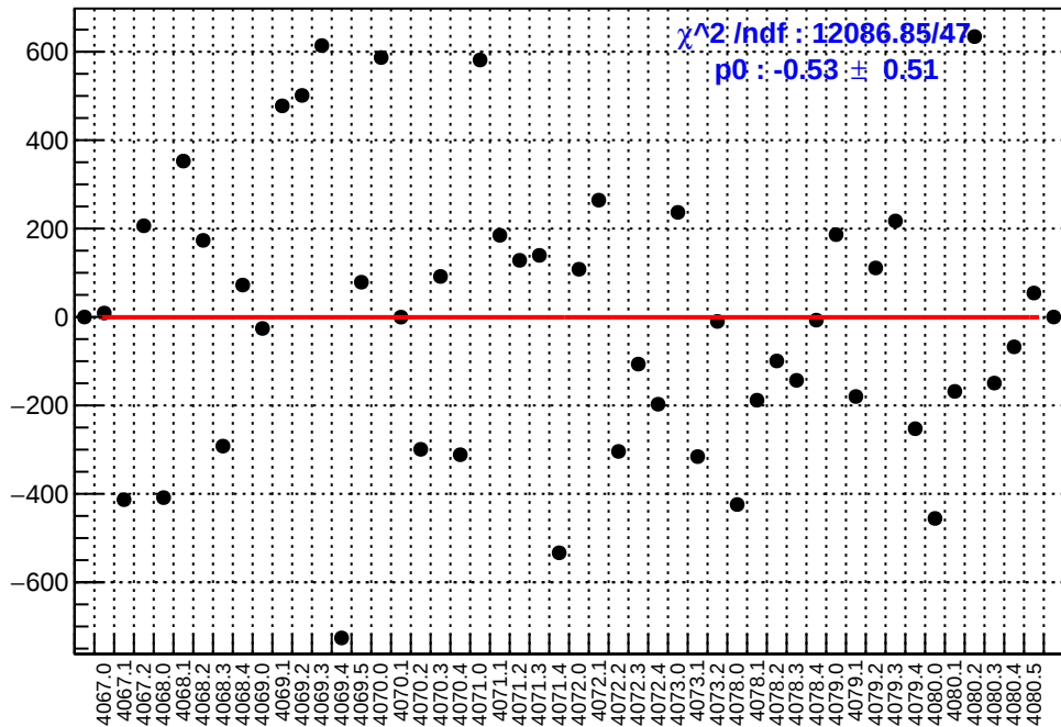
slug43: asym_right_dd.mean/ppb-reg_asym_right_dd.mean/ppb
