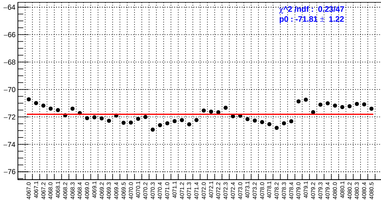
slug43: left_avg_bpm4eX/(ppb/nm)
