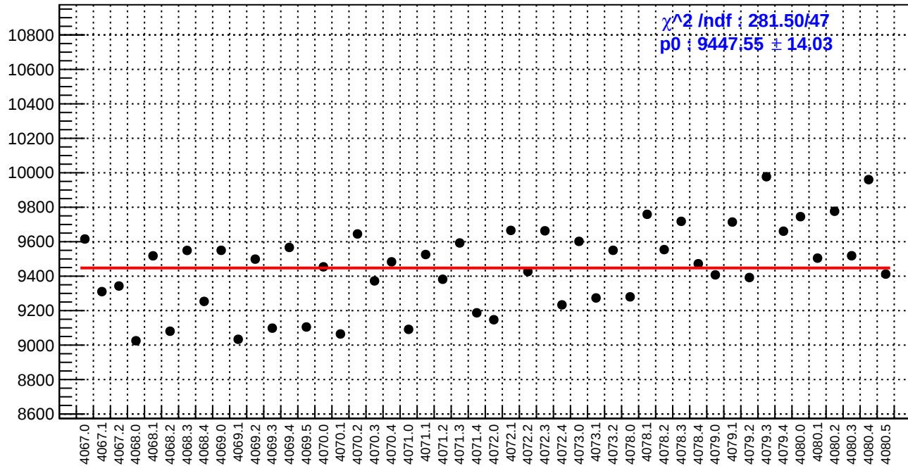
slug43: diff_bpm4eX.rms/nm
