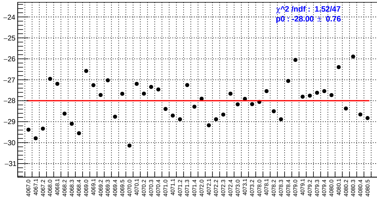
slug43: right_avg_bpm4aX/(ppb/nm)
