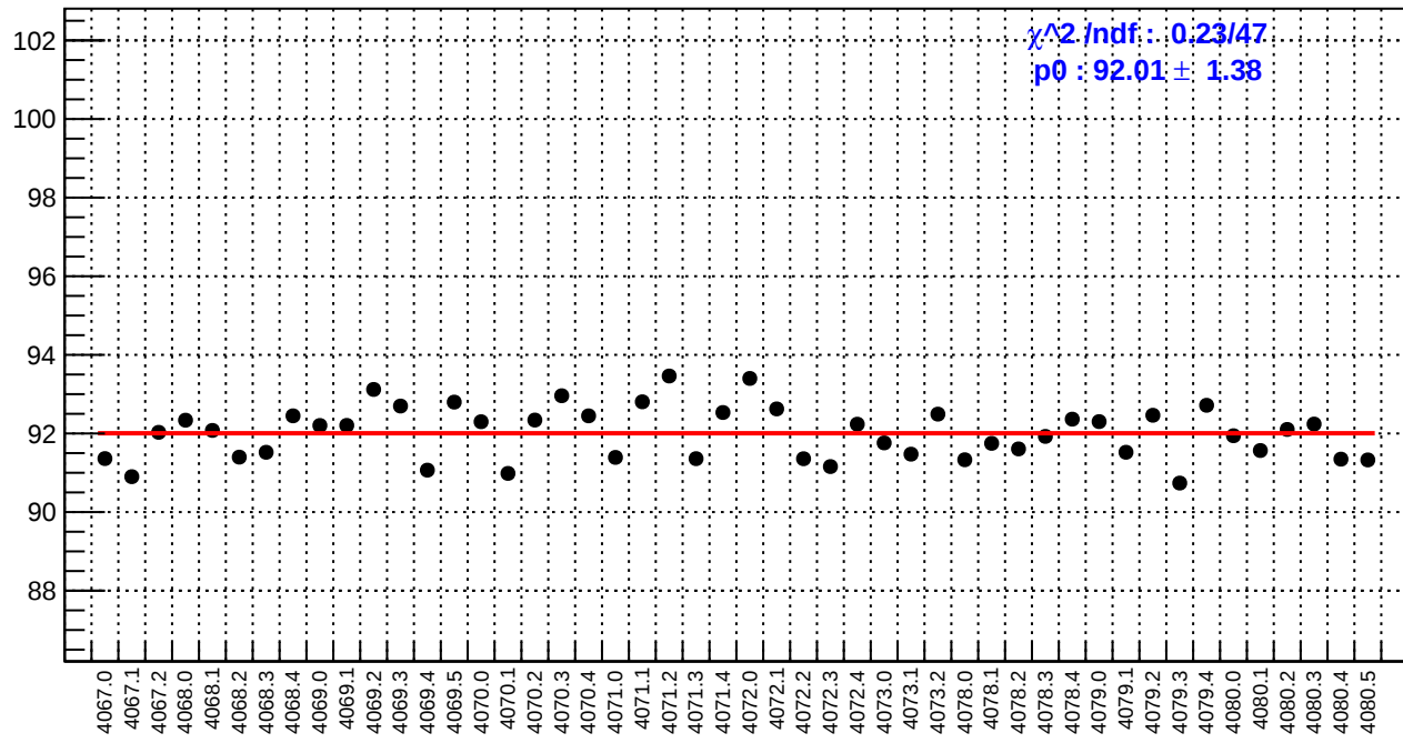
slug43: reg_asym_us_dd.rms/ppm
