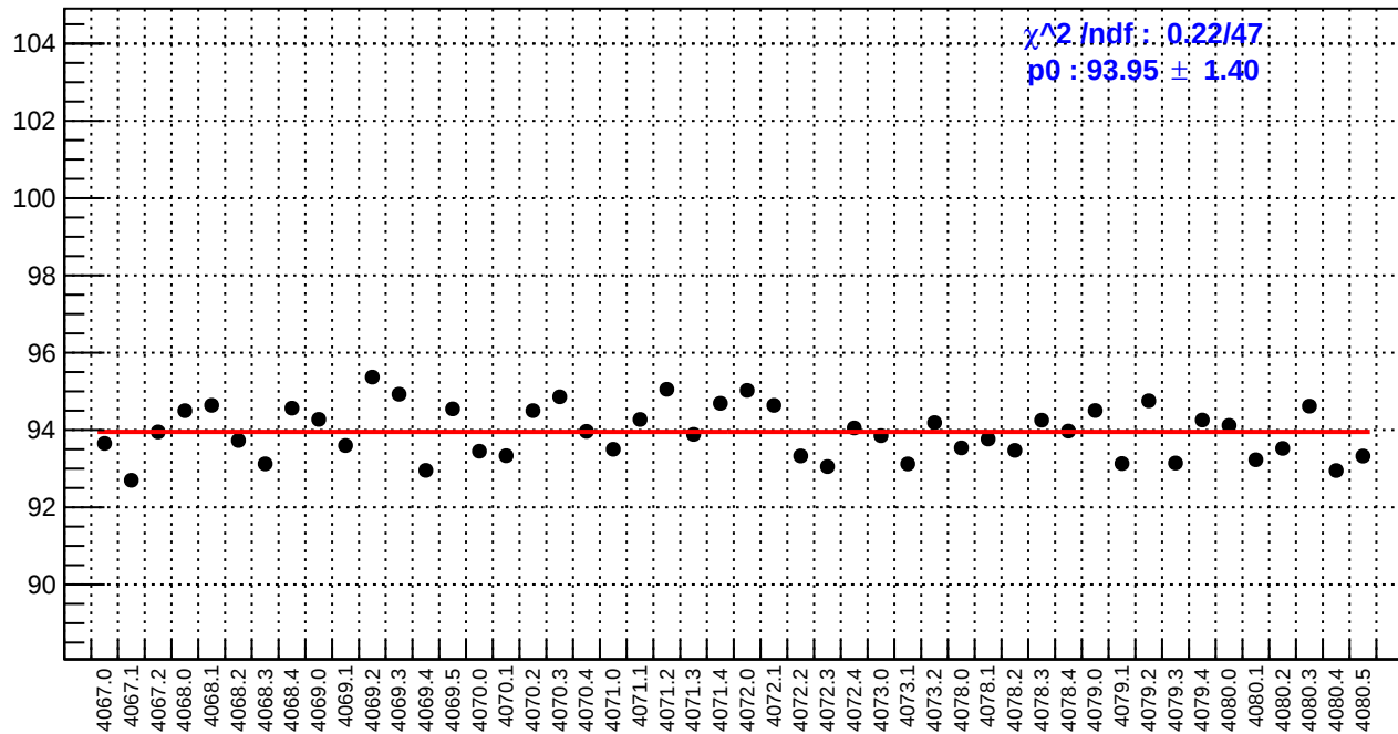
slug43: reg_asym_ds_dd.rms/ppm
