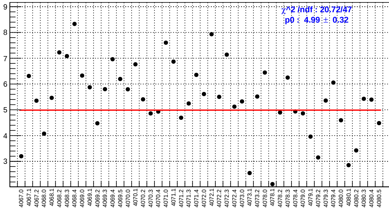
slug43: dsl_bpm4eY/(ppb/nm)
