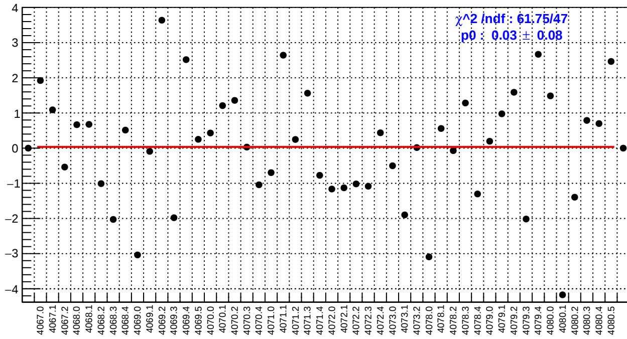
slug43: right_avg_bpm4eY/(ppb/nm)
