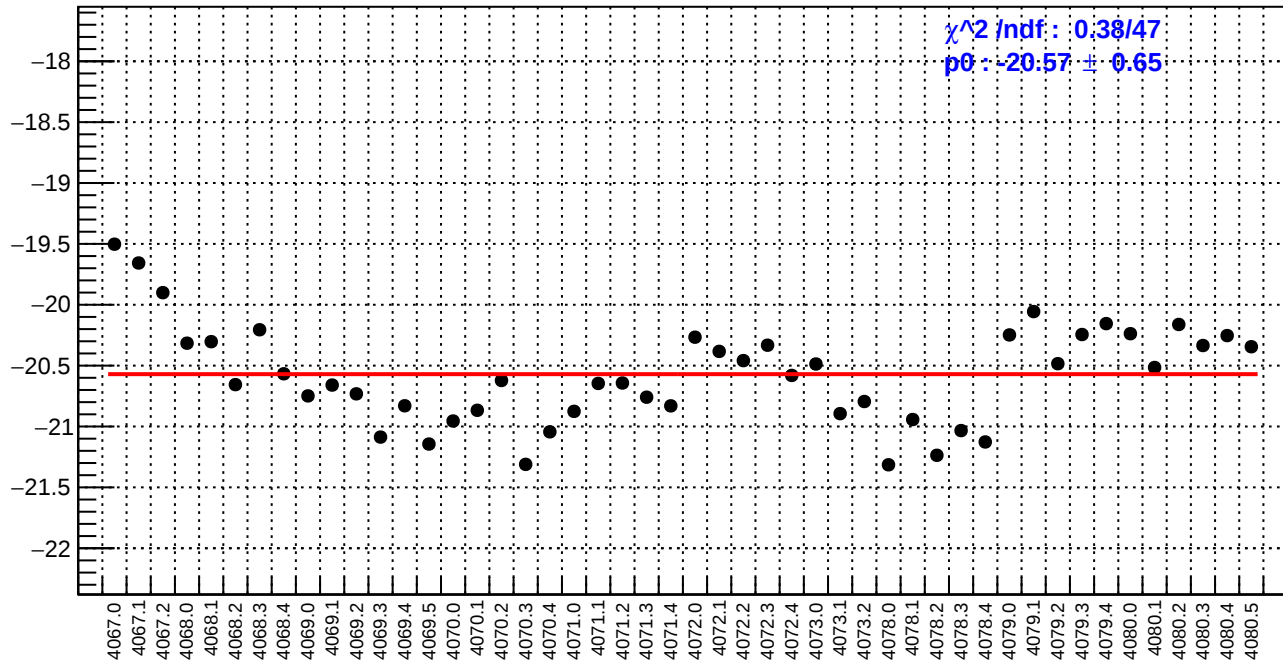
slug43: us_avg_bpm4eX/(ppb/nm)
