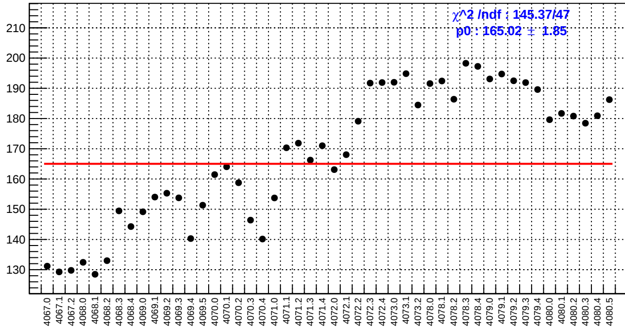
slug43: asym_bcm_an_ds3.rms/ppm
