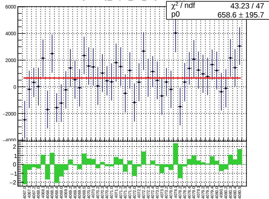
slug43: reg_asym_left_avg.mean/ppb
