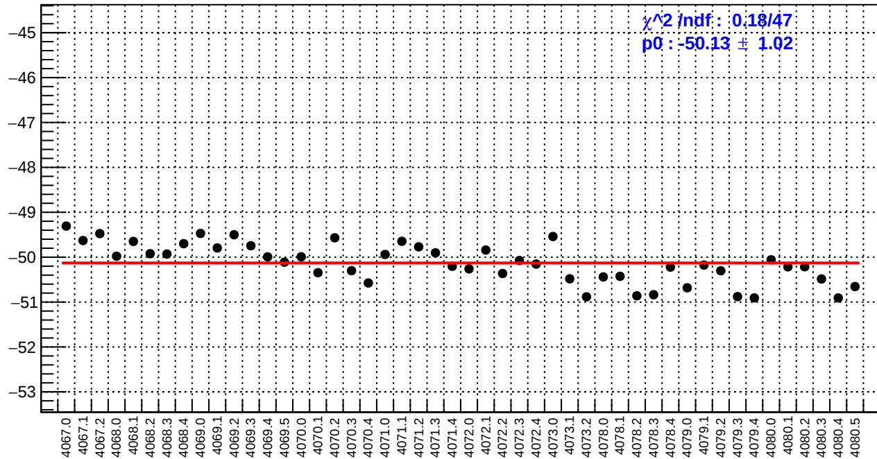
slug43: left_avg_bpm12X/(ppb/nm)
