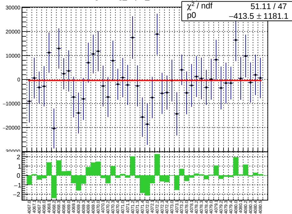
slug43: reg_asym_sam3.mean/ppb
