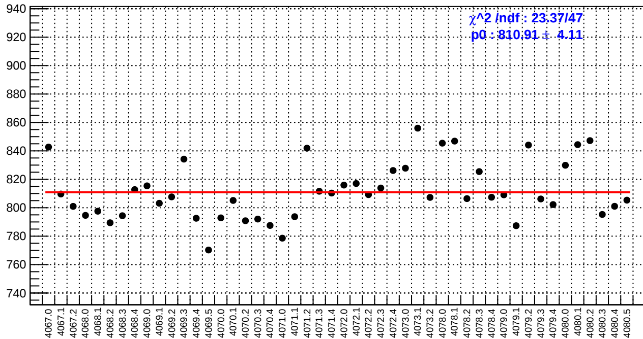
slug43: reg_asym_sam3.rms/ppm
