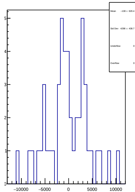
slug43: 1D Corr asym_usr.mean/ppb-reg_asym_usr.mean/ppb
