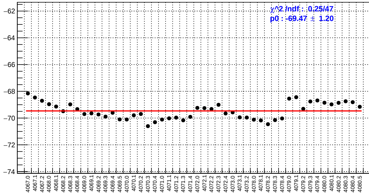
slug43: usl_bpm4eX/(ppb/nm)
