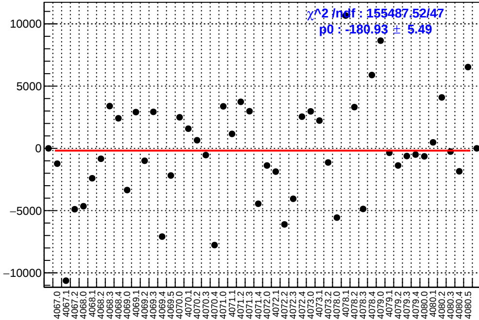
slug43: asym_right_avg.mean/ppb-reg_asym_right_avg.mean/ppb
