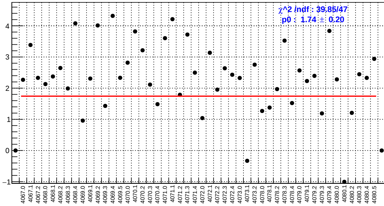
slug43: us_avg_bpm4eY/(ppb/nm)
