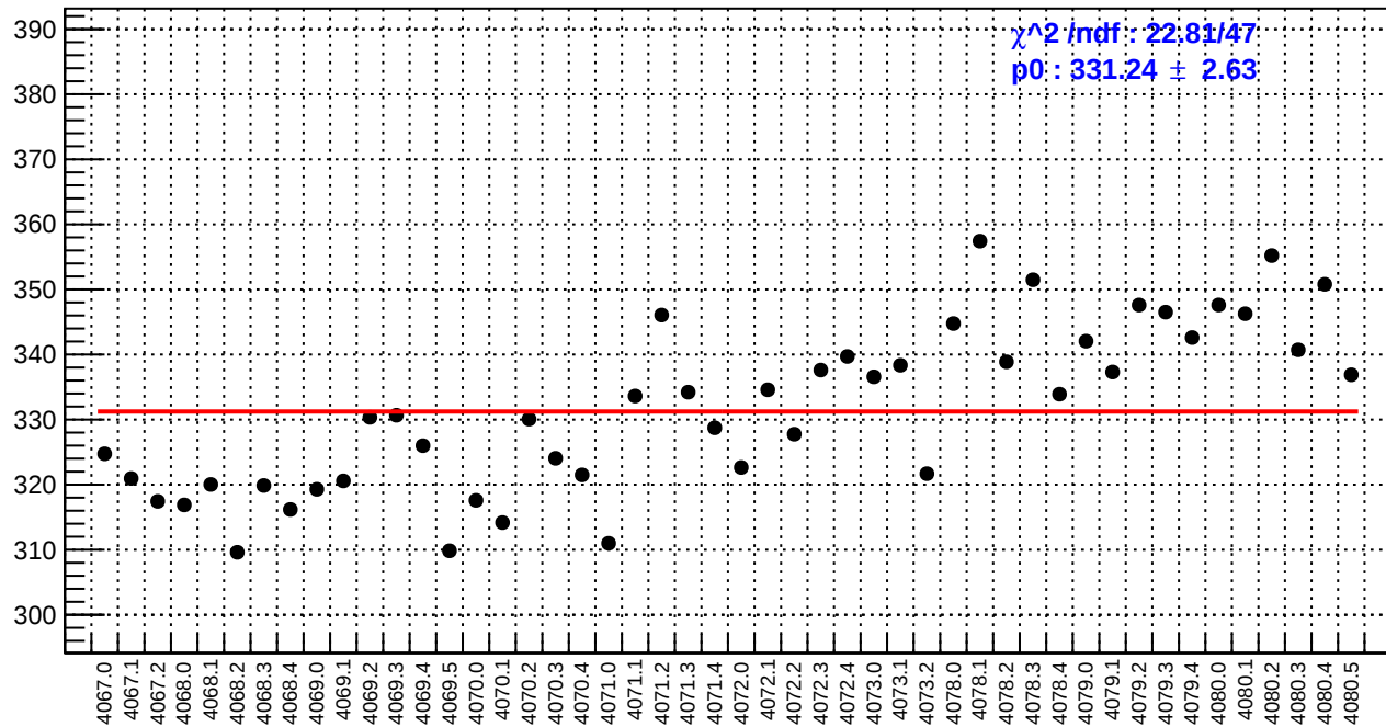
slug43: reg_asym_sam5.rms/ppm
