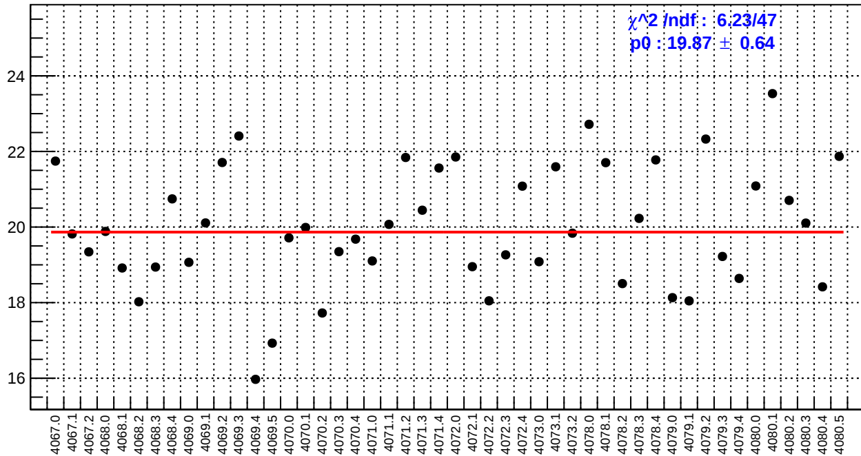
slug43: usl_bpm4aX/(ppb/nm)
