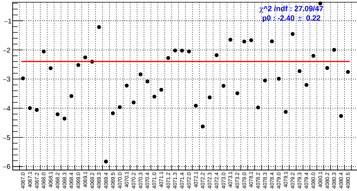
slug43: ds_avg_bpm4aX/(ppb/nm)
