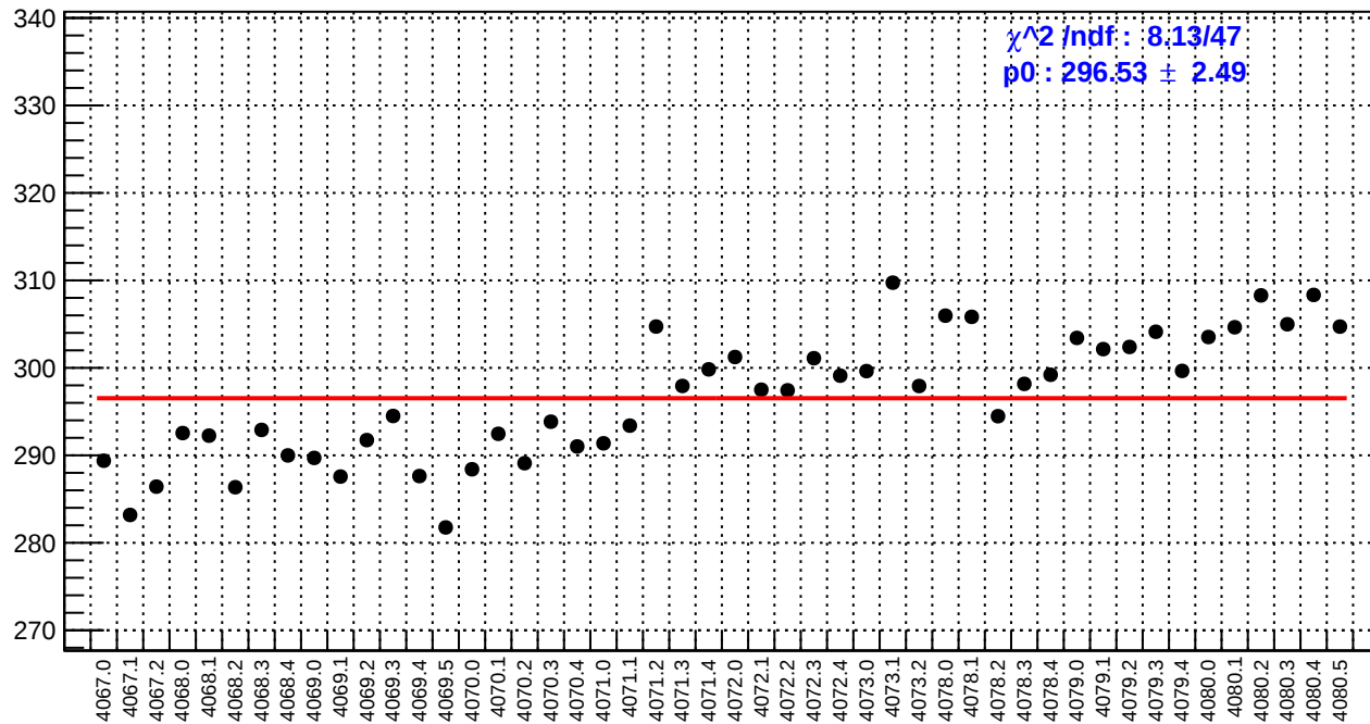
slug43: reg_asym_sam7.rms/ppm
