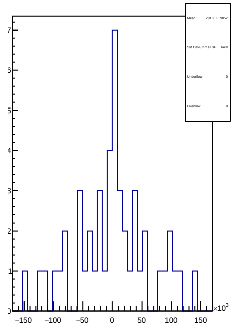
slug43: 1D Corr asym_sam2.mean/ppb-reg_asym_sam2.mean/ppb
