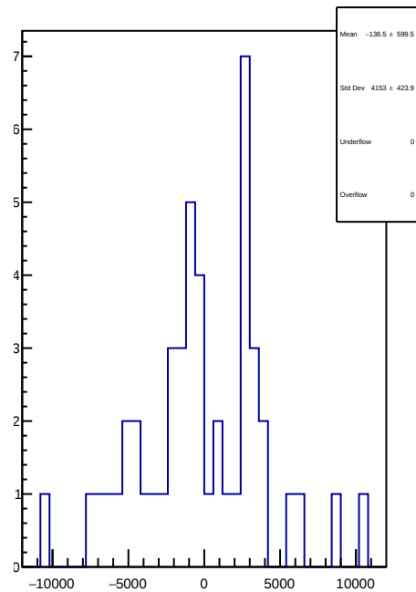
slug43: 1D Corr asym_right_avg.mean/ppb-reg_asym_right_avg.mean/ppb
