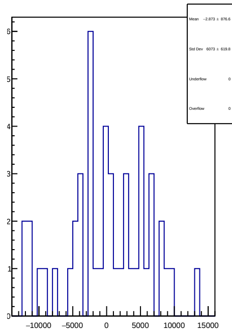
slug43: 1D Corr asym_dsl.mean/ppb-reg_asym_dsl.mean/ppb
