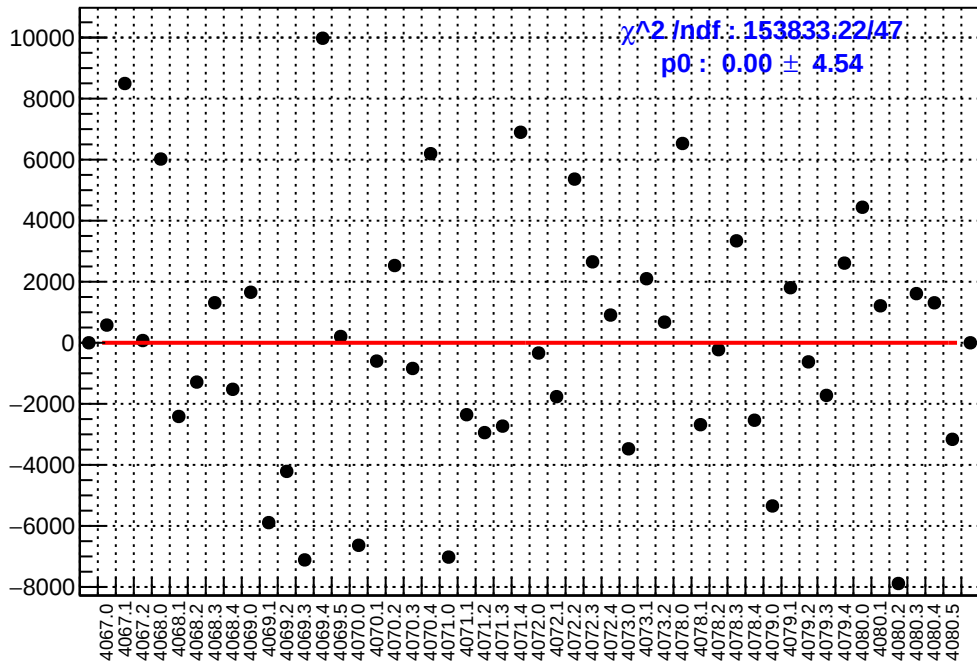
slug43: asym_ds_dd.mean/ppb-reg_asym_ds_dd.mean/ppb
