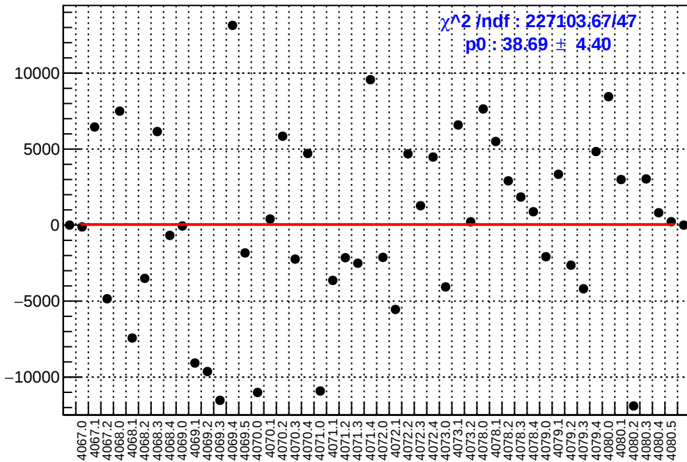
slug43: asym_left_avg.mean/ppb-reg_asym_left_avg.mean/ppb
