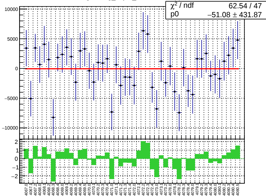
slug43: reg_asym_sam7.mean/ppb
