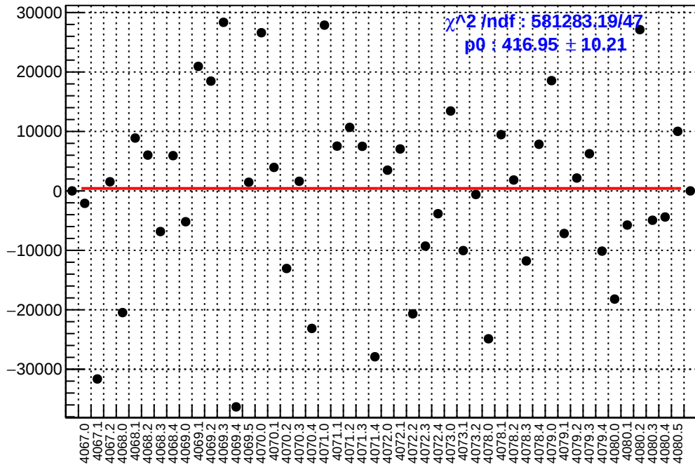
slug43: asym_sam7.mean/ppb-reg_asym_sam7.mean/ppb
