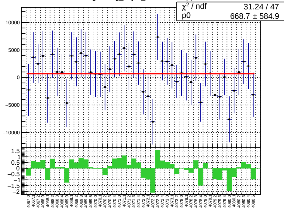
slug43: reg_asym_sam1.mean/ppb
