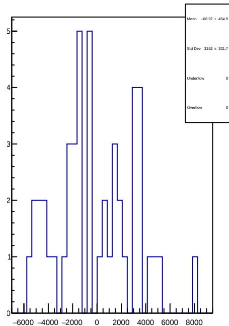
slug43: 1D Corr asym_ds_avg.mean/ppb-reg_asym_ds_avg.mean/ppb
