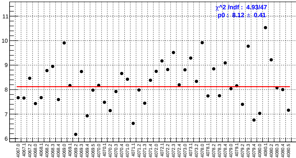
slug43: right_avg_bpm4aY/(ppb/nm)
