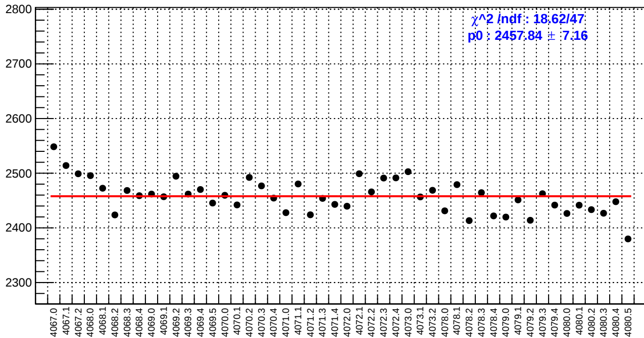
slug43: reg_asym_sam2.rms/ppm
