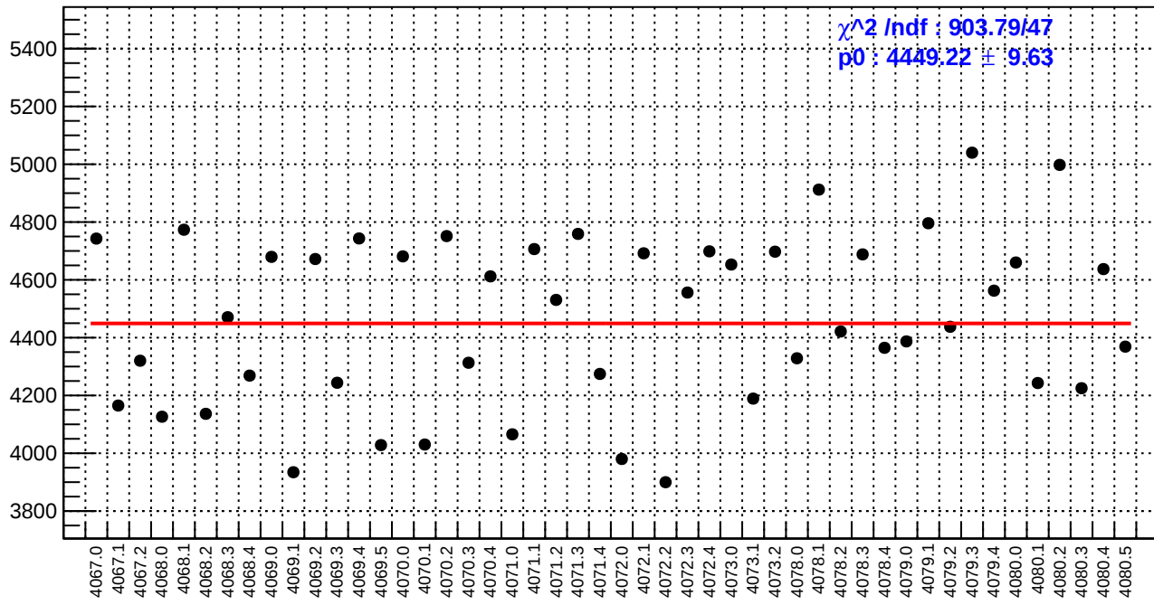
slug43: diff_bpm4eY.rms/nm
