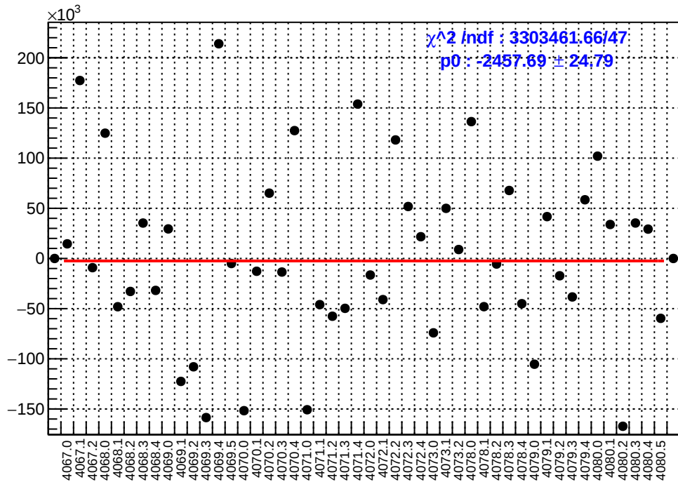
slug43: asym_sam3.mean/ppb-reg_asym_sam3.mean/ppb
