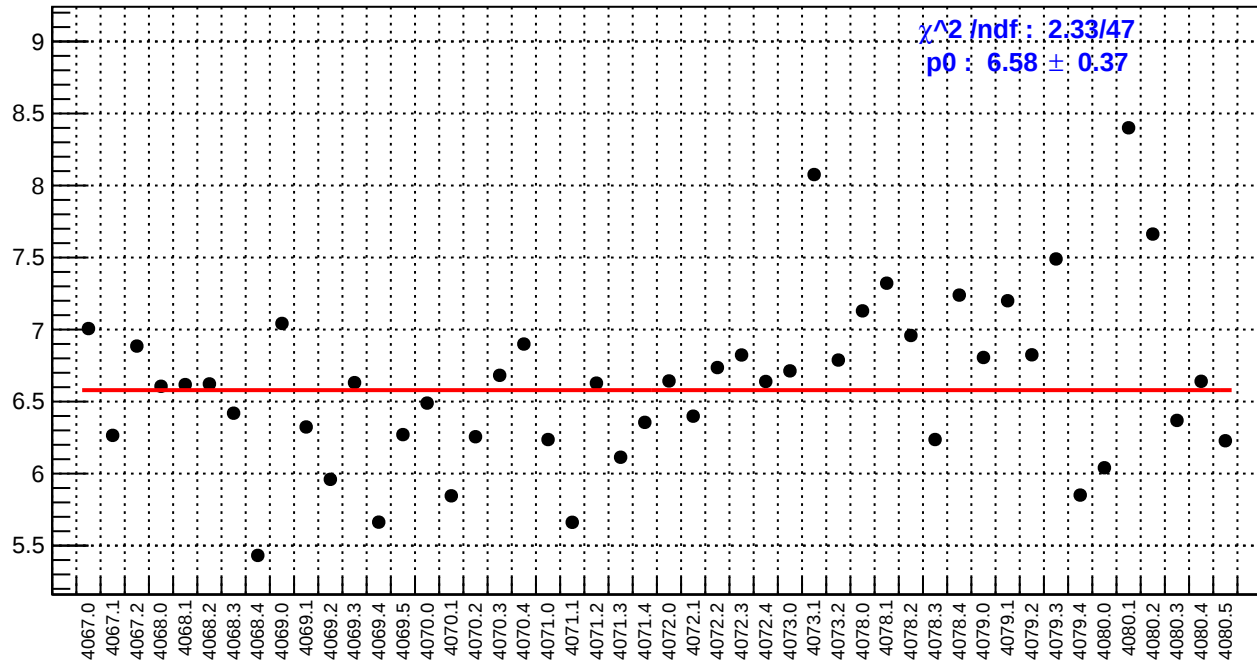
slug43: ds_avg_bpm4aY/(ppb/nm)
