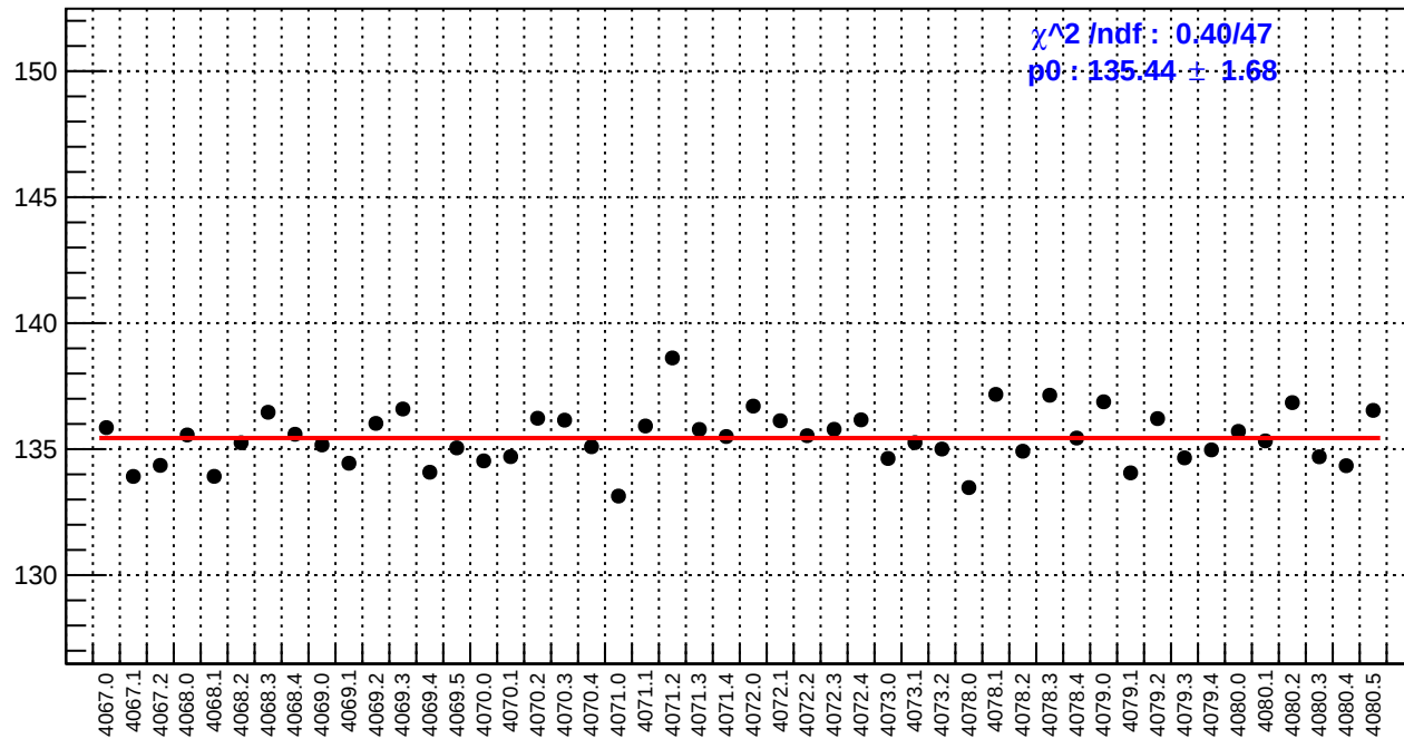
slug43: reg_asym_usl.rms/ppm
