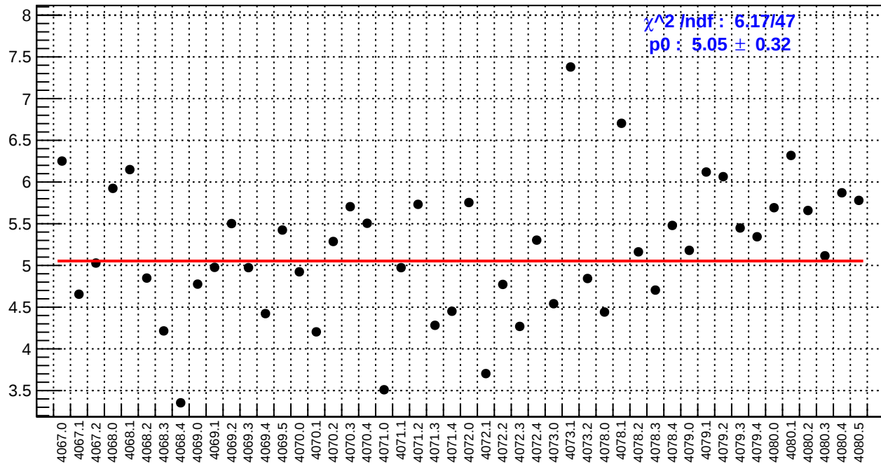
slug43: usl_bpm4aY/(ppb/nm)
