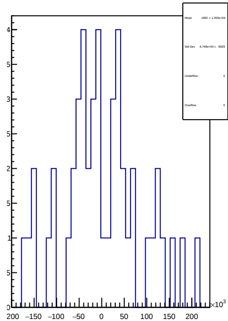
slug43: 1D Corr asym_sam3.mean/ppb-reg_asym_sam3.mean/ppb
