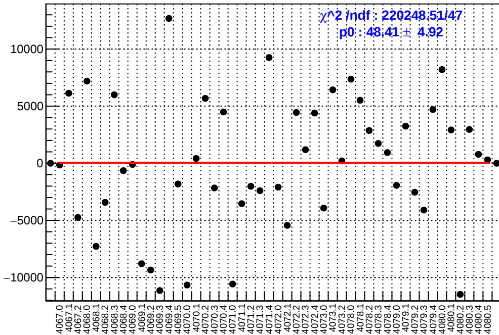
slug43: asym_usl.mean/ppb-reg_asym_usl.mean/ppb
