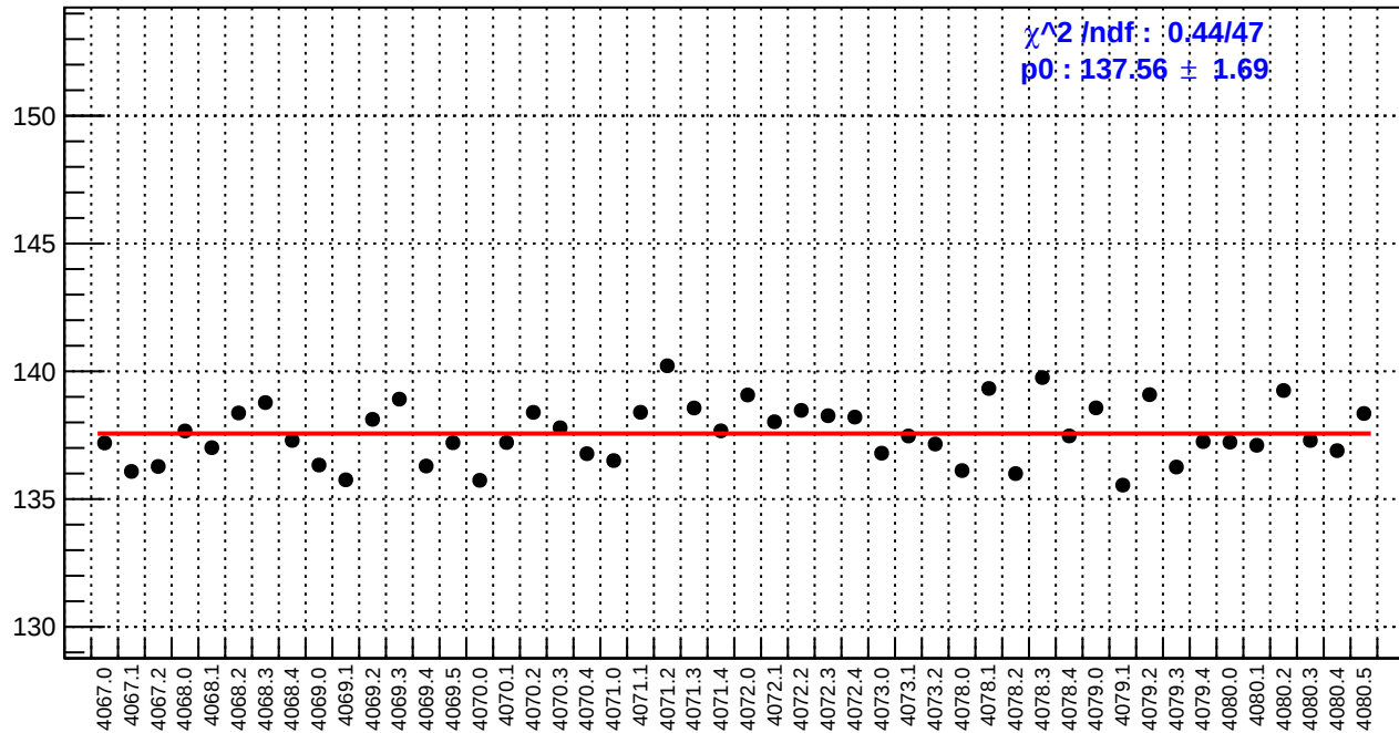
slug43: reg_asym_dsl.rms/ppm
