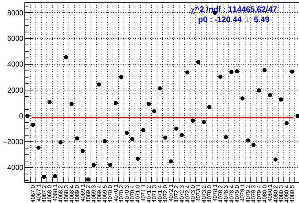
slug43: asym_us_avg.mean/ppb-reg_asym_us_avg.mean/ppb
