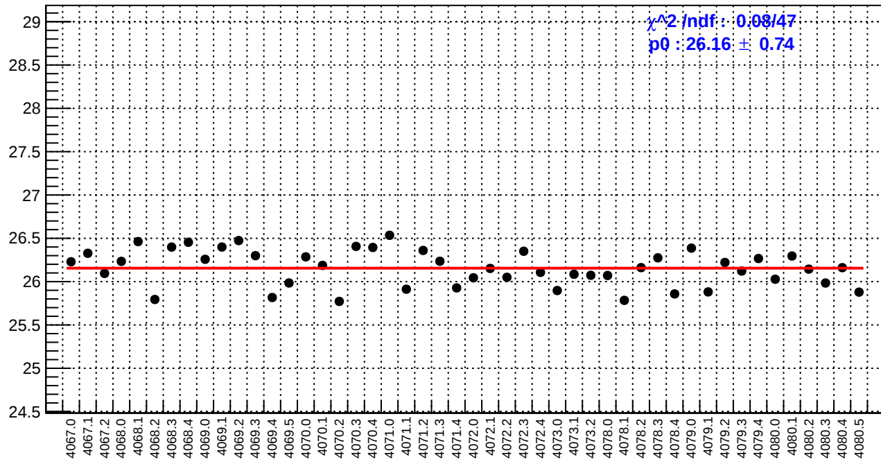
slug43: reg_asym_right_dd.rms/ppm
