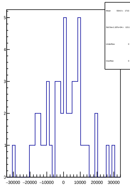
slug43: 1D Corr asym_sam5.mean/ppb-reg_asym_sam5.mean/ppb
