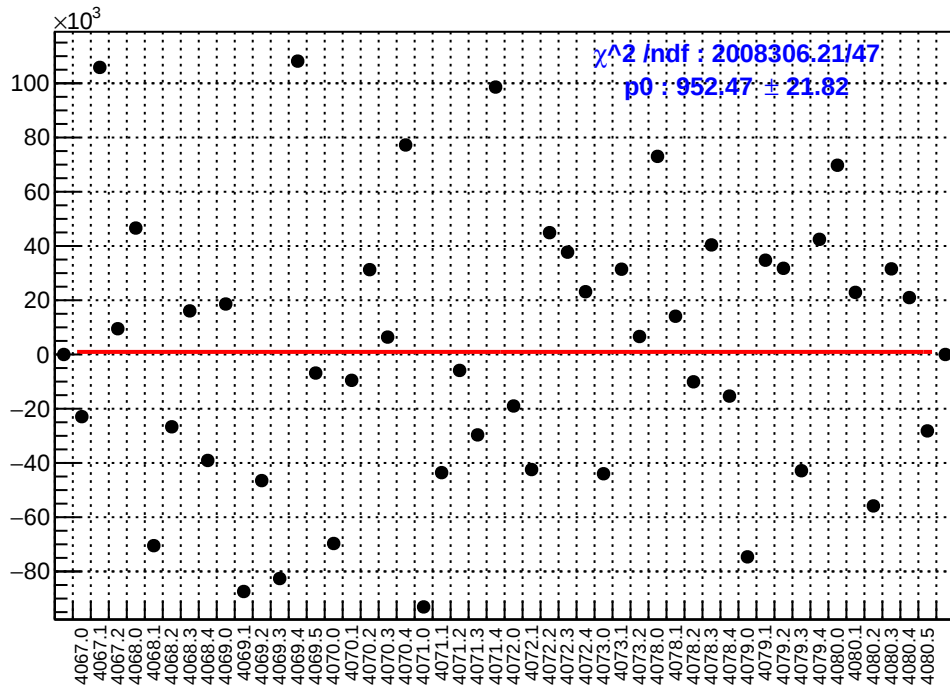
slug43: asym_sam4.mean/ppb-reg_asym_sam4.mean/ppb
