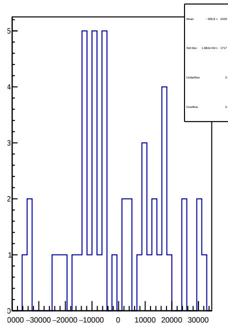
slug43: 1D Corr asym_sam8.mean/ppb-reg_asym_sam8.mean/ppb
