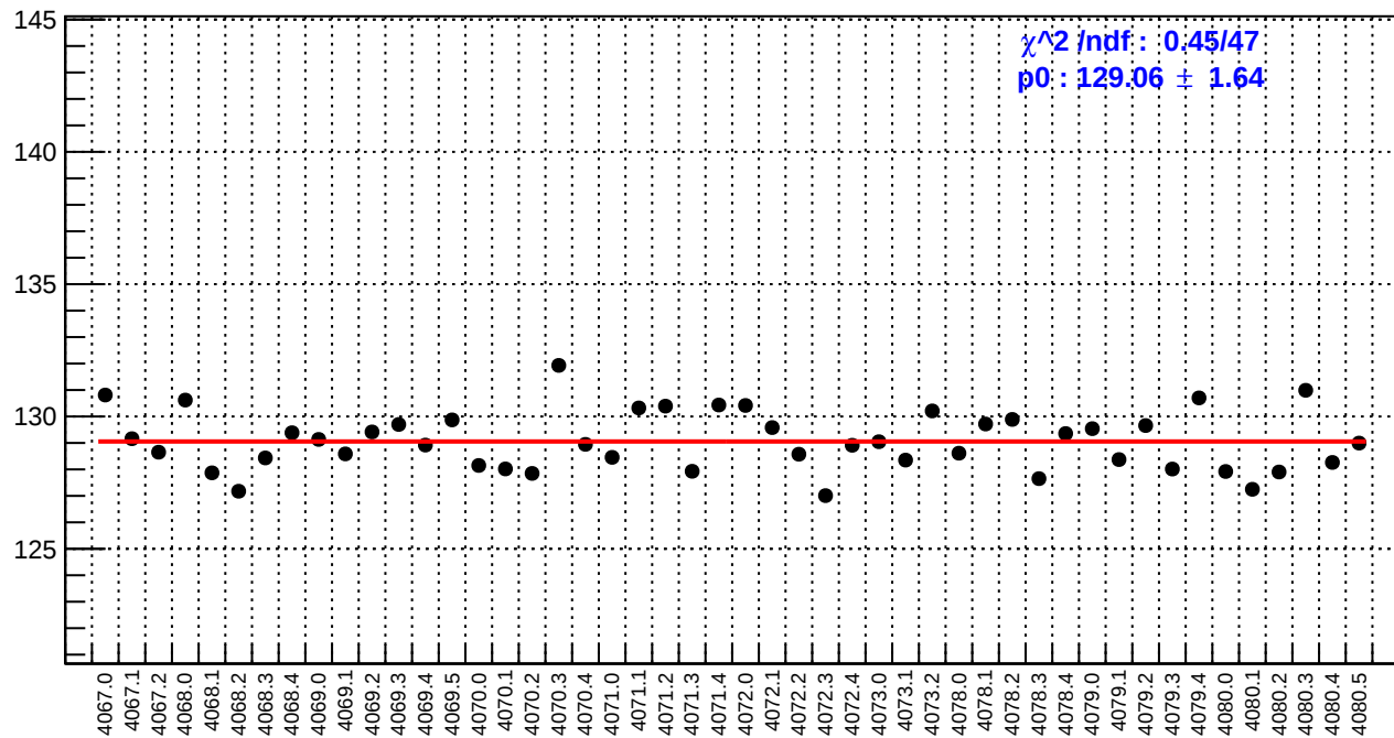
slug43: reg_asym_right_avg.rms/ppm
