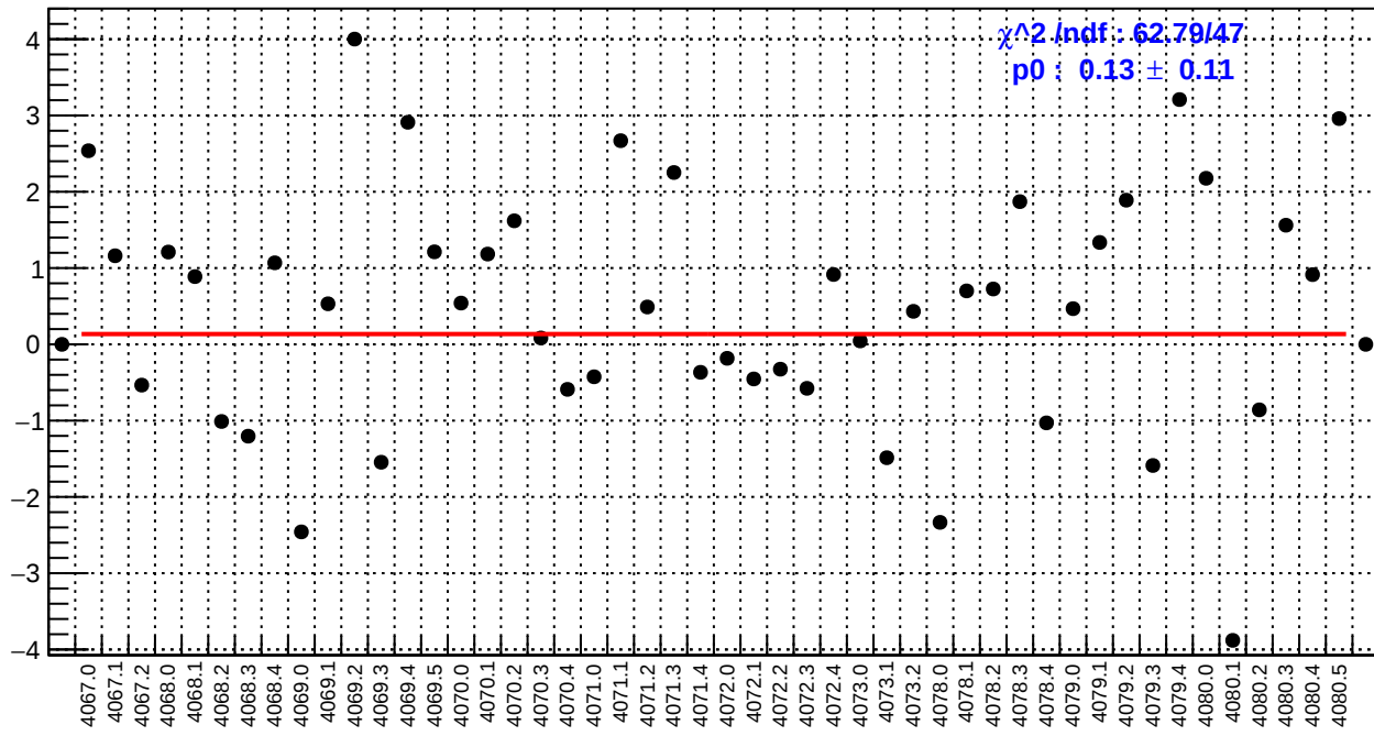
slug43: dsr_bpm4eY/(ppb/nm)
