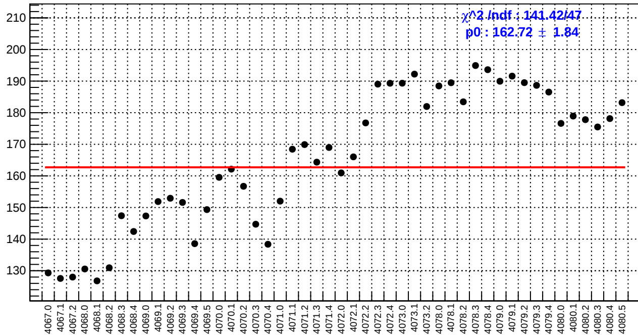
slug43: asym_bcm_an_ds.rms/ppm
