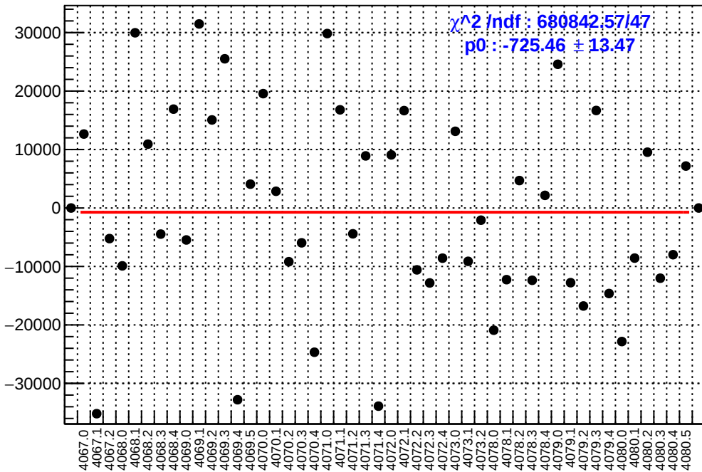
slug43: asym_sam8.mean/ppb-reg_asym_sam8.mean/ppb
