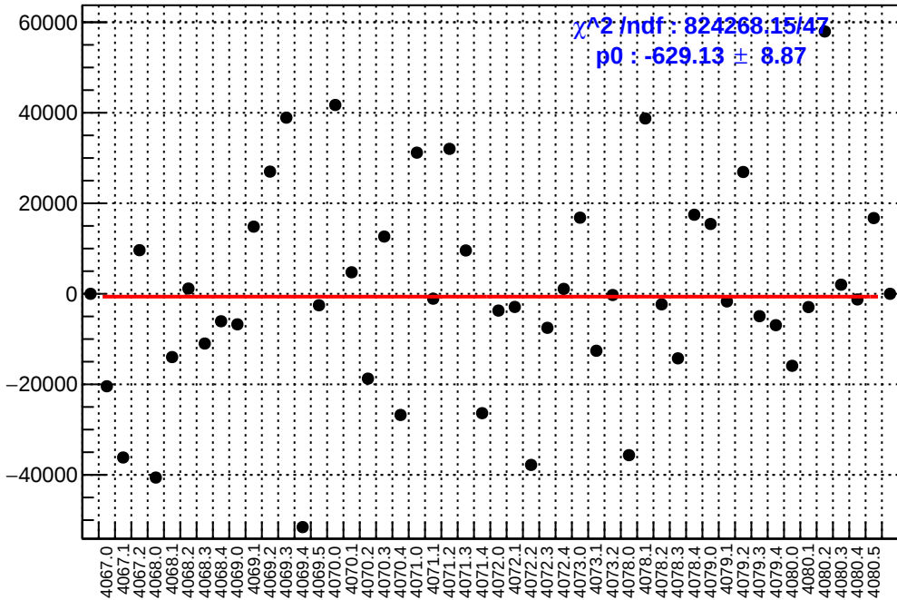
slug43: asym_sam6.mean/ppb-reg_asym_sam6.mean/ppb
