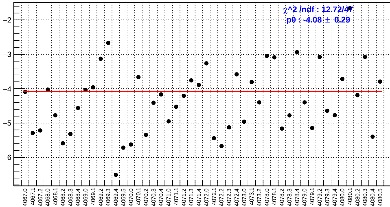
slug43: us_avg_bpm4aX/(ppb/nm)
