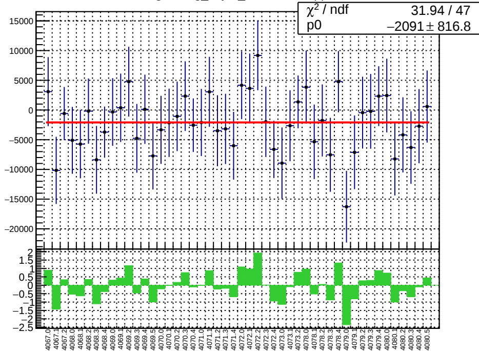
slug43: reg_asym_sam6.mean/ppb
