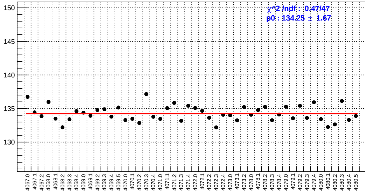
slug43: reg_asym_dsr.rms/ppm
