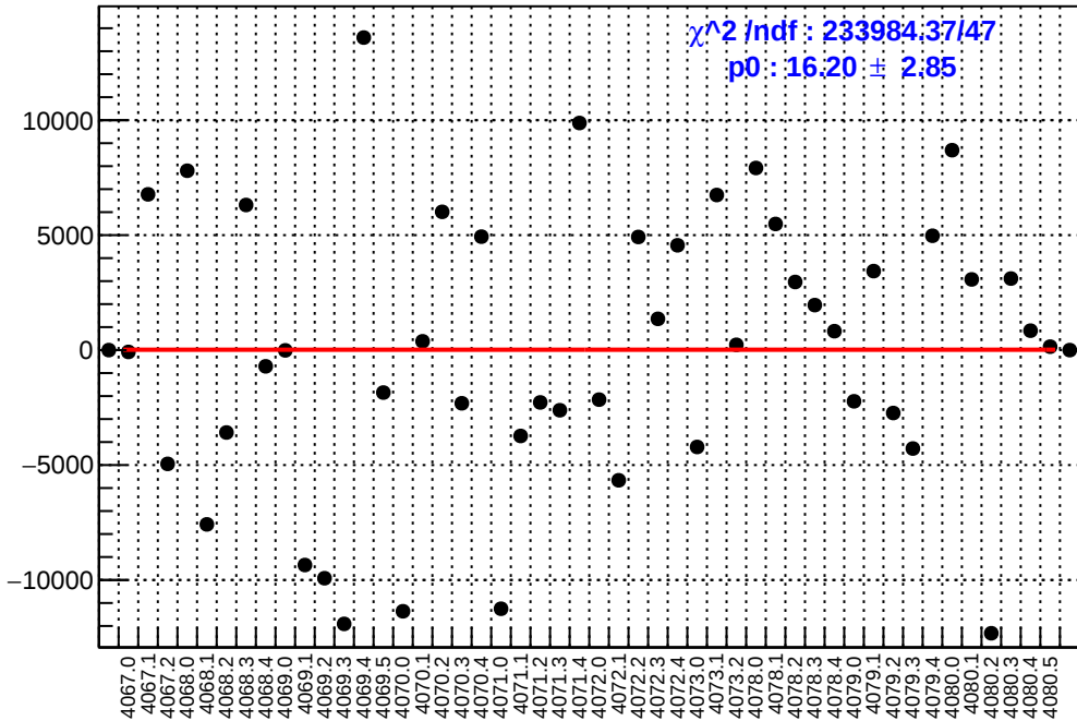
slug43: asym_dsl.mean/ppb-reg_asym_dsl.mean/ppb
