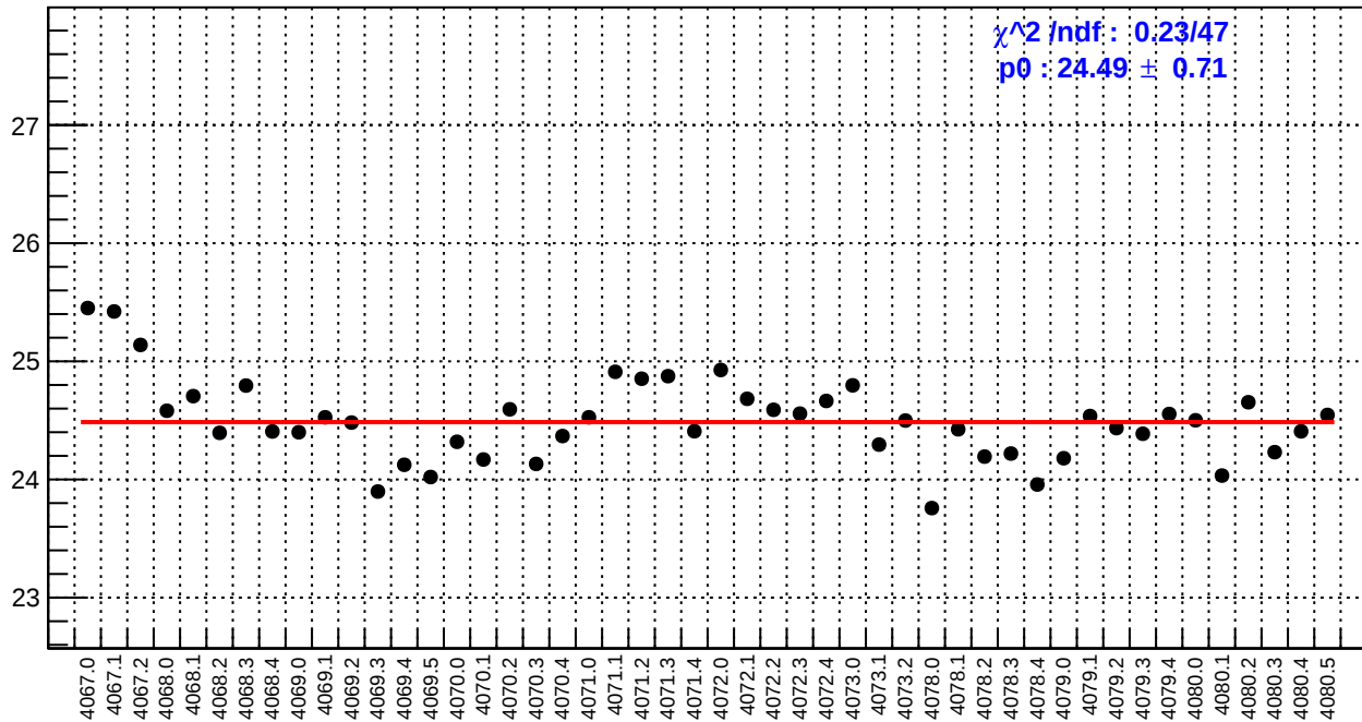
slug43: right_avg_bpm4eX/(ppb/nm)
