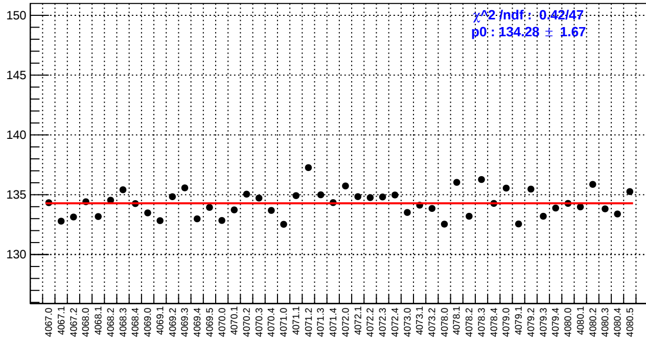
slug43: reg_asym_left_avg.rms/ppm
