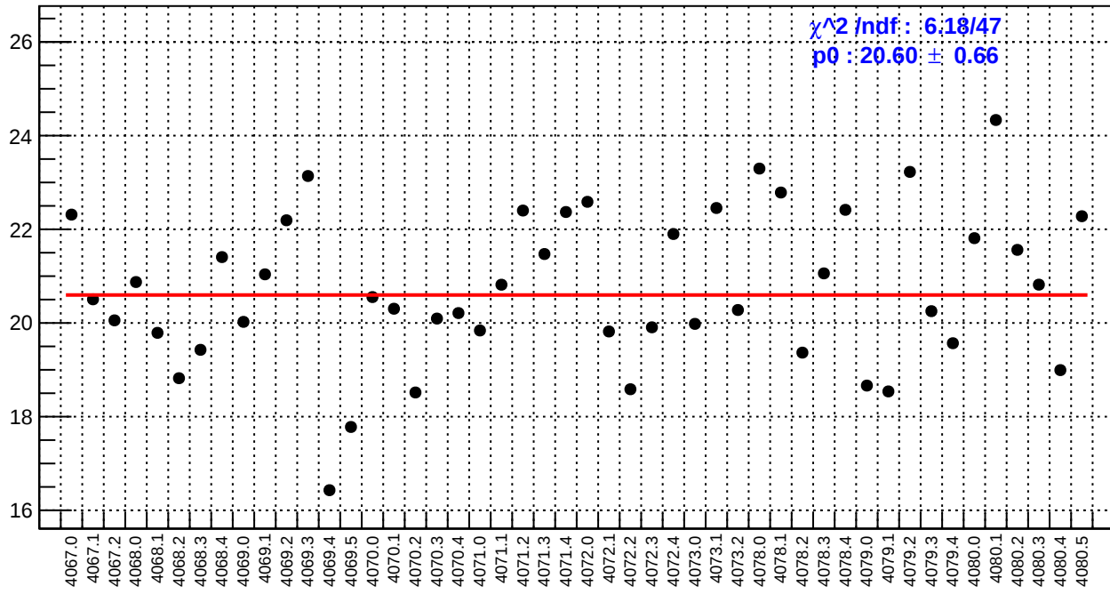
slug43: left_avg_bpm4aX/(ppb/nm)
