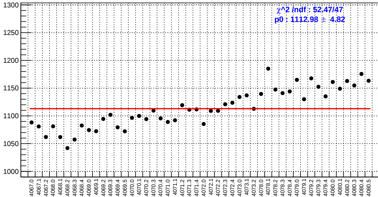
slug43: reg_asym_sam4.rms/ppm
