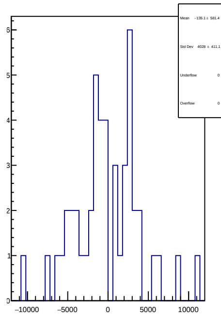
slug43: 1D Corr asym_dsr.mean/ppb-reg_asym_dsr.mean/ppb
