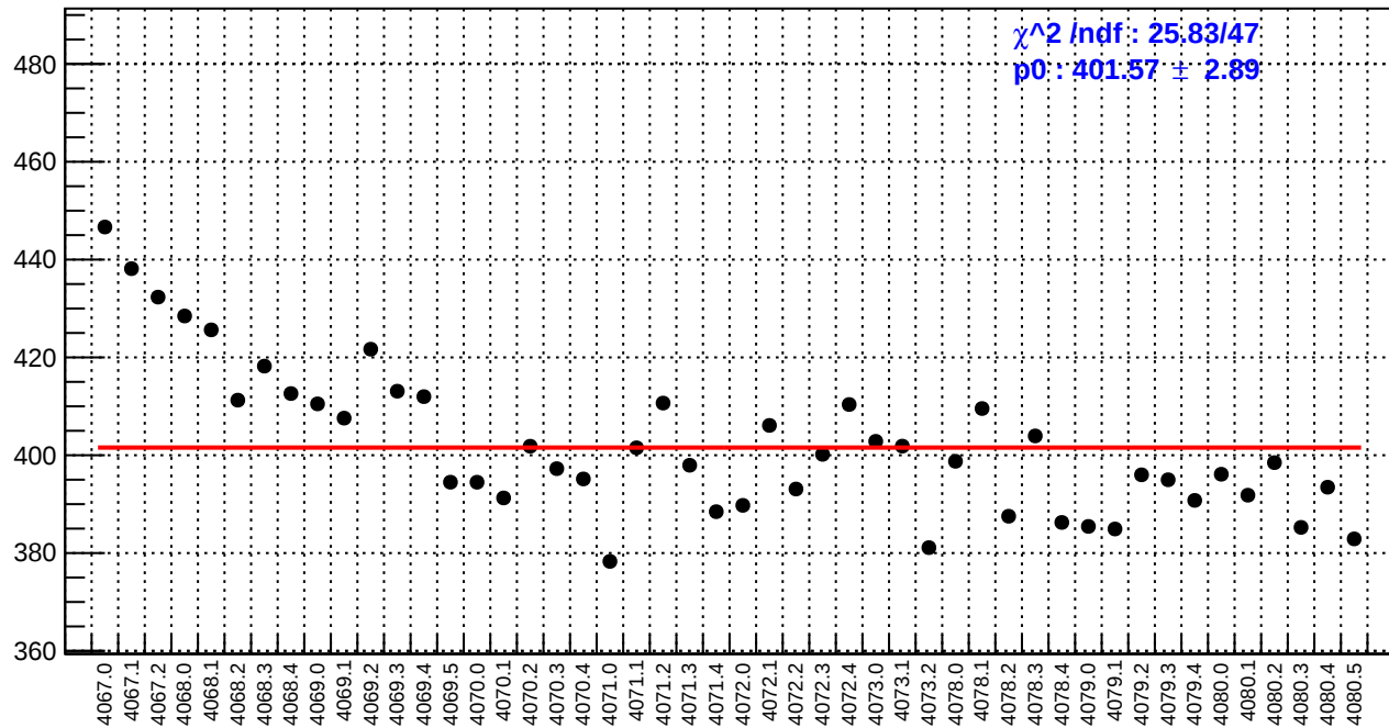
slug43: reg_asym_sam1.rms/ppm
