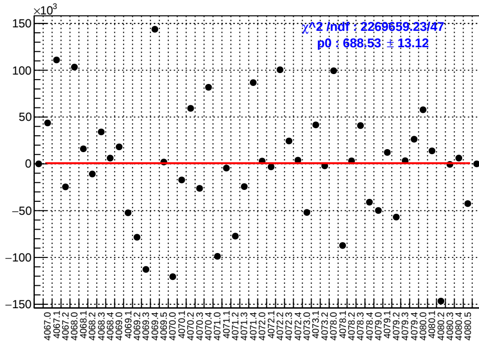
slug43: asym_sam2.mean/ppb-reg_asym_sam2.mean/ppb
