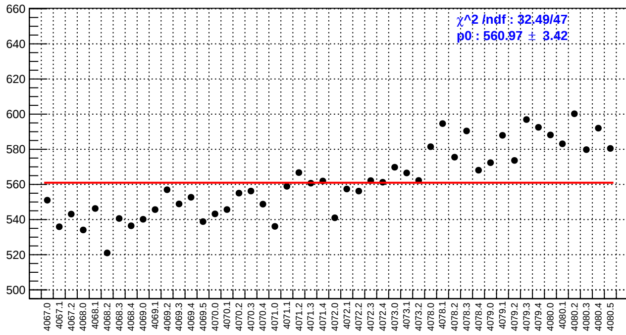
slug43: reg_asym_sam6.rms/ppm
