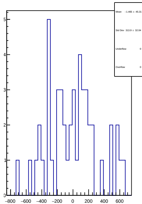
slug43: 1D Corr asym_right_dd.mean/ppb-reg_asym_right_dd.mean/ppb
