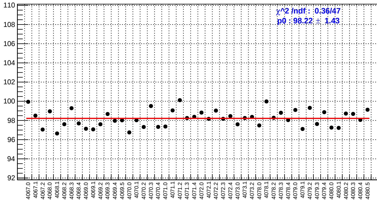
slug43: reg_asym_ds_avg.rms/ppm
