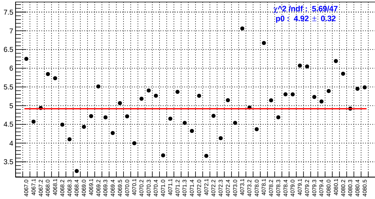
slug43: left_avg_bpm4aY/(ppb/nm)
