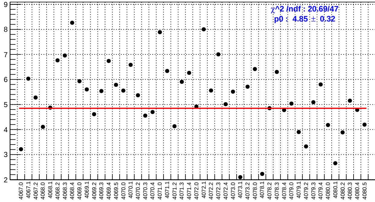
slug43: left_avg_bpm4eY/(ppb/nm)
