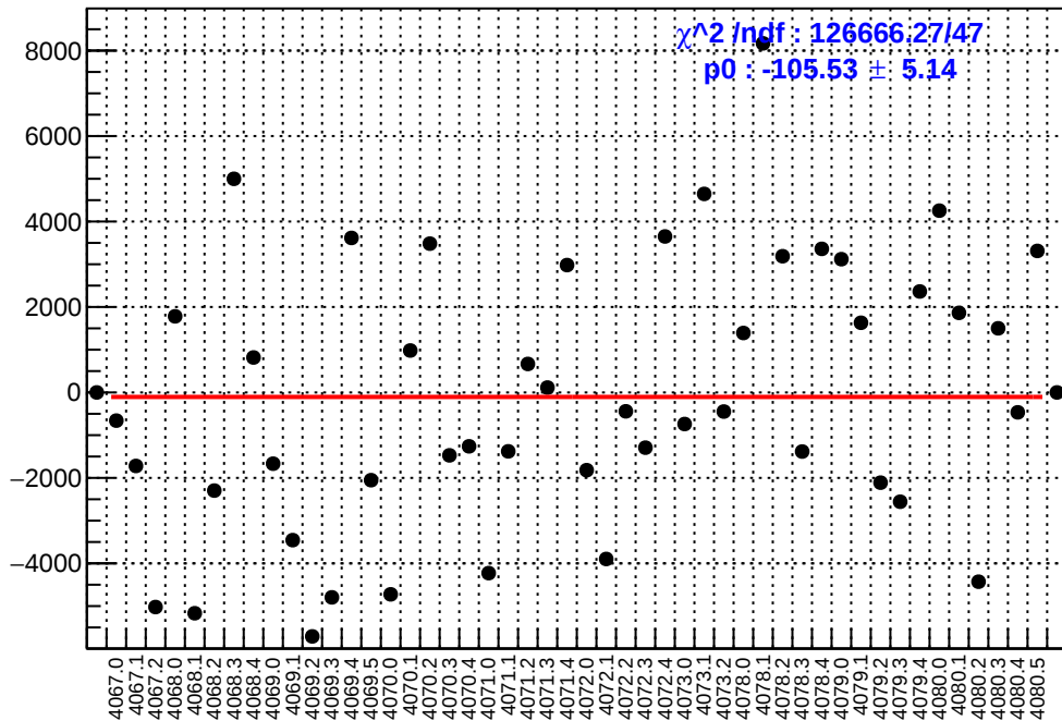
slug43: asym_ds_avg.mean/ppb-reg_asym_ds_avg.mean/ppb
