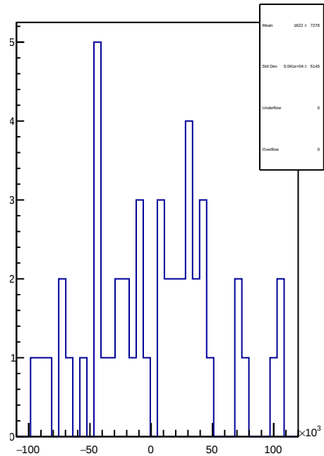
slug43: 1D Corr asym_sam4.mean/ppb-reg_asym_sam4.mean/ppb
