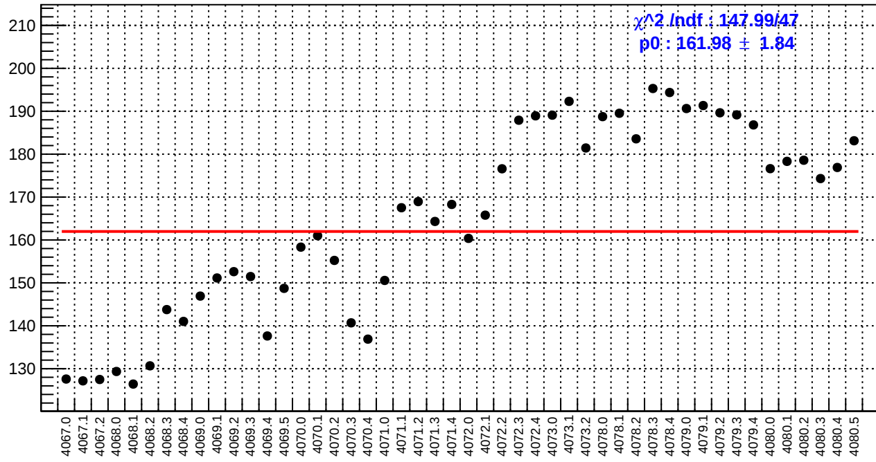
slug43: asym_bcm_an_us.rms/ppm
