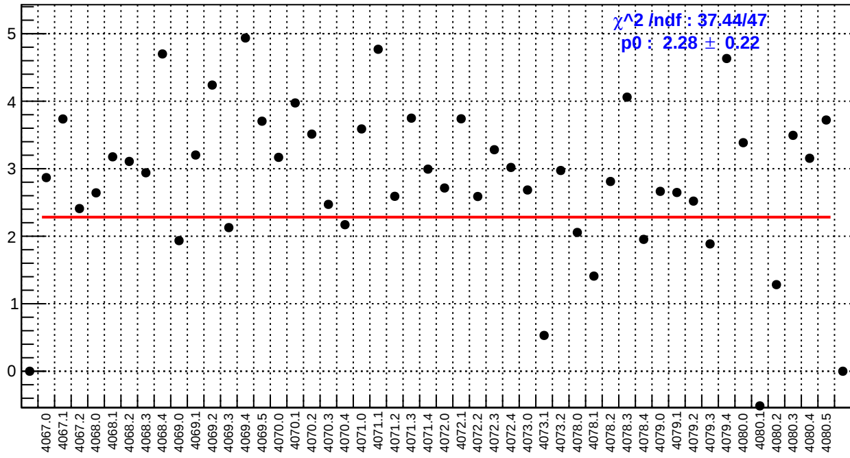
slug43: ds_avg_bpm4eY/(ppb/nm)
