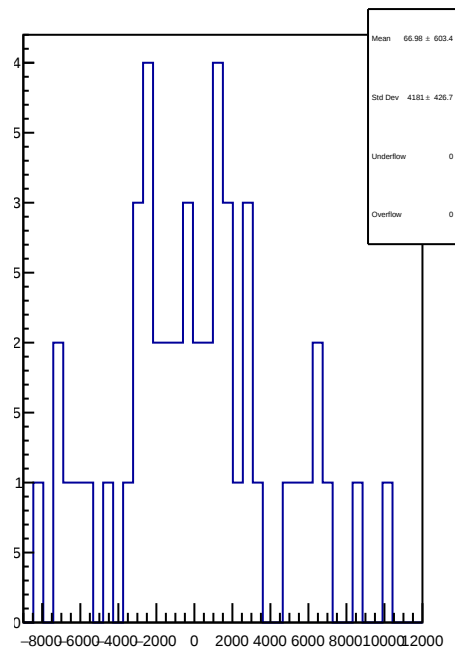
slug43: 1D Corr asym_us_dd.mean/ppb-reg_asym_us_dd.mean/ppb
