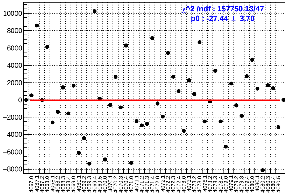
slug43: asym_us_dd.mean/ppb-reg_asym_us_dd.mean/ppb
