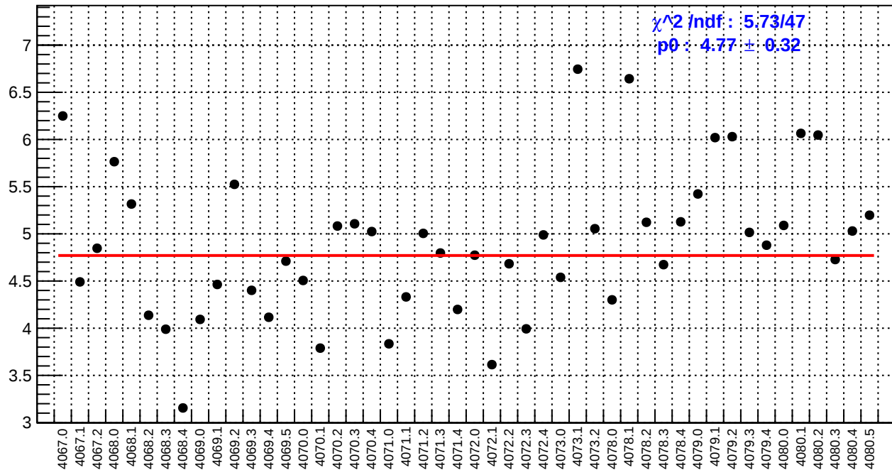
slug43: dsl_bpm4aY/(ppb/nm)
