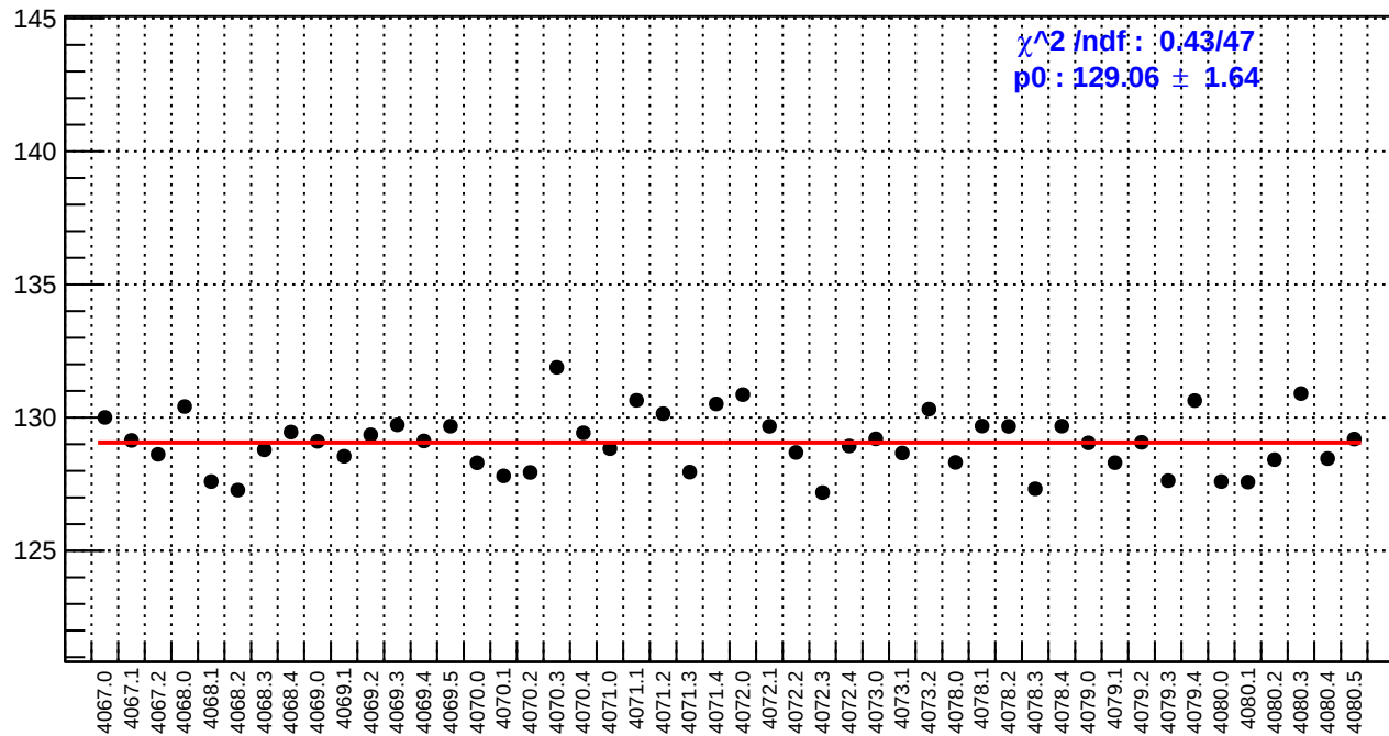
slug43: reg_asym_usr.rms/ppm
