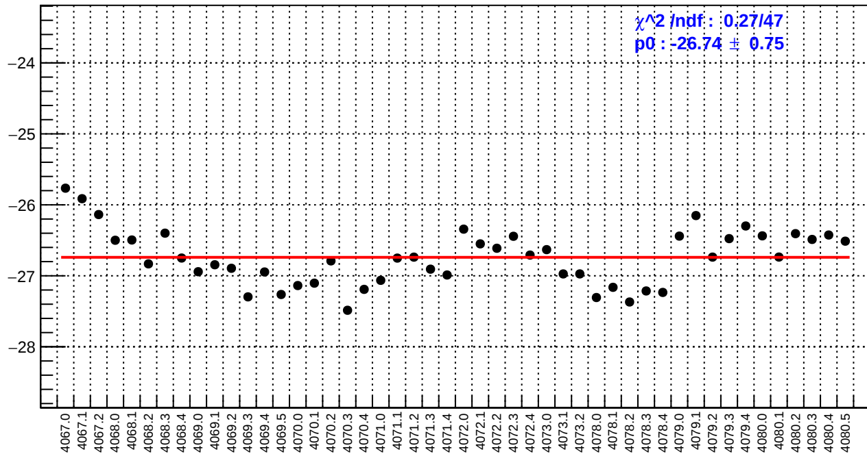
slug43: ds_avg_bpm4eX/(ppb/nm)
