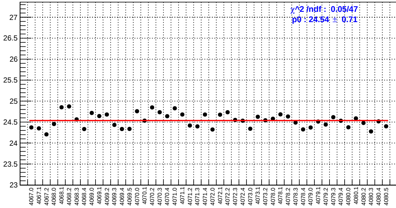
slug43: reg_asym_left_dd.rms/ppm
