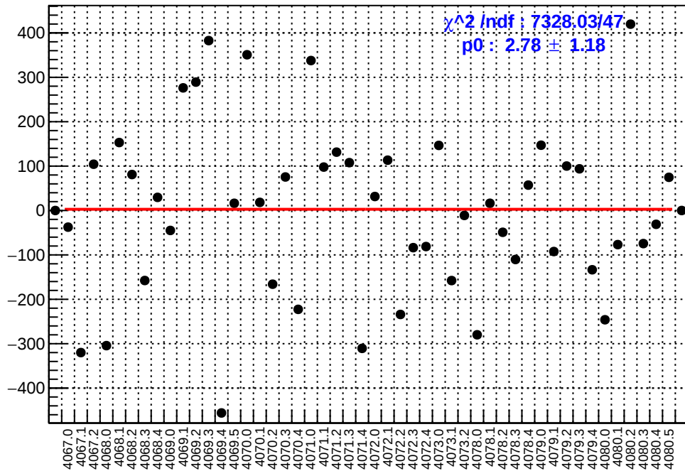
slug43: asym_left_dd.mean/ppb-reg_asym_left_dd.mean/ppb
