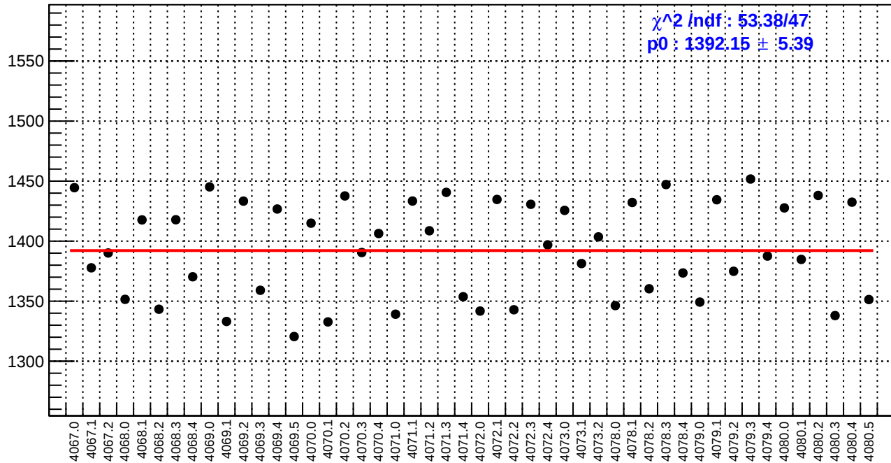
slug43: diff_bpm4aX.rms/nm
