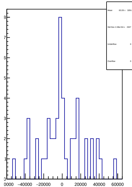
slug43: 1D Corr asym_sam6.mean/ppb-reg_asym_sam6.mean/ppb
