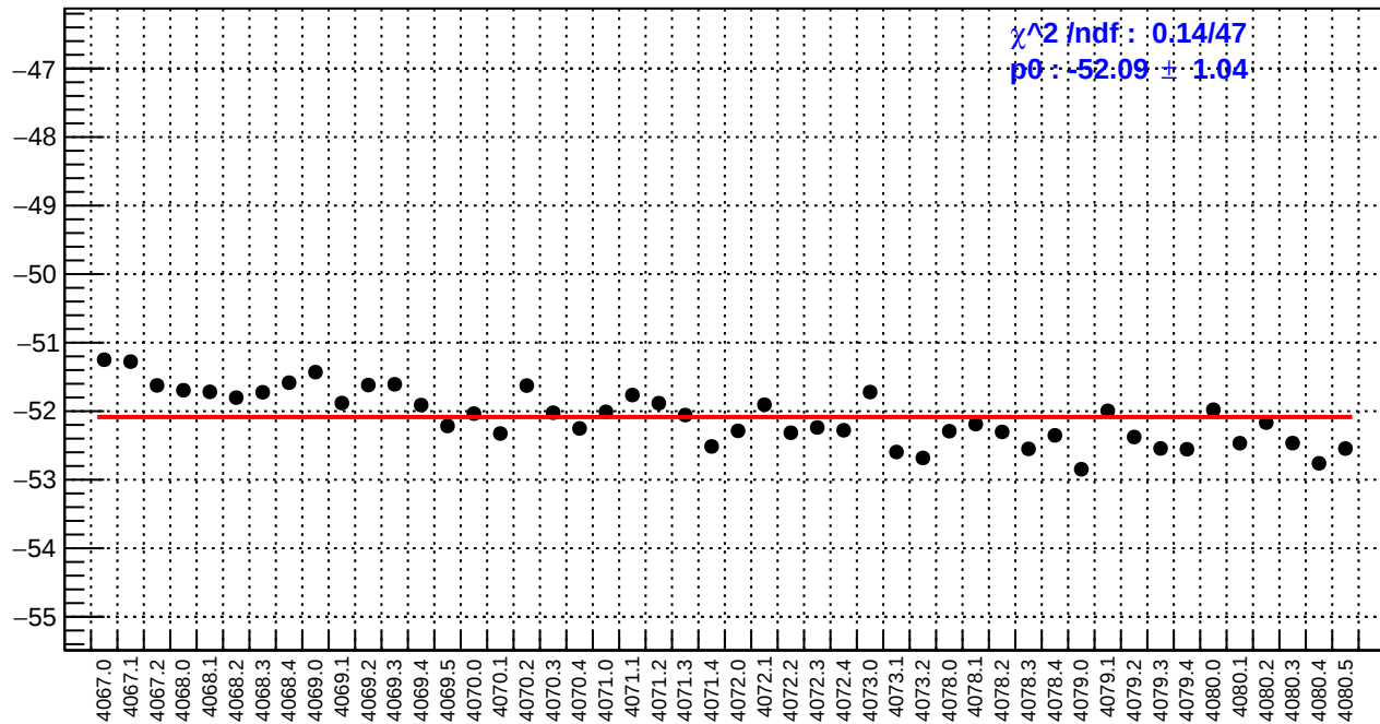
slug43: us_avg_bpm12X/(ppb/nm)
