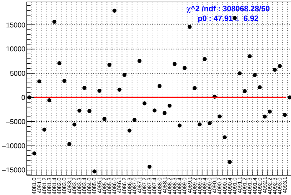
slug44: asym_usl.mean/ppb-reg_asym_usl.mean/ppb
