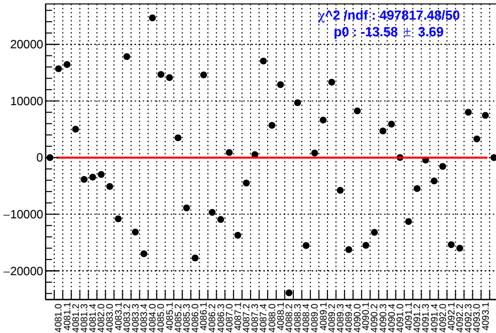
slug44: asym_sam1.mean/ppb-reg_asym_sam1.mean/ppb
