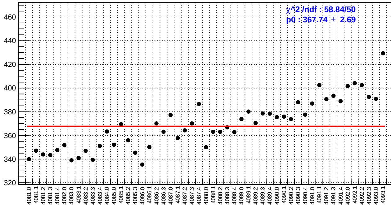
slug44: reg_asym_sam5.rms/ppm
