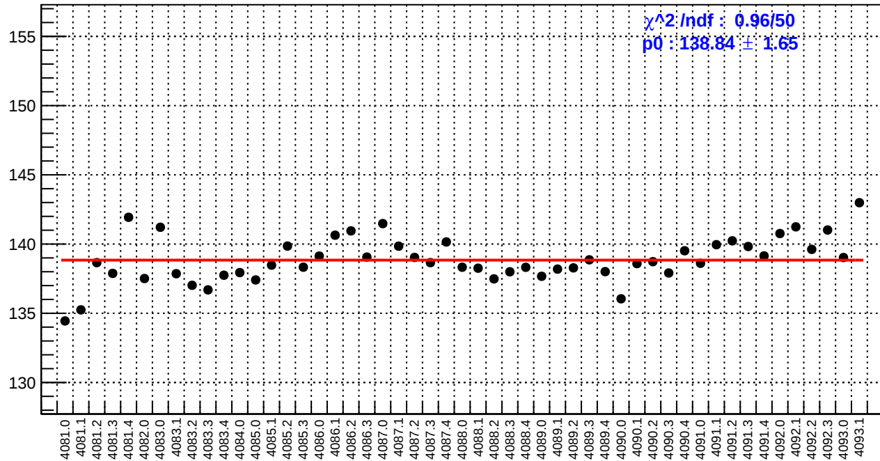
slug44: reg_asym_dsl.rms/ppm
