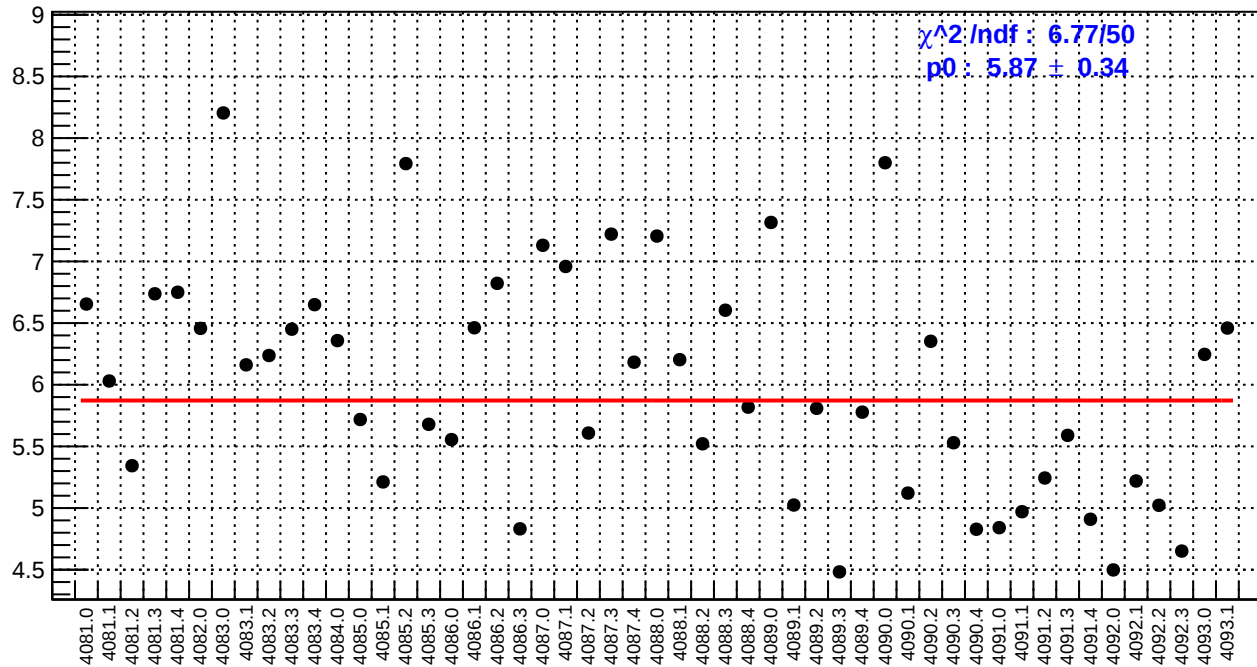
slug44: ds_avg_bpm4aY/(ppb/nm)
