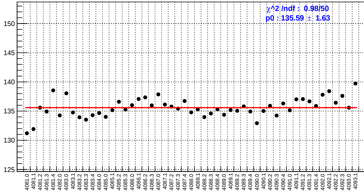
slug44: reg_asym_left_avg.rms/ppm
