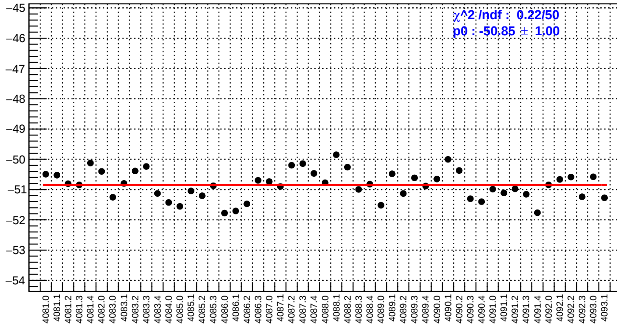
slug44: left_avg_bpm12X/(ppb/nm)
