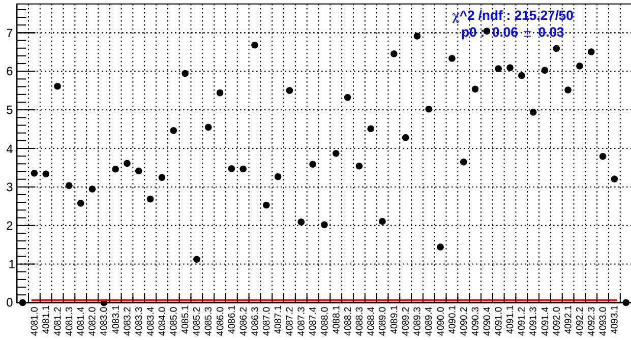
slug44: ds_avg_bpm4eY/(ppb/nm)
