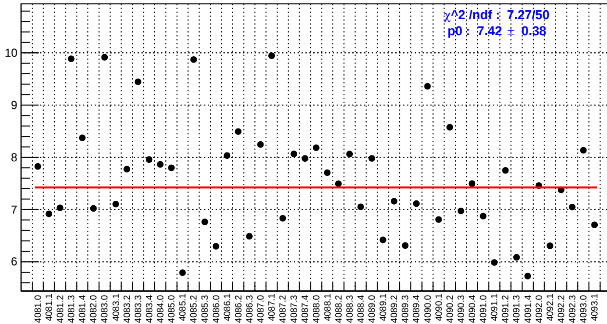
slug44: right_avg_bpm4aY/(ppb/nm)
