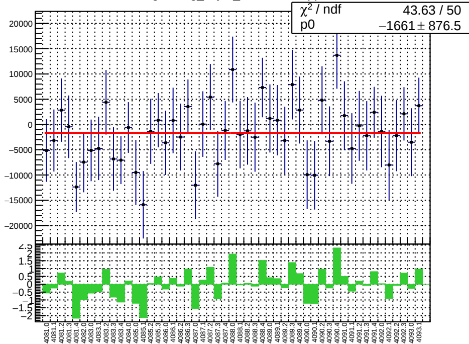
slug44: reg_asym_sam6.mean/ppb
