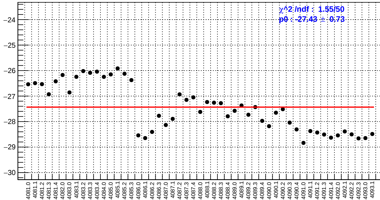
slug44: ds_avg_bpm4eX/(ppb/nm)
