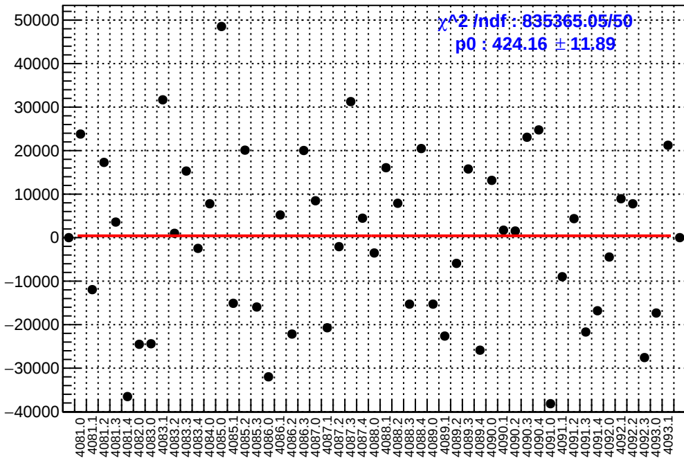
slug44: asym_sam7.mean/ppb-reg_asym_sam7.mean/ppb
