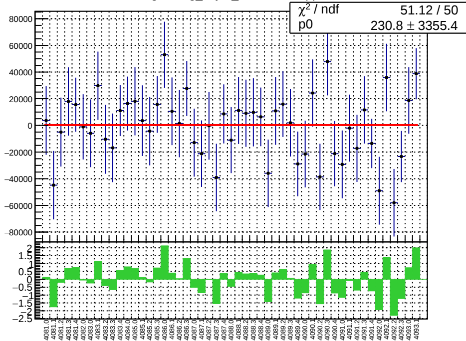
slug44: reg_asym_sam2.mean/ppb
