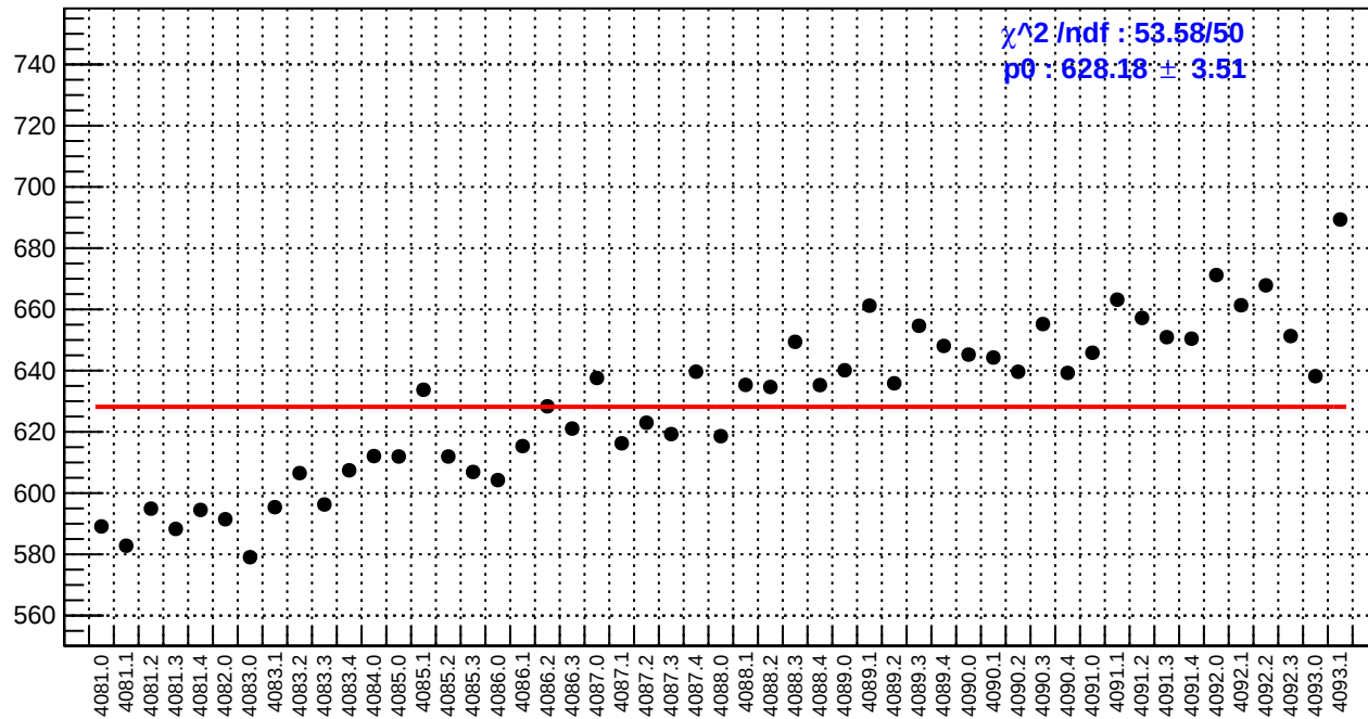
slug44: reg_asym_sam6.rms/ppm
