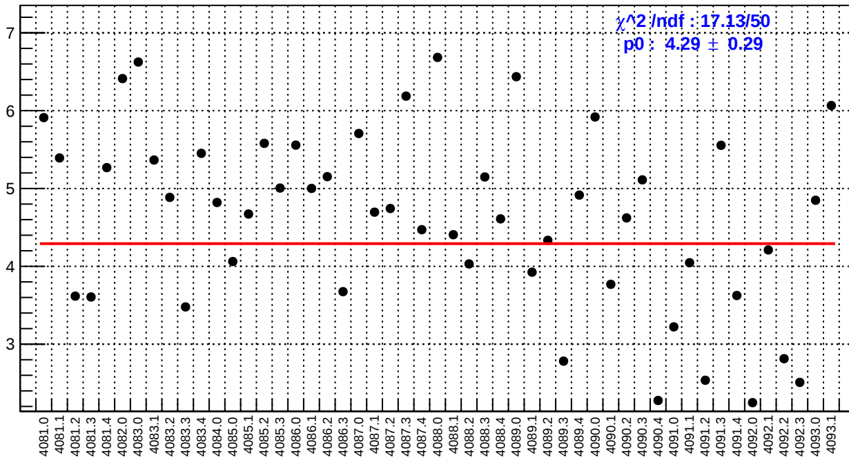
slug44: usl_bpm4aY/(ppb/nm)
