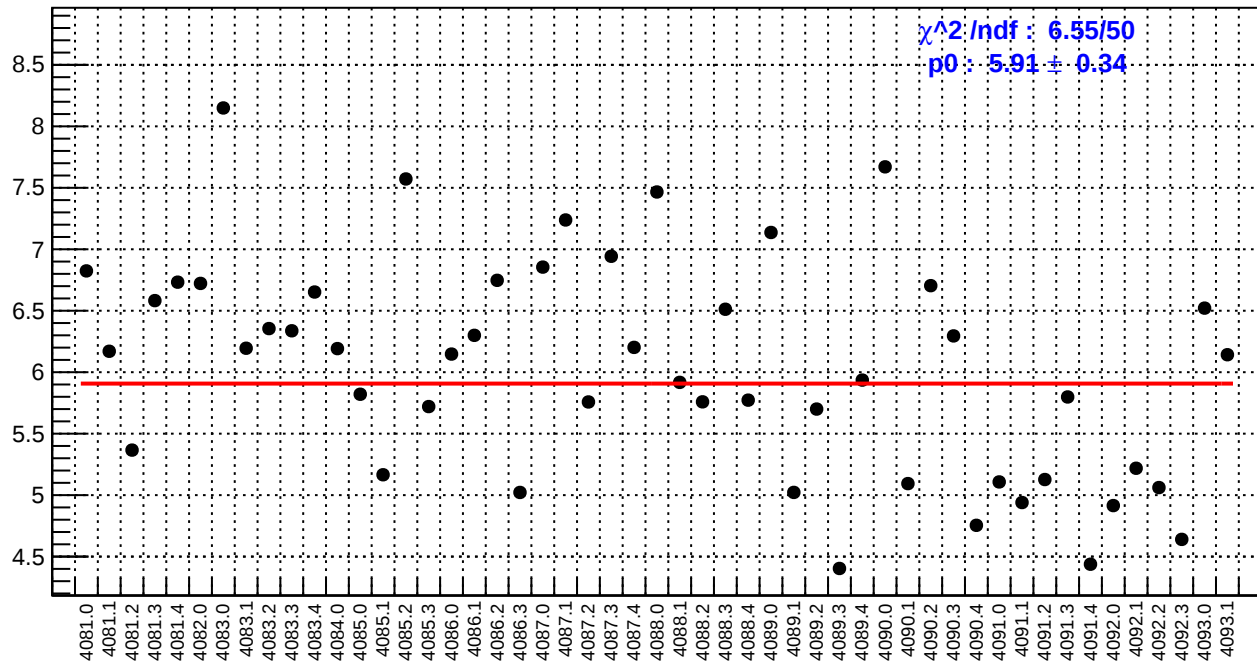
slug44: us_avg_bpm4aY/(ppb/nm)
