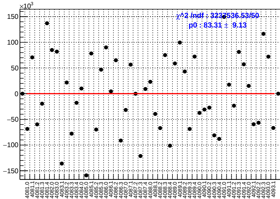
slug44: asym_sam2.mean/ppb-reg_asym_sam2.mean/ppb
