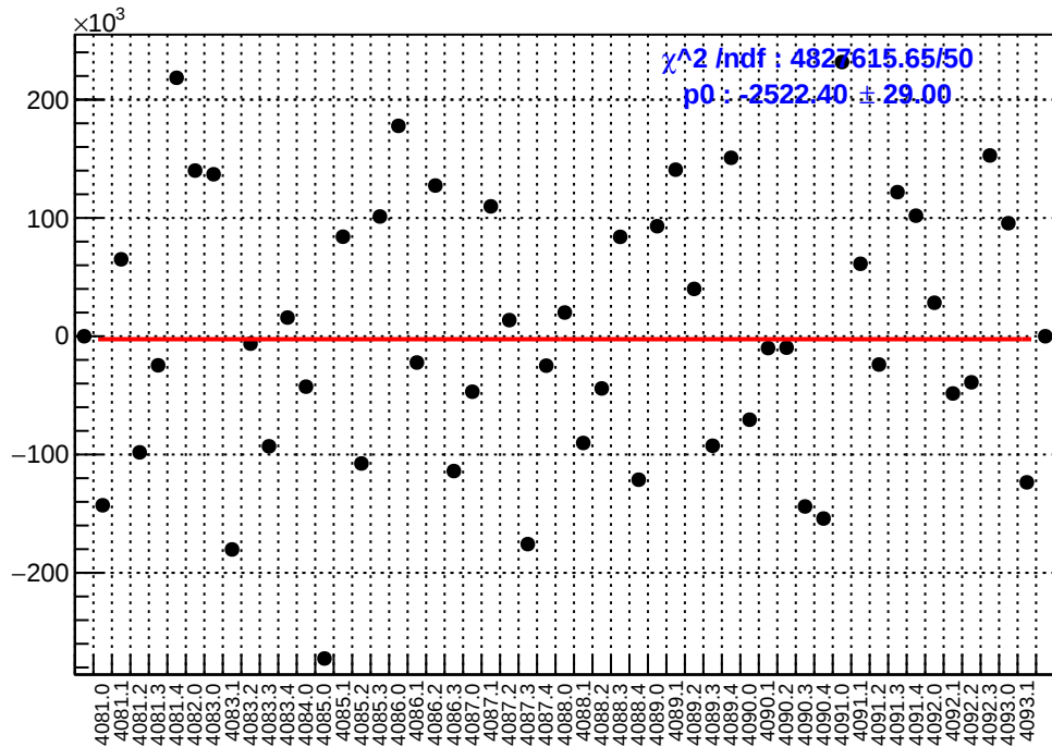
slug44: asym_sam3.mean/ppb-reg_asym_sam3.mean/ppb
