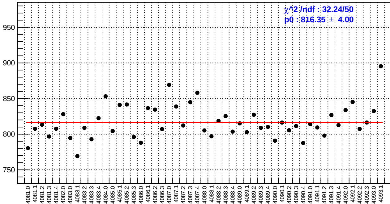
slug44: reg_asym_sam3.rms/ppm
