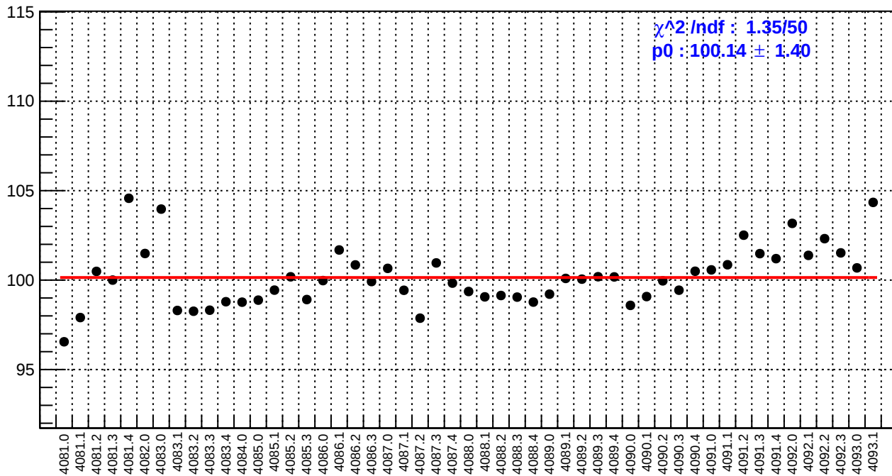
slug44: reg_asym_ds_avg.rms/ppm
