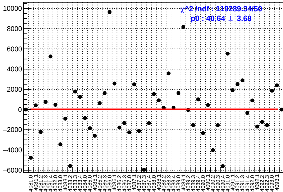
slug44: asym_us_avg.mean/ppb-reg_asym_us_avg.mean/ppb
