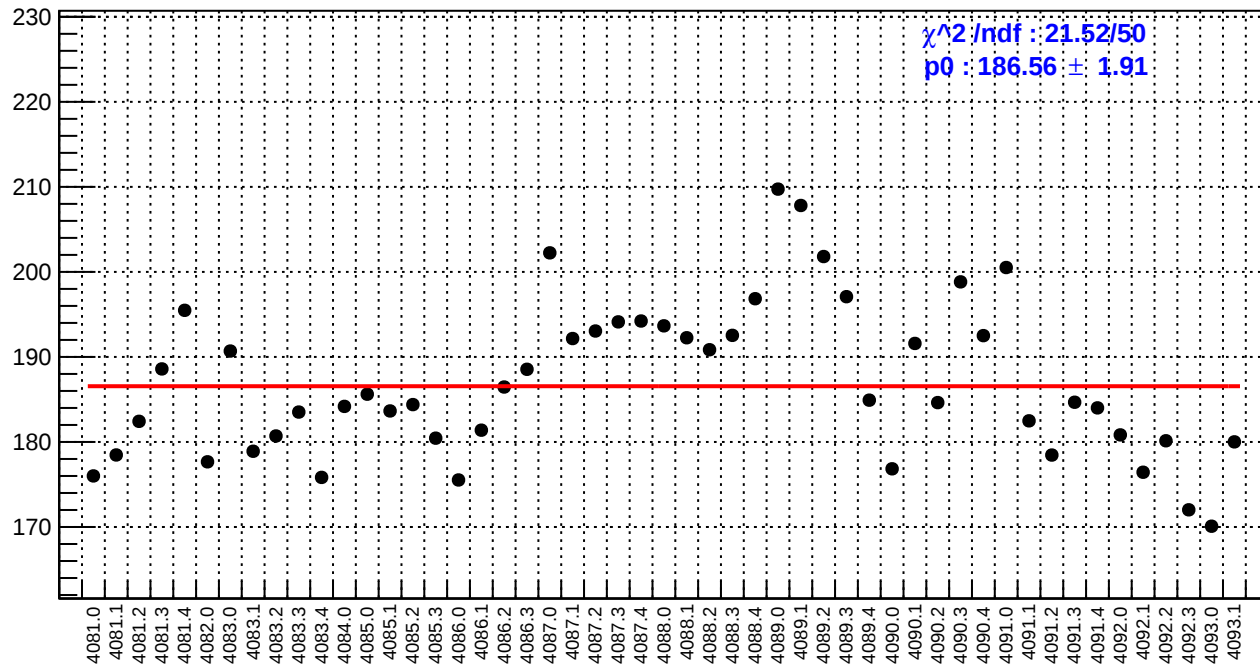
slug44: asym_bcm_an_ds.rms/ppm
