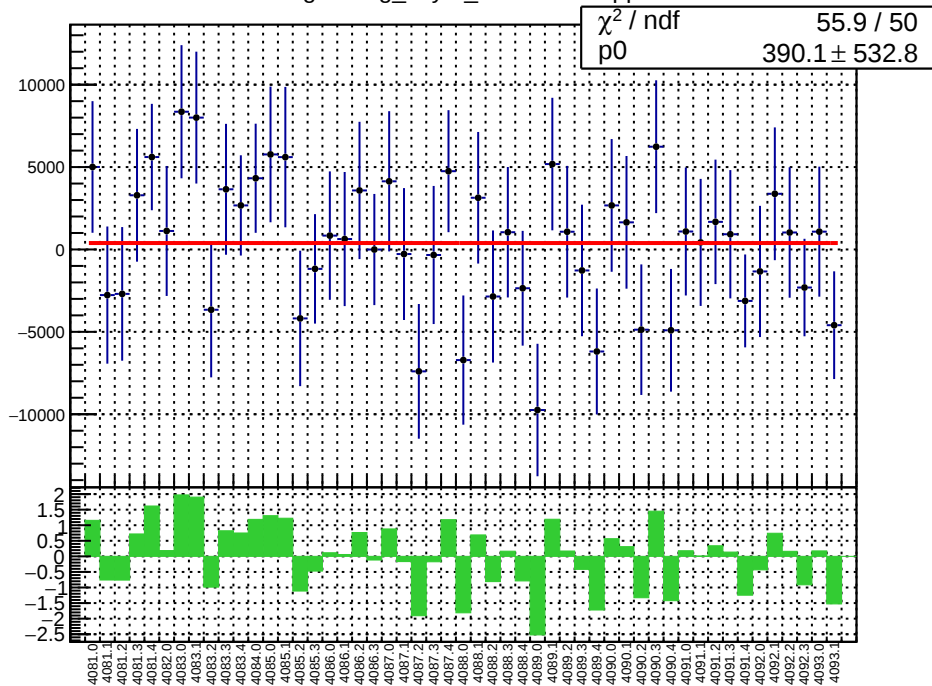
slug44: reg_asym_sam1.mean/ppb
