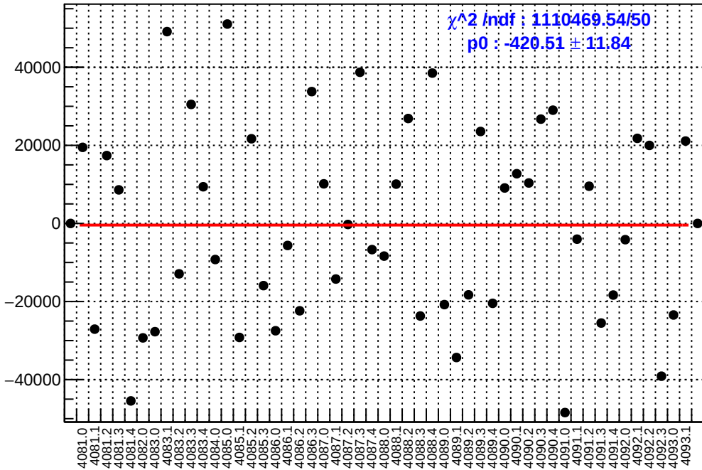
slug44: asym_sam6.mean/ppb-reg_asym_sam6.mean/ppb
