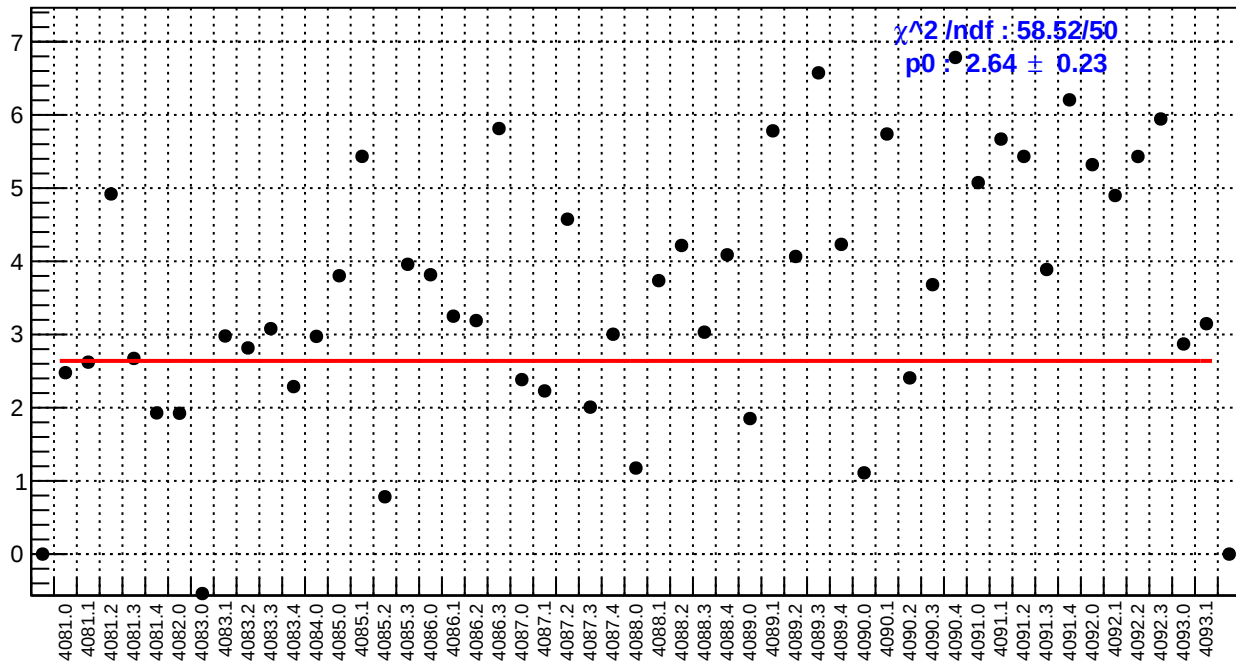
slug44: us_avg_bpm4eY/(ppb/nm)
