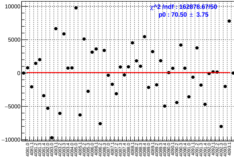
slug44: asym_dsr.mean/ppb-reg_asym_dsr.mean/ppb
