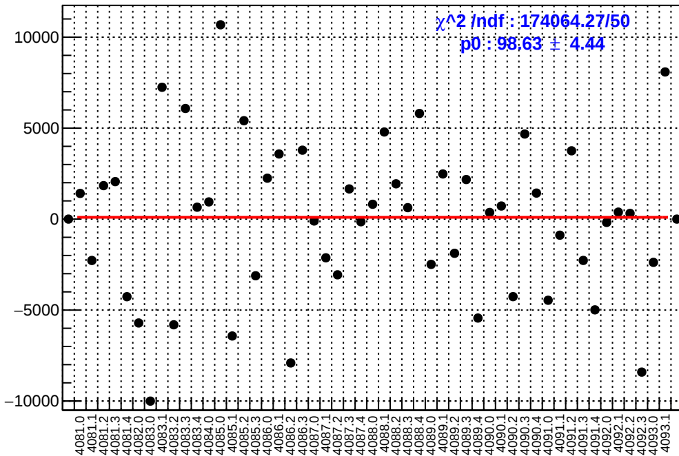
slug44: asym_right_avg.mean/ppb-reg_asym_right_avg.mean/ppb
