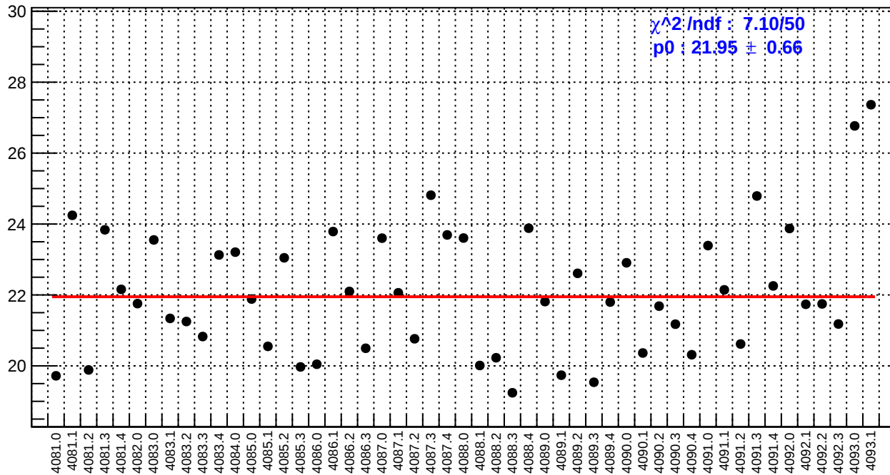
slug44: left_avg_bpm4aX/(ppb/nm)
