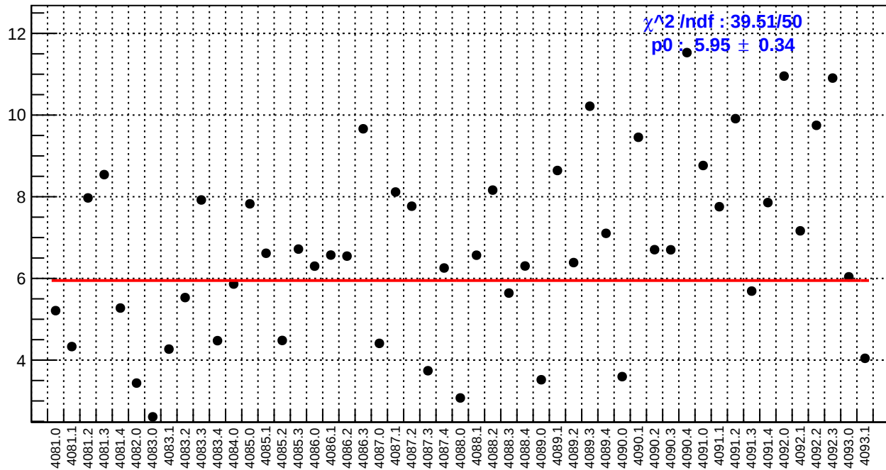
slug44: dsl_bpm4eY/(ppb/nm)
