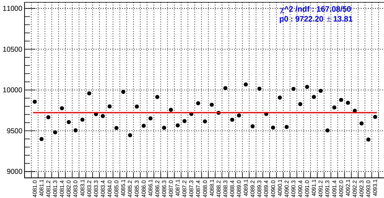
slug44: diff_bpm4eX.rms/nm
