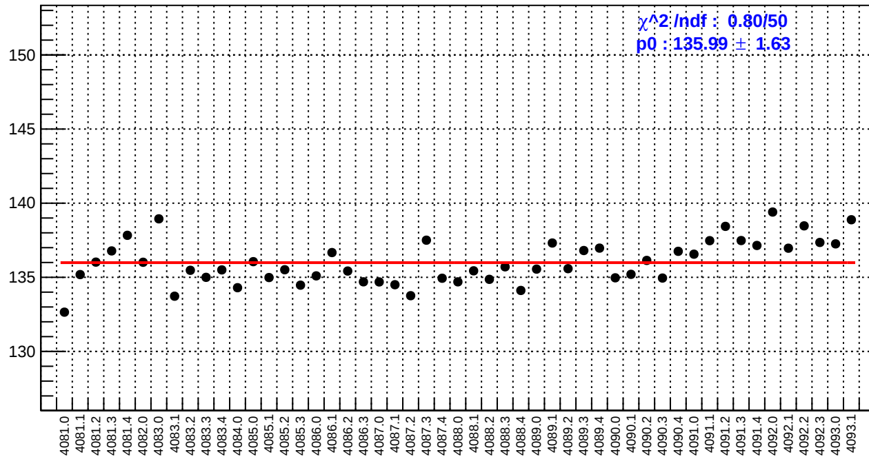
slug44: reg_asym_dsr.rms/ppm
