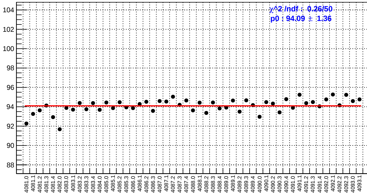
slug44: reg_asym_ds_dd.rms/ppm
