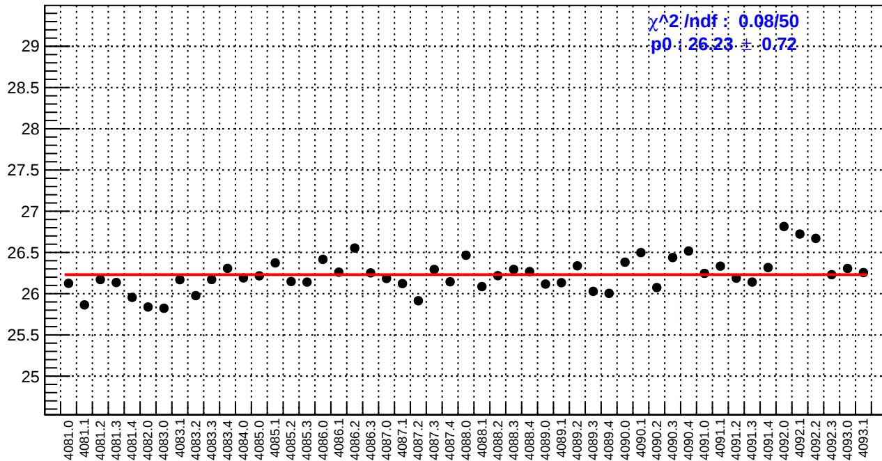
slug44: reg_asym_right_dd.rms/ppm
