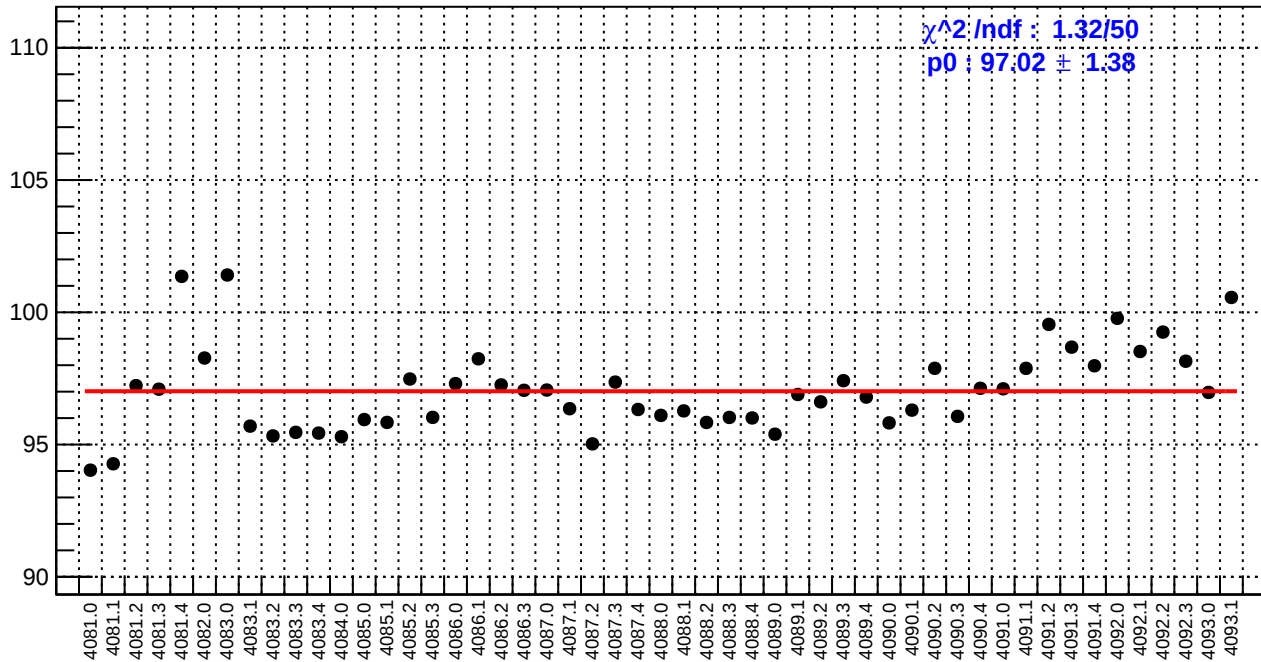
slug44: reg_asym_us_avg.rms/ppm
