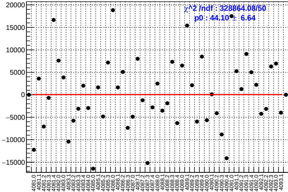
slug44: asym_dsl.mean/ppb-reg_asym_dsl.mean/ppb
