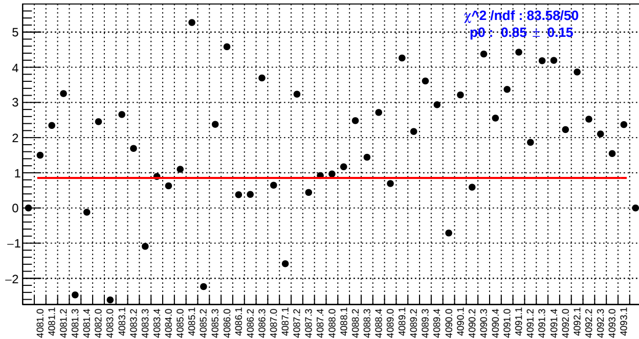
slug44: dsr_bpm4eY/(ppb/nm)
