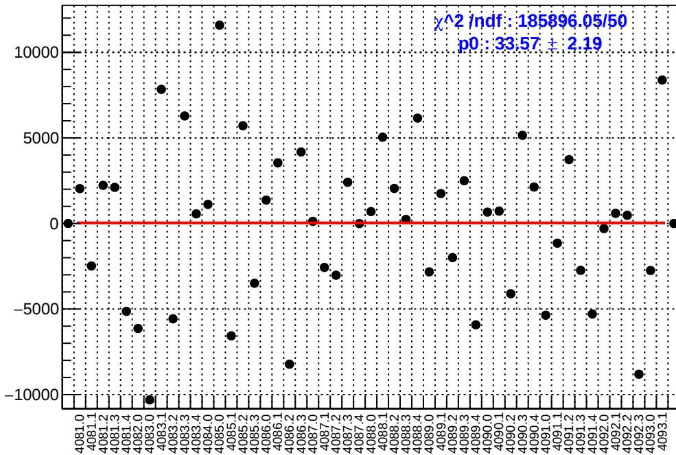
slug44: asym_usr.mean/ppb-reg_asym_usr.mean/ppb
