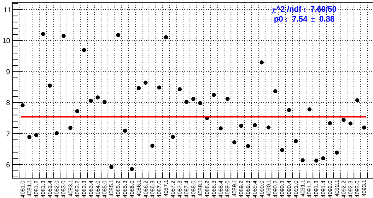
slug44: dsr_bpm4aY/(ppb/nm)
