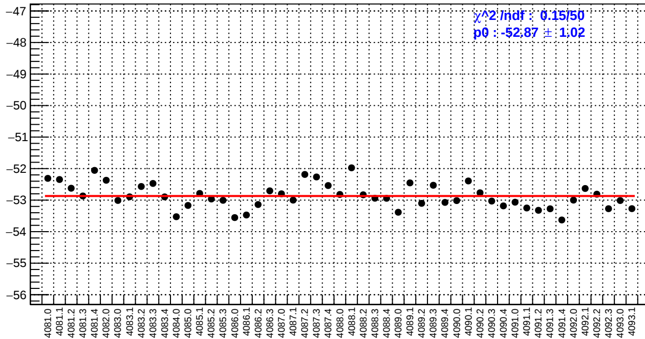
slug44: us_avg_bpm12X/(ppb/nm)
