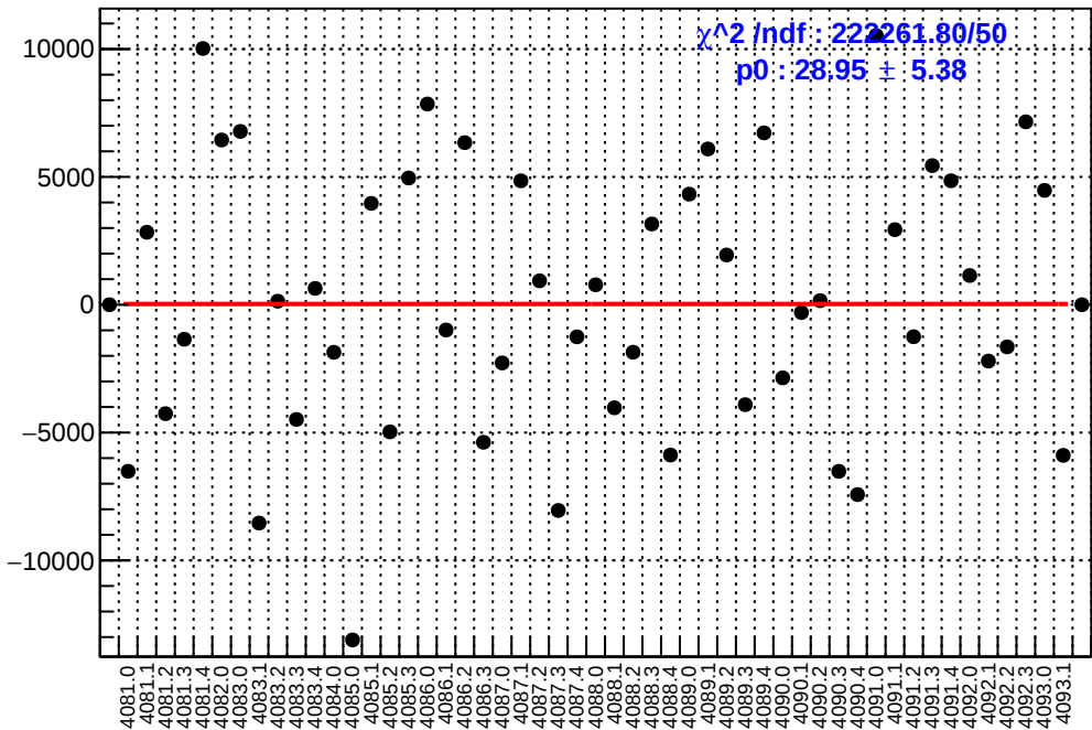
slug44: asym_ds_dd.mean/ppb-reg_asym_ds_dd.mean/ppb
