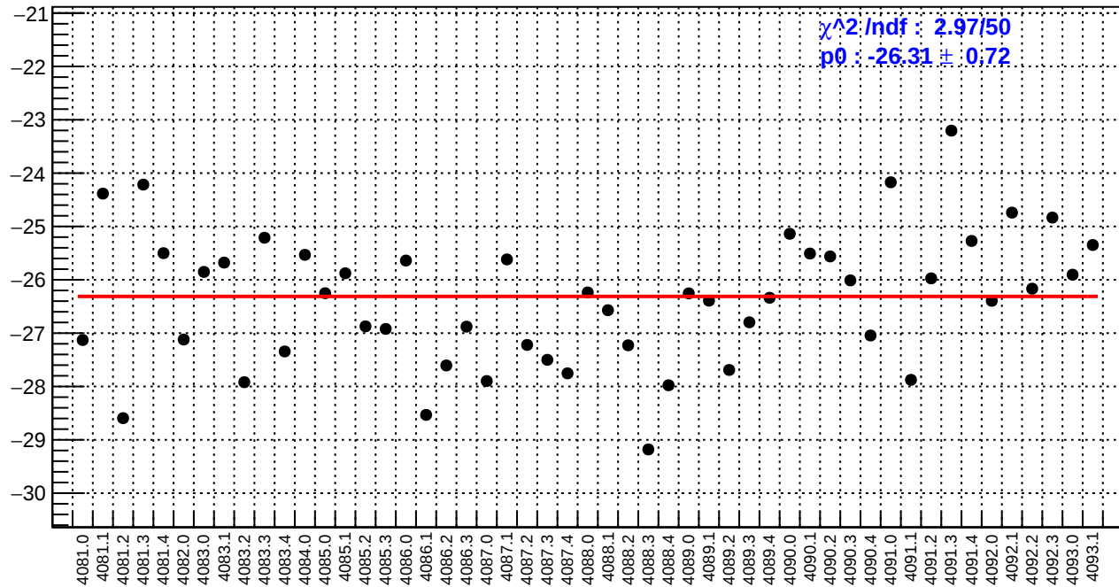
slug44: dsr_bpm4aX/(ppb/nm)
