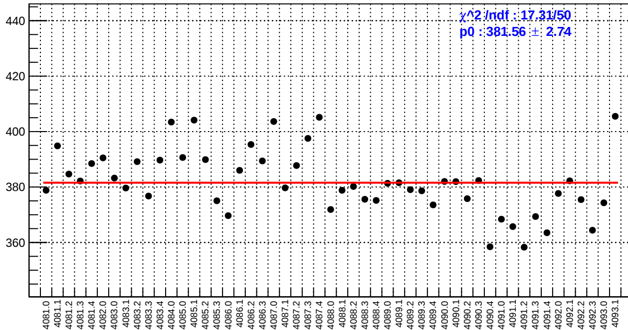
slug44: reg_asym_sam1.rms/ppm
