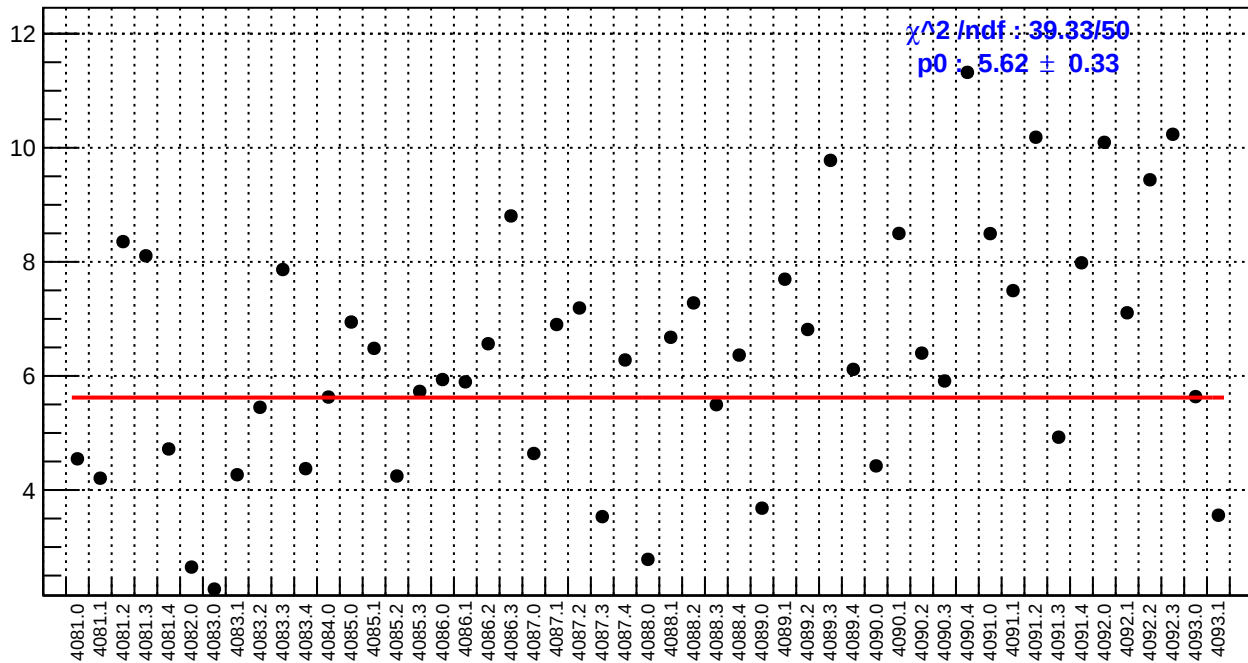
slug44: usl_bpm4eY/(ppb/nm)
