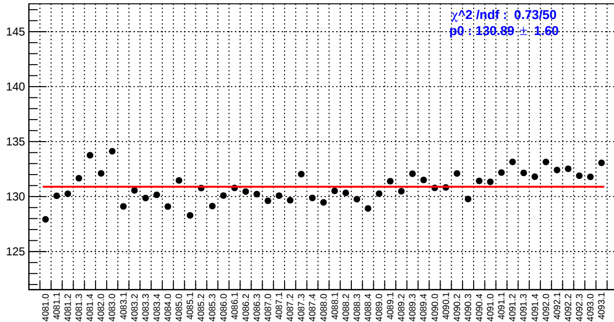
slug44: reg_asym_usr.rms/ppm
