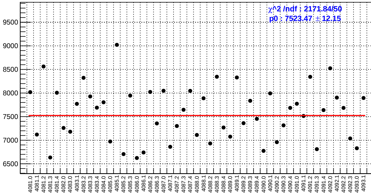
slug44: diff_bpm4aY.rms/nm
