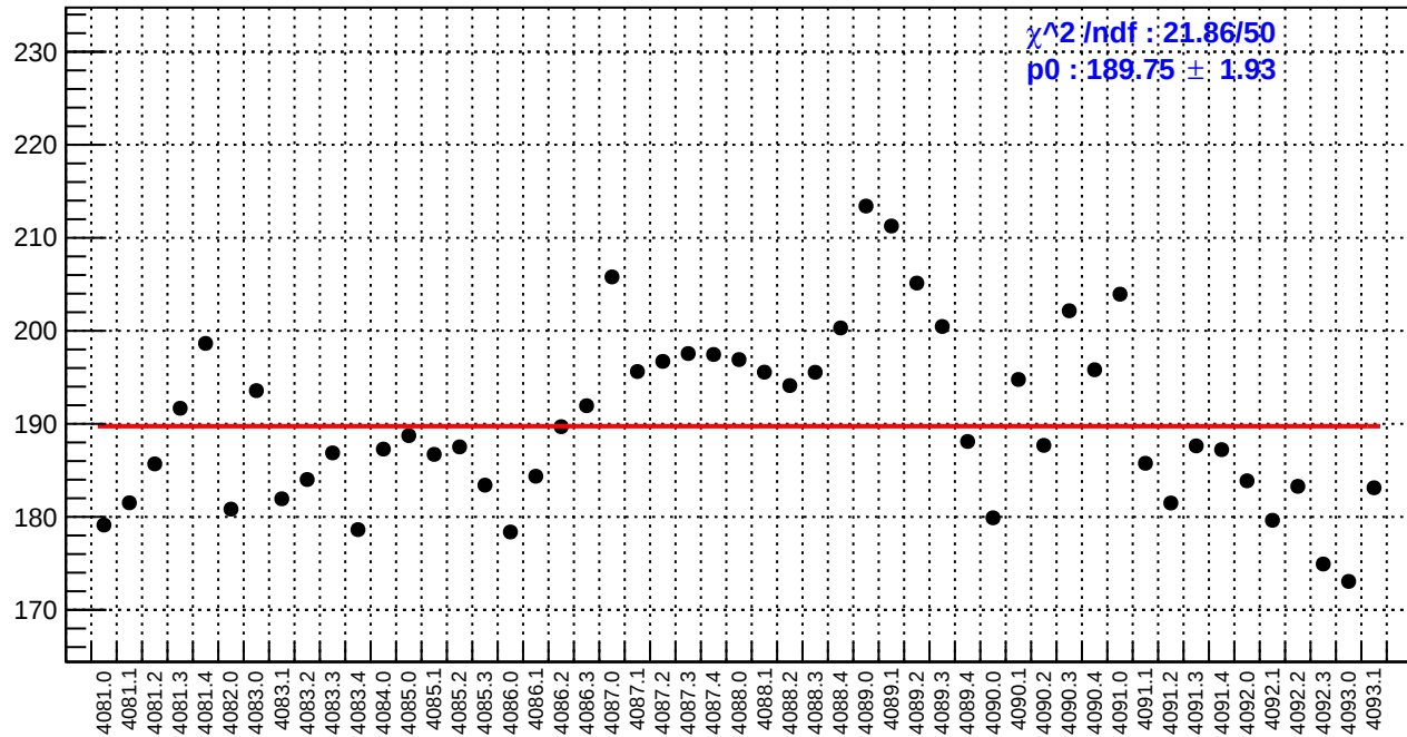
slug44: asym_bcm_an_ds3.rms/ppm
