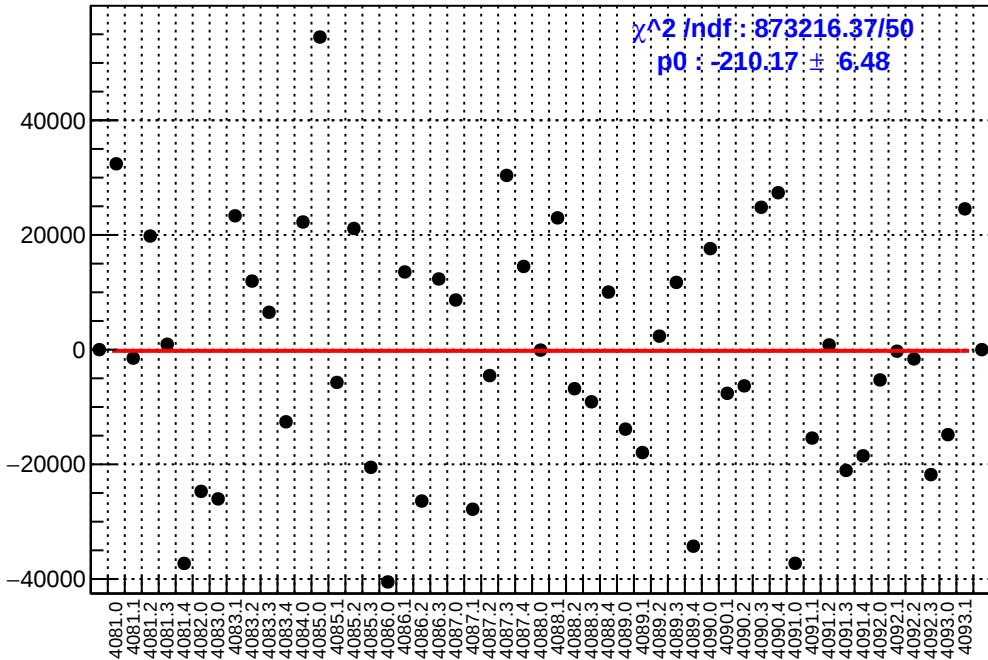
slug44: asym_sam8.mean/ppb-reg_asym_sam8.mean/ppb
