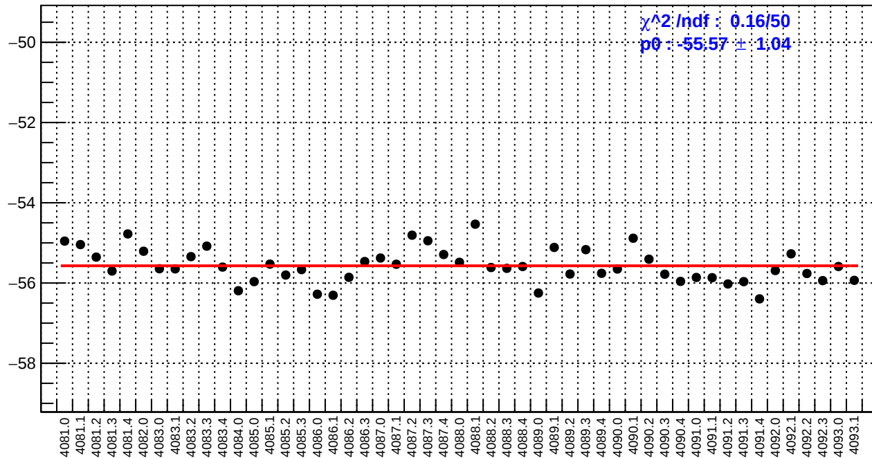
slug44: ds_avg_bpm12X/(ppb/nm)
