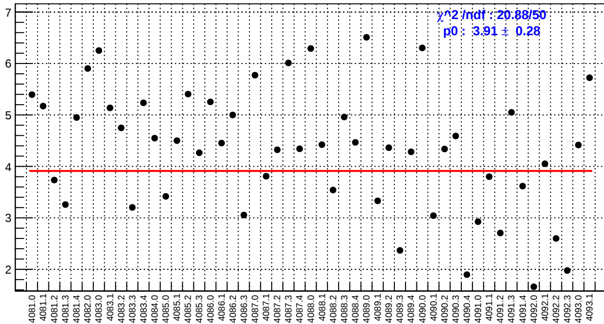
slug44: dsl_bpm4aY/(ppb/nm)
