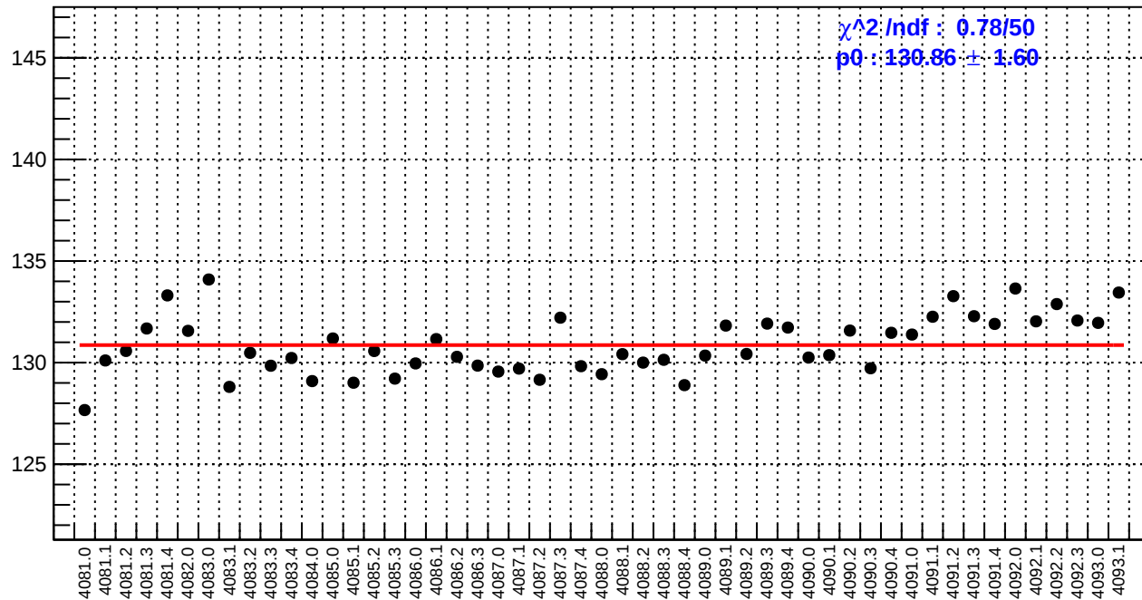
slug44: reg_asym_right_avg.rms/ppm
