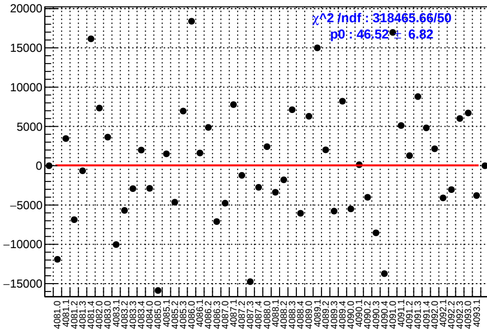
slug44: asym_left_avg.mean/ppb-reg_asym_left_avg.mean/ppb
