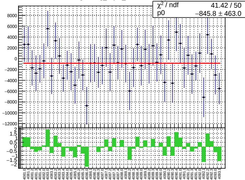
slug44: reg_asym_sam7.mean/ppb
