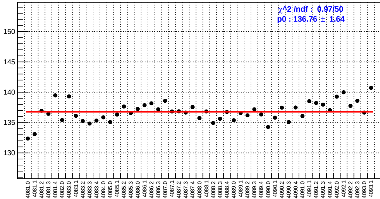
slug44: reg_asym_usl.rms/ppm
