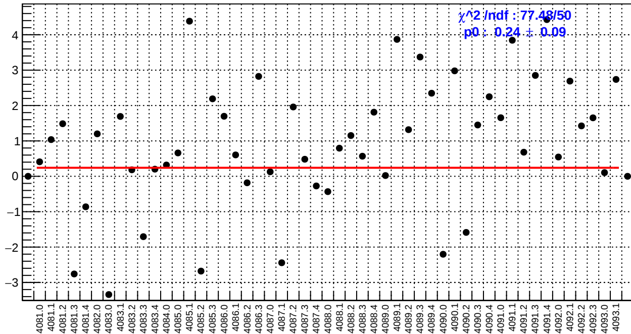
slug44: usr_bpm4eY/(ppb/nm)
