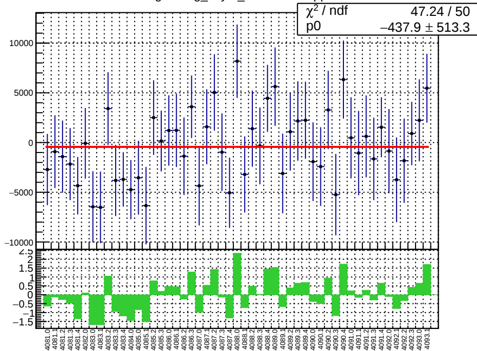
slug44: reg_asym_sam5.mean/ppb
