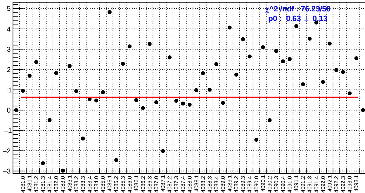
slug44: right_avg_bpm4eY/(ppb/nm)
