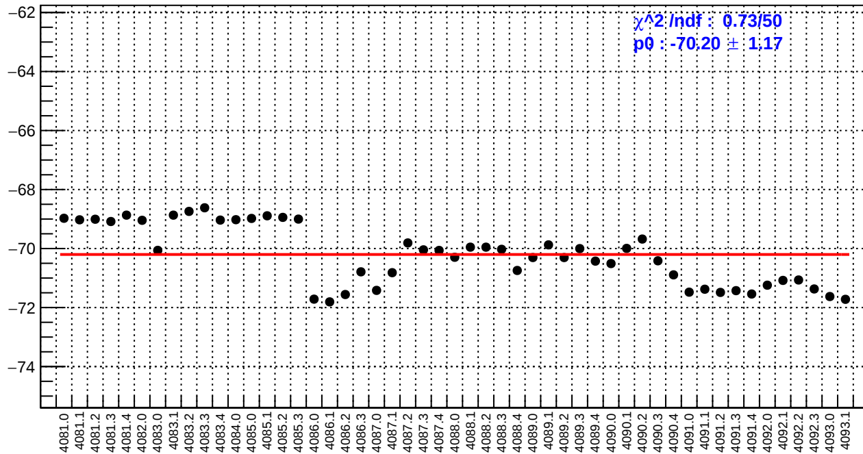
slug44: usl_bpm4eX/(ppb/nm)
