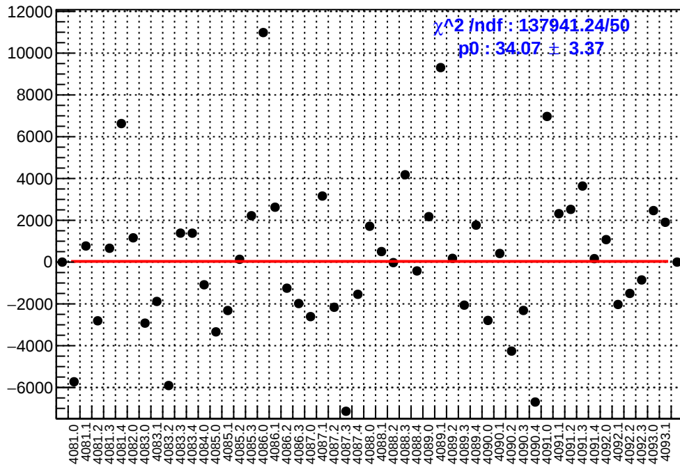
slug44: asym_ds_avg.mean/ppb-reg_asym_ds_avg.mean/ppb
