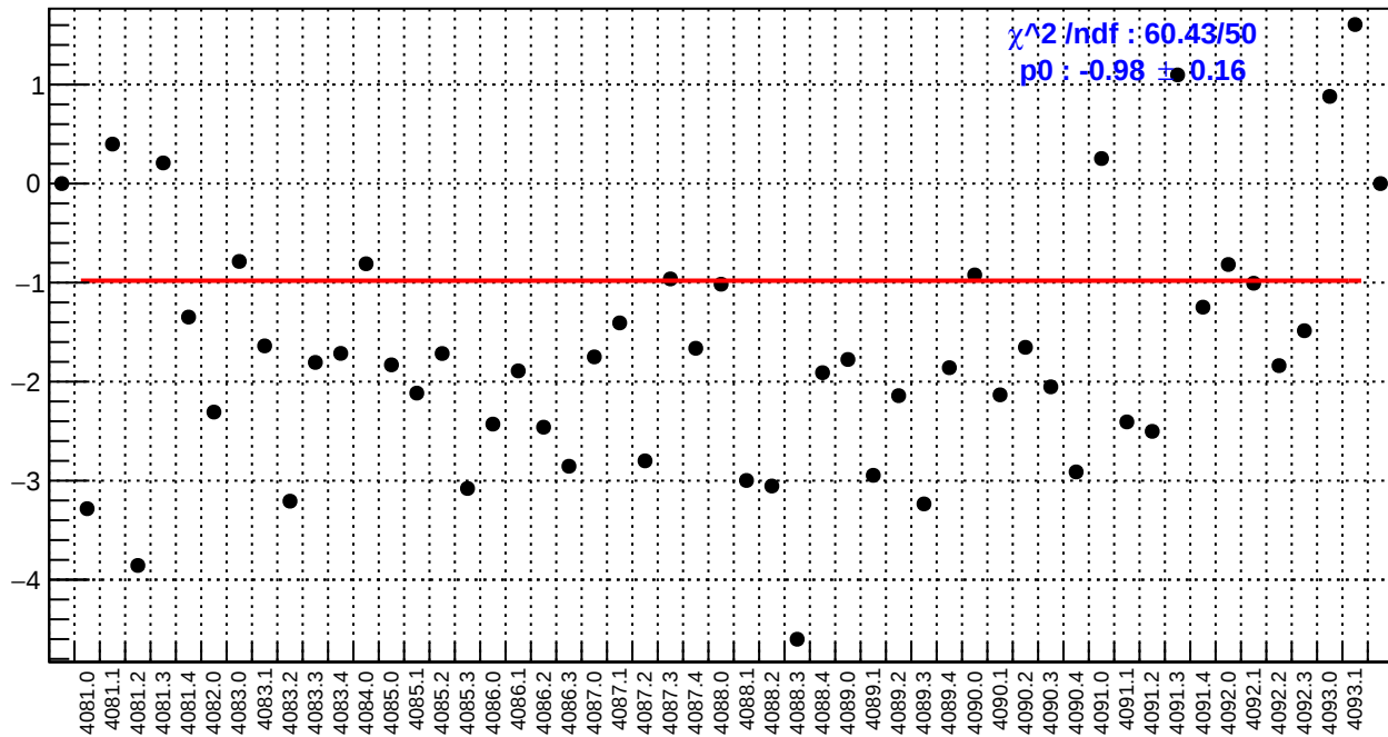
slug44: ds_avg_bpm4aX/(ppb/nm)
