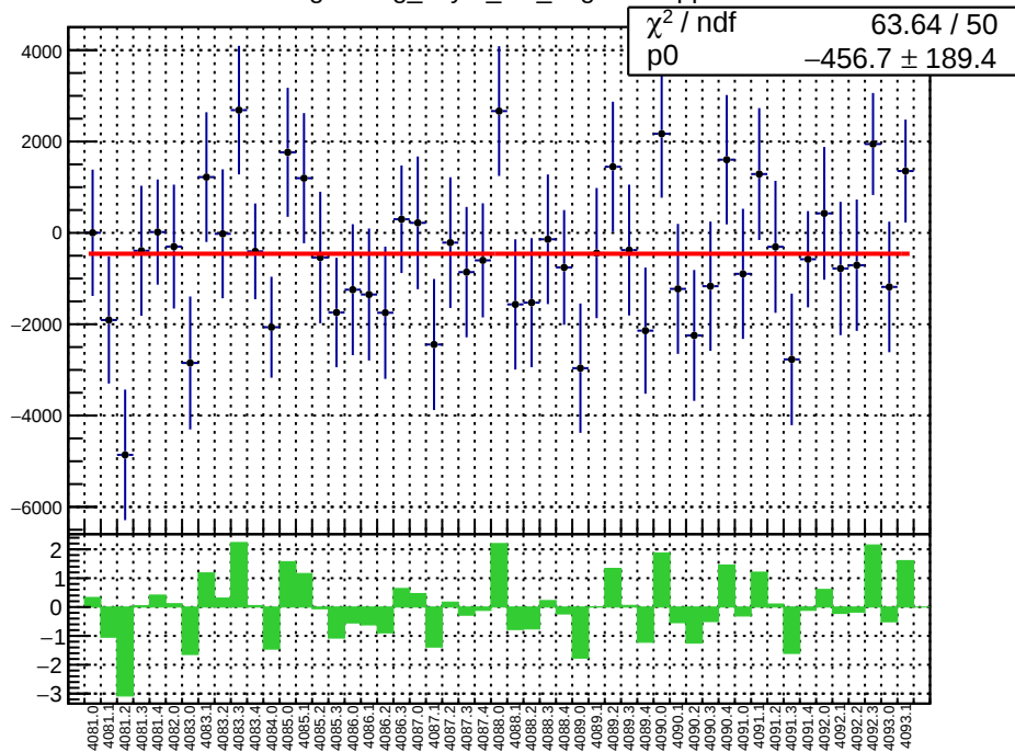
slug44: reg_asym_left_avg.mean/ppb
