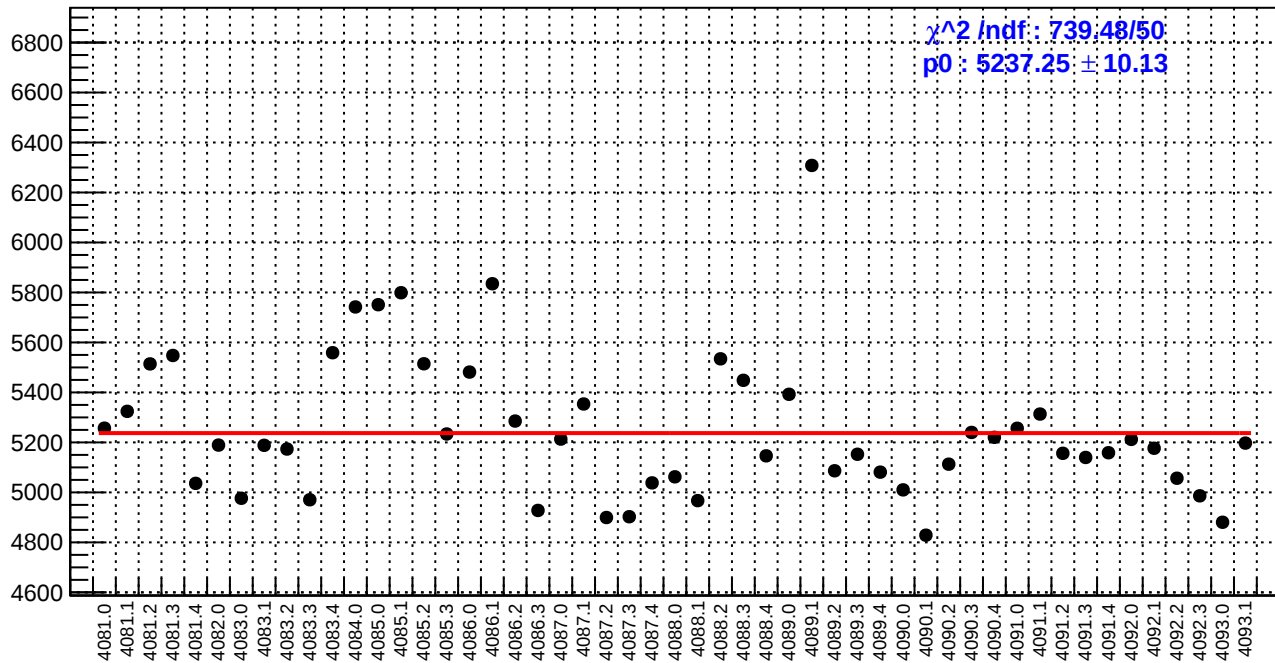
slug44: diff_bpm11X.rms/nm
