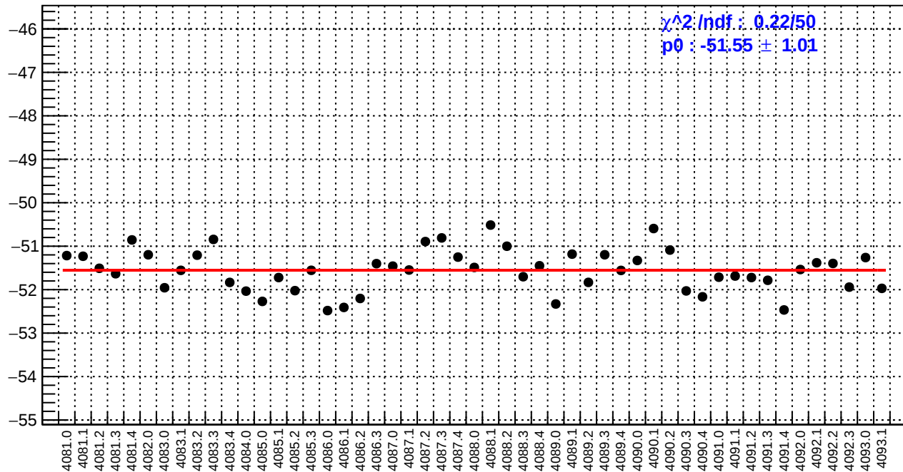
slug44: dsl_bpm12X/(ppb/nm)
