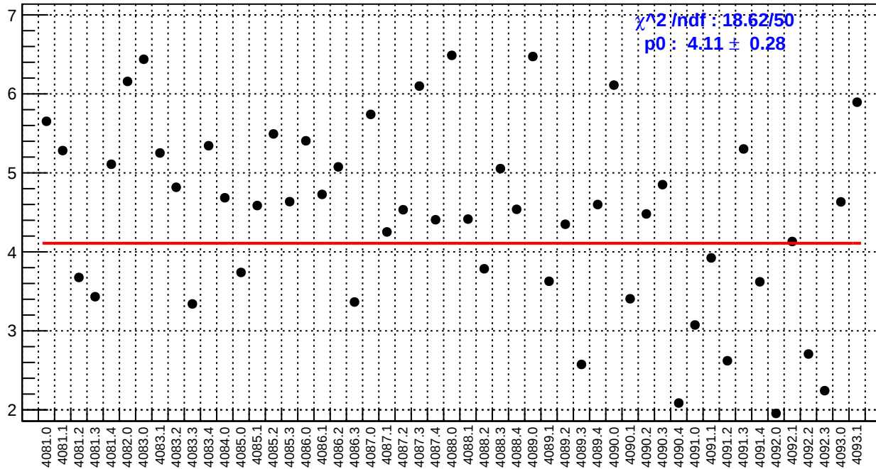
slug44: left_avg_bpm4aY/(ppb/nm)
