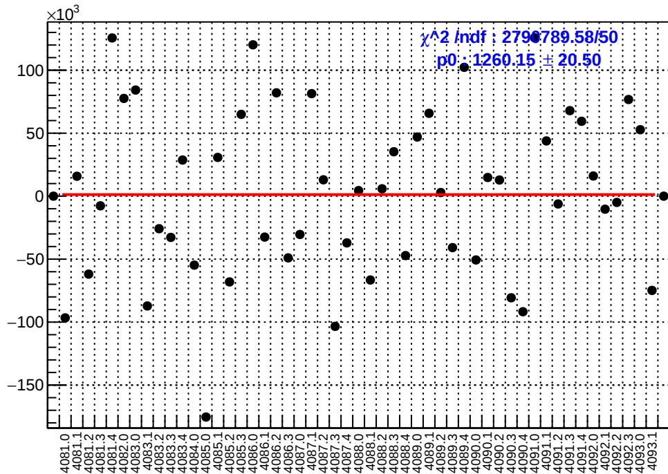
slug44: asym_sam4.mean/ppb-reg_asym_sam4.mean/ppb
