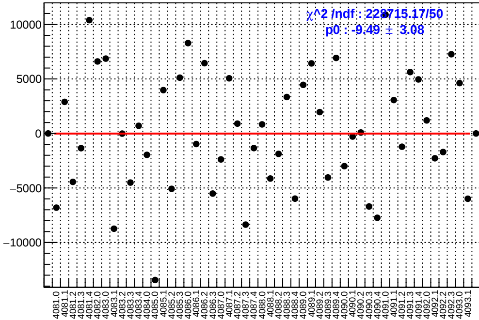
slug44: asym_us_dd.mean/ppb-reg_asym_us_dd.mean/ppb
