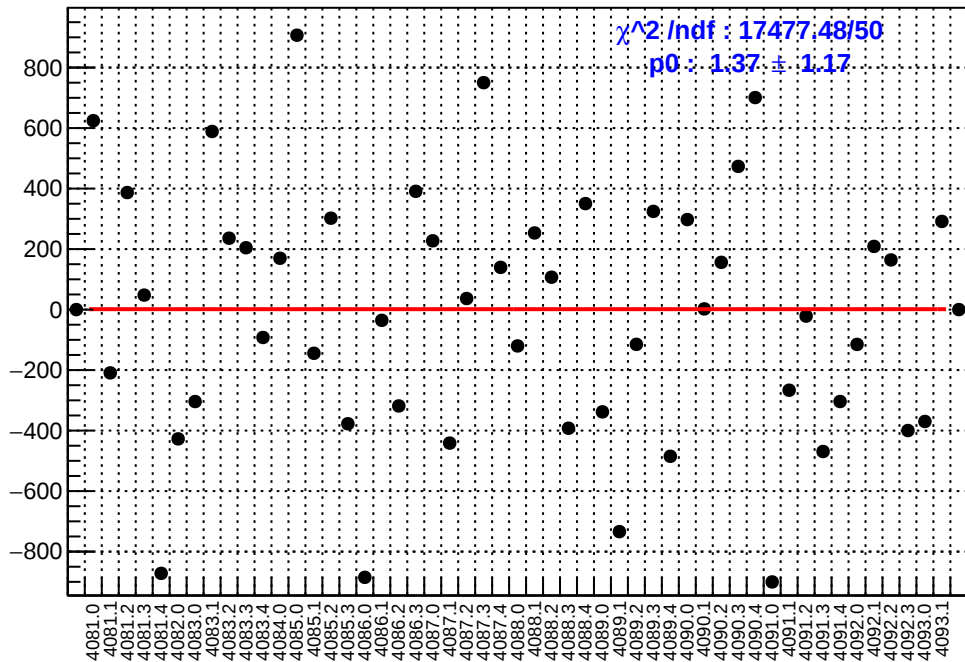
slug44: asym_right_dd.mean/ppb-reg_asym_right_dd.mean/ppb
