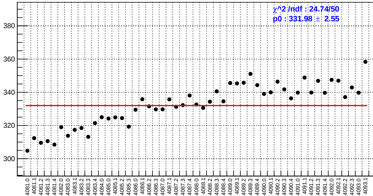
slug44: reg_asym_sam7.rms/ppm
