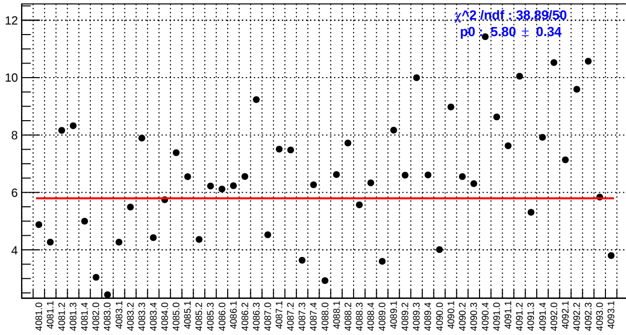
slug44: left_avg_bpm4eY/(ppb/nm)
