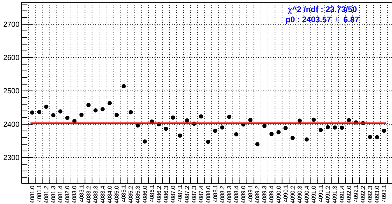
slug44: reg_asym_sam2.rms/ppm
