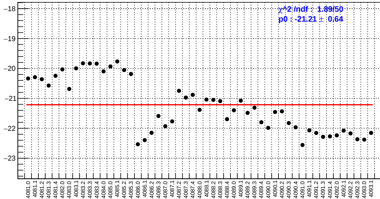
slug44: us_avg_bpm4eX/(ppb/nm)
