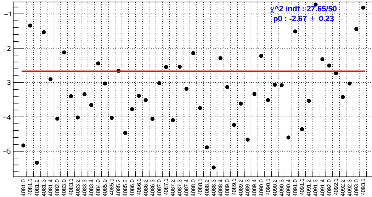
slug44: us_avg_bpm4aX/(ppb/nm)
