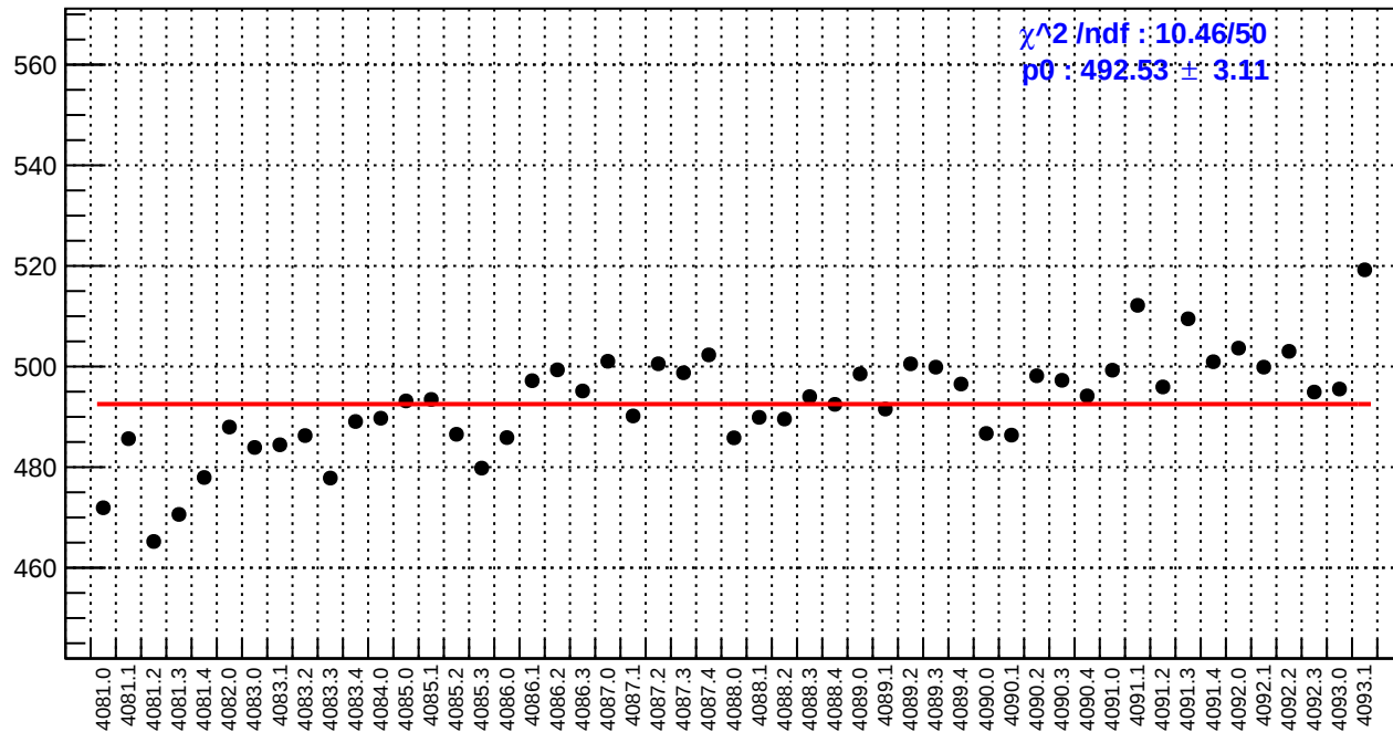
slug44: reg_asym_sam8.rms/ppm
