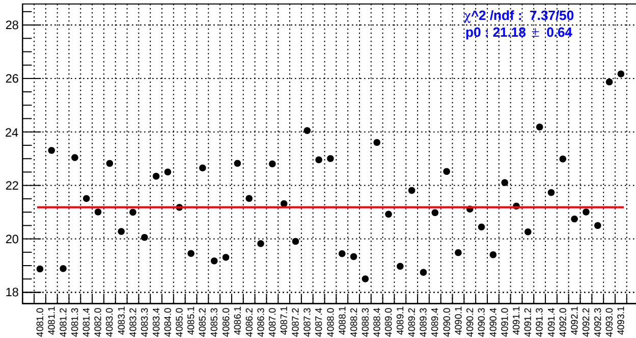
slug44: usl_bpm4aX/(ppb/nm)
