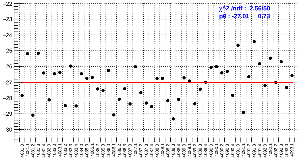
slug44: right_avg_bpm4aX/(ppb/nm)
