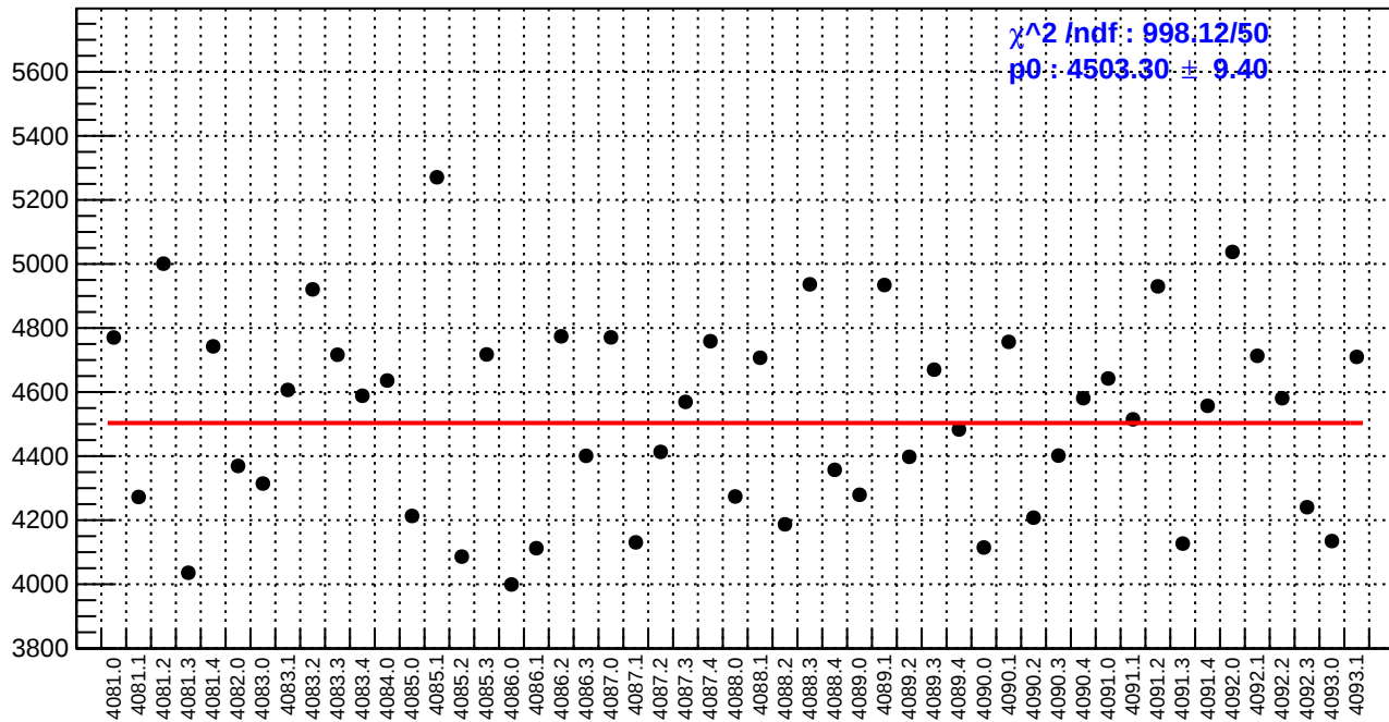
slug44: diff_bpm4eY.rms/nm
