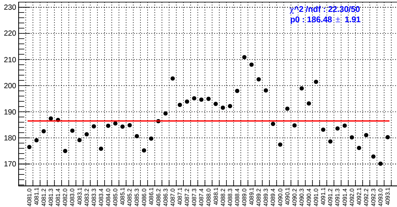
slug44: asym_bcm_an_us.rms/ppm
