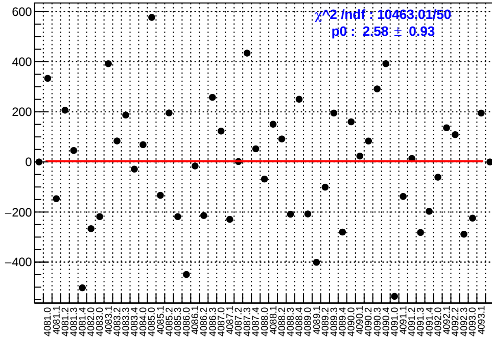
slug44: asym_left_dd.mean/ppb-reg_asym_left_dd.mean/ppb
