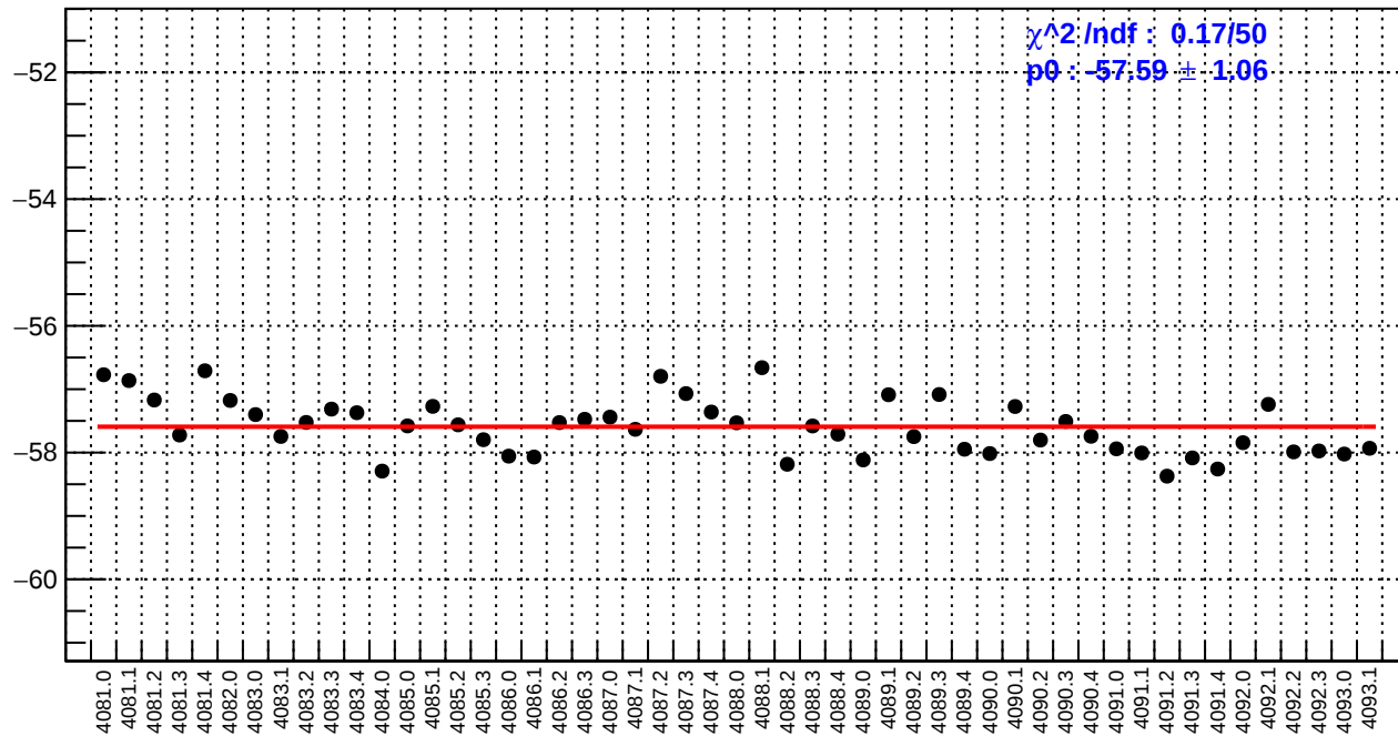
slug44: right_avg_bpm12X/(ppb/nm)
