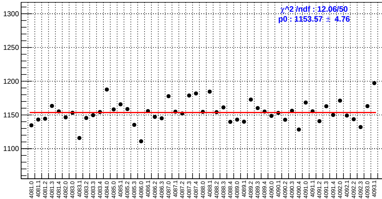
slug44: reg_asym_sam4.rms/ppm
