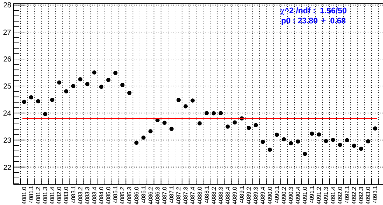
slug44: right_avg_bpm4eX/(ppb/nm)
