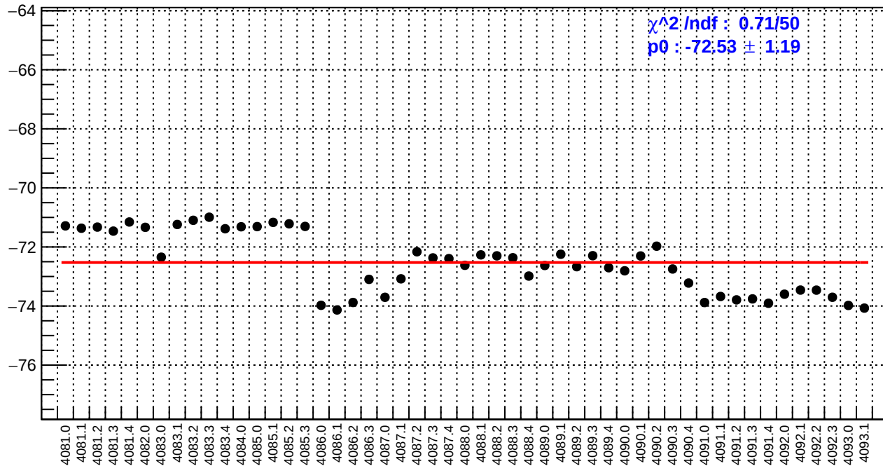
slug44: left_avg_bpm4eX/(ppb/nm)
