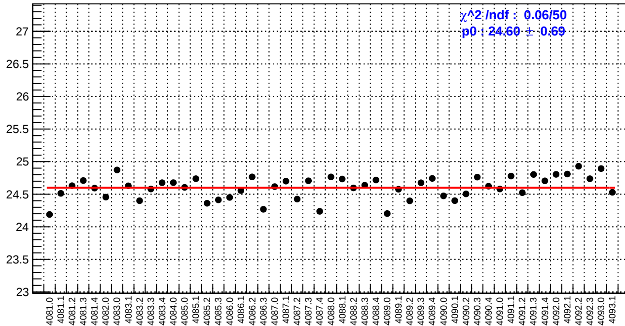
slug44: reg_asym_left_dd.rms/ppm
