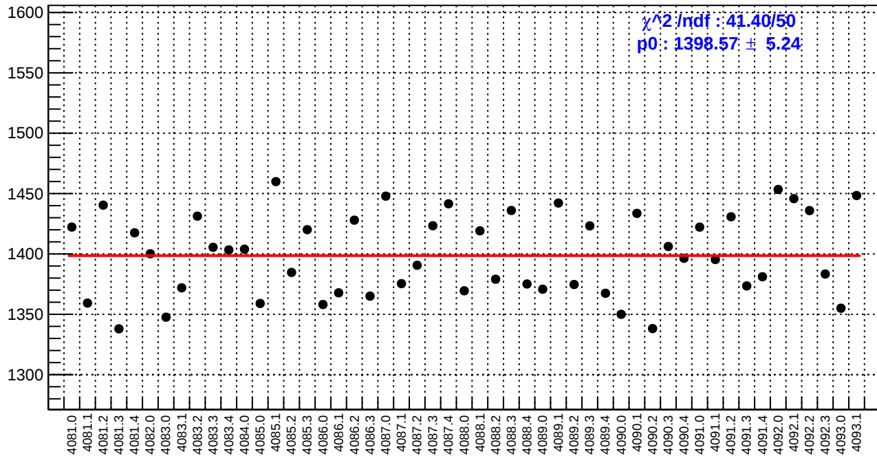
slug44: diff_bpm4aX.rms/nm
