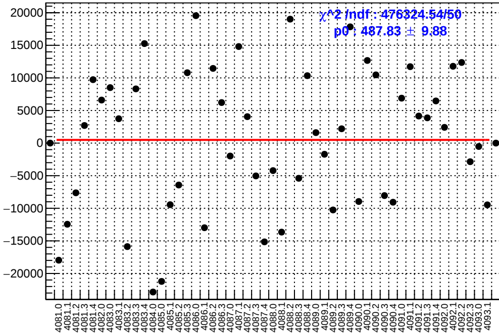
slug44: asym_sam5.mean/ppb-reg_asym_sam5.mean/ppb
