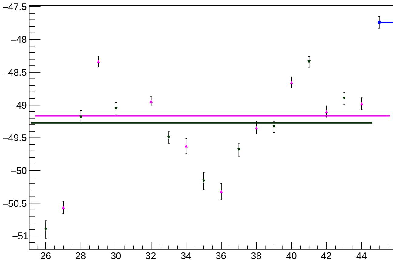
reg_asym_us_dd_diff_bpm4eX_slope vs slug
