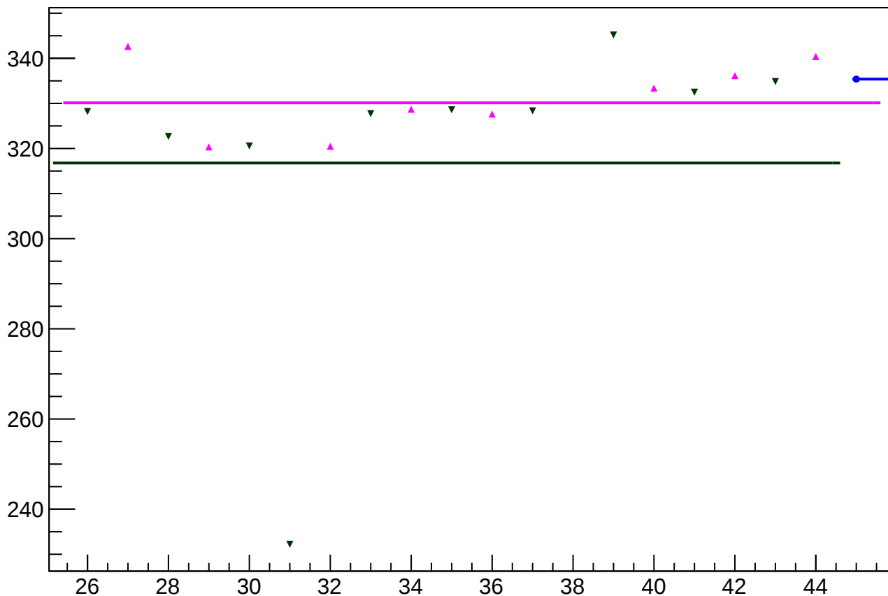
reg_asym_atl1r2_dd_rms vs slug
