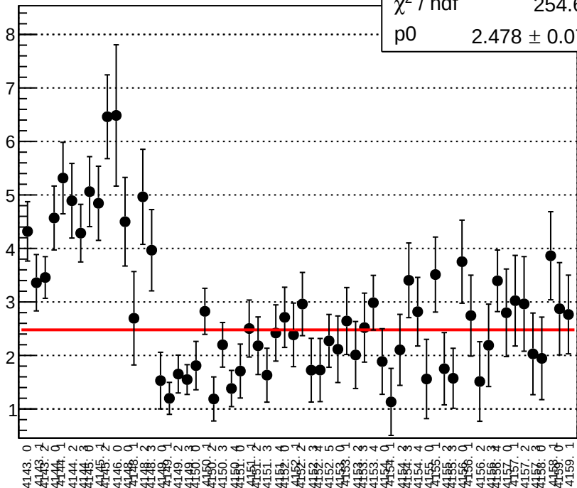
reg_asym_bcm_dg_us_diff_bpm11X_slope vs run
