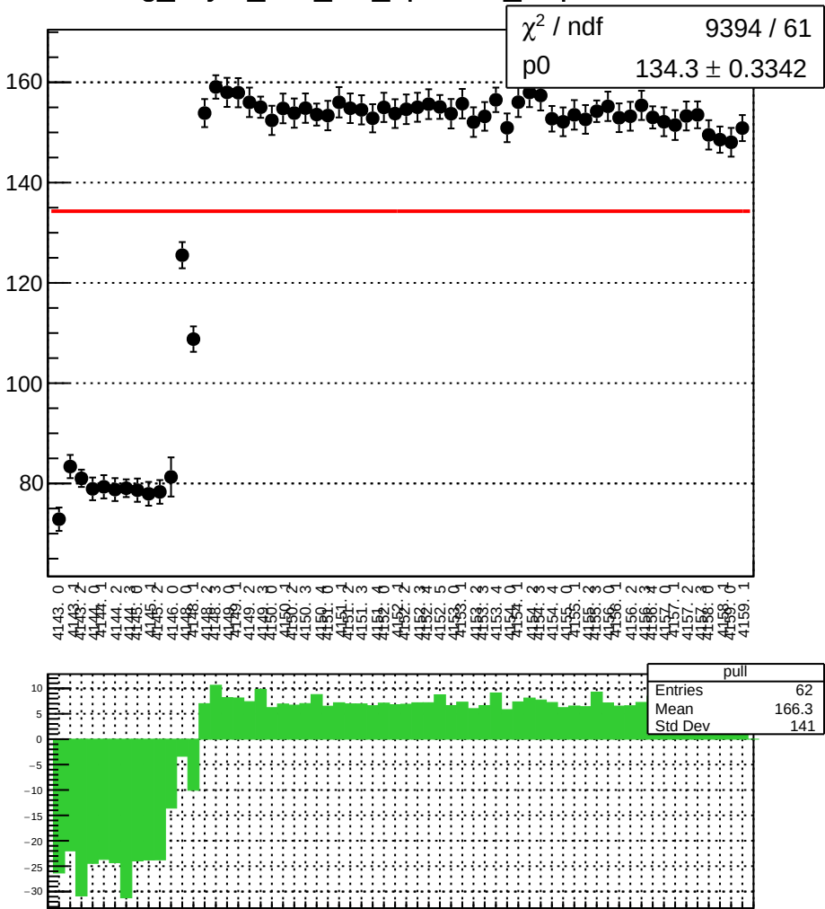
reg_asym_atl1_diff_bpm11X_slope vs run
