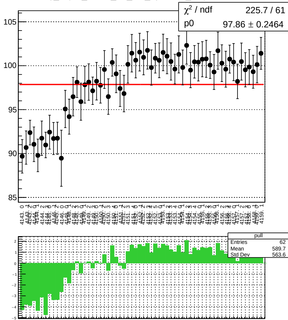
reg_asym_atl1r2_dd_diff_bpm4eX_slope vs run
