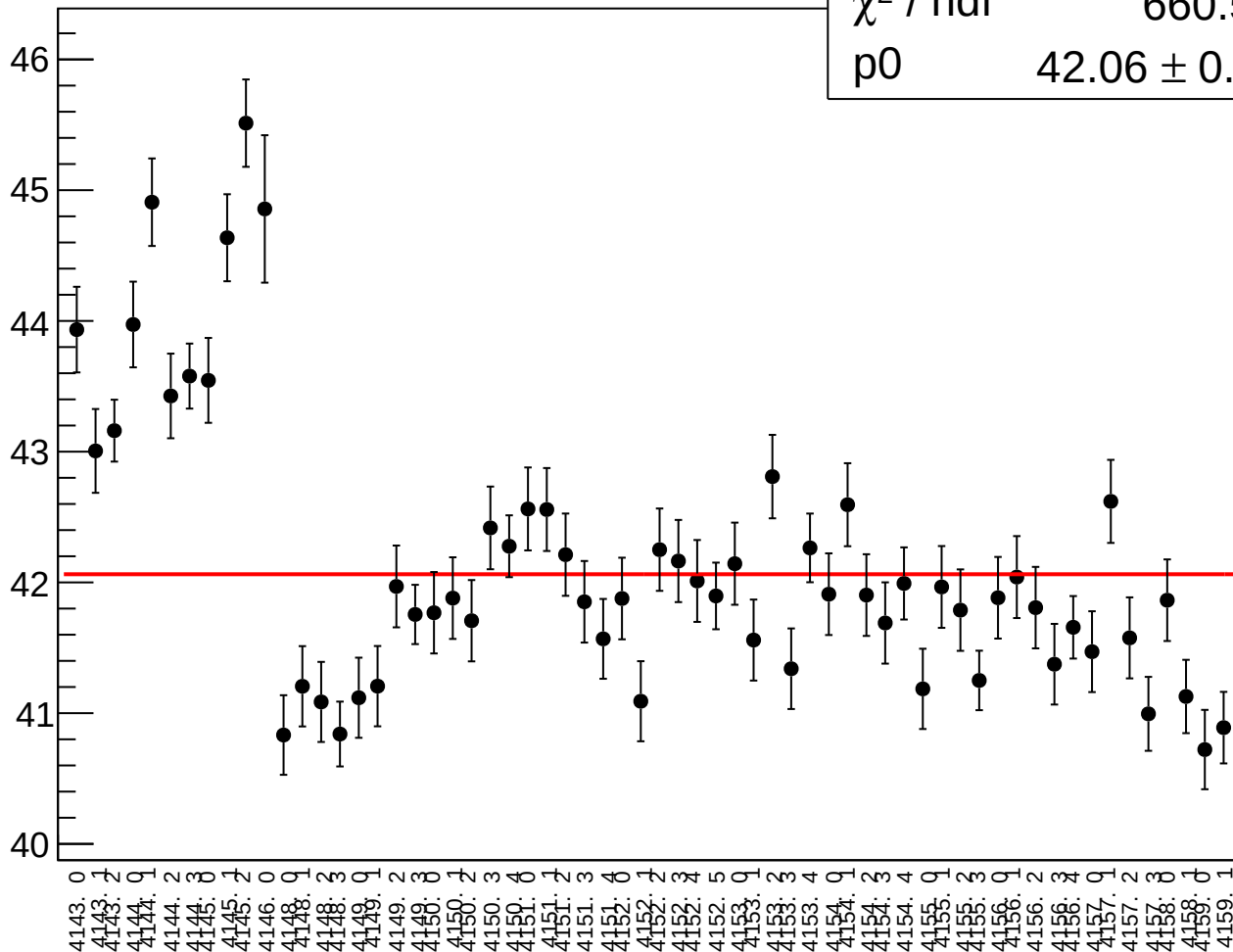
asym_right_dd_rms vs run
