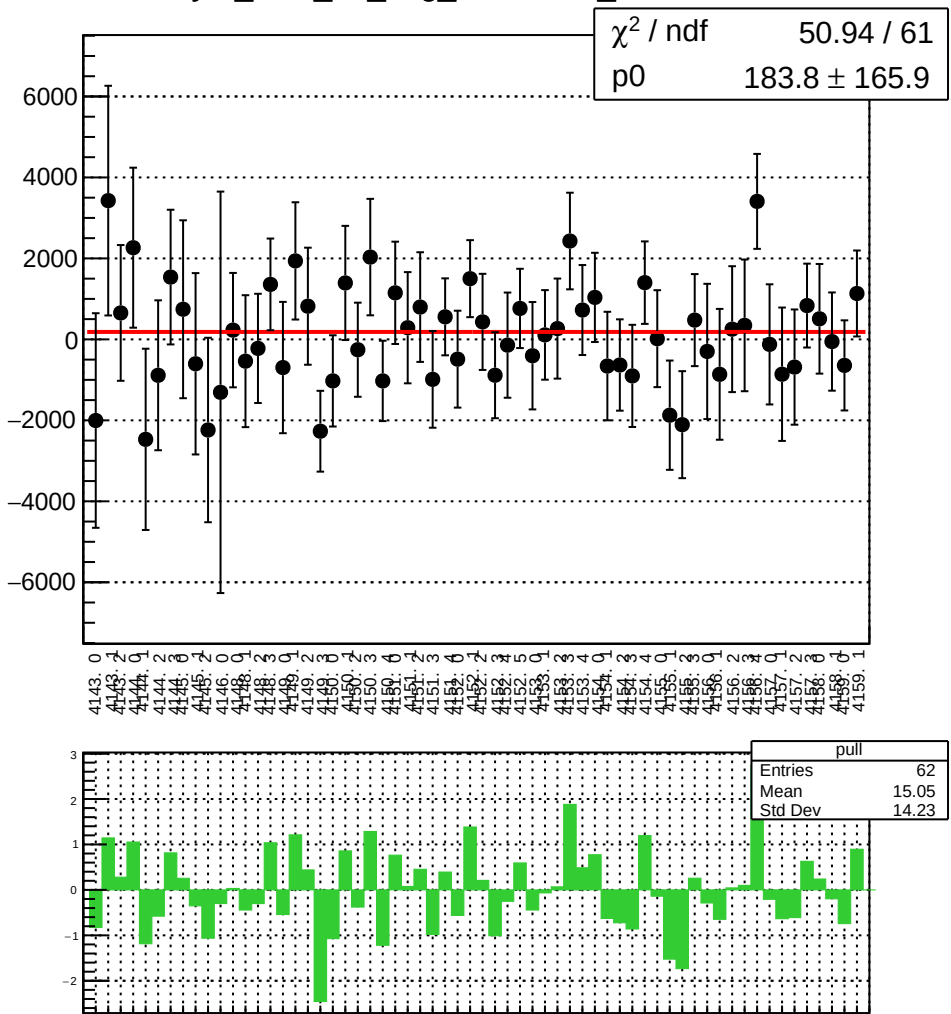
asym_sam_15_avg_correction_mean vs run
