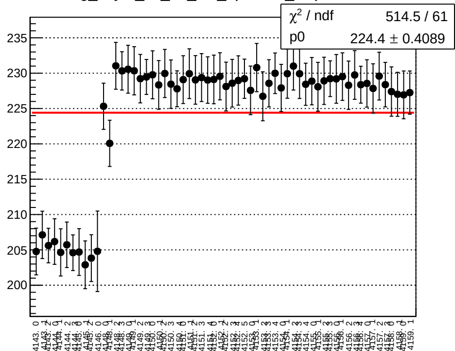
reg_asym_atl_dd_diff_bpm11X_slope vs run
