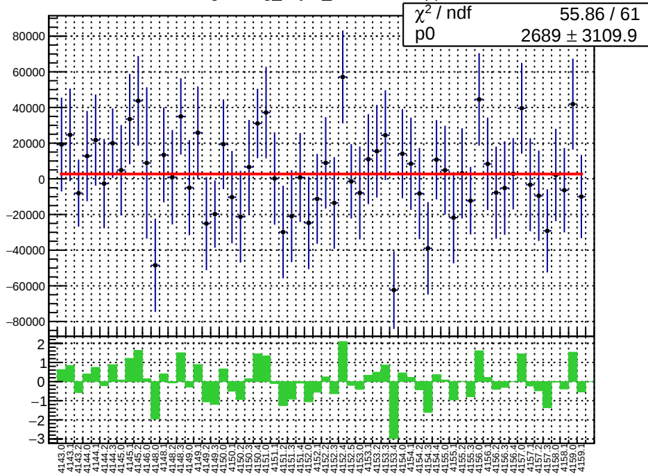
slug45: reg_asym_sam2.mean/ppb
