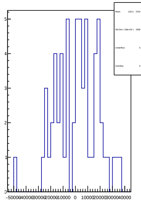
slug45: 1D Corr asym_sam1.mean/ppb-reg_asym_sam1.mean/ppb
