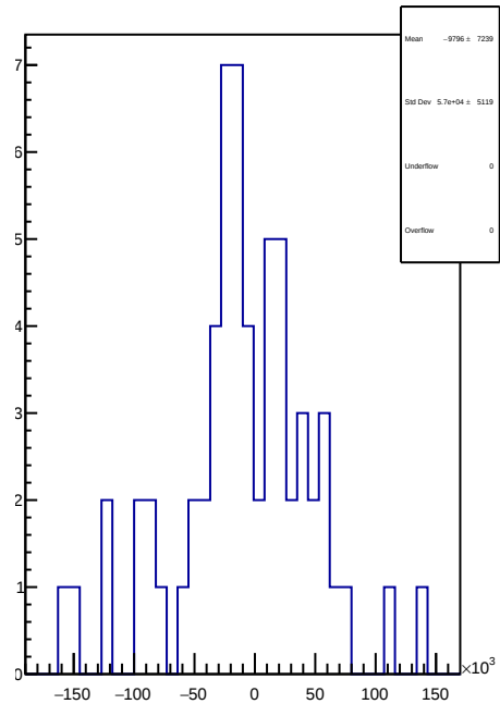
slug45: 1D Corr asym_sam4.mean/ppb-reg_asym_sam4.mean/ppb
