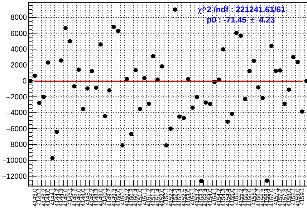
slug45: asym_ds_dd.mean/ppb-reg_asym_ds_dd.mean/ppb
