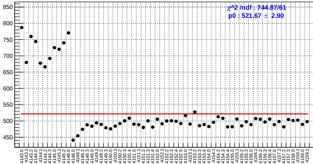
slug45: reg_asym_sam6.rms/ppm
