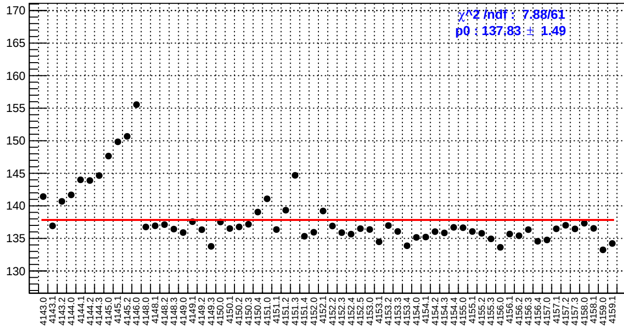
slug45: reg_asym_dsr.rms/ppm
