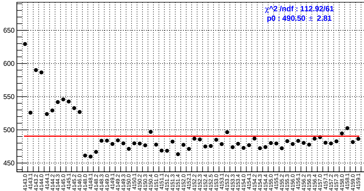
slug45: reg_asym_sam8.rms/ppm
