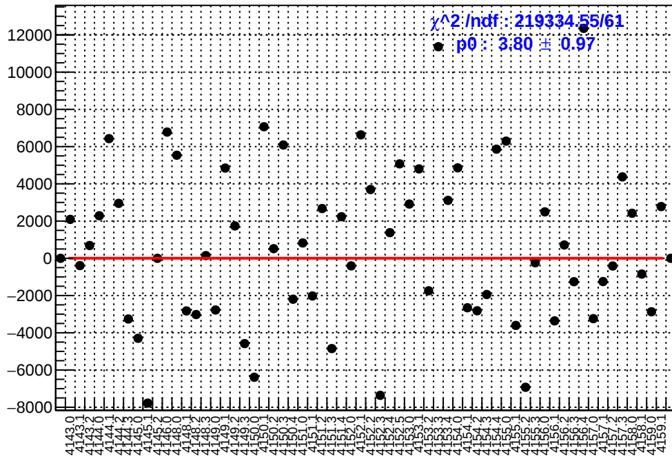
slug45: asym_dsr.mean/ppb-reg_asym_dsr.mean/ppb
