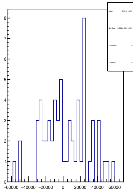
slug45: 1D Corr asym_sam6.mean/ppb-reg_asym_sam6.mean/ppb
