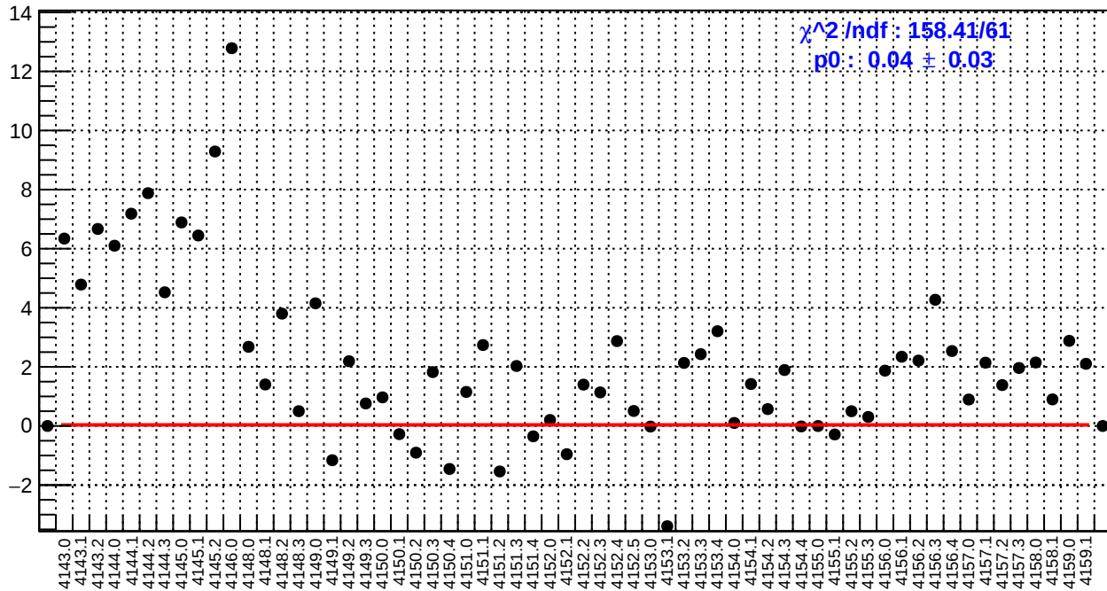
slug45: right_avg_bpm4eY/(ppb/nm)
