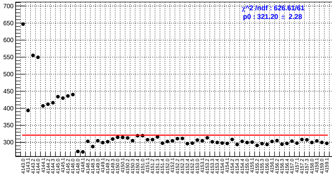
slug45: reg_asym_sam7.rms/ppm
