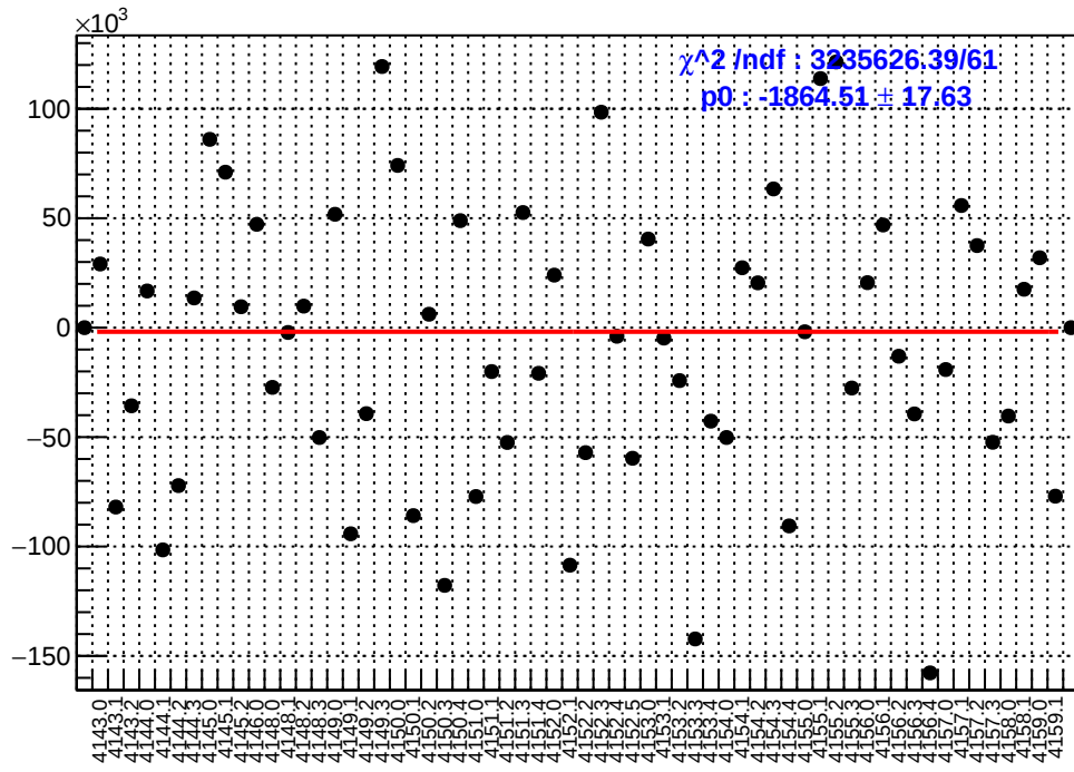
slug45: asym_sam2.mean/ppb-reg_asym_sam2.mean/ppb
