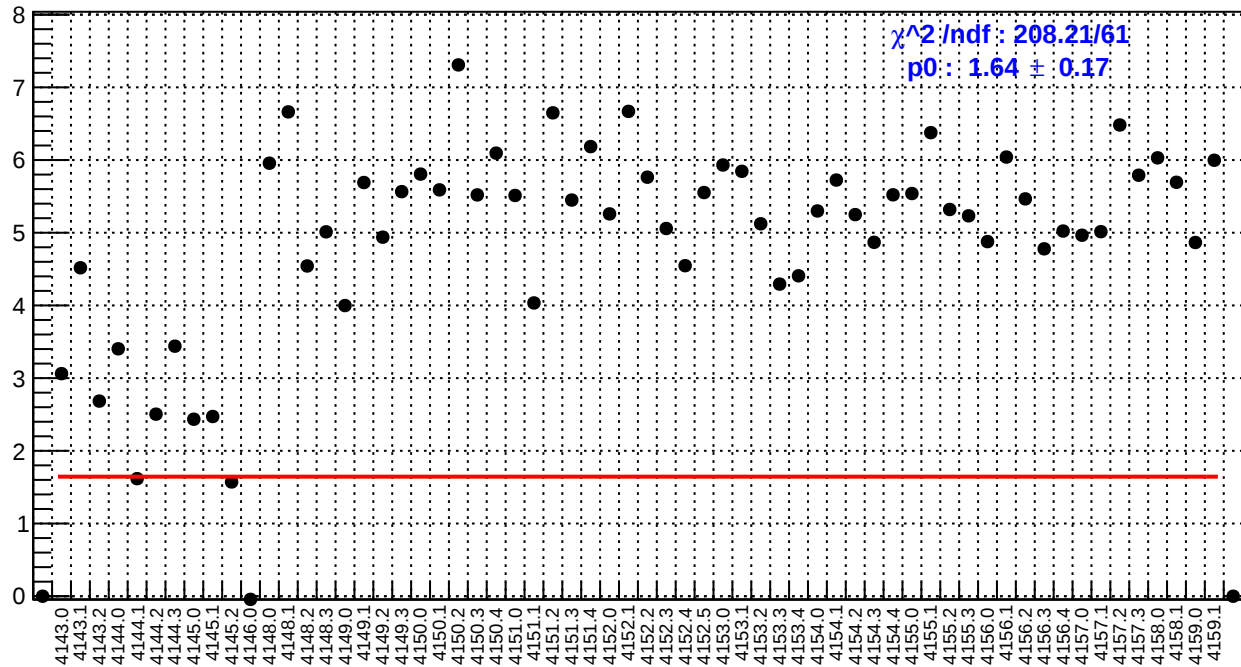
slug45: us_avg_bpm4aY/(ppb/nm)
