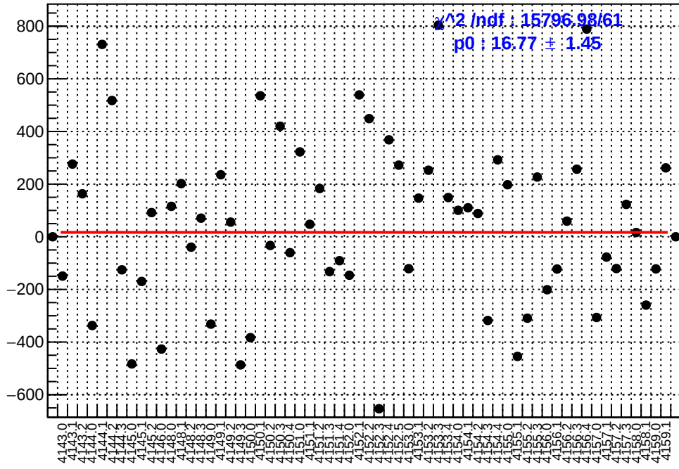
slug45: asym_right_dd.mean/ppb-reg_asym_right_dd.mean/ppb
