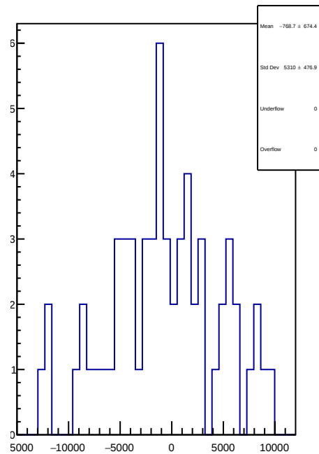
slug45: 1D Corr asym_usl.mean/ppb-reg_asym_usl.mean/ppb
