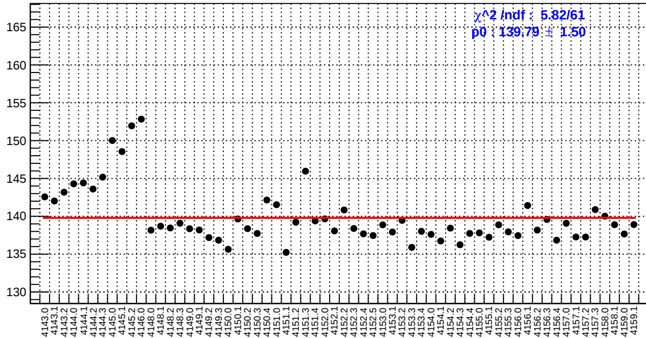
slug45: reg_asym_dsl.rms/ppm
