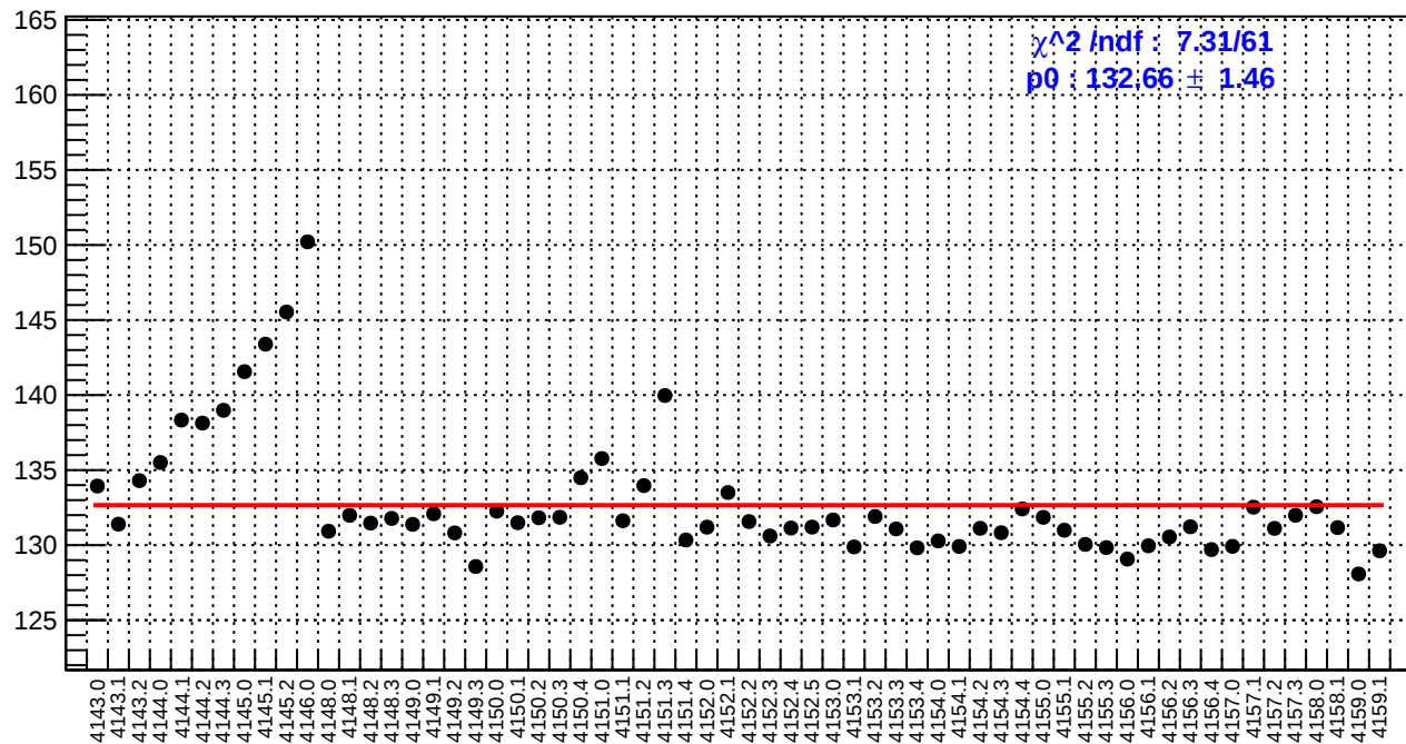
slug45: reg_asym_usr.rms/ppm
