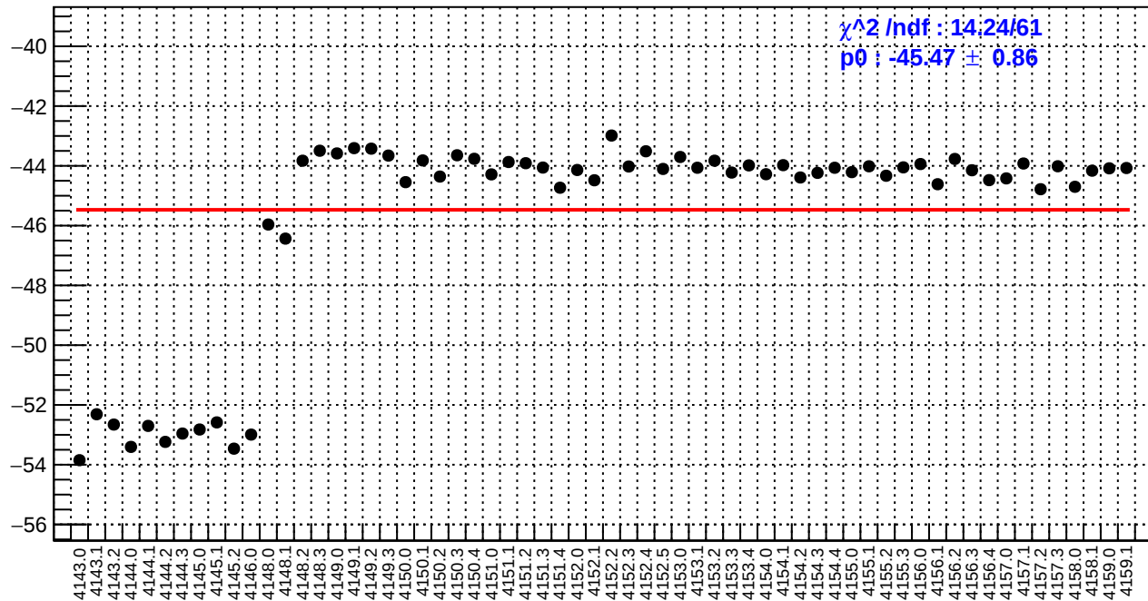
slug45: ds_avg_bpm12X/(ppb/nm)
