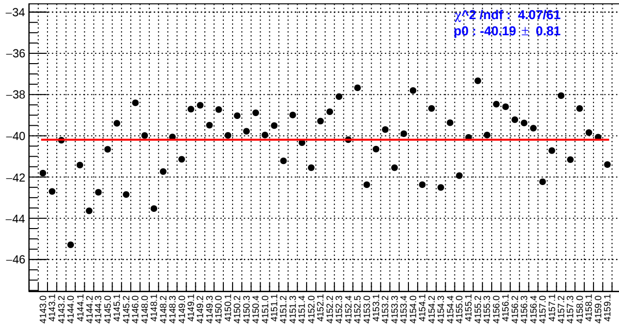
slug45: usr_bpm4aX/(ppb/nm)
