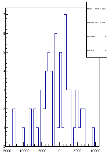
slug45: 1D Corr asym_us_dd.mean/ppb-reg_asym_us_dd.mean/ppb
