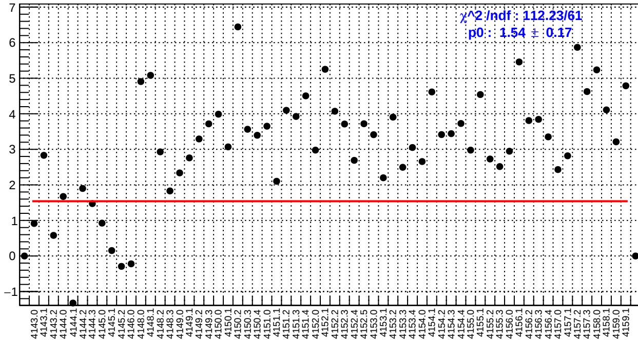
slug45: left_avg_bpm4aY/(ppb/nm)
