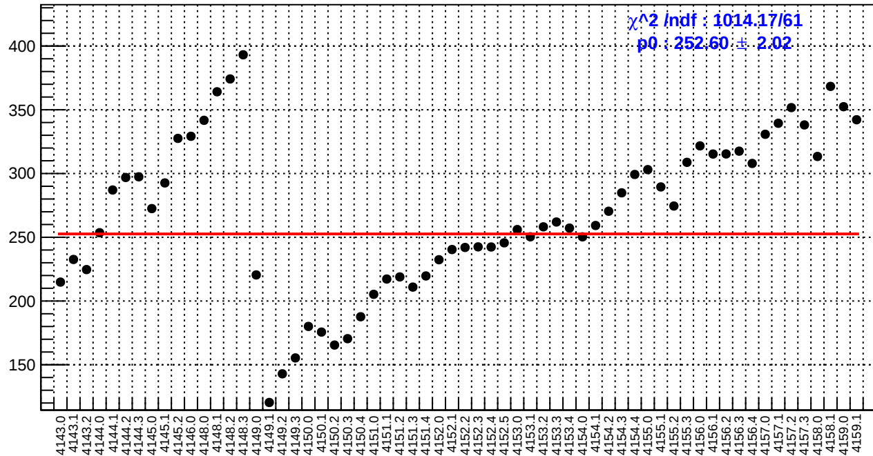
slug45: asym_bcm_an_us.rms/ppm
