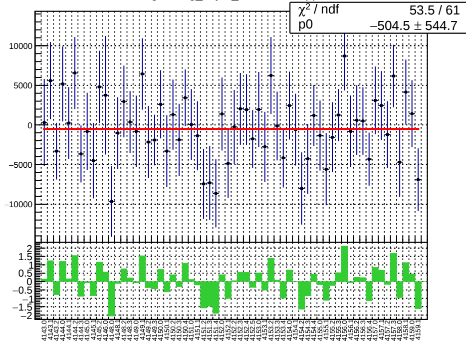
slug45: reg_asym_sam1.mean/ppb
