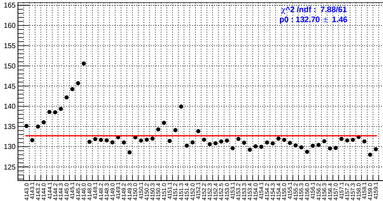
slug45: reg_asym_right_avg.rms/ppm
