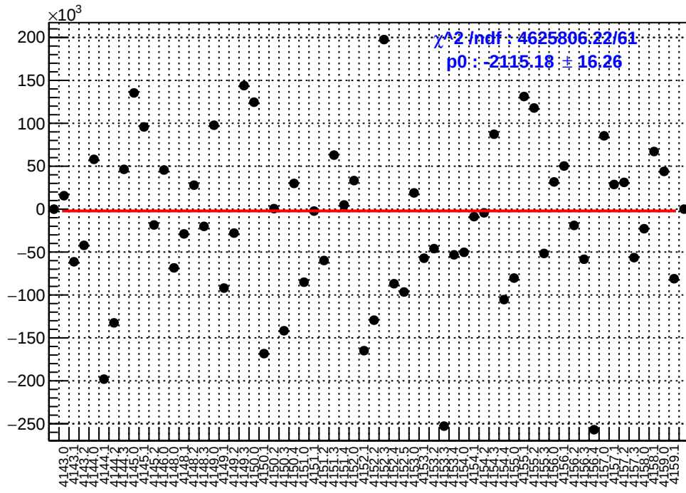
slug45: asym_sam3.mean/ppb-reg_asym_sam3.mean/ppb
