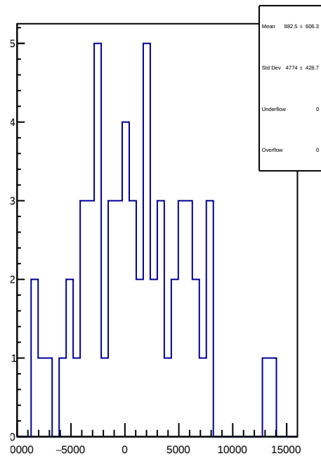
slug45: 1D Corr asym_usr.mean/ppb-reg_asym_usr.mean/ppb
