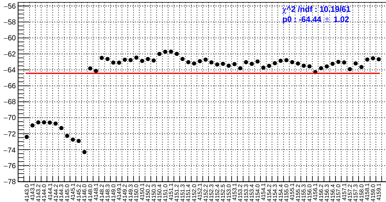
slug45: left_avg_bpm4eX/(ppb/nm)
