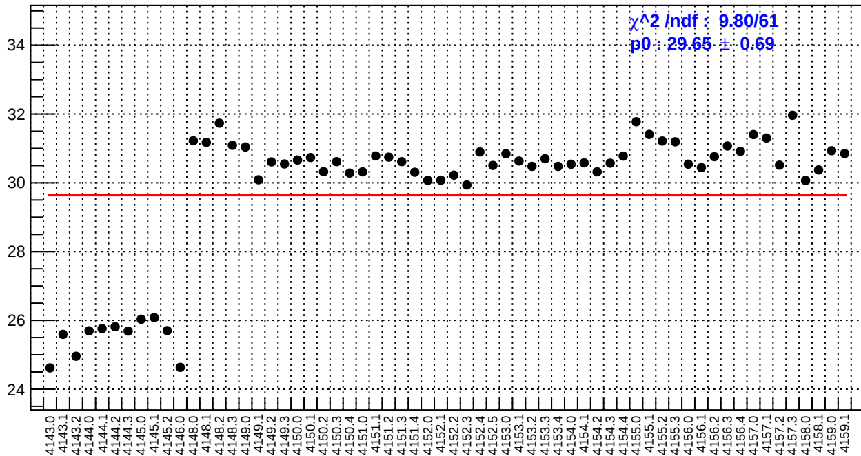
slug45: right_avg_bpm4eX/(ppb/nm)
