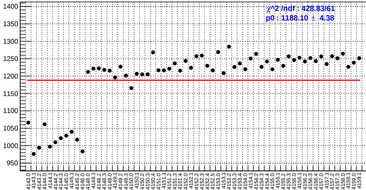
slug45: reg_asym_sam4.rms/ppm
