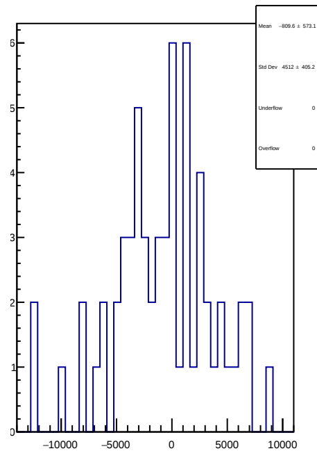
slug45: 1D Corr asym_ds_dd.mean/ppb-reg_asym_ds_dd.mean/ppb
