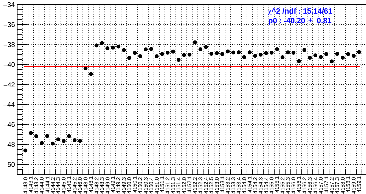
slug45: left_avg_bpm12X/(ppb/nm)
