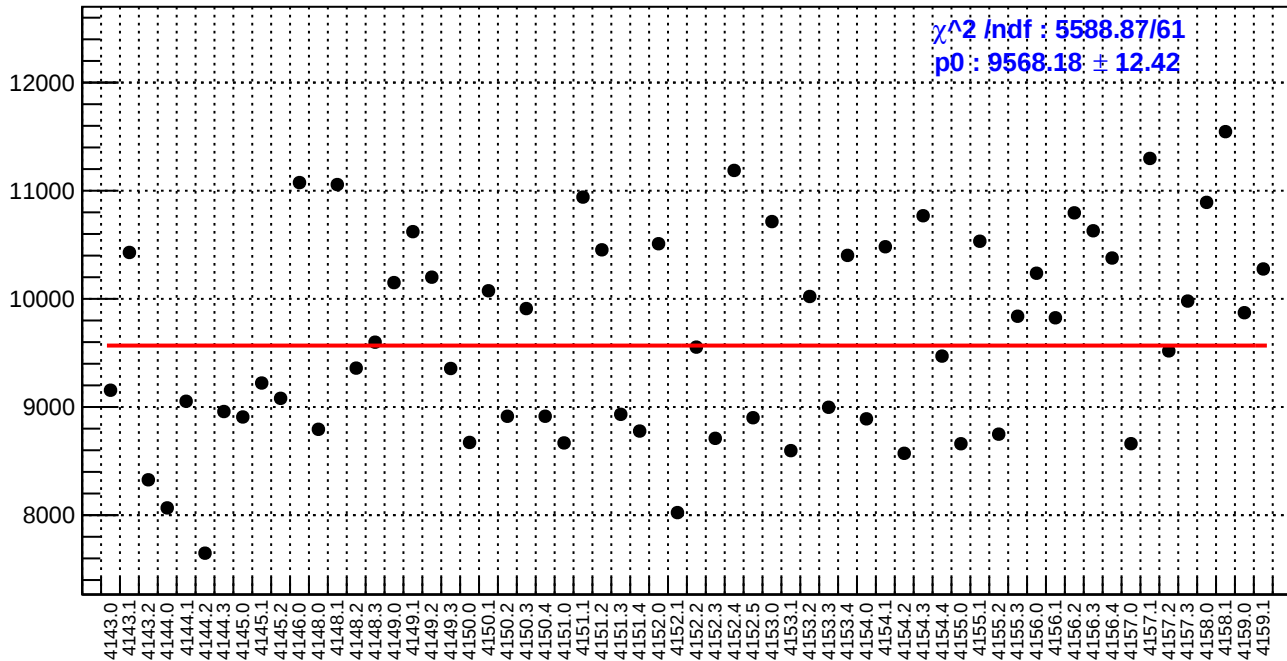
slug45: diff_bpm4aY.rms/nm
