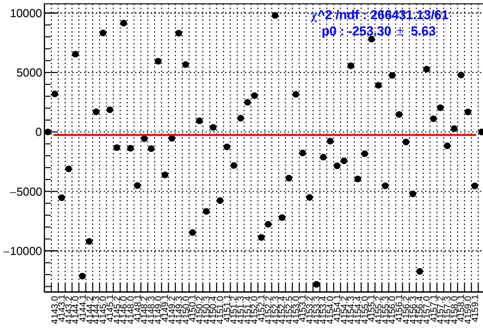
slug45: asym_usl.mean/ppb-reg_asym_usl.mean/ppb
