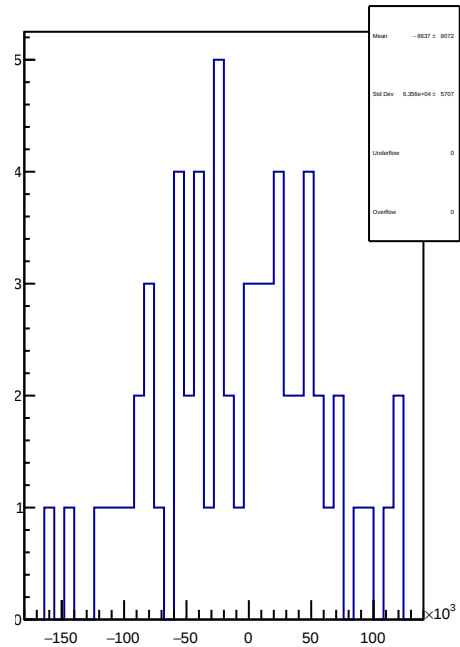
slug45: 1D Corr asym_sam2.mean/ppb-reg_asym_sam2.mean/ppb
