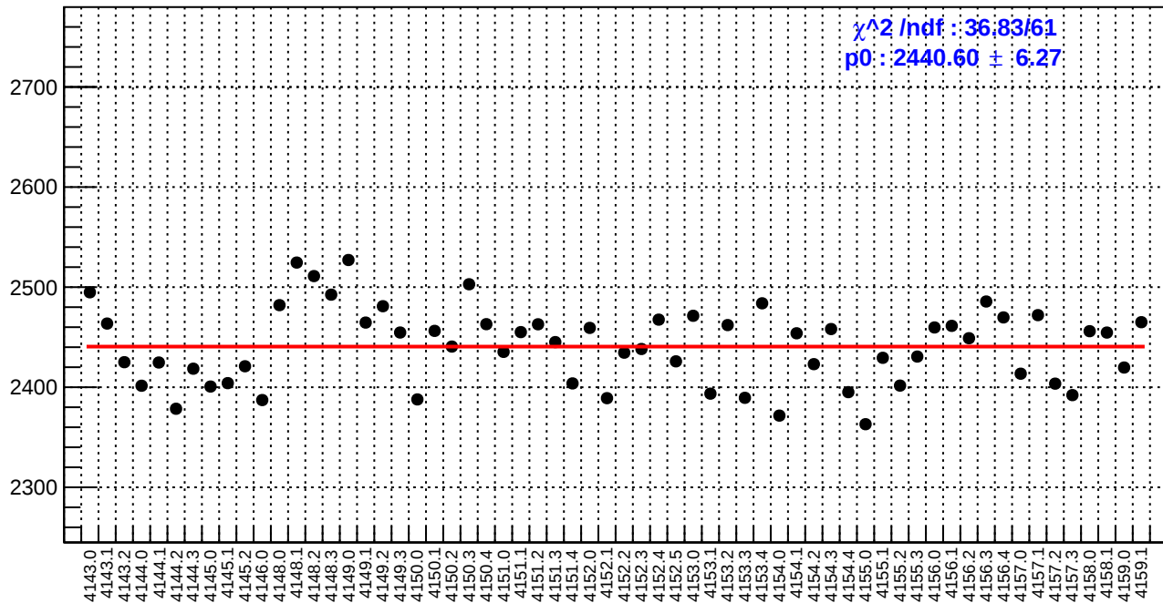
slug45: reg_asym_sam2.rms/ppm
