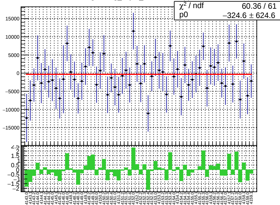
slug45: reg_asym_sam8.mean/ppb
