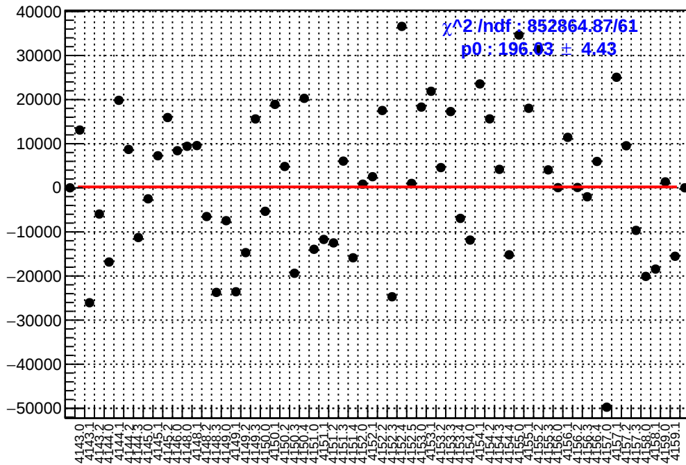
slug45: asym_sam1.mean/ppb-reg_asym_sam1.mean/ppb
