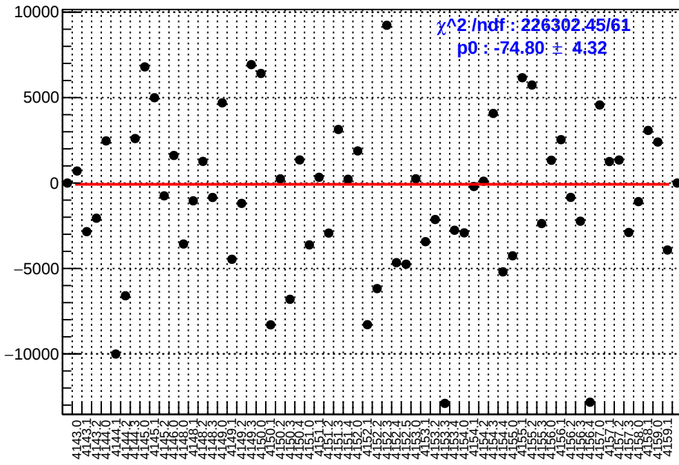
slug45: asym_us_dd.mean/ppb-reg_asym_us_dd.mean/ppb
