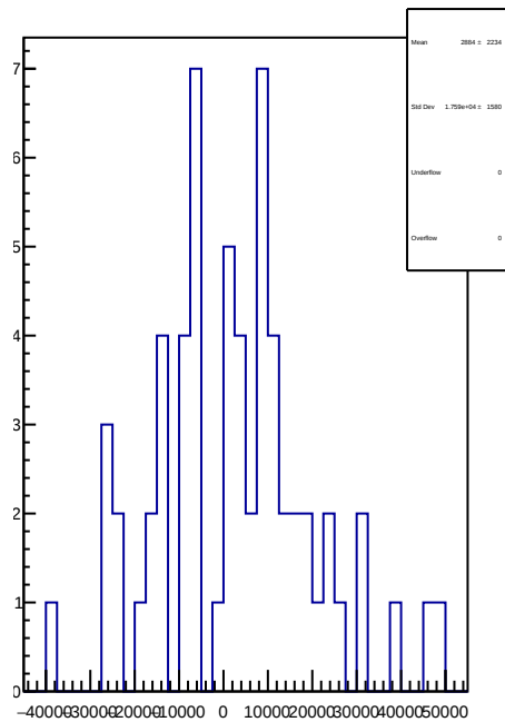
slug45: 1D Corr asym_sam7.mean/ppb-reg_asym_sam7.mean/ppb
