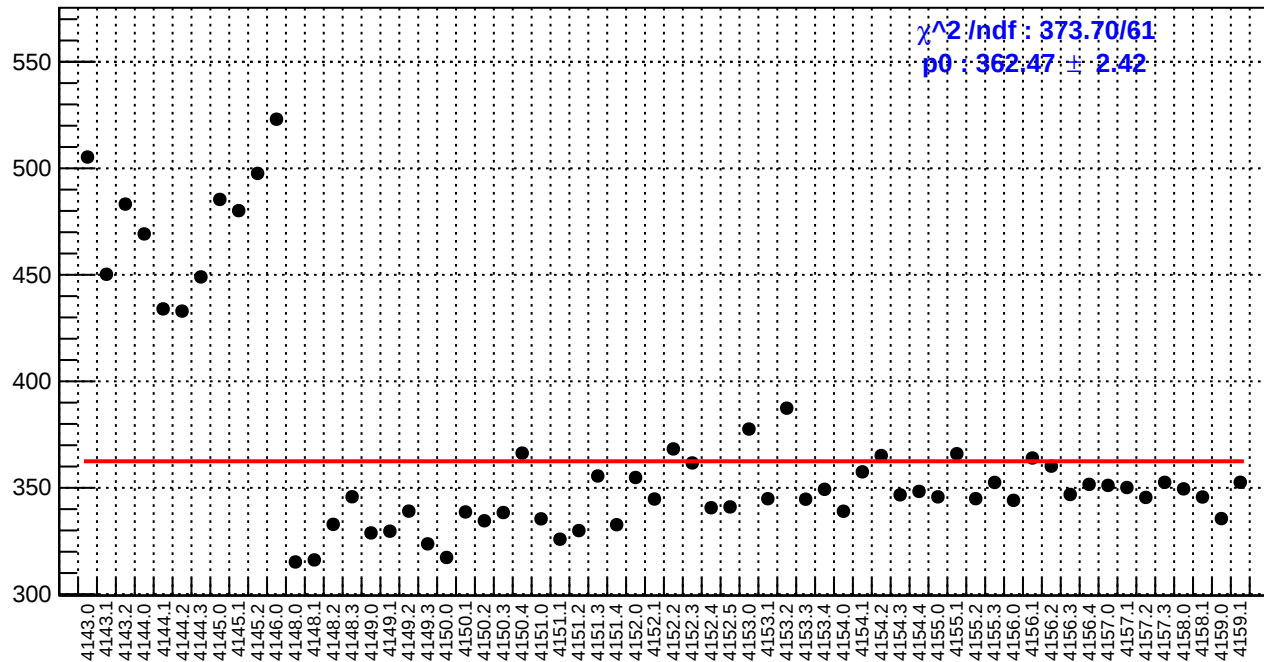
slug45: reg_asym_sam5.rms/ppm
