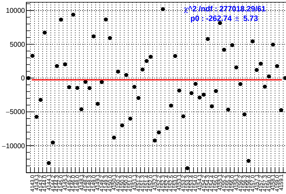
slug45: asym_left_avg.mean/ppb-reg_asym_left_avg.mean/ppb
