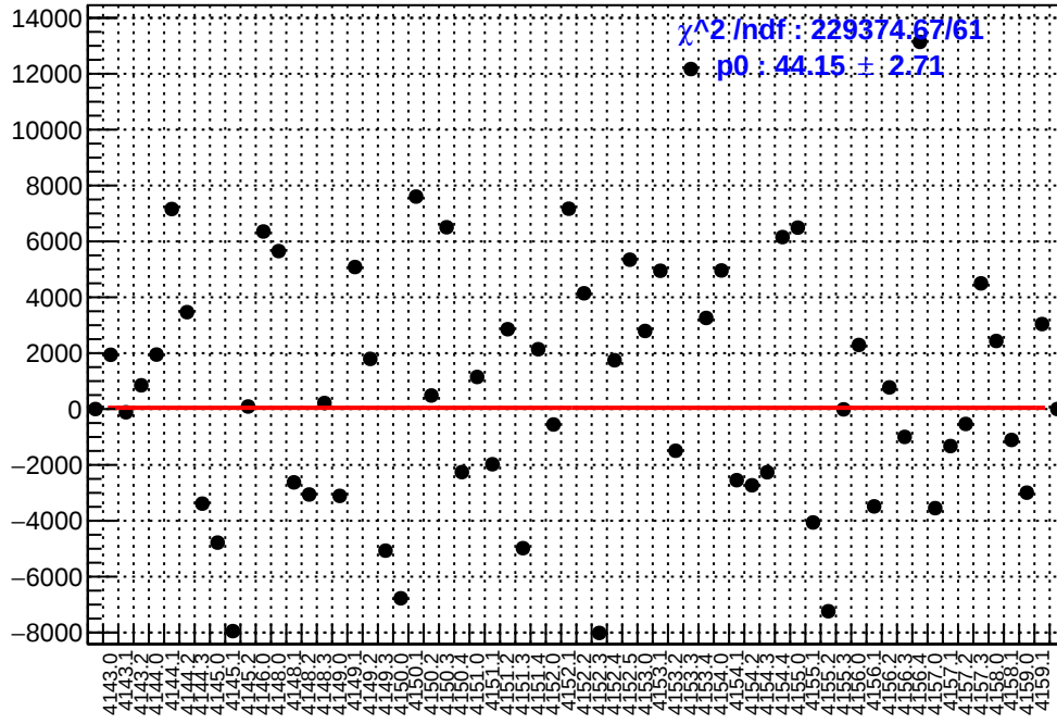
slug45: asym_right_avg.mean/ppb-reg_asym_right_avg.mean/ppb
