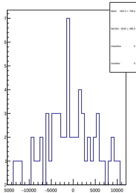
slug45: 1D Corr asym_left_avg.mean/ppb-reg_asym_left_avg.mean/ppb
