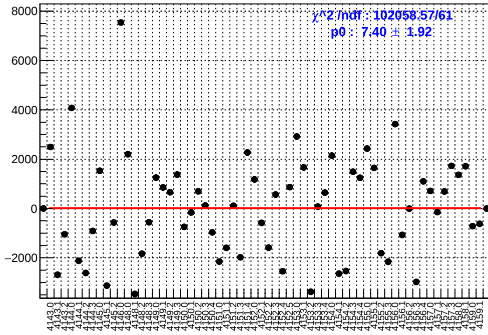
slug45: asym_us_avg.mean/ppb-reg_asym_us_avg.mean/ppb
