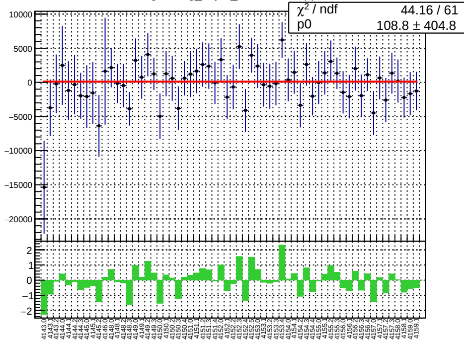
slug45: reg_asym_sam7.mean/ppb
