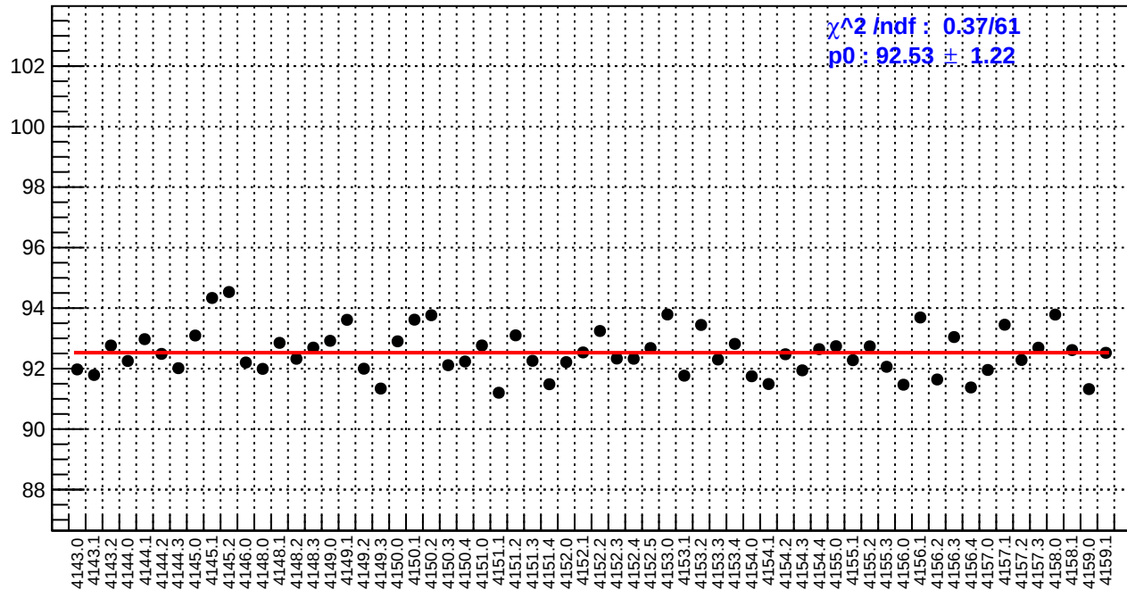
slug45: reg_asym_us_dd.rms/ppm
