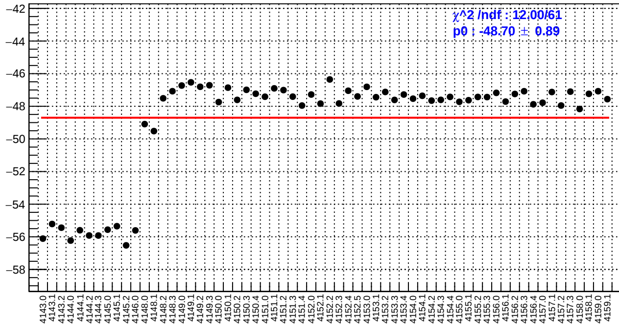
slug45: right_avg_bpm12X/(ppb/nm)
