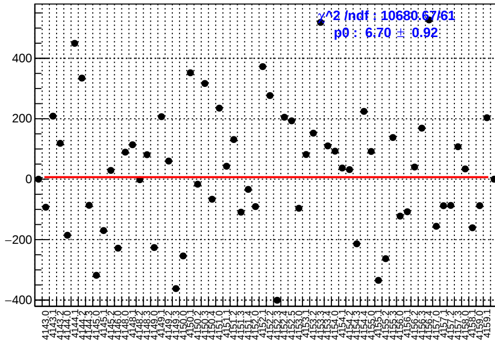
slug45: asym_left_dd.mean/ppb-reg_asym_left_dd.mean/ppb
