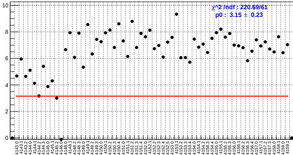
slug45: right_avg_bpm4aY/(ppb/nm)
