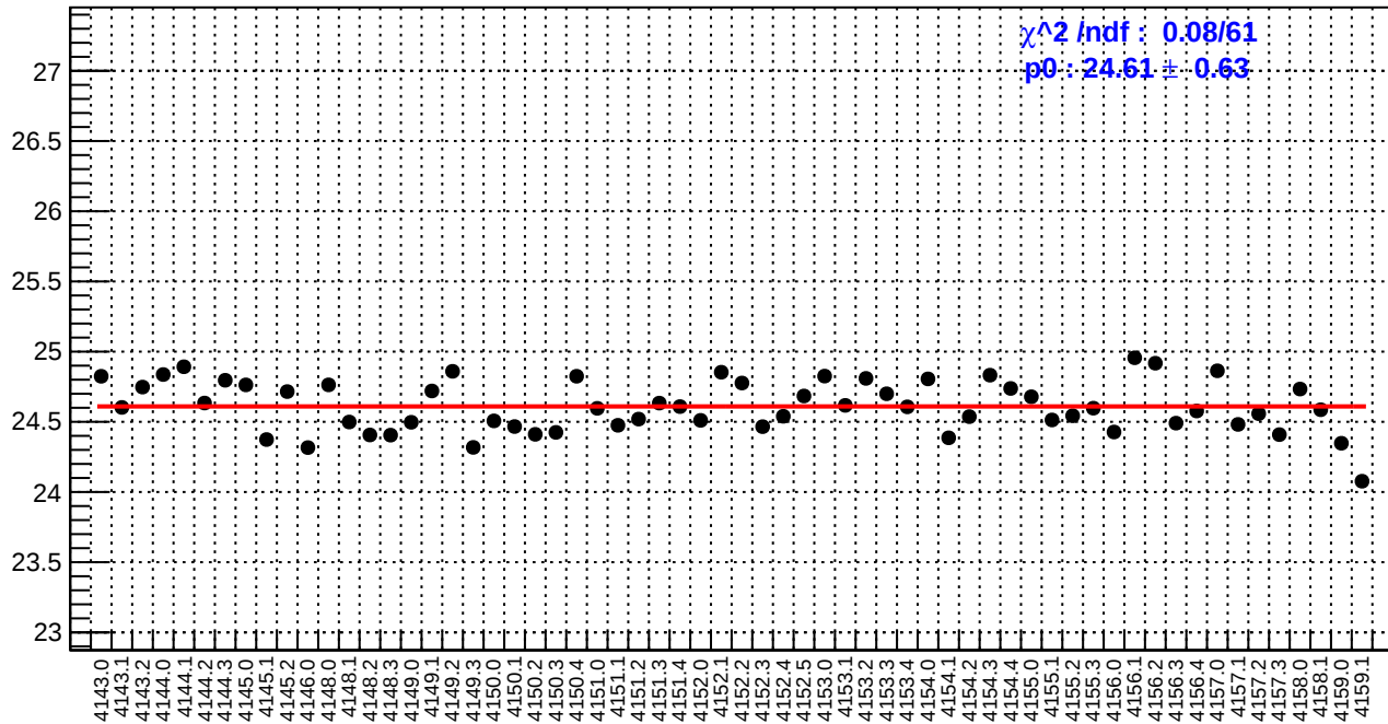
slug45: reg_asym_left_dd.rms/ppm
