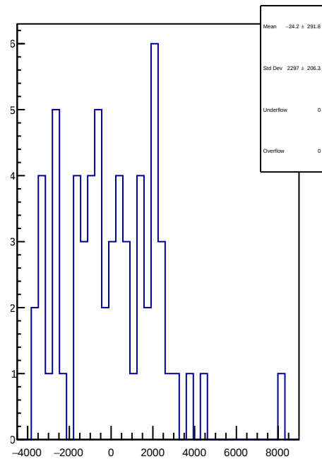
slug45: 1D Corr asym_ds_avg.mean/ppb-reg_asym_ds_avg.mean/ppb
