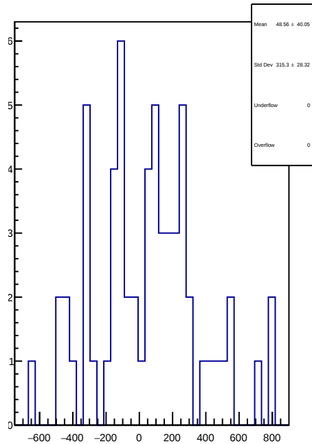
slug45: 1D Corr asym_right_dd.mean/ppb-reg_asym_right_dd.mean/ppb
