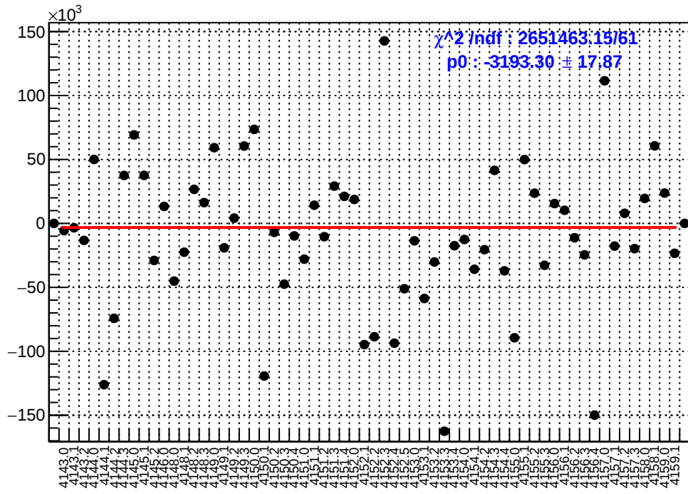
slug45: asym_sam4.mean/ppb-reg_asym_sam4.mean/ppb
