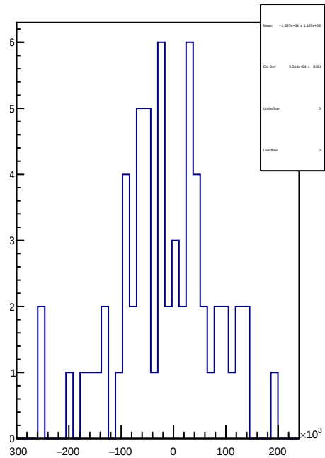
slug45: 1D Corr asym_sam3.mean/ppb-reg_asym_sam3.mean/ppb
