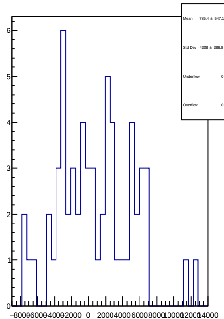
slug45: 1D Corr asym_dsr.mean/ppb-reg_asym_dsr.mean/ppb
