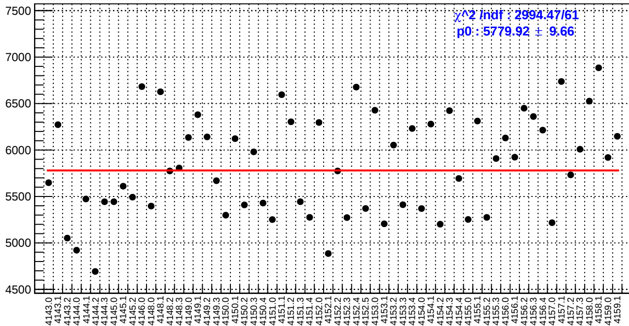
slug45: diff_bpm4eY.rms/nm
