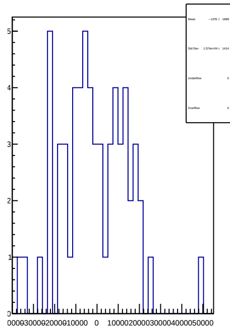
slug45: 1D Corr asym_sam5.mean/ppb-reg_asym_sam5.mean/ppb
