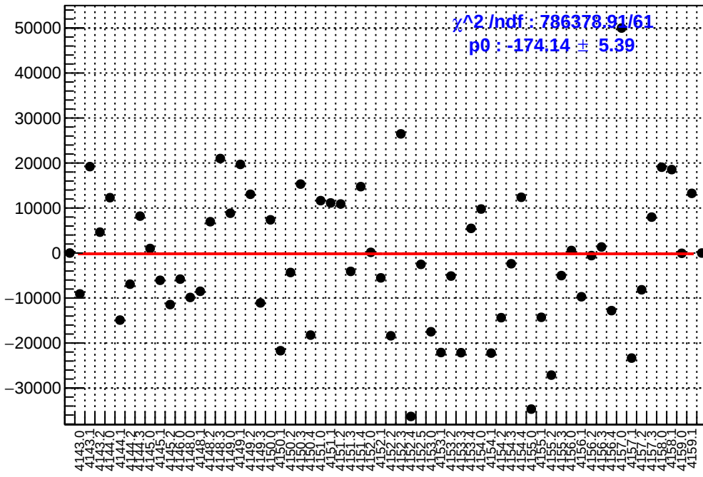
slug45: asym_sam5.mean/ppb-reg_asym_sam5.mean/ppb
