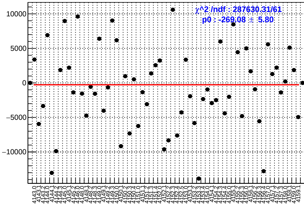
slug45: asym_dsl.mean/ppb-reg_asym_dsl.mean/ppb
