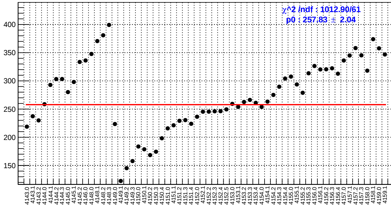
slug45: asym_bcm_an_ds3.rms/ppm
