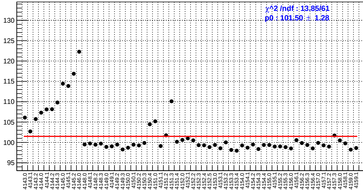
slug45: reg_asym_ds_avg.rms/ppm
