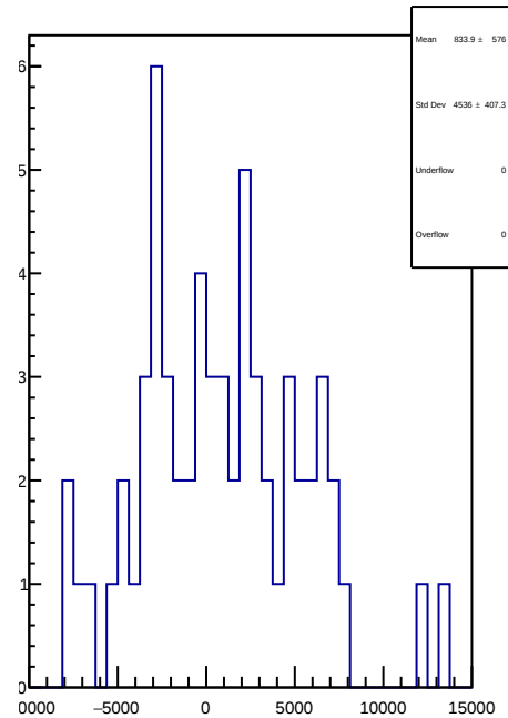
slug45: 1D Corr asym_right_avg.mean/ppb-reg_asym_right_avg.mean/ppb
