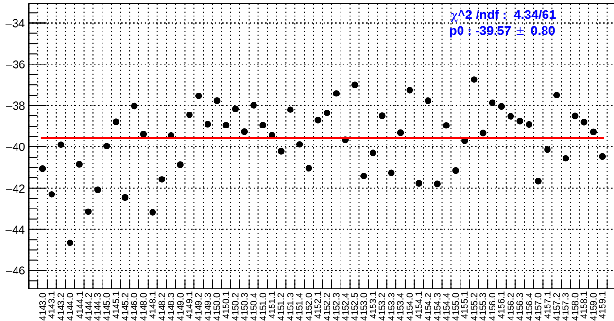
slug45: right_avg_bpm4aX/(ppb/nm)
