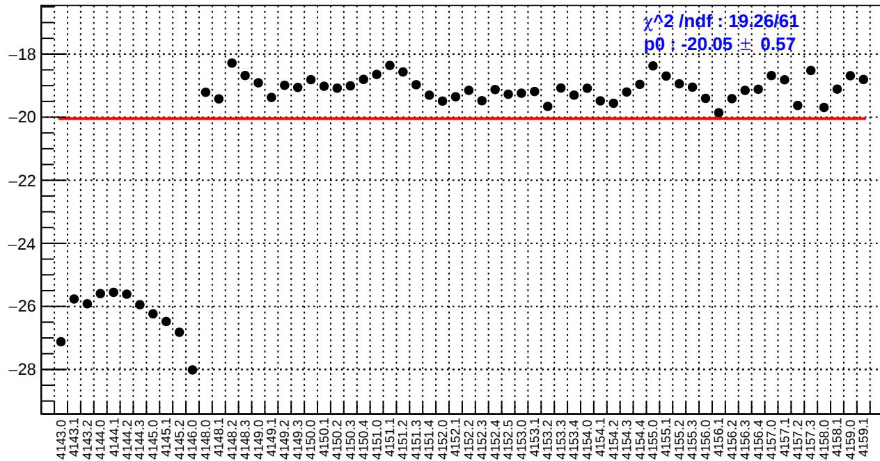
slug45: ds_avg_bpm4eX/(ppb/nm)
