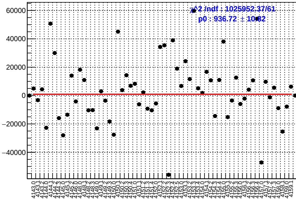
slug45: asym_sam8.mean/ppb-reg_asym_sam8.mean/ppb
