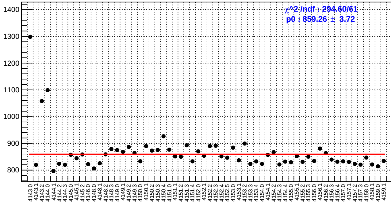
slug45: reg_asym_sam3.rms/ppm
