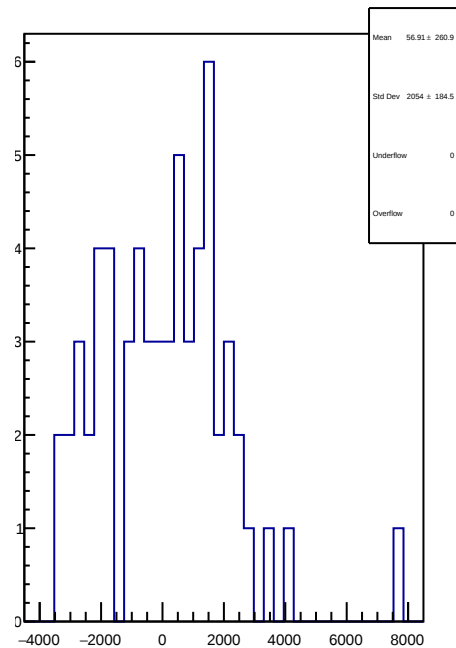
slug45: 1D Corr asym_us_avg.mean/ppb-reg_asym_us_avg.mean/ppb
