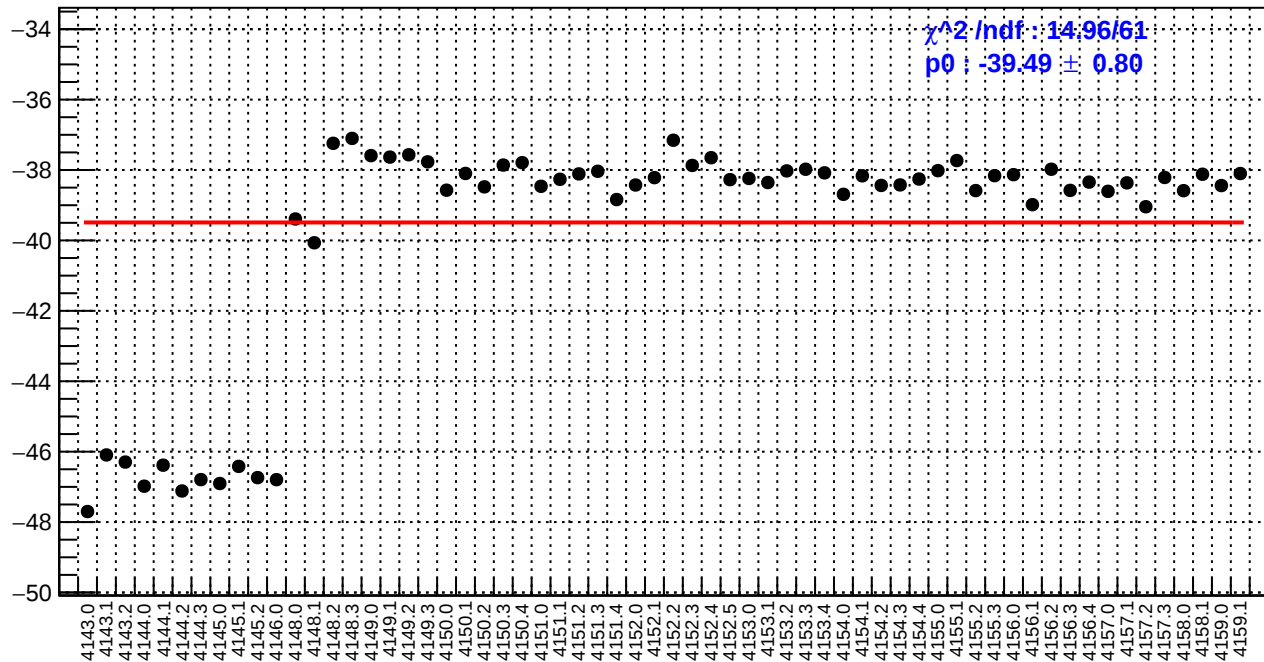
slug45: usl_bpm12X/(ppb/nm)
