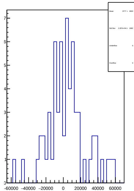
slug45: 1D Corr asym_sam8.mean/ppb-reg_asym_sam8.mean/ppb
