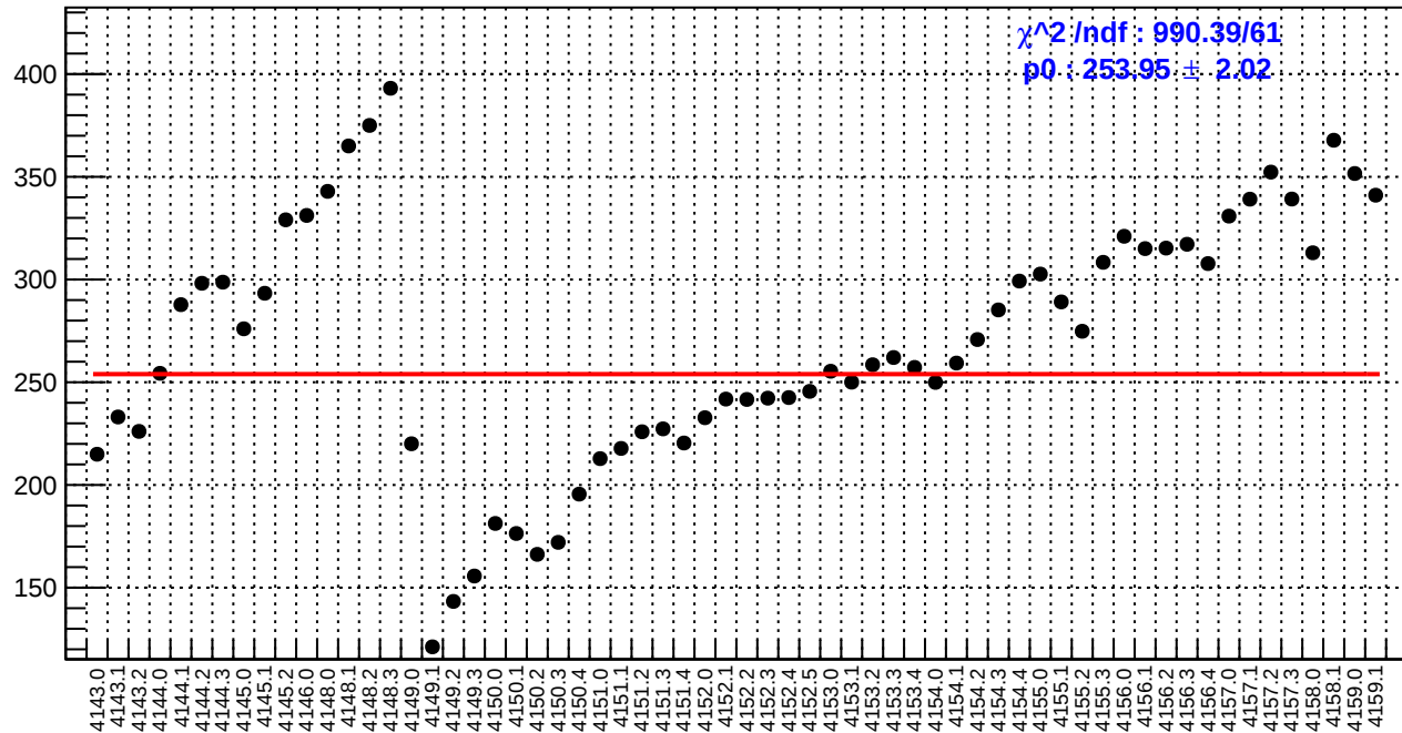
slug45: asym_bcm_an_ds.rms/ppm
