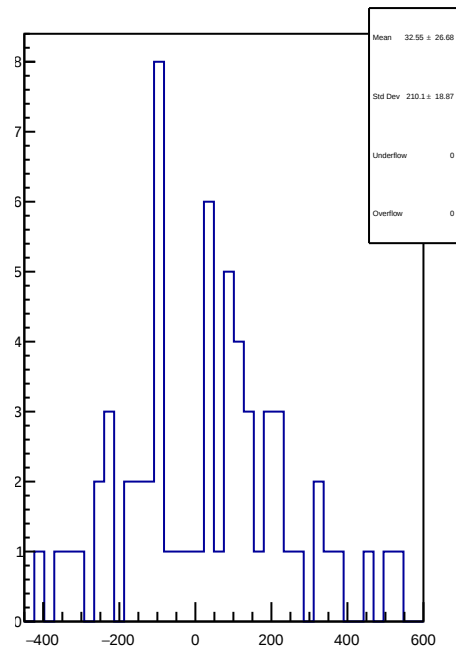
slug45: 1D Corr asym_left_dd.mean/ppb-reg_asym_left_dd.mean/ppb
