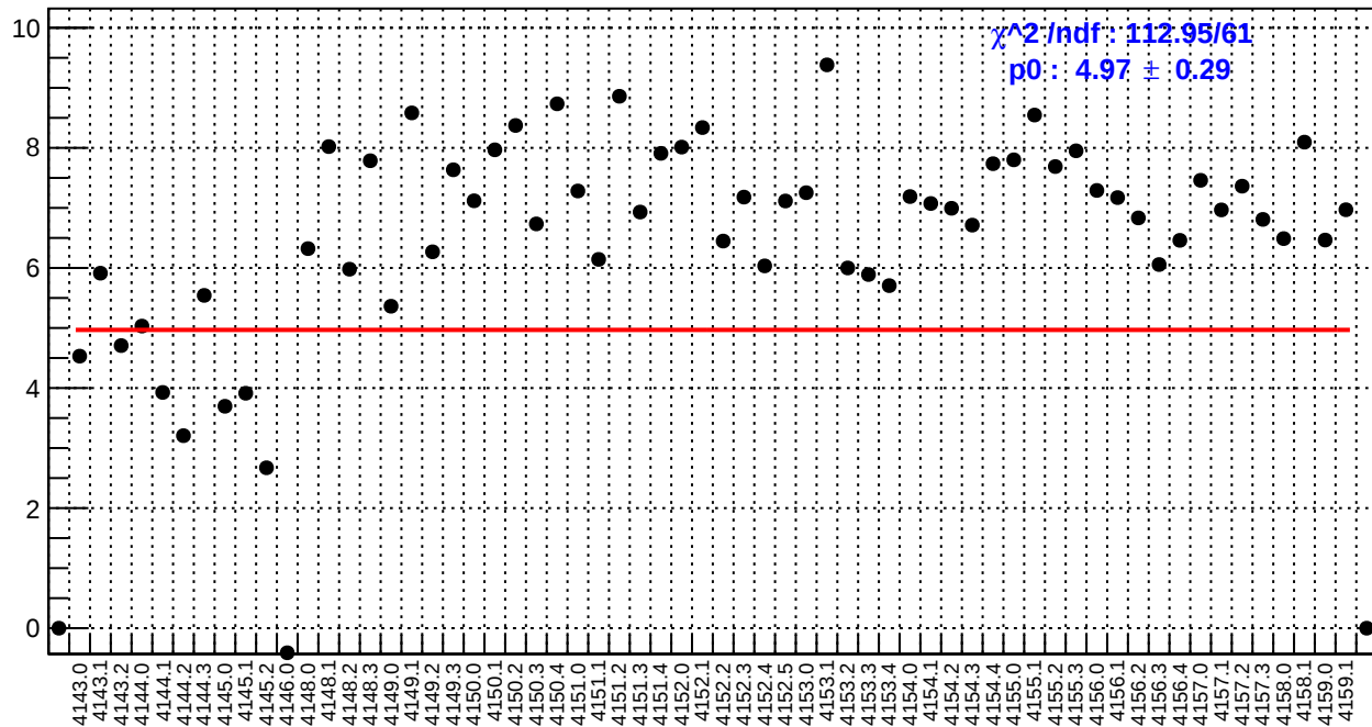
slug45: dsr_bpm4aY/(ppb/nm)
