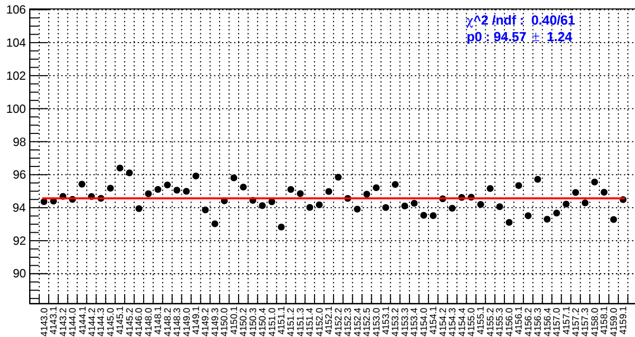
slug45: reg_asym_ds_dd.rms/ppm
