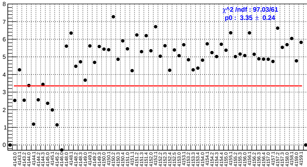
slug45: ds_avg_bpm4aY/(ppb/nm)
