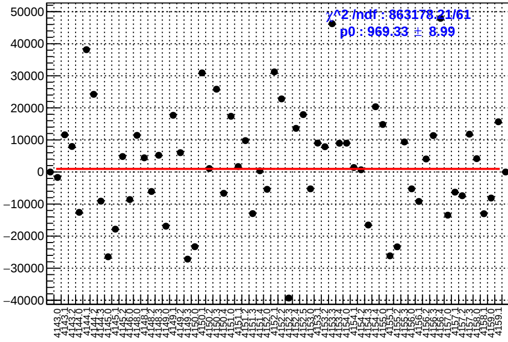
slug45: asym_sam7.mean/ppb-reg_asym_sam7.mean/ppb
