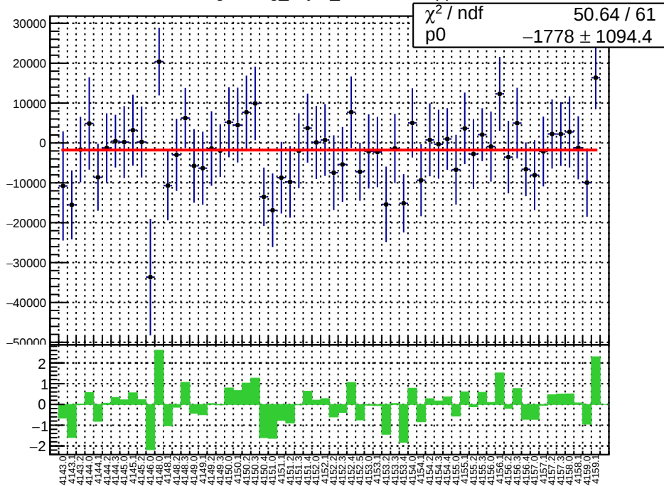
slug45: reg_asym_sam3.mean/ppb
