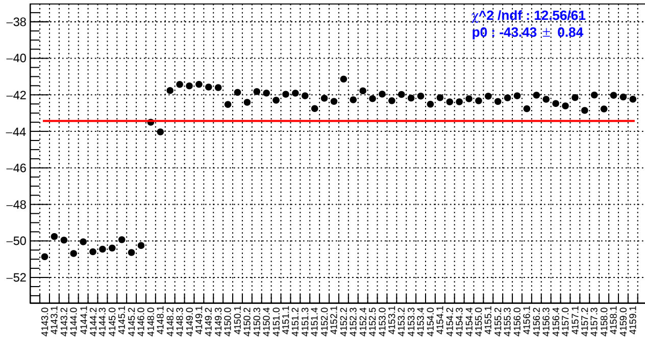
slug45: us_avg_bpm12X/(ppb/nm)
