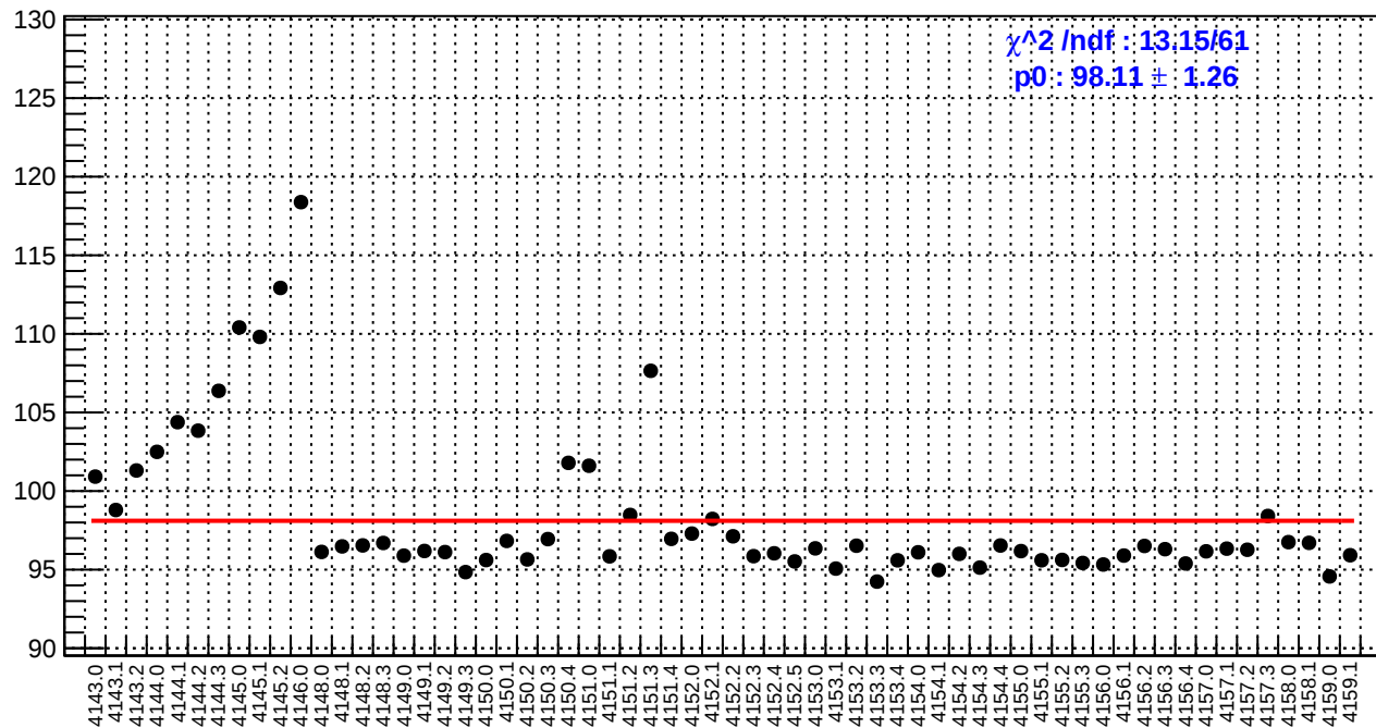
slug45: reg_asym_us_avg.rms/ppm
