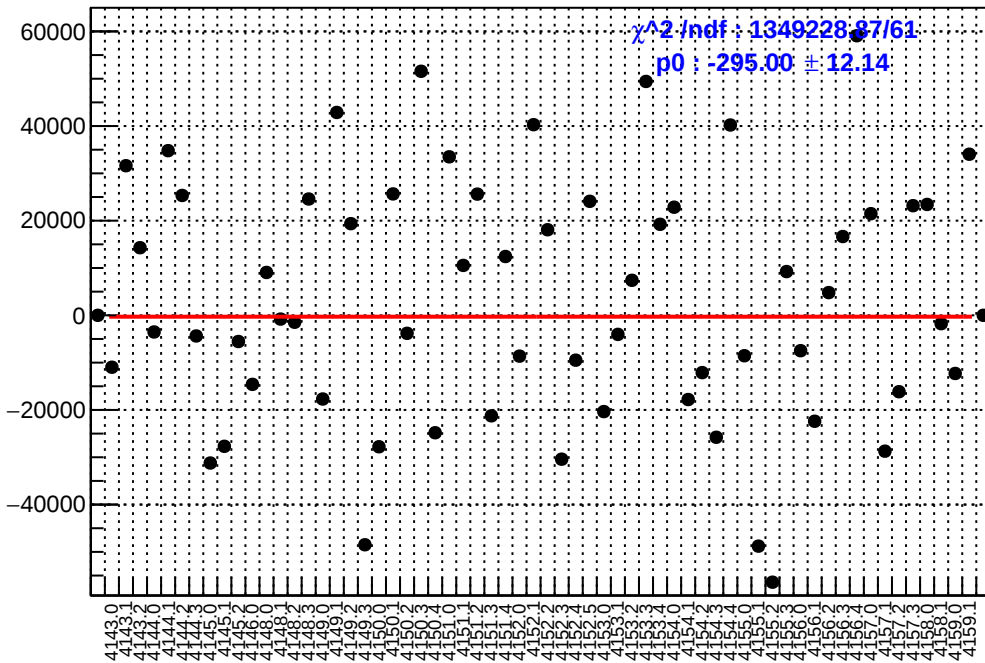
slug45: asym_sam6.mean/ppb-reg_asym_sam6.mean/ppb
