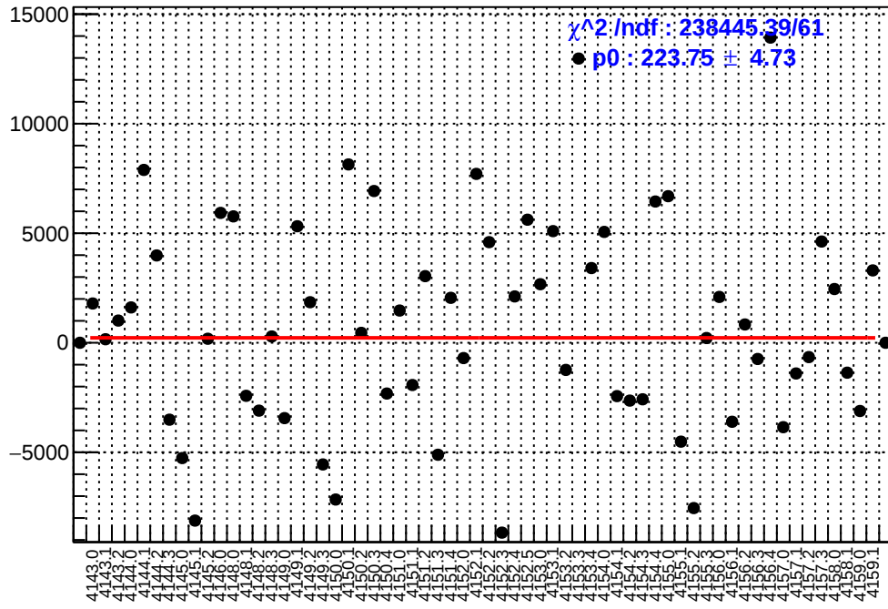
slug45: asym_usr.mean/ppb-reg_asym_usr.mean/ppb
