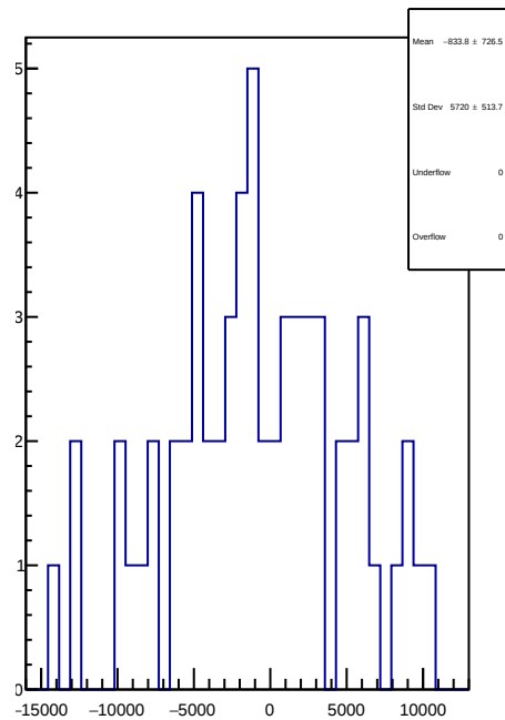
slug45: 1D Corr asym_dsl.mean/ppb-reg_asym_dsl.mean/ppb
