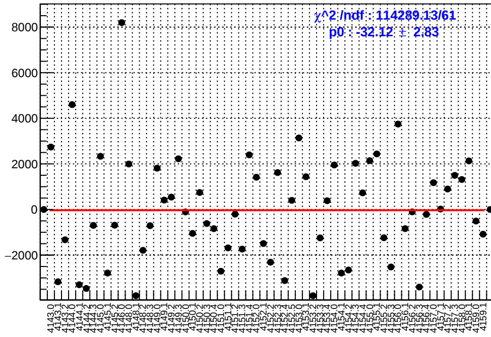
slug45: asym_ds_avg.mean/ppb-reg_asym_ds_avg.mean/ppb
