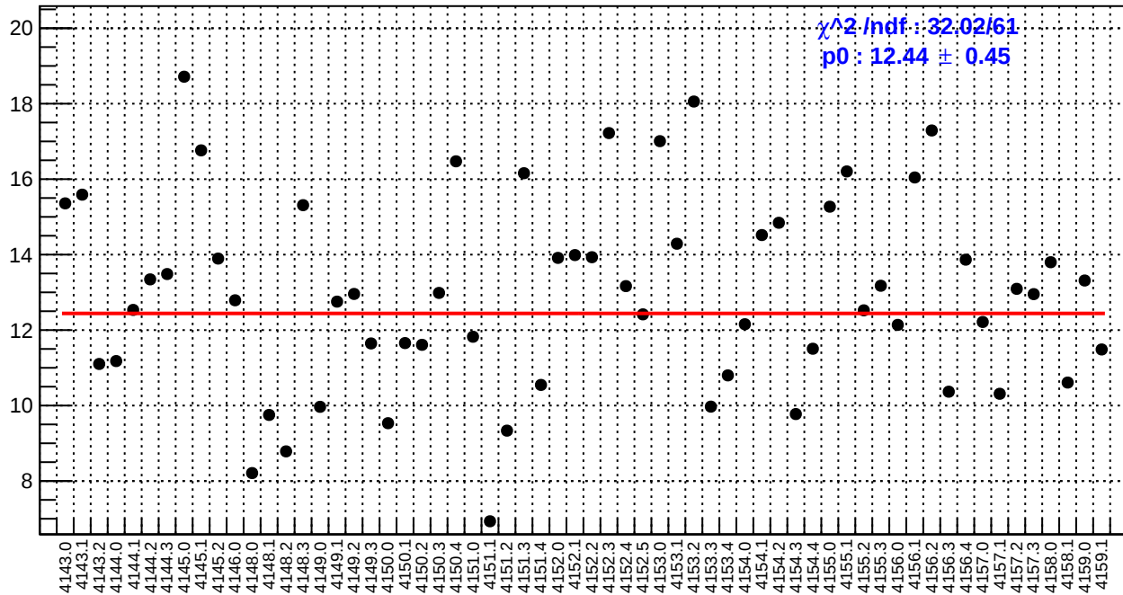
slug45: left_avg_bpm4aX/(ppb/nm)
