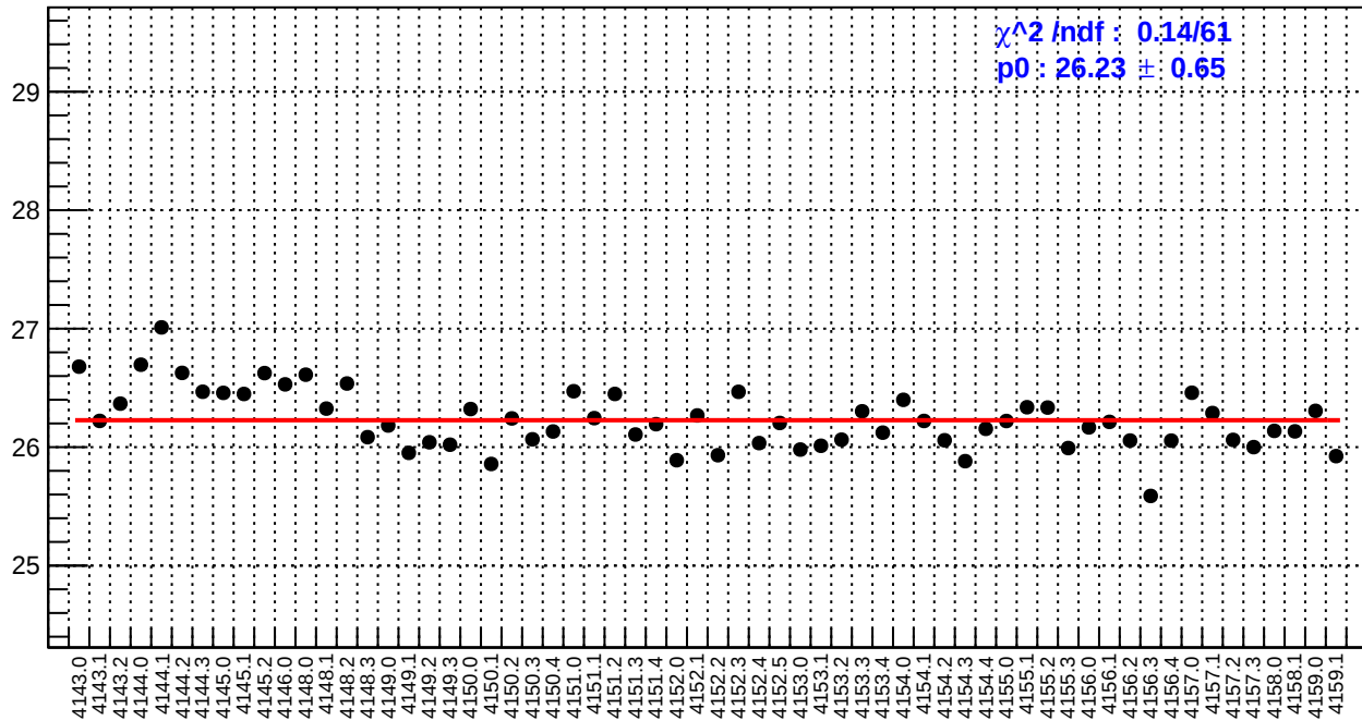
slug45: reg_asym_right_dd.rms/ppm
