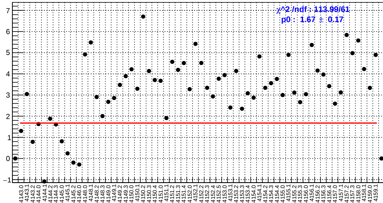
slug45: usl_bpm4aY/(ppb/nm)
