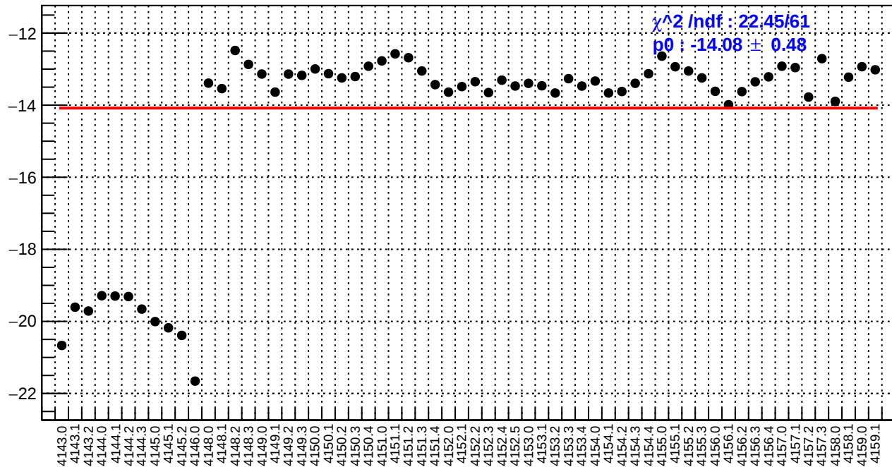
slug45: us_avg_bpm4eX/(ppb/nm)
