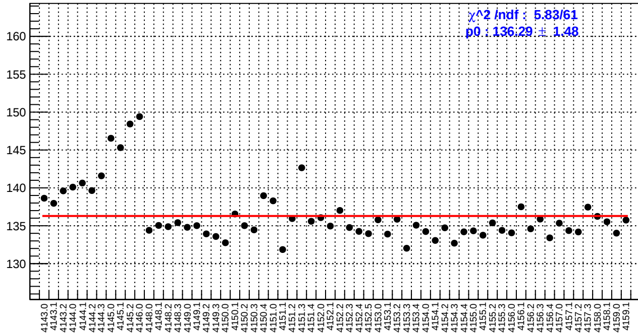
slug45: reg_asym_left_avg.rms/ppm
