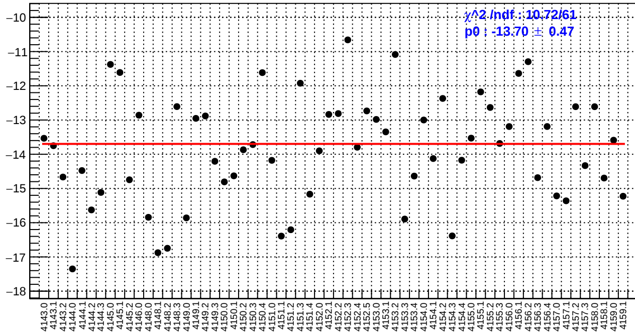
slug45: us_avg_bpm4aX/(ppb/nm)
