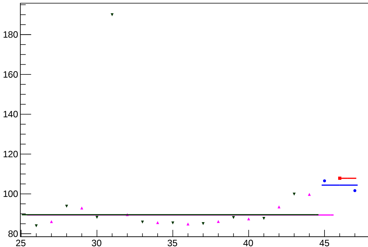
reg_asym_atr1l2_dd_diff_bpm11X_slope vs slug
