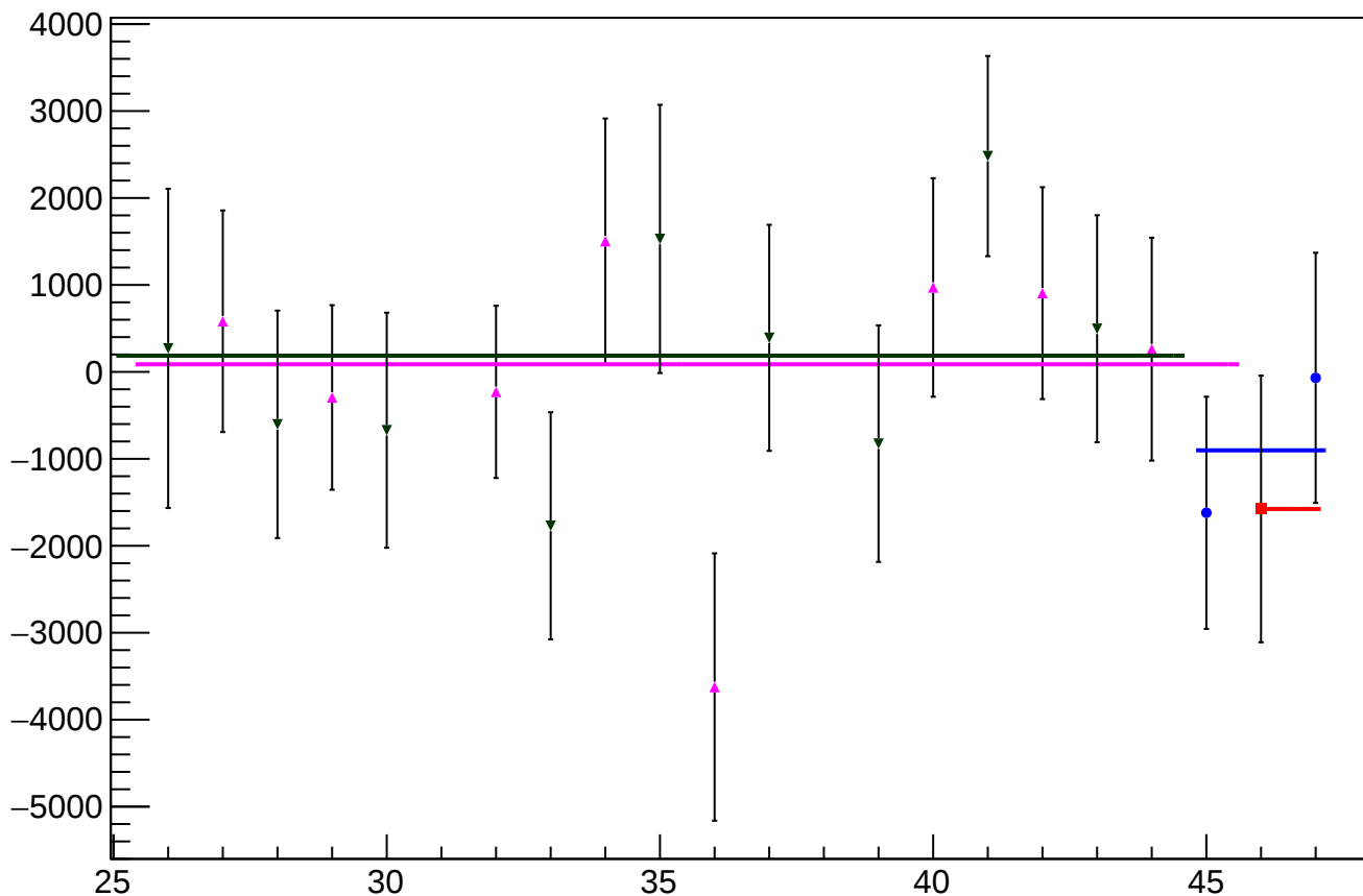
asym_atr_dd_mean vs slug
