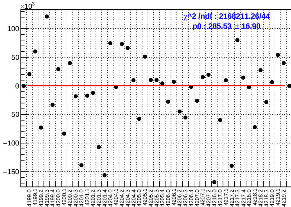
slug48: asym_sam2.mean/ppb-reg_asym_sam2.mean/ppb
