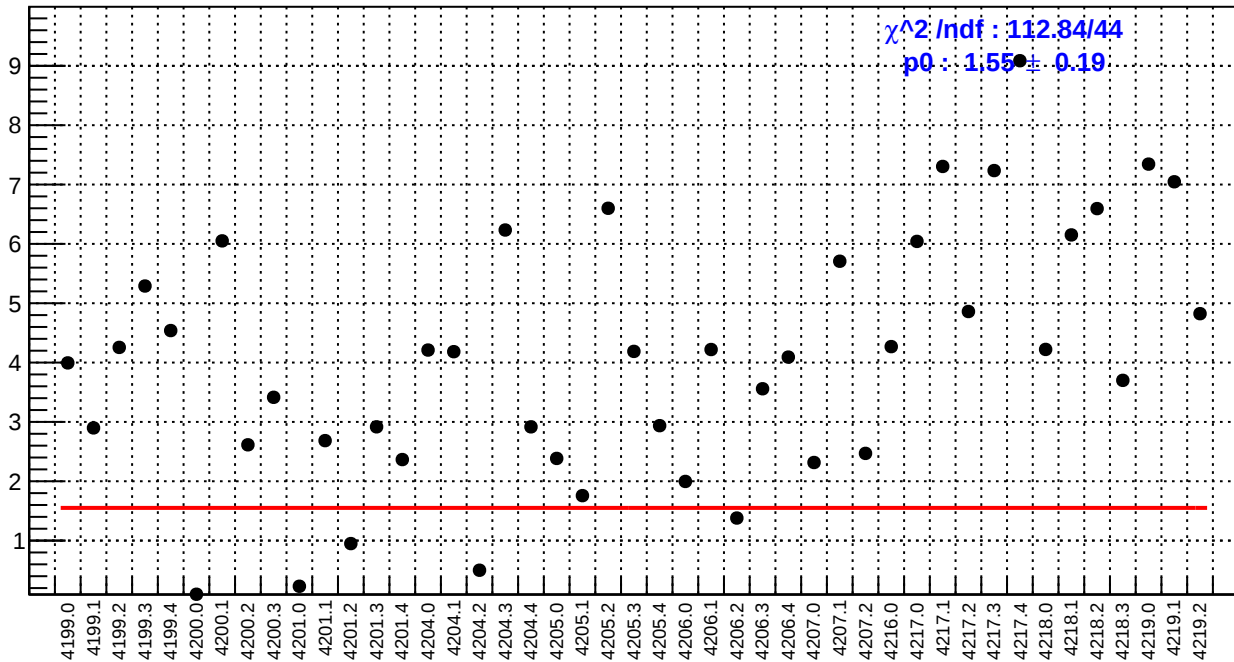
slug48: us_avg_bpm4eY/(ppb/nm)
