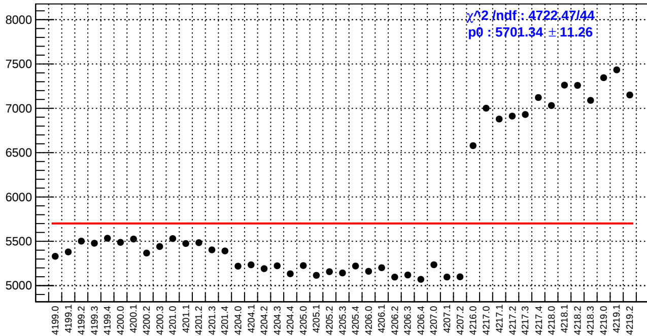
slug48: diff_bpm11X.rms/nm
