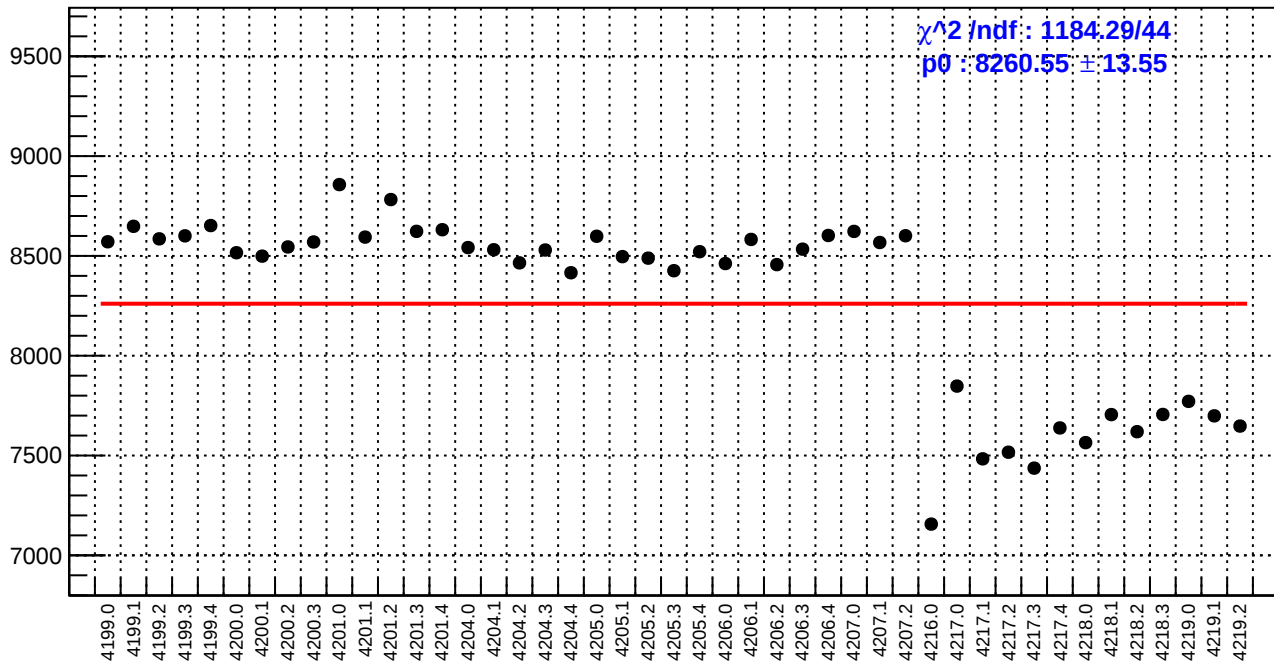
slug48: diff_bpm4eX.rms/nm
