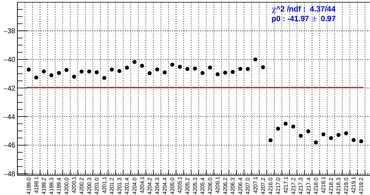
slug48: left_avg_bpm12X/(ppb/nm)
