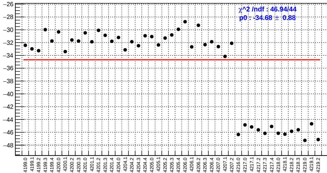
slug48: usr_bpm4aX/(ppb/nm)
