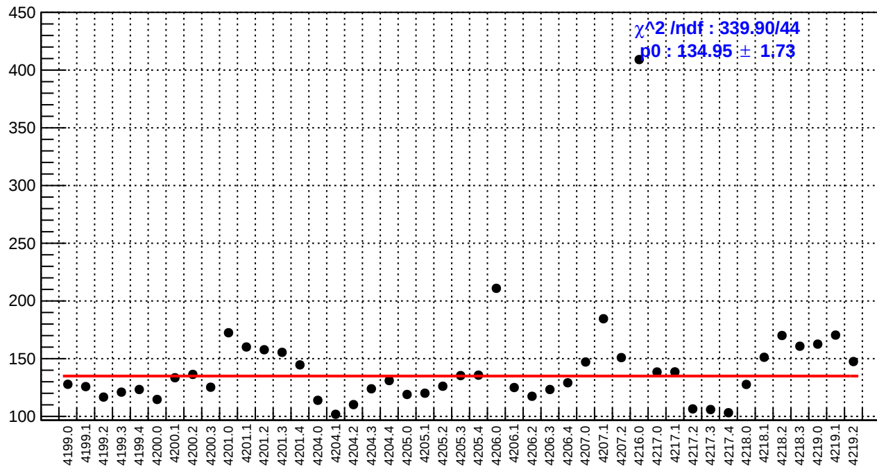
slug48: asym_bcm_an_us.rms/ppm
