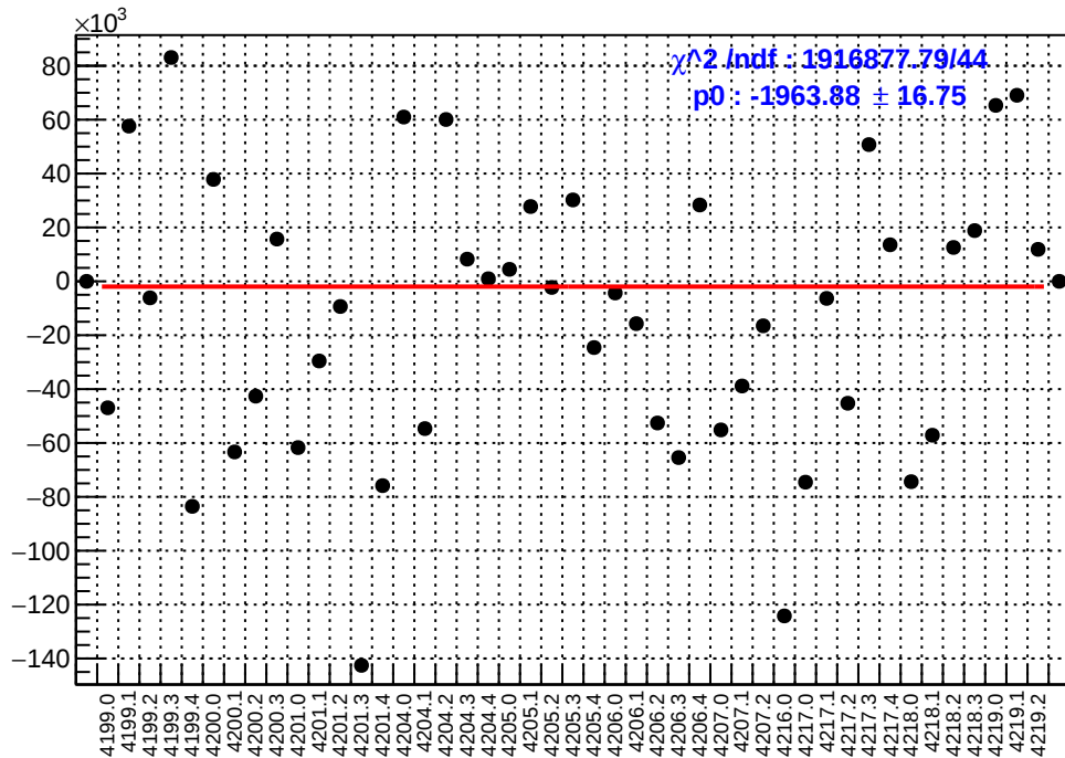
slug48: asym_sam4.mean/ppb-reg_asym_sam4.mean/ppb
