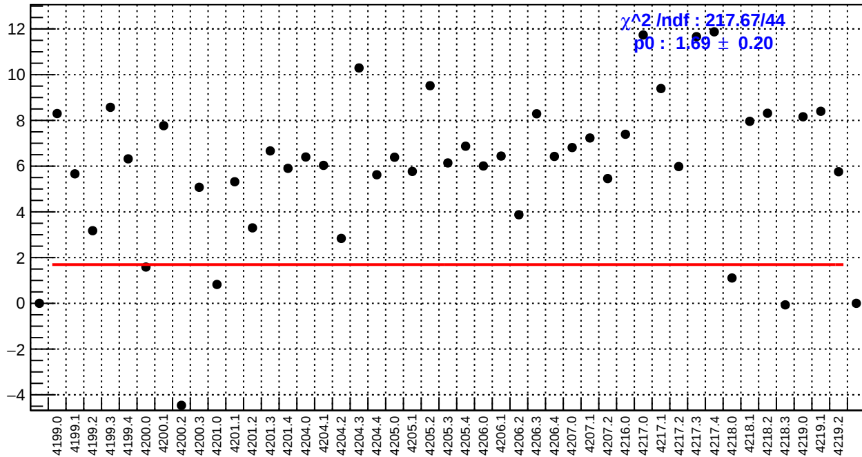
slug48: dsl_bpm4eY/(ppb/nm)
