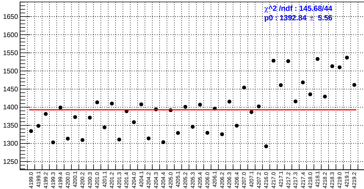
slug48: diff_bpm4aX.rms/nm
