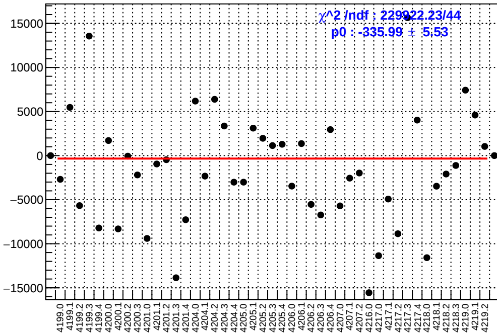
slug48: asym_left_avg.mean/ppb-reg_asym_left_avg.mean/ppb
