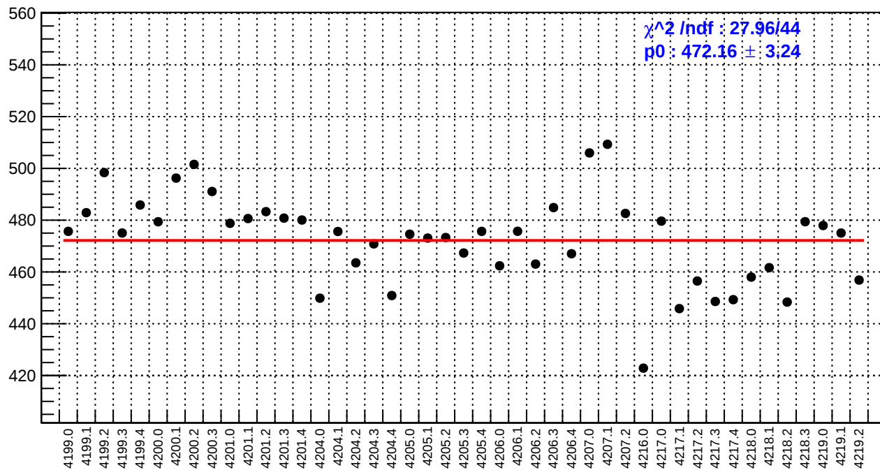
slug48: reg_asym_sam6.rms/ppm
