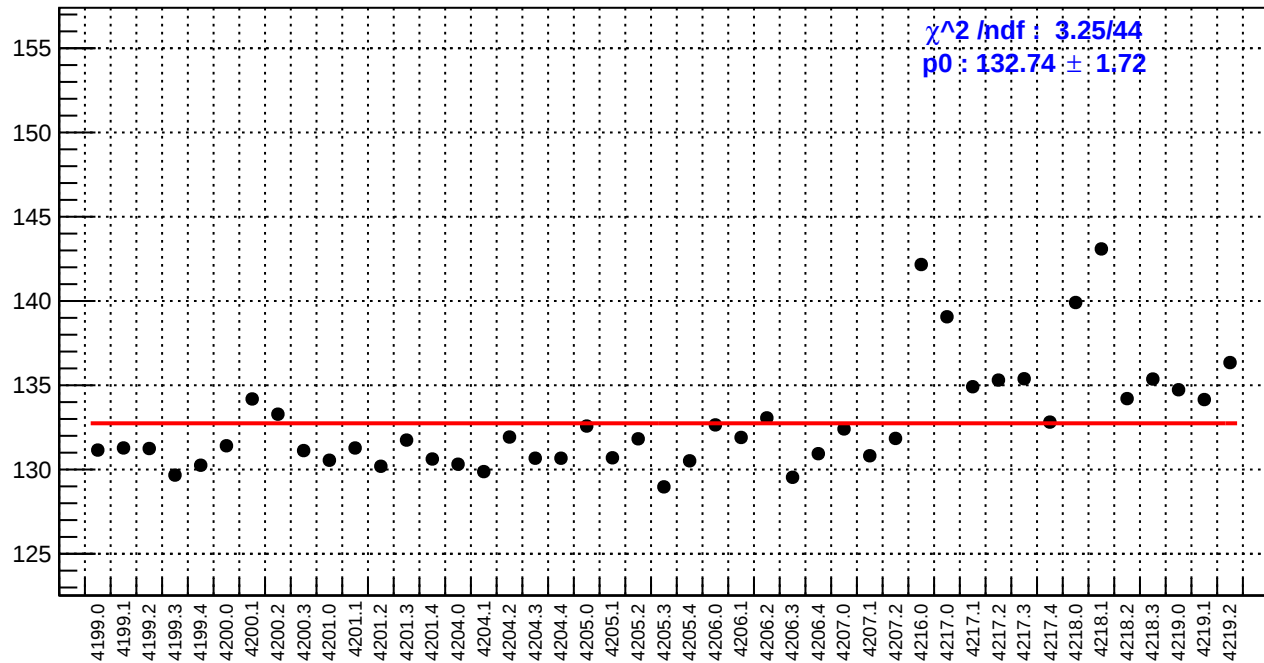
slug48: reg_asym_usr.rms/ppm
