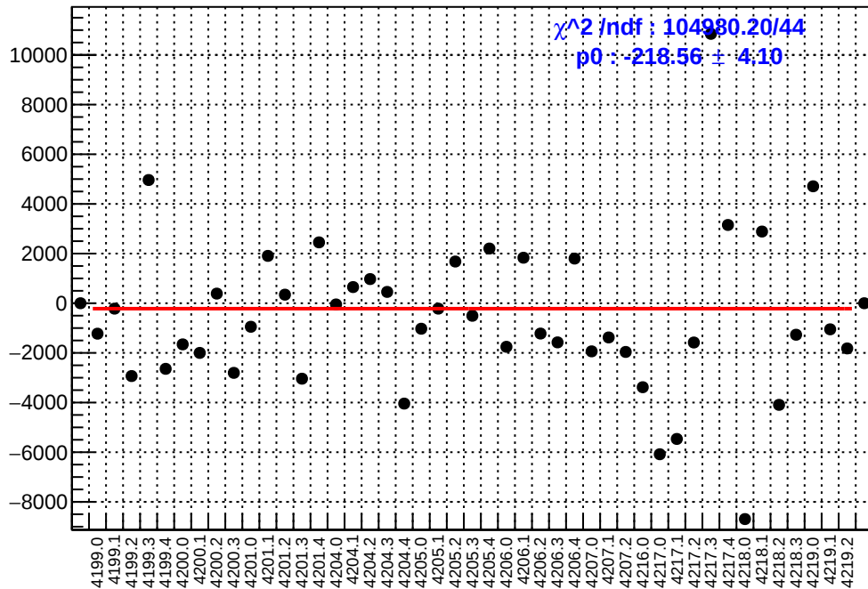
slug48: asym_us_avg.mean/ppb-reg_asym_us_avg.mean/ppb
