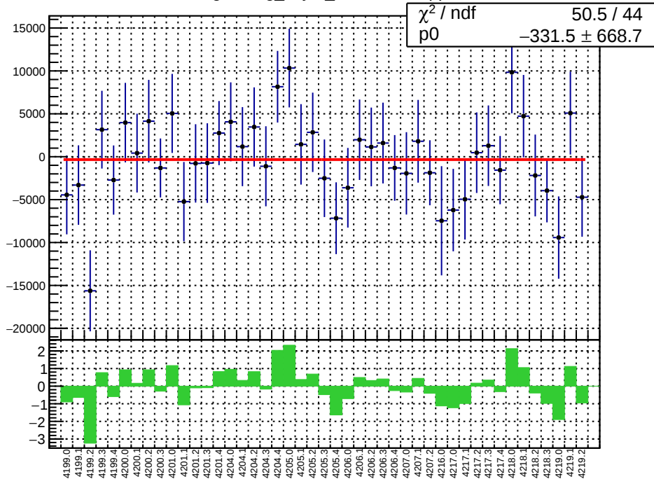
slug48: reg_asym_sam8.mean/ppb
