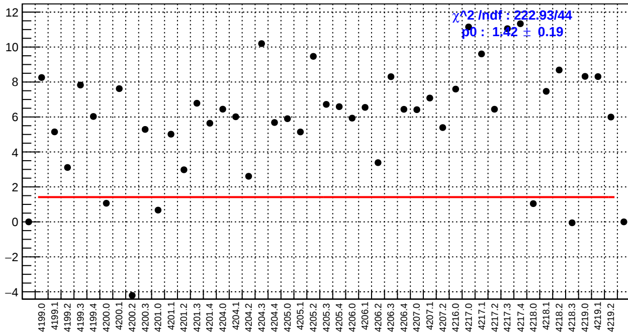
slug48: left_avg_bpm4eY/(ppb/nm)
