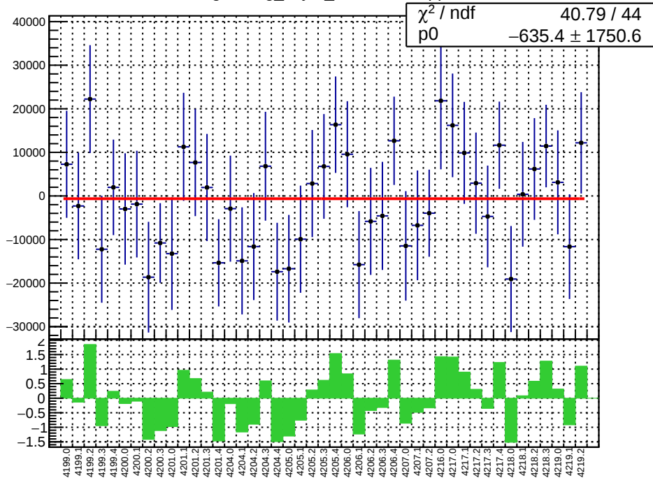
slug48: reg_asym_sam4.mean/ppb
