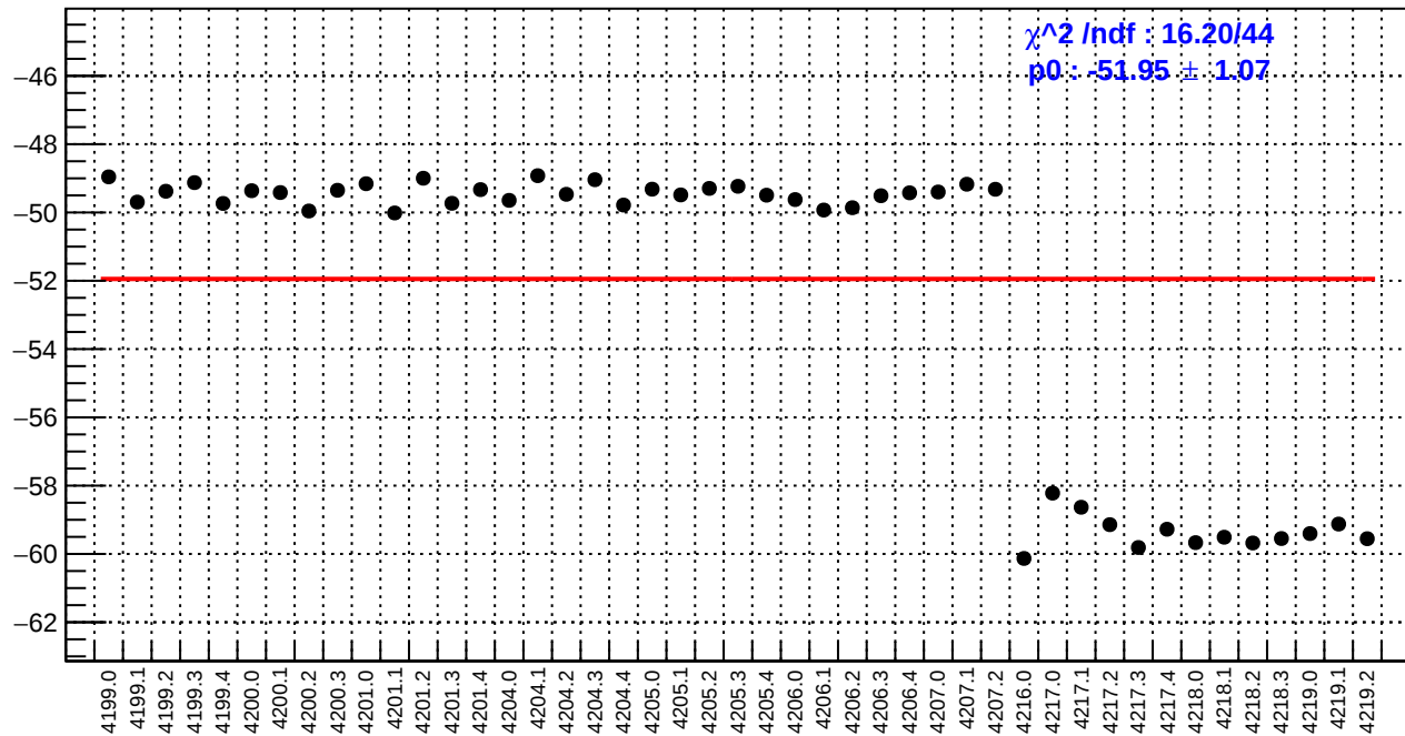
slug48: right_avg_bpm12X/(ppb/nm)
