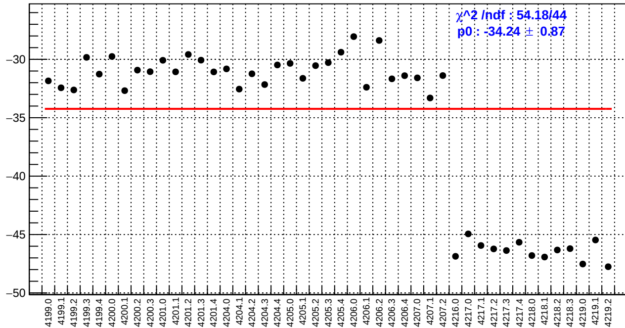
slug48: right_avg_bpm4aX/(ppb/nm)
