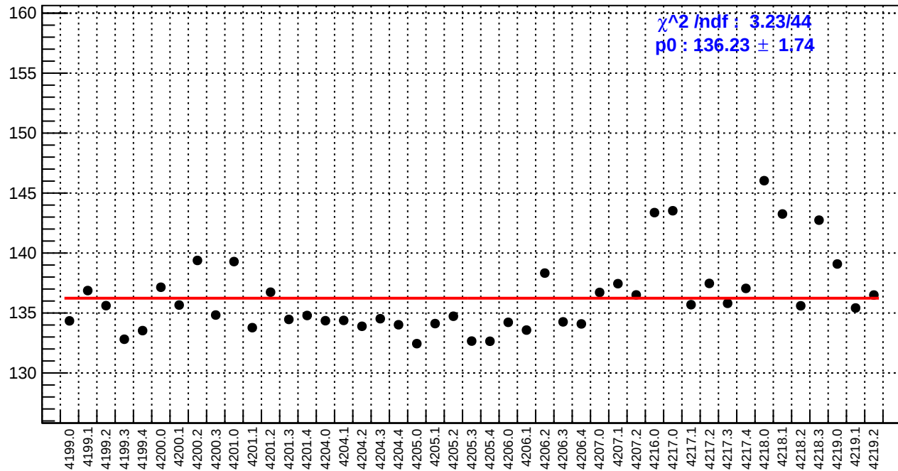
slug48: reg_asym_left_avg.rms/ppm
