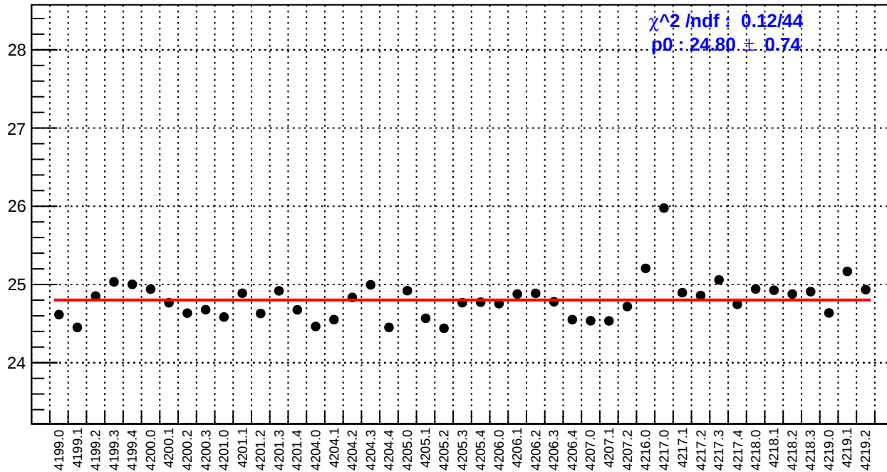
slug48: reg_asym_left_dd.rms/ppm
