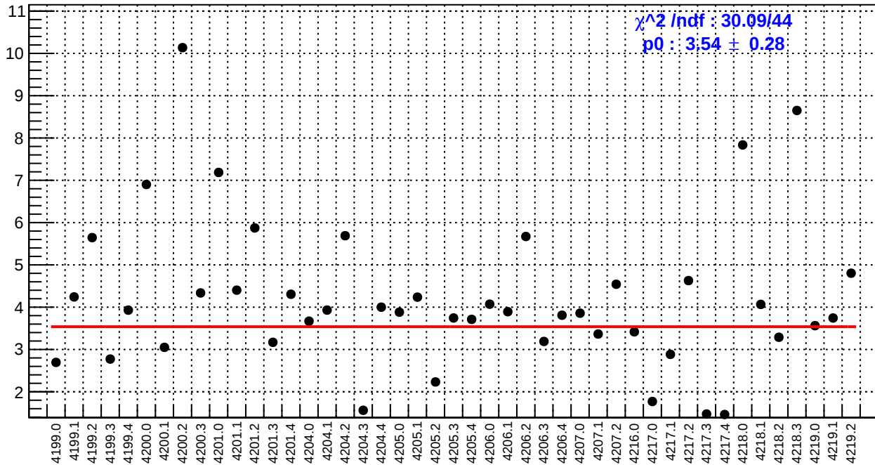
slug48: left_avg_bpm4aY/(ppb/nm)
