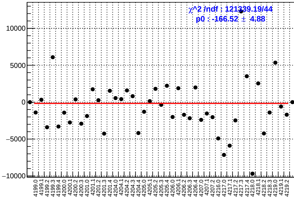
slug48: asym_ds_avg.mean/ppb-reg_asym_ds_avg.mean/ppb
