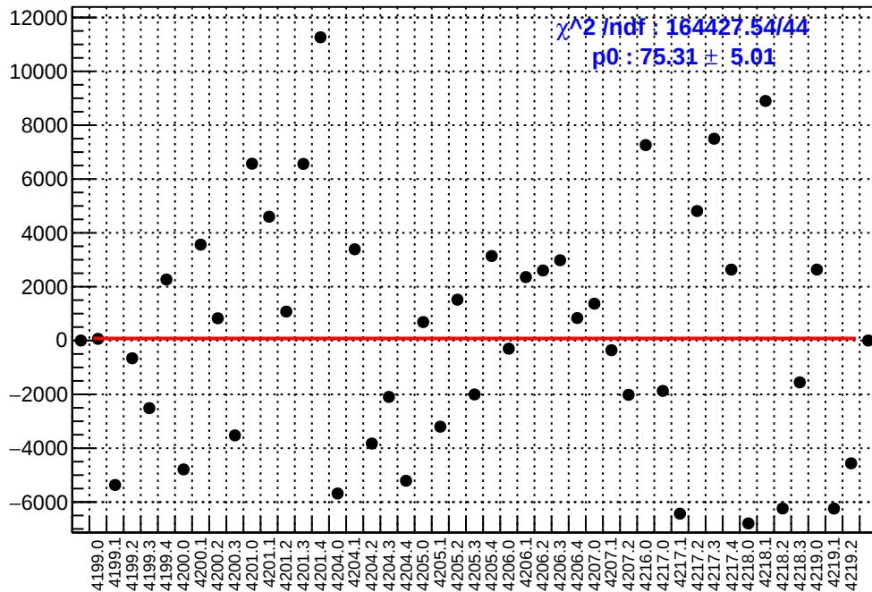
slug48: asym_right_avg.mean/ppb-reg_asym_right_avg.mean/ppb
