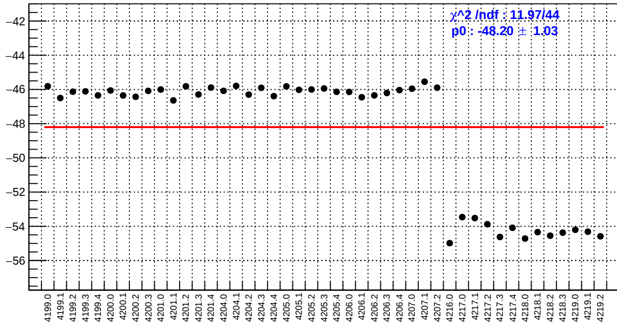
slug48: ds_avg_bpm12X/(ppb/nm)
