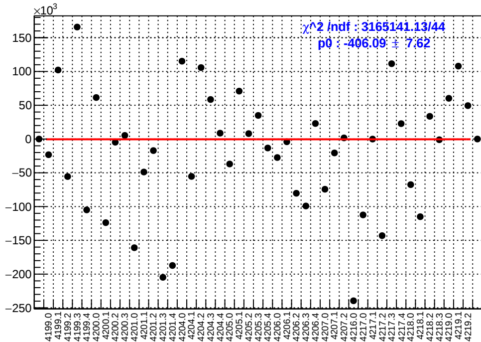
slug48: asym_sam3.mean/ppb-reg_asym_sam3.mean/ppb
