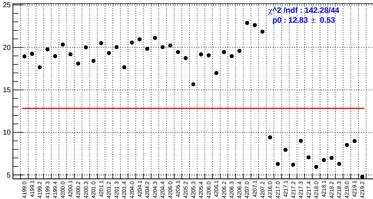
slug48: left_avg_bpm4aX/(ppb/nm)
