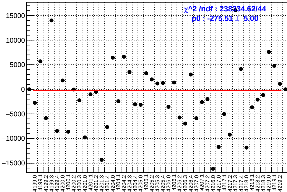
slug48: asym_dsl.mean/ppb-reg_asym_dsl.mean/ppb
