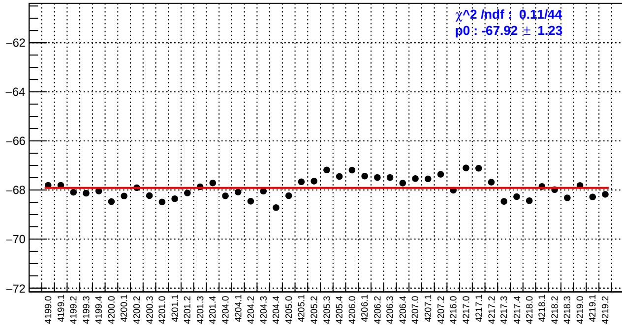
slug48: left_avg_bpm4eX/(ppb/nm)
