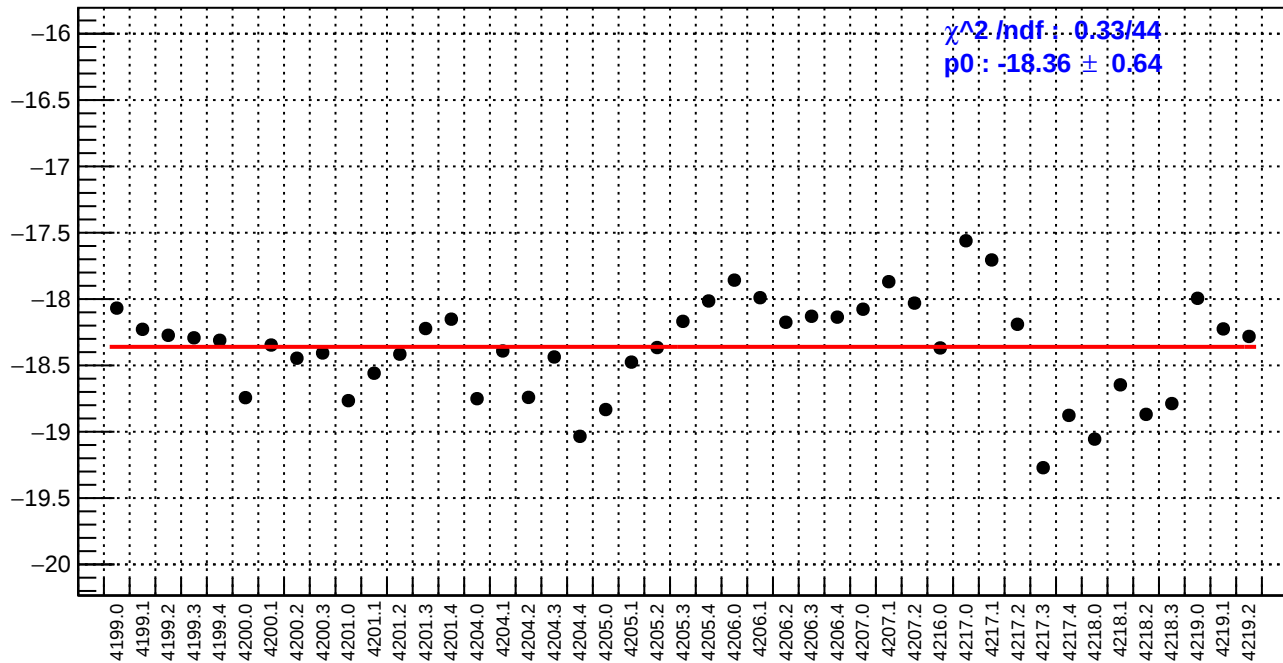
slug48: us_avg_bpm4eX/(ppb/nm)
