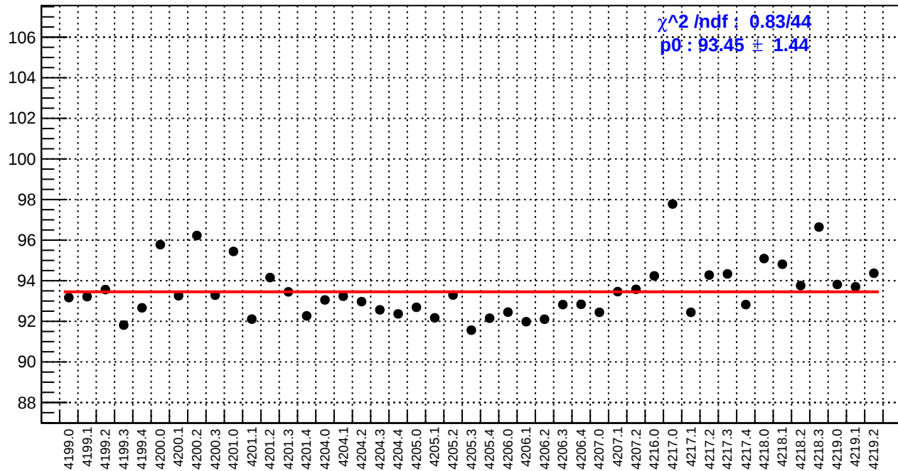
slug48: reg_asym_us_dd.rms/ppm
