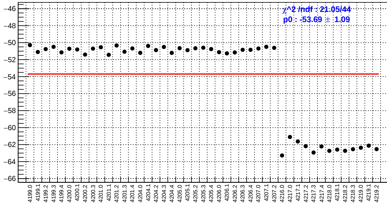
slug48: dsr_bpm12X/(ppb/nm)
