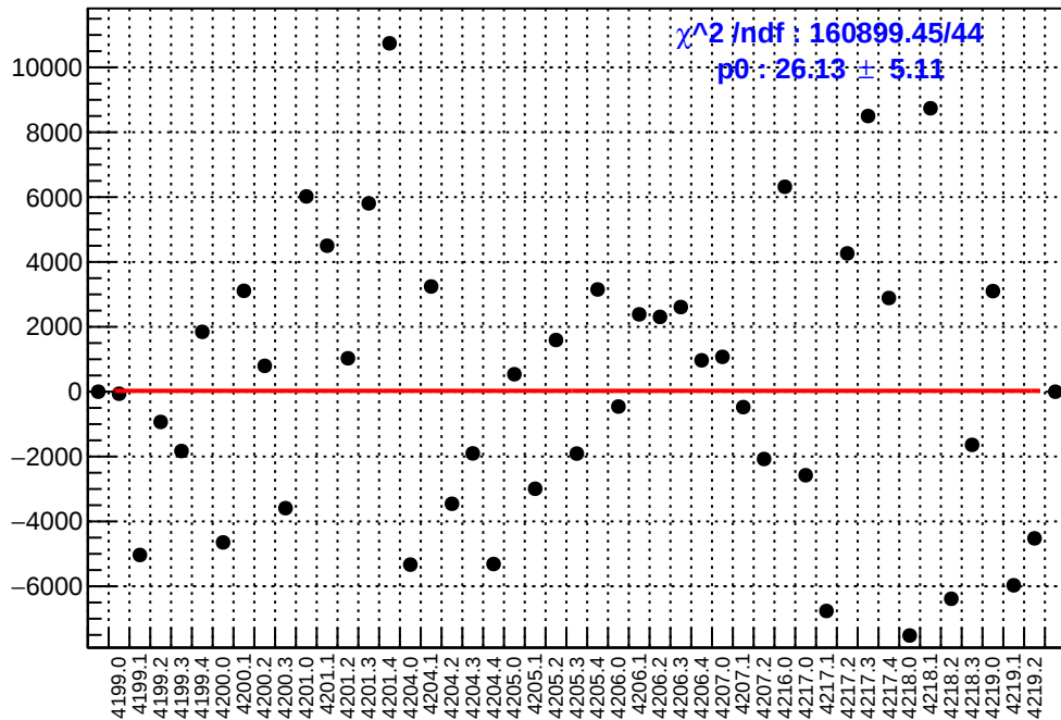
slug48: asym_dsr.mean/ppb-reg_asym_dsr.mean/ppb
