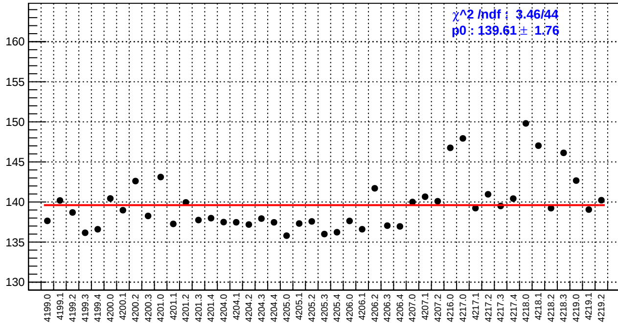
slug48: reg_asym_dsl.rms/ppm
