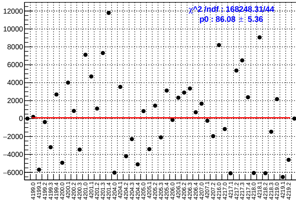
slug48: asym_usr.mean/ppb-reg_asym_usr.mean/ppb
