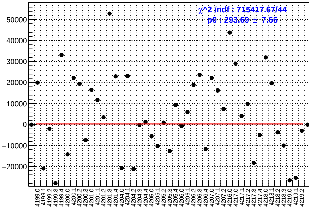
slug48: asym_sam8.mean/ppb-reg_asym_sam8.mean/ppb
