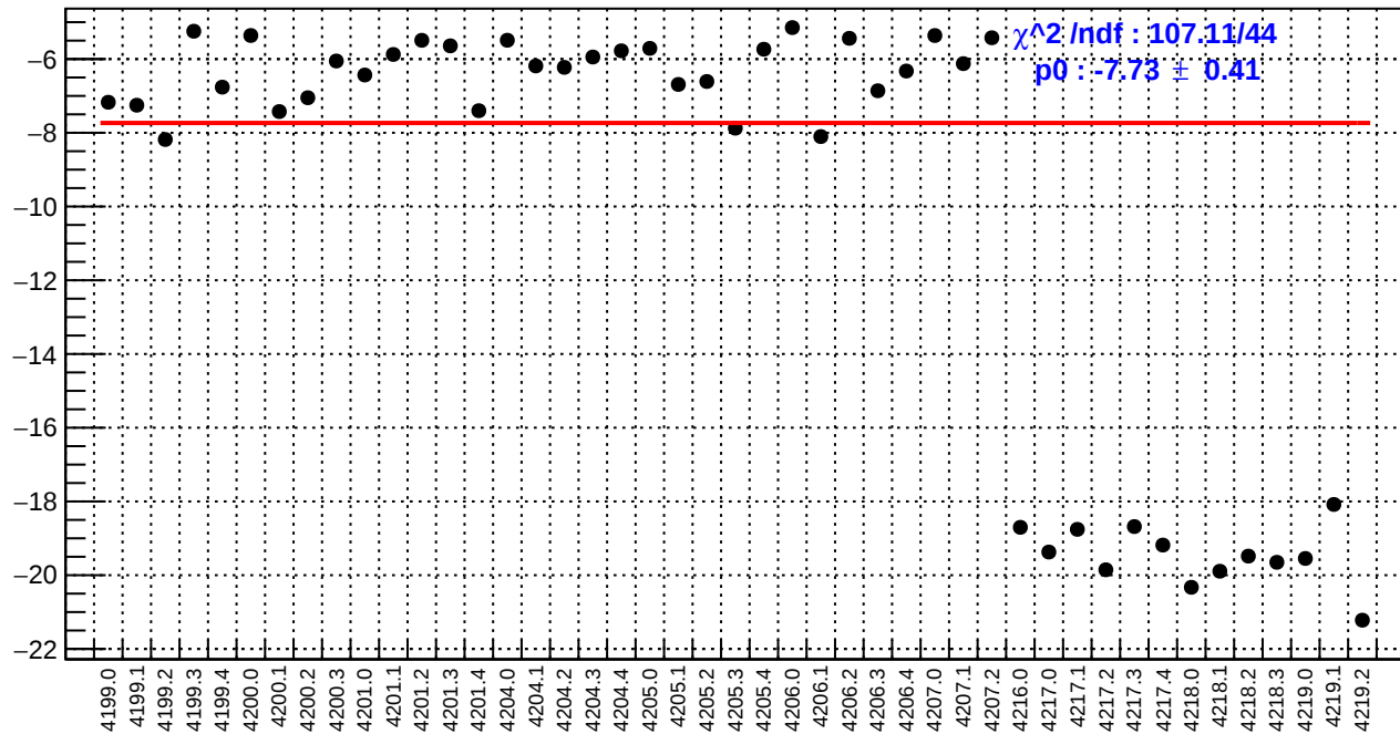
slug48: us_avg_bpm4aX/(ppb/nm)
