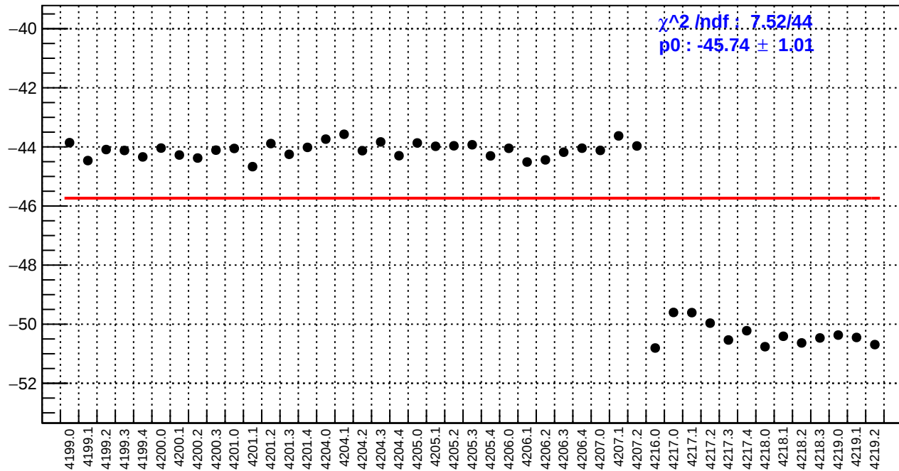
slug48: us_avg_bpm12X/(ppb/nm)
