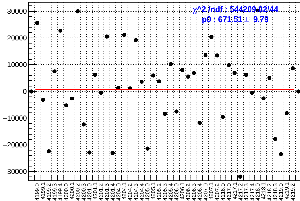
slug48: asym_sam1.mean/ppb-reg_asym_sam1.mean/ppb
