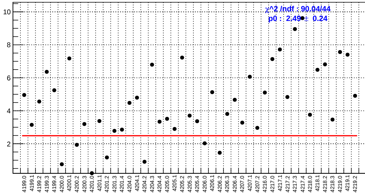
slug48: ds_avg_bpm4eY/(ppb/nm)
