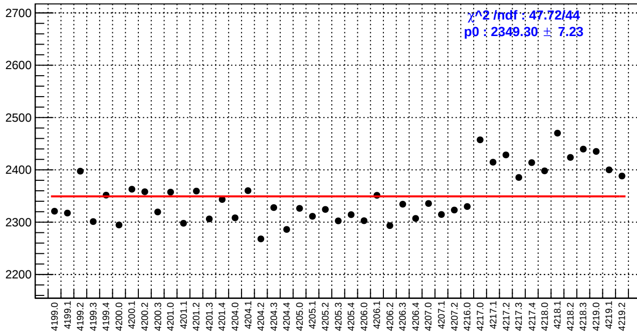
slug48: reg_asym_sam2.rms/ppm
