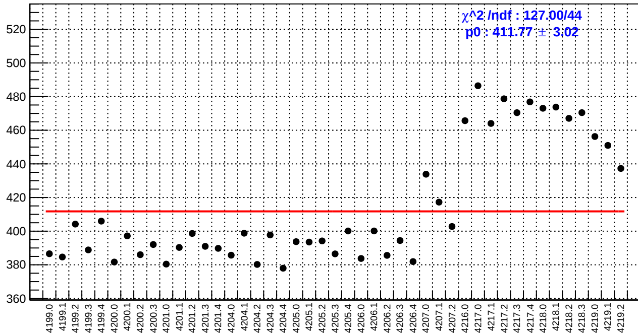
slug48: reg_asym_sam1.rms/ppm
