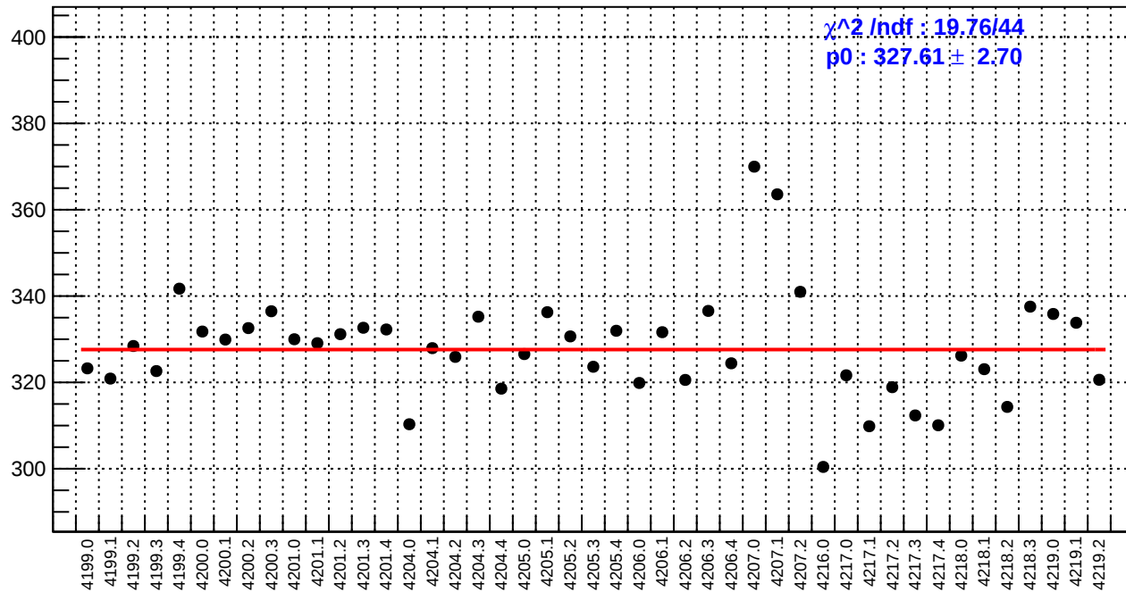
slug48: reg_asym_sam5.rms/ppm
