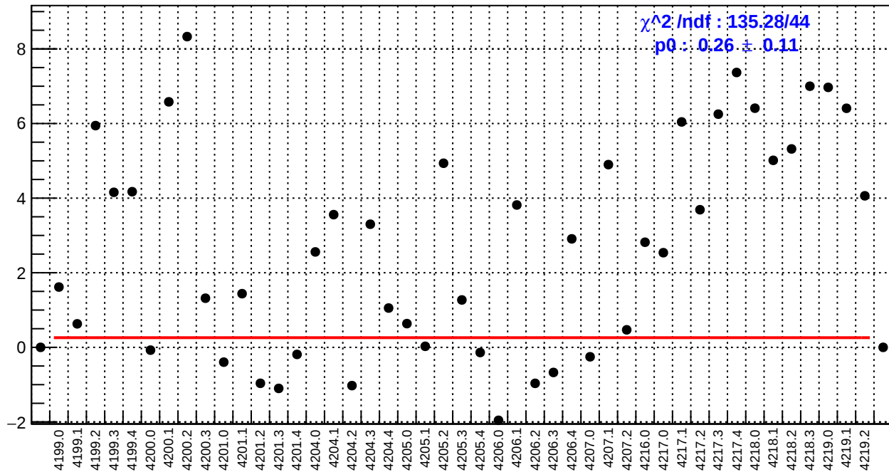
slug48: dsr_bpm4eY/(ppb/nm)
