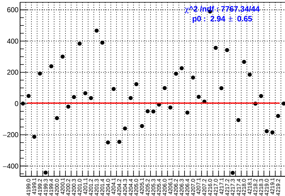
slug48: asym_left_dd.mean/ppb-reg_asym_left_dd.mean/ppb
