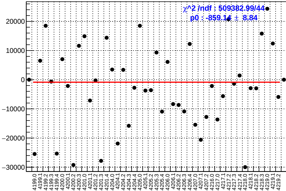
slug48: asym_sam5.mean/ppb-reg_asym_sam5.mean/ppb
