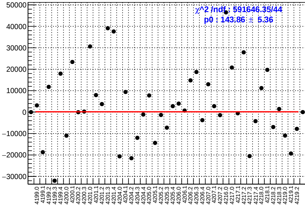
slug48: asym_sam7.mean/ppb-reg_asym_sam7.mean/ppb
