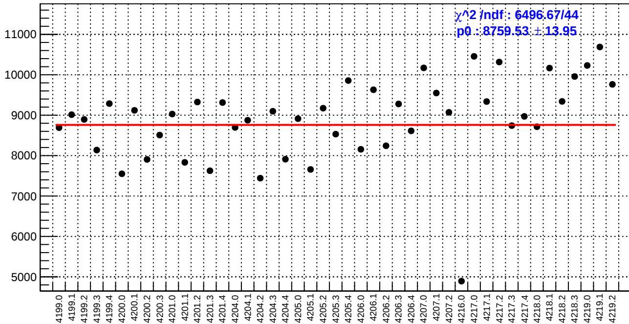
slug48: diff_bpm4aY.rms/nm
