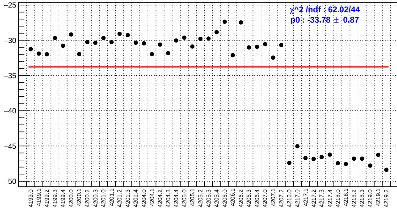
slug48: dsr_bpm4aX/(ppb/nm)
