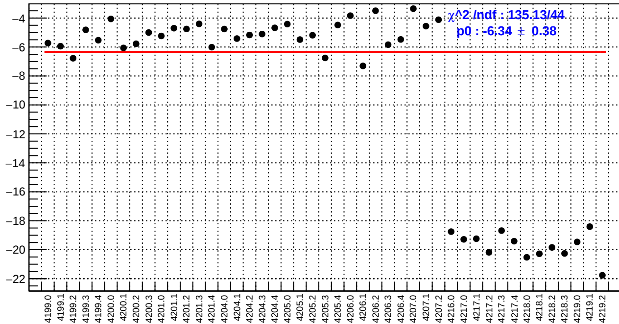
slug48: ds_avg_bpm4aX/(ppb/nm)
