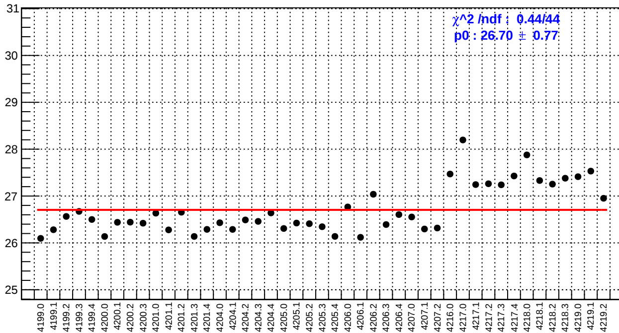
slug48: reg_asym_right_dd.rms/ppm
