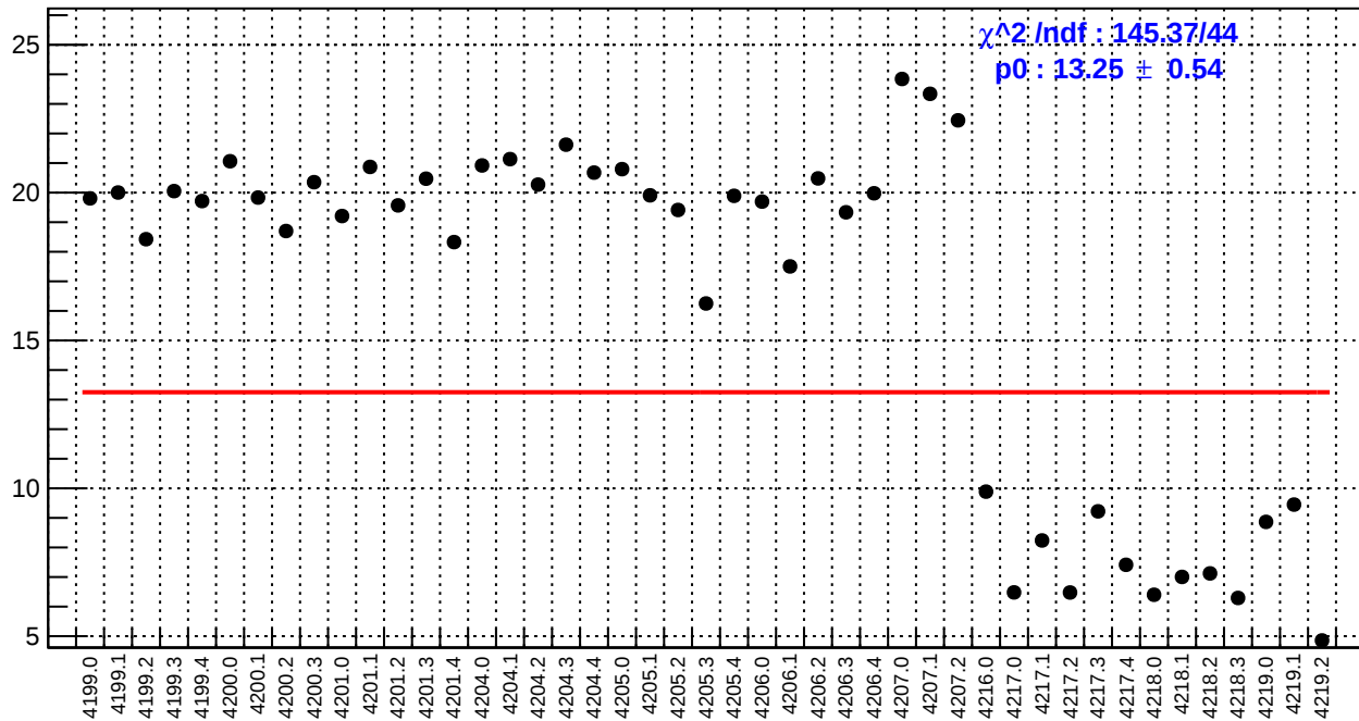
slug48: dsl_bpm4aX/(ppb/nm)
