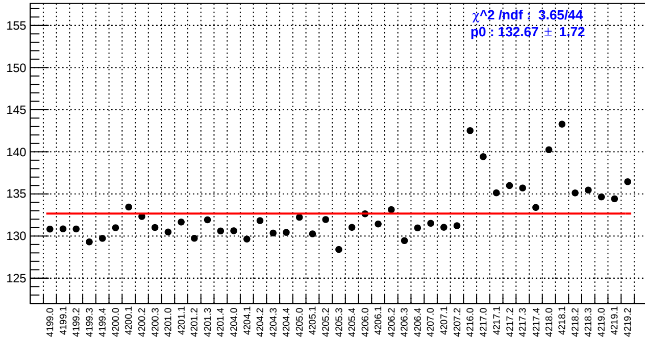
slug48: reg_asym_right_avg.rms/ppm
