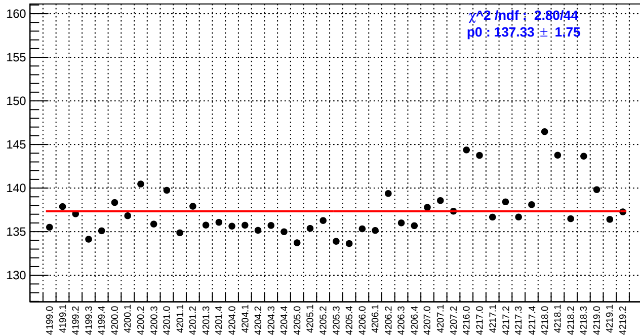
slug48: reg_asym_usl.rms/ppm
