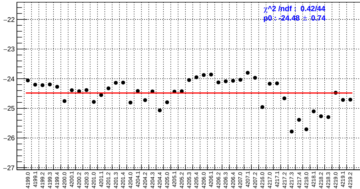
slug48: ds_avg_bpm4eX/(ppb/nm)
