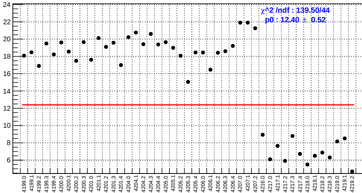
slug48: usl_bpm4aX/(ppb/nm)
