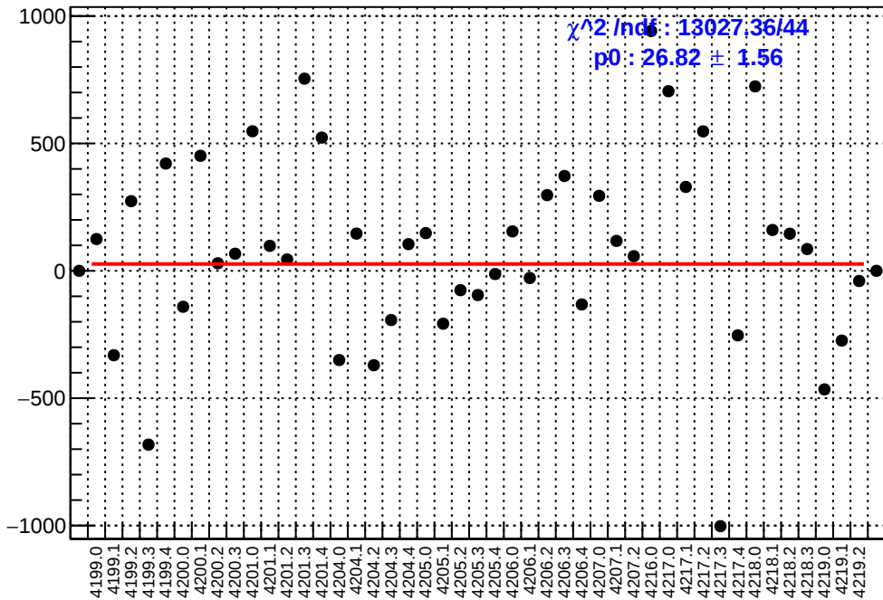
slug48: asym_right_dd.mean/ppb-reg_asym_right_dd.mean/ppb
