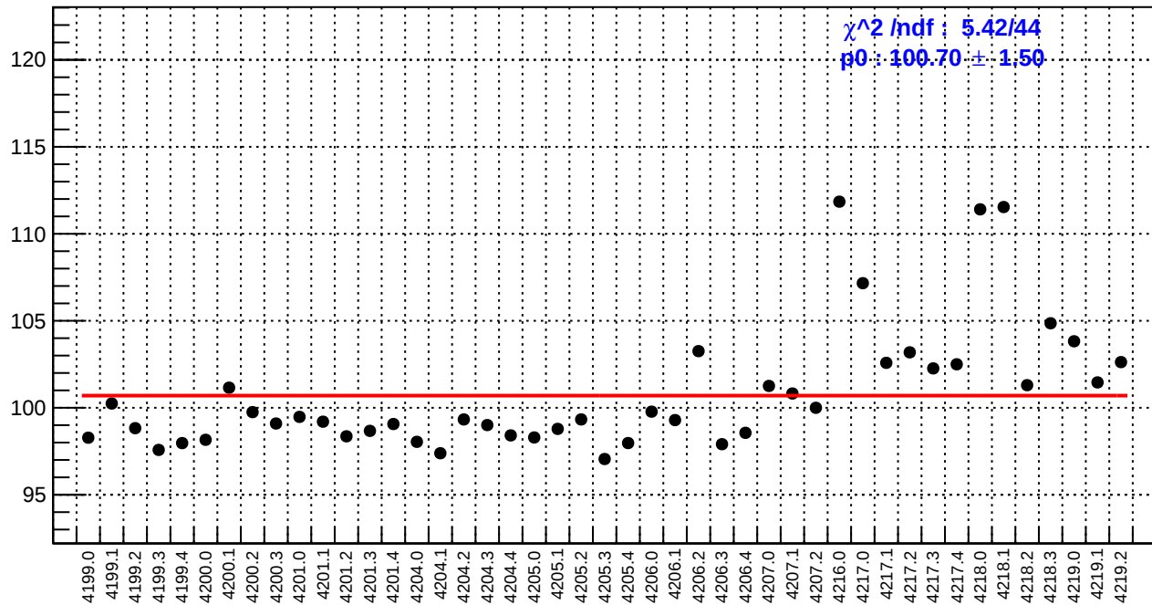
slug48: reg_asym_ds_avg.rms/ppm
