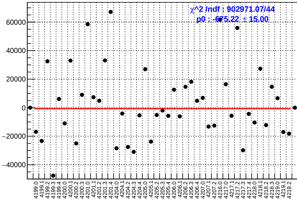
slug48: asym_sam6.mean/ppb-reg_asym_sam6.mean/ppb
