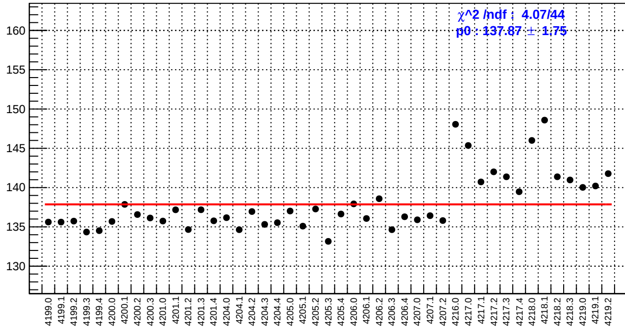
slug48: reg_asym_dsr.rms/ppm
