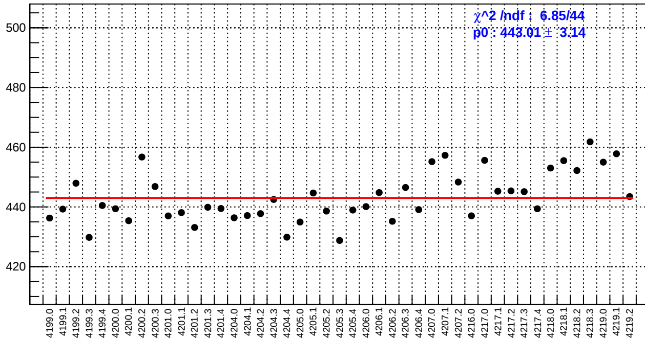
slug48: reg_asym_sam8.rms/ppm
