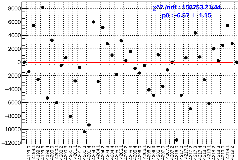
slug48: asym_us_dd.mean/ppb-reg_asym_us_dd.mean/ppb
