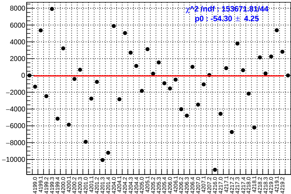
slug48: asym_ds_dd.mean/ppb-reg_asym_ds_dd.mean/ppb
