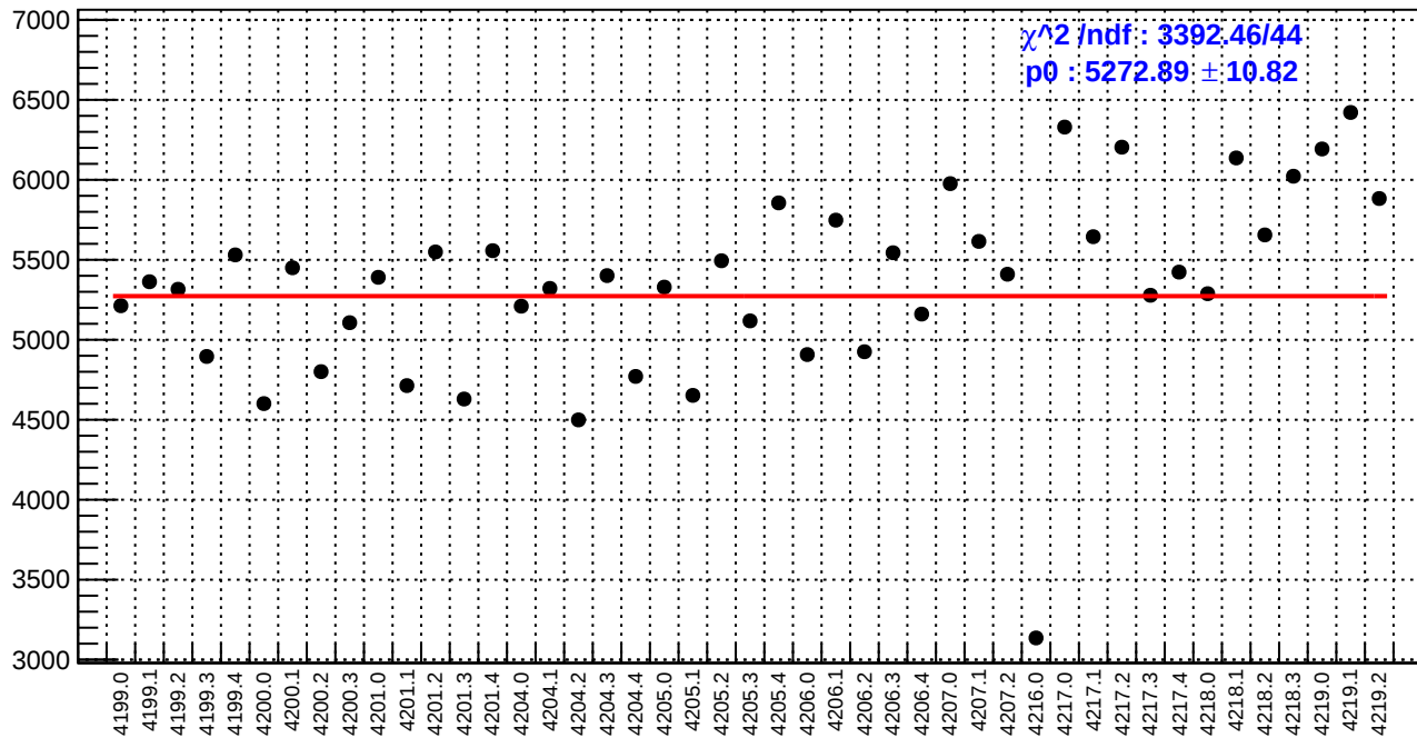
slug48: diff_bpm4eY.rms/nm
