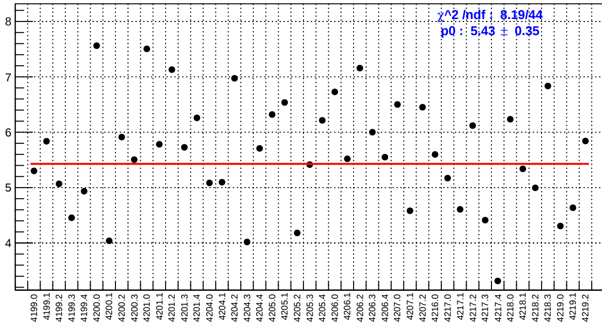
slug48: us_avg_bpm4aY/(ppb/nm)
