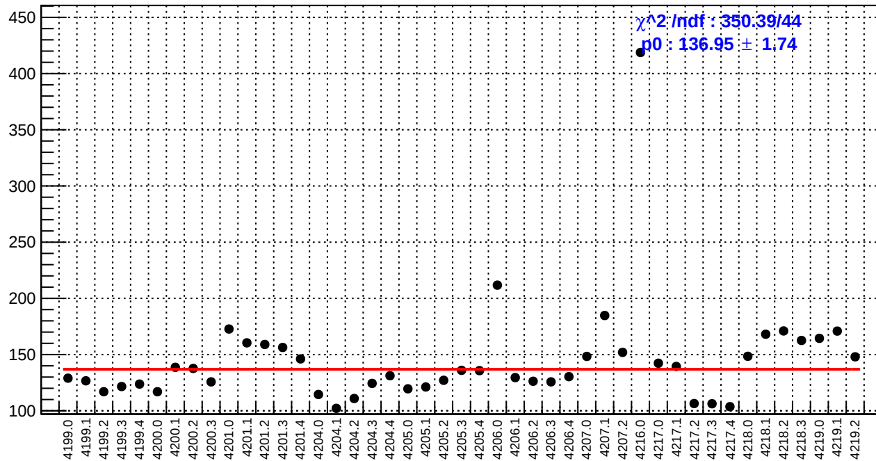
slug48: asym_bcm_an_ds.rms/ppm
