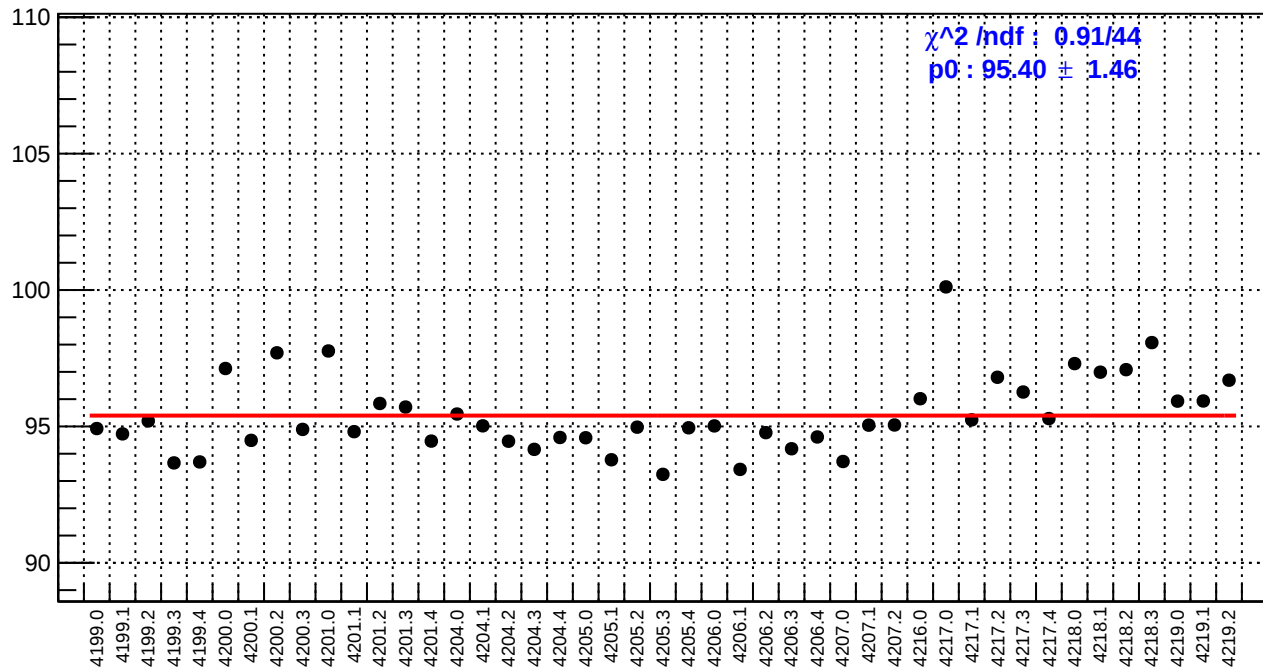
slug48: reg_asym_ds_dd.rms/ppm
