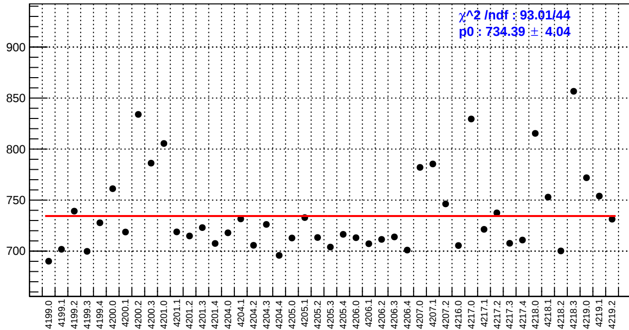
slug48: reg_asym_sam3.rms/ppm
