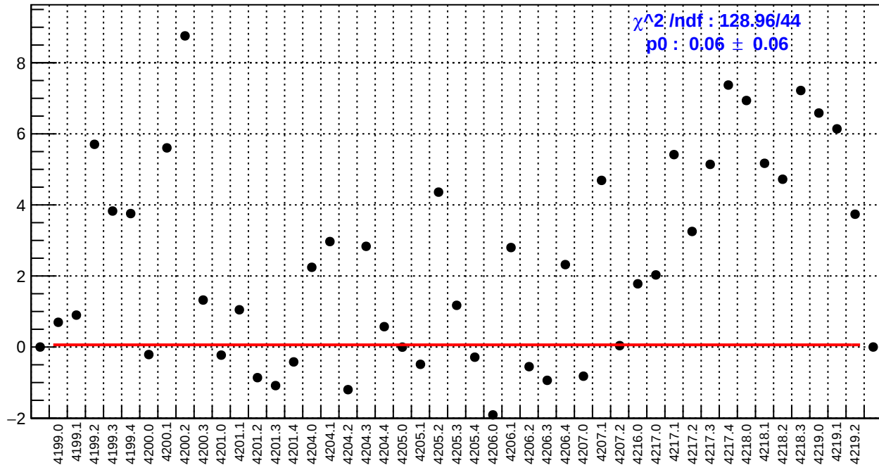
slug48: right_avg_bpm4eY/(ppb/nm)
