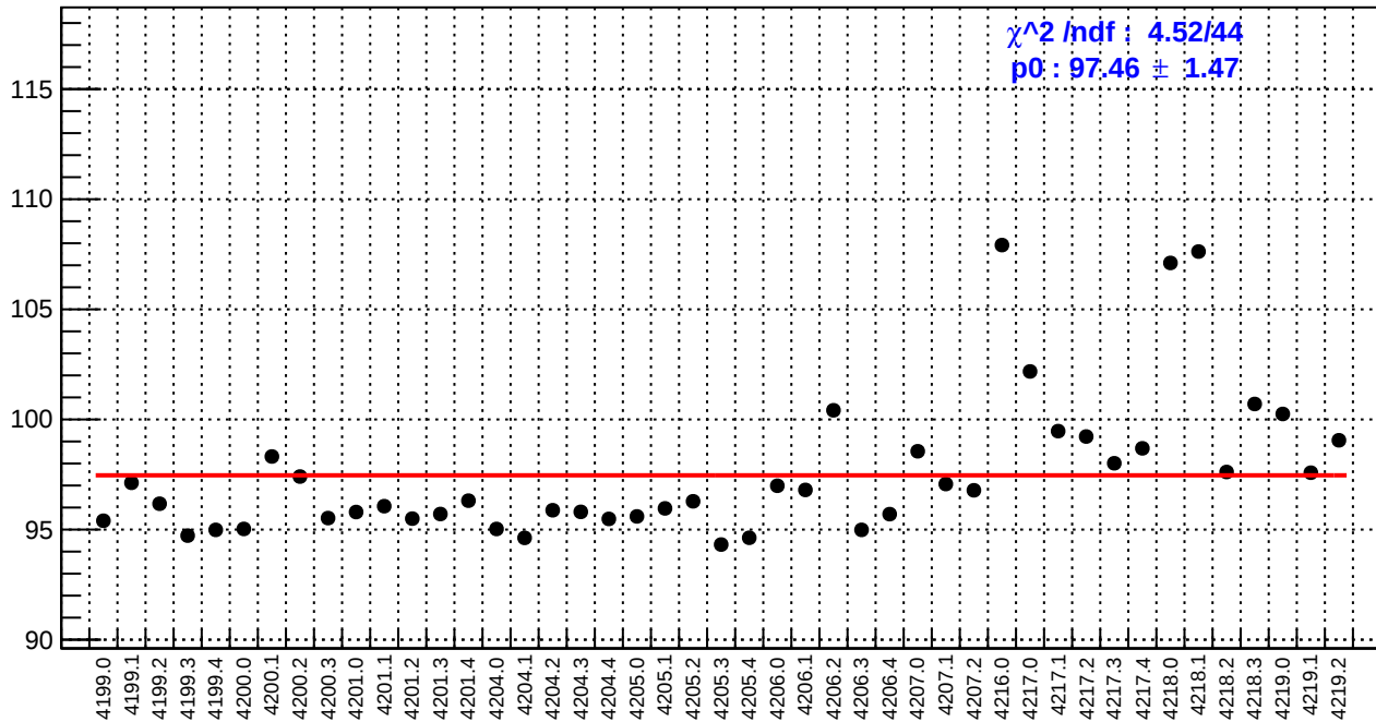
slug48: reg_asym_us_avg.rms/ppm
