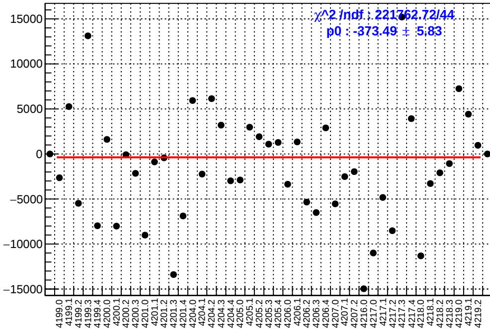
slug48: asym_usl.mean/ppb-reg_asym_usl.mean/ppb
