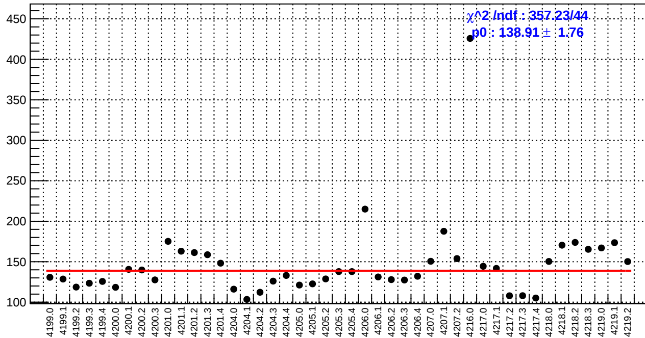
slug48: asym_bcm_an_ds3.rms/ppm
