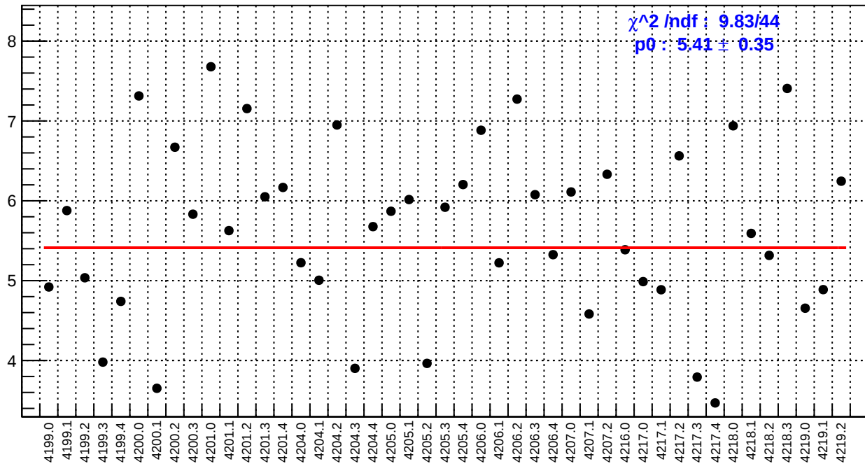
slug48: ds_avg_bpm4aY/(ppb/nm)
