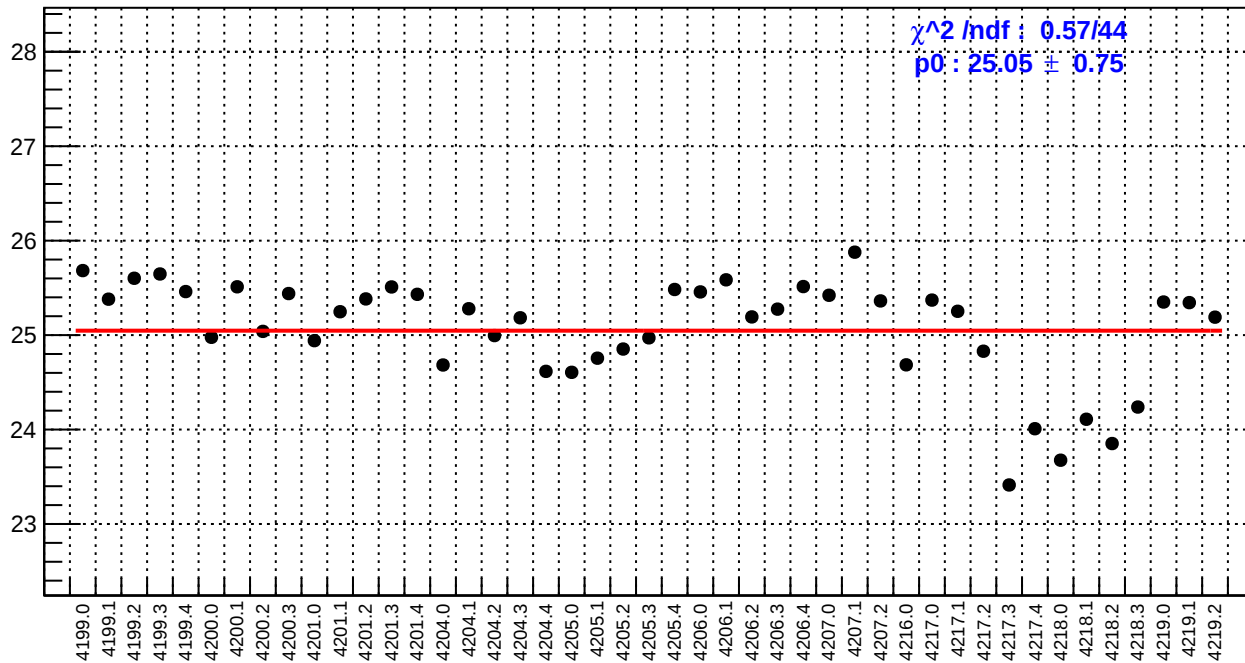
slug48: right_avg_bpm4eX/(ppb/nm)
