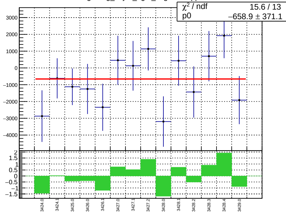
slug5: reg_asym_right_avg.mean/ppb
