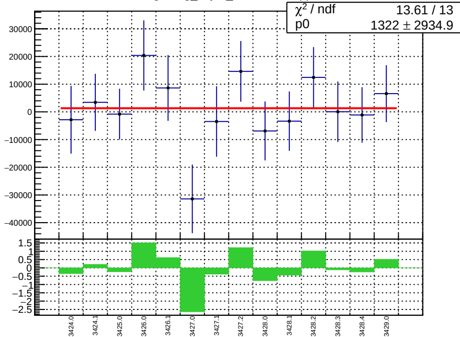
slug5: reg_asym_sam4.mean/ppb
