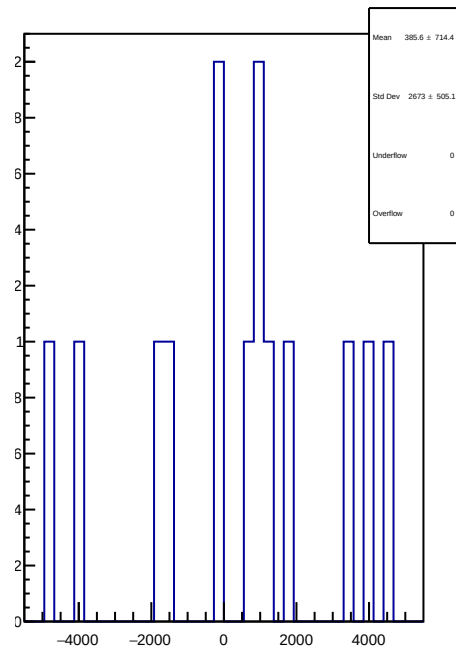
slug5: 1D Corr asym_us_avg.mean/ppb-reg_asym_us_avg.mean/ppb
