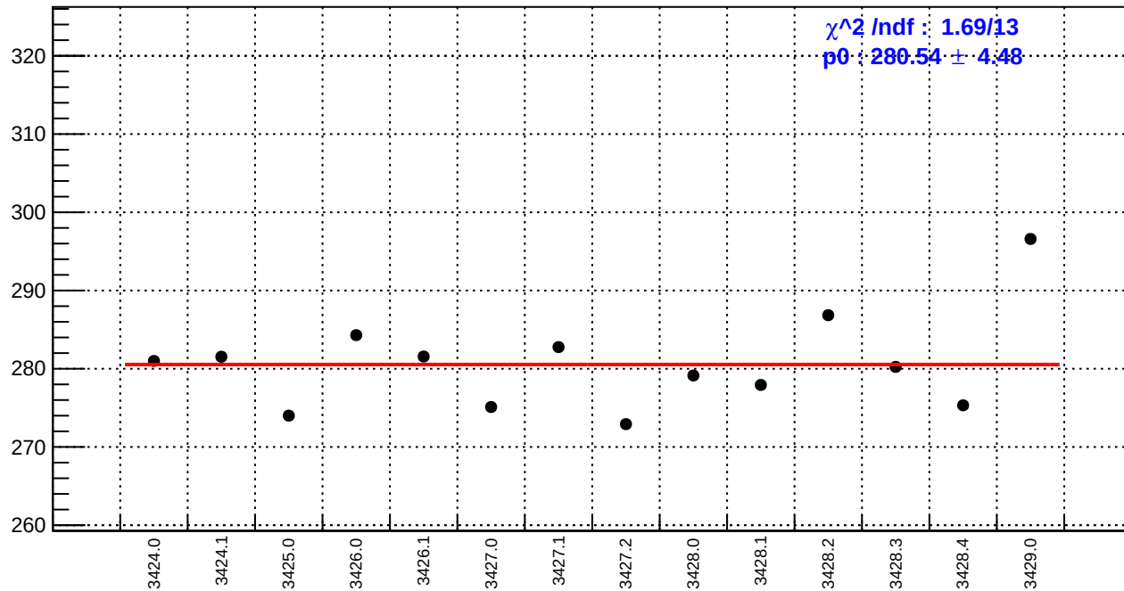
slug5: reg_asym_sam1.rms/ppm
