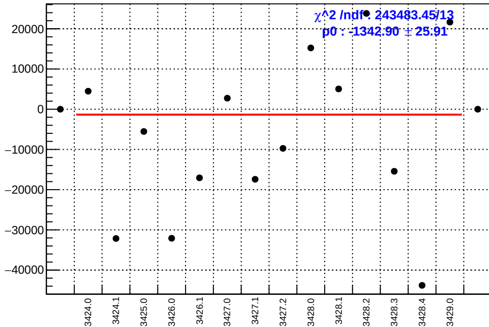
slug5: asym_sam8.mean/ppb-reg_asym_sam8.mean/ppb
