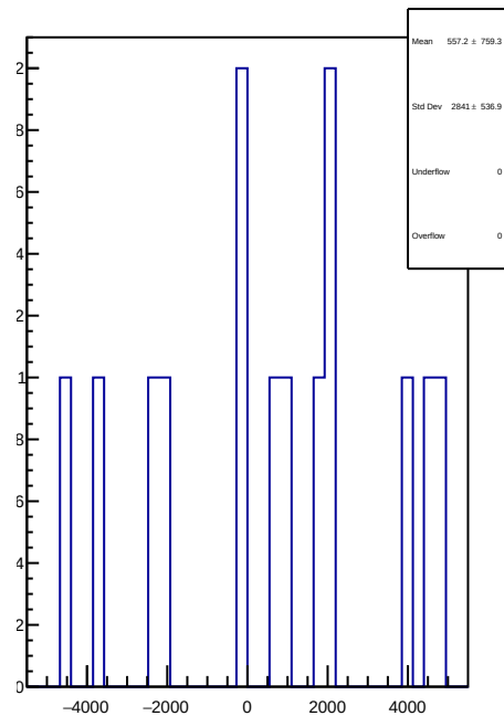
slug5: 1D Corr asym_ds_avg.mean/ppb-reg_asym_ds_avg.mean/ppb
