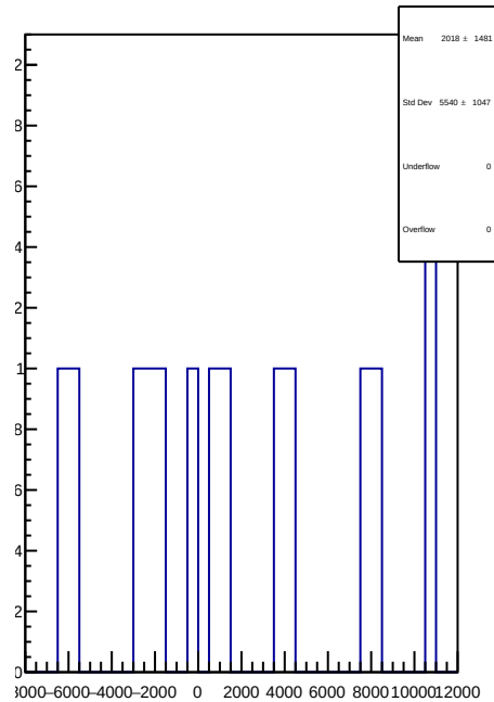
slug5: 1D Corr asym_usl.mean/ppb-reg_asym_usl.mean/ppb
