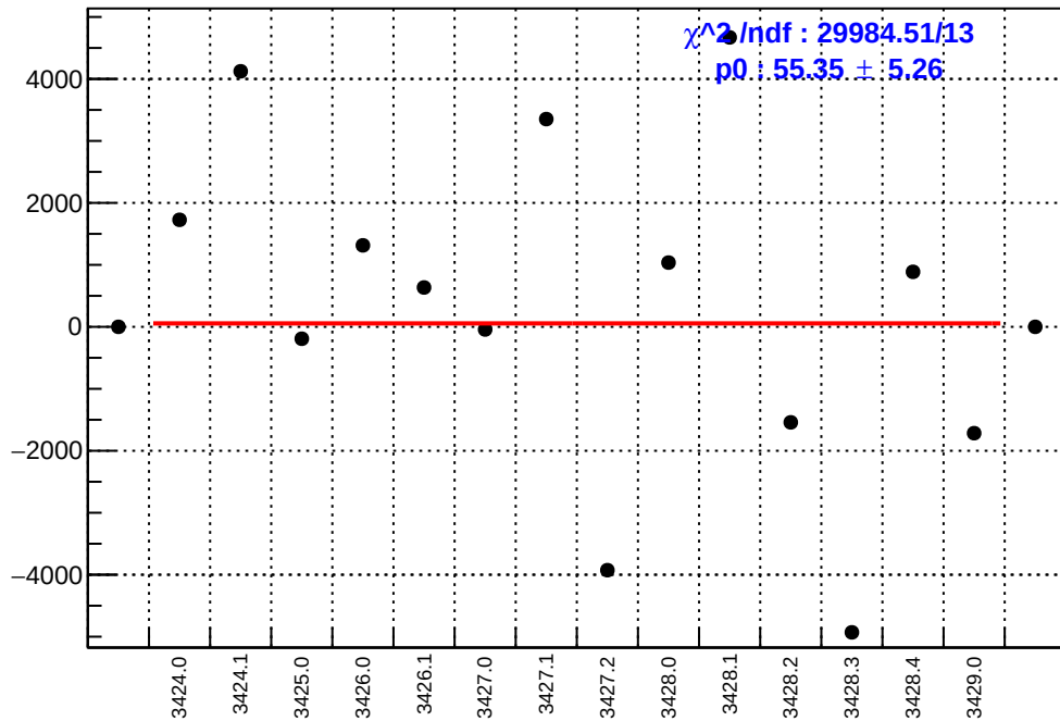
slug5: asym_us_avg.mean/ppb-reg_asym_us_avg.mean/ppb
