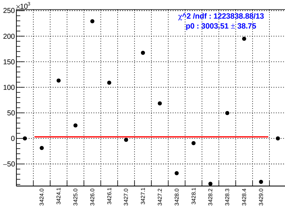
slug5: asym_sam3.mean/ppb-reg_asym_sam3.mean/ppb
