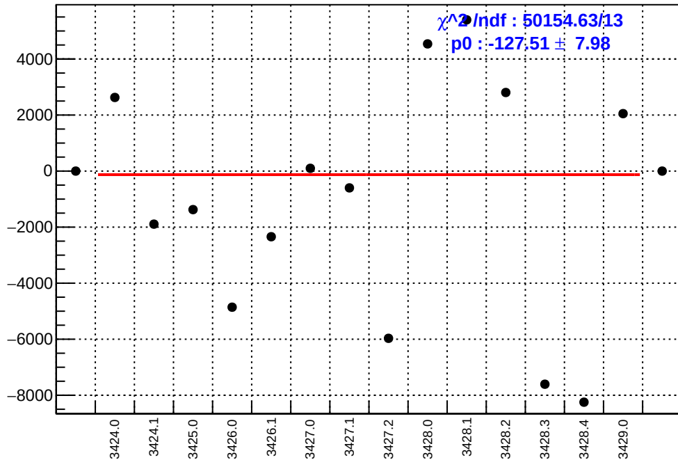
slug5: asym_right_avg.mean/ppb-reg_asym_right_avg.mean/ppb
