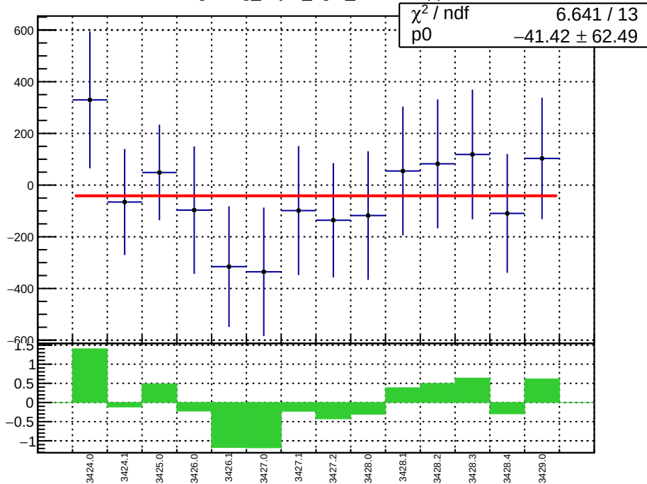
slug5: reg_asym_right_dd.mean/ppb
