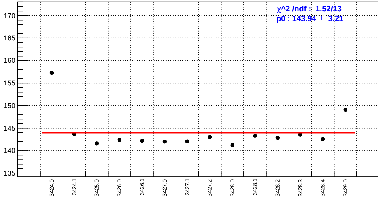
slug5: reg_asym_left_avg.rms/ppm
