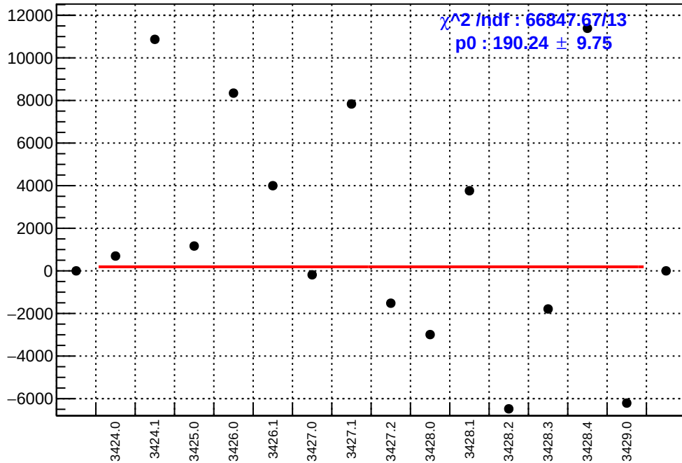
slug5: asym_dsl.mean/ppb-reg_asym_dsl.mean/ppb
