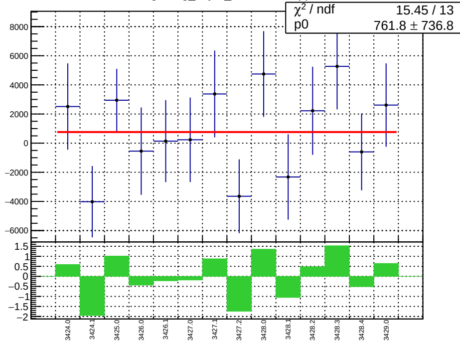
slug5: reg_asym_sam1.mean/ppb
