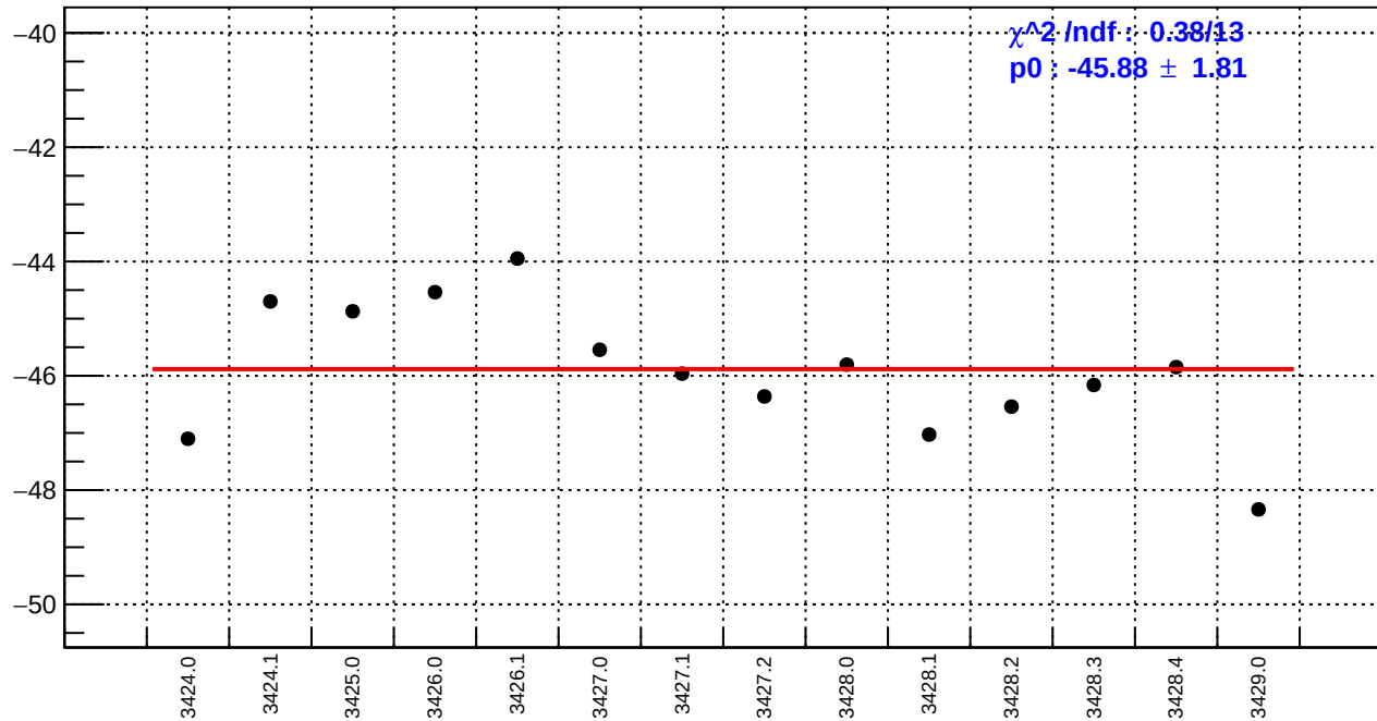
slug5: dsl_bpm12X/(ppb/nm)
