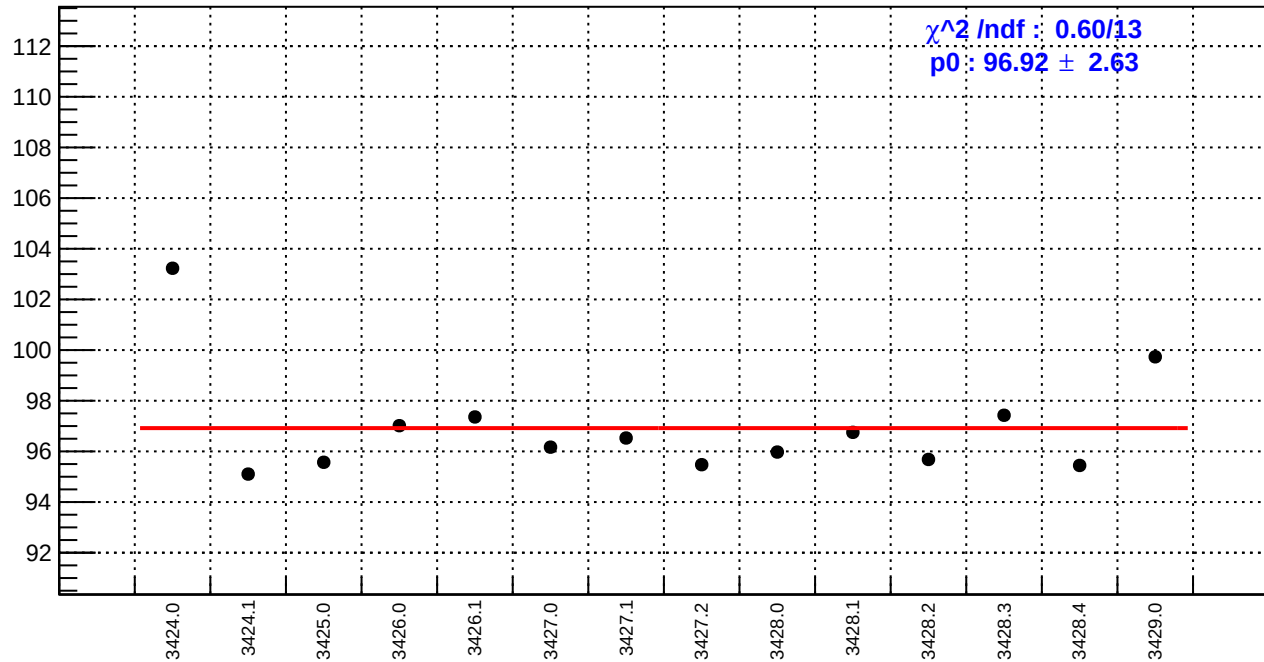
slug5: reg_asym_us_dd.rms/ppm
