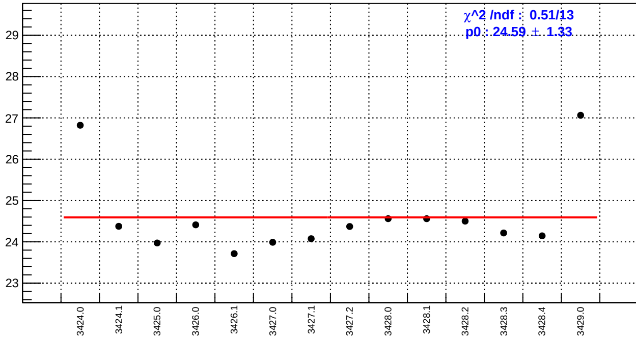
slug5: reg_asym_left_dd.rms/ppm
