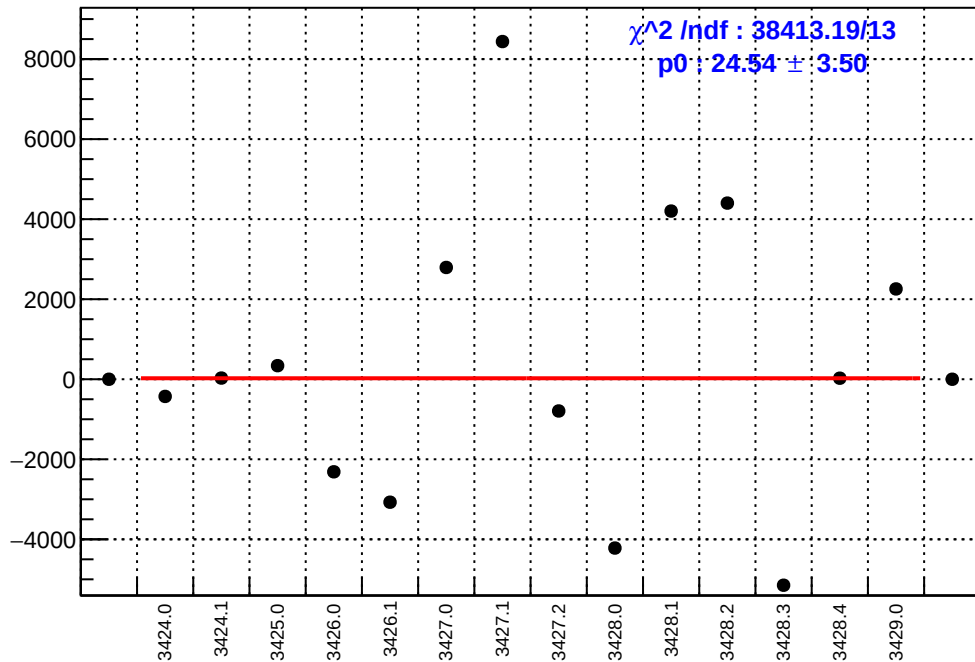
slug5: asym_sam1.mean/ppb-reg_asym_sam1.mean/ppb
