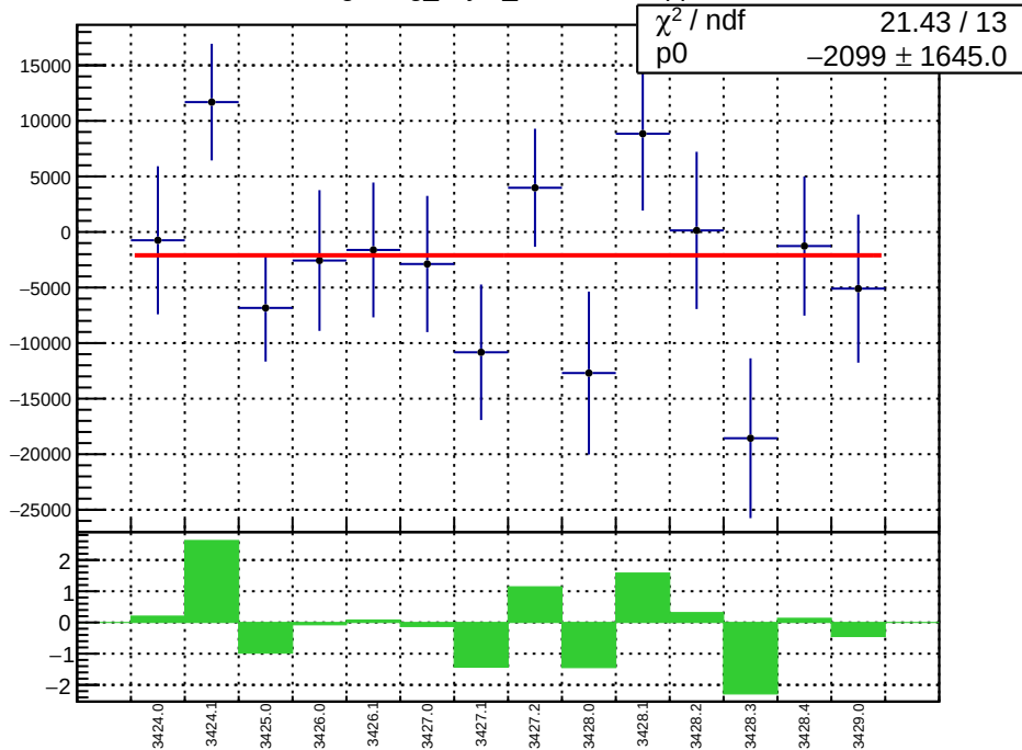
slug5: reg_asym_sam6.mean/ppb
