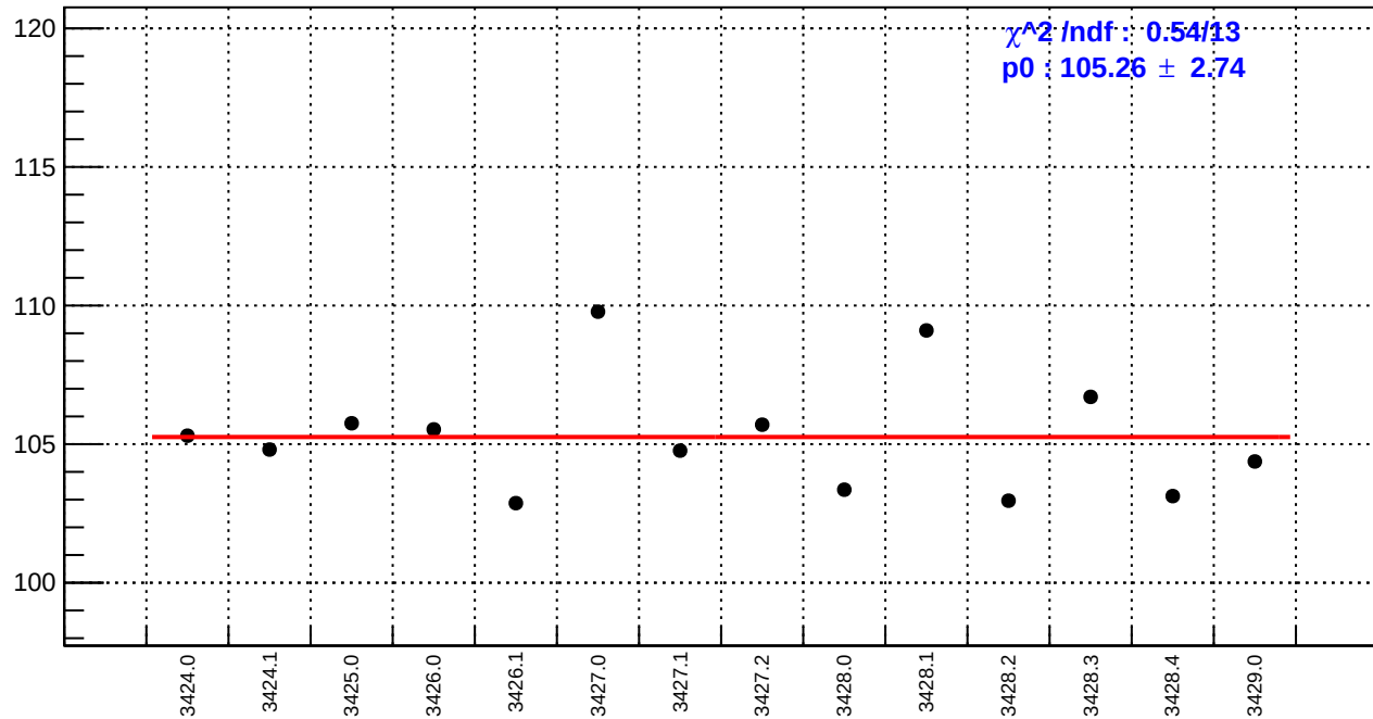
slug5: left_avg_bpm4aX/(ppb/nm)
