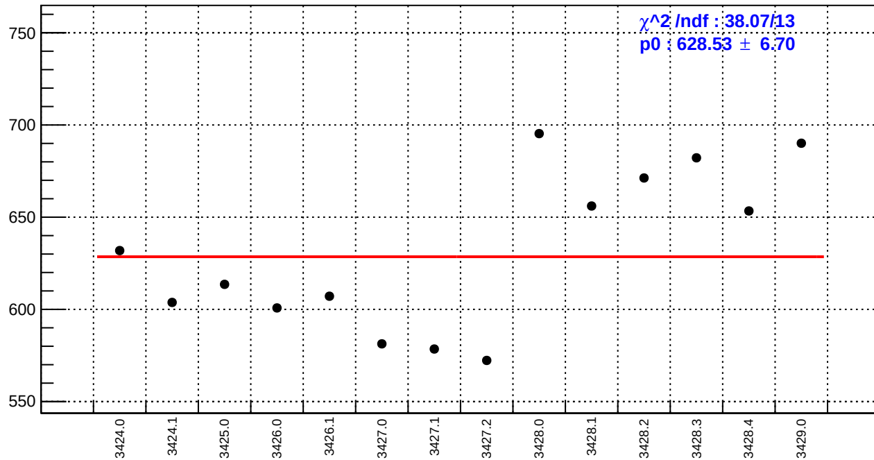
slug5: reg_asym_sam6.rms/ppm
