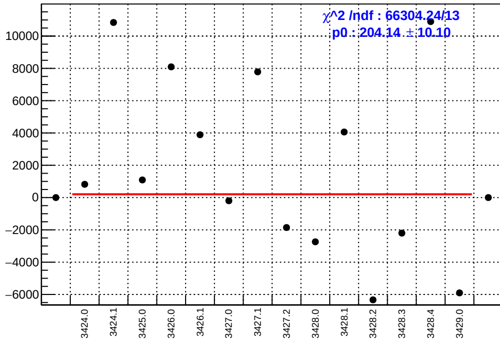
slug5: asym_usl.mean/ppb-reg_asym_usl.mean/ppb
