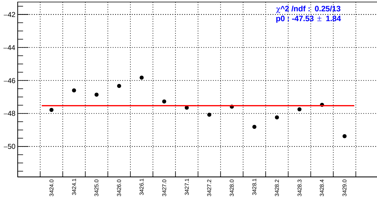
slug5: left_avg_bpm12X/(ppb/nm)
