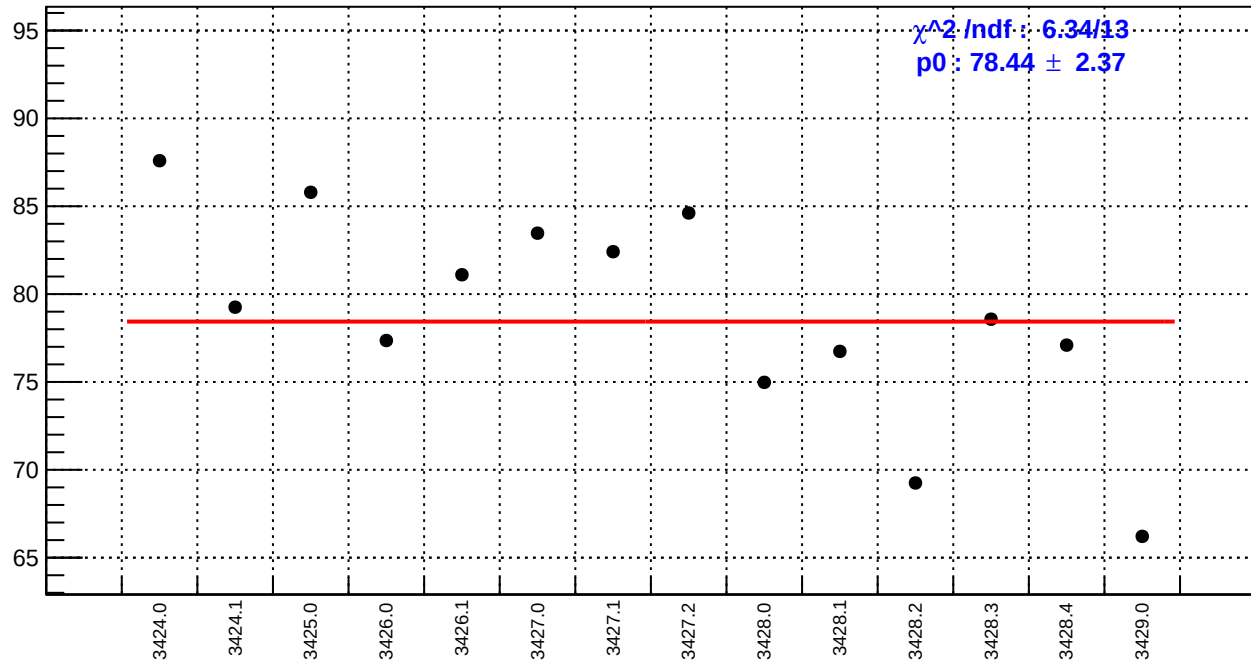
slug5: right_avg_bpm4aX/(ppb/nm)
