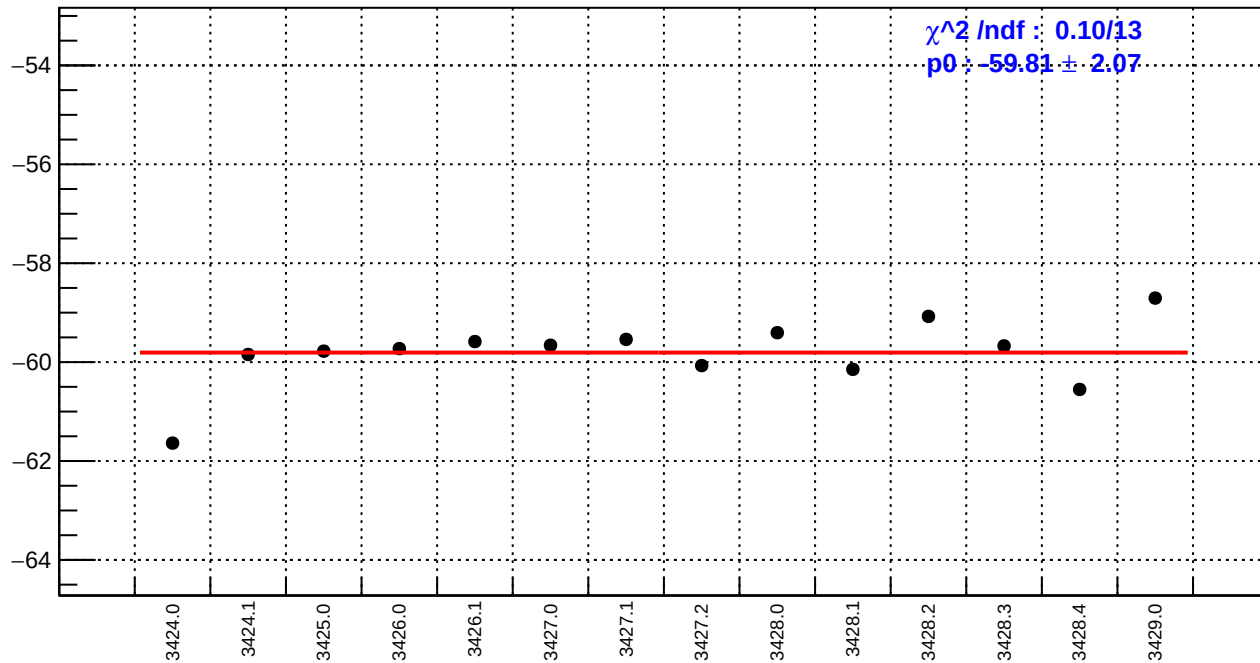
slug5: right_avg_bpm12X/(ppb/nm)
