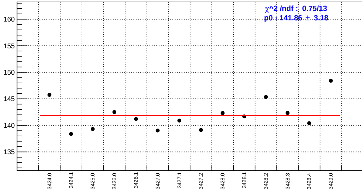
slug5: reg_asym_usr.rms/ppm
