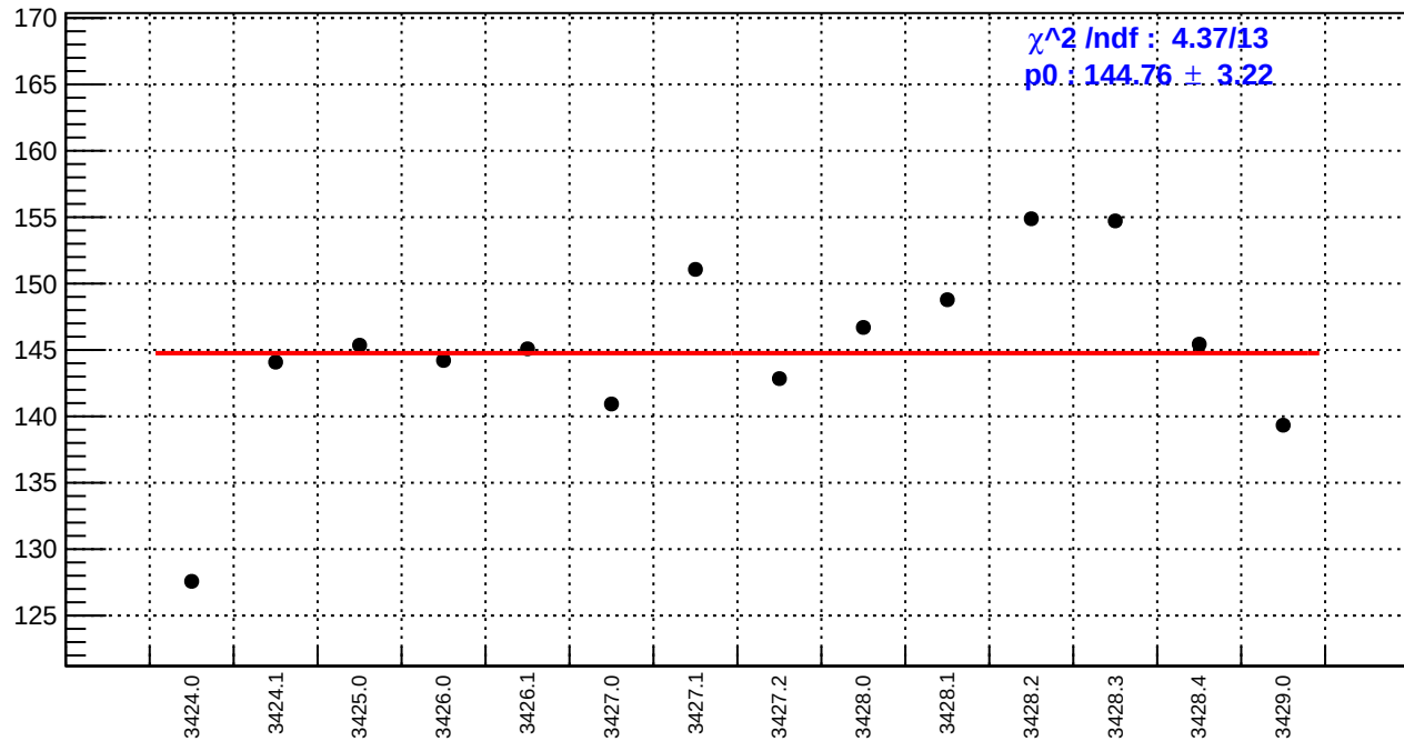
slug5: asym_bcm_an_us.rms/ppm
