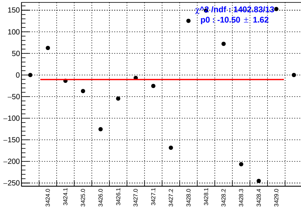
slug5: asym_left_dd.mean/ppb-reg_asym_left_dd.mean/ppb
