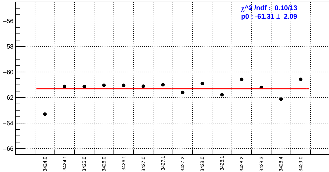
slug5: dsr_bpm12X/(ppb/nm)
