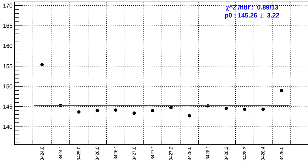
slug5: reg_asym_usl.rms/ppm
