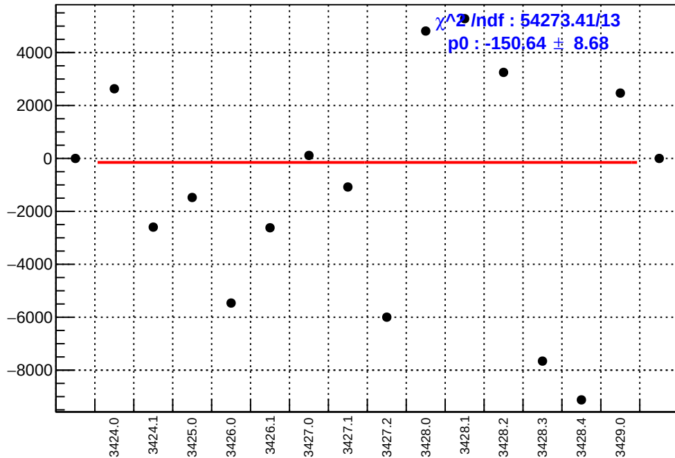
slug5: asym_usr.mean/ppb-reg_asym_usr.mean/ppb
