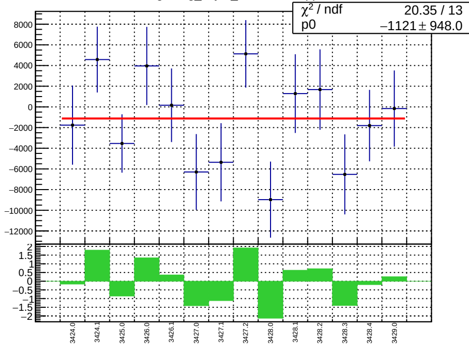
slug5: reg_asym_sam5.mean/ppb
