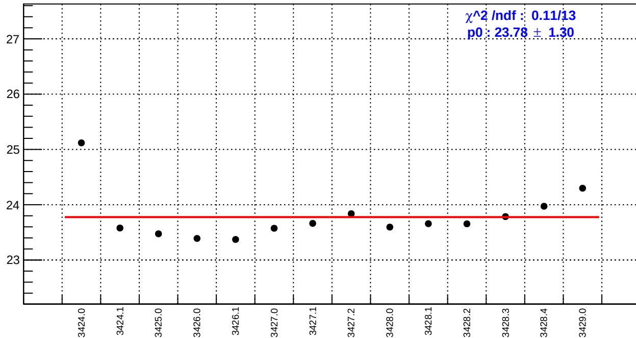
slug5: reg_asym_right_dd.rms/ppm
