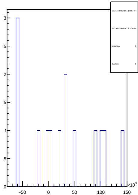
slug5: 1D Corr asym_sam2.mean/ppb-reg_asym_sam2.mean/ppb
