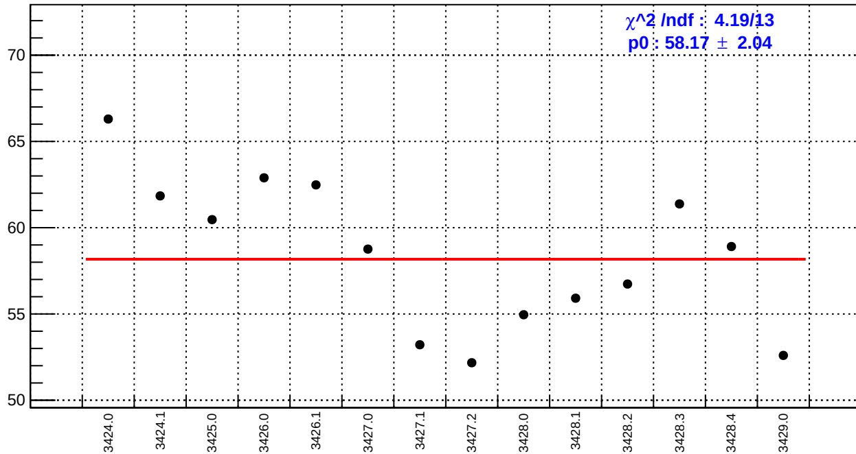
slug5: dsl_bpm4eY/(ppb/nm)
