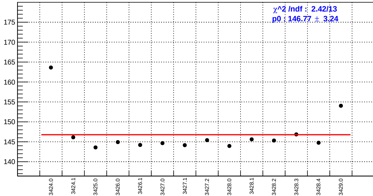
slug5: reg_asym_dsl.rms/ppm
