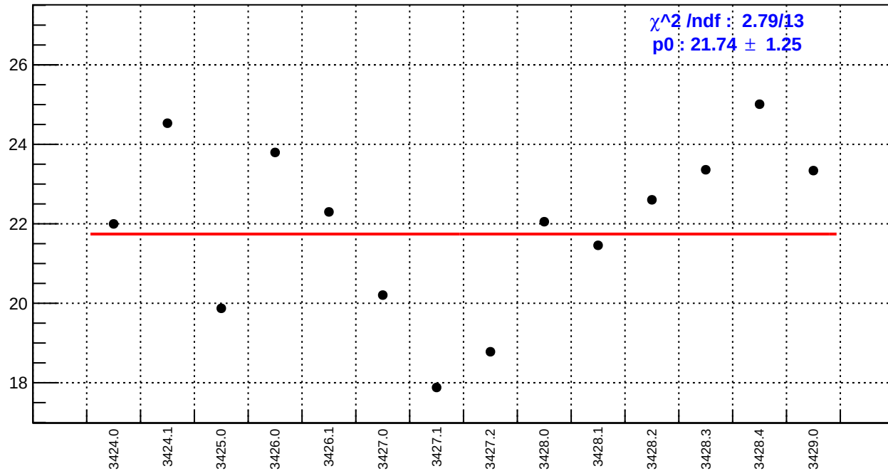
slug5: right_avg_bpm4aY/(ppb/nm)
