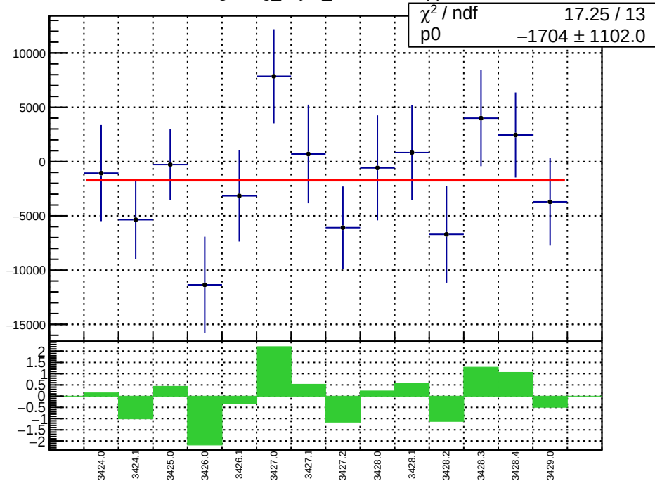
slug5: reg_asym_sam8.mean/ppb
