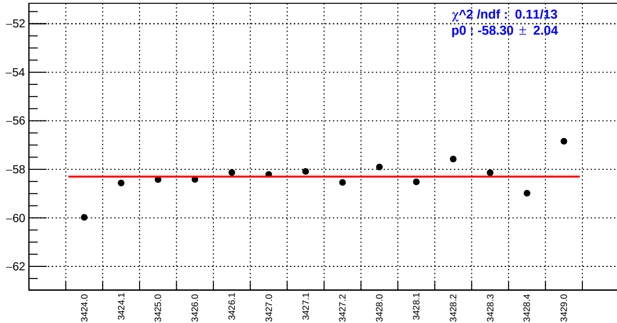
slug5: usr_bpm12X/(ppb/nm)
