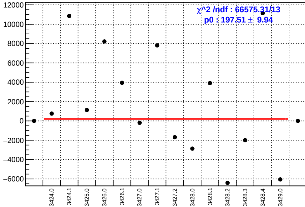
slug5: asym_left_avg.mean/ppb-reg_asym_left_avg.mean/ppb
