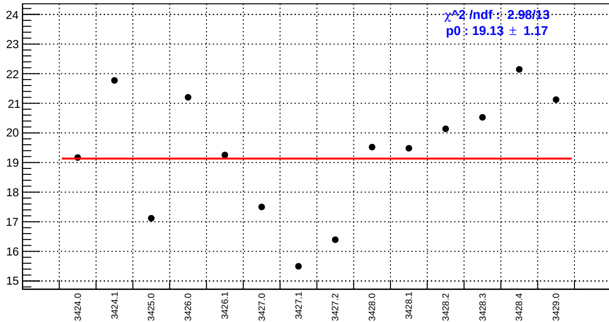
slug5: dsr_bpm4aY/(ppb/nm)
