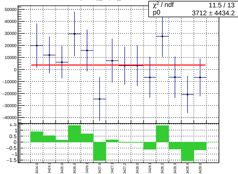
slug5: reg_asym_sam2.mean/ppb
