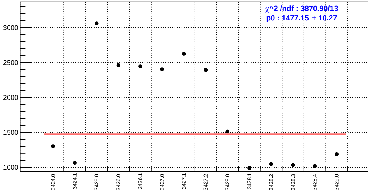
slug5: reg_asym_sam3.rms/ppm
