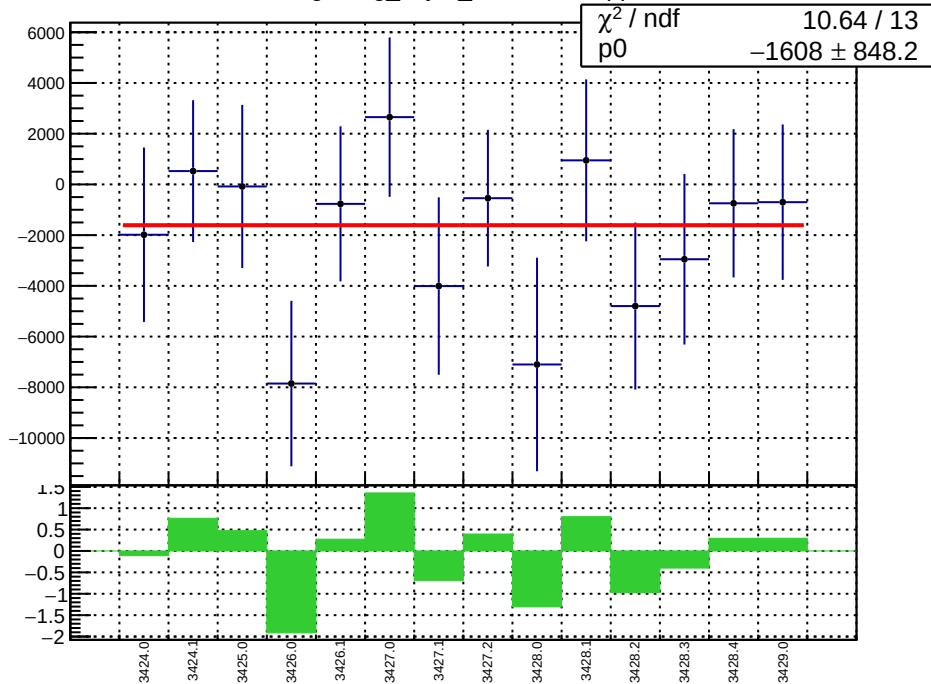
slug5: reg_asym_sam7.mean/ppb
