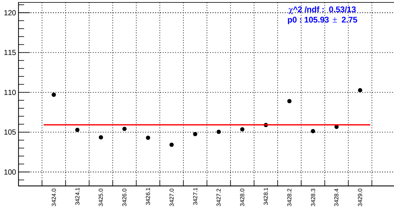
slug5: reg_asym_us_avg.rms/ppm
