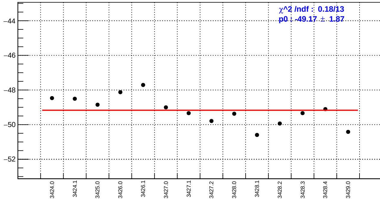
slug5: usl_bpm12X/(ppb/nm)
