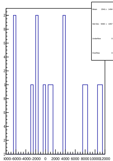
slug5: 1D Corr asym_left_avg.mean/ppb-reg_asym_left_avg.mean/ppb
