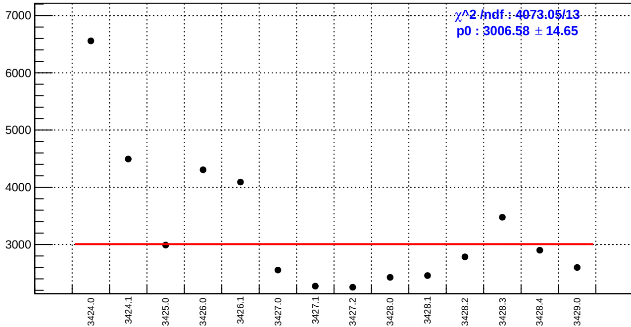
slug5: diff_bpm4eY.rms/nm
