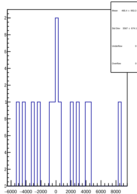
slug5: 1D Corr asym_sam1.mean/ppb-reg_asym_sam1.mean/ppb
