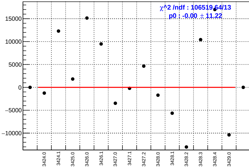
slug5: asym_sam5.mean/ppb-reg_asym_sam5.mean/ppb
