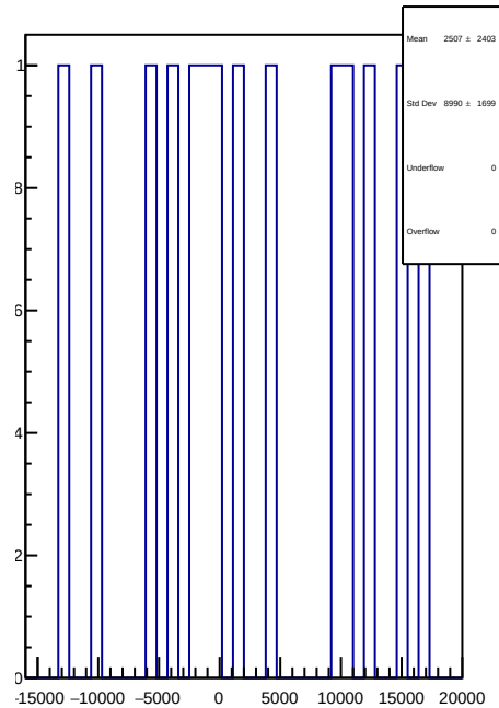
slug5: 1D Corr asym_sam5.mean/ppb-reg_asym_sam5.mean/ppb
