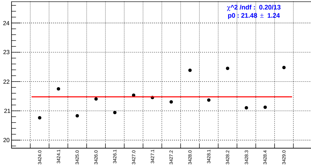
slug5: right_avg_bpm4eX/(ppb/nm)
