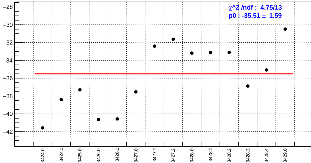
slug5: dsl_bpm4aY/(ppb/nm)
