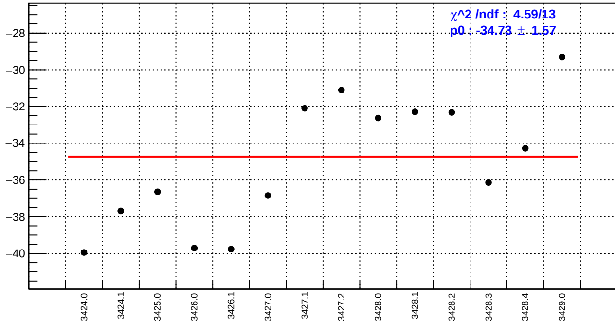
slug5: left_avg_bpm4aY/(ppb/nm)
