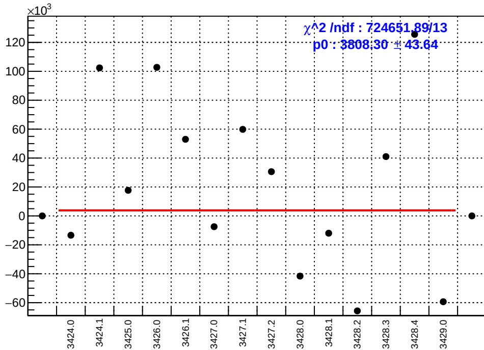
slug5: asym_sam4.mean/ppb-reg_asym_sam4.mean/ppb
