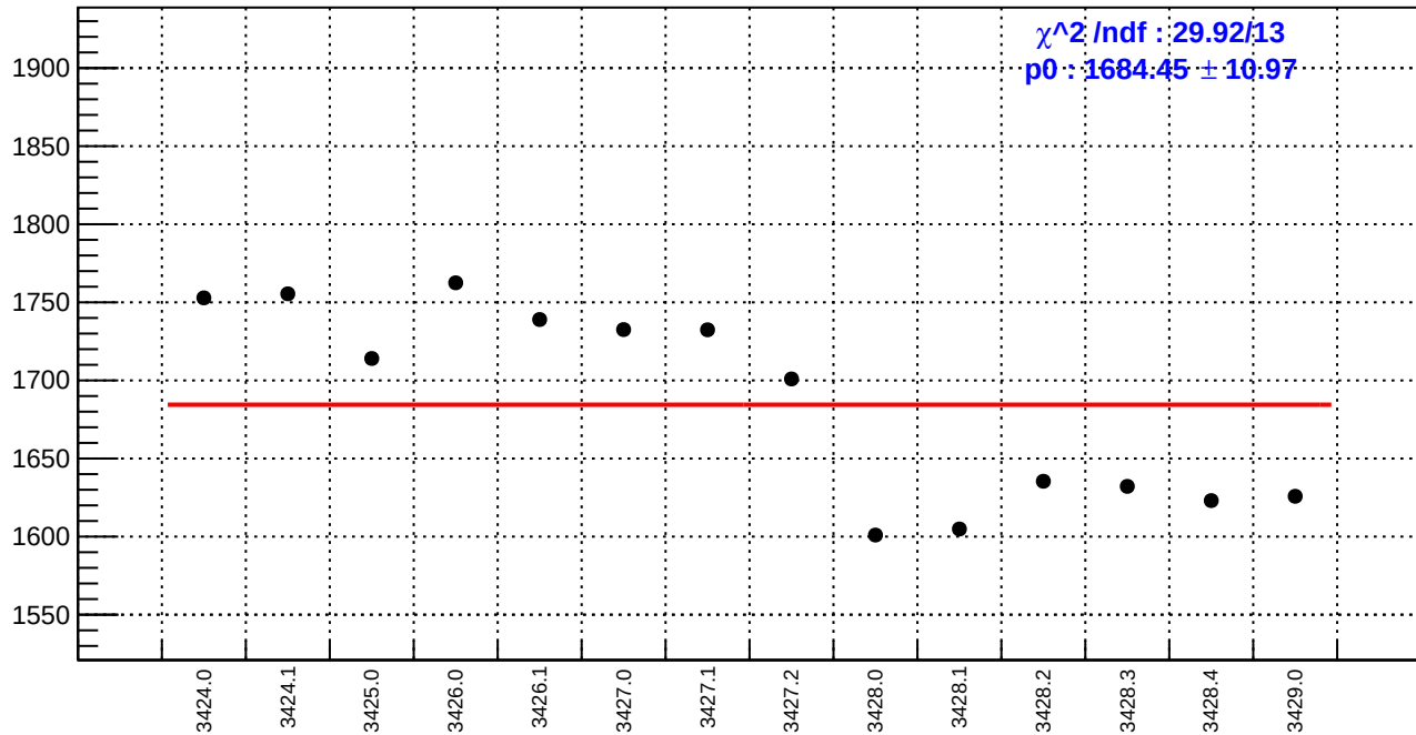
slug5: reg_asym_sam2.rms/ppm
