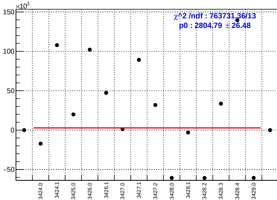
slug5: asym_sam2.mean/ppb-reg_asym_sam2.mean/ppb
