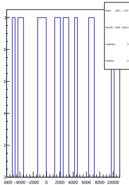
slug5: 1D Corr asym_us_dd.mean/ppb-reg_asym_us_dd.mean/ppb
