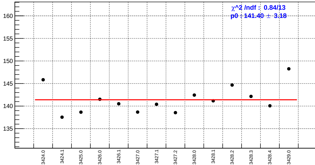
slug5: reg_asym_right_avg.rms/ppm
