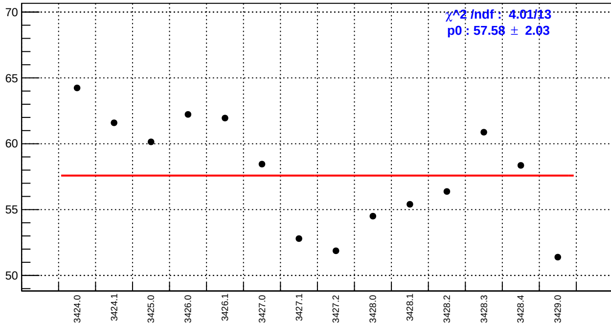
slug5: left_avg_bpm4eY/(ppb/nm)
