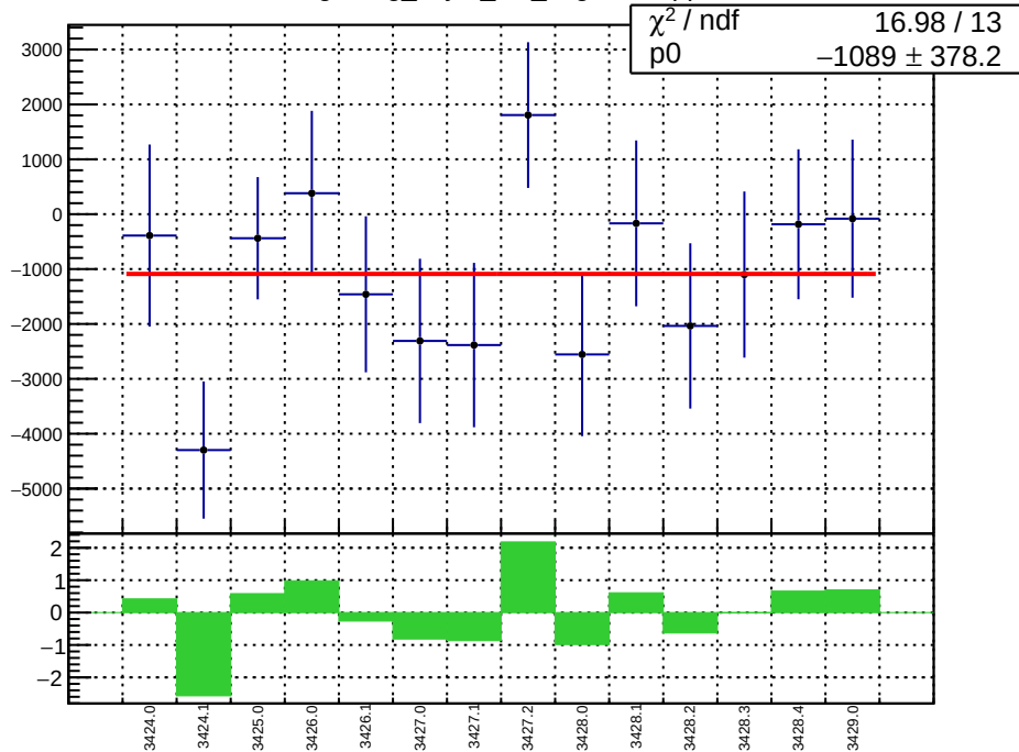
slug5: reg_asym_left_avg.mean/ppb
