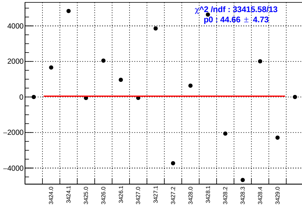
slug5: asym_ds_avg.mean/ppb-reg_asym_ds_avg.mean/ppb
