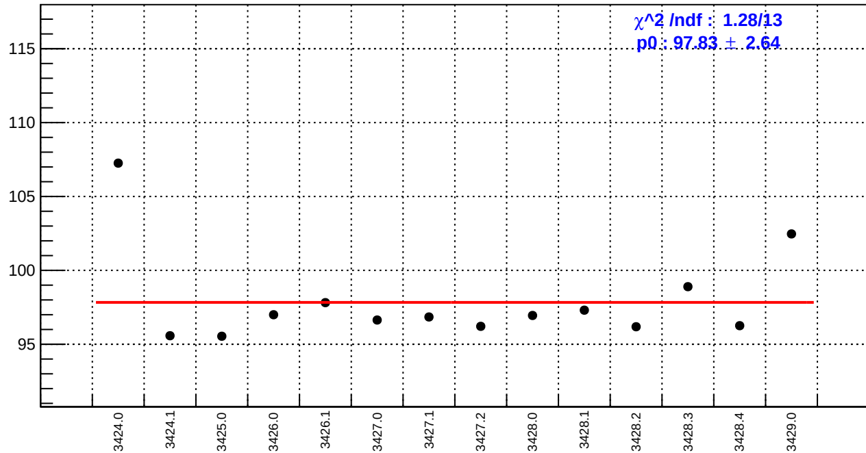
slug5: reg_asym_ds_dd.rms/ppm
