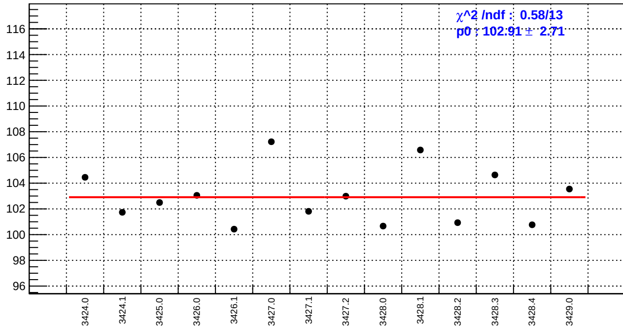
slug5: dsl_bpm4aX/(ppb/nm)
