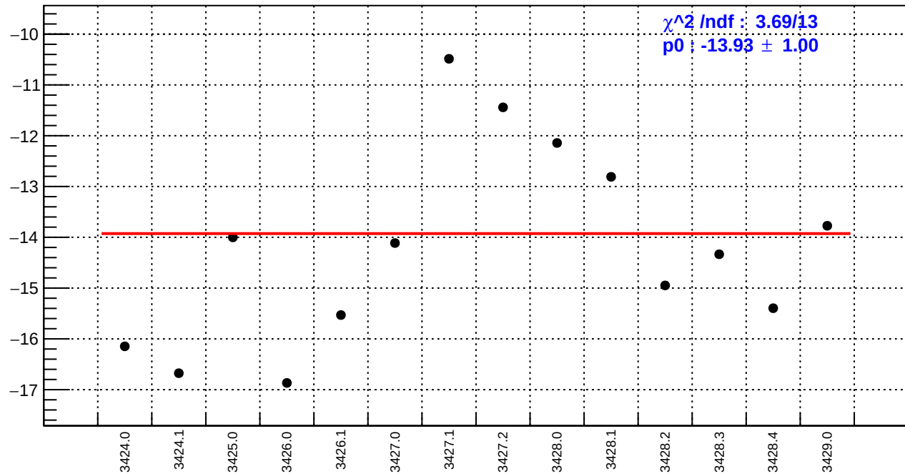
slug5: dsr_bpm4eY/(ppb/nm)
