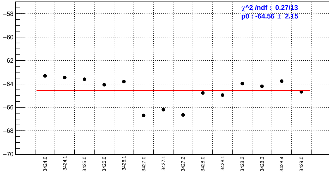
slug5: usl_bpm4eX/(ppb/nm)
