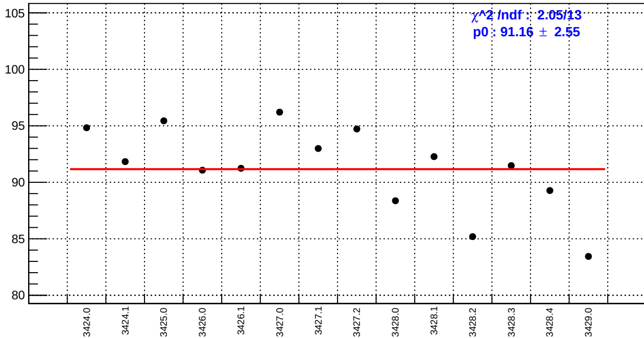
slug5: us_avg_bpm4aX/(ppb/nm)
