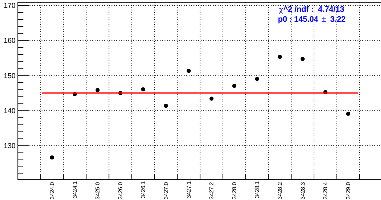
slug5: asym_bcm_an_ds.rms/ppm
