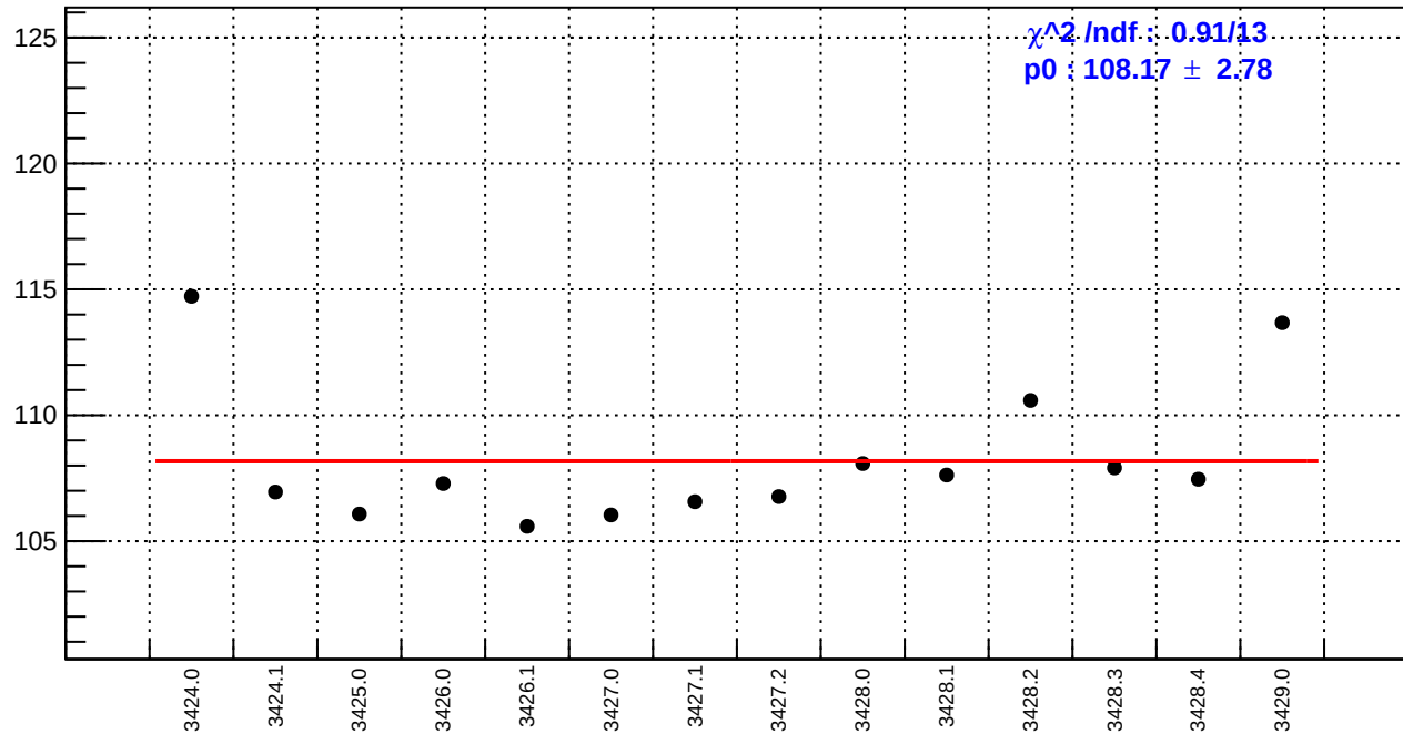
slug5: reg_asym_ds_avg.rms/ppm
