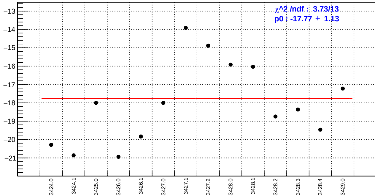
slug5: right_avg_bpm4eY/(ppb/nm)
