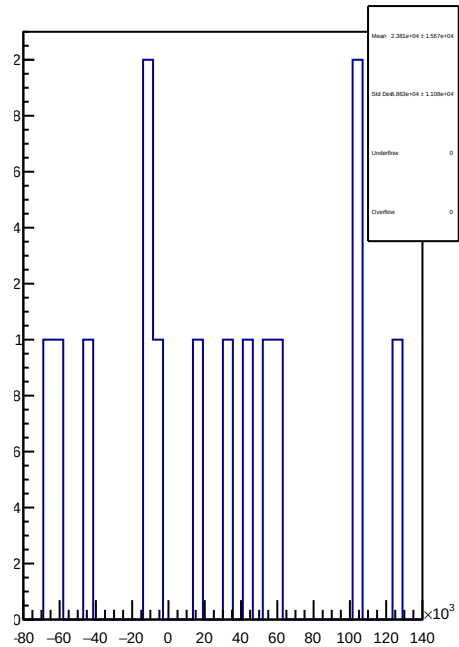
slug5: 1D Corr asym_sam4.mean/ppb-reg_asym_sam4.mean/ppb
