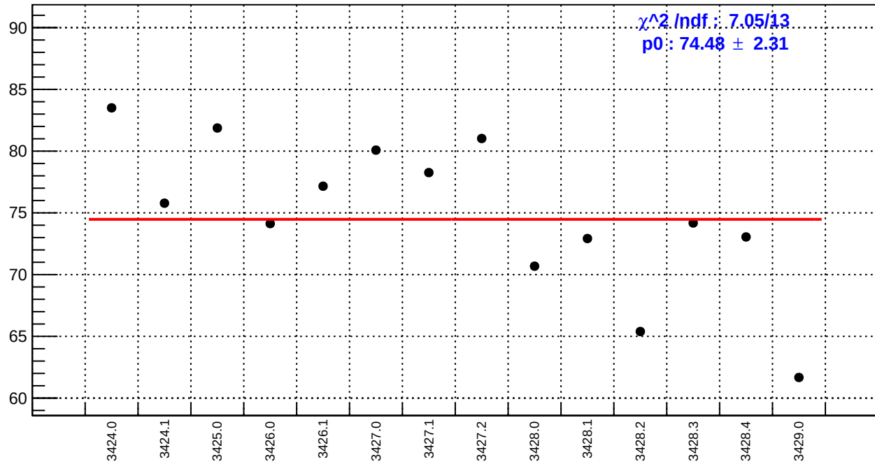
slug5: usr_bpm4aX/(ppb/nm)
