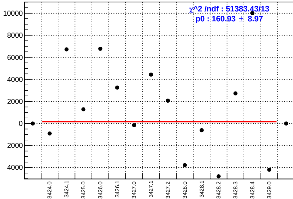
slug5: asym_us_dd.mean/ppb-reg_asym_us_dd.mean/ppb
