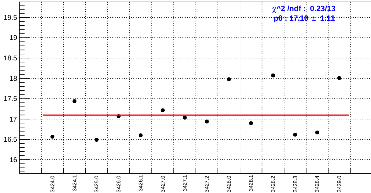
slug5: dsr_bpm4eX/(ppb/nm)
