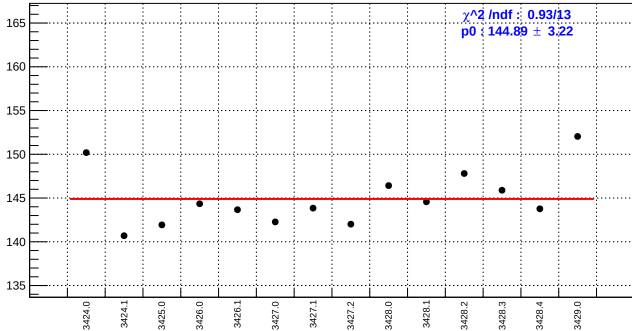
slug5: reg_asym_dsr.rms/ppm
