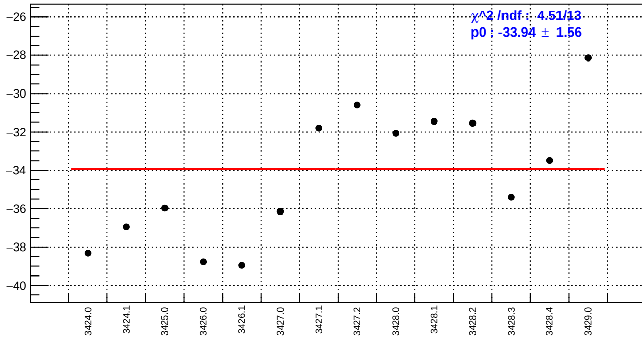
slug5: usl_bpm4aY/(ppb/nm)
