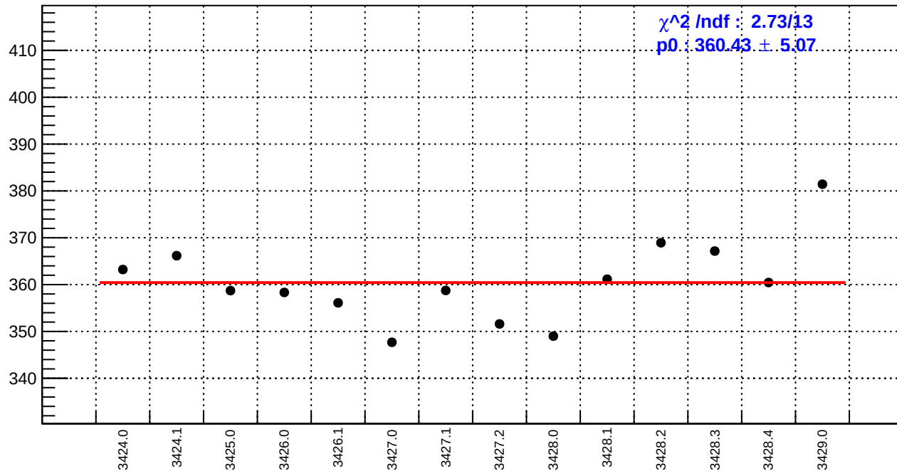
slug5: reg_asym_sam5.rms/ppm
