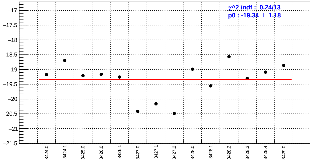
slug5: us_avg_bpm4eX/(ppb/nm)
