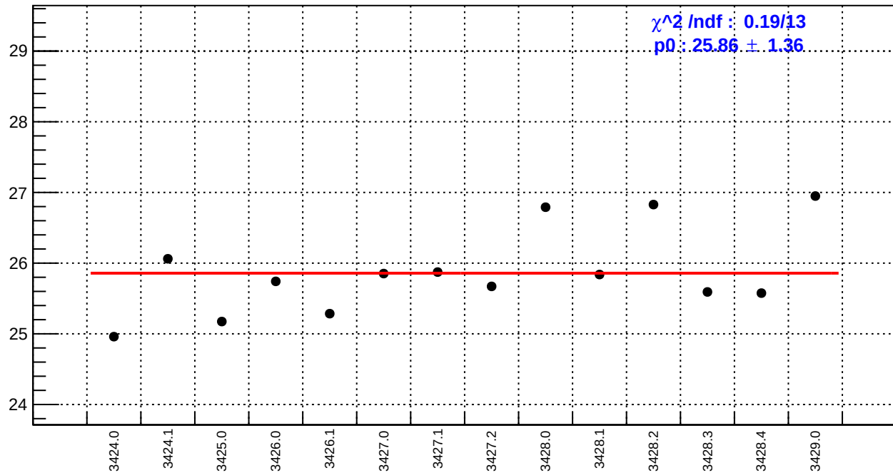
slug5: usr_bpm4eX/(ppb/nm)
