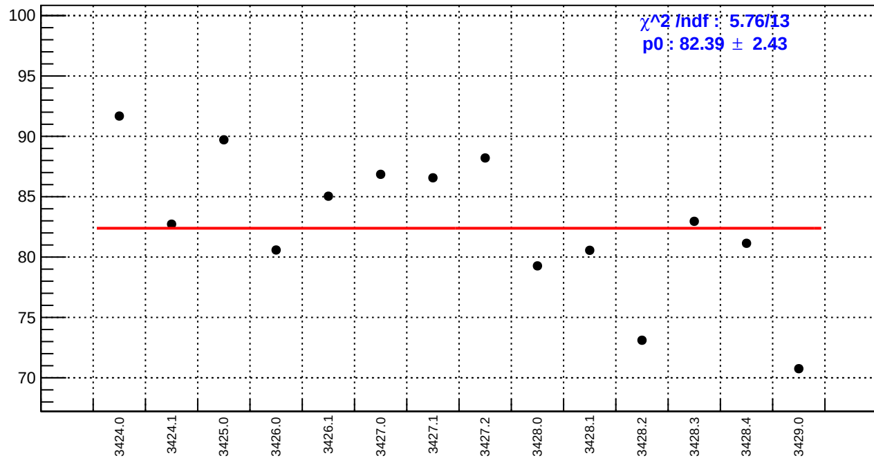
slug5: dsr_bpm4aX/(ppb/nm)
