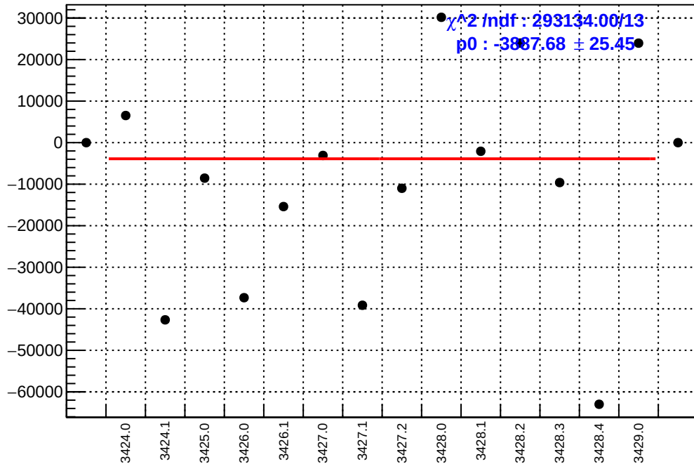
slug5: asym_sam6.mean/ppb-reg_asym_sam6.mean/ppb
