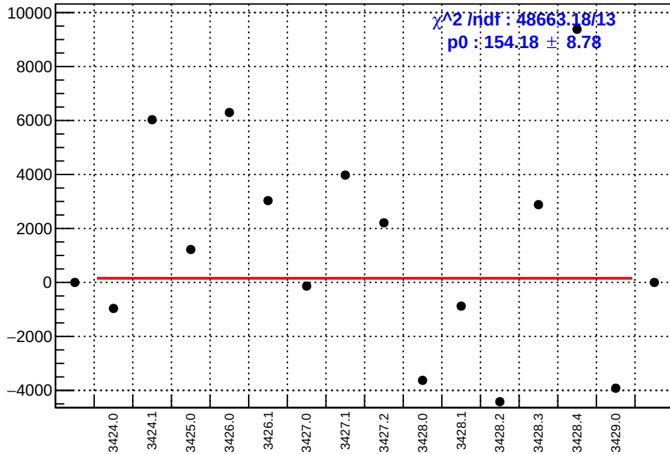
slug5: asym_ds_dd.mean/ppb-reg_asym_ds_dd.mean/ppb
