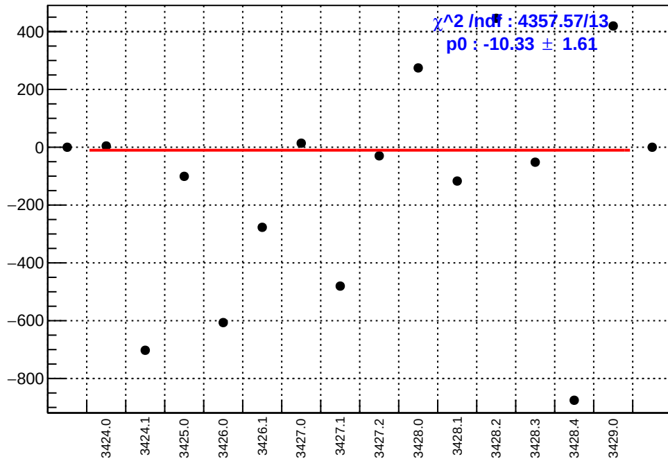
slug5: asym_right_dd.mean/ppb-reg_asym_right_dd.mean/ppb
