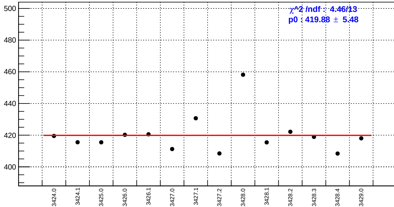
slug5: reg_asym_sam8.rms/ppm
