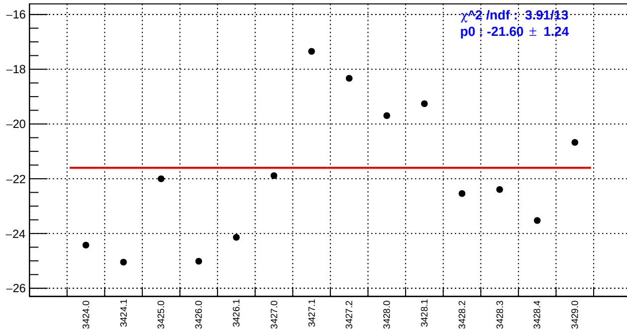
slug5: usr_bpm4eY/(ppb/nm)
