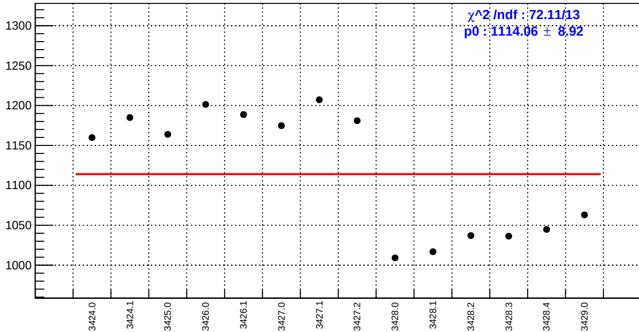
slug5: reg_asym_sam4.rms/ppm
