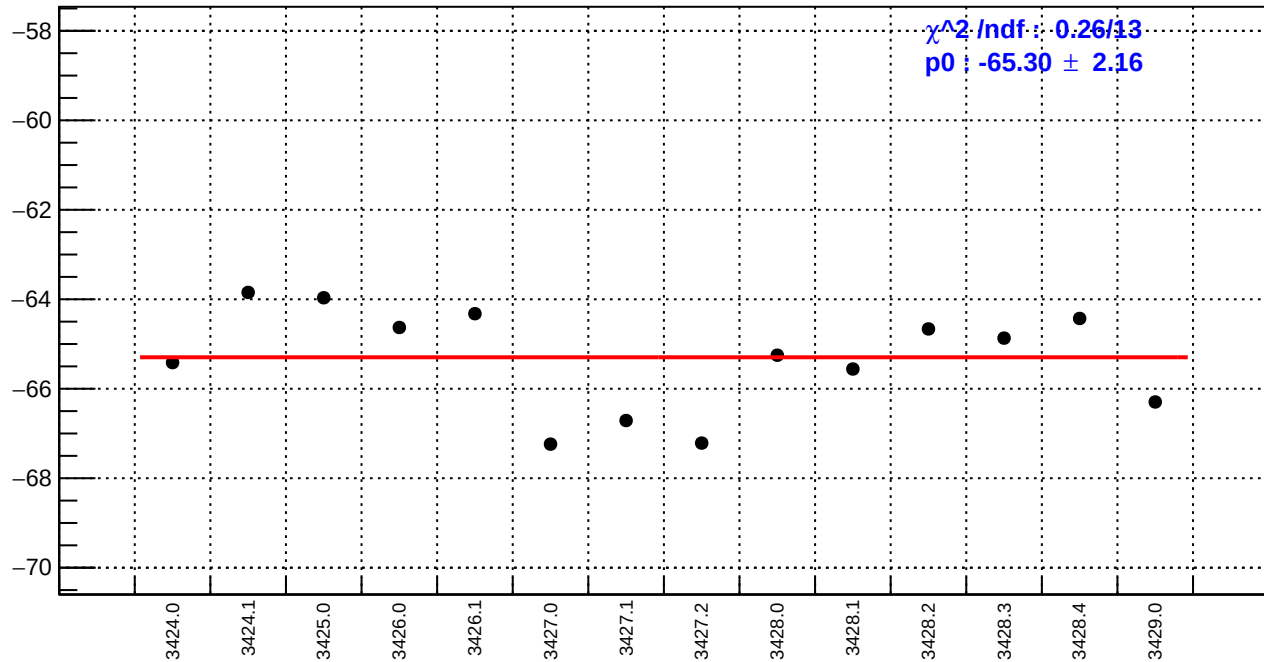
slug5: left_avg_bpm4eX/(ppb/nm)
