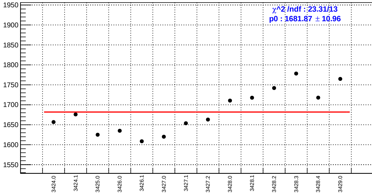
slug5: diff_bpm4aX.rms/nm
