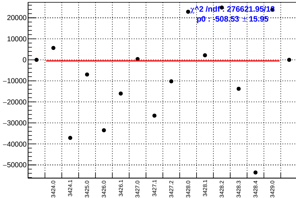
slug5: asym_sam7.mean/ppb-reg_asym_sam7.mean/ppb
