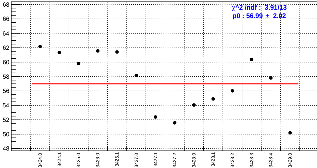
slug5: usl_bpm4eY/(ppb/nm)
