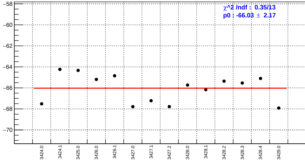
slug5: dsl_bpm4eX/(ppb/nm)
