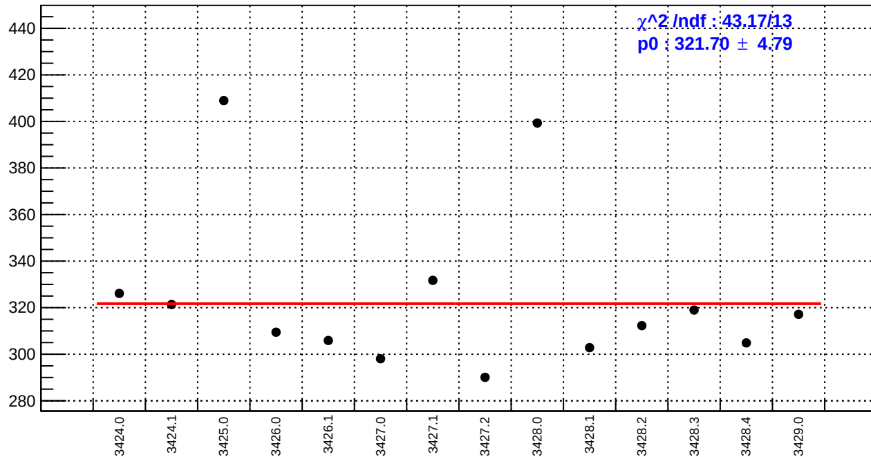
slug5: reg_asym_sam7.rms/ppm
