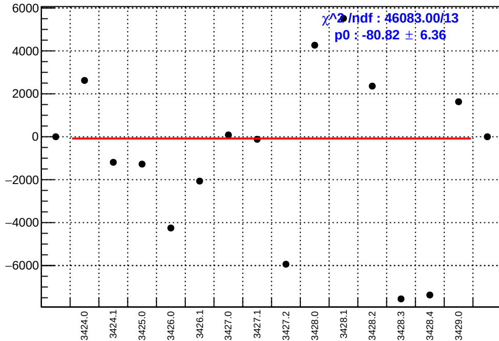
slug5: asym_dsr.mean/ppb-reg_asym_dsr.mean/ppb
