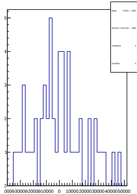
slug50: 1D Corr asym_sam1.mean/ppb-reg_asym_sam1.mean/ppb
