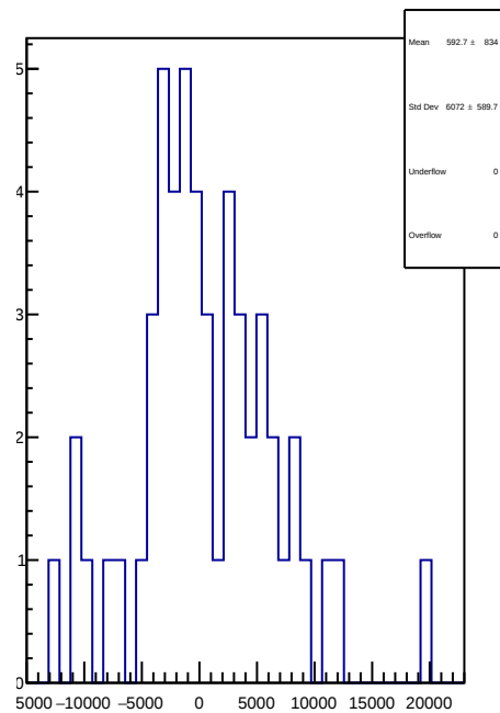
slug50: 1D Corr asym_left_avg.mean/ppb-reg_asym_left_avg.mean/ppb
