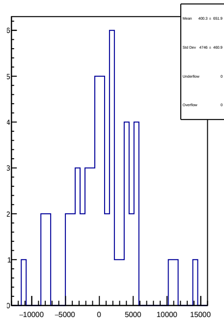
slug50: 1D Corr asym_us_dd.mean/ppb-reg_asym_us_dd.mean/ppb
