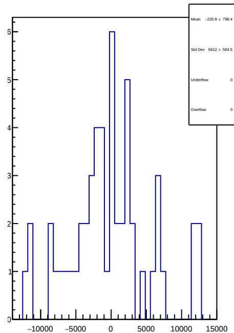
slug50: 1D Corr asym_usr.mean/ppb-reg_asym_usr.mean/ppb
