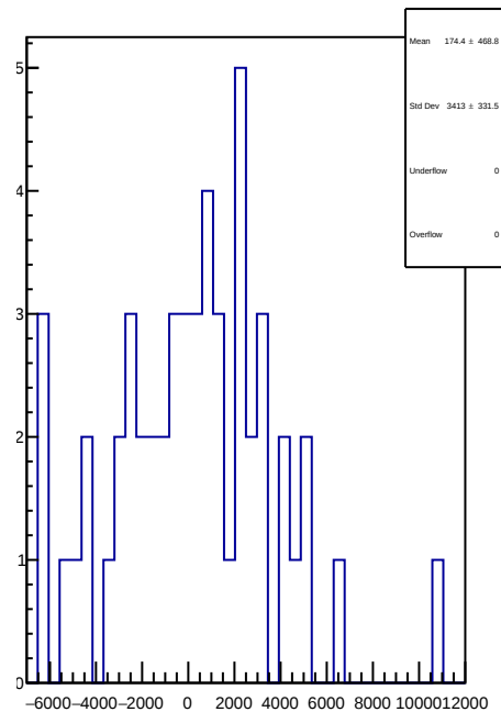
slug50: 1D Corr asym_us_avg.mean/ppb-reg_asym_us_avg.mean/ppb
