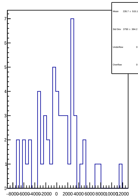
slug50: 1D Corr asym_ds_avg.mean/ppb-reg_asym_ds_avg.mean/ppb
