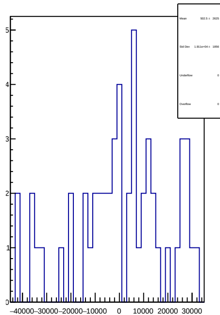
slug50: 1D Corr asym_sam5.mean/ppb-reg_asym_sam5.mean/ppb
