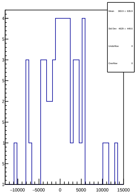
slug50: 1D Corr asym_ds_dd.mean/ppb-reg_asym_ds_dd.mean/ppb
