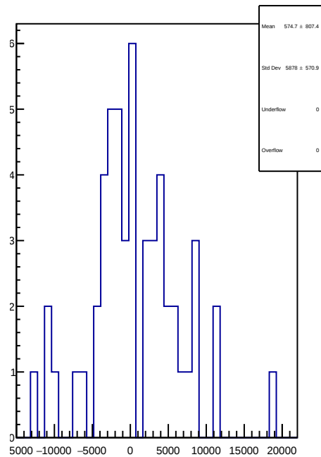
slug50: 1D Corr asym_usl.mean/ppb-reg_asym_usl.mean/ppb
