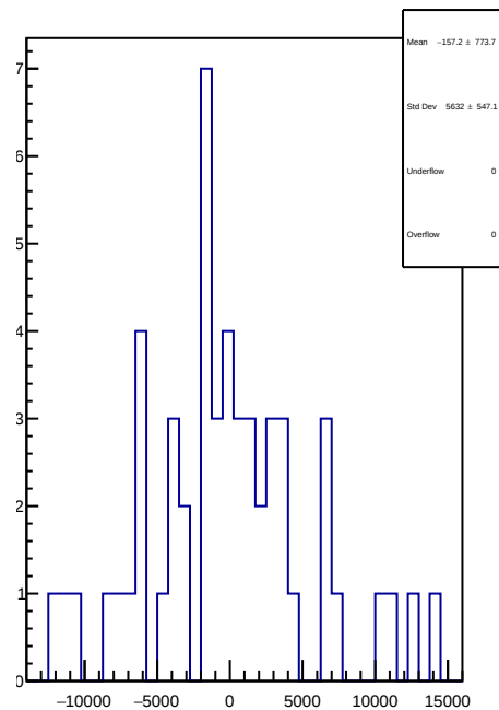
slug50: 1D Corr asym_dsr.mean/ppb-reg_asym_dsr.mean/ppb
