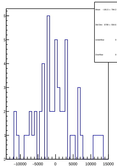
slug50: 1D Corr asym_right_avg.mean/ppb-reg_asym_right_avg.mean/ppb
