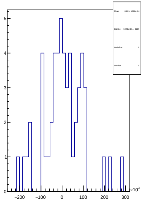
slug50: 1D Corr asym_sam3.mean/ppb-reg_asym_sam3.mean/ppb
