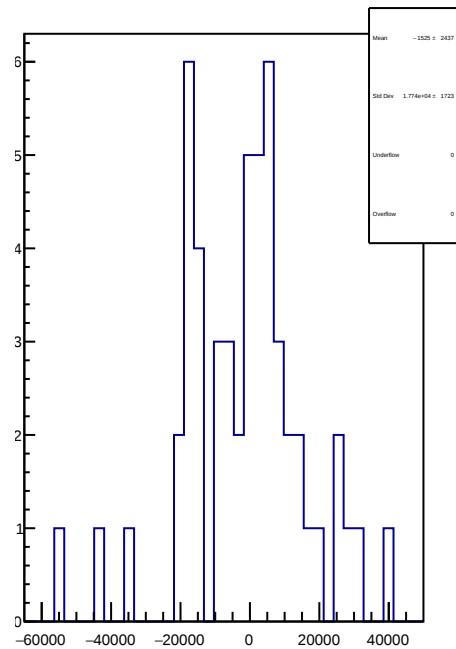
slug50: 1D Corr asym_sam7.mean/ppb-reg_asym_sam7.mean/ppb
