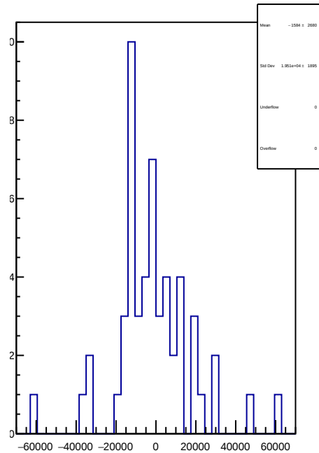
slug50: 1D Corr asym_sam8.mean/ppb-reg_asym_sam8.mean/ppb
