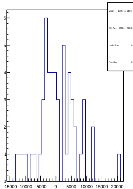
slug50: 1D Corr asym_dsl.mean/ppb-reg_asym_dsl.mean/ppb
