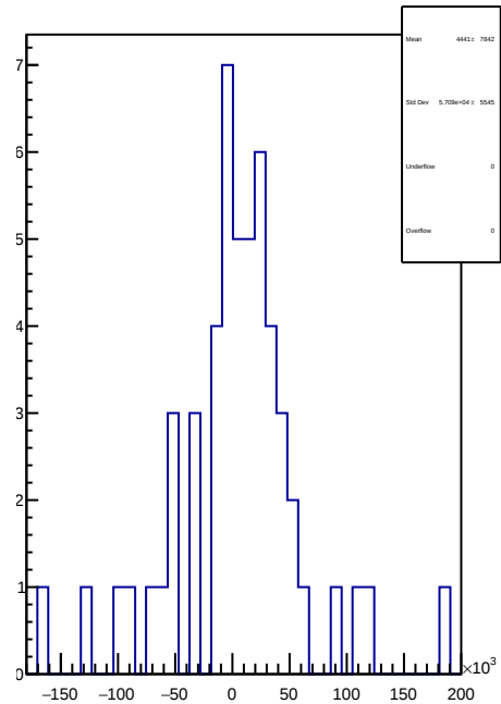
slug50: 1D Corr asym_sam4.mean/ppb-reg_asym_sam4.mean/ppb
