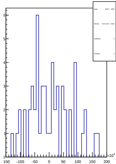
slug50: 1D Corr asym_sam2.mean/ppb-reg_asym_sam2.mean/ppb
