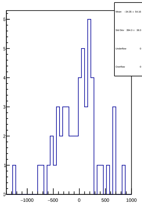
slug50: 1D Corr asym_right_dd.mean/ppb-reg_asym_right_dd.mean/ppb
