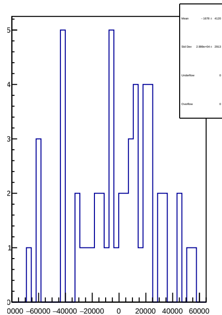
slug50: 1D Corr asym_sam6.mean/ppb-reg_asym_sam6.mean/ppb
