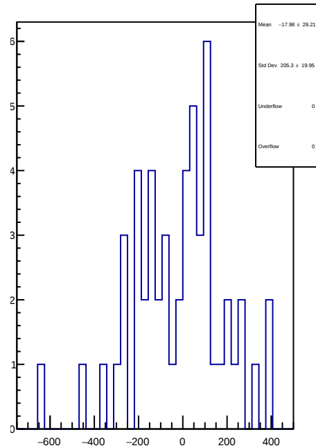
slug50: 1D Corr asym_left_dd.mean/ppb-reg_asym_left_dd.mean/ppb
