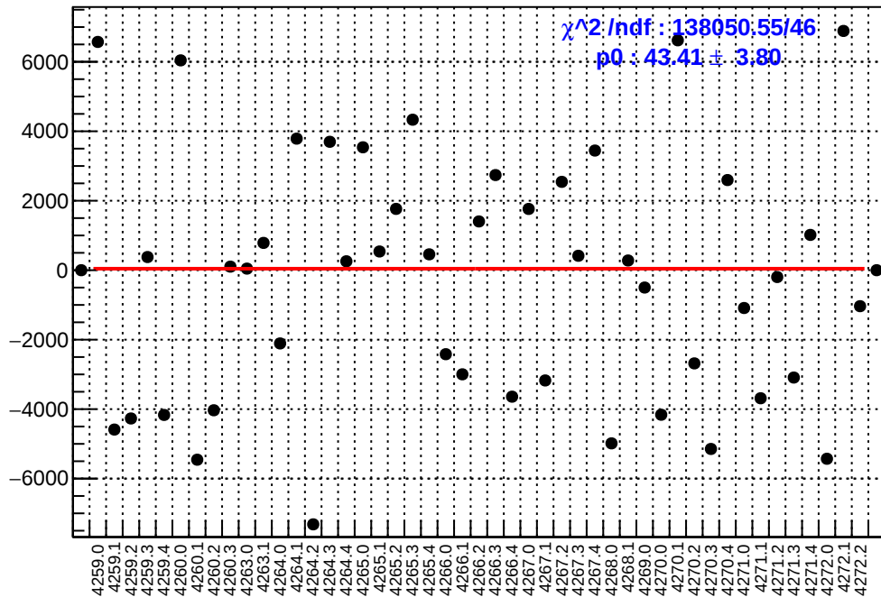
slug51: asym_ds_avg.mean/ppb-reg_asym_ds_avg.mean/ppb
