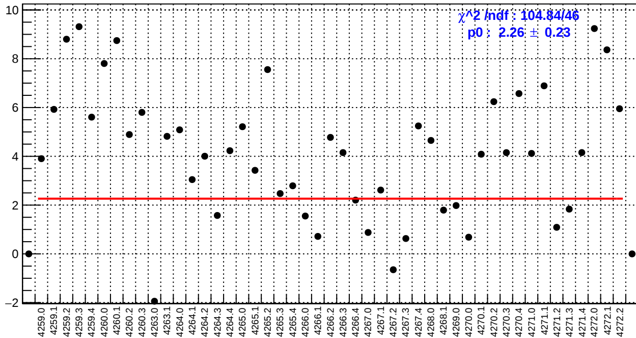
slug51: left_avg_bpm4aX/(ppb/nm)
