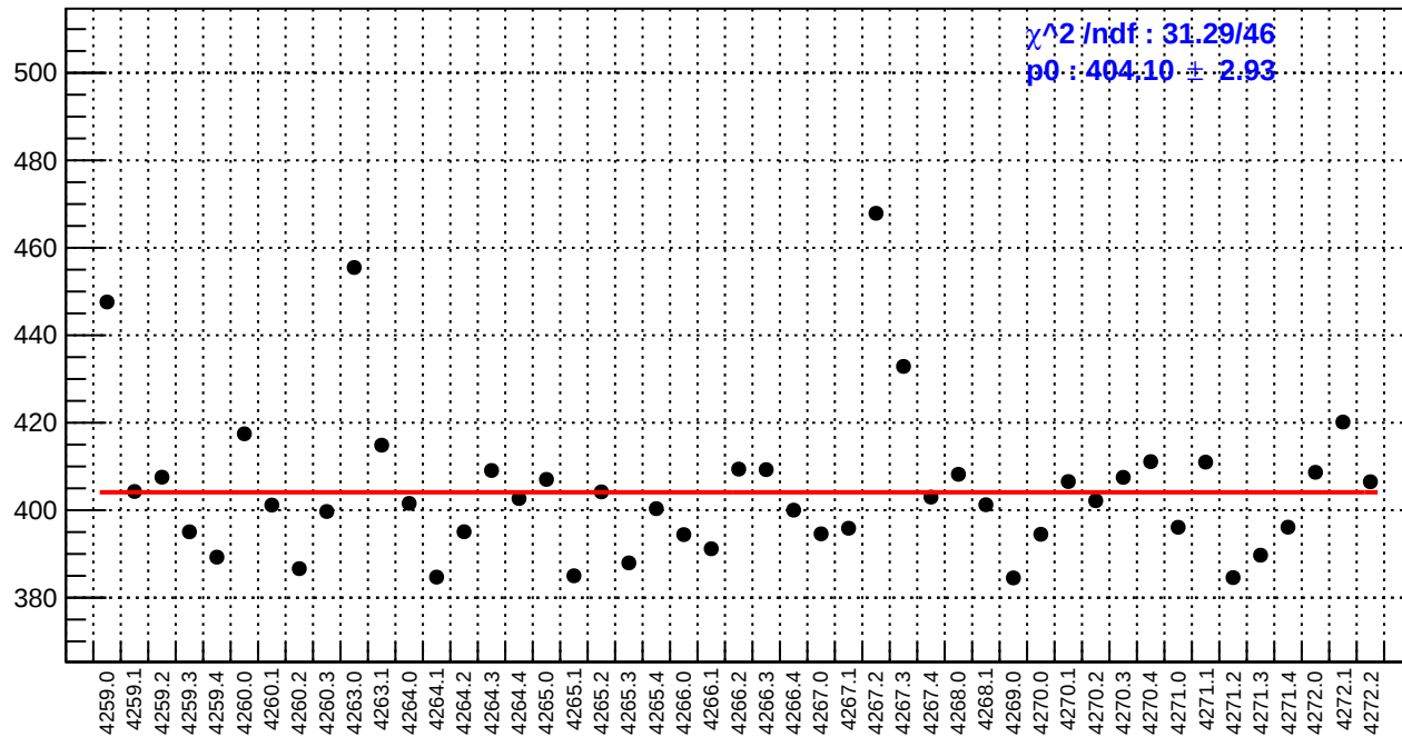
slug51: reg_asym_atr1l2_avg.rms/ppm
