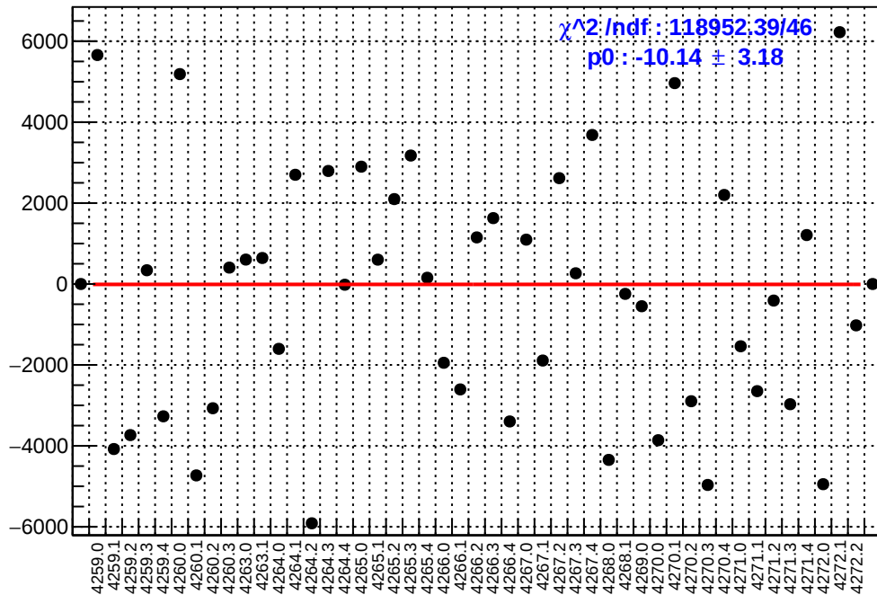
slug51: asym_us_avg.mean/ppb-reg_asym_us_avg.mean/ppb
