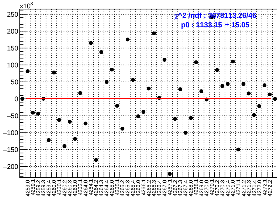
slug51: asym_sam3.mean/ppb-reg_asym_sam3.mean/ppb
