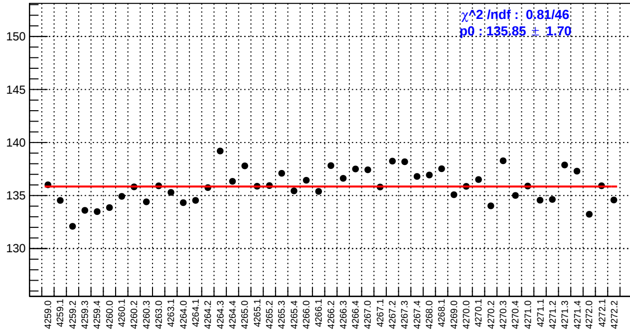
slug51: reg_asym_usr.rms/ppm
