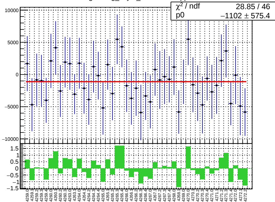
slug51: reg_asym_sam5.mean/ppb
