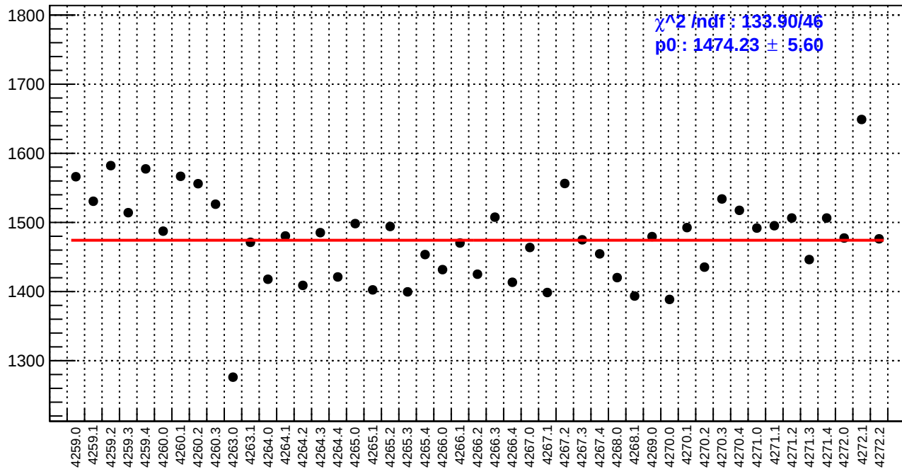
slug51: diff_bpm4aX.rms/nm
