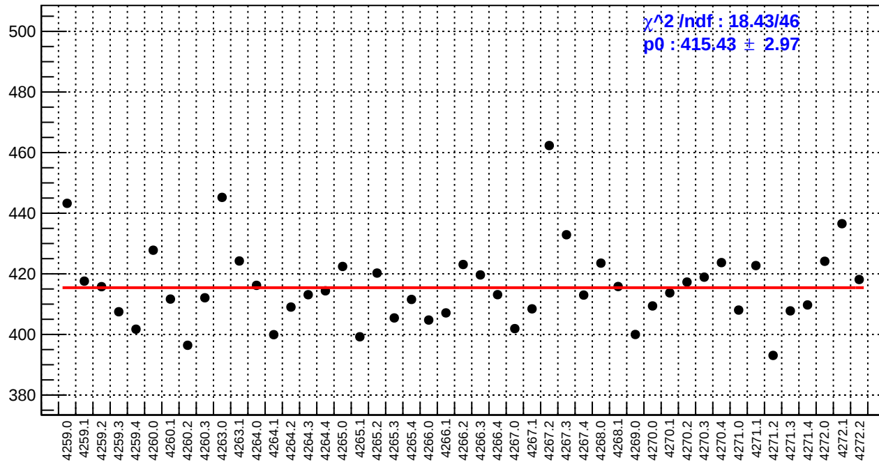
slug51: reg_asym_atr_avg.rms/ppm
