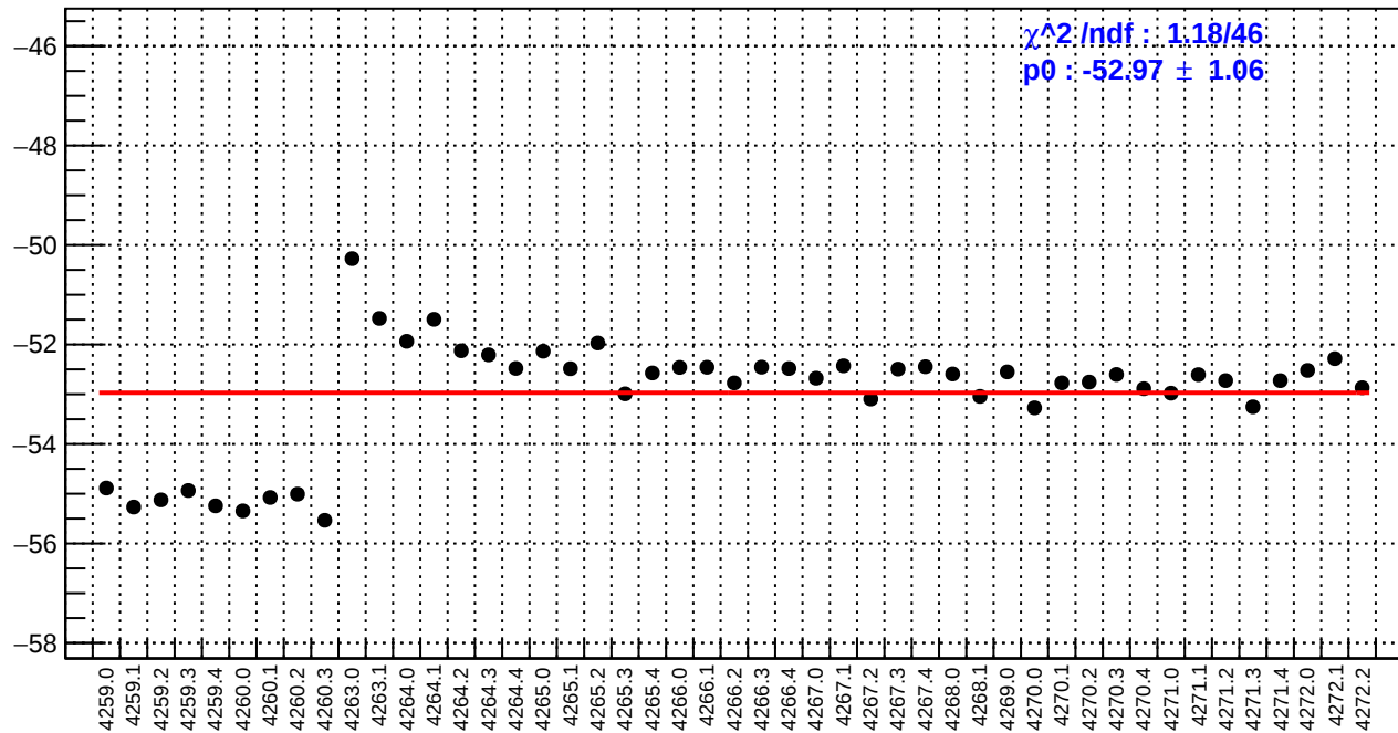
slug51: us_avg_bpm12X/(ppb/nm)
