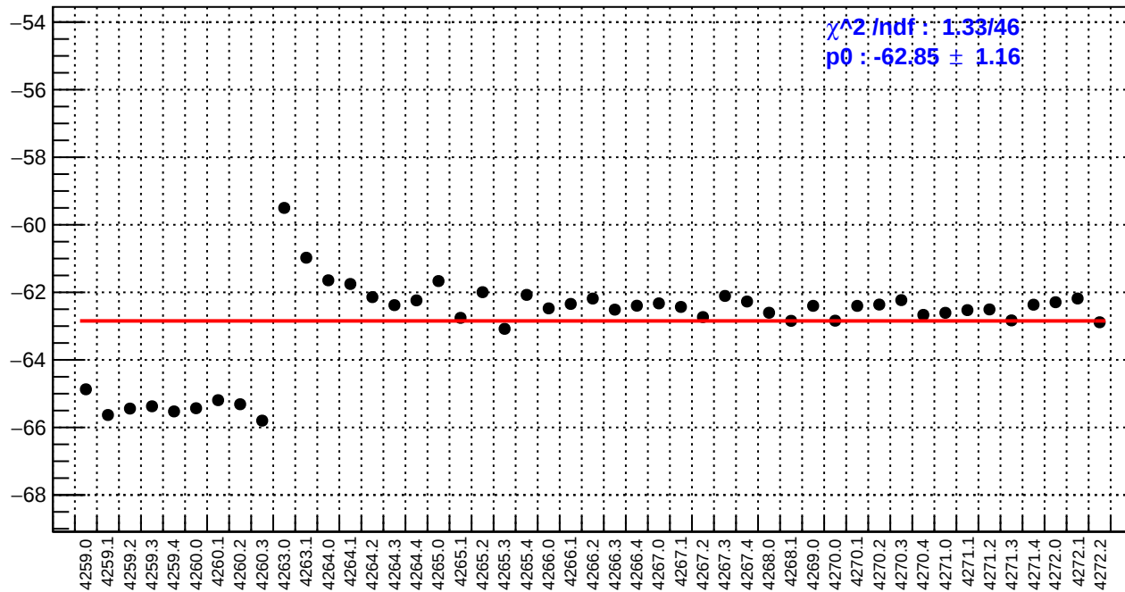
slug51: right_avg_bpm12X/(ppb/nm)
