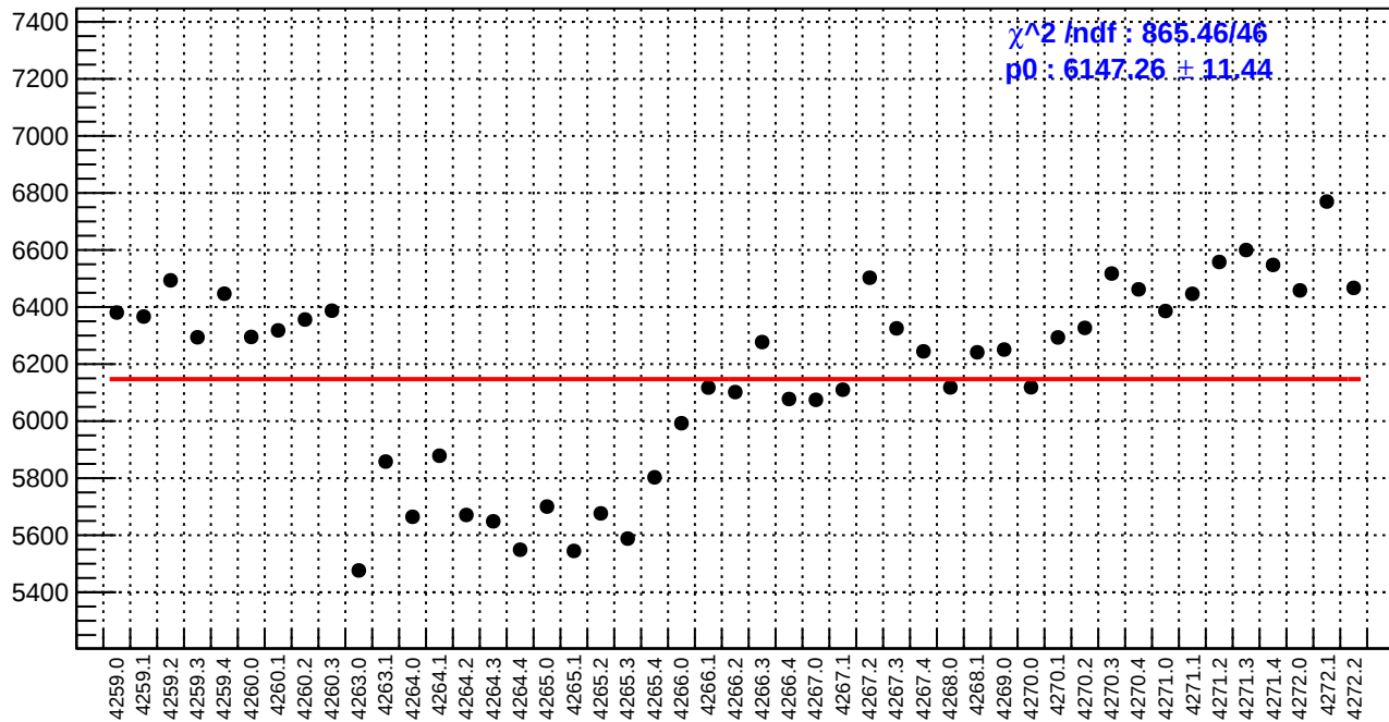
slug51: diff_bpm11X.rms/nm
