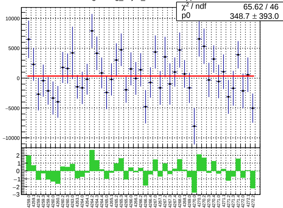
slug51: reg_asym_sam7.mean/ppb
