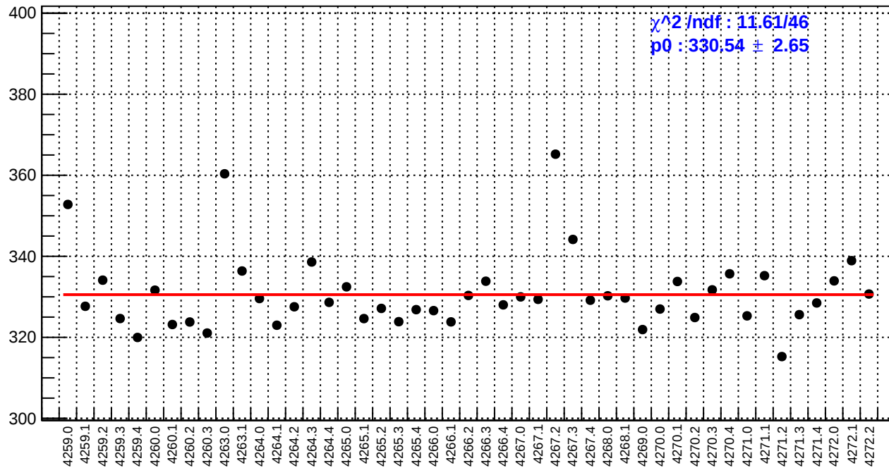
slug51: reg_asym_atl_dd.rms/ppm
