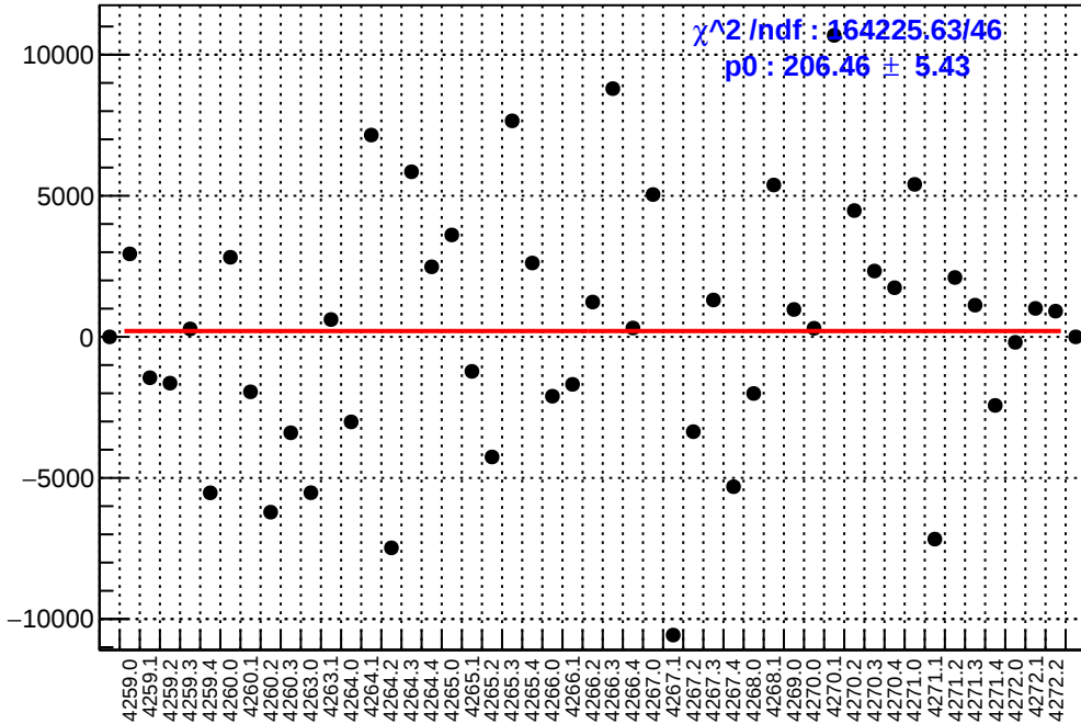
slug51: asym_ds_dd.mean/ppb-reg_asym_ds_dd.mean/ppb
