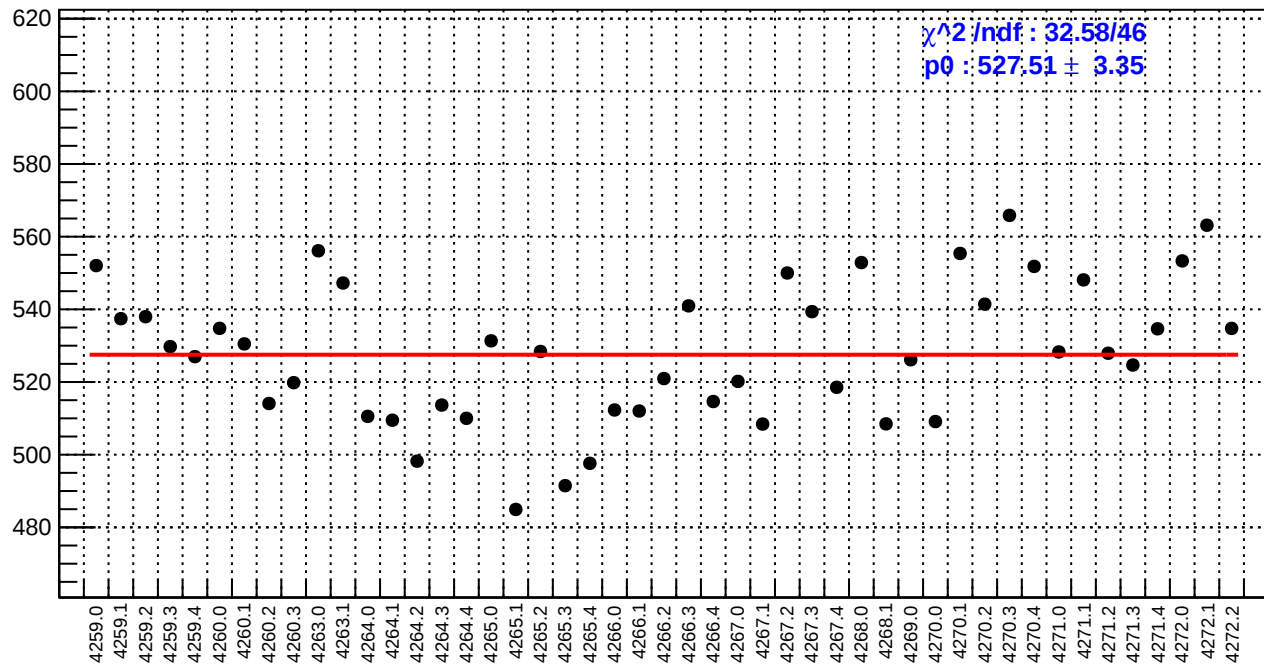
slug51: reg_asym_sam6.rms/ppm
