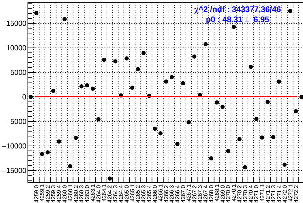
slug51: asym_atl_avg.mean/ppb-reg_asym_atl_avg.mean/ppb
