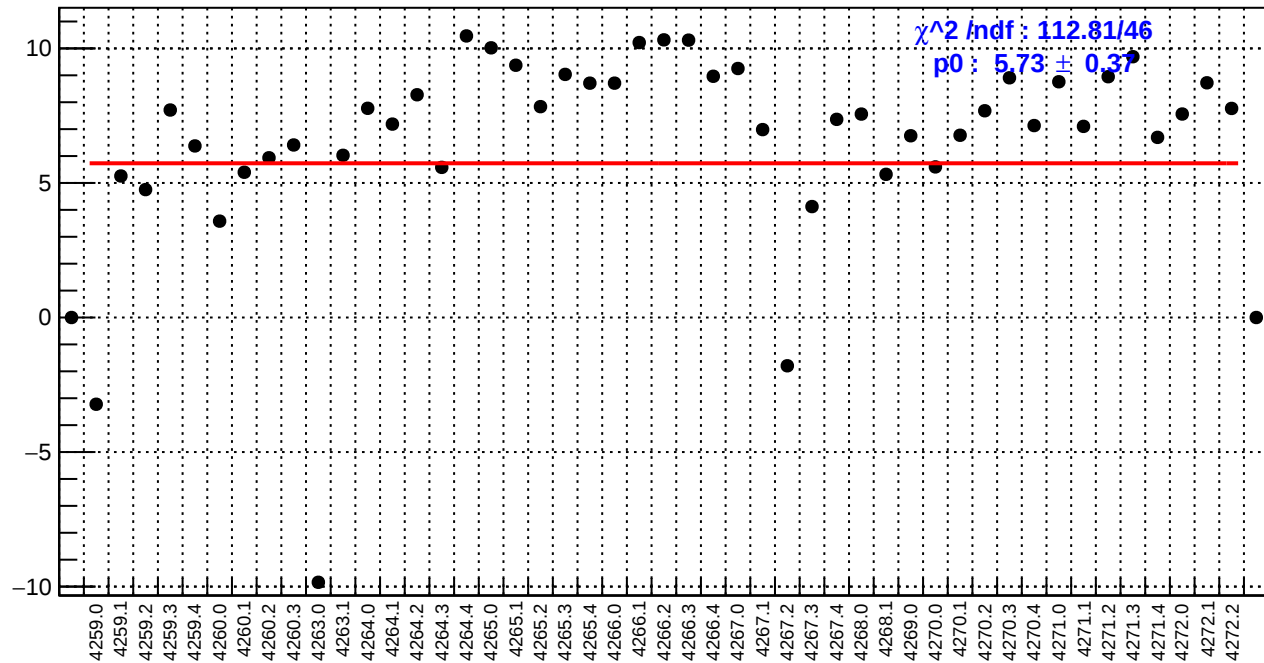
slug51: us_avg_bpm4eY/(ppb/nm)
