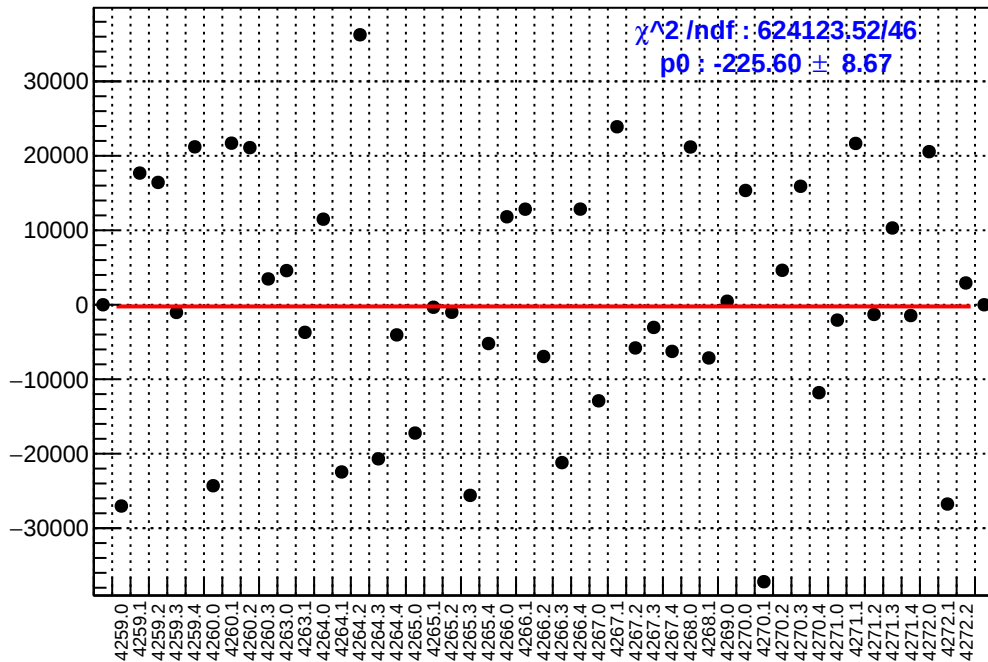
slug51: asym_atl_dd.mean/ppb-reg_asym_atl_dd.mean/ppb
