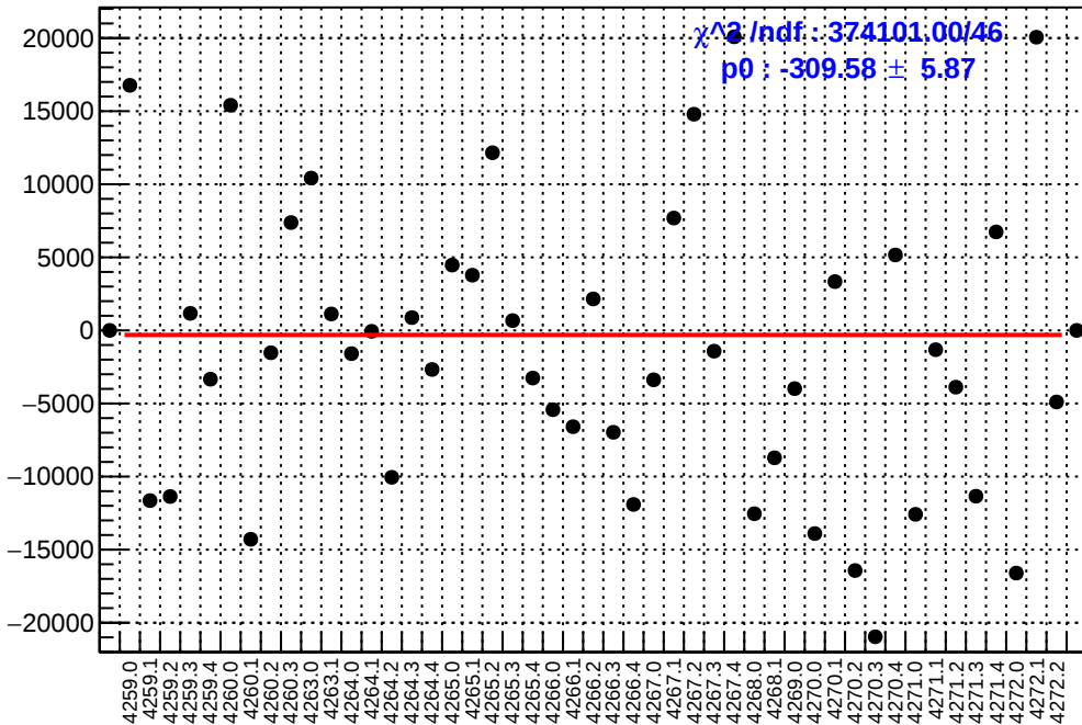
slug51: asym_atl1r2_avg.mean/ppb-reg_asym_atl1r2_avg.mean/ppb
