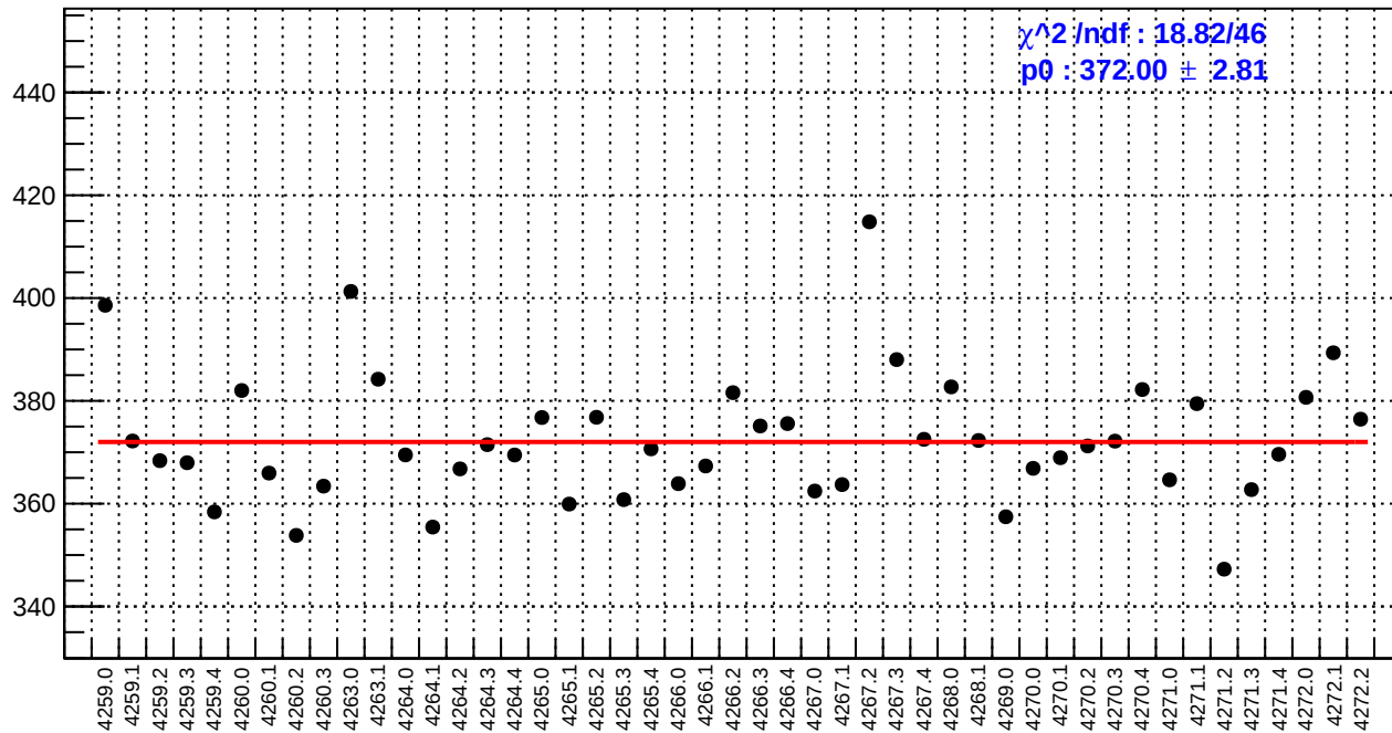
slug51: reg_asym_at2_avg.rms/ppm
