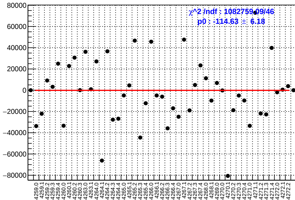
slug51: asym_sam6.mean/ppb-reg_asym_sam6.mean/ppb
