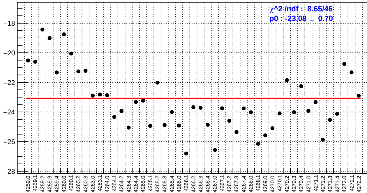
slug51: us_avg_bpm4aX/(ppb/nm)
