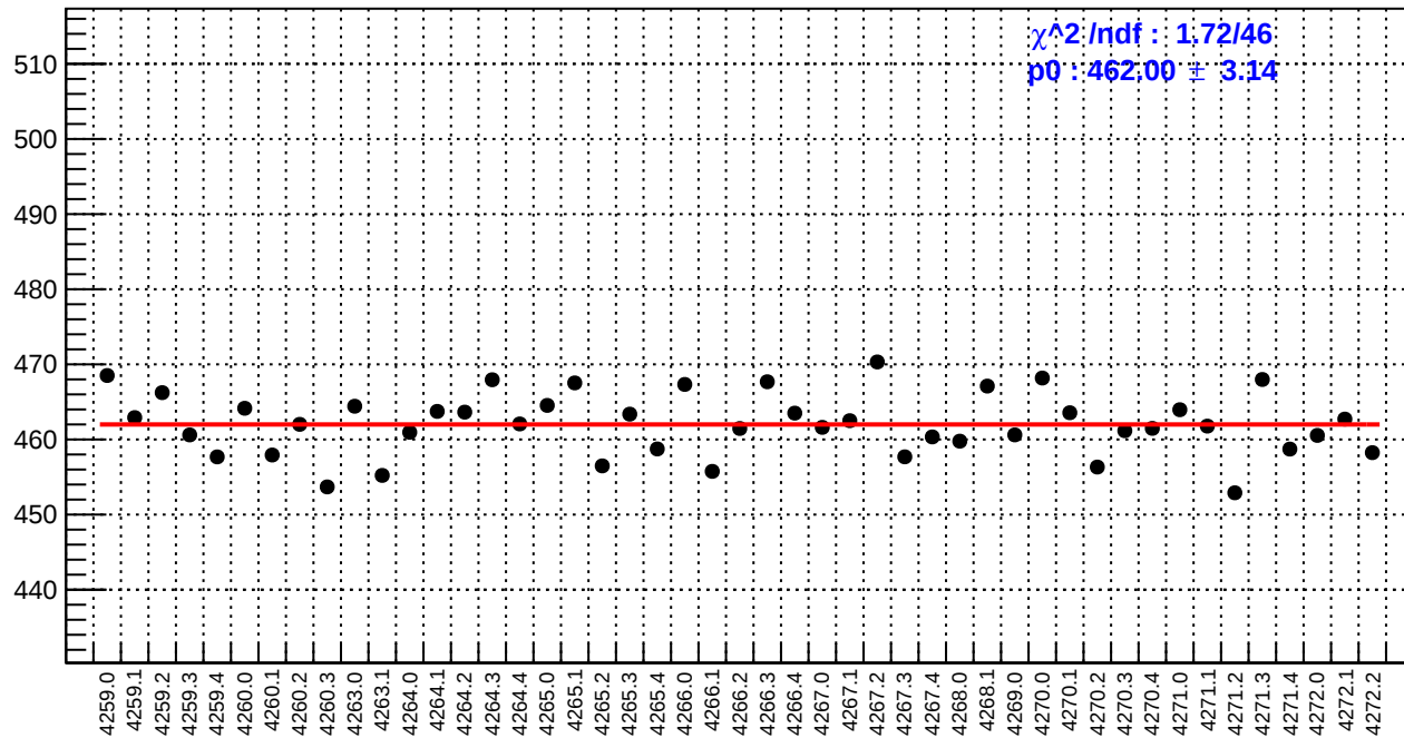
slug51: reg_asym_atl1.rms/ppm
