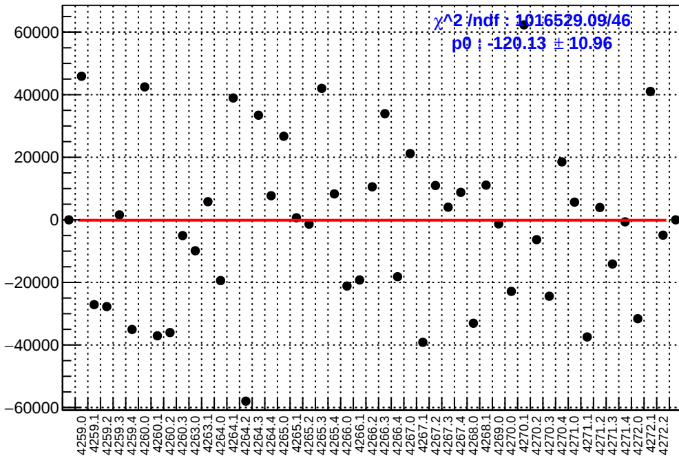
slug51: asym_atr1.mean/ppb-reg_asym_atr1.mean/ppb
