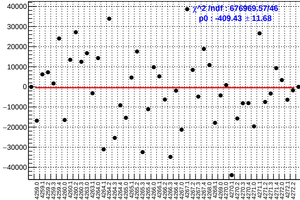
slug51: asym_sam7.mean/ppb-reg_asym_sam7.mean/ppb
