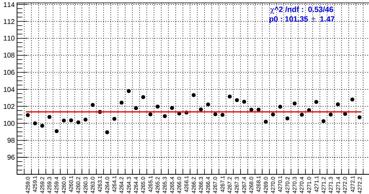
slug51: reg_asym_us_avg.rms/ppm
