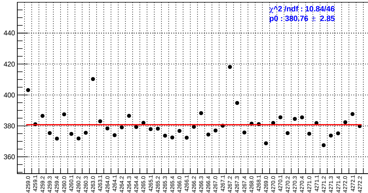
slug51: reg_asym_at1_dd.rms/ppm
