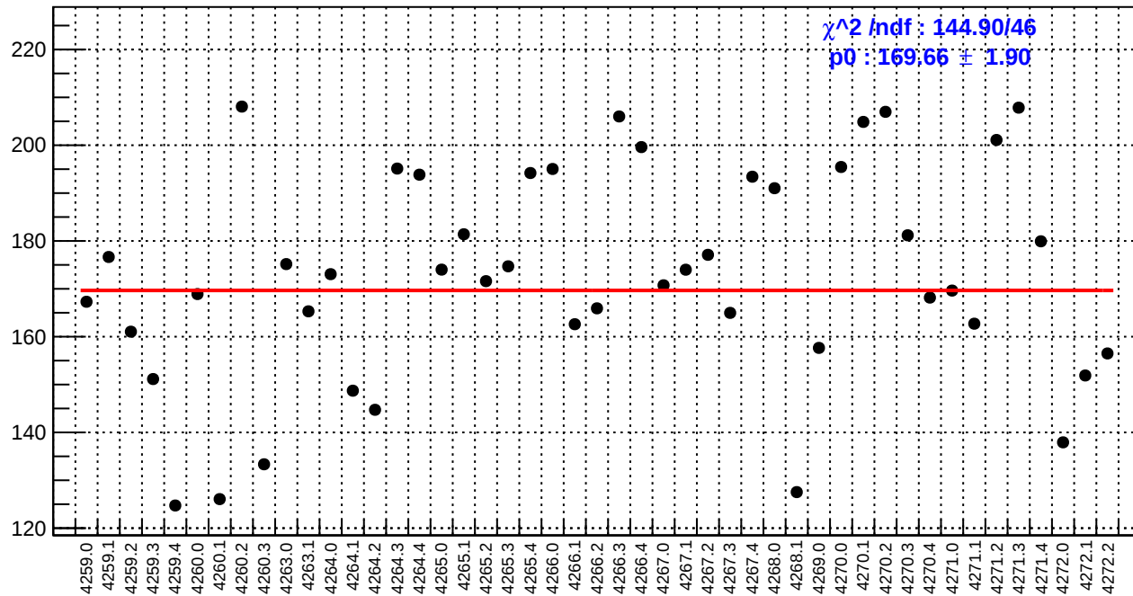
slug51: asym_bcm_an_ds3.rms/ppm
