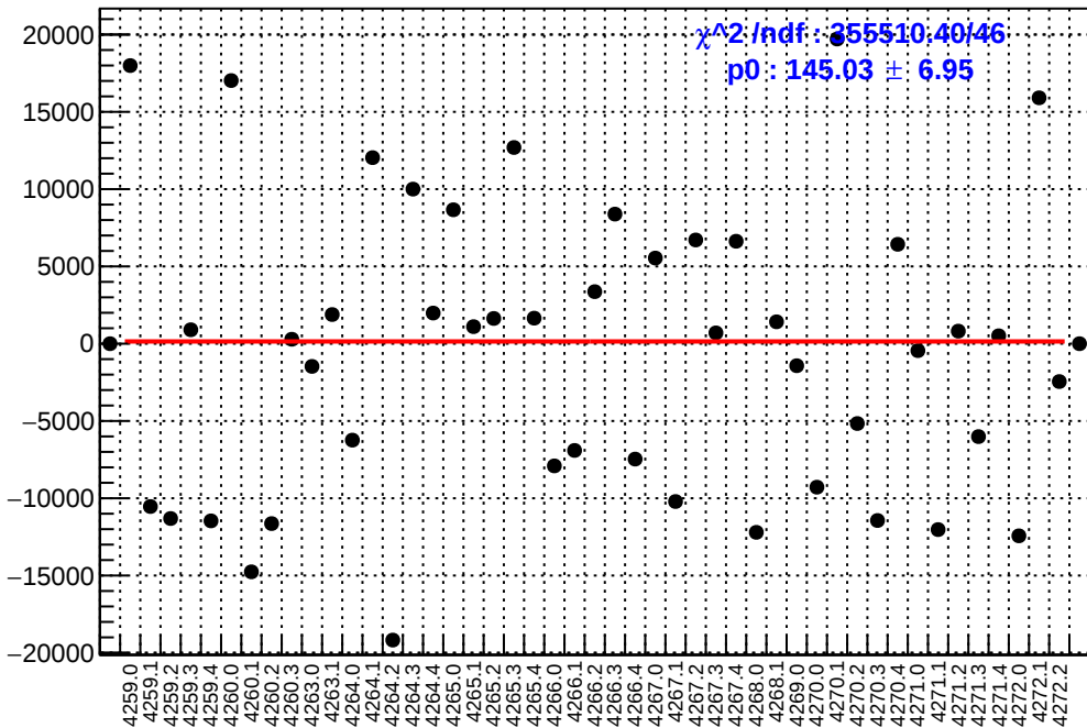
slug51: asym_at1_avg.mean/ppb-reg_asym_at1_avg.mean/ppb
