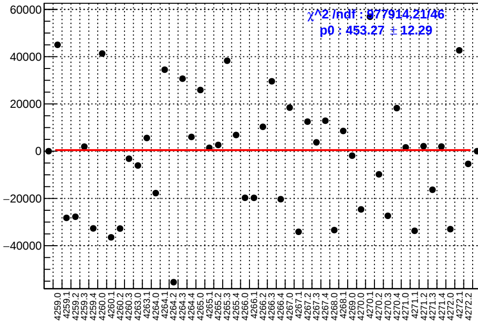
slug51: asym_atr1l2_avg.mean/ppb-reg_asym_atr1l2_avg.mean/ppb
