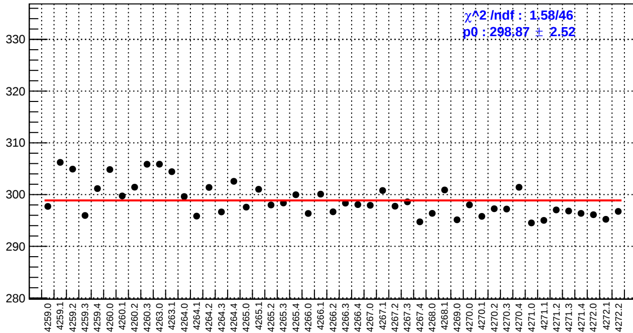
slug51: reg_asym_atr1l2_dd.rms/ppm
