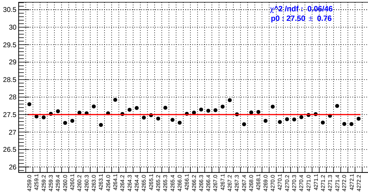
slug51: reg_asym_right_dd.rms/ppm
