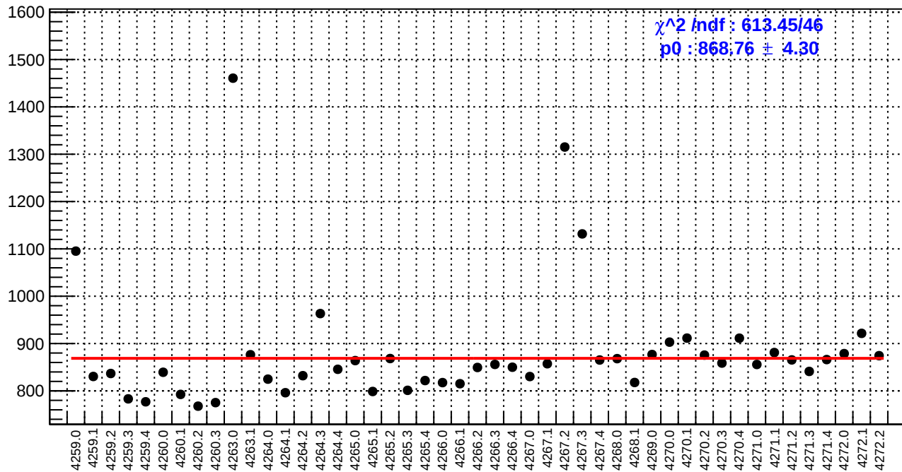
slug51: reg_asym_sam3.rms/ppm
