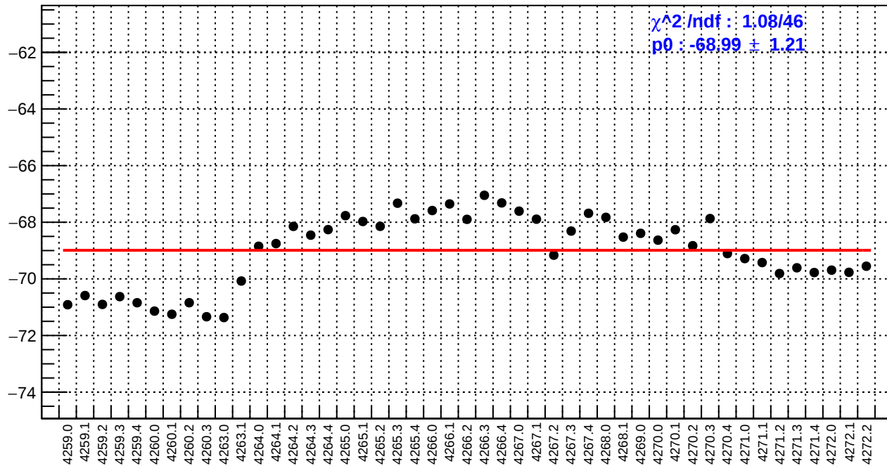
slug51: left_avg_bpm4eX/(ppb/nm)
