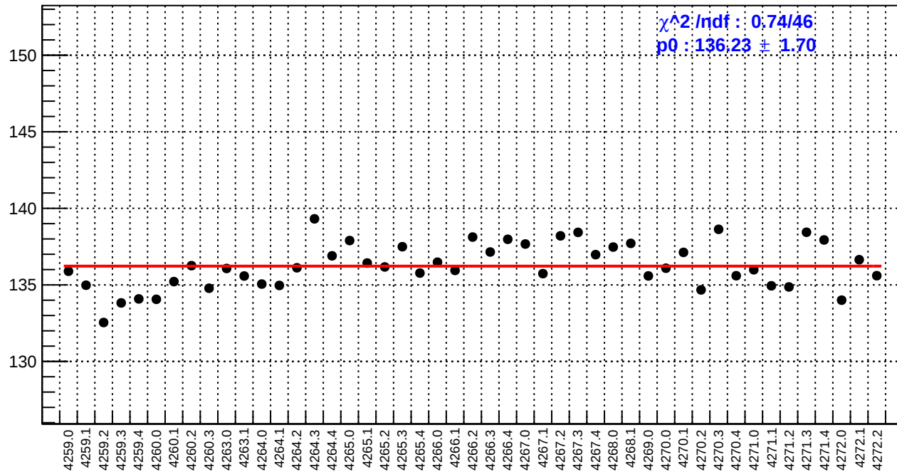
slug51: reg_asym_right_avg.rms/ppm
