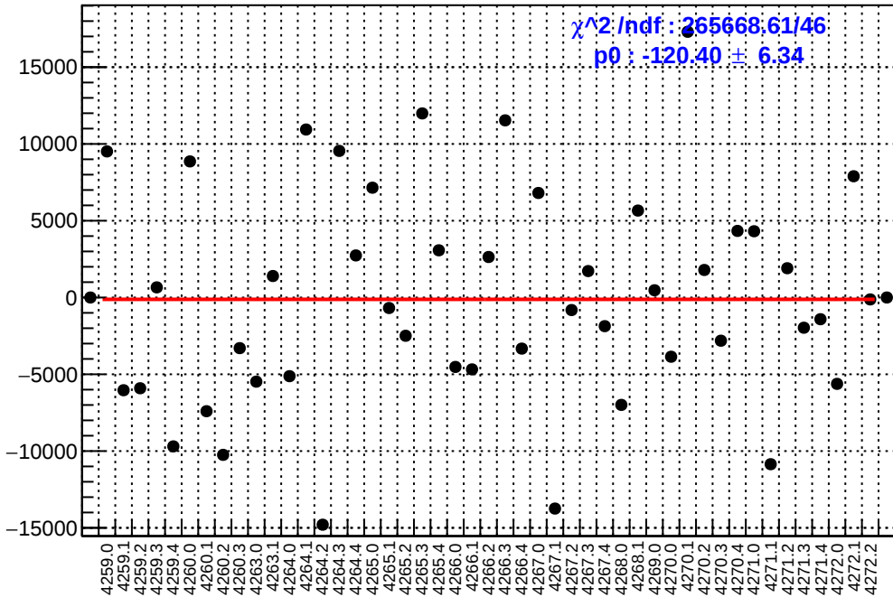
slug51: asym_dsl.mean/ppb-reg_asym_dsl.mean/ppb
