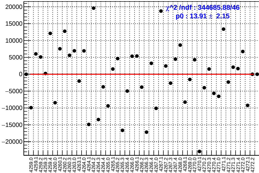
slug51: asym_atl1.mean/ppb-reg_asym_atl1.mean/ppb
