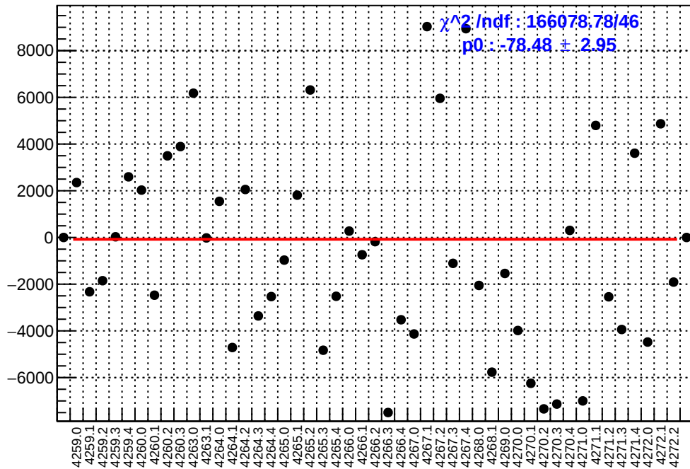
slug51: asym_usr.mean/ppb-reg_asym_usr.mean/ppb
