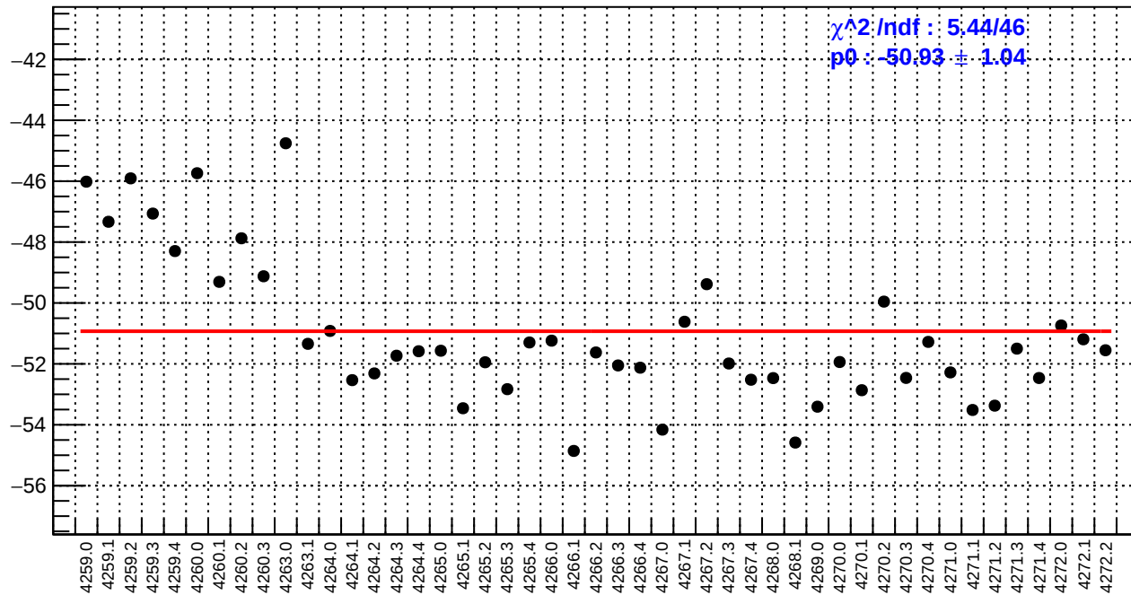
slug51: right_avg_bpm4aX/(ppb/nm)
