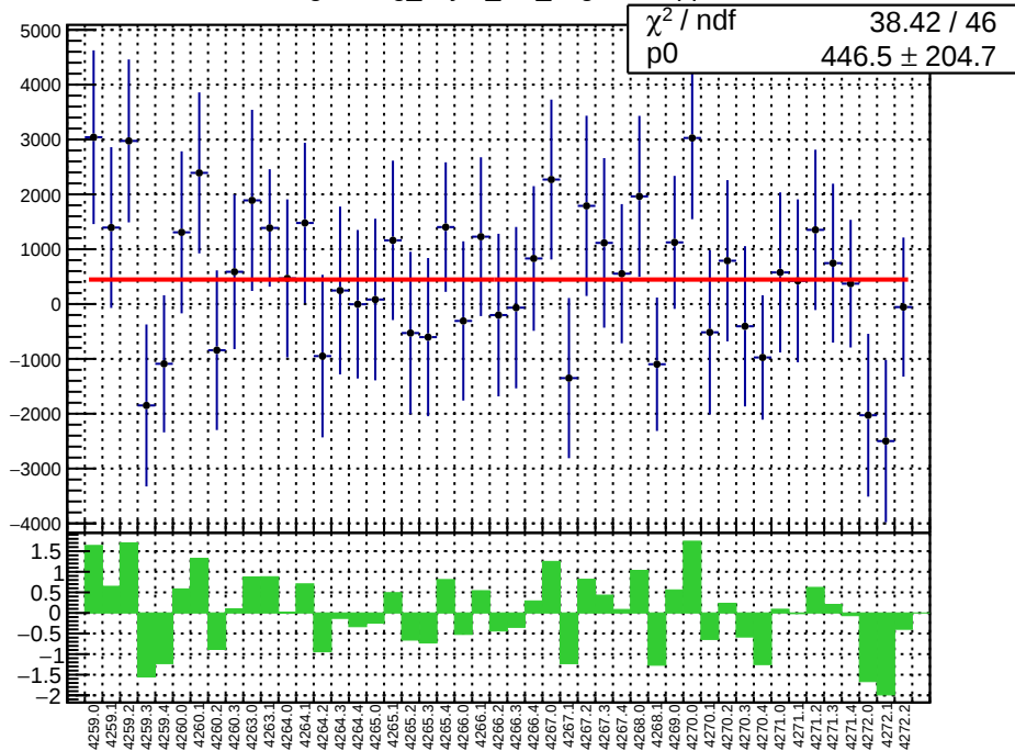
slug51: reg_asym_left_avg.mean/ppb
