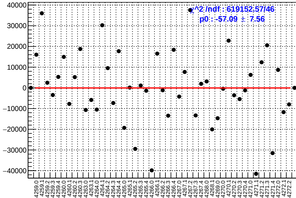
slug51: asym_sam1.mean/ppb-reg_asym_sam1.mean/ppb
