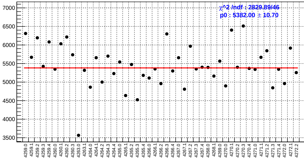
slug51: diff_bpm4eY.rms/nm
