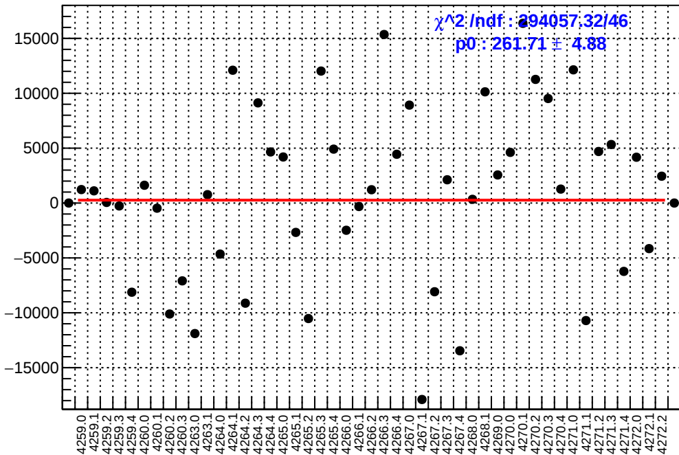
slug51: asym_atr_dd.mean/ppb-reg_asym_atr_dd.mean/ppb
