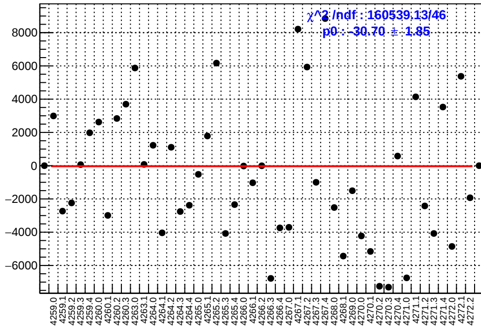
slug51: asym_right_avg.mean/ppb-reg_asym_right_avg.mean/ppb
