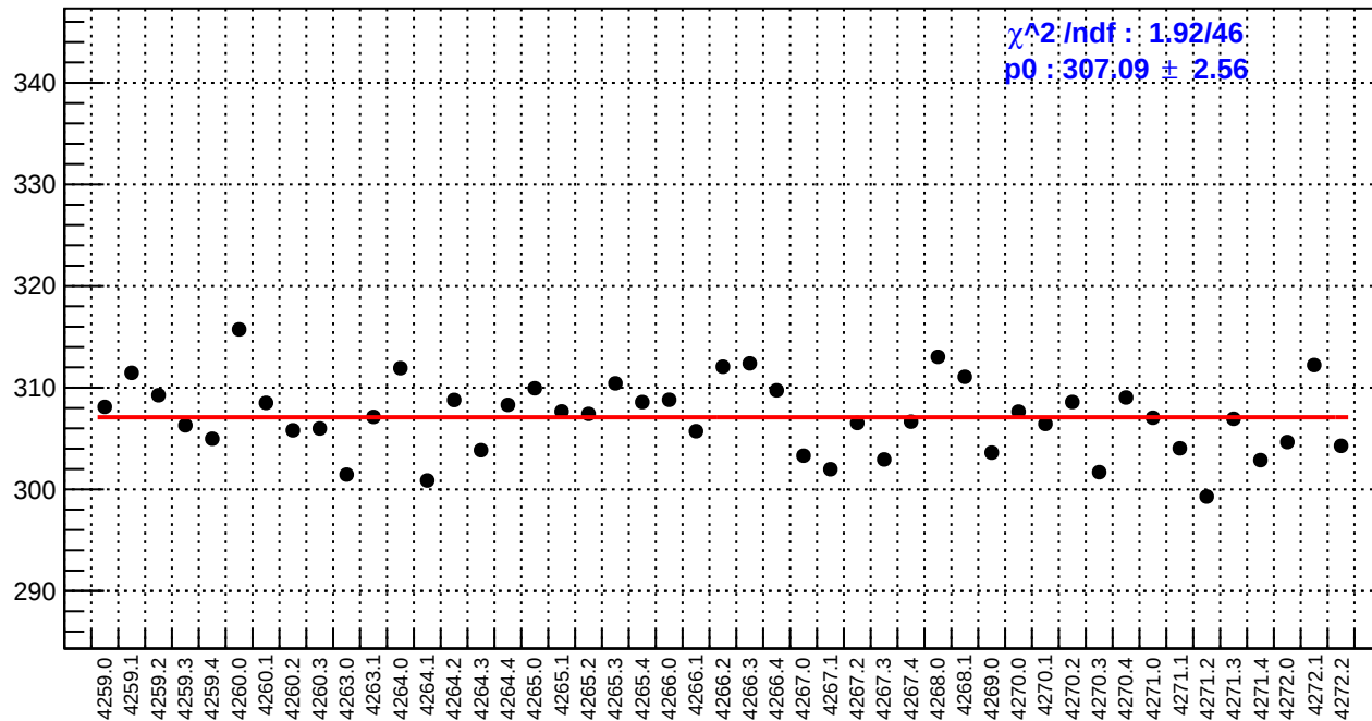
slug51: reg_asym_atl1r2_avg.rms/ppm
