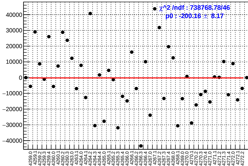
slug51: asym_sam8.mean/ppb-reg_asym_sam8.mean/ppb
