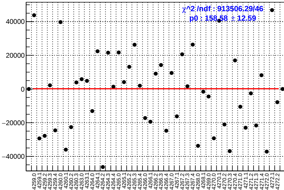
slug51: asym_at2_avg.mean/ppb-reg_asym_at2_avg.mean/ppb
