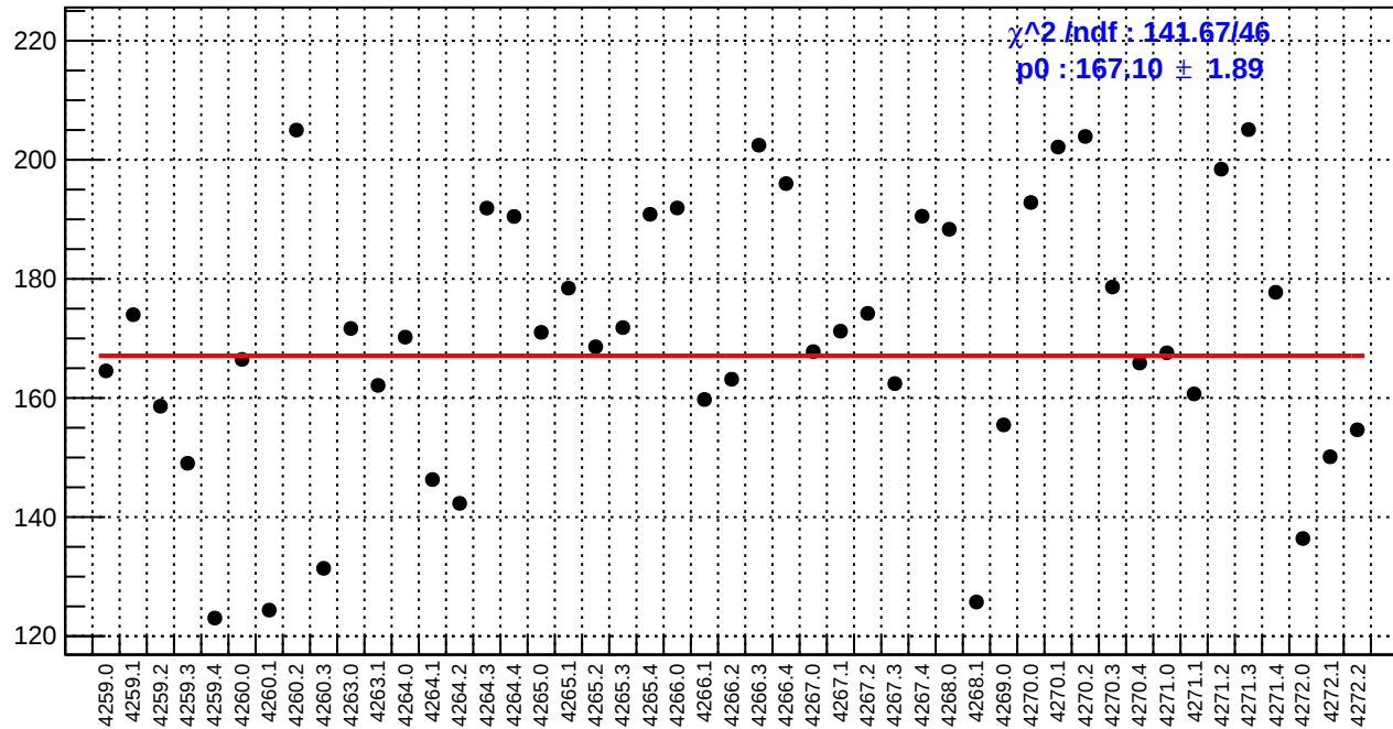
slug51: asym_bcm_an_ds.rms/ppm
