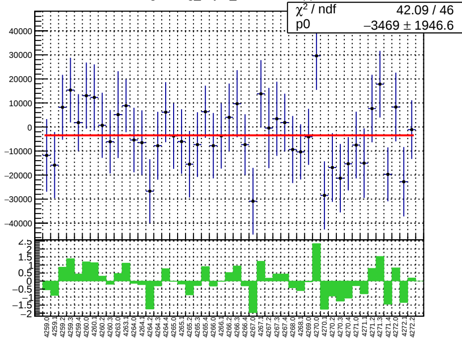
slug51: reg_asym_sam4.mean/ppb
