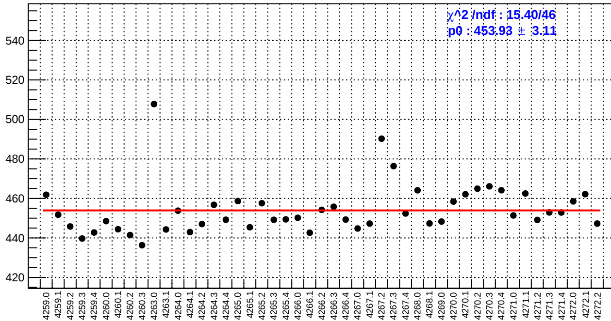
slug51: reg_asym_sam8.rms/ppm
