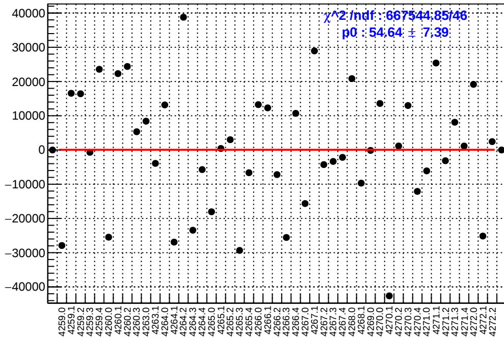
slug51: asym_at1_dd.mean/ppb-reg_asym_at1_dd.mean/ppb
