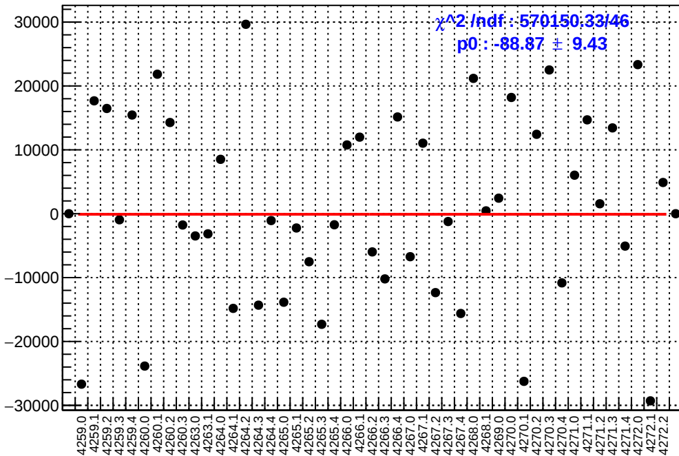
slug51: asym_atl1r2_dd.mean/ppb-reg_asym_atl1r2_dd.mean/ppb
