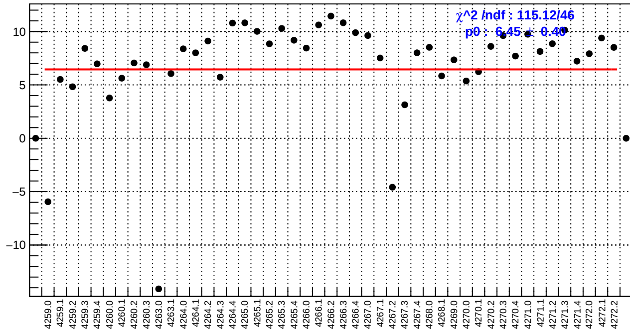
slug51: ds_avg_bpm4eY/(ppb/nm)
