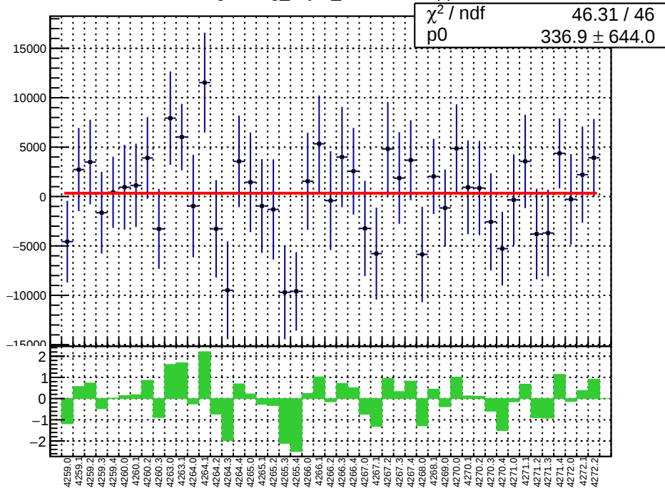
slug51: reg_asym_sam1.mean/ppb
