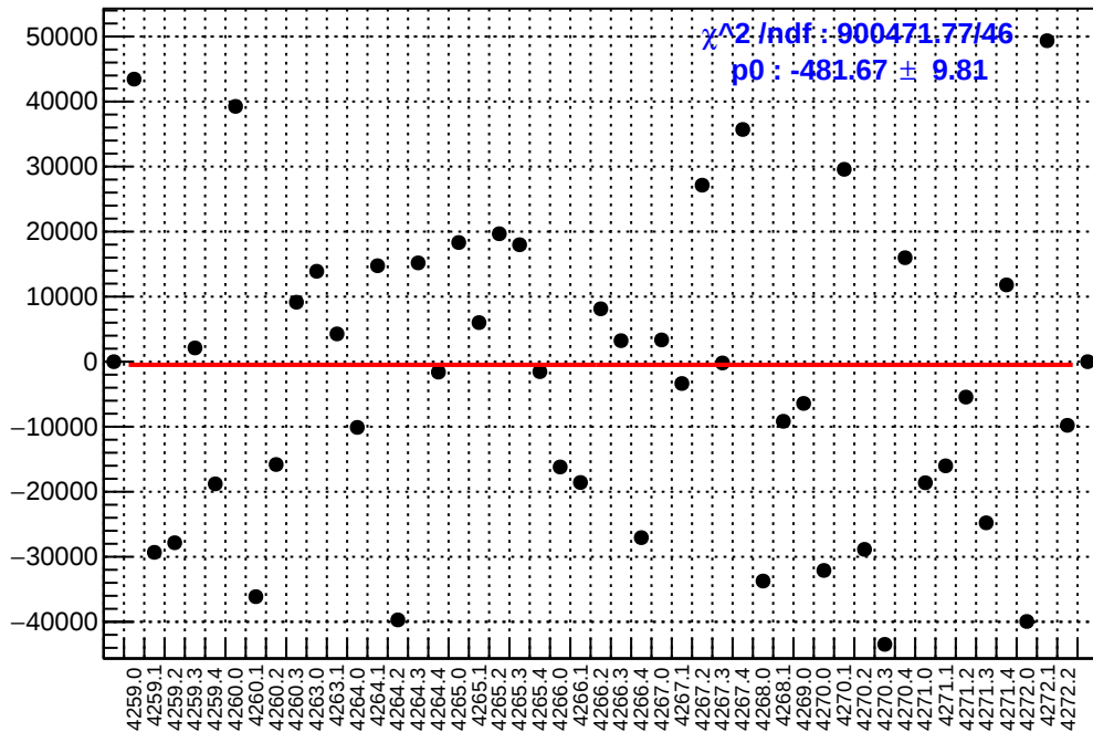
slug51: asym_atr2.mean/ppb-reg_asym_atr2.mean/ppb
