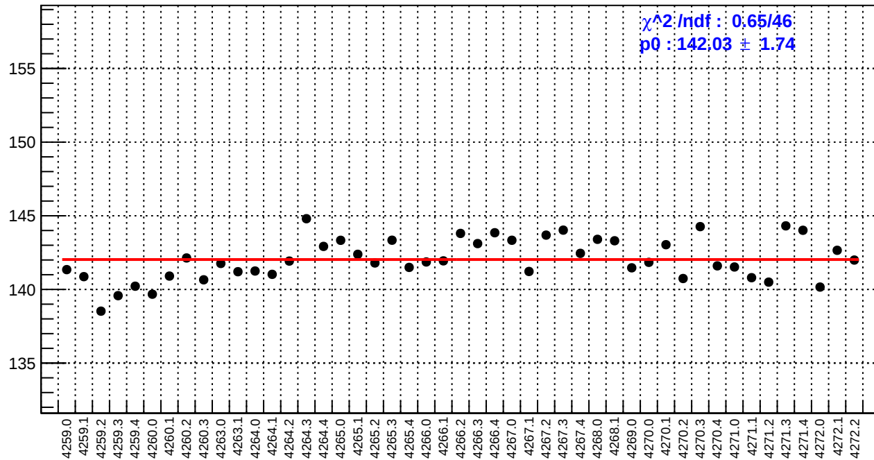
slug51: reg_asym_dsr.rms/ppm
