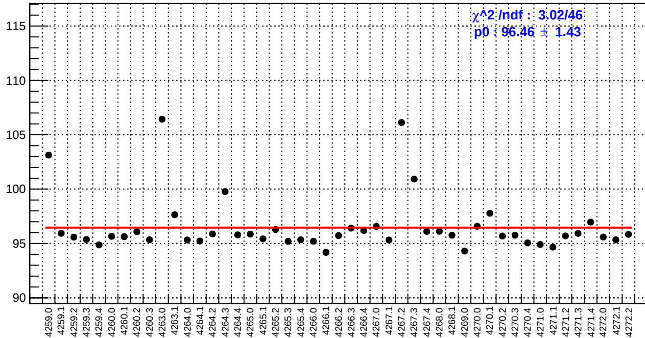
slug51: reg_asym_ds_dd.rms/ppm
