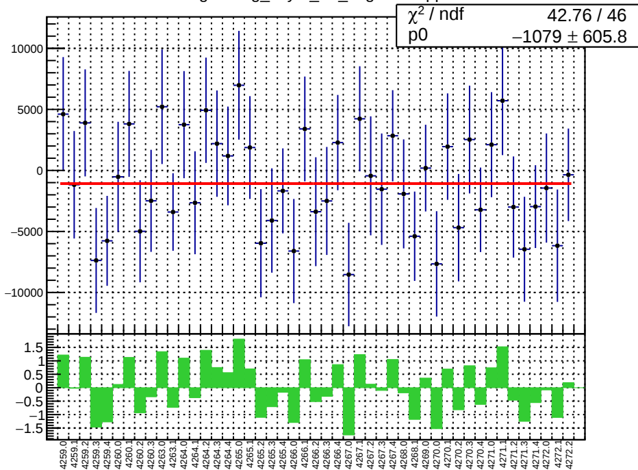
slug51: reg_asym_atr_avg.mean/ppb
