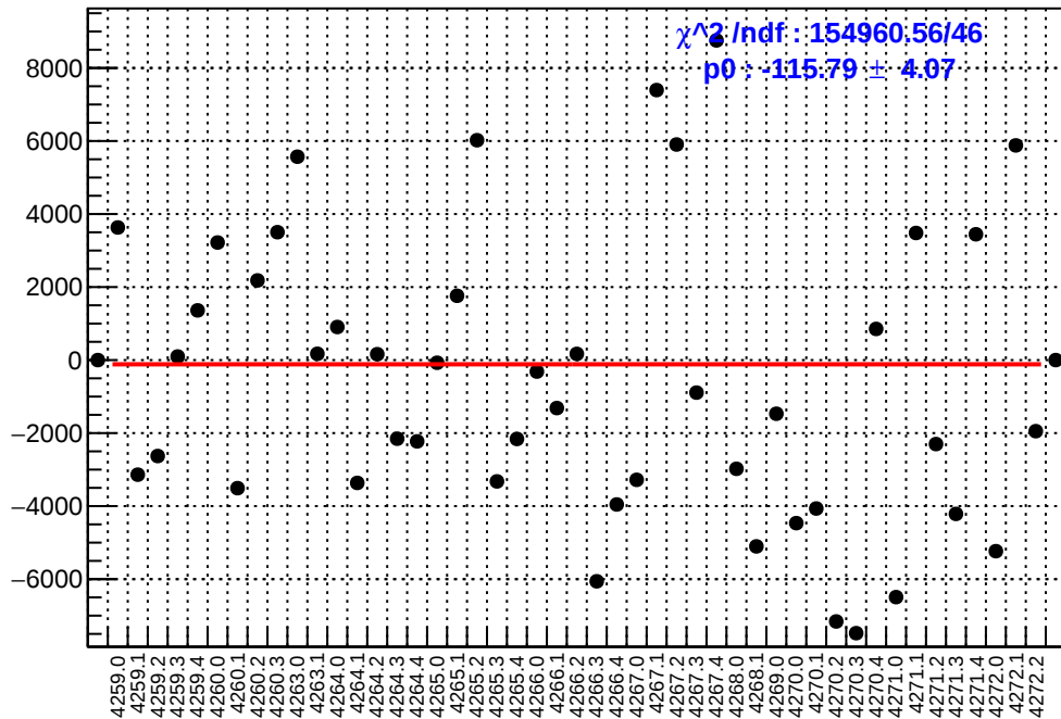
slug51: asym_dsr.mean/ppb-reg_asym_dsr.mean/ppb
