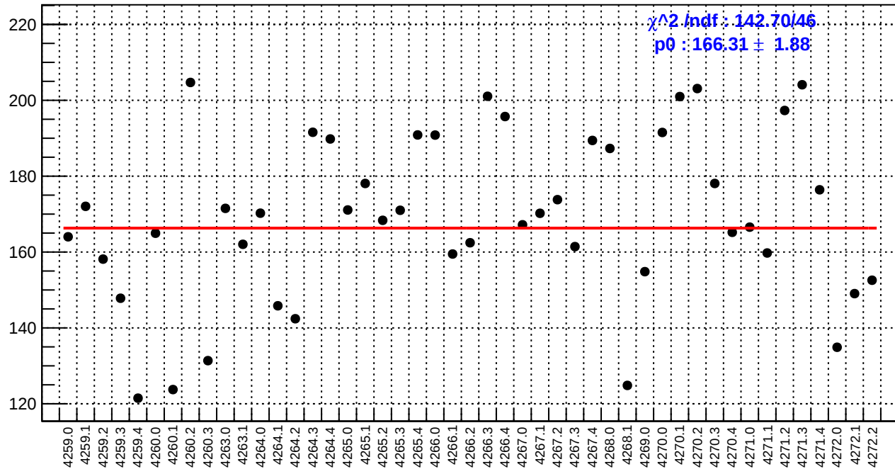
slug51: asym_bcm_an_us.rms/ppm
