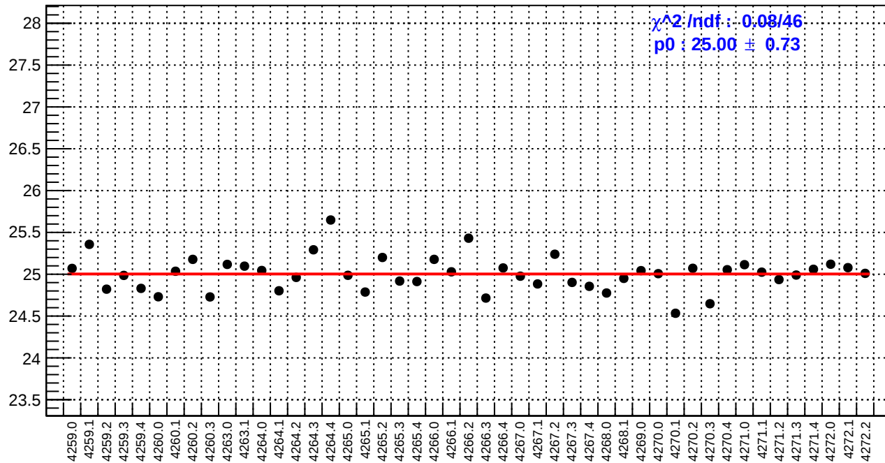
slug51: reg_asym_left_dd.rms/ppm
