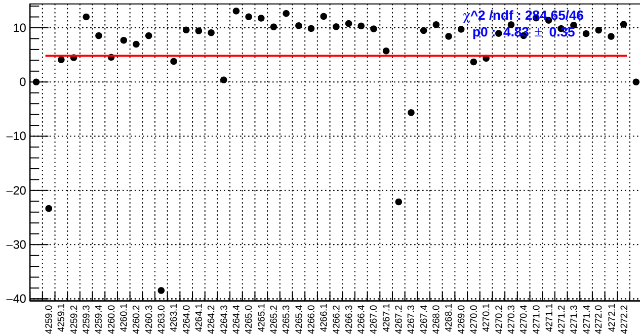
slug51: dsl_bpm4eY/(ppb/nm)
