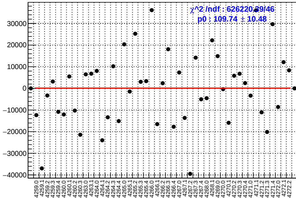
slug51: asym_sam5.mean/ppb-reg_asym_sam5.mean/ppb
