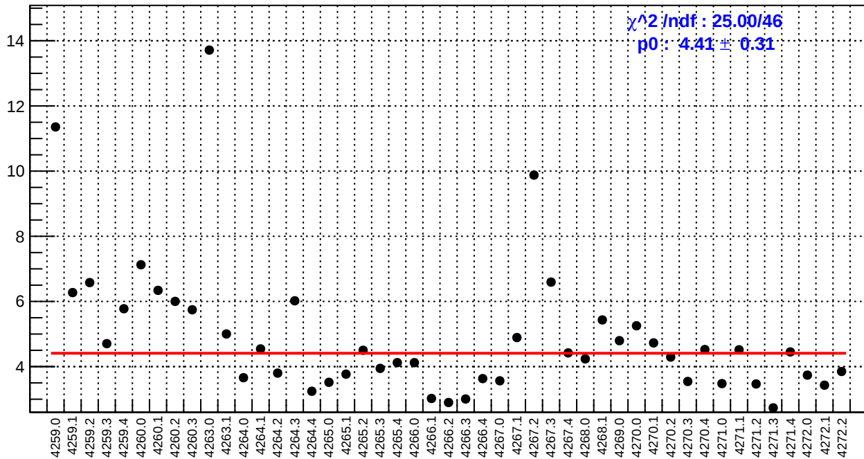
slug51: us_avg_bpm4aY/(ppb/nm)
