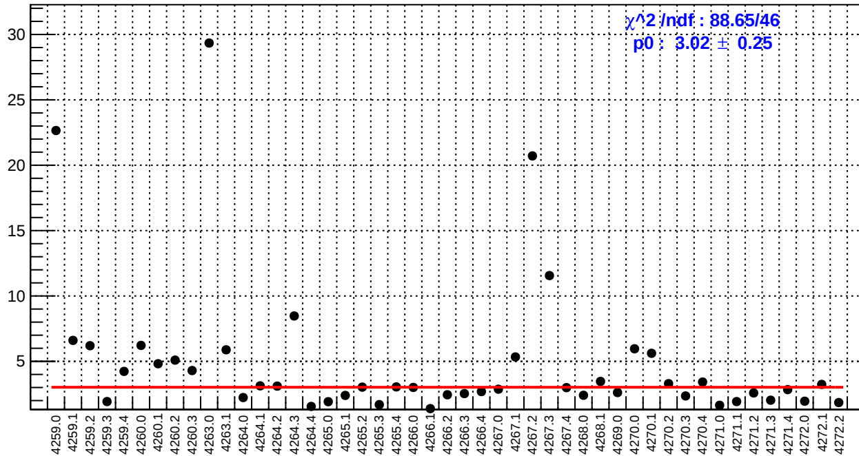
slug51: left_avg_bpm4aY/(ppb/nm)
