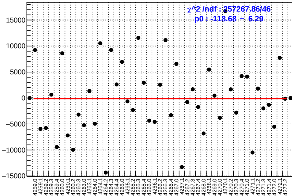
slug51: asym_left_avg.mean/ppb-reg_asym_left_avg.mean/ppb
