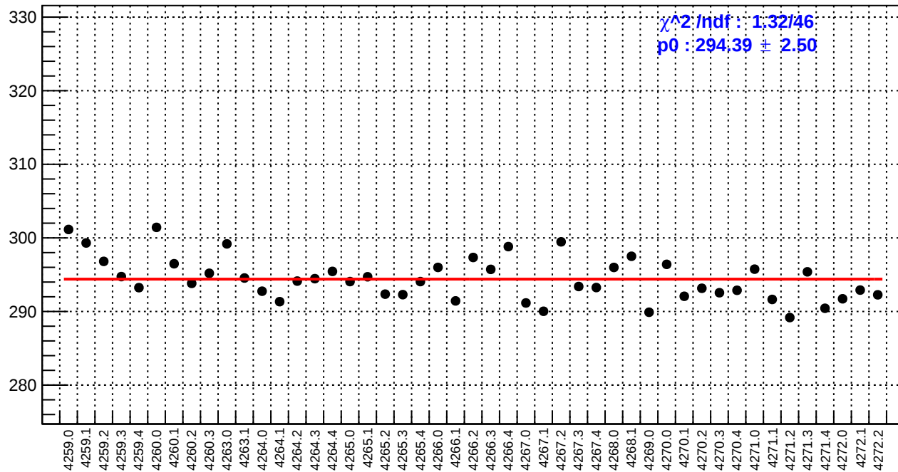
slug51: reg_asym_atl_avg.rms/ppm
