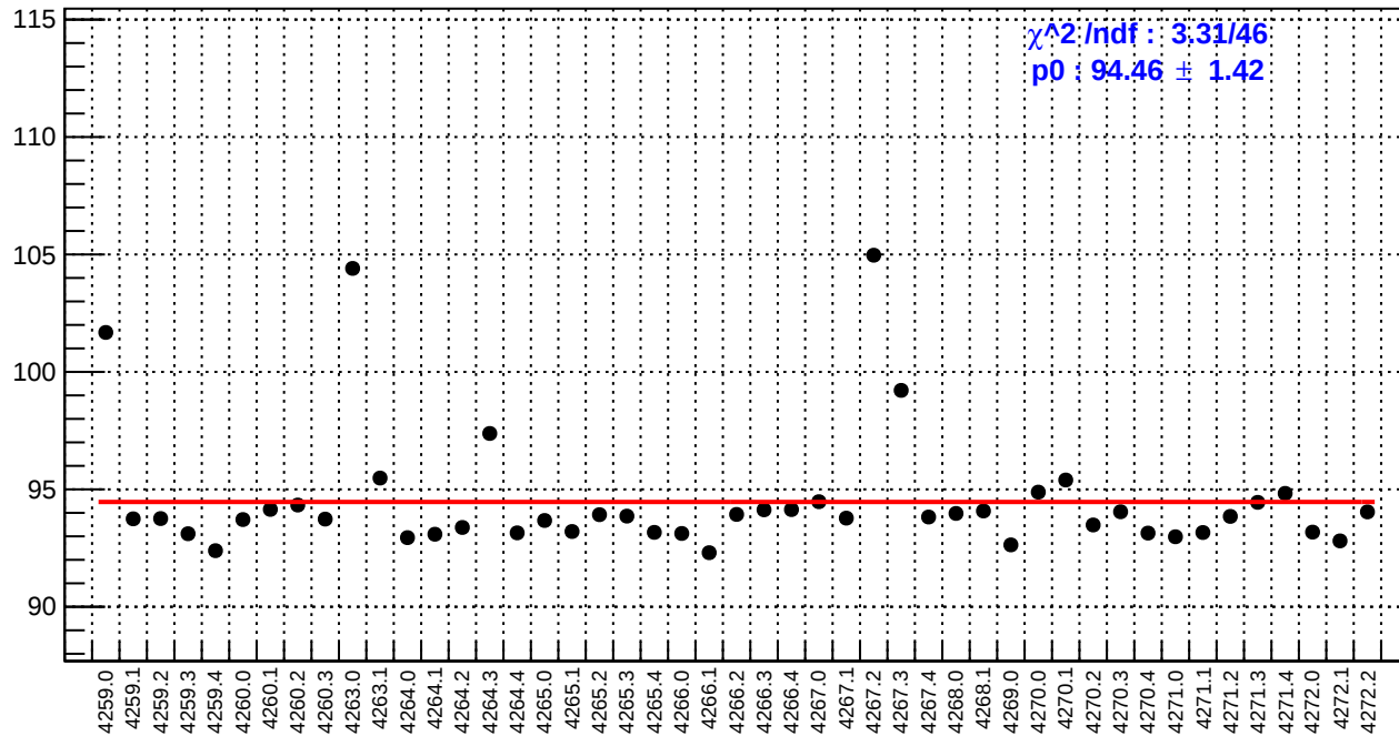
slug51: reg_asym_us_dd.rms/ppm
