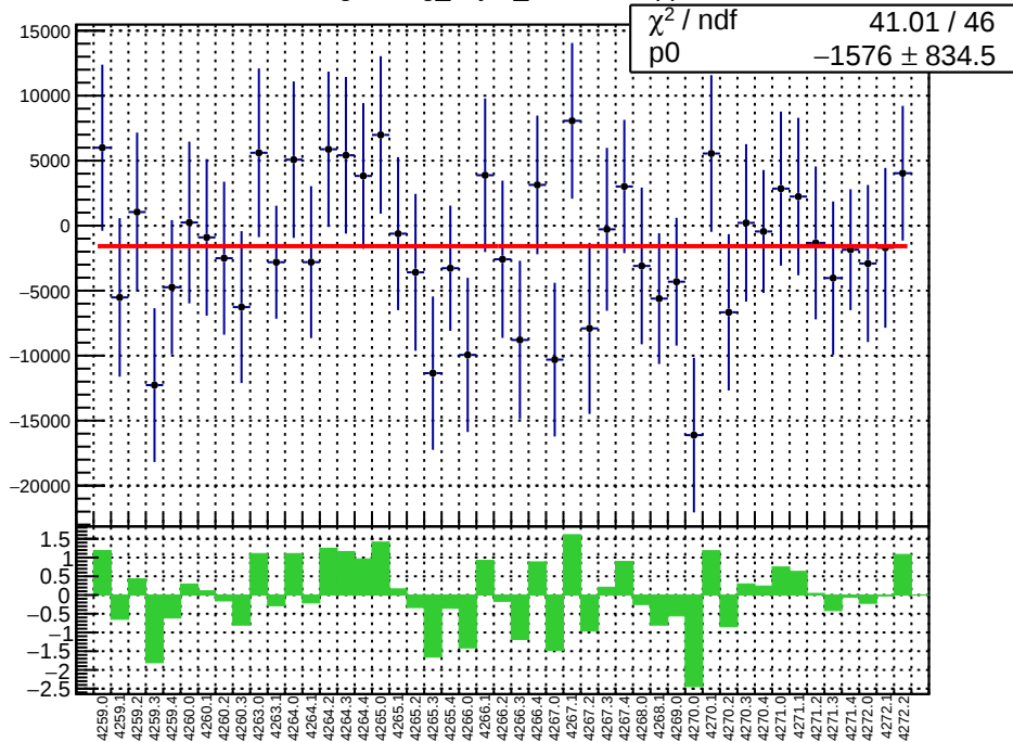
slug51: reg_asym_atr1.mean/ppb
