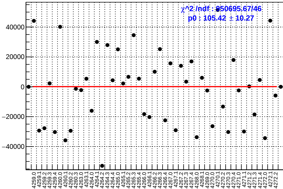
slug51: asym_atl2.mean/ppb-reg_asym_atl2.mean/ppb
