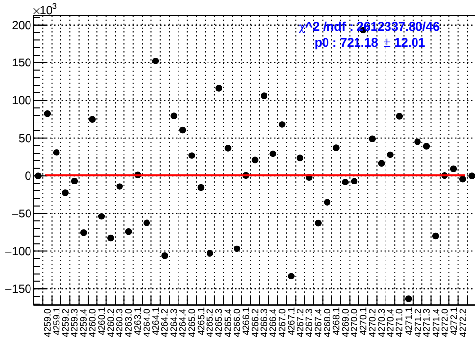
slug51: asym_sam2.mean/ppb-reg_asym_sam2.mean/ppb
