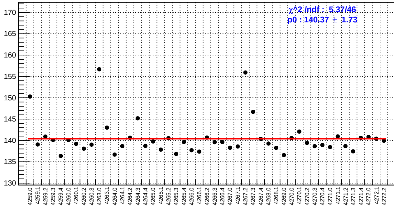
slug51: reg_asym_left_avg.rms/ppm
