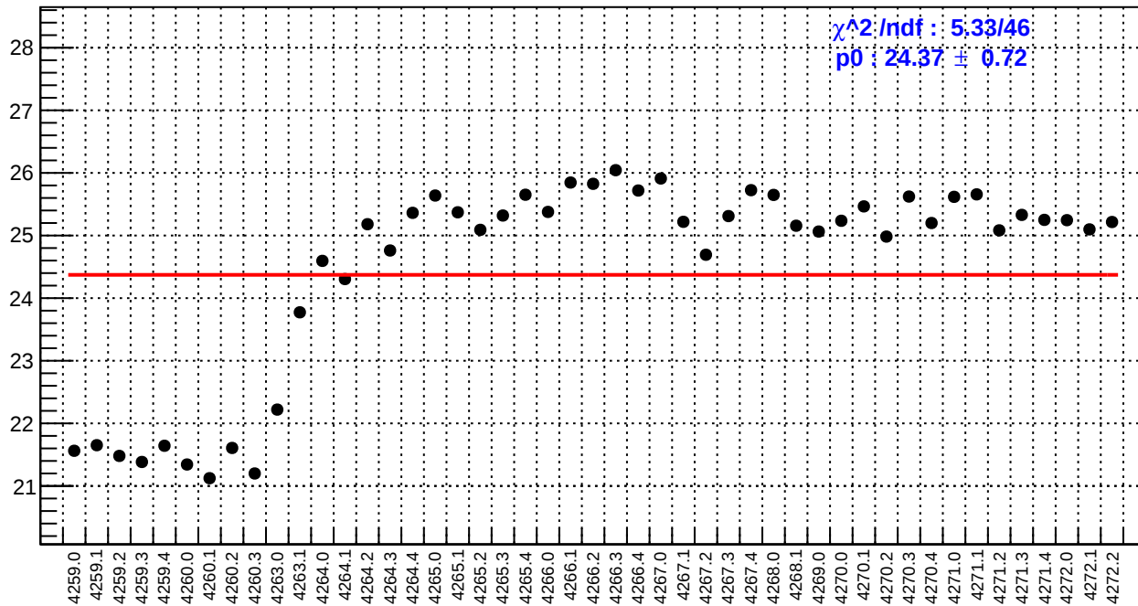
slug51: right_avg_bpm4eX/(ppb/nm)
