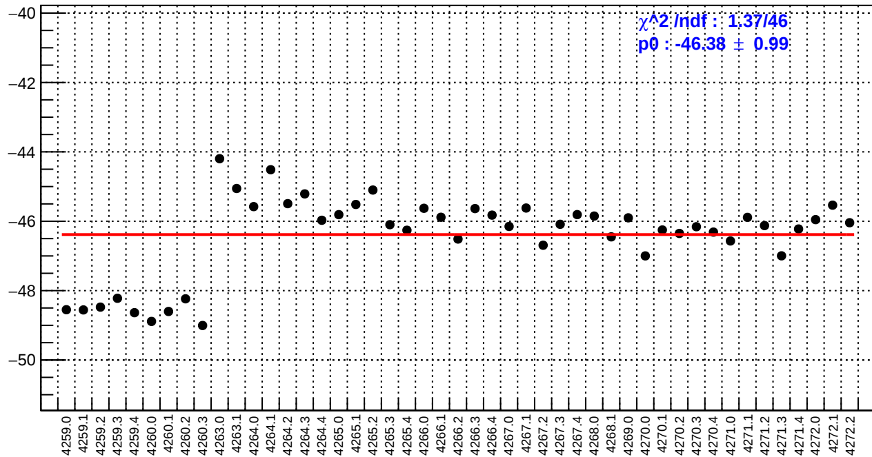
slug51: usl_bpm12X/(ppb/nm)
