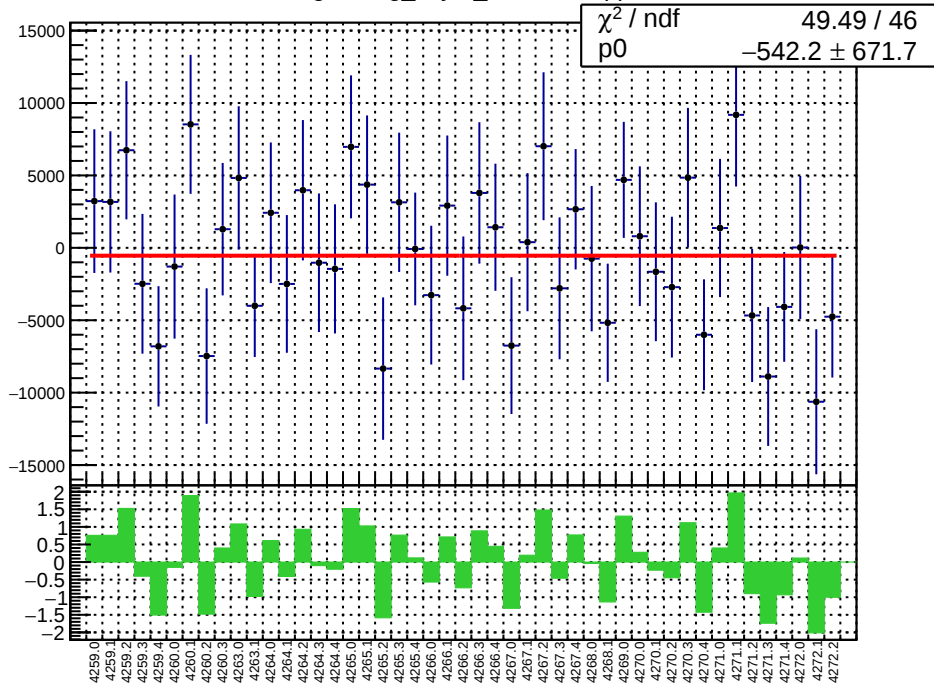
slug51: reg_asym_atr2.mean/ppb
