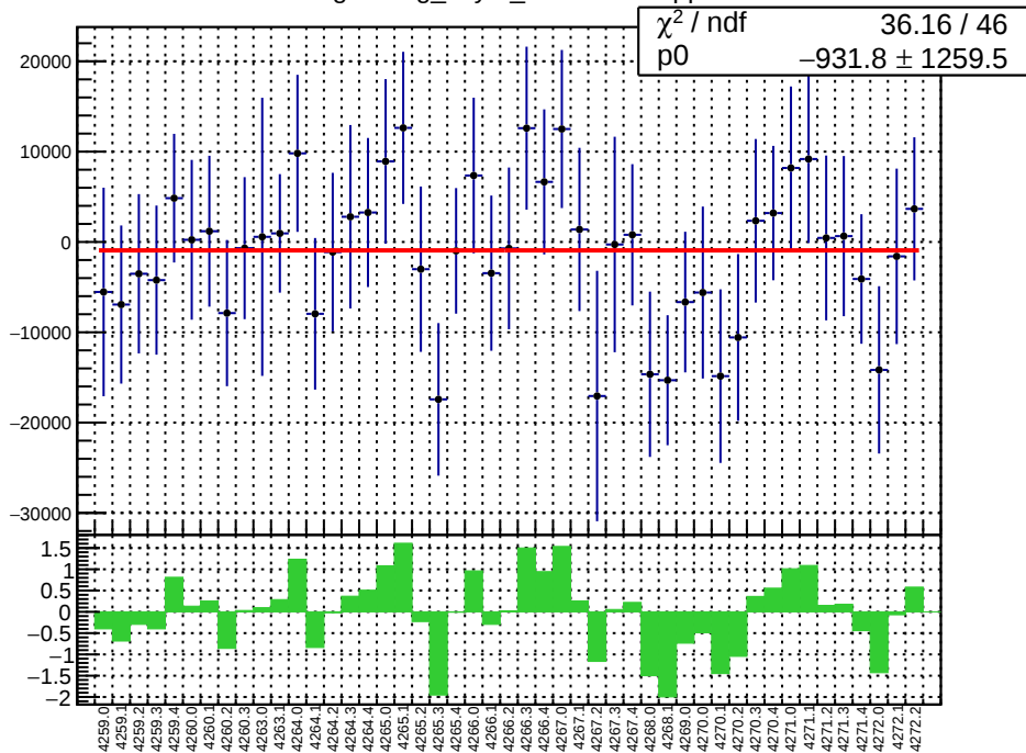
slug51: reg_asym_sam3.mean/ppb
