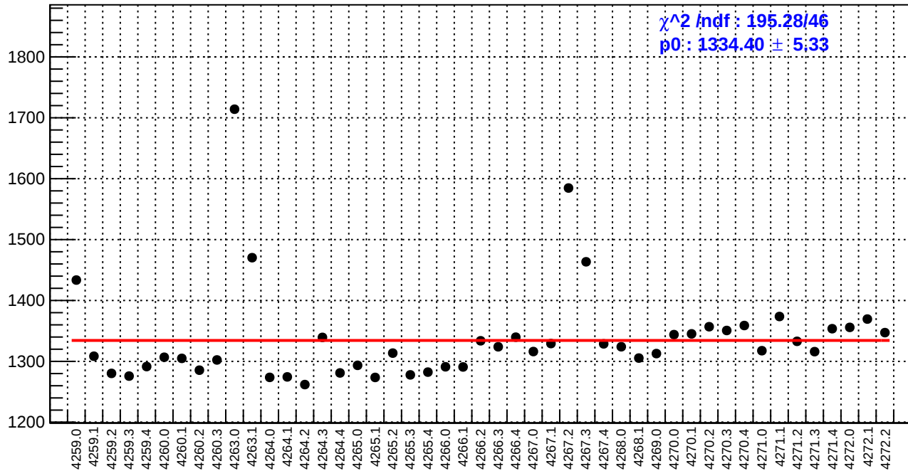
slug51: reg_asym_sam4.rms/ppm
