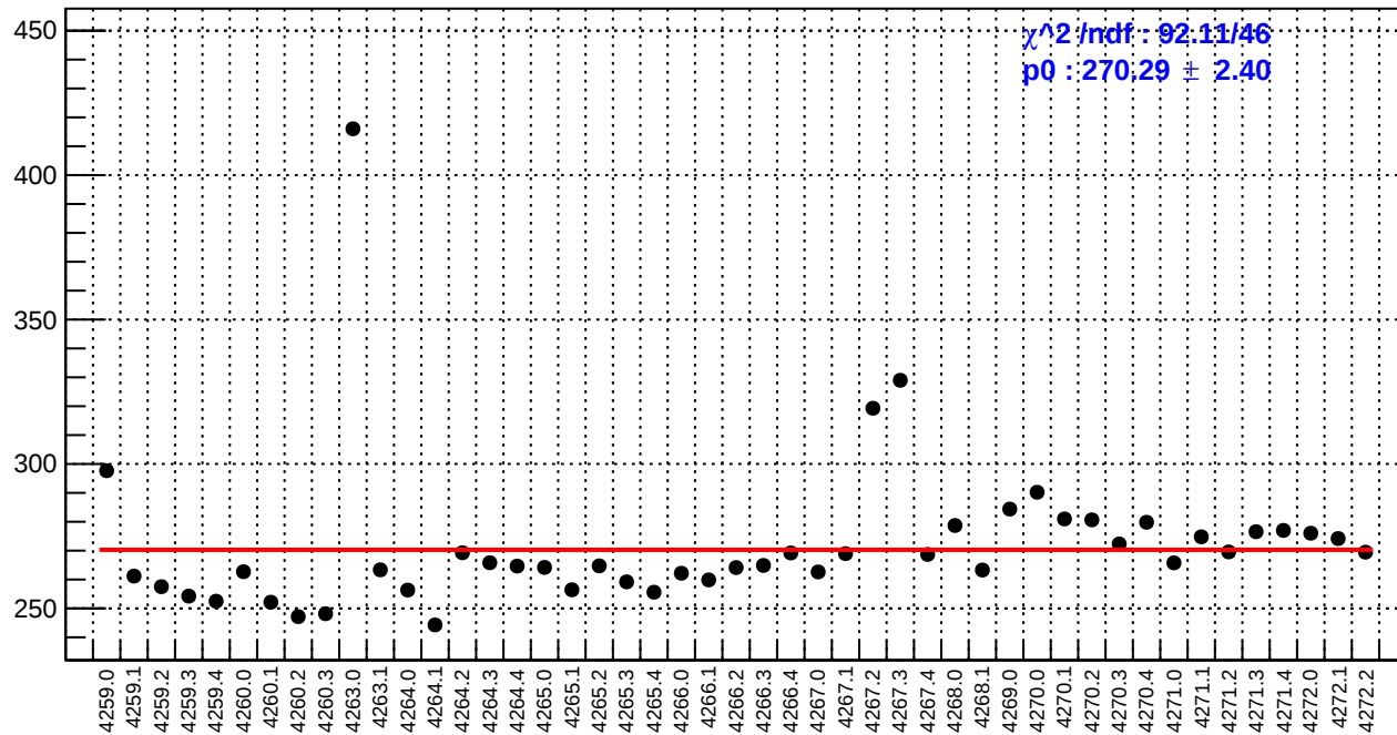
slug51: reg_asym_sam7.rms/ppm
