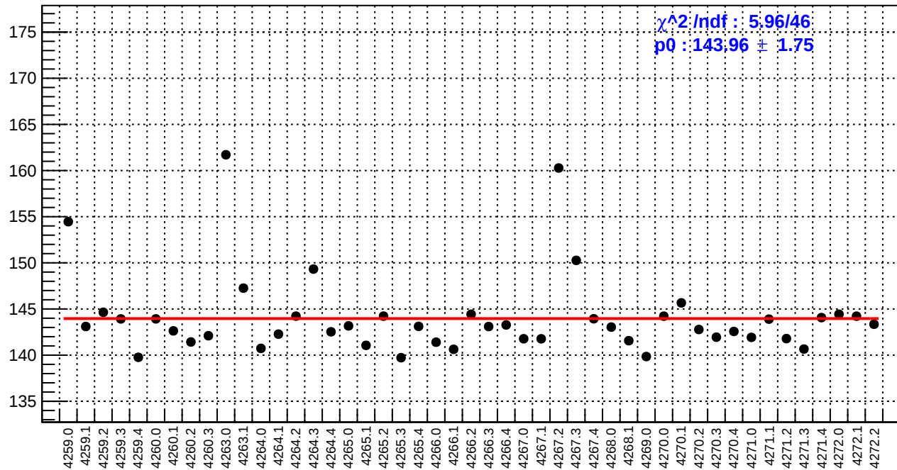
slug51: reg_asym_dsl.rms/ppm
