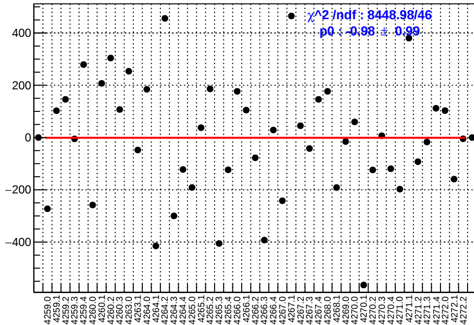
slug51: asym_left_dd.mean/ppb-reg_asym_left_dd.mean/ppb
