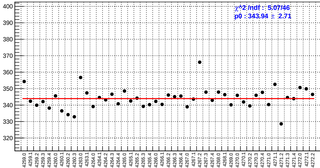
slug51: reg_asym_atl1r2_dd.rms/ppm
