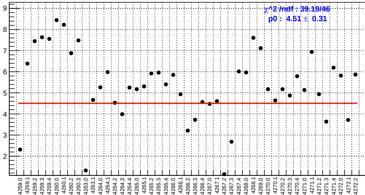
slug51: right_avg_bpm4aY/(ppb/nm)
