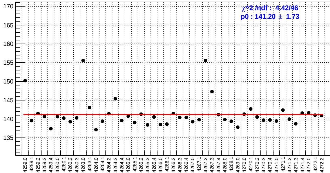
slug51: reg_asym_usl.rms/ppm
