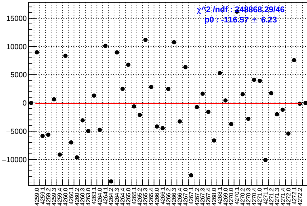
slug51: asym_usl.mean/ppb-reg_asym_usl.mean/ppb
