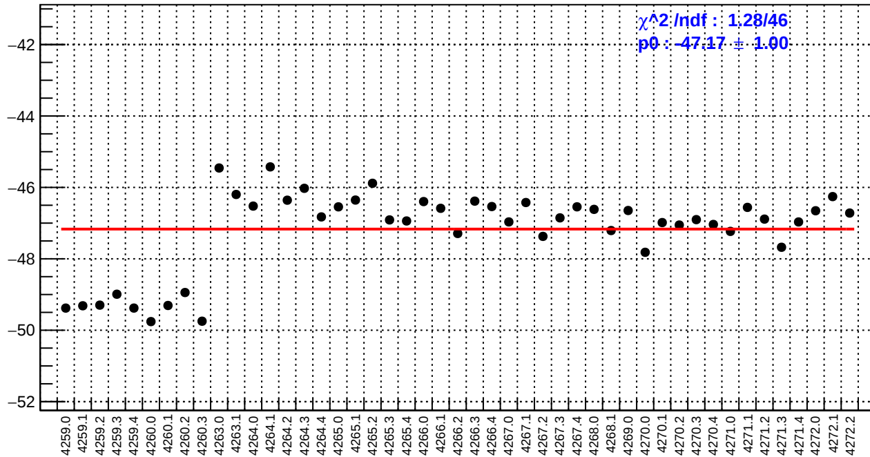
slug51: left_avg_bpm12X/(ppb/nm)
