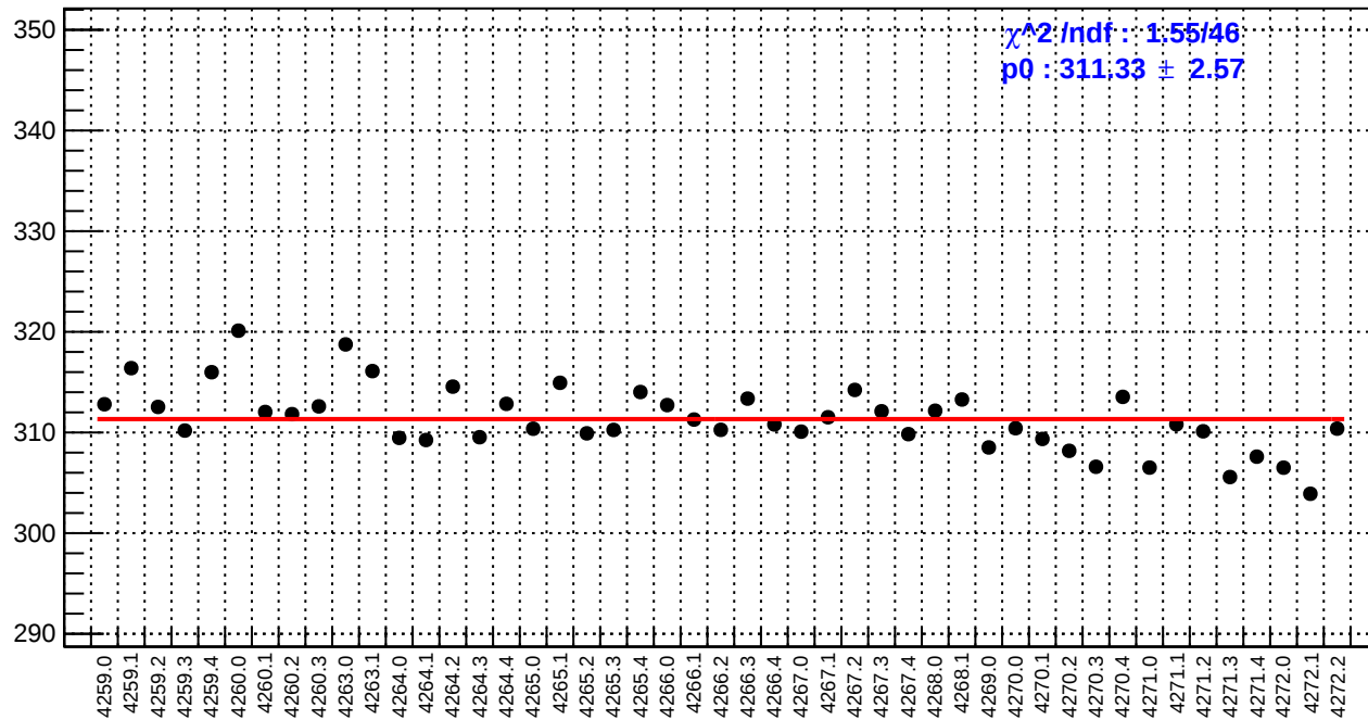
slug51: reg_asym_atr_dd.rms/ppm
