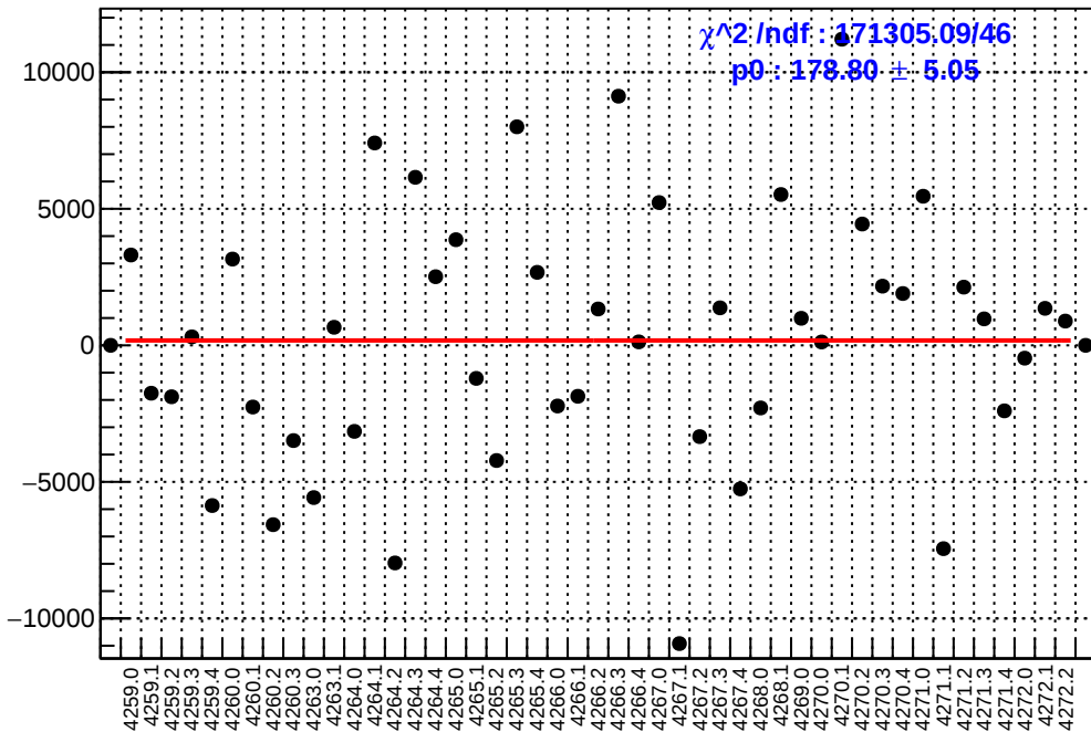
slug51: asym_us_dd.mean/ppb-reg_asym_us_dd.mean/ppb
