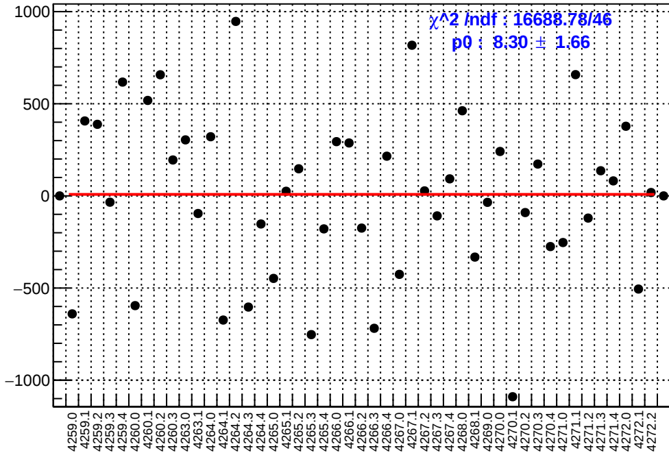
slug51: asym_right_dd.mean/ppb-reg_asym_right_dd.mean/ppb
