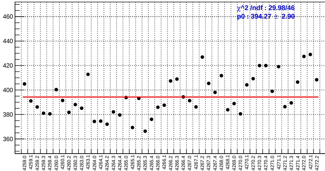
slug51: reg_asym_sam5.rms/ppm
