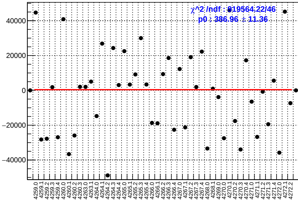
slug51: asym_atr_avg.mean/ppb-reg_asym_atr_avg.mean/ppb
