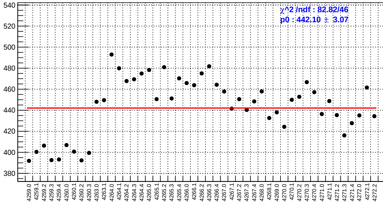
slug51: reg_asym_sam1.rms/ppm
