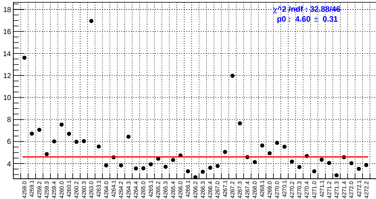
slug51: ds_avg_bpm4aY/(ppb/nm)
