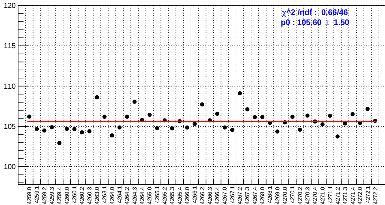
slug51: reg_asym_ds_avg.rms/ppm
