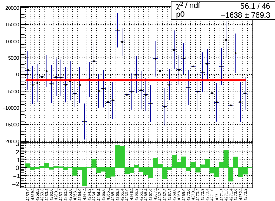
slug51: reg_asym_sam6.mean/ppb
