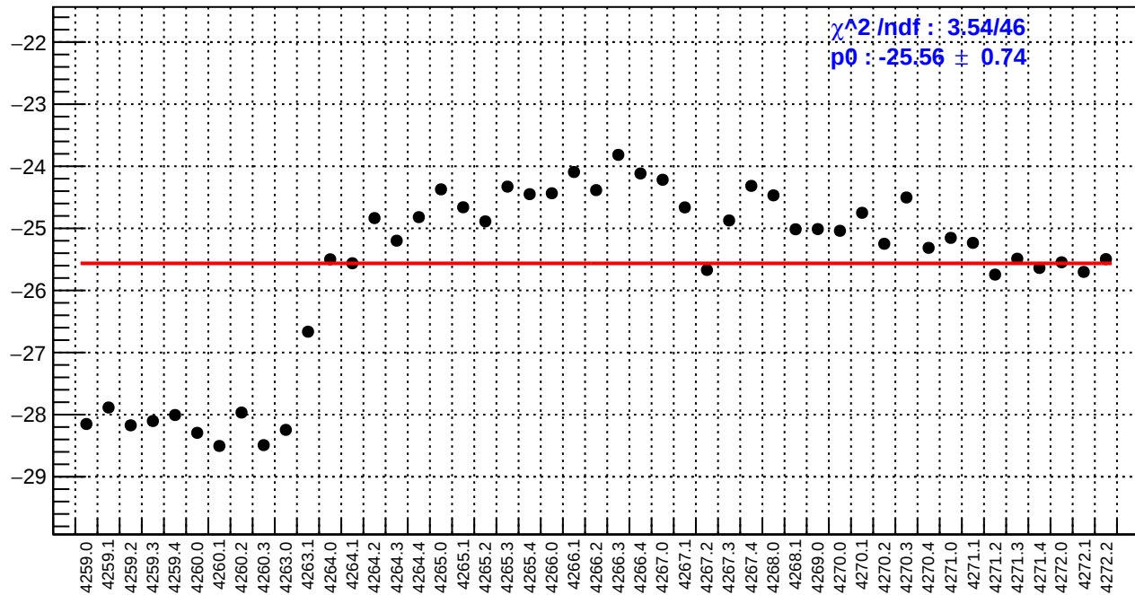
slug51: ds_avg_bpm4eX/(ppb/nm)
