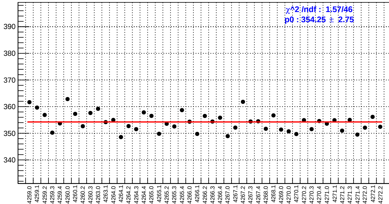
slug51: reg_asym_at1_avg.rms/ppm
