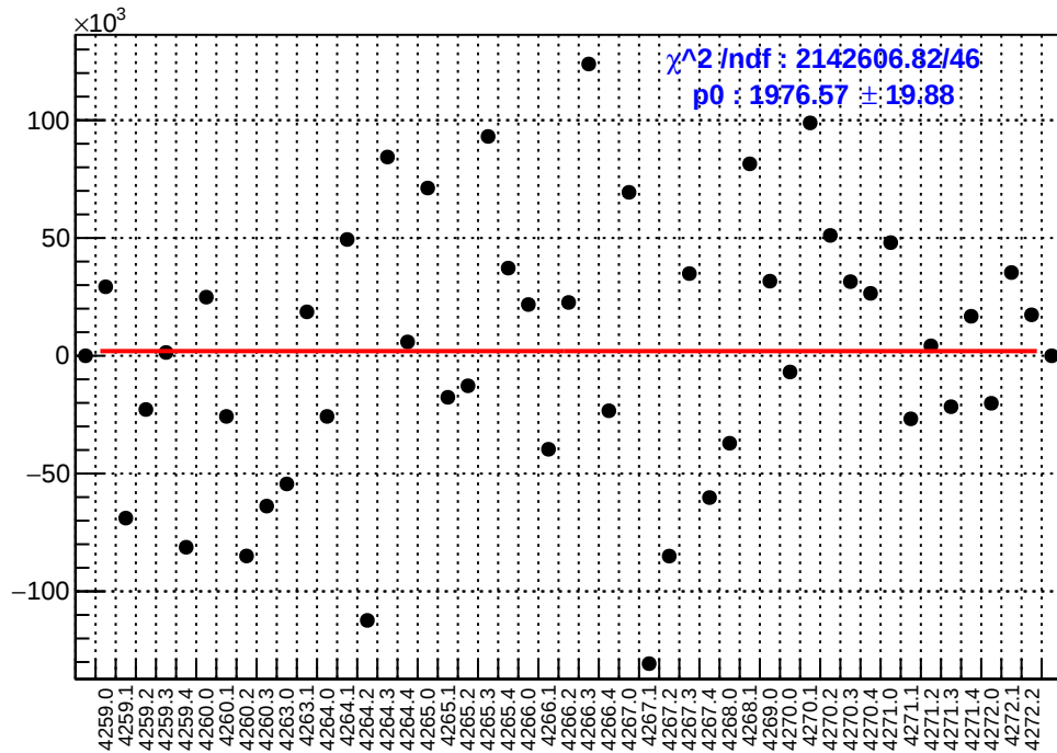
slug51: asym_sam4.mean/ppb-reg_asym_sam4.mean/ppb
