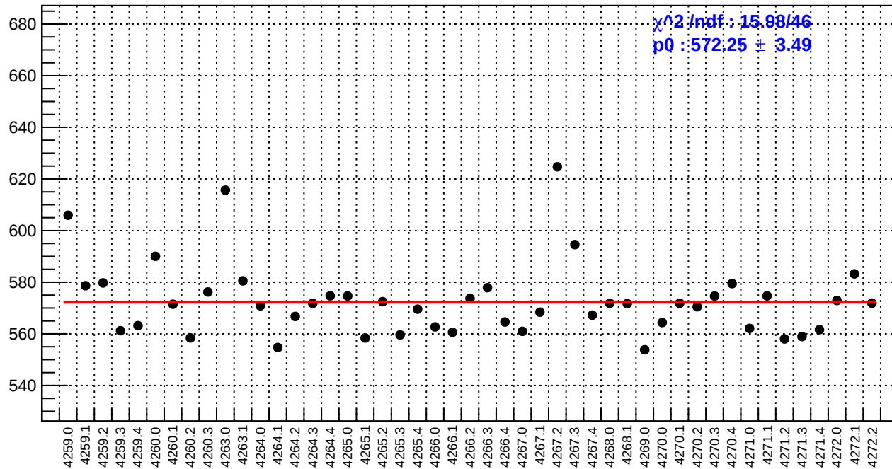
slug51: reg_asym_atr1.rms/ppm
