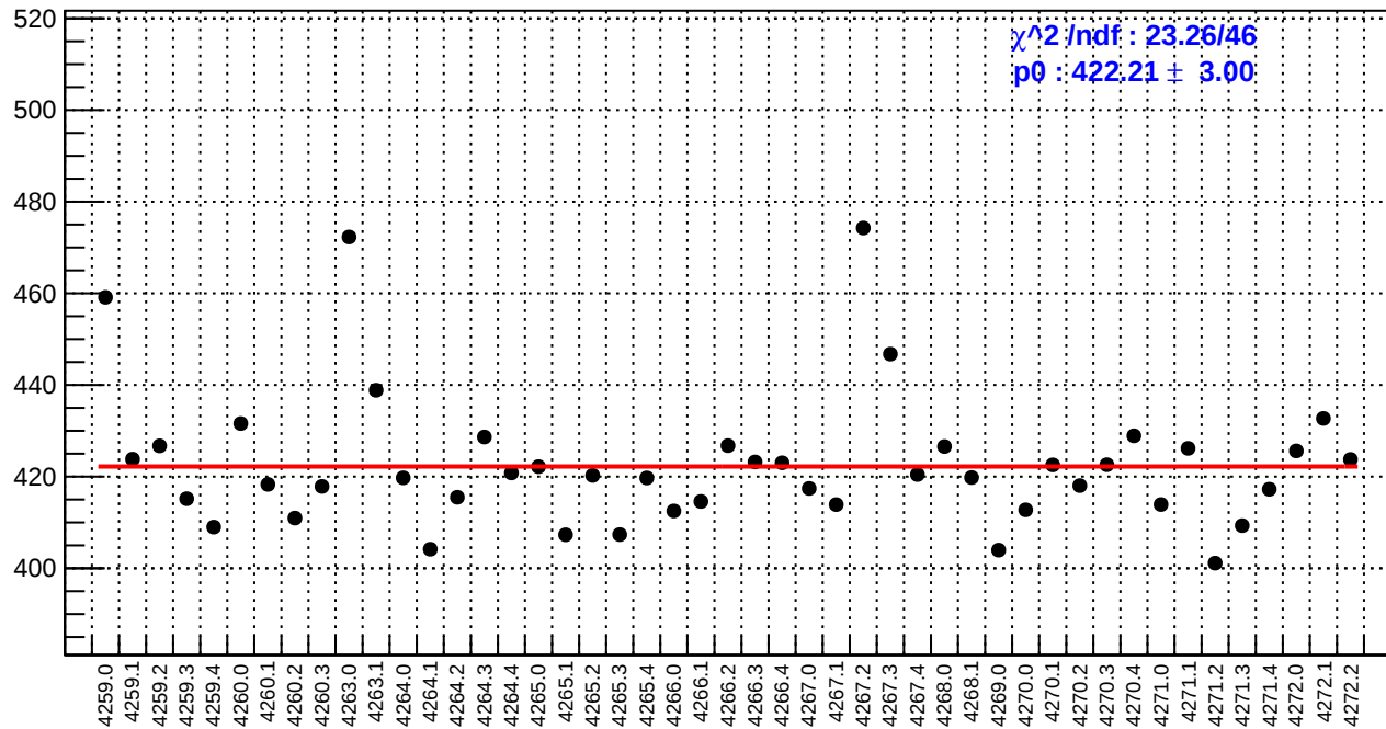
slug51: reg_asym_atl2.rms/ppm
