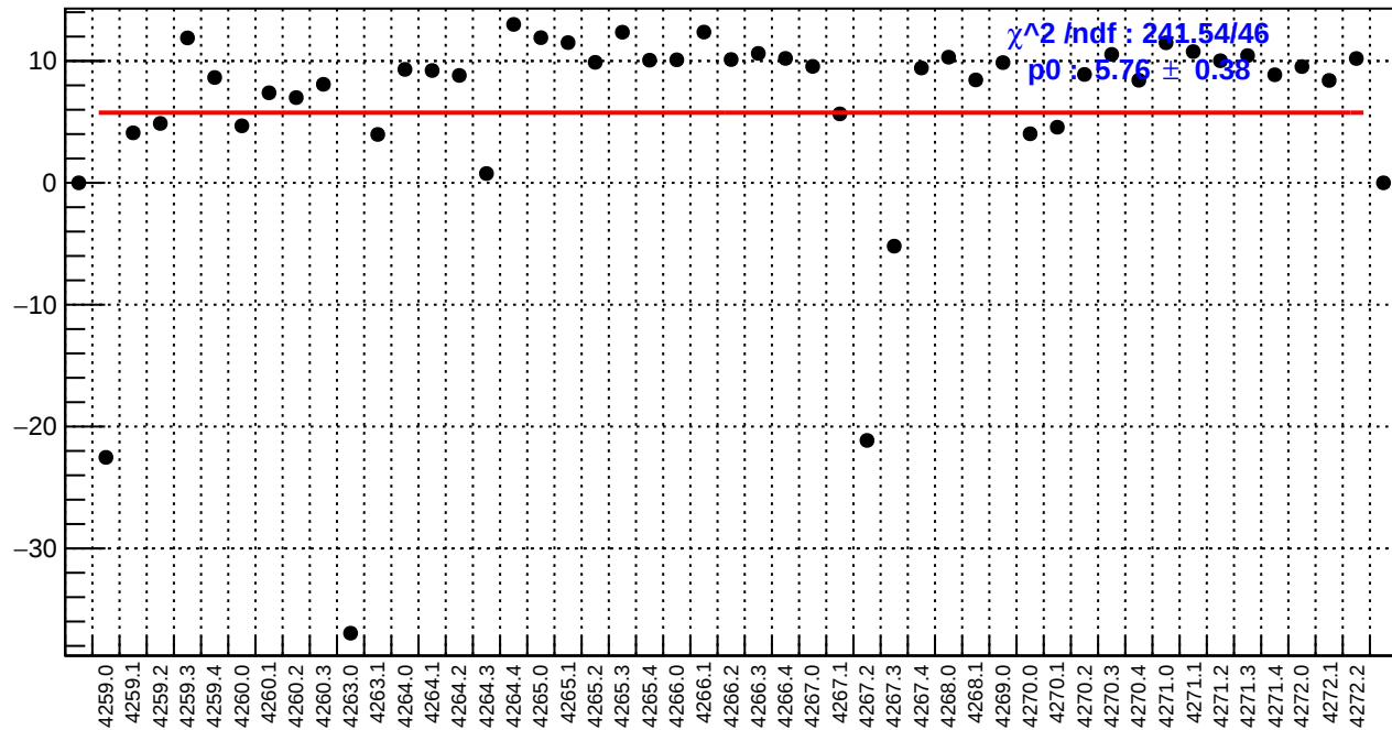
slug51: left_avg_bpm4eY/(ppb/nm)
