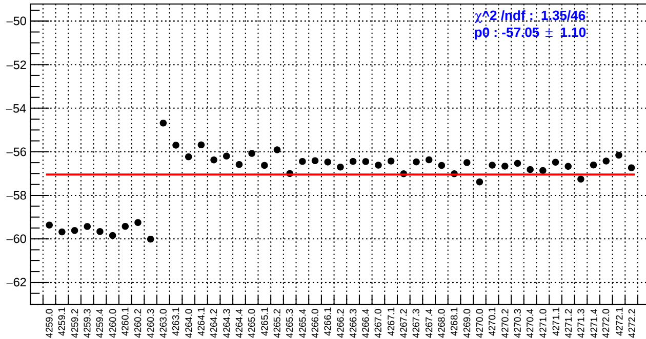
slug51: ds_avg_bpm12X/(ppb/nm)
