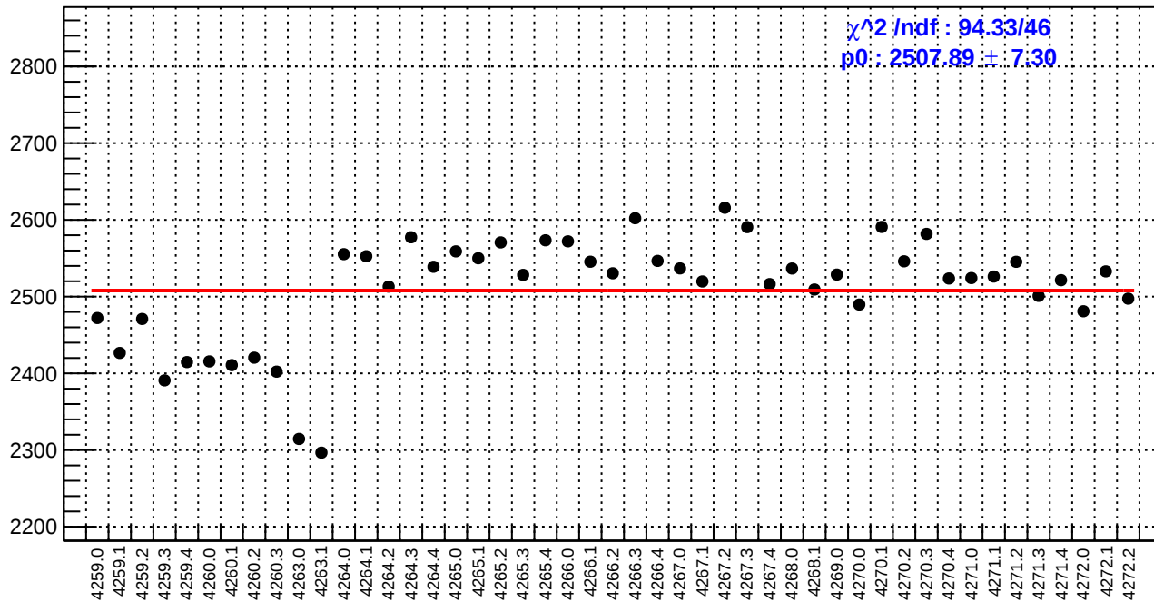
slug51: reg_asym_sam2.rms/ppm
