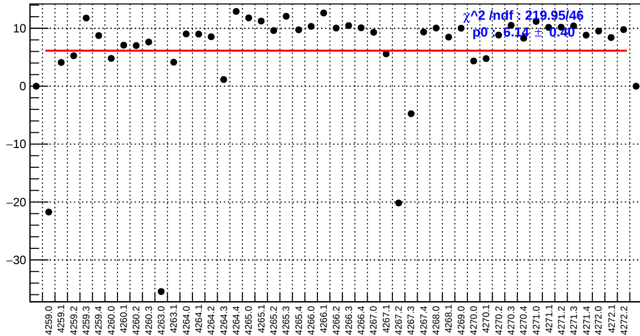
slug51: usl_bpm4eY/(ppb/nm)
