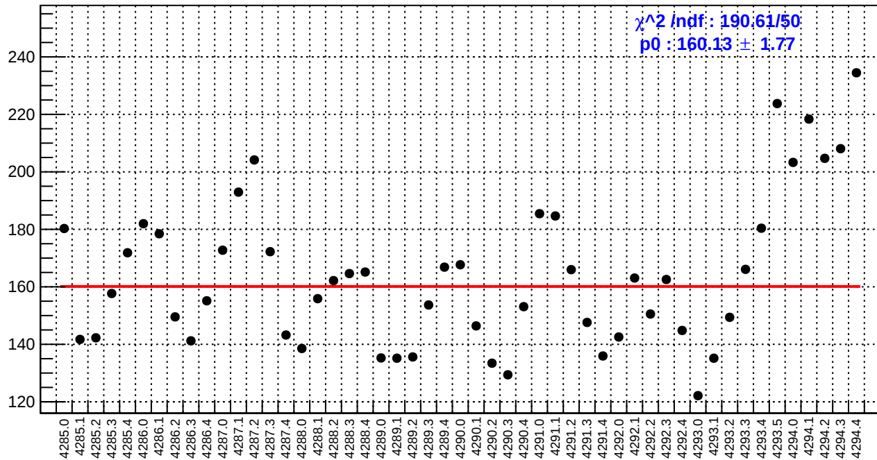
slug53: asym_bcm_an_ds.rms/ppm
