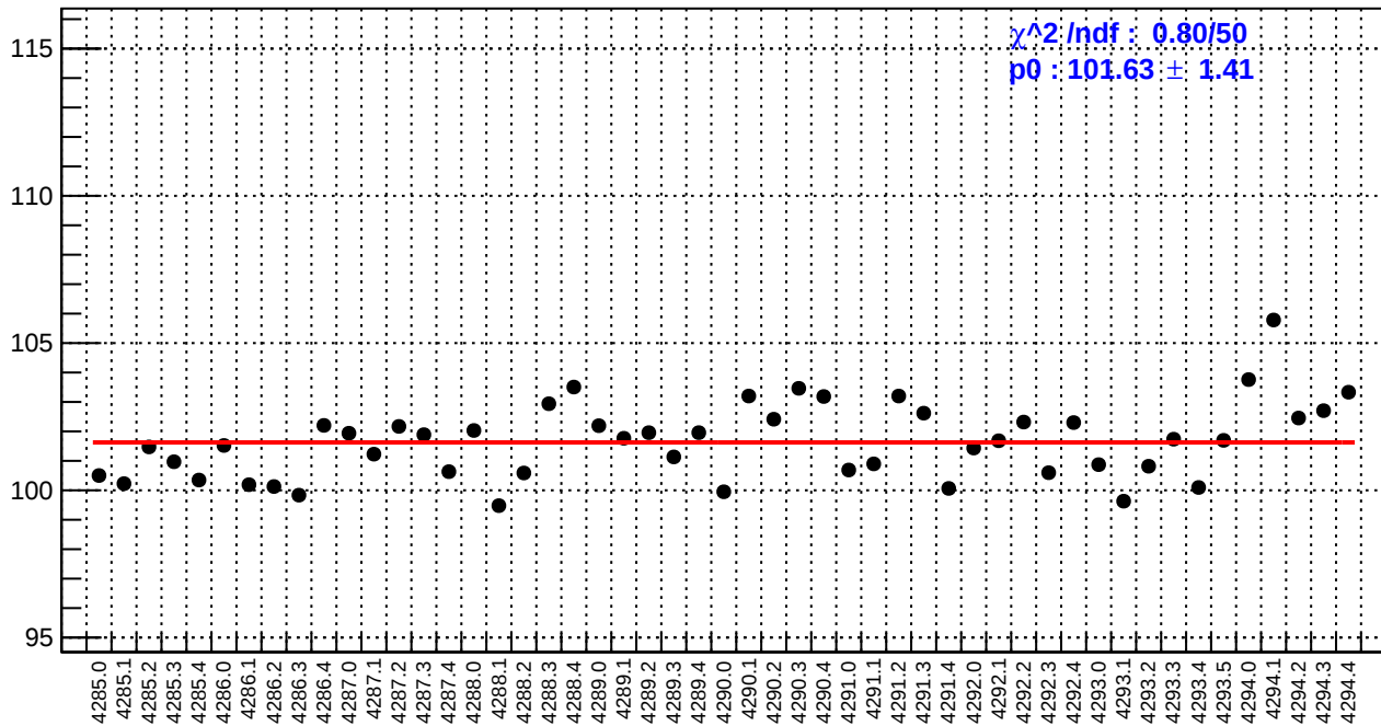
slug53: reg_asym_us_avg.rms/ppm
