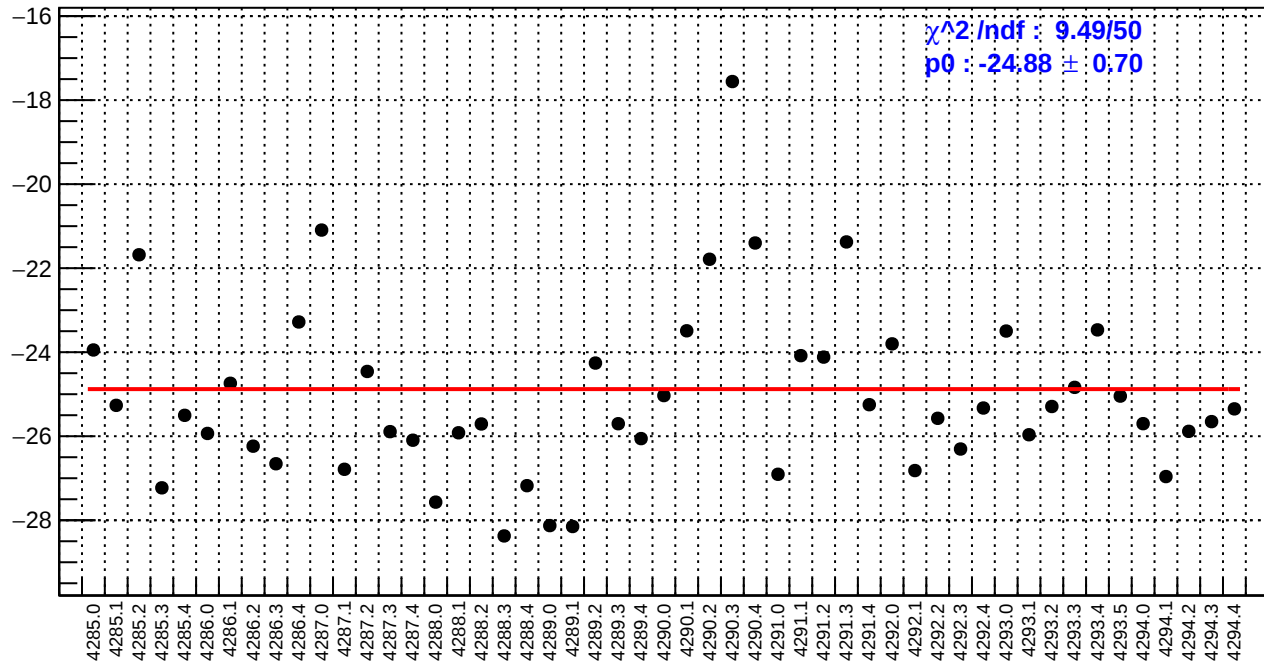
slug53: ds_avg_bpm4aX/(ppb/nm)
