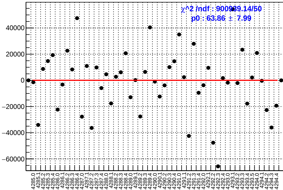
slug53: asym_sam6.mean/ppb-reg_asym_sam6.mean/ppb
