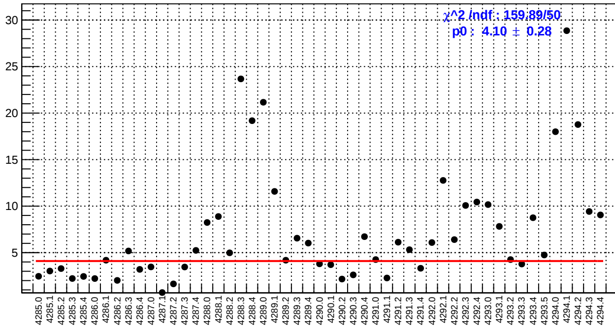
slug53: usl_bpm4aY/(ppb/nm)
