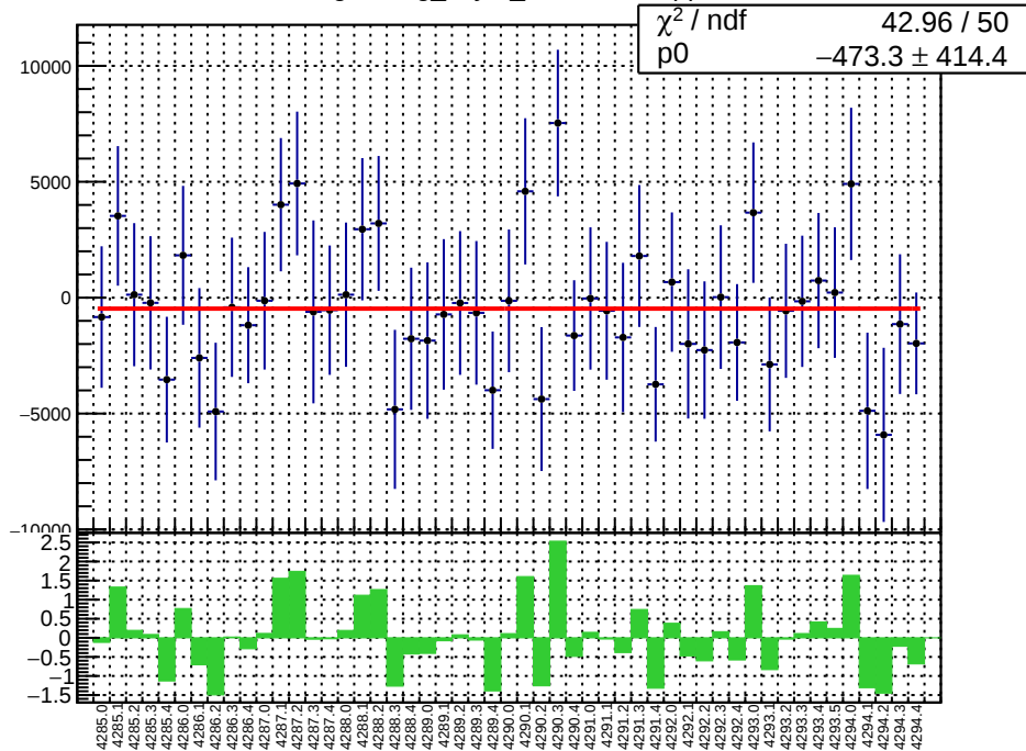
slug53: reg_asym_sam7.mean/ppb
