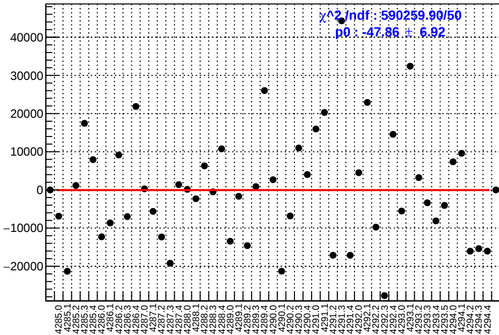
slug53: asym_sam7.mean/ppb-reg_asym_sam7.mean/ppb
