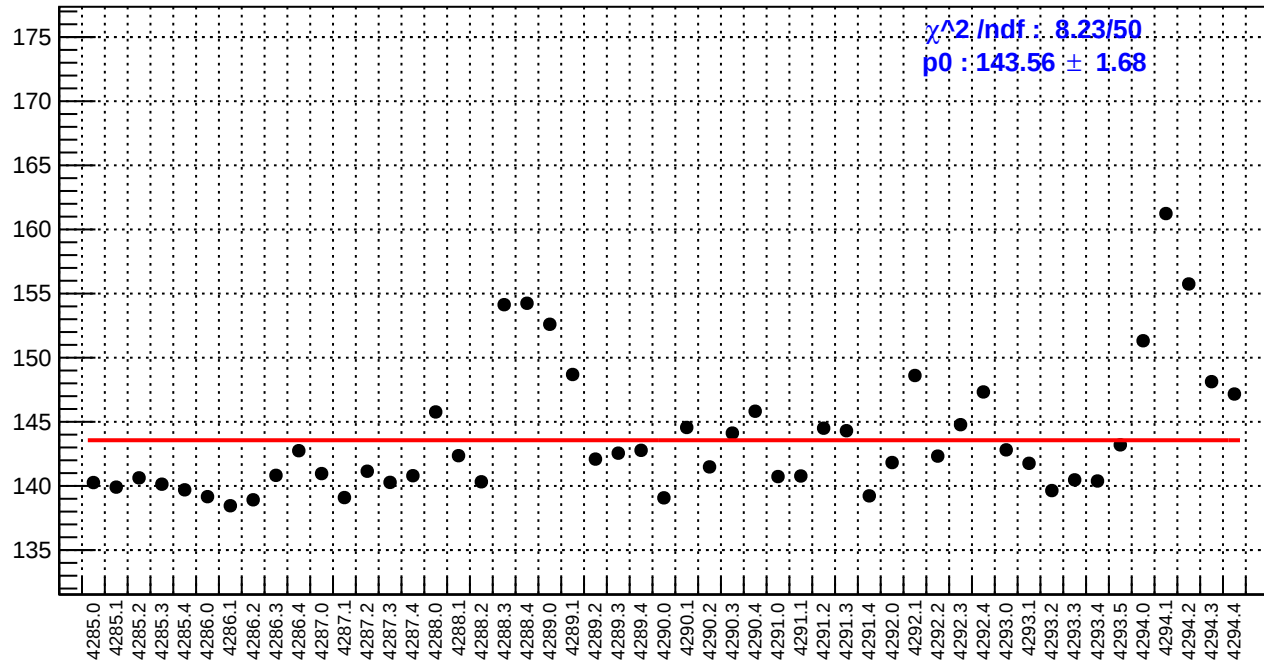
slug53: reg_asym_usl.rms/ppm
