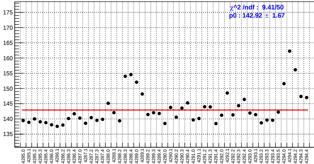
slug53: reg_asym_left_avg.rms/ppm
