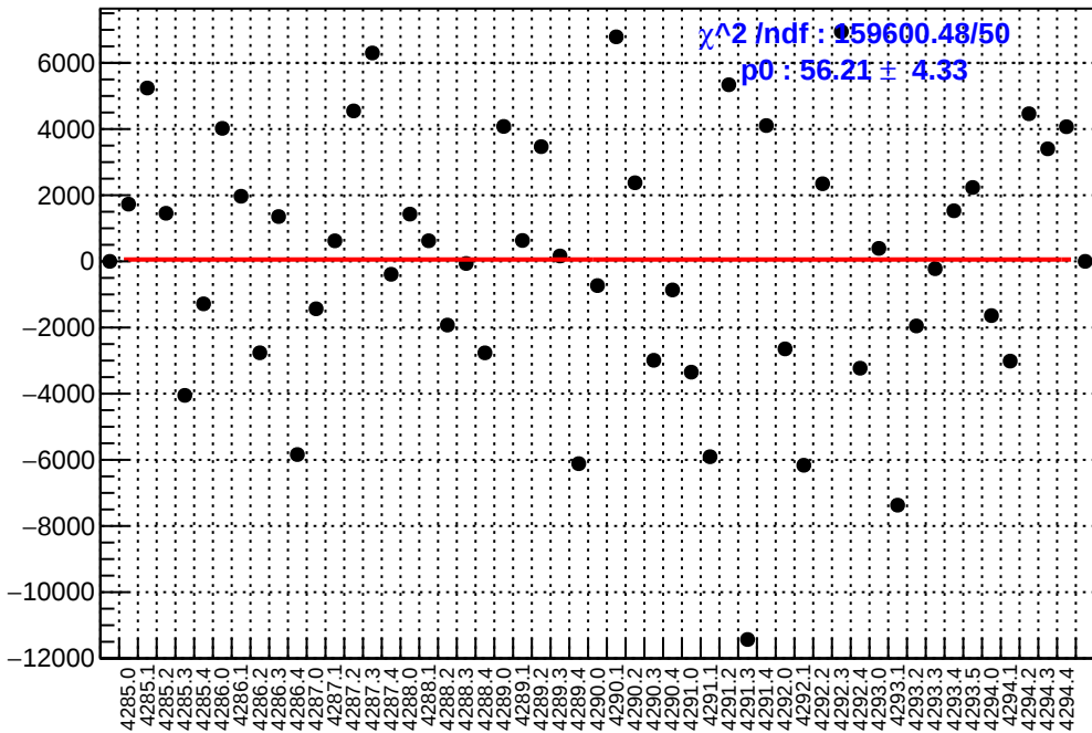
slug53: asym_ds_dd.mean/ppb-reg_asym_ds_dd.mean/ppb
