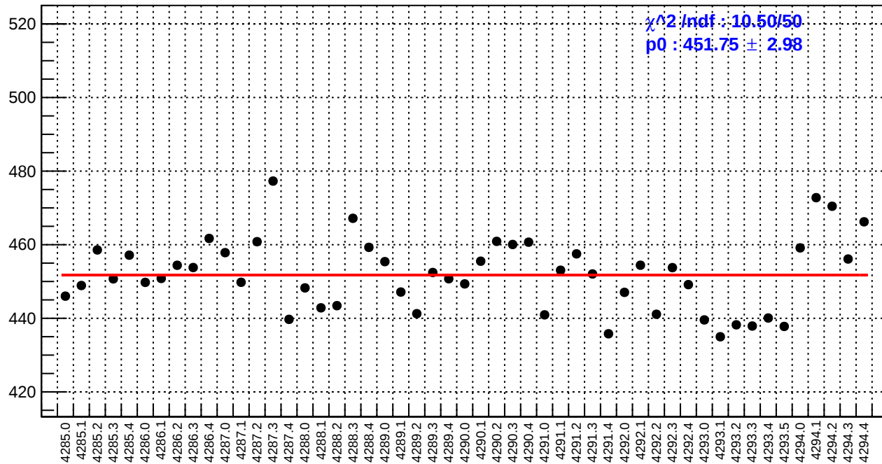
slug53: reg_asym_sam8.rms/ppm
