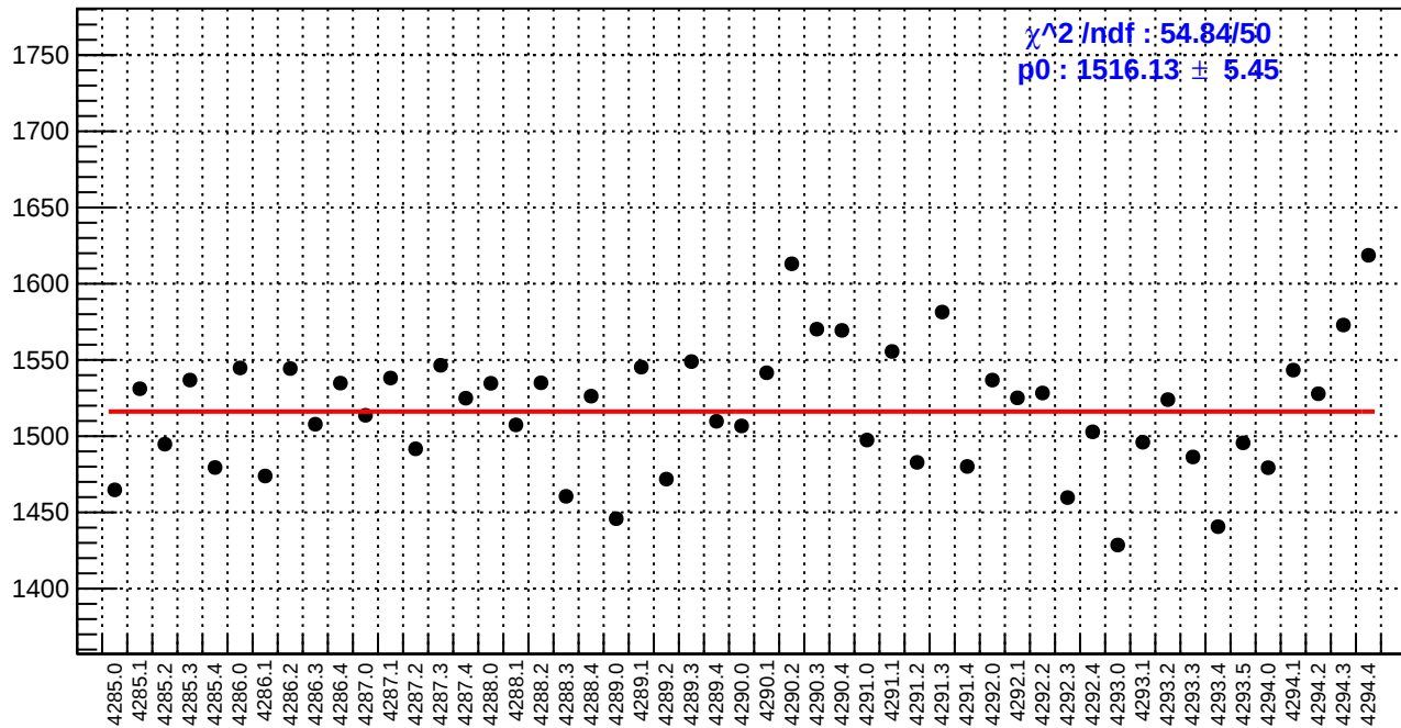
slug53: diff_bpm4aX.rms/nm
