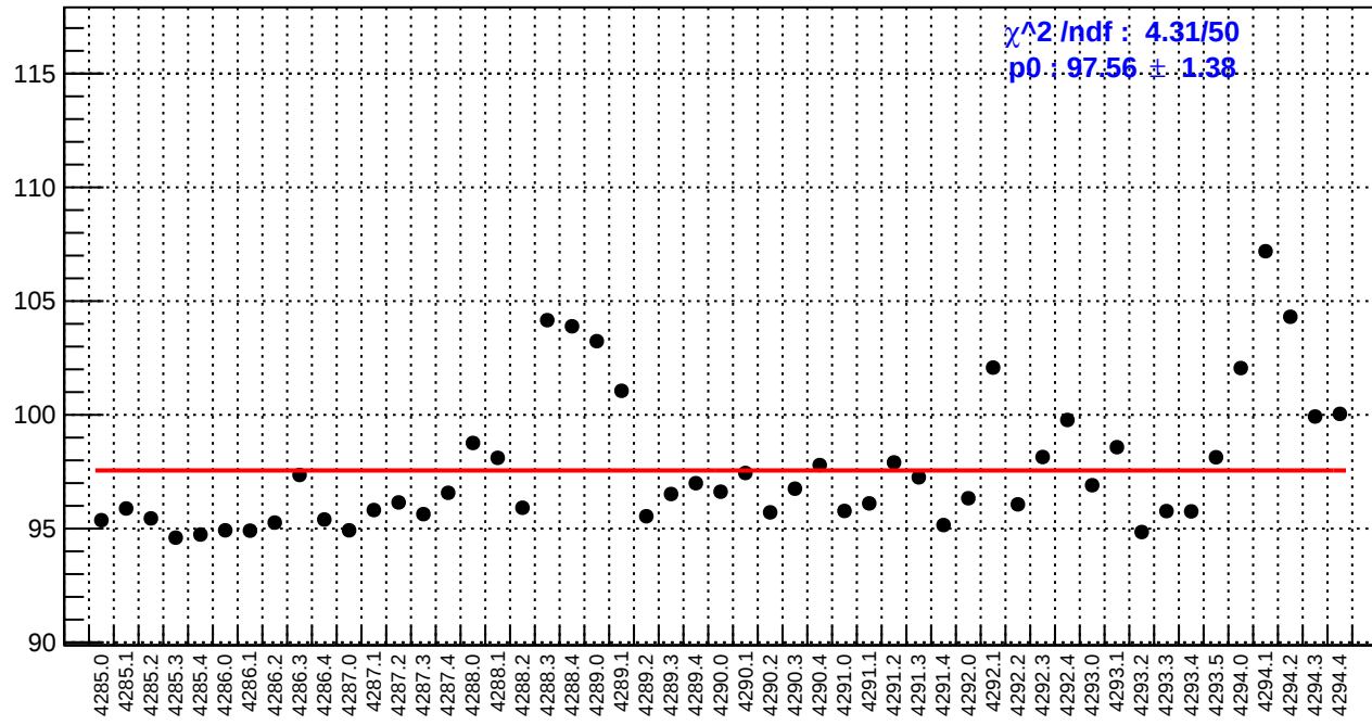
slug53: reg_asym_ds_dd.rms/ppm
