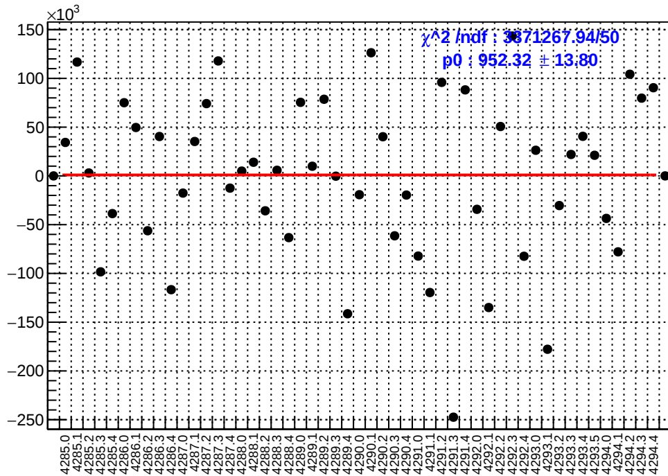
slug53: asym_sam3.mean/ppb-reg_asym_sam3.mean/ppb
