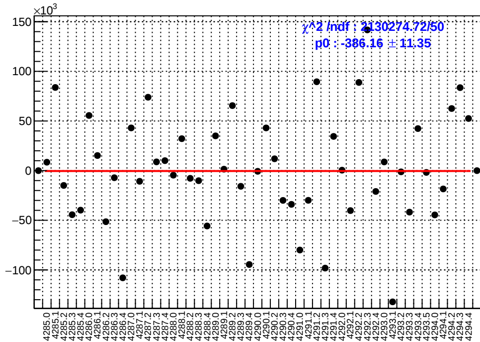
slug53: asym_sam2.mean/ppb-reg_asym_sam2.mean/ppb
