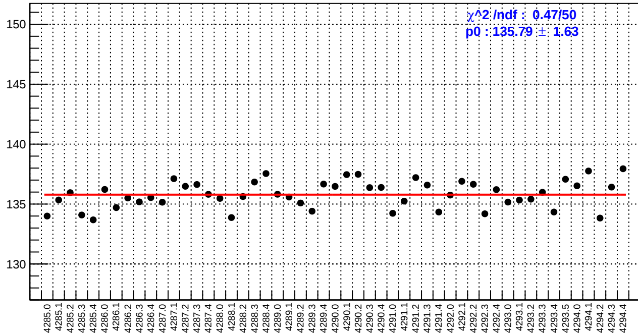
slug53: reg_asym_right_avg.rms/ppm
