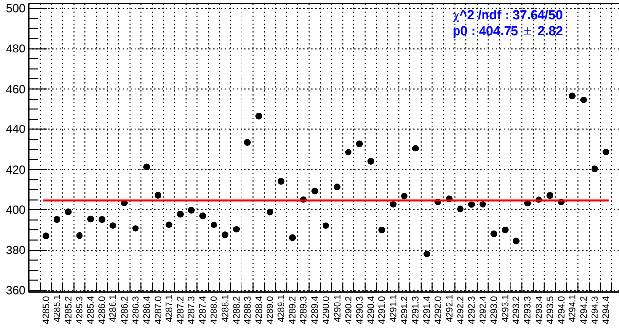
slug53: reg_asym_sam5.rms/ppm
