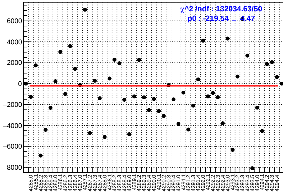
slug53: asym_us_avg.mean/ppb-reg_asym_us_avg.mean/ppb
