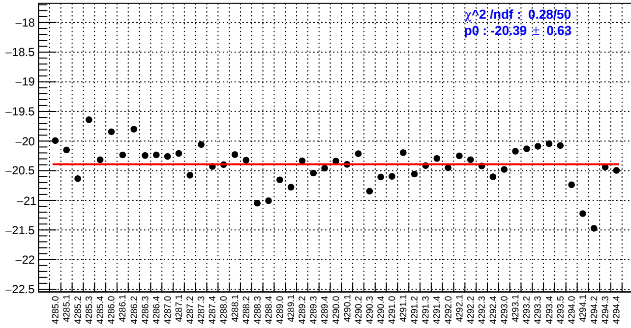
slug53: us_avg_bpm4eX/(ppb/nm)
