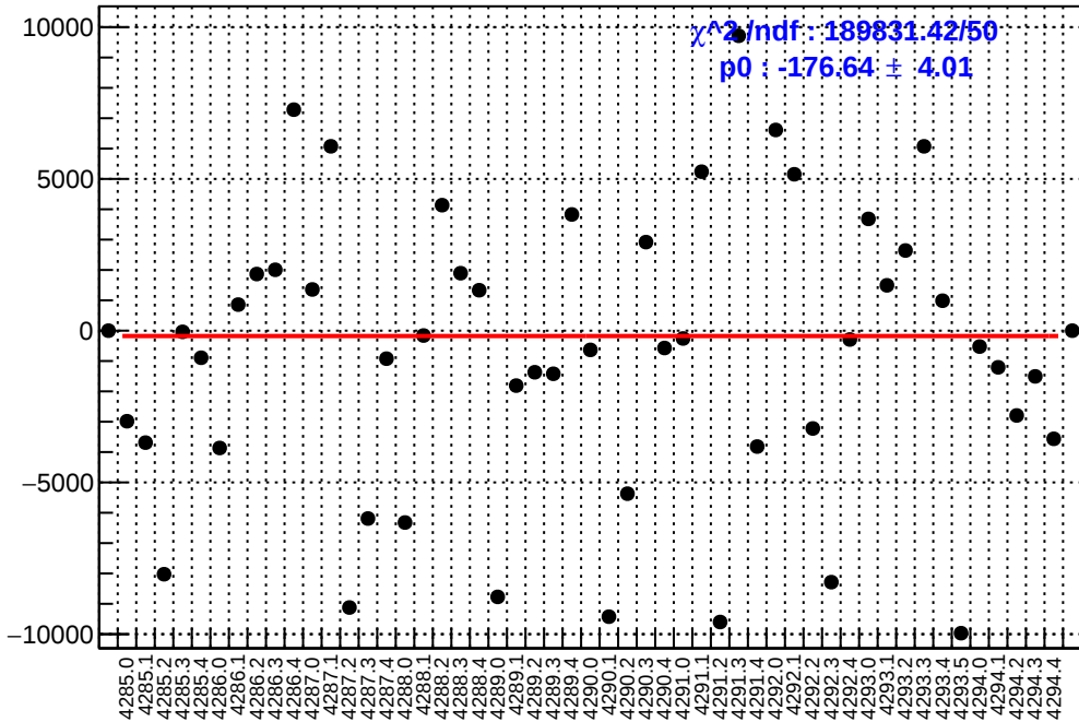
slug53: asym_usr.mean/ppb-reg_asym_usr.mean/ppb
