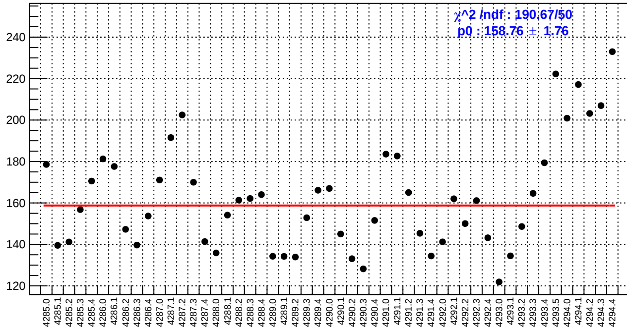
slug53: asym_bcm_an_us.rms/ppm
