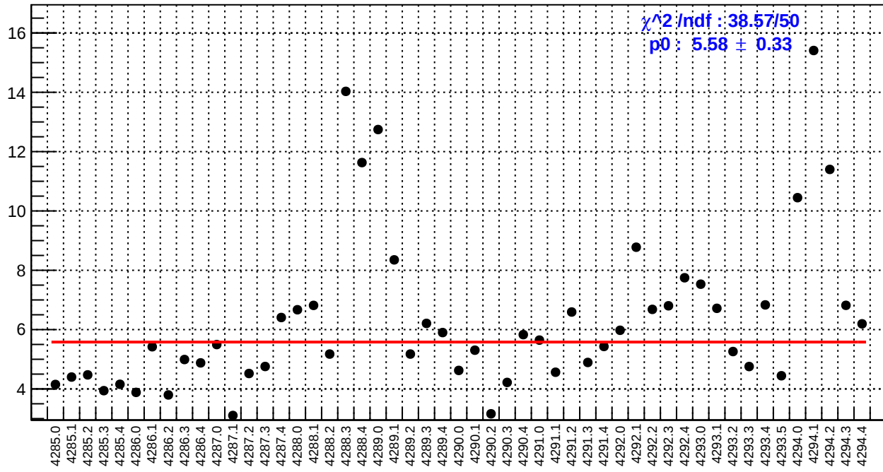
slug53: ds_avg_bpm4aY/(ppb/nm)
