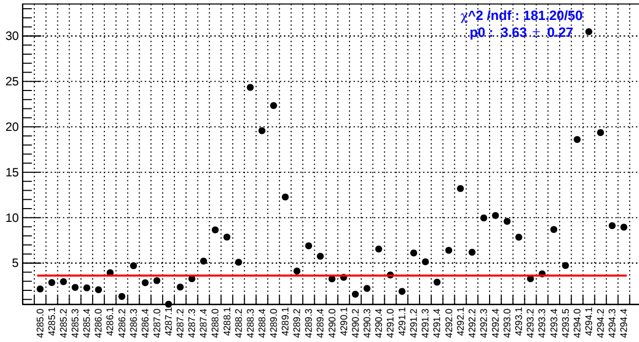
slug53: dsl_bpm4aY/(ppb/nm)
