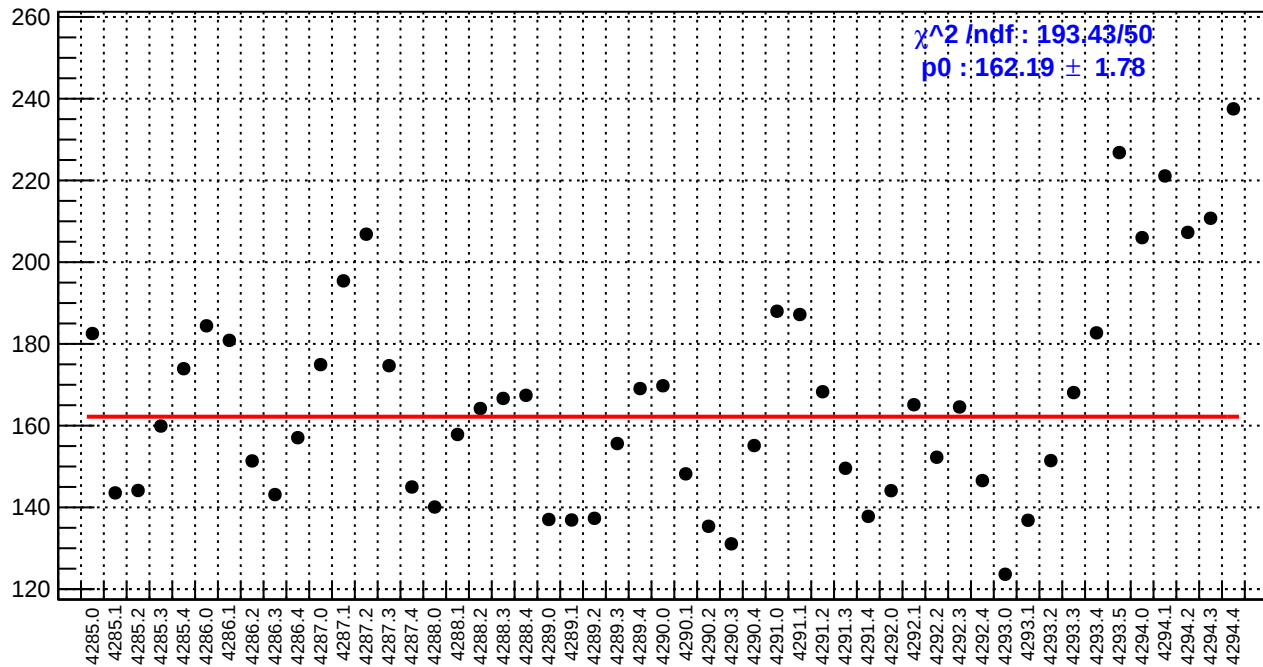
slug53: asym_bcm_an_ds3.rms/ppm
