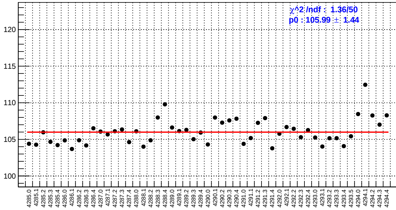
slug53: reg_asym_ds_avg.rms/ppm
