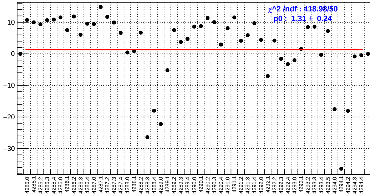
slug53: left_avg_bpm4eY/(ppb/nm)
