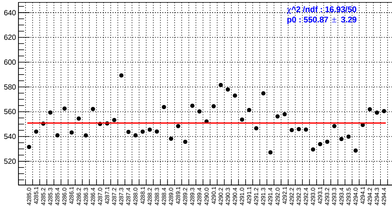
slug53: reg_asym_sam6.rms/ppm
