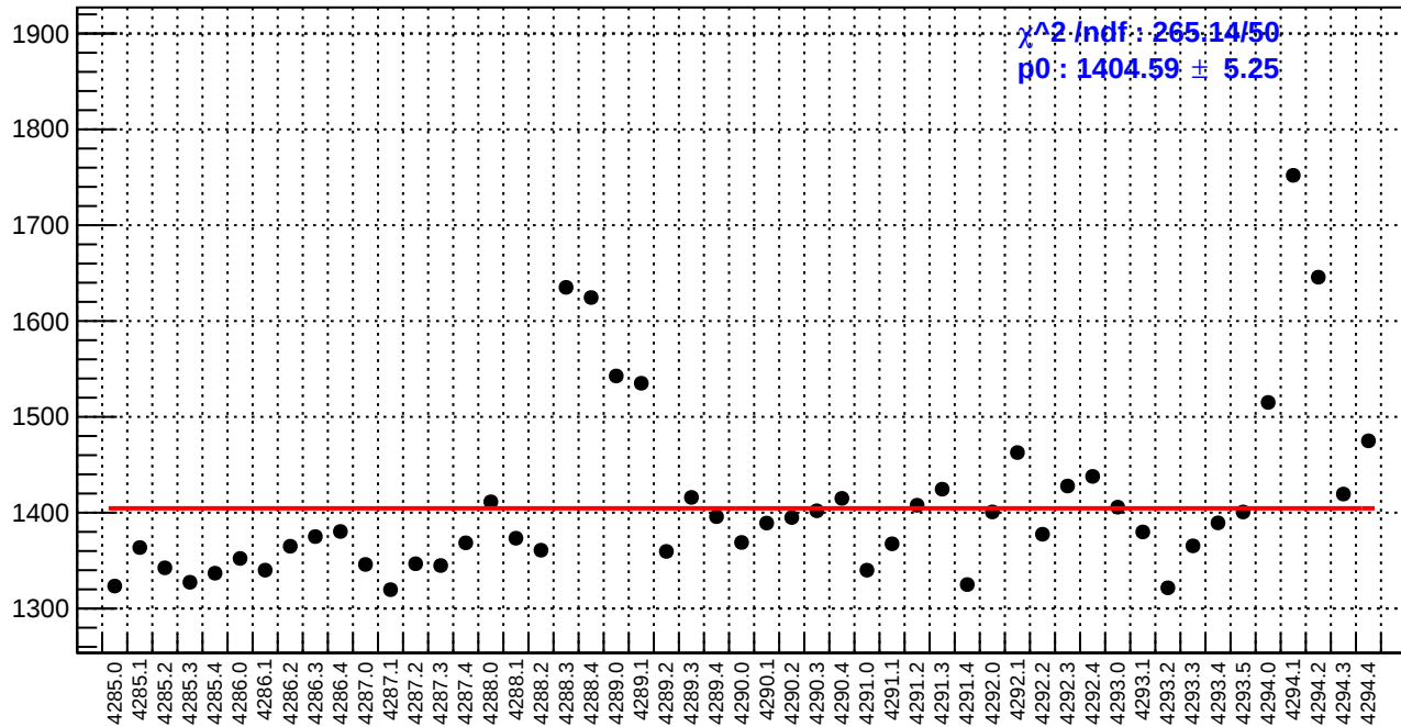
slug53: reg_asym_sam4.rms/ppm
