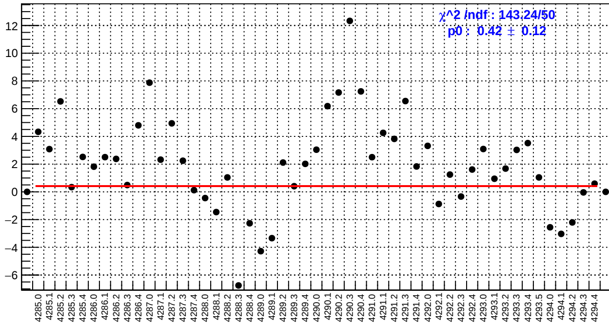
slug53: usl_bpm4aX/(ppb/nm)
