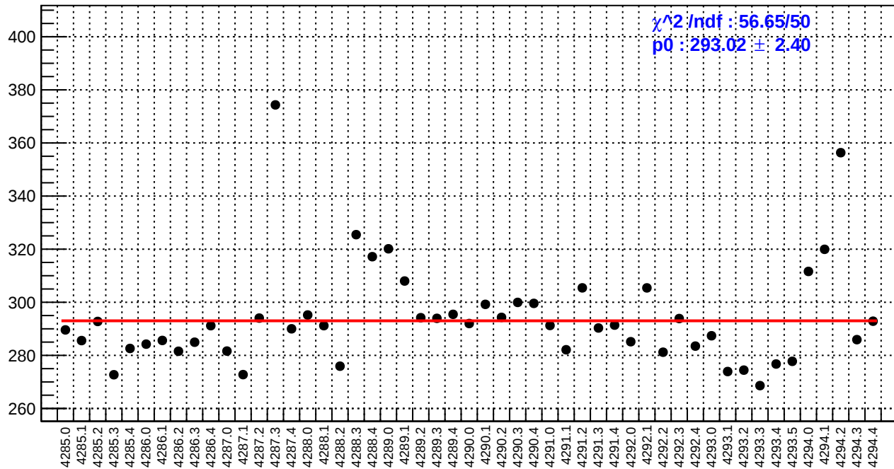
slug53: reg_asym_sam7.rms/ppm
