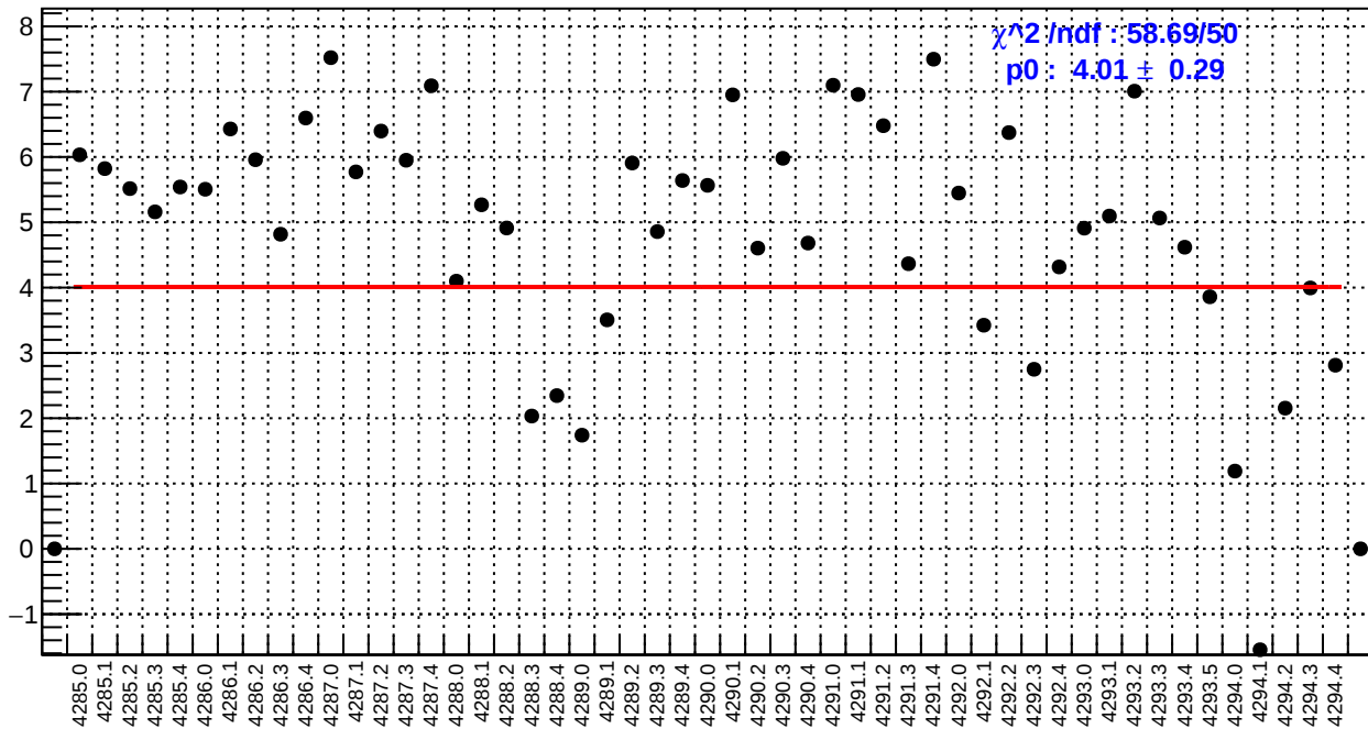
slug53: right_avg_bpm4aY/(ppb/nm)
