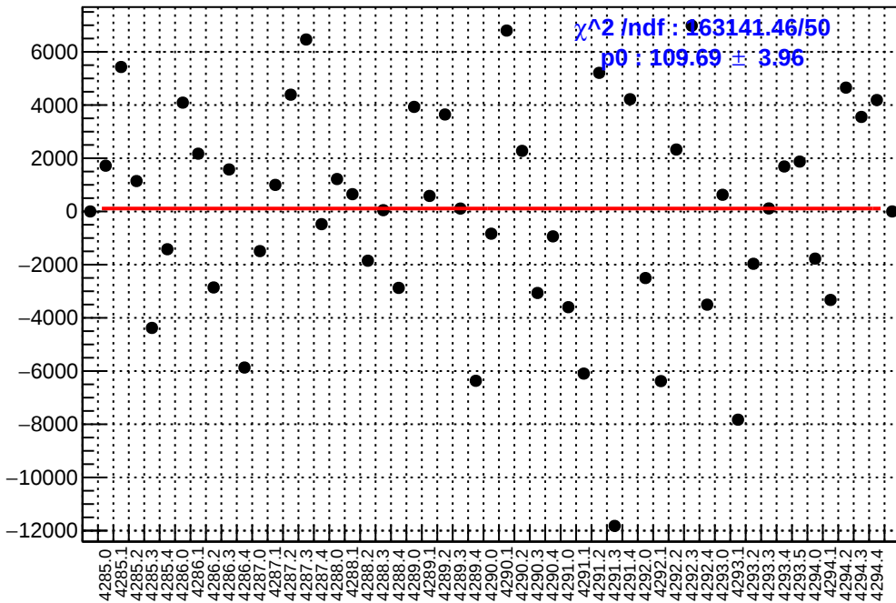
slug53: asym_us_dd.mean/ppb-reg_asym_us_dd.mean/ppb
