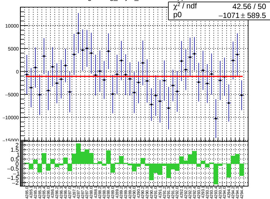
slug53: reg_asym_sam1.mean/ppb
