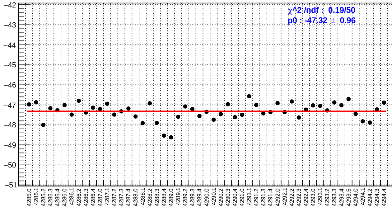
slug53: usl_bpm12X/(ppb/nm)
