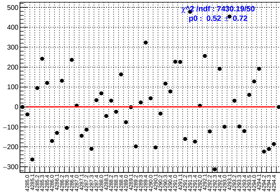
slug53: asym_left_dd.mean/ppb-reg_asym_left_dd.mean/ppb
