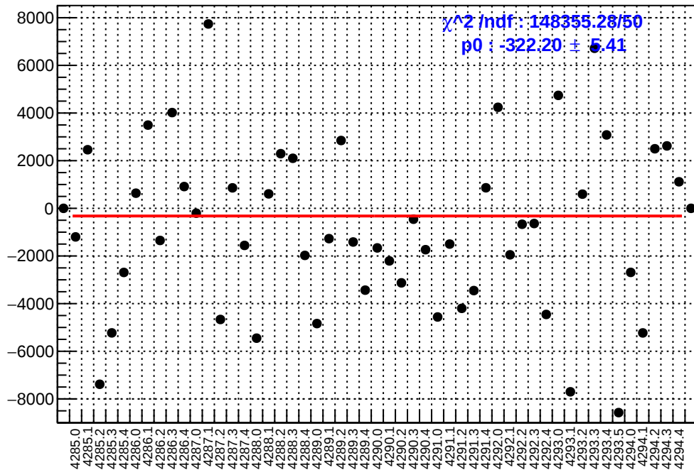
slug53: asym_ds_avg.mean/ppb-reg_asym_ds_avg.mean/ppb
