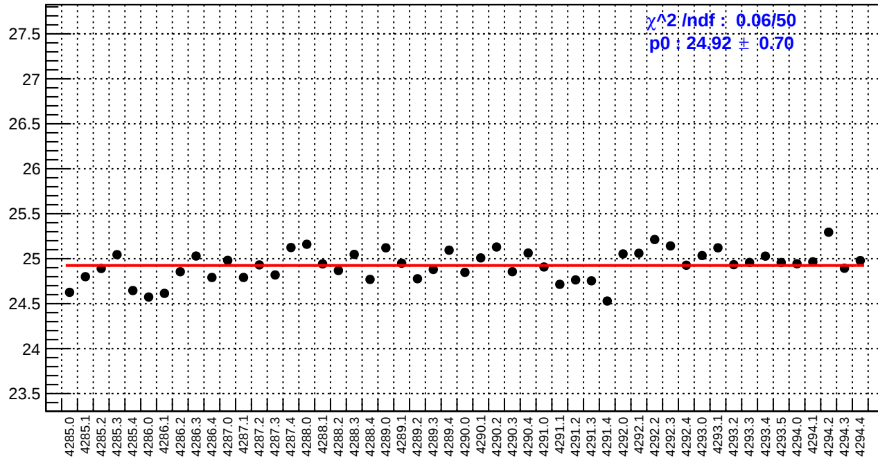
slug53: reg_asym_left_dd.rms/ppm
