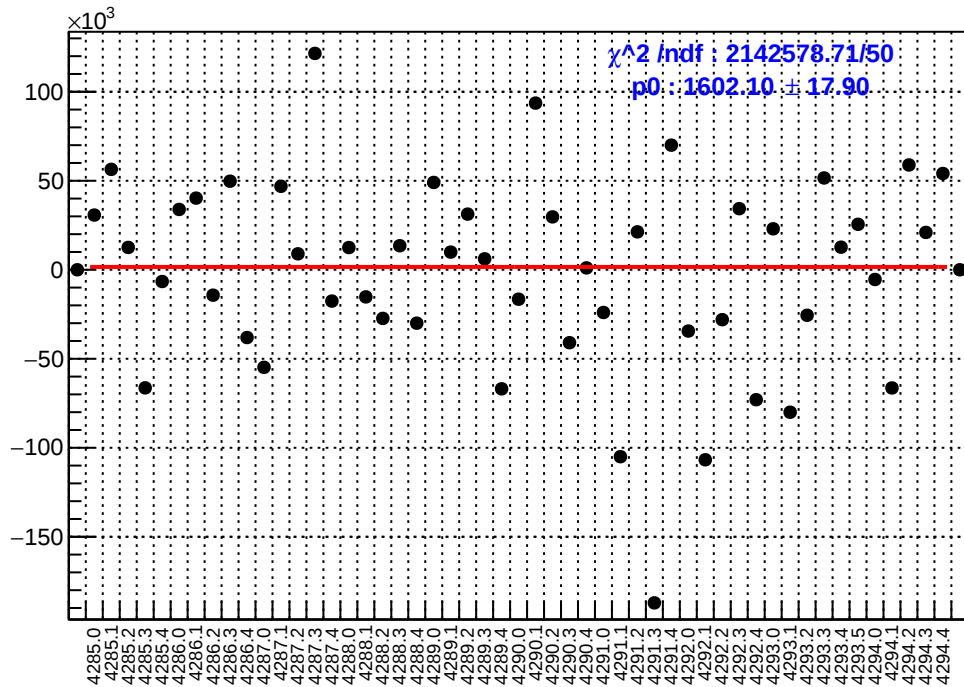
slug53: asym_sam4.mean/ppb-reg_asym_sam4.mean/ppb
