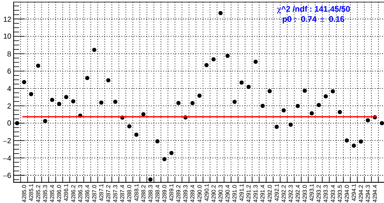
slug53: left_avg_bpm4aX/(ppb/nm)
