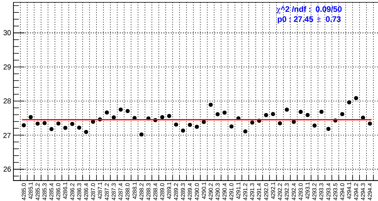
slug53: reg_asym_right_dd.rms/ppm
