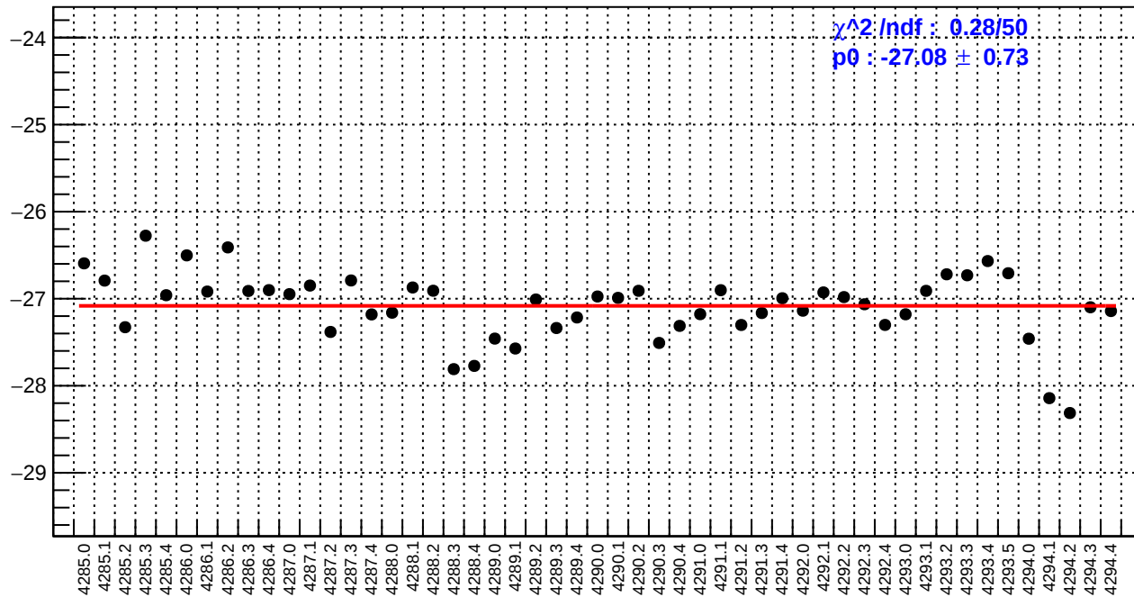
slug53: ds_avg_bpm4eX/(ppb/nm)
