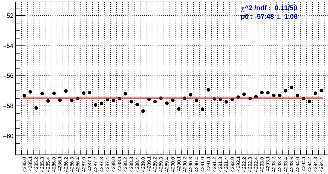
slug53: ds_avg_bpm12X/(ppb/nm)
