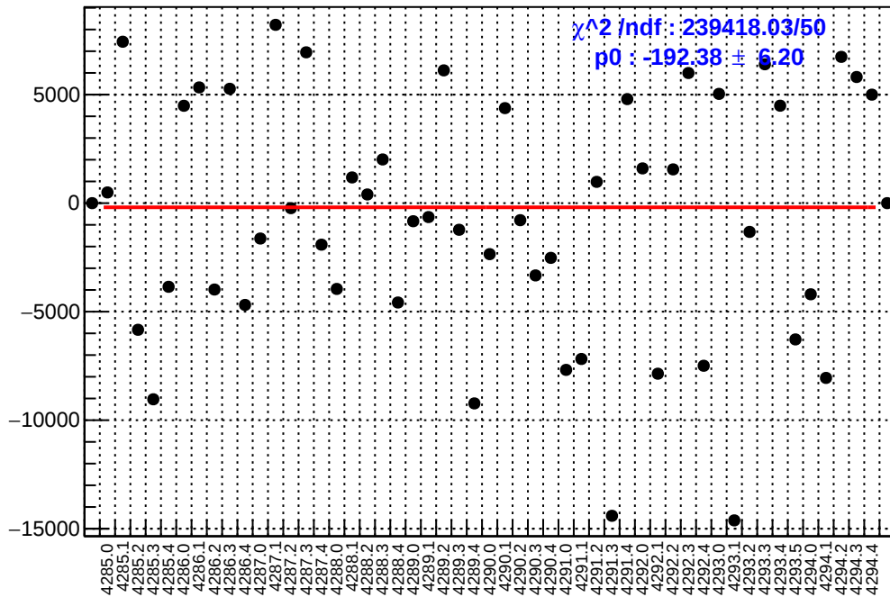
slug53: asym_left_avg.mean/ppb-reg_asym_left_avg.mean/ppb
