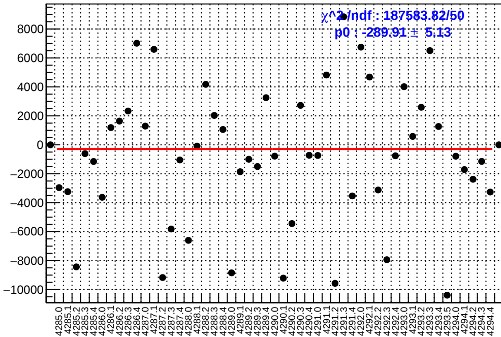
slug53: asym_right_avg.mean/ppb-reg_asym_right_avg.mean/ppb
