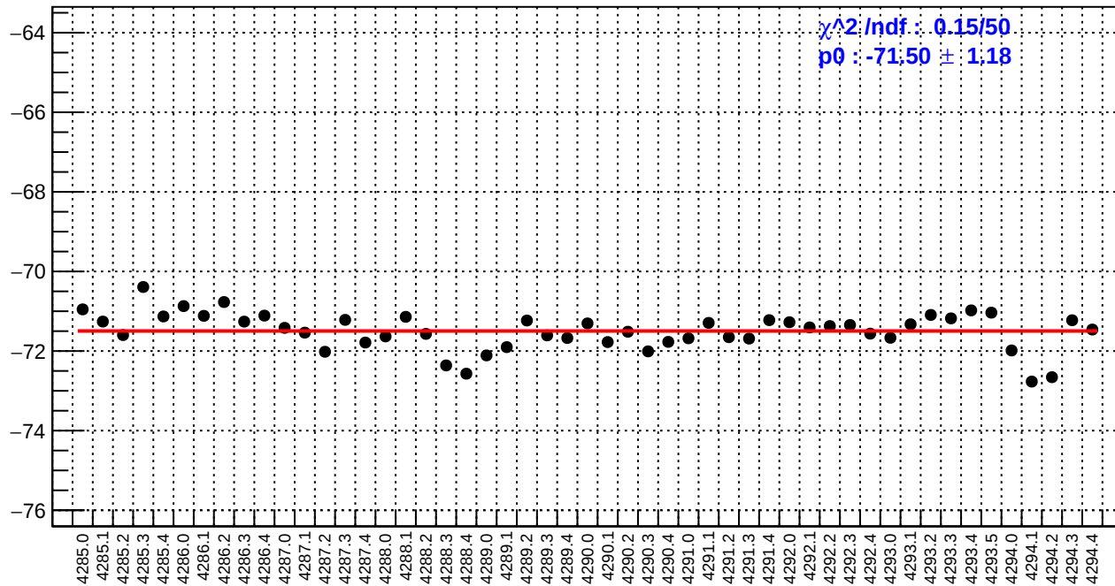
slug53: left_avg_bpm4eX/(ppb/nm)
