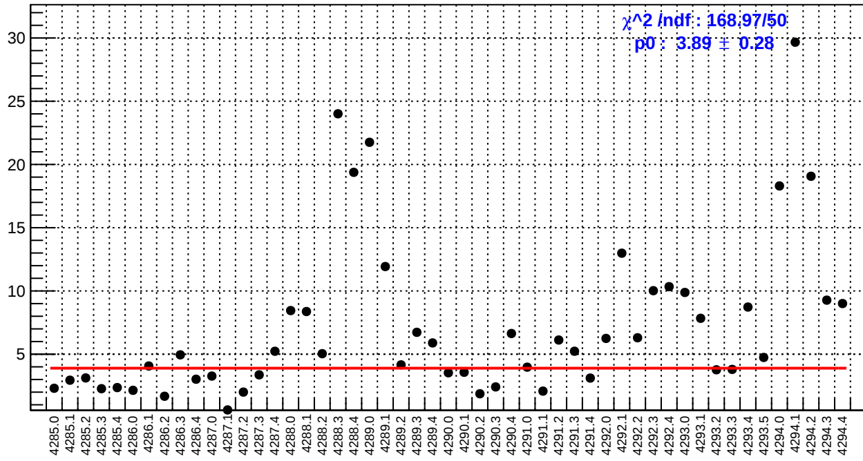
slug53: left_avg_bpm4aY/(ppb/nm)
