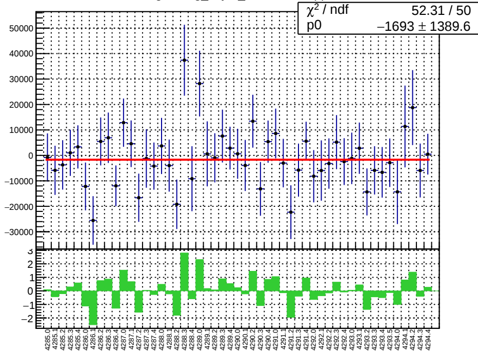
slug53: reg_asym_sam3.mean/ppb
