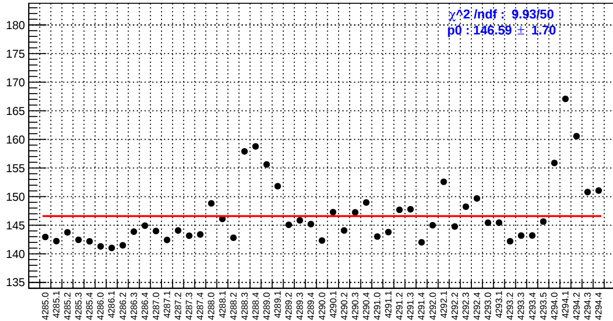
slug53: reg_asym_dsl.rms/ppm
