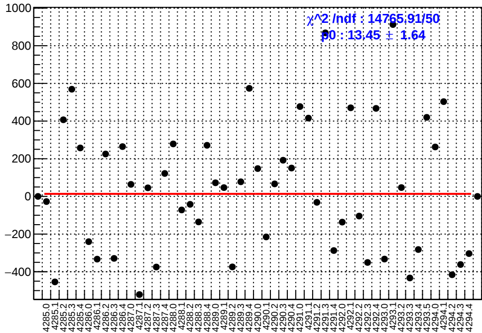
slug53: asym_right_dd.mean/ppb-reg_asym_right_dd.mean/ppb
