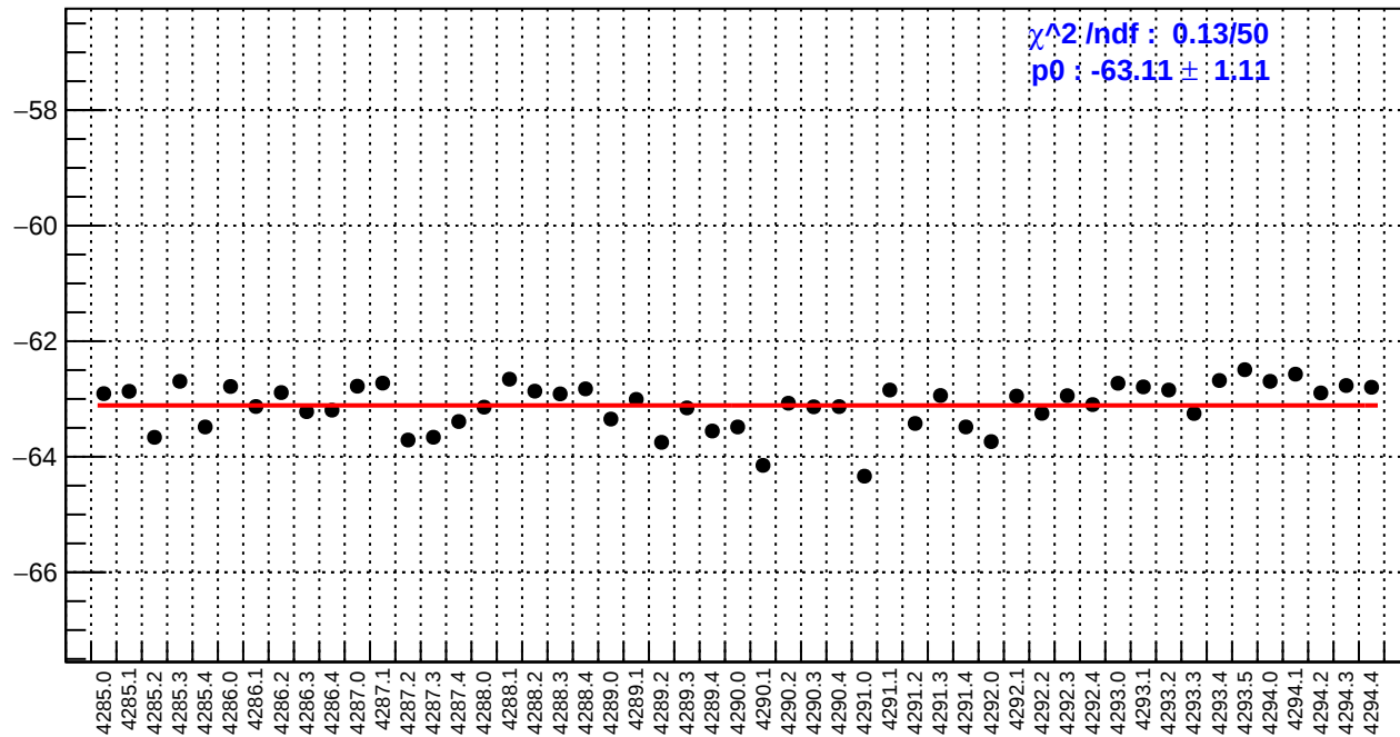
slug53: right_avg_bpm12X/(ppb/nm)
