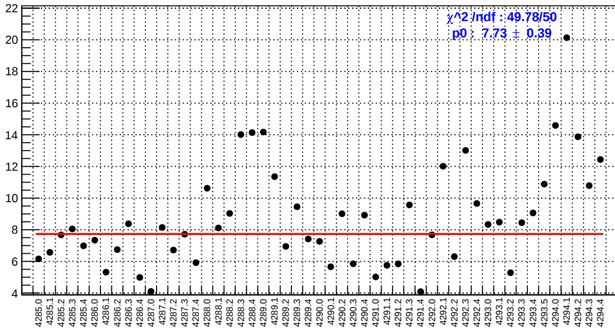
slug53: right_avg_bpm4eY/(ppb/nm)
