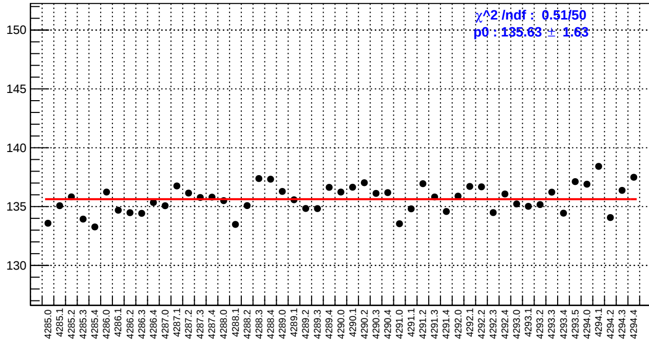
slug53: reg_asym_usr.rms/ppm
