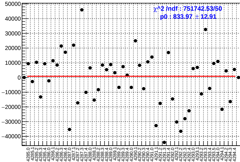
slug53: asym_sam5.mean/ppb-reg_asym_sam5.mean/ppb
