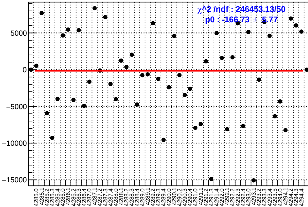
slug53: asym_dsl.mean/ppb-reg_asym_dsl.mean/ppb
