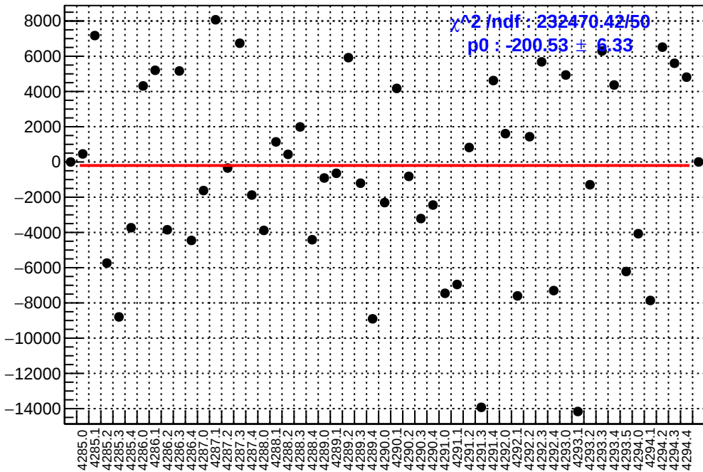
slug53: asym_usl.mean/ppb-reg_asym_usl.mean/ppb
