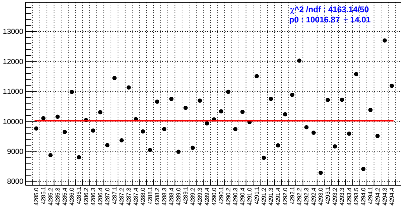
slug53: diff_bpm4aY.rms/nm
