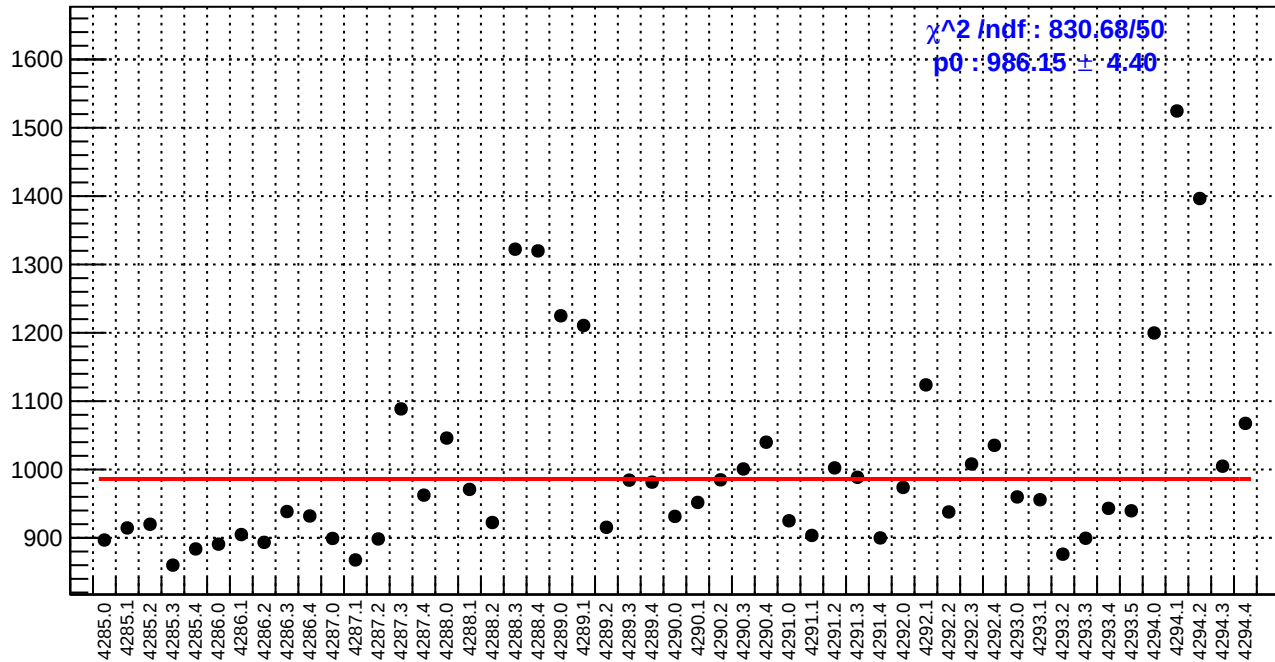
slug53: reg_asym_sam3.rms/ppm
