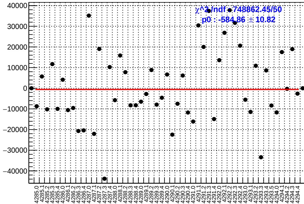
slug53: asym_sam1.mean/ppb-reg_asym_sam1.mean/ppb
