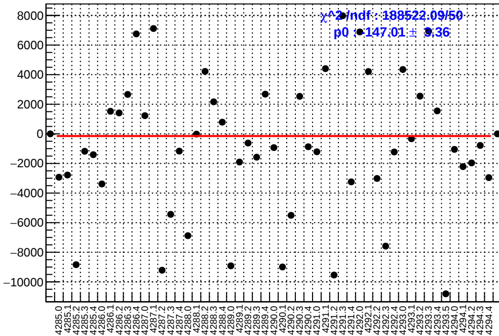
slug53: asym_dsr.mean/ppb-reg_asym_dsr.mean/ppb
