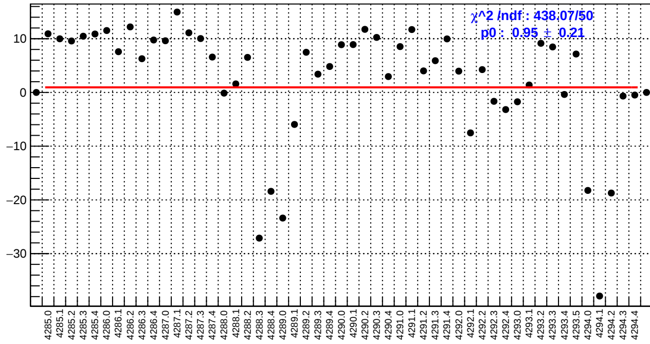
slug53: dsl_bpm4eY/(ppb/nm)
