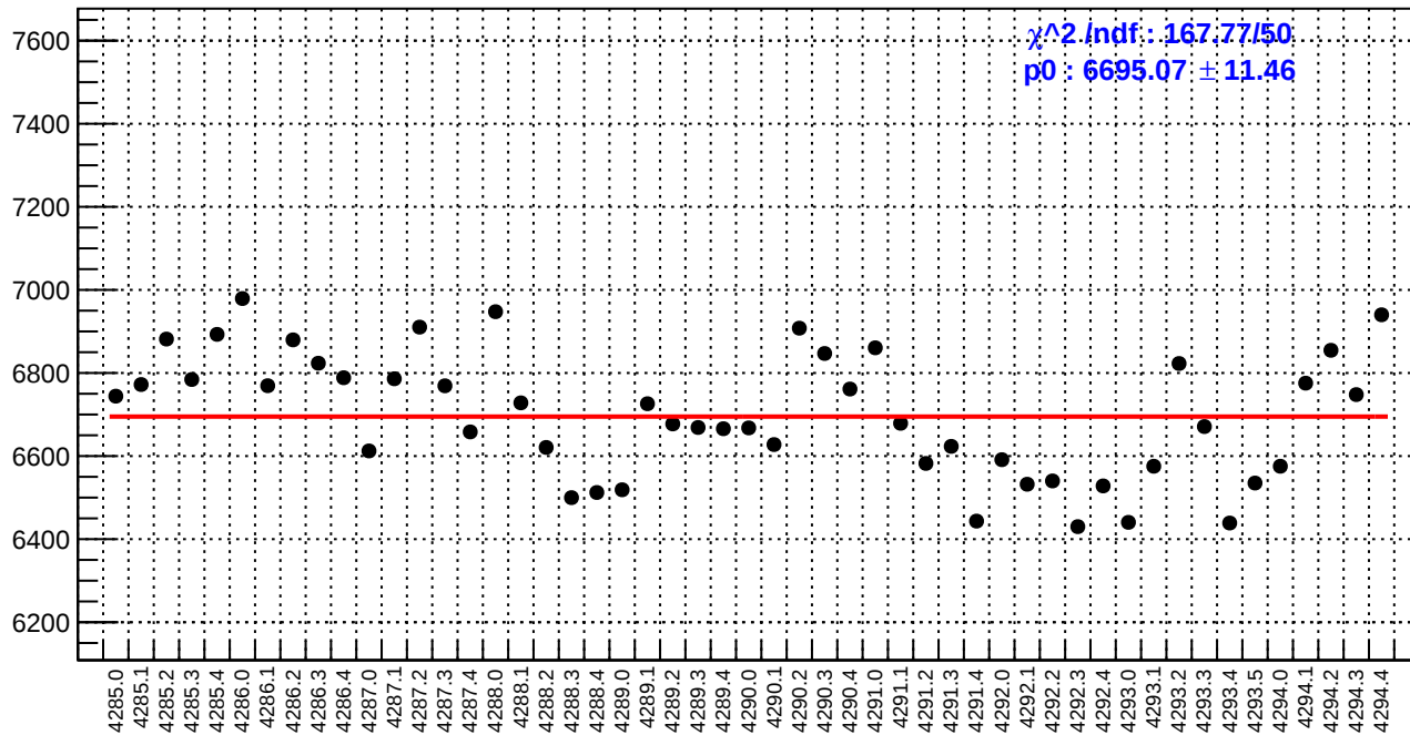
slug53: diff_bpm11X.rms/nm
