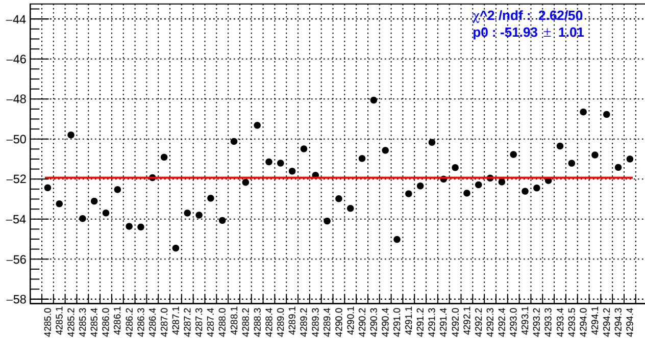
slug53: right_avg_bpm4aX/(ppb/nm)
