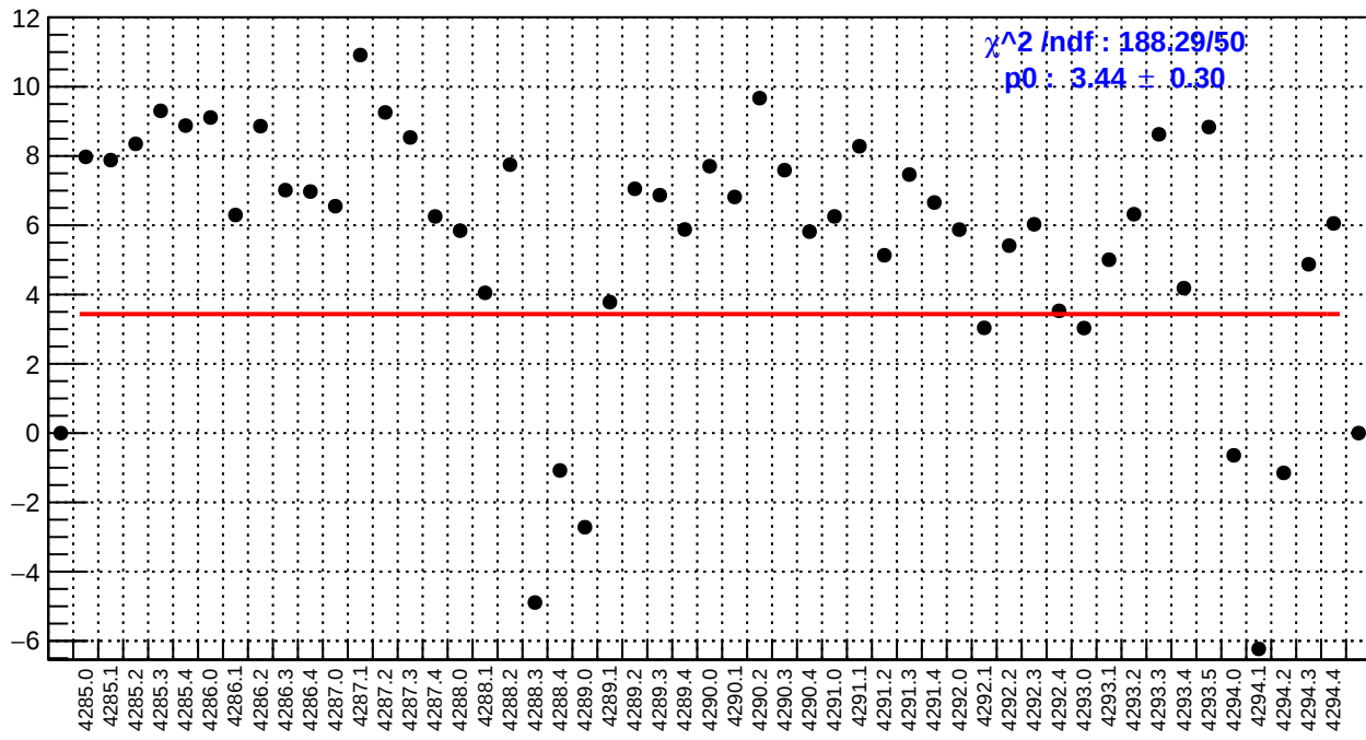
slug53: us_avg_bpm4eY/(ppb/nm)
