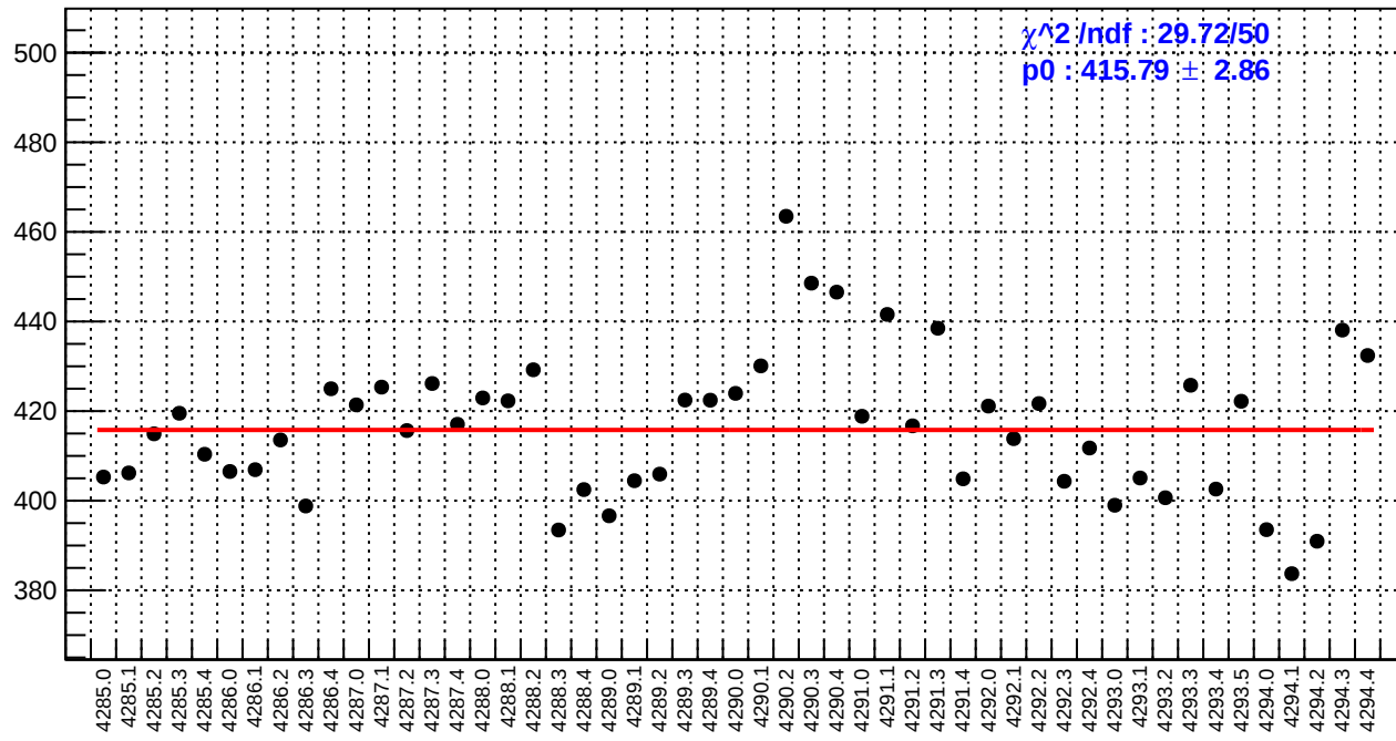
slug53: reg_asym_sam1.rms/ppm
