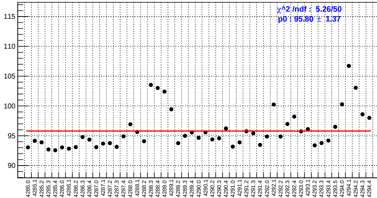
slug53: reg_asym_us_dd.rms/ppm
