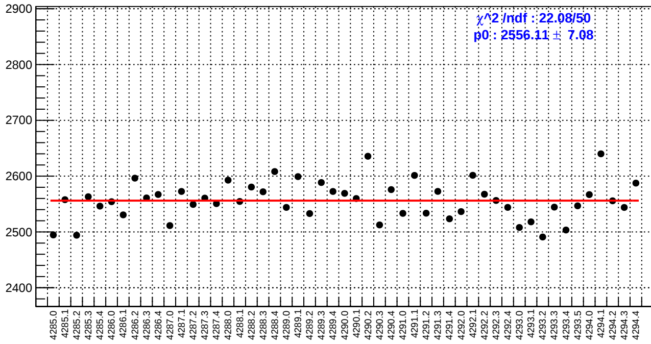
slug53: reg_asym_sam2.rms/ppm
