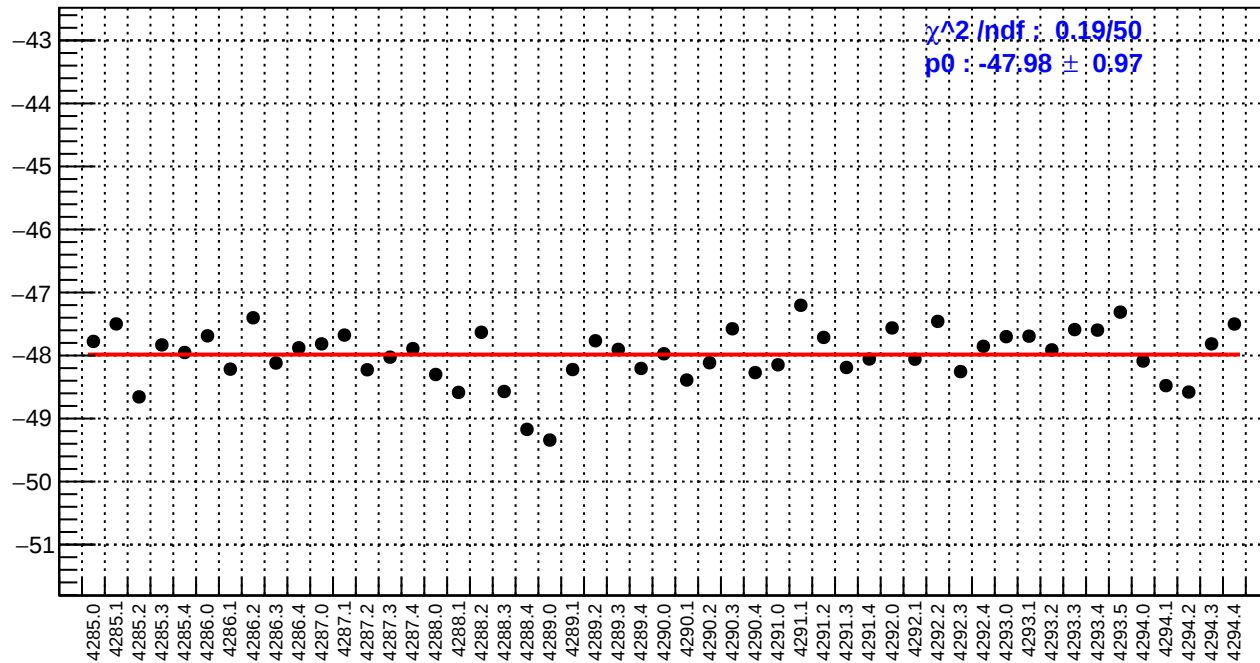
slug53: left_avg_bpm12X/(ppb/nm)
