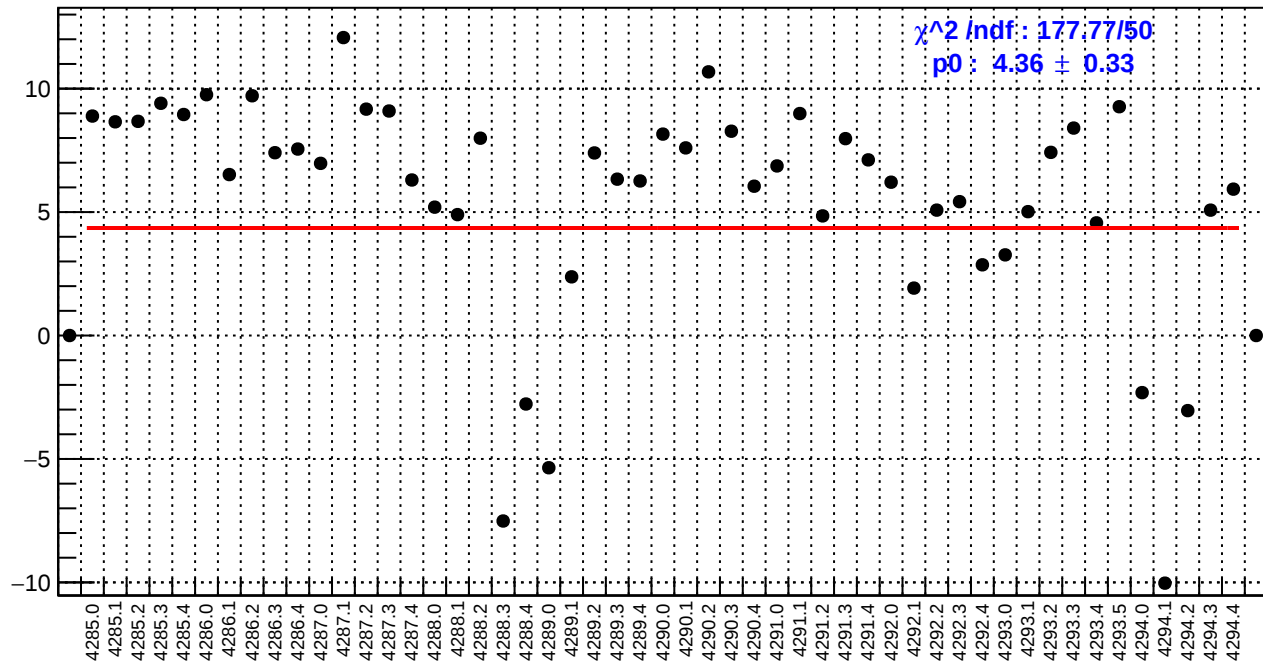
slug53: ds_avg_bpm4eY/(ppb/nm)
