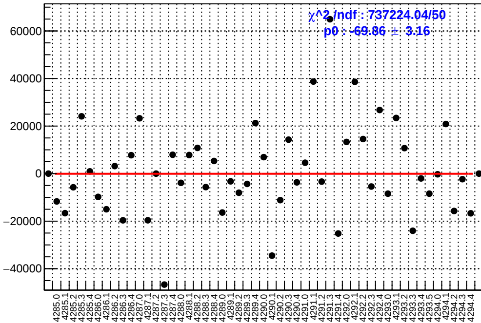
slug53: asym_sam8.mean/ppb-reg_asym_sam8.mean/ppb
