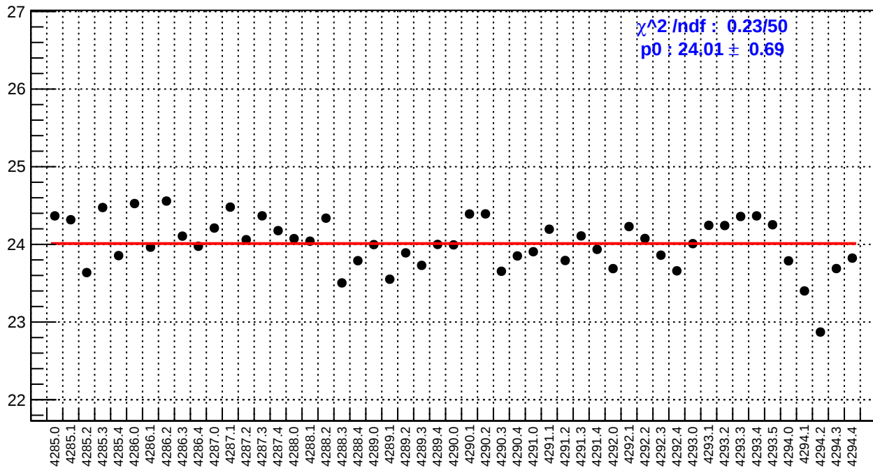
slug53: right_avg_bpm4eX/(ppb/nm)
