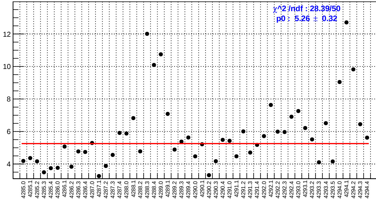
slug53: us_avg_bpm4aY/(ppb/nm)
