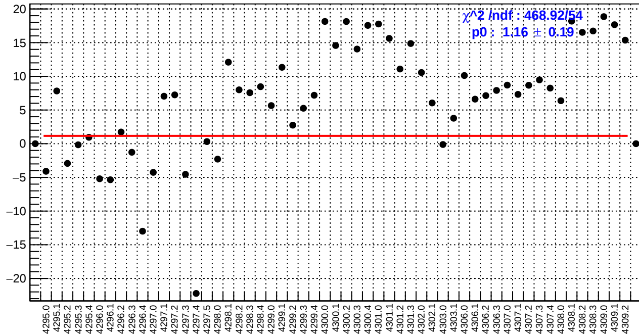
slug54: ds_avg_bpm4eY/(ppb/nm)
