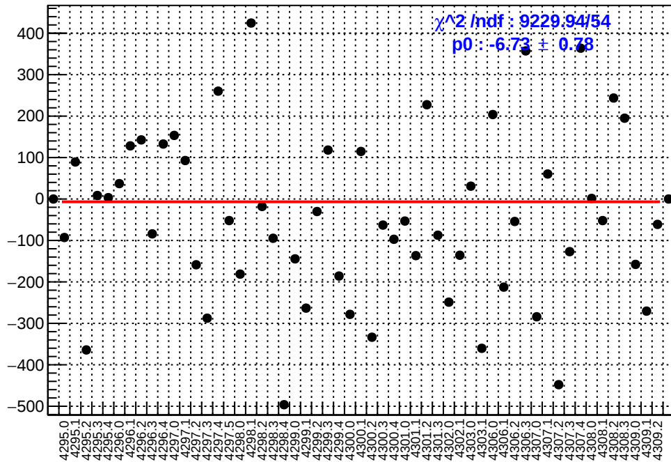
slug54: asym_left_dd.mean/ppb-reg_asym_left_dd.mean/ppb
