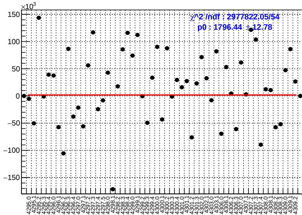
slug54: asym_sam2.mean/ppb-reg_asym_sam2.mean/ppb
