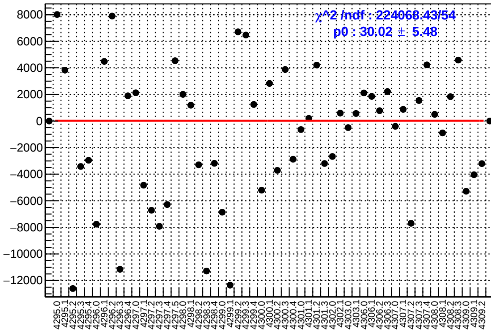
slug54: asym_right_avg.mean/ppb-reg_asym_right_avg.mean/ppb
