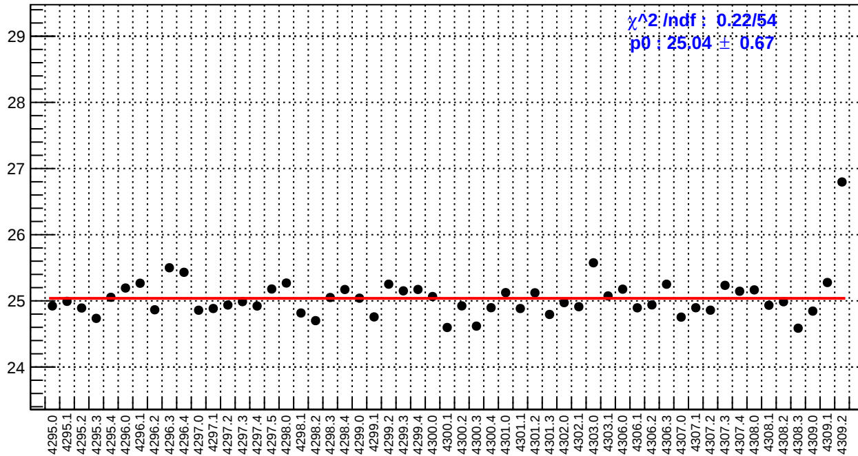
slug54: reg_asym_left_dd.rms/ppm
