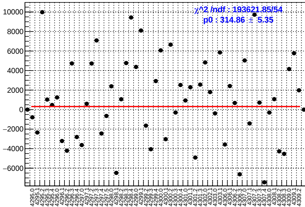
slug54: asym_ds_dd.mean/ppb-reg_asym_ds_dd.mean/ppb
