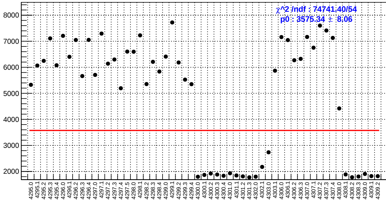
slug54: diff_bpm4eY.rms/nm
