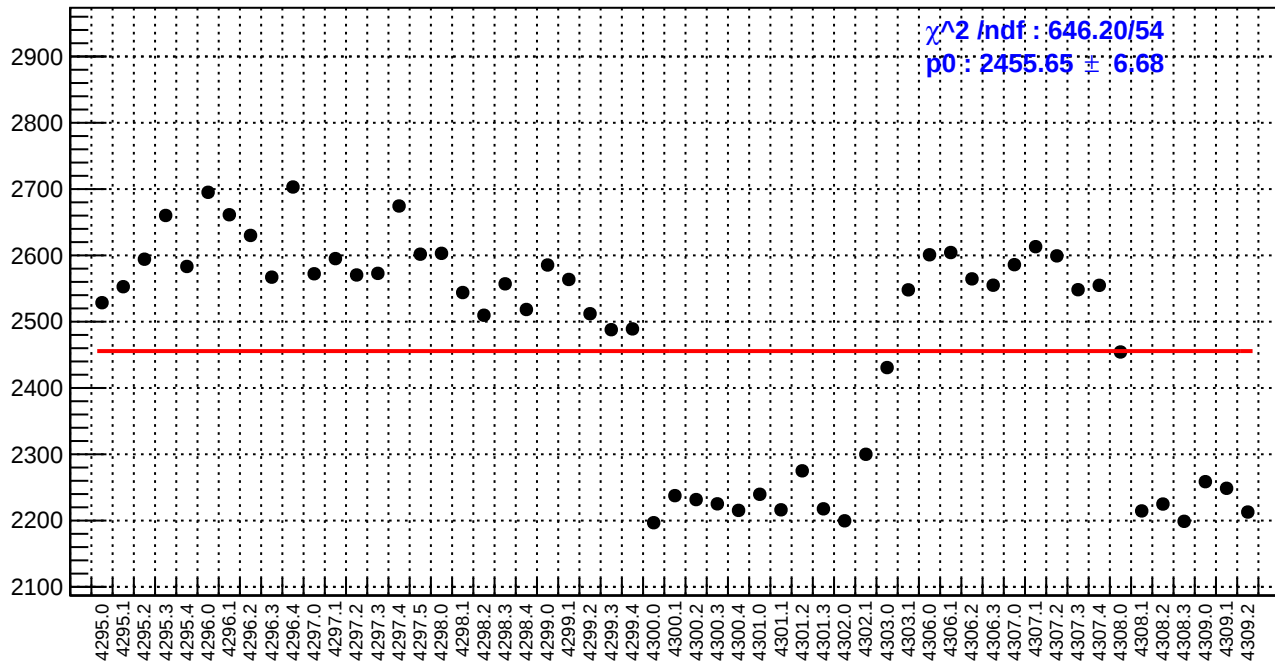
slug54: reg_asym_sam2.rms/ppm
