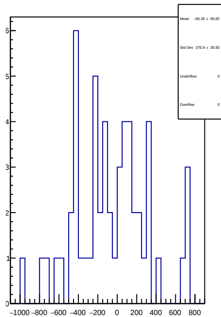
slug54: 1D Corr asym_right_dd.mean/ppb-reg_asym_right_dd.mean/ppb
