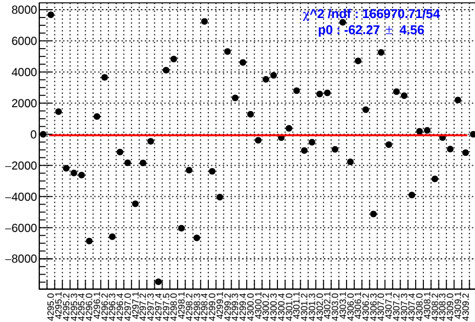
slug54: asym_ds_avg.mean/ppb-reg_asym_ds_avg.mean/ppb
