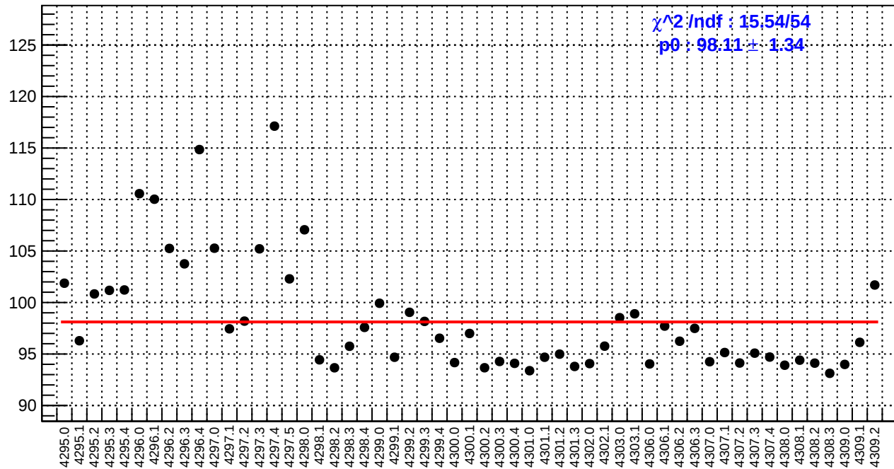
slug54: reg_asym_us_dd.rms/ppm
