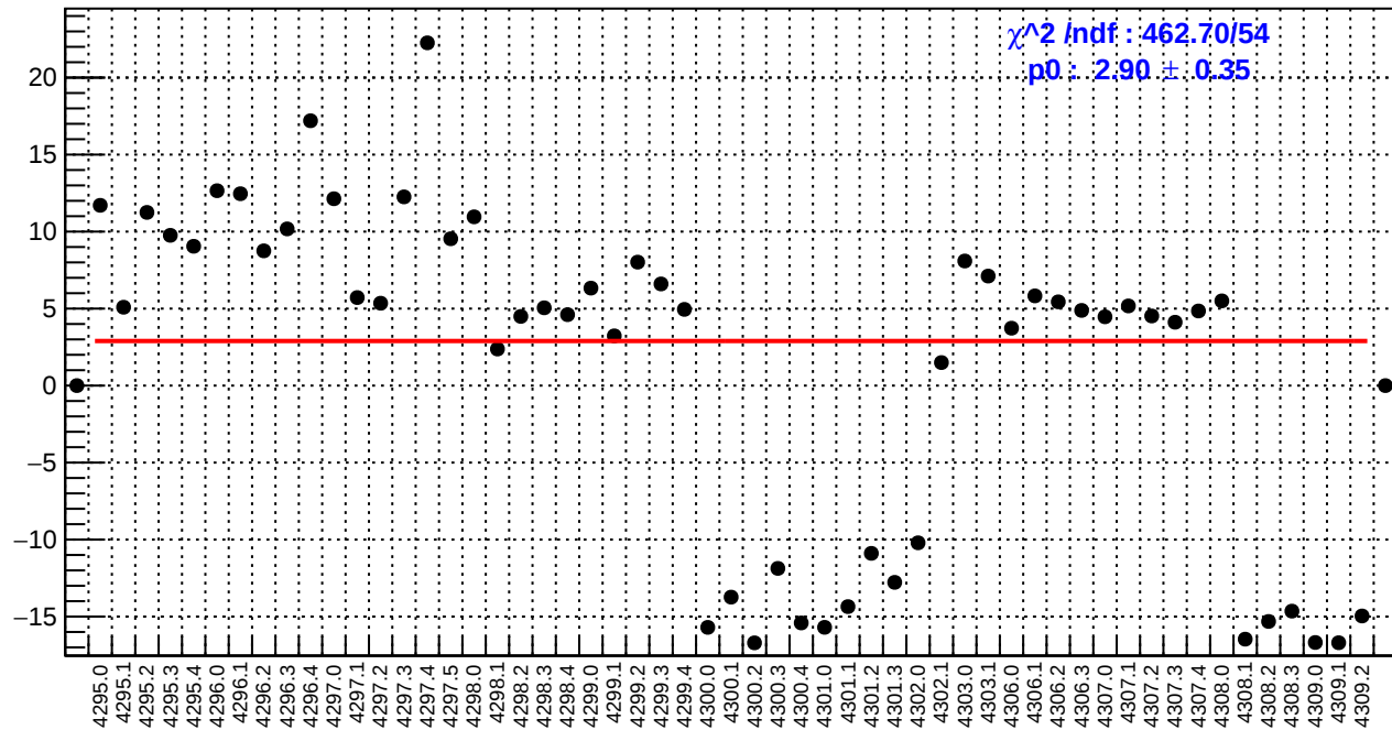
slug54: ds_avg_bpm4aY/(ppb/nm)
