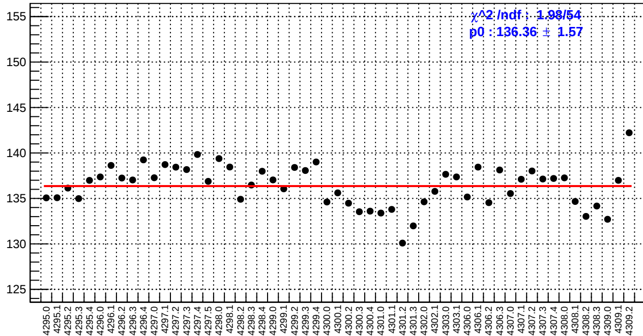
slug54: reg_asym_right_avg.rms/ppm
