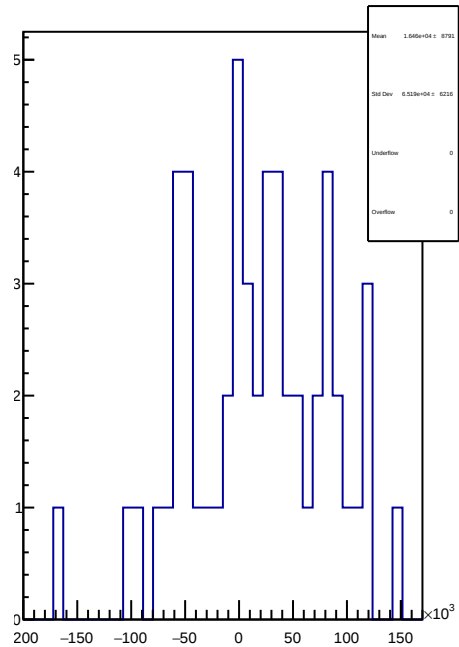
slug54: 1D Corr asym_sam2.mean/ppb-reg_asym_sam2.mean/ppb
