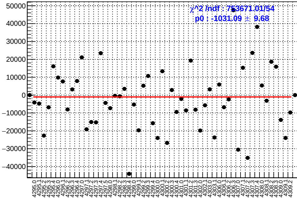
slug54: asym_sam8.mean/ppb-reg_asym_sam8.mean/ppb
