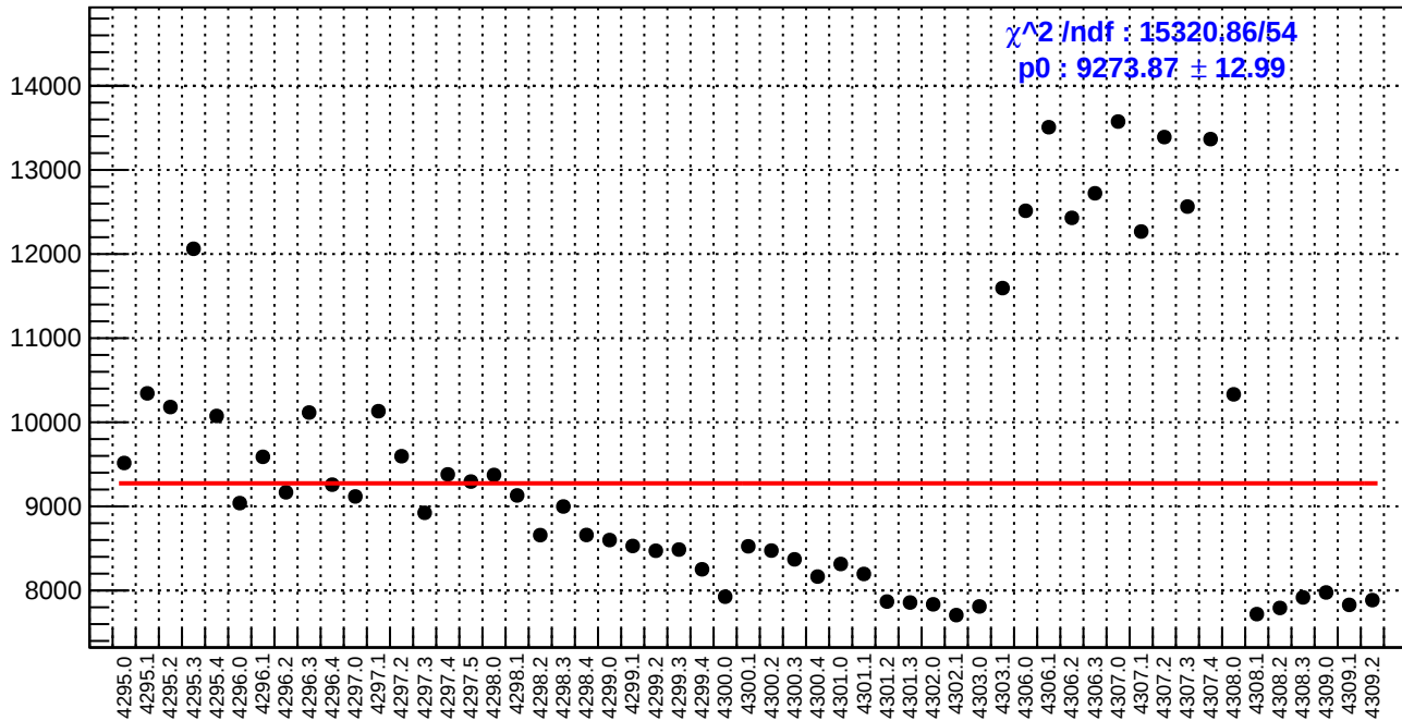
slug54: diff_bpm4eX.rms/nm
