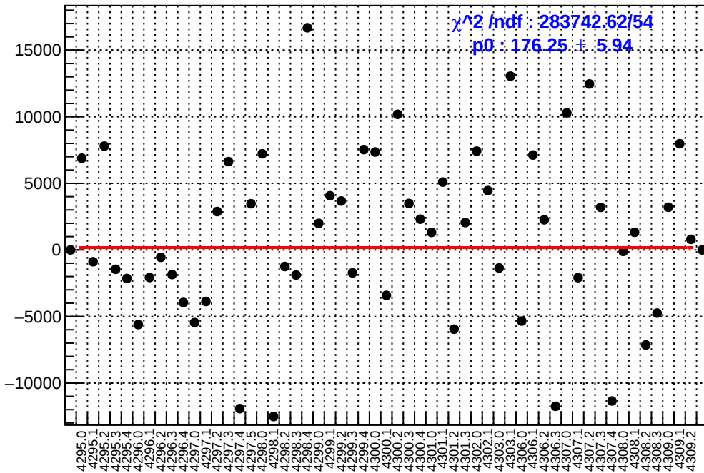
slug54: asym_dsl.mean/ppb-reg_asym_dsl.mean/ppb
