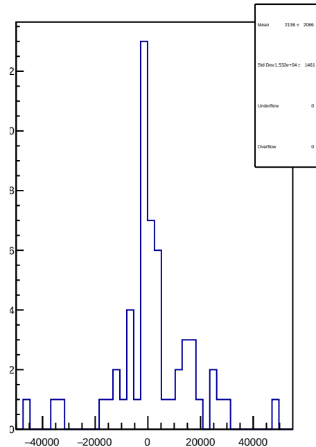
slug54: 1D Corr asym_sam1.mean/ppb-reg_asym_sam1.mean/ppb
