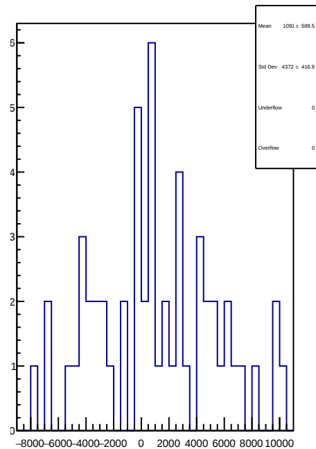
slug54: 1D Corr asym_us_dd.mean/ppb-reg_asym_us_dd.mean/ppb
