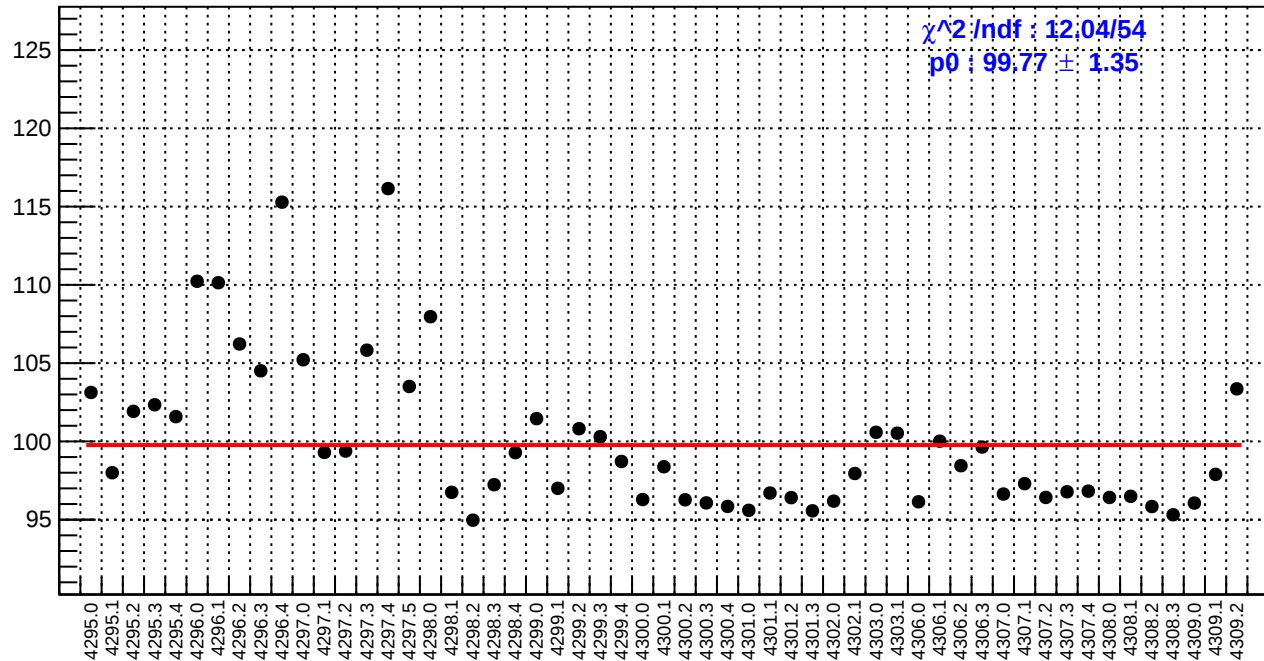
slug54: reg_asym_ds_dd.rms/ppm
