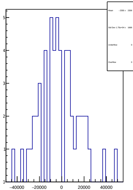
slug54: 1D Corr asym_sam8.mean/ppb-reg_asym_sam8.mean/ppb
