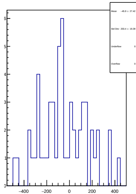
slug54: 1D Corr asym_left_dd.mean/ppb-reg_asym_left_dd.mean/ppb
