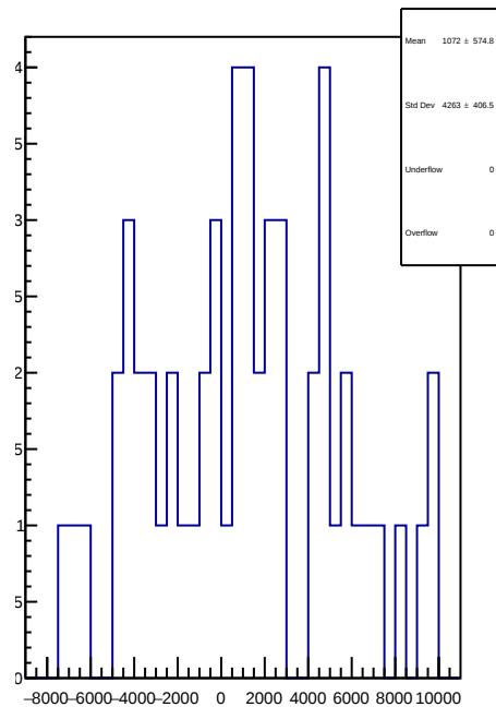
slug54: 1D Corr asym_ds_dd.mean/ppb-reg_asym_ds_dd.mean/ppb
