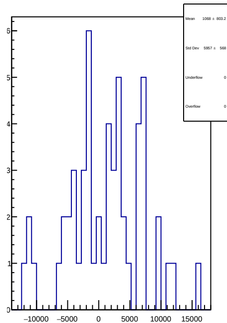
slug54: 1D Corr asym_usl.mean/ppb-reg_asym_usl.mean/ppb
