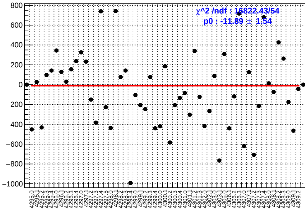
slug54: asym_right_dd.mean/ppb-reg_asym_right_dd.mean/ppb
