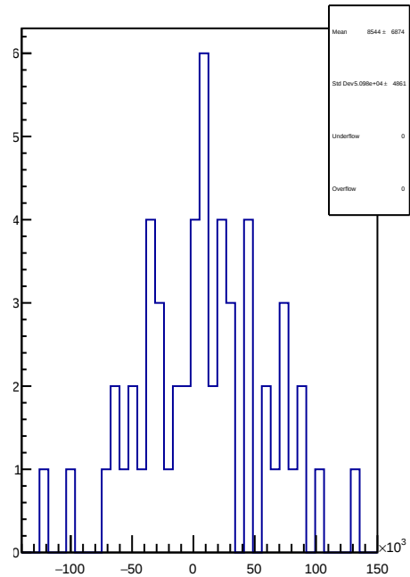
slug54: 1D Corr asym_sam4.mean/ppb-reg_asym_sam4.mean/ppb
