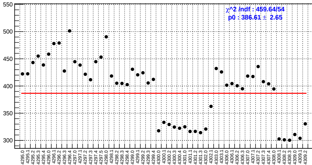
slug54: reg_asym_sam5.rms/ppm
