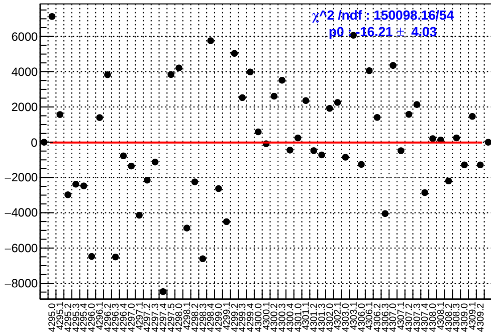
slug54: asym_us_avg.mean/ppb-reg_asym_us_avg.mean/ppb
