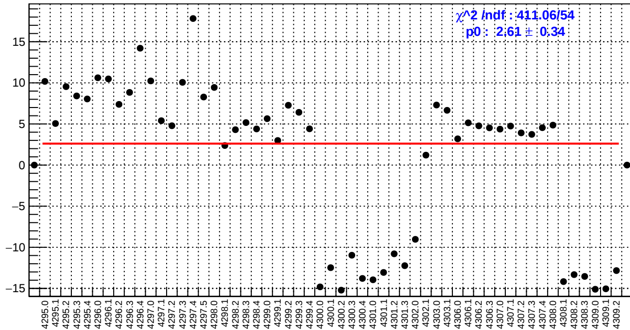
slug54: us_avg_bpm4aY/(ppb/nm)
