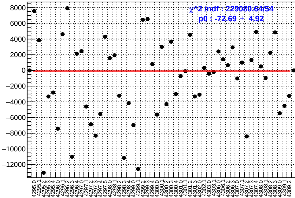
slug54: asym_usr.mean/ppb-reg_asym_usr.mean/ppb
