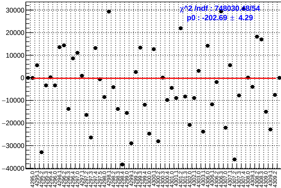
slug54: asym_sam7.mean/ppb-reg_asym_sam7.mean/ppb
