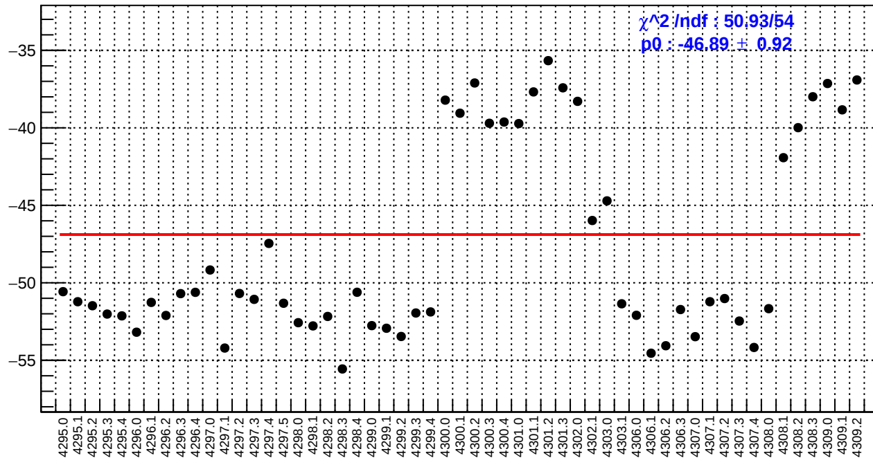
slug54: right_avg_bpm4aX/(ppb/nm)
