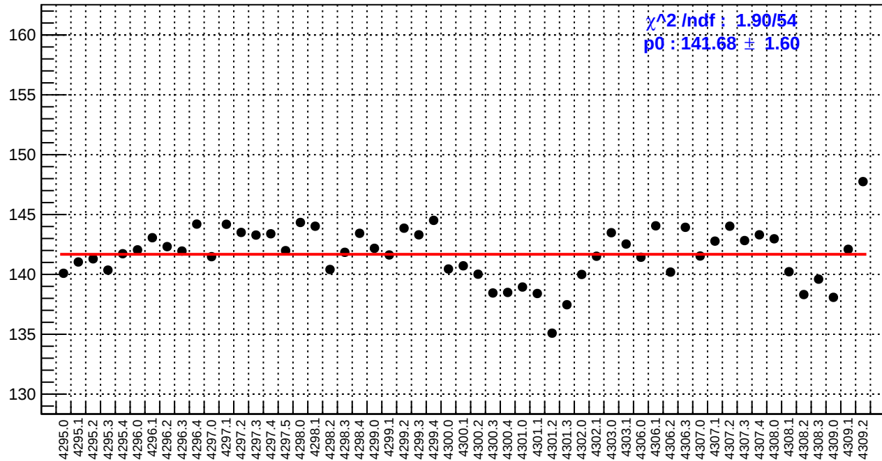
slug54: reg_asym_dsr.rms/ppm
