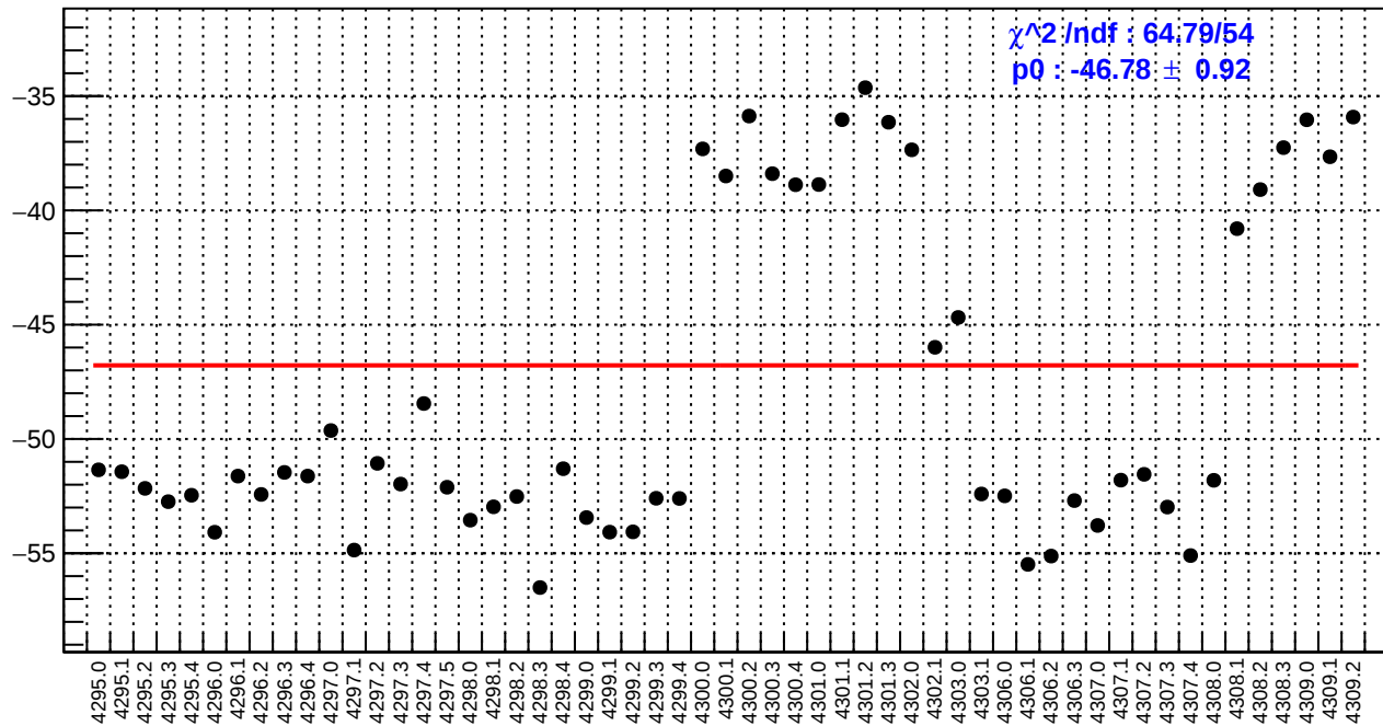
slug54: dsr_bpm4aX/(ppb/nm)
