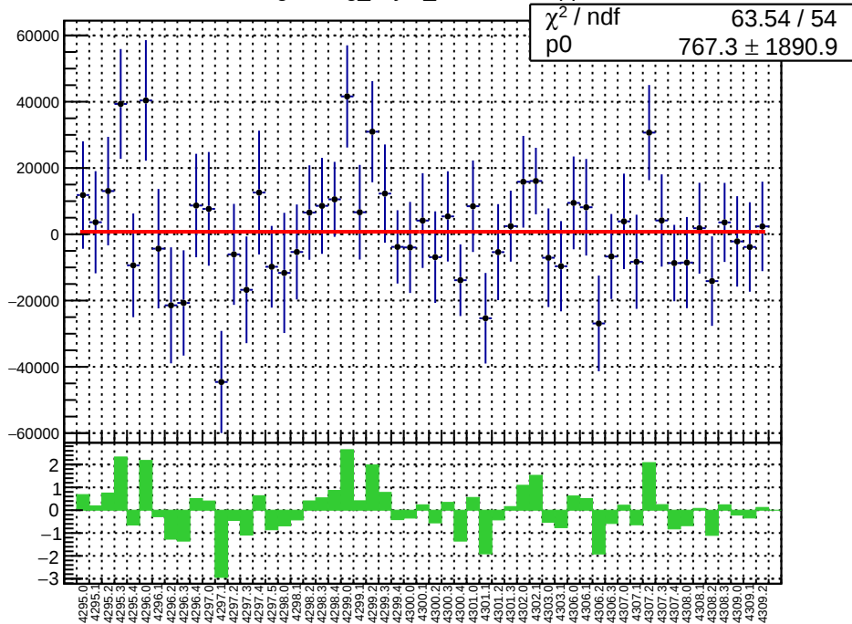
slug54: reg_asym_sam4.mean/ppb
