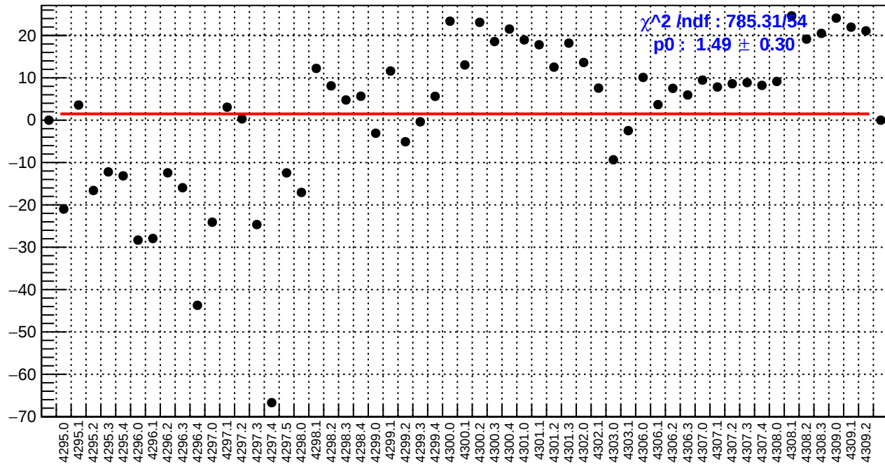
slug54: left_avg_bpm4eY/(ppb/nm)
