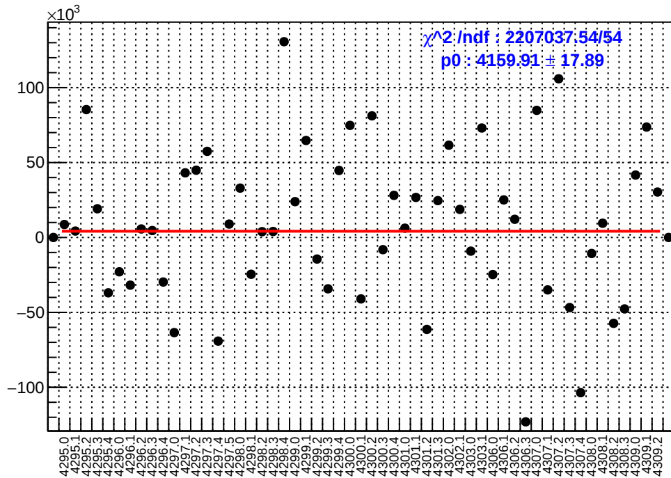
slug54: asym_sam4.mean/ppb-reg_asym_sam4.mean/ppb
