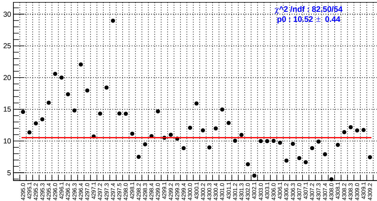
slug54: right_avg_bpm4eY/(ppb/nm)
