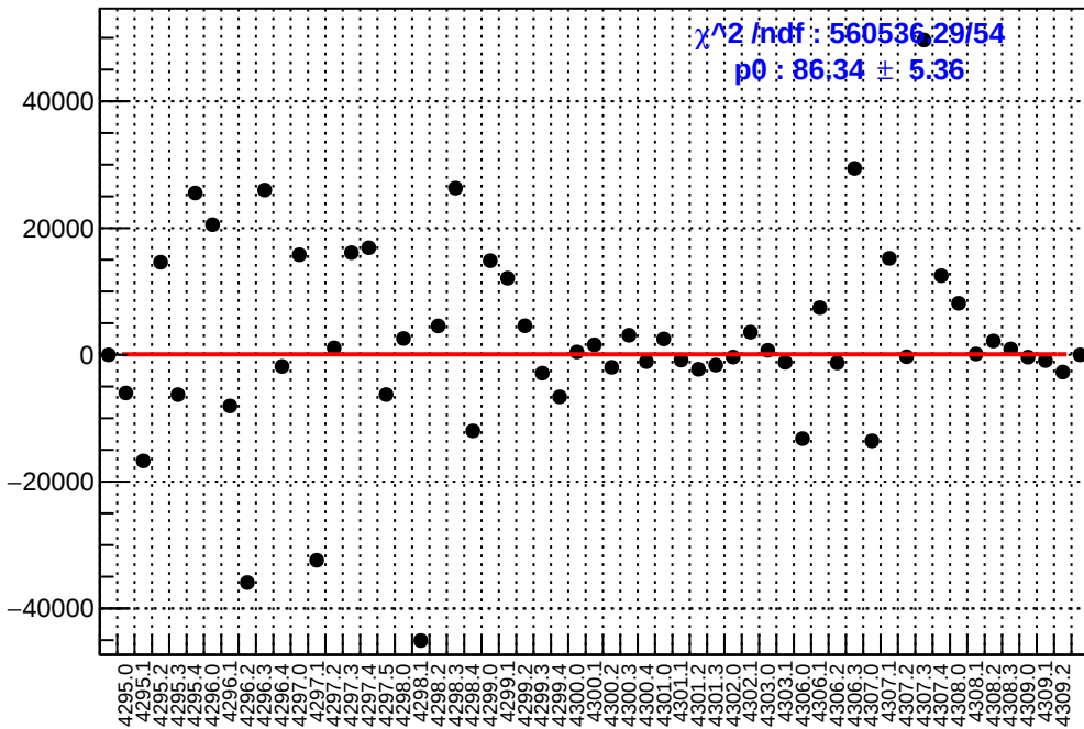
slug54: asym_sam1.mean/ppb-reg_asym_sam1.mean/ppb
