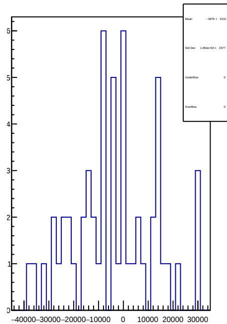
slug54: 1D Corr asym_sam7.mean/ppb-reg_asym_sam7.mean/ppb
