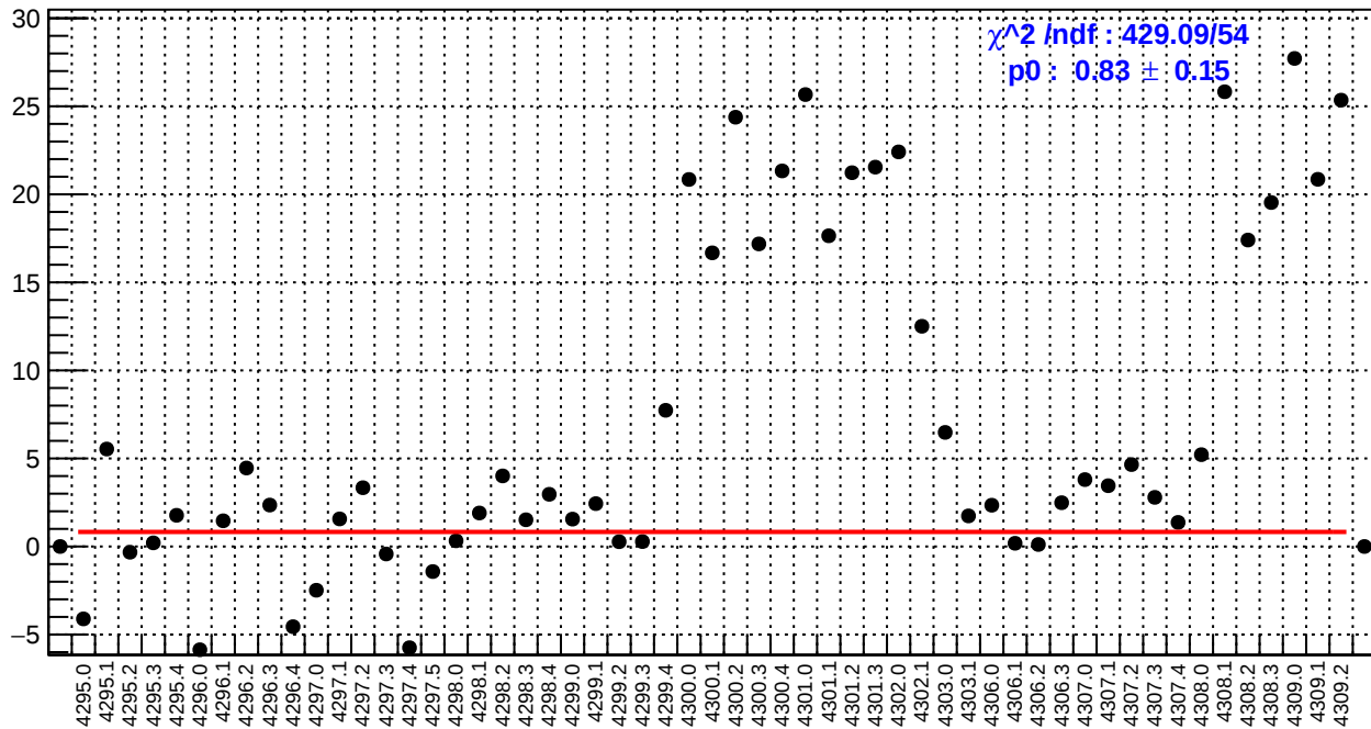
slug54: dsl_bpm4aX/(ppb/nm)
