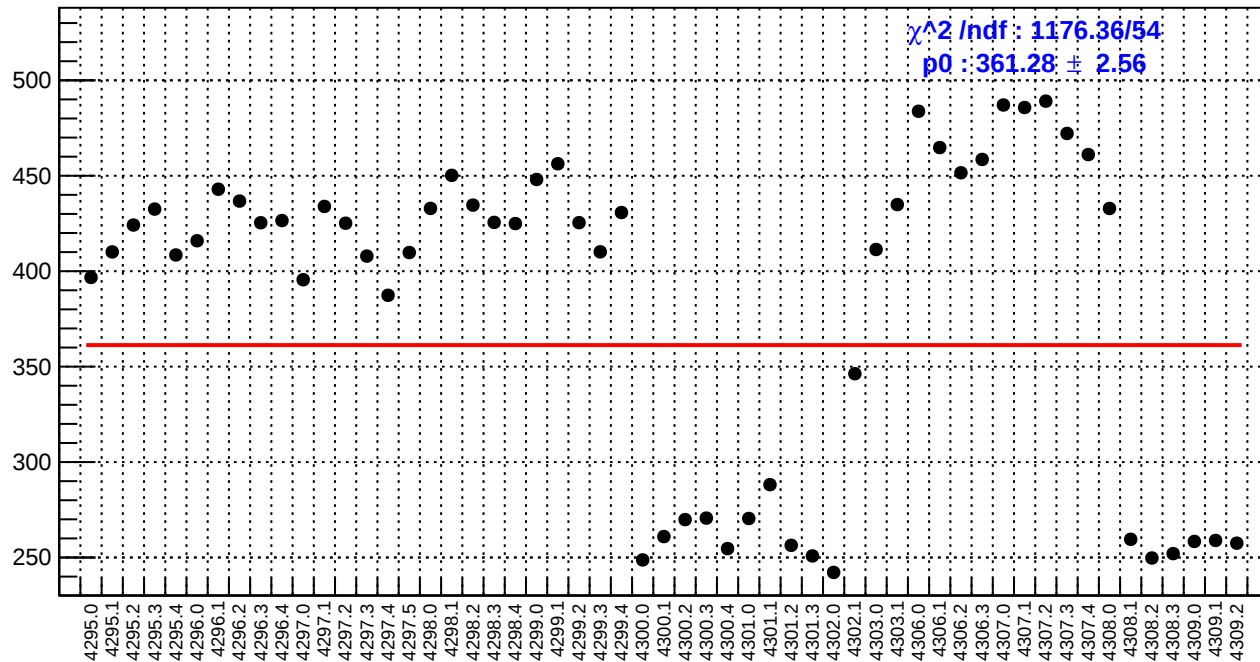
slug54: reg_asym_sam1.rms/ppm
