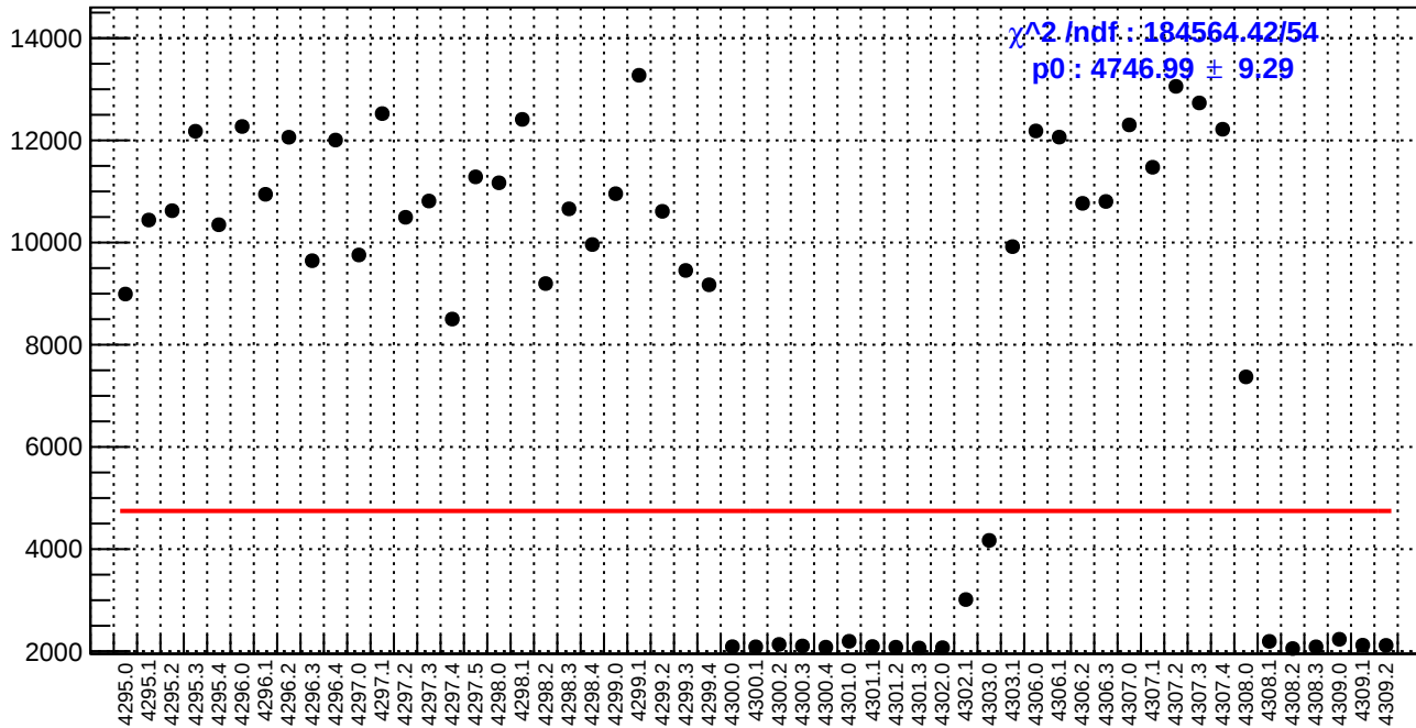
slug54: diff_bpm4aY.rms/nm
