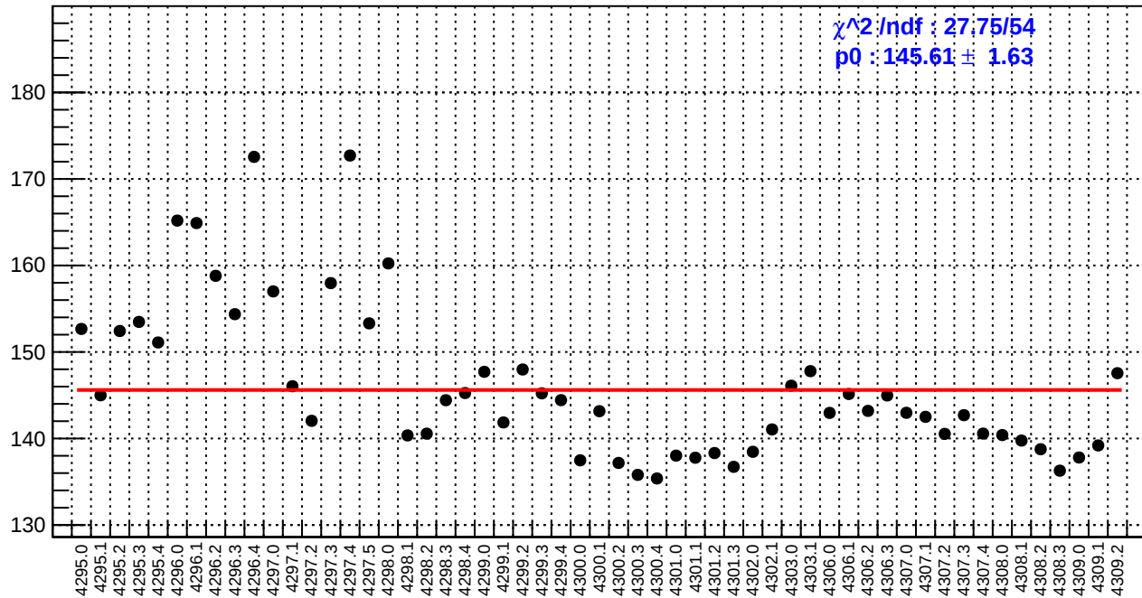
slug54: reg_asym_usl.rms/ppm
