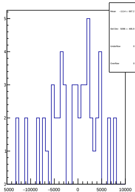
slug54: 1D Corr asym_usr.mean/ppb-reg_asym_usr.mean/ppb
