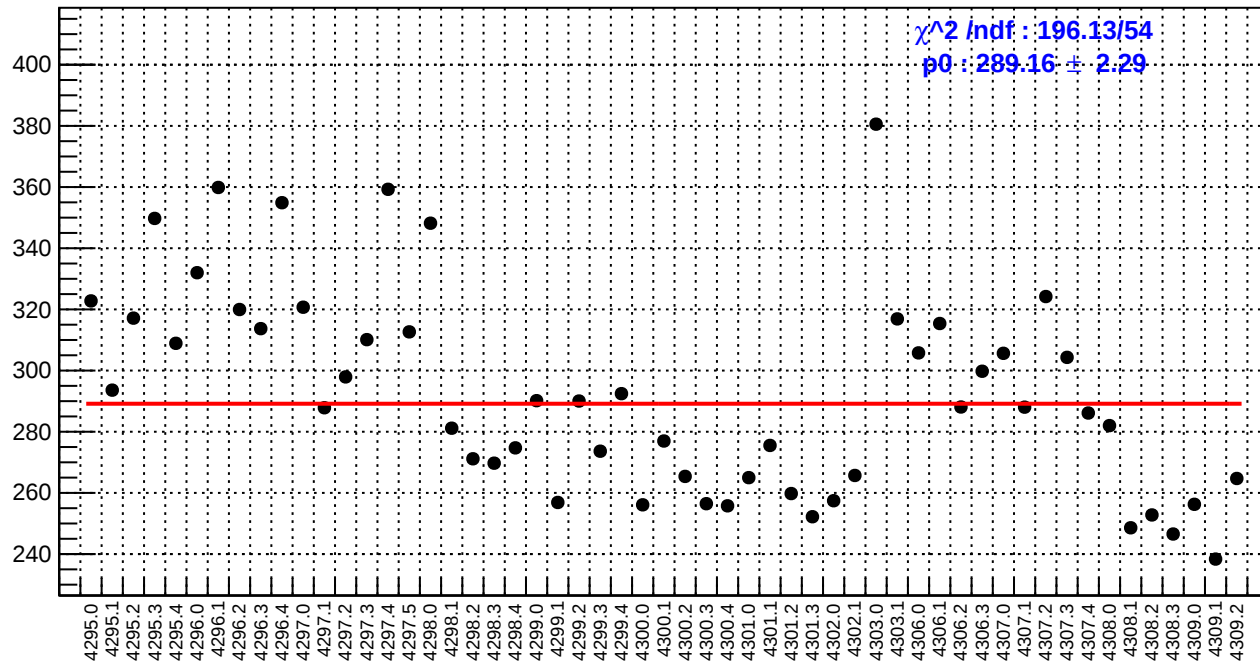
slug54: reg_asym_sam7.rms/ppm
