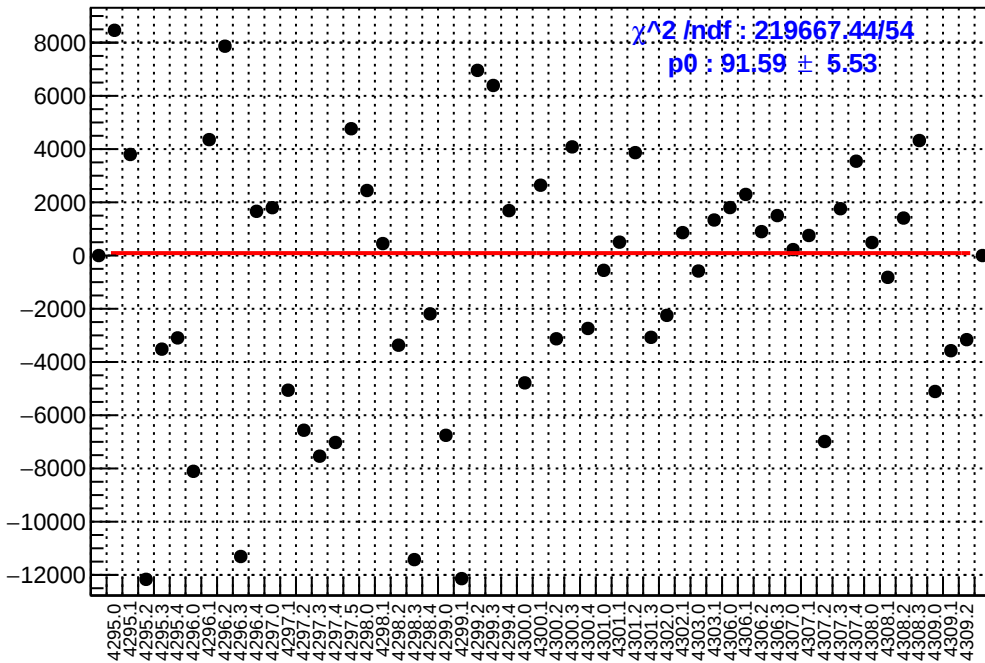
slug54: asym_dsr.mean/ppb-reg_asym_dsr.mean/ppb
