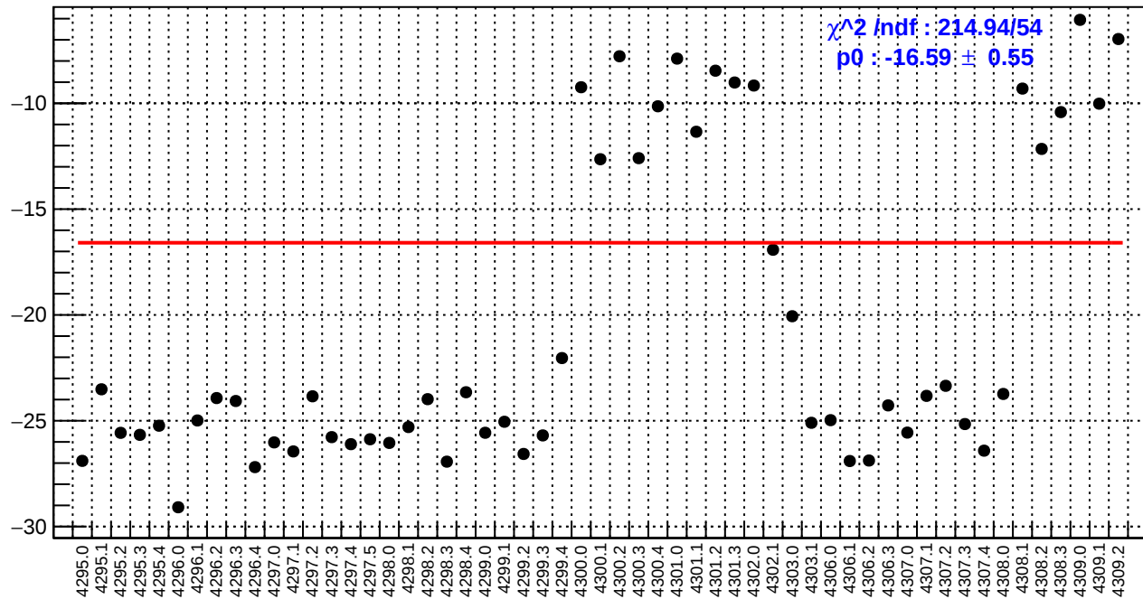
slug54: us_avg_bpm4aX/(ppb/nm)
