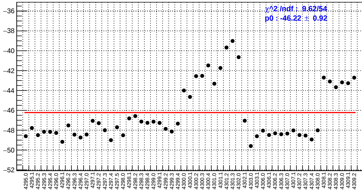
slug54: left_avg_bpm12X/(ppb/nm)
