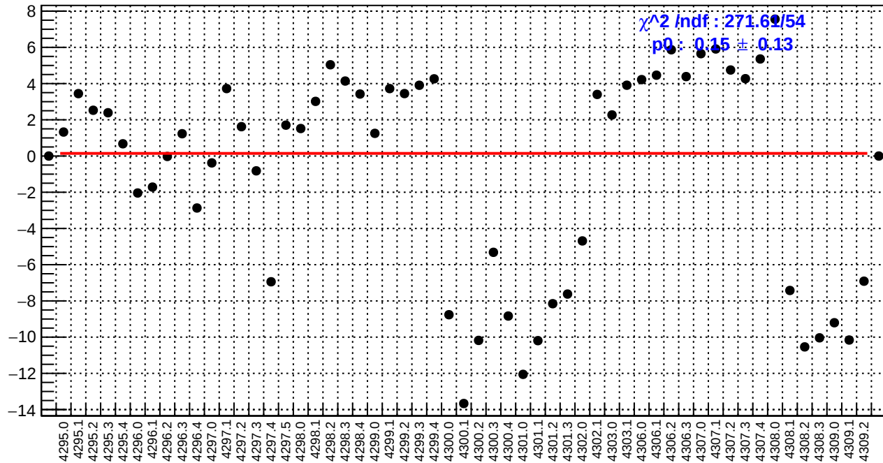
slug54: right_avg_bpm4aY/(ppb/nm)
