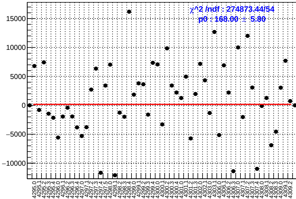
slug54: asym_left_avg.mean/ppb-reg_asym_left_avg.mean/ppb
