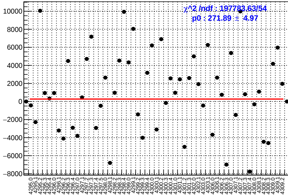
slug54: asym_us_dd.mean/ppb-reg_asym_us_dd.mean/ppb
