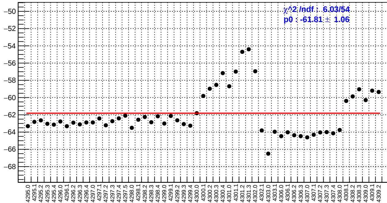
slug54: right_avg_bpm12X/(ppb/nm)
