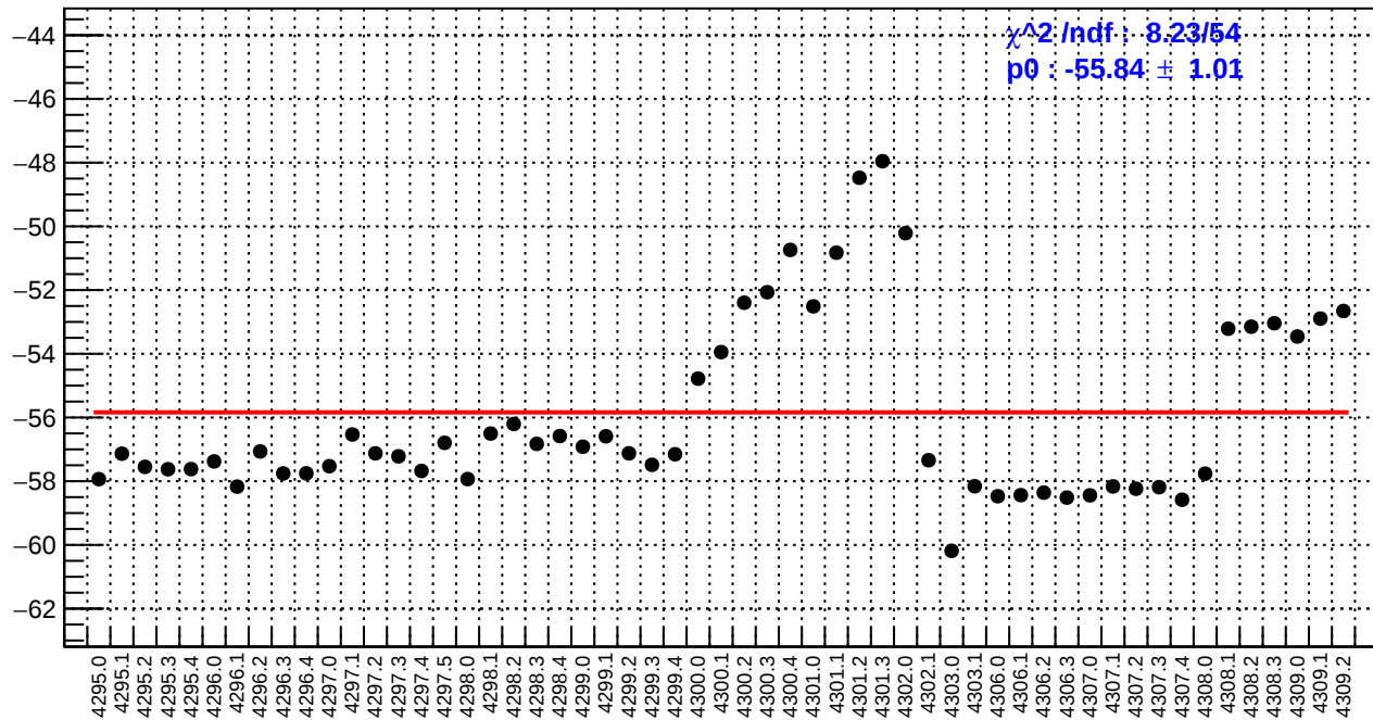
slug54: ds_avg_bpm12X/(ppb/nm)
