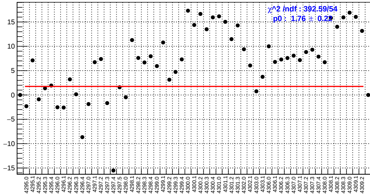
slug54: us_avg_bpm4eY/(ppb/nm)
