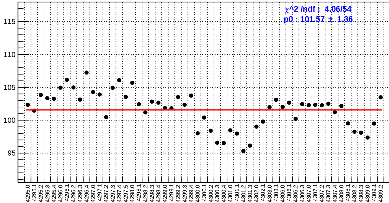
slug54: reg_asym_us_avg.rms/ppm
