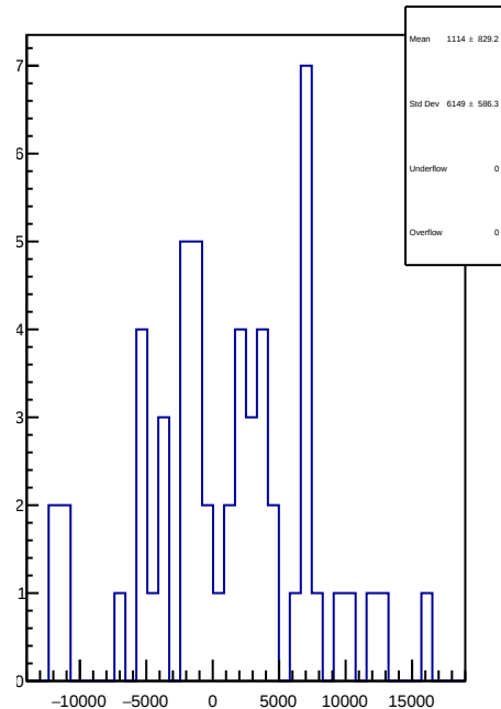
slug54: 1D Corr asym_left_avg.mean/ppb-reg_asym_left_avg.mean/ppb
