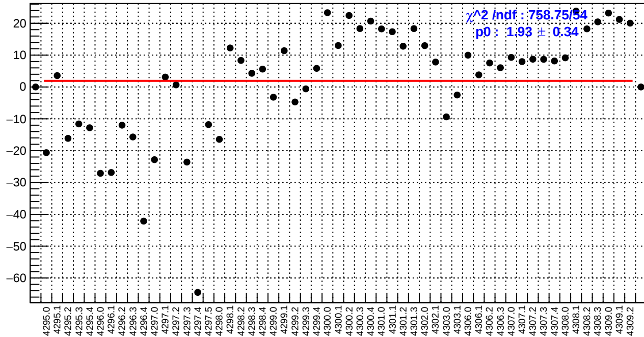
slug54: usl_bpm4eY/(ppb/nm)
