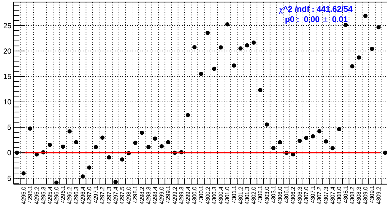
slug54: left_avg_bpm4aX/(ppb/nm)
