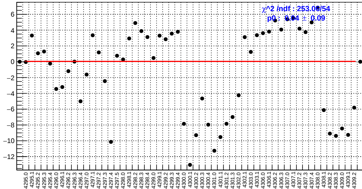
slug54: usr_bpm4aY/(ppb/nm)
