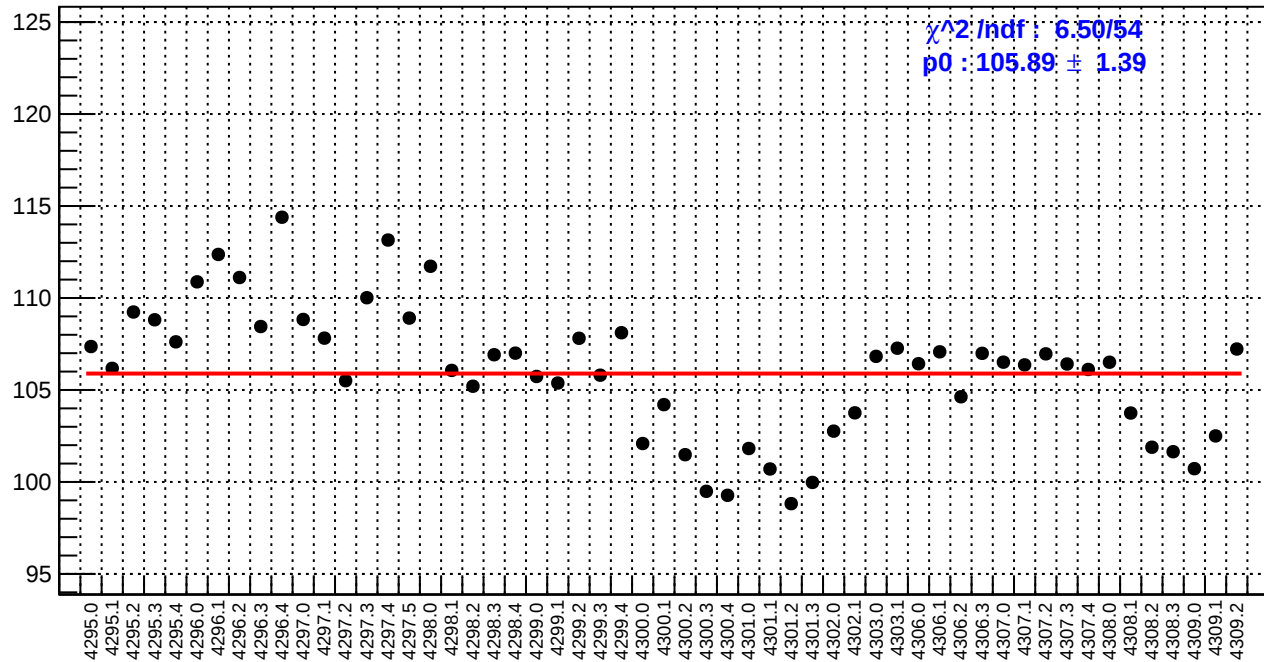
slug54: reg_asym_ds_avg.rms/ppm
