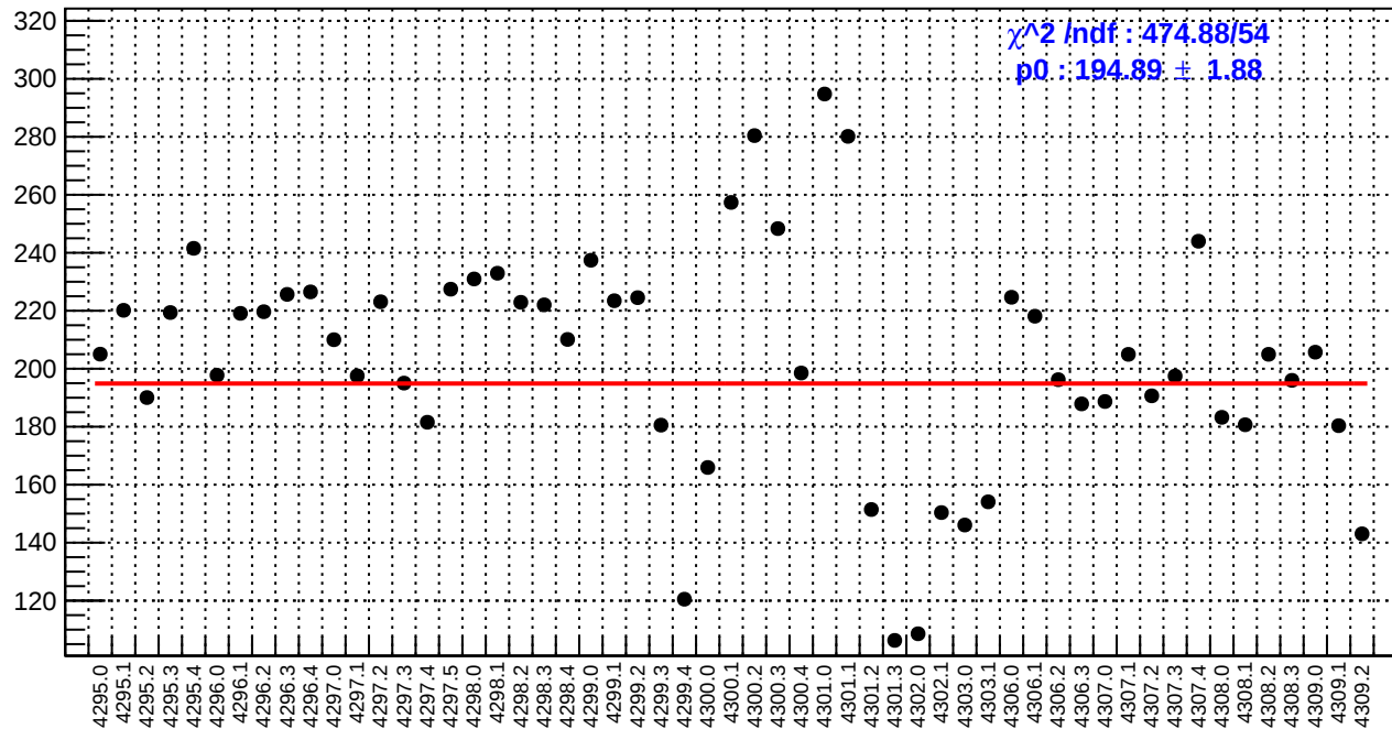
slug54: asym_bcm_an_ds3.rms/ppm
