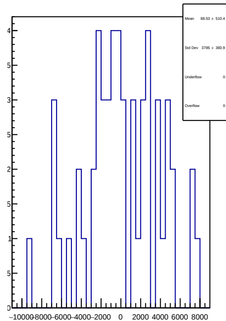
slug54: 1D Corr asym_ds_avg.mean/ppb-reg_asym_ds_avg.mean/ppb
