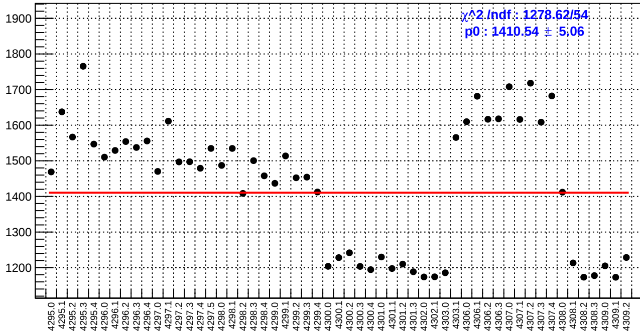
slug54: diff_bpm4aX.rms/nm
