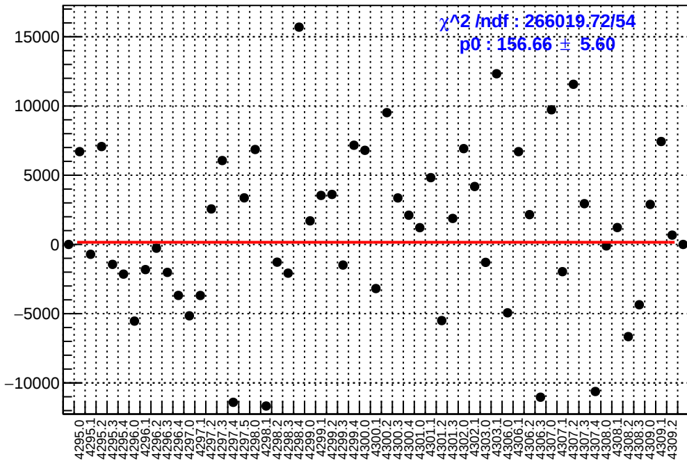
slug54: asym_usl.mean/ppb-reg_asym_usl.mean/ppb
