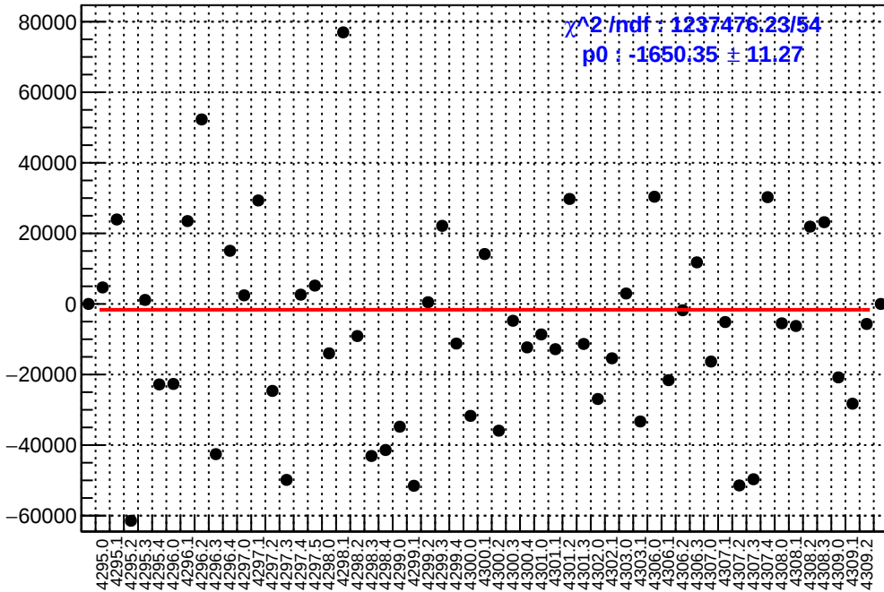
slug54: asym_sam6.mean/ppb-reg_asym_sam6.mean/ppb
