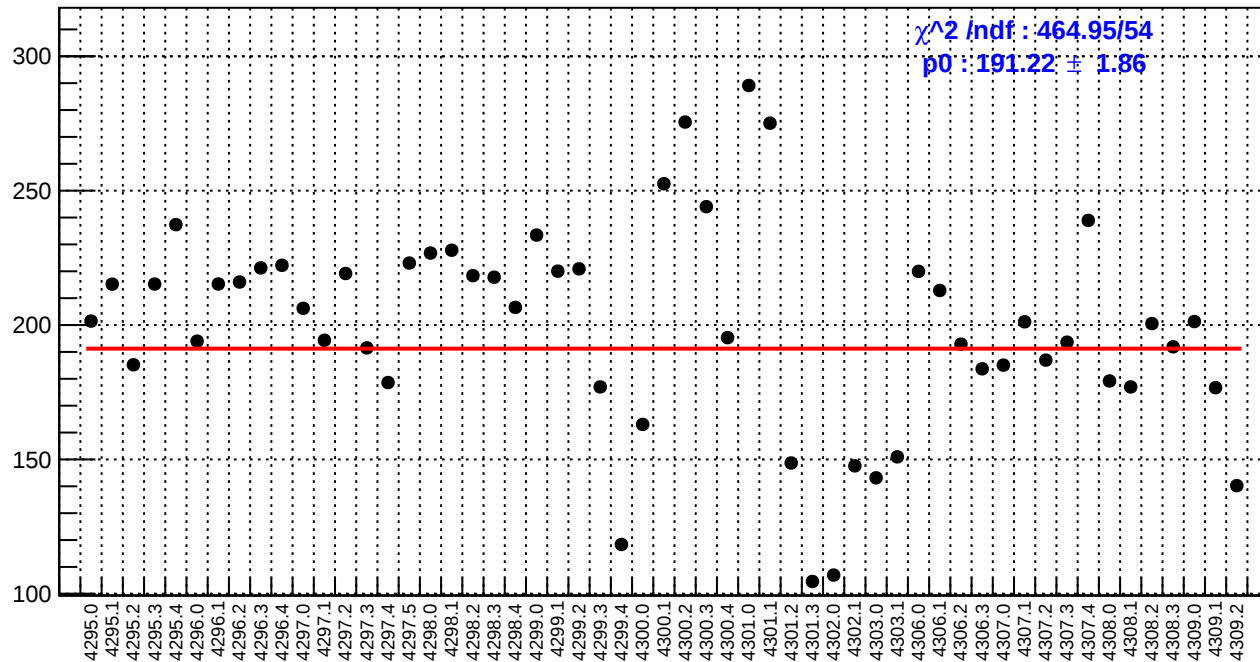
slug54: asym_bcm_an_us.rms/ppm
