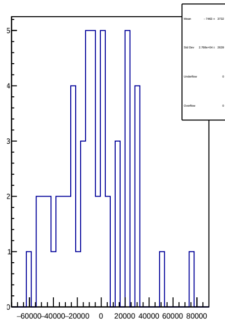
slug54: 1D Corr asym_sam6.mean/ppb-reg_asym_sam6.mean/ppb
