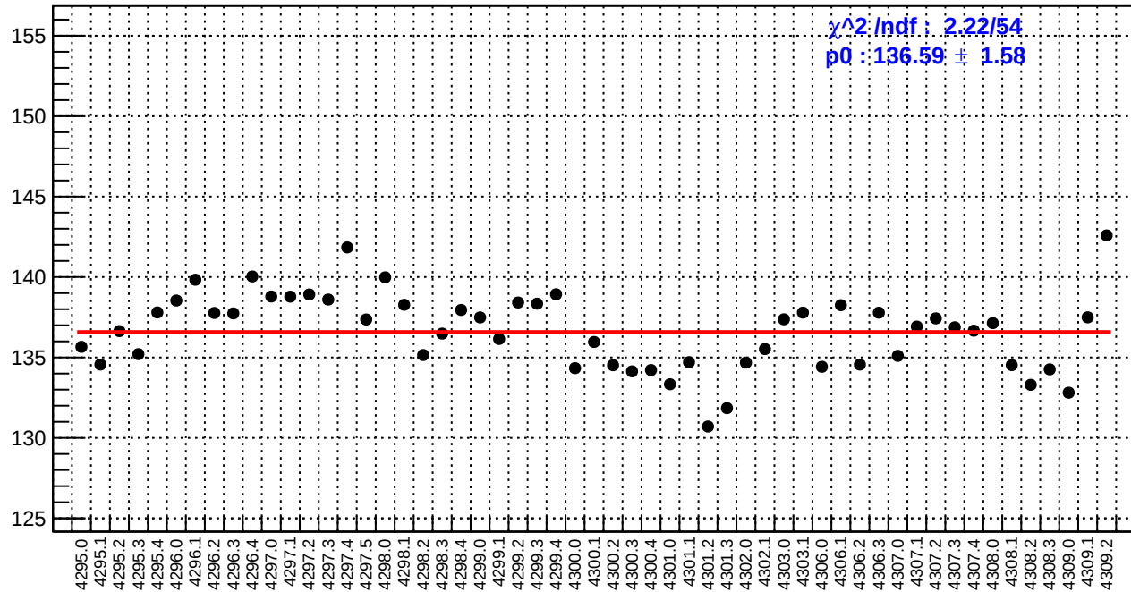
slug54: reg_asym_usr.rms/ppm
