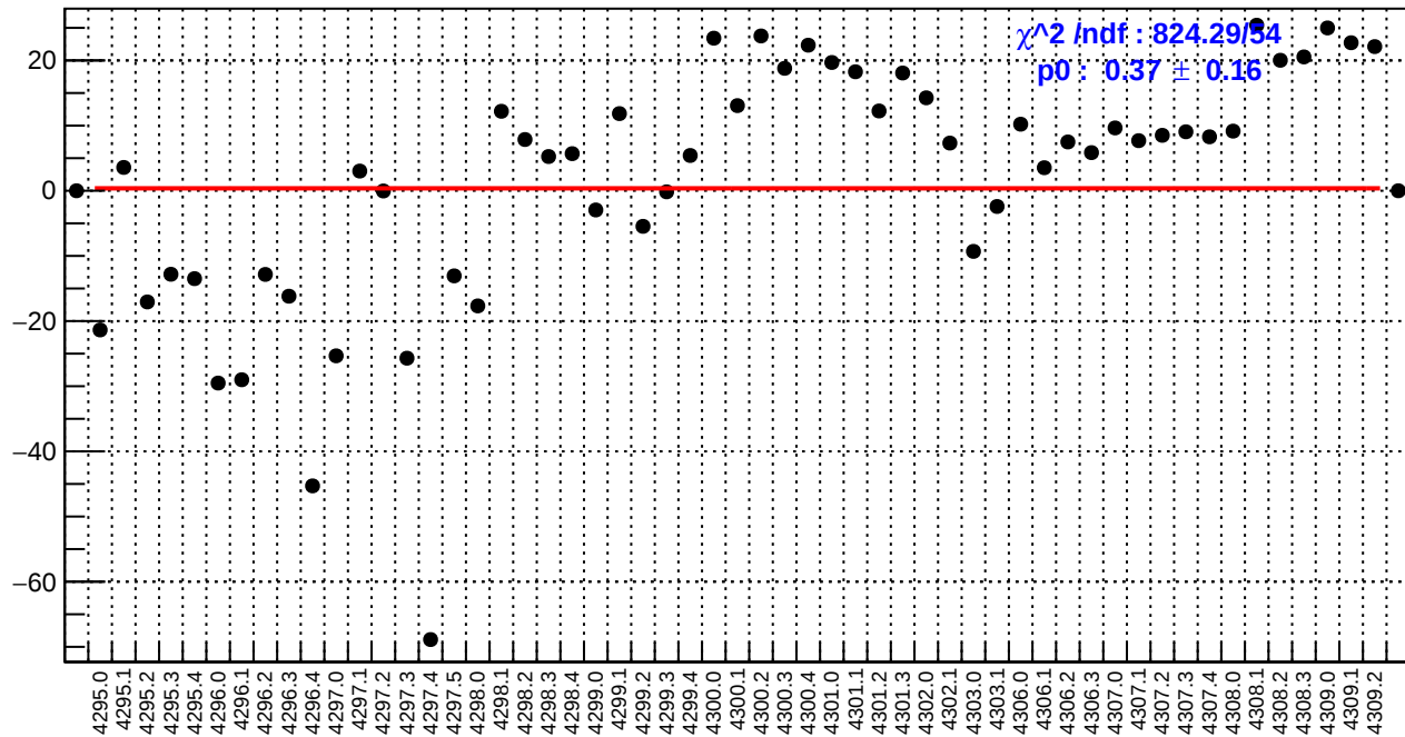
slug54: dsl_bpm4eY/(ppb/nm)
