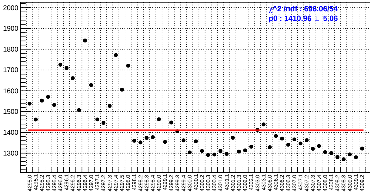
slug54: reg_asym_sam4.rms/ppm
