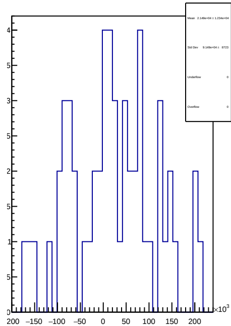
slug54: 1D Corr asym_sam3.mean/ppb-reg_asym_sam3.mean/ppb
