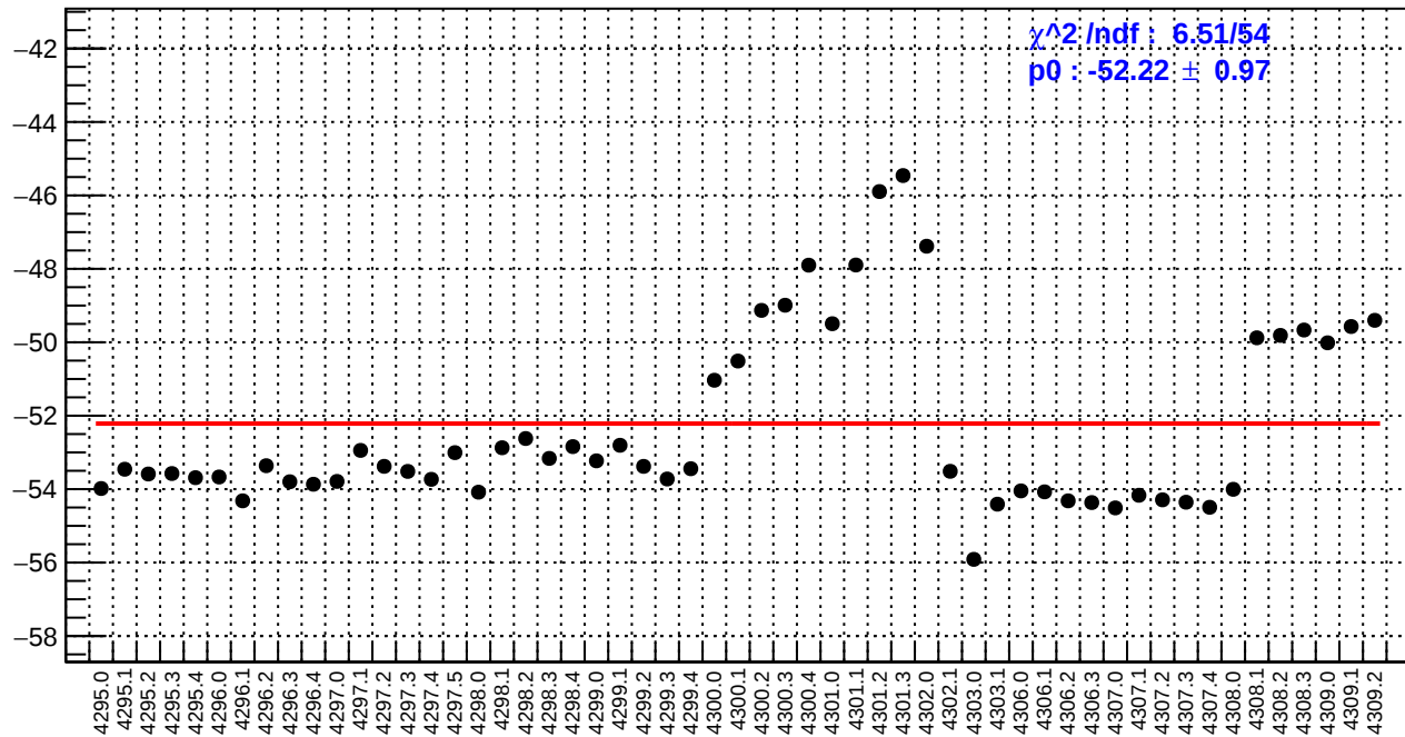
slug54: us_avg_bpm12X/(ppb/nm)
