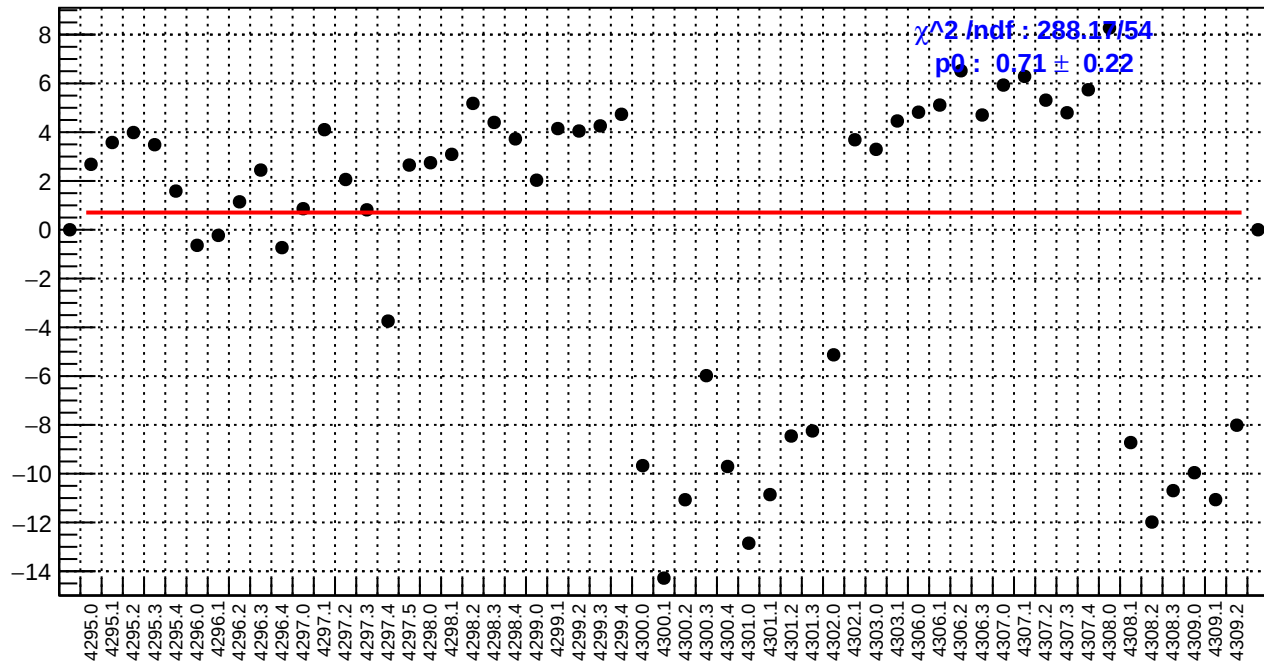
slug54: dsr_bpm4aY/(ppb/nm)
