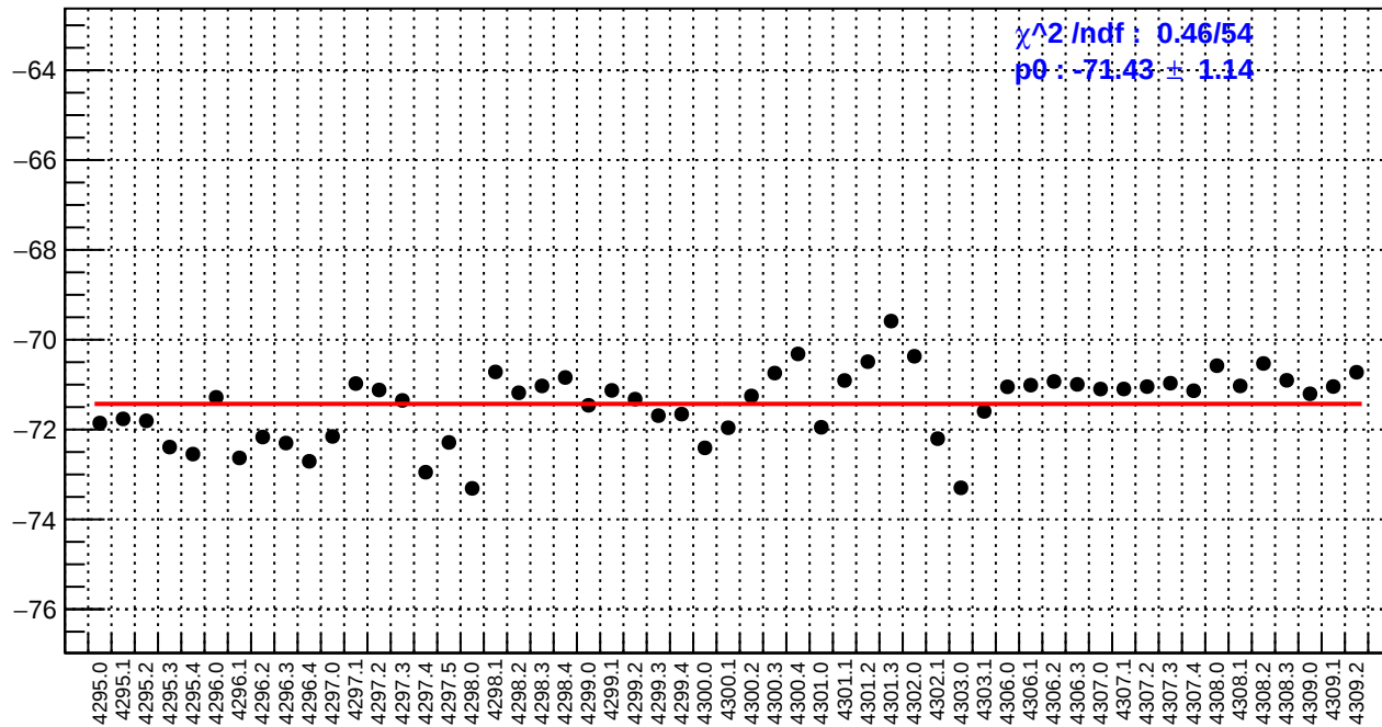
slug54: left_avg_bpm4eX/(ppb/nm)
