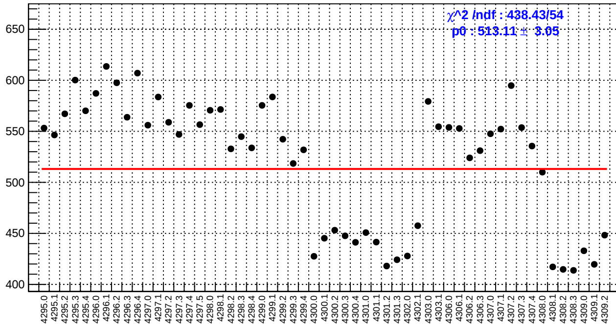
slug54: reg_asym_sam6.rms/ppm
