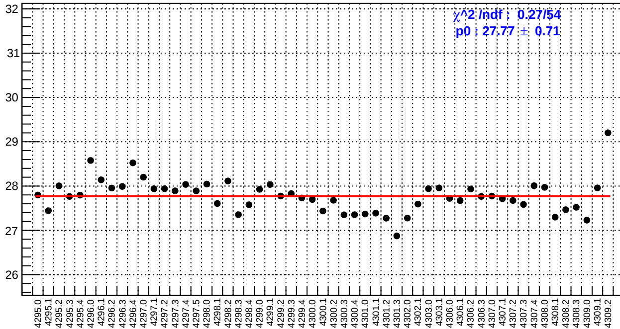
slug54: reg_asym_right_dd.rms/ppm
