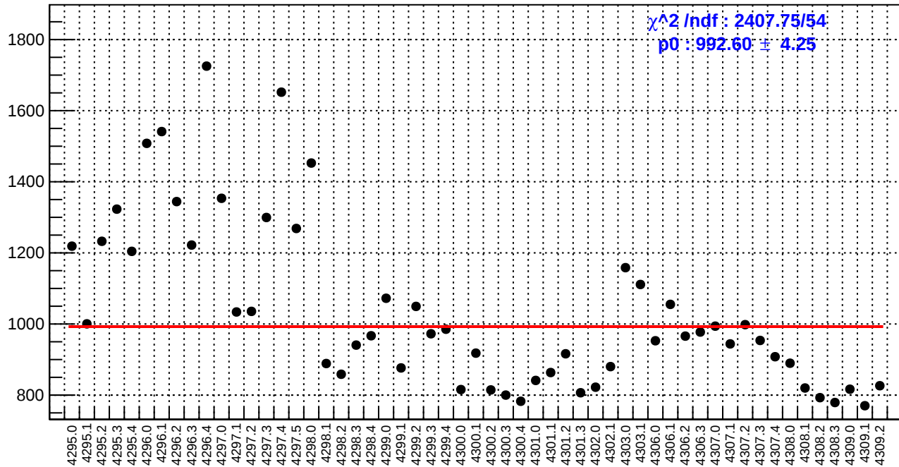
slug54: reg_asym_sam3.rms/ppm
