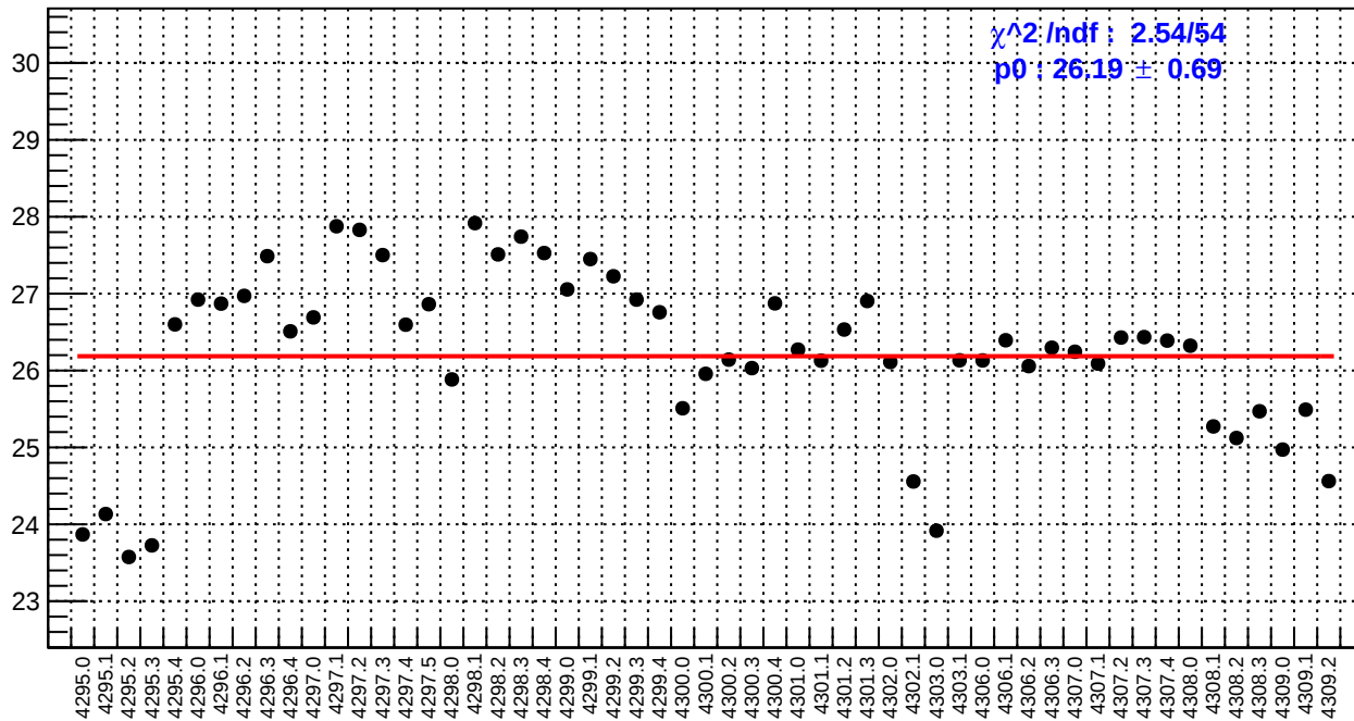
slug54: right_avg_bpm4eX/(ppb/nm)
