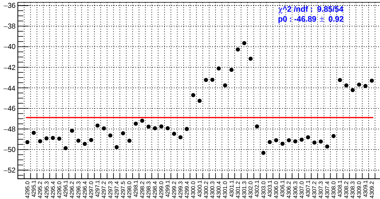
slug54: dsl_bpm12X/(ppb/nm)
