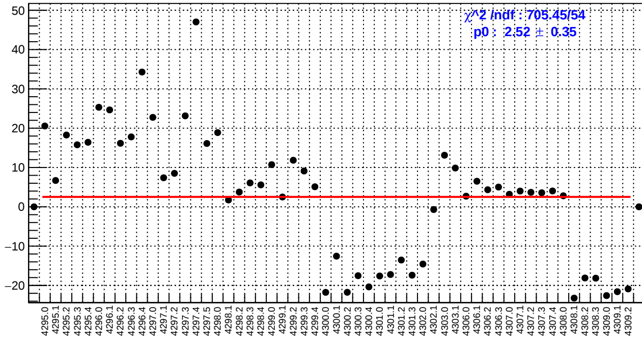
slug54: left_avg_bpm4aY/(ppb/nm)
