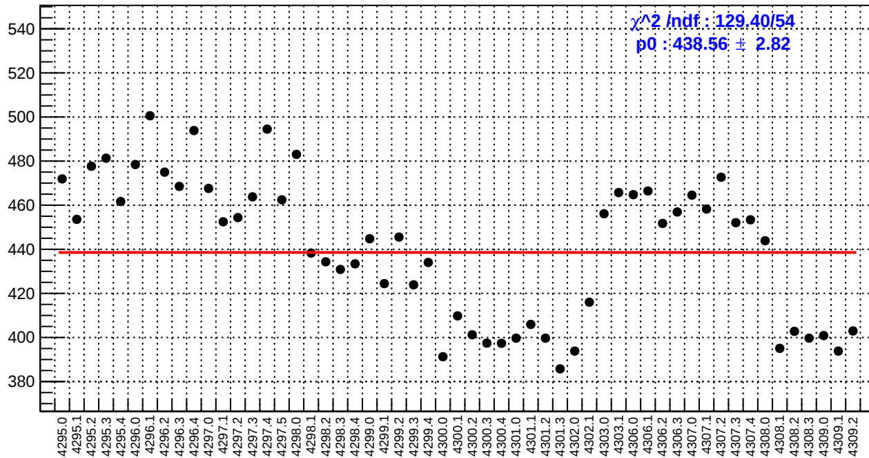
slug54: reg_asym_sam8.rms/ppm
