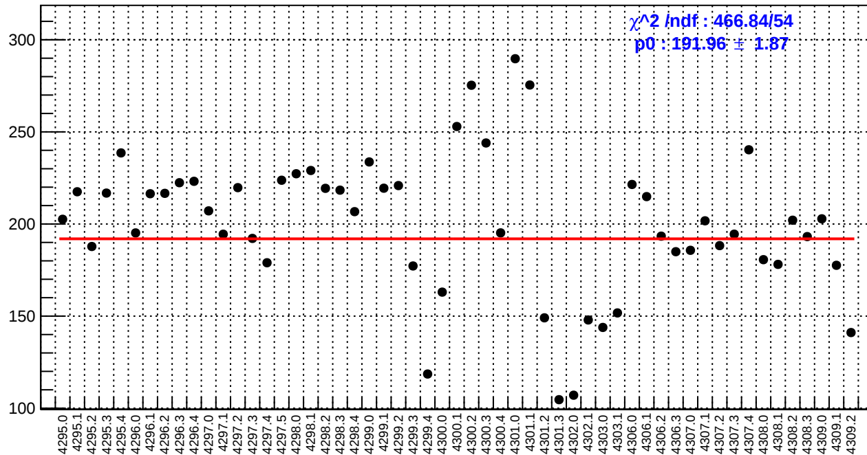
slug54: asym_bcm_an_ds.rms/ppm
