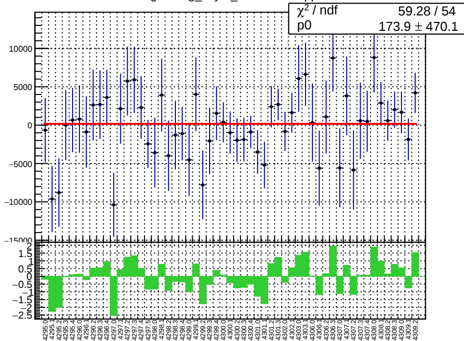
slug54: reg_asym_sam1.mean/ppb
