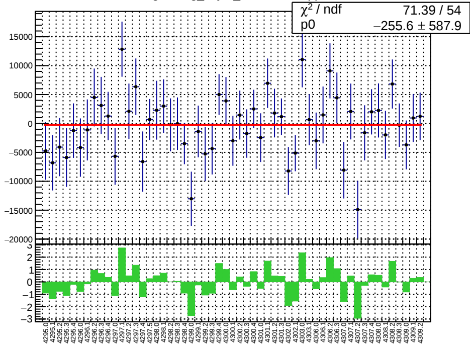
slug54: reg_asym_sam8.mean/ppb
