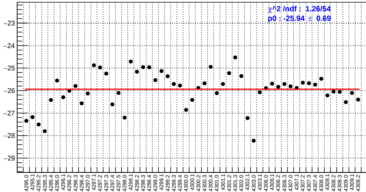
slug54: ds_avg_bpm4eX/(ppb/nm)
