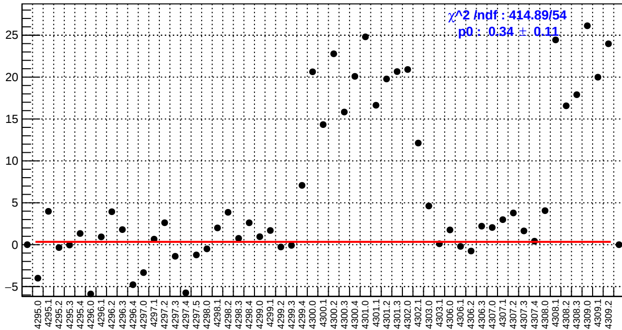
slug54: usl_bpm4aX/(ppb/nm)
