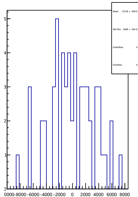
slug54: 1D Corr asym_us_avg.mean/ppb-reg_asym_us_avg.mean/ppb
