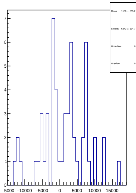
slug54: 1D Corr asym_dsl.mean/ppb-reg_asym_dsl.mean/ppb
