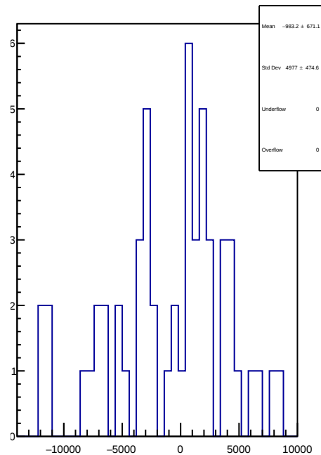
slug54: 1D Corr asym_dsr.mean/ppb-reg_asym_dsr.mean/ppb
