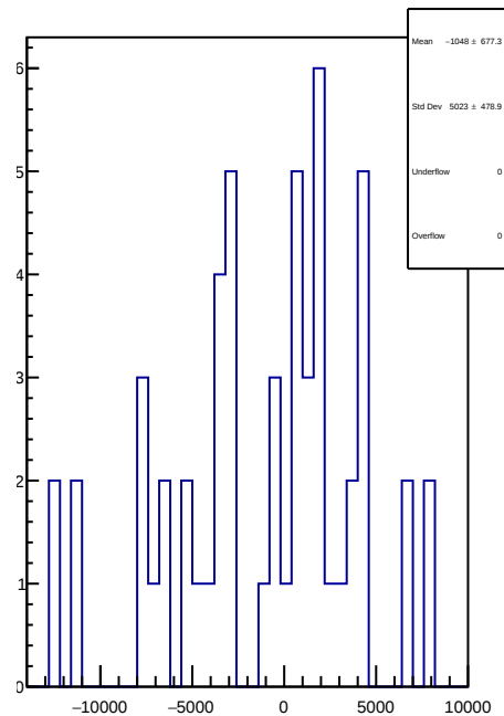
slug54: 1D Corr asym_right_avg.mean/ppb-reg_asym_right_avg.mean/ppb
