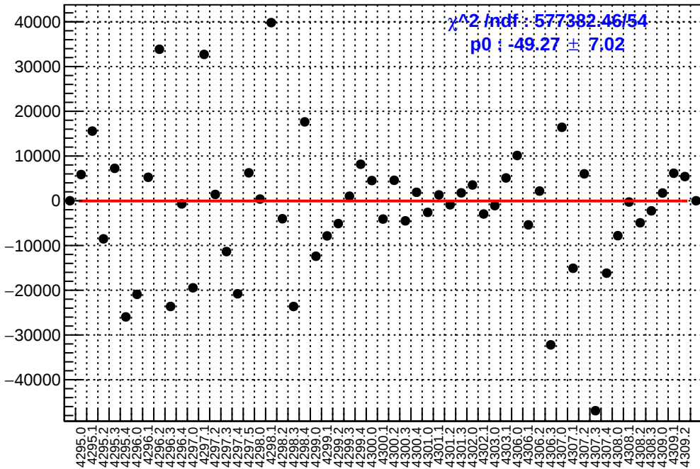
slug54: asym_sam5.mean/ppb-reg_asym_sam5.mean/ppb
