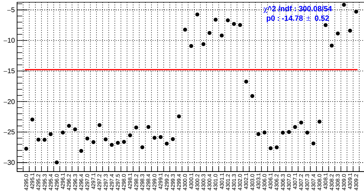
slug54: ds_avg_bpm4aX/(ppb/nm)
