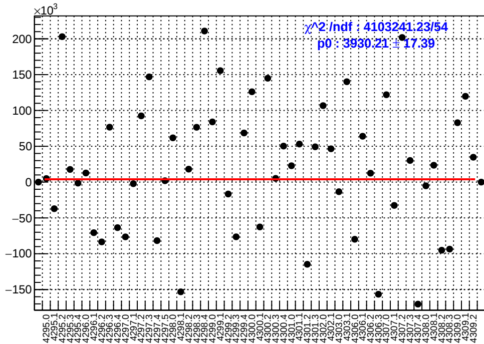
slug54: asym_sam3.mean/ppb-reg_asym_sam3.mean/ppb
