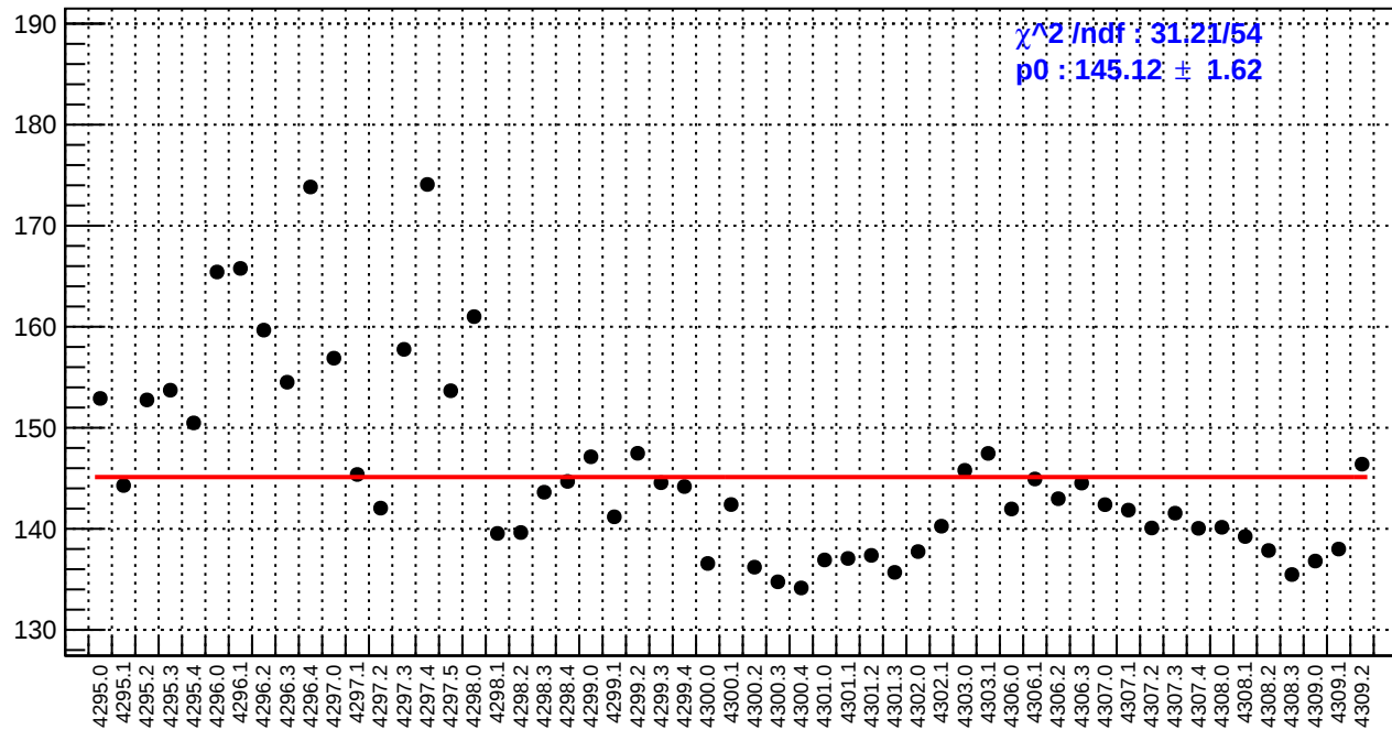
slug54: reg_asym_left_avg.rms/ppm
