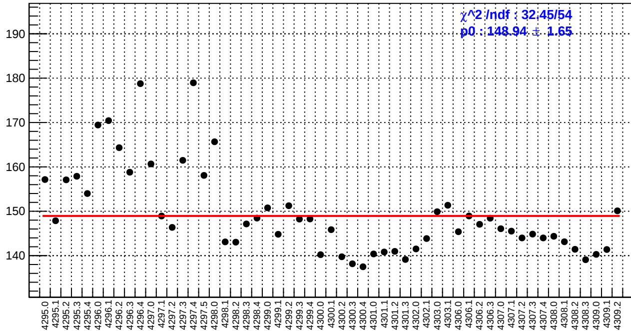
slug54: reg_asym_dsl.rms/ppm
