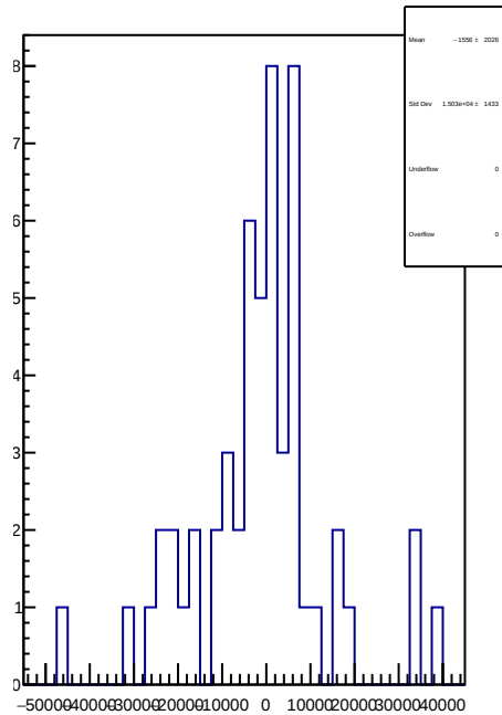
slug54: 1D Corr asym_sam5.mean/ppb-reg_asym_sam5.mean/ppb
