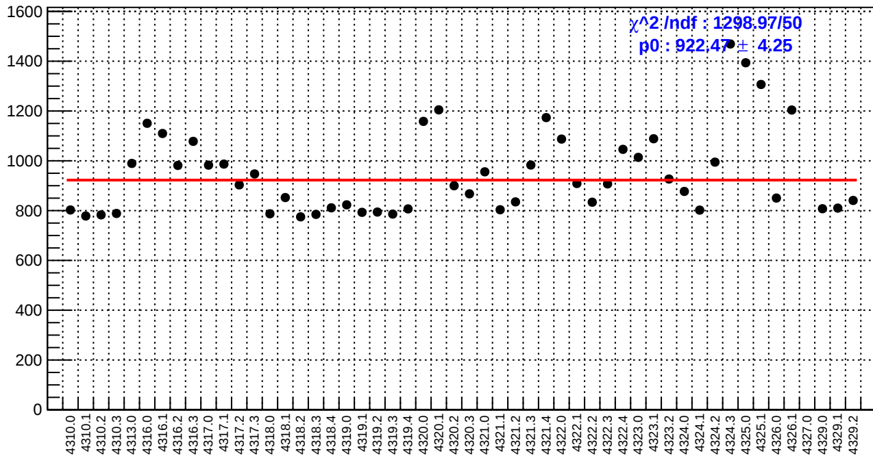
slug55: reg_asym_sam3.rms/ppm
