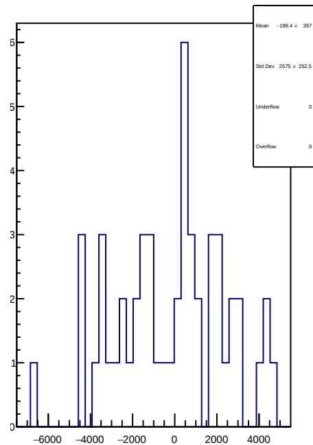
slug55: 1D Corr asym_us_avg.mean/ppb-reg_asym_us_avg.mean/ppb
