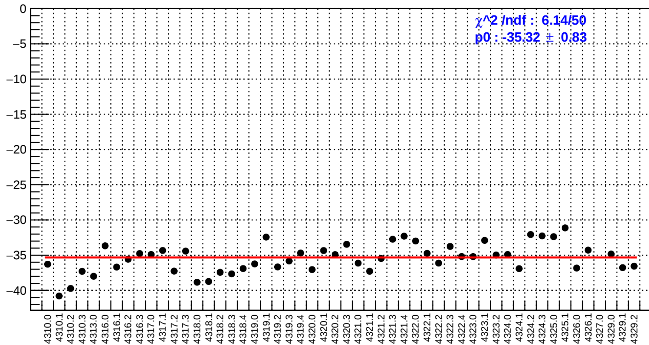
slug55: right_avg_bpm4aX/(ppb/nm)
