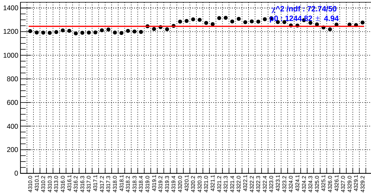
slug55: diff_bpm4aX.rms/nm
