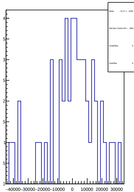
slug55: 1D Corr asym_sam7.mean/ppb-reg_asym_sam7.mean/ppb
