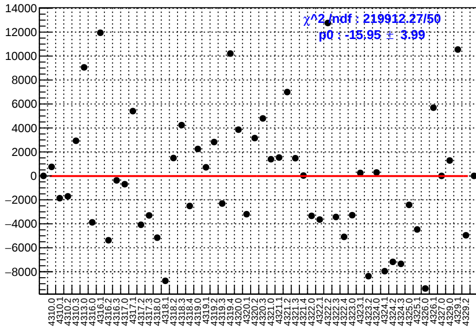
slug55: asym_dsl.mean/ppb-reg_asym_dsl.mean/ppb
