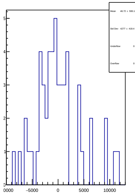
slug55: 1D Corr asym_us_dd.mean/ppb-reg_asym_us_dd.mean/ppb
