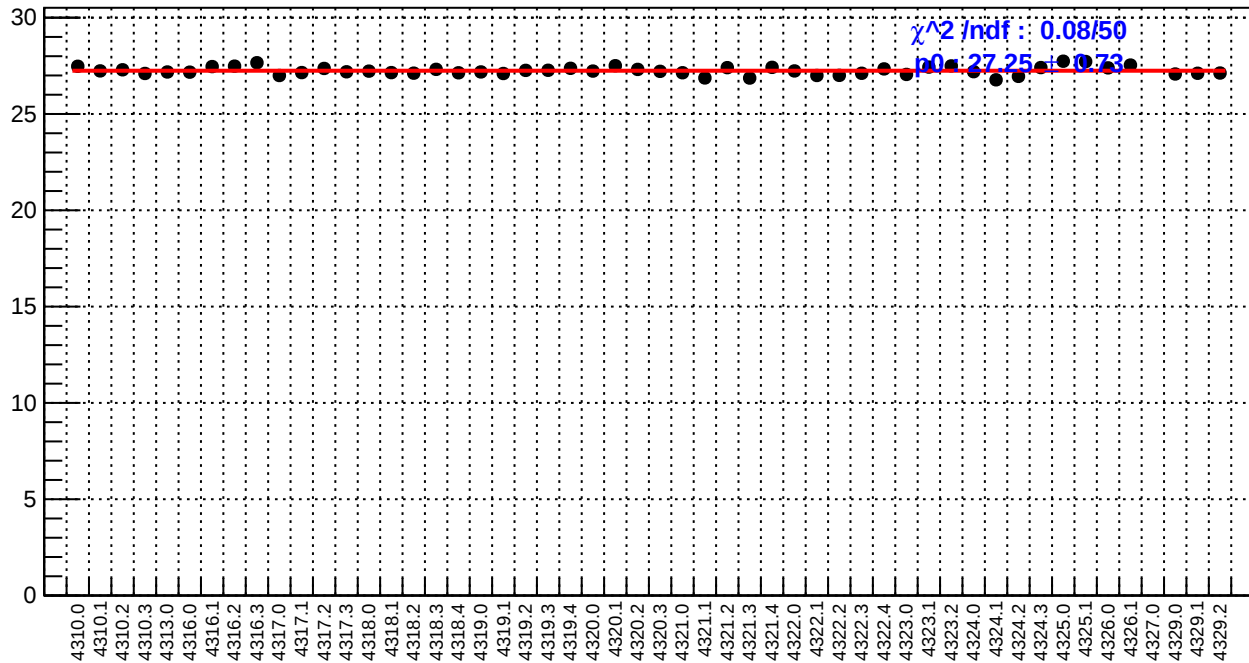
slug55: reg_asym_right_dd.rms/ppm
