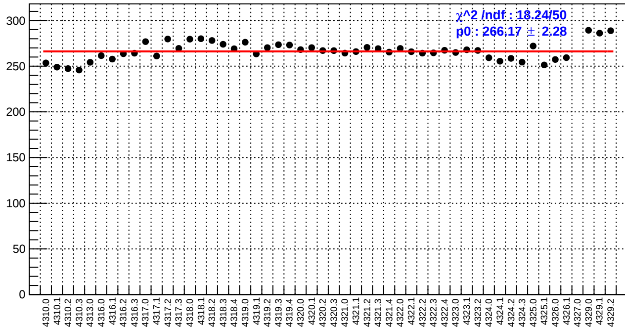
slug55: reg_asym_sam1.rms/ppm
