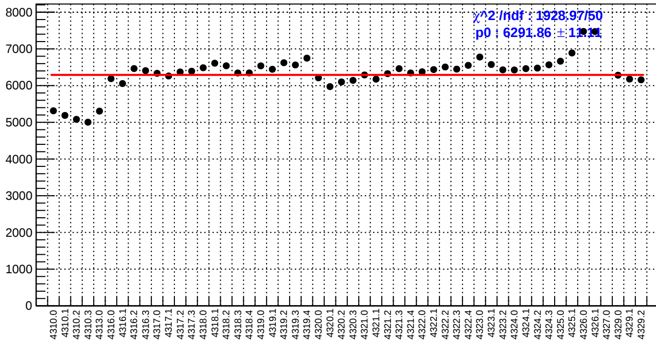
slug55: diff_bpm11X.rms/nm
