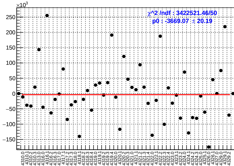
slug55: asym_sam3.mean/ppb-reg_asym_sam3.mean/ppb
