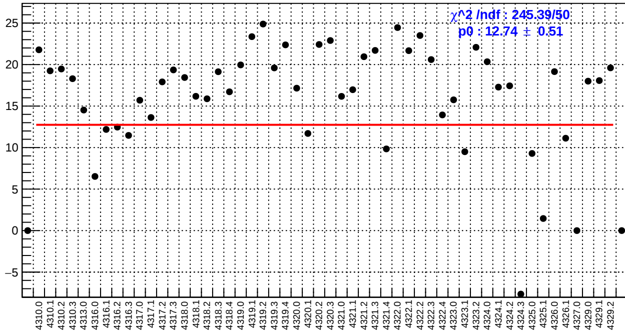
slug55: dsl_bpm4aX/(ppb/nm)
