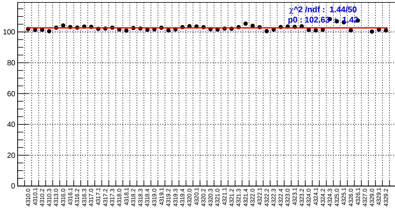
slug55: reg_asym_ds_avg.rms/ppm
