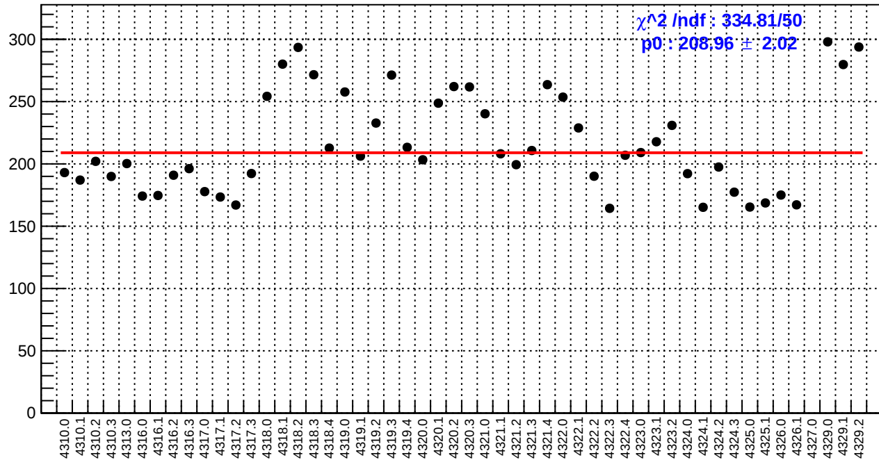
slug55: asym_bcm_an_ds3.rms/ppm
