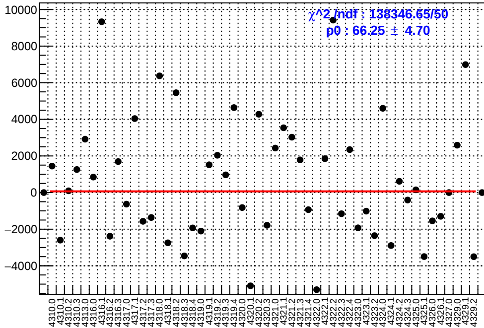
slug55: asym_sam5.mean/ppb-reg_asym_sam5.mean/ppb
