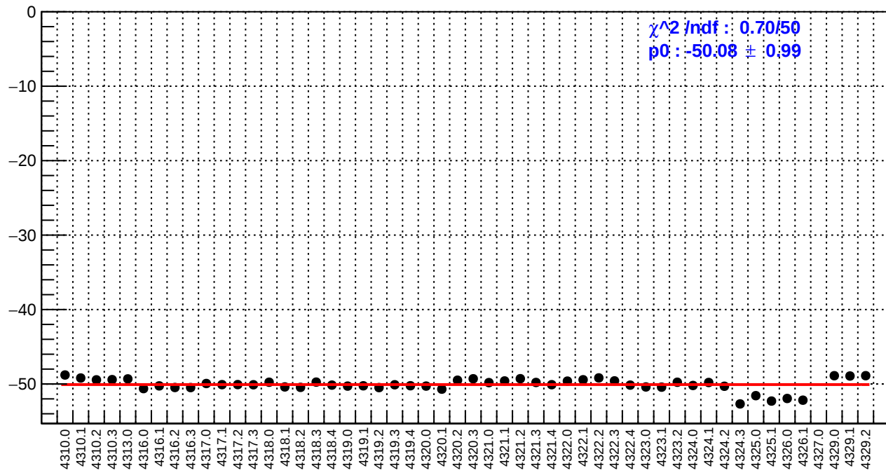
slug55: us_avg_bpm12X/(ppb/nm)
