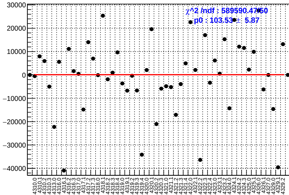
slug55: asym_sam8.mean/ppb-reg_asym_sam8.mean/ppb
