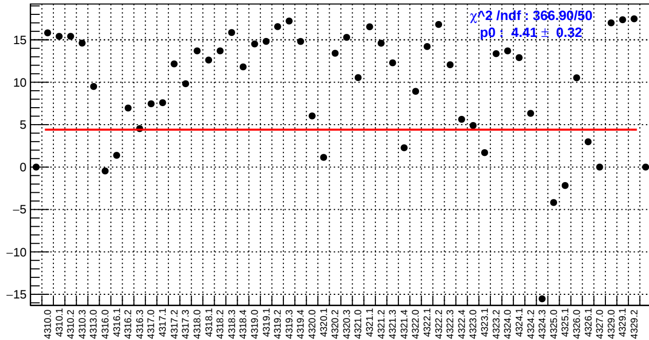
slug55: us_avg_bpm4eY/(ppb/nm)
