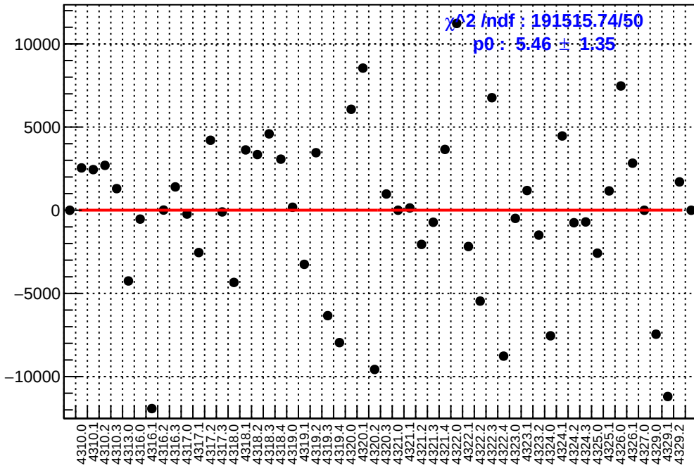
slug55: asym_right_avg.mean/ppb-reg_asym_right_avg.mean/ppb
