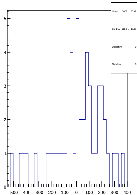
slug55: 1D Corr asym_left_dd.mean/ppb-reg_asym_left_dd.mean/ppb
