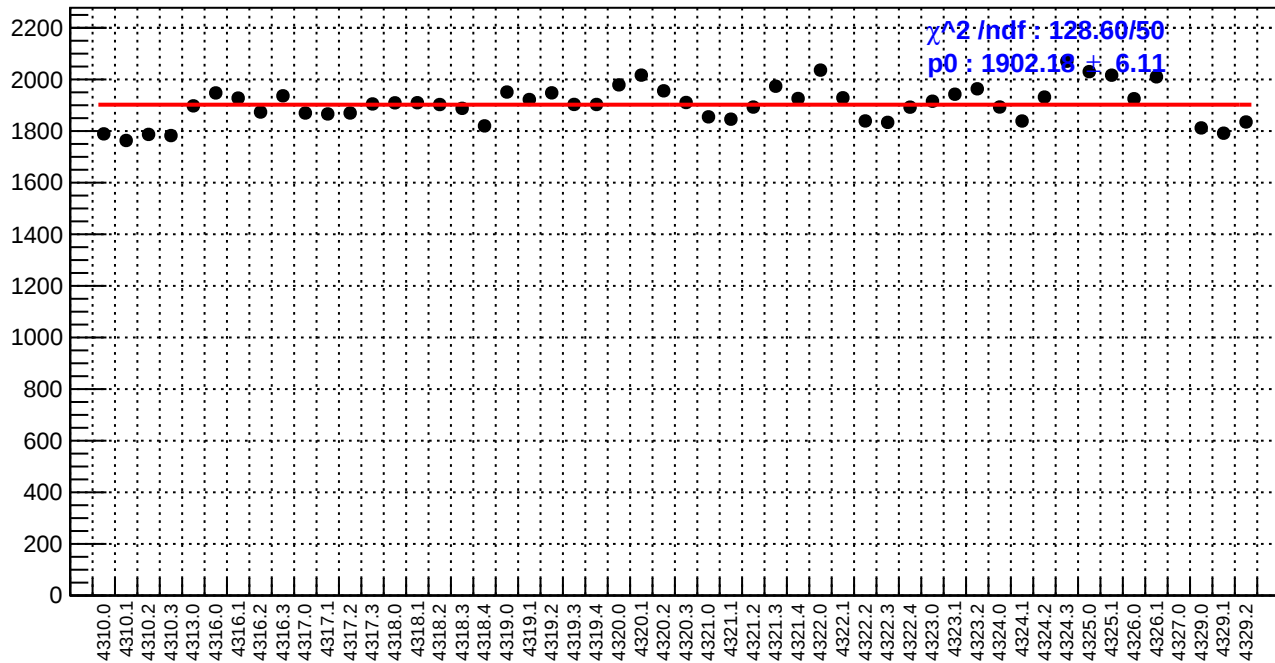
slug55: diff_bpm4eY.rms/nm
