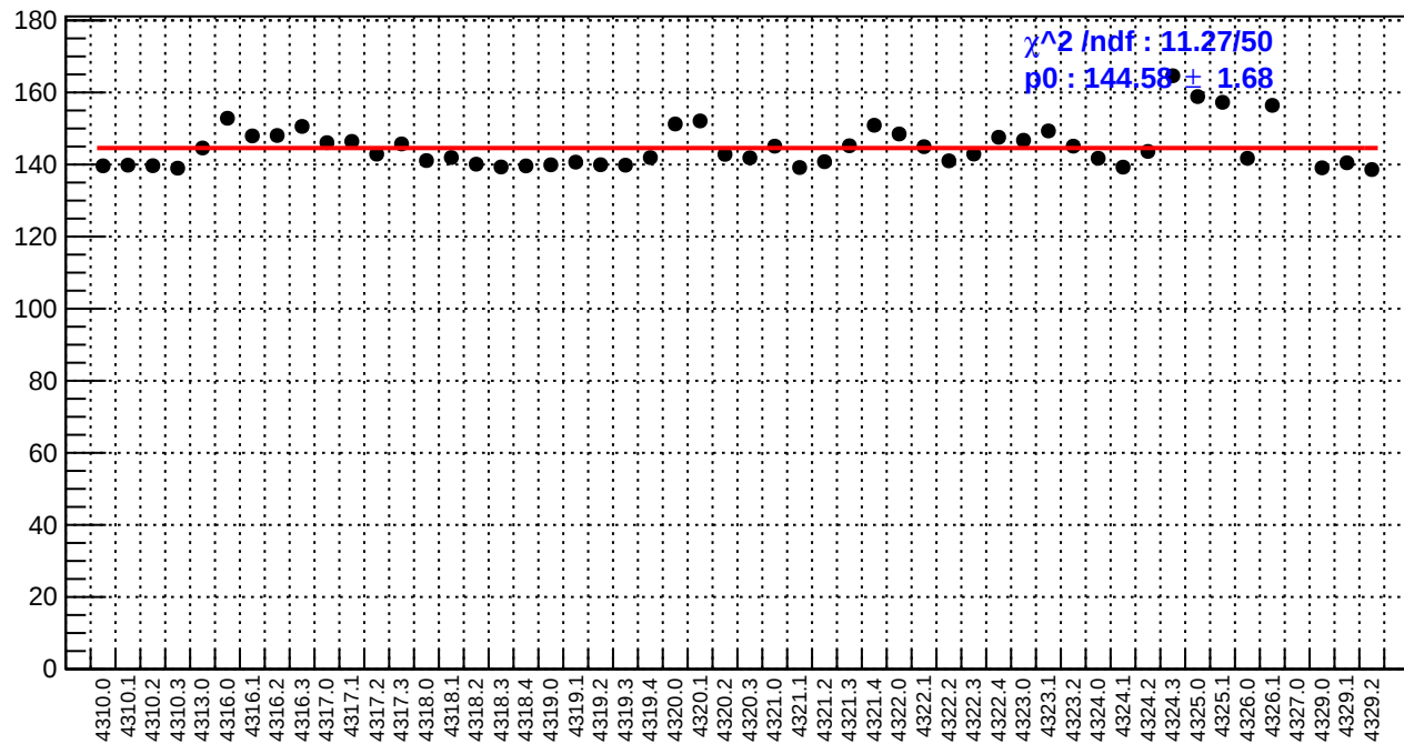
slug55: reg_asym_dsl.rms/ppm
