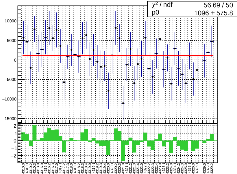
slug55: reg_asym_sam8.mean/ppb
