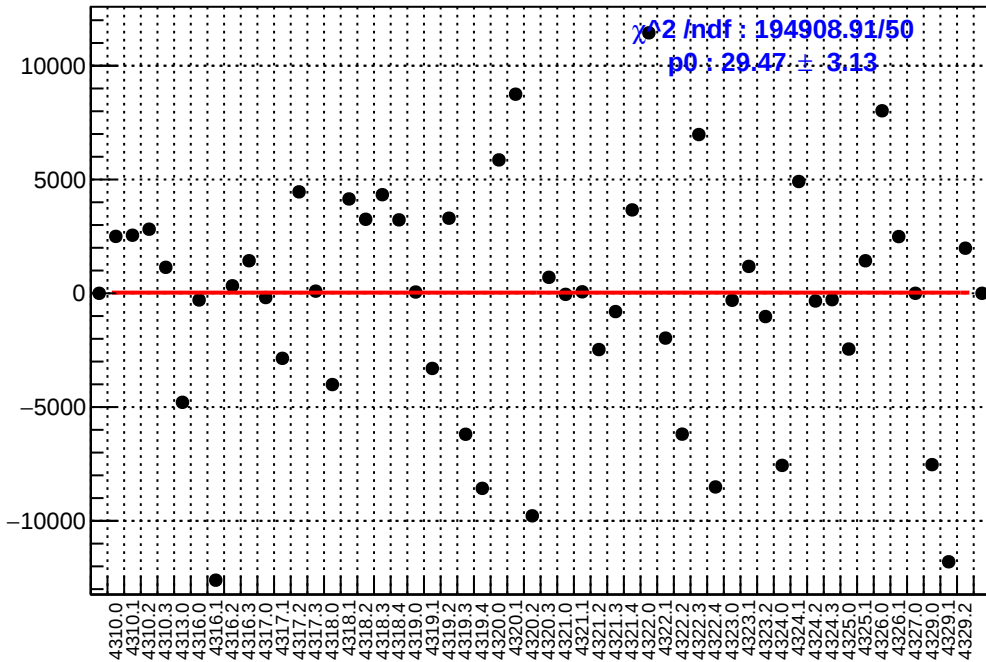
slug55: asym_usr.mean/ppb-reg_asym_usr.mean/ppb
