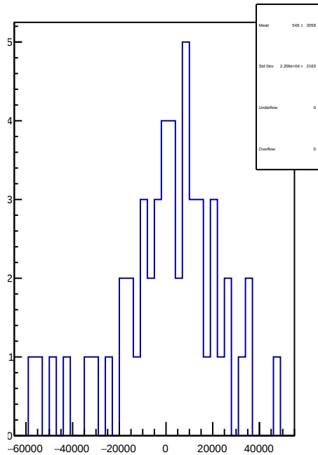
slug55: 1D Corr asym_sam6.mean/ppb-reg_asym_sam6.mean/ppb
