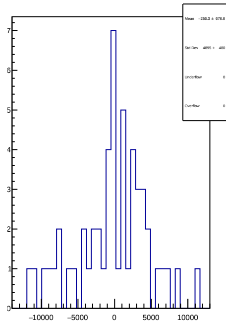
slug55: 1D Corr asym_right_avg.mean/ppb-reg_asym_right_avg.mean/ppb
