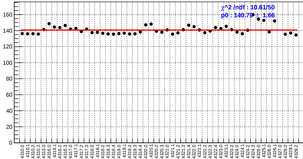
slug55: reg_asym_left_avg.rms/ppm
