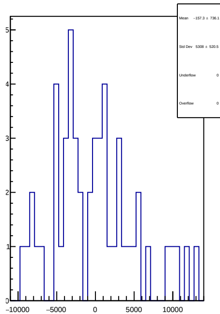
slug55: 1D Corr asym_dsl.mean/ppb-reg_asym_dsl.mean/ppb
