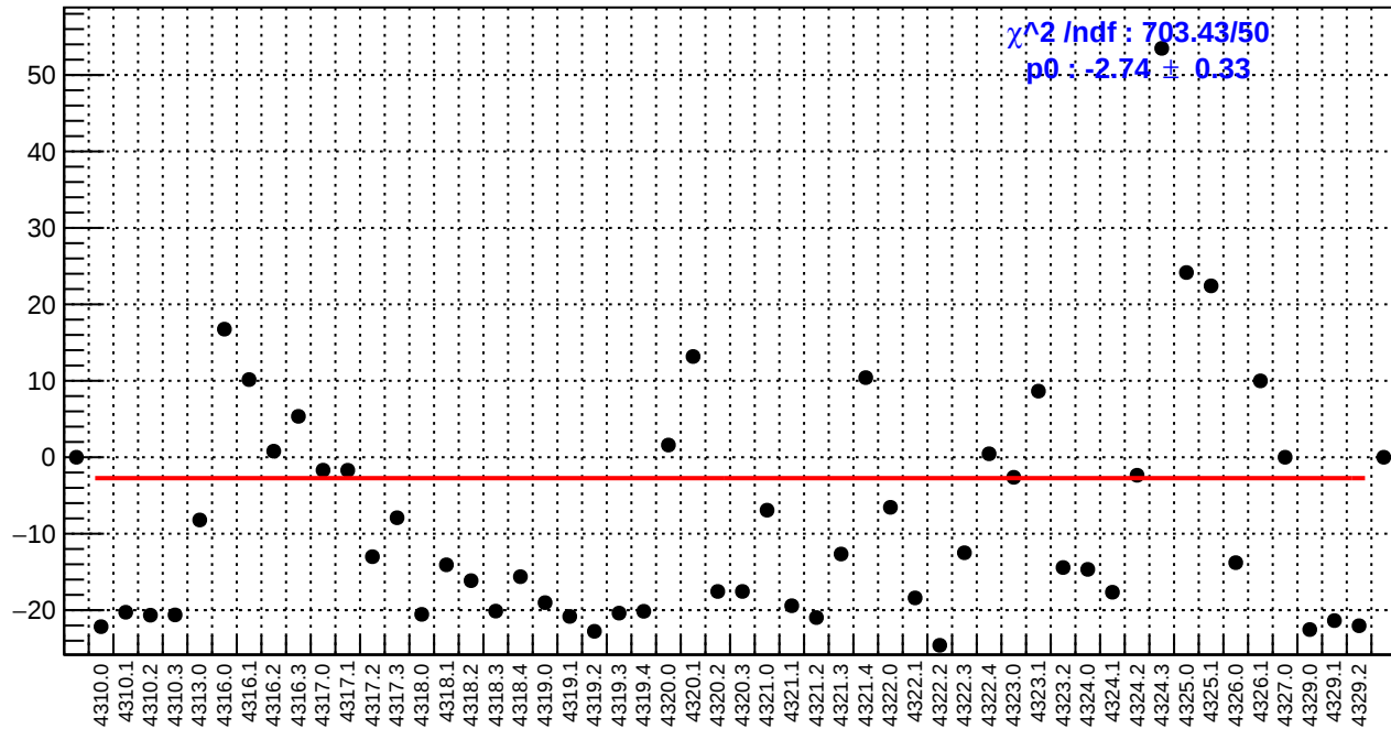
slug55: dsl_bpm4aY/(ppb/nm)
