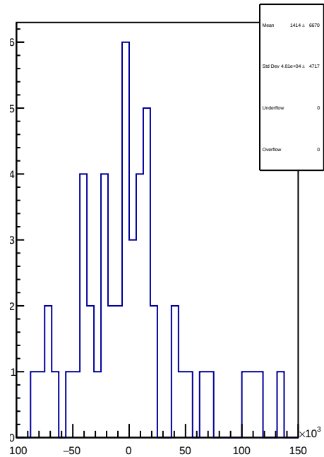
slug55: 1D Corr asym_sam4.mean/ppb-reg_asym_sam4.mean/ppb
