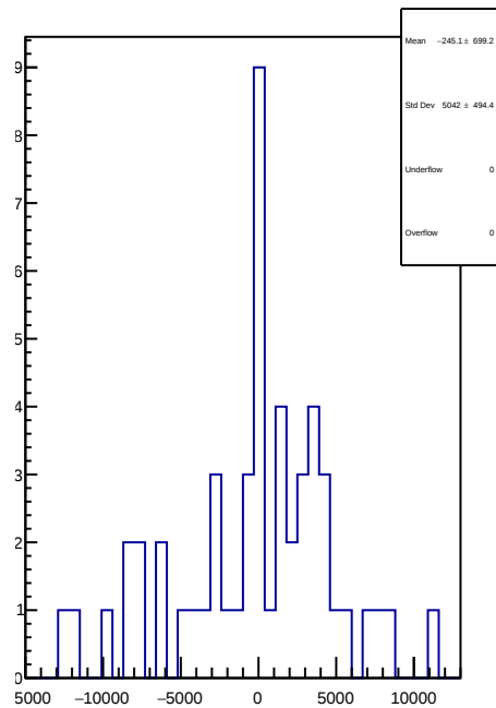
slug55: 1D Corr asym_usr.mean/ppb-reg_asym_usr.mean/ppb
