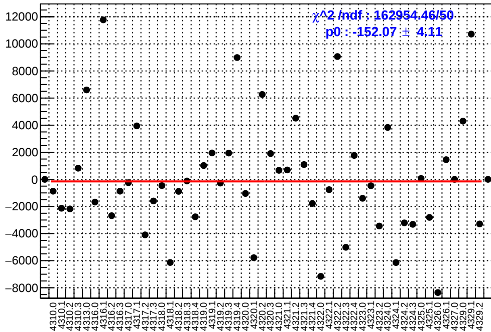
slug55: asym_us_dd.mean/ppb-reg_asym_us_dd.mean/ppb
