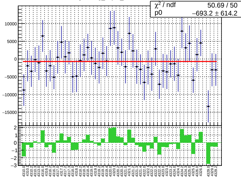
slug55: reg_asym_sam6.mean/ppb
