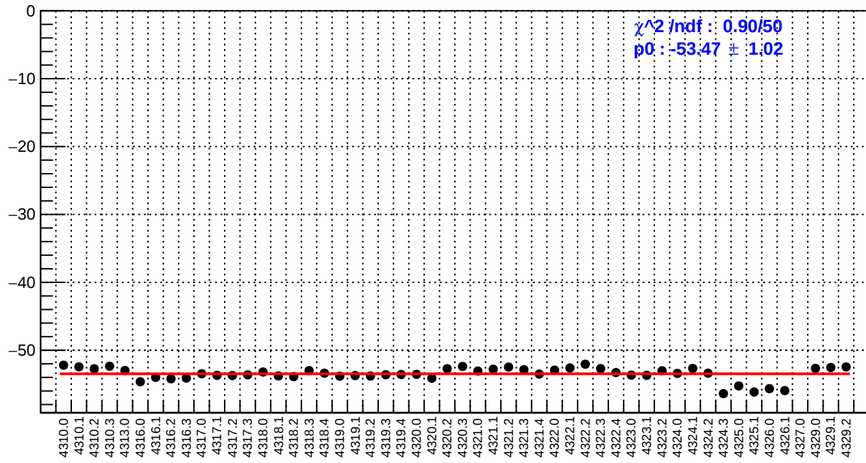
slug55: ds_avg_bpm12X/(ppb/nm)
