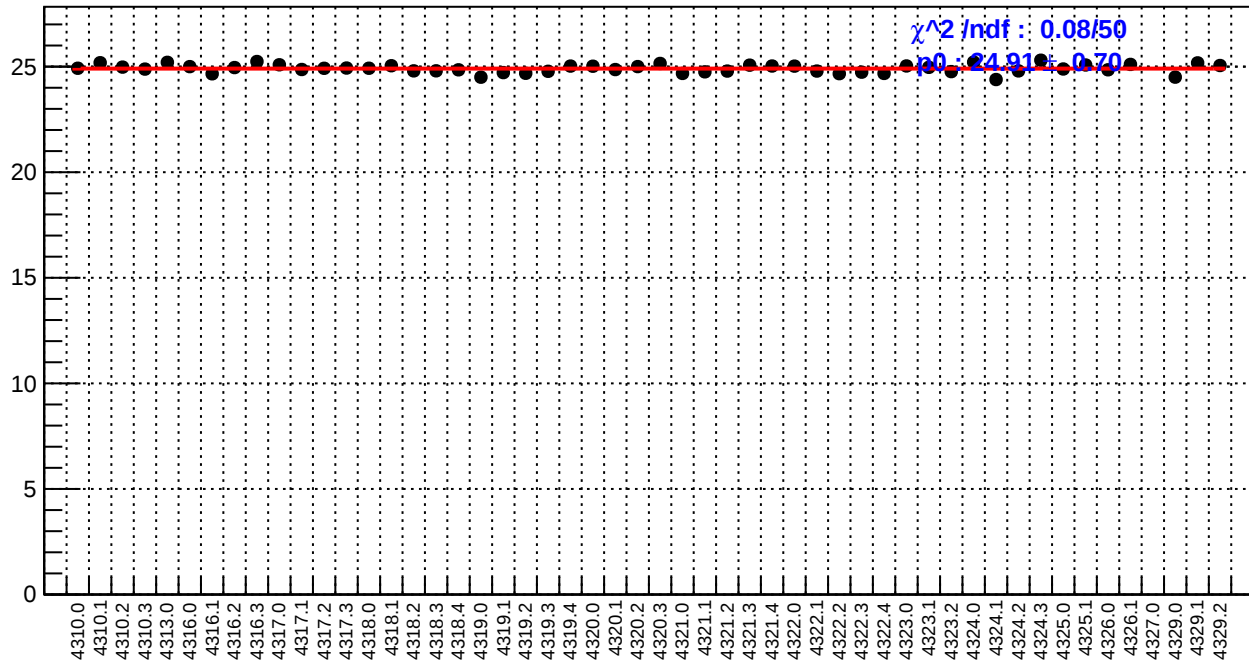
slug55: reg_asym_left_dd.rms/ppm
