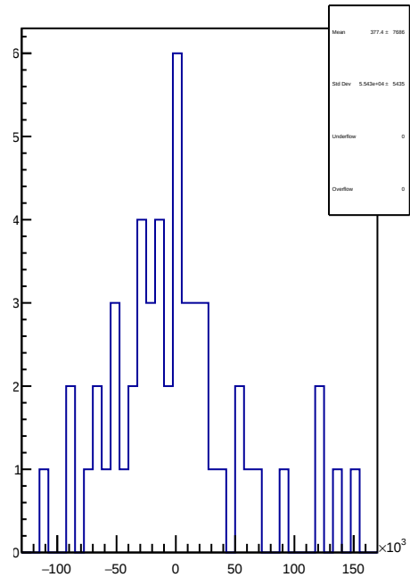
slug55: 1D Corr asym_sam2.mean/ppb-reg_asym_sam2.mean/ppb
