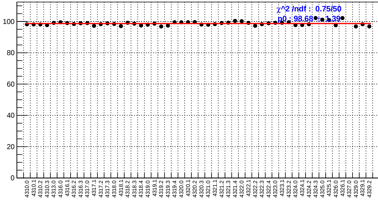
slug55: reg_asym_us_avg.rms/ppm
