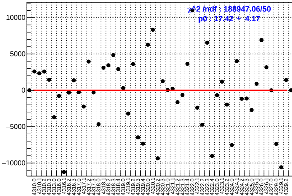
slug55: asym_dsr.mean/ppb-reg_asym_dsr.mean/ppb
