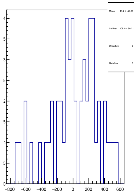
slug55: 1D Corr asym_right_dd.mean/ppb-reg_asym_right_dd.mean/ppb
