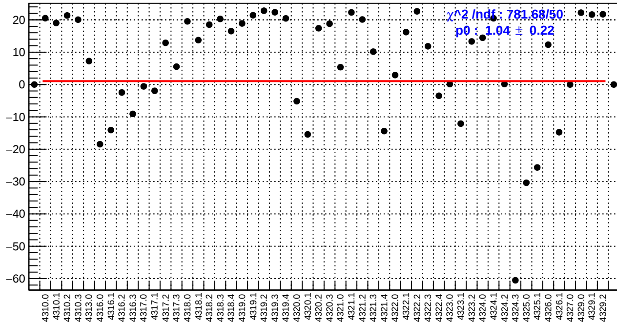
slug55: usl_bpm4eY/(ppb/nm)
