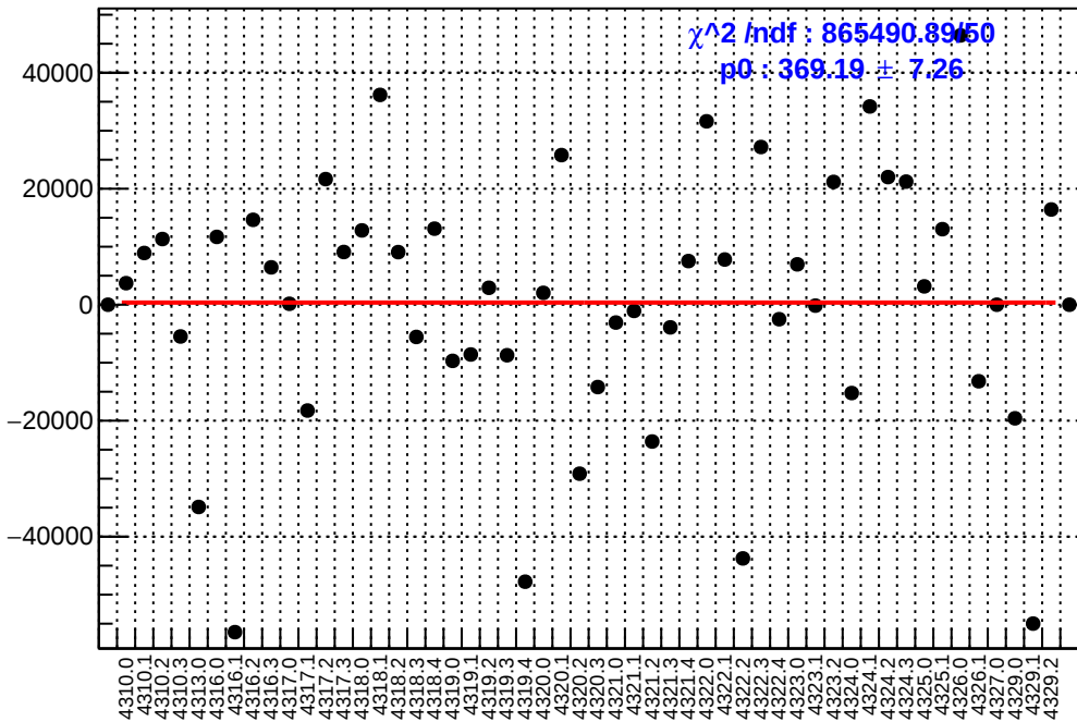
slug55: asym_sam6.mean/ppb-reg_asym_sam6.mean/ppb
