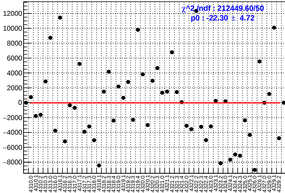
slug55: asym_left_avg.mean/ppb-reg_asym_left_avg.mean/ppb
