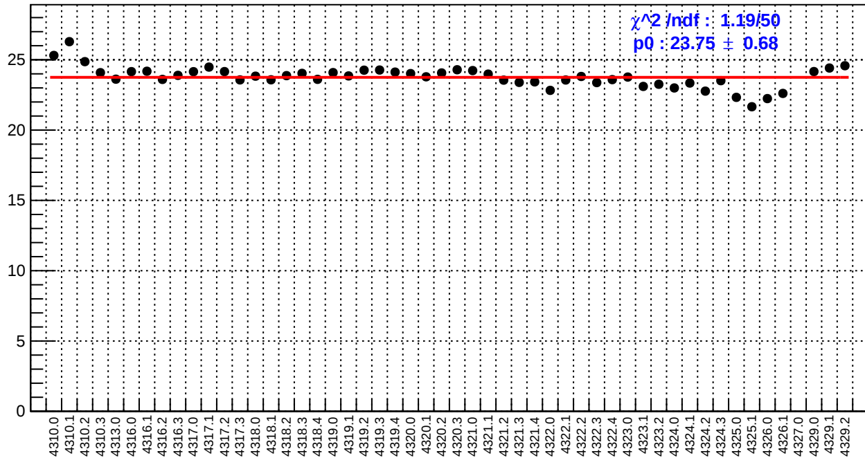
slug55: right_avg_bpm4eX/(ppb/nm)
