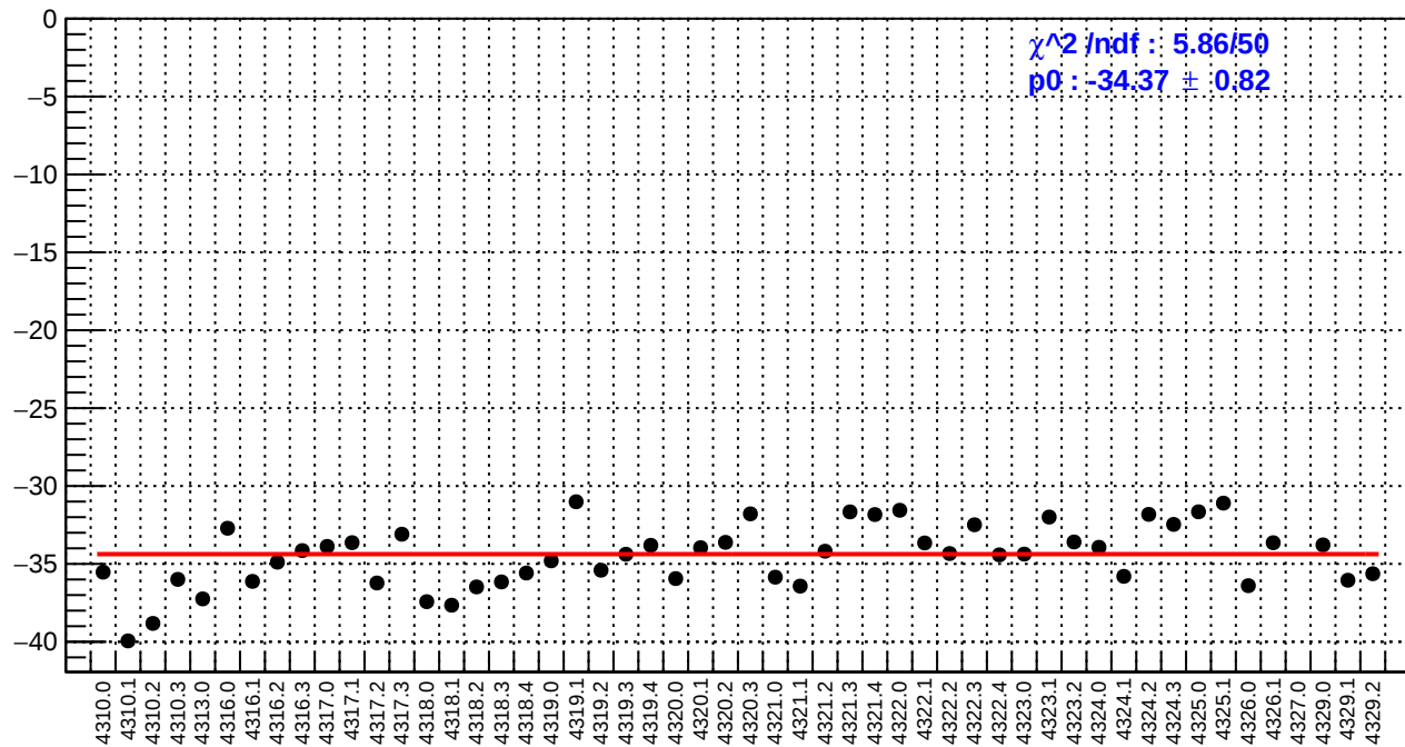
slug55: dsr_bpm4aX/(ppb/nm)
