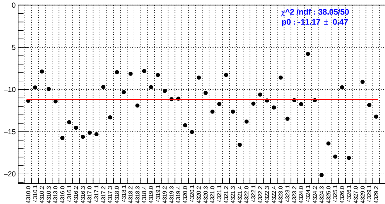
slug55: right_avg_bpm4aY/(ppb/nm)
