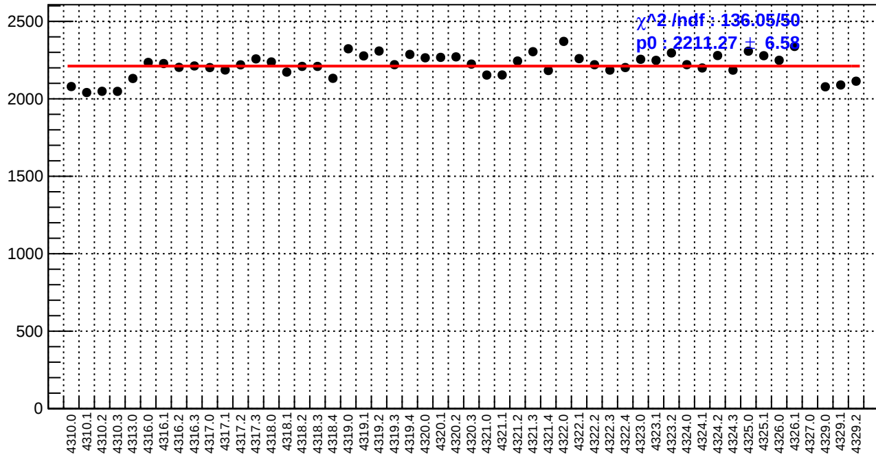
slug55: diff_bpm4aY.rms/nm
