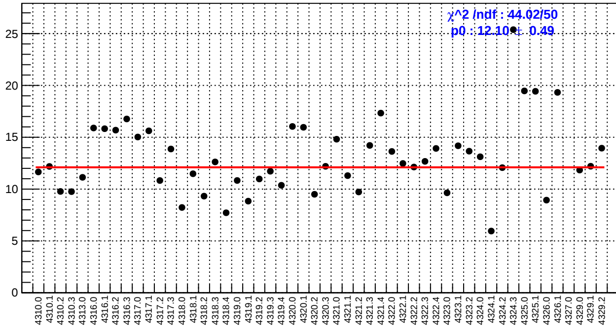
slug55: right_avg_bpm4eY/(ppb/nm)
