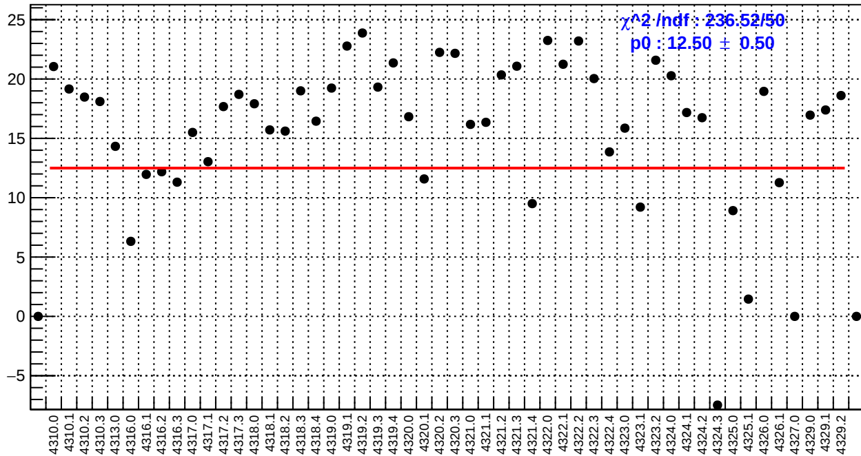
slug55: left_avg_bpm4aX/(ppb/nm)
