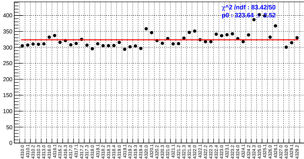
slug55: reg_asym_sam5.rms/ppm
