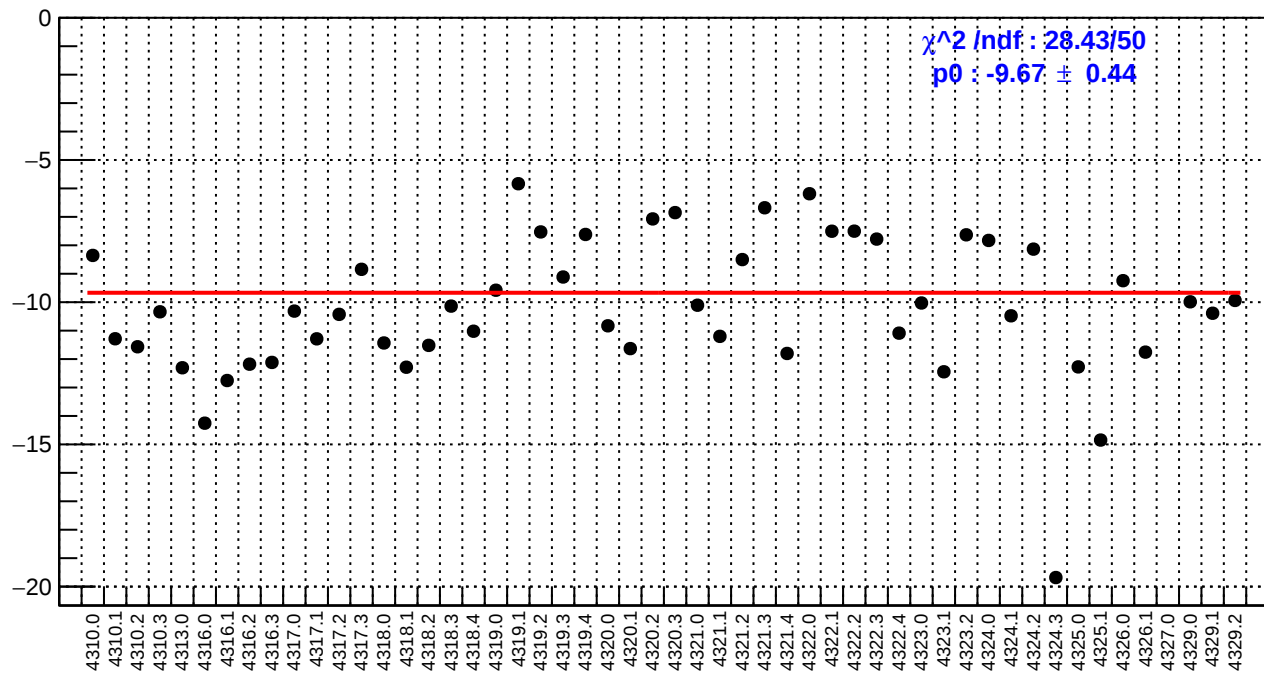
slug55: us_avg_bpm4aX/(ppb/nm)
