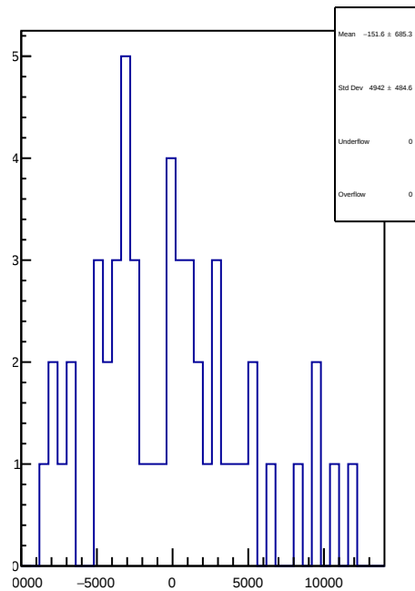
slug55: 1D Corr asym_usl.mean/ppb-reg_asym_usl.mean/ppb
