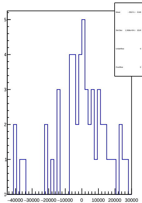
slug55: 1D Corr asym_sam8.mean/ppb-reg_asym_sam8.mean/ppb
