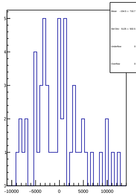
slug55: 1D Corr asym_left_avg.mean/ppb-reg_asym_left_avg.mean/ppb
