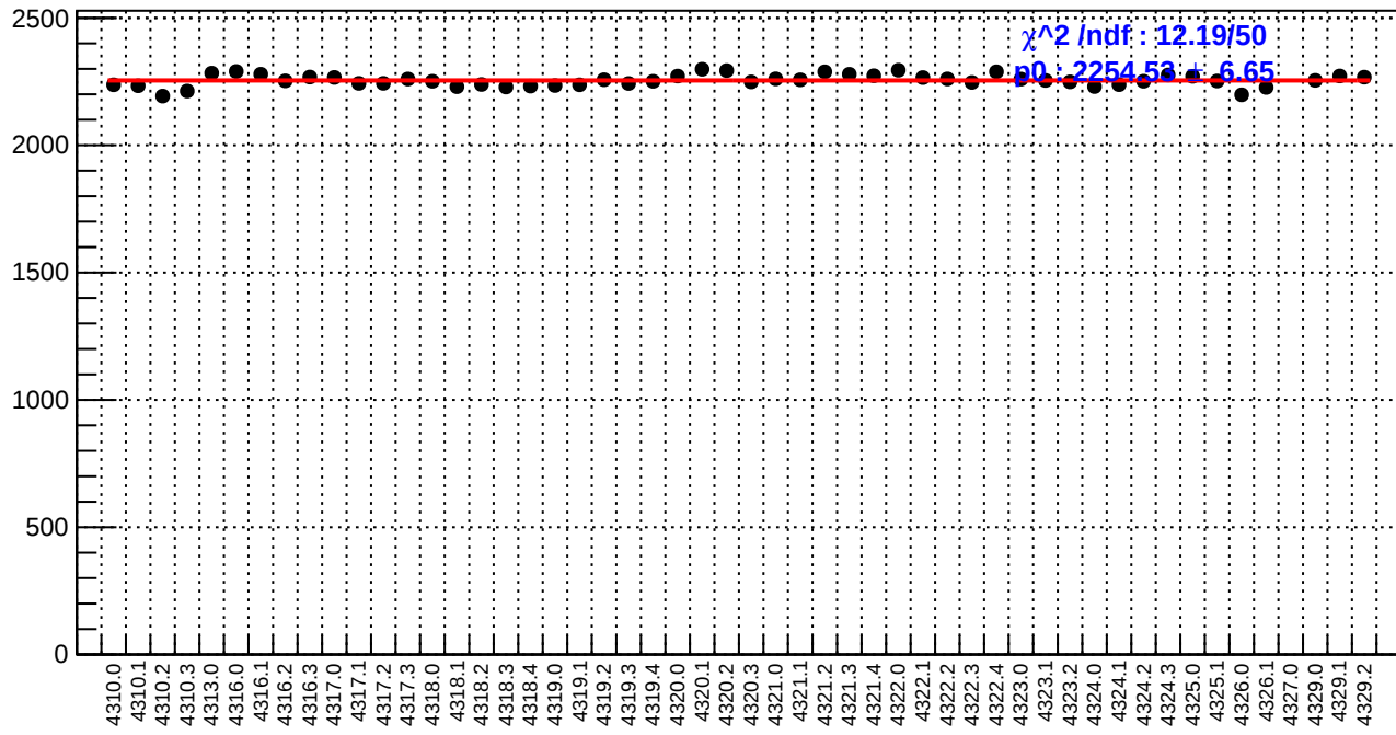
slug55: reg_asym_sam2.rms/ppm
