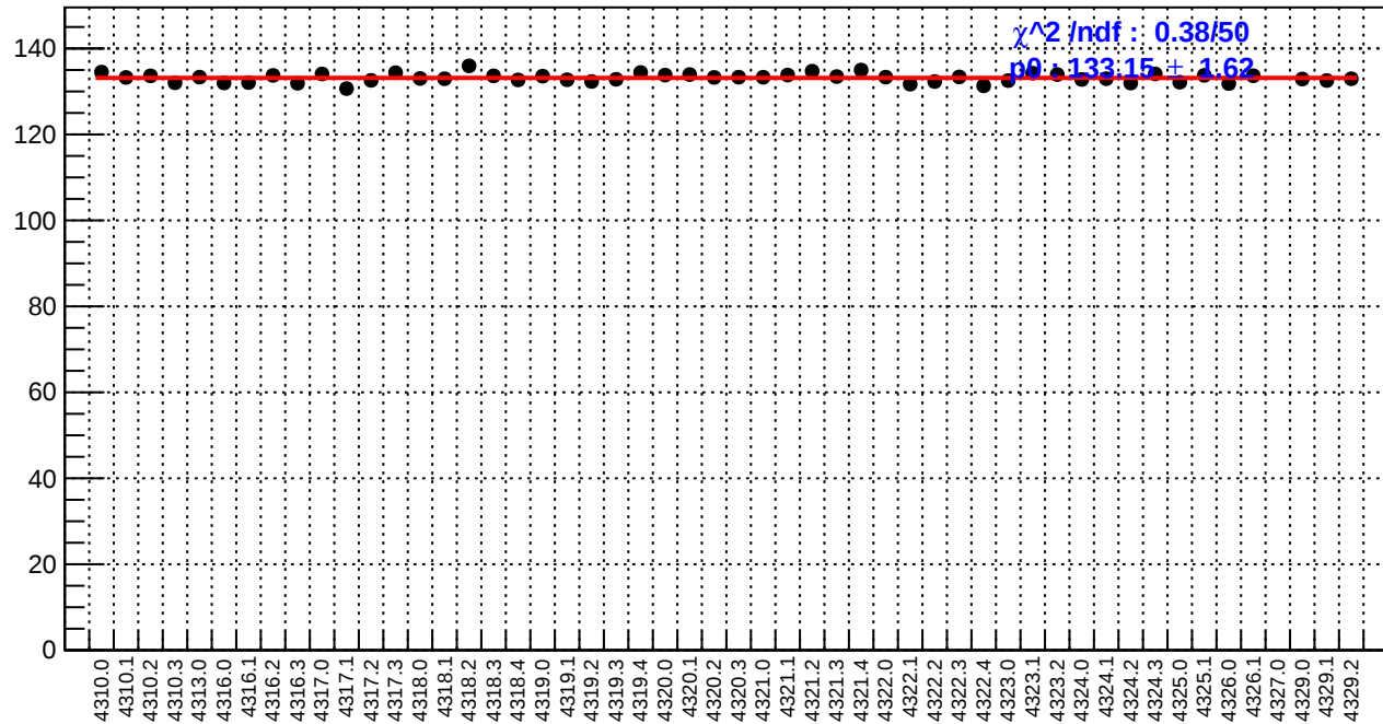
slug55: reg_asym_usr.rms/ppm
