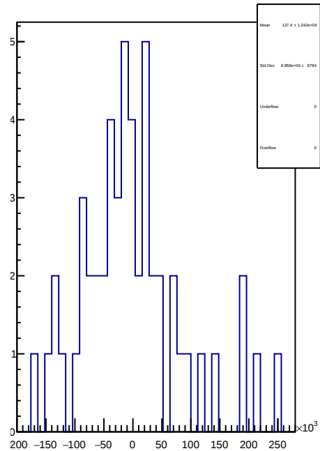
slug55: 1D Corr asym_sam3.mean/ppb-reg_asym_sam3.mean/ppb
