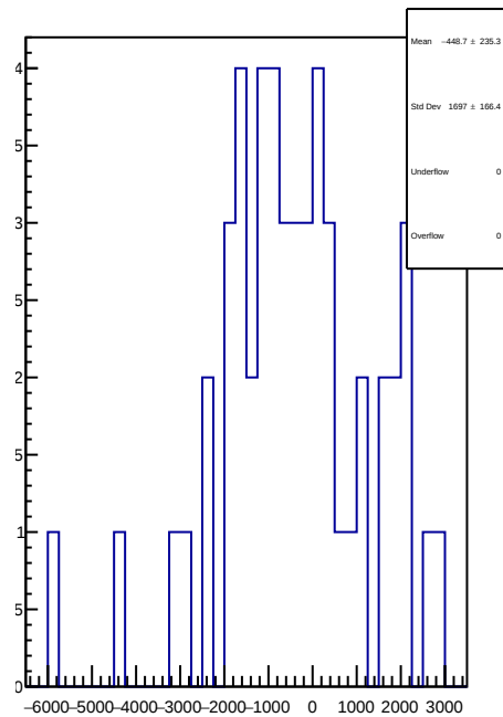
slug55: 1D Corr asym_sam1.mean/ppb-reg_asym_sam1.mean/ppb
