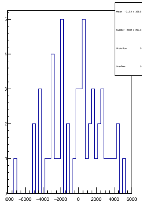
slug55: 1D Corr asym_ds_avg.mean/ppb-reg_asym_ds_avg.mean/ppb
