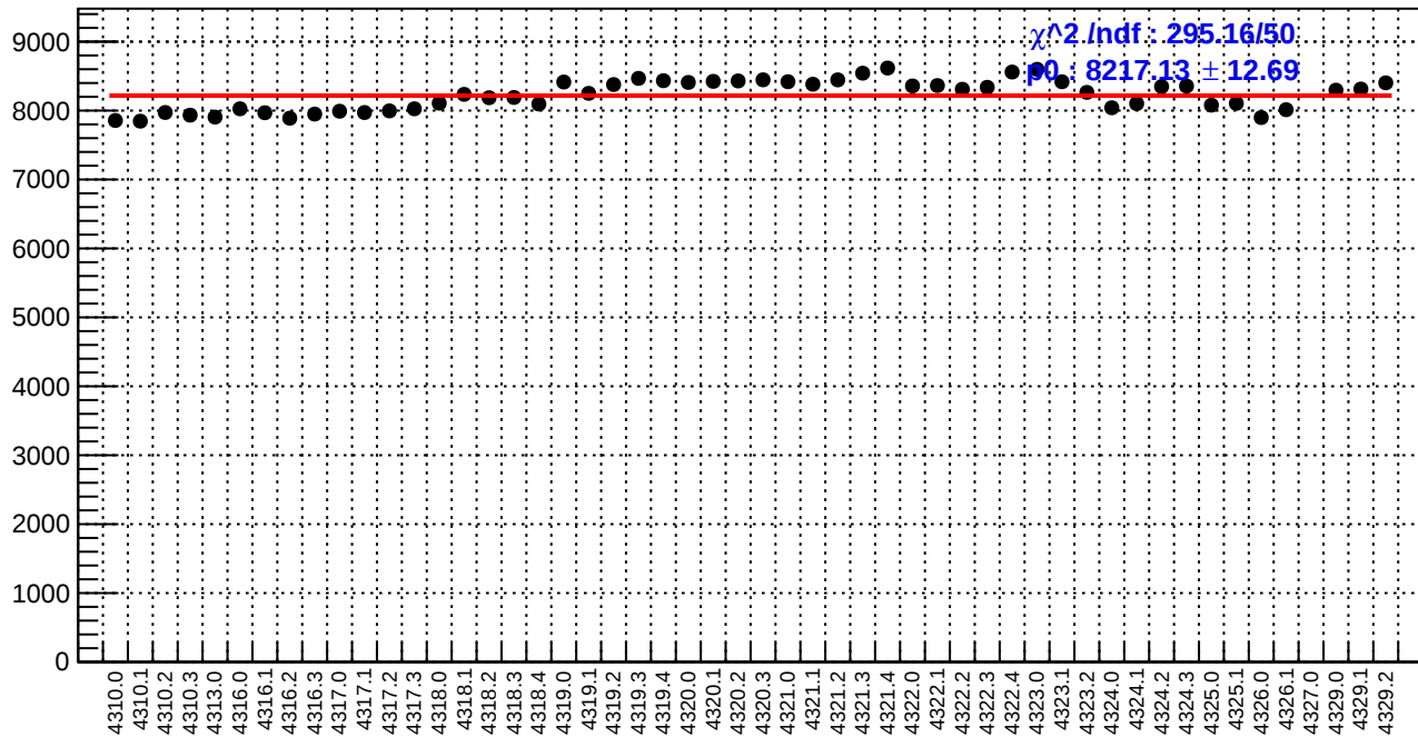
slug55: diff_bpm4eX.rms/nm
