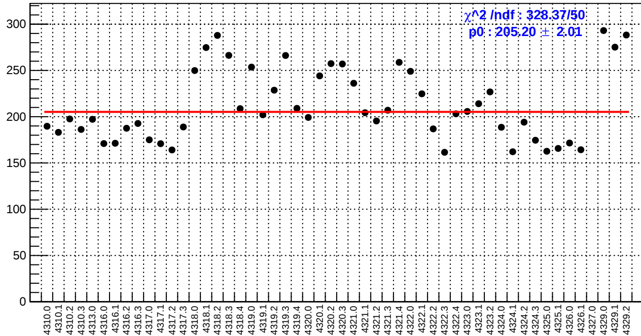
slug55: asym_bcm_an_us.rms/ppm
