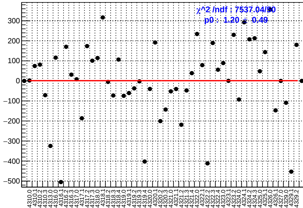
slug55: asym_left_dd.mean/ppb-reg_asym_left_dd.mean/ppb
