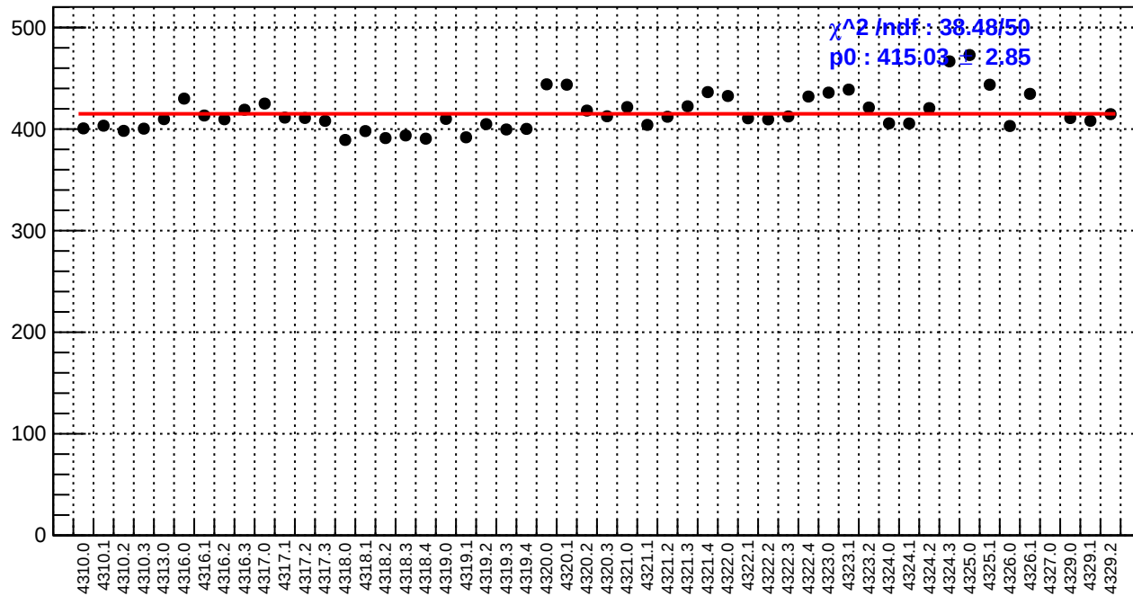
slug55: reg_asym_sam8.rms/ppm
