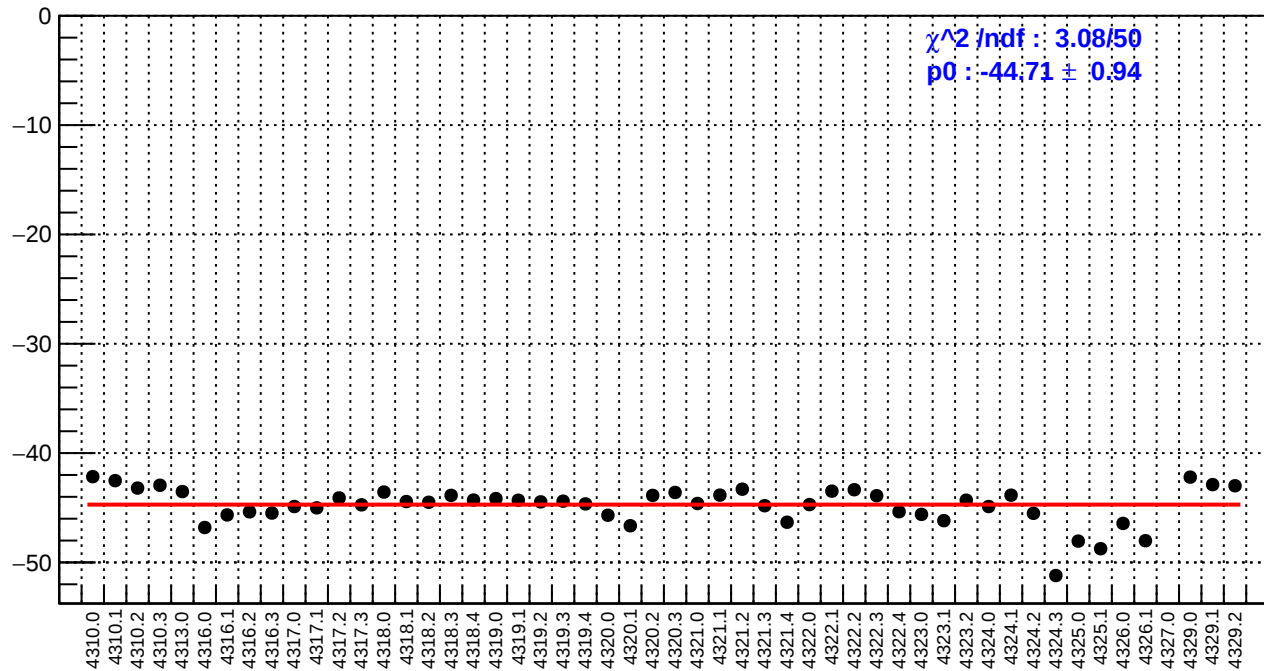
slug55: left_avg_bpm12X/(ppb/nm)
