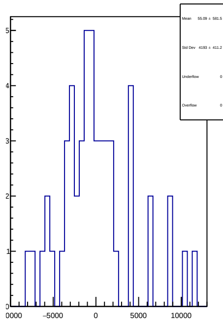
slug55: 1D Corr asym_ds_dd.mean/ppb-reg_asym_ds_dd.mean/ppb
