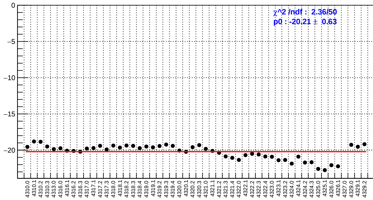
slug55: us_avg_bpm4eX/(ppb/nm)
