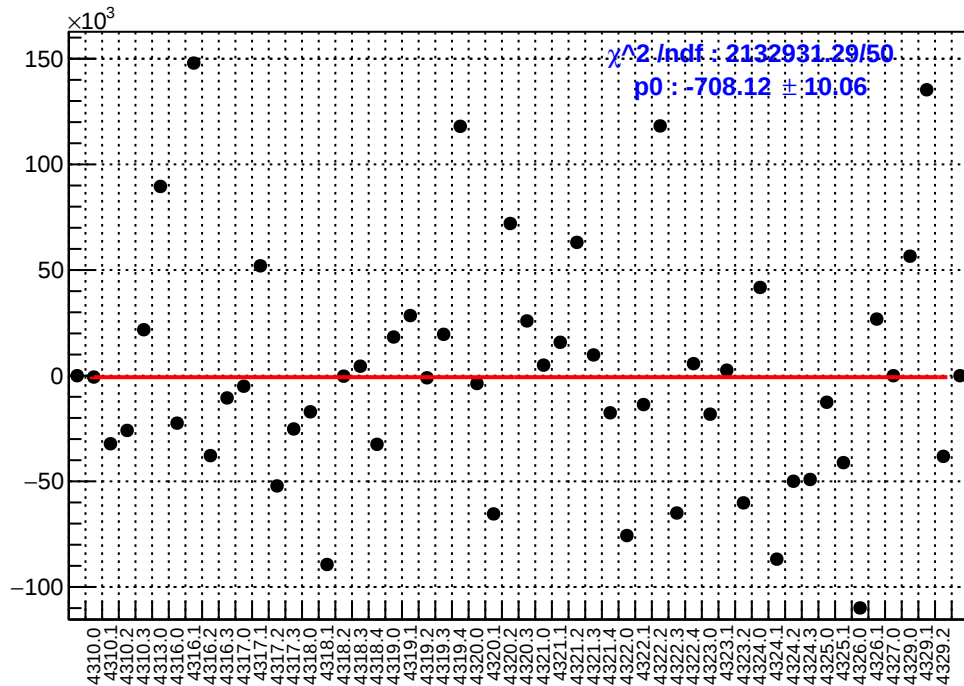
slug55: asym_sam2.mean/ppb-reg_asym_sam2.mean/ppb
