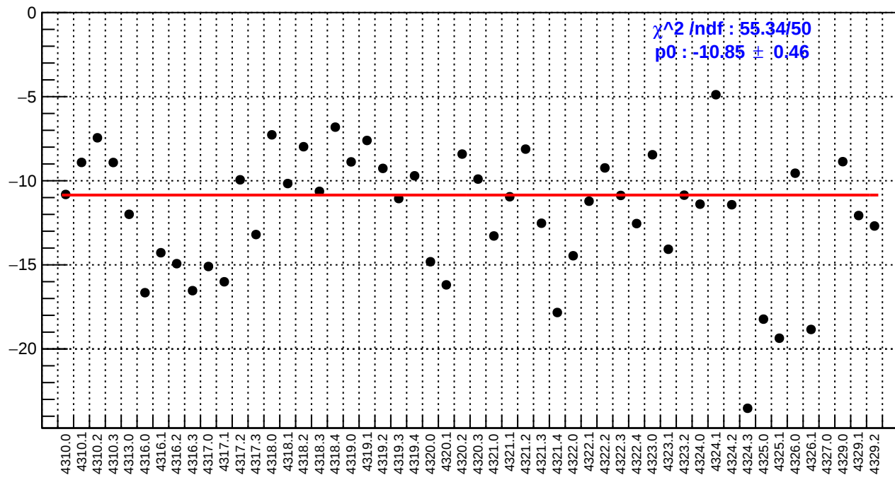
slug55: usr_bpm4aY/(ppb/nm)
