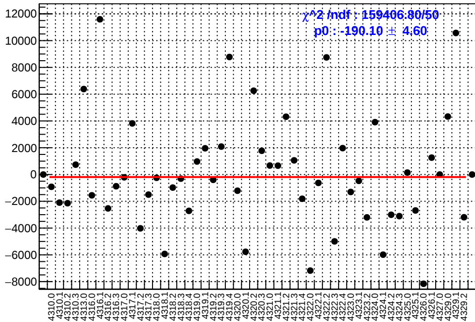
slug55: asym_ds_dd.mean/ppb-reg_asym_ds_dd.mean/ppb
