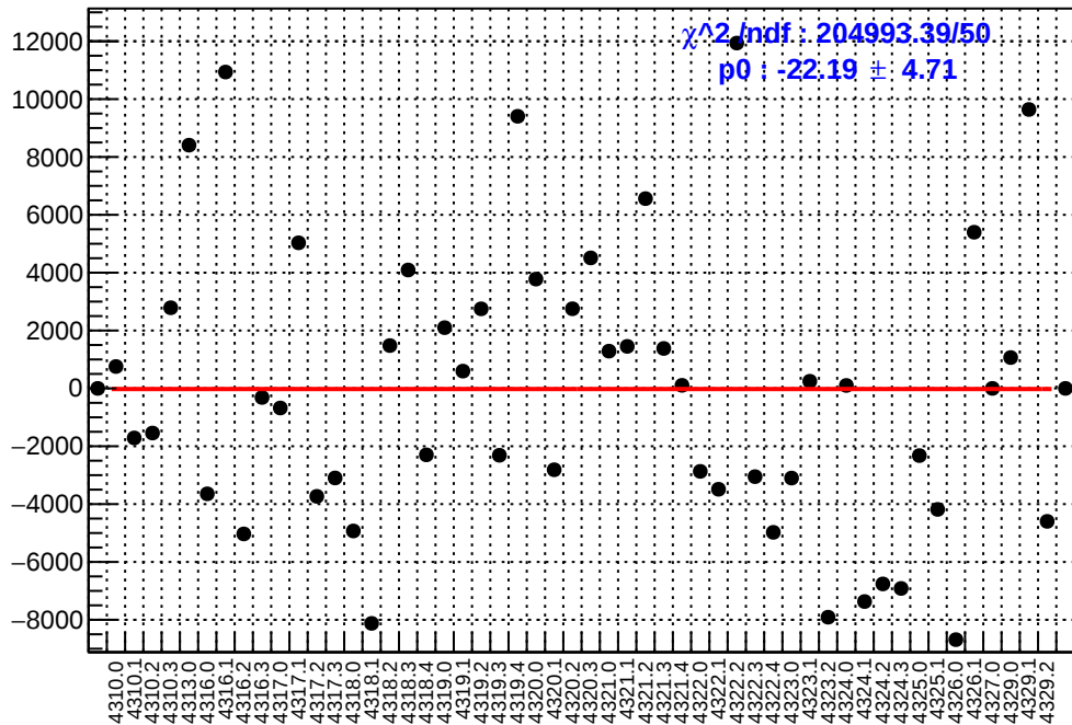
slug55: asym_usl.mean/ppb-reg_asym_usl.mean/ppb
