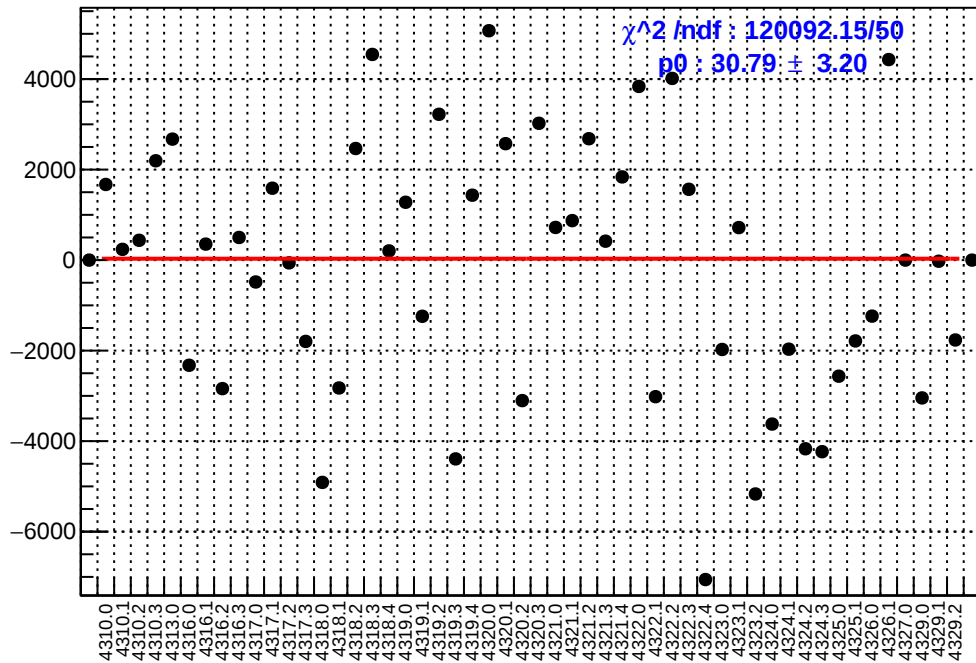
slug55: asym_ds_avg.mean/ppb-reg_asym_ds_avg.mean/ppb
