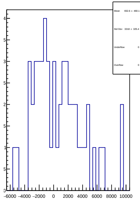
slug55: 1D Corr asym_sam5.mean/ppb-reg_asym_sam5.mean/ppb
