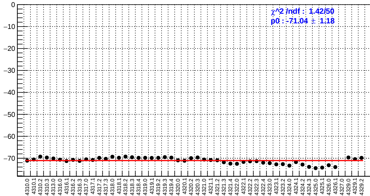
slug55: left_avg_bpm4eX/(ppb/nm)
