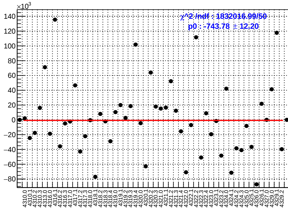
slug55: asym_sam4.mean/ppb-reg_asym_sam4.mean/ppb
