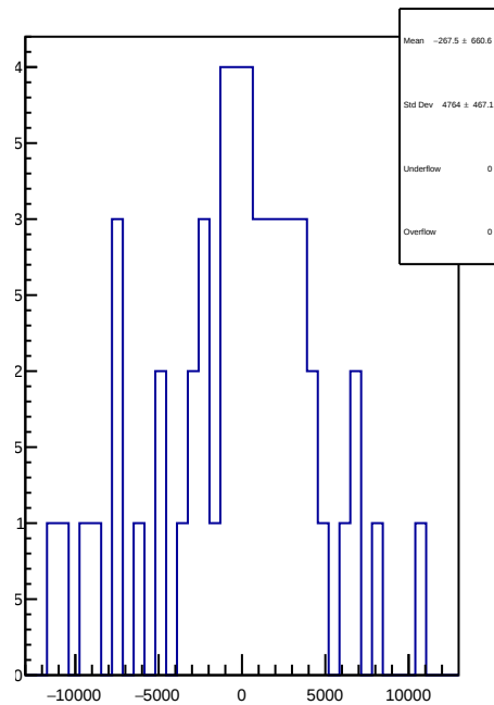
slug55: 1D Corr asym_dsr.mean/ppb-reg_asym_dsr.mean/ppb
