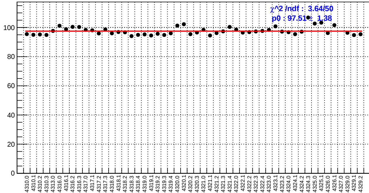
slug55: reg_asym_ds_dd.rms/ppm
