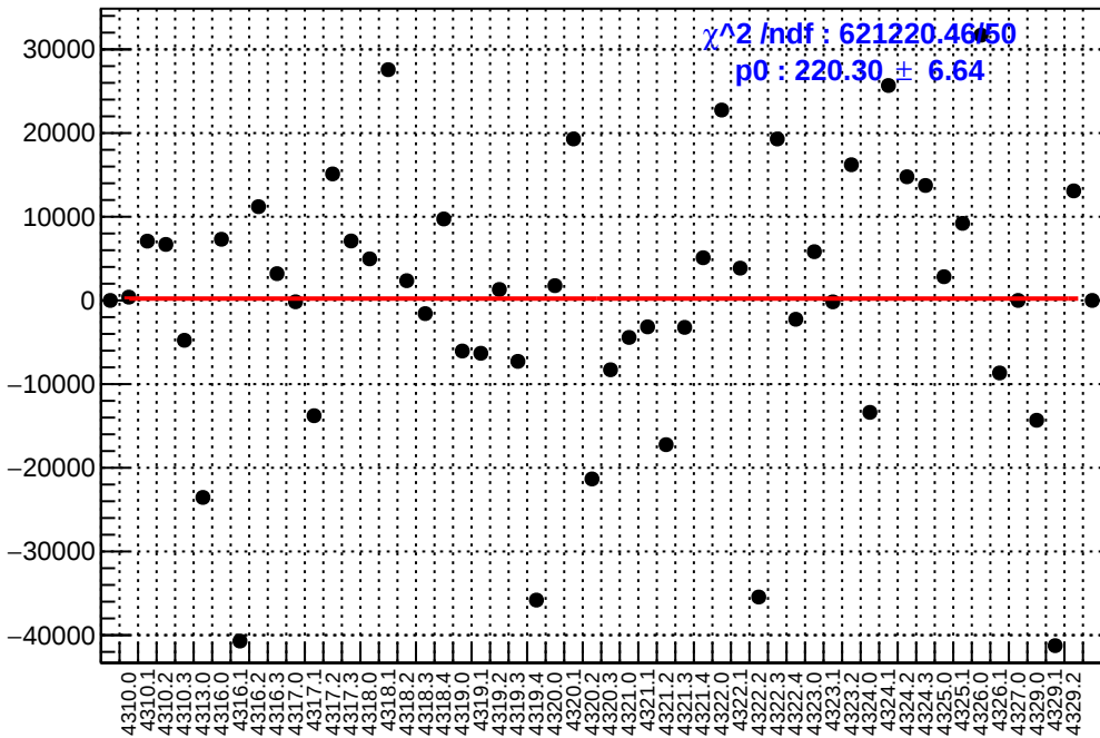
slug55: asym_sam7.mean/ppb-reg_asym_sam7.mean/ppb
