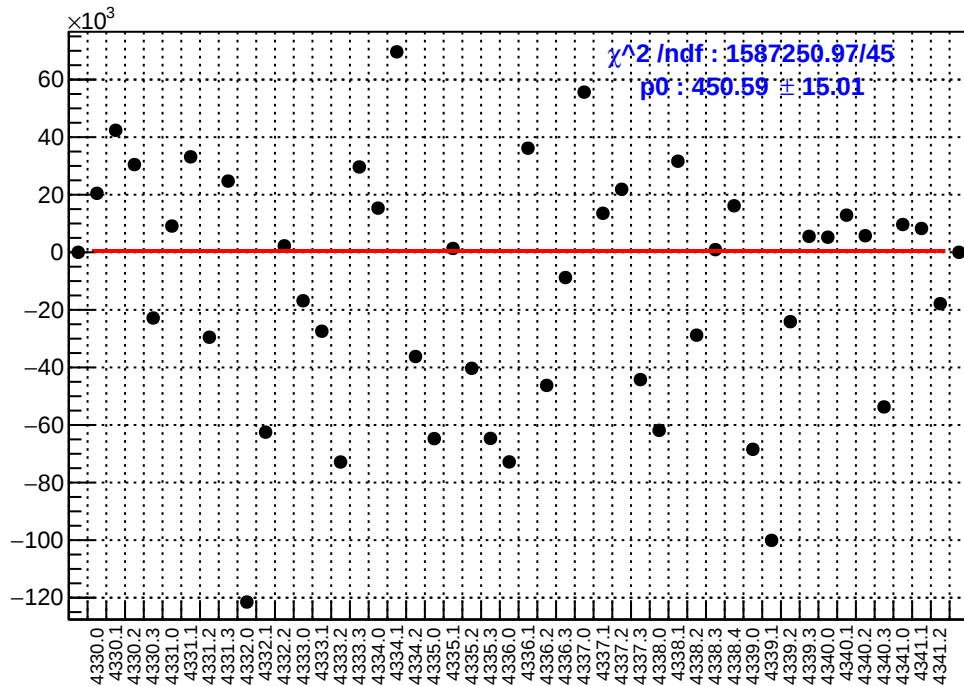
slug56: asym_sam2.mean/ppb-reg_asym_sam2.mean/ppb
