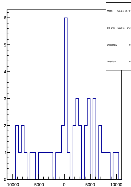
slug56: 1D Corr asym_right_avg.mean/ppb-reg_asym_right_avg.mean/ppb
