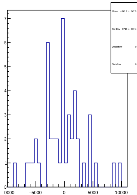
slug56: 1D Corr asym_ds_avg.mean/ppb-reg_asym_ds_avg.mean/ppb
