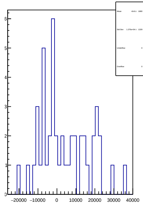
slug56: 1D Corr asym_sam7.mean/ppb-reg_asym_sam7.mean/ppb
