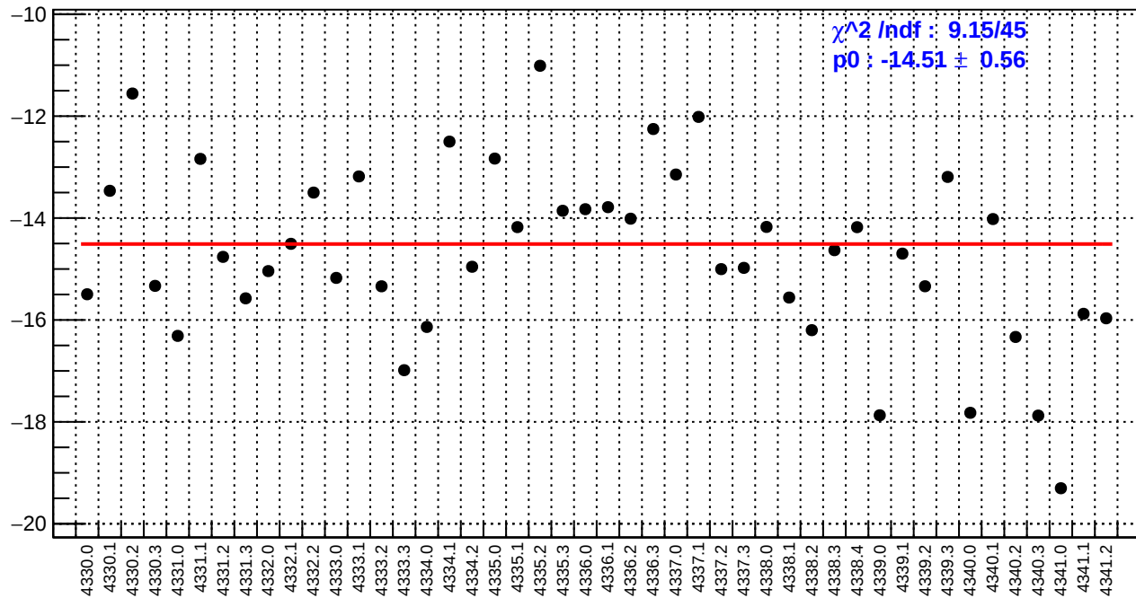
slug56: ds_avg_bpm4aY/(ppb/nm)
