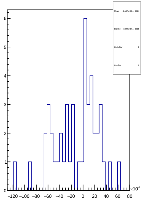
slug56: 1D Corr asym_sam4.mean/ppb-reg_asym_sam4.mean/ppb
