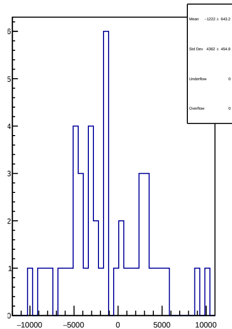
slug56: 1D Corr asym_usl.mean/ppb-reg_asym_usl.mean/ppb
