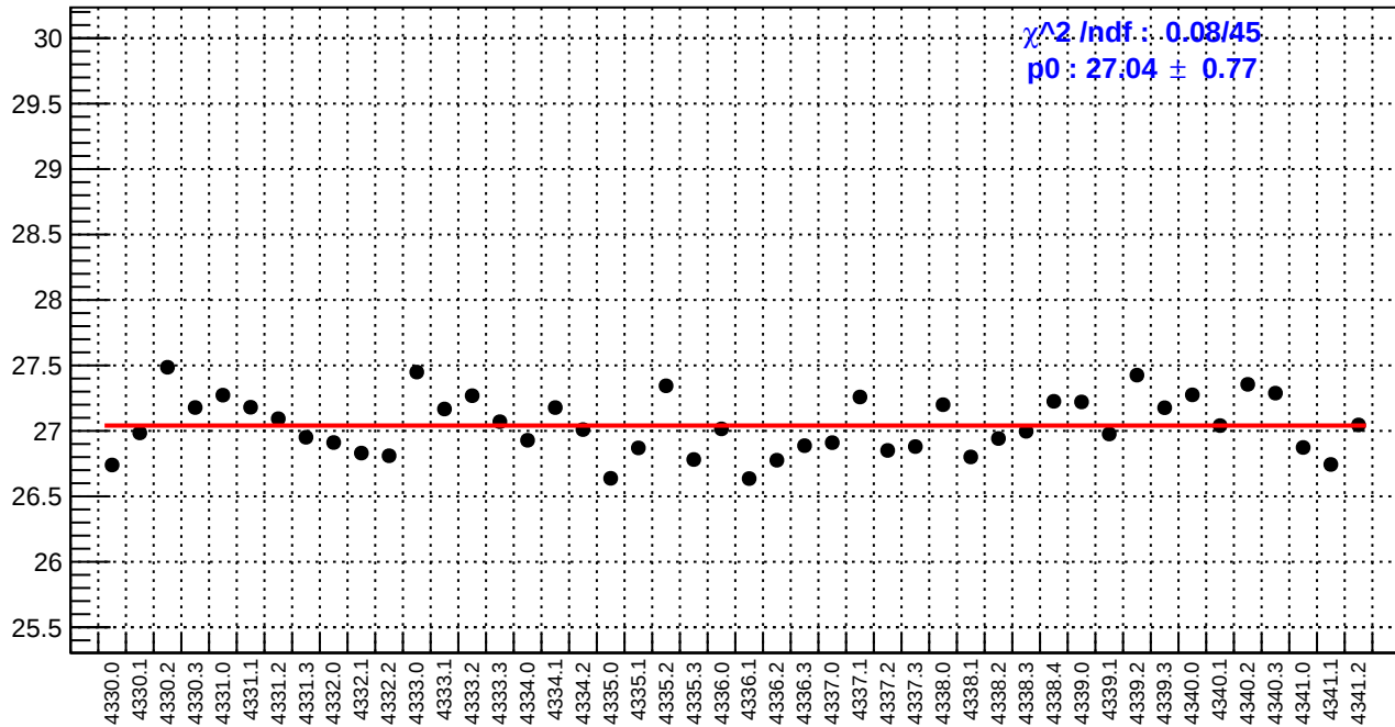
slug56: reg_asym_right_dd.rms/ppm
