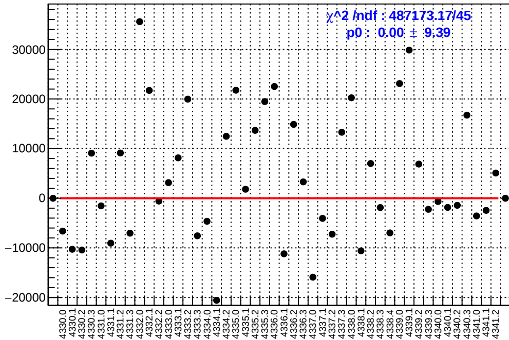
slug56: asym_sam7.mean/ppb-reg_asym_sam7.mean/ppb
