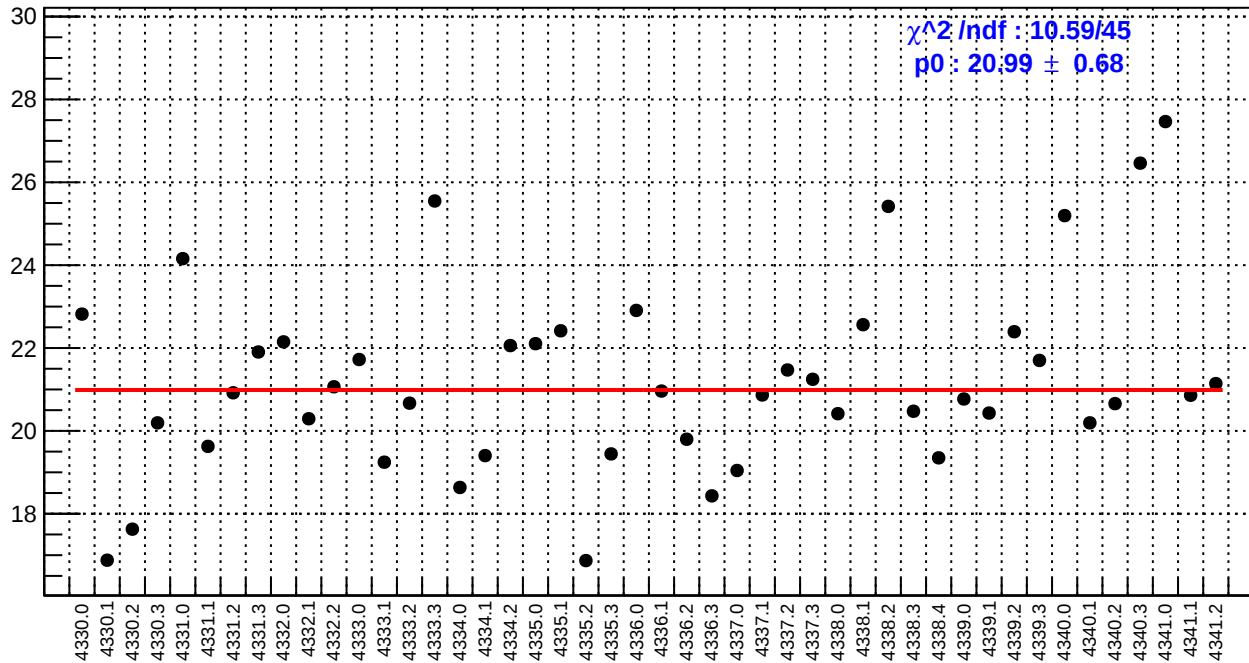
slug56: left_avg_bpm4eY/(ppb/nm)
