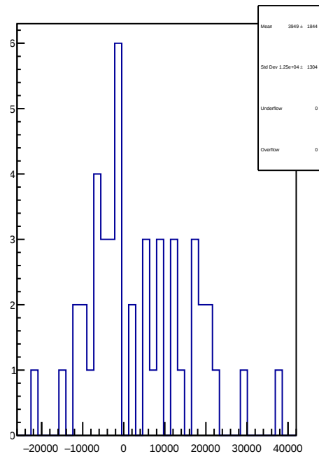
slug56: 1D Corr asym_sam8.mean/ppb-reg_asym_sam8.mean/ppb
