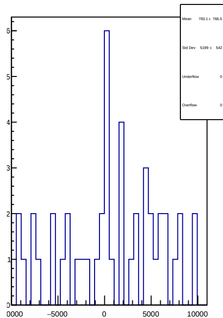
slug56: 1D Corr asym_usr.mean/ppb-reg_asym_usr.mean/ppb
