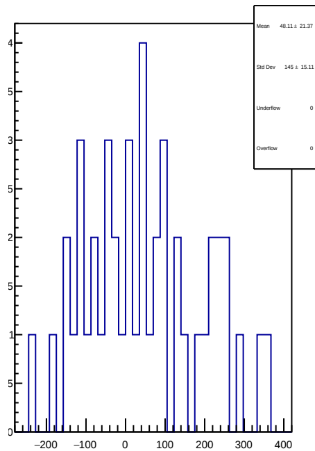
slug56: 1D Corr asym_left_dd.mean/ppb-reg_asym_left_dd.mean/ppb
