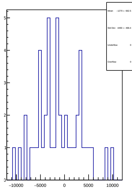
slug56: 1D Corr asym_left_avg.mean/ppb-reg_asym_left_avg.mean/ppb
