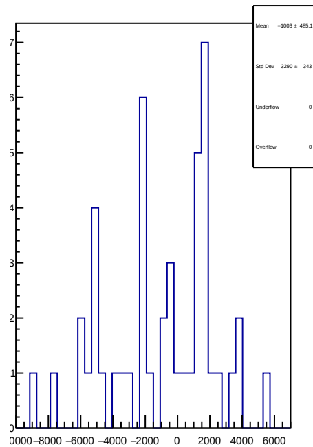
slug56: 1D Corr asym_us_dd.mean/ppb-reg_asym_us_dd.mean/ppb
