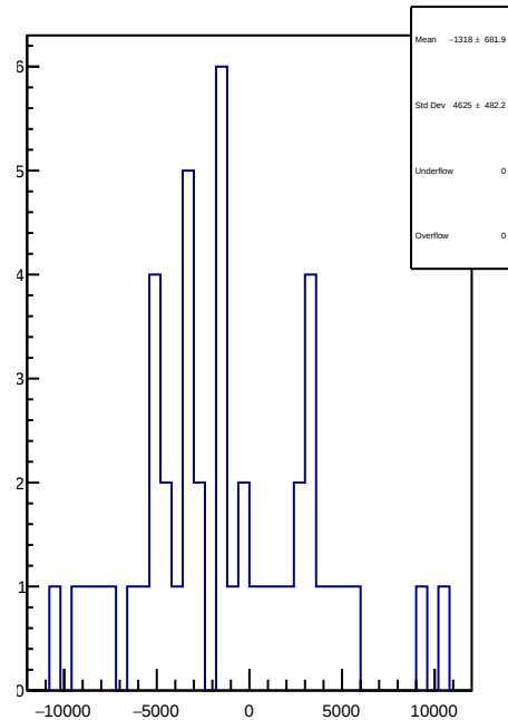
slug56: 1D Corr asym_dsl.mean/ppb-reg_asym_dsl.mean/ppb
