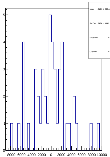
slug56: 1D Corr asym_us_avg.mean/ppb-reg_asym_us_avg.mean/ppb
