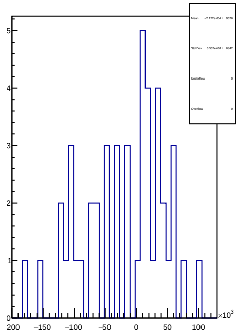
slug56: 1D Corr asym_sam3.mean/ppb-reg_asym_sam3.mean/ppb
