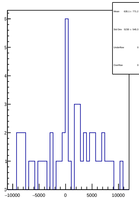
slug56: 1D Corr asym_dsr.mean/ppb-reg_asym_dsr.mean/ppb
