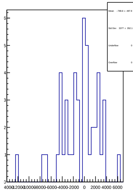
slug56: 1D Corr asym_sam5.mean/ppb-reg_asym_sam5.mean/ppb
