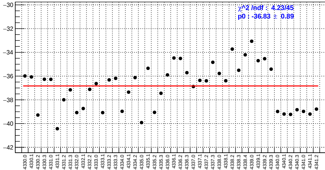
slug56: right_avg_bpm4aX/(ppb/nm)
