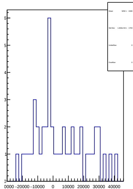
slug56: 1D Corr asym_sam6.mean/ppb-reg_asym_sam6.mean/ppb
