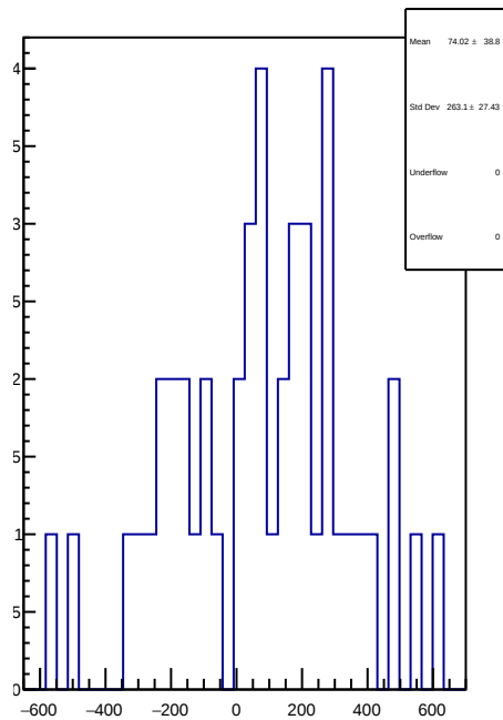
slug56: 1D Corr asym_right_dd.mean/ppb-reg_asym_right_dd.mean/ppb
