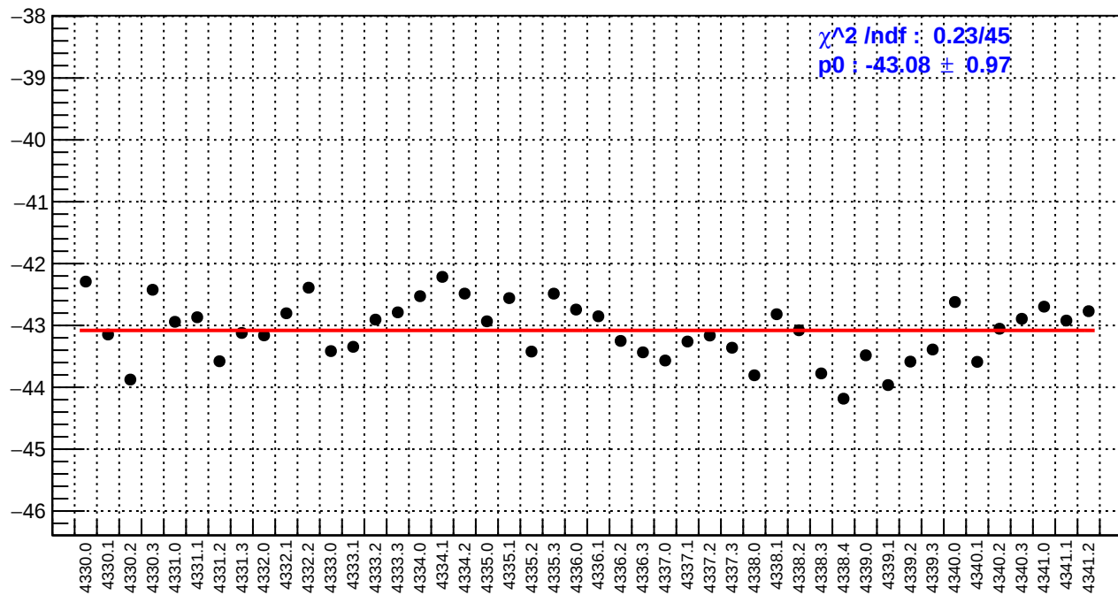
slug56: usl_bpm12X/(ppb/nm)
