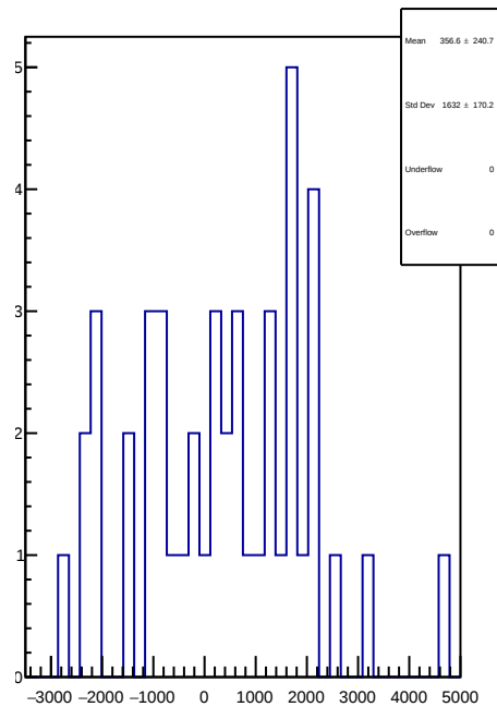
slug56: 1D Corr asym_sam1.mean/ppb-reg_asym_sam1.mean/ppb
