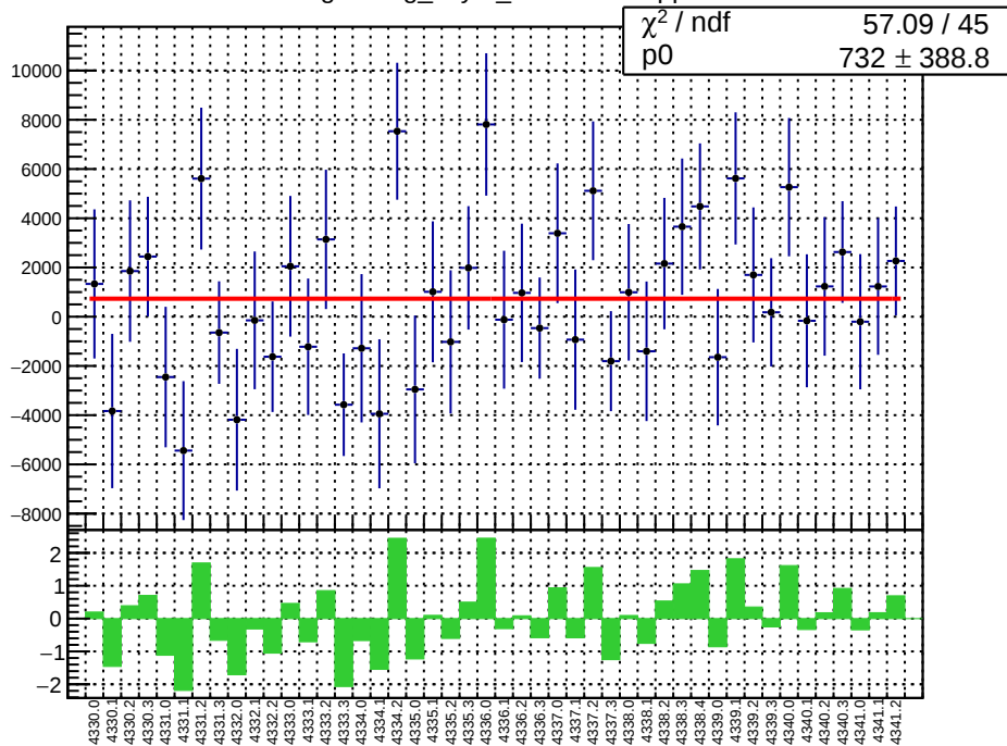
slug56: reg_asym_sam1.mean/ppb
