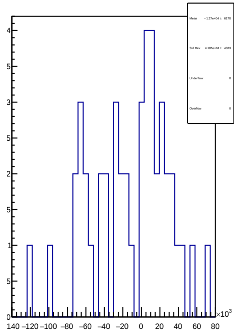
slug56: 1D Corr asym_sam2.mean/ppb-reg_asym_sam2.mean/ppb
