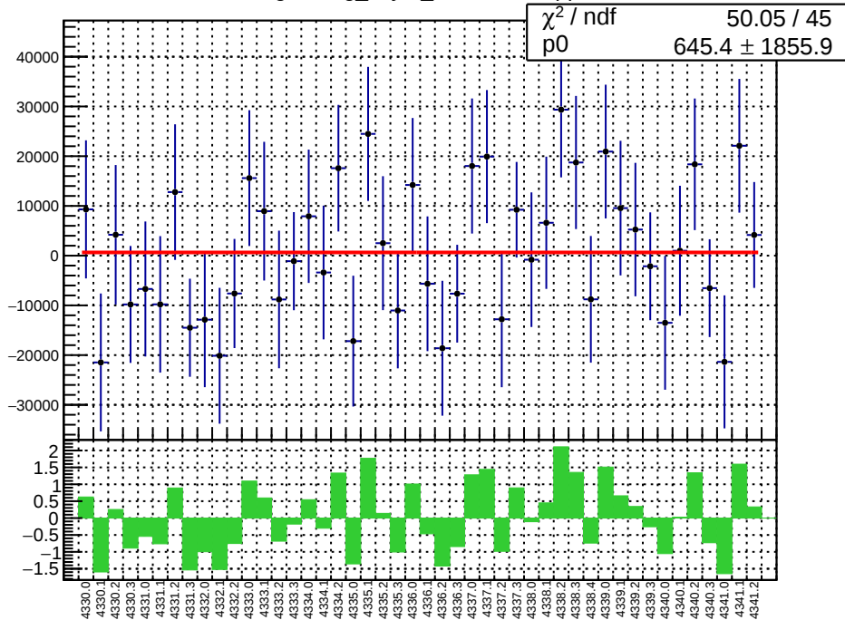
slug56: reg_asym_sam4.mean/ppb
