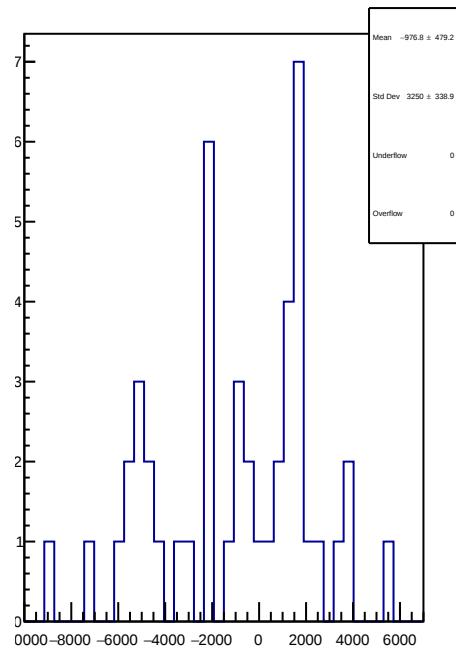
slug56: 1D Corr asym_ds_dd.mean/ppb-reg_asym_ds_dd.mean/ppb
