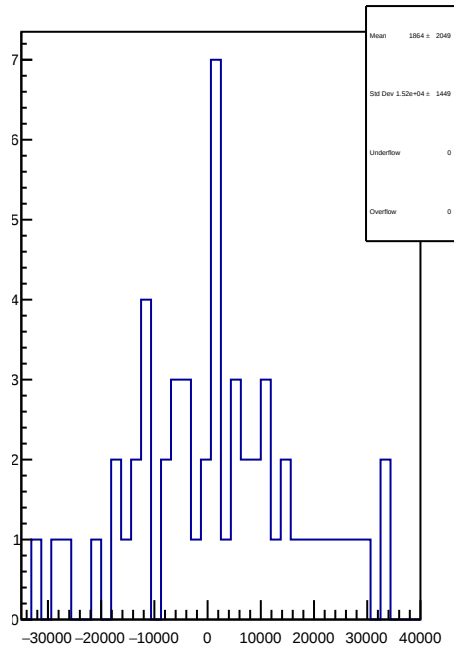
slug57: 1D Corr asym_sam7.mean/ppb-reg_asym_sam7.mean/ppb
