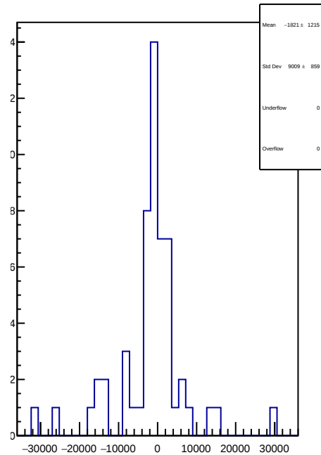
slug57: 1D Corr asym_sam1.mean/ppb-reg_asym_sam1.mean/ppb
