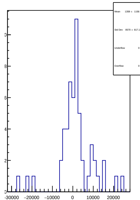
slug57: 1D Corr asym_sam5.mean/ppb-reg_asym_sam5.mean/ppb
