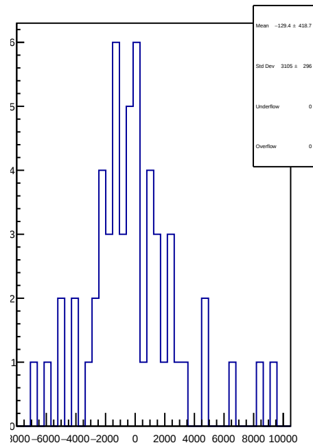
slug57: 1D Corr asym_us_avg.mean/ppb-reg_asym_us_avg.mean/ppb
