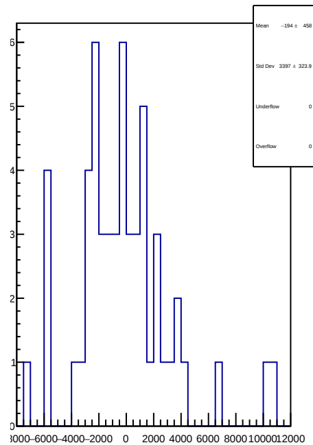
slug57: 1D Corr asym_ds_avg.mean/ppb-reg_asym_ds_avg.mean/ppb
