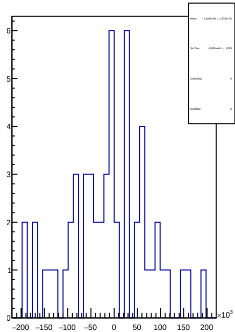
slug57: 1D Corr asym_sam3.mean/ppb-reg_asym_sam3.mean/ppb
