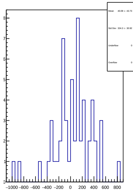
slug57: 1D Corr asym_right_dd.mean/ppb-reg_asym_right_dd.mean/ppb
