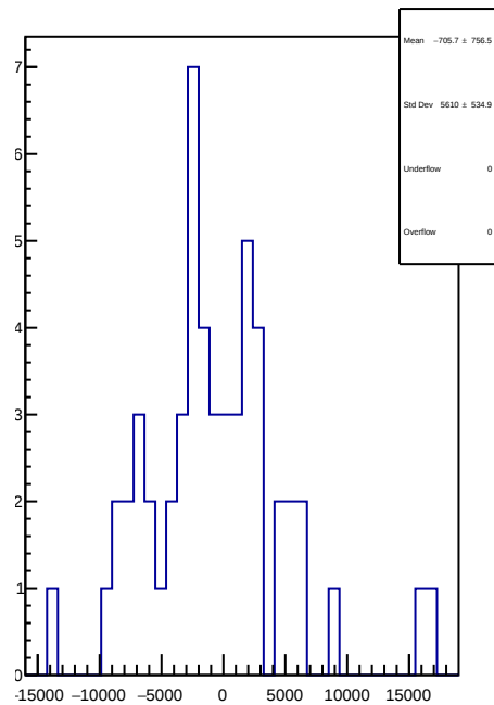
slug57: 1D Corr asym_dsl.mean/ppb-reg_asym_dsl.mean/ppb
