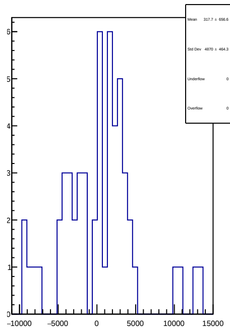
slug57: 1D Corr asym_dsr.mean/ppb-reg_asym_dsr.mean/ppb
