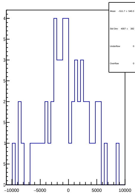
slug57: 1D Corr asym_ds_dd.mean/ppb-reg_asym_ds_dd.mean/ppb
