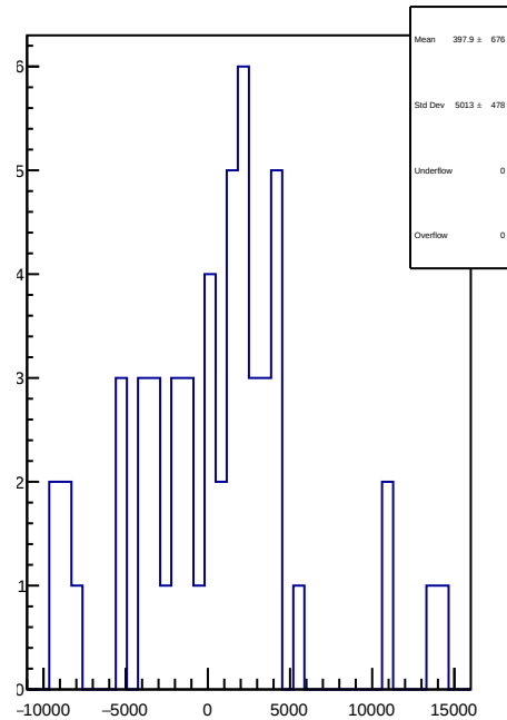
slug57: 1D Corr asym_usr.mean/ppb-reg_asym_usr.mean/ppb
