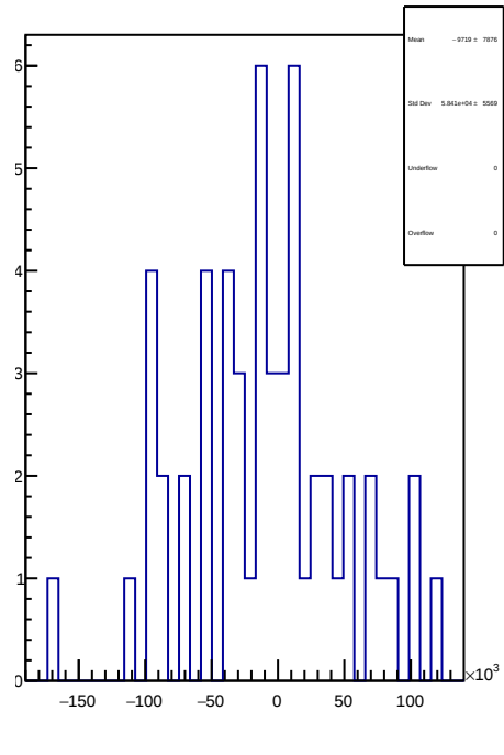
slug57: 1D Corr asym_sam2.mean/ppb-reg_asym_sam2.mean/ppb
