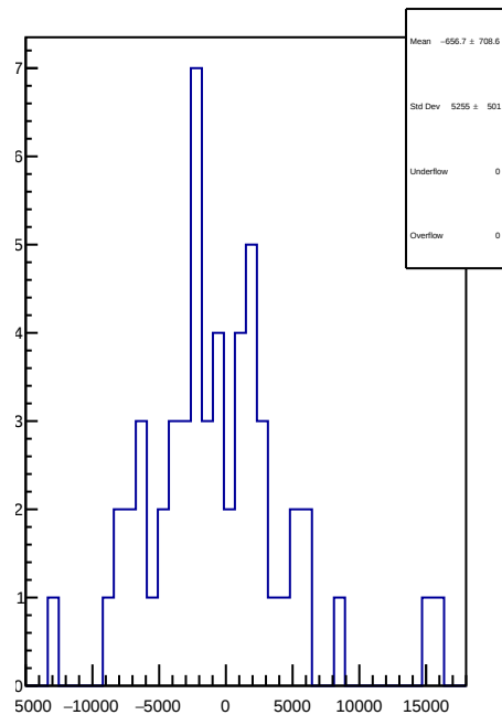
slug57: 1D Corr asym_usl.mean/ppb-reg_asym_usl.mean/ppb
