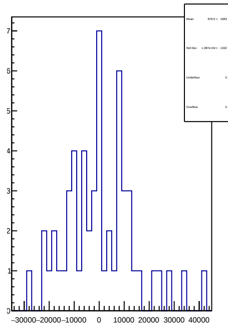
slug57: 1D Corr asym_sam8.mean/ppb-reg_asym_sam8.mean/ppb
