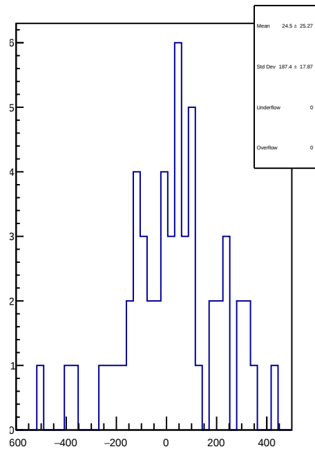
slug57: 1D Corr asym_left_dd.mean/ppb-reg_asym_left_dd.mean/ppb
