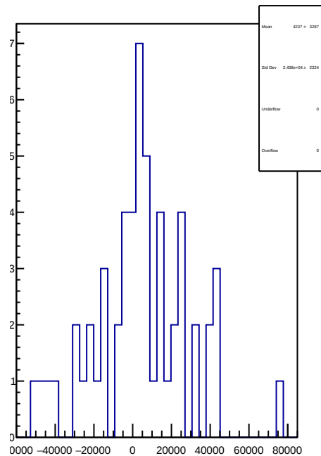
slug57: 1D Corr asym_sam6.mean/ppb-reg_asym_sam6.mean/ppb
