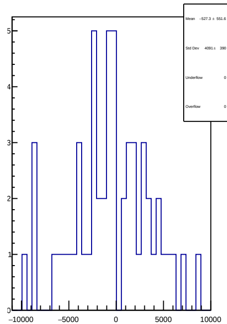
slug57: 1D Corr asym_us_dd.mean/ppb-reg_asym_us_dd.mean/ppb
