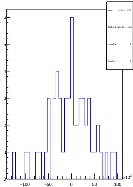
slug57: 1D Corr asym_sam4.mean/ppb-reg_asym_sam4.mean/ppb
