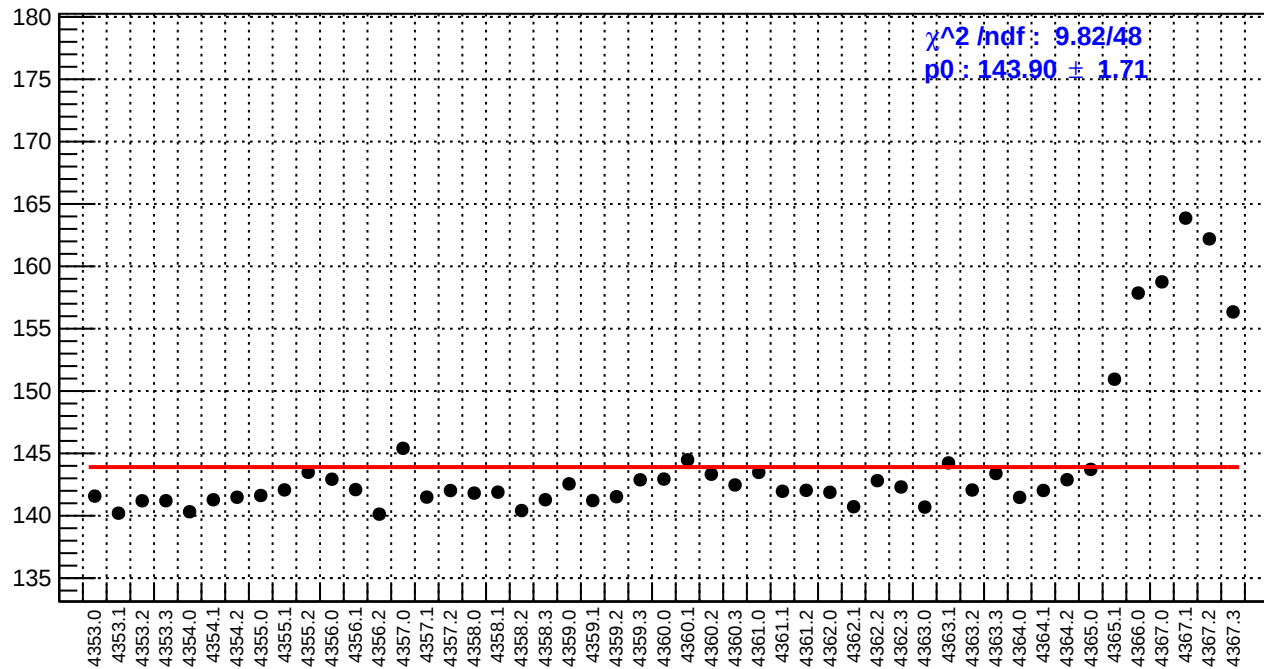
slug58: reg_asym_dsl.rms/ppm
