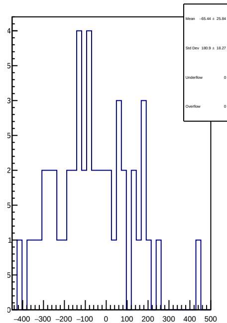
slug58: 1D Corr asym_left_dd.mean/ppb-reg_asym_left_dd.mean/ppb
