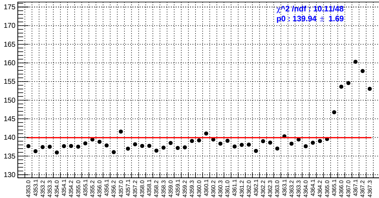
slug58: reg_asym_left_avg.rms/ppm
