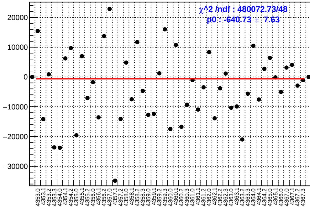
slug58: asym_sam8.mean/ppb-reg_asym_sam8.mean/ppb
