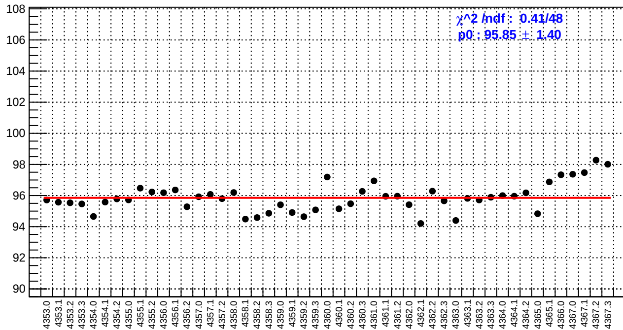
slug58: reg_asym_ds_dd.rms/ppm
