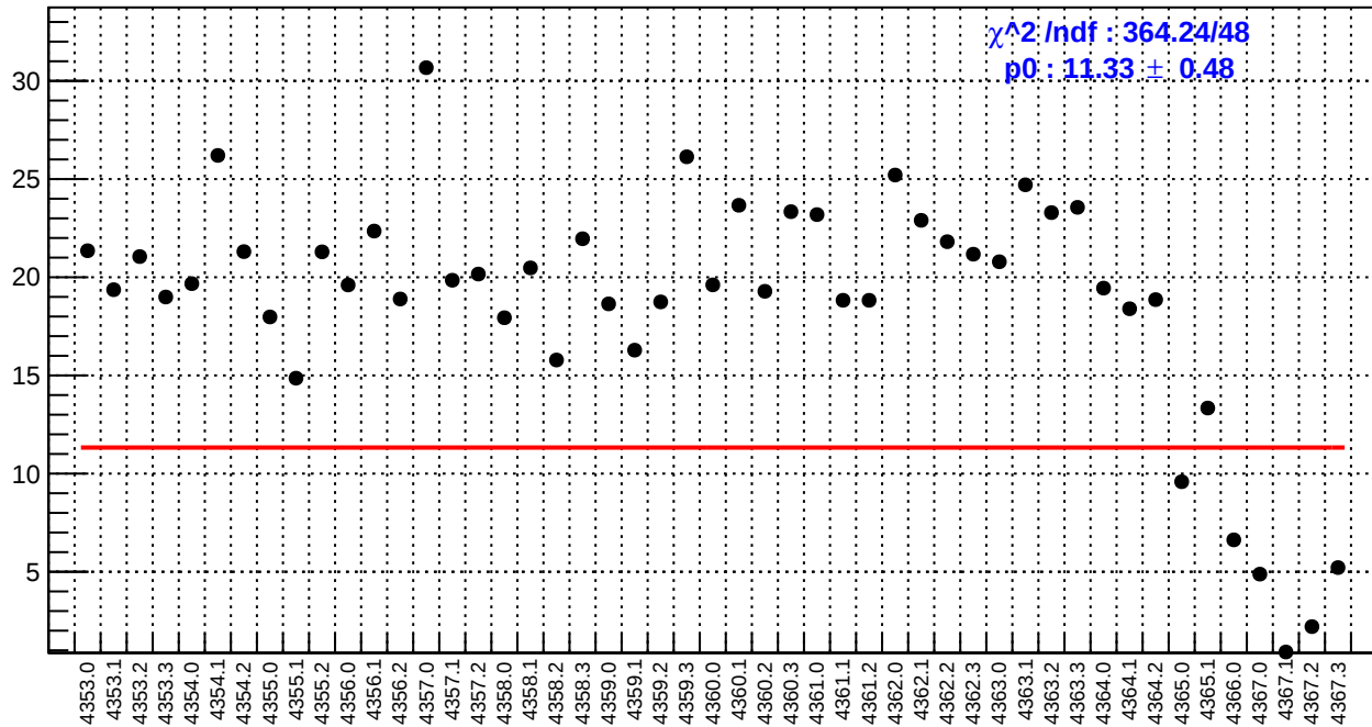
slug58: left_avg_bpm4aX/(ppb/nm)
