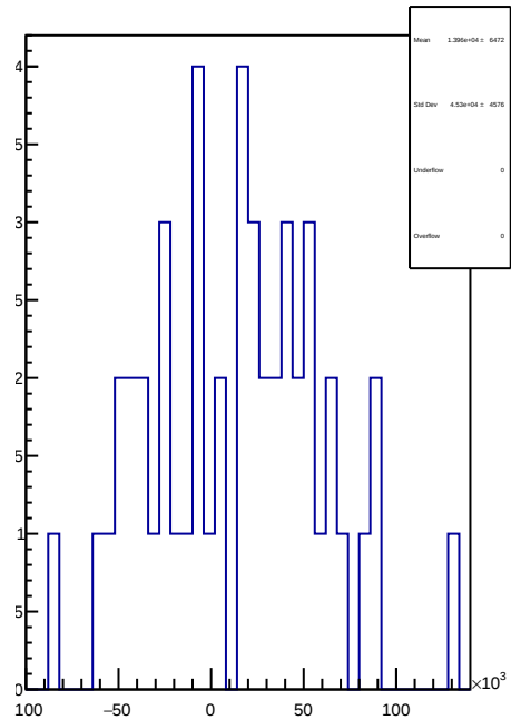
slug58: 1D Corr asym_sam4.mean/ppb-reg_asym_sam4.mean/ppb
