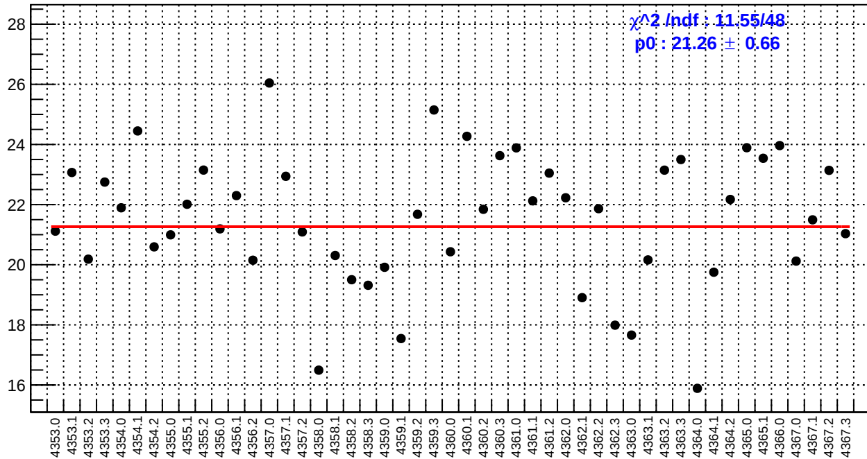
slug58: usl_bpm4eY/(ppb/nm)
