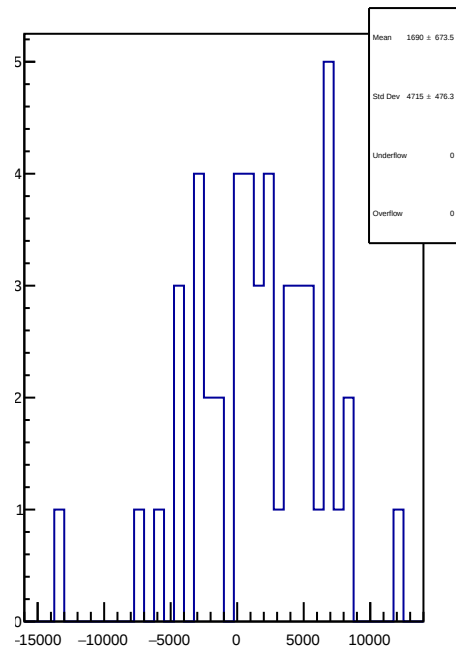
slug58: 1D Corr asym_left_avg.mean/ppb-reg_asym_left_avg.mean/ppb
