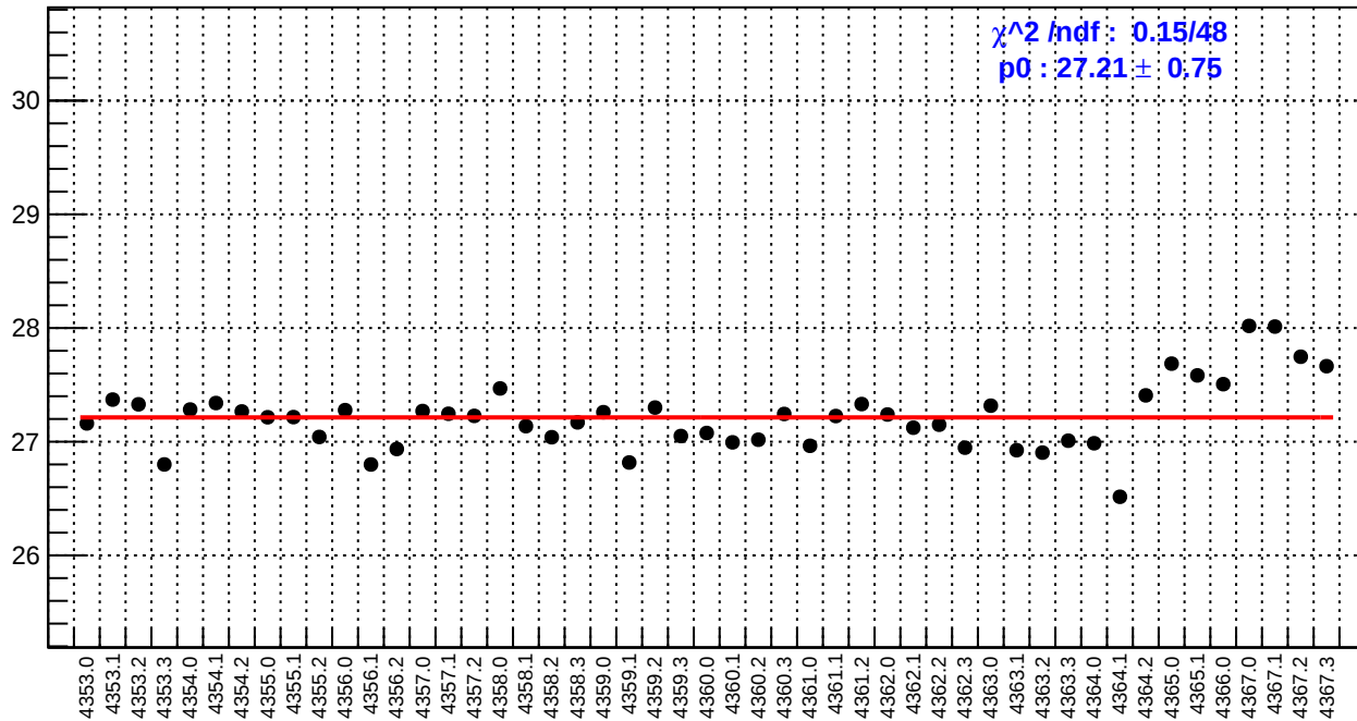
slug58: reg_asym_right_dd.rms/ppm
