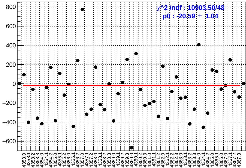
slug58: asym_right_dd.mean/ppb-reg_asym_right_dd.mean/ppb
