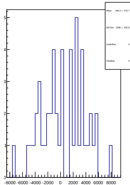
slug58: 1D Corr asym_sam5.mean/ppb-reg_asym_sam5.mean/ppb
