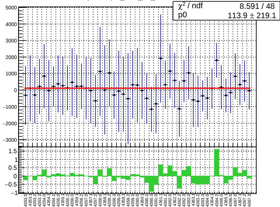
slug58: asym_bcm_an_ds.mean/ppb
