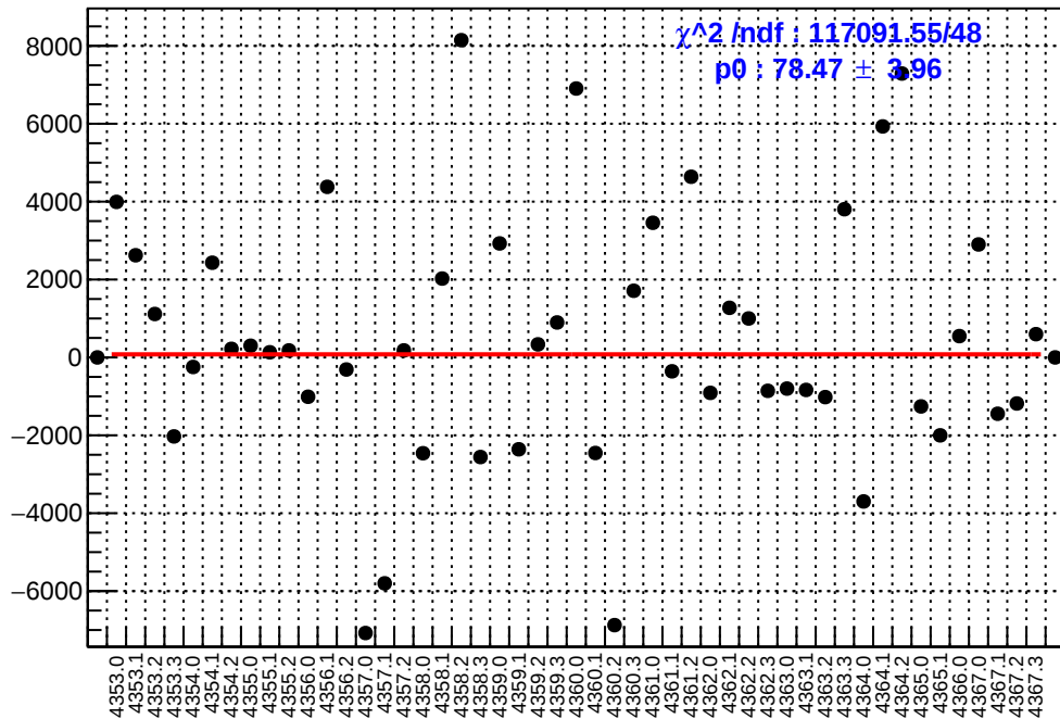
slug58: asym_ds_avg.mean/ppb-reg_asym_ds_avg.mean/ppb
