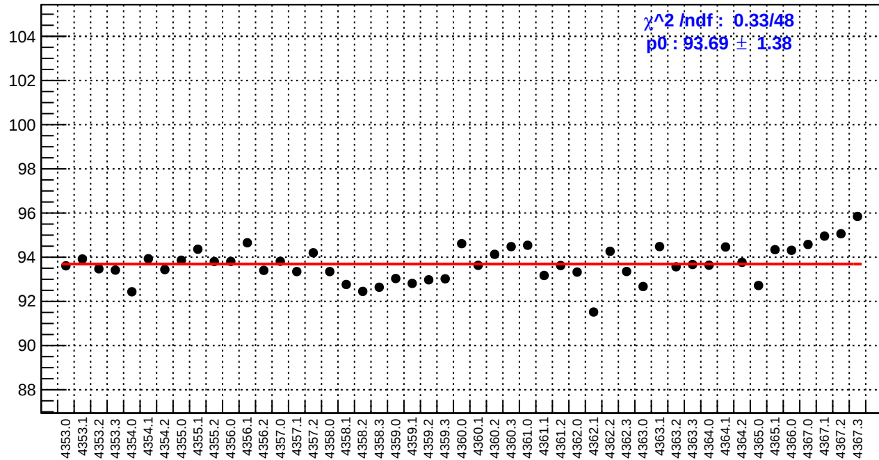
slug58: reg_asym_us_dd.rms/ppm
