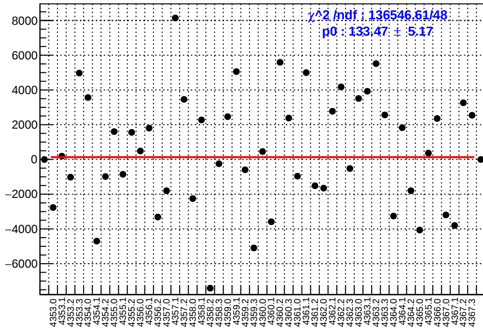
slug58: asym_sam5.mean/ppb-reg_asym_sam5.mean/ppb
