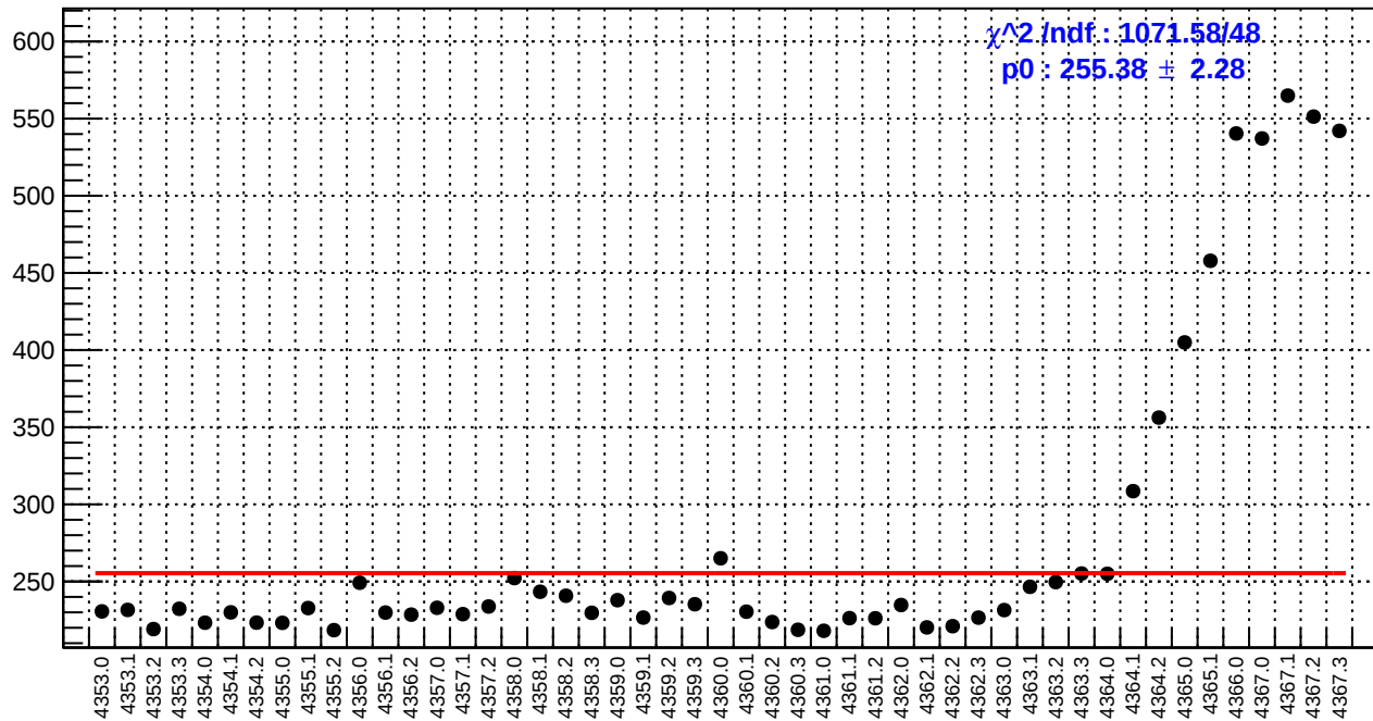
slug58: reg_asym_sam1.rms/ppm
