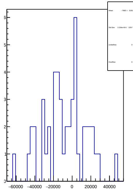
slug58: 1D Corr asym_sam6.mean/ppb-reg_asym_sam6.mean/ppb
