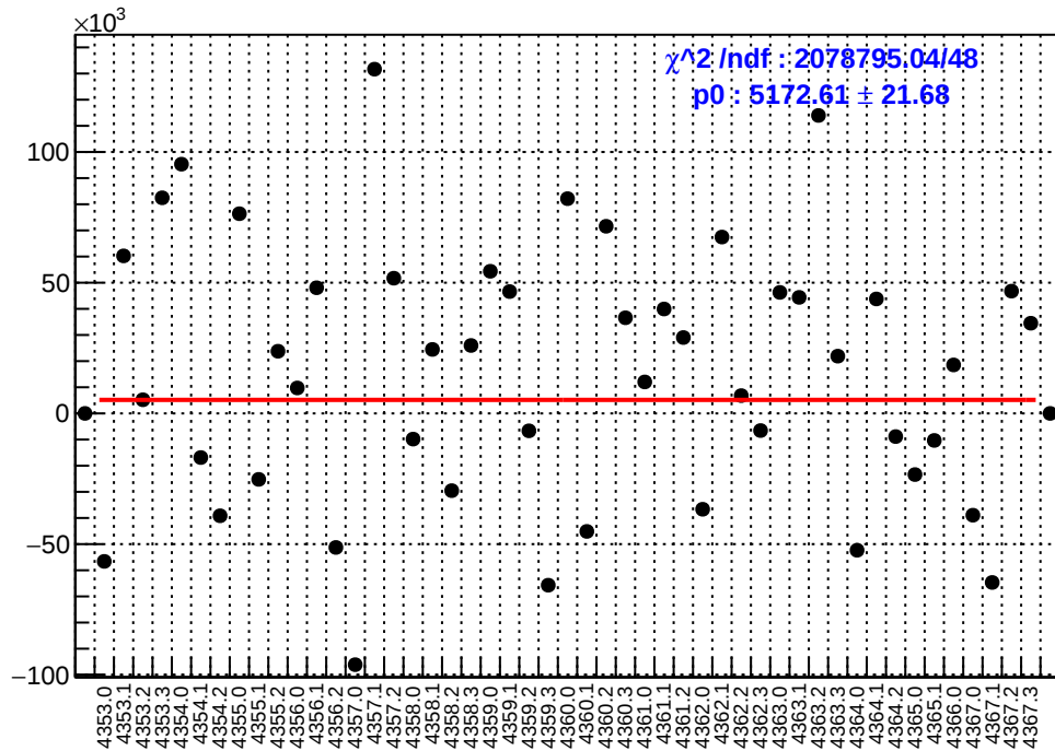
slug58: asym_sam2.mean/ppb-reg_asym_sam2.mean/ppb
