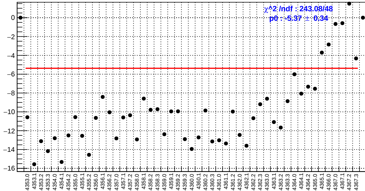
slug58: right_avg_bpm4aY/(ppb/nm)
