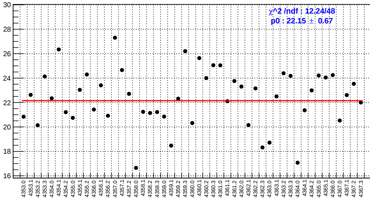
slug58: dsl_bpm4eY/(ppb/nm)
