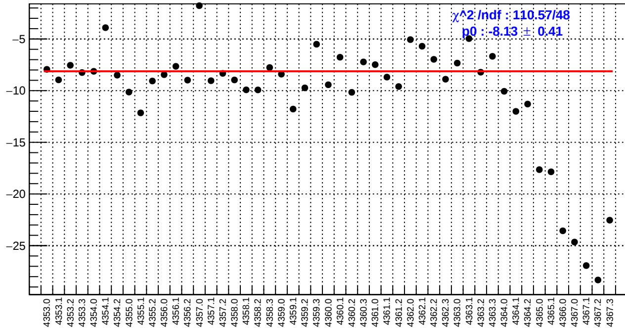
slug58: ds_avg_bpm4aX/(ppb/nm)
