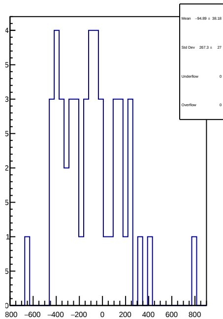
slug58: 1D Corr asym_right_dd.mean/ppb-reg_asym_right_dd.mean/ppb
