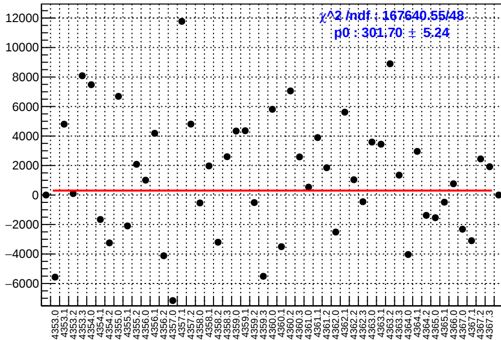
slug58: asym_us_dd.mean/ppb-reg_asym_us_dd.mean/ppb
