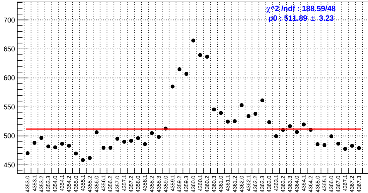
slug58: reg_asym_sam6.rms/ppm
