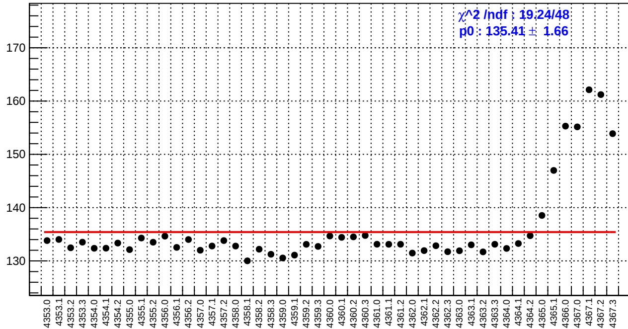
slug58: reg_asym_usr.rms/ppm
