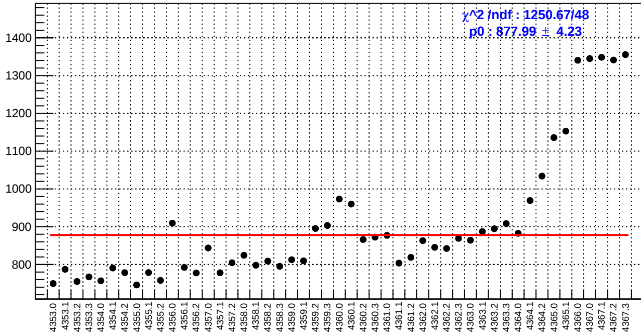
slug58: reg_asym_sam3.rms/ppm
