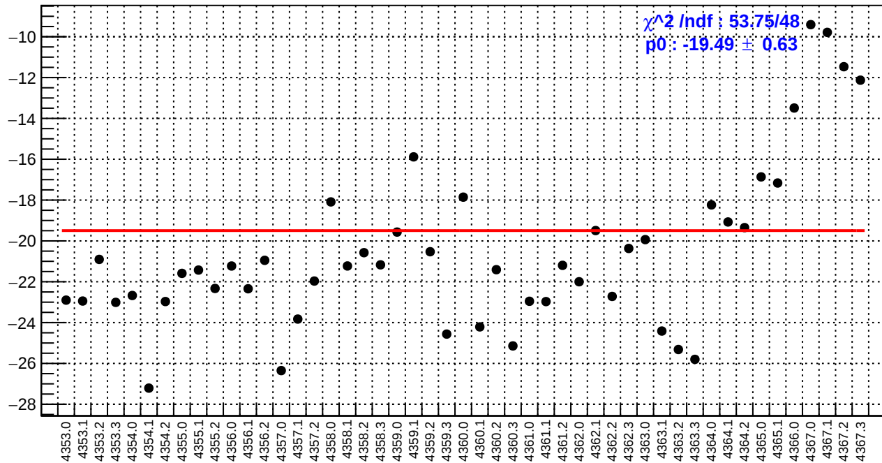
slug58: left_avg_bpm4aY/(ppb/nm)
