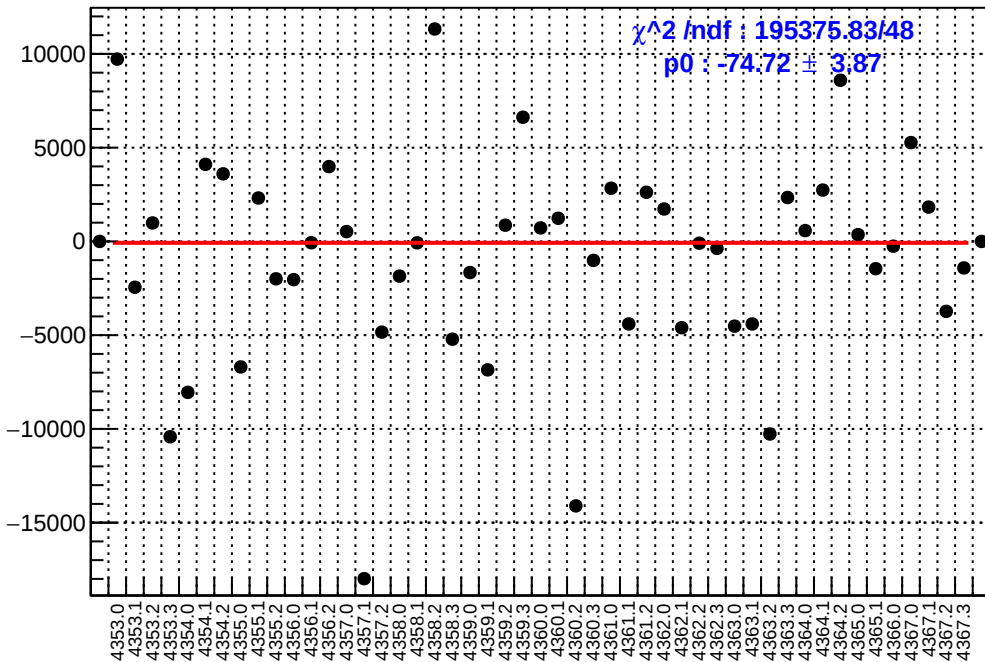
slug58: asym_right_avg.mean/ppb-reg_asym_right_avg.mean/ppb
