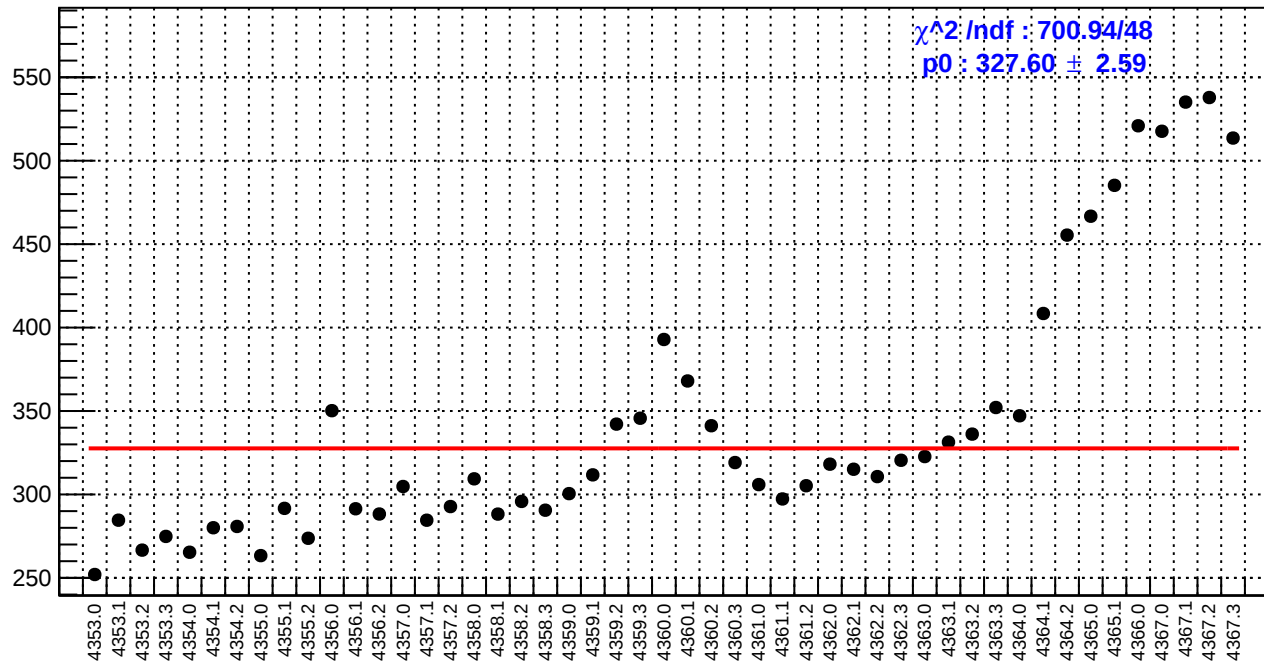
slug58: reg_asym_sam7.rms/ppm
