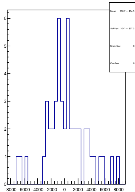
slug58: 1D Corr asym_us_avg.mean/ppb-reg_asym_us_avg.mean/ppb
