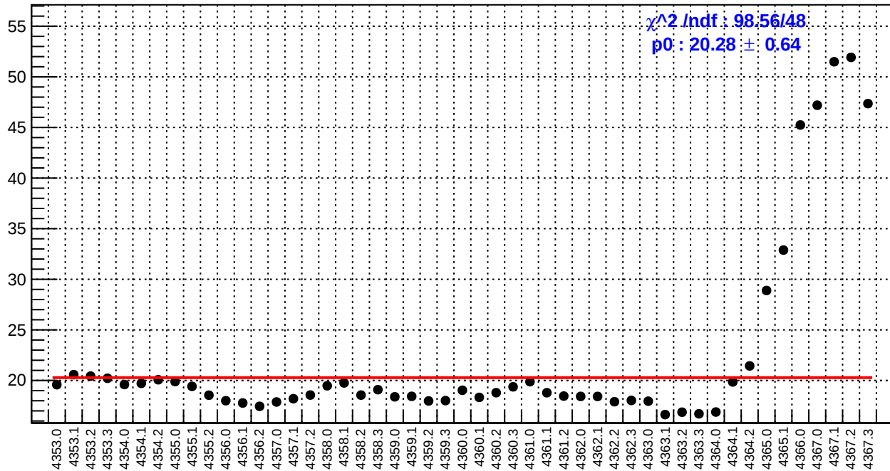
slug58: dsr_bpm4eX/(ppb/nm)
