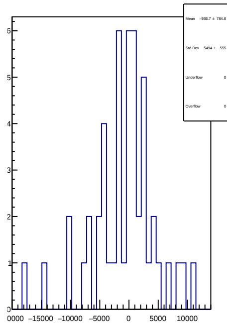
slug58: 1D Corr asym_right_avg.mean/ppb-reg_asym_right_avg.mean/ppb
