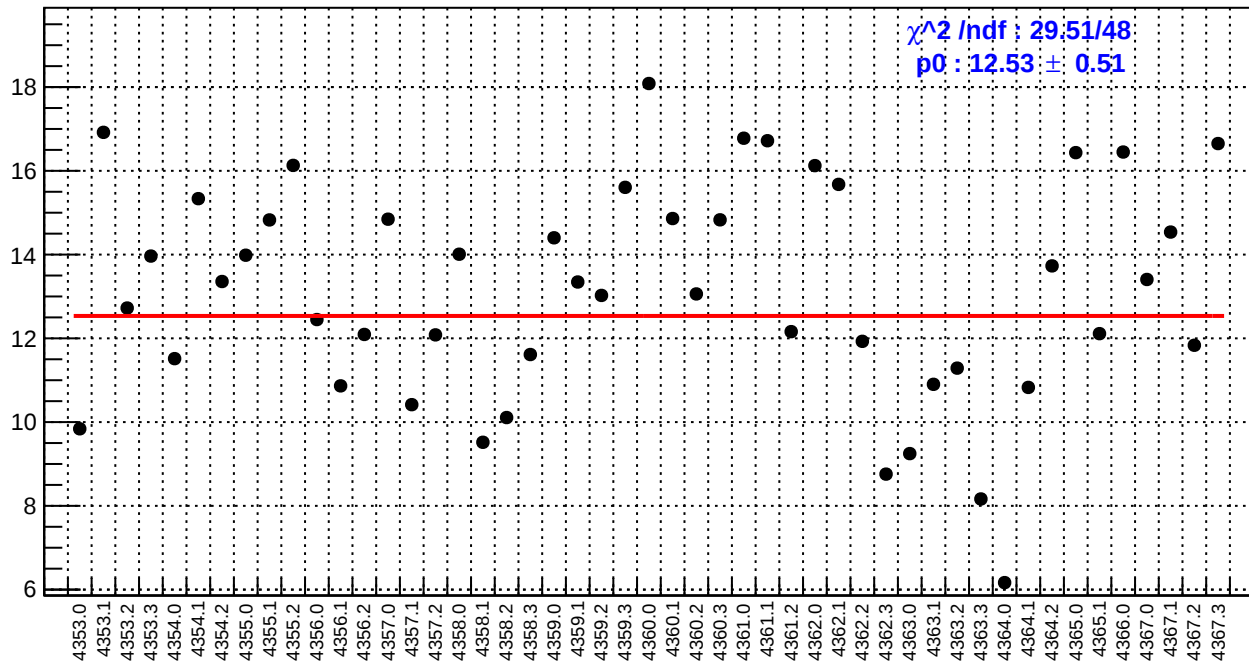
slug58: right_avg_bpm4eY/(ppb/nm)
