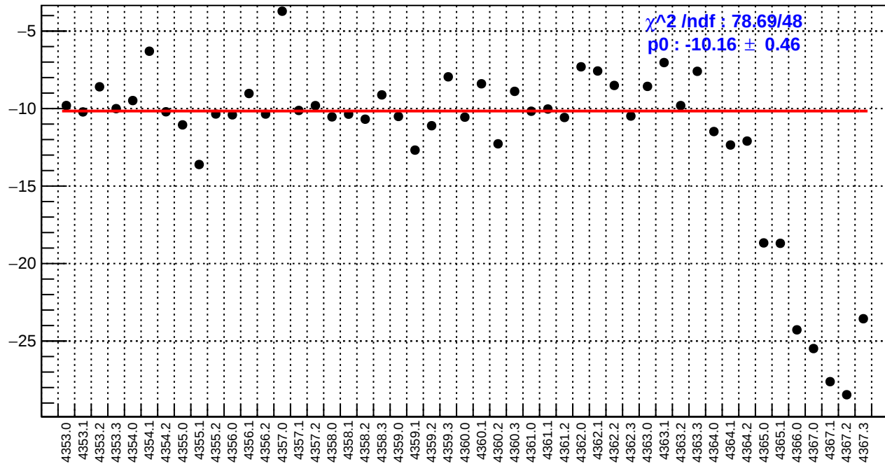
slug58: us_avg_bpm4aX/(ppb/nm)
