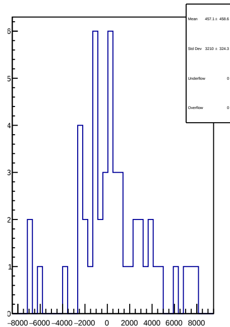
slug58: 1D Corr asym_ds_avg.mean/ppb-reg_asym_ds_avg.mean/ppb
