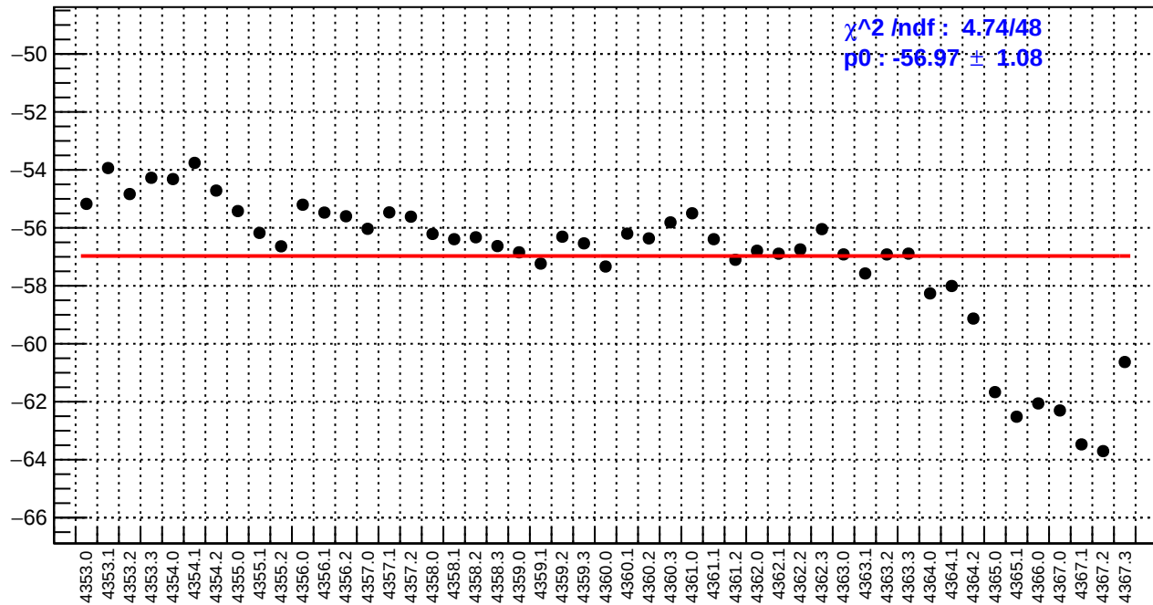
slug58: ds_avg_bpm12X/(ppb/nm)
