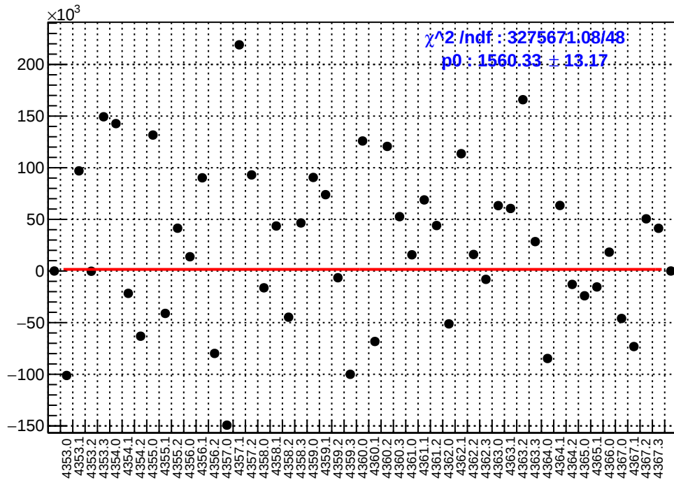
slug58: asym_sam3.mean/ppb-reg_asym_sam3.mean/ppb
