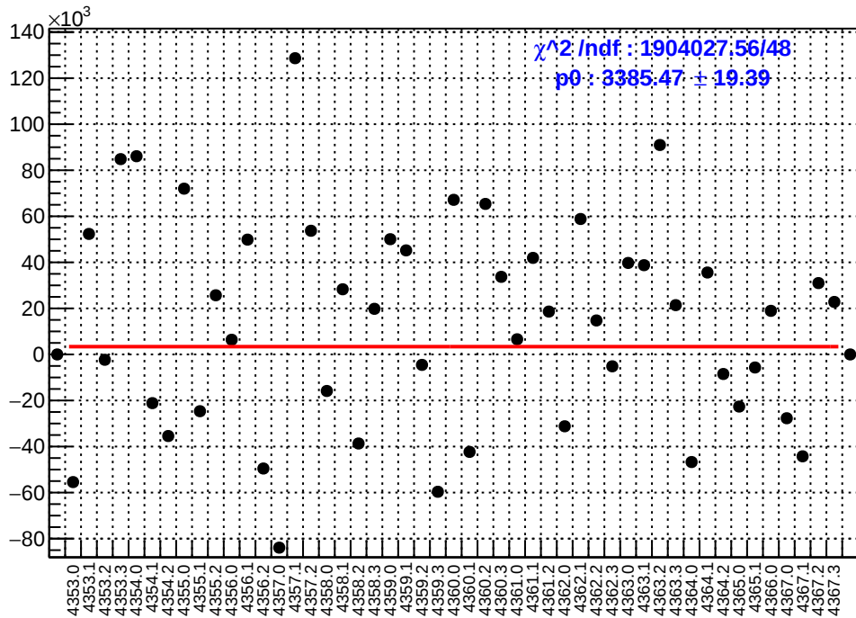
slug58: asym_sam4.mean/ppb-reg_asym_sam4.mean/ppb
