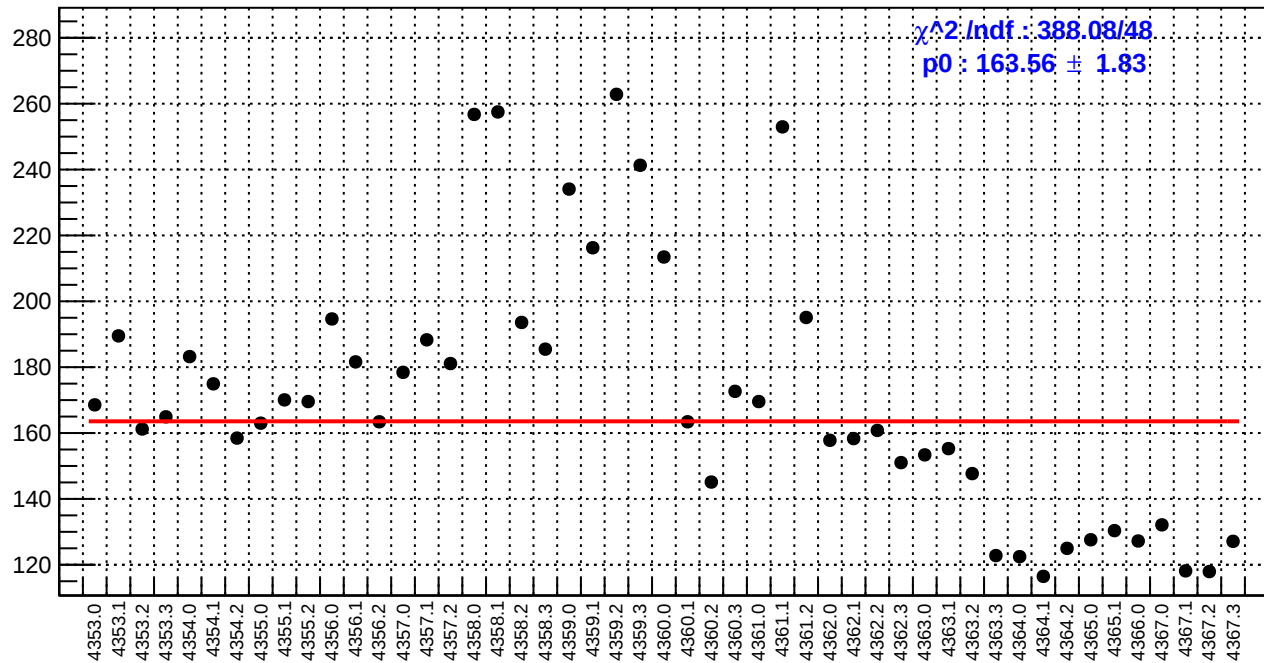
slug58: asym_bcm_an_us.rms/ppm
