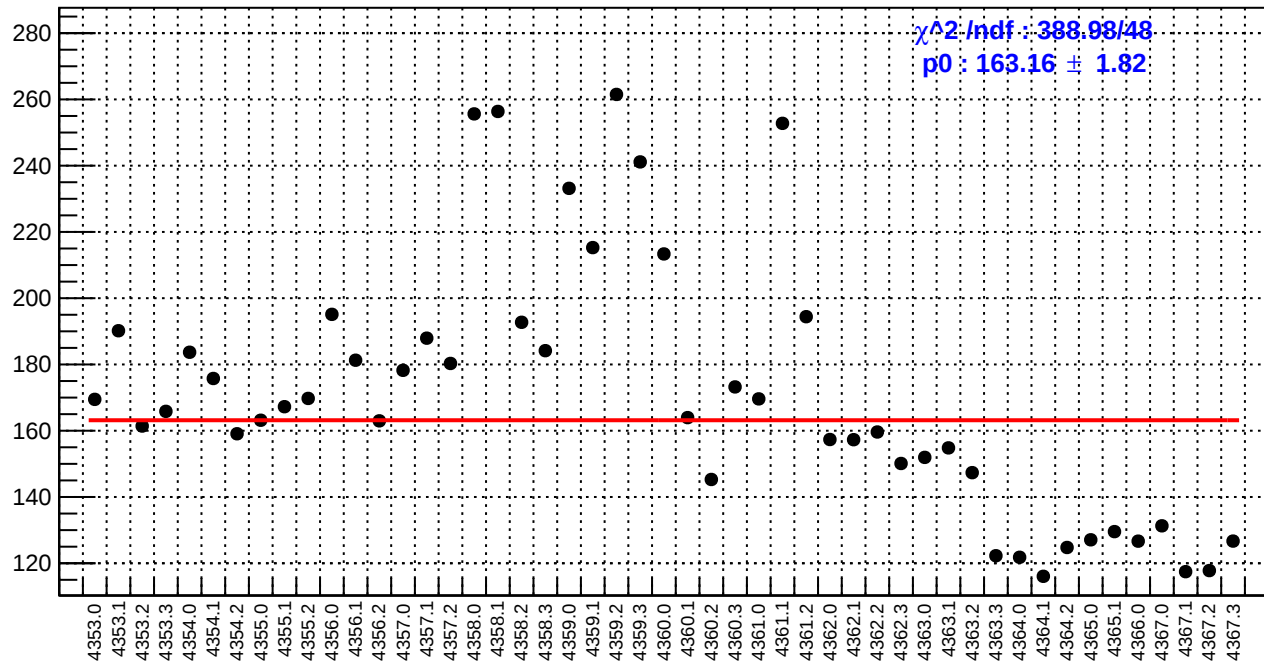
slug58: asym_bcm_an_ds.rms/ppm
