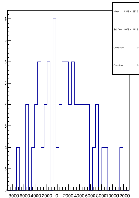
slug58: 1D Corr asym_us_dd.mean/ppb-reg_asym_us_dd.mean/ppb
