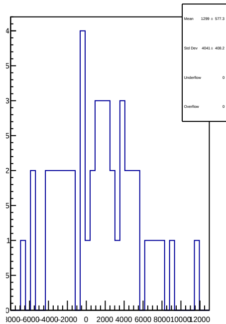
slug58: 1D Corr asym_ds_dd.mean/ppb-reg_asym_ds_dd.mean/ppb
