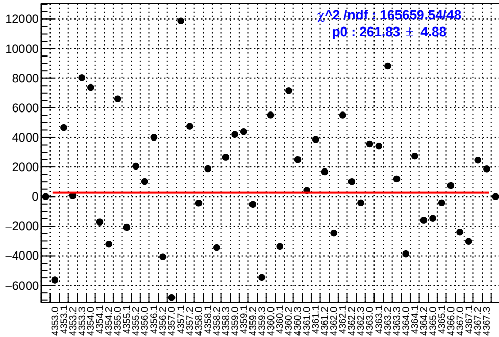
slug58: asym_ds_dd.mean/ppb-reg_asym_ds_dd.mean/ppb
