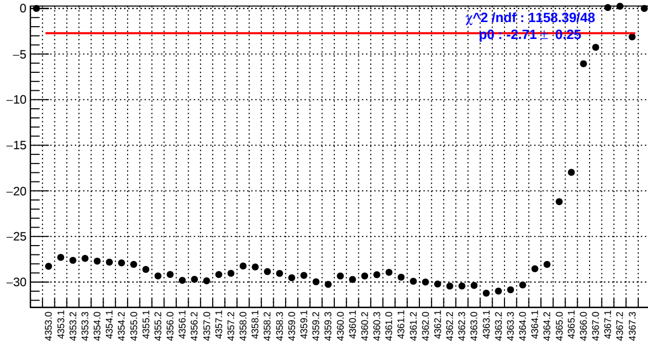
slug58: ds_avg_bpm4eX/(ppb/nm)
