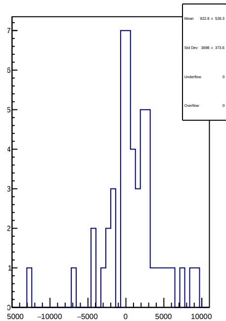
slug58: 1D Corr asym_sam1.mean/ppb-reg_asym_sam1.mean/ppb
