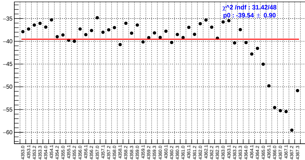
slug58: dsr_bpm4aX/(ppb/nm)
