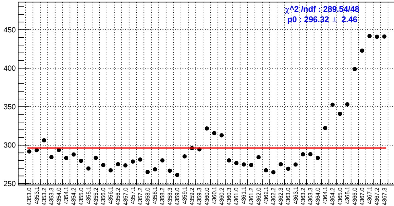
slug58: reg_asym_sam5.rms/ppm
