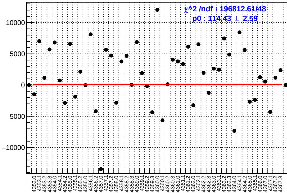
slug58: asym_left_avg.mean/ppb-reg_asym_left_avg.mean/ppb
