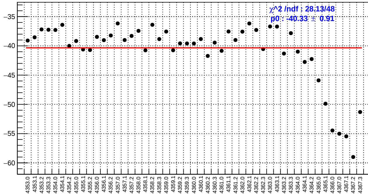
slug58: right_avg_bpm4aX/(ppb/nm)
