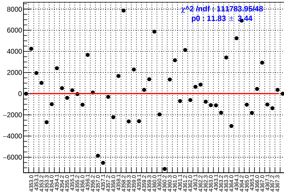
slug58: asym_us_avg.mean/ppb-reg_asym_us_avg.mean/ppb
