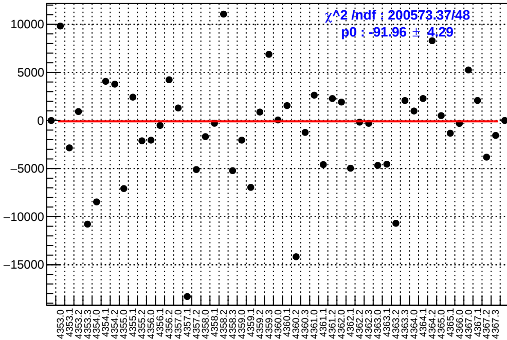
slug58: asym_usr.mean/ppb-reg_asym_usr.mean/ppb
