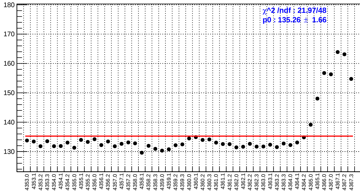
slug58: reg_asym_right_avg.rms/ppm
