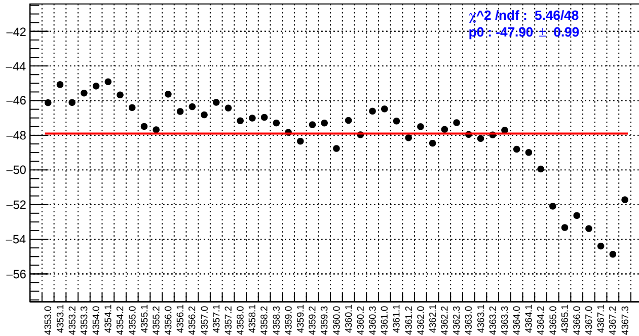
slug58: left_avg_bpm12X/(ppb/nm)
