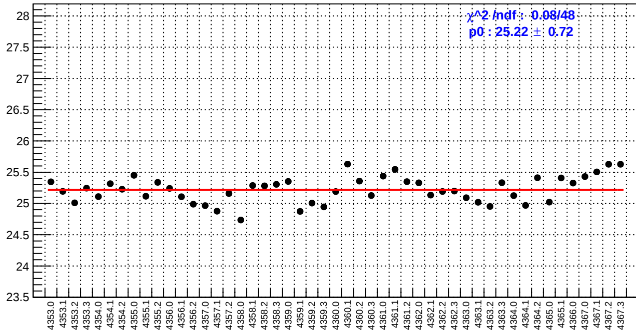
slug58: reg_asym_left_dd.rms/ppm
