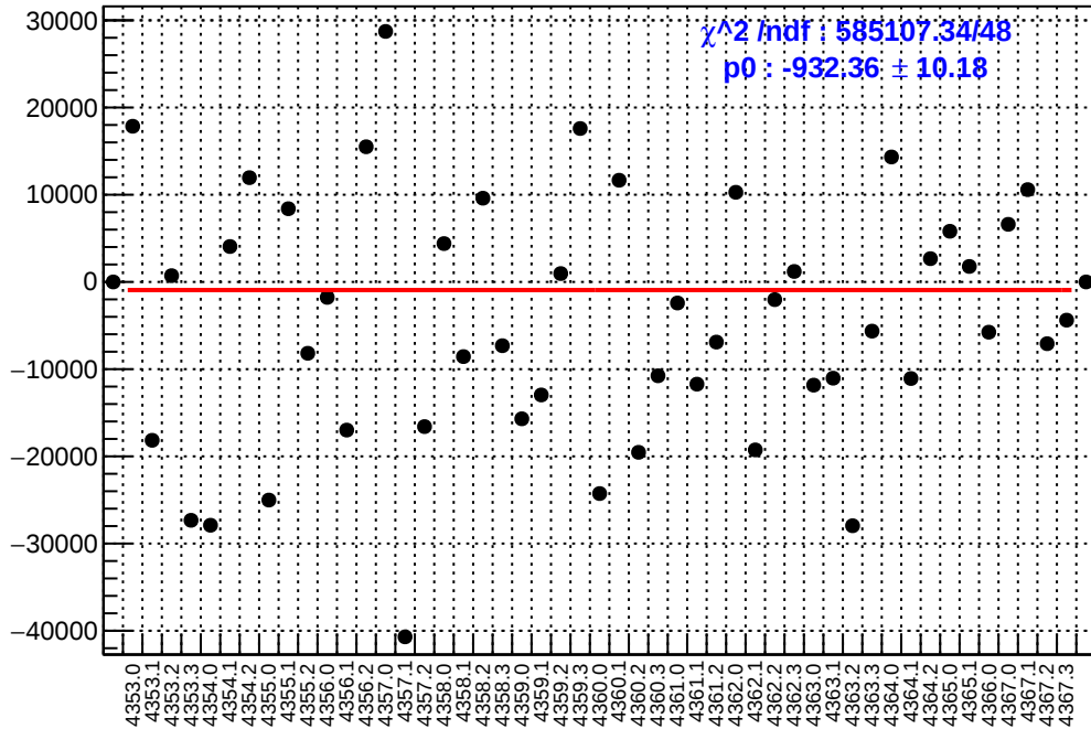
slug58: asym_sam7.mean/ppb-reg_asym_sam7.mean/ppb
