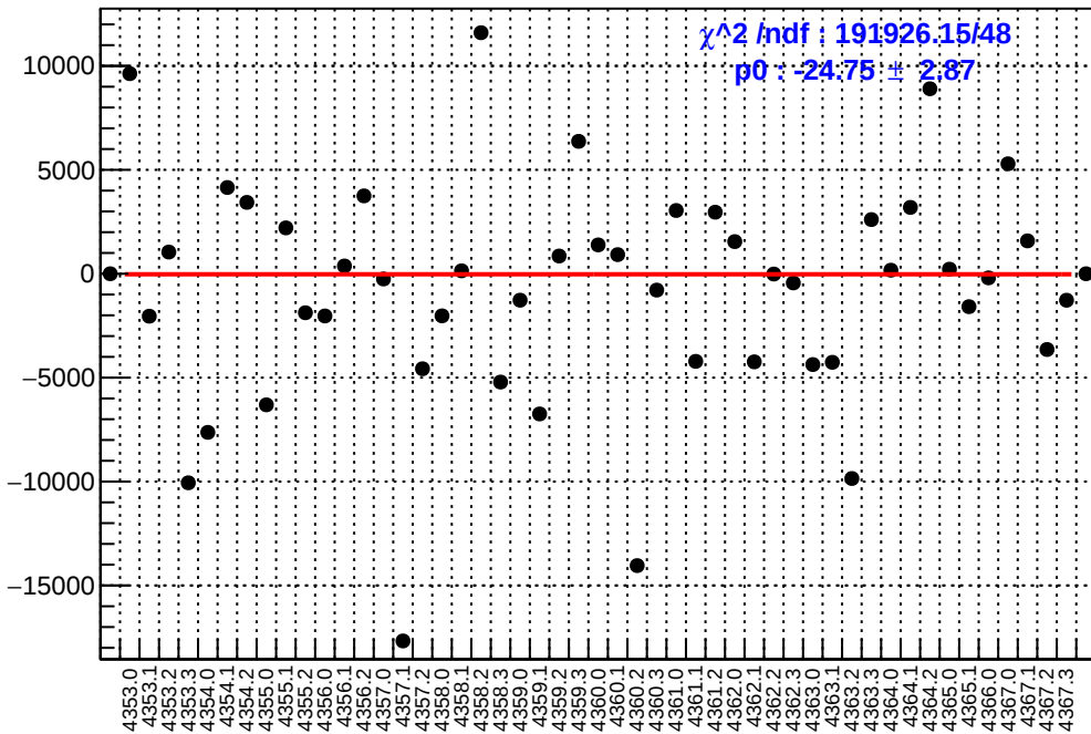
slug58: asym_dsr.mean/ppb-reg_asym_dsr.mean/ppb
