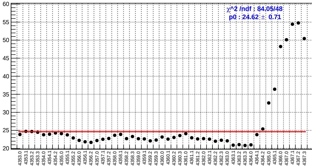
slug58: right_avg_bpm4eX/(ppb/nm)
