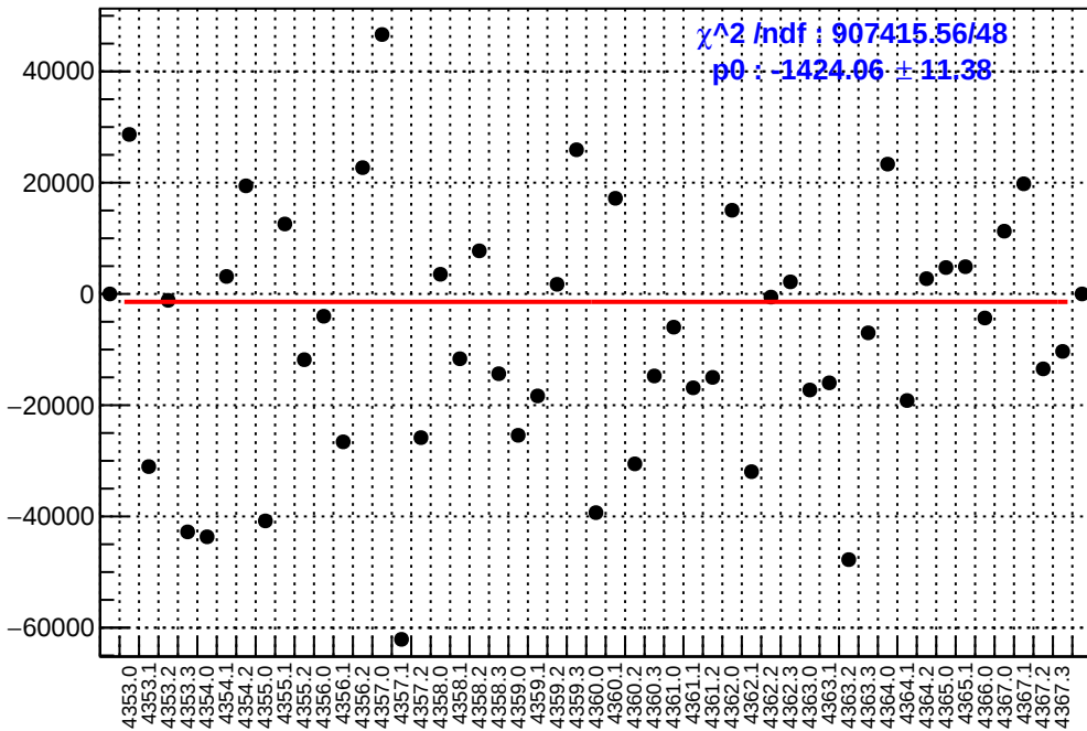
slug58: asym_sam6.mean/ppb-reg_asym_sam6.mean/ppb
