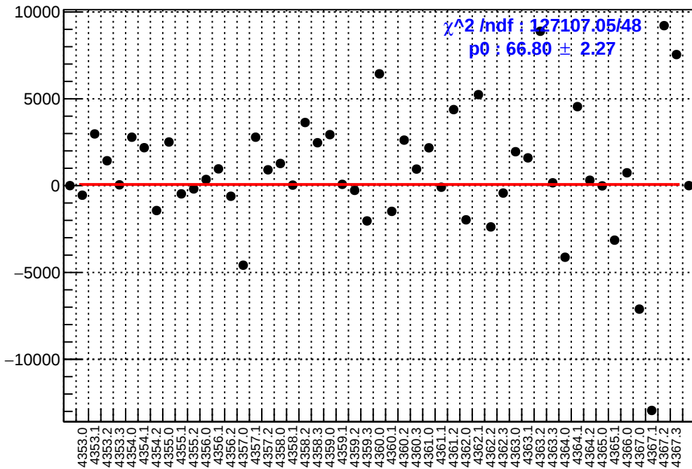
slug58: asym_sam1.mean/ppb-reg_asym_sam1.mean/ppb
