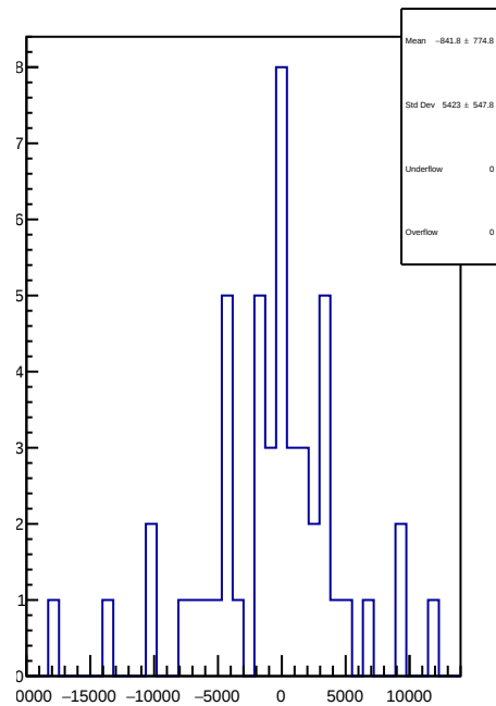
slug58: 1D Corr asym_dsr.mean/ppb-reg_asym_dsr.mean/ppb
