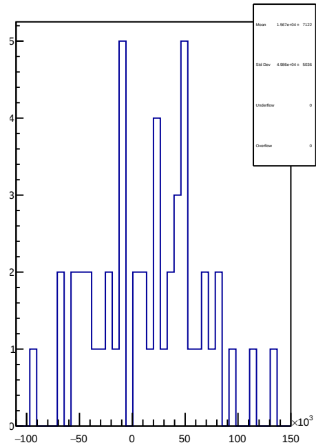
slug58: 1D Corr asym_sam2.mean/ppb-reg_asym_sam2.mean/ppb
