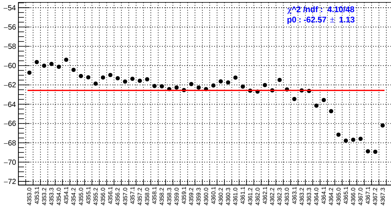
slug58: right_avg_bpm12X/(ppb/nm)
