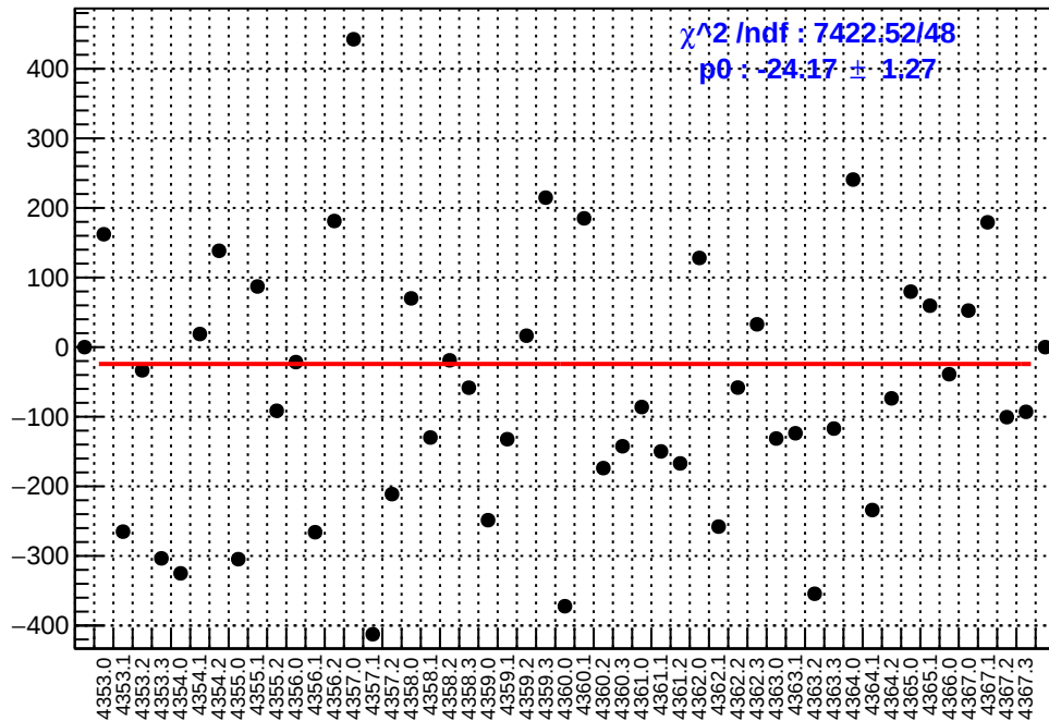
slug58: asym_left_dd.mean/ppb-reg_asym_left_dd.mean/ppb
