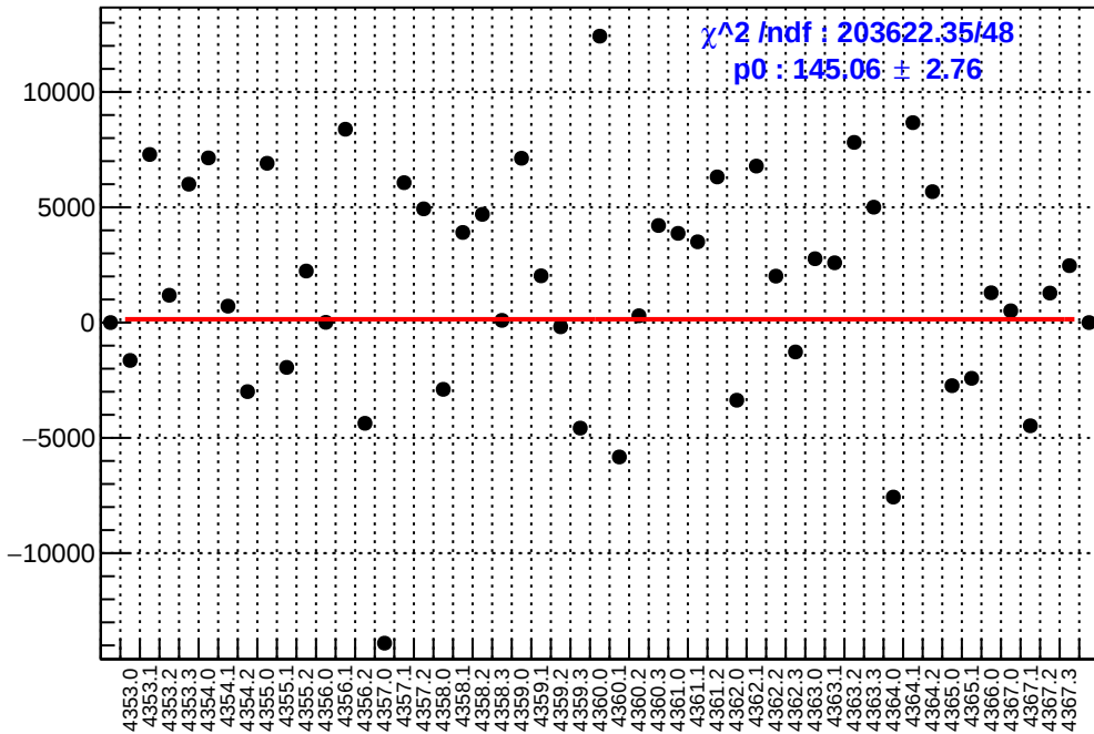
slug58: asym_dsl.mean/ppb-reg_asym_dsl.mean/ppb
