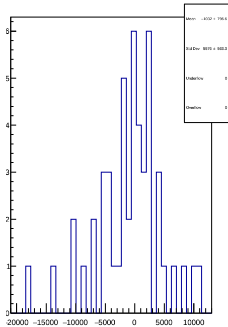
slug58: 1D Corr asym_usr.mean/ppb-reg_asym_usr.mean/ppb
