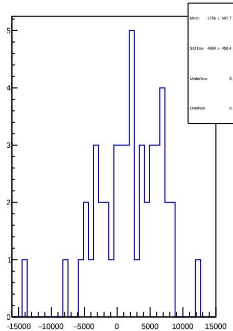
slug58: 1D Corr asym_dsl.mean/ppb-reg_asym_dsl.mean/ppb
