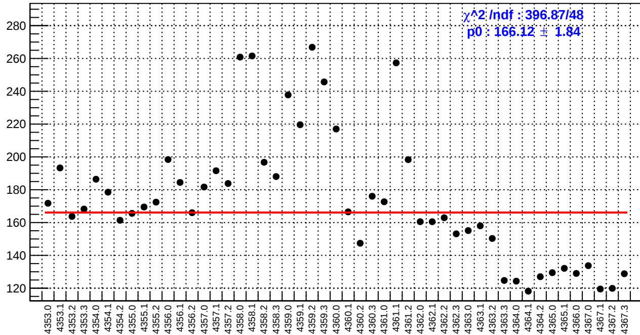
slug58: asym_bcm_an_ds3.rms/ppm
