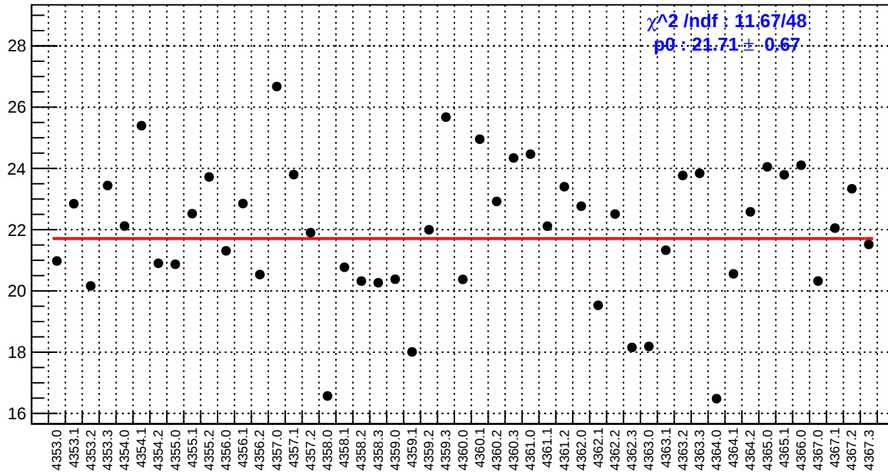
slug58: left_avg_bpm4eY/(ppb/nm)
