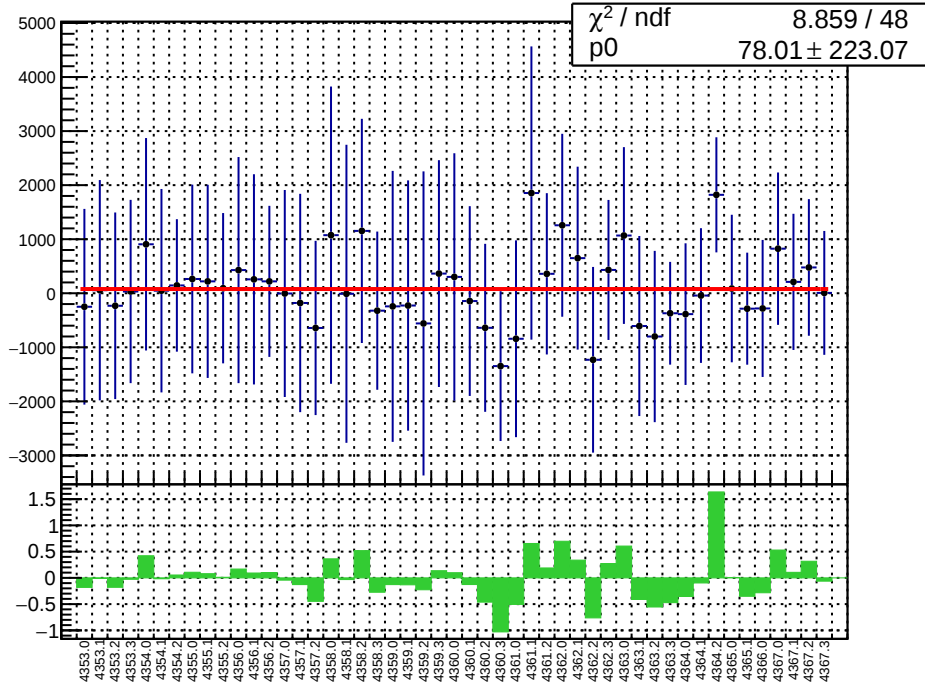
slug58: asym_bcm_an_ds3.mean/ppb
