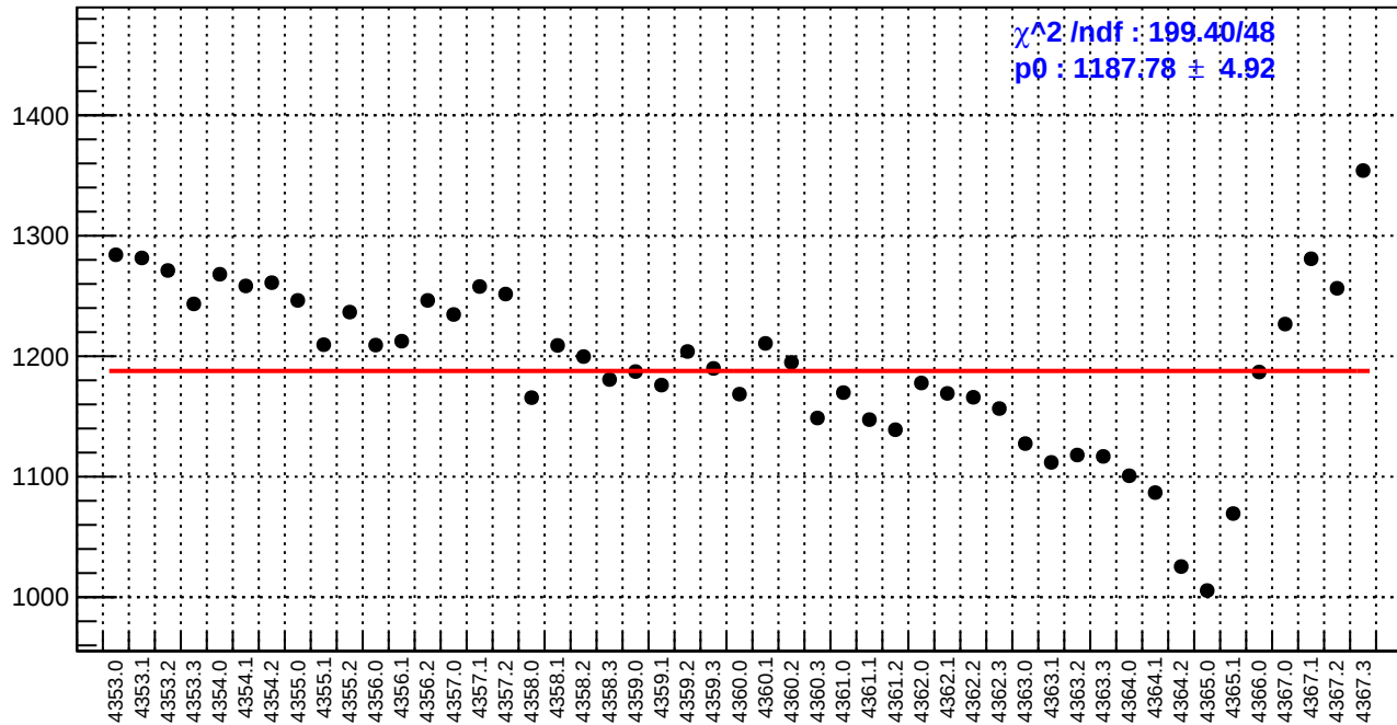
slug58: reg_asym_sam4.rms/ppm
