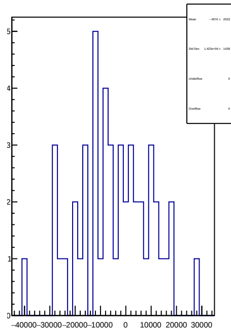
slug58: 1D Corr asym_sam7.mean/ppb-reg_asym_sam7.mean/ppb
