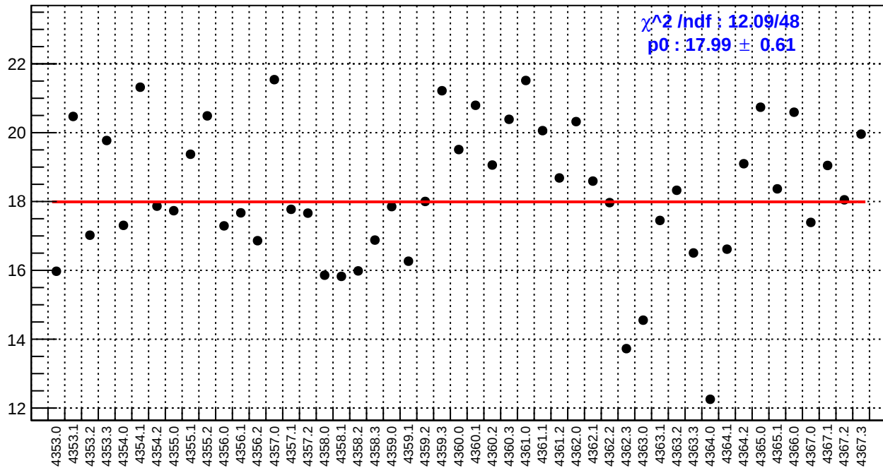
slug58: ds_avg_bpm4eY/(ppb/nm)
