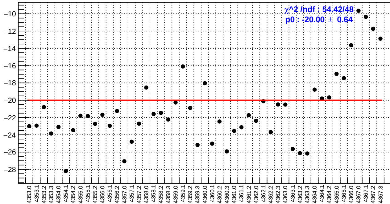
slug58: dsl_bpm4aY/(ppb/nm)
