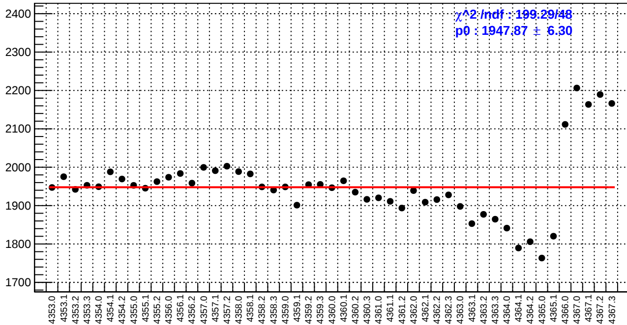
slug58: reg_asym_sam2.rms/ppm
