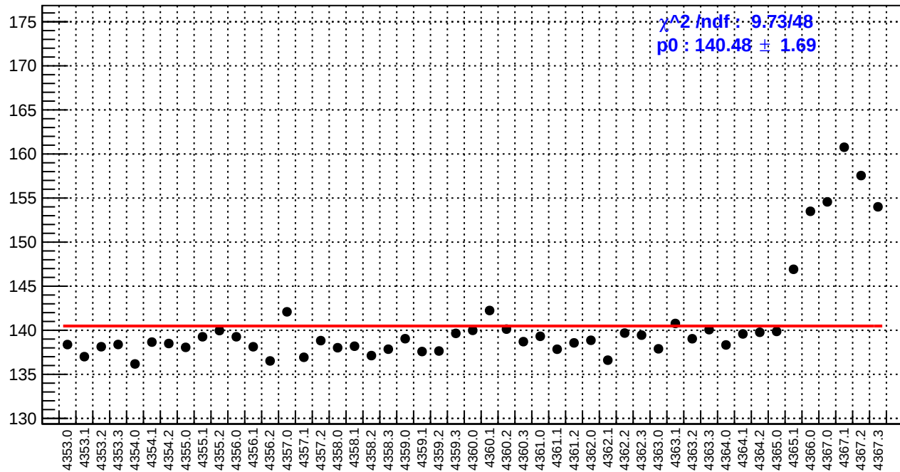
slug58: reg_asym_usl.rms/ppm
