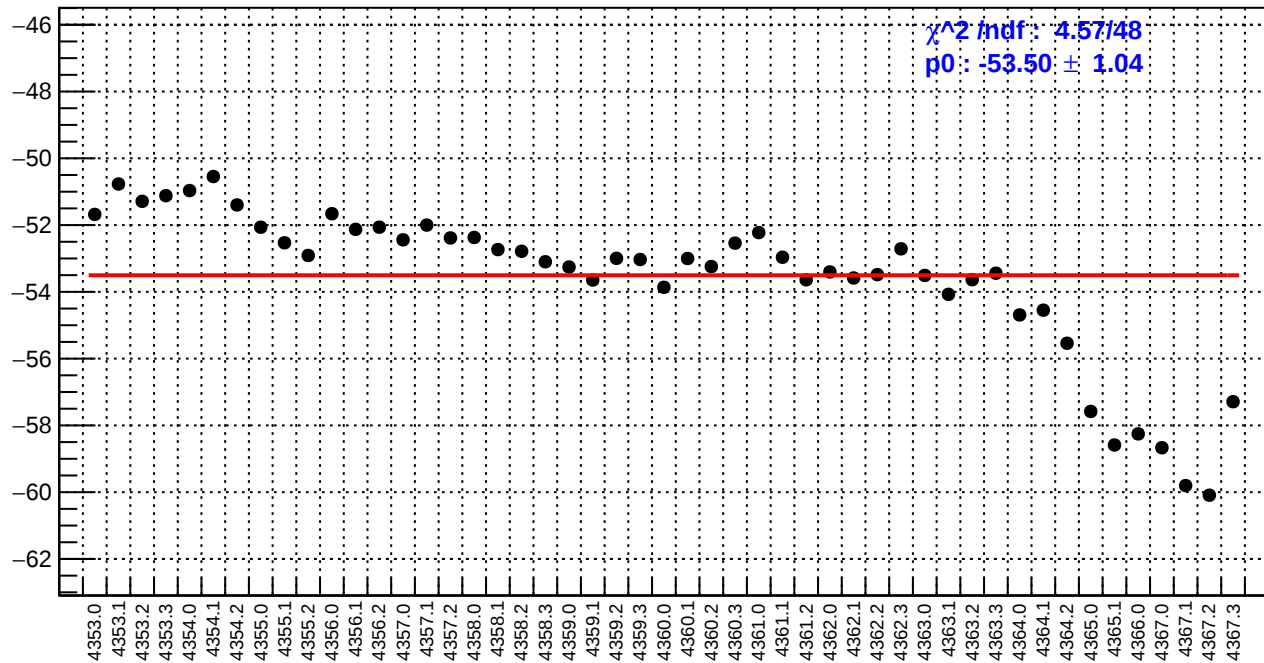
slug58: us_avg_bpm12X/(ppb/nm)
