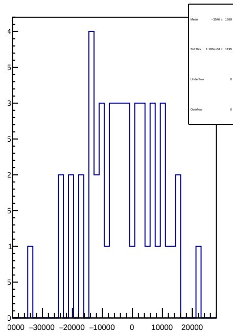
slug58: 1D Corr asym_sam8.mean/ppb-reg_asym_sam8.mean/ppb
