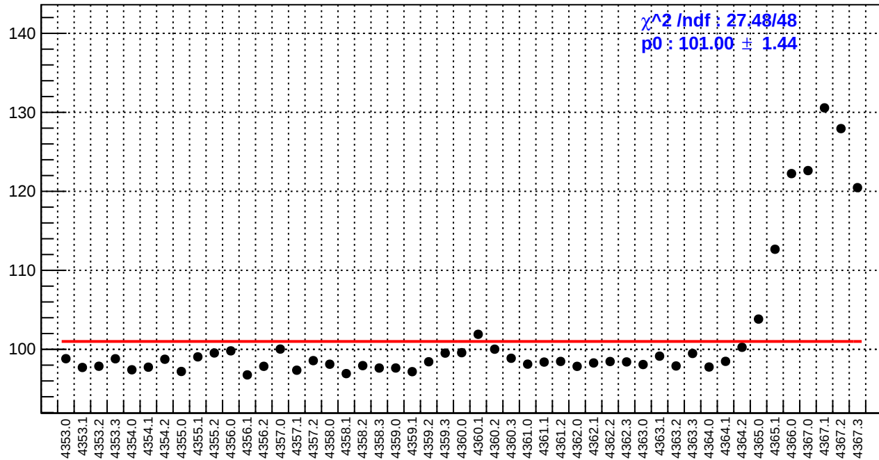
slug58: reg_asym_us_avg.rms/ppm
