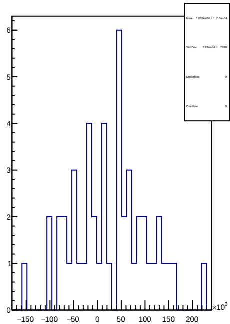
slug58: 1D Corr asym_sam3.mean/ppb-reg_asym_sam3.mean/ppb
