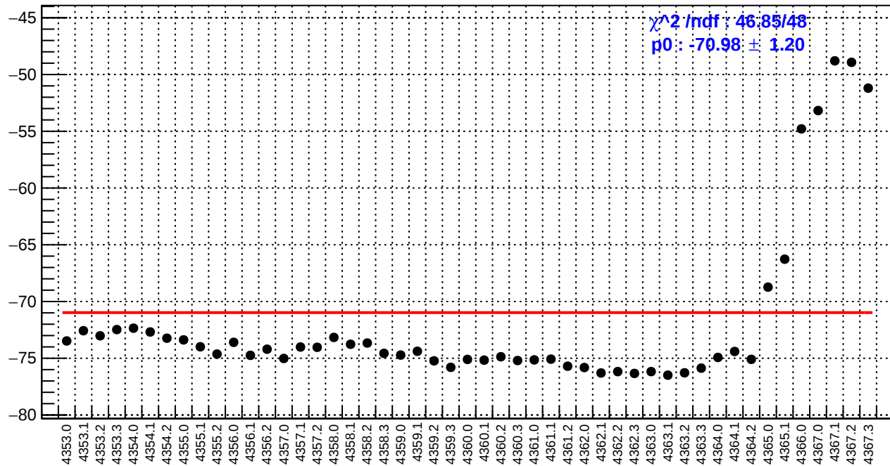
slug58: left_avg_bpm4eX/(ppb/nm)
