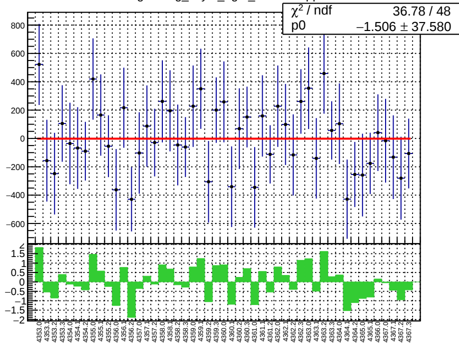
slug58: reg_asym_right_dd.mean/ppb
