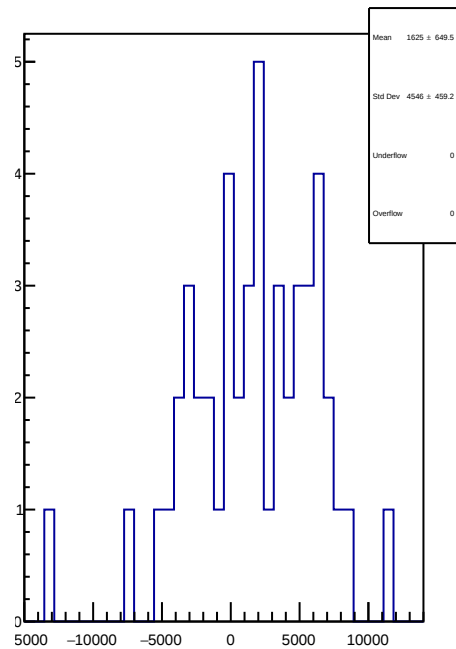
slug58: 1D Corr asym_usl.mean/ppb-reg_asym_usl.mean/ppb
