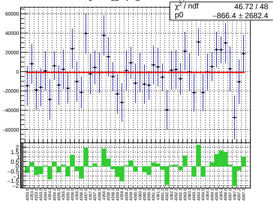
slug58: reg_asym_sam2.mean/ppb
