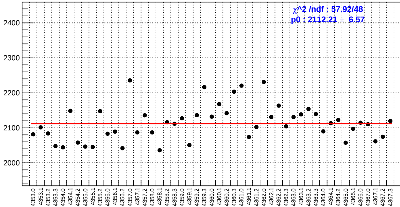
slug58: diff_bpm4aY.rms/nm
