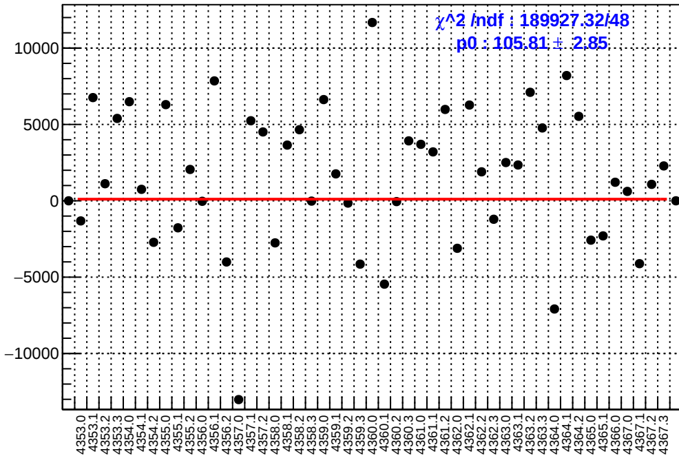
slug58: asym_usl.mean/ppb-reg_asym_usl.mean/ppb
