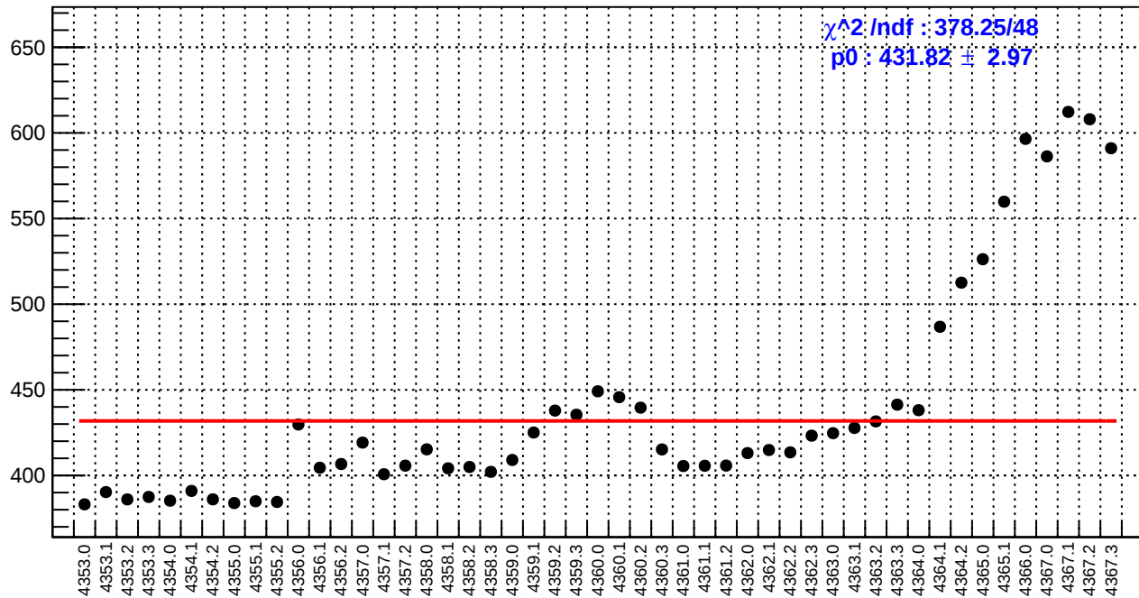
slug58: reg_asym_sam8.rms/ppm
