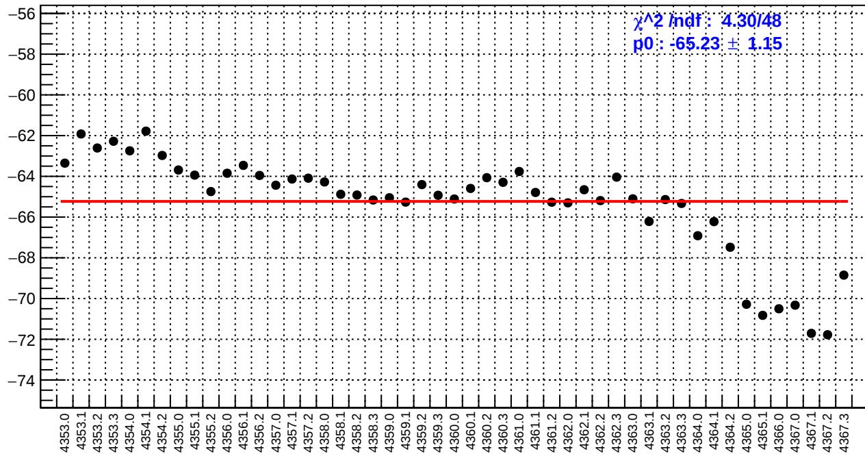
slug58: dsr_bpm12X/(ppb/nm)
