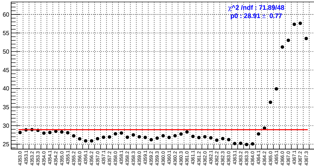
slug58: usr_bpm4eX/(ppb/nm)
