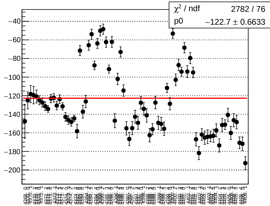
reg_asym_sam_15_dd_diff_bpm4eY_slope vs run
