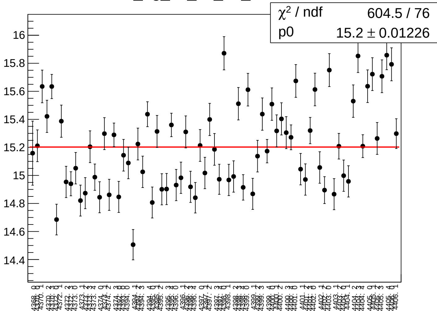
bcm_dg_ds_ds_dd_rms vs run
