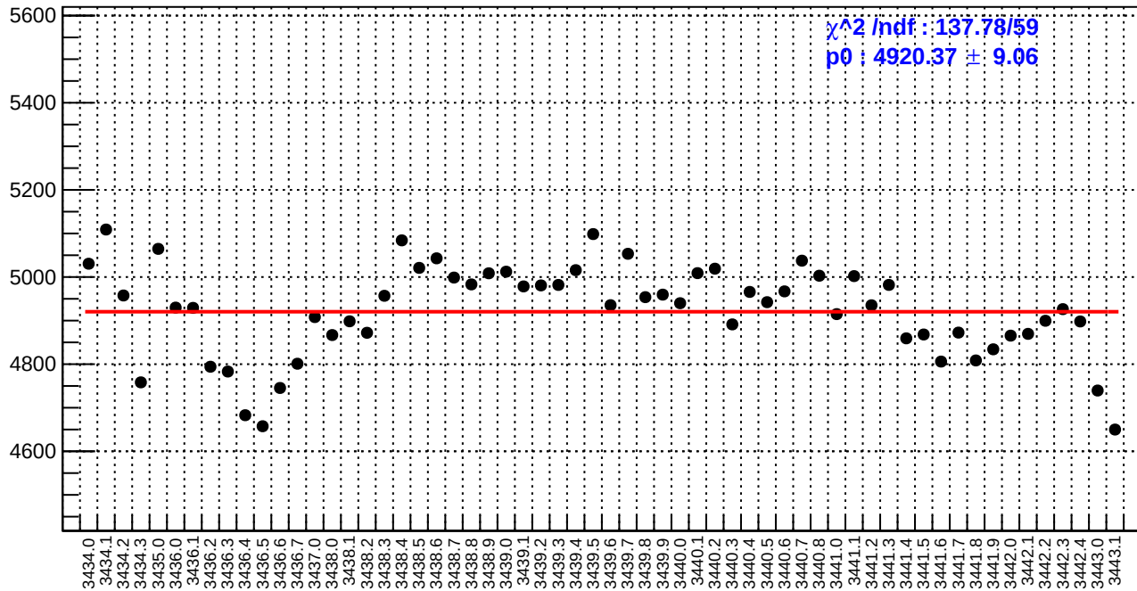
slug6: diff_bpm12X.rms/nm
