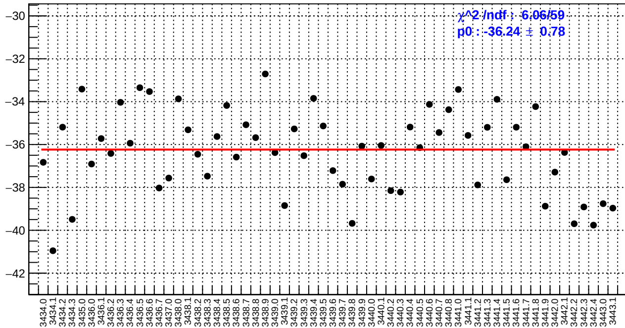
slug6: dsl_bpm4aY/(ppb/nm)
