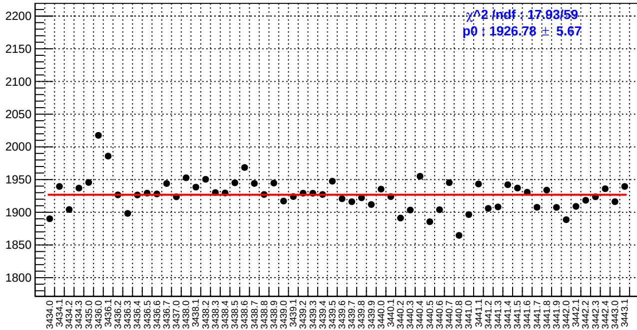
slug6: reg_asym_sam2.rms/ppm
