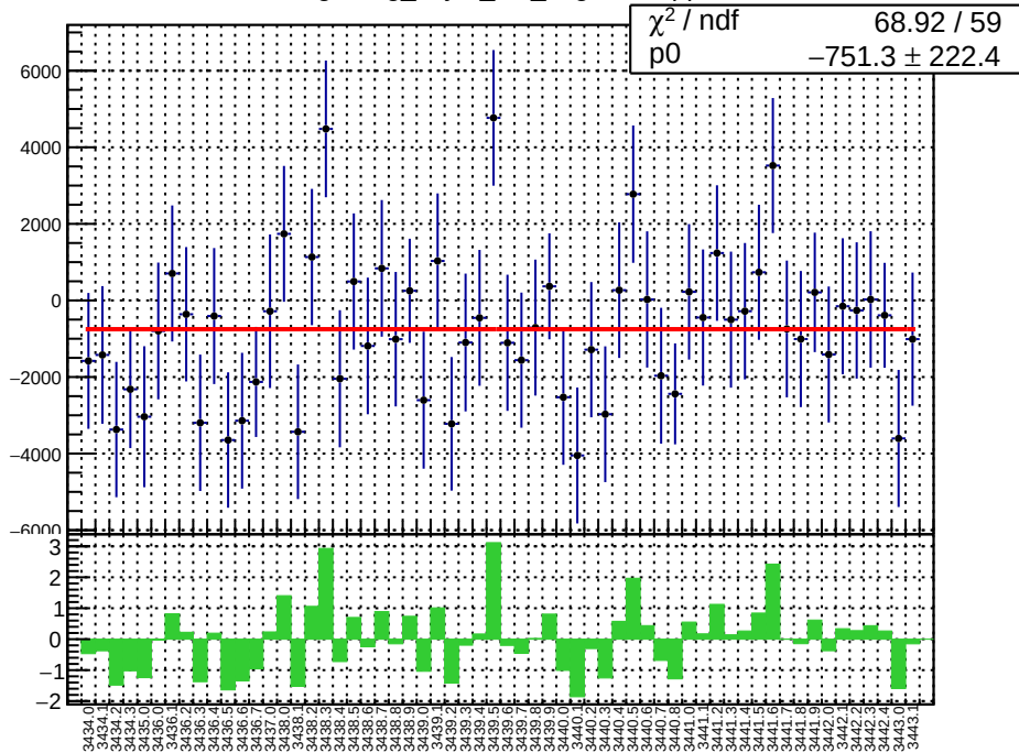
slug6: reg_asym_left_avg.mean/ppb
