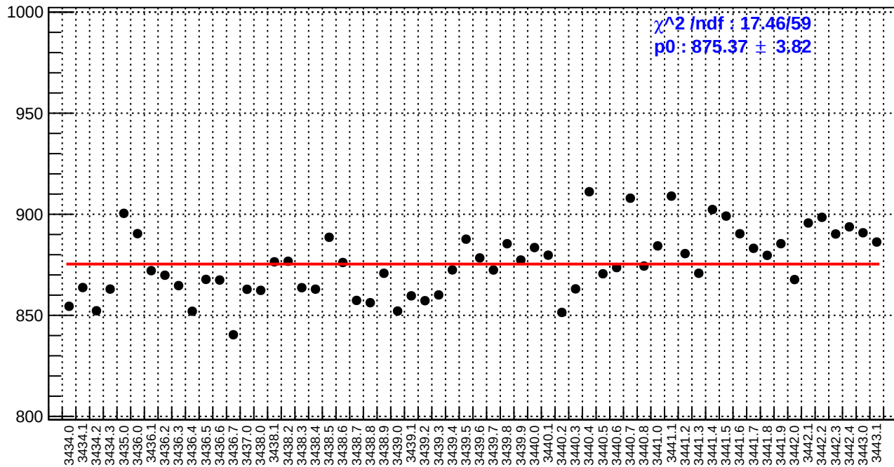
slug6: reg_asym_sam6.rms/ppm
