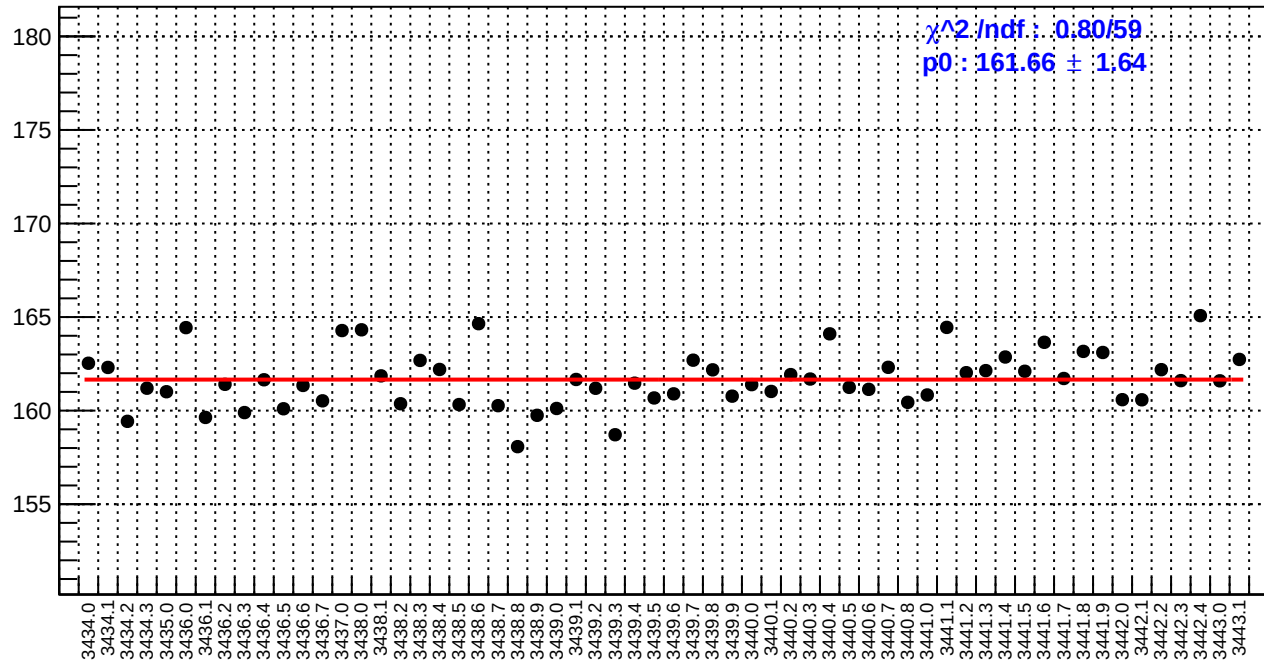
slug6: reg_asym_right_avg.rms/ppm
