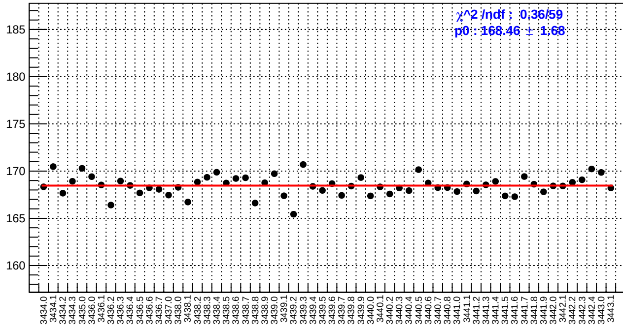
slug6: reg_asym_left_avg.rms/ppm
