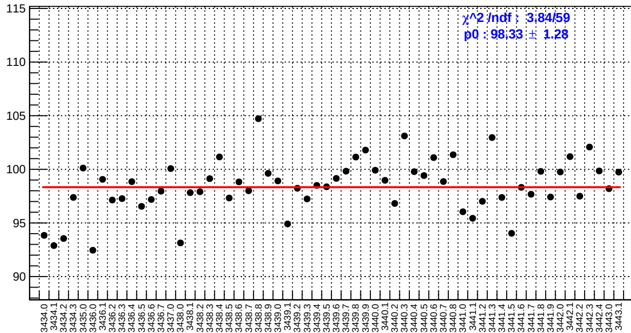
slug6: ds_avg_bpm4aX/(ppb/nm)
