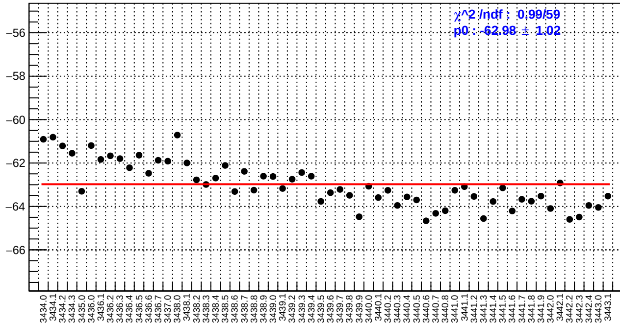
slug6: dsr_bpm12X/(ppb/nm)
