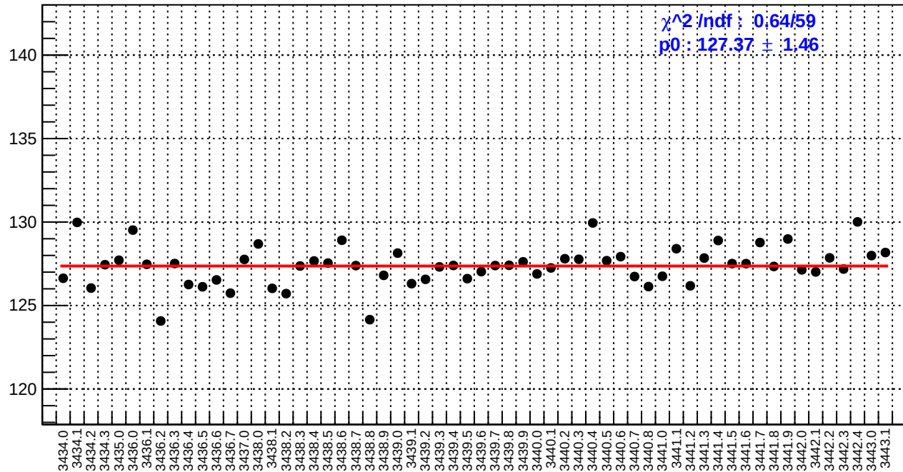
slug6: reg_asym_ds_avg.rms/ppm
