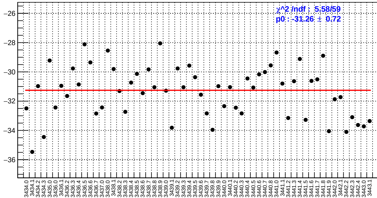
slug6: usl_bpm4aY/(ppb/nm)
