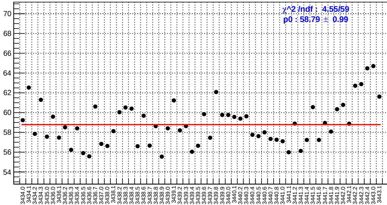
slug6: left_avg_bpm4eY/(ppb/nm)
