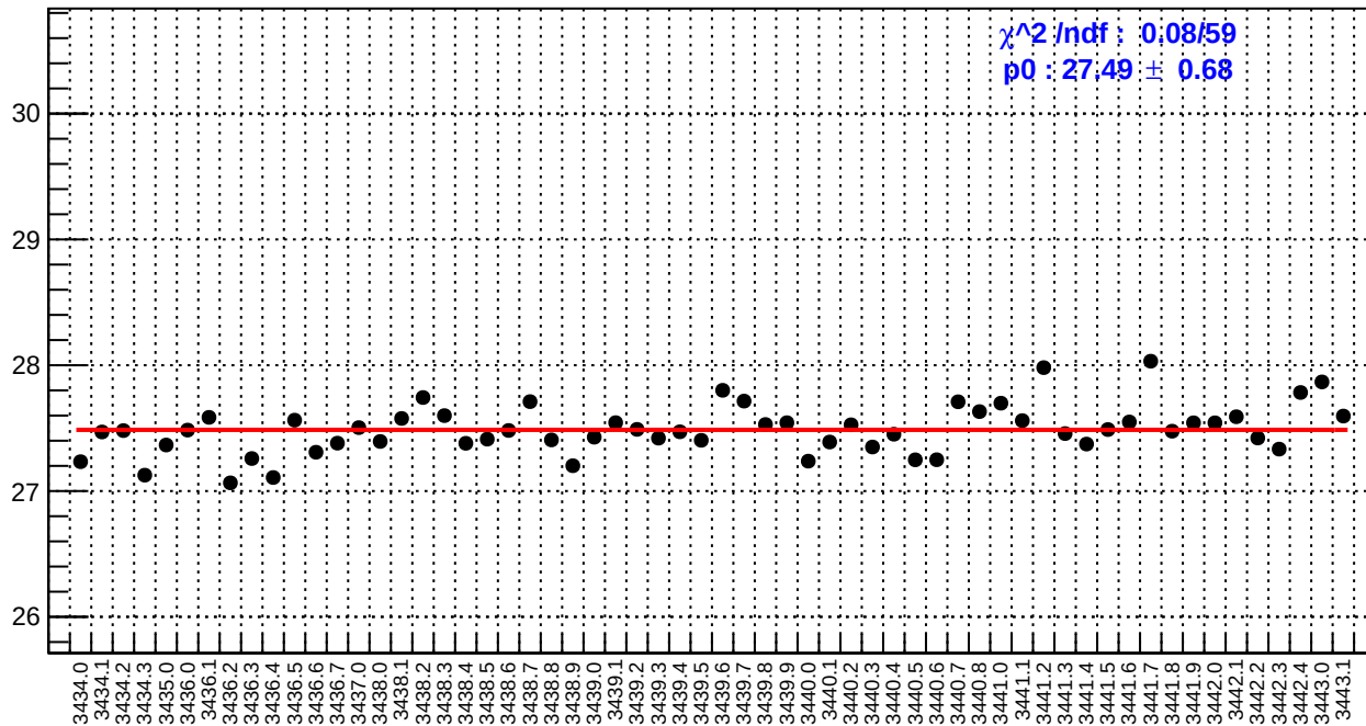
slug6: reg_asym_right_dd.rms/ppm
