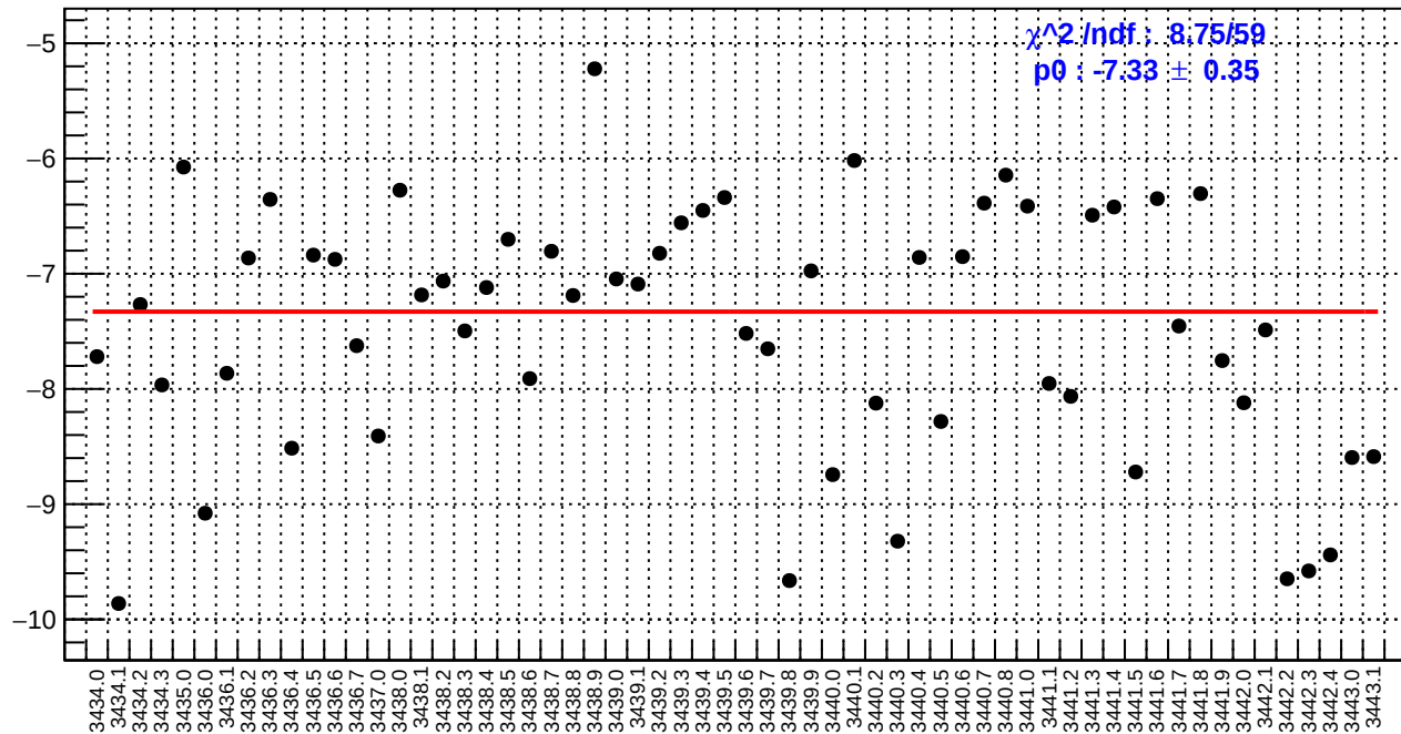
slug6: ds_avg_bpm4aY/(ppb/nm)
