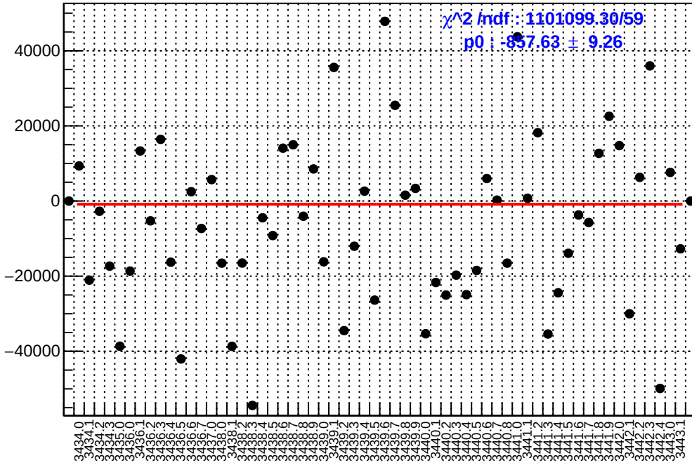
slug6: asym_sam7.mean/ppb-reg_asym_sam7.mean/ppb
