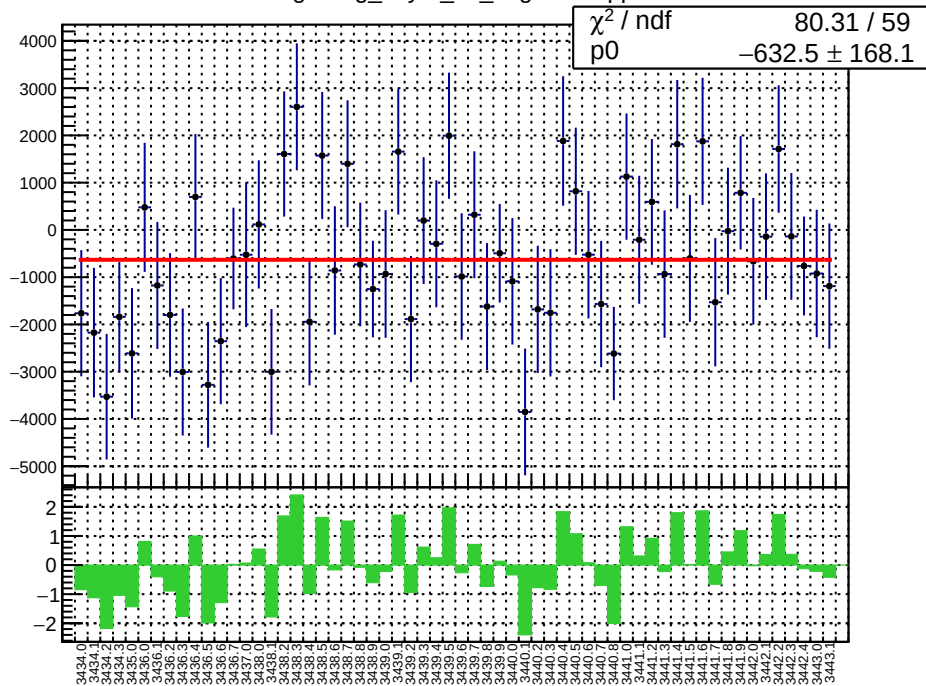
slug6: reg_asym_ds_avg.mean/ppb
