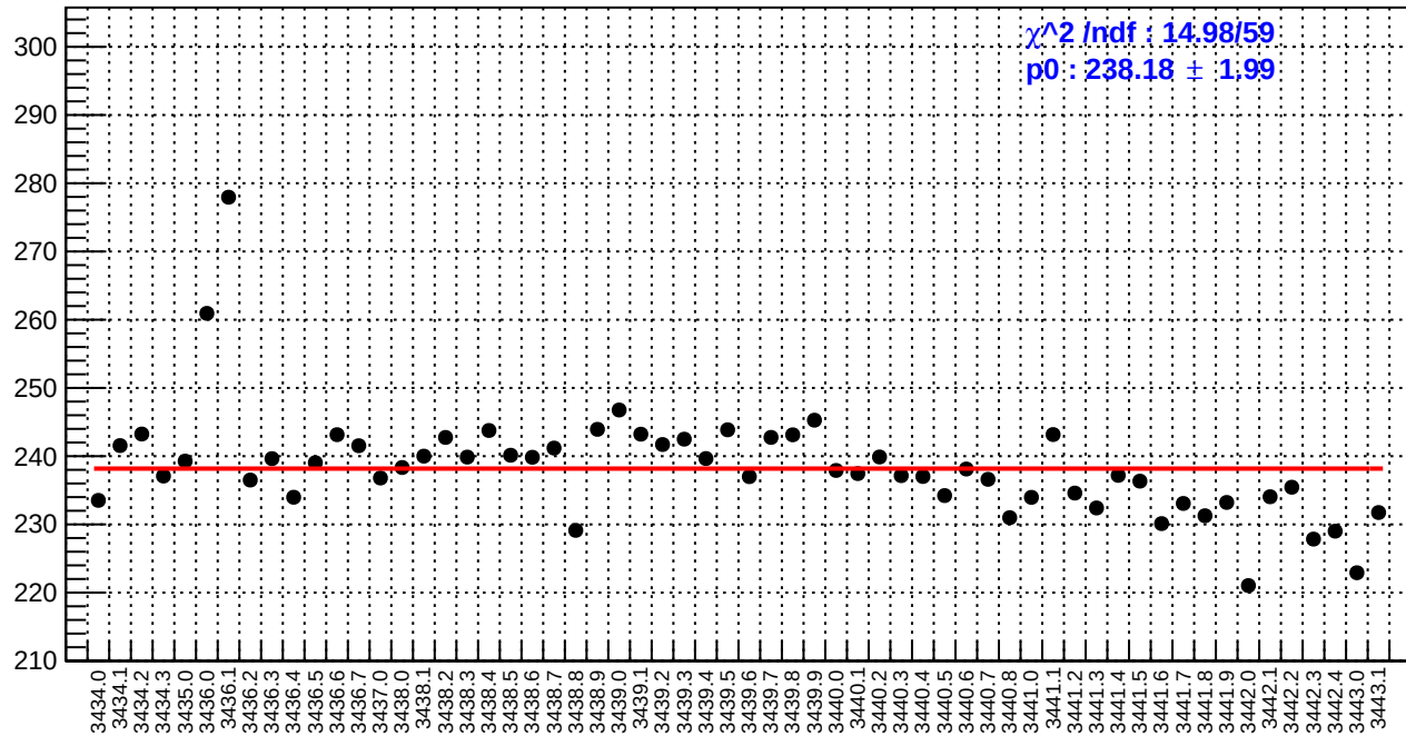
slug6: reg_asym_sam8.rms/ppm
