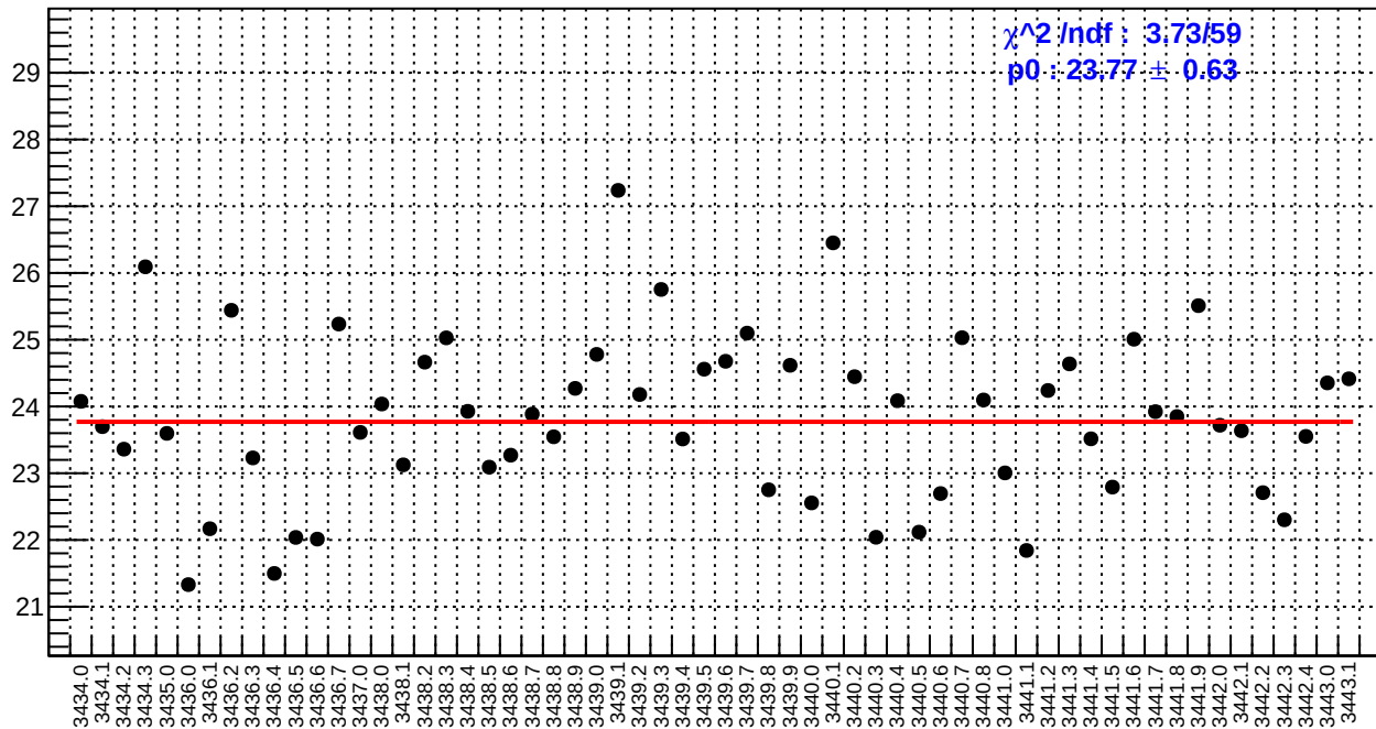
slug6: right_avg_bpm4aY/(ppb/nm)
