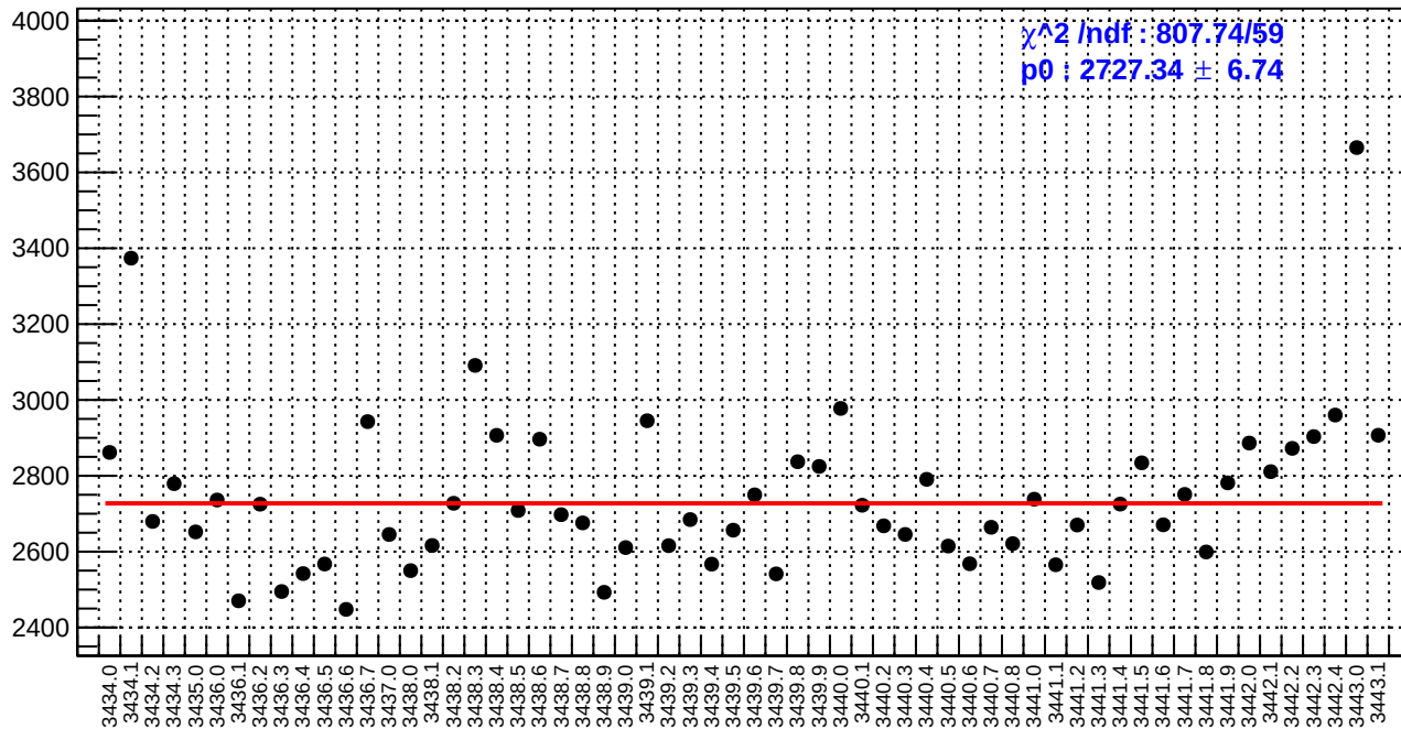
slug6: diff_bpm4eY.rms/nm
