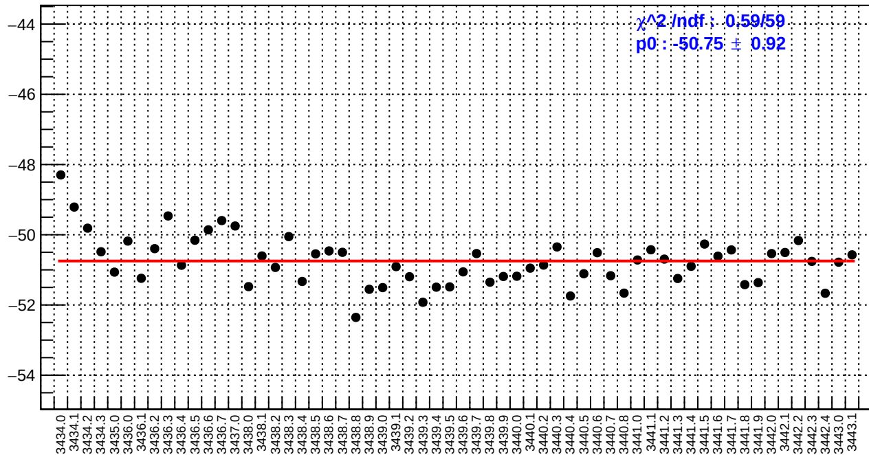
slug6: left_avg_bpm12X/(ppb/nm)
