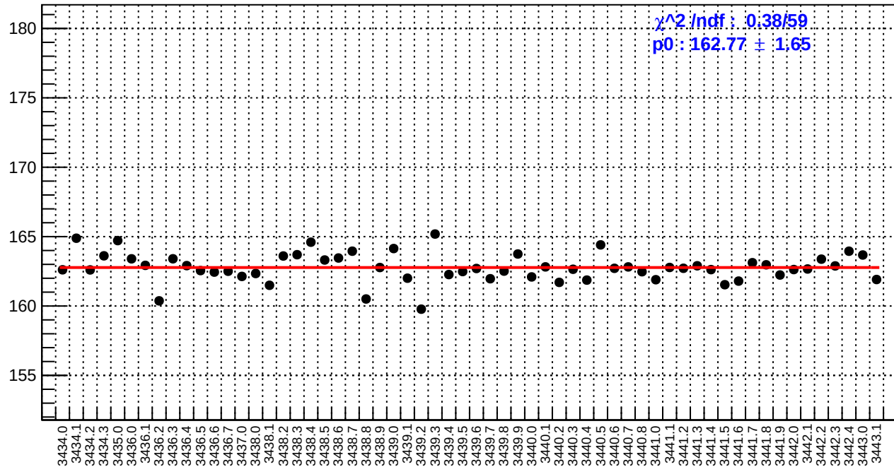
slug6: reg_asym_usl.rms/ppm
