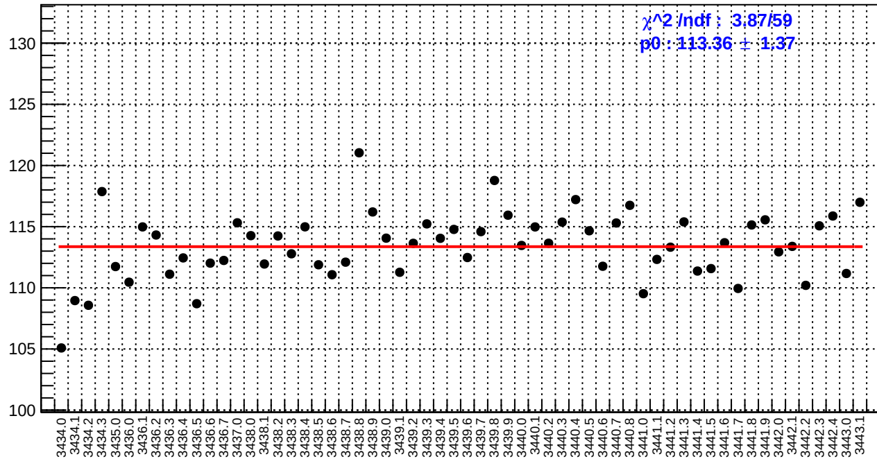
slug6: dsl_bpm4aX/(ppb/nm)
