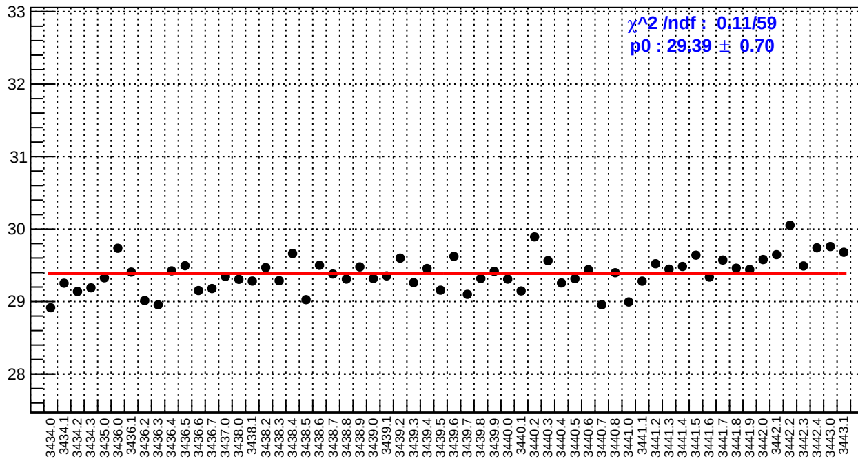
slug6: reg_asym_left_dd.rms/ppm
