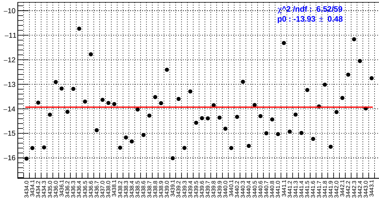
slug6: dsr_bpm4eY/(ppb/nm)
