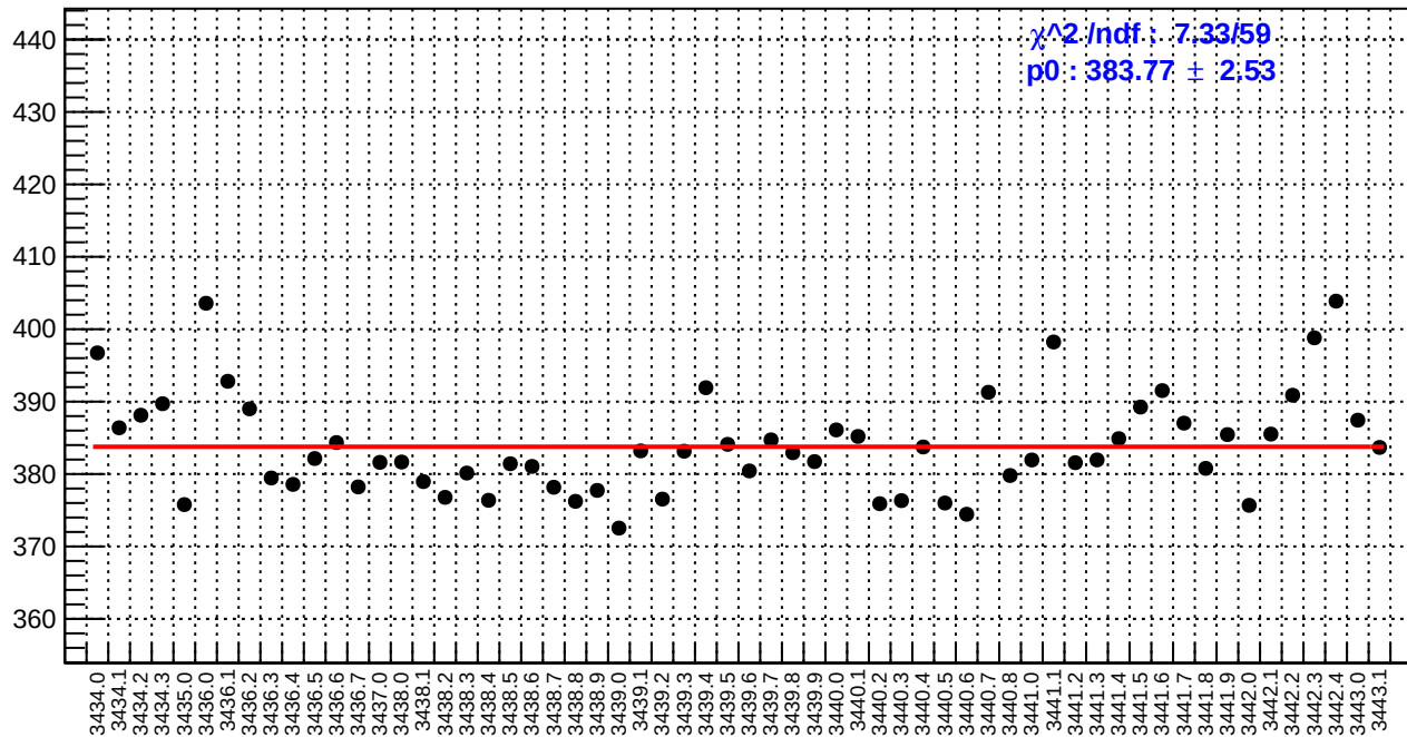
slug6: reg_asym_sam5.rms/ppm
