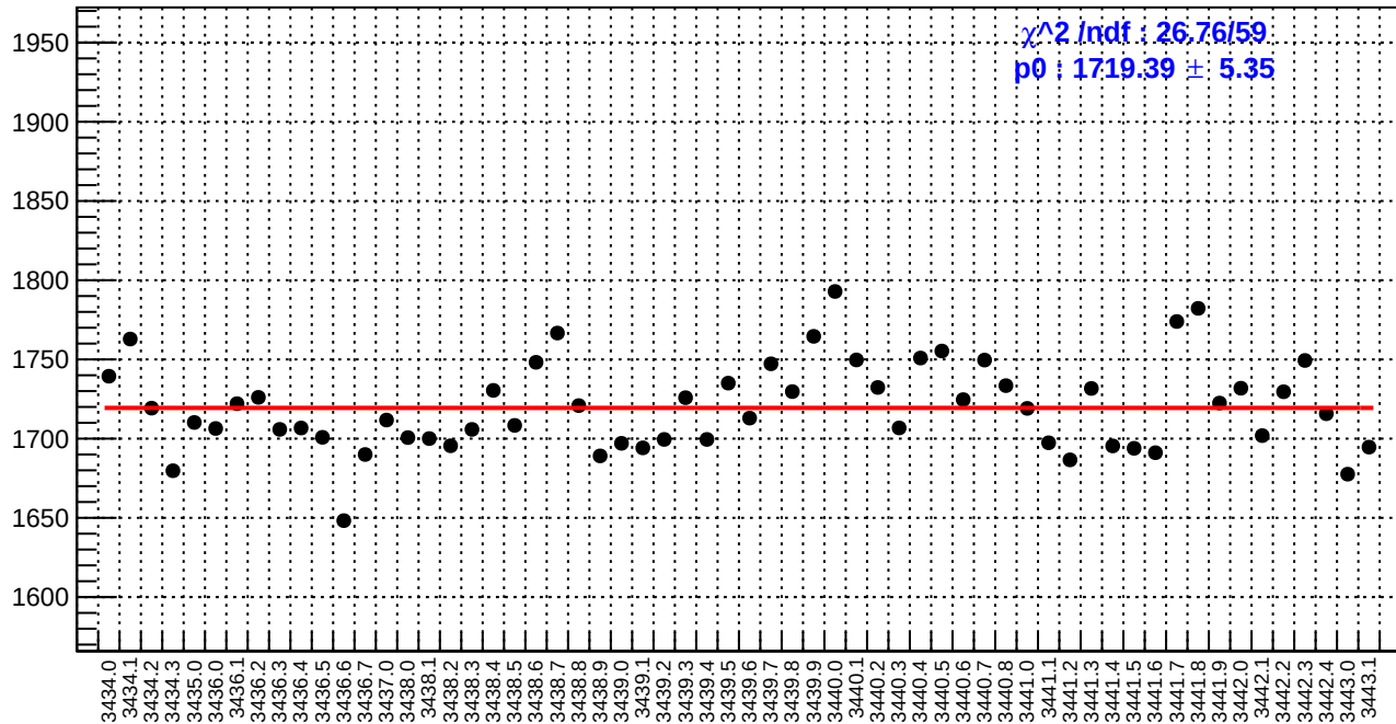
slug6: diff_bpm4aX.rms/nm
