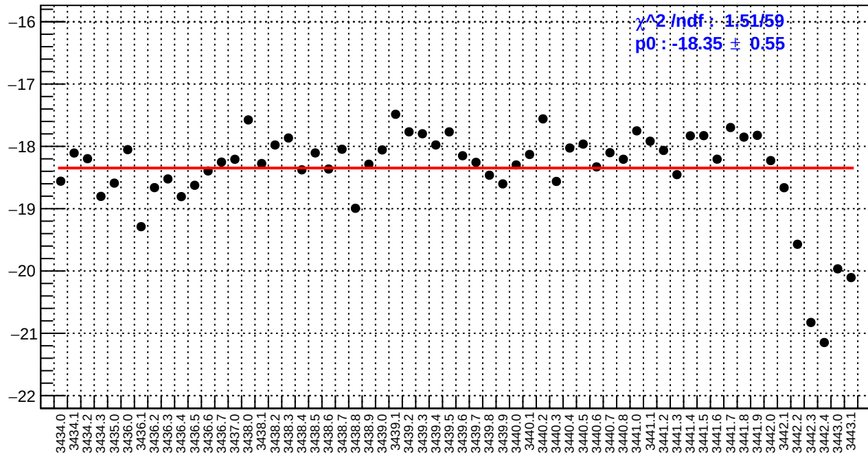
slug6: us_avg_bpm4eX/(ppb/nm)
