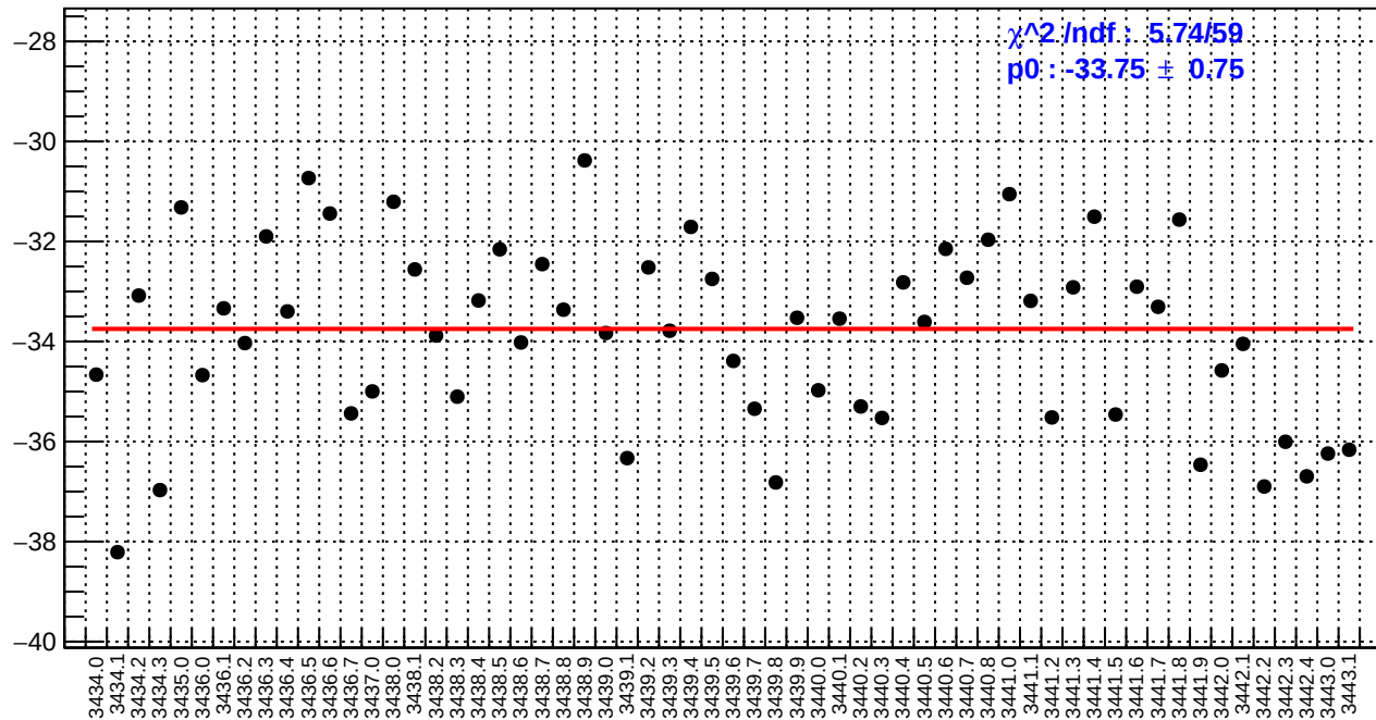
slug6: left_avg_bpm4aY/(ppb/nm)
