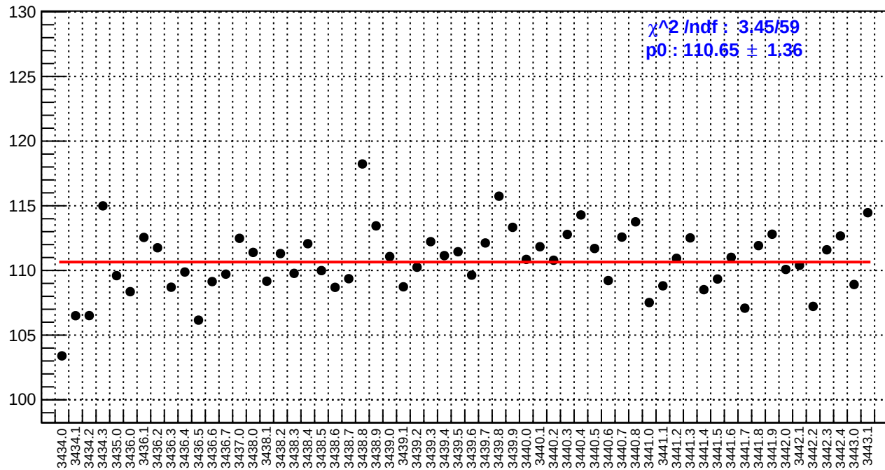
slug6: left_avg_bpm4aX/(ppb/nm)
