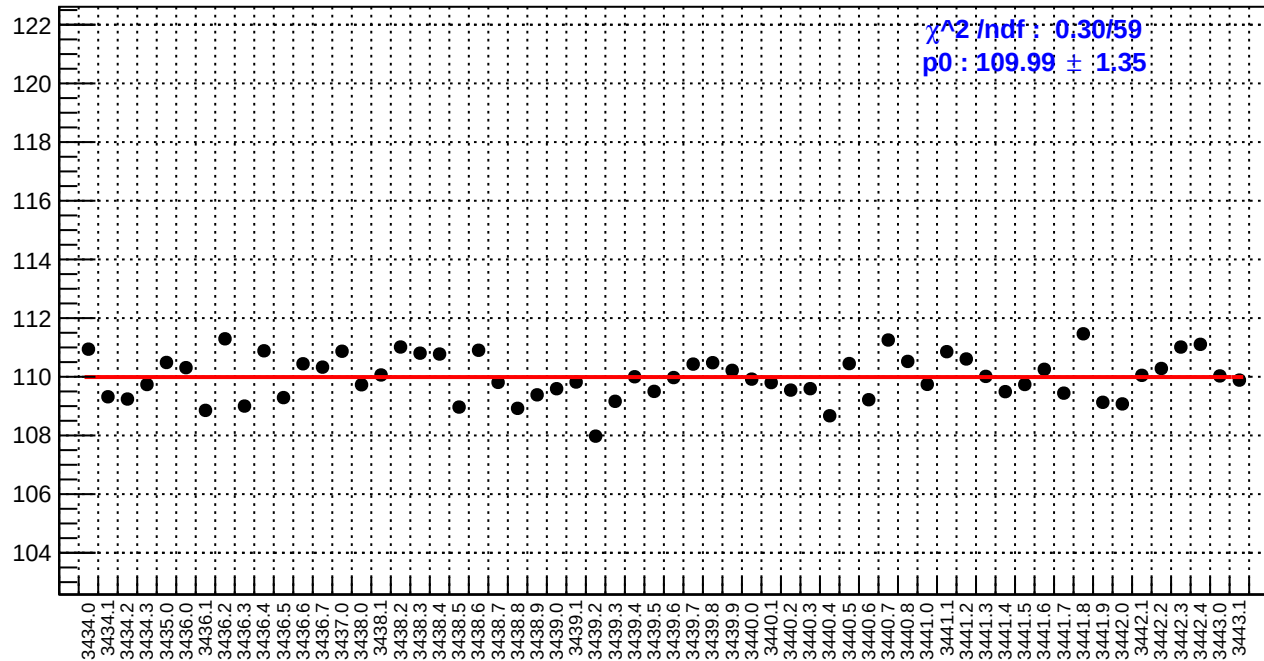
slug6: reg_asym_us_dd.rms/ppm
