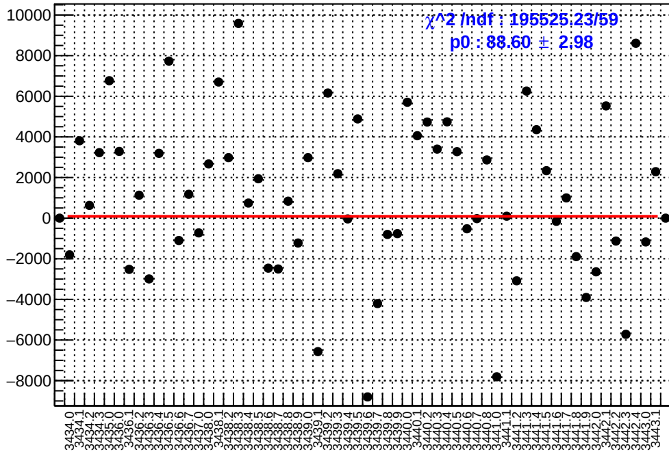
slug6: asym_us_dd.mean/ppb-reg_asym_us_dd.mean/ppb
