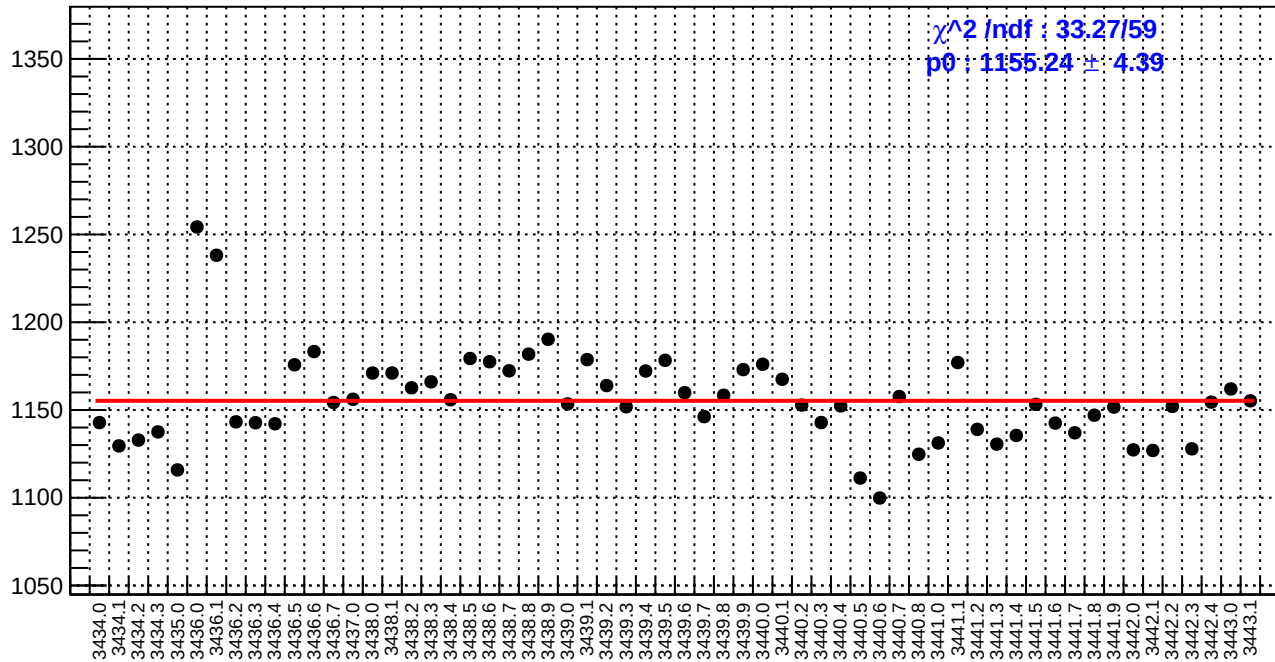
slug6: reg_asym_sam4.rms/ppm
