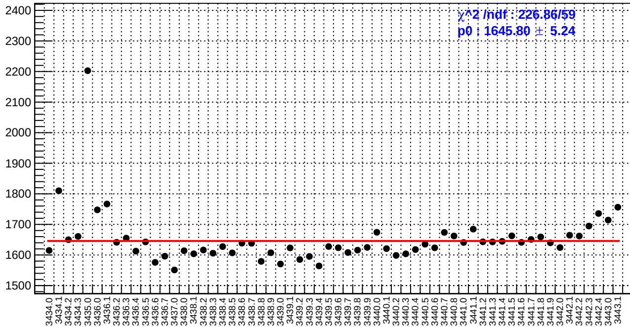
slug6: reg_asym_sam3.rms/ppm
