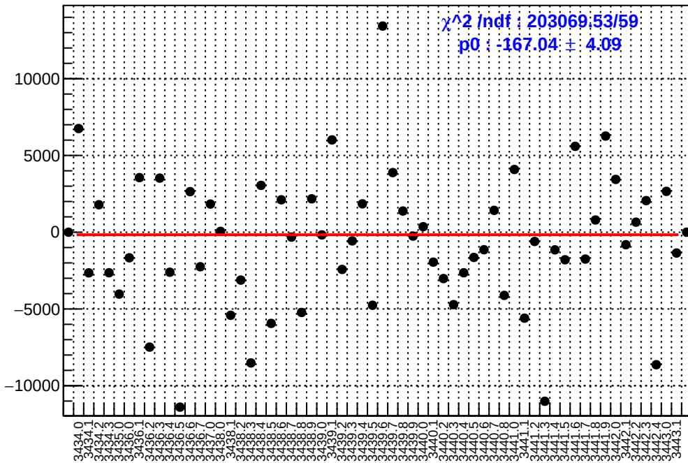
slug6: asym_usr.mean/ppb-reg_asym_usr.mean/ppb
