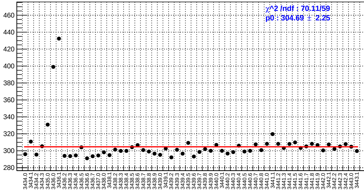
slug6: reg_asym_sam7.rms/ppm
