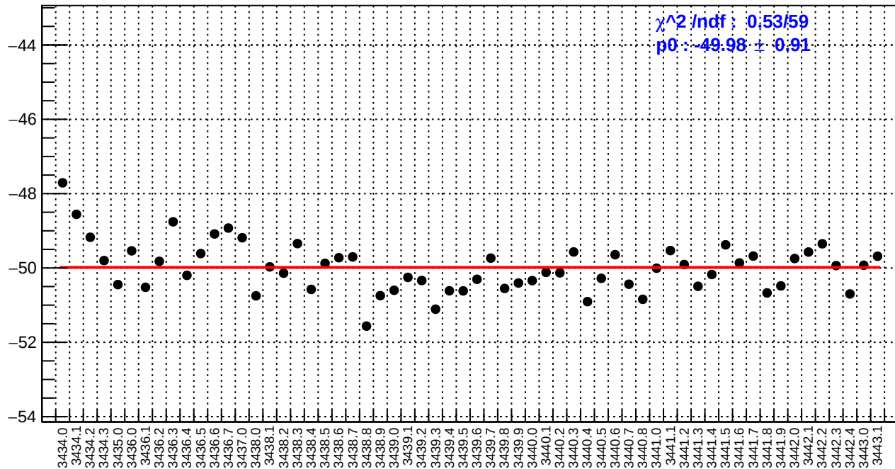
slug6: usl_bpm12X/(ppb/nm)
