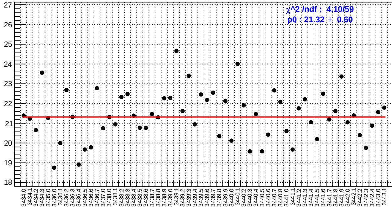
slug6: dsr_bpm4aY/(ppb/nm)
