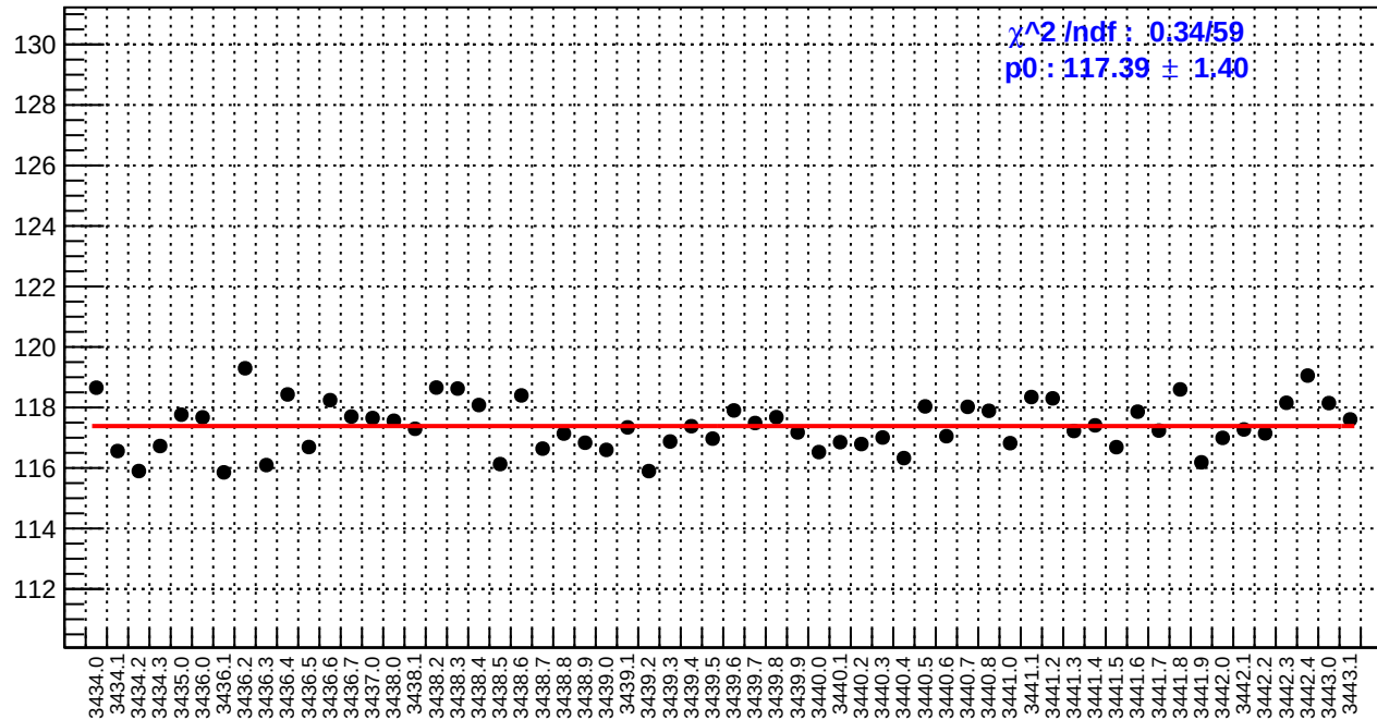
slug6: reg_asym_ds_dd.rms/ppm
