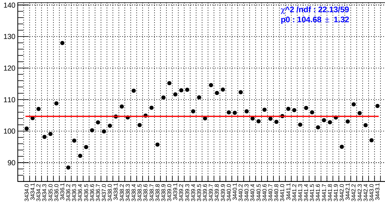
slug6: asym_bcm_an_ds3.rms/ppm
