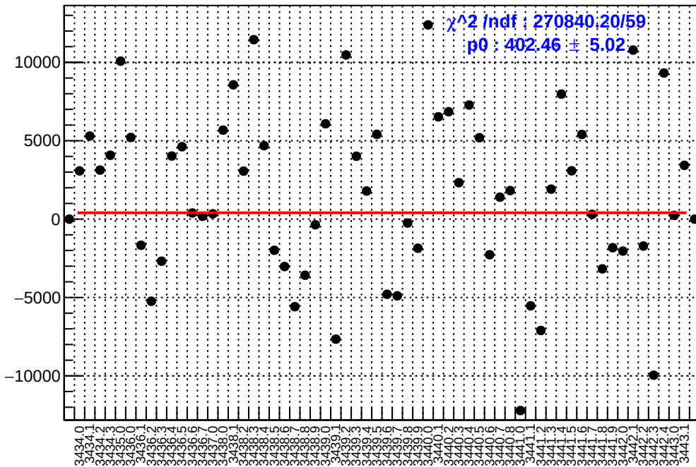
slug6: asym_left_avg.mean/ppb-reg_asym_left_avg.mean/ppb
