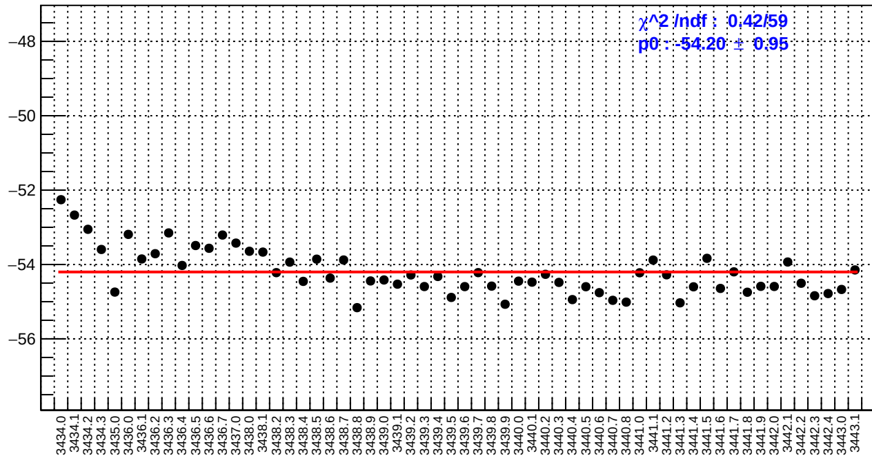
slug: us_avg_bpm12X/(ppb/nm)
