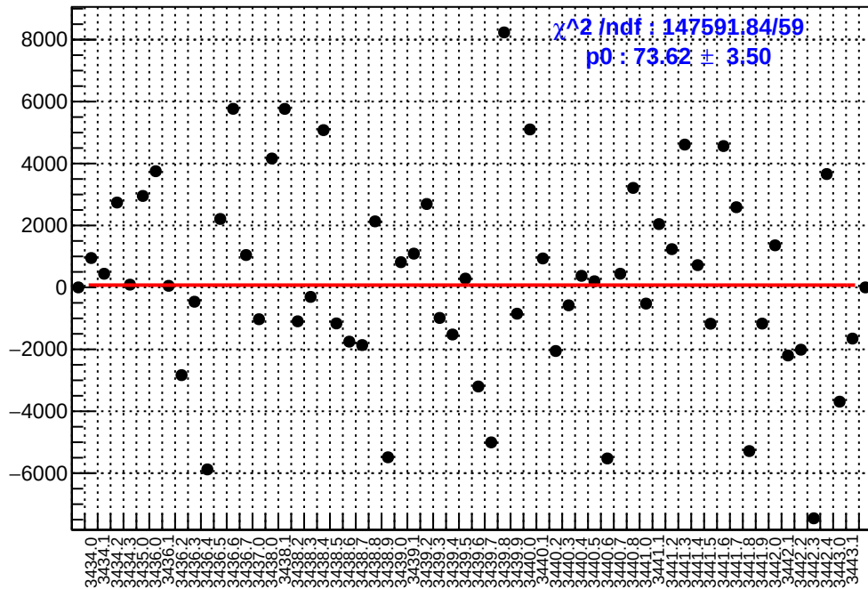
slug6: asym_sam1.mean/ppb-reg_asym_sam1.mean/ppb
