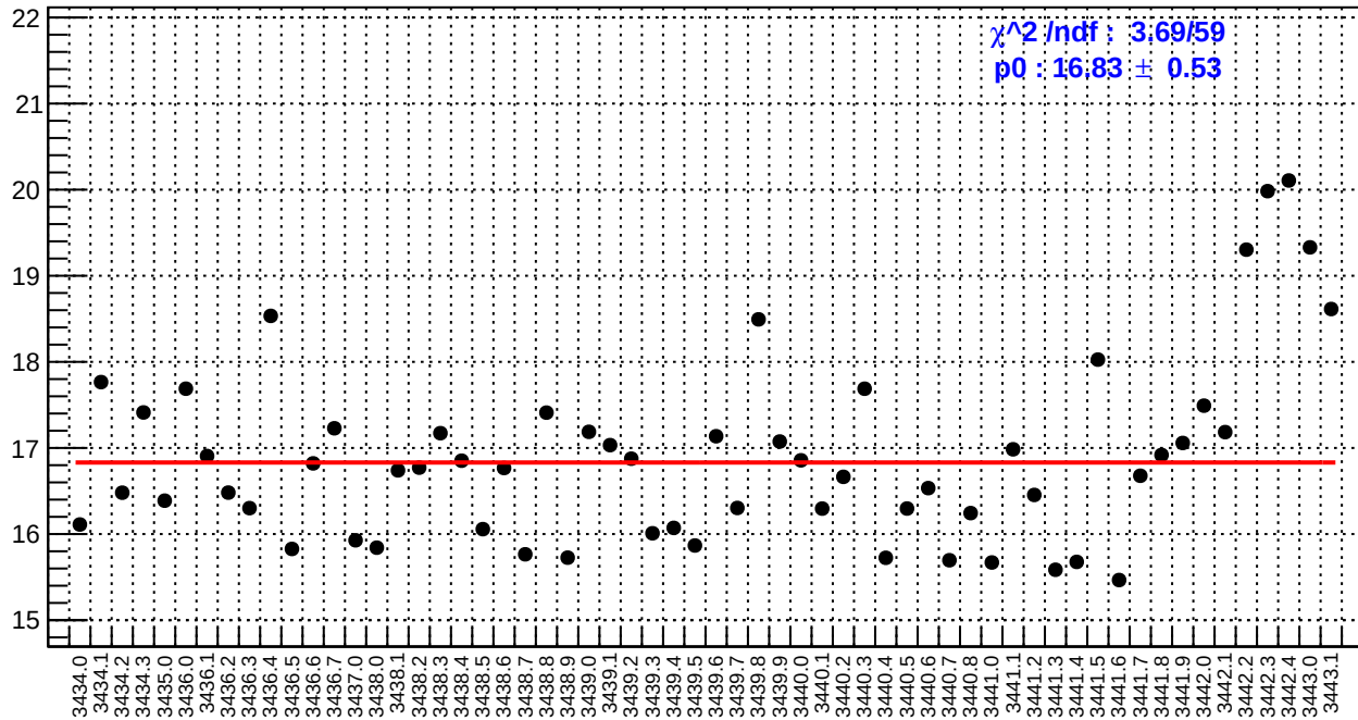
slug6: us_avg_bpm4eY/(ppb/nm)
