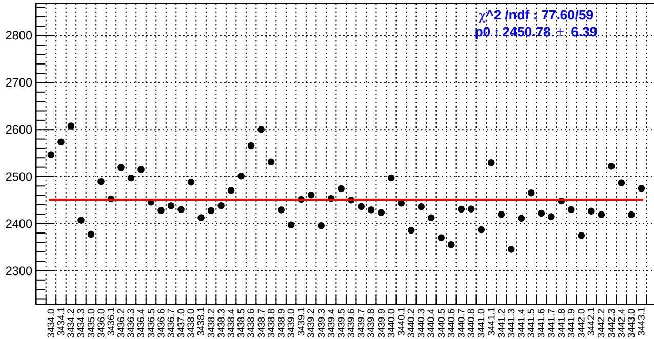
slug6: diff_bpm4aY.rms/nm
