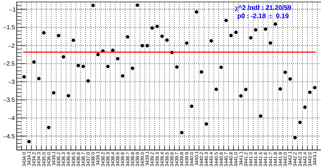
slug6: us_avg_bpm4aY/(ppb/nm)
