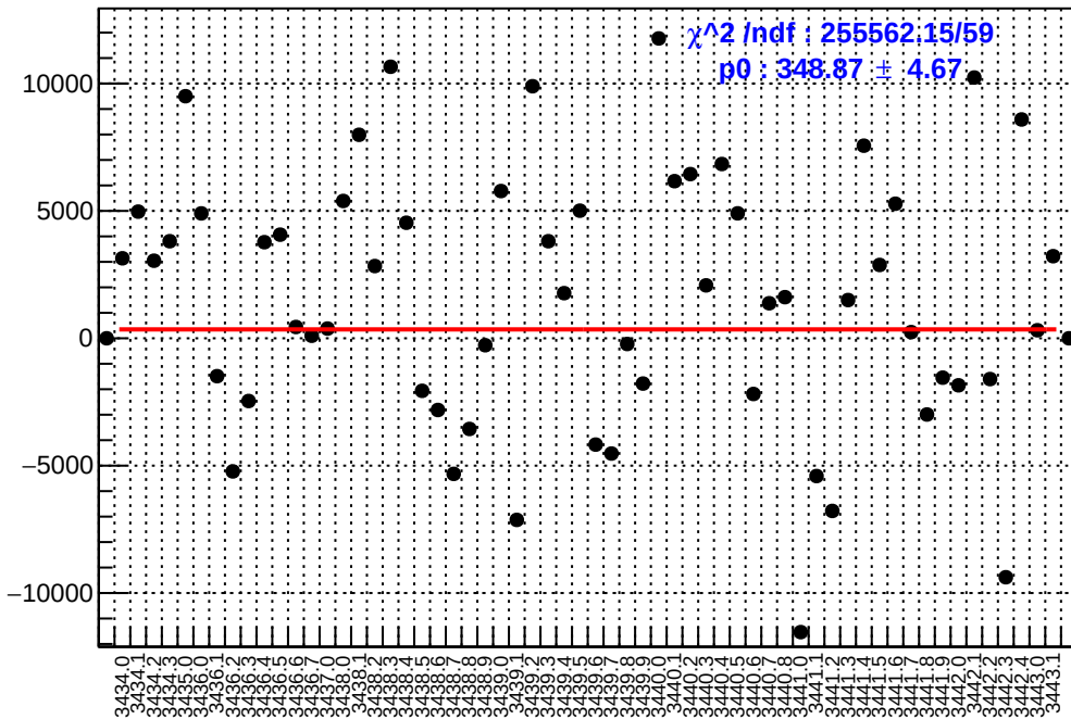
slug6: asym_usl.mean/ppb-reg_asym_usl.mean/ppb
