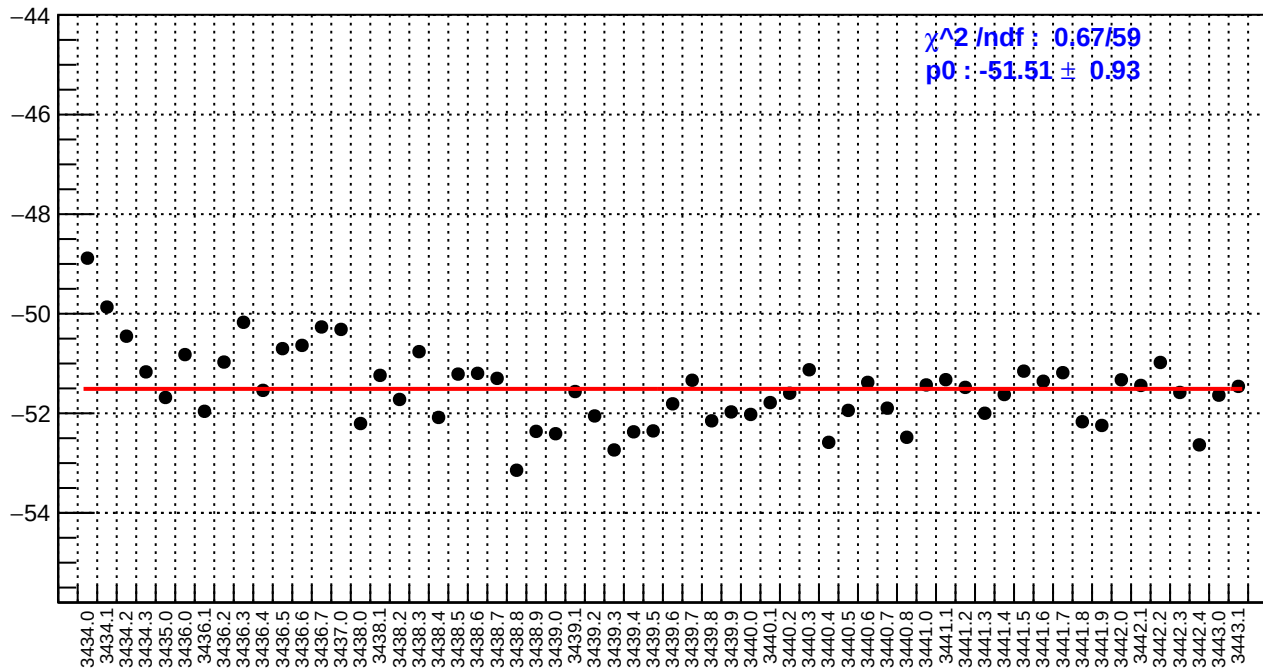
slug6: dsl_bpm12X/(ppb/nm)
