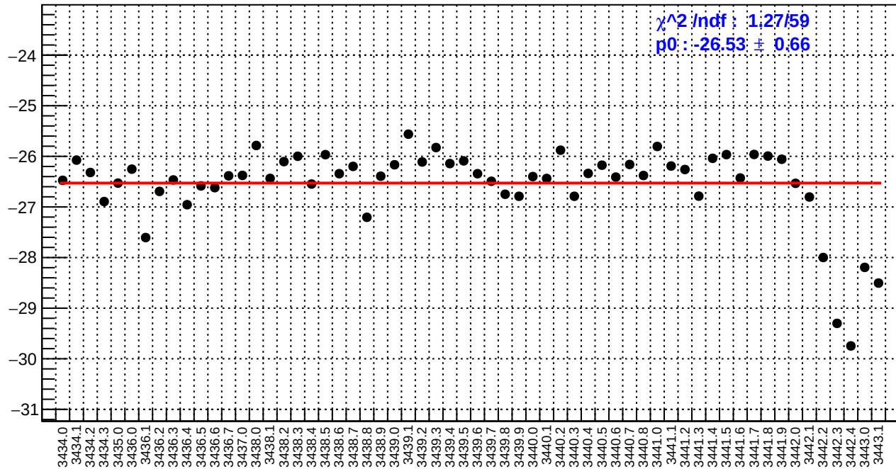
slug6: ds_avg_bpm4eX/(ppb/nm)
