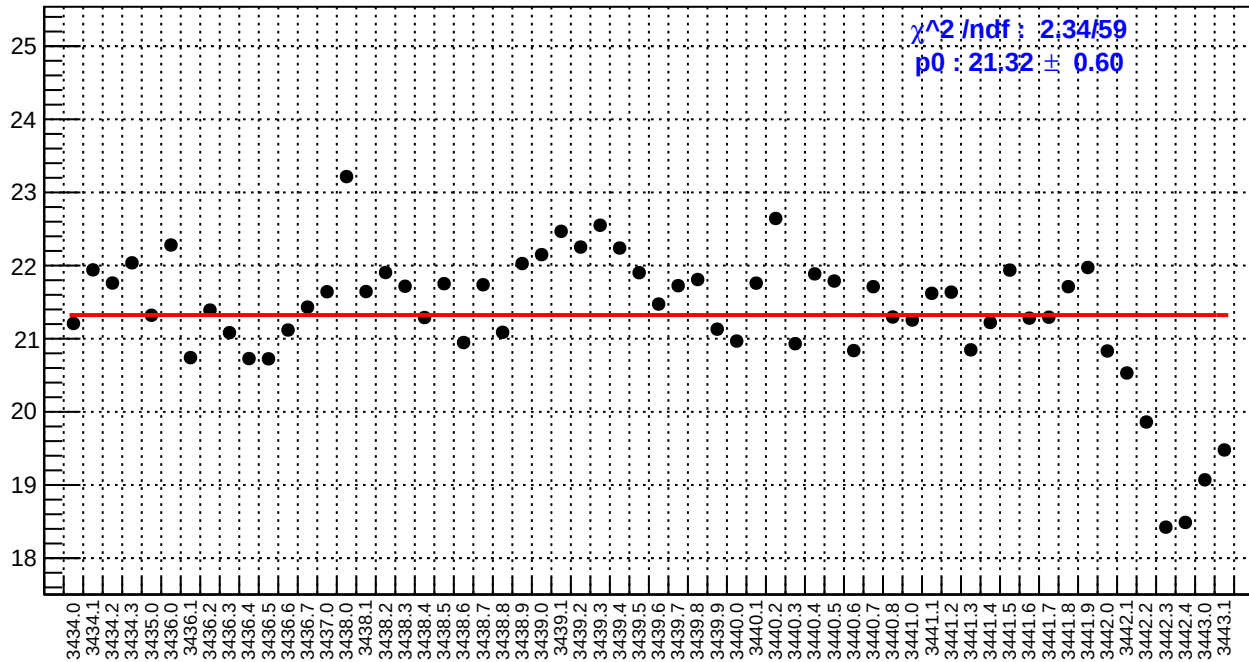
slug6: right_avg_bpm4eX/(ppb/nm)
