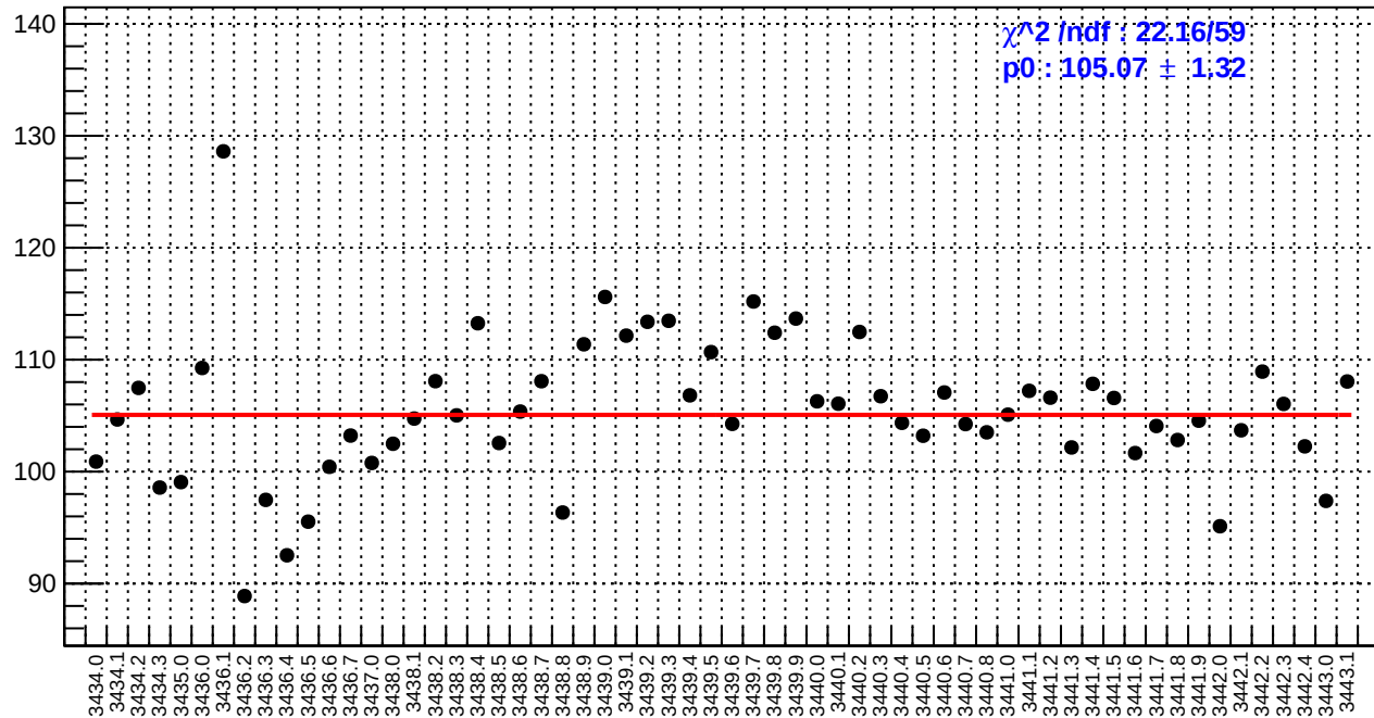
slug6: asym_bcm_an_us.rms/ppm
