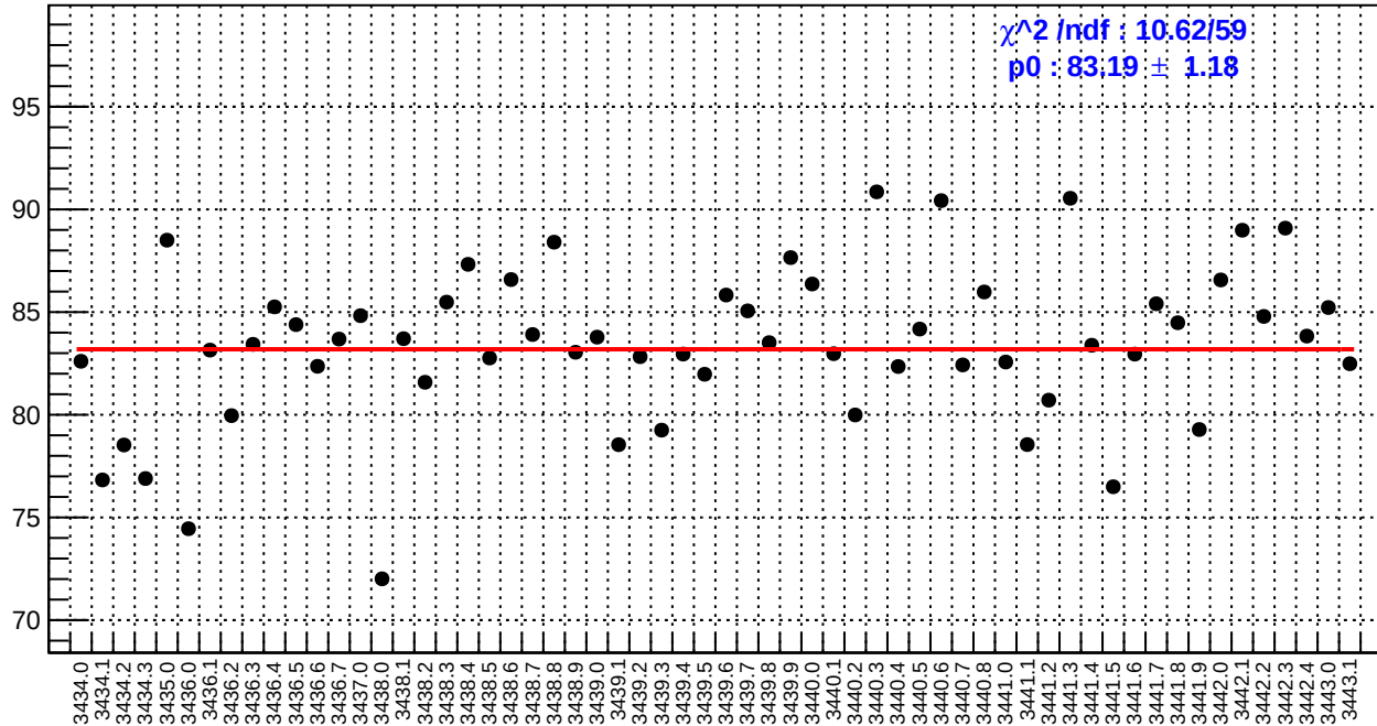
slug6: dsr_bpm4aX/(ppb/nm)
