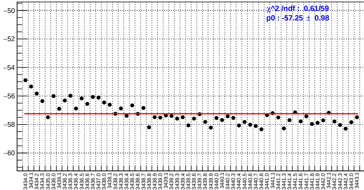
slug6: ds_avg_bpm12X/(ppb/nm)
