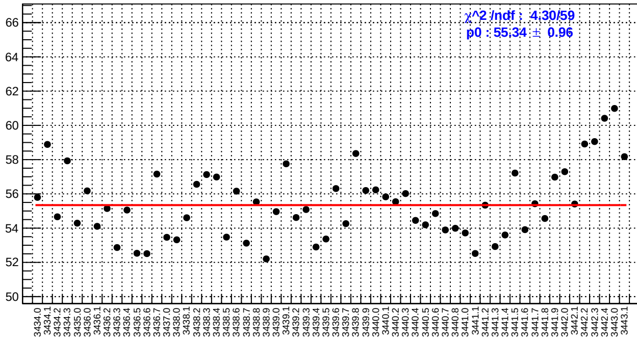
slug6: usl_bpm4eY/(ppb/nm)
