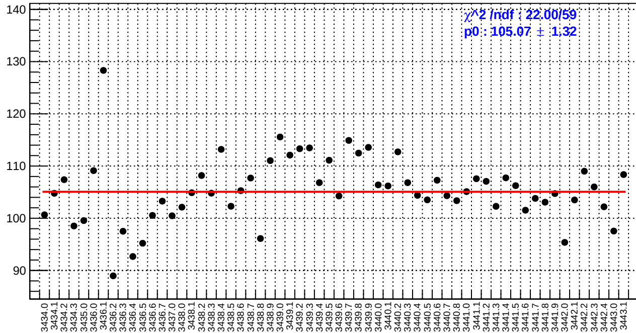
slug6: asym_bcm_an_ds.rms/ppm
