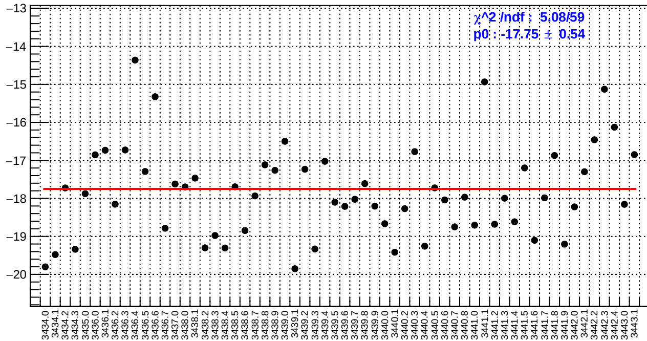
slug6: right_avg_bpm4eY/(ppb/nm)
