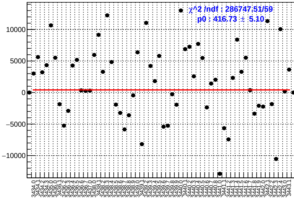
slug6: asym_dsl.mean/ppb-reg_asym_dsl.mean/ppb
