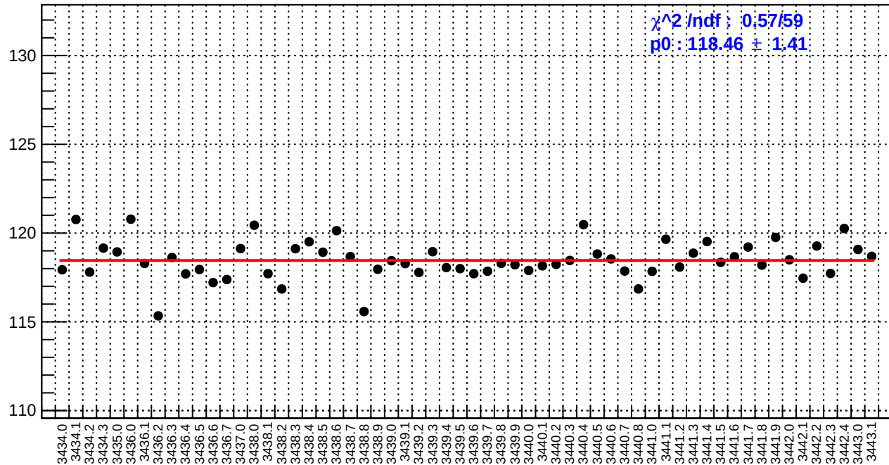
slug6: reg_asym_us_avg.rms/ppm
