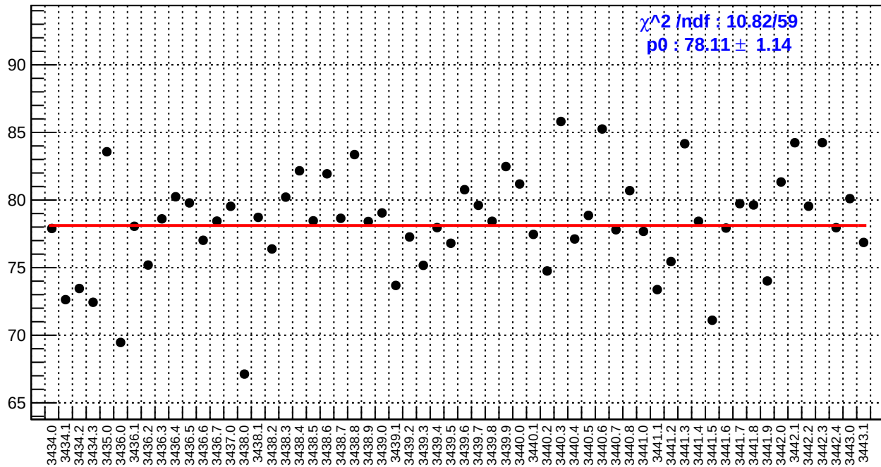
slug6: right_avg_bpm4aX/(ppb/nm)
