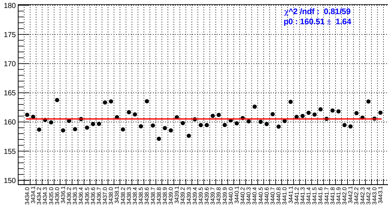
slug6: reg_asym_usr.rms/ppm
