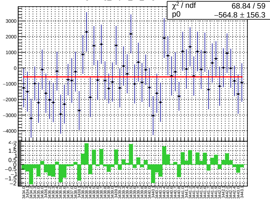
slug6: reg_asym_us_avg.mean/ppb
