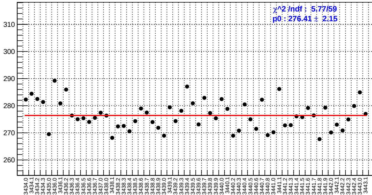
slug6: reg_asym_sam1.rms/ppm
