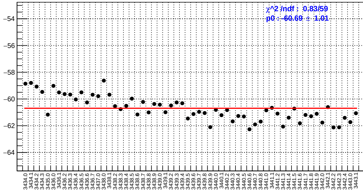
slug6: right_avg_bpm12X/(ppb/nm)
