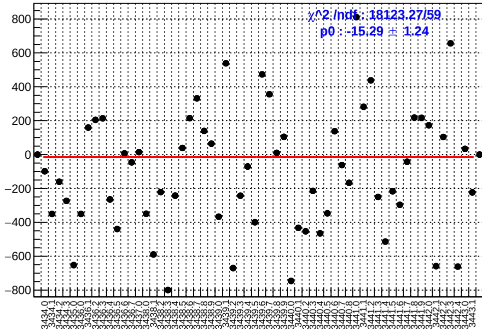
slug6: asym_right_dd.mean/ppb-reg_asym_right_dd.mean/ppb
