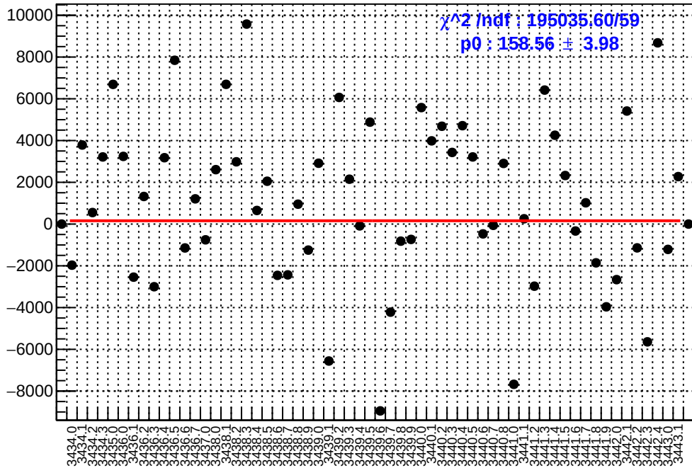
slug6: asym_ds_dd.mean/ppb-reg_asym_ds_dd.mean/ppb
