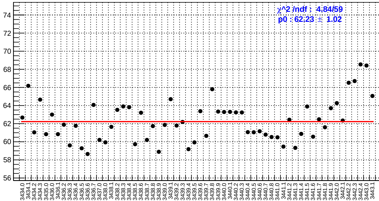
slug6: dsl_bpm4eY/(ppb/nm)
