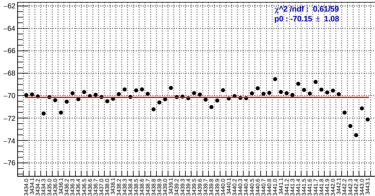
slug6: dsl_bpm4eX/(ppb/nm)
