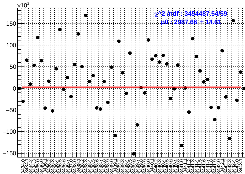
slug6: asym_sam2.mean/ppb-reg_asym_sam2.mean/ppb
