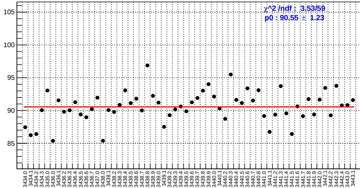
slug6: us_avg_bpm4aX/(ppb/nm)
