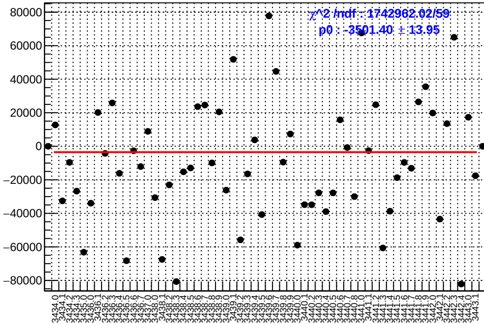
slug6: asym_sam6.mean/ppb-reg_asym_sam6.mean/ppb
