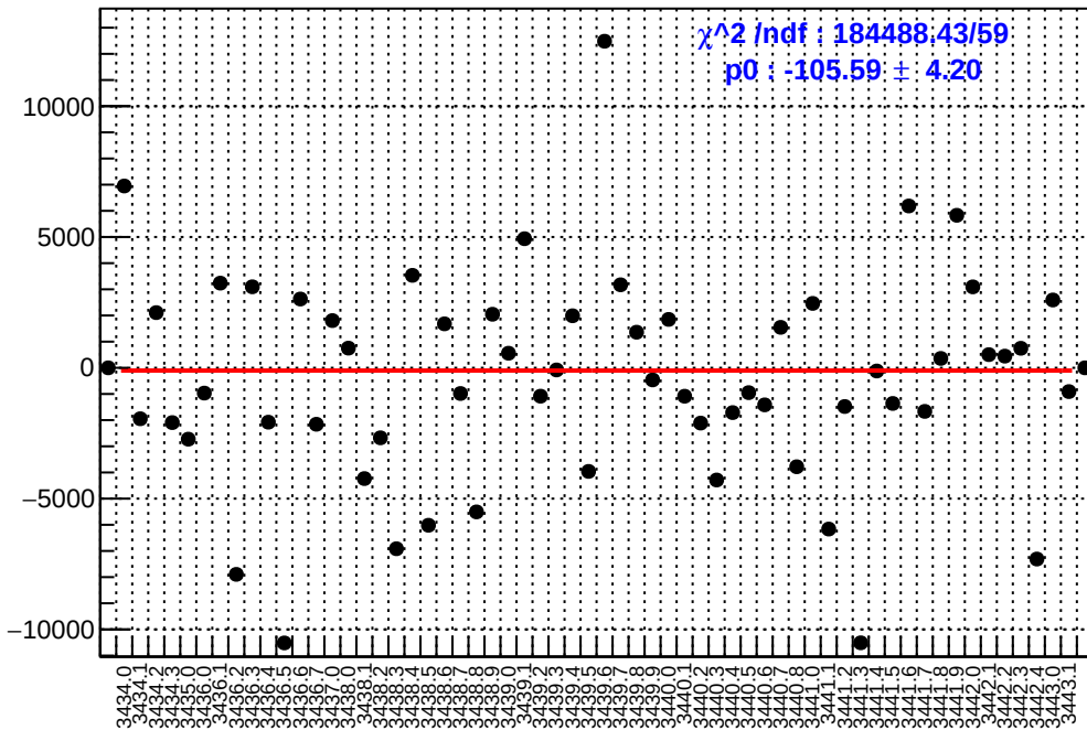
slug6: asym_dsr.mean/ppb-reg_asym_dsr.mean/ppb
