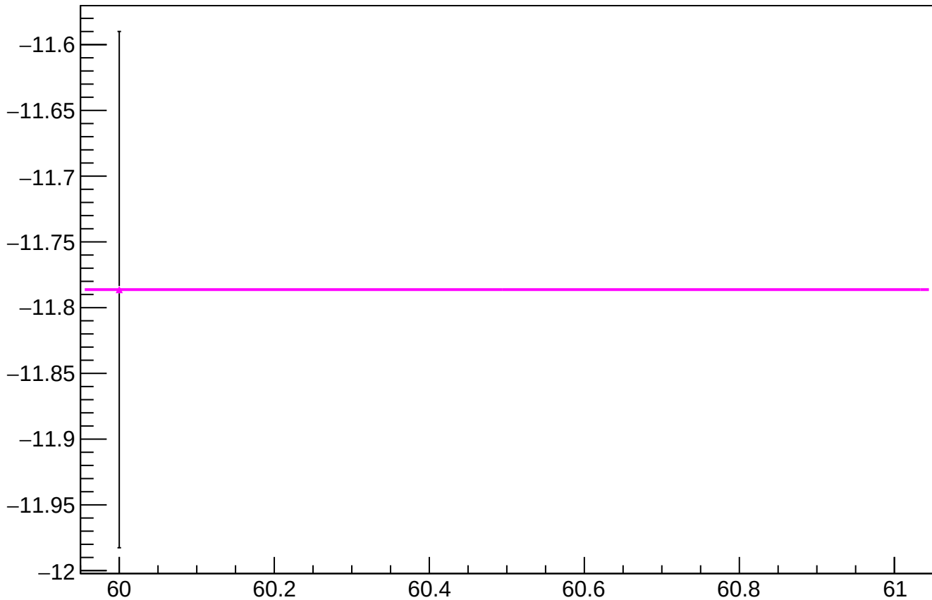
reg_asym_bcm_an_ds_diff_bpm4aX_slope vs slug
