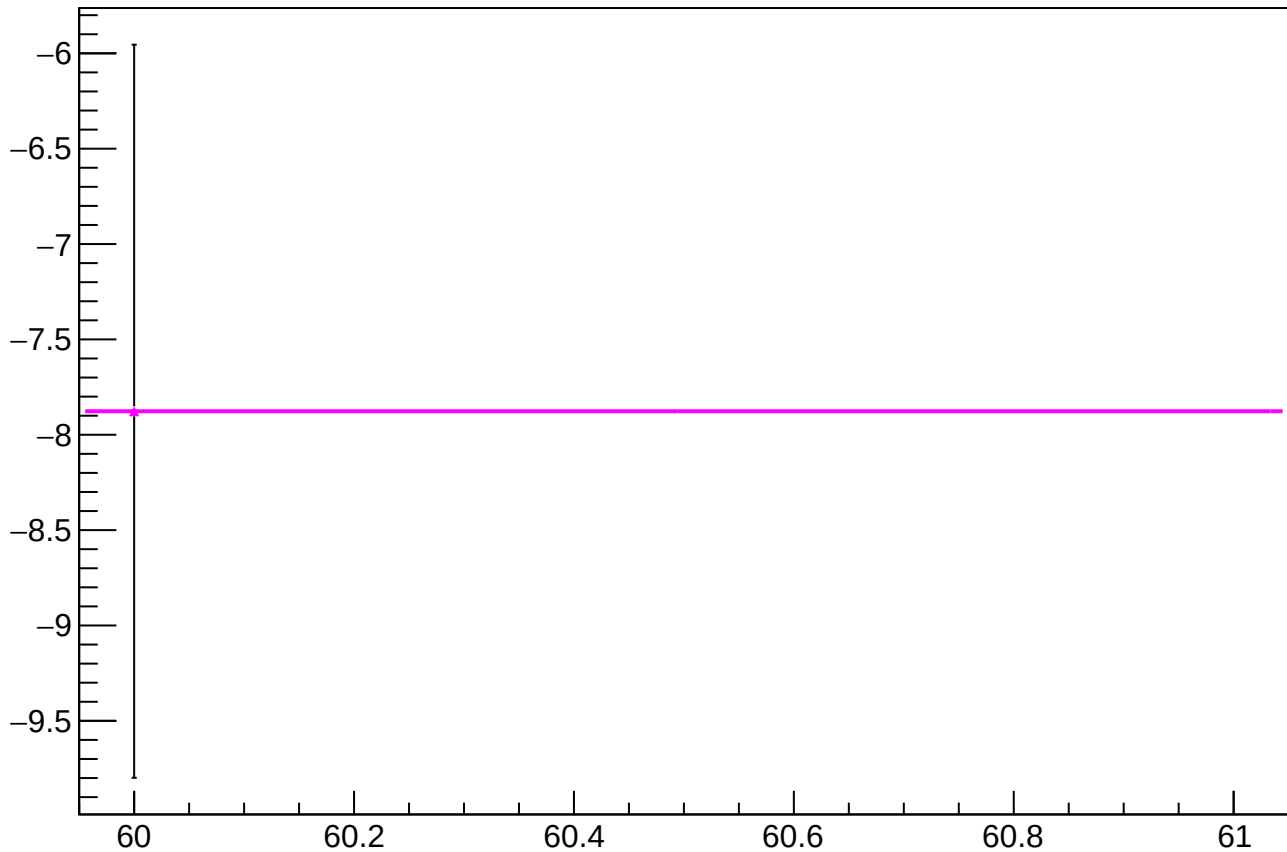
reg_asym_at1_avg_diff_bpm4aY_slope vs slug
