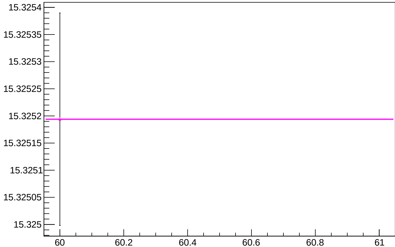
yield_sam7_mean vs slug
