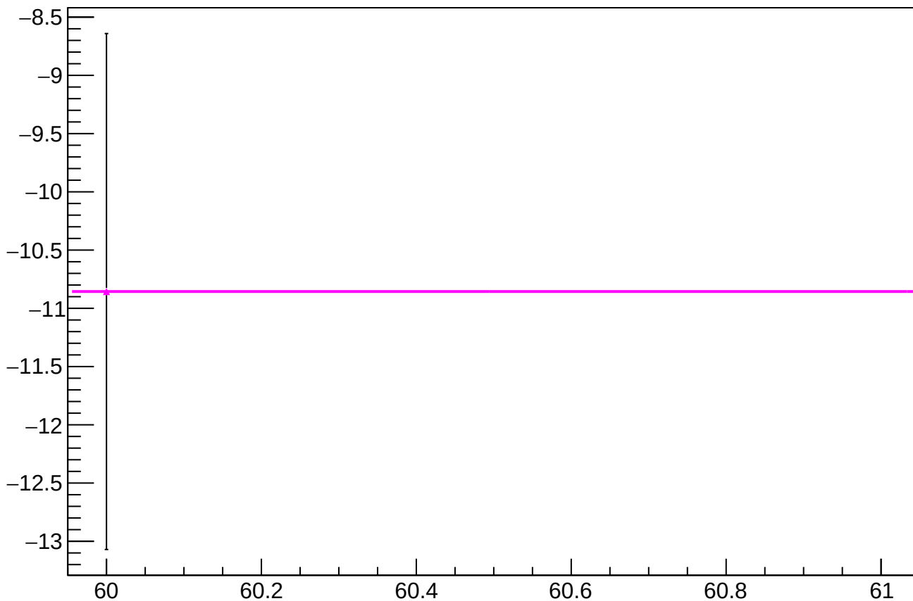
reg_asym_at2_avg_diff_bpm4aY_slope vs slug
