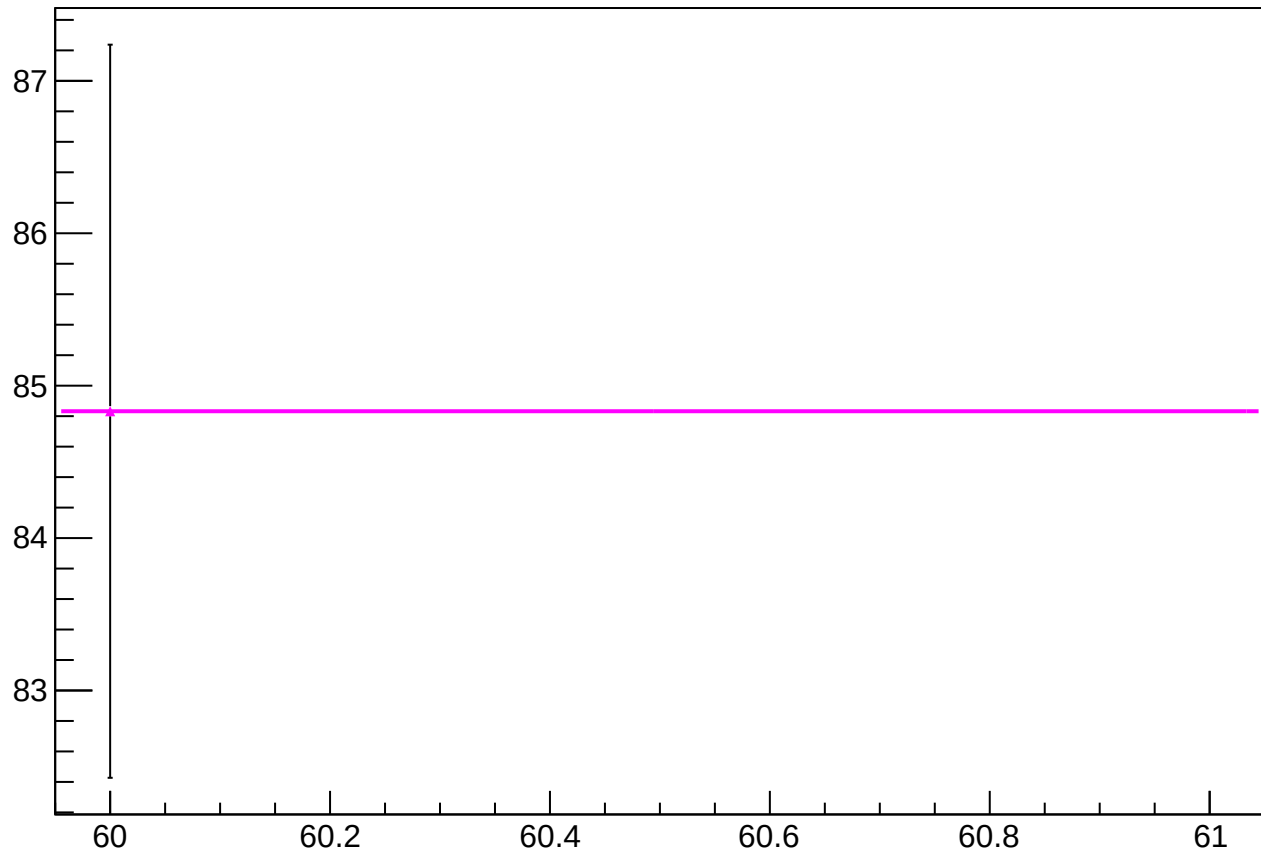
reg_asym_atr1l2_avg_diff_bpm4aX_slope vs slug
