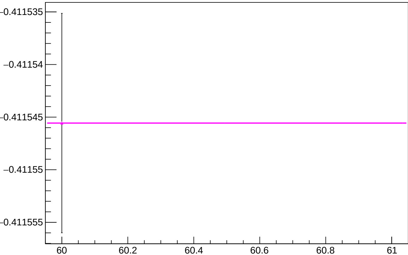
yield_bpm4acX_mean vs slug
