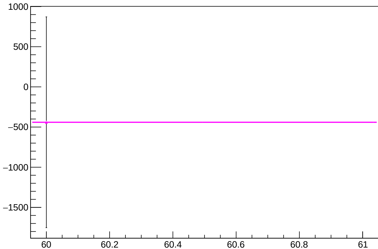
asym_at1_avg_correction_mean vs slug
