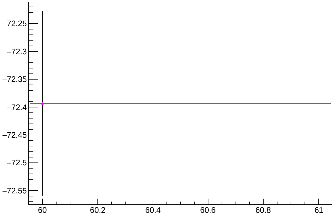
reg_asym_left_avg_diff_bpm4eX_slope vs slug
