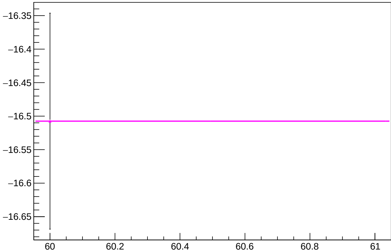
reg_asym_sam_15_dd_diff_bpm11X_slope vs slug
