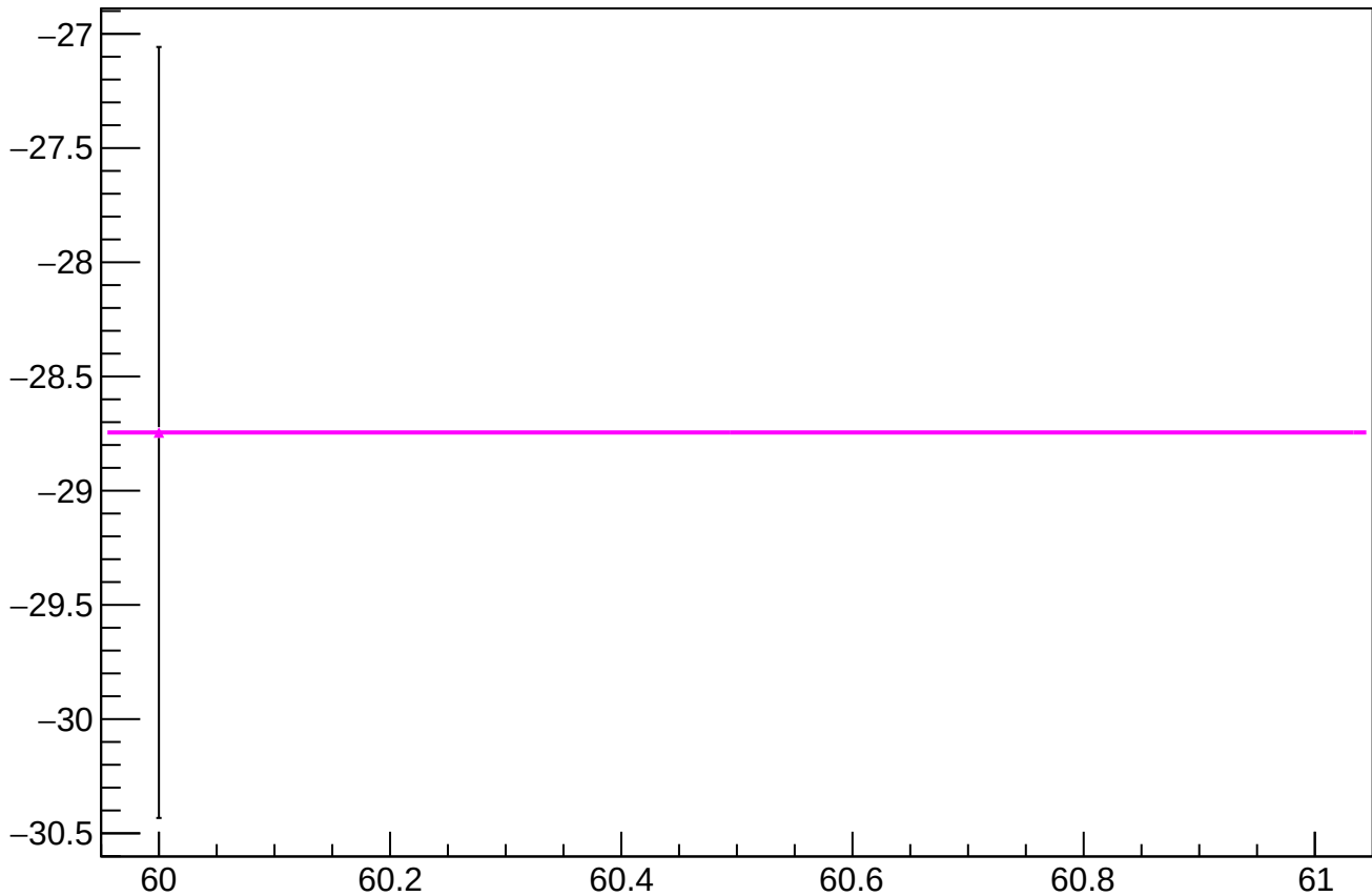
reg_asym_sam_26_dd_diff_bpm11X_slope vs slug
