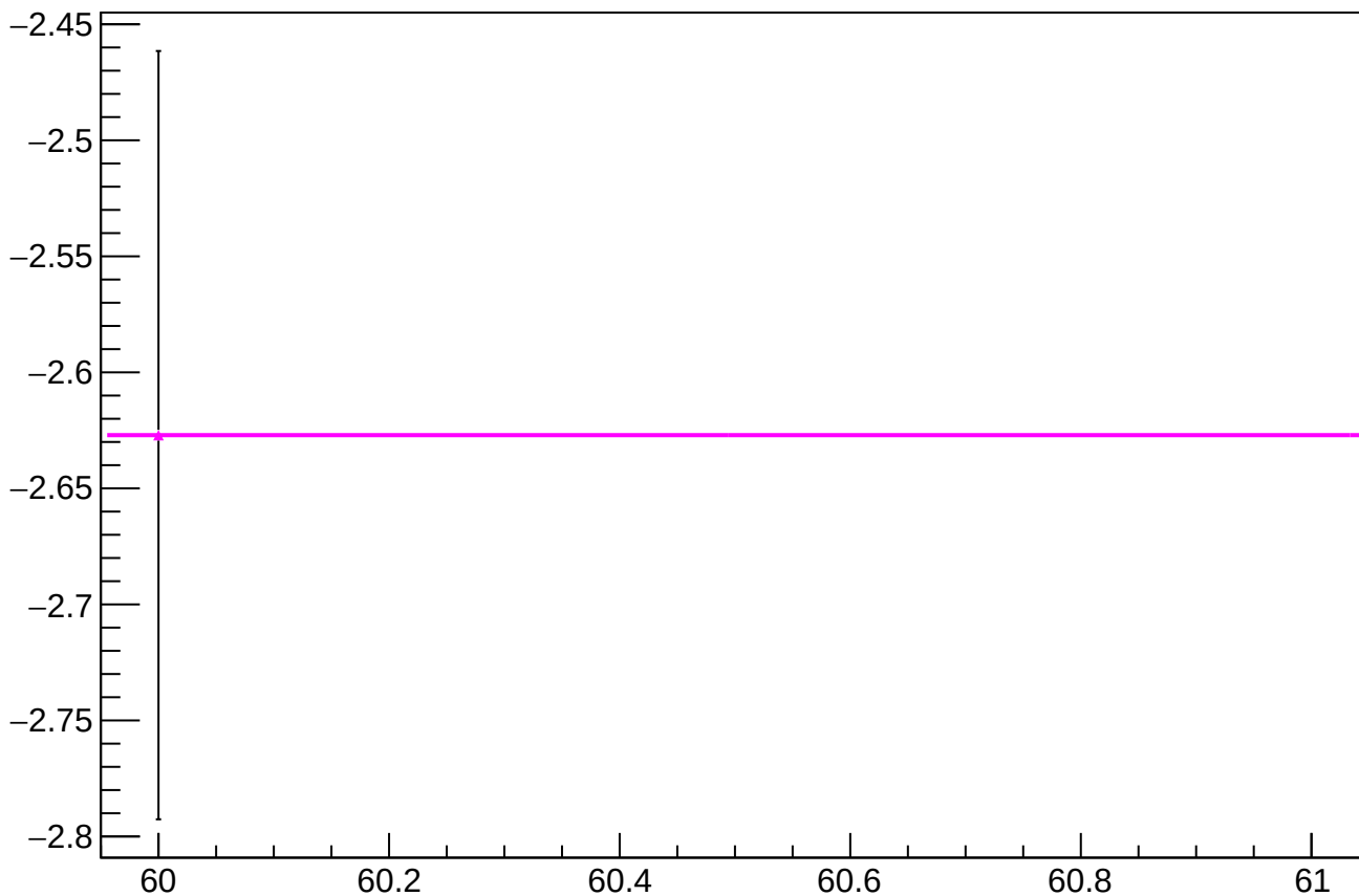
reg_asym_bcm_an_us_diff_bpm4aY_slope vs slug
