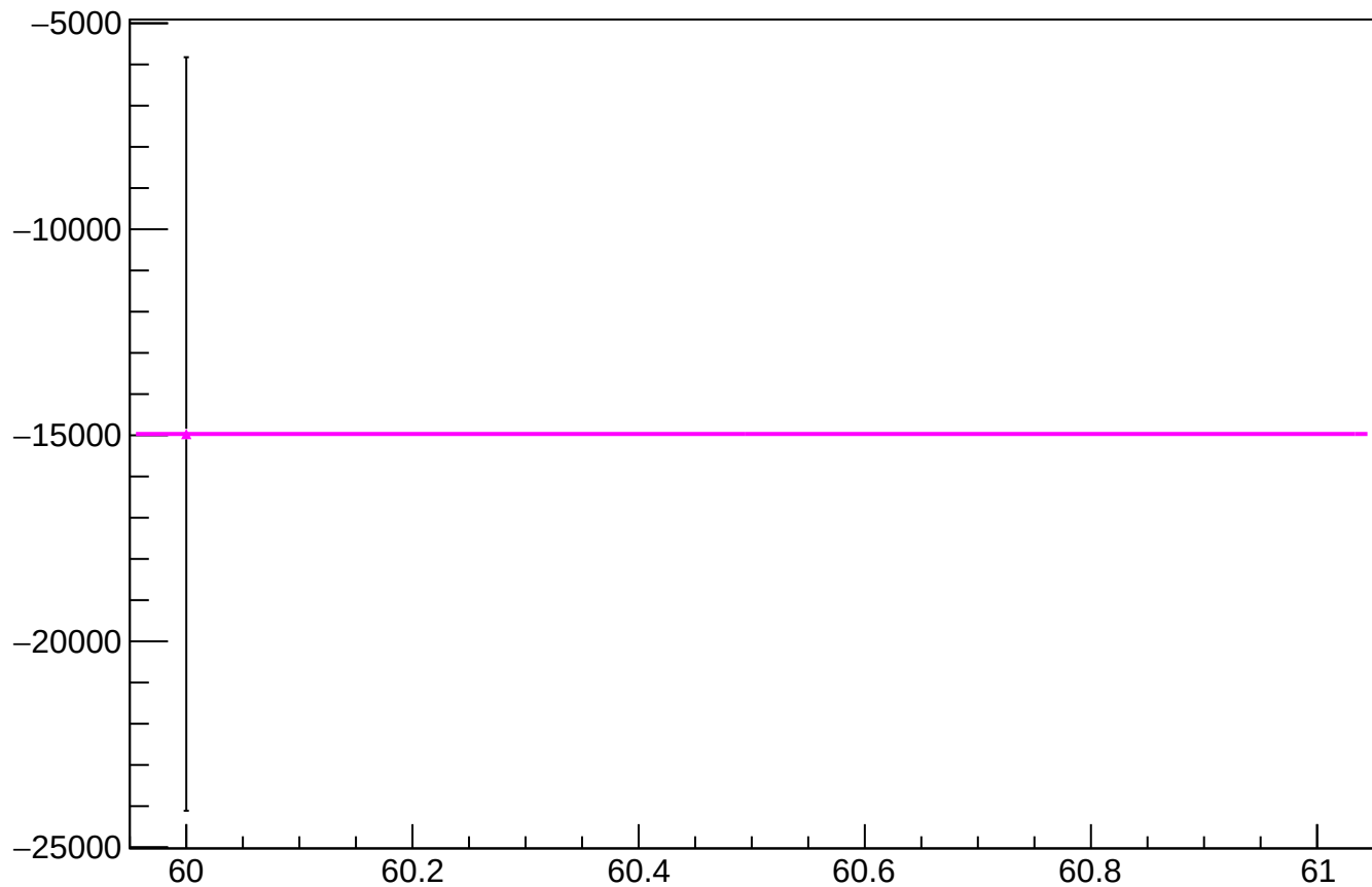
asym_sam_37_dd_mean vs slug
