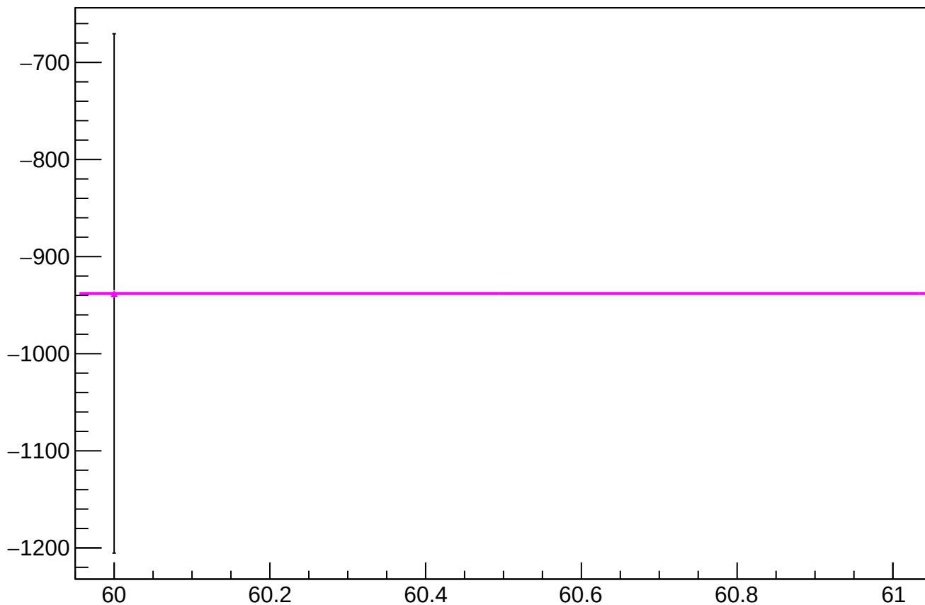
reg_asym_sam1_mean vs slug
