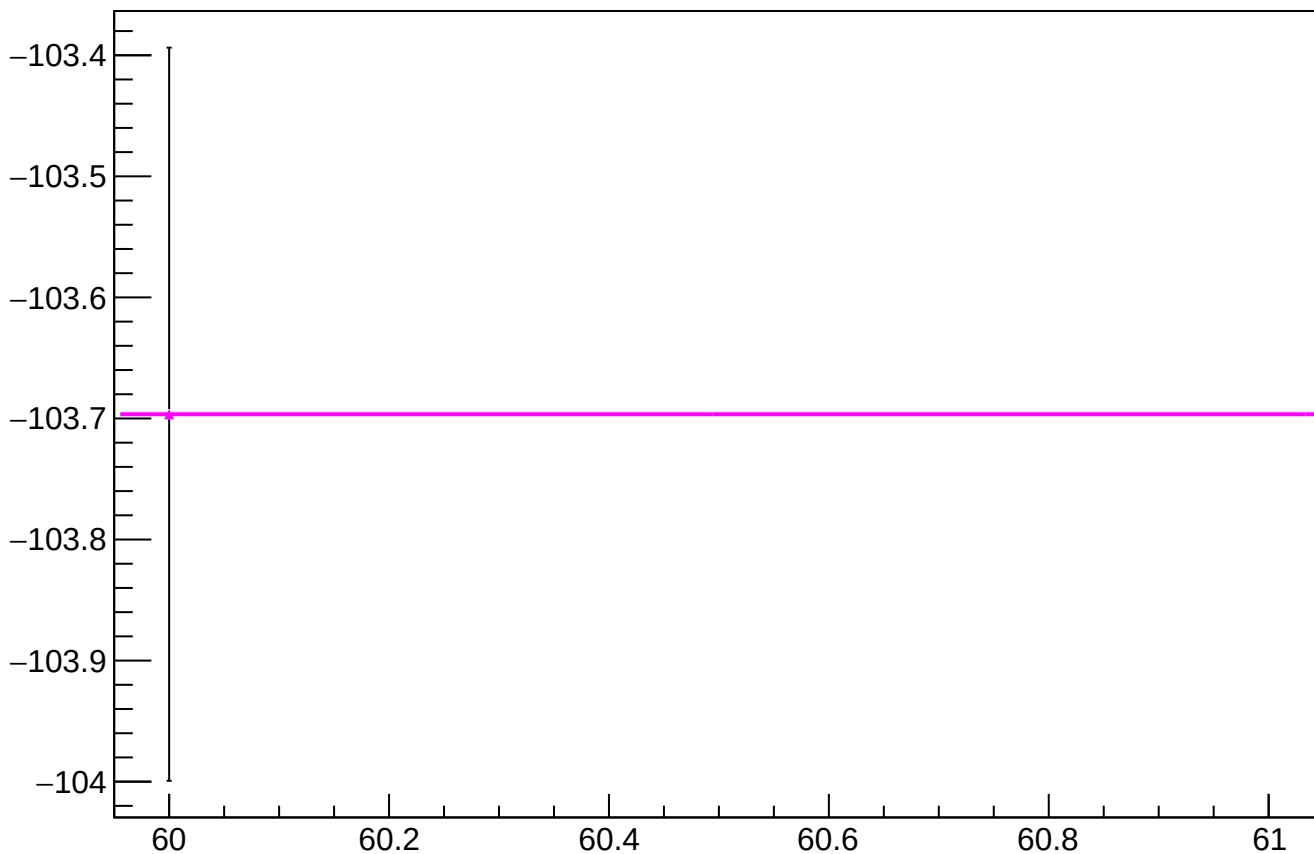
reg_asym_at1_avg_diff_bpm4eX_slope vs slug
