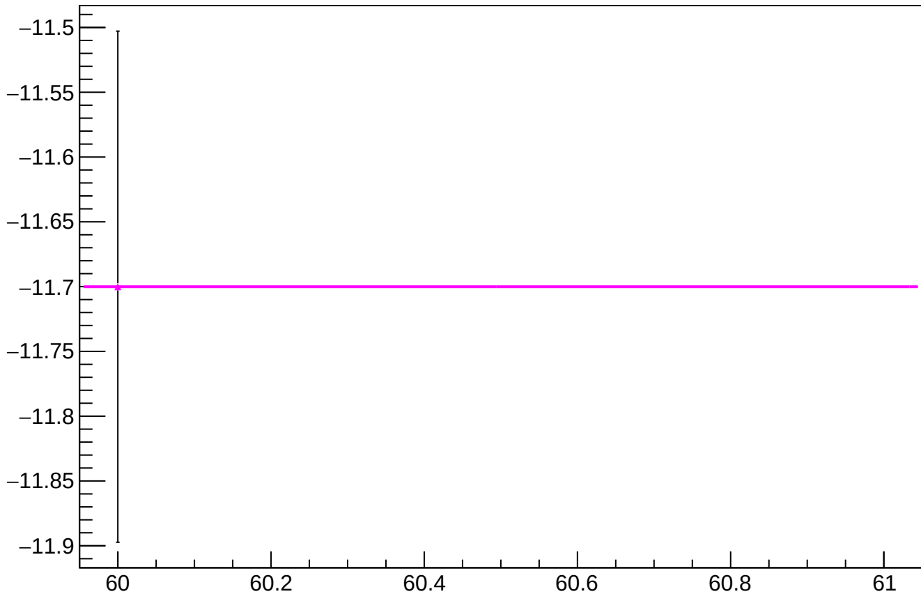
reg_asym_bcm_dg_ds_diff_bpm4aX_slope vs slug
