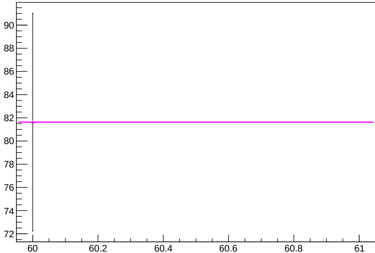
reg_asym_sam_26_dd_diff_bpm4eY_slope vs slug
