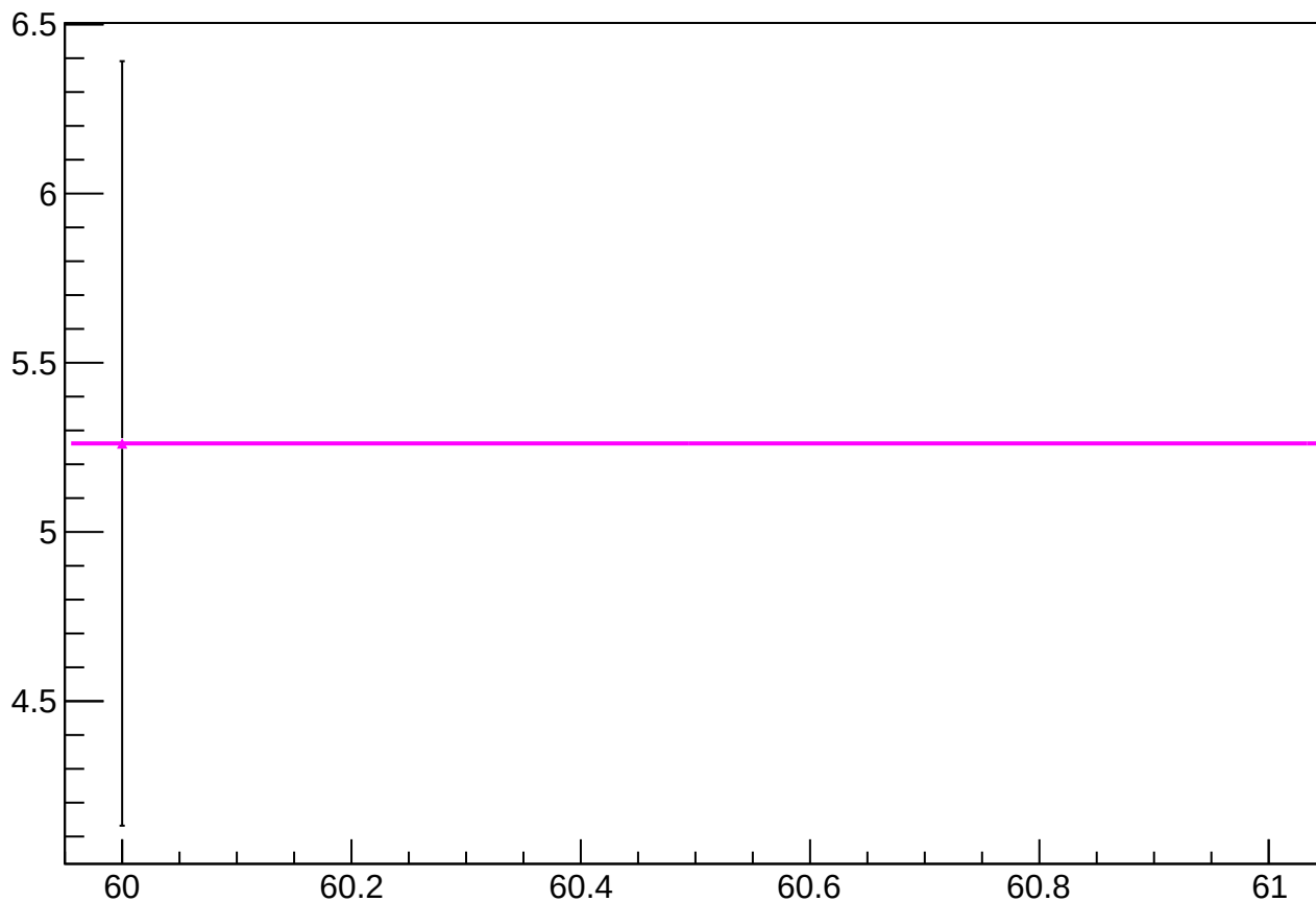
reg_asym_usr_diff_bpm4eY_slope vs slug
