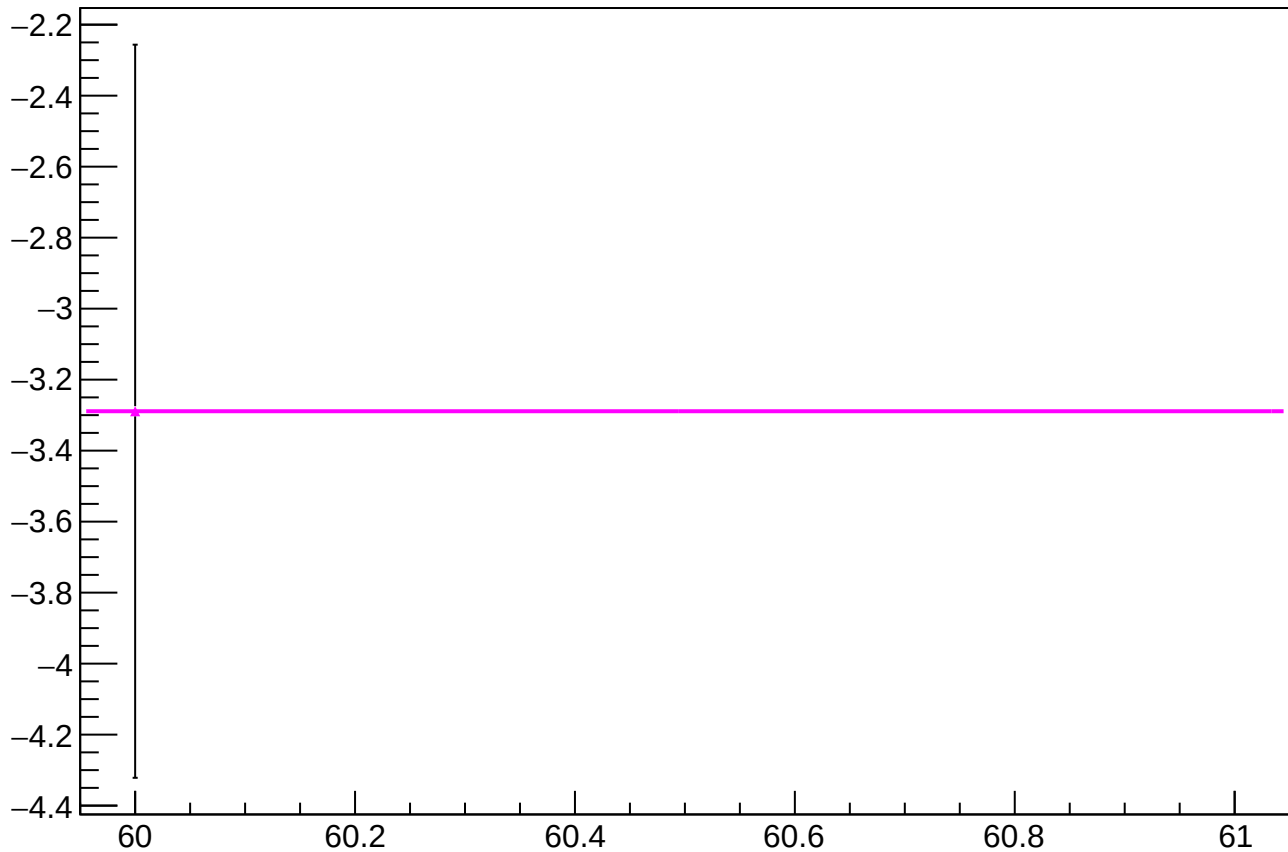
reg_asym_left_avg_diff_bpm4aY_slope vs slug
