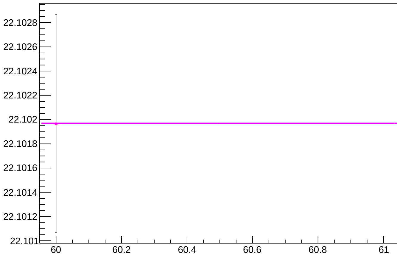
yield_sam4_mean vs slug
