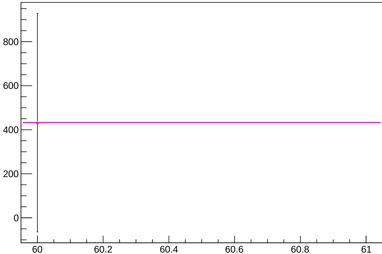
reg_asym_sam7_mean vs slug
