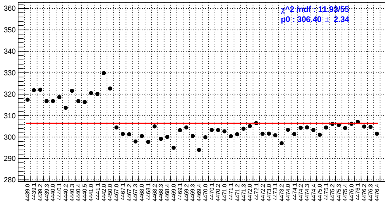
slug60: reg_asym_atr2.rms/ppm
