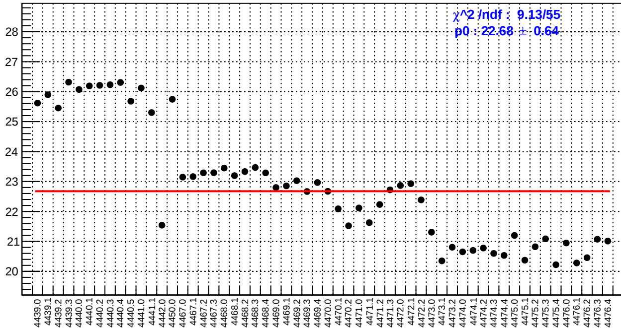
slug60: right_avg_bpm4eX/(ppb/nm)
