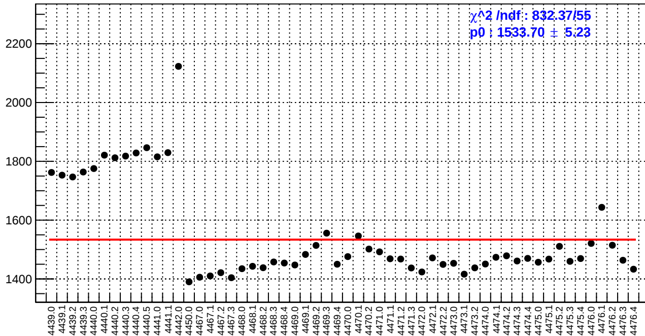
slug60: reg_asym_sam4.rms/ppm
