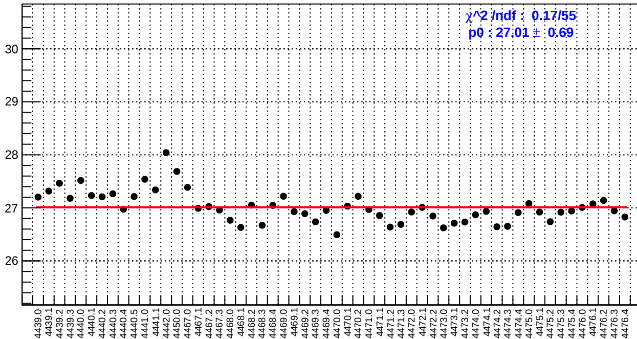
slug60: reg_asym_right_dd.rms/ppm
