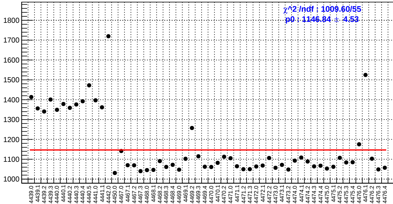
slug60: reg_asym_sam3.rms/ppm
