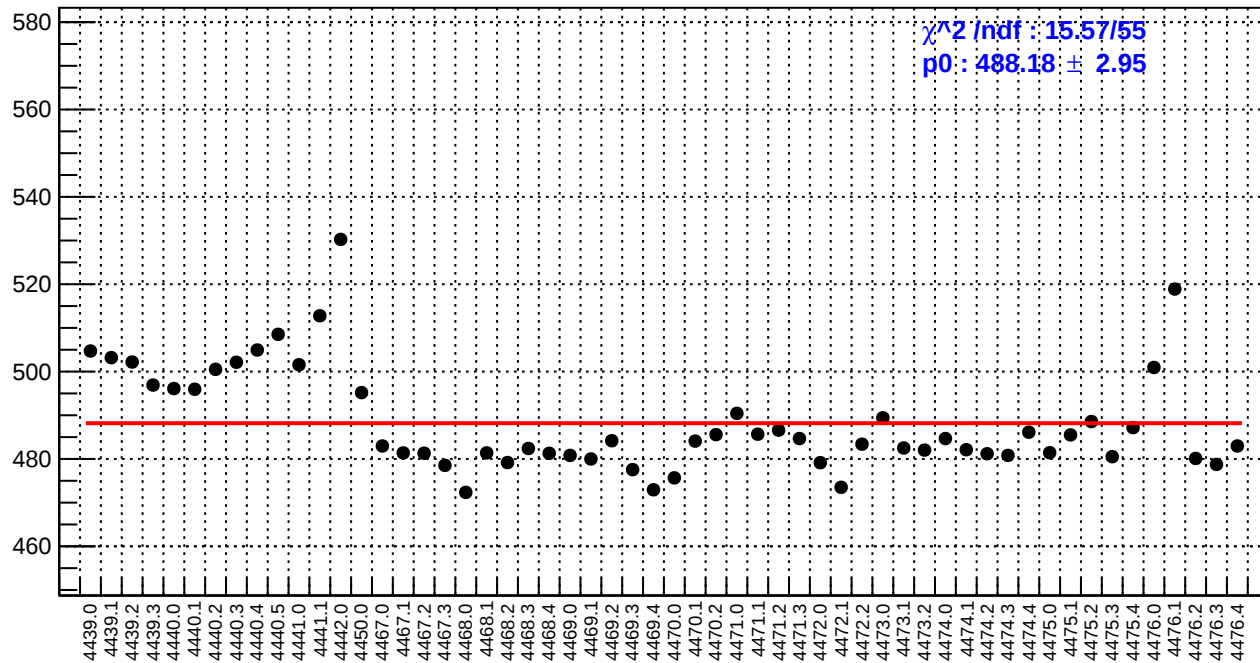
slug60: reg_asym_atr1.rms/ppm
