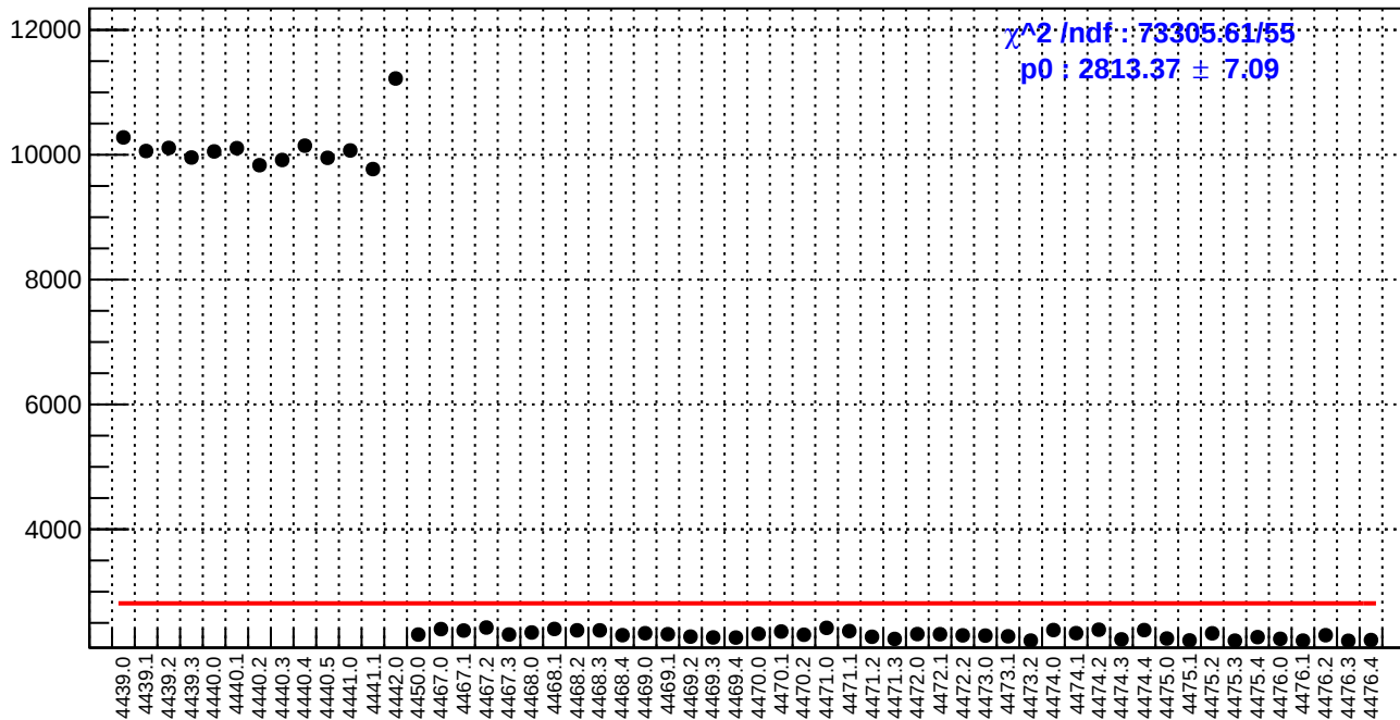
slug60: diff_bpm4aY.rms/nm
