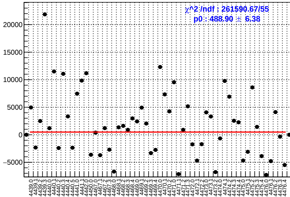
slug60: asym_right_avg.mean/ppb-reg_asym_right_avg.mean/ppb
