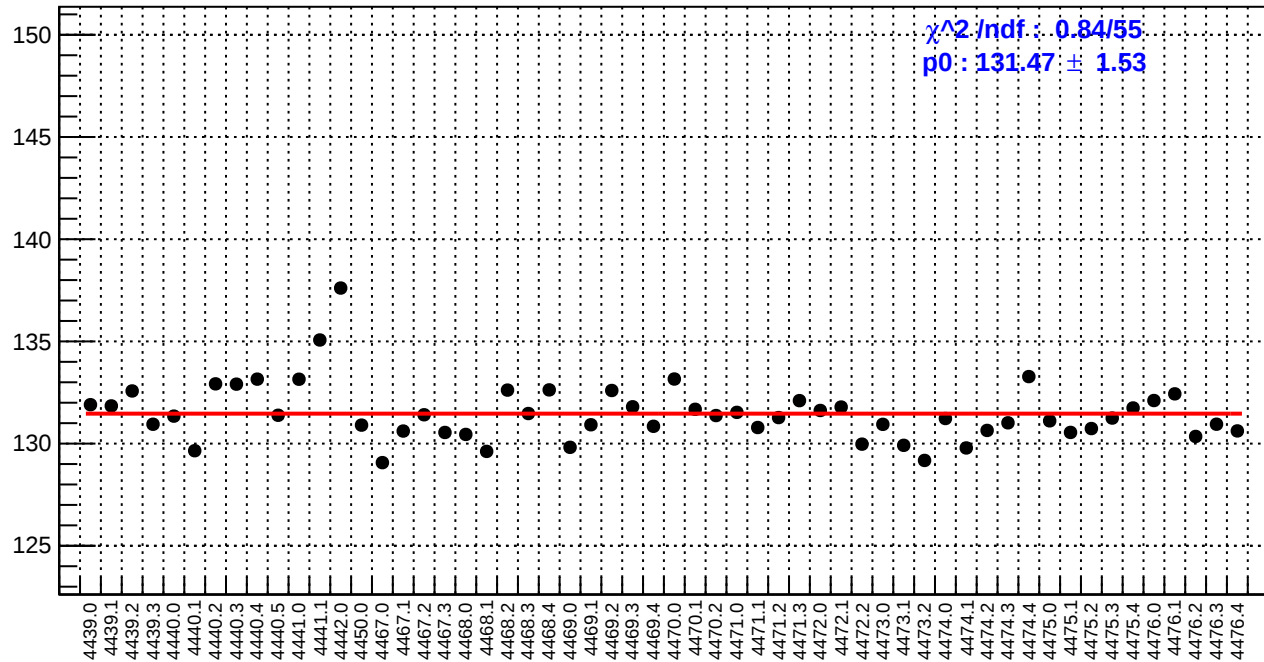
slug60: reg_asym_usr.rms/ppm
