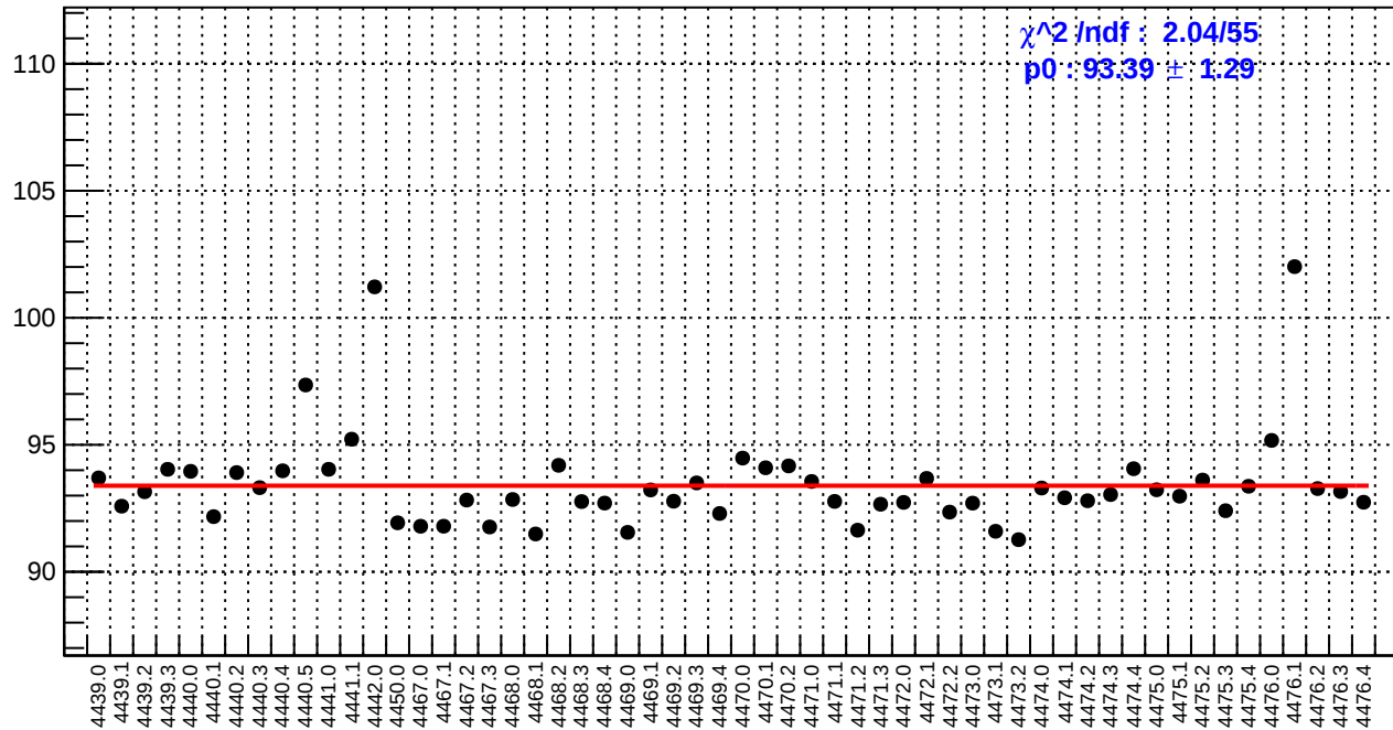
slug60: reg_asym_us_dd.rms/ppm
