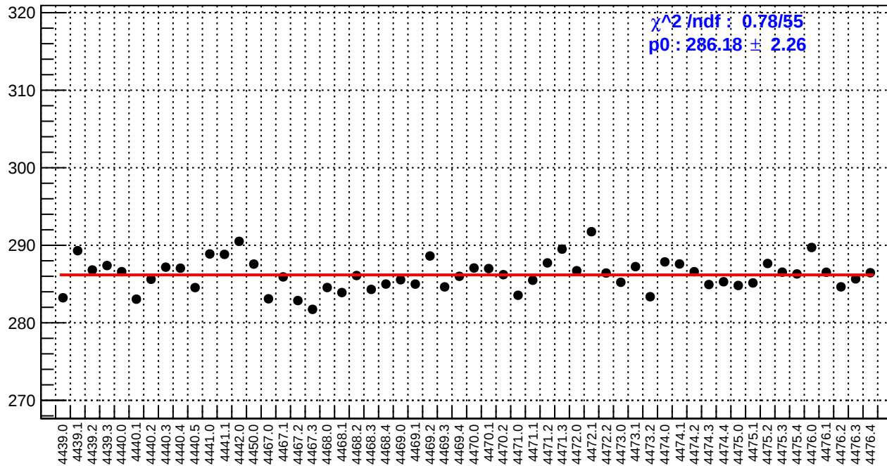
slug60: reg_asym_atl1r2_dd.rms/ppm
