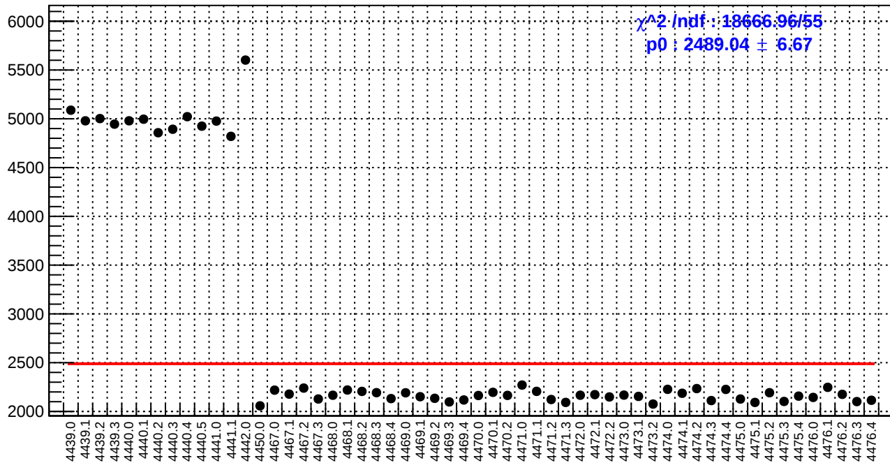
slug60: diff_bpm4eY.rms/nm
