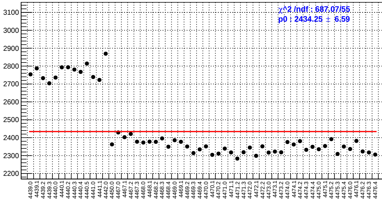
slug60: reg_asym_sam2.rms/ppm
