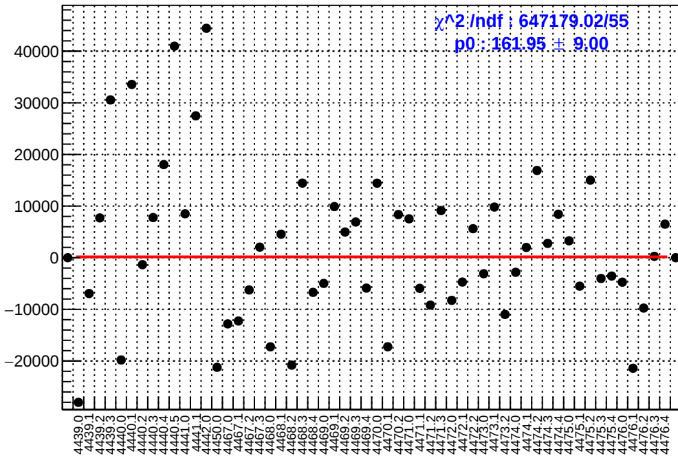
slug60: asym_at1_avg.mean/ppb-reg_asym_at1_avg.mean/ppb
