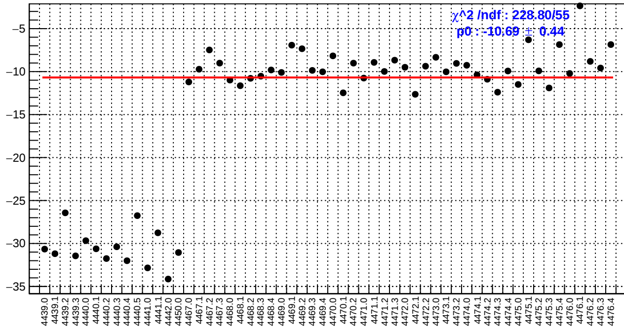
slug60: usr_bpm4aX/(ppb/nm)
