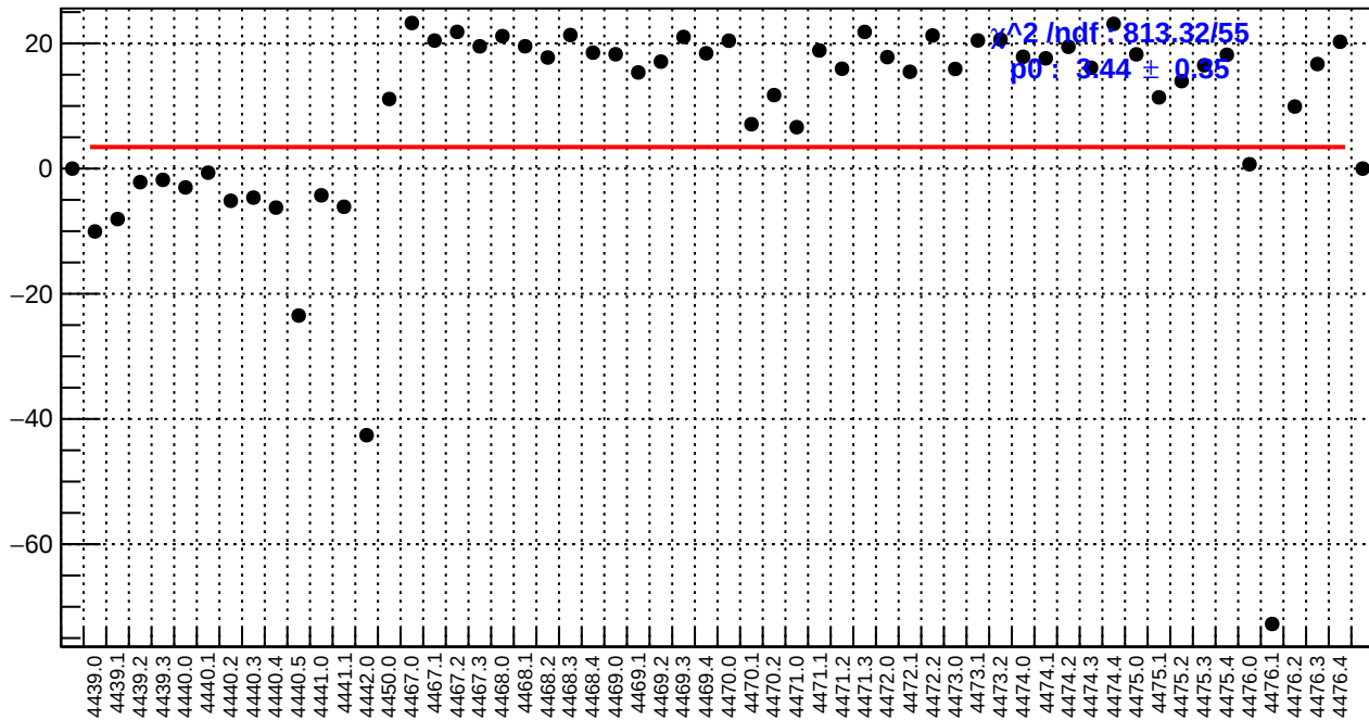
slug60: left_avg_bpm4eY/(ppb/nm)
