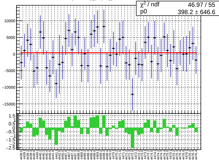
slug60: reg_asym_sam8.mean/ppb
