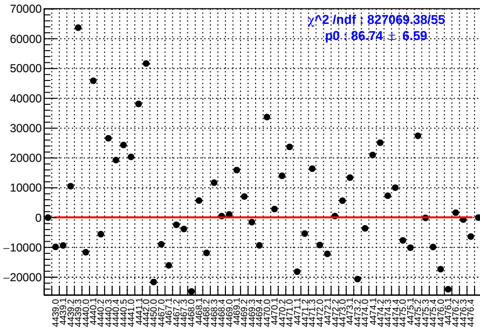
slug60: asym_atl1r2_avg.mean/ppb-reg_asym_atl1r2_avg.mean/ppb
