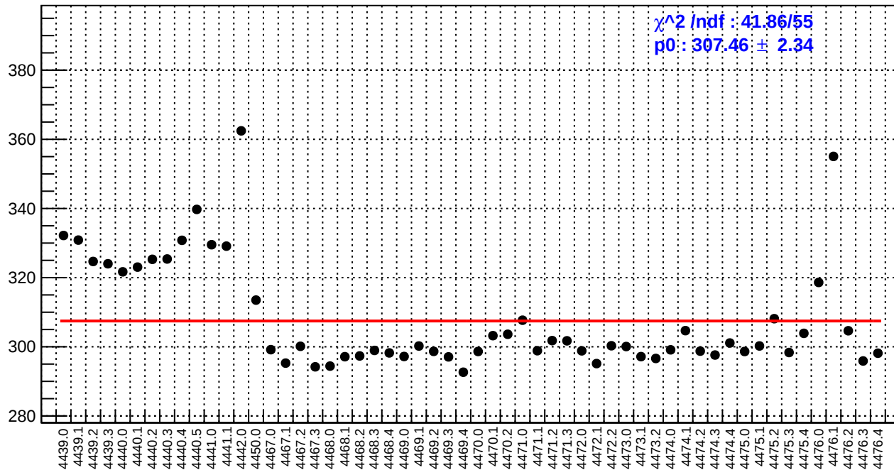
slug60: reg_asym_atr1l2_avg.rms/ppm
