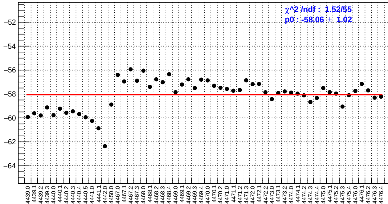
slug60: right_avg_bpm12X/(ppb/nm)
