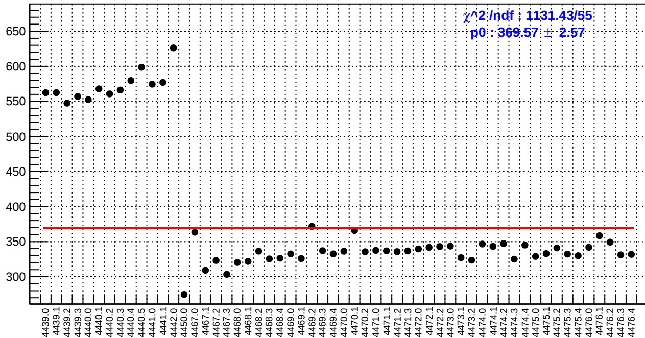
slug60: reg_asym_sam6.rms/ppm
