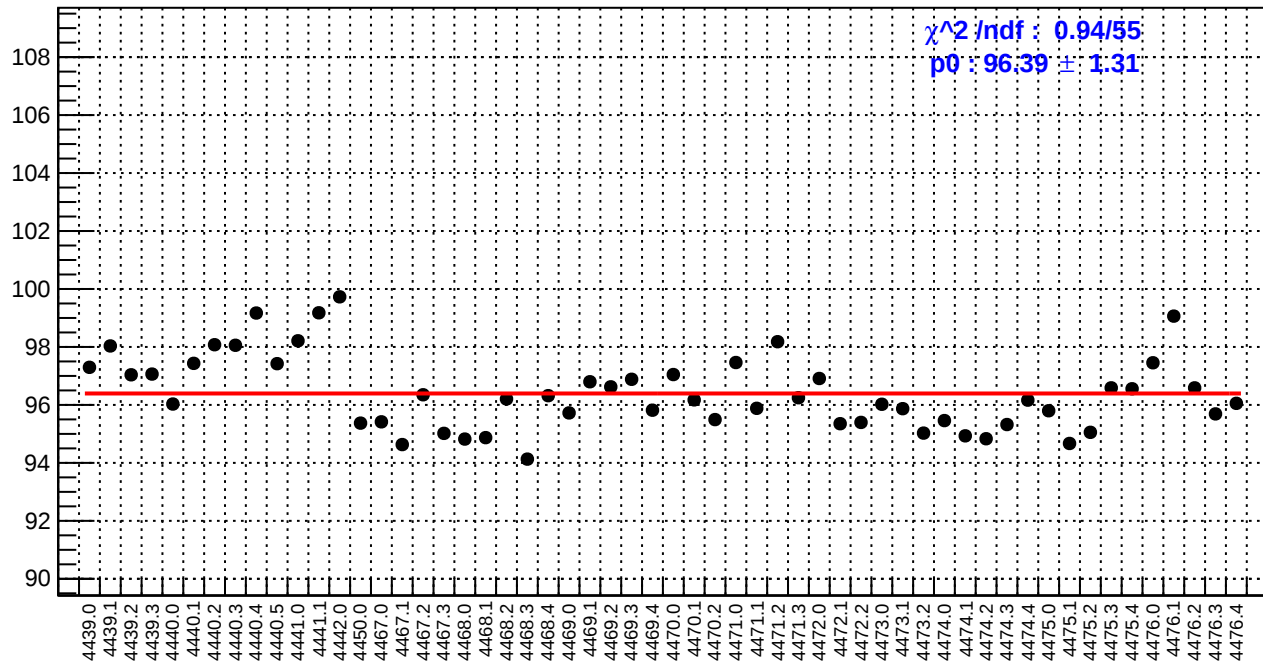
slug60: reg_asym_us_avg.rms/ppm
