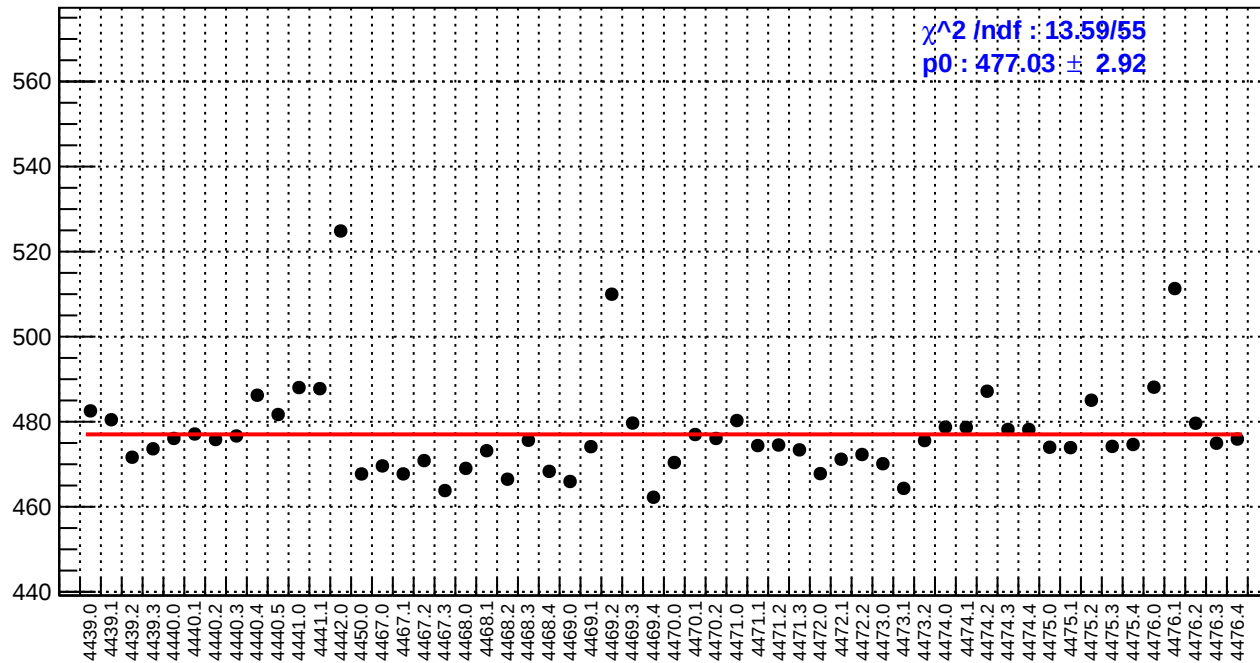
slug60: reg_asym_sam8.rms/ppm
