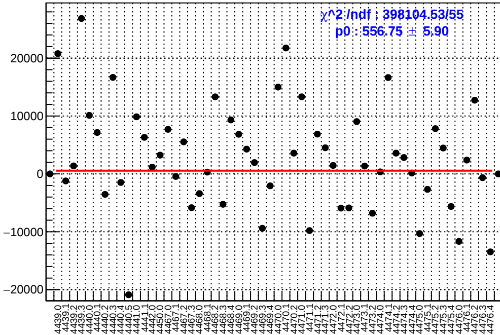
slug60: asym_atl_dd.mean/ppb-reg_asym_atl_dd.mean/ppb
