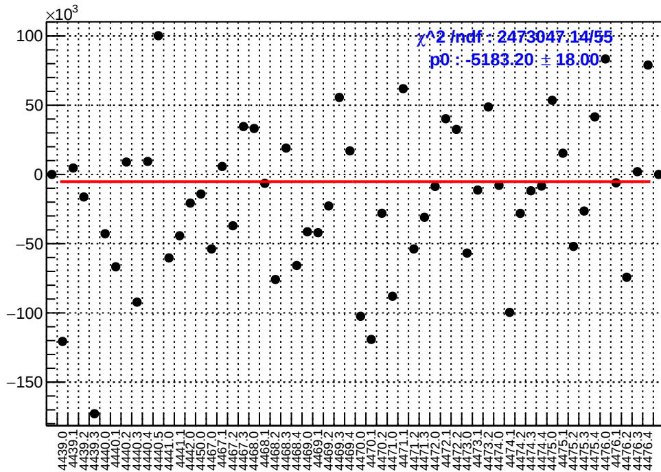
slug60: asym_sam4.mean/ppb-reg_asym_sam4.mean/ppb
