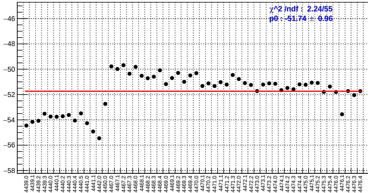
slug60: ds_avg_bpm12X/(ppb/nm)
