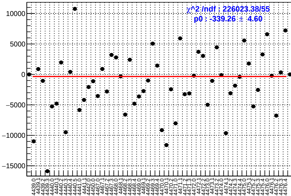
slug60: asym_us_dd.mean/ppb-reg_asym_us_dd.mean/ppb
