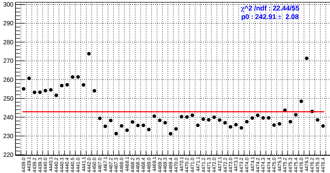
slug60: reg_asym_at2_avg.rms/ppm
