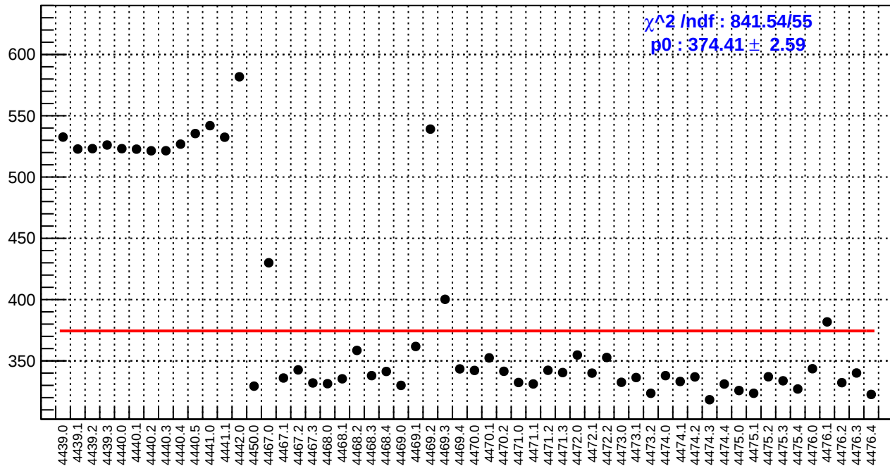
slug60: reg_asym_sam7.rms/ppm
