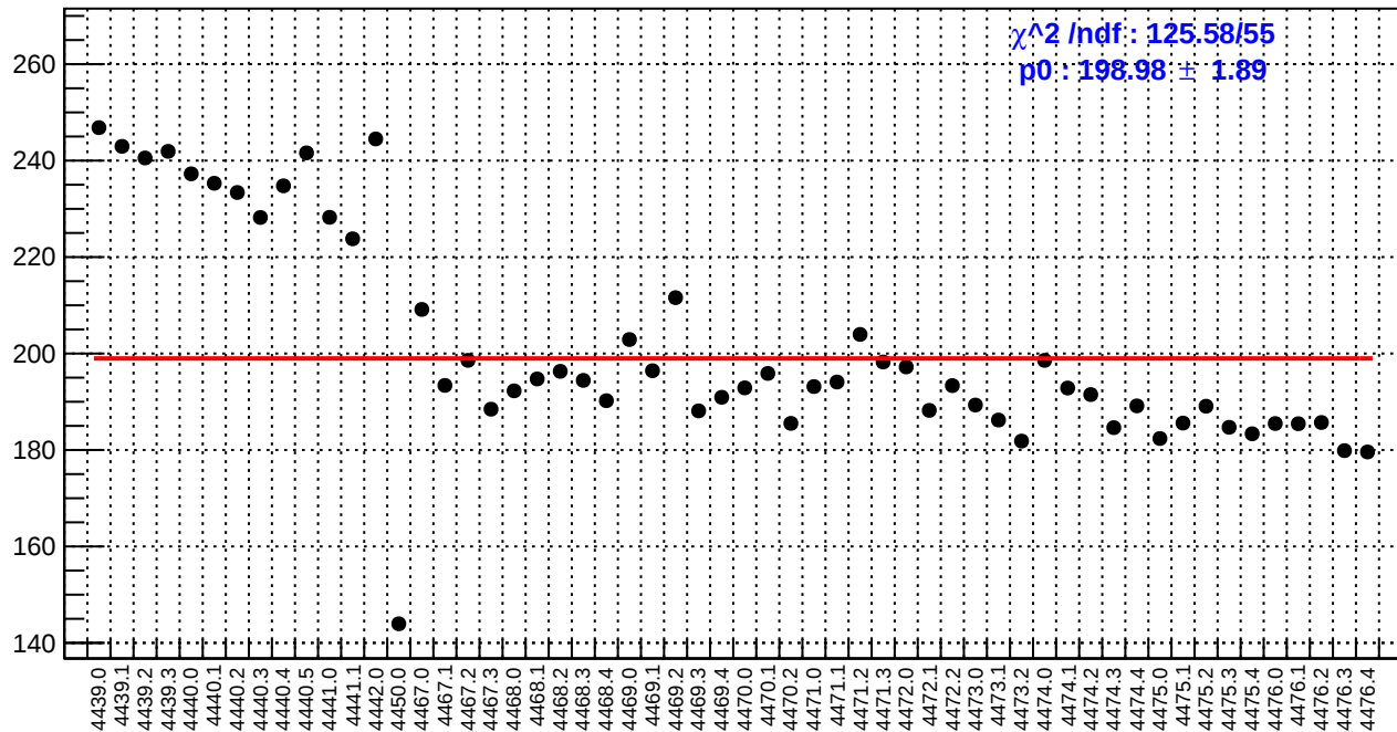
slug60: reg_asym_sam1.rms/ppm
