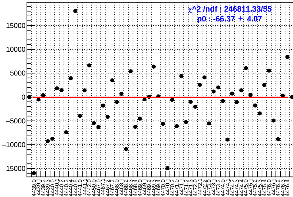
slug60: asym_usl.mean/ppb-reg_asym_usl.mean/ppb
