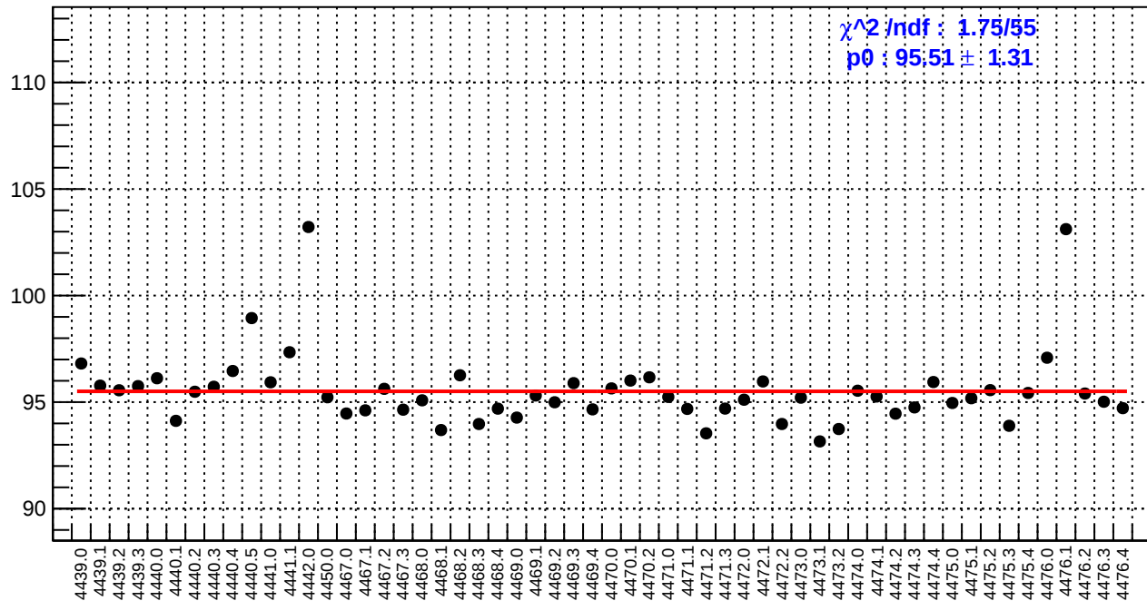
slug60: reg_asym_ds_dd.rms/ppm
