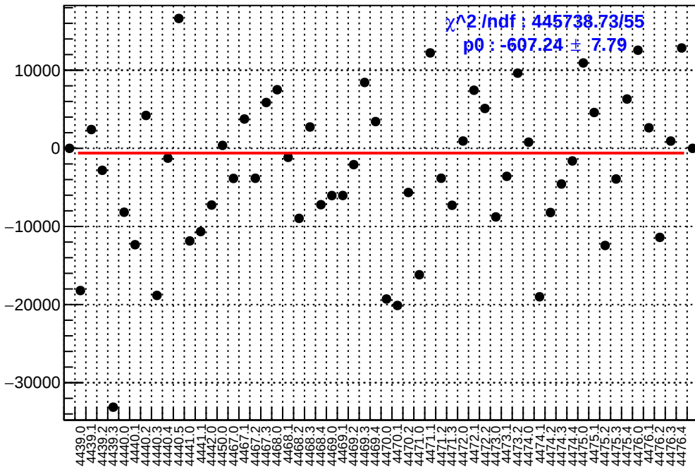
slug60: asym_atr_dd.mean/ppb-reg_asym_atr_dd.mean/ppb
