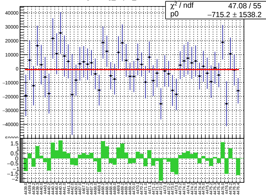
slug60: reg_asym_sam3.mean/ppb
