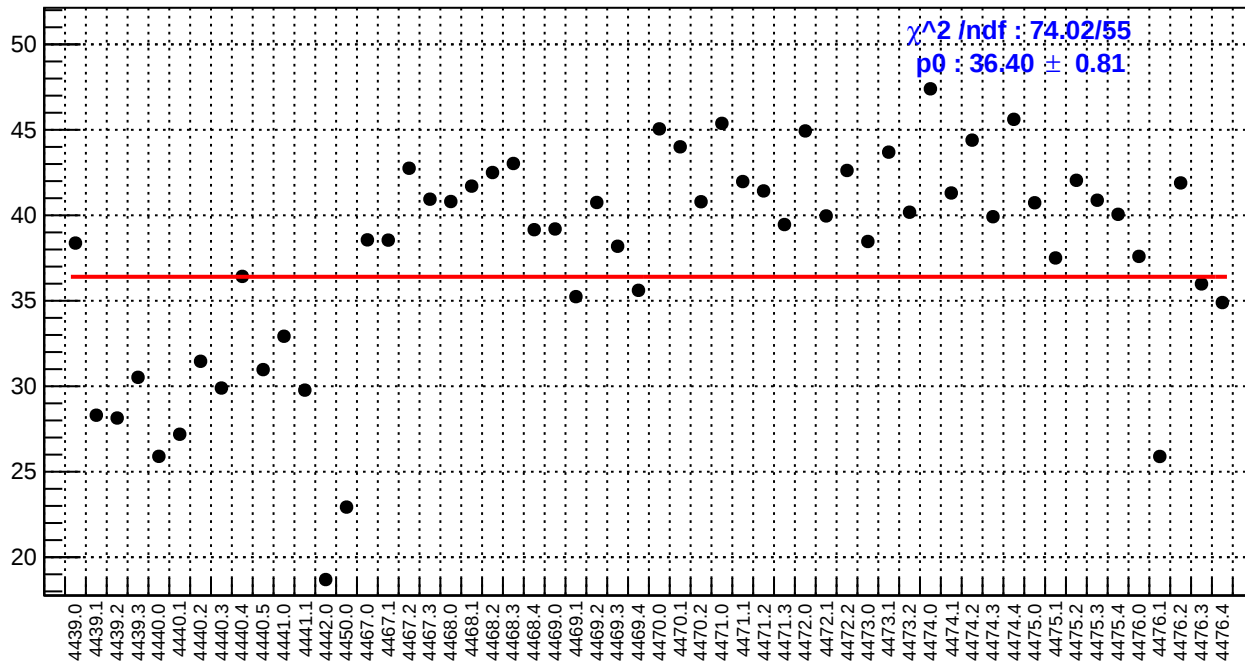
slug60: usl_bpm4aX/(ppb/nm)
