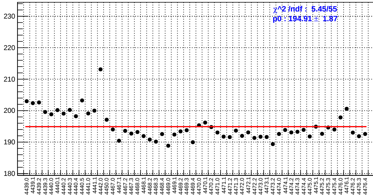
slug60: reg_asym_at2_dd.rms/ppm
