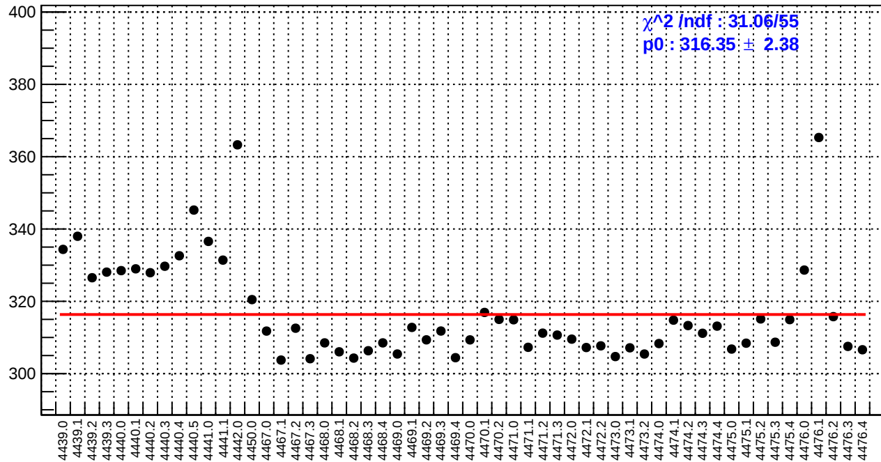
slug60: reg_asym_atl2.rms/ppm
