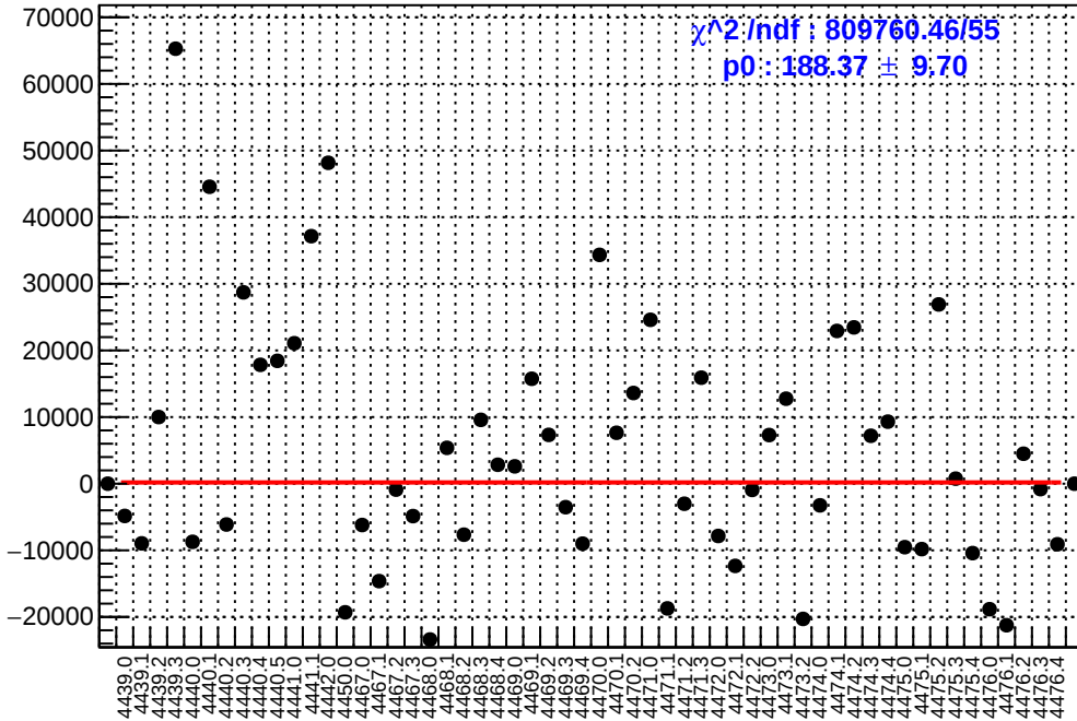
slug60: asym_atl1.mean/ppb-reg_asym_atl1.mean/ppb
