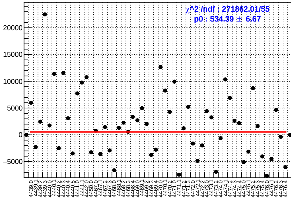
slug60: asym_usr.mean/ppb-reg_asym_usr.mean/ppb
