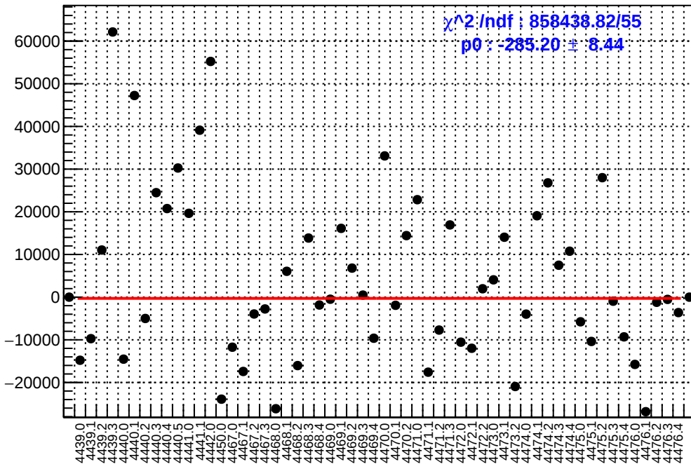
slug60: asym_atr2.mean/ppb-reg_asym_atr2.mean/ppb
