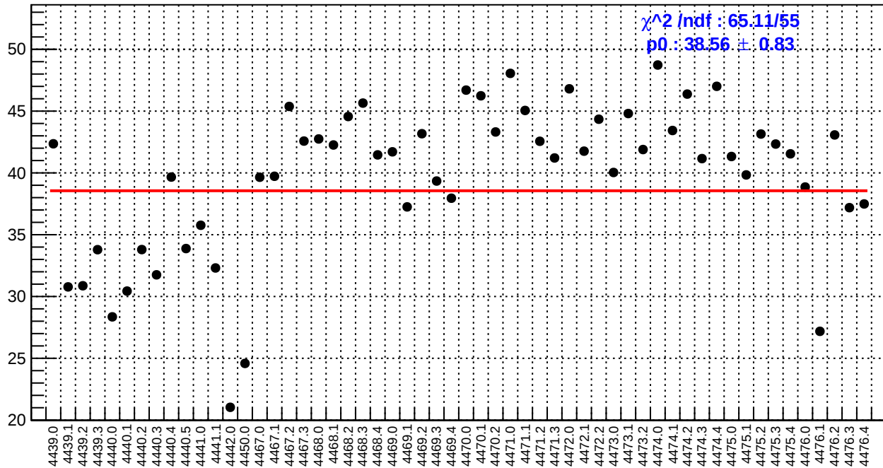
slug60: dsl_bpm4aX/(ppb/nm)
