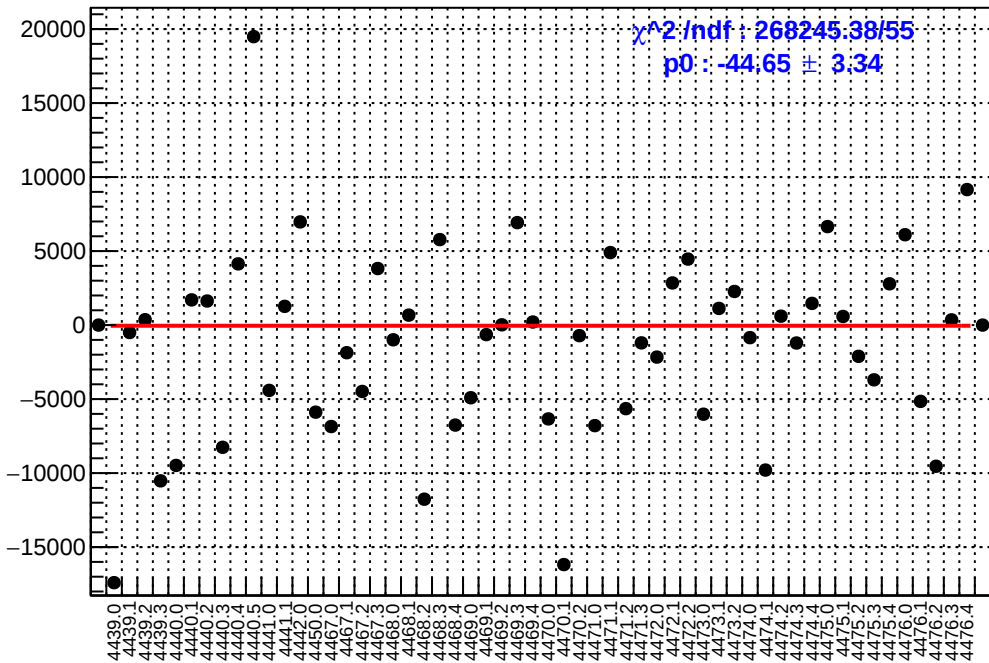
slug60: asym_dsl.mean/ppb-reg_asym_dsl.mean/ppb
