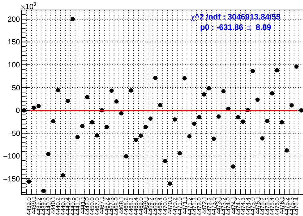
slug60: asym_sam2.mean/ppb-reg_asym_sam2.mean/ppb
