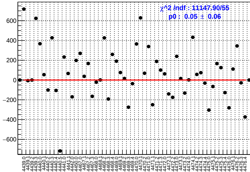
slug60: asym_left_dd.mean/ppb-reg_asym_left_dd.mean/ppb
