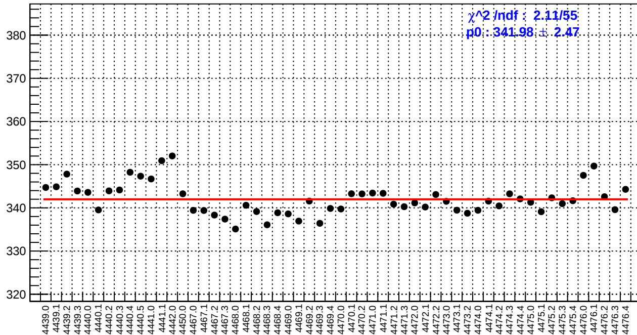
slug60: reg_asym_at1_dd.rms/ppm
