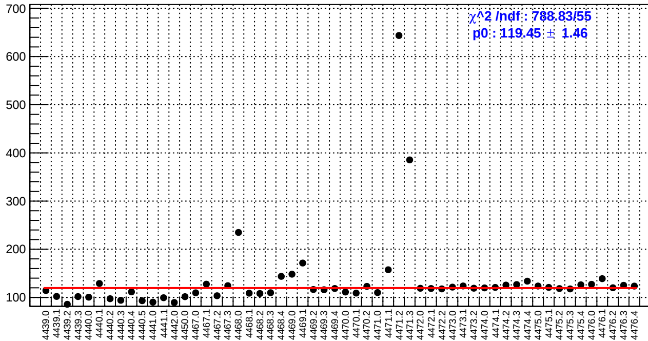
slug60: asym_bcm_an_ds3.rms/ppm
