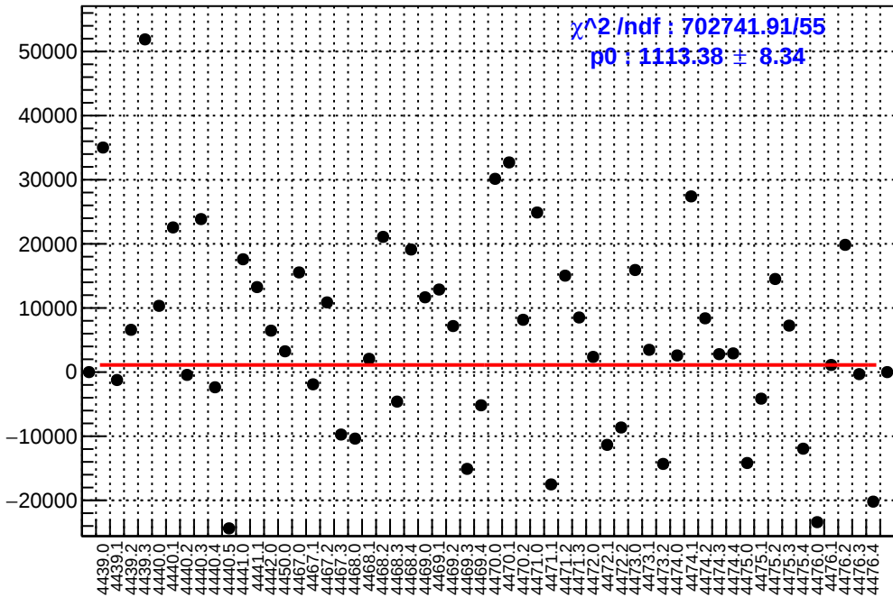
slug60: asym_sam8.mean/ppb-reg_asym_sam8.mean/ppb
