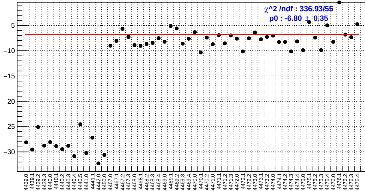
slug60: right_avg_bpm4aX/(ppb/nm)
