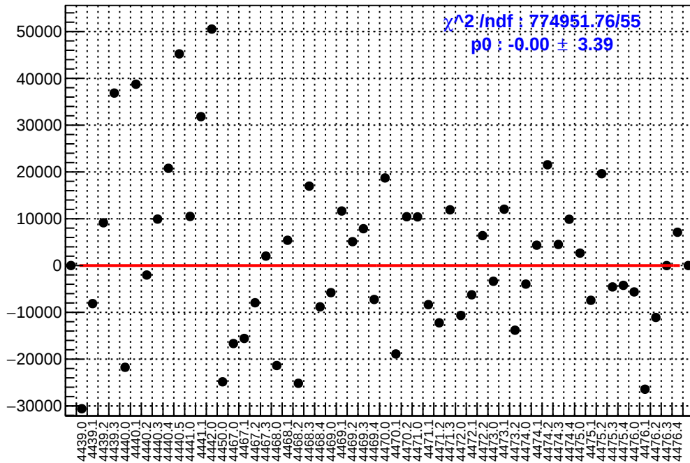
slug60: asym_at2_avg.mean/ppb-reg_asym_at2_avg.mean/ppb
