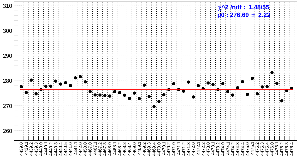
slug60: reg_asym_atr_dd.rms/ppm
