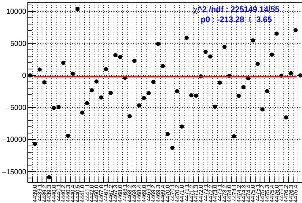
slug60: asym_ds_dd.mean/ppb-reg_asym_ds_dd.mean/ppb
