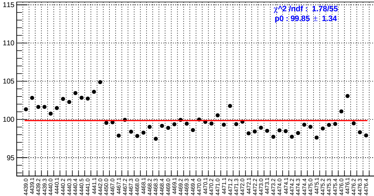
slug60: reg_asym_ds_avg.rms/ppm
