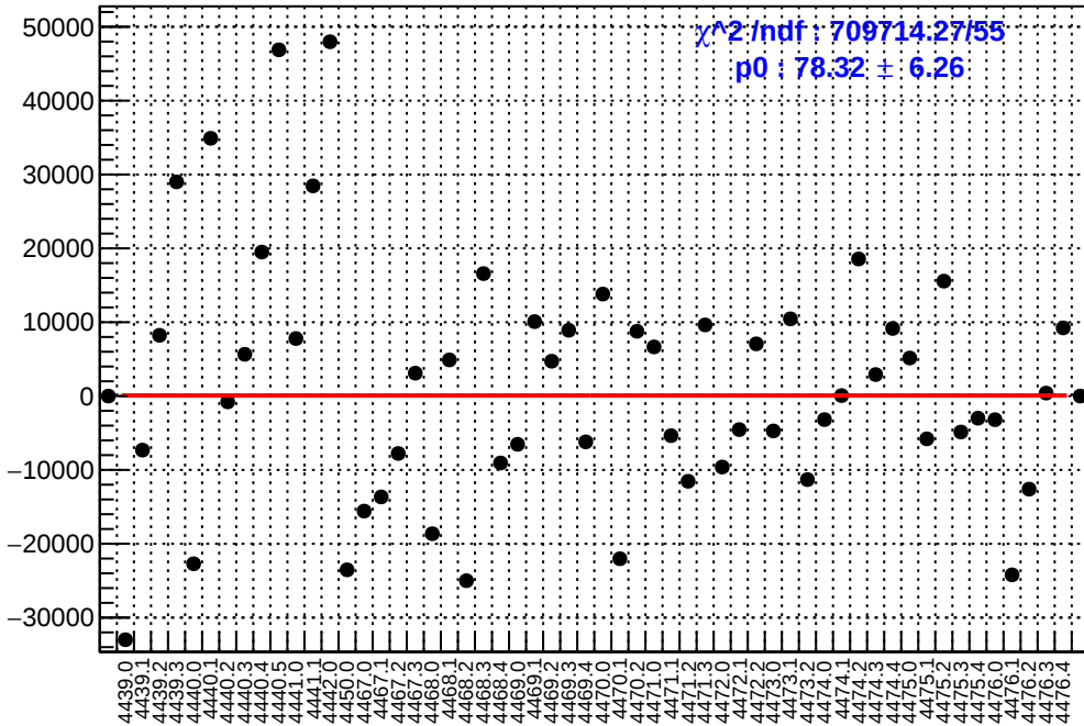
slug60: asym_atr_avg.mean/ppb-reg_asym_atr_avg.mean/ppb
