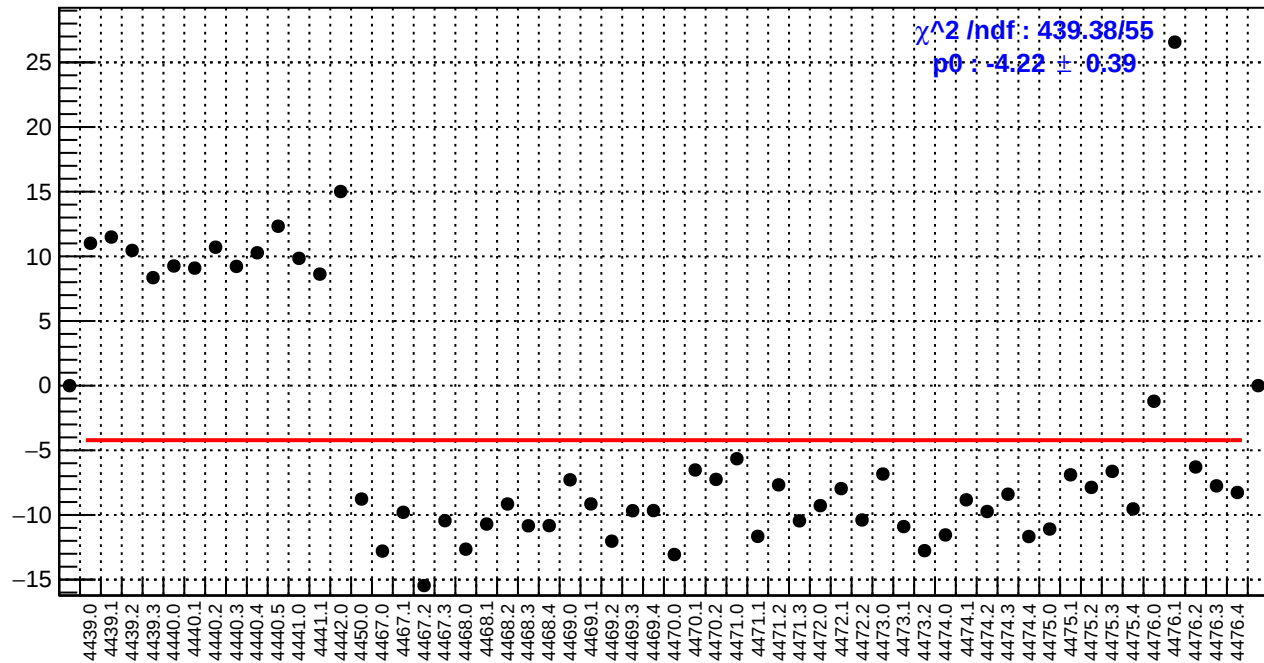
slug60: ds_avg_bpm4aY/(ppb/nm)
