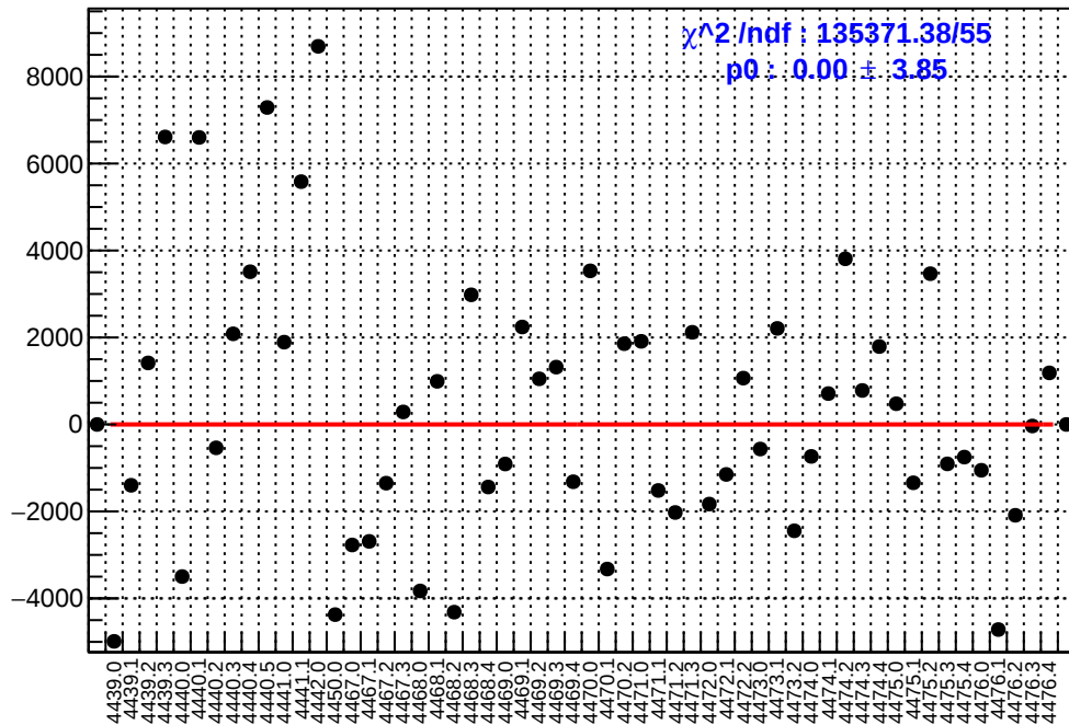
slug60: asym_us_avg.mean/ppb-reg_asym_us_avg.mean/ppb
