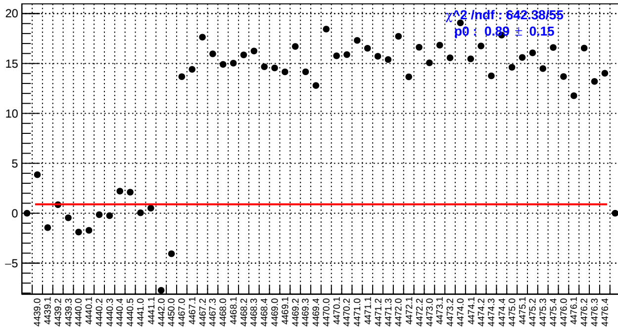
slug60: us_avg_bpm4aX/(ppb/nm)
