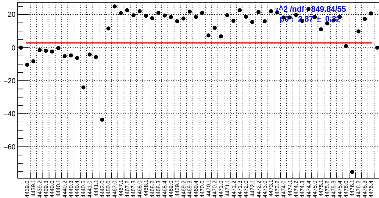
slug60: dsl_bpm4eY/(ppb/nm)
