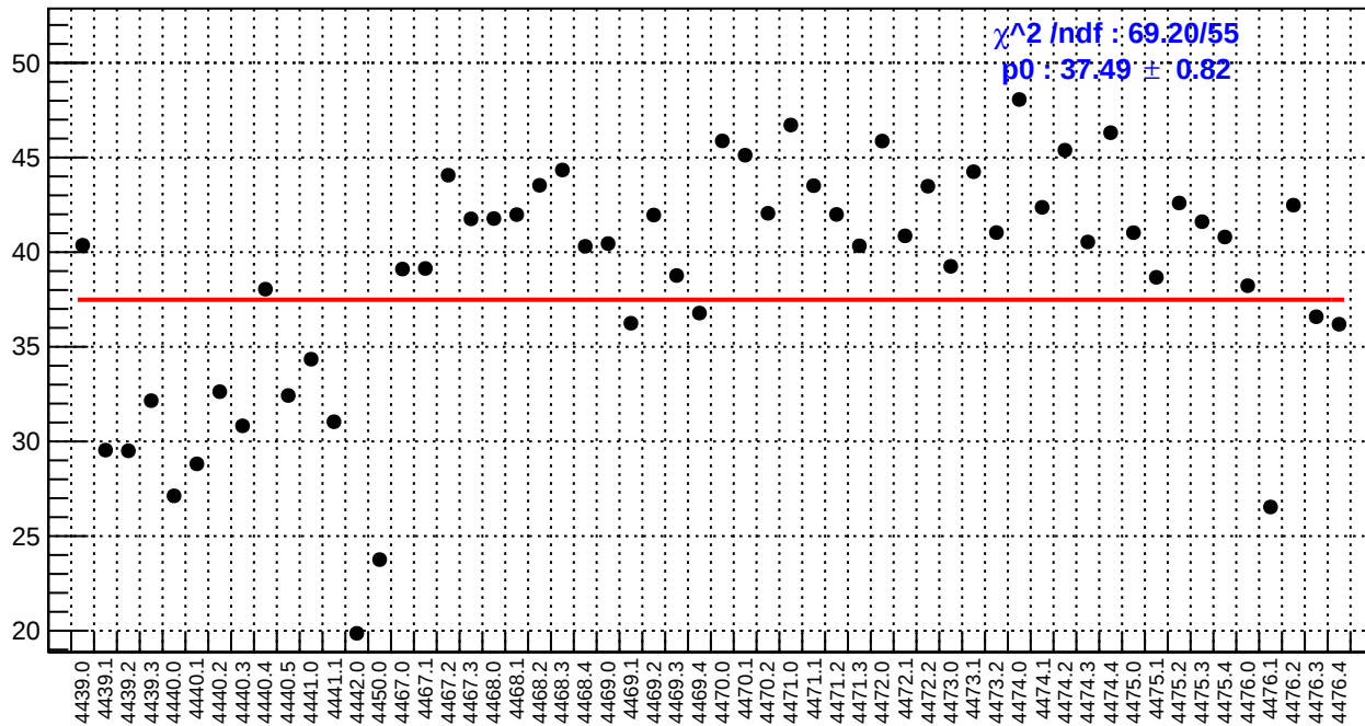
slug60: left_avg_bpm4aX/(ppb/nm)
