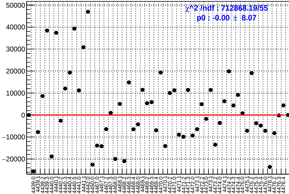
slug60: asym_atl_avg.mean/ppb-reg_asym_atl_avg.mean/ppb
