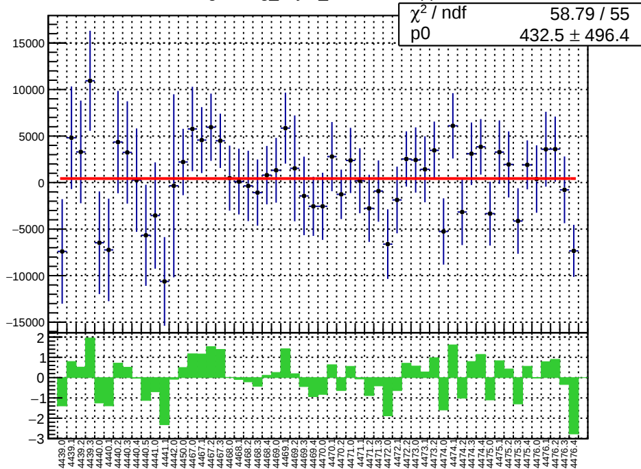
slug60: reg_asym_sam7.mean/ppb
