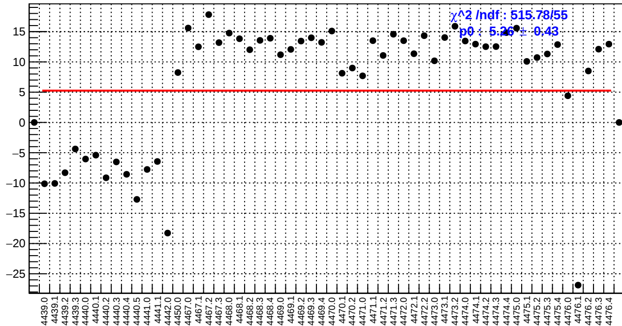
slug60: ds_avg_bpm4eY/(ppb/nm)
