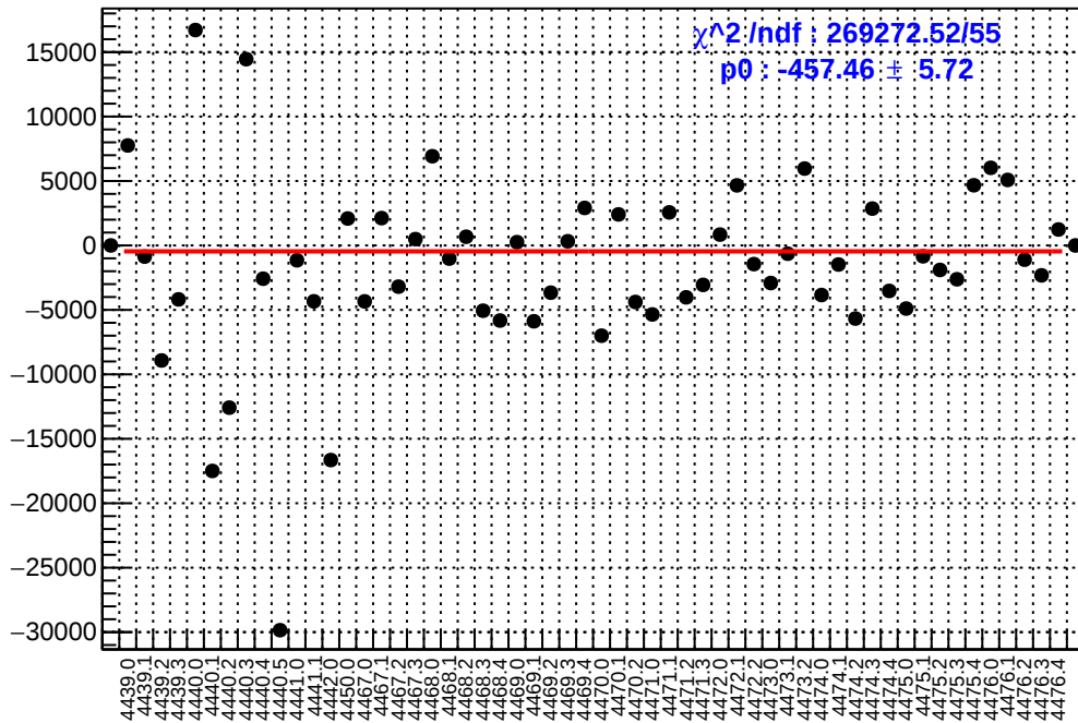
slug60: asym_sam5.mean/ppb-reg_asym_sam5.mean/ppb
