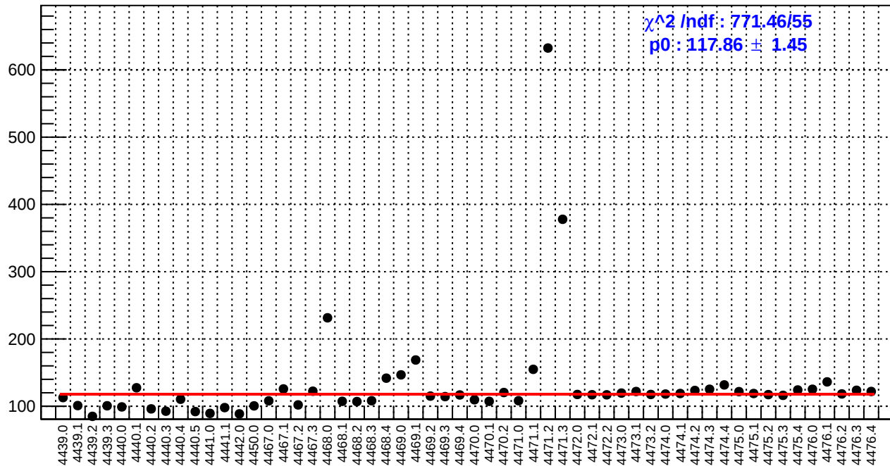
slug60: asym_bcm_an_us.rms/ppm
