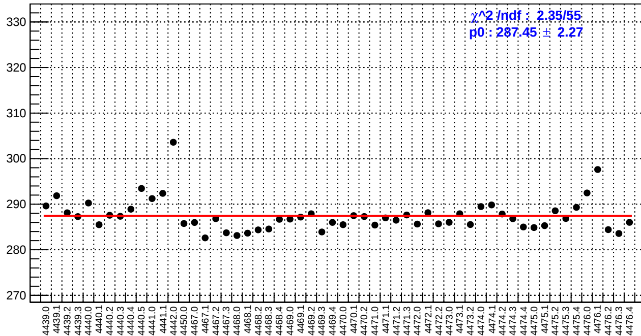
slug60: reg_asym_atl_dd.rms/ppm
