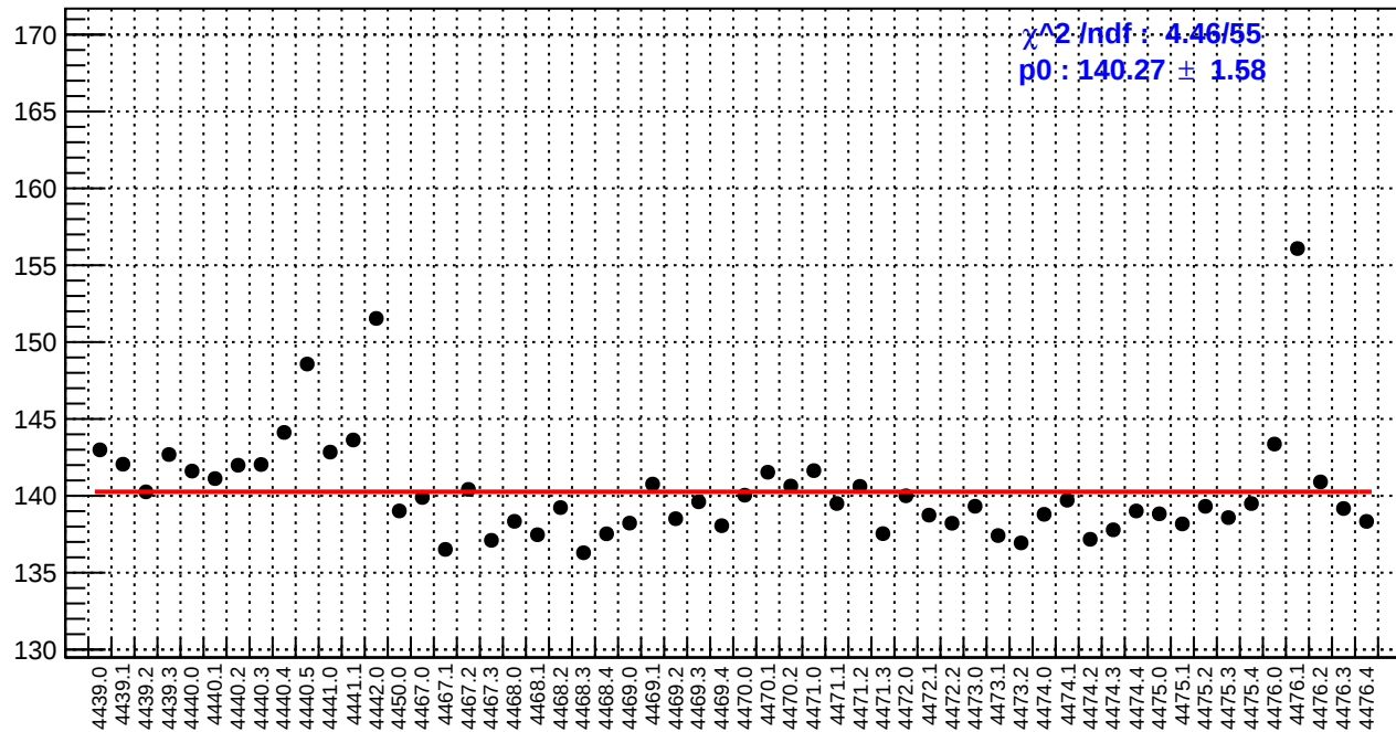
slug60: reg_asym_dsl.rms/ppm
