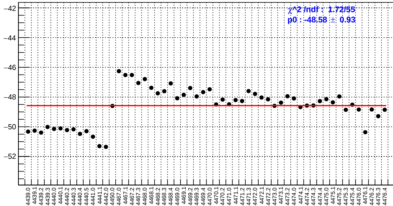
slug60: us_avg_bpm12X/(ppb/nm)
