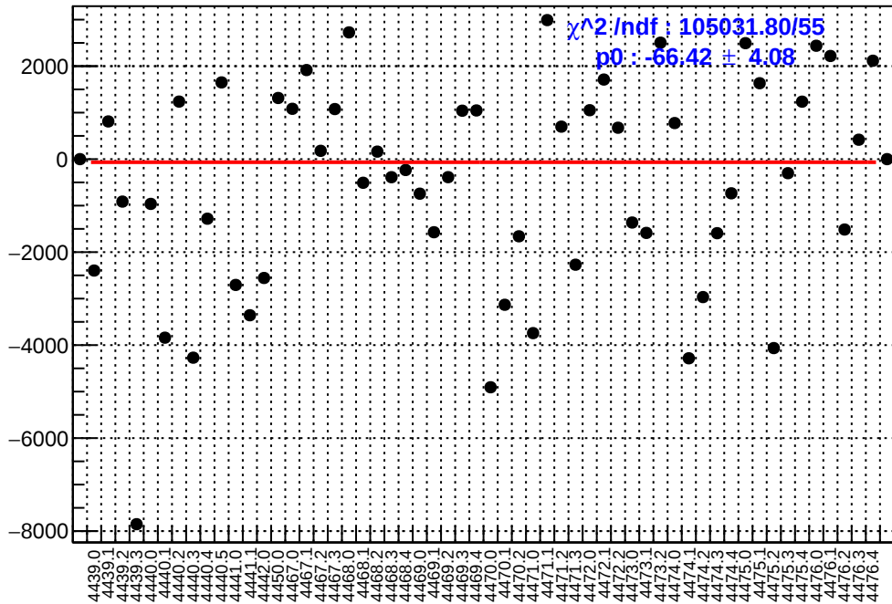
slug60: asym_atr1l2_dd.mean/ppb-reg_asym_atr1l2_dd.mean/ppb
