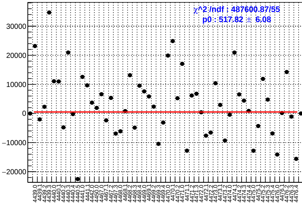
slug60: asym_at1_dd.mean/ppb-reg_asym_at1_dd.mean/ppb
