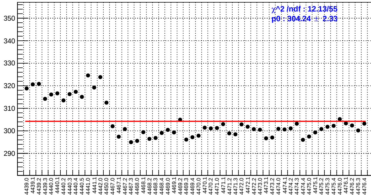
slug60: reg_asym_atl1r2_avg.rms/ppm
