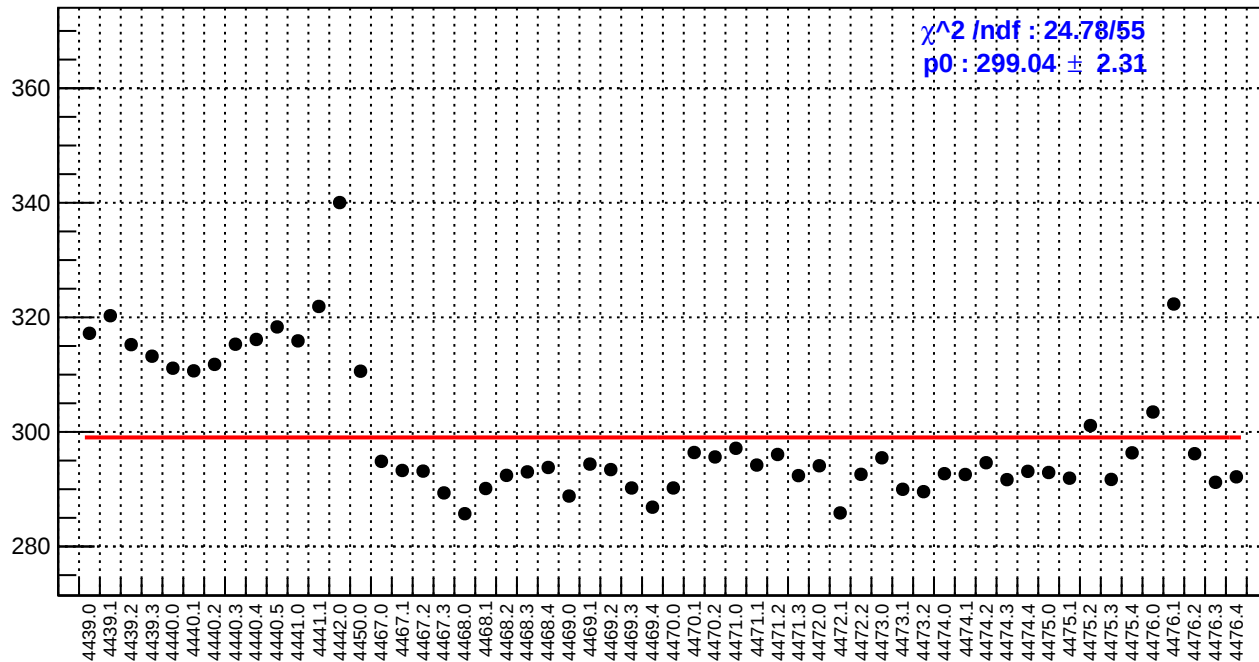
slug60: reg_asym_atr_avg.rms/ppm
