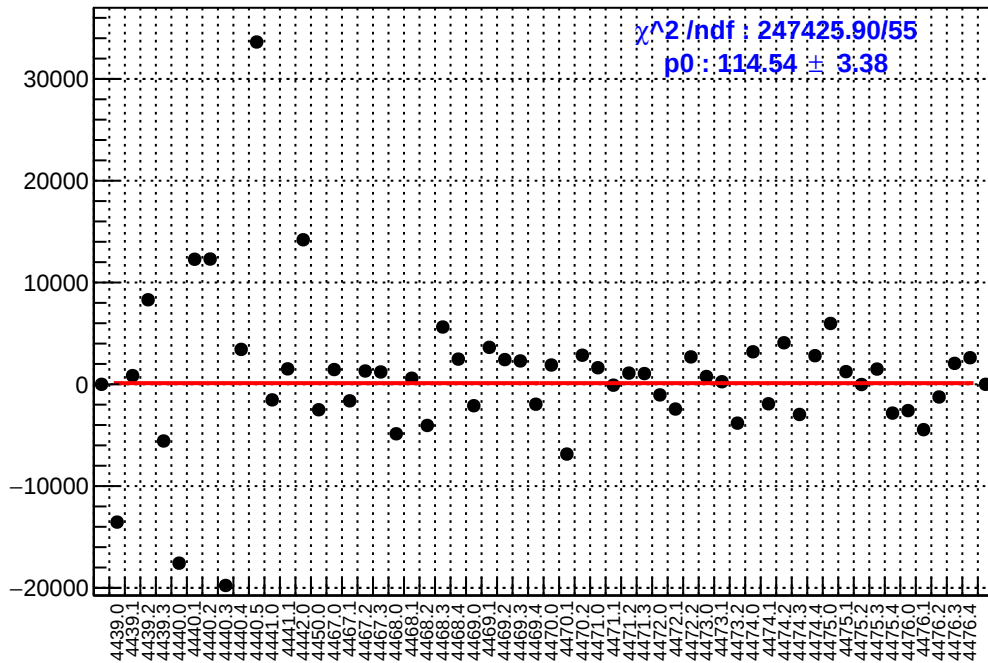
slug60: asym_sam1.mean/ppb-reg_asym_sam1.mean/ppb
