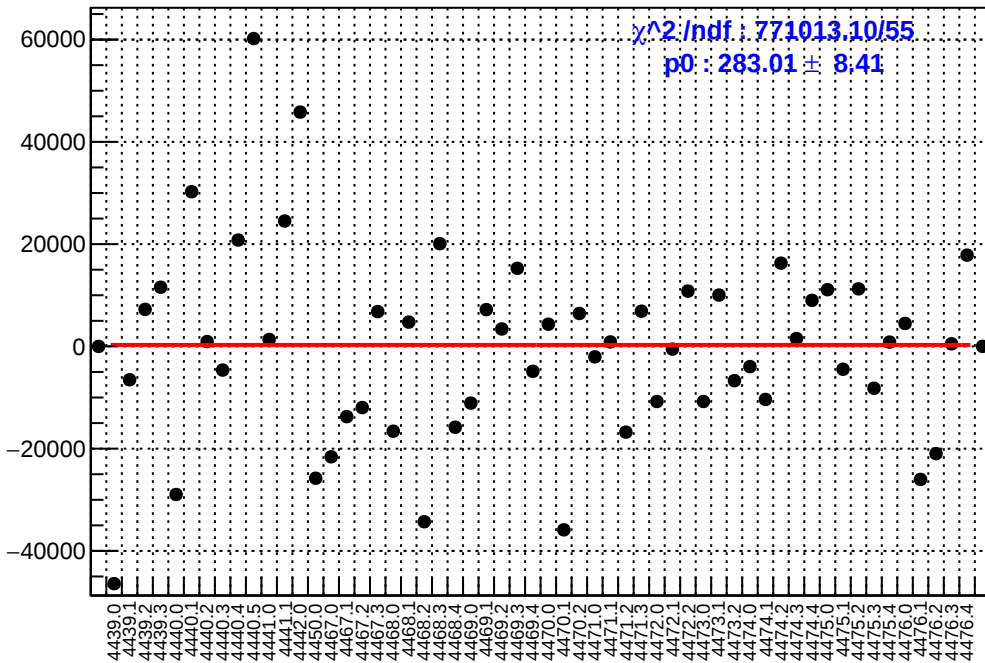
slug60: asym_atl2.mean/ppb-reg_asym_atl2.mean/ppb
