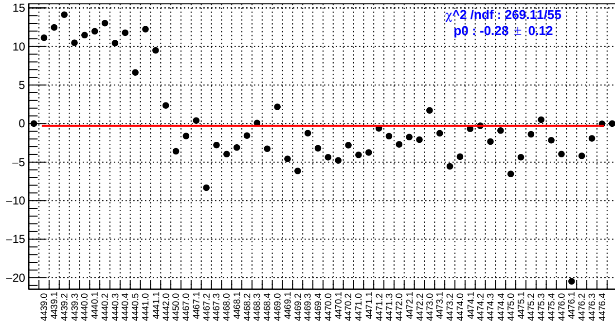
slug60: right_avg_bpm4aY/(ppb/nm)
