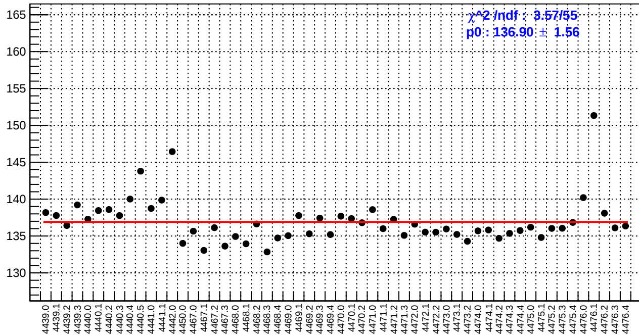
slug60: reg_asym_usl.rms/ppm
