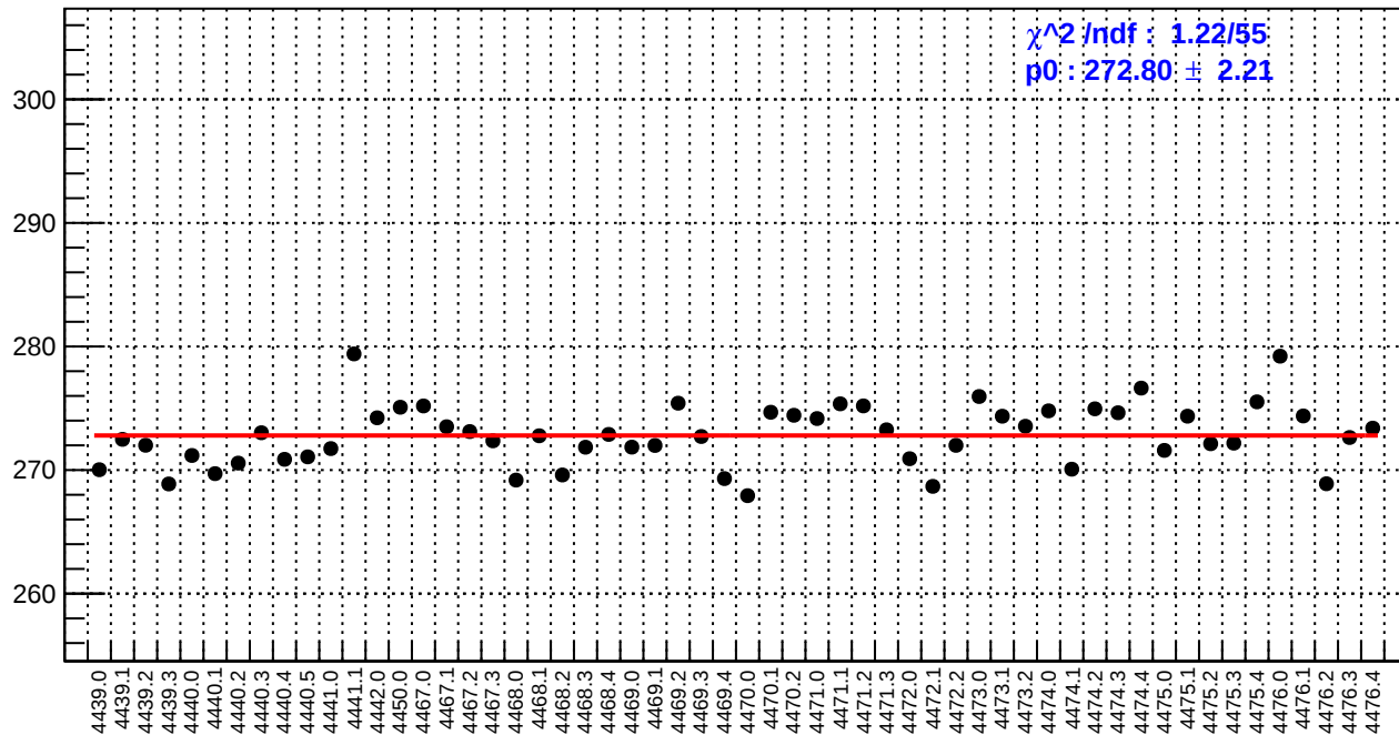
slug60: reg_asym_atr1l2_dd.rms/ppm
