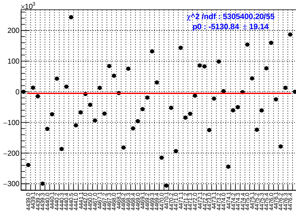
slug60: asym_sam3.mean/ppb-reg_asym_sam3.mean/ppb
