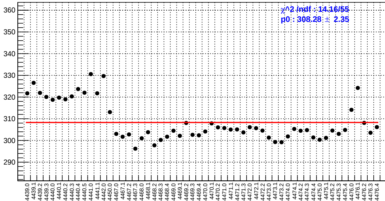
slug60: reg_asym_atl_avg.rms/ppm
