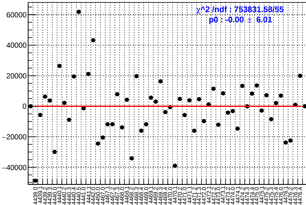
slug60: asym_atr1l2_avg.mean/ppb-reg_asym_atr1l2_avg.mean/ppb
