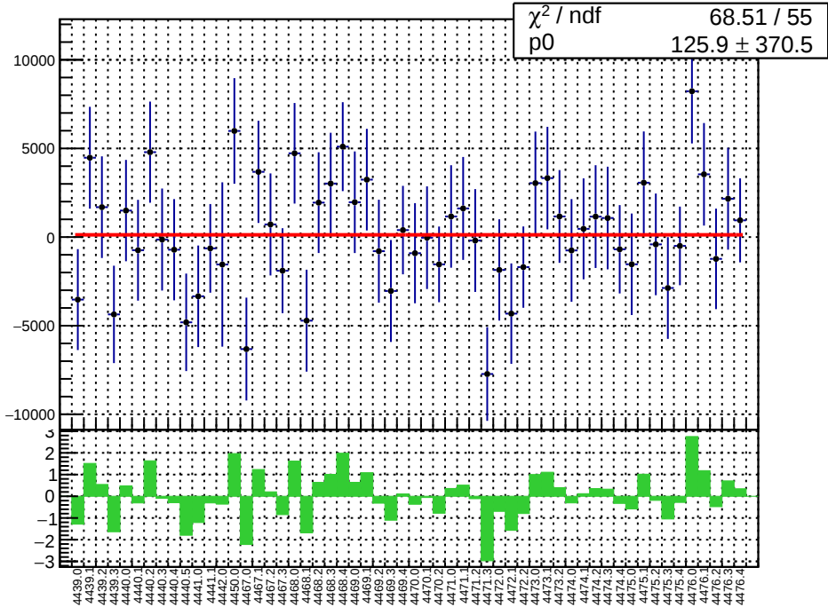
slug60: reg_asym_atr1l2_dd.mean/ppb
