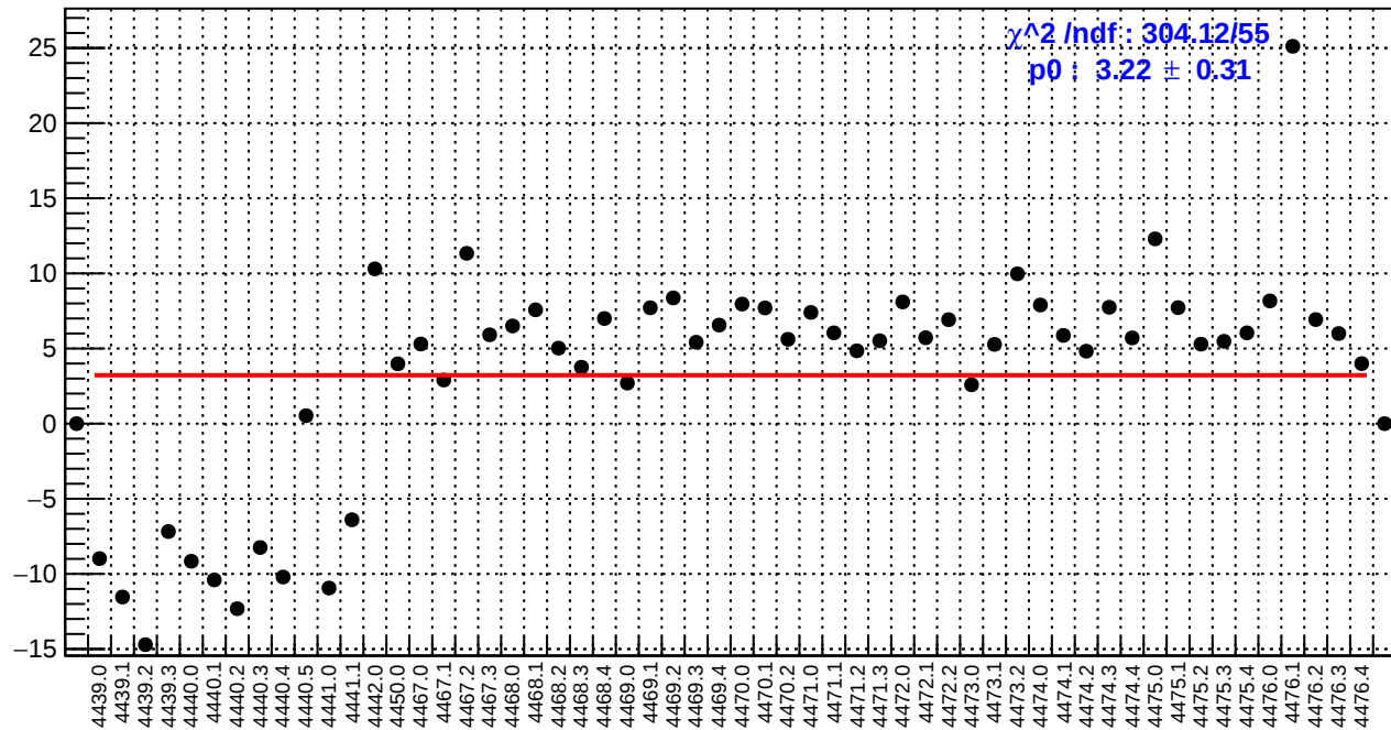
slug60: right_avg_bpm4eY/(ppb/nm)
