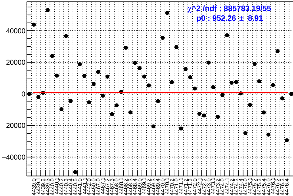
slug60: asym_sam7.mean/ppb-reg_asym_sam7.mean/ppb
