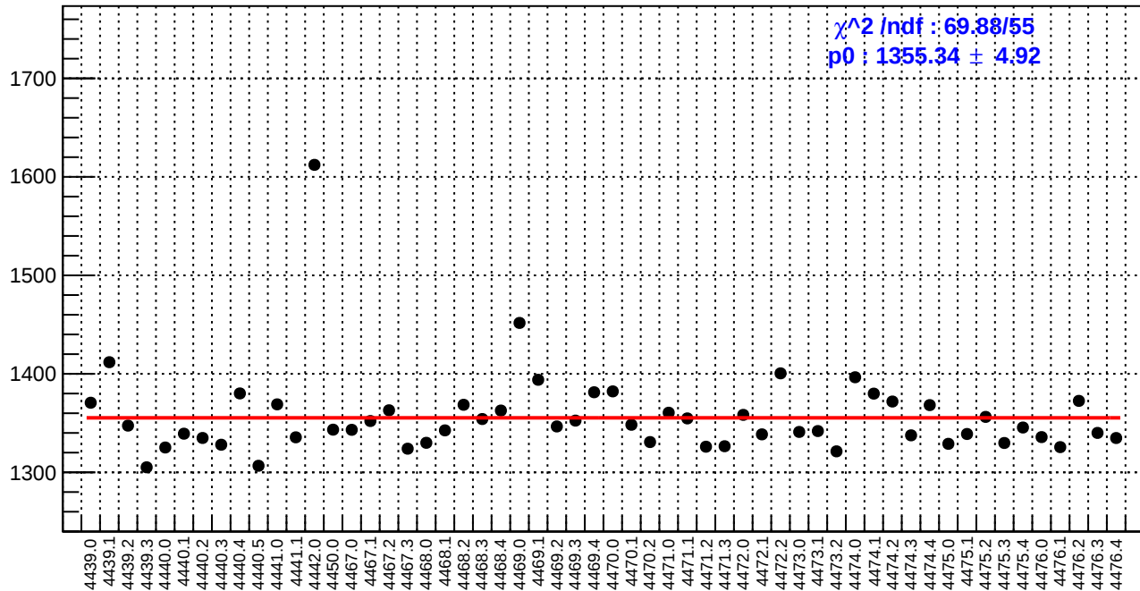
slug60: diff_bpm4aX.rms/nm
