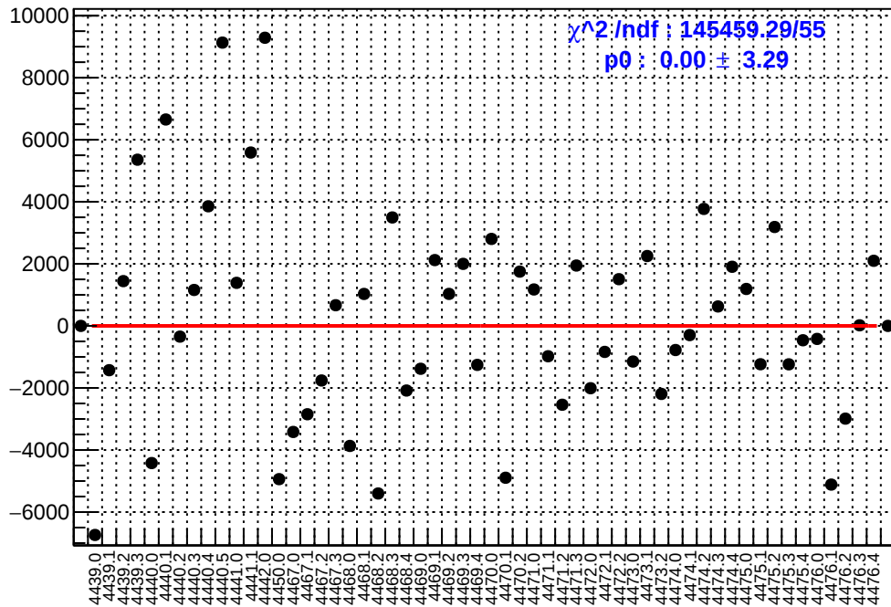
slug60: asym_ds_avg.mean/ppb-reg_asym_ds_avg.mean/ppb
