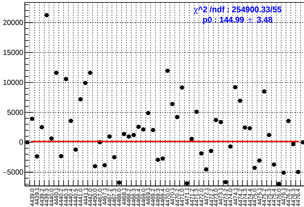
slug60: asym_dsr.mean/ppb-reg_asym_dsr.mean/ppb
