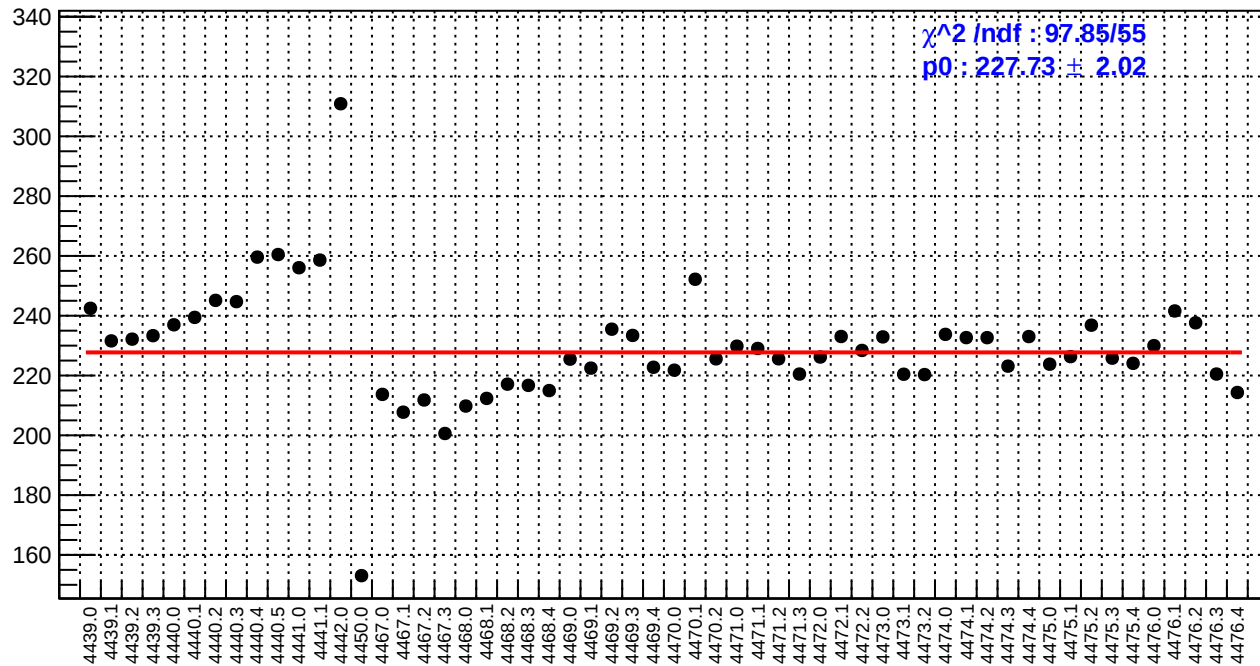
slug60: reg_asym_sam5.rms/ppm
