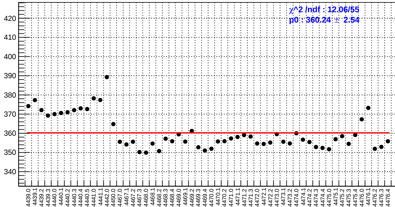
slug60: reg_asym_at1_avg.rms/ppm
