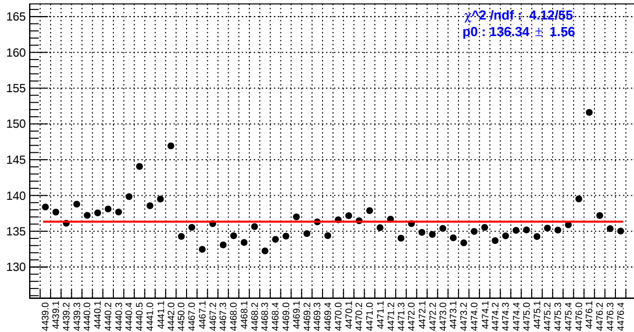
slug60: reg_asym_left_avg.rms/ppm
