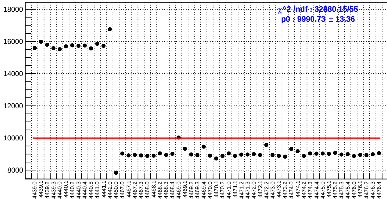
slug60: diff_bpm4eX.rms/nm
