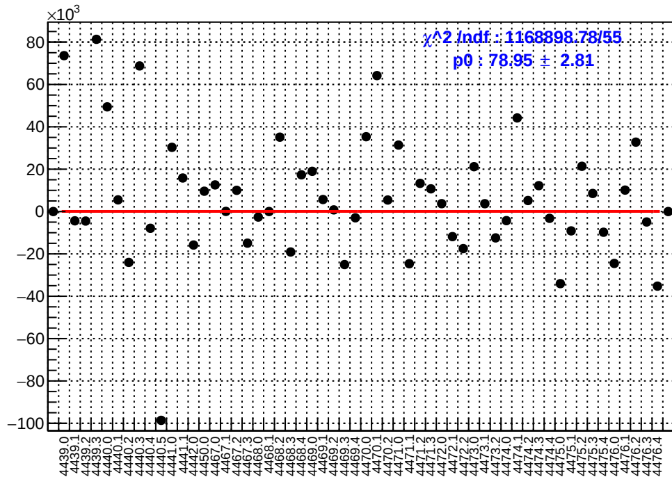
slug60: asym_sam6.mean/ppb-reg_asym_sam6.mean/ppb
