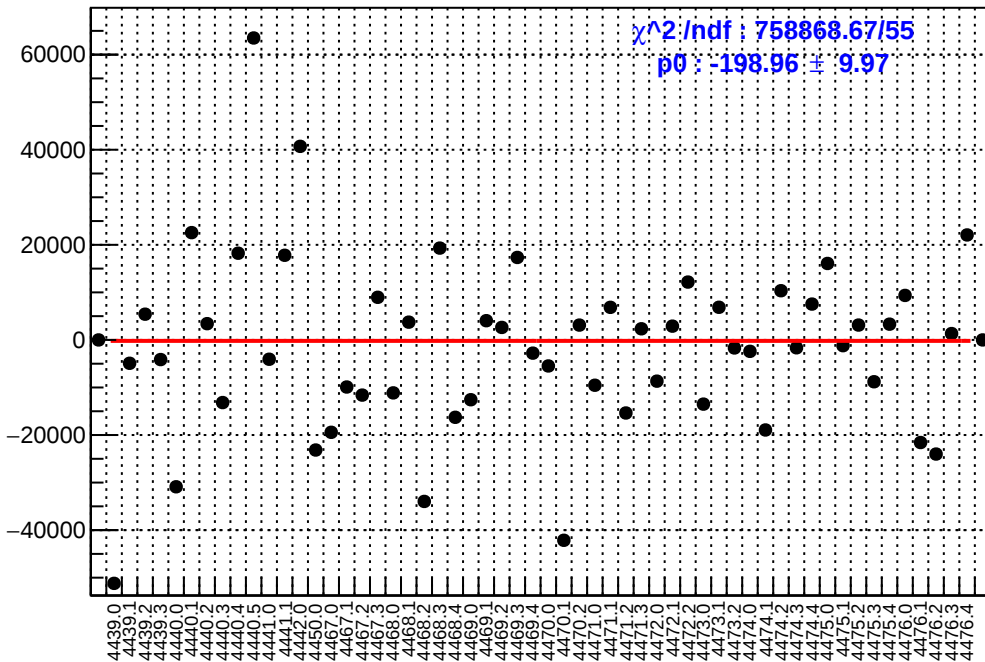
slug60: asym_atr1.mean/ppb-reg_asym_atr1.mean/ppb
