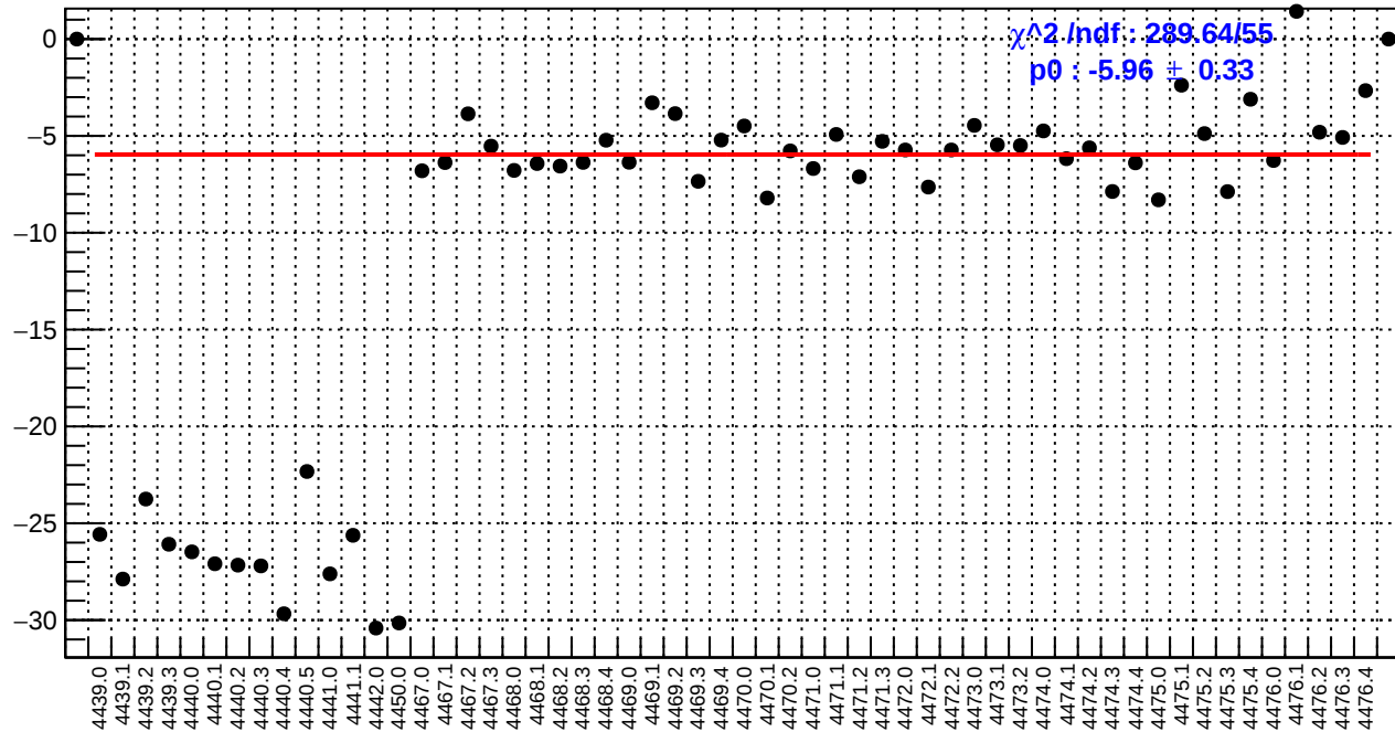
slug60: dsr_bpm4aX/(ppb/nm)
