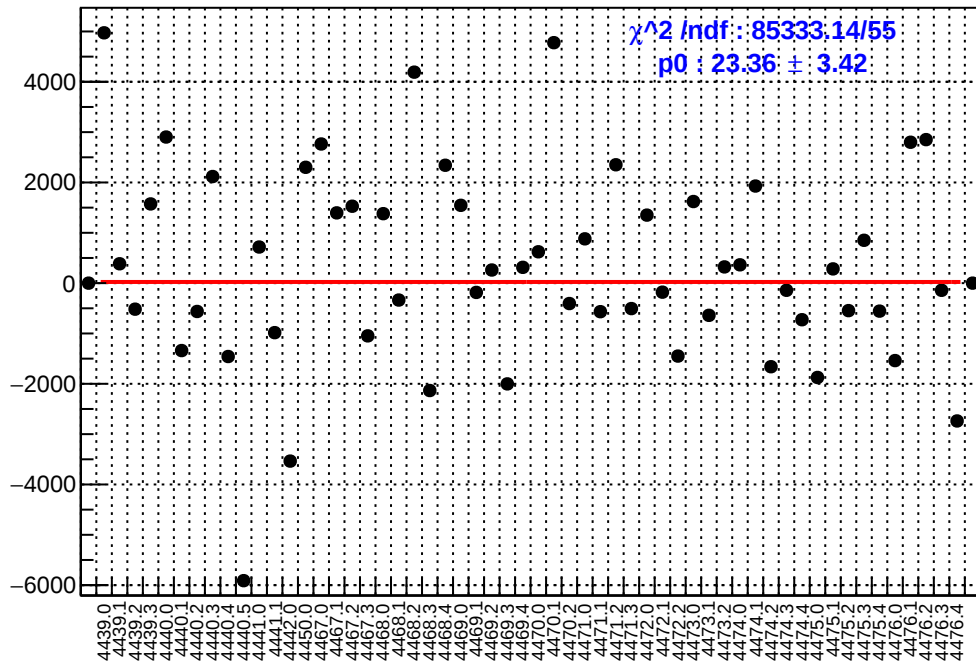
slug60: asym_atl1r2_dd.mean/ppb-reg_asym_atl1r2_dd.mean/ppb
