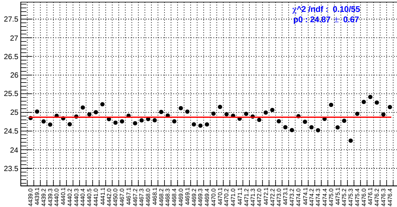
slug60: reg_asym_left_dd.rms/ppm
