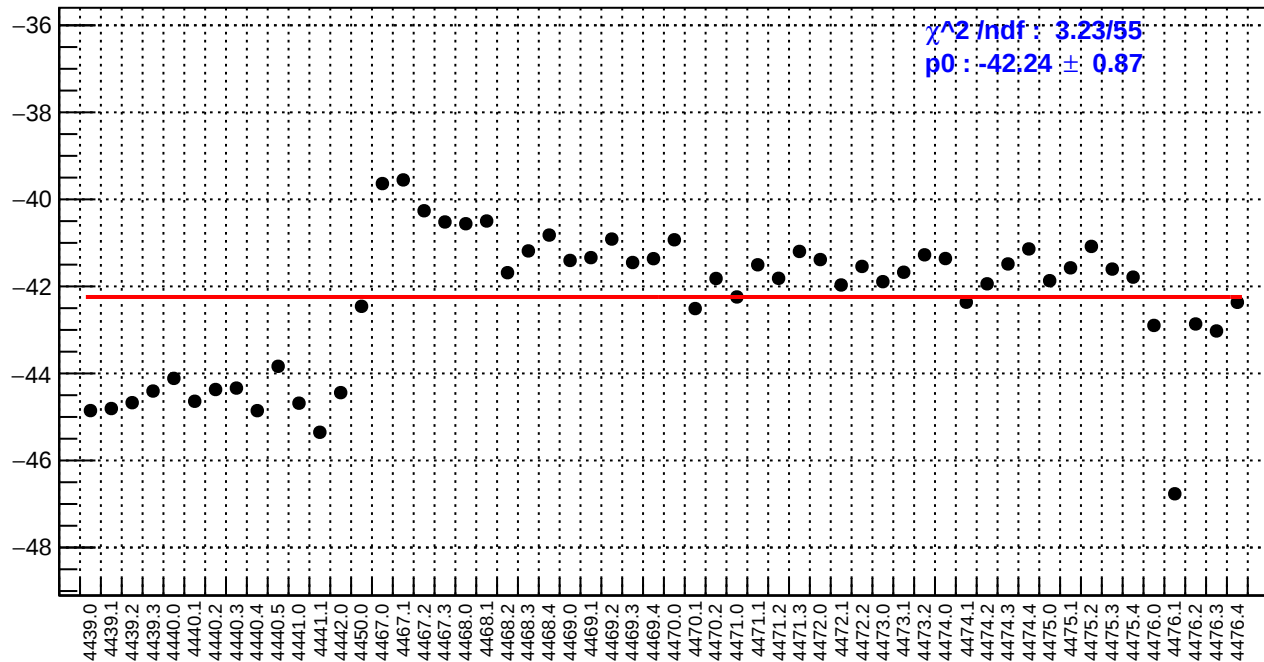
slug60: left_avg_bpm12X/(ppb/nm)
