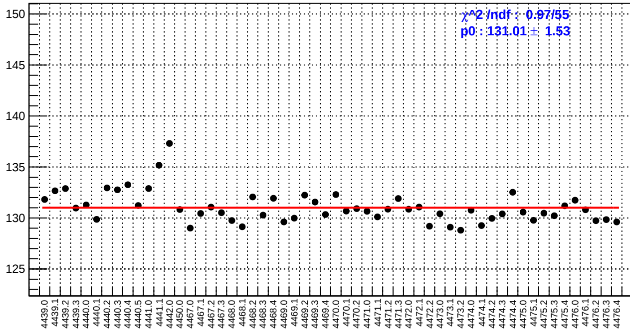
slug60: reg_asym_right_avg.rms/ppm
