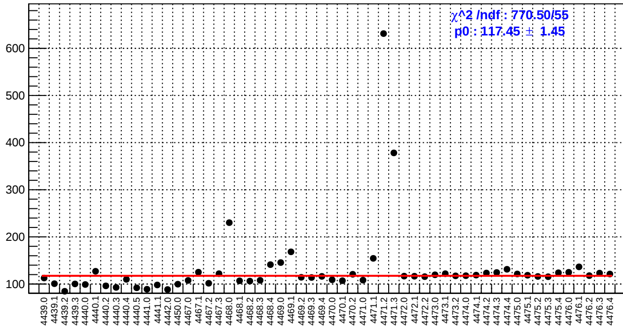
slug60: asym_bcm_an_ds.rms/ppm
