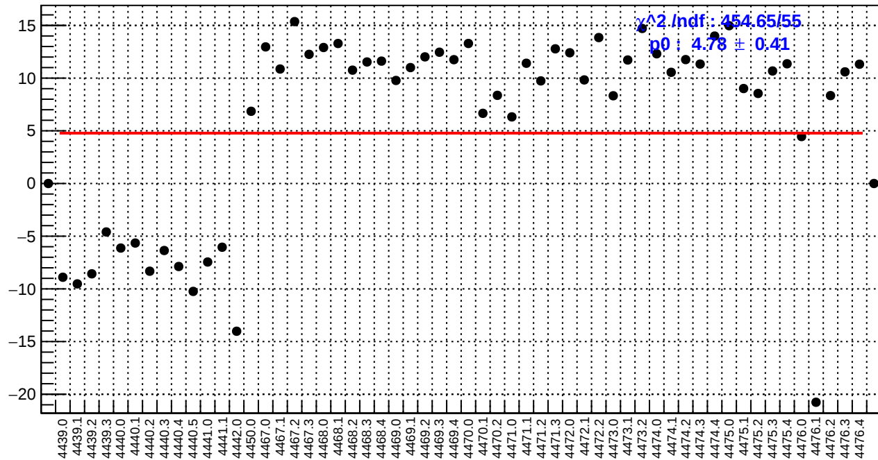
slug60: us_avg_bpm4eY/(ppb/nm)
