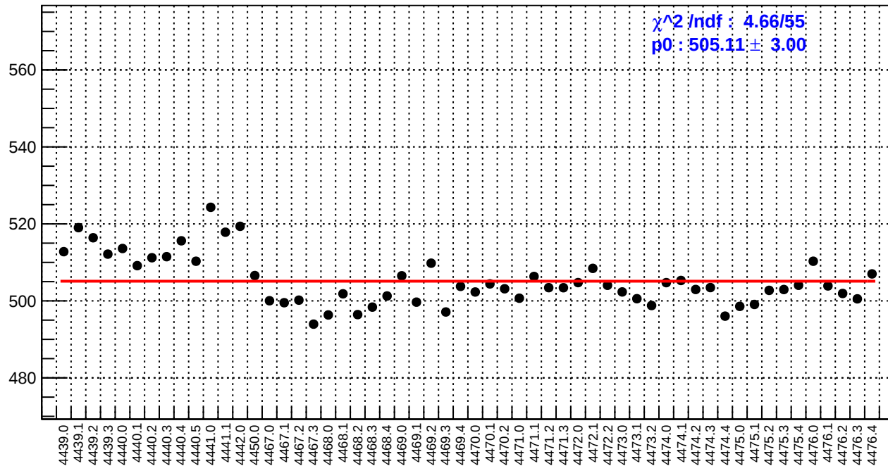
slug60: reg_asym_atl1.rms/ppm
