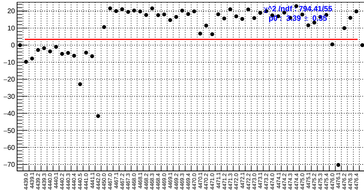
slug60: usl_bpm4eY/(ppb/nm)
