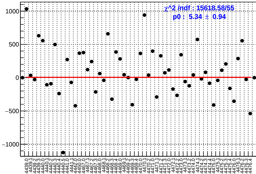
slug60: asym_right_dd.mean/ppb-reg_asym_right_dd.mean/ppb
