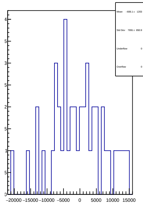
slug61: 1D Corr asym_at1_avg.mean/ppb-reg_asym_at1_avg.mean/ppb
