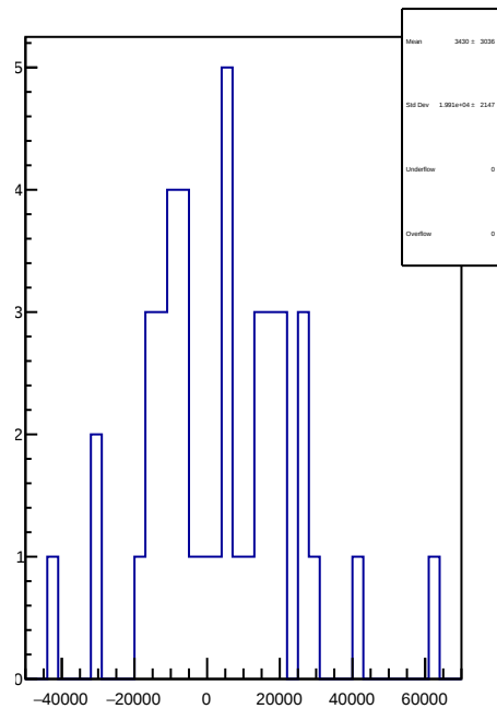
slug61: 1D Corr asym_sam6.mean/ppb-reg_asym_sam6.mean/ppb
