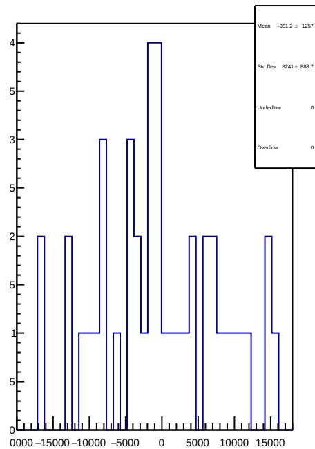
slug61: 1D Corr asym_atl_avg.mean/ppb-reg_asym_atl_avg.mean/ppb
