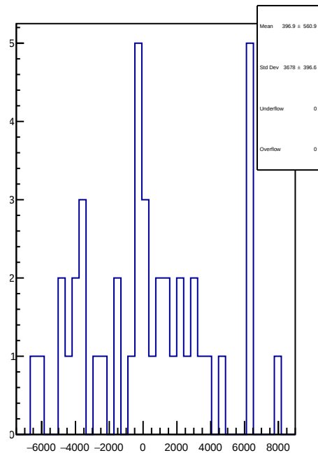
slug61: 1D Corr asym_dsr.mean/ppb-reg_asym_dsr.mean/ppb
