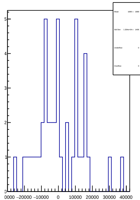
slug61: 1D Corr asym_sam8.mean/ppb-reg_asym_sam8.mean/ppb
