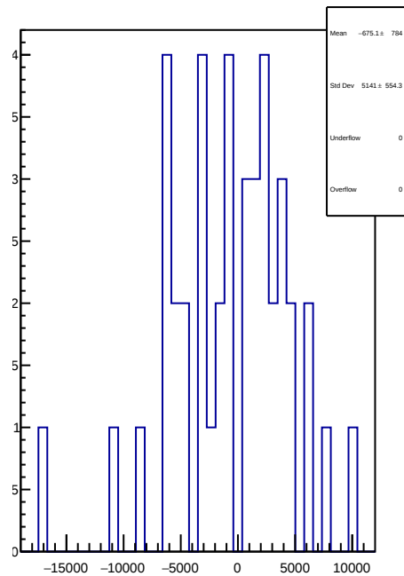
slug61: 1D Corr asym_usl.mean/ppb-reg_asym_usl.mean/ppb
