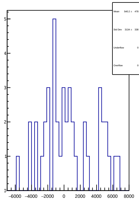
slug61: 1D Corr asym_sam5.mean/ppb-reg_asym_sam5.mean/ppb
