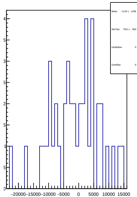
slug61: 1D Corr asym_atr_dd.mean/ppb-reg_asym_atr_dd.mean/ppb
