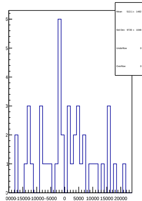
slug61: 1D Corr asym_atl1r2_avg.mean/ppb-reg_asym_atl1r2_avg.mean/ppb
