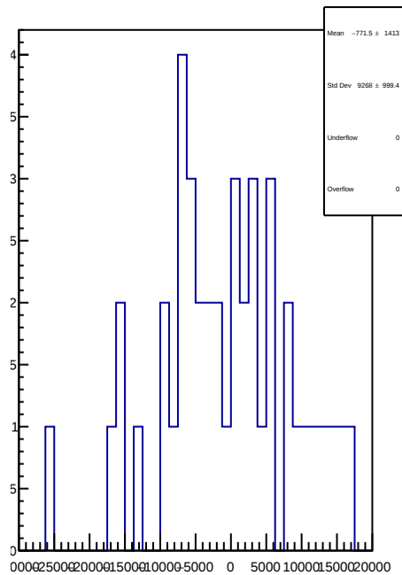
slug61: 1D Corr asym_atr_avg.mean/ppb-reg_asym_atr_avg.mean/ppb
