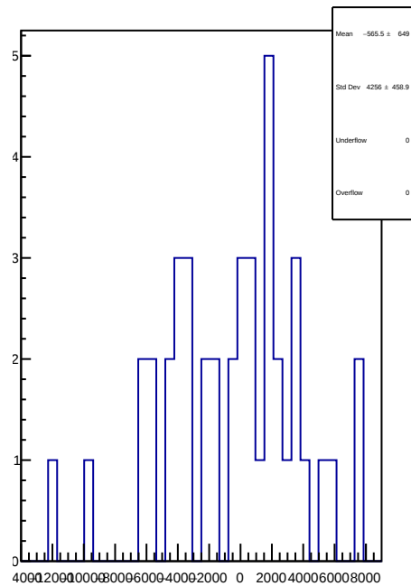
slug61: 1D Corr asym_ds_dd.mean/ppb-reg_asym_ds_dd.mean/ppb
