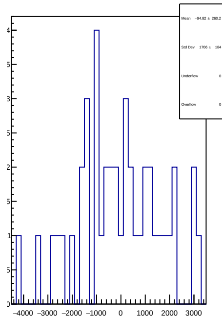
slug61: 1D Corr asym_us_avg.mean/ppb-reg_asym_us_avg.mean/ppb
