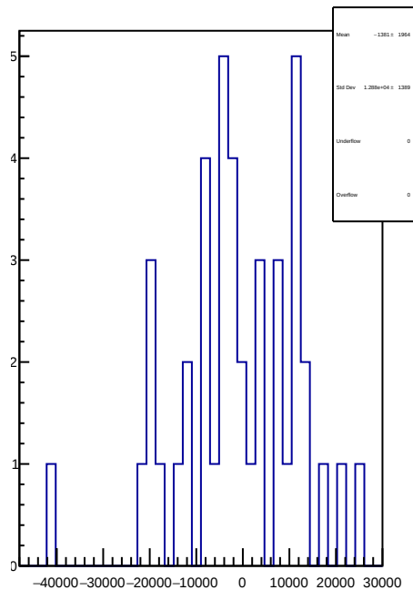
slug61: 1D Corr asym_atl2.mean/ppb-reg_asym_atl2.mean/ppb
