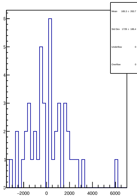
slug61: 1D Corr asym_atl1r2_dd.mean/ppb-reg_asym_atl1r2_dd.mean/ppb
