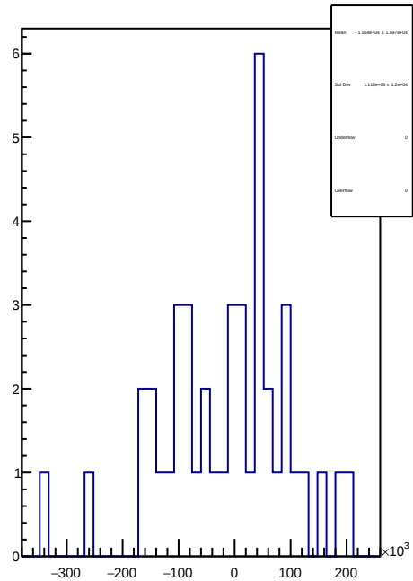
slug61: 1D Corr asym_sam3.mean/ppb-reg_asym_sam3.mean/ppb
