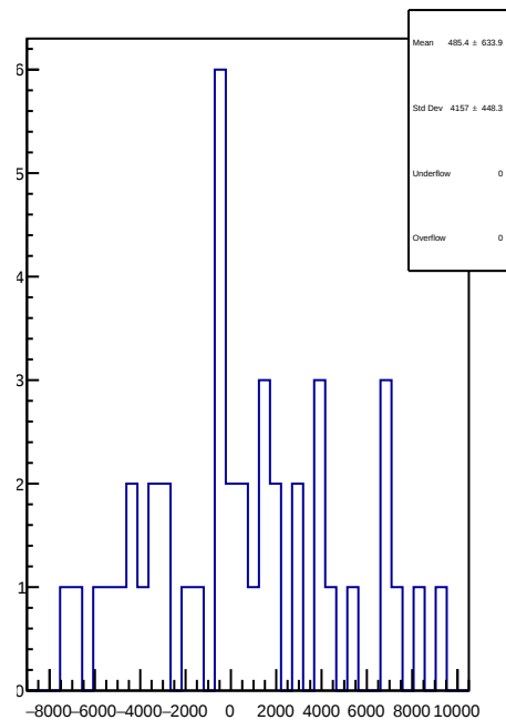
slug61: 1D Corr asym_usr.mean/ppb-reg_asym_usr.mean/ppb
