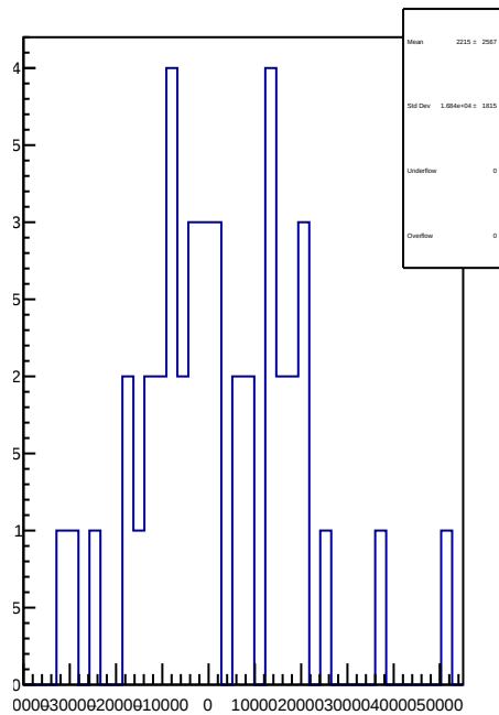
slug61: 1D Corr asym_sam7.mean/ppb-reg_asym_sam7.mean/ppb
