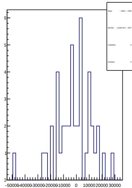
slug61: 1D Corr asym_atr1.mean/ppb-reg_asym_atr1.mean/ppb
