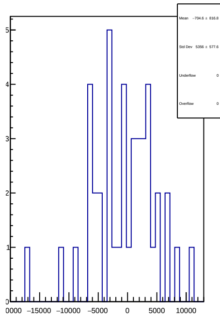
slug61: 1D Corr asym_left_avg.mean/ppb-reg_asym_left_avg.mean/ppb
