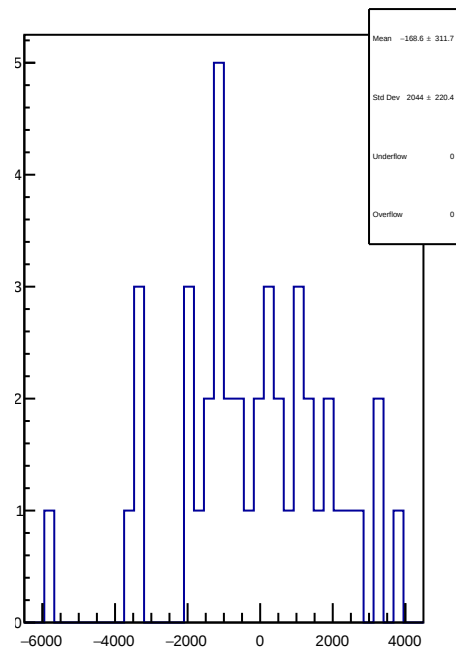
slug61: 1D Corr asym_ds_avg.mean/ppb-reg_asym_ds_avg.mean/ppb
