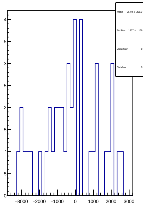
slug61: 1D Corr asym_atr1l2_dd.mean/ppb-reg_asym_atr1l2_dd.mean/ppb
