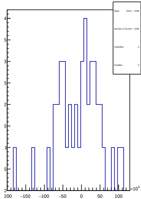
slug61: 1D Corr asym_sam2.mean/ppb-reg_asym_sam2.mean/ppb
