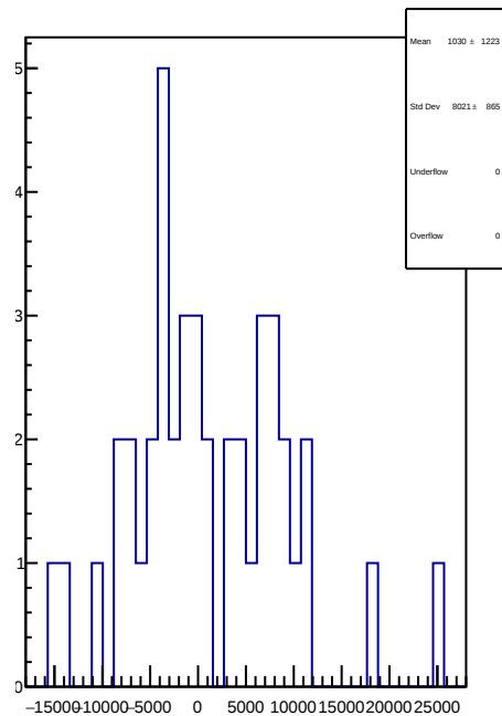
slug61: 1D Corr asym_atl_dd.mean/ppb-reg_asym_atl_dd.mean/ppb
