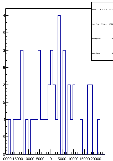
slug61: 1D Corr asym_atl1.mean/ppb-reg_asym_atl1.mean/ppb
