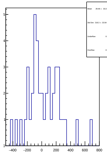
slug61: 1D Corr asym_left_dd.mean/ppb-reg_asym_left_dd.mean/ppb
