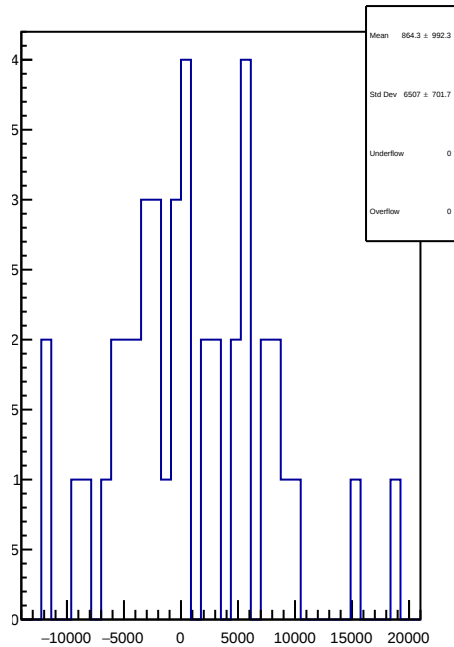
slug61: 1D Corr asym at2 dd.mean/ppb-reg asym at2 dd.mean/ppb
