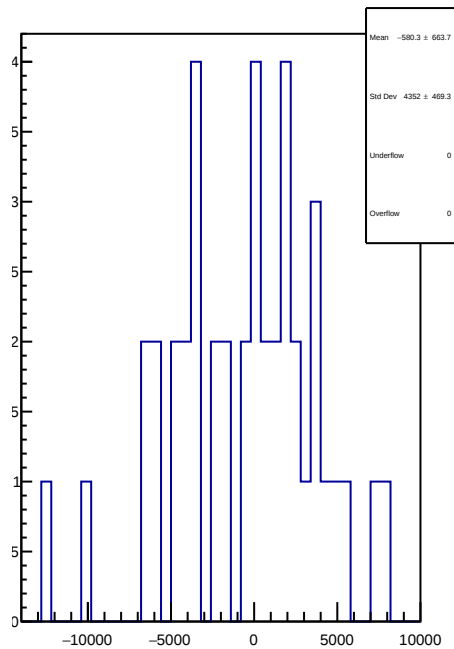
slug61: 1D Corr asym_us_dd.mean/ppb-reg_asym_us_dd.mean/ppb
