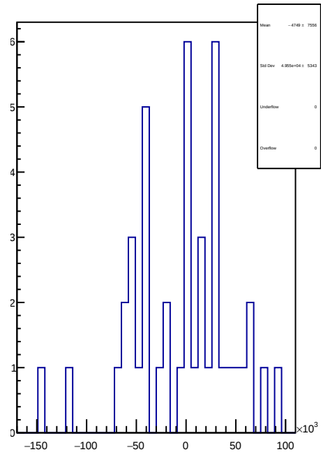
slug61: 1D Corr asym_sam4.mean/ppb-reg_asym_sam4.mean/ppb
