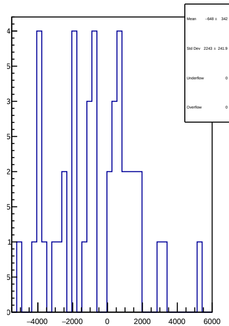
slug61: 1D Corr asym_sam1.mean/ppb-reg_asym_sam1.mean/ppb
