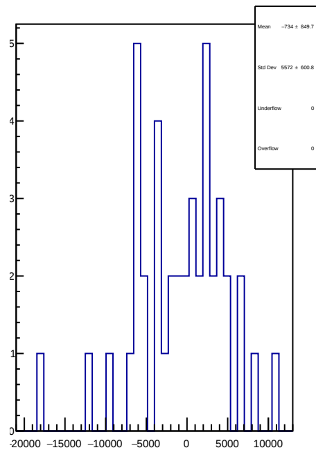
slug61: 1D Corr asym_dsl.mean/ppb-reg_asym_dsl.mean/ppb
