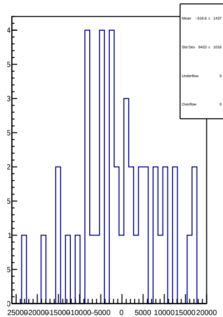
slug61: 1D Corr asym_at2_avg.mean/ppb-reg_asym_at2_avg.mean/ppb
