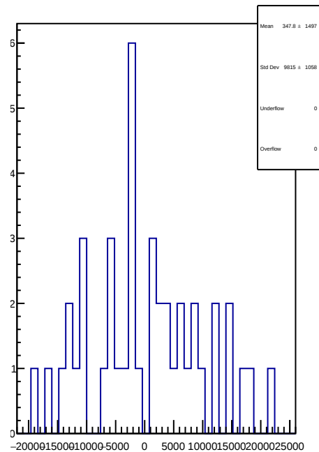
slug61: 1D Corr asym_atr2.mean/ppb-reg_asym_atr2.mean/ppb
