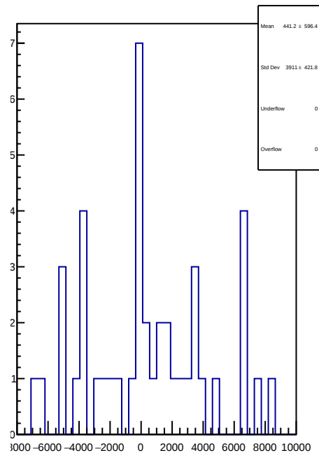
slug61: 1D Corr asym_right_avg.mean/ppb-reg_asym_right_avg.mean/ppb
