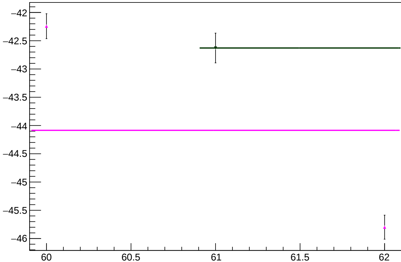
reg_asym_left_avg_diff_bpm11X_slope vs slug
