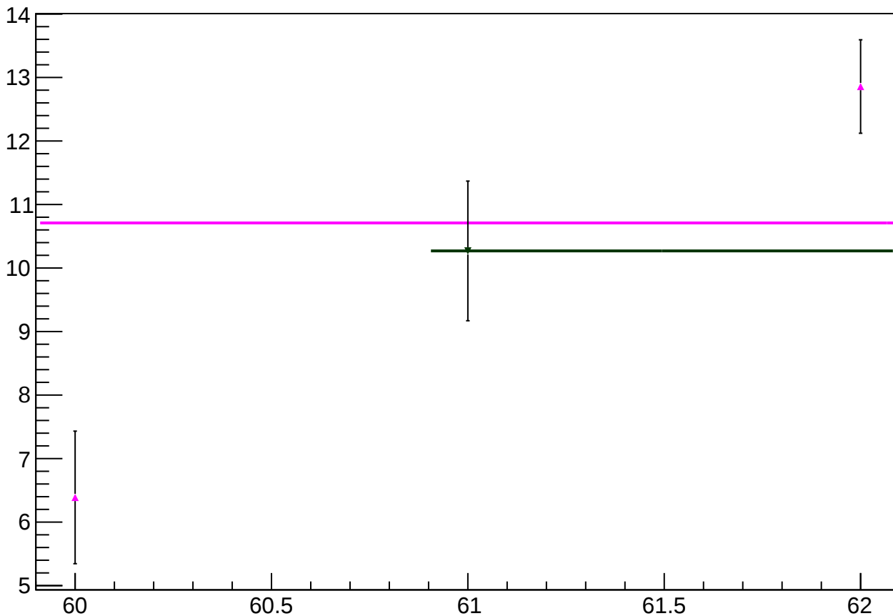
reg_asym_dsr_diff_bpm4eY_slope vs slug
