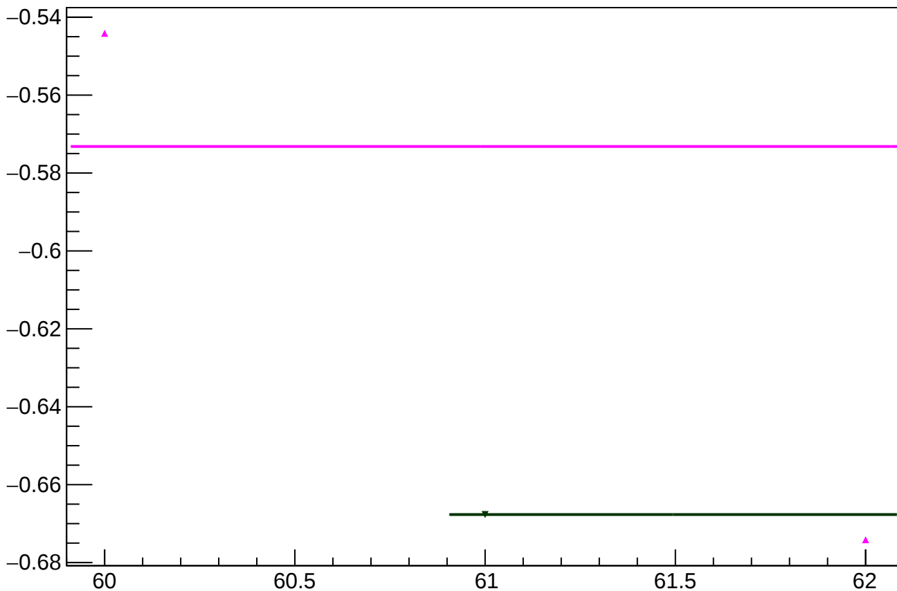
yield_bpm1X_mean vs slug
