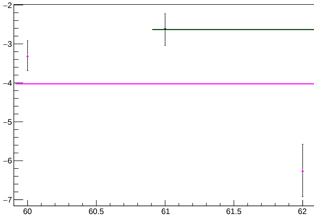
reg_asym_atl_dd_atr_dd_avg_diff_bpm4aX_slope vs slug
