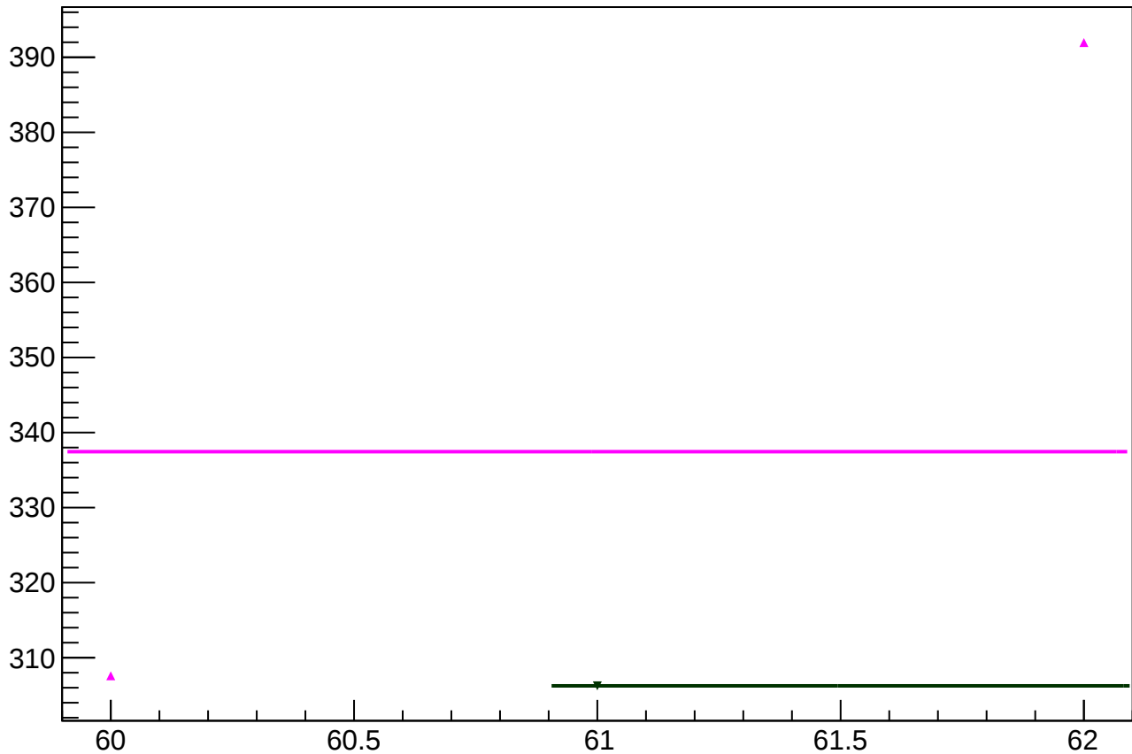
reg_asym_atl_avg_rms vs slug
