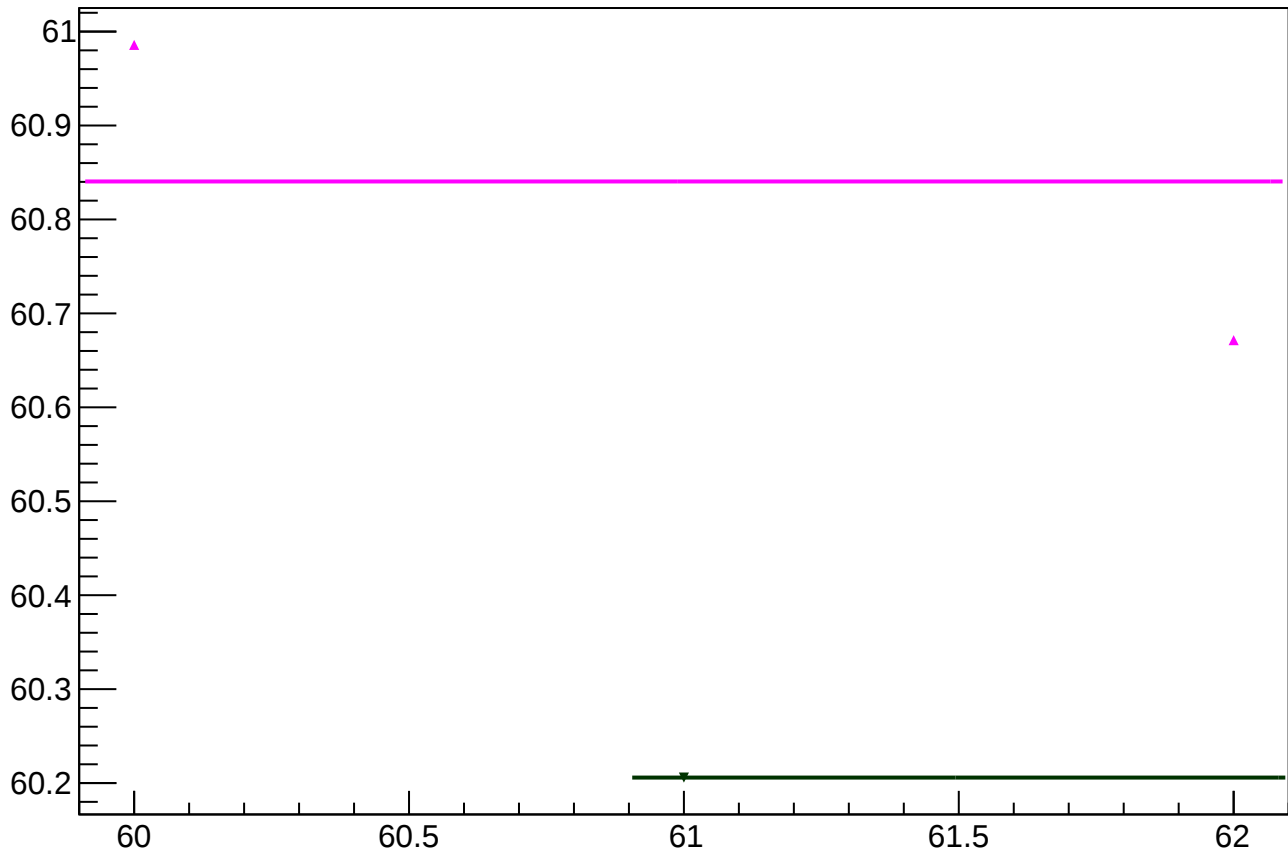
yield_usr_mean vs slug
