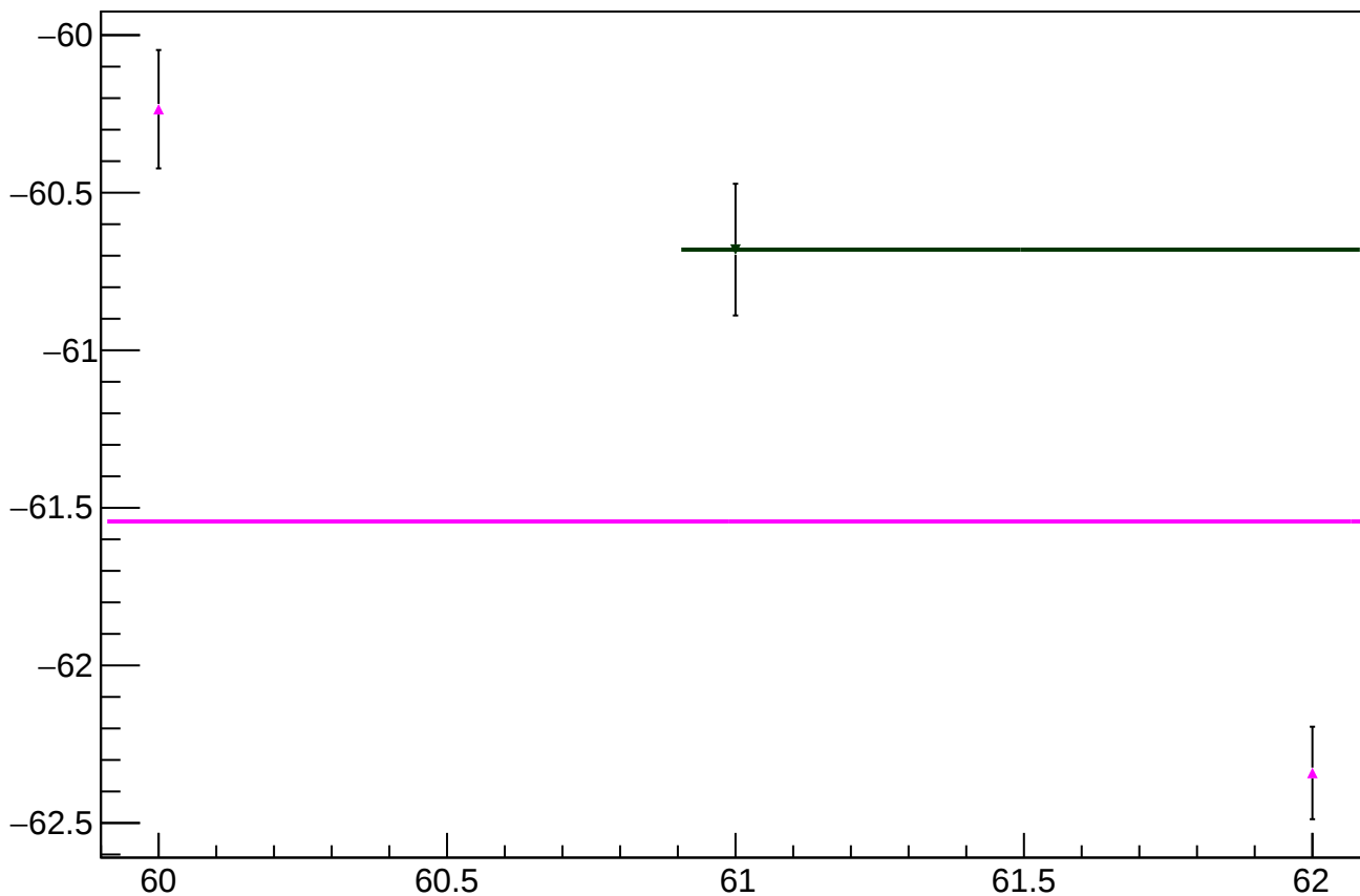
reg_asym_dsr_diff_bpm11X_slope vs slug
