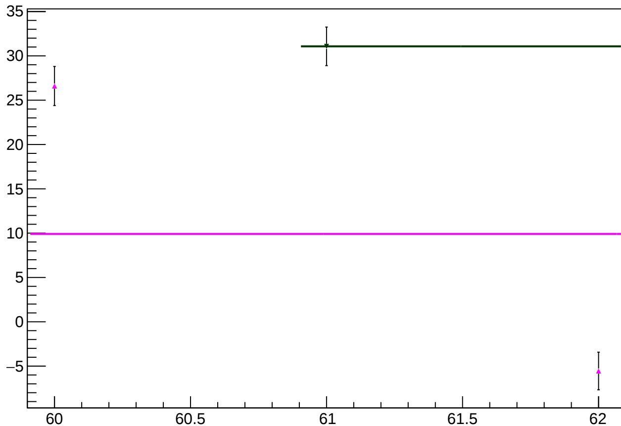
reg_asym_atl1r2_avg_diff_bpm4aX_slope vs slug
