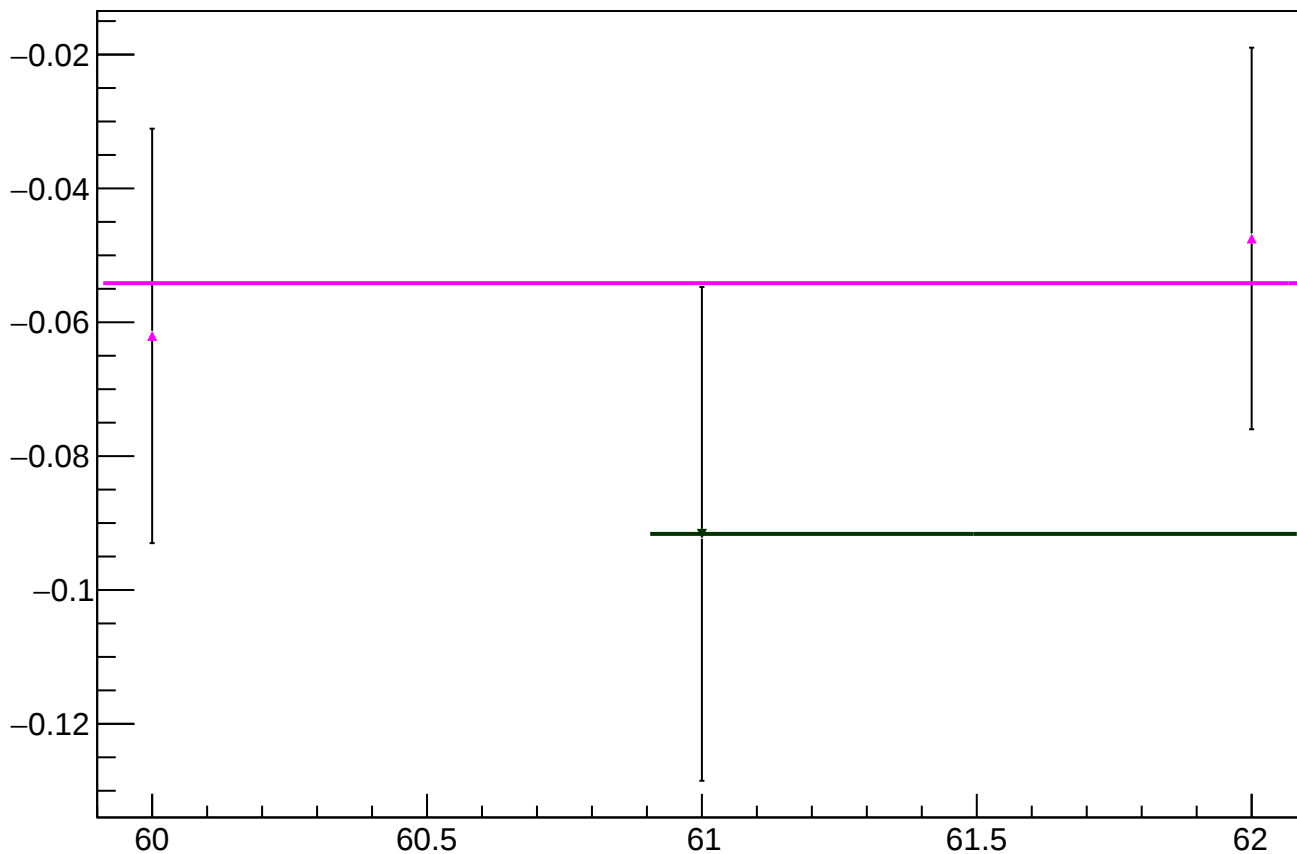
reg_bcm_dg_ds_ds_dd_diff_bpm4eY_slope vs slug
