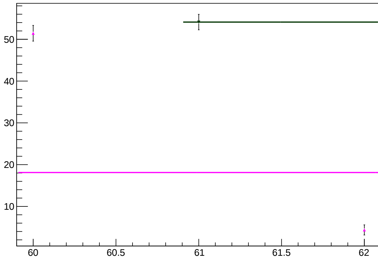
reg_asym_atr_avg_diff_bpm4aX_slope vs slug
