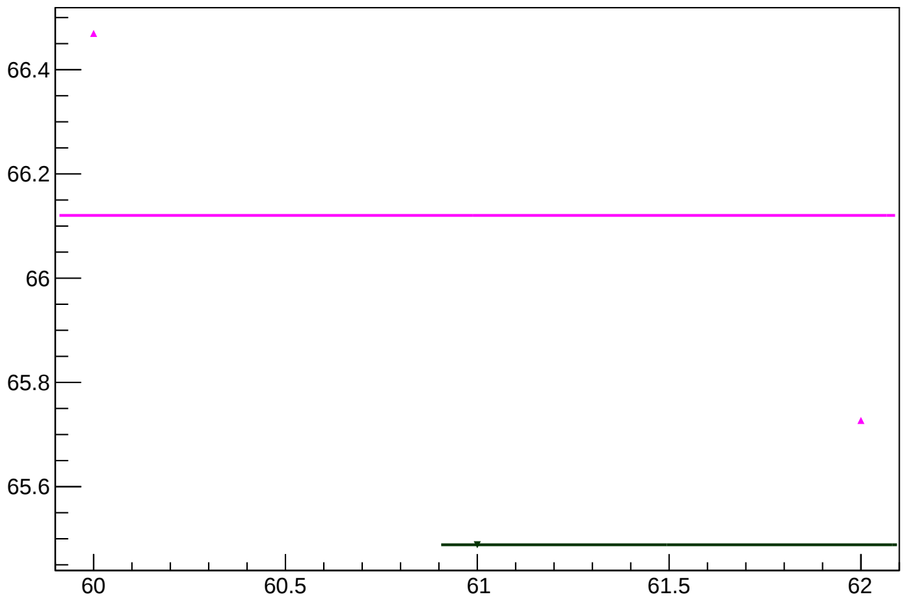
yield_usl_mean vs slug
