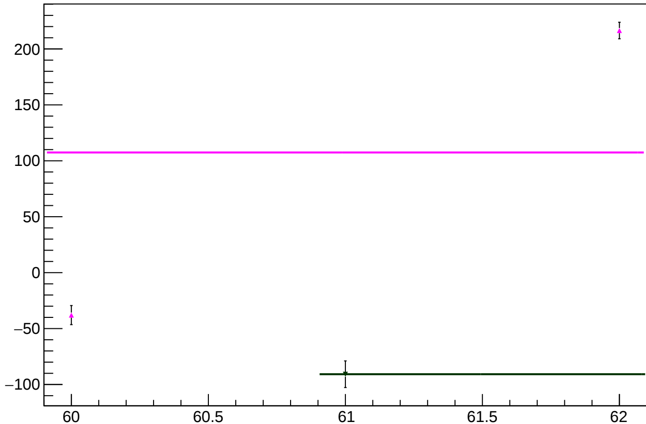
reg_asym_sam_37_avg_diff_bpm4aY_slope vs slug
