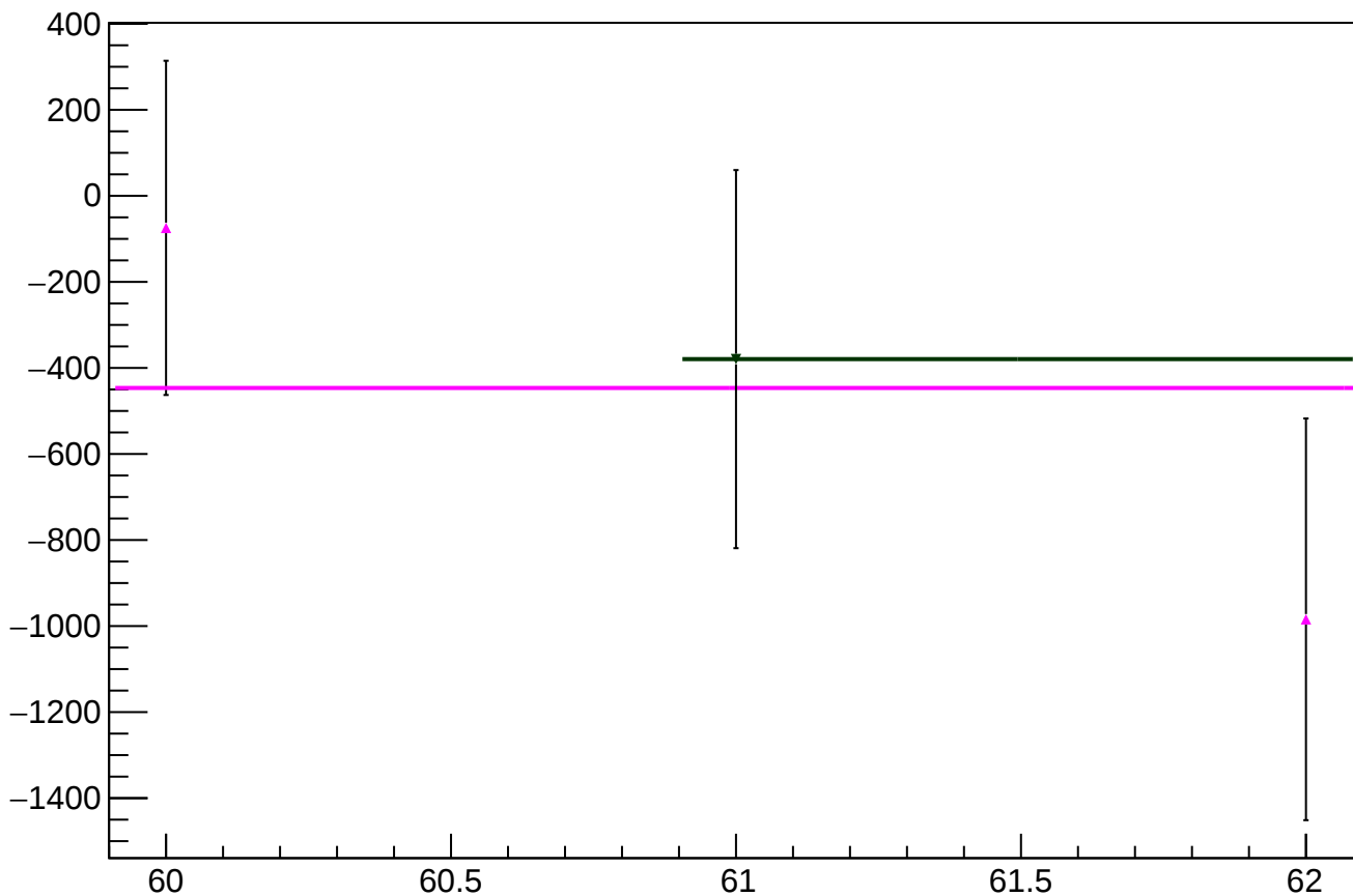
reg_asym_atl1r2_dd_mean vs slug
