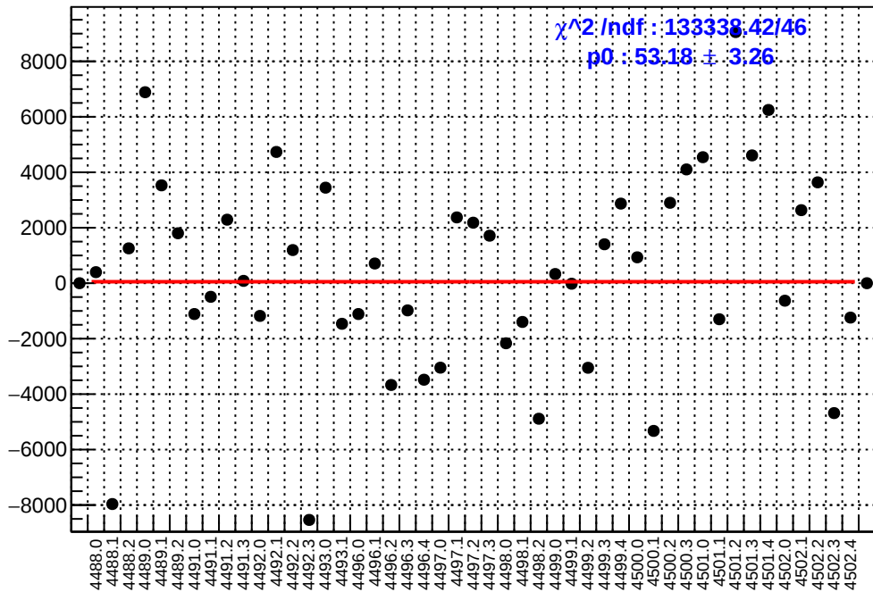
slug62: asym_ds_dd.mean/ppb-reg_asym_ds_dd.mean/ppb
