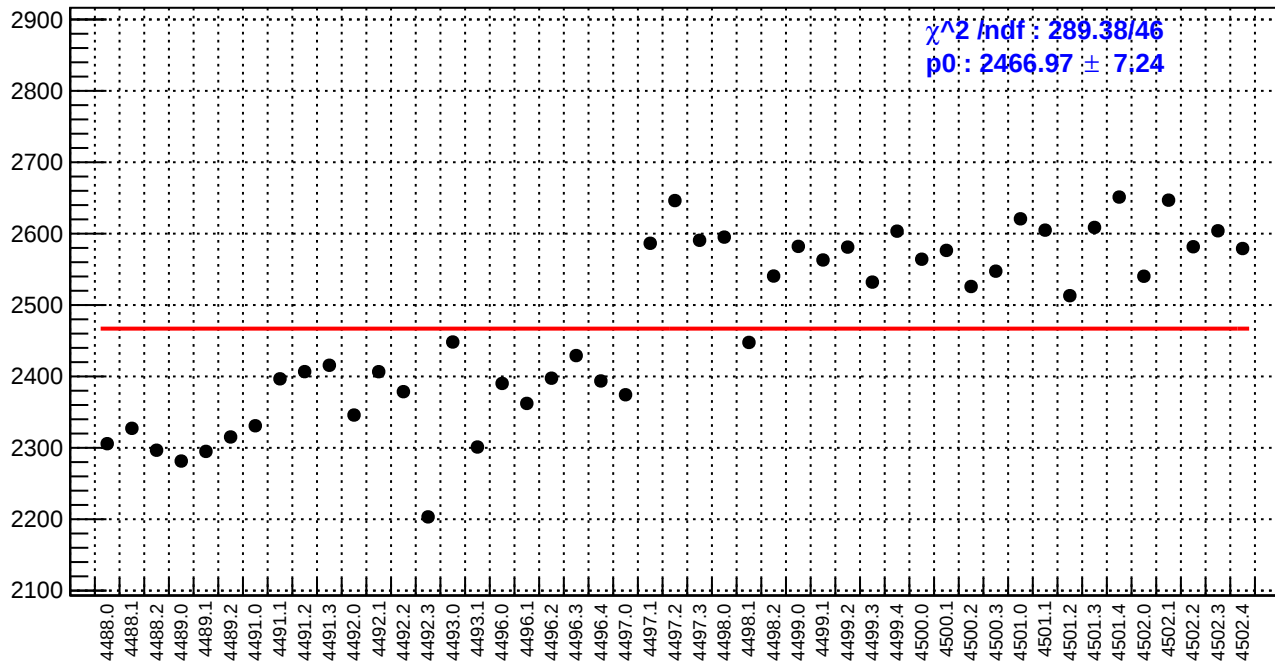
slug62: reg_asym_sam2.rms/ppm
