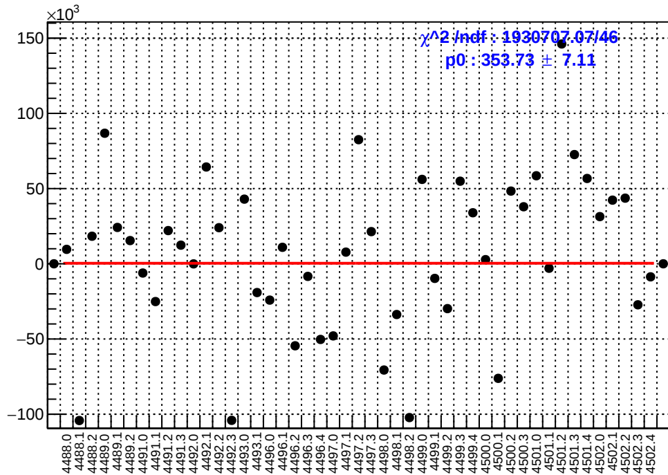
slug62: asym_sam2.mean/ppb-reg_asym_sam2.mean/ppb
