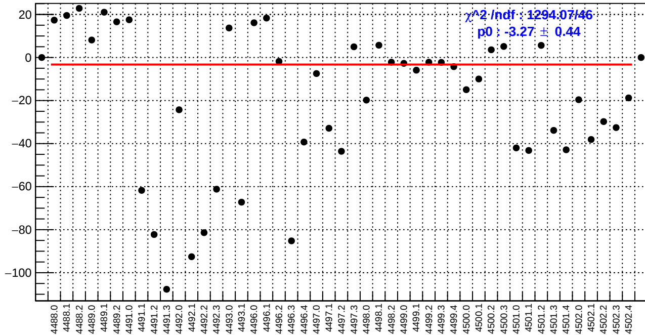
slug62: left_avg_bpm4eY/(ppb/nm)
