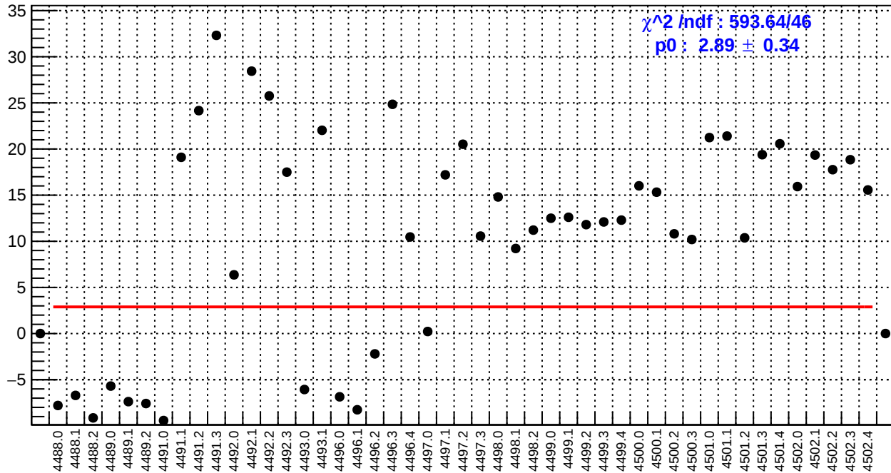
slug62: us_avg_bpm4aY/(ppb/nm)
