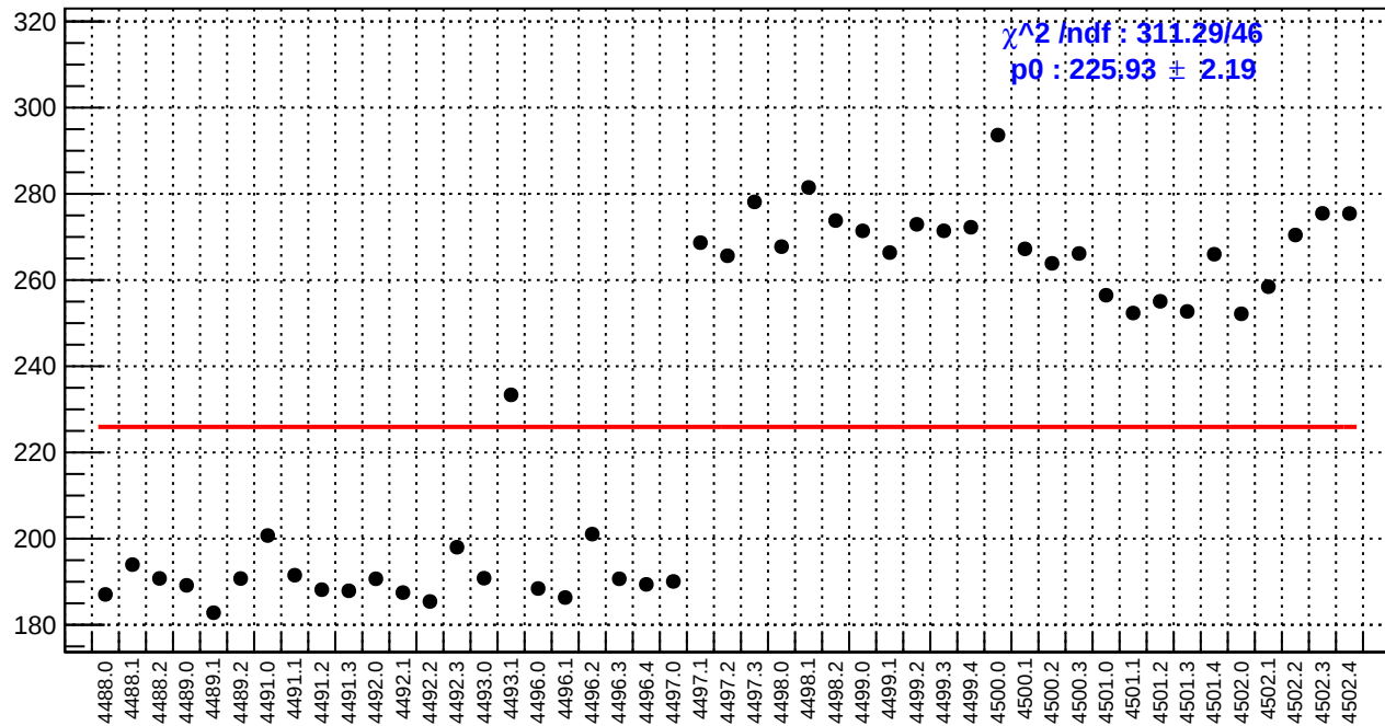
slug62: reg_asym_sam1.rms/ppm
