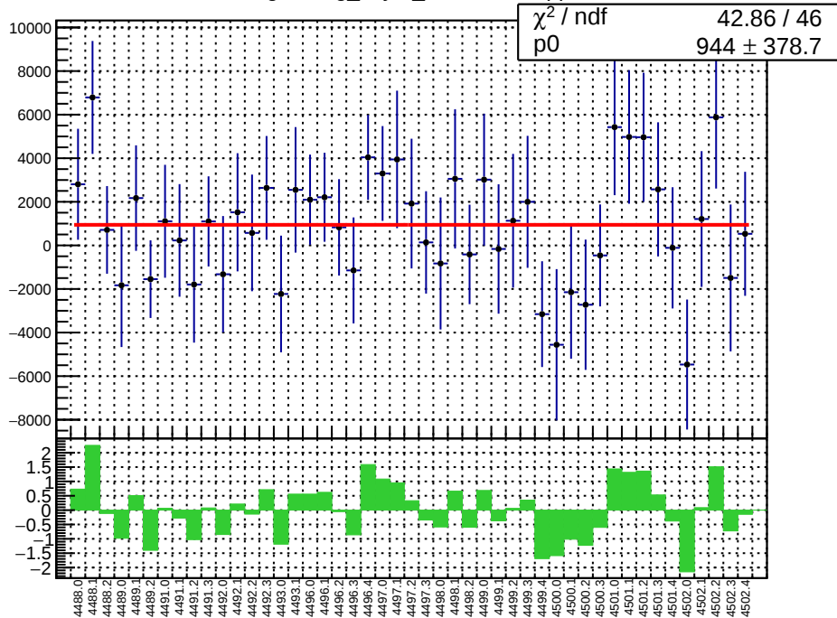
slug62: reg_asym_sam5.mean/ppb
