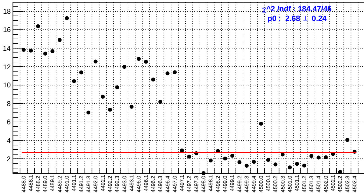
slug62: us_avg_bpm4aX/(ppb/nm)
