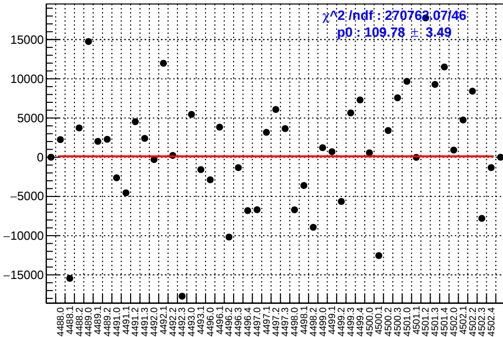
slug62: asym_atr1.mean/ppb-reg_asym_atr1.mean/ppb
