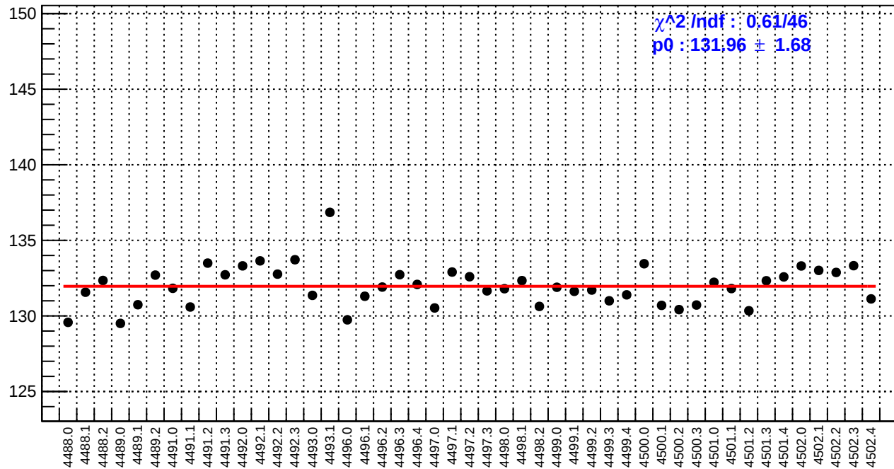
slug62: reg_asym_usr.rms/ppm
