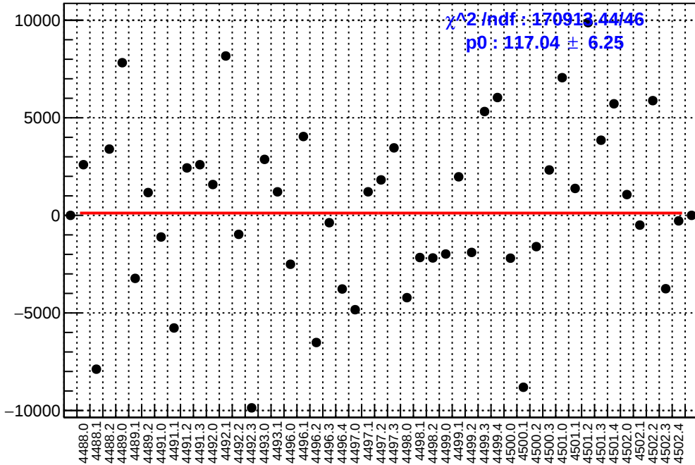
slug62: asym_left_avg.mean/ppb-reg_asym_left_avg.mean/ppb
