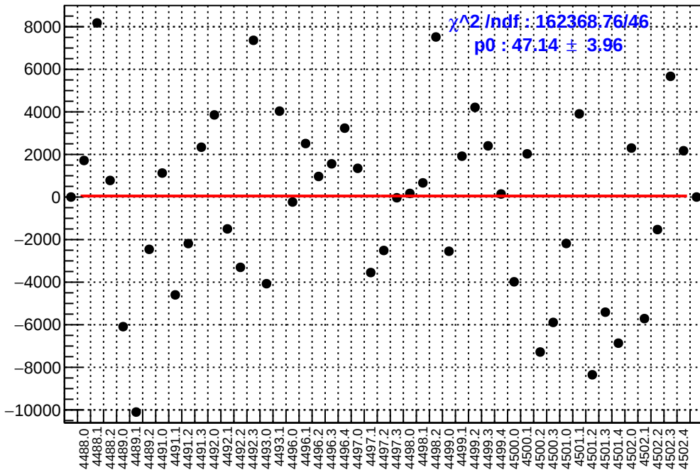
slug62: asym_right_avg.mean/ppb-reg_asym_right_avg.mean/ppb
