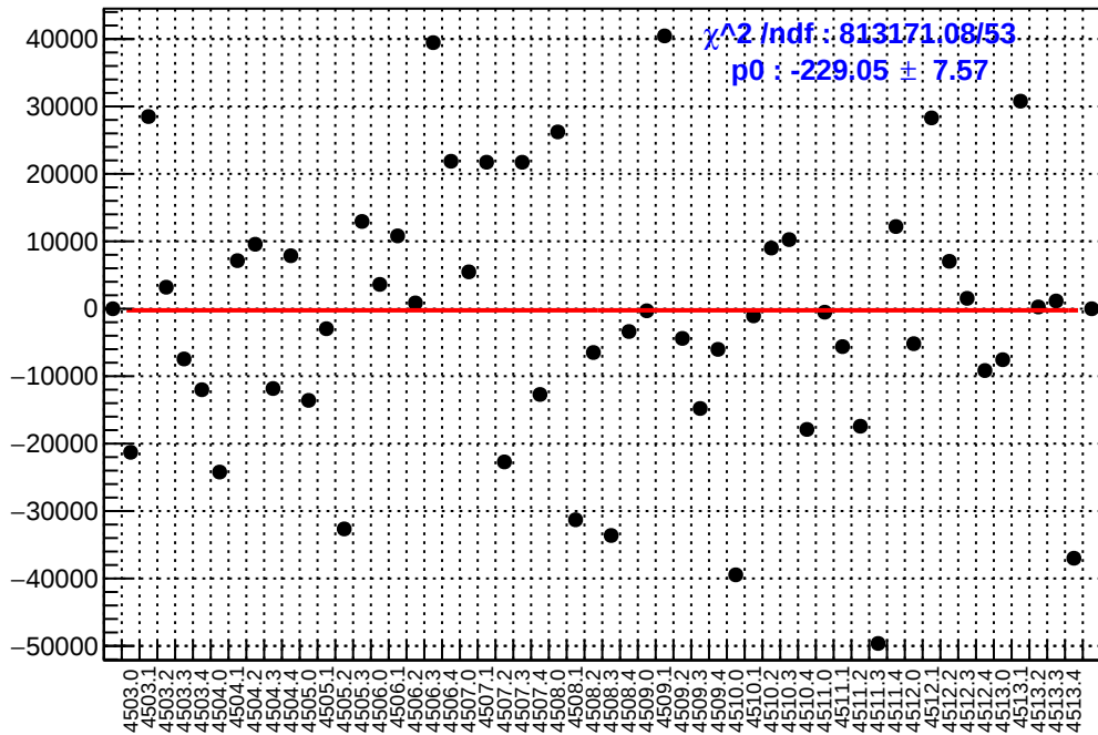
slug63: asym_at2_avg.mean/ppb-reg_asym_at2_avg.mean/ppb
