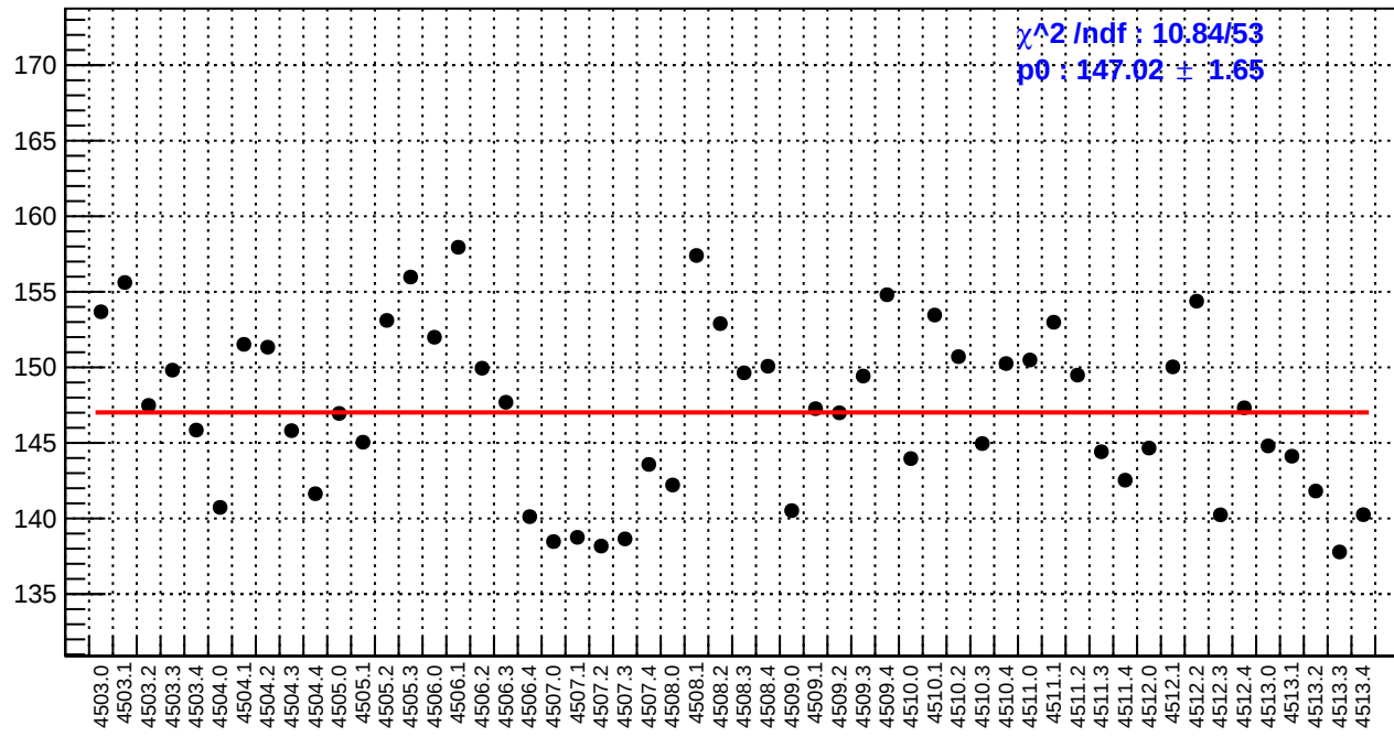
slug63: reg_asym_dsl.rms/ppm
