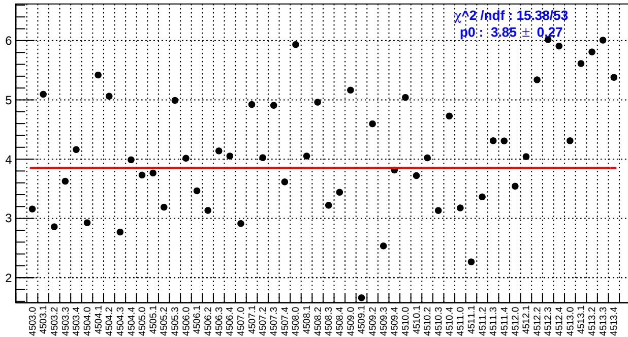
slug63: ds_avg_bpm4aX/(ppb/nm)
