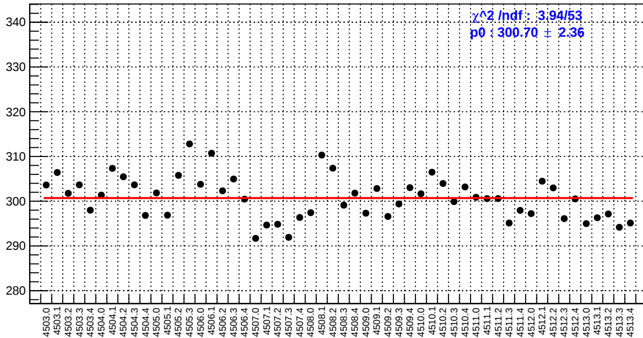
slug63: reg_asym_atr1l2_dd.rms/ppm
