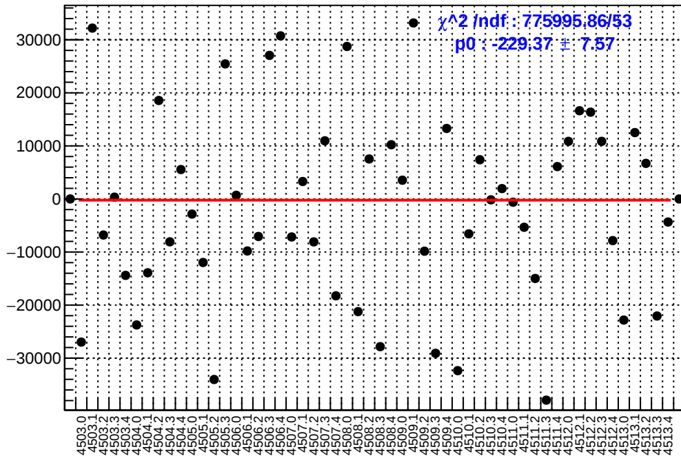
slug63: asym_atl1r2_avg.mean/ppb-reg_asym_atl1r2_avg.mean/ppb
