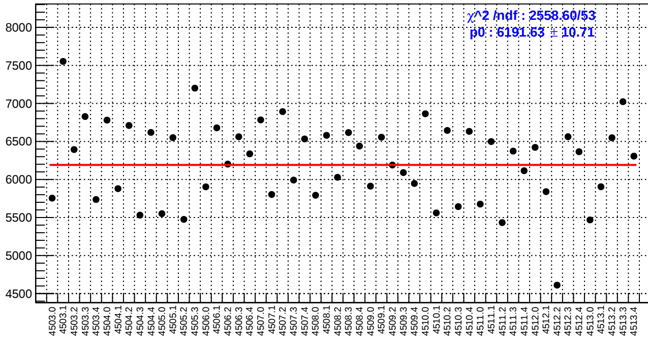
slug63: diff_bpm4eY.rms/nm
