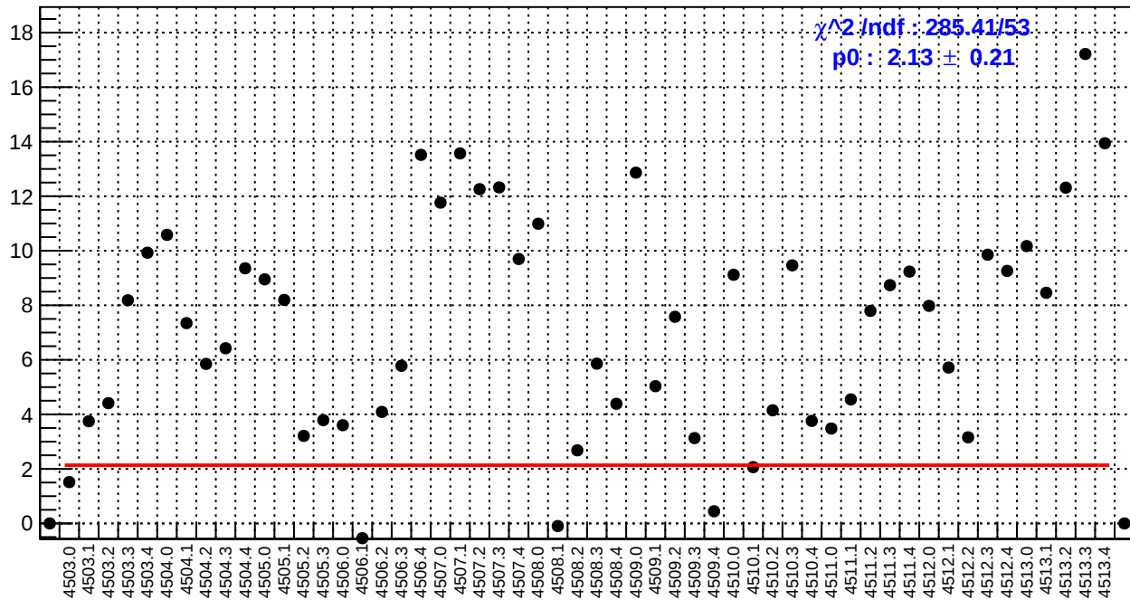
slug63: right_avg_bpm4aY/(ppb/nm)
