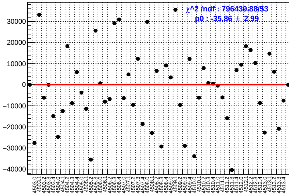
slug63: asym_atr2.mean/ppb-reg_asym_atr2.mean/ppb
