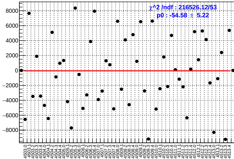
slug63: asym_dsr.mean/ppb-reg_asym_dsr.mean/ppb
