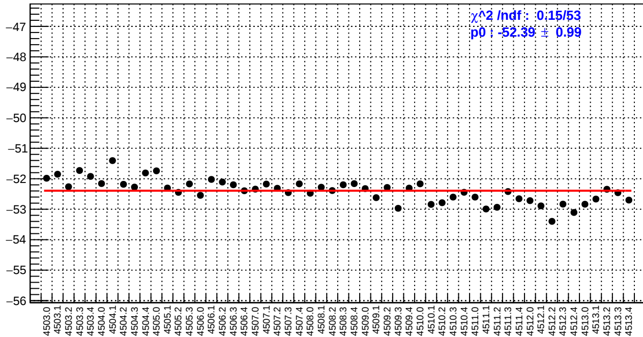
slug63: us_avg_bpm12X/(ppb/nm)
