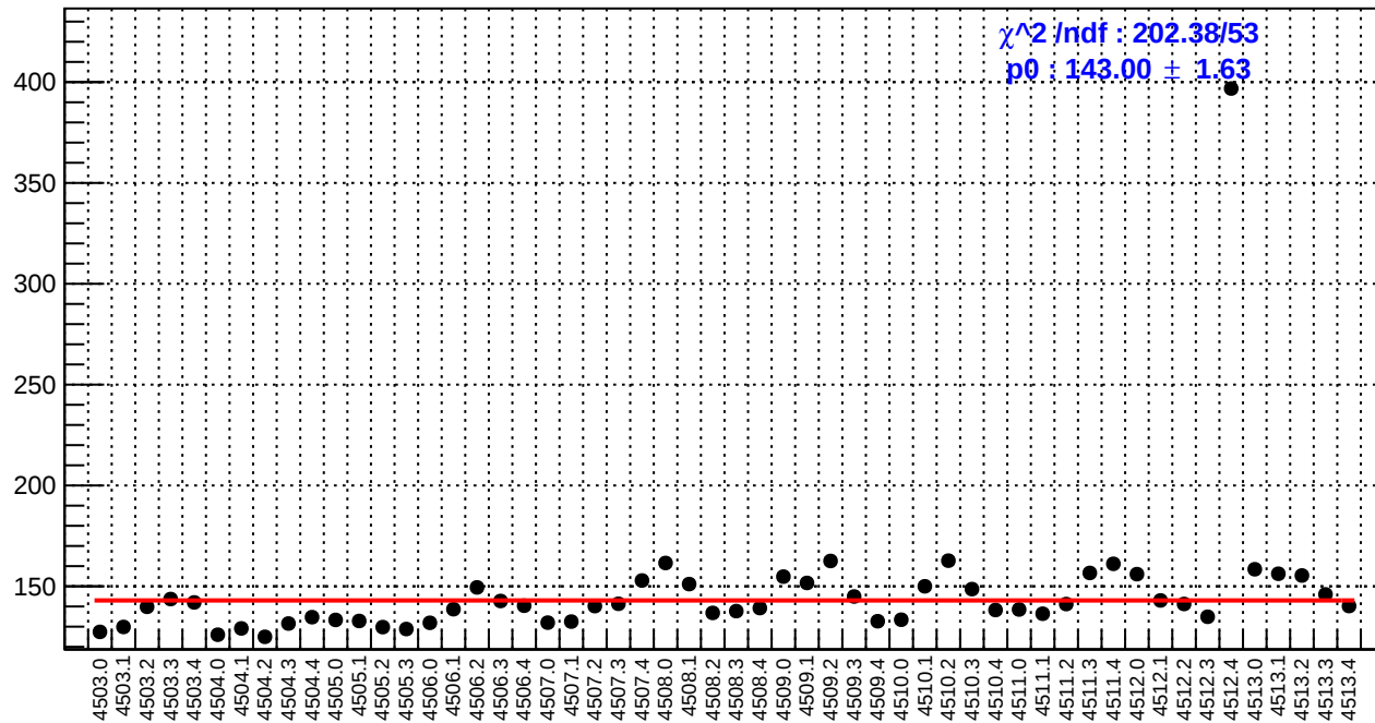
slug63: asym_bcm_an_us.rms/ppm
