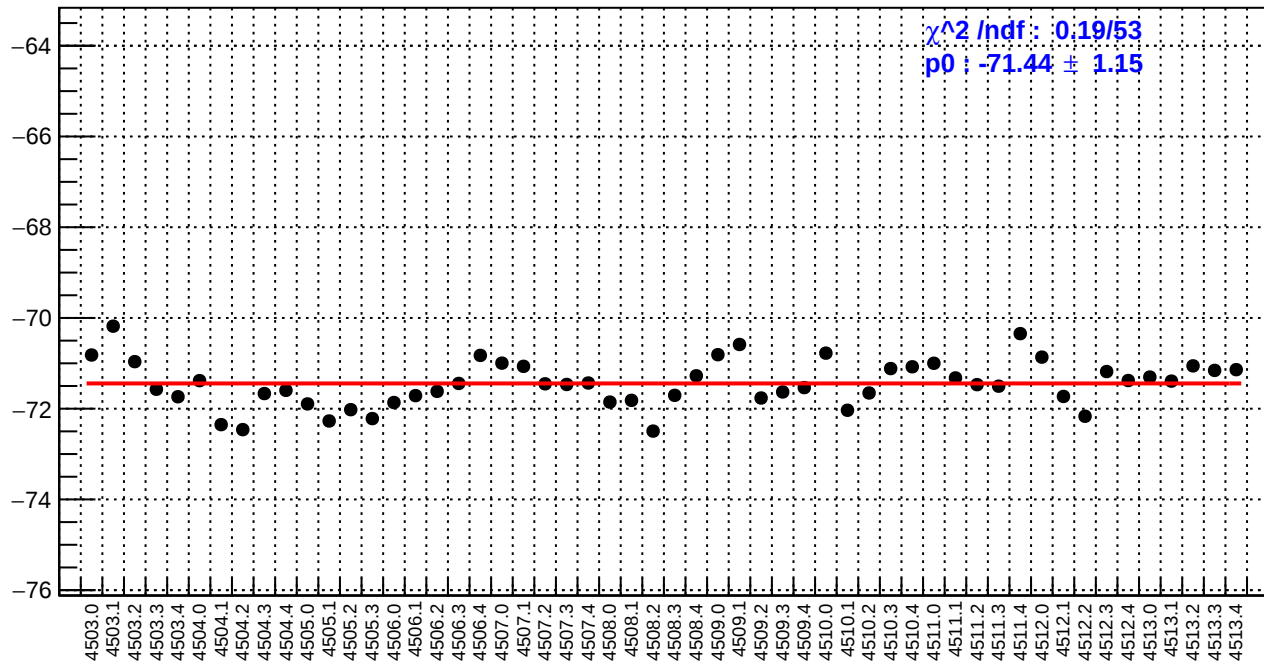
slug63: usl_bpm4eX/(ppb/nm)
