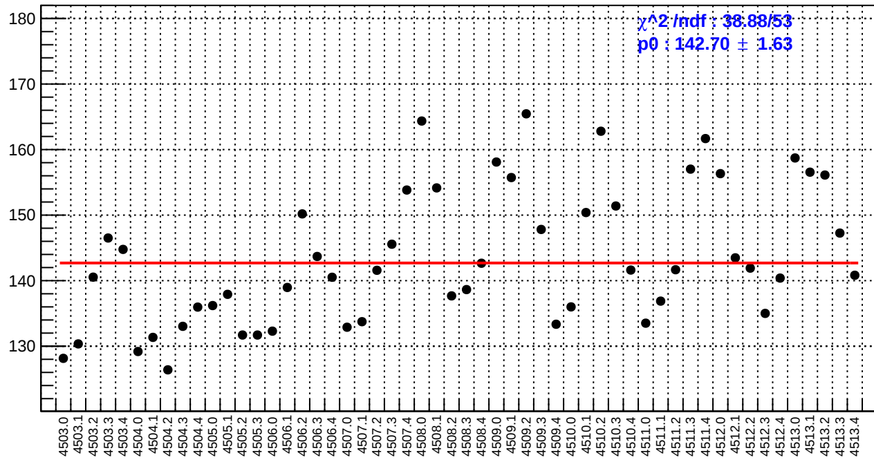
slug63: asym_bcm_an_ds.rms/ppm
