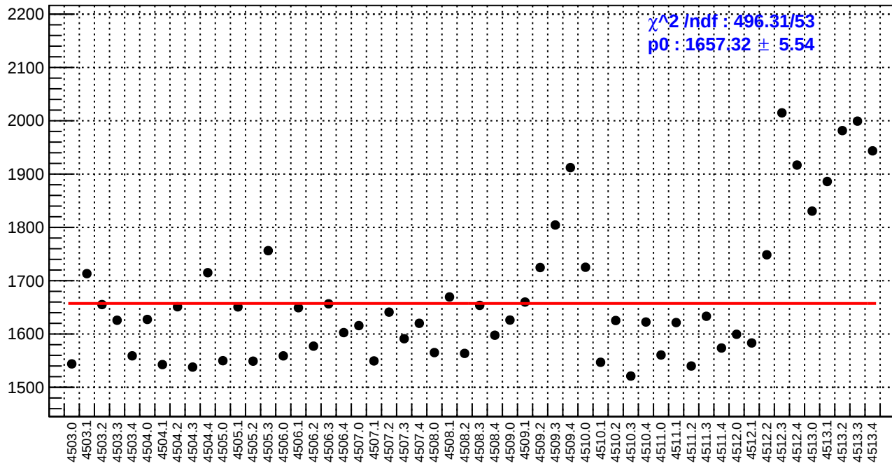
slug63: diff_bpm4aX.rms/nm
