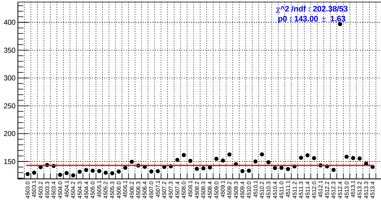
slug63: asym_bcm_an_us.rms/ppm
