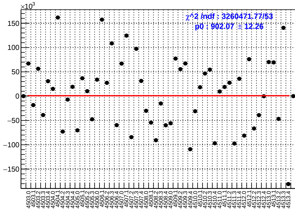
slug63: asym_sam4.mean/ppb-reg_asym_sam4.mean/ppb
