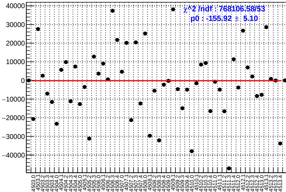
slug63: asym_atl_avg.mean/ppb-reg_asym_atl_avg.mean/ppb
