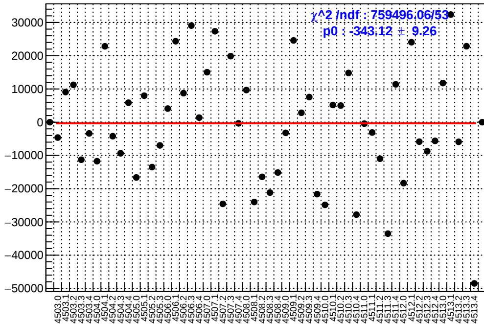
slug63: asym_atr1l2_avg.mean/ppb-reg_asym_atr1l2_avg.mean/ppb
