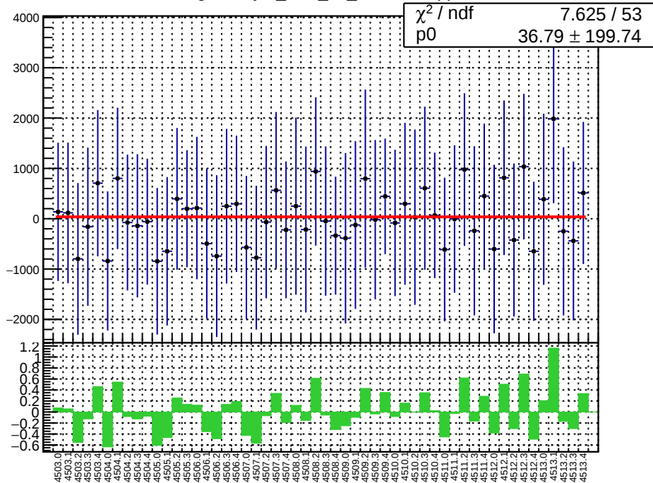
slug63: asym_bcm_an_ds3.mean/ppb
