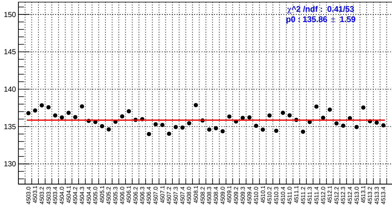
slug63: reg_asym_dsr.rms/ppm
