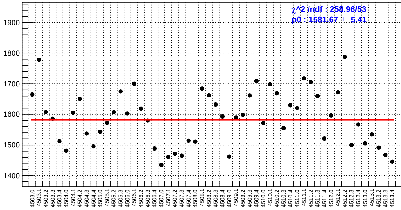
slug63: reg_asym_sam4.rms/ppm
