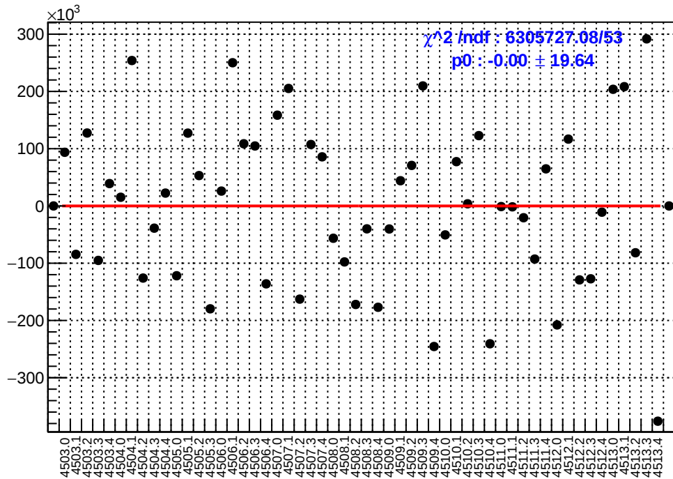
slug63: asym_sam3.mean/ppb-reg_asym_sam3.mean/ppb
