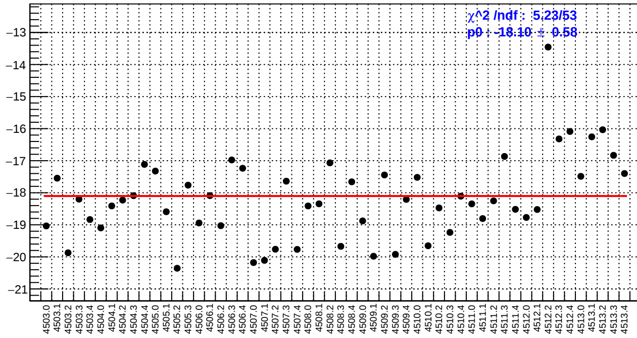
slug63: dsr_bpm4aX/(ppb/nm)
