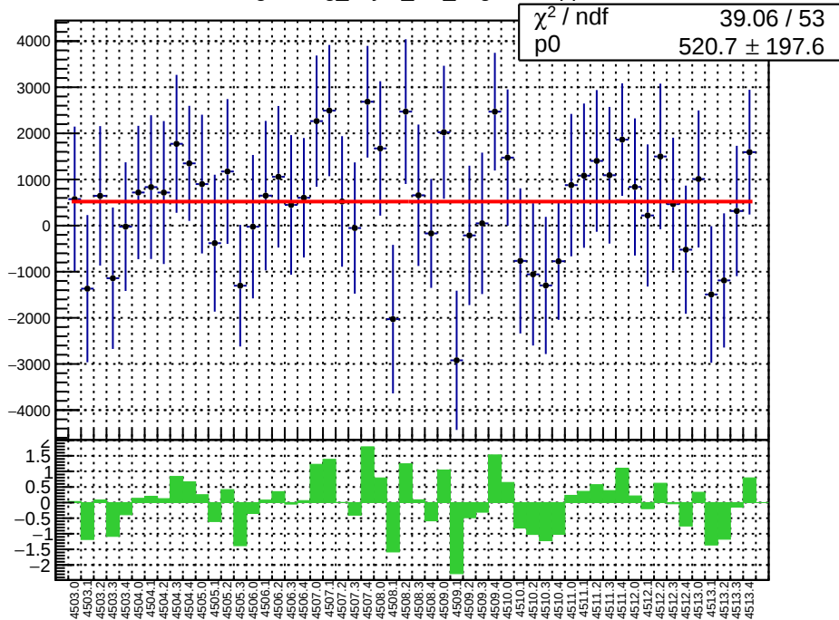
slug63: reg_asym_left_avg.mean/ppb
