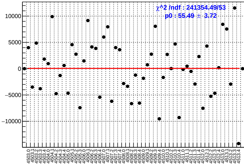
slug63: asym_us_dd.mean/ppb-reg_asym_us_dd.mean/ppb
