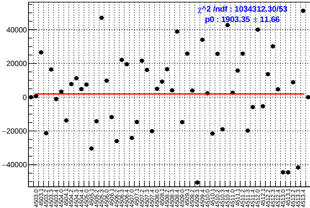
slug63: asym_sam6.mean/ppb-reg_asym_sam6.mean/ppb
