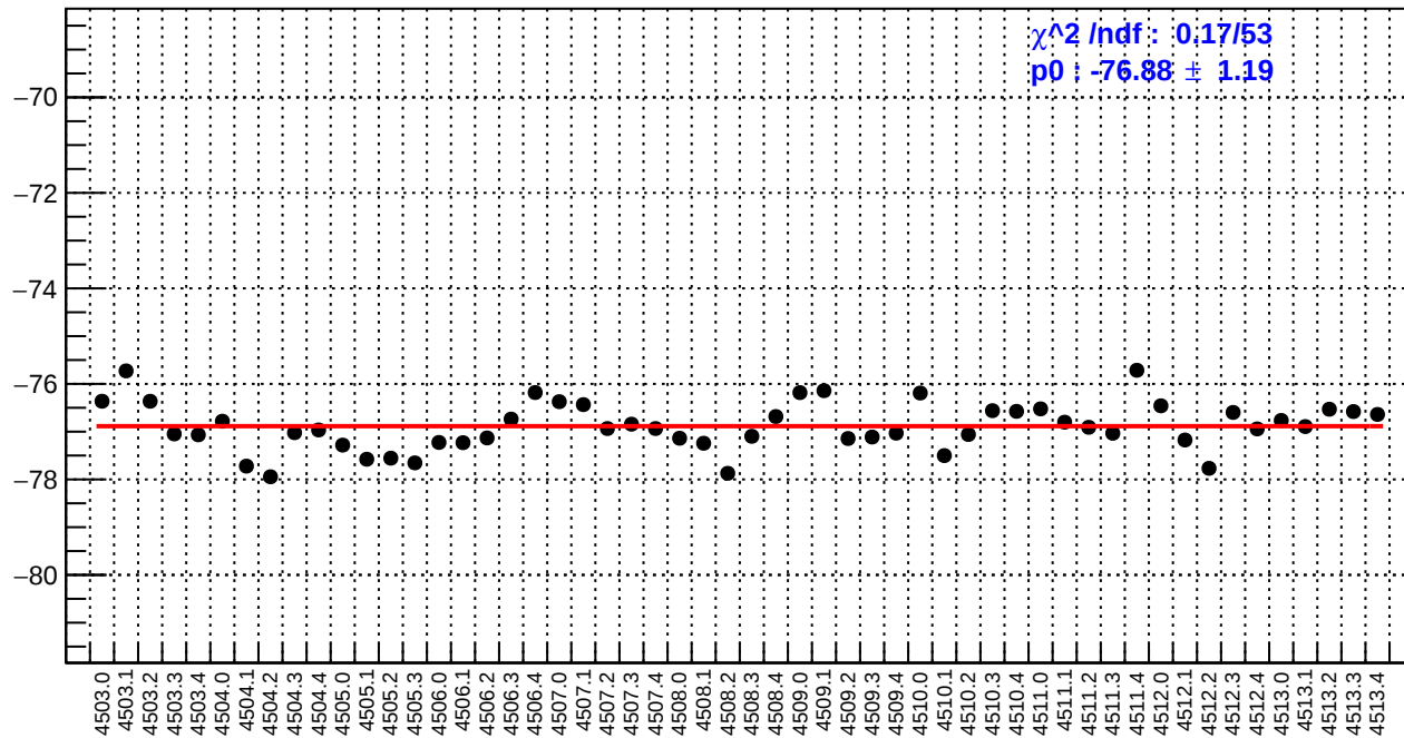
slug63: dsl_bpm4eX/(ppb/nm)
