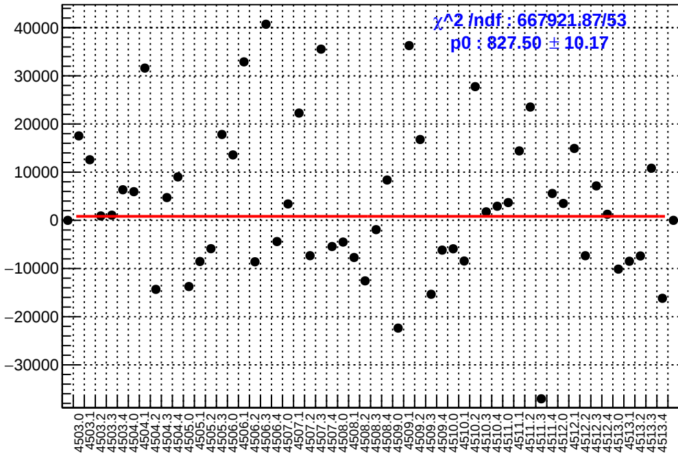
slug63: asym_sam5.mean/ppb-reg_asym_sam5.mean/ppb
