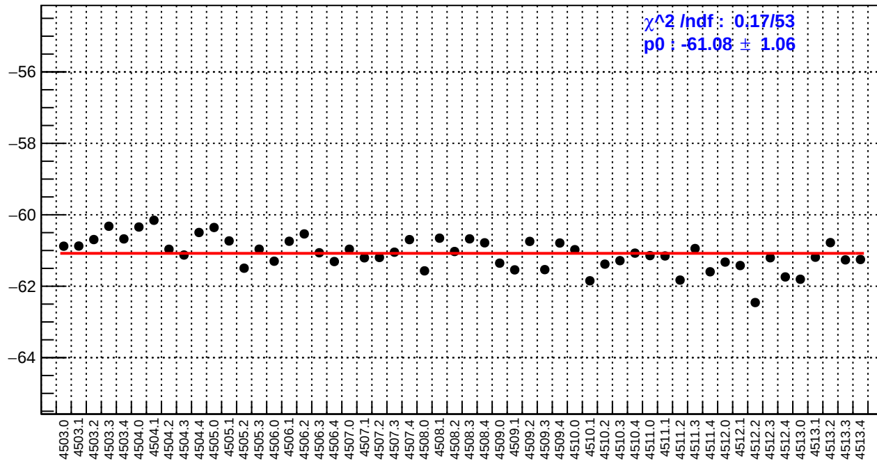
slug63: right_avg_bpm12X/(ppb/nm)
