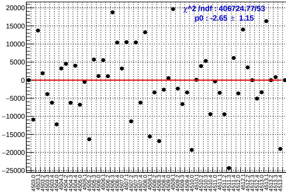
slug63: asym_atr_avg.mean/ppb-reg_asym_atr_avg.mean/ppb
