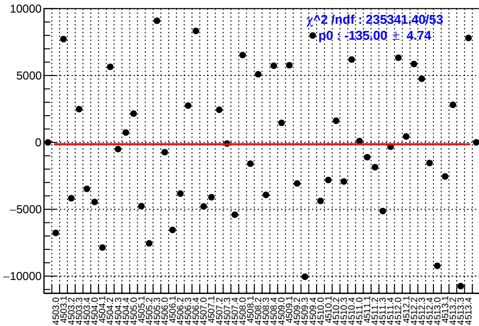
slug63: asym_usr.mean/ppb-reg_asym_usr.mean/ppb
