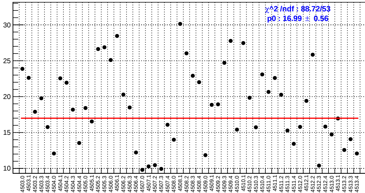
slug63: ds_avg_bpm4aY/(ppb/nm)
