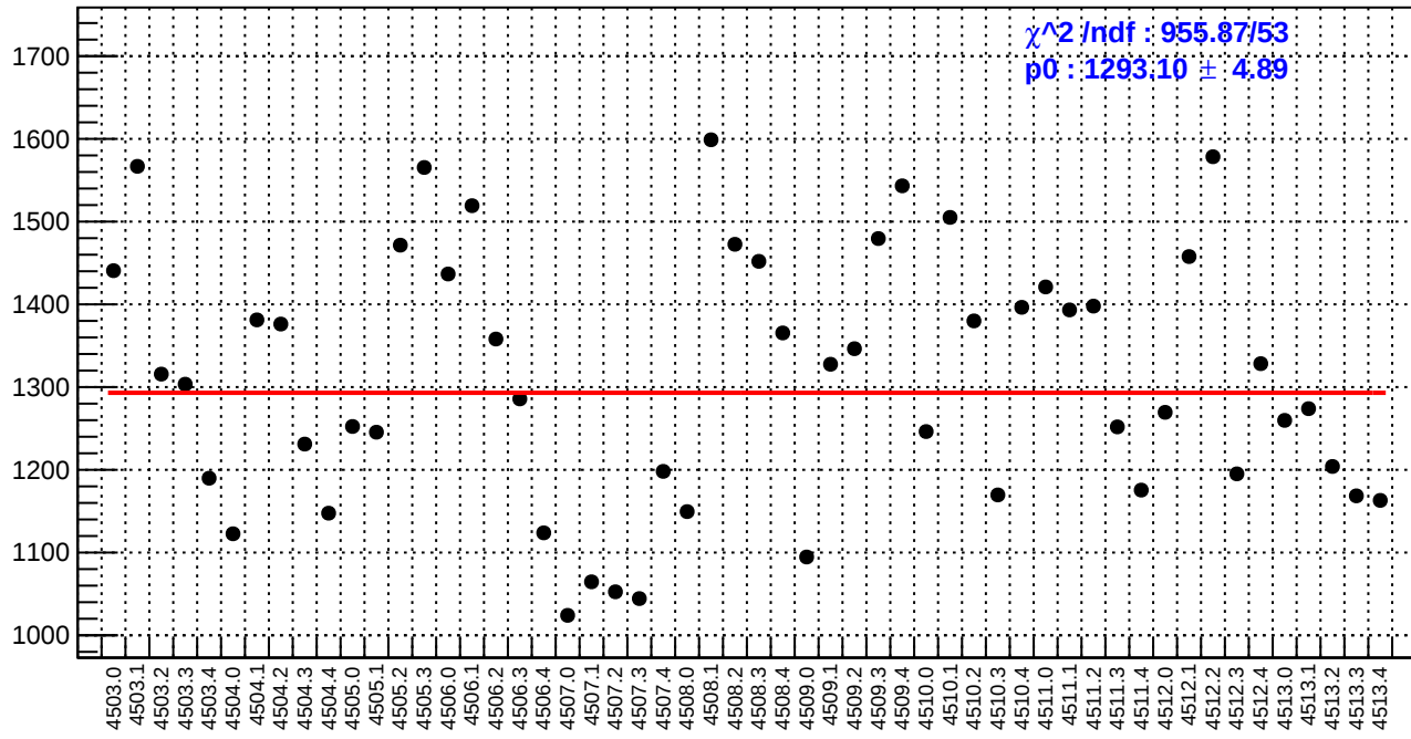
slug63: reg_asym_sam3.rms/ppm
