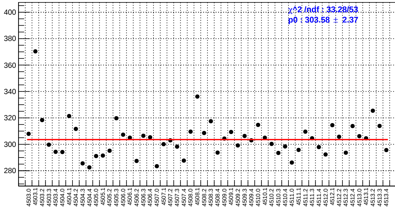
slug63: reg_asym_sam5.rms/ppm
