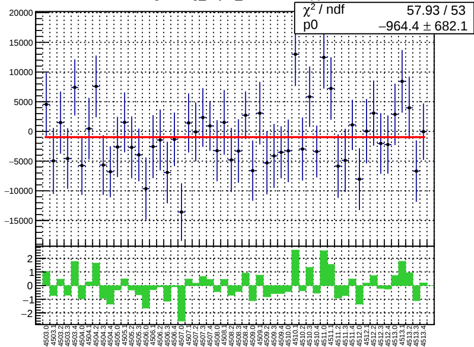
slug63: reg_asym_sam8.mean/ppb
