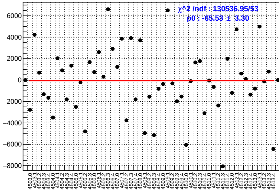
slug63: asym_us_avg.mean/ppb-reg_asym_us_avg.mean/ppb
