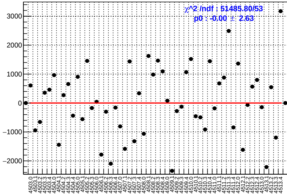
slug63: asym_atl1r2_dd.mean/ppb-reg_asym_atl1r2_dd.mean/ppb
