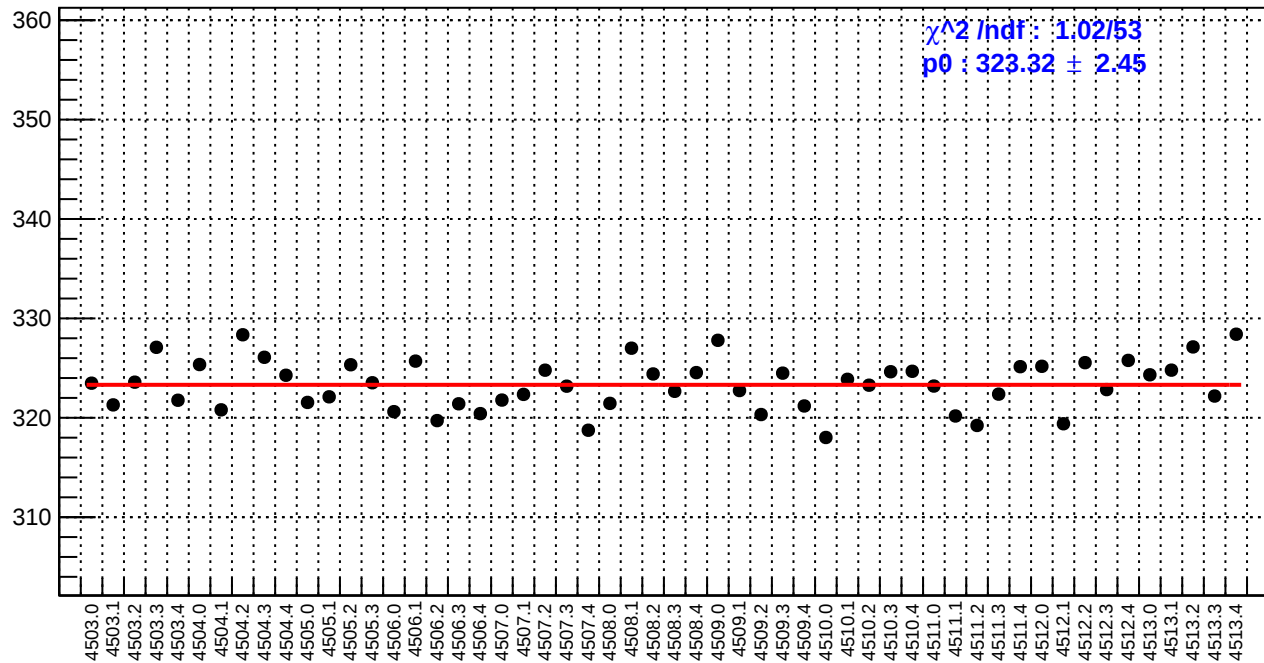
slug63: reg_asym_atl1r2_dd.rms/ppm
