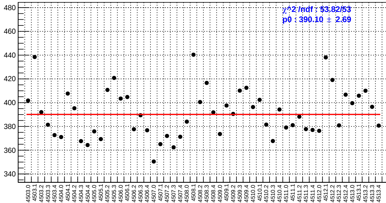
slug63: reg_asym_sam6.rms/ppm
