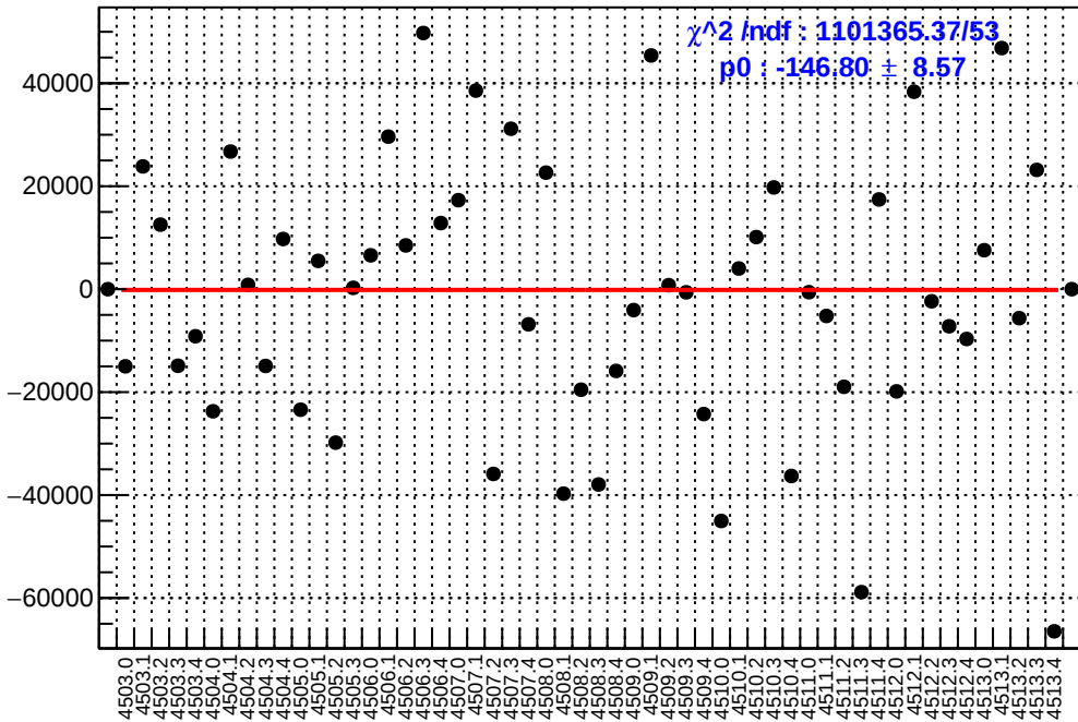
slug63: asym_atl2.mean/ppb-reg_asym_atl2.mean/ppb
