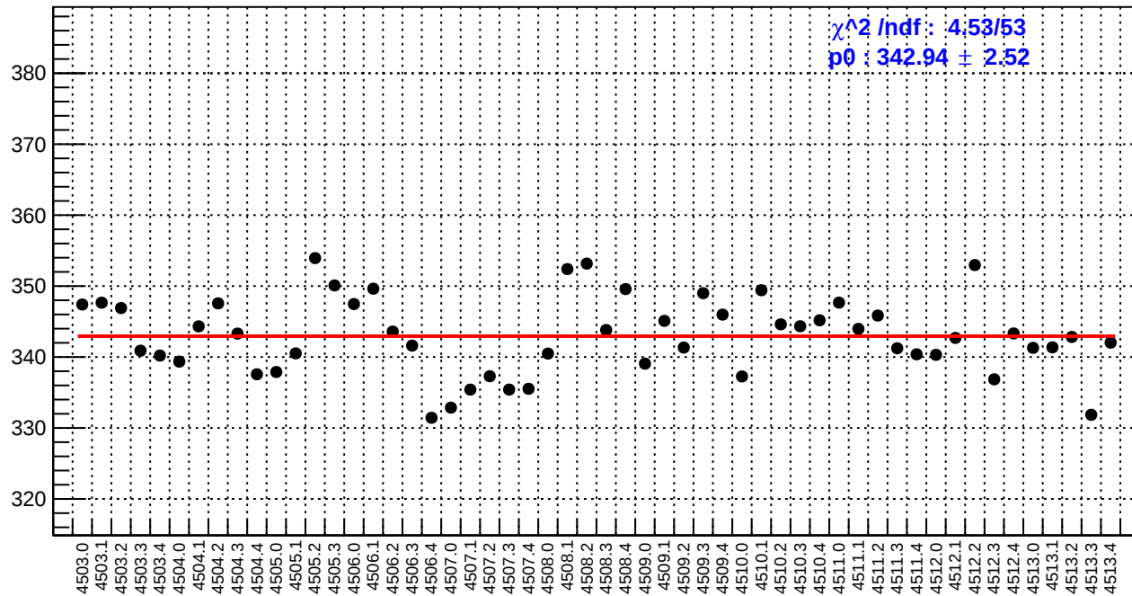
slug63: reg_asym_atl_dd.rms/ppm
