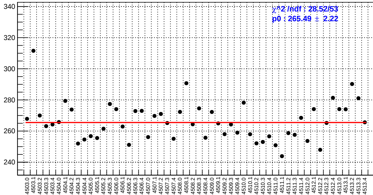
slug63: reg_asym_sam1.rms/ppm
