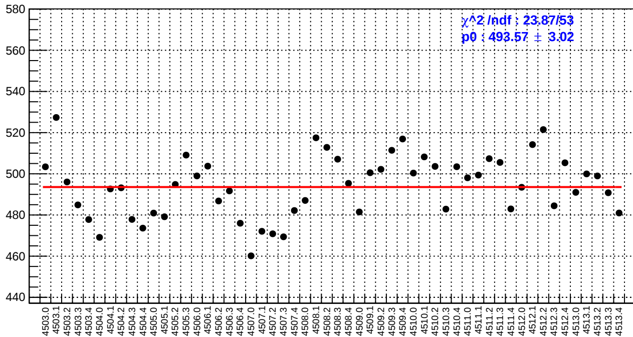
slug63: reg_asym_sam8.rms/ppm
