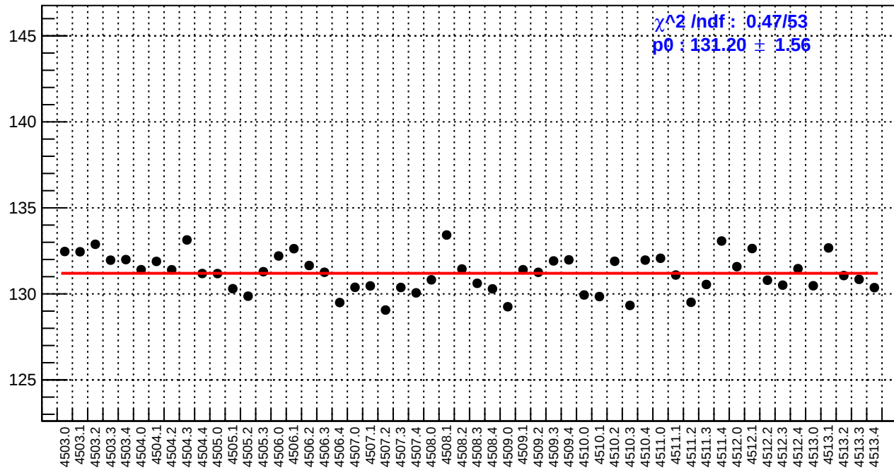
slug63: reg_asym_right_avg.rms/ppm
