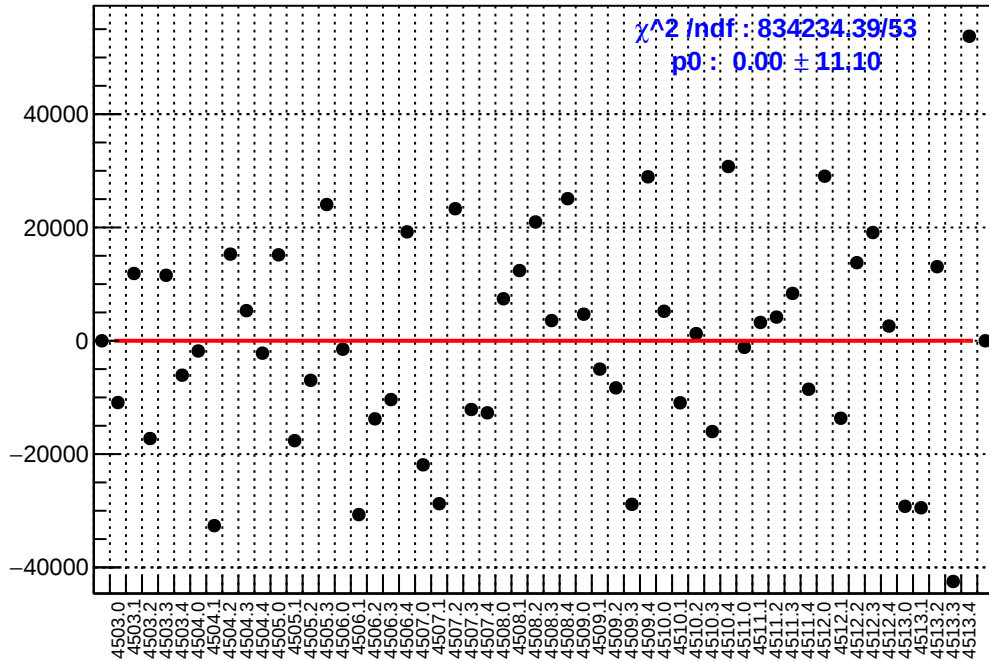
slug63: asym_sam7.mean/ppb-reg_asym_sam7.mean/ppb
