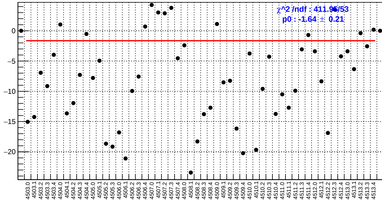
slug63: ds_avg_bpm4eY/(ppb/nm)
