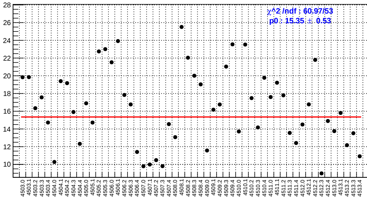
slug63: us_avg_bpm4aY/(ppb/nm)
