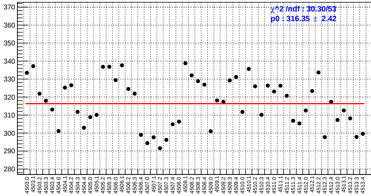
slug63: reg_asym_atr1l2_avg.rms/ppm
