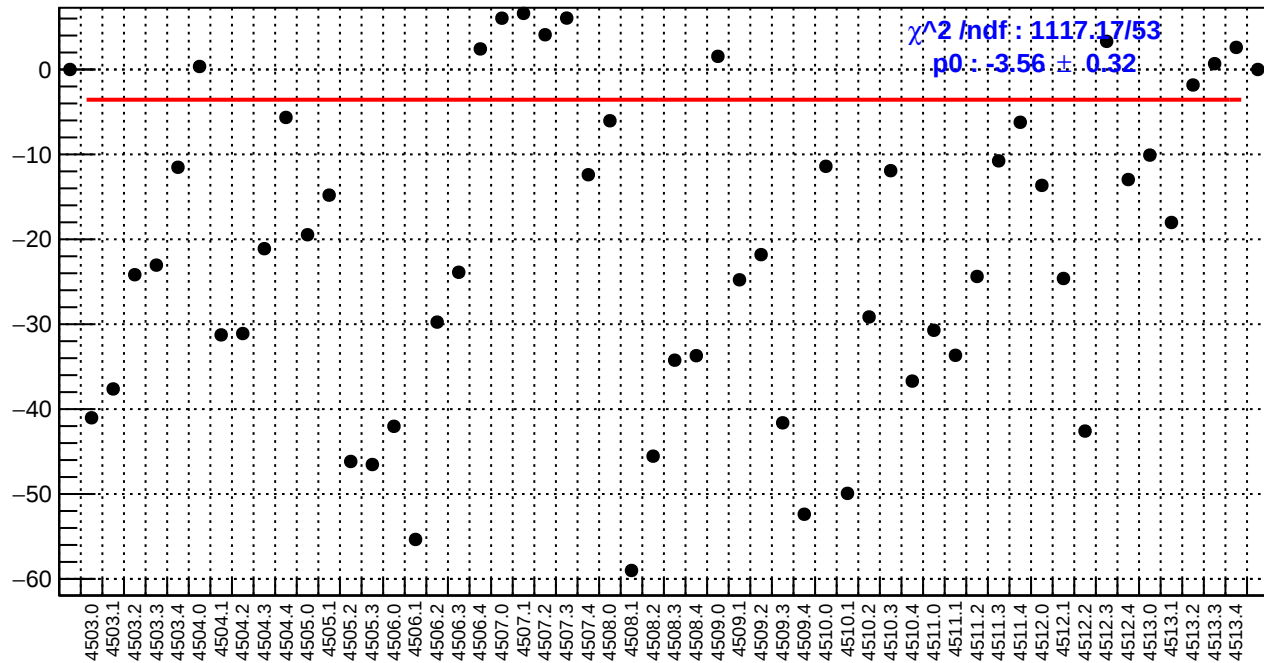
slug63: left_avg_bpm4eY/(ppb/nm)
