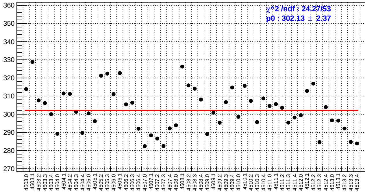
slug63: reg_asym_at2_avg.rms/ppm
