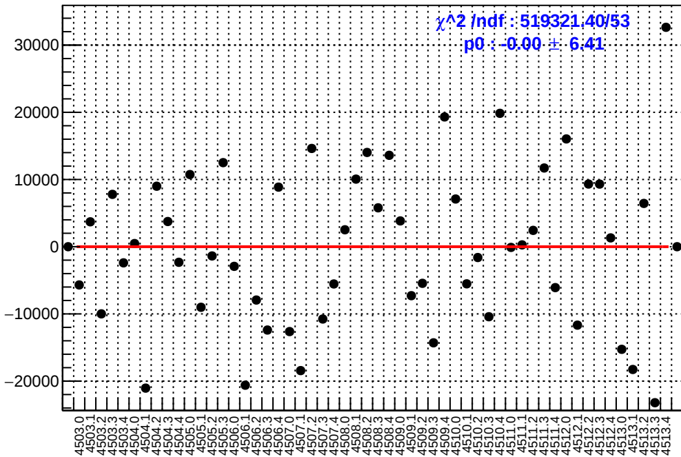
slug63: asym_atl_dd.mean/ppb-reg_asym_atl_dd.mean/ppb
