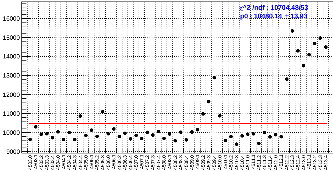
slug63: diff_bpm4eX.rms/nm
