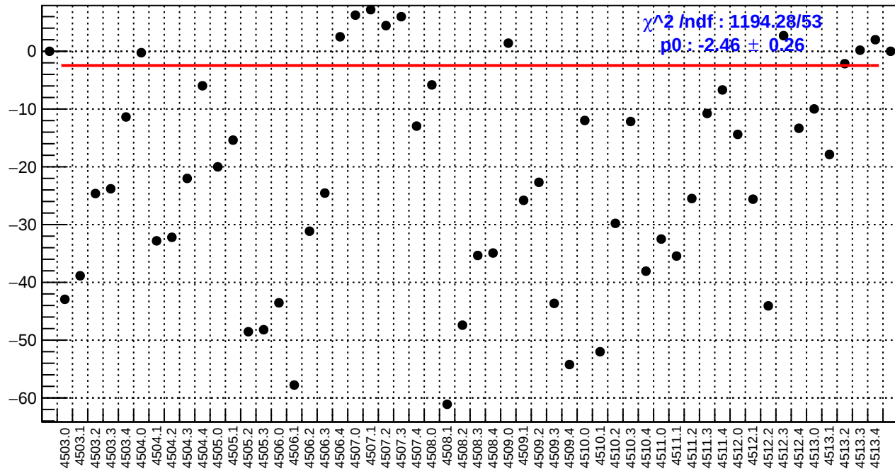
slug63: dsl_bpm4eY/(ppb/nm)
