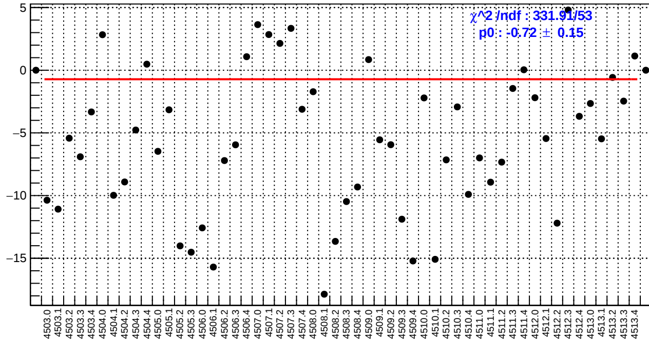
slug63: us_avg_bpm4eY/(ppb/nm)
