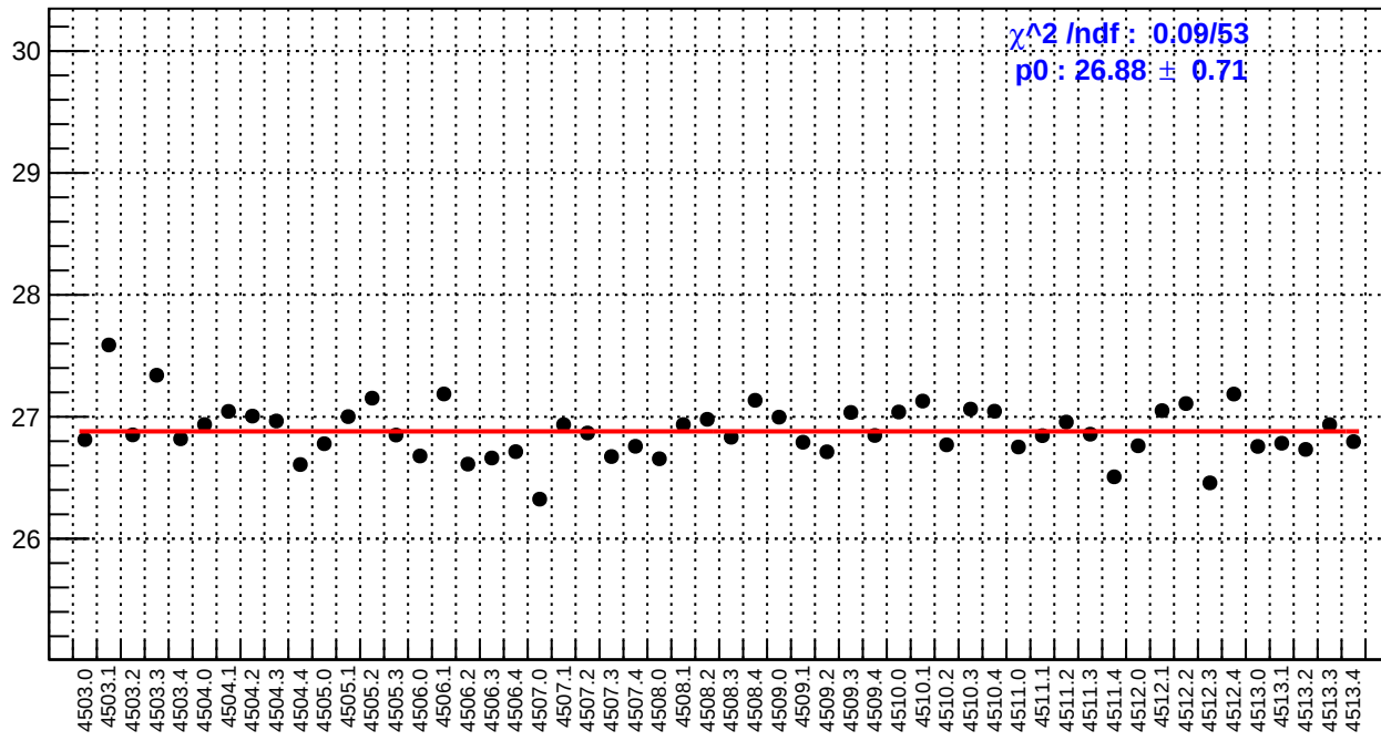
slug63: reg_asym_right_dd.rms/ppm
