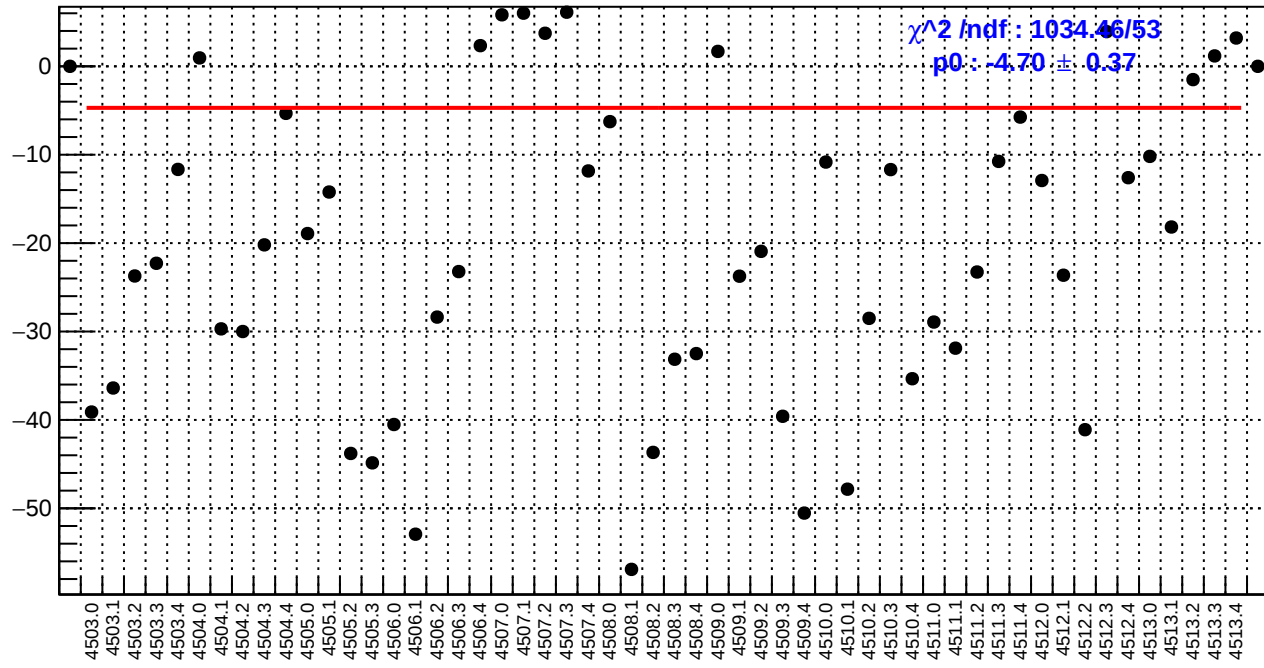
slug63: usl_bpm4eY/(ppb/nm)
