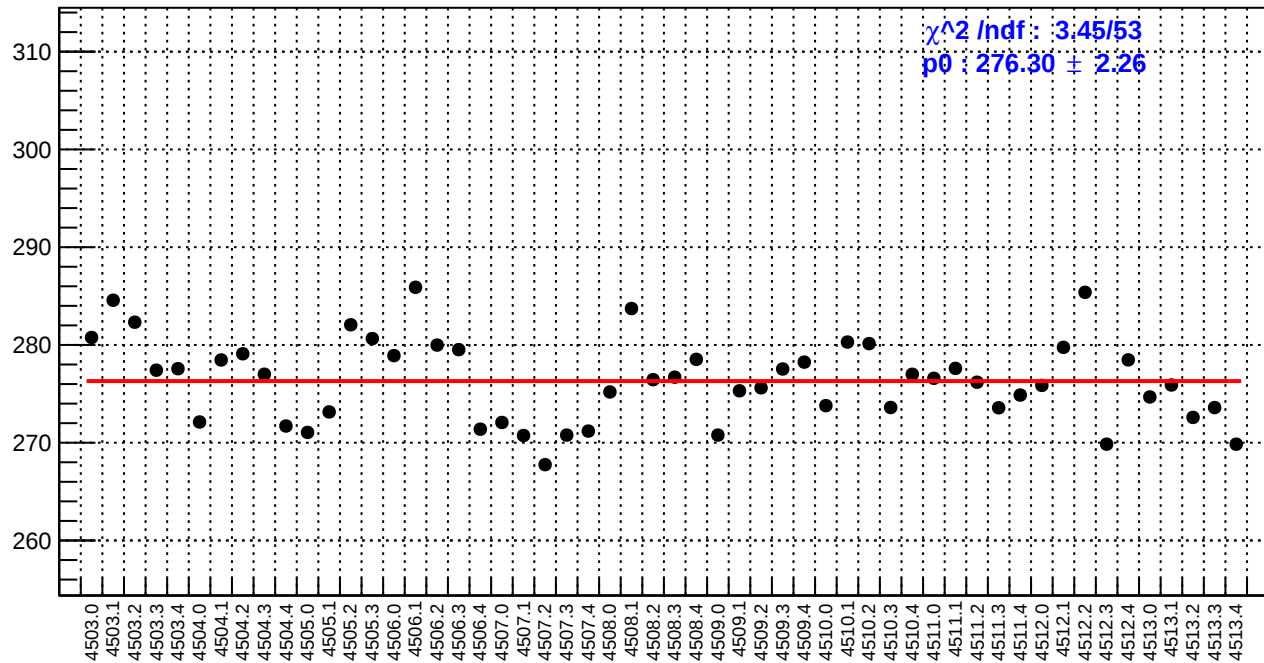
slug63: reg_asym_atr_avg.rms/ppm
