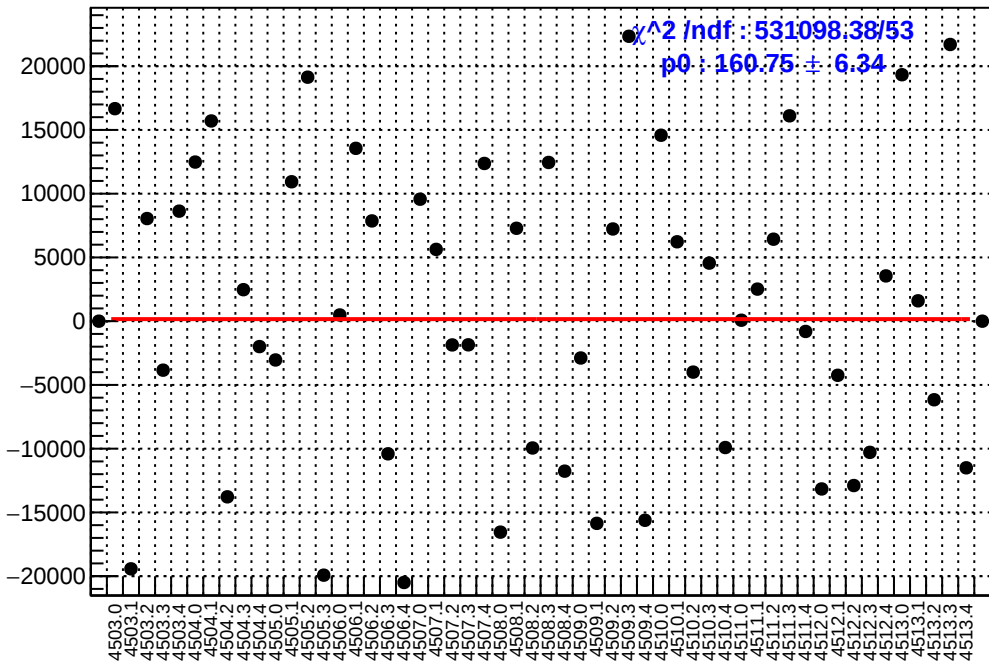
slug63: asym_atr_dd.mean/ppb-reg_asym_atr_dd.mean/ppb
