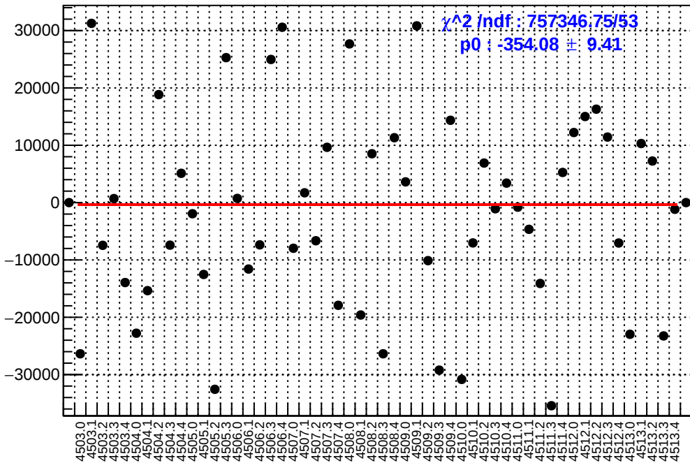
slug63: asym_atl1.mean/ppb-reg_asym_atl1.mean/ppb
