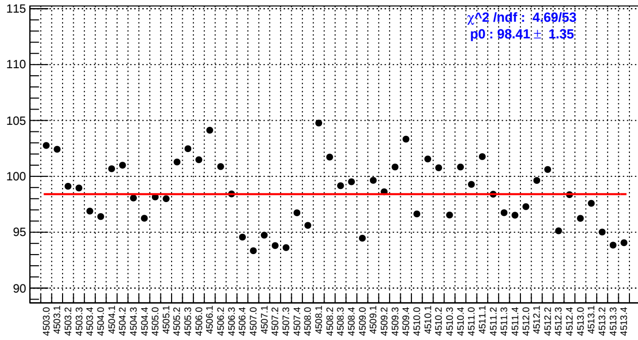
slug63: reg_asym_ds_dd.rms/ppm
