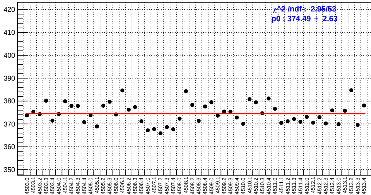
slug63: reg_asym_at1_avg.rms/ppm
