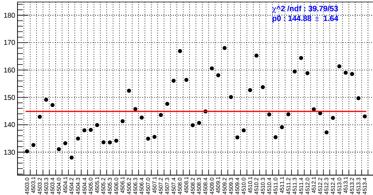
slug63: asym_bcm_an_ds3.rms/ppm
