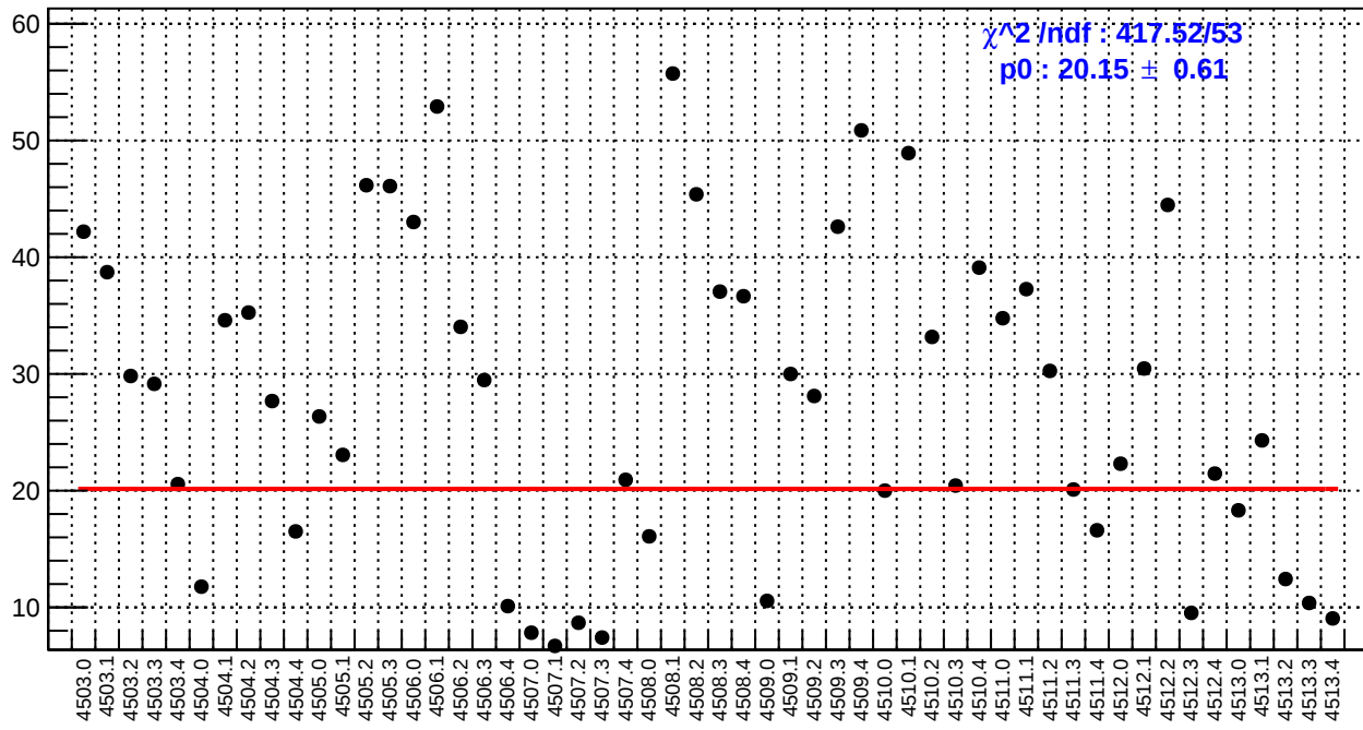
slug63: left_avg_bpm4aY/(ppb/nm)
