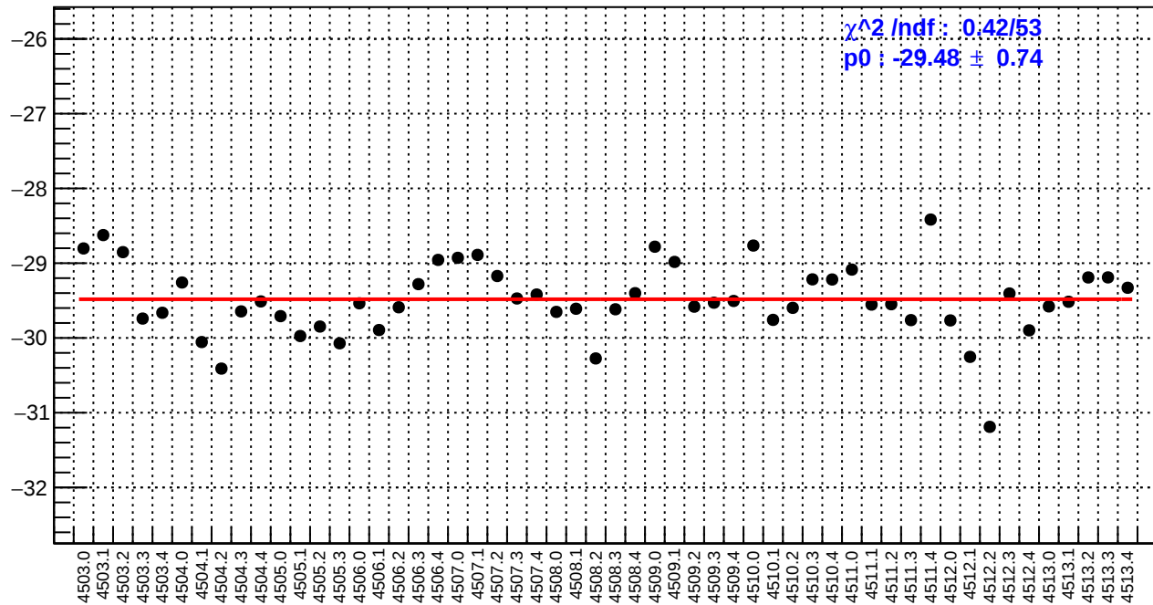
slug63: ds_avg_bpm4eX/(ppb/nm)
