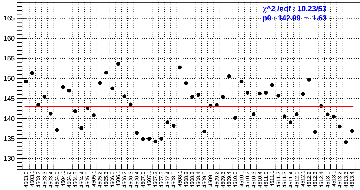
slug63: reg_asym_left_avg.rms/ppm
