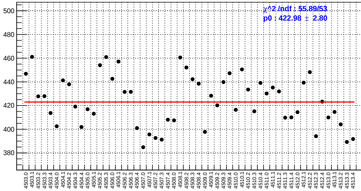
slug63: reg_asym_atl2.rms/ppm
