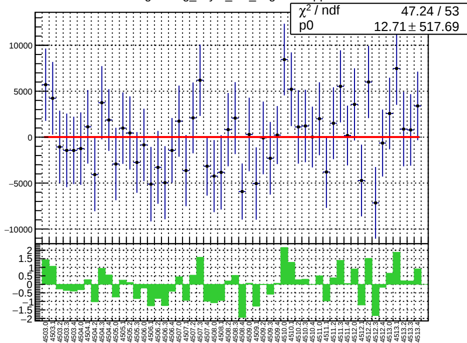
slug63: reg_asym_at1_avg.mean/ppb
