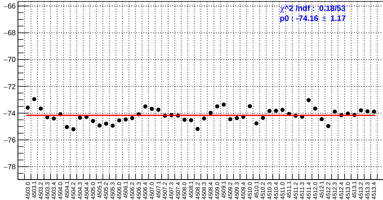
slug63: left_avg_bpm4eX/(ppb/nm)
