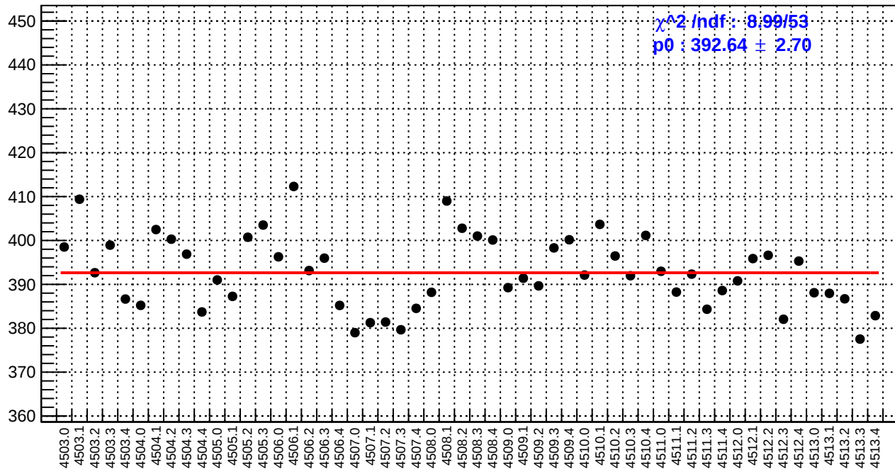
slug63: reg_asym_atl_avg.rms/ppm
