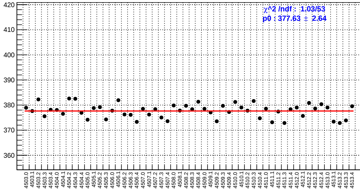
slug63: reg_asym_at1_dd.rms/ppm
