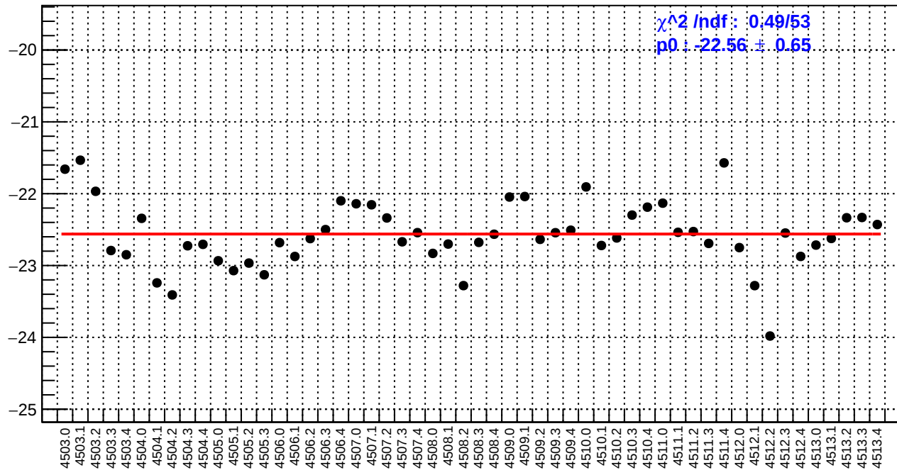
slug63: us_avg_bpm4eX/(ppb/nm)
