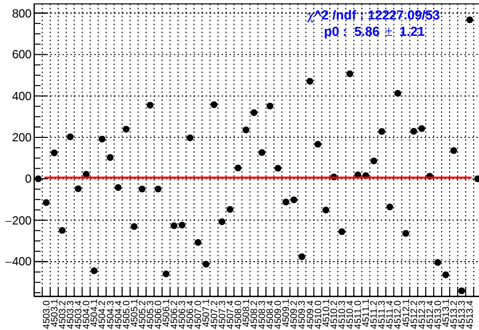
slug63: asym_left_dd.mean/ppb-reg_asym_left_dd.mean/ppb
