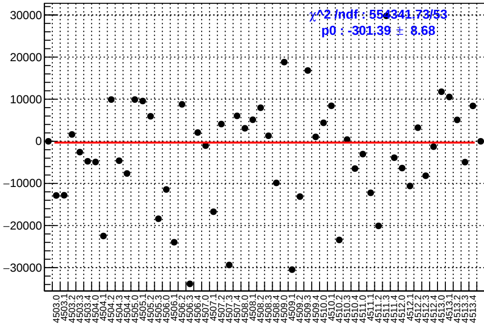
slug63: asym_sam1.mean/ppb-reg_asym_sam1.mean/ppb
