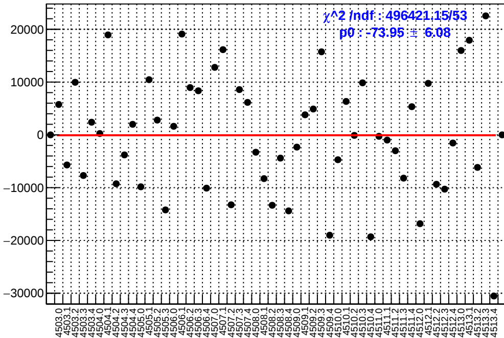
slug63: asym_atr1.mean/ppb-reg_asym_atr1.mean/ppb
