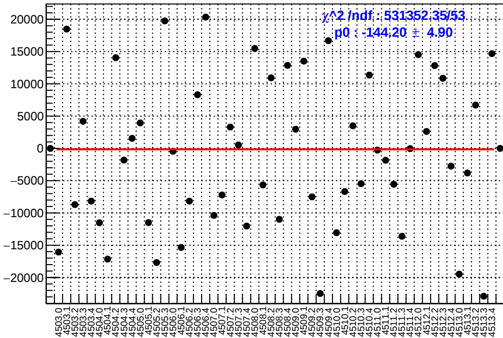
slug63: asym_at1_dd.mean/ppb-reg_asym_at1_dd.mean/ppb
