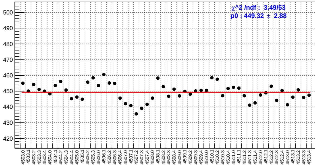
slug63: reg_asym_atr1.rms/ppm
