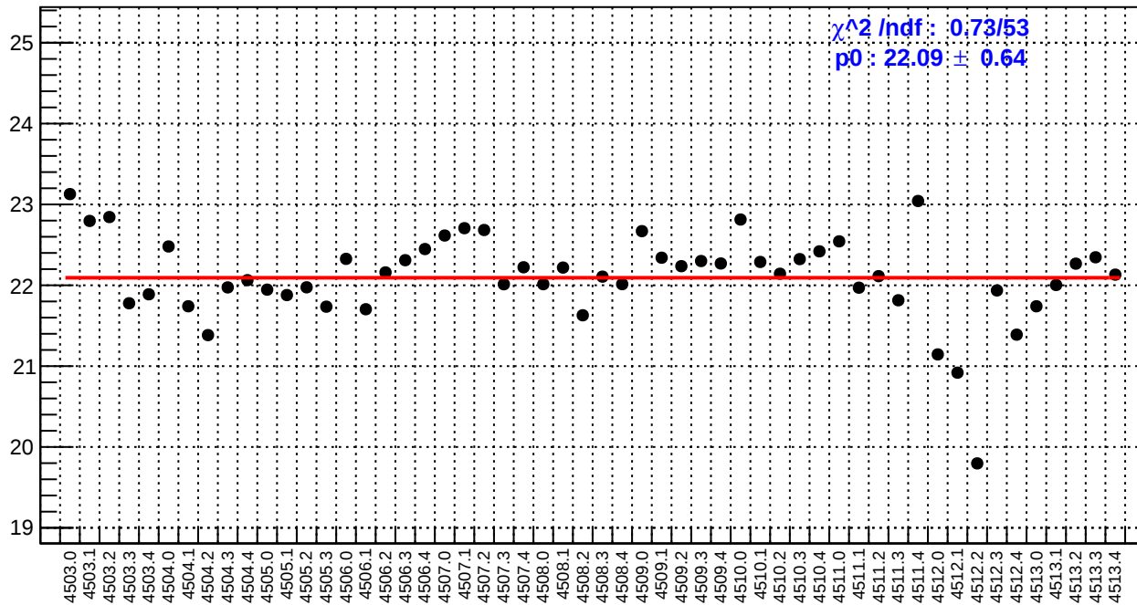
slug63: right_avg_bpm4eX/(ppb/nm)
