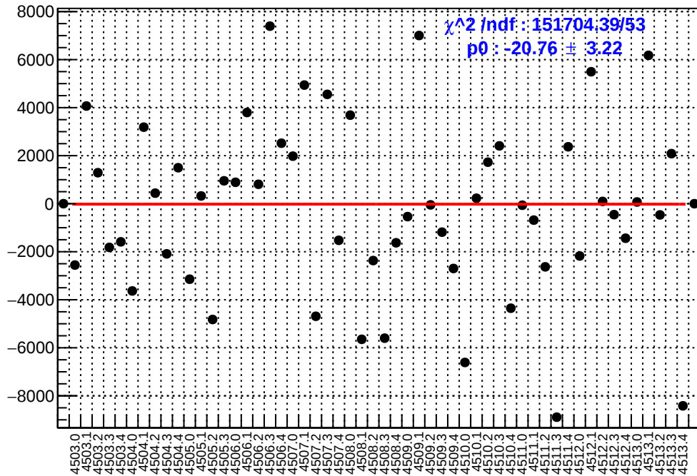
slug63: asym_ds_avg.mean/ppb-reg_asym_ds_avg.mean/ppb
