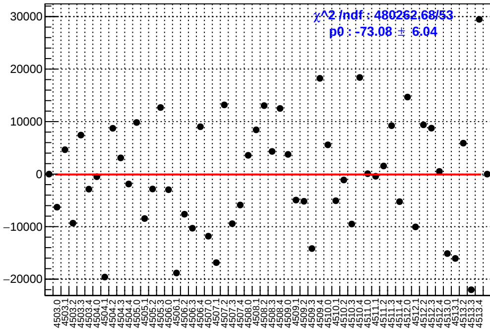
slug63: asym_at2_dd.mean/ppb-reg_asym_at2_dd.mean/ppb
