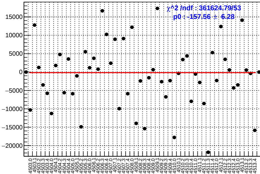
slug63: asym_at1_avg.mean/ppb-reg_asym_at1_avg.mean/ppb
