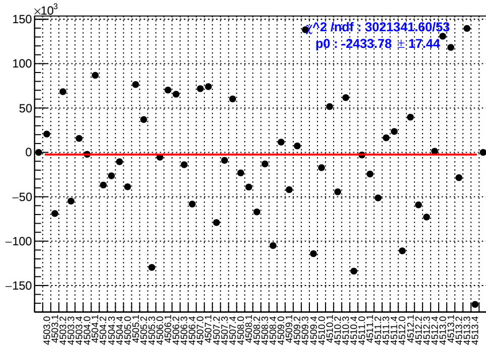
slug63: asym_sam2.mean/ppb-reg_asym_sam2.mean/ppb
