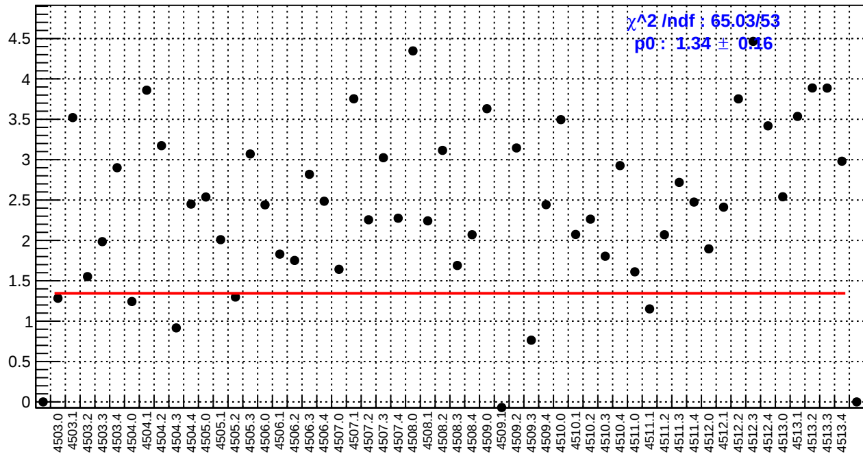
slug63: us_avg_bpm4aX/(ppb/nm)
