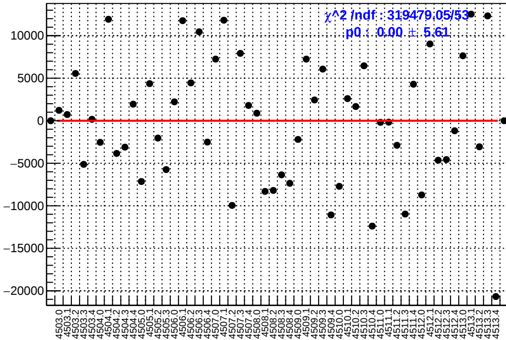
slug63: asym_usl.mean/ppb-reg_asym_usl.mean/ppb
