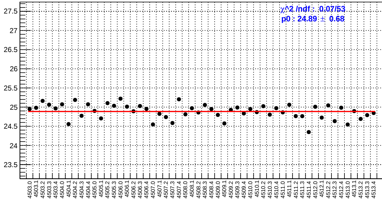
slug63: reg_asym_left_dd.rms/ppm
