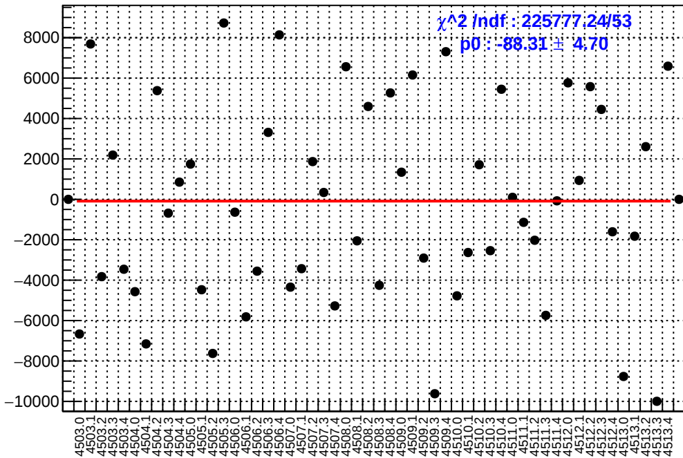
slug63: asym_right_avg.mean/ppb-reg_asym_right_avg.mean/ppb
