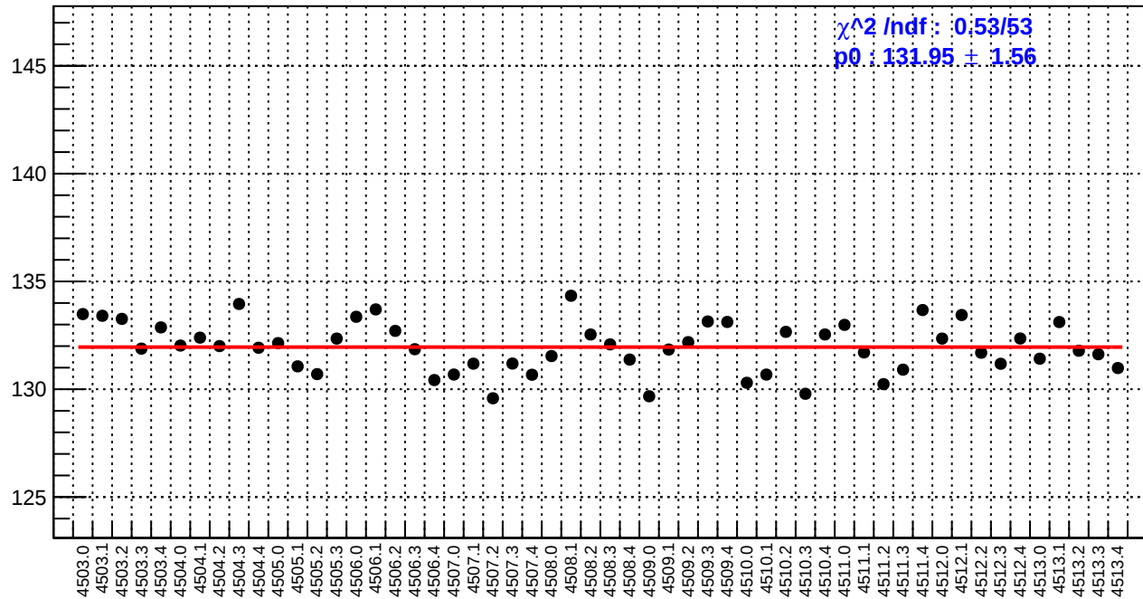
slug63: reg_asym_usr.rms/ppm
