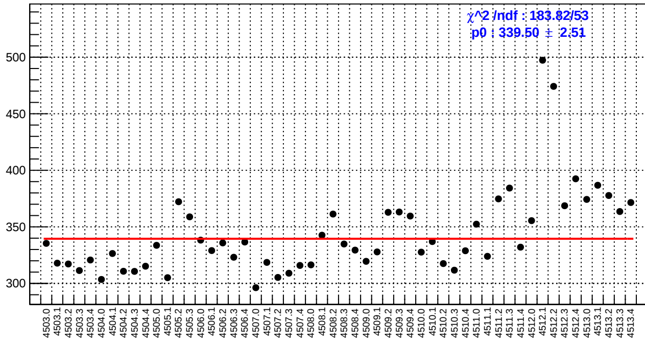
slug63: reg_asym_sam7.rms/ppm
