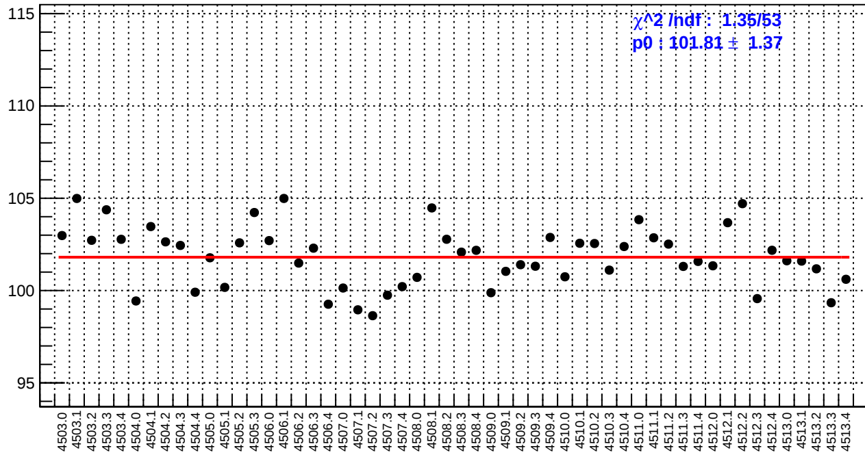
slug63: reg_asym_ds_avg.rms/ppm
