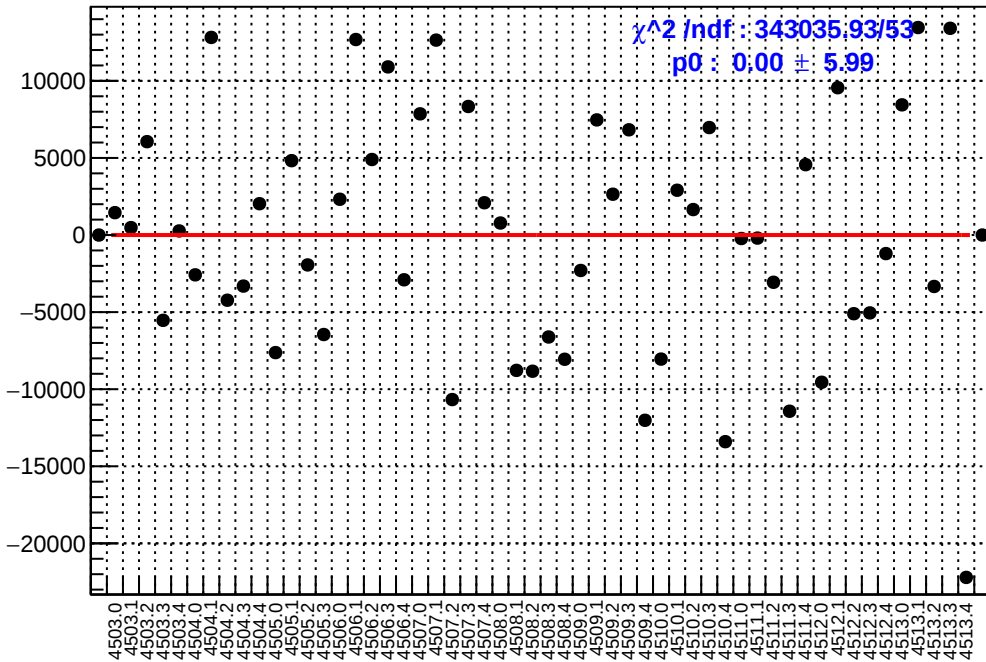
slug63: asym_dsl.mean/ppb-reg_asym_dsl.mean/ppb
