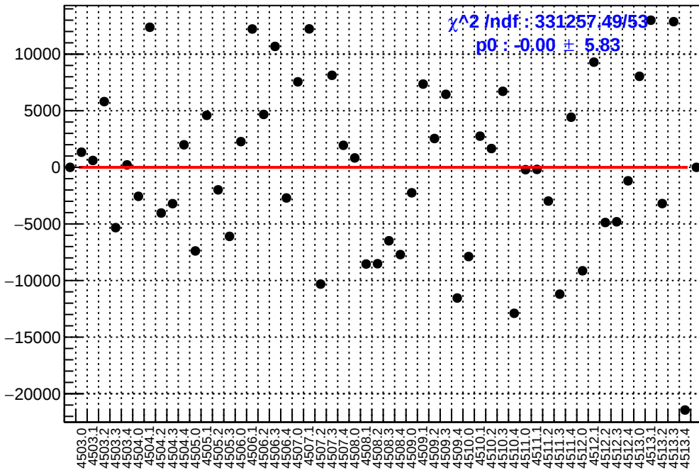
slug63: asym_left_avg.mean/ppb-reg_asym_left_avg.mean/ppb
