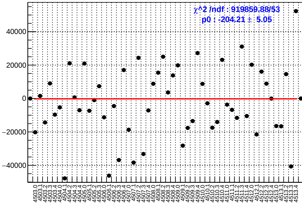
slug63: asym_sam8.mean/ppb-reg_asym_sam8.mean/ppb
