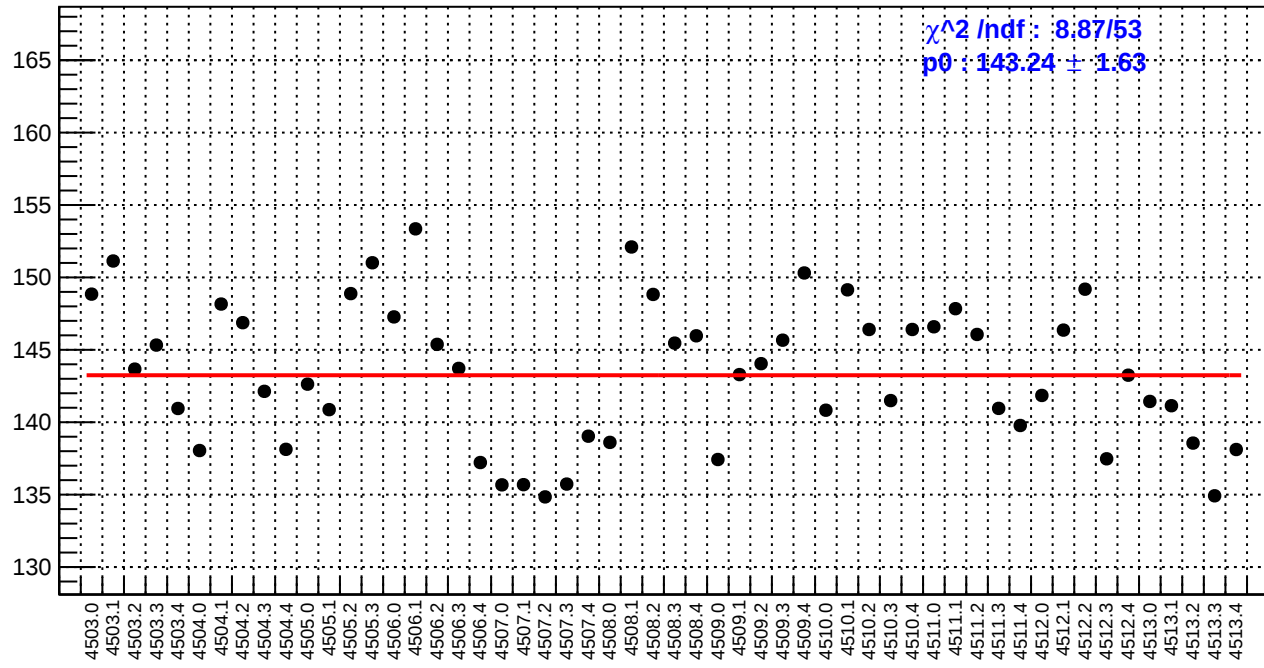
slug63: reg_asym_usl.rms/ppm
