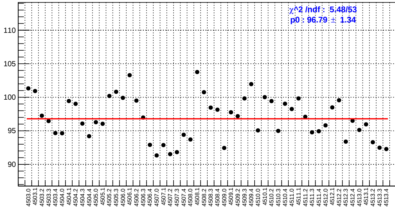
slug63: reg_asym_us_dd.rms/ppm
