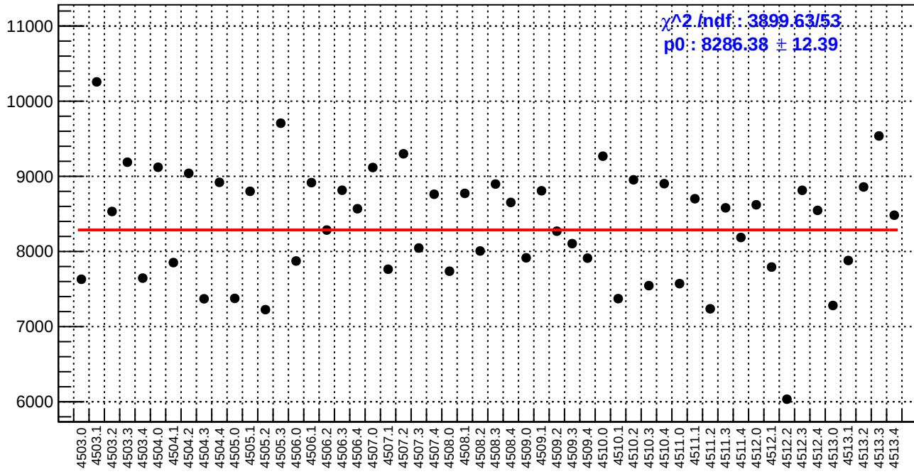
slug63: diff_bpm4aY.rms/nm
