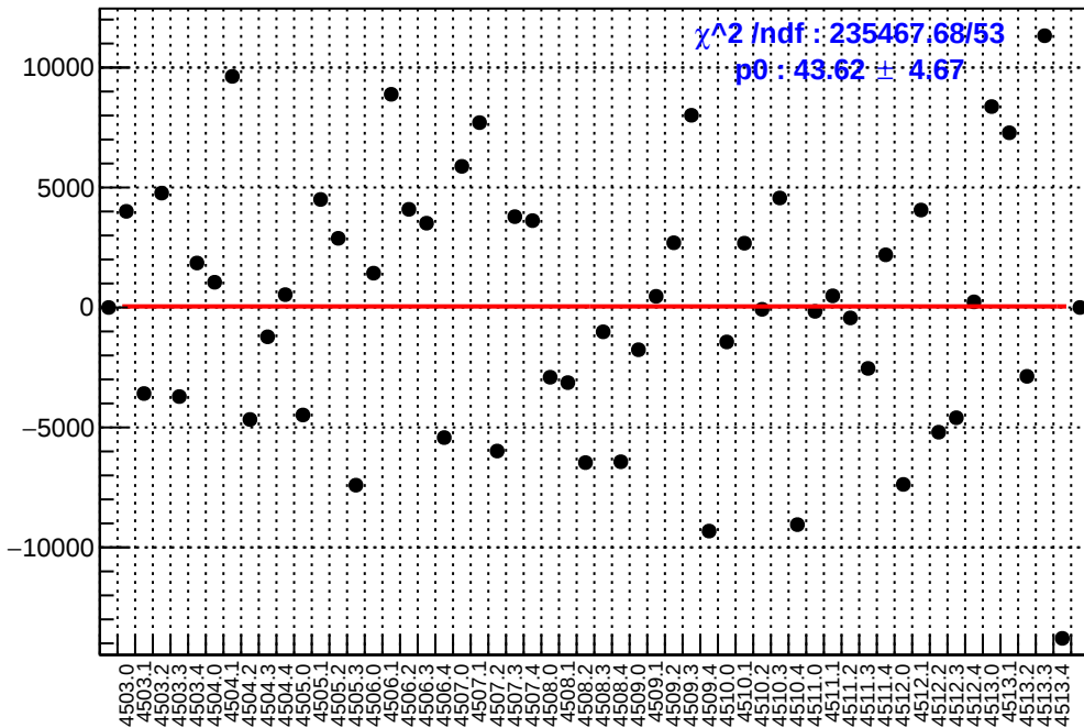
slug63: asym_ds_dd.mean/ppb-reg_asym_ds_dd.mean/ppb
