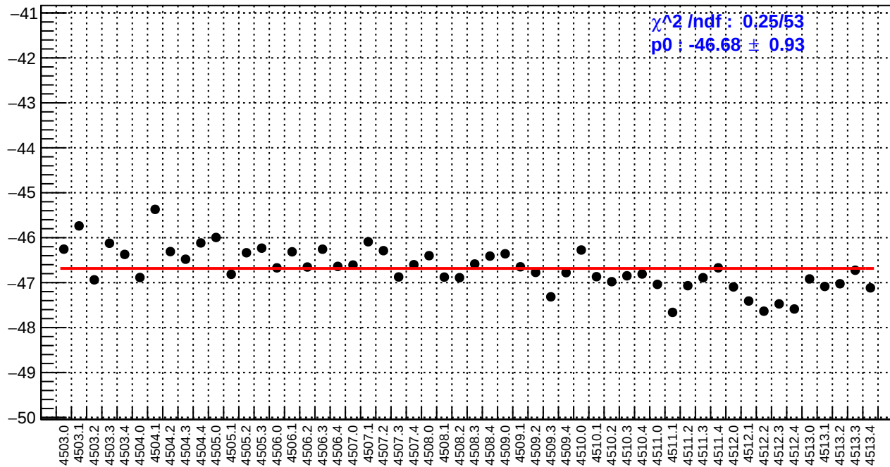
slug63: left_avg_bpm12X/(ppb/nm)
