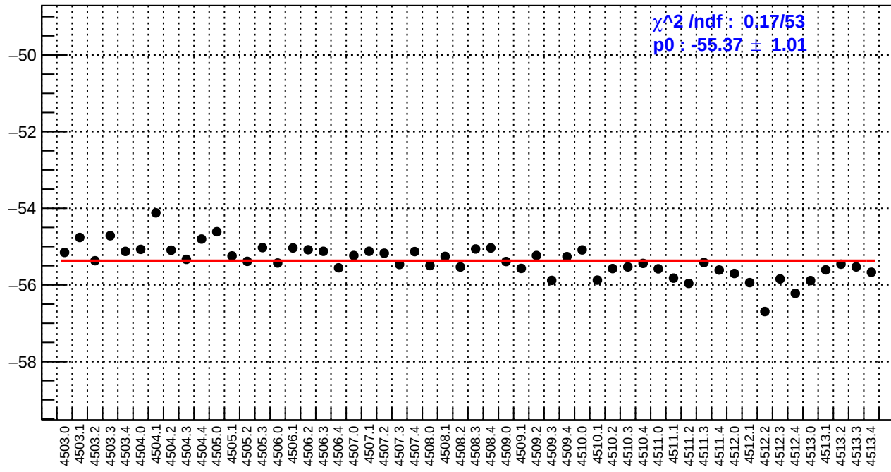
slug63: ds_avg_bpm12X/(ppb/nm)
