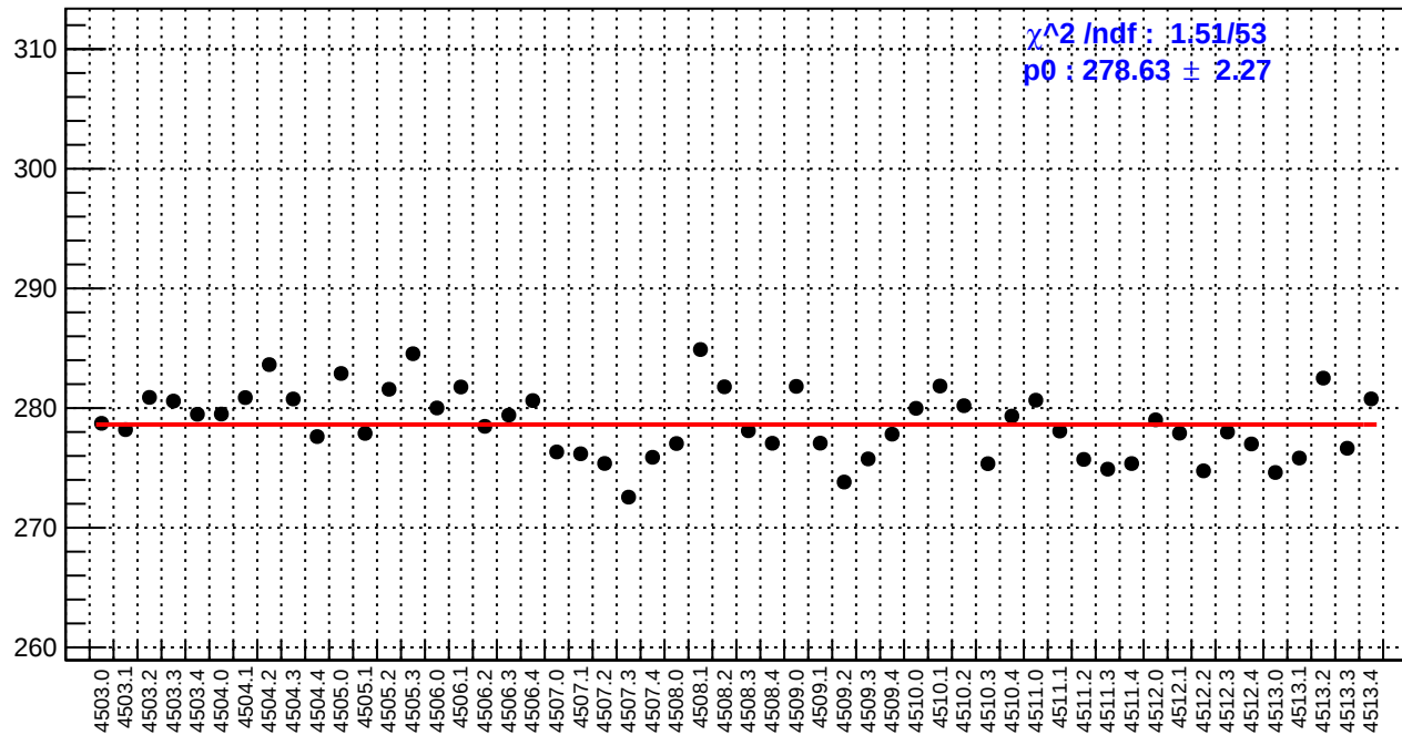
slug63: reg_asym_atr_dd.rms/ppm
