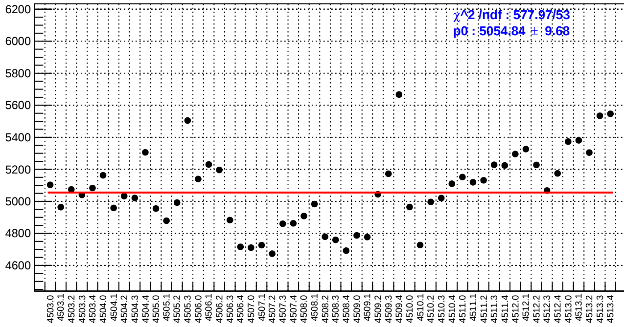
slug63: diff_bpm11X.rms/nm
