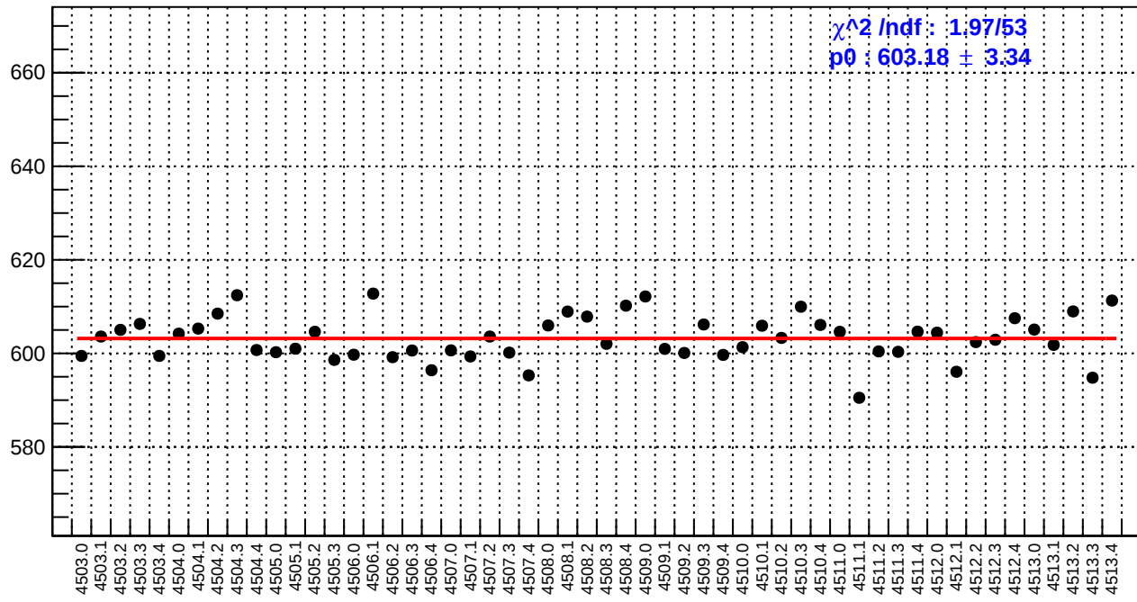
slug63: reg_asym_atl1.rms/ppm
