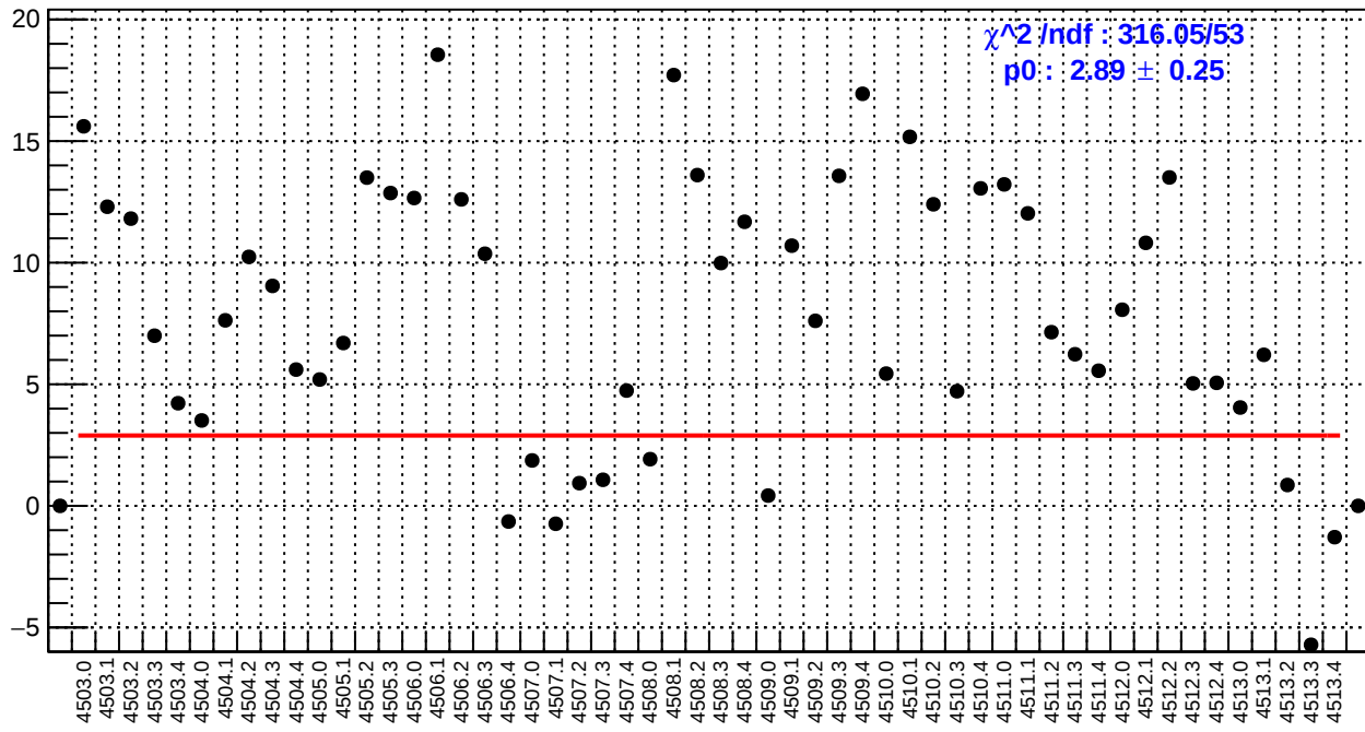
slug63: right_avg_bpm4eY/(ppb/nm)
