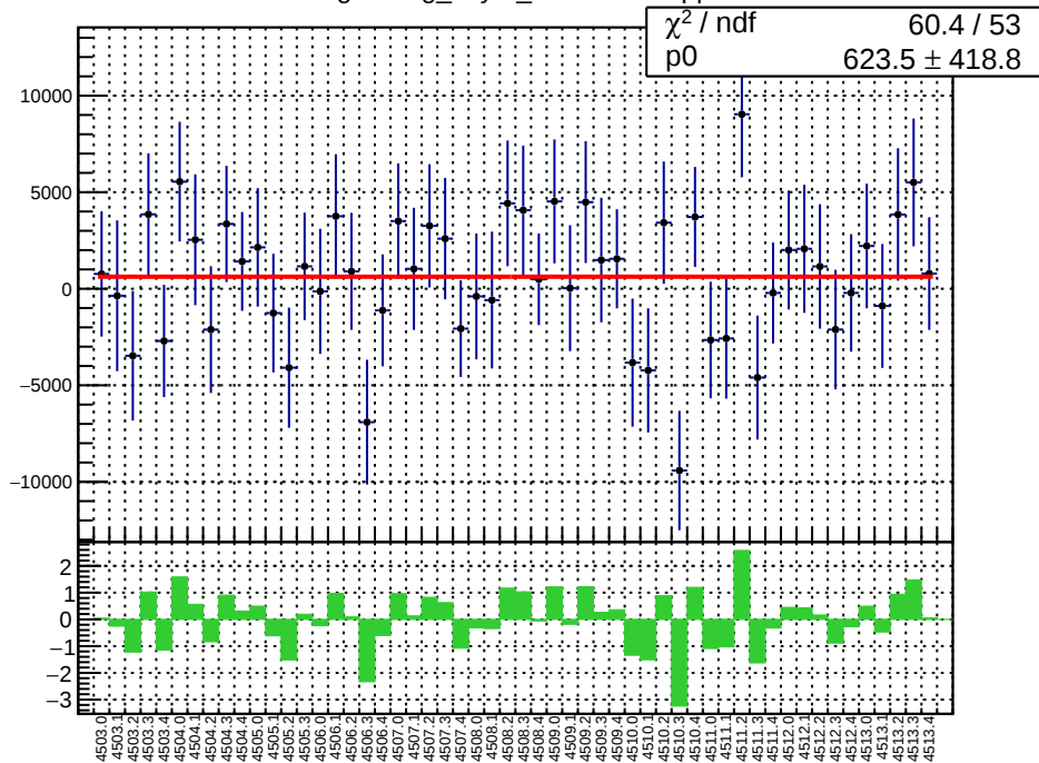
slug63: reg_asym_sam5.mean/ppb
