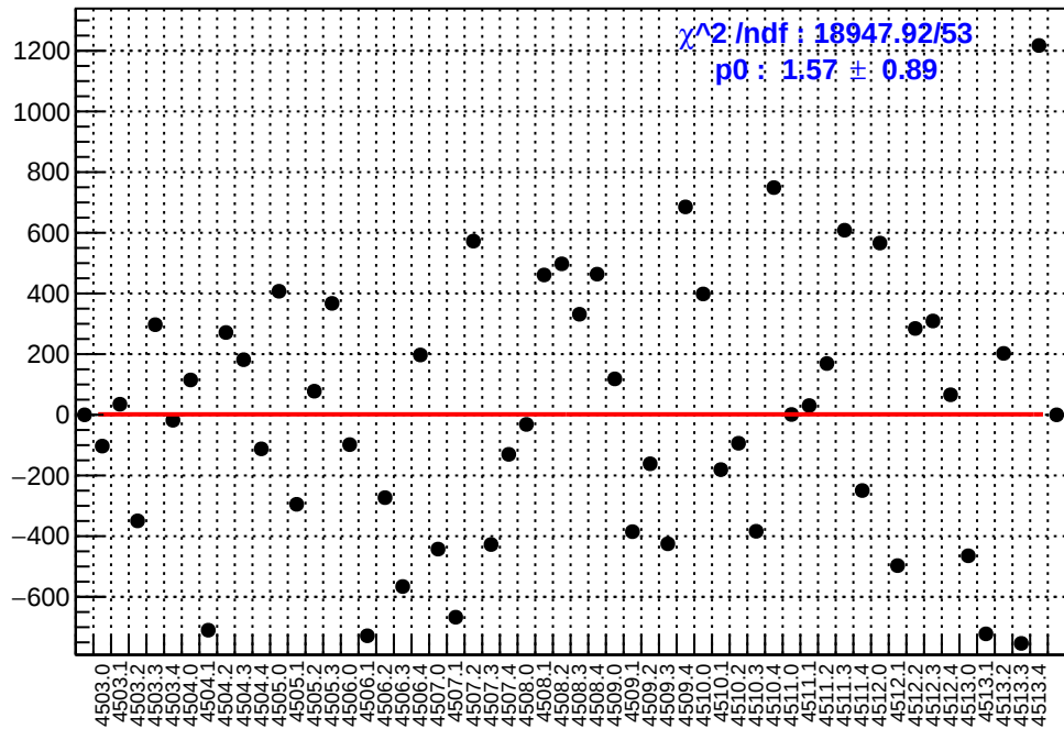
slug63: asym_right_dd.mean/ppb-reg_asym_right_dd.mean/ppb
