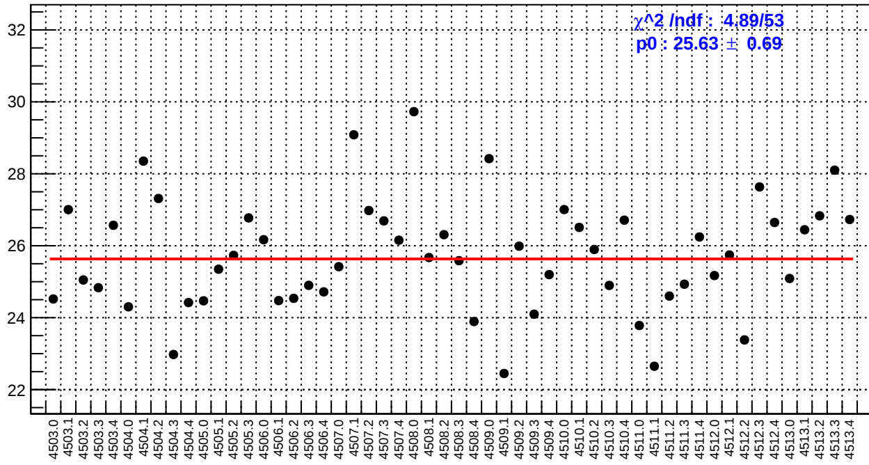
slug63: left_avg_bpm4aX/(ppb/nm)
