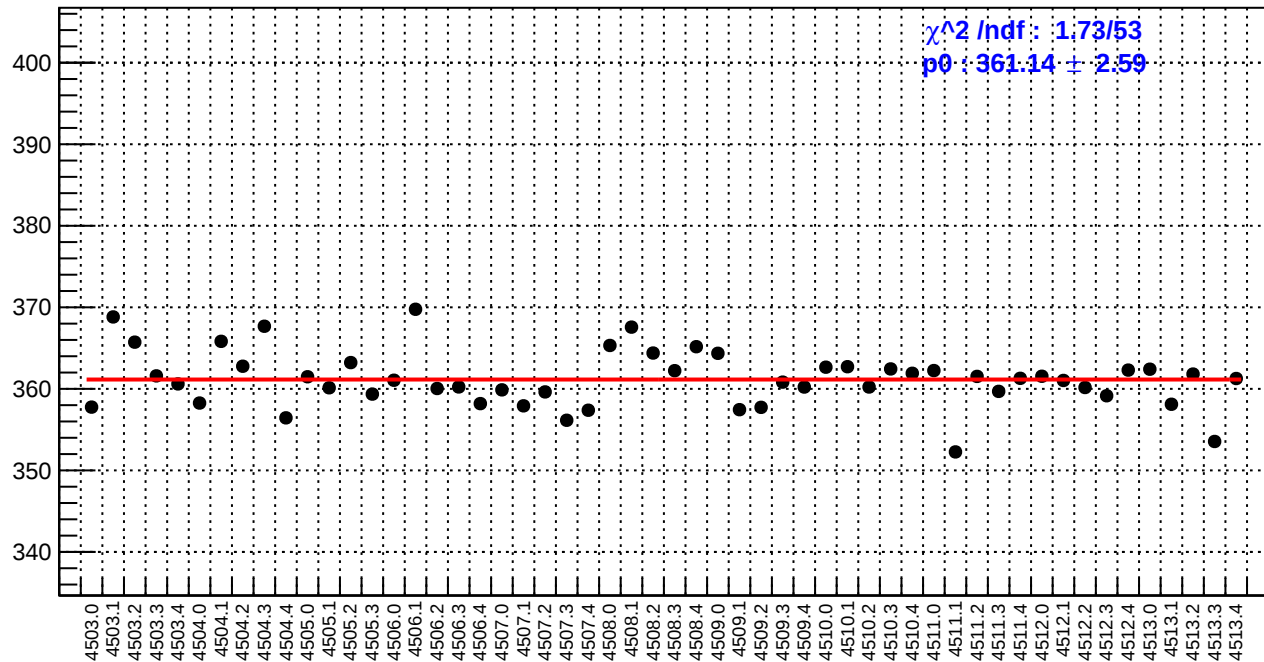
slug63: reg_asym_atl1r2_avg.rms/ppm
