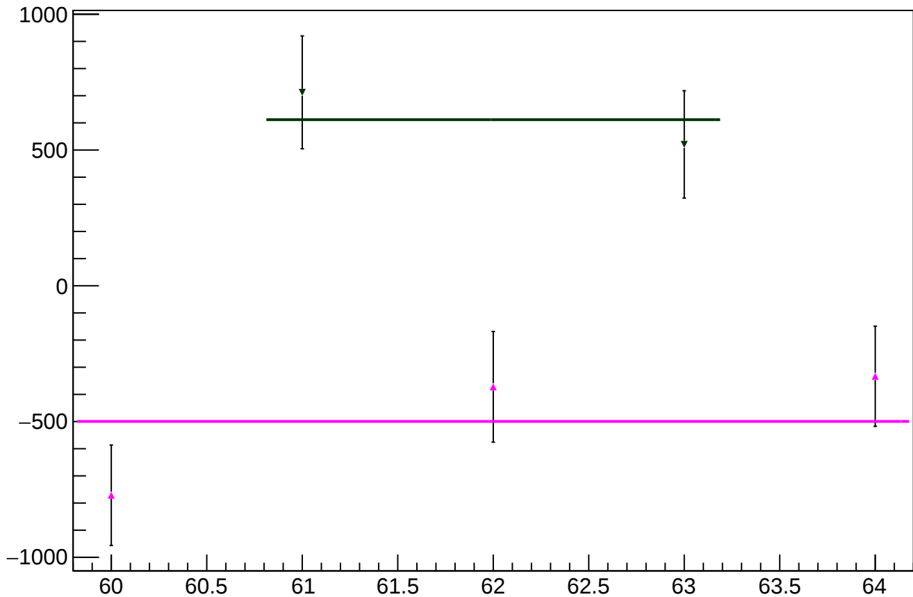
reg_asym_left_avg_mean vs slug
