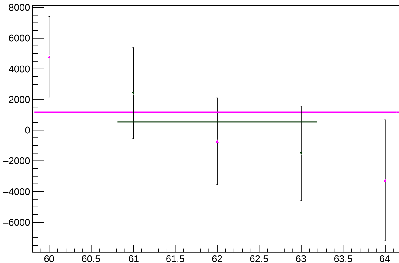
asym_sam_48_avg_correction_mean vs slug
