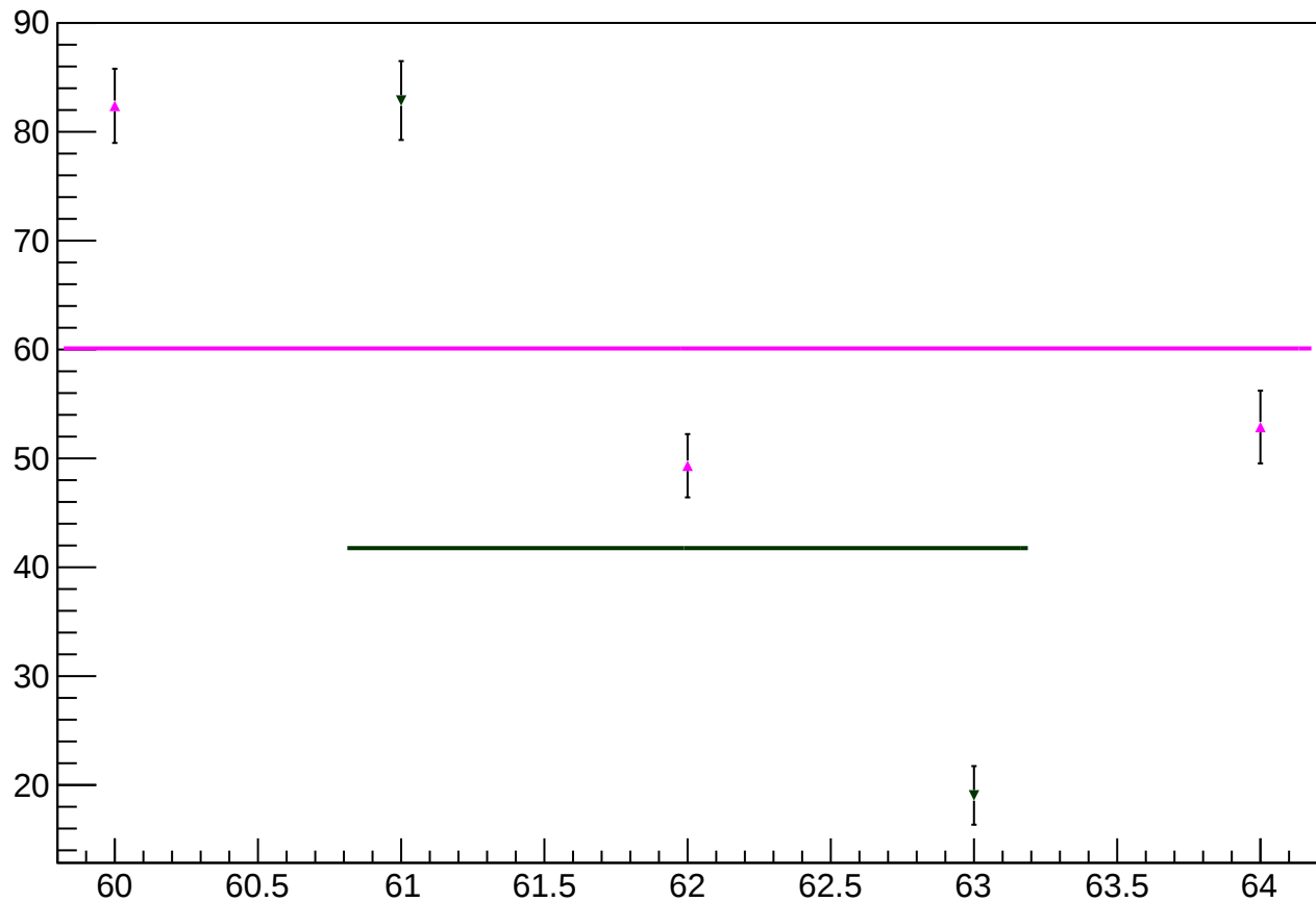
reg_asym_sam6_diff_bpm4aX_slope vs slug
