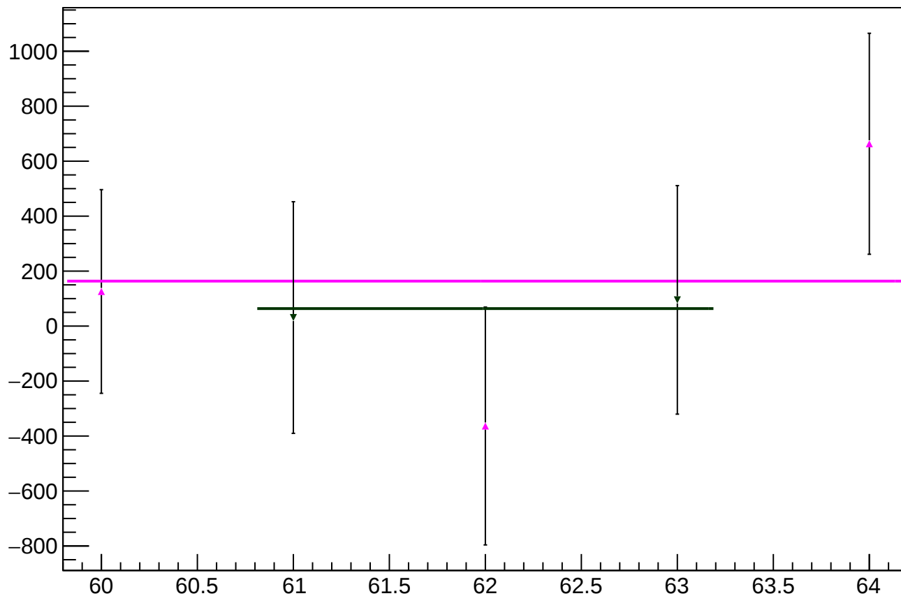
reg_asym_atr1l2_dd_mean vs slug
