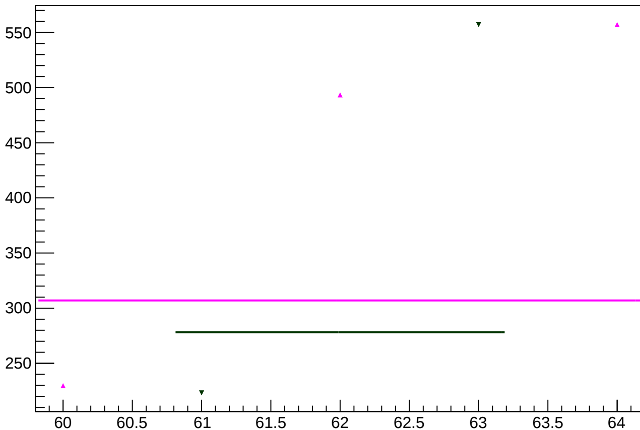
asym_atl_dd_atr_dd_avg_rms vs slug
