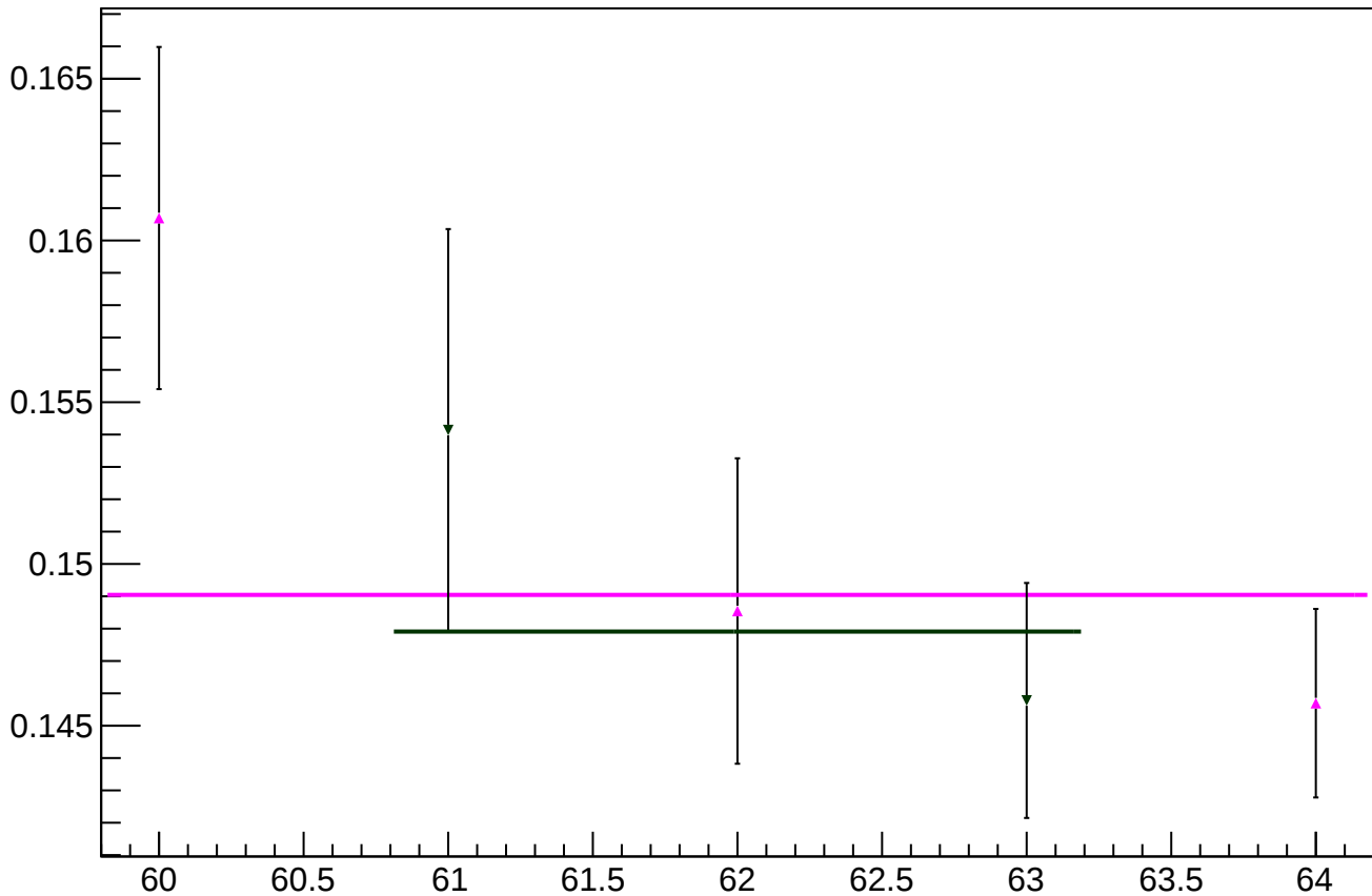
reg_bcm_cav4cQ_ds_dd_diff_bpm4eX_slope vs slug
