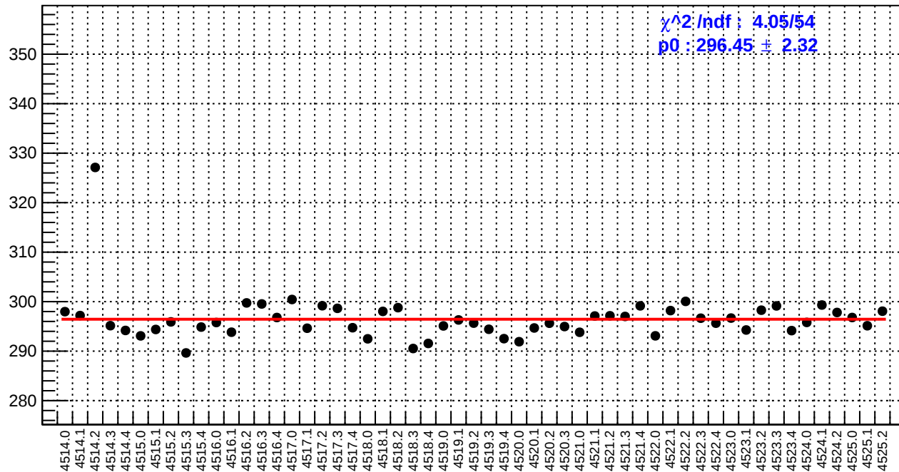
slug64: reg_asym_atr1l2_avg.rms/ppm
