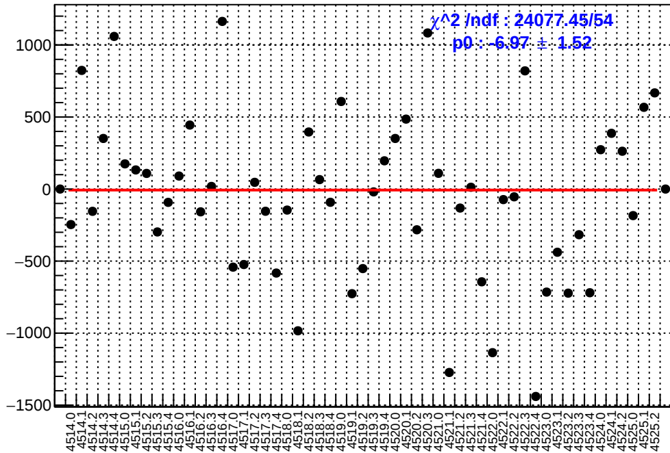
slug64: asym_right_dd.mean/ppb-reg_asym_right_dd.mean/ppb
