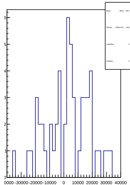
slug64: 1D Corr asym_atr2.mean/ppb-reg_asym_atr2.mean/ppb
