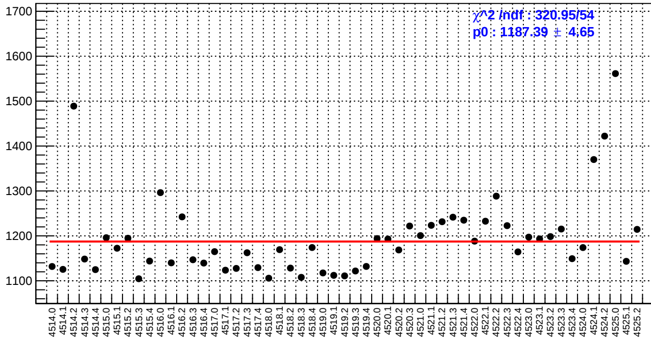
slug64: reg_asym_sam3.rms/ppm
