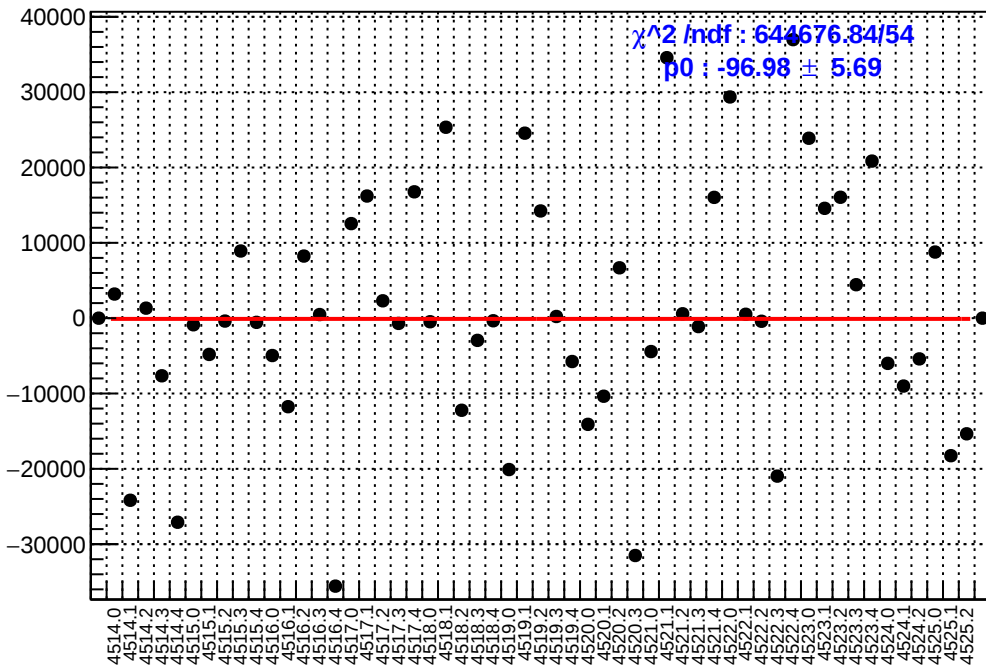
slug64: asym_atr1.mean/ppb-reg_asym_atr1.mean/ppb
