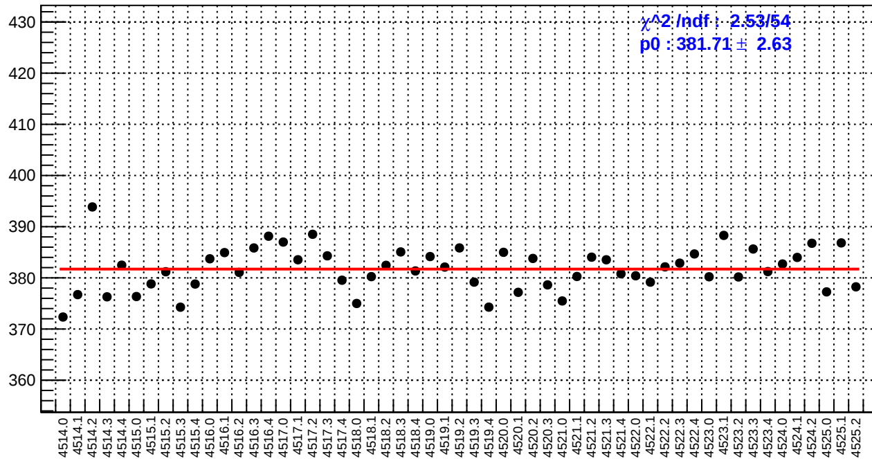
slug64: reg_asym_atl_avg.rms/ppm
