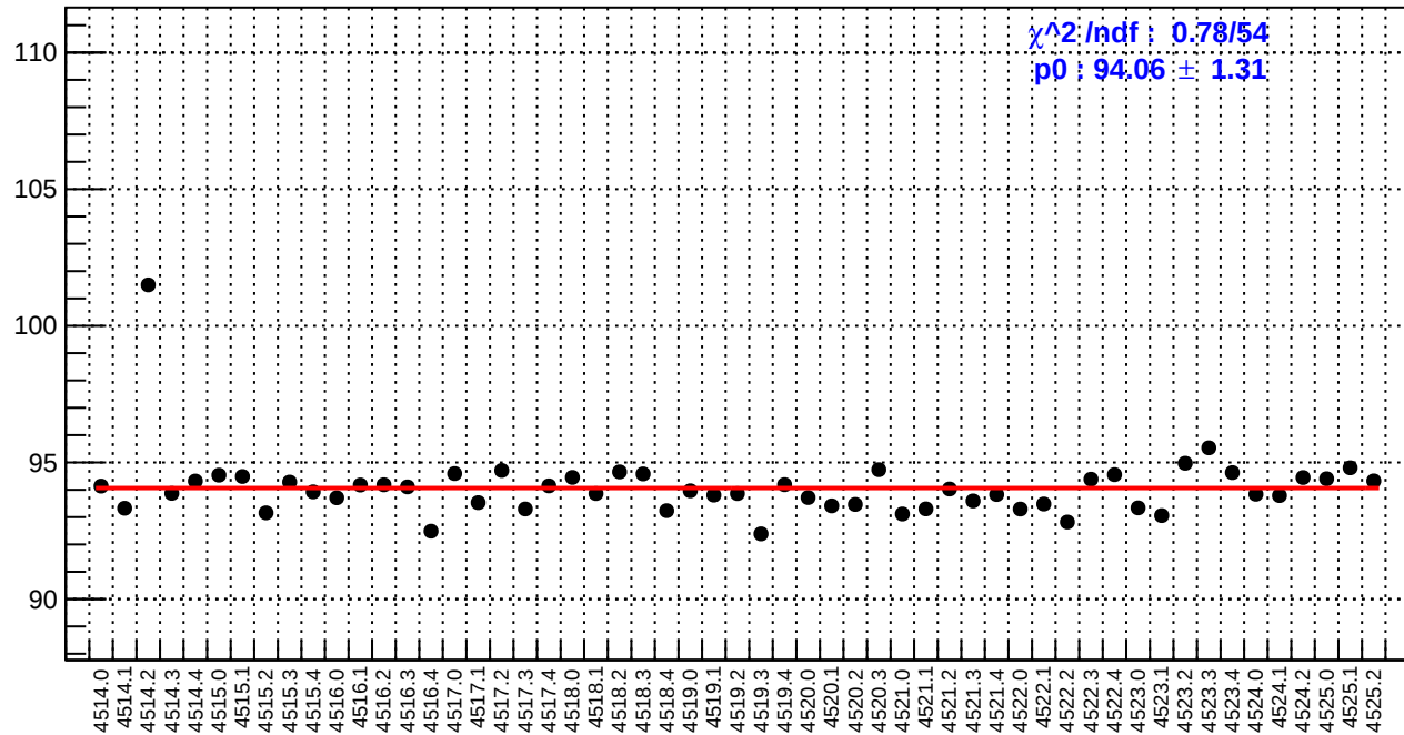
slug64: reg_asym_ds_dd.rms/ppm
