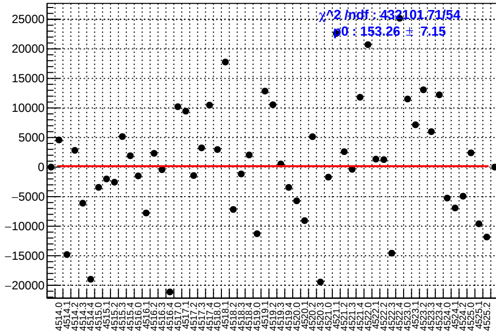
slug64: asym_dsl.mean/ppb-reg_asym_dsl.mean/ppb
