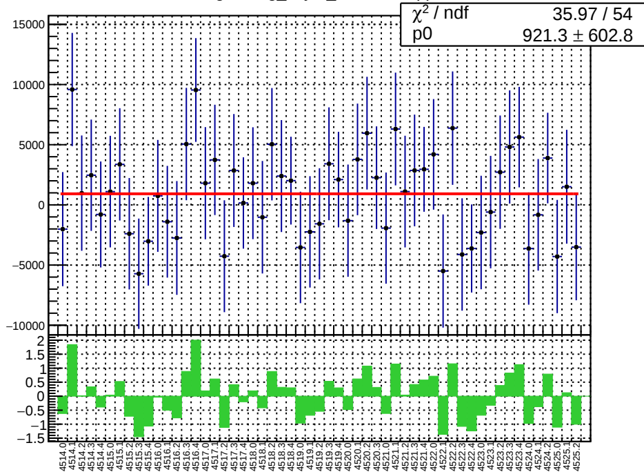
slug64: reg_asym_atr1.mean/ppb
