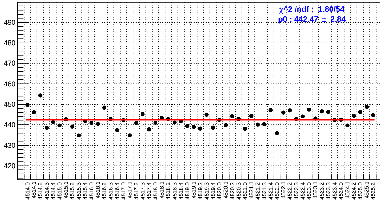
slug64: reg_asym_atr1.rms/ppm
