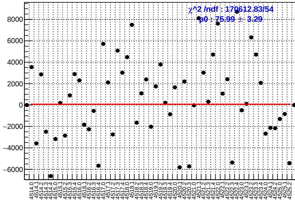
slug64: asym_ds_avg.mean/ppb-reg_asym_ds_avg.mean/ppb
