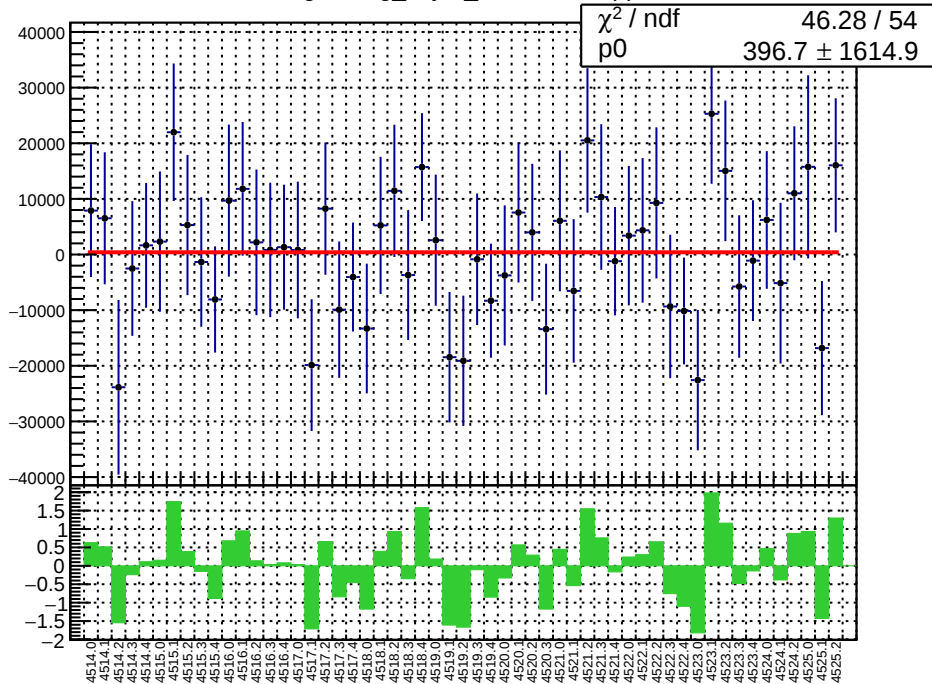
slug64: reg_asym_sam3.mean/ppb
