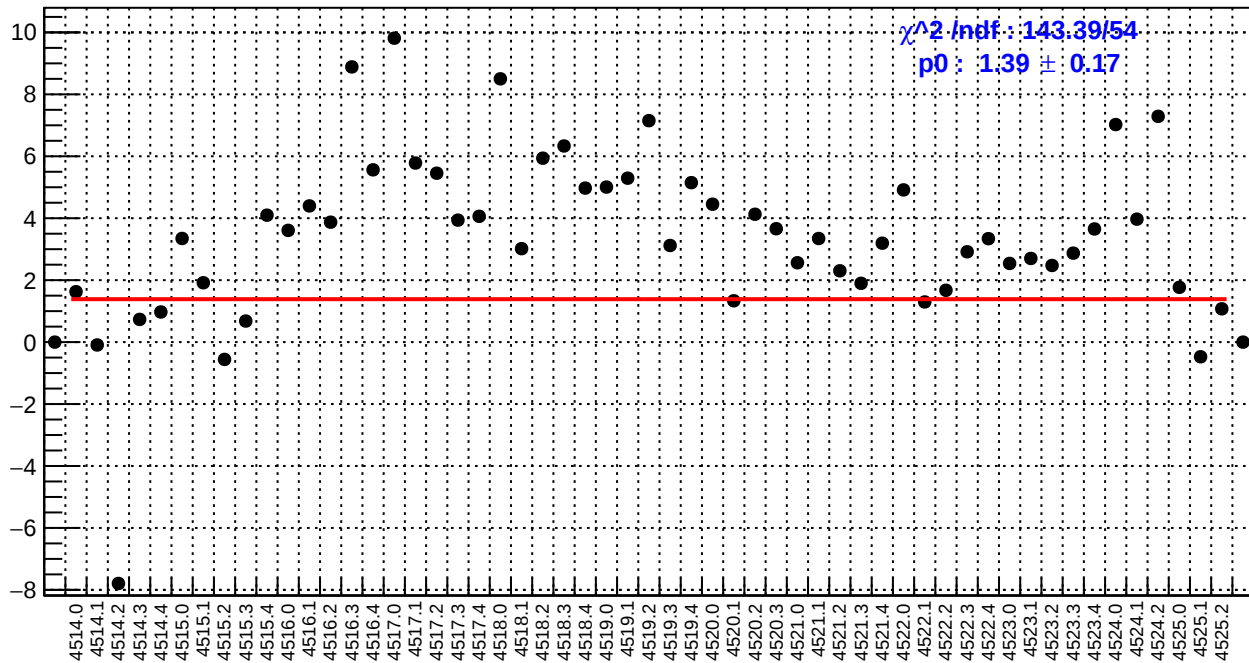
slug64: us_avg_bpm4eY/(ppb/nm)
