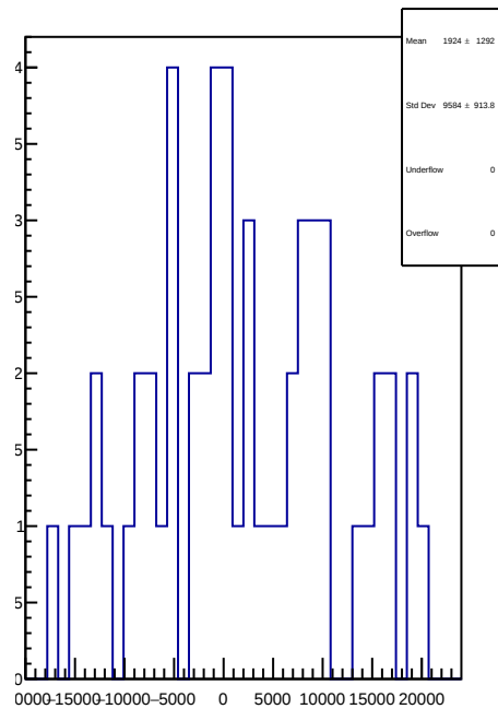
slug64: 1D Corr asym_atr_avg.mean/ppb-reg_asym_atr_avg.mean/ppb
