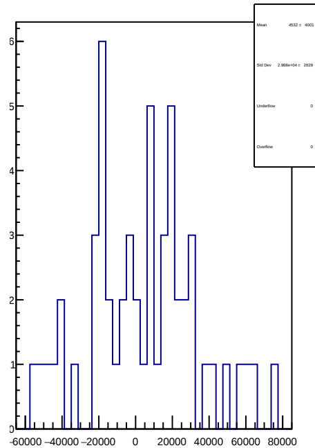
slug64: 1D Corr asym_atl2.mean/ppb-reg_asym_atl2.mean/ppb
