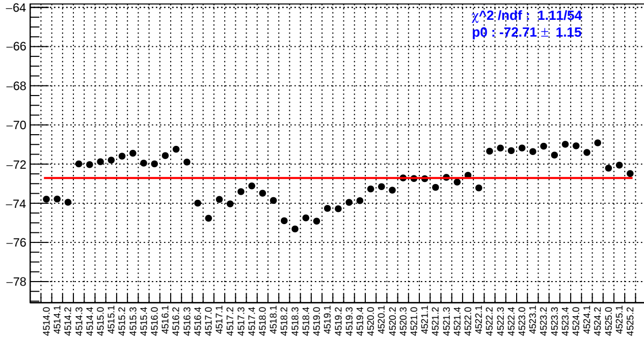
slug64: left_avg_bpm4eX/(ppb/nm)
