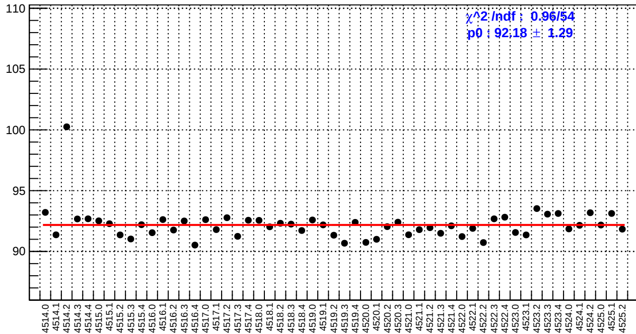
slug64: reg_asym_us_dd.rms/ppm
