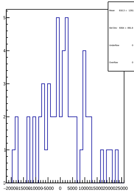
slug64: 1D Corr asym_usl.mean/ppb-reg_asym_usl.mean/ppb
