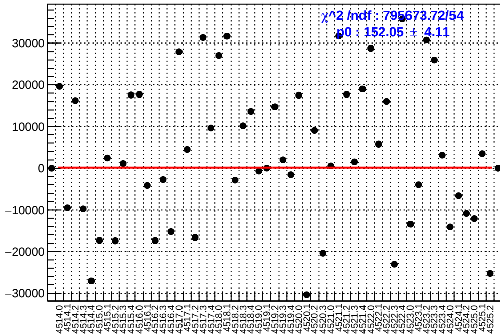
slug64: asym_atl_avg.mean/ppb-reg_asym_atl_avg.mean/ppb
