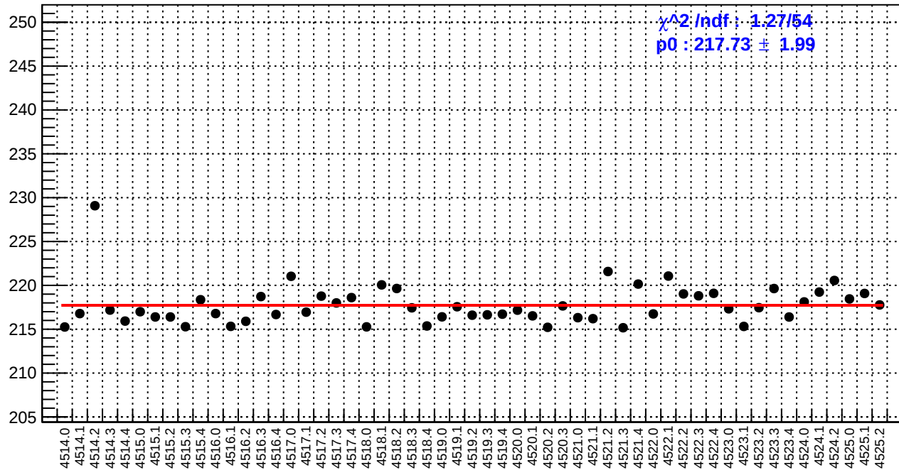
slug64: reg_asym_at2_dd.rms/ppm
