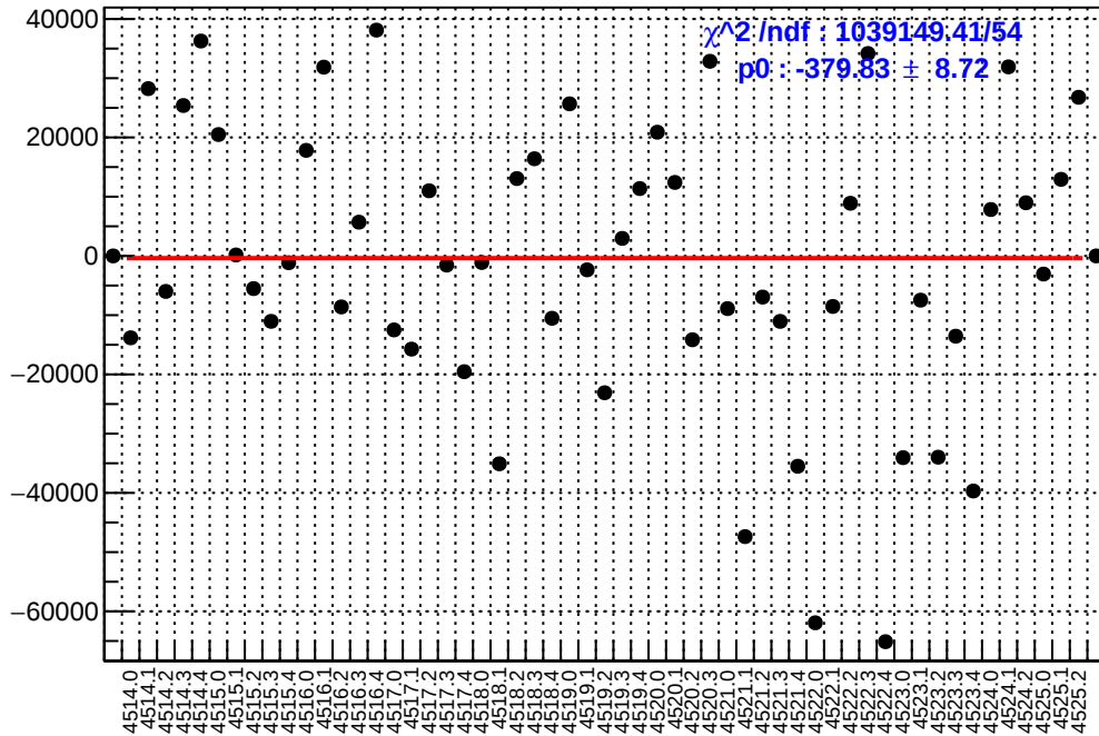
slug64: asym_sam8.mean/ppb-reg_asym_sam8.mean/ppb
