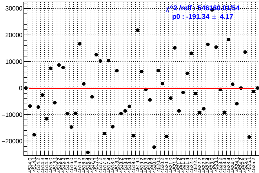
slug64: asym_atr_dd.mean/ppb-reg_asym_atr_dd.mean/ppb
