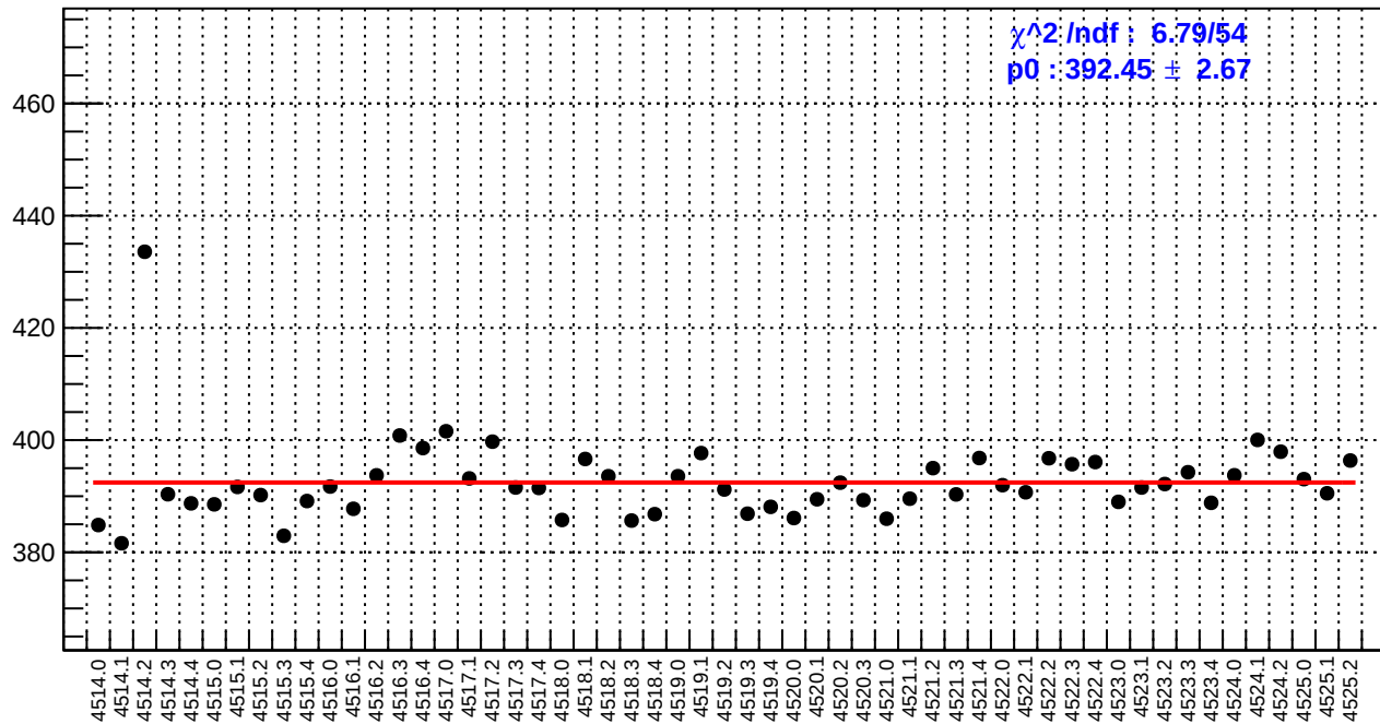
slug64: reg_asym_atl2.rms/ppm
