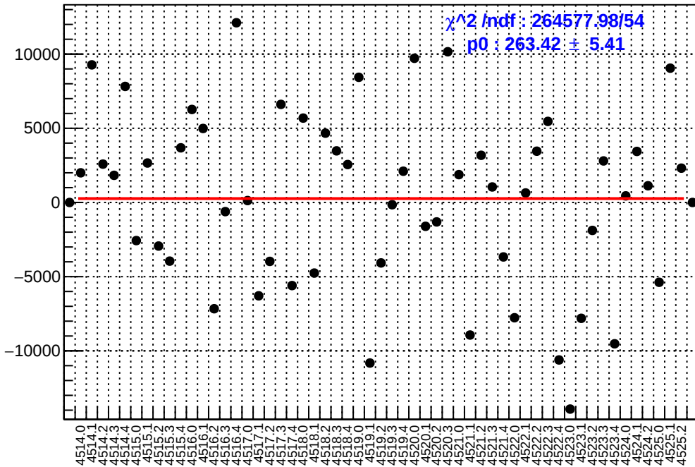
slug64: asym_usr.mean/ppb-reg_asym_usr.mean/ppb
