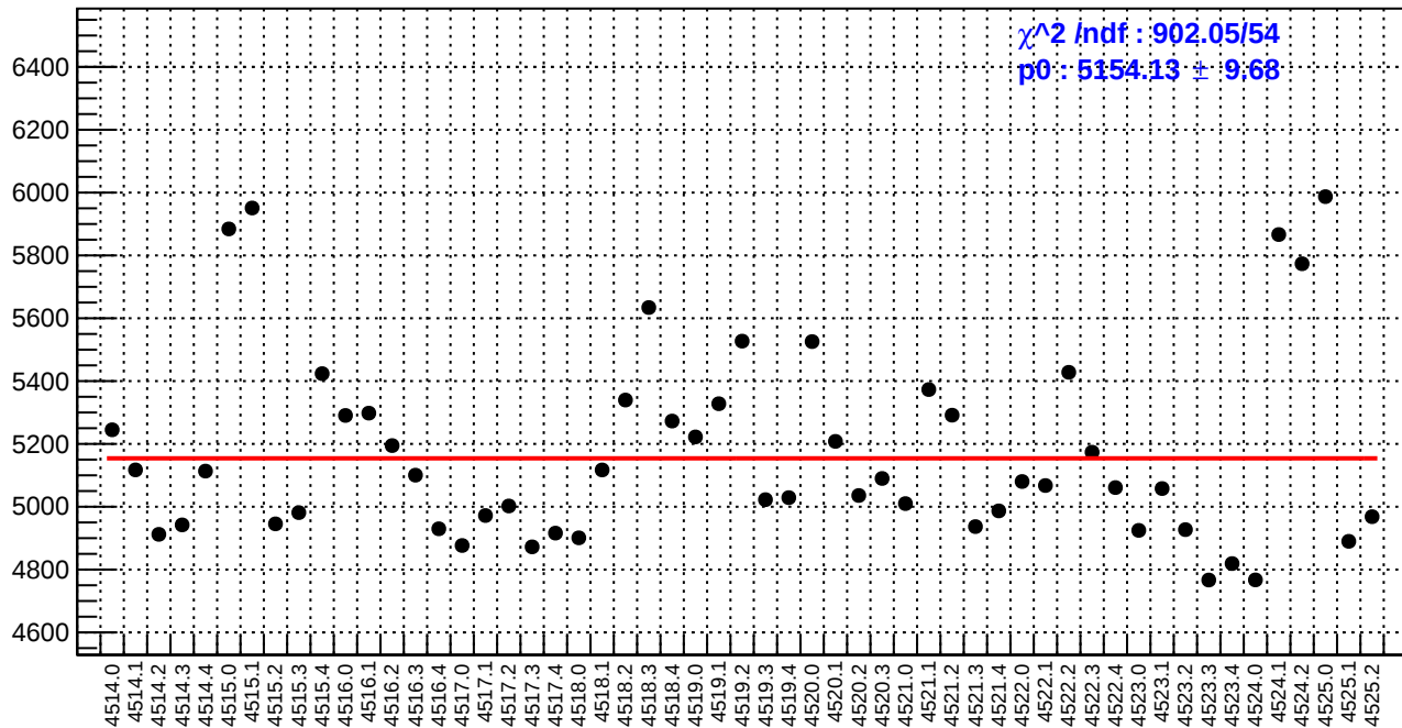
slug64: diff_bpm11X.rms/nm
