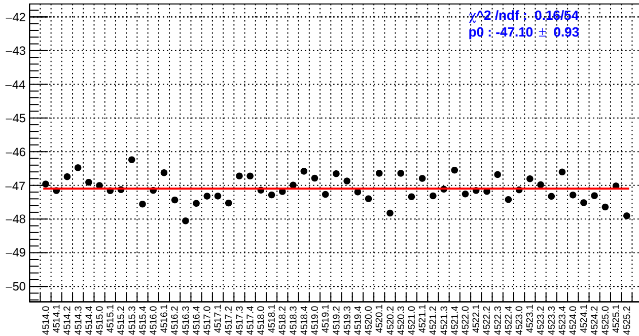
slug64: left_avg_bpm12X/(ppb/nm)
