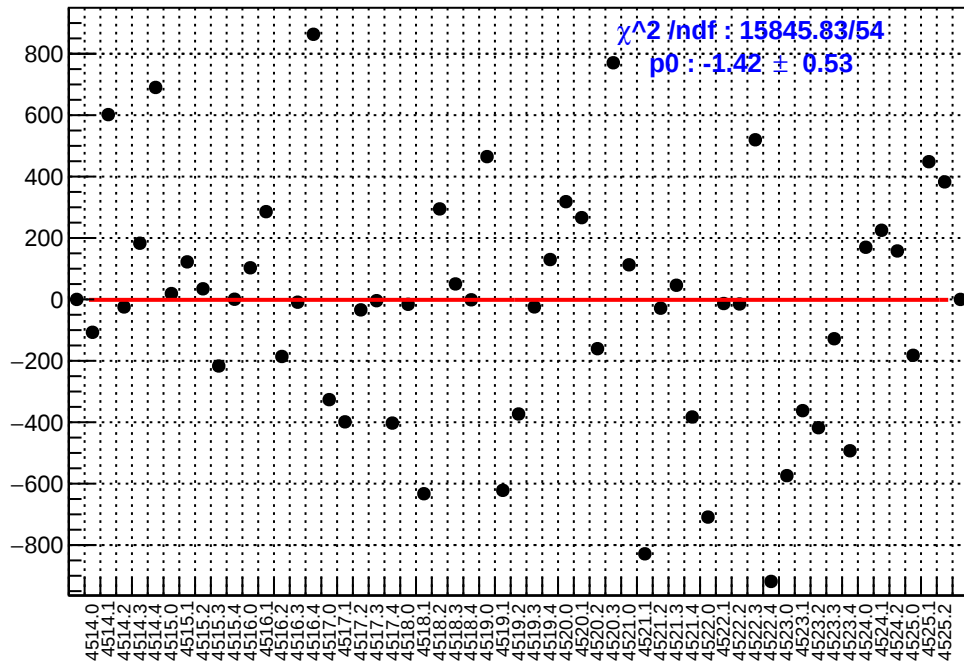
slug64: asym_left_dd.mean/ppb-reg_asym_left_dd.mean/ppb
