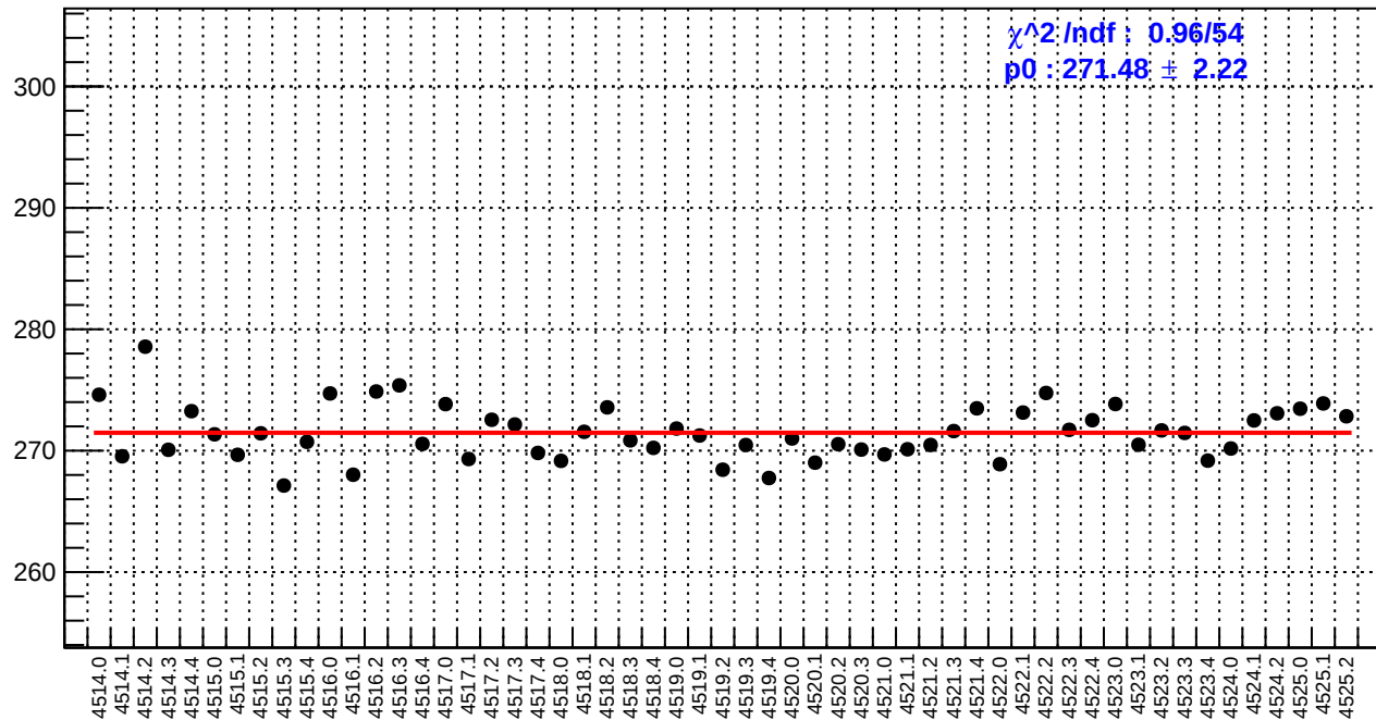
slug64: reg_asym_atr_avg.rms/ppm
