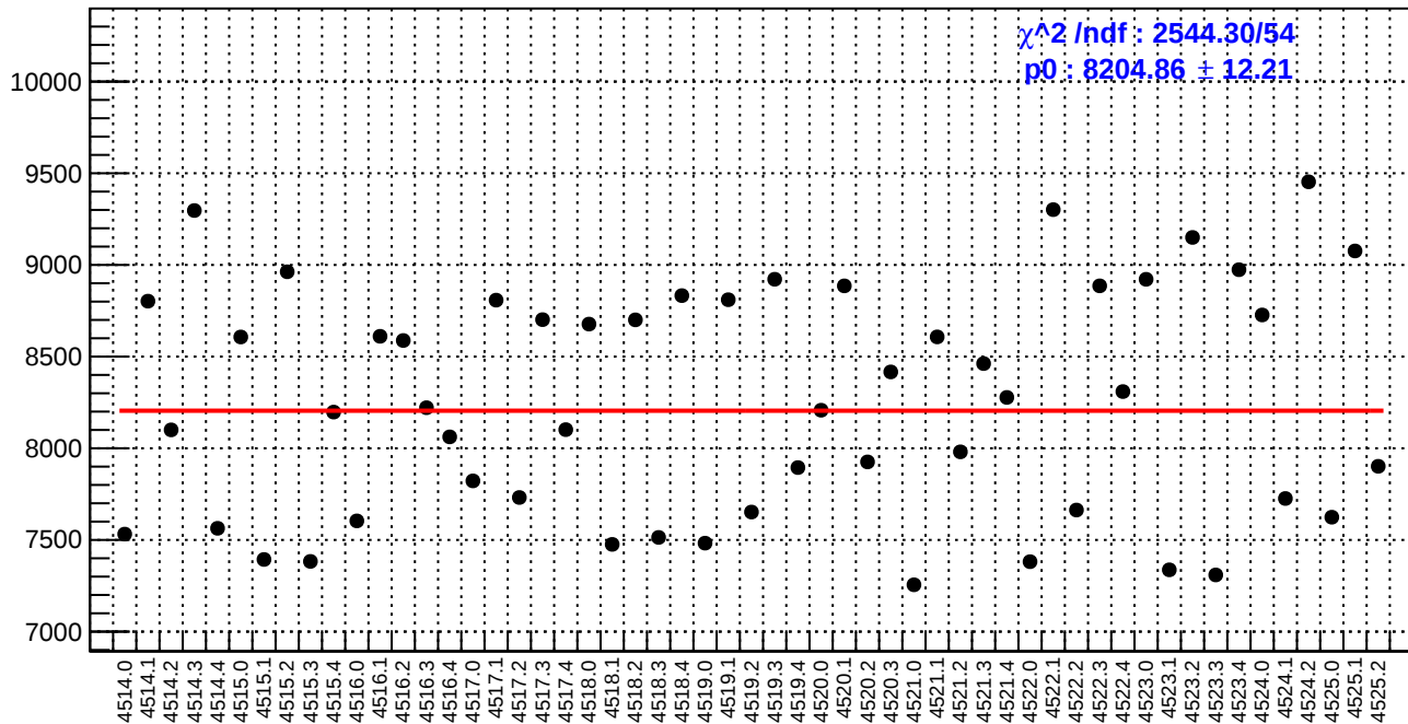
slug64: diff_bpm4aY.rms/nm
