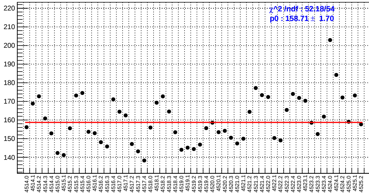
slug64: asym_bcm_an_ds.rms/ppm
