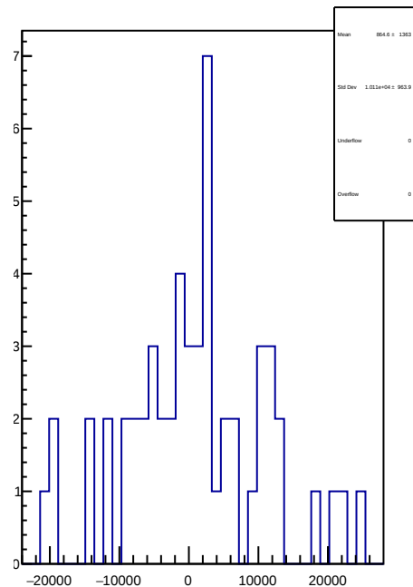
slug64: 1D Corr asym_dsl.mean/ppb-reg_asym_dsl.mean/ppb
