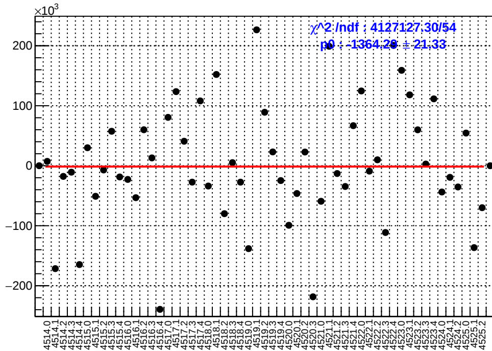
slug64: asym_sam2.mean/ppb-reg_asym_sam2.mean/ppb
