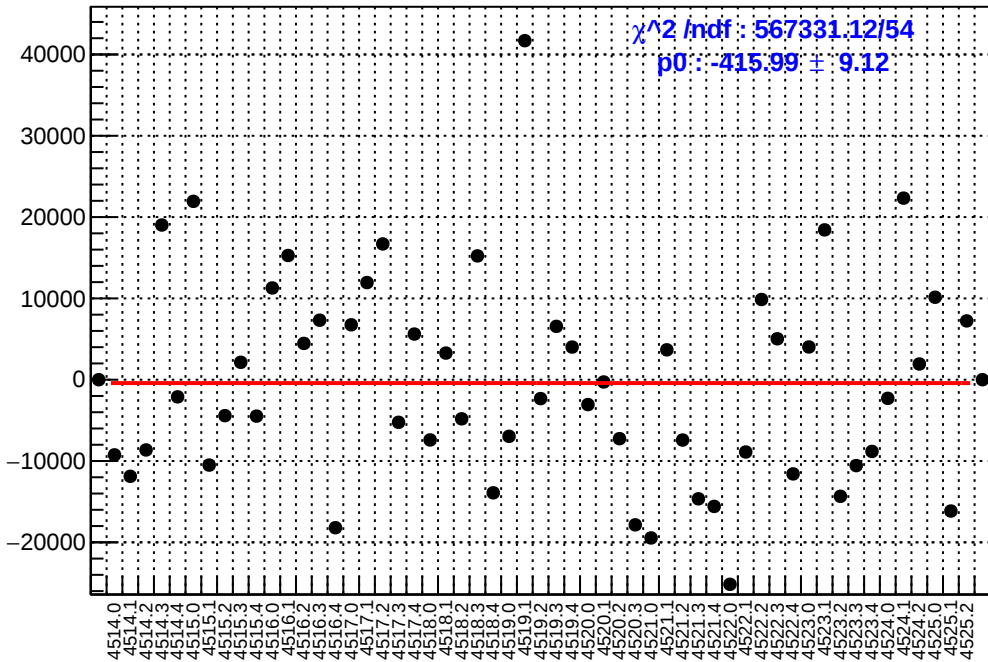
slug64: asym_sam1.mean/ppb-reg_asym_sam1.mean/ppb
