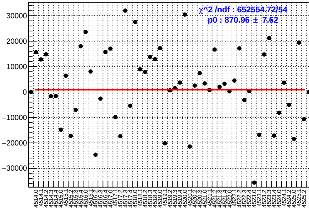
slug64: asym_atl1r2_avg.mean/ppb-reg_asym_atl1r2_avg.mean/ppb
