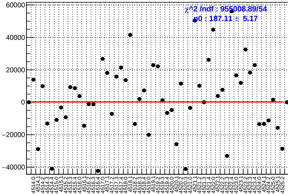
slug64: asym_atr1l2_avg.mean/ppb-reg_asym_atr1l2_avg.mean/ppb
