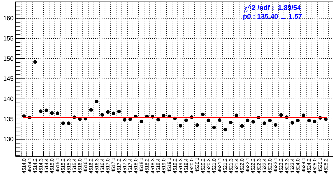
slug64: reg_asym_left_avg.rms/ppm
