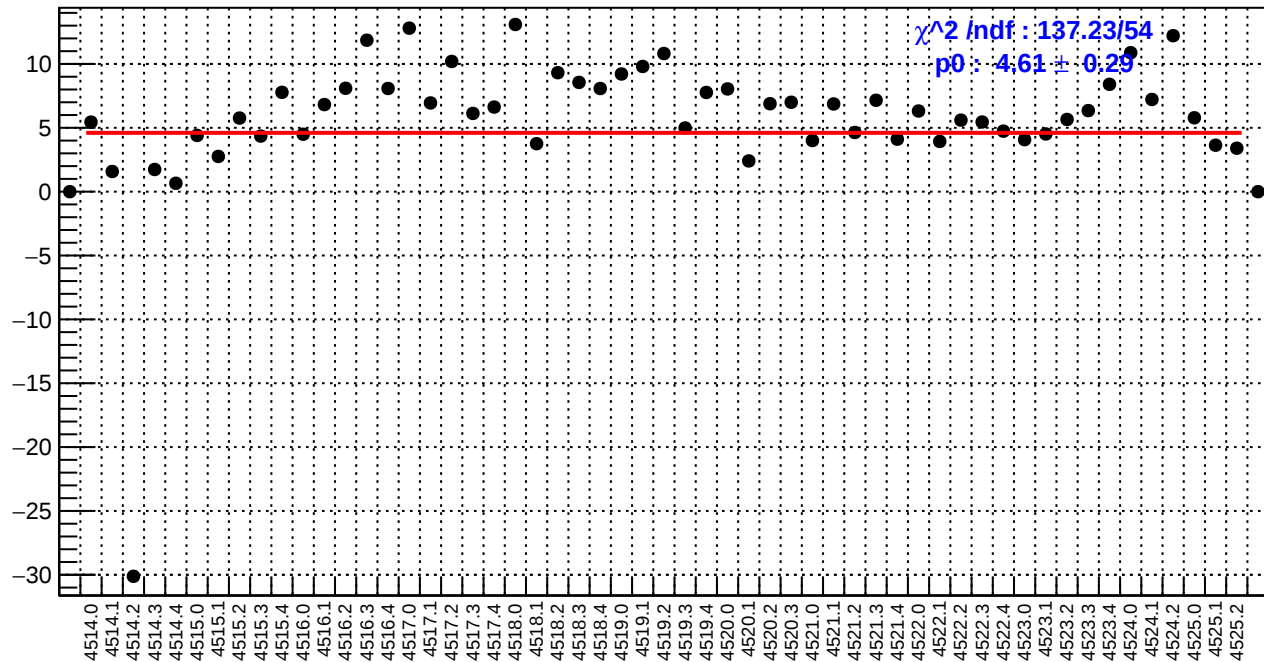
slug64: dsl_bpm4eY/(ppb/nm)
