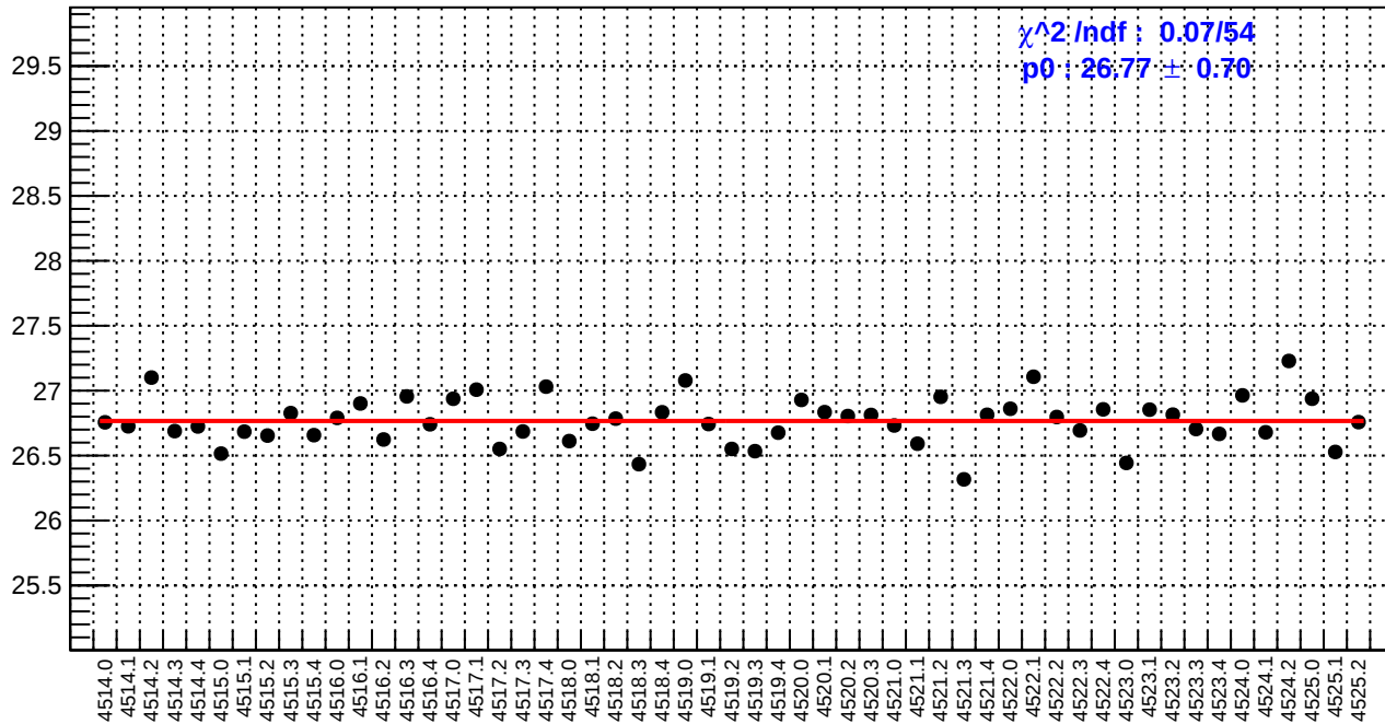
slug64: reg_asym_right_dd.rms/ppm
