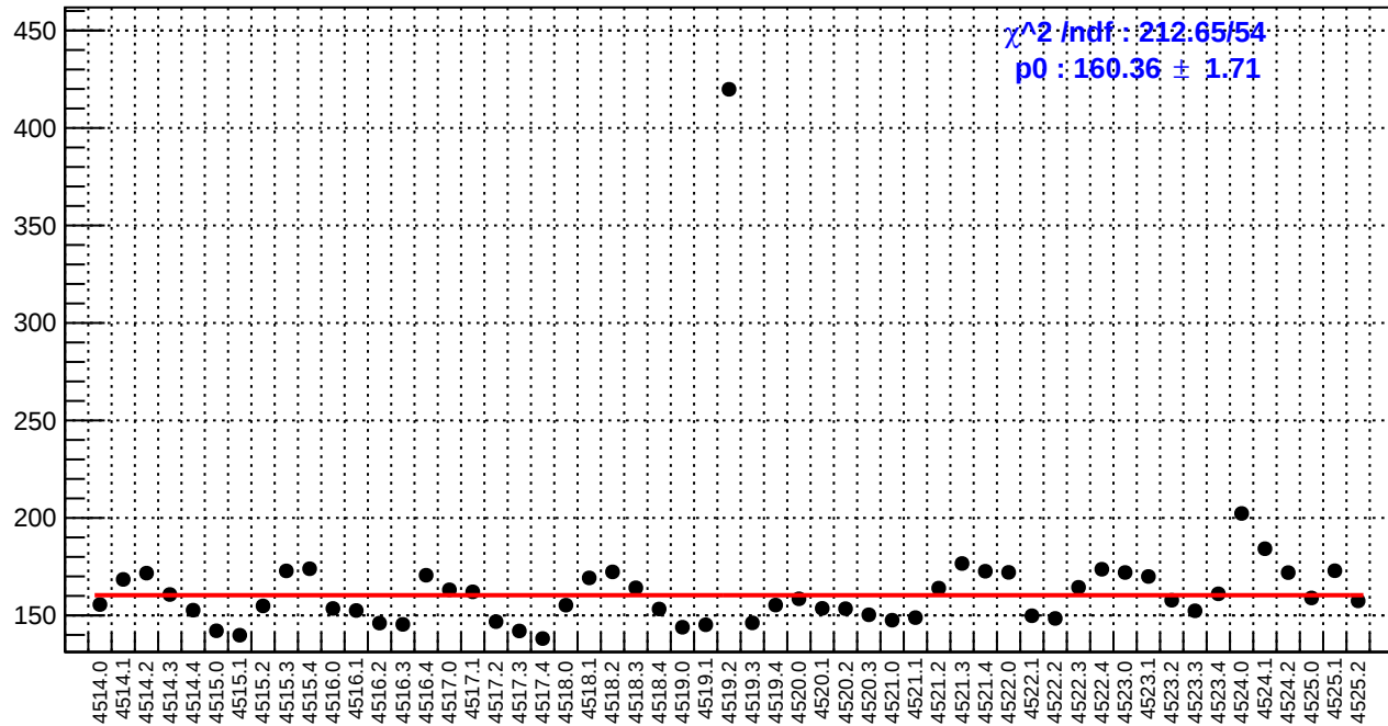
slug64: asym_bcm_an_us.rms/ppm
