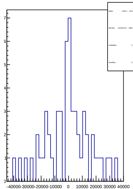
slug64: 1D Corr asym_atl_dd.mean/ppb-reg_asym_atl_dd.mean/ppb
