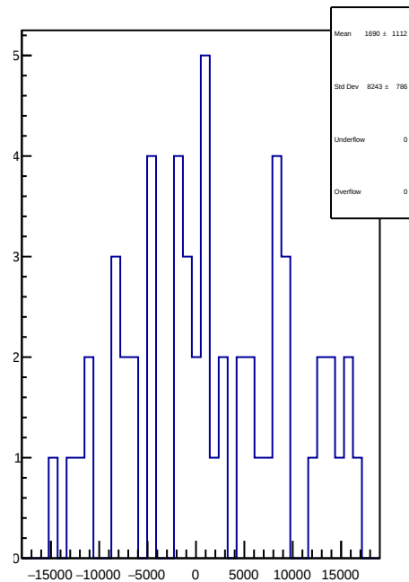
slug64: 1D Corr asym_at1_avg.mean/ppb-reg_asym_at1_avg.mean/ppb
