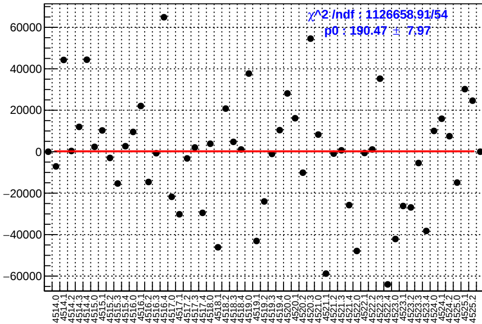
slug64: asym_sam7.mean/ppb-reg_asym_sam7.mean/ppb
