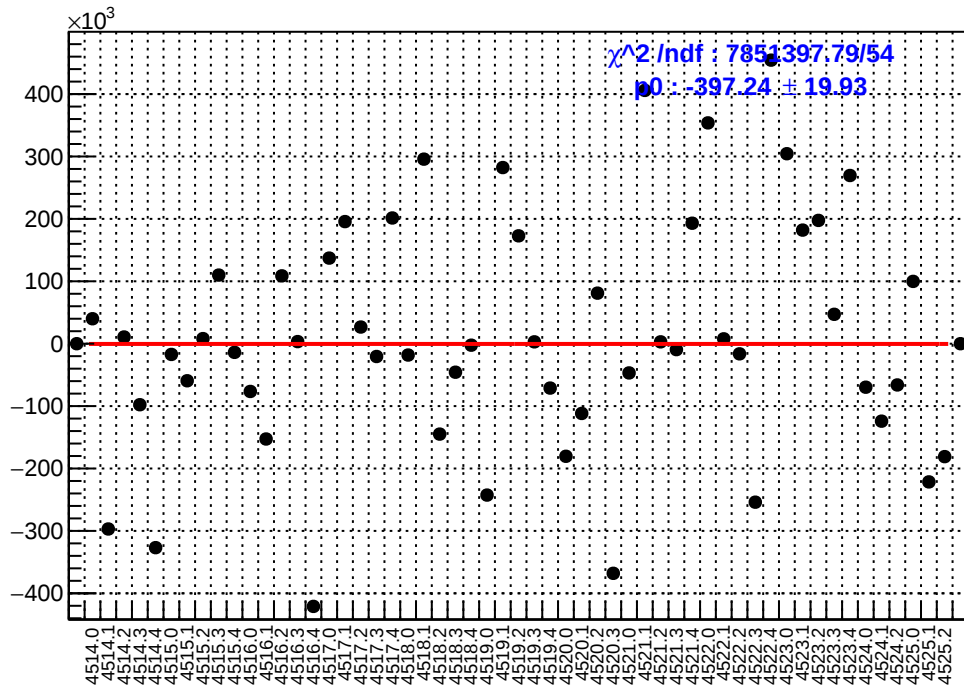
slug64: asym_sam3.mean/ppb-reg_asym_sam3.mean/ppb
