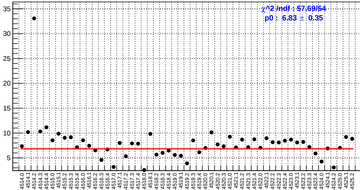
slug64: left_avg_bpm4aY/(ppb/nm)
