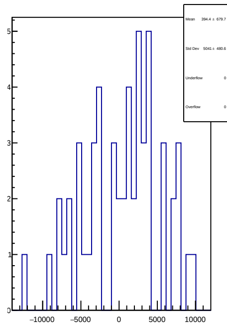
slug64: 1D Corr asym_dsr.mean/ppb-reg_asym_dsr.mean/ppb
