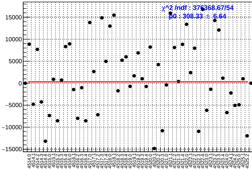
slug64: asym_at1_avg.mean/ppb-reg_asym_at1_avg.mean/ppb
