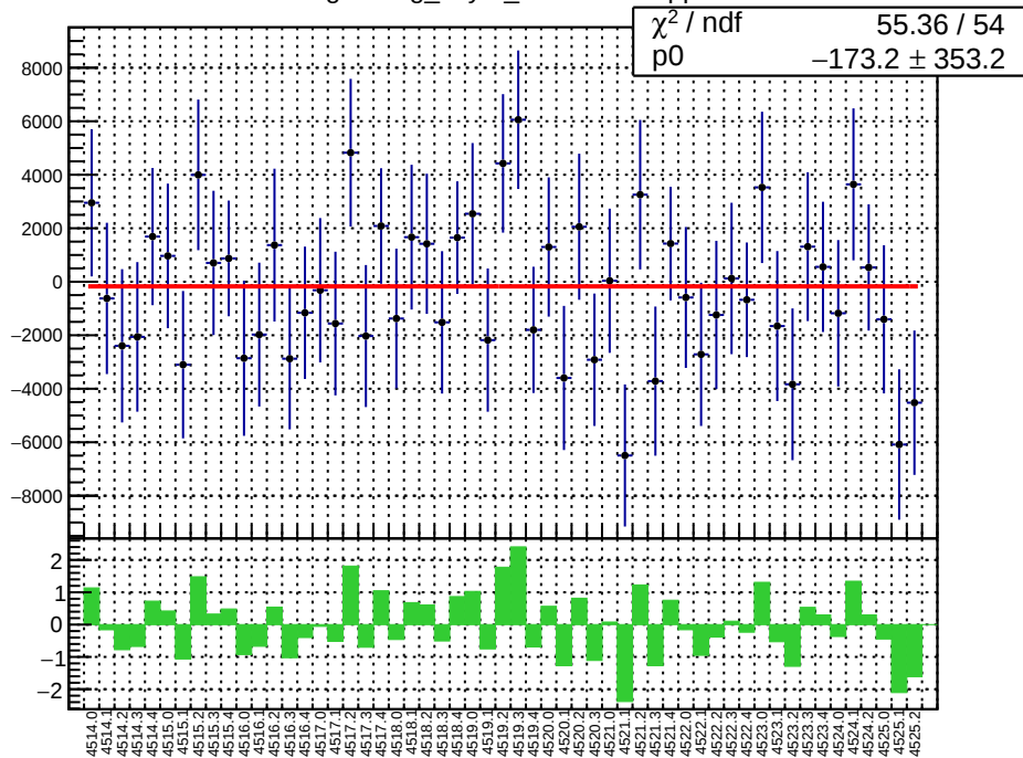
slug64: reg_asym_sam1.mean/ppb
