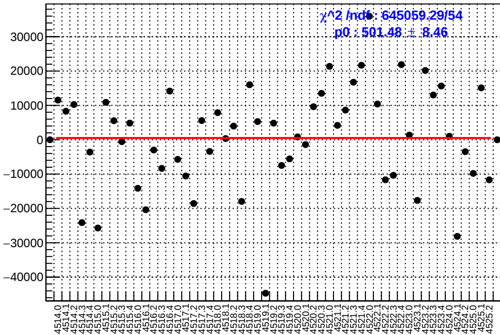
slug64: asym_sam5.mean/ppb-reg_asym_sam5.mean/ppb
