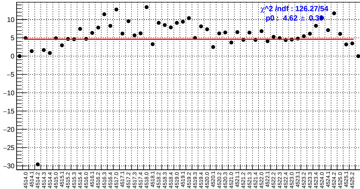
slug64: left_avg_bpm4eY/(ppb/nm)
