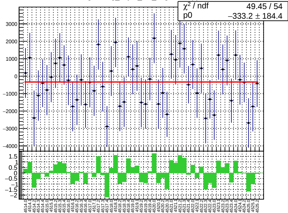
slug64: reg_asym_left_avg.mean/ppb
