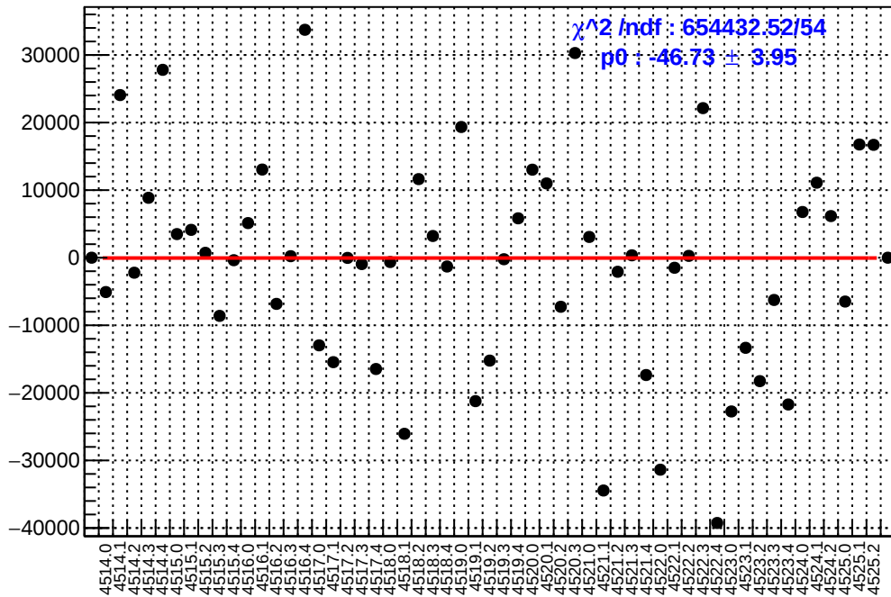
slug64: asym_atl_dd.mean/ppb-reg_asym_atl_dd.mean/ppb
