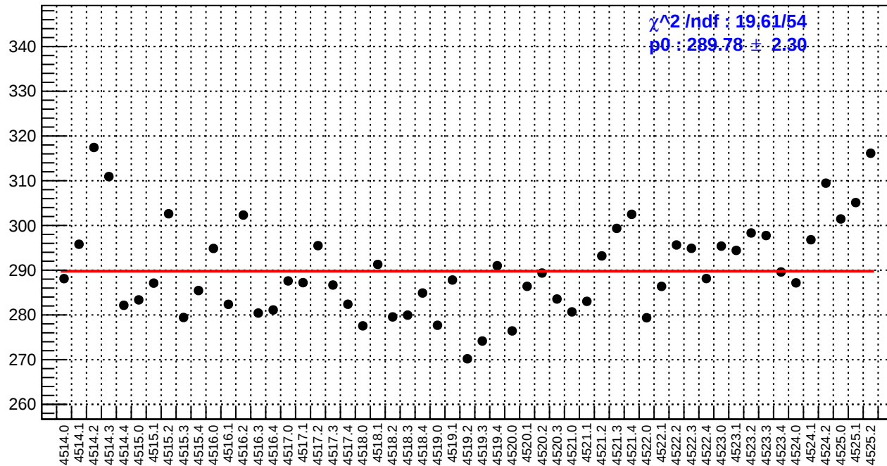
slug64: reg_asym_sam5.rms/ppm
