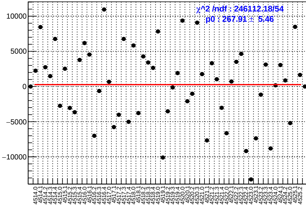
slug64: asym_right_avg.mean/ppb-reg_asym_right_avg.mean/ppb
