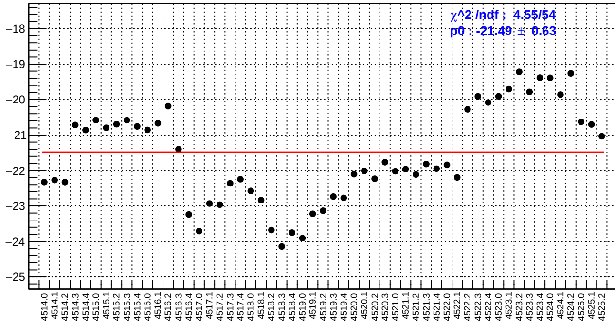
slug64: us_avg_bpm4eX/(ppb/nm)
