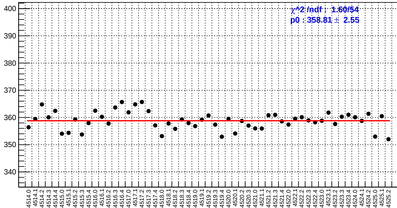
slug64: reg_asym_atl1r2_avg.rms/ppm
