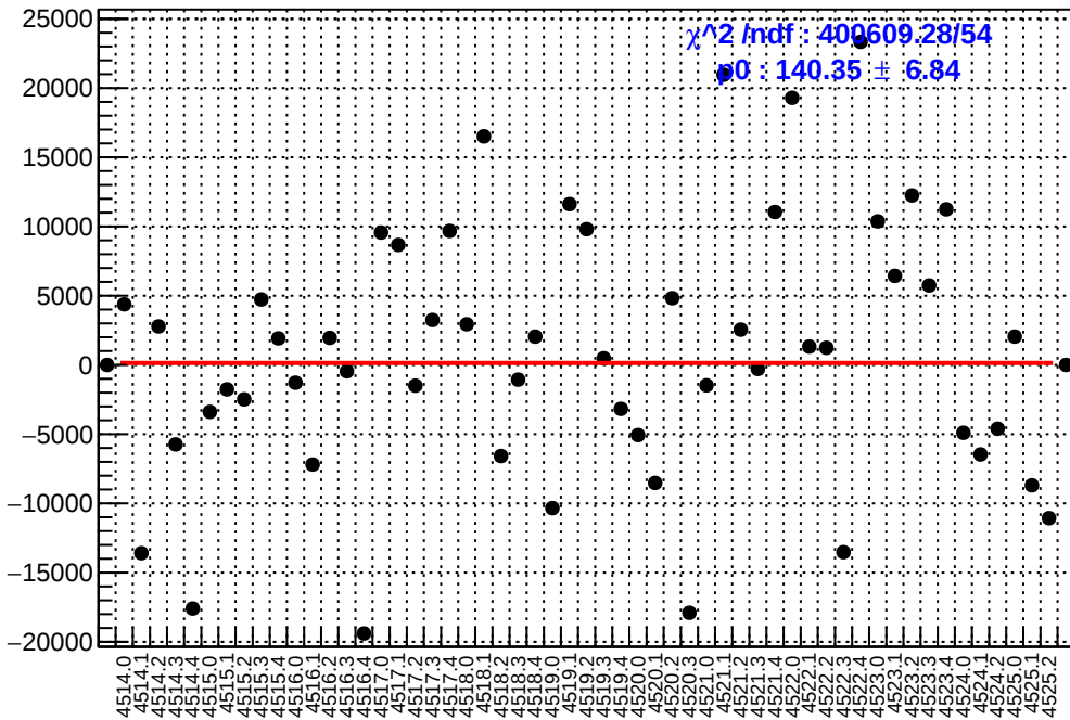
slug64: asym_usl.mean/ppb-reg_asym_usl.mean/ppb
