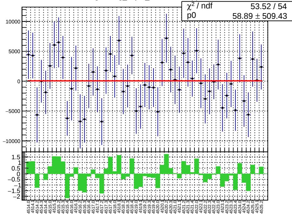
slug64: reg_asym_sam7.mean/ppb
