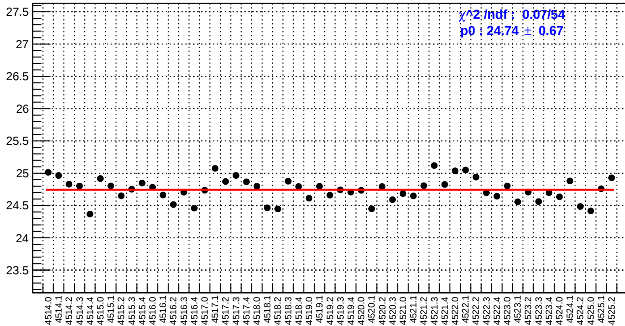
slug64: reg_asym_left_dd.rms/ppm
