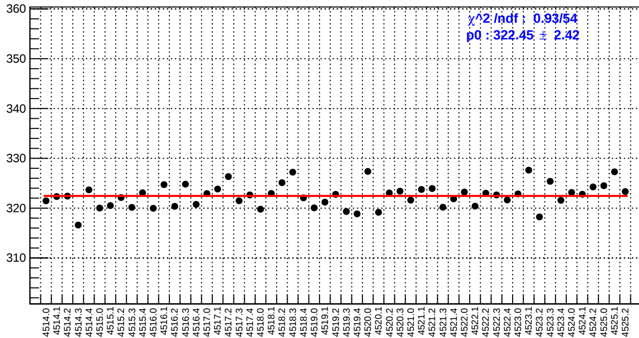
slug64: reg_asym_atl1r2_dd.rms/ppm
