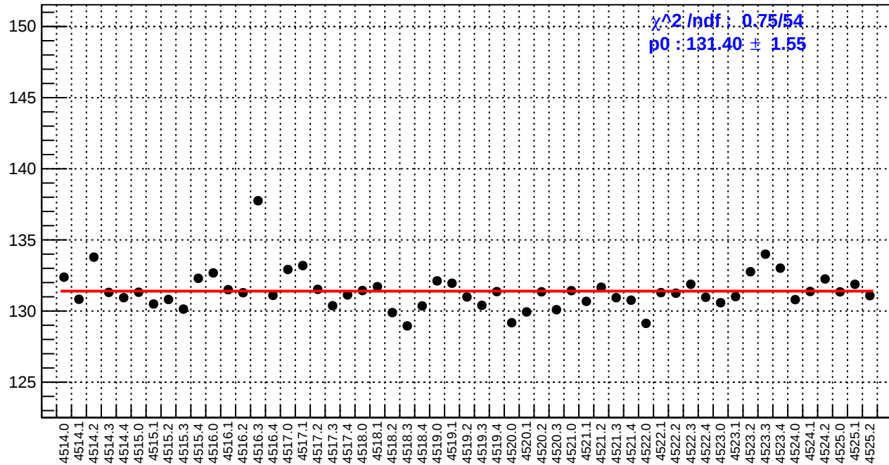
slug64: reg_asym_usr.rms/ppm
