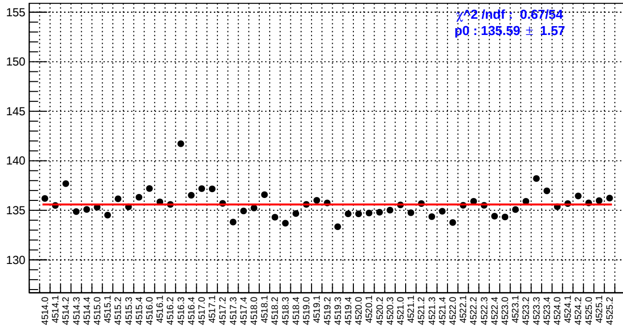
slug64: reg_asym_dsr.rms/ppm
