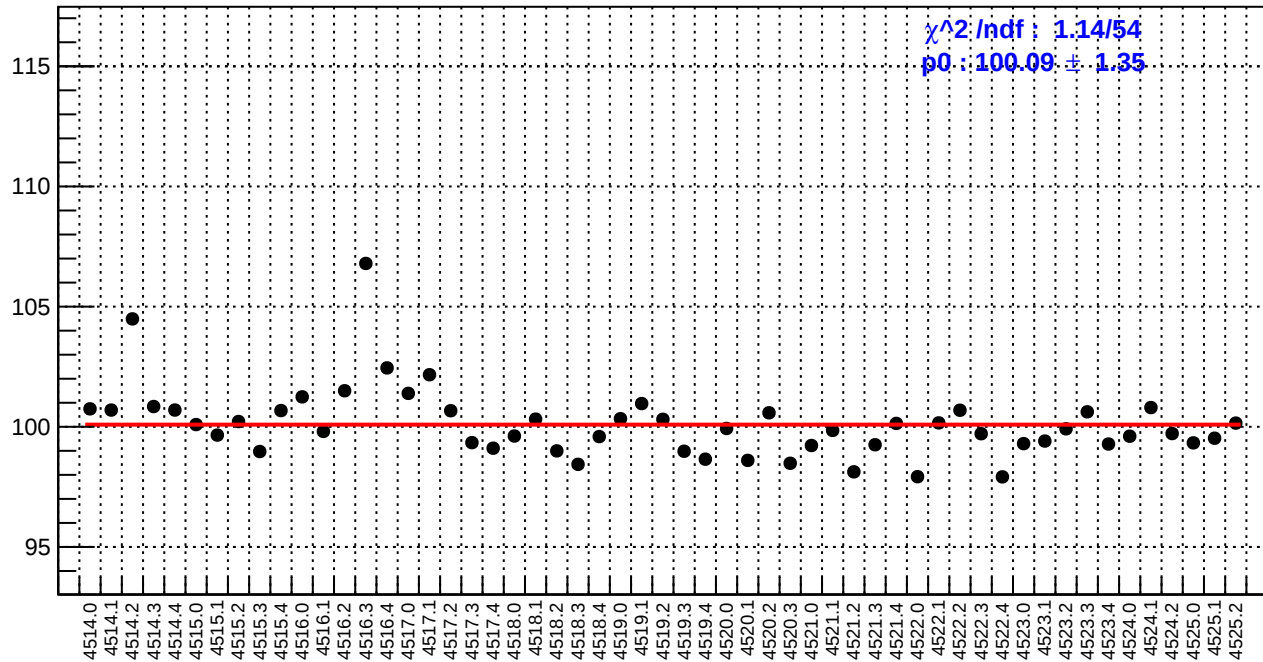
slug64: reg_asym_ds_avg.rms/ppm
