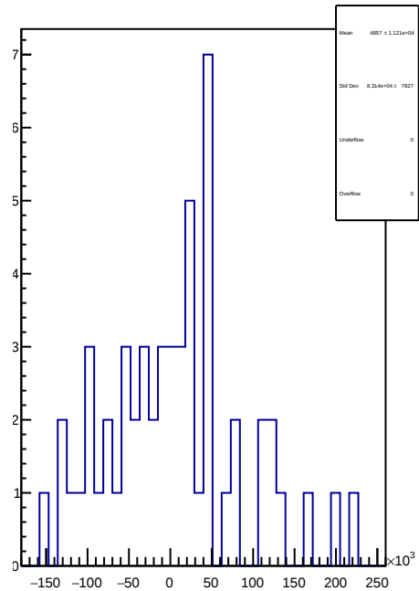
slug64: 1D Corr asym_sam4.mean/ppb-reg_asym_sam4.mean/ppb
