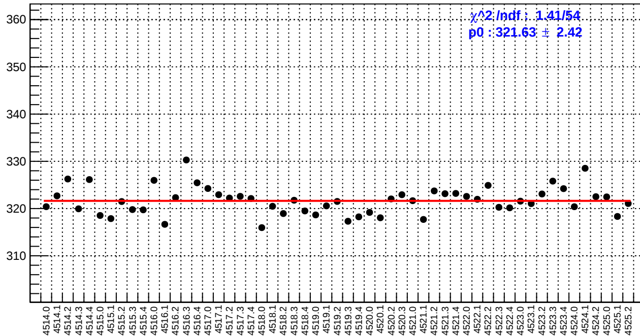
slug64: reg_asym_atr2.rms/ppm
