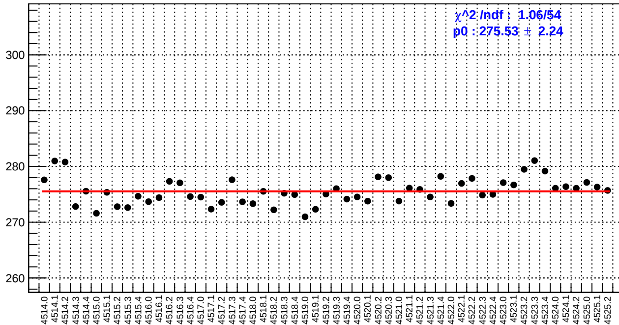
slug64: reg_asym_atr_dd.rms/ppm
