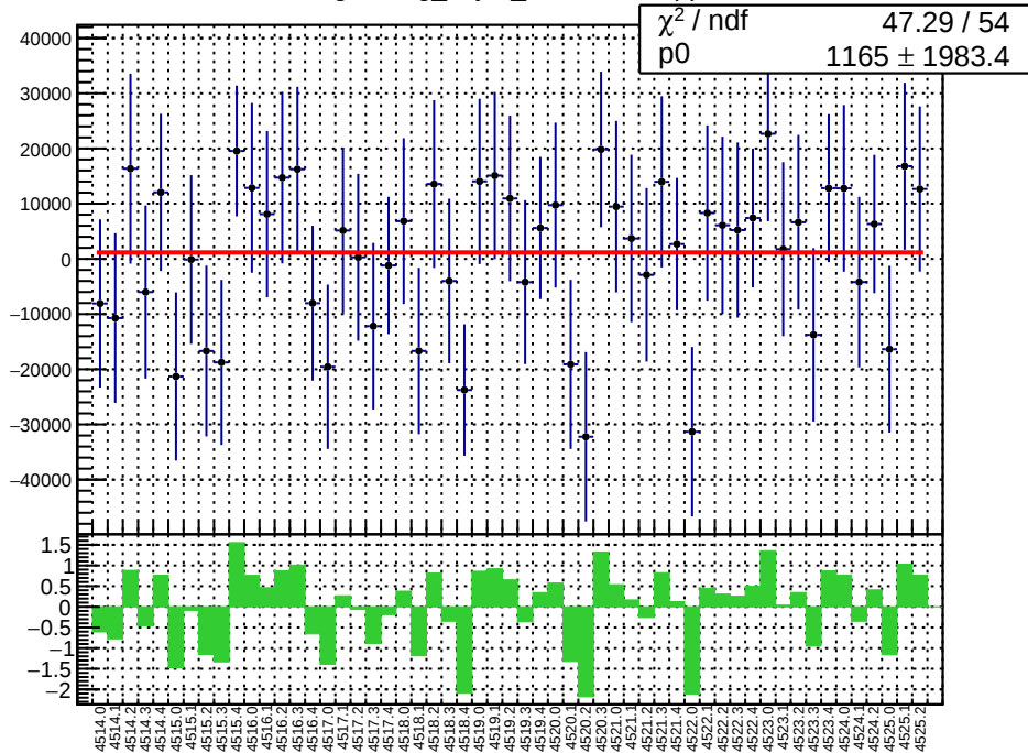
slug64: reg_asym_sam4.mean/ppb
