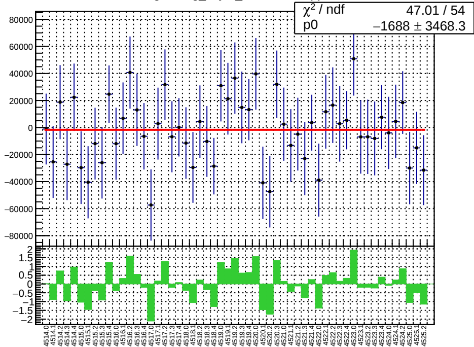
slug64: reg_asym_sam2.mean/ppb
