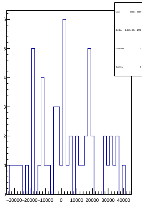
slug64: 1D Corr asym_at2_avg.mean/ppb-reg_asym_at2_avg.mean/ppb
