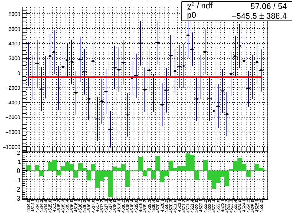
slug64: reg_asym_at2_avg.mean/ppb
