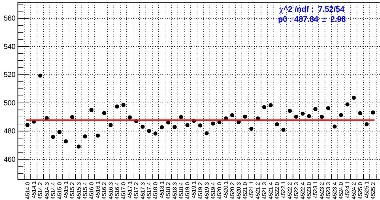
slug64: reg_asym_sam8.rms/ppm
