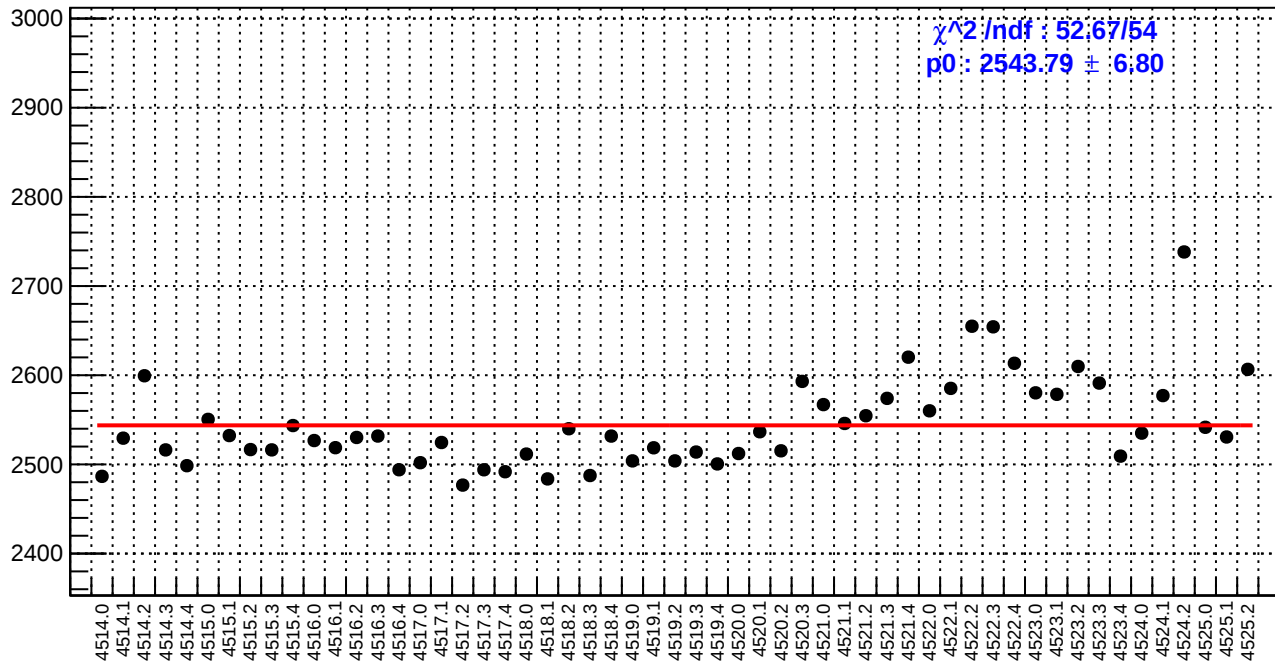
slug64: reg_asym_sam2.rms/ppm
