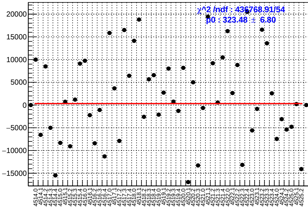
slug64: asym_atr_avg.mean/ppb-reg_asym_atr_avg.mean/ppb
