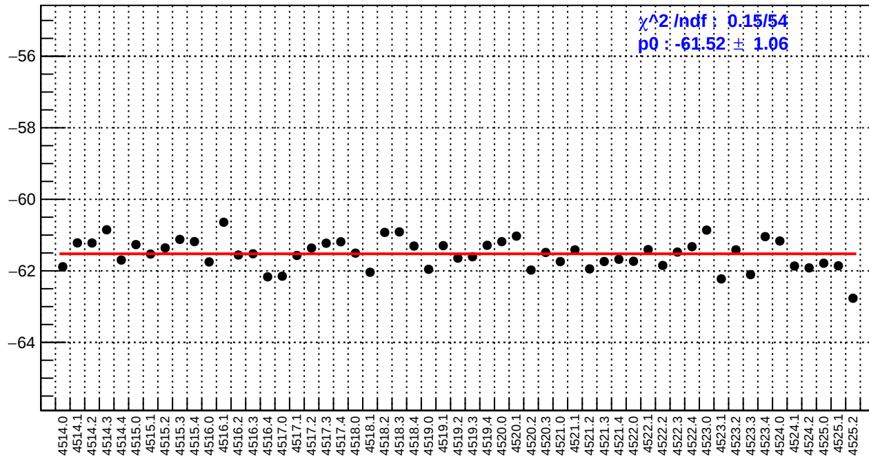
slug64: right_avg_bpm12X/(ppb/nm)
