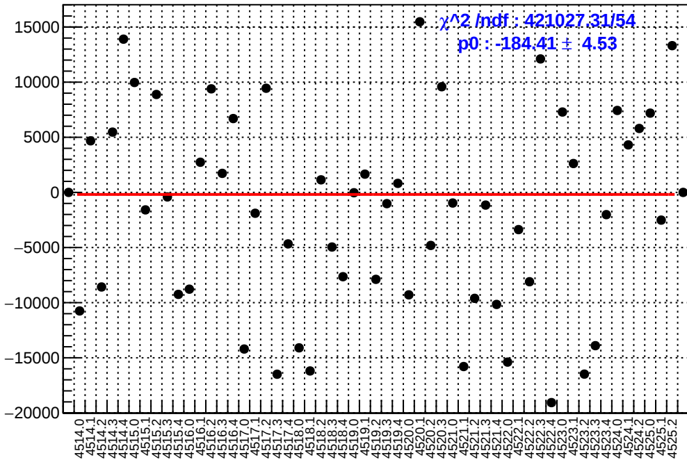
slug64: asym_atr1l2_dd.mean/ppb-reg_asym_atr1l2_dd.mean/ppb
