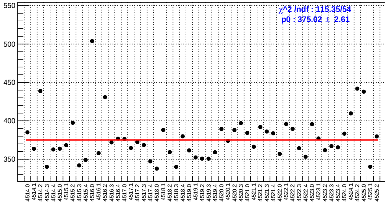
slug64: reg_asym_sam7.rms/ppm
