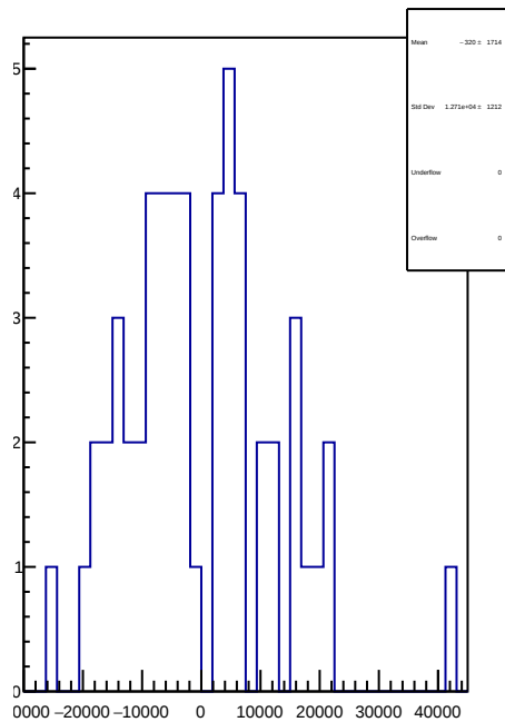
slug64: 1D Corr asym_sam1.mean/ppb-reg_asym_sam1.mean/ppb
