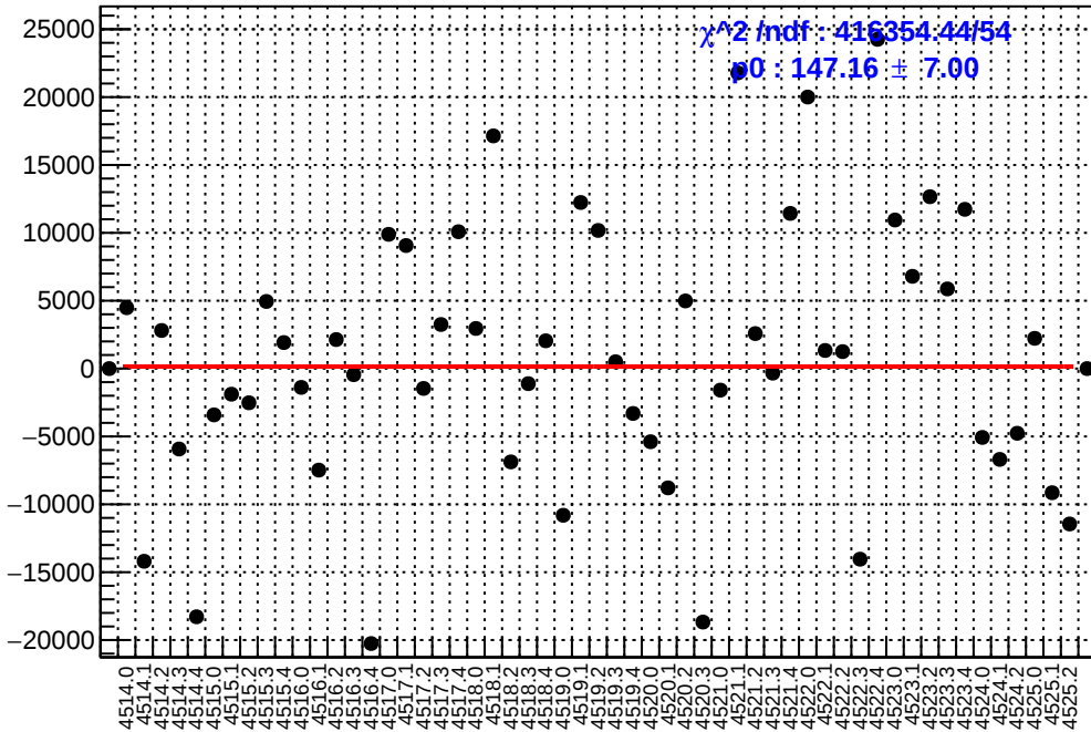
slug64: asym_left_avg.mean/ppb-reg_asym_left_avg.mean/ppb
