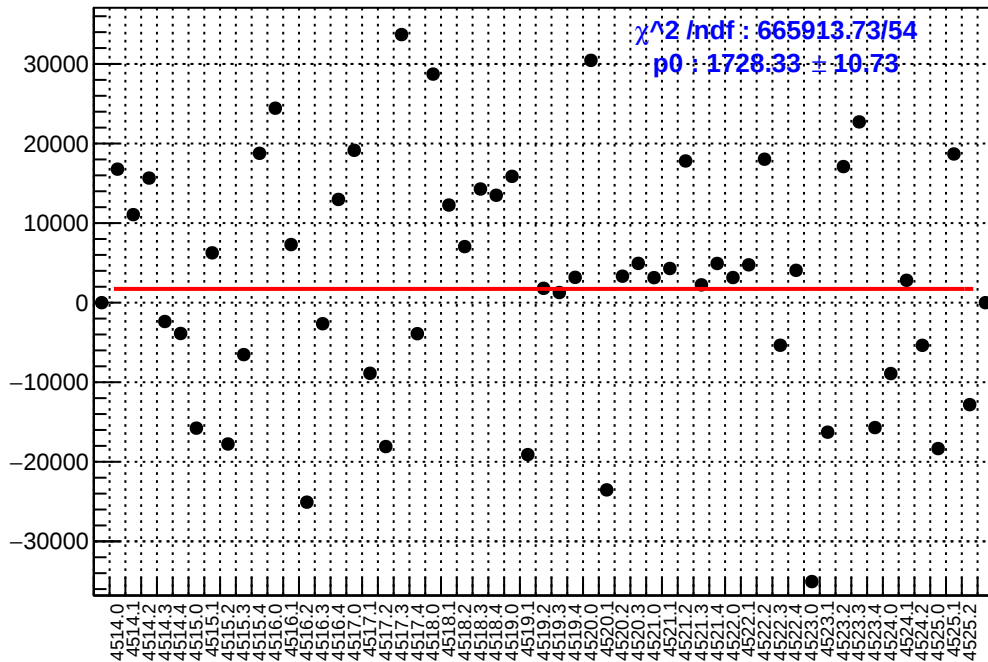
slug64: asym_atr2.mean/ppb-reg_asym_atr2.mean/ppb
