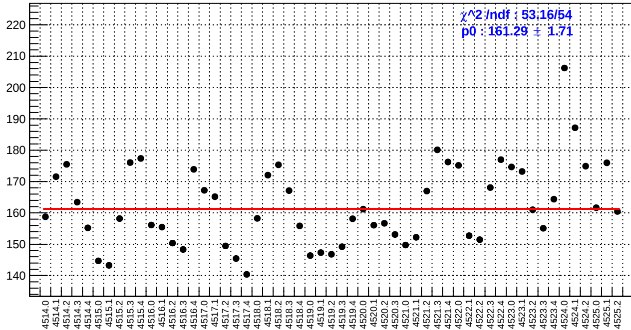
slug64: asym_bcm_an_ds3.rms/ppm
