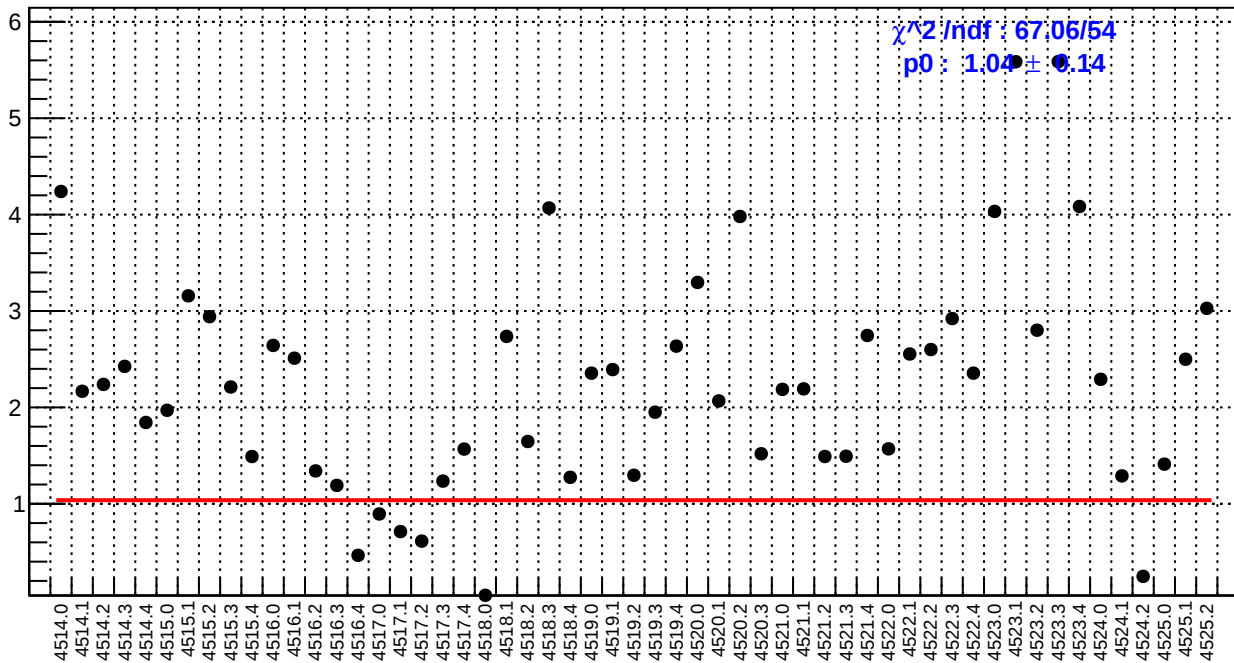
slug64: us_avg_bpm4aX/(ppb/nm)
