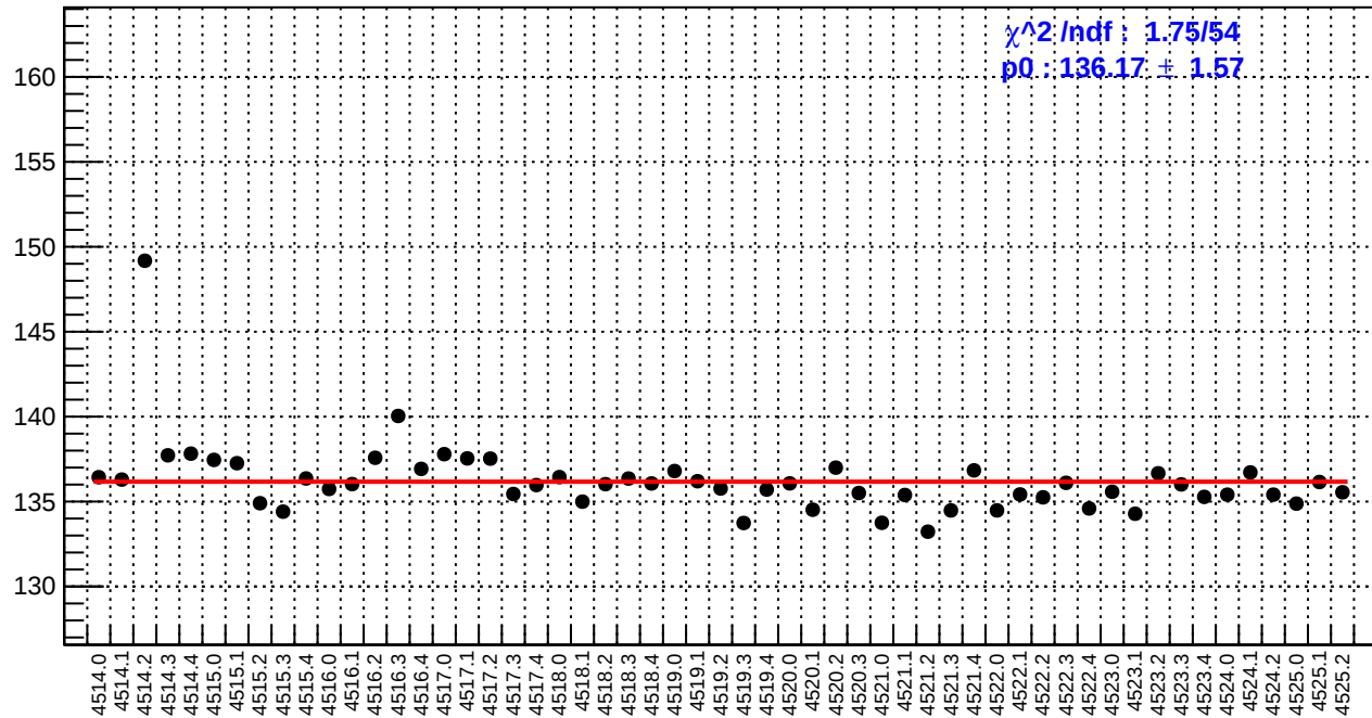
slug64: reg_asym_usl.rms/ppm
