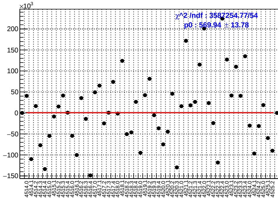
slug64: asym_sam4.mean/ppb-reg_asym_sam4.mean/ppb
