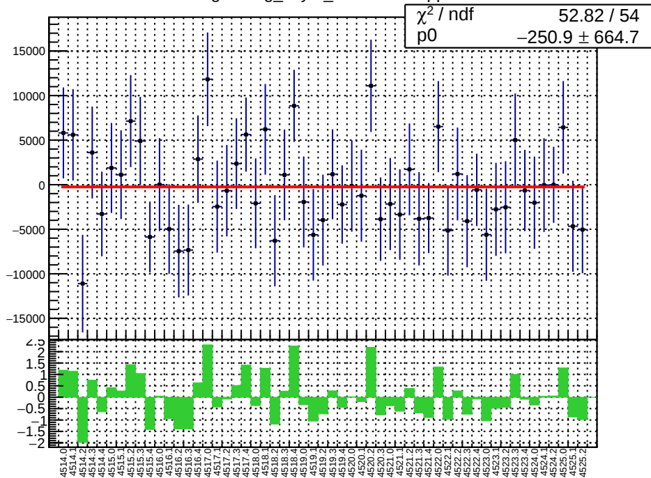
slug64: reg_asym_sam8.mean/ppb
