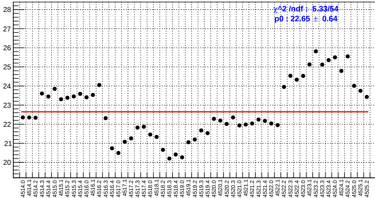
slug64: right_avg_bpm4eX/(ppb/nm)
