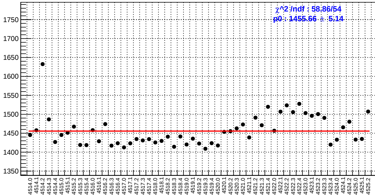
slug64: reg_asym_sam4.rms/ppm
