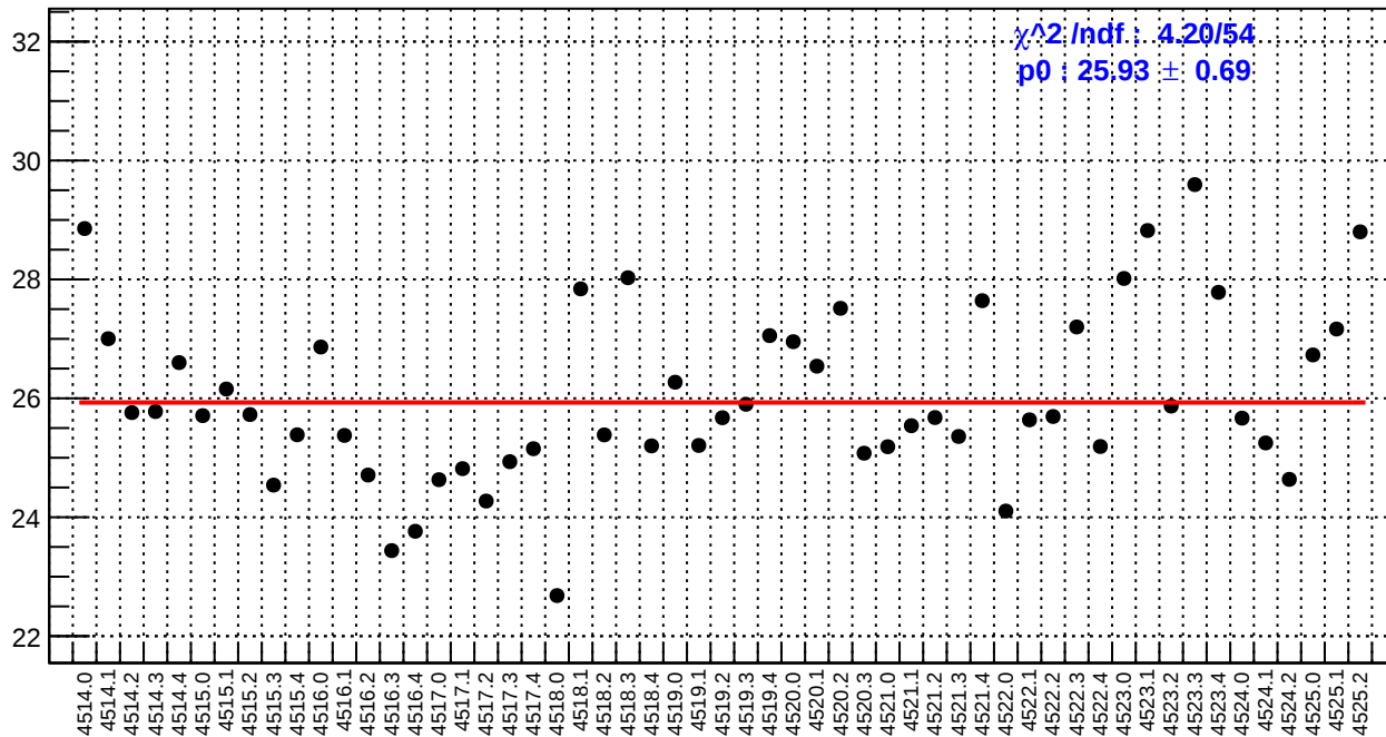
slug64: dsl_bpm4aX/(ppb/nm)
