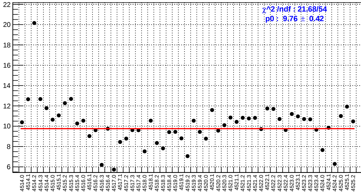
slug64: ds_avg_bpm4aY/(ppb/nm)
