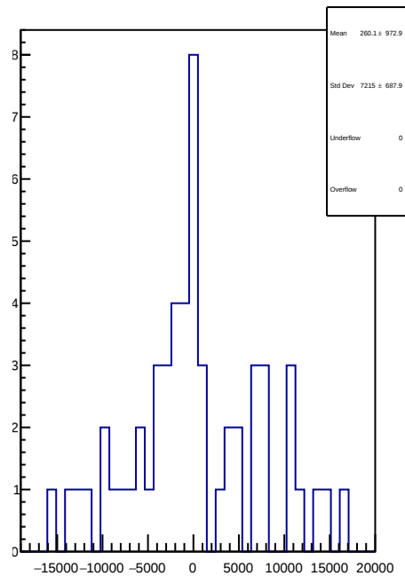
slug64: 1D Corr asym_us_dd.mean/ppb-reg_asym_us_dd.mean/ppb
