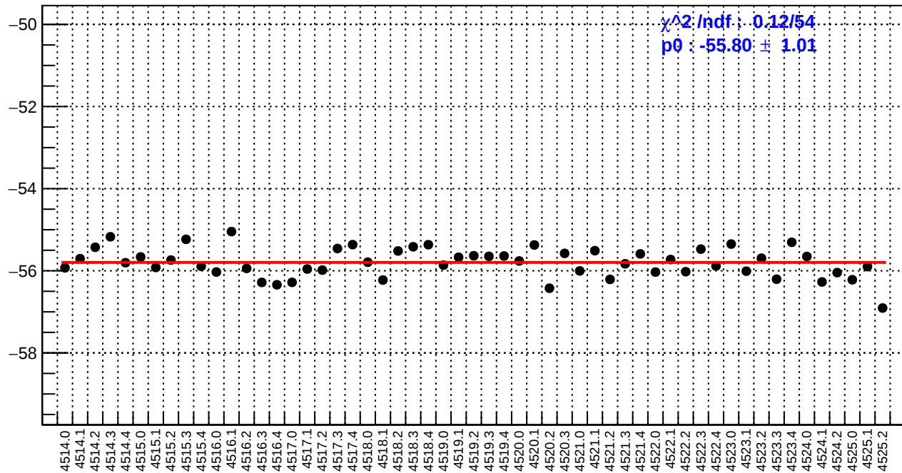
slug64: ds_avg_bpm12X/(ppb/nm)
