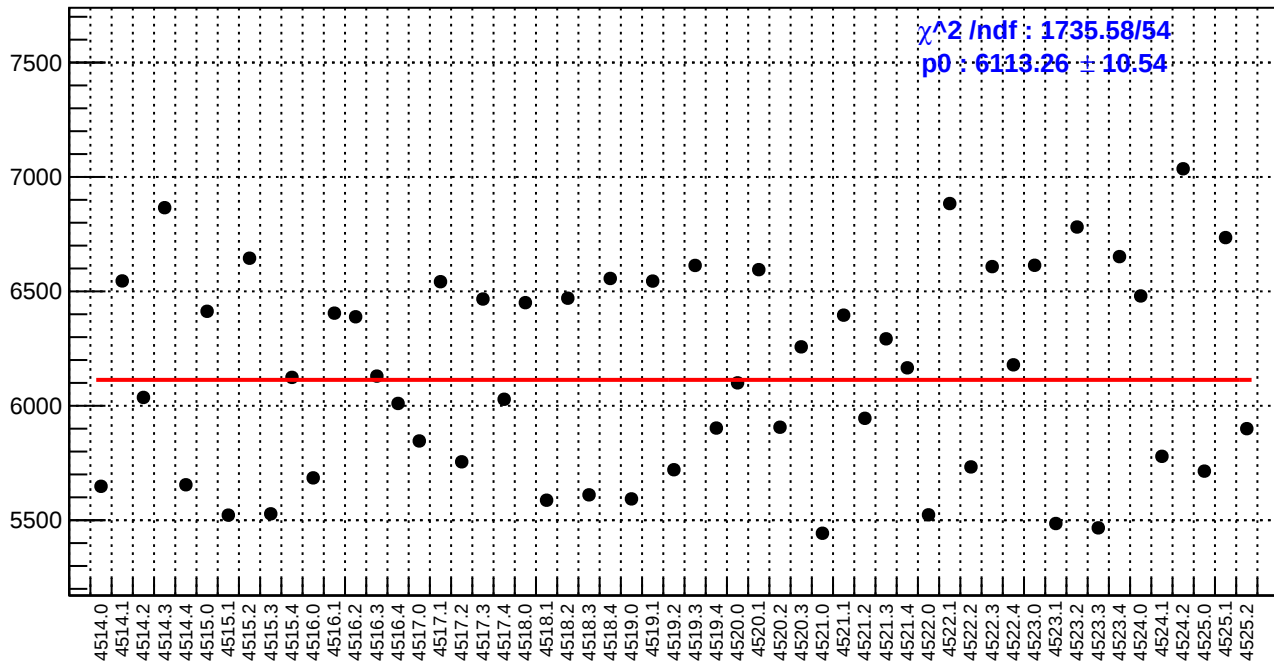
slug64: diff_bpm4eY.rms/nm
