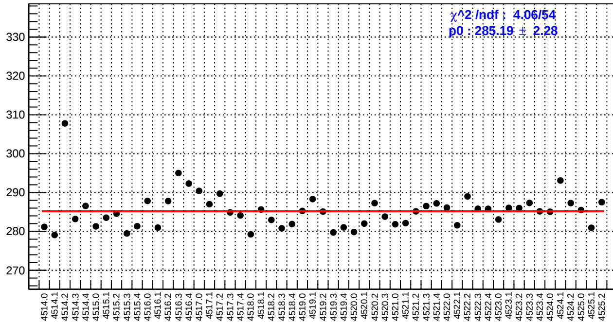
slug64: reg_asym_at2_avg.rms/ppm
