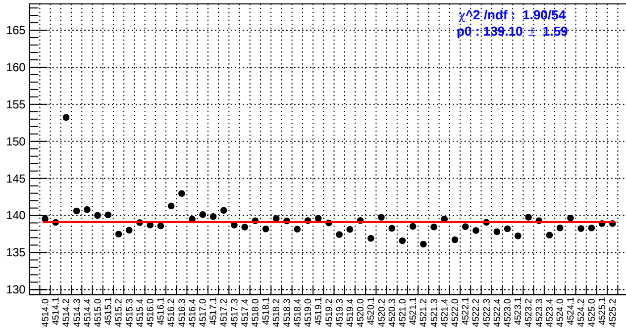
slug64: reg_asym_dsl.rms/ppm
