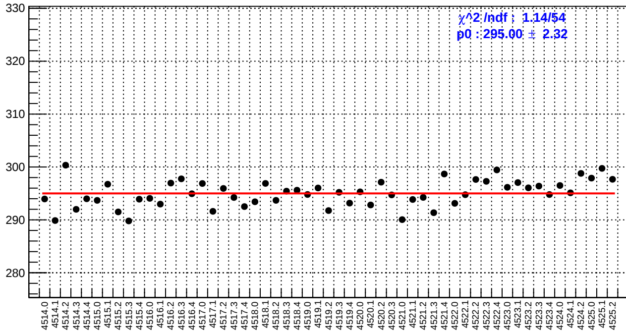
slug64: reg_asym_atr1l2_dd.rms/ppm
