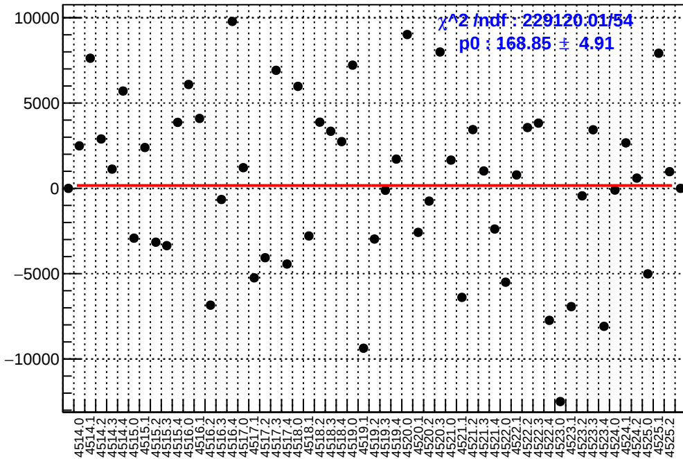
slug64: asym_dsr.mean/ppb-reg_asym_dsr.mean/ppb
