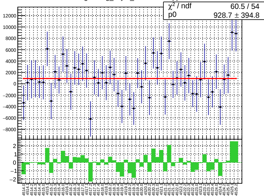
slug64: reg_asym_sam5.mean/ppb
