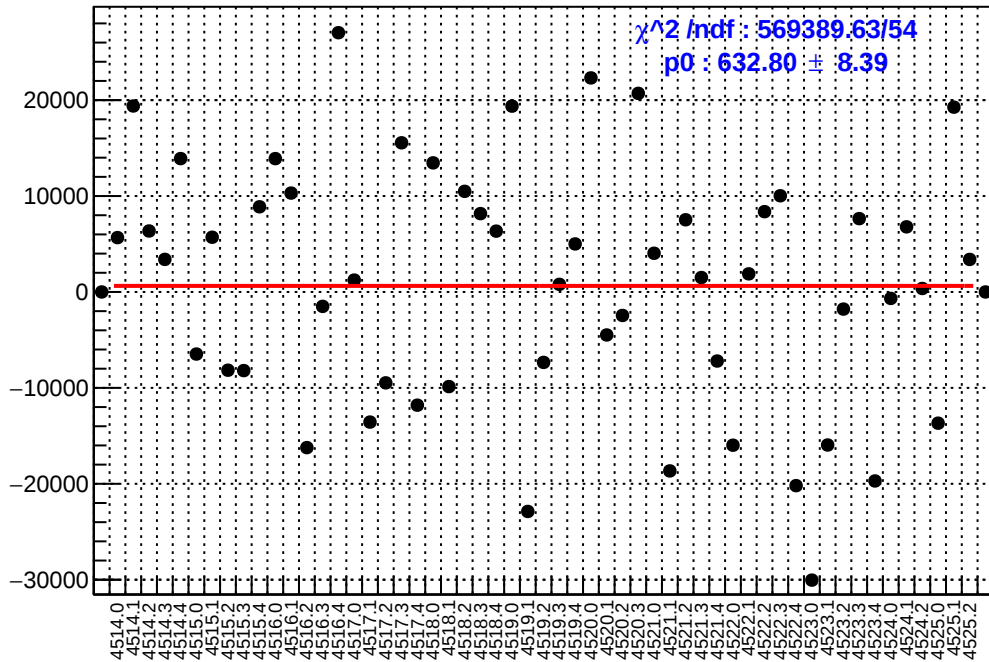
slug64: asym_at1_dd.mean/ppb-reg_asym_at1_dd.mean/ppb
