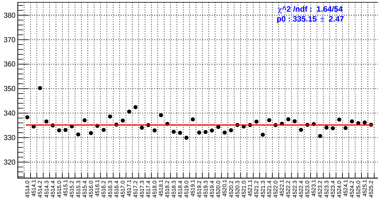
slug64: reg_asym_atl_dd.rms/ppm
