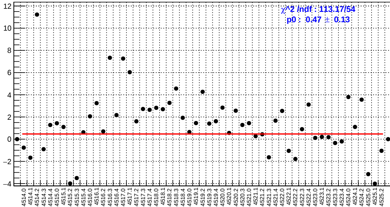
slug64: right_avg_bpm4eY/(ppb/nm)
