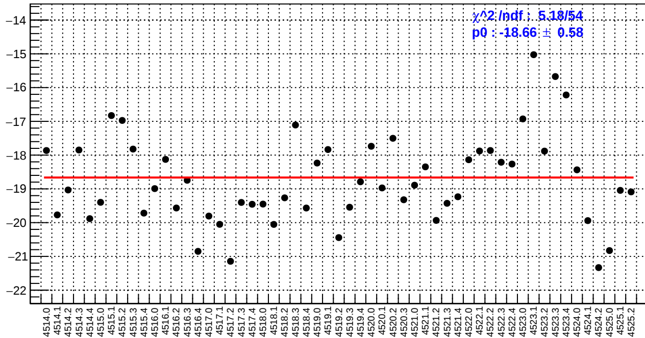
slug64: right_avg_bpm4aX/(ppb/nm)
