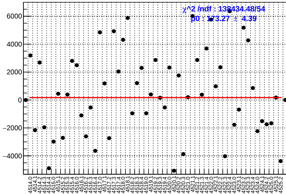
slug64: asym_us_avg.mean/ppb-reg_asym_us_avg.mean/ppb
