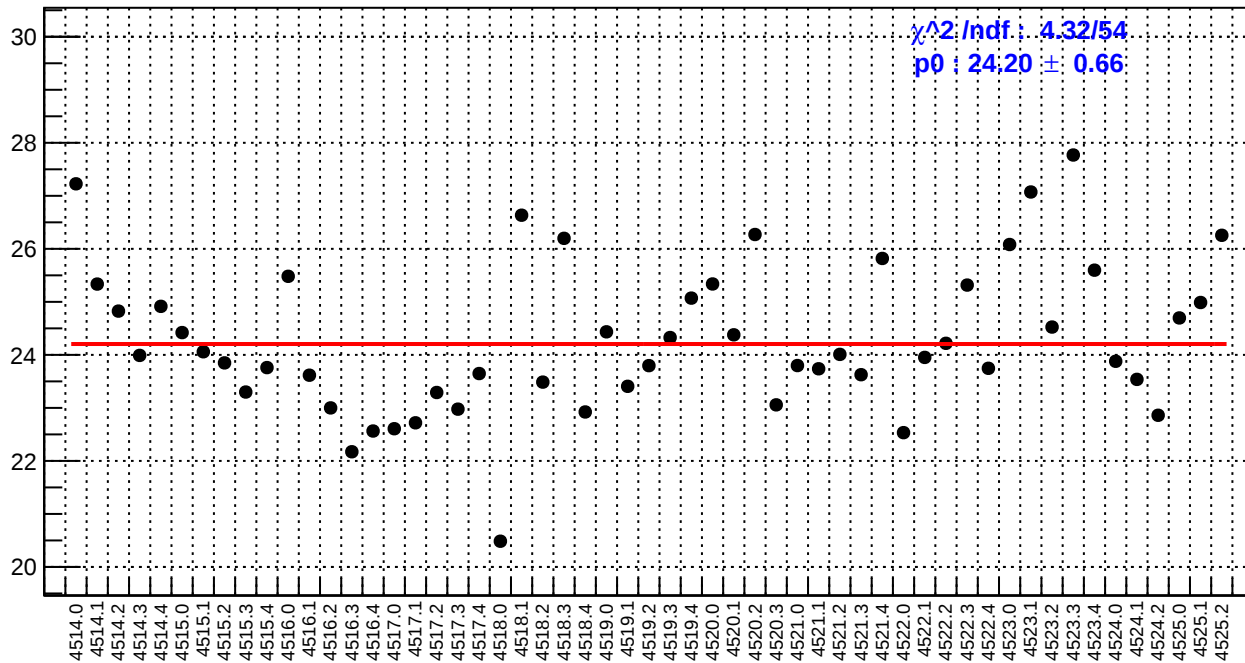
slug64: usl_bpm4aX/(ppb/nm)
