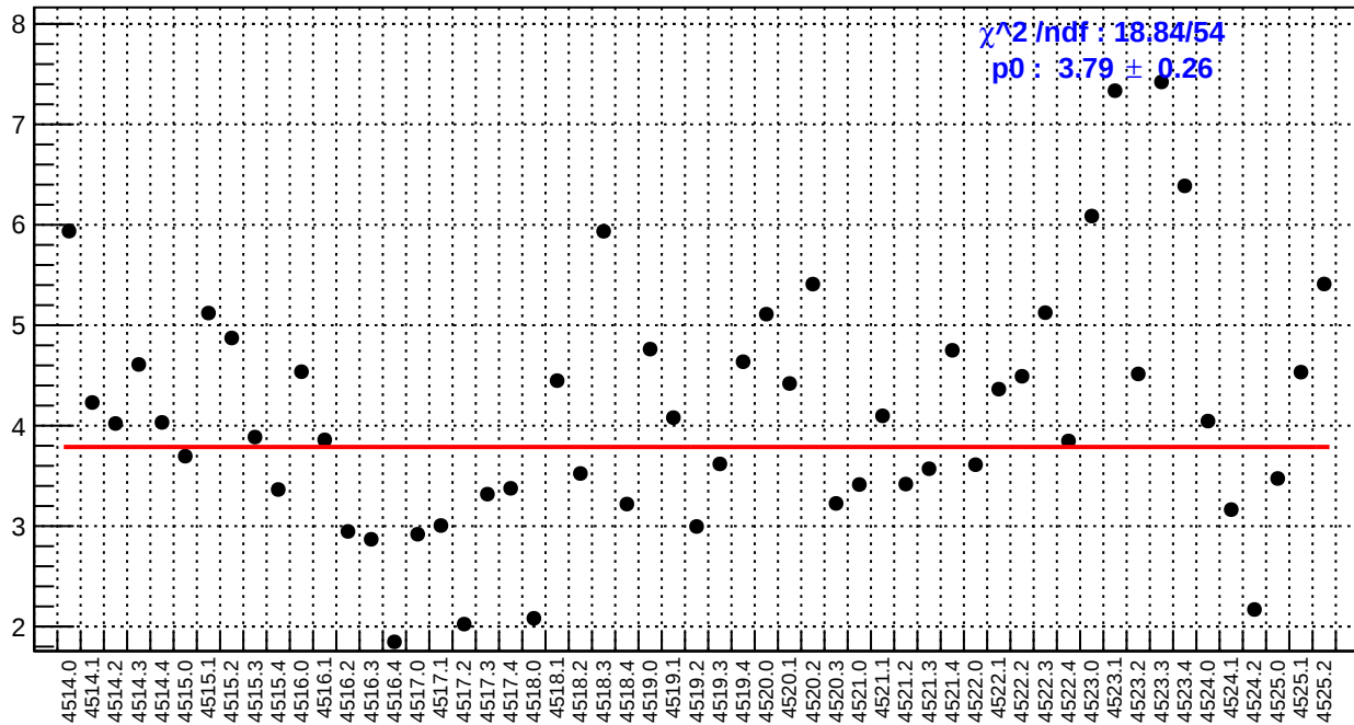
slug64: ds_avg_bpm4aX/(ppb/nm)
