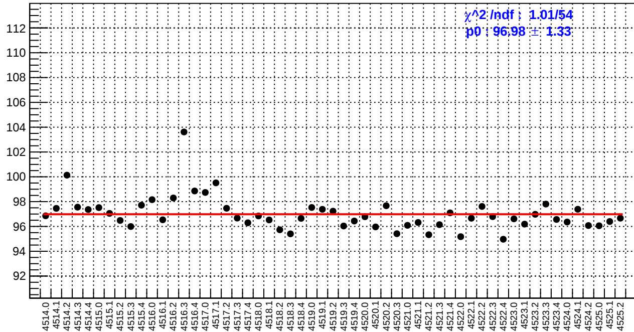
slug64: reg_asym_us_avg.rms/ppm
