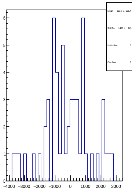
slug64: 1D Corr asym_atl1r2_dd.mean/ppb-reg_asym_atl1r2_dd.mean/ppb
