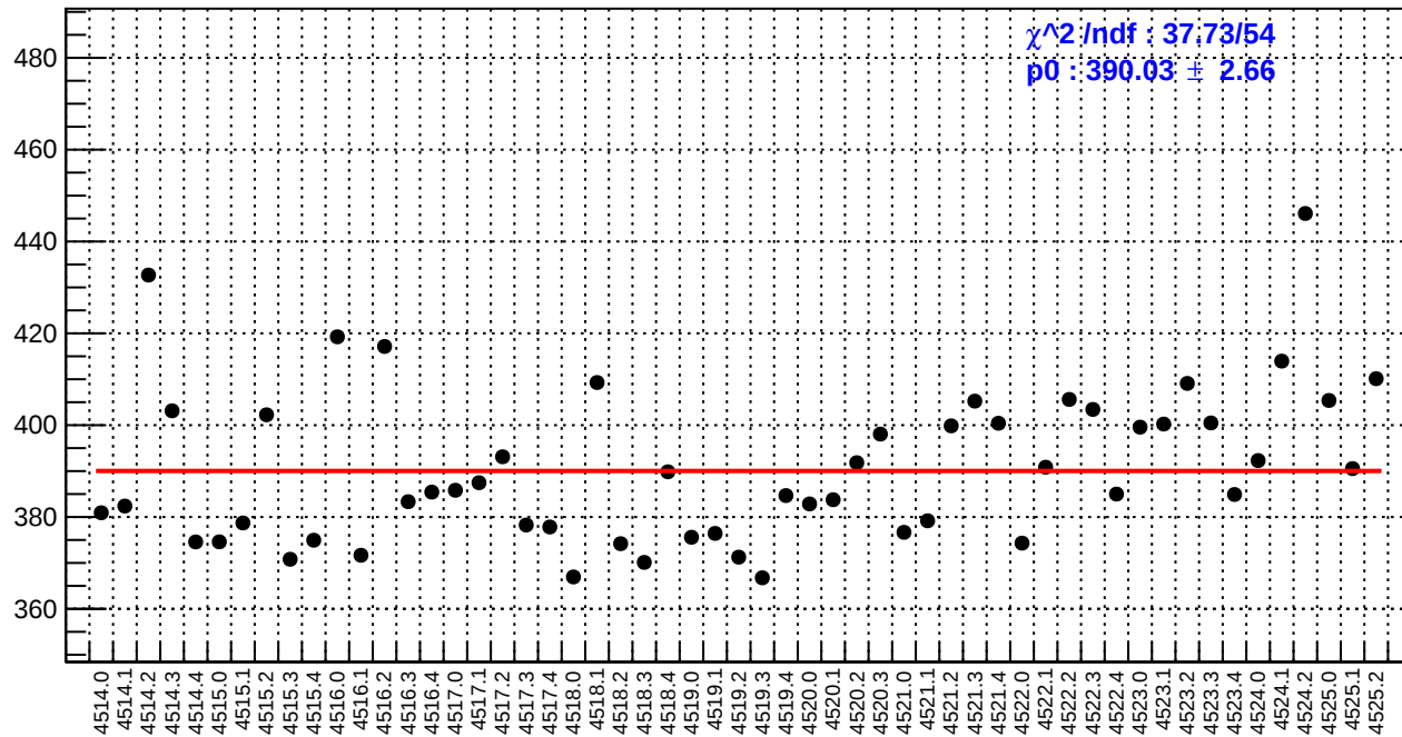
slug64: reg_asym_sam6.rms/ppm
