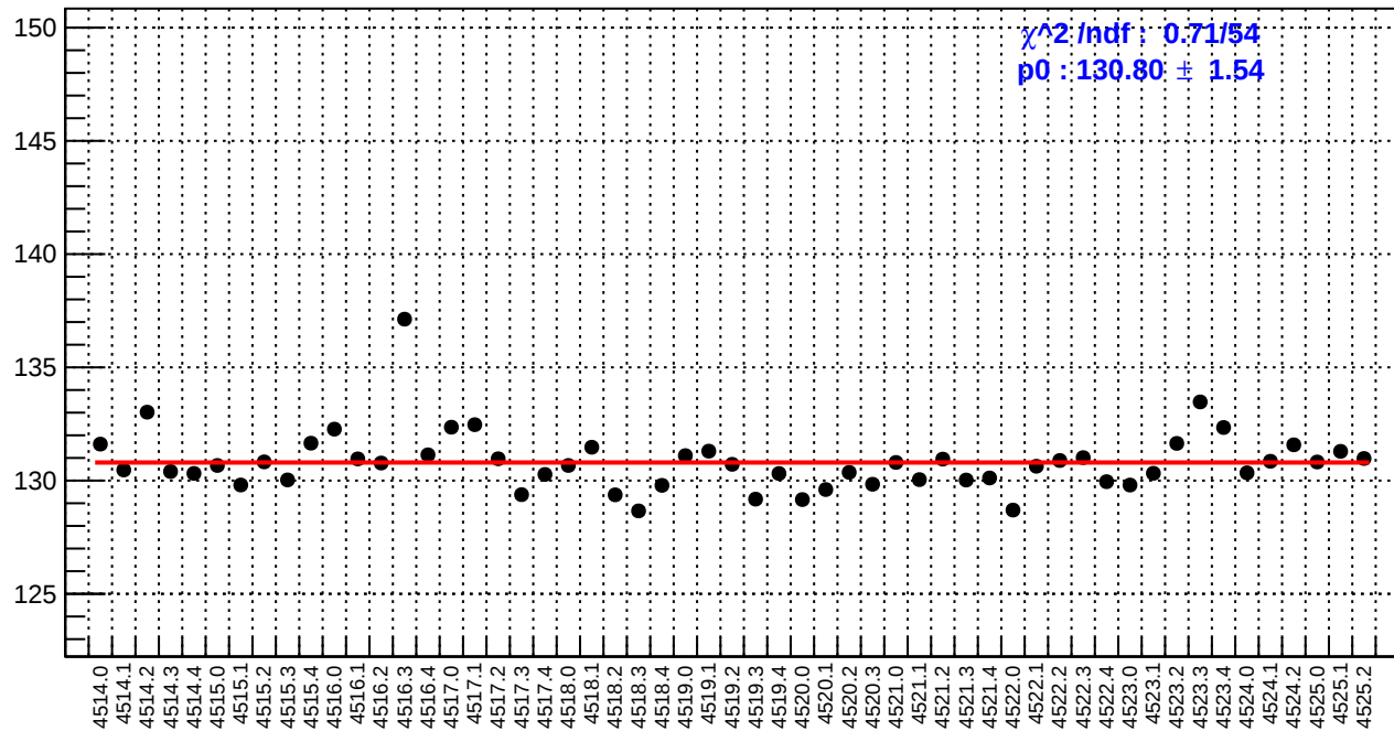
slug64: reg_asym_right_avg.rms/ppm
