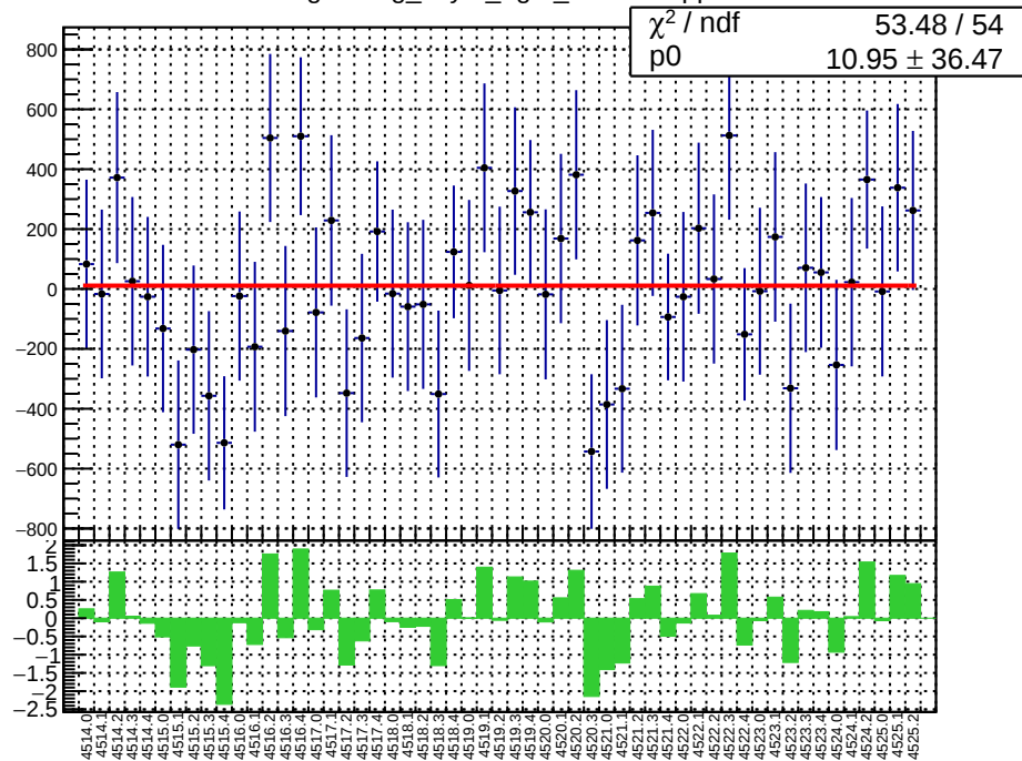
slug64: reg_asym_right_dd.mean/ppb
