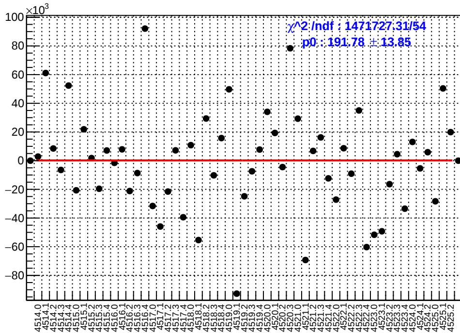
slug64: asym_sam6.mean/ppb-reg_asym_sam6.mean/ppb
