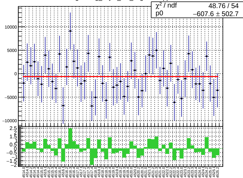
slug64: reg_asym_at1_avg.mean/ppb
