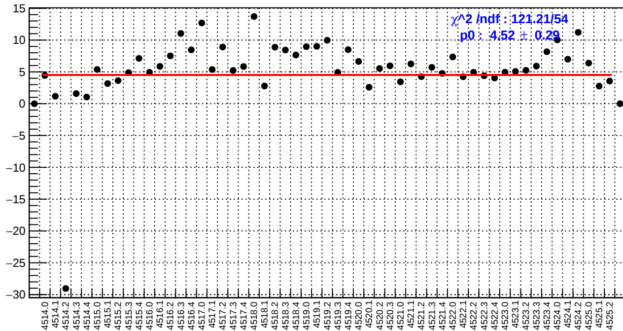
slug64: usl_bpm4eY/(ppb/nm)
