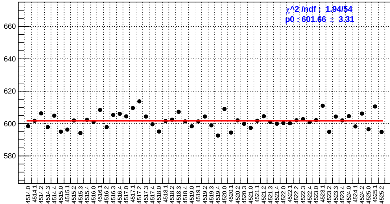
slug64: reg_asym_atl1.rms/ppm
