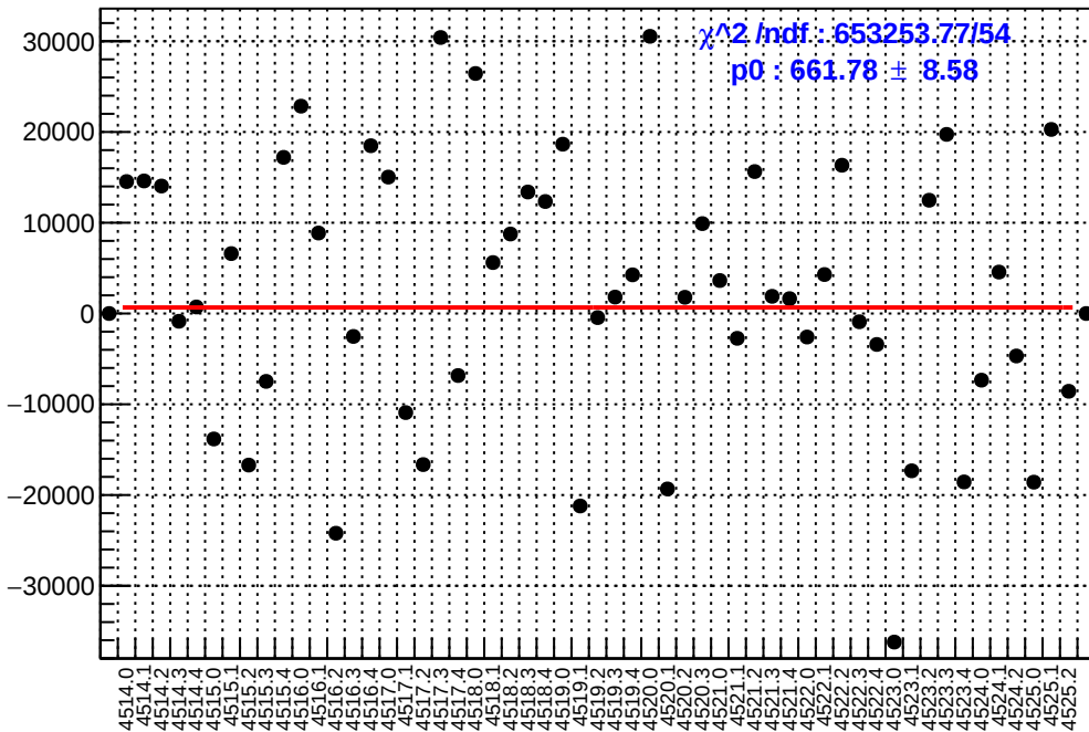
slug64: asym_atl1.mean/ppb-reg_asym_atl1.mean/ppb
