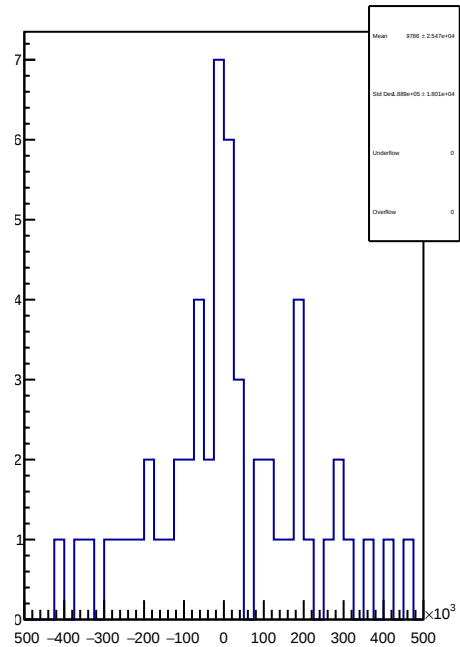
slug64: 1D Corr asym_sam3.mean/ppb-reg_asym_sam3.mean/ppb
