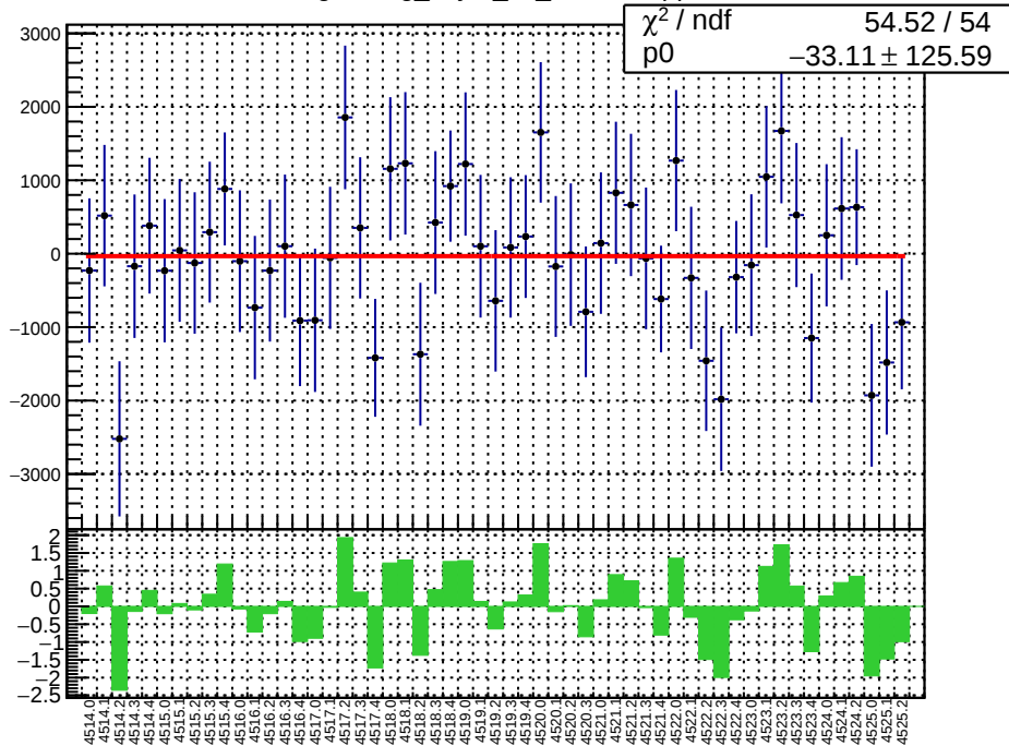
slug64: reg_asym_us_dd.mean/ppb
