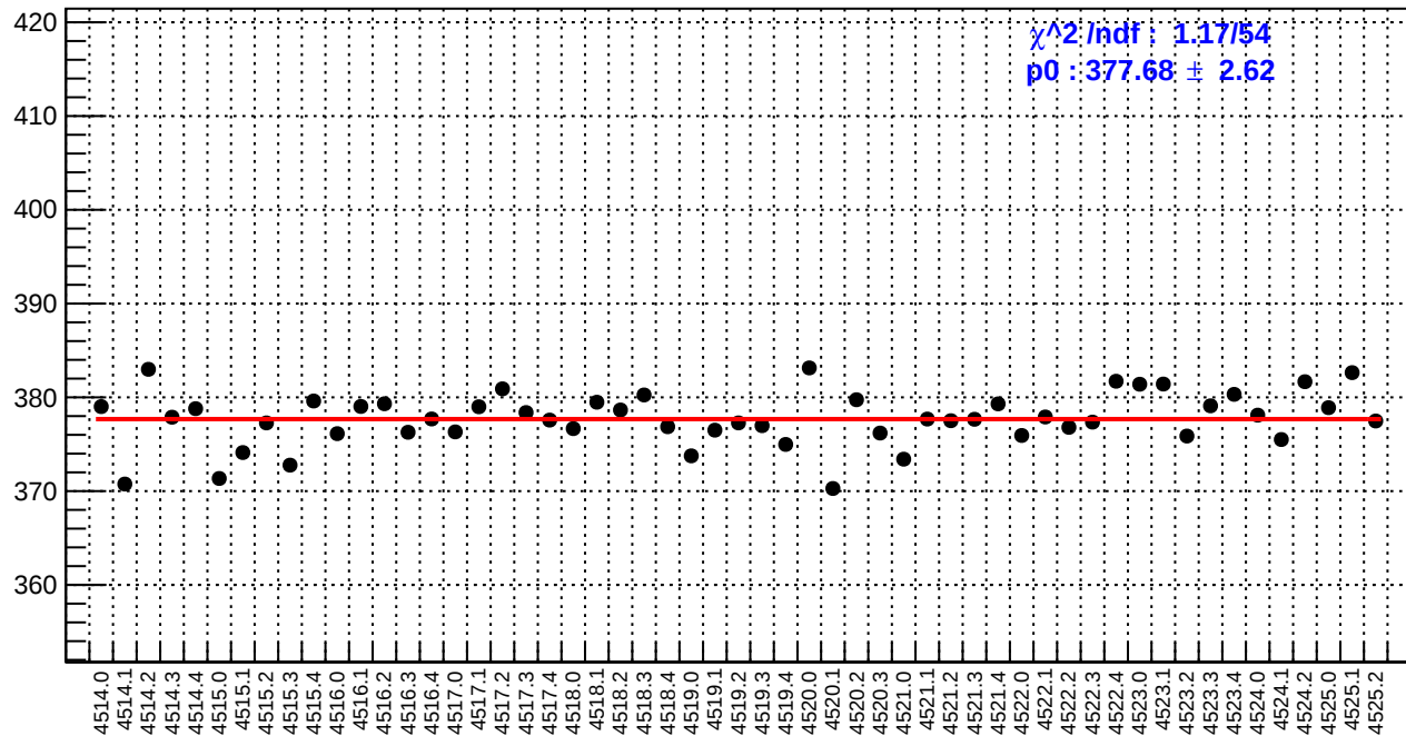
slug64: reg_asym_at1_dd.rms/ppm
