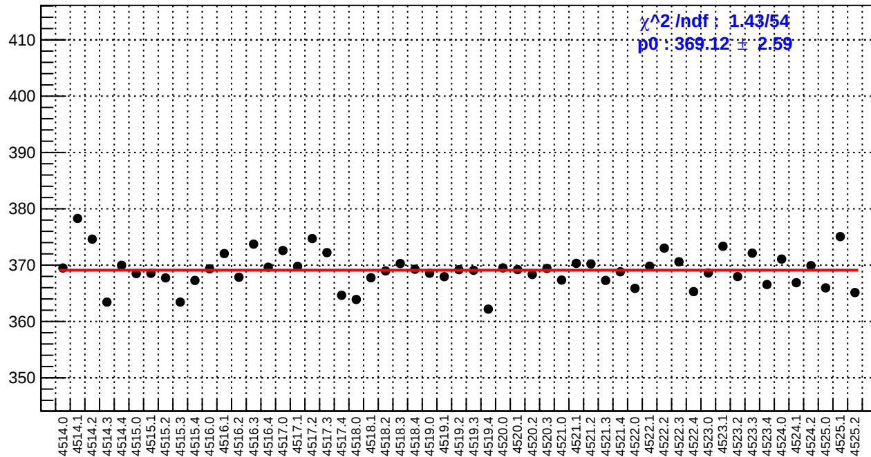
slug64: reg_asym_at1_avg.rms/ppm
