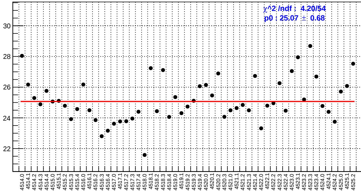
slug64: left_avg_bpm4aX/(ppb/nm)
