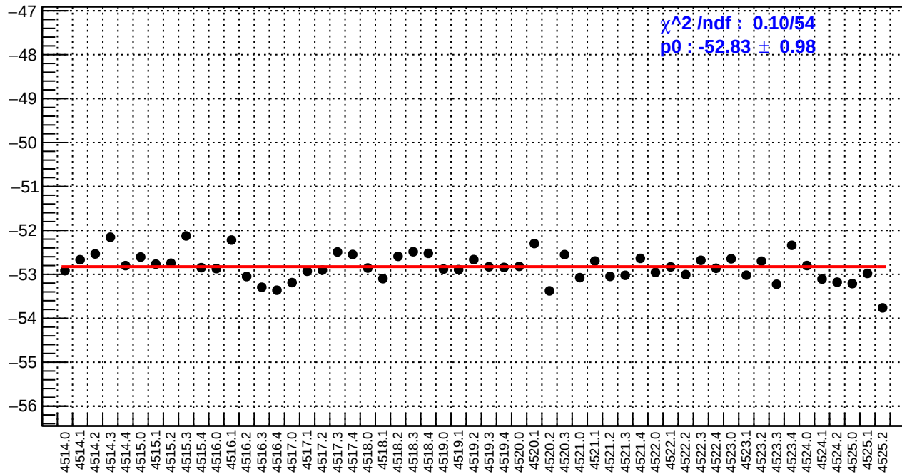
slug64: us_avg_bpm12X/(ppb/nm)
