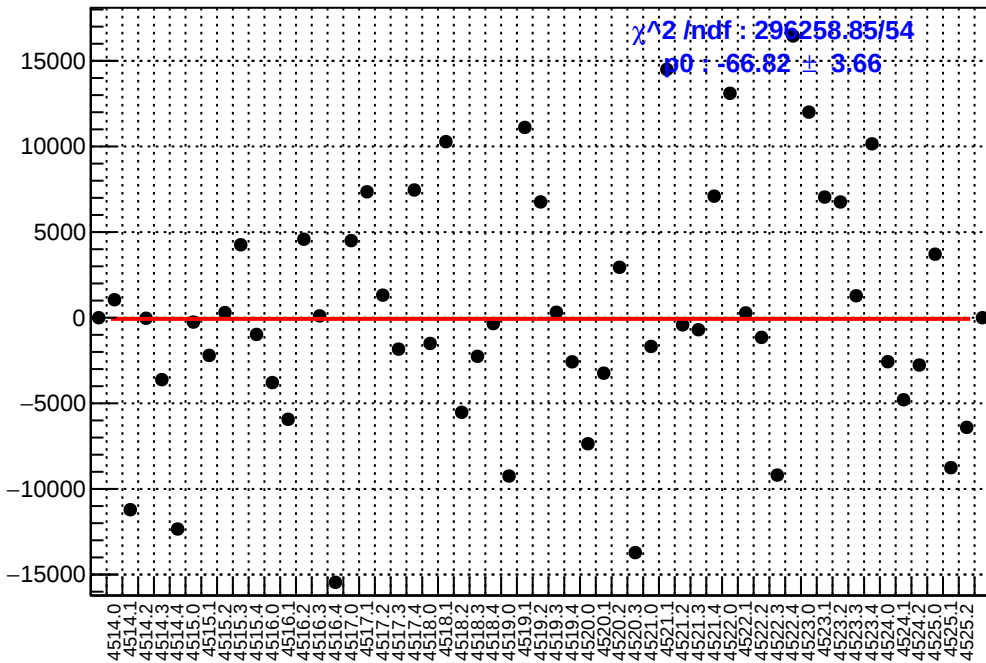
slug64: asym_ds_dd.mean/ppb-reg_asym_ds_dd.mean/ppb
