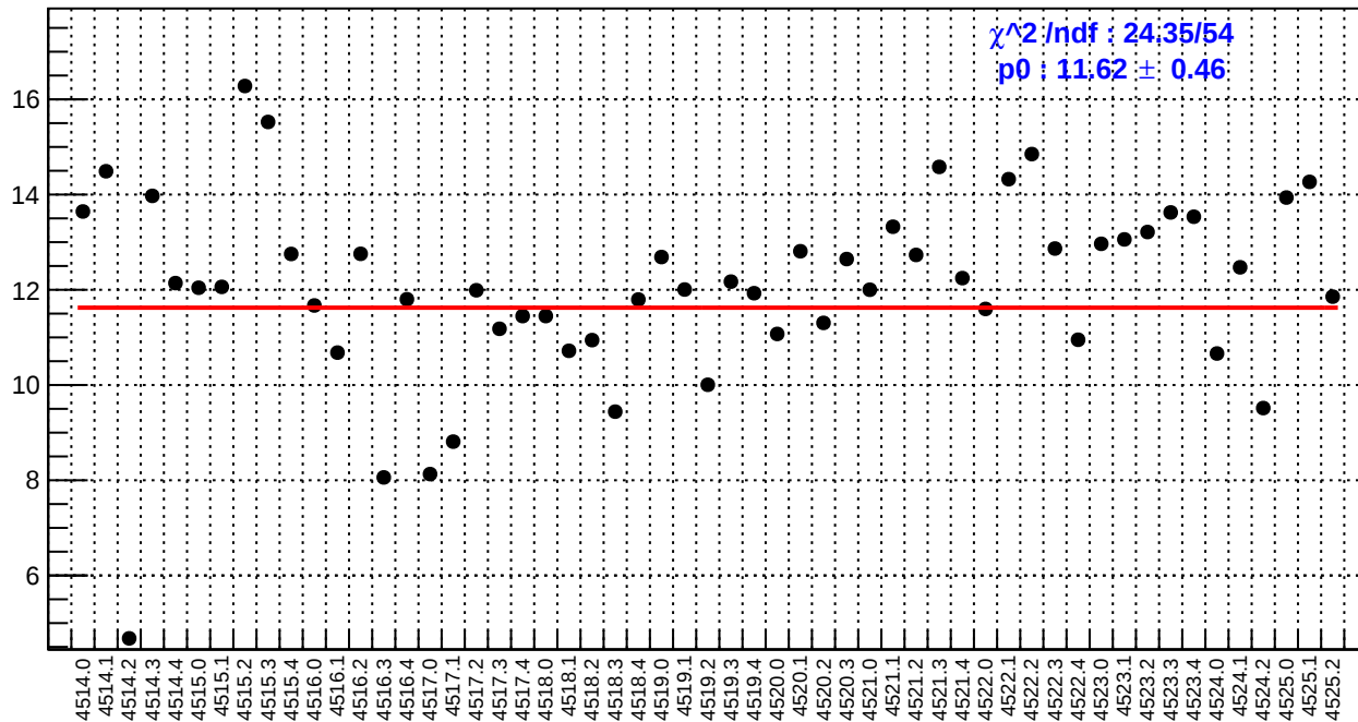
slug64: right_avg_bpm4aY/(ppb/nm)
