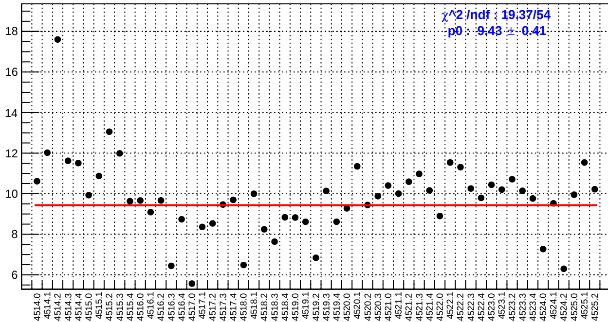
slug64: us_avg_bpm4aY/(ppb/nm)
