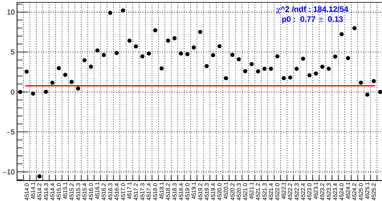
slug64: ds_avg_bpm4eY/(ppb/nm)
