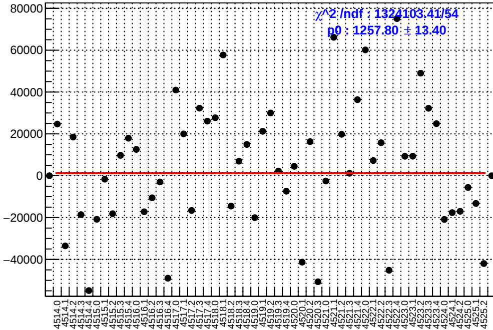
slug64: asym_atl2.mean/ppb-reg_asym_atl2.mean/ppb
