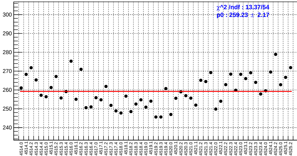
slug64: reg_asym_sam1.rms/ppm
