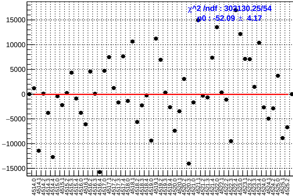
slug64: asym_us_dd.mean/ppb-reg_asym_us_dd.mean/ppb
