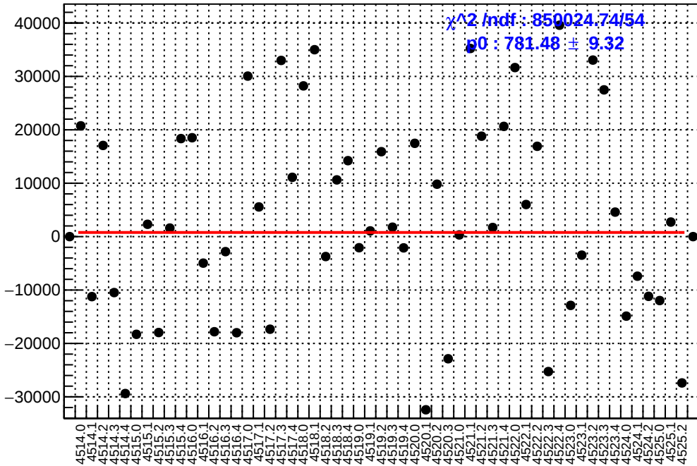
slug64: asym_at2_avg.mean/ppb-reg_asym_at2_avg.mean/ppb
