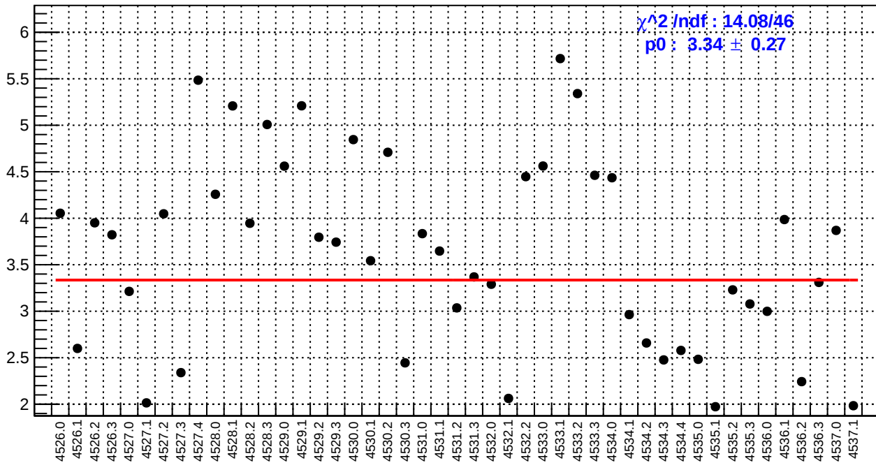
slug65: ds_avg_bpm4aX/(ppb/nm)
