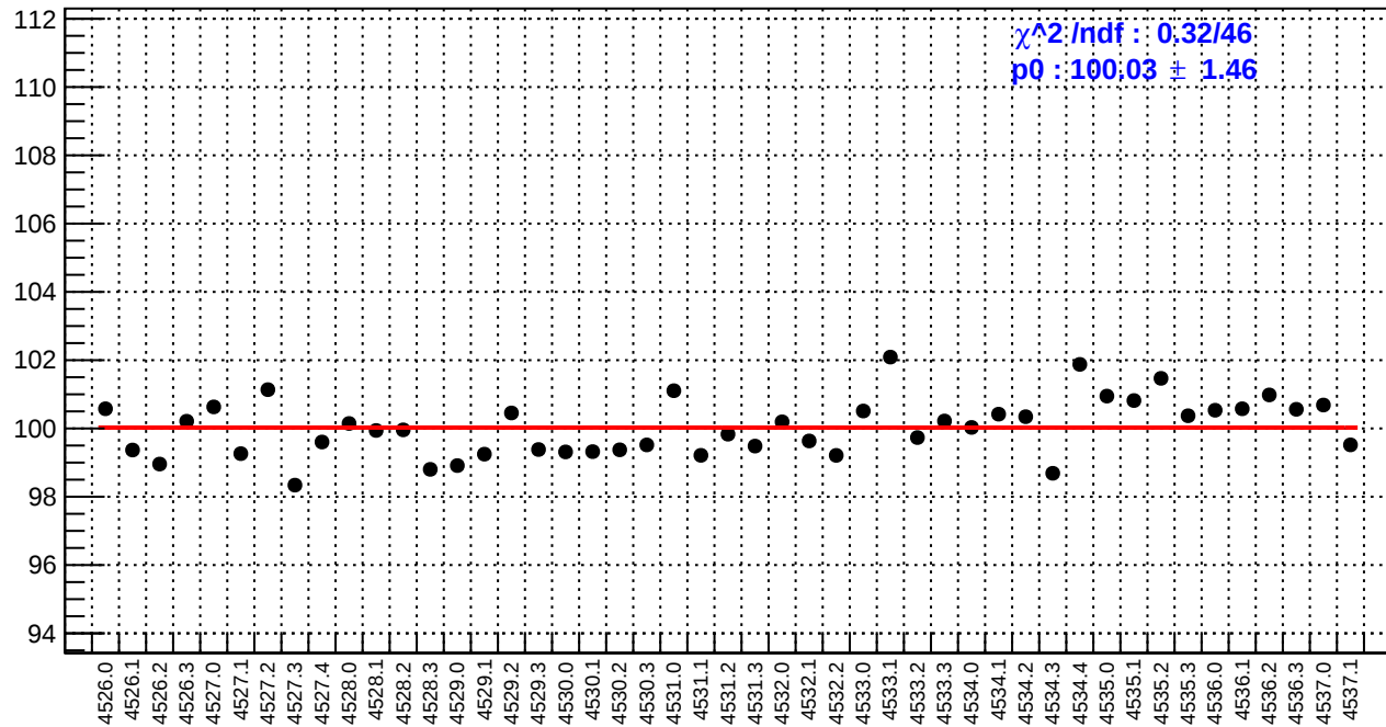
slug65: reg_asym_ds_avg.rms/ppm
