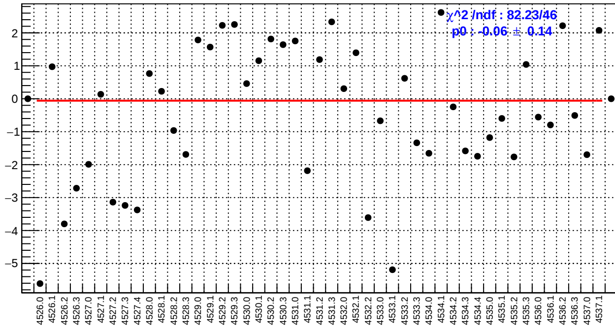
slug65: usr_bpm4eY/(ppb/nm)
