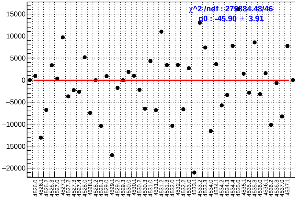
slug65: asym_left_avg.mean/ppb-reg_asym_left_avg.mean/ppb
