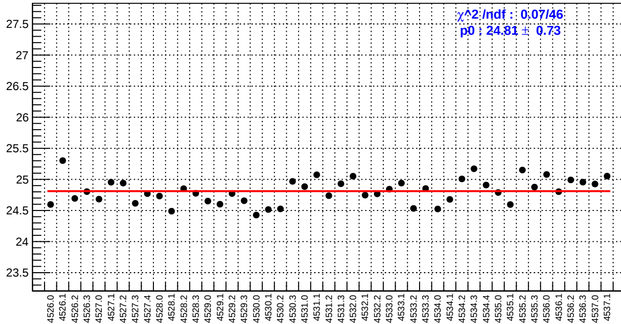
slug65: reg_asym_left_dd.rms/ppm
