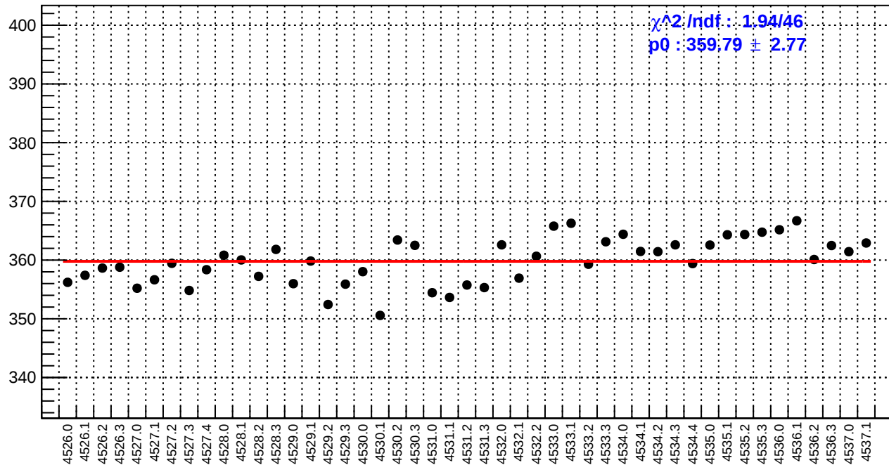
slug65: reg_asym_atl1r2_avg.rms/ppm
