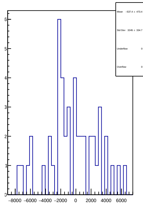
slug65: 1D Corr asym_us_avg.mean/ppb-reg_asym_us_avg.mean/ppb
