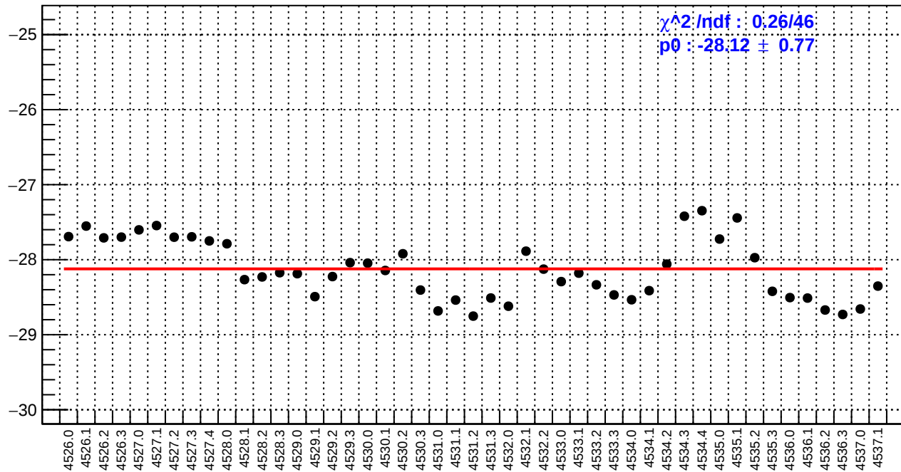
slug65: ds_avg_bpm4eX/(ppb/nm)
