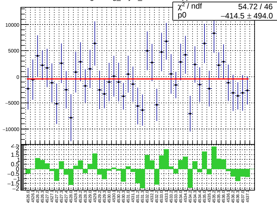
slug65: reg_asym_sam7.mean/ppb
