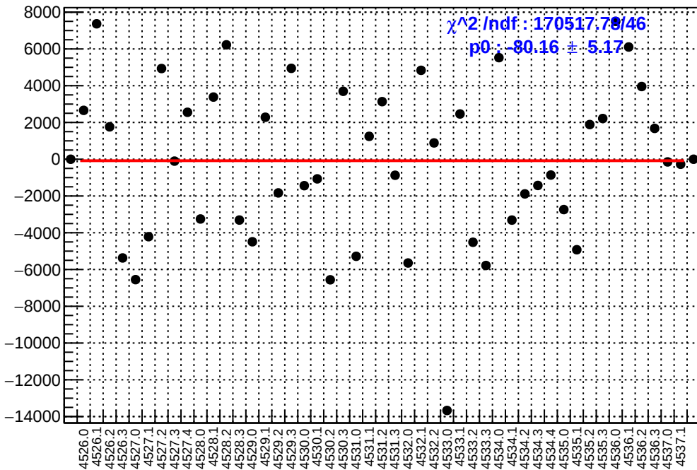
slug65: asym_dsr.mean/ppb-reg_asym_dsr.mean/ppb
