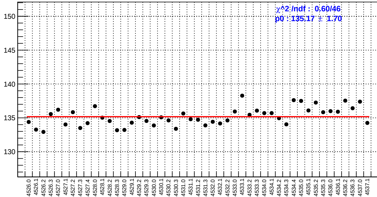
slug65: reg_asym_left_avg.rms/ppm
