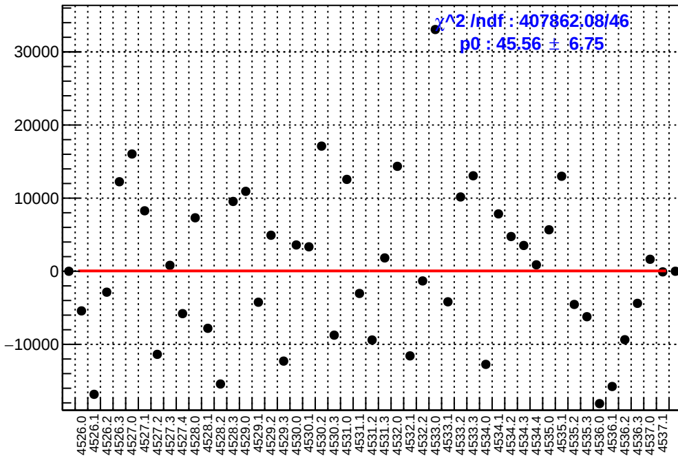
slug65: asym_atr_dd.mean/ppb-reg_asym_atr_dd.mean/ppb
