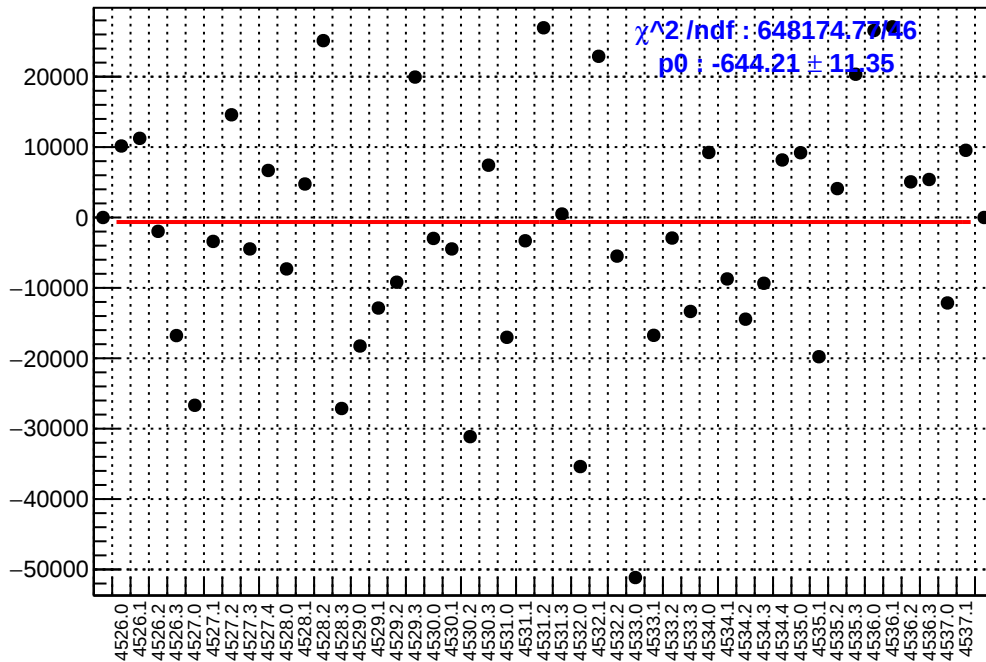
slug65: asym_atl1r2_avg.mean/ppb-reg_asym_atl1r2_avg.mean/ppb
