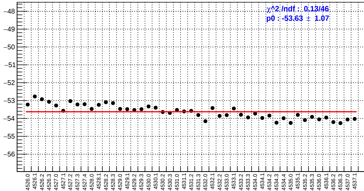
slug65: us_avg_bpm12X/(ppb/nm)
