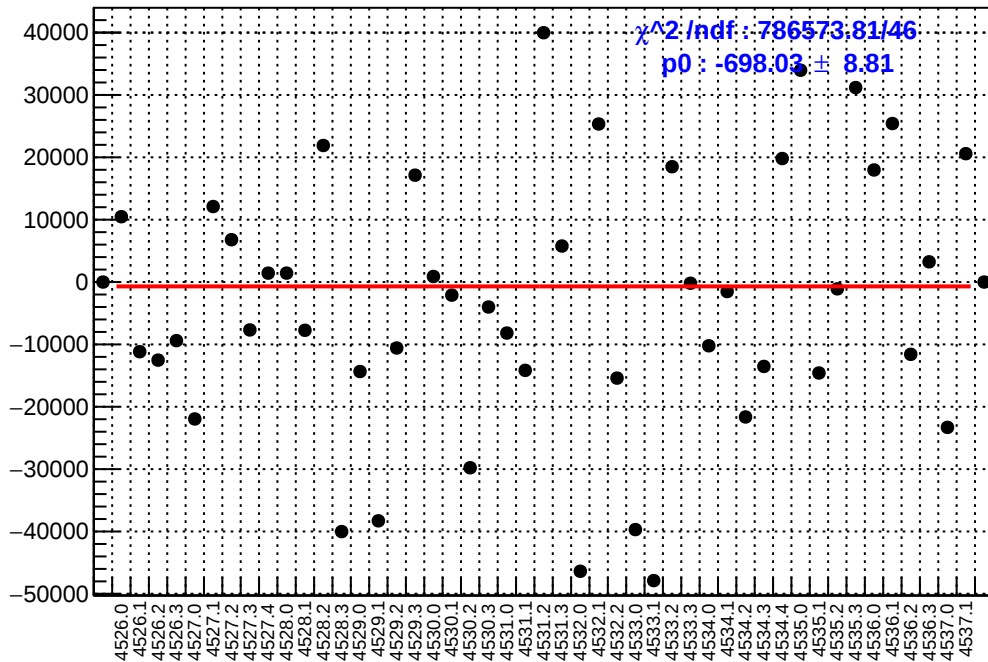
slug65: asym_at2_avg.mean/ppb-reg_asym_at2_avg.mean/ppb
