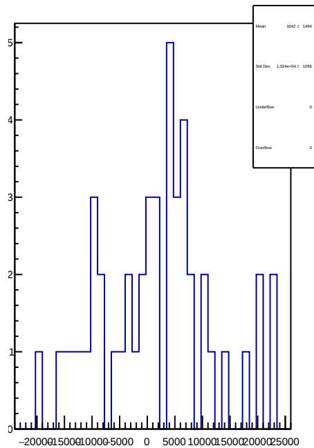
slug65: 1D Corr asym_atr1l2_dd.mean/ppb-reg_asym_atr1l2_dd.mean/ppb
