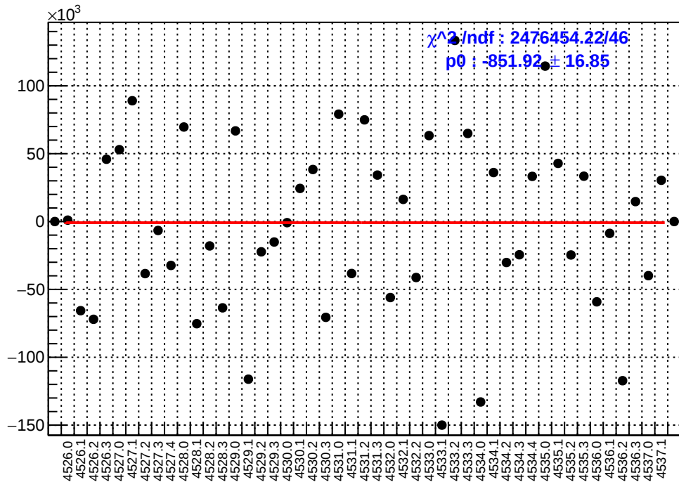
slug65: asym_sam4.mean/ppb-reg_asym_sam4.mean/ppb
