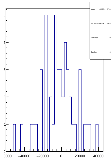
slug65: 1D Corr asym_atr1l2_avg.mean/ppb-reg_asym_atr1l2_avg.mean/ppb
