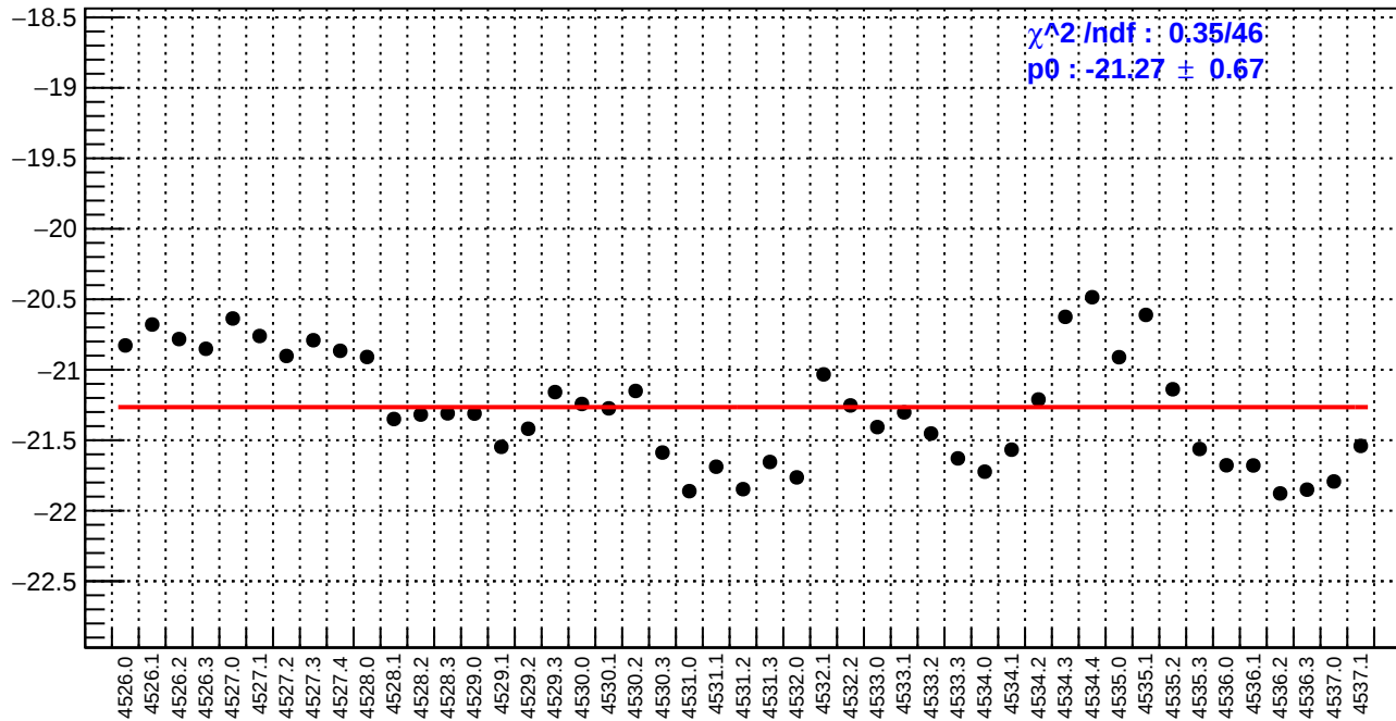
slug65: us_avg_bpm4eX/(ppb/nm)
