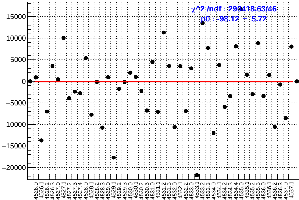
slug65: asym_dsl.mean/ppb-reg_asym_dsl.mean/ppb
