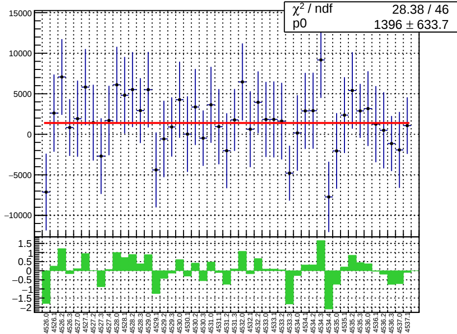
slug65: reg_asym_atr1.mean/ppb
