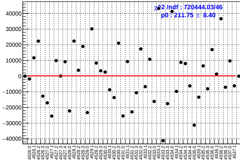
slug65: asym_sam8.mean/ppb-reg_asym_sam8.mean/ppb
