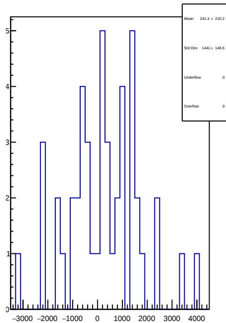
slug65: 1D Corr asym_atl1r2_dd.mean/ppb-reg_asym_atl1r2_dd.mean/ppb
