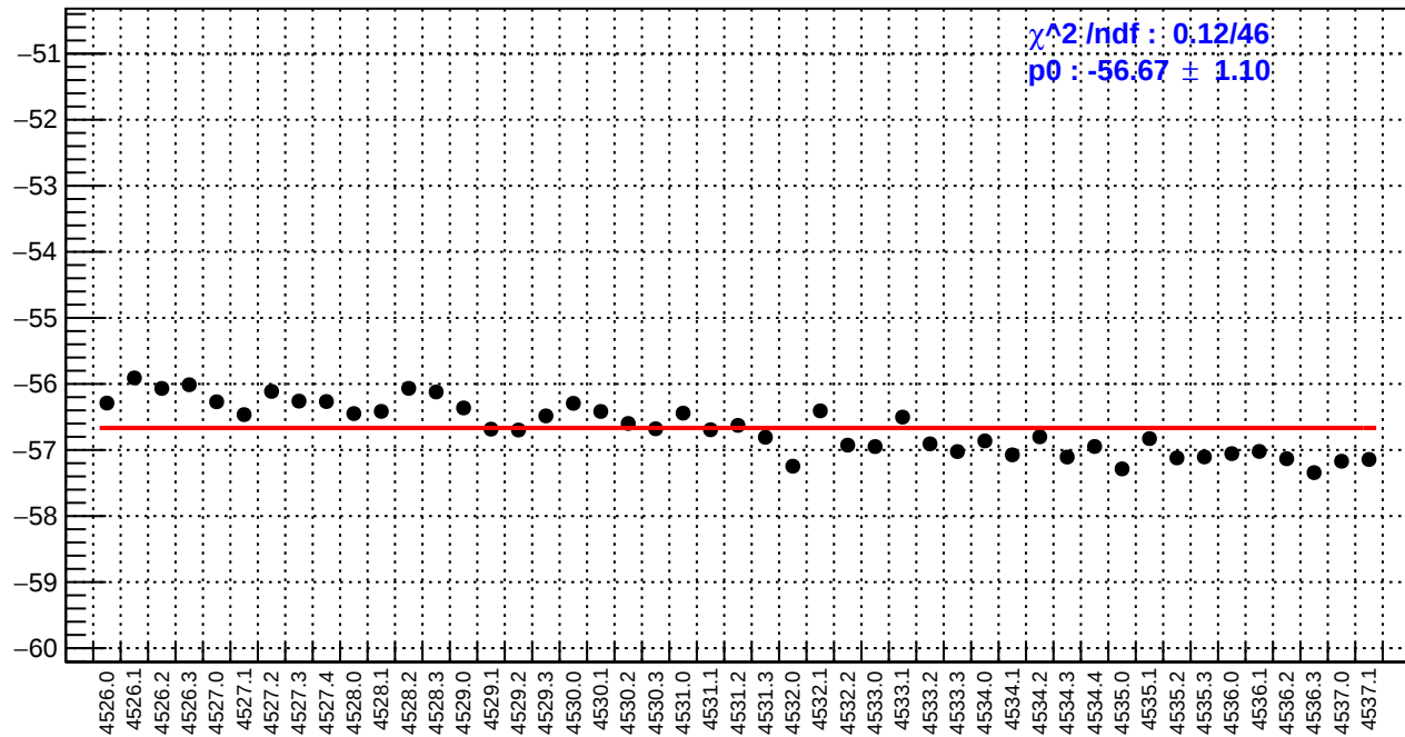
slug65: ds_avg_bpm12X/(ppb/nm)
