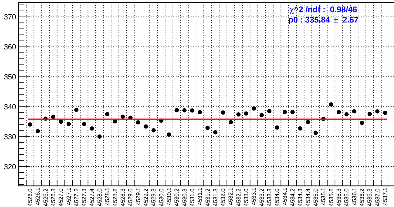
slug65: reg_asym_atl_dd.rms/ppm
