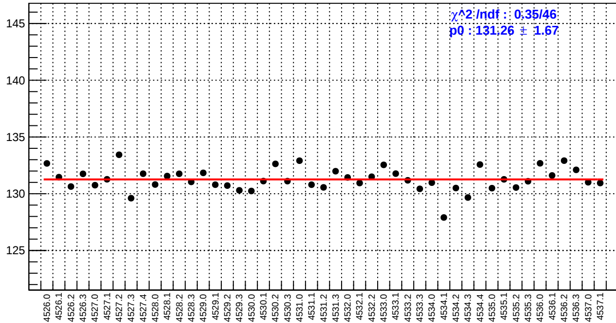
slug65: reg_asym_usr.rms/ppm
