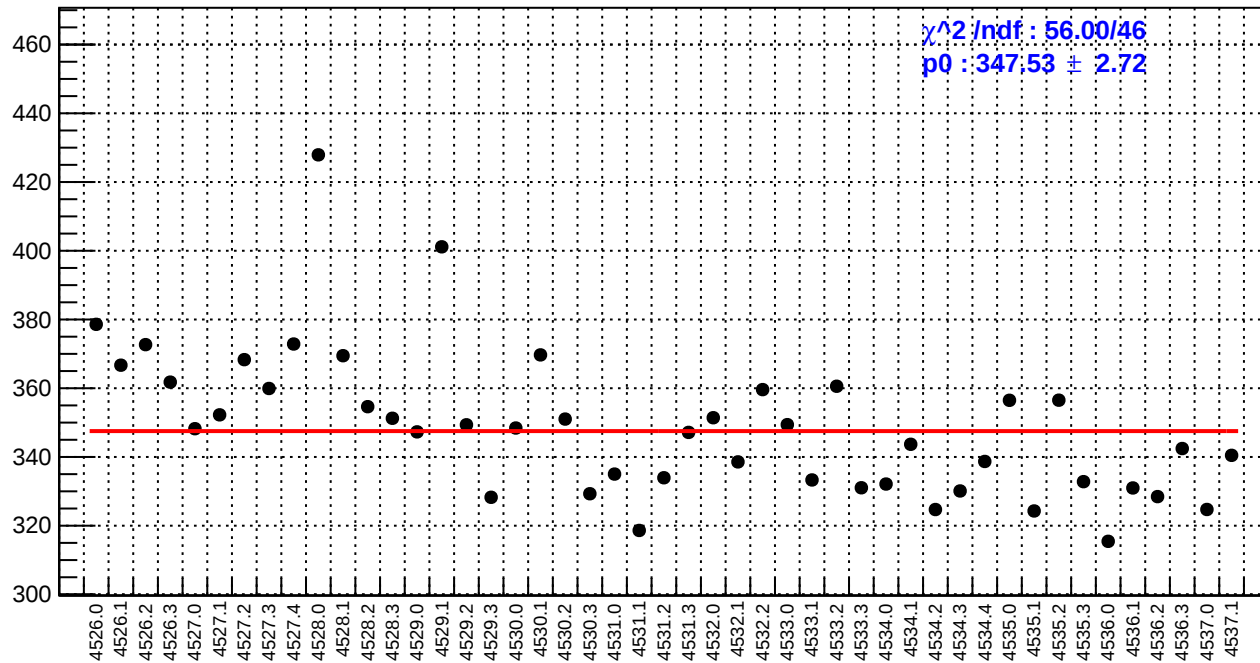
slug65: reg_asym_sam7.rms/ppm
