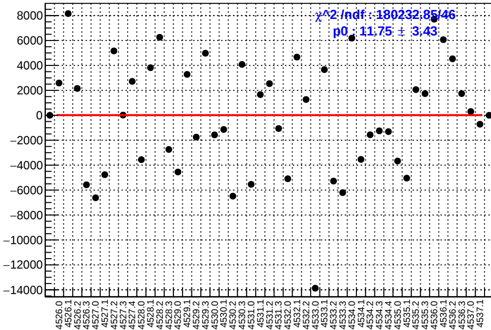
slug65: asym_right_avg.mean/ppb-reg_asym_right_avg.mean/ppb
