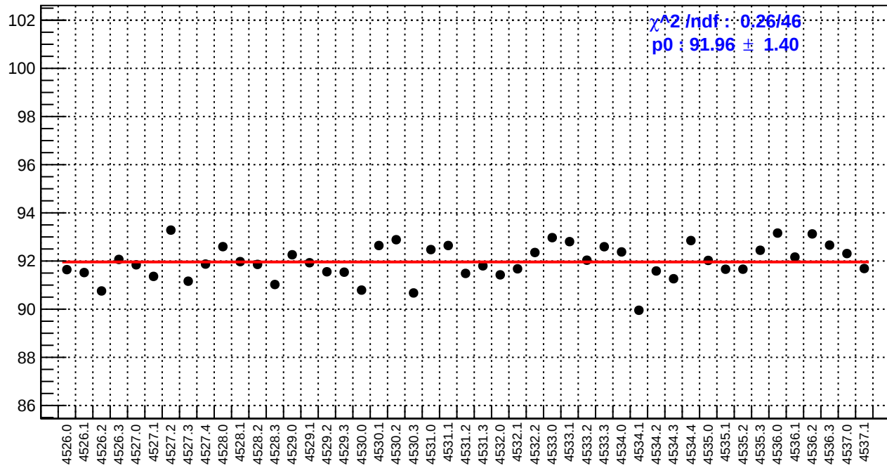
slug65: reg_asym_us_dd.rms/ppm
