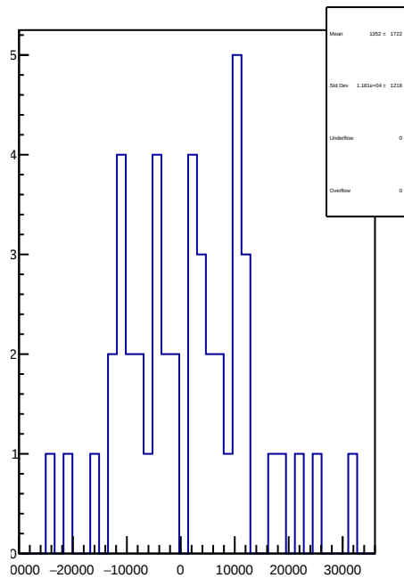
slug65: 1D Corr asym_atl_dd.mean/ppb-reg_asym_atl_dd.mean/ppb
