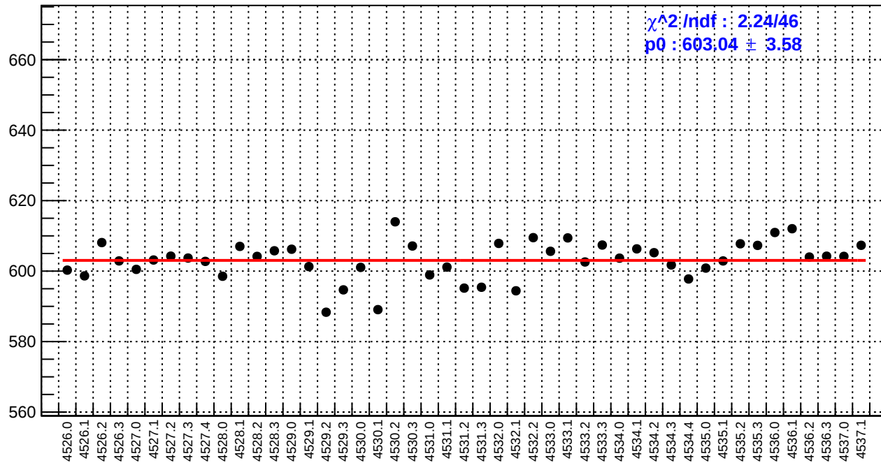
slug65: reg_asym_atl1.rms/ppm
