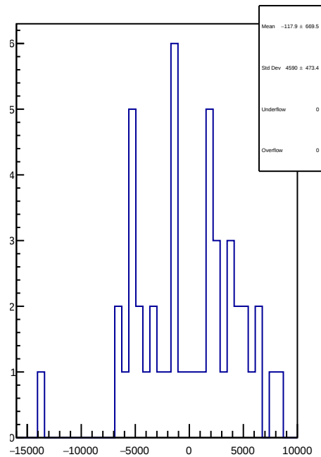
slug65: 1D Corr asym_right_avg.mean/ppb-reg_asym_right_avg.mean/ppb
