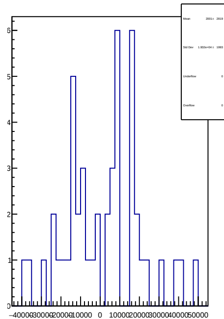
slug65: 1D Corr asym_sam7.mean/ppb-reg_asym_sam7.mean/ppb
