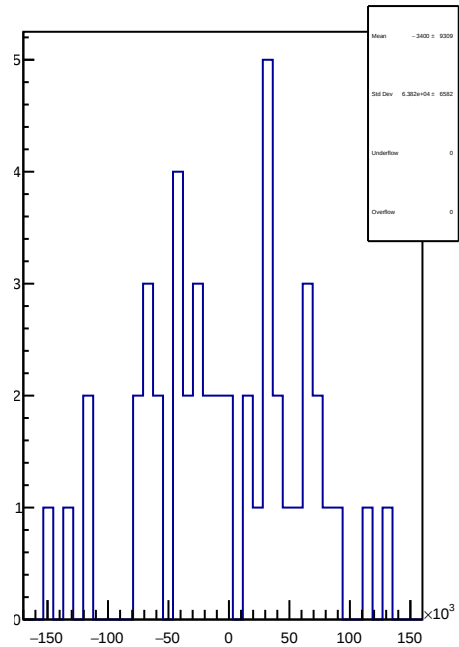
slug65: 1D Corr asym_sam4.mean/ppb-reg_asym_sam4.mean/ppb
