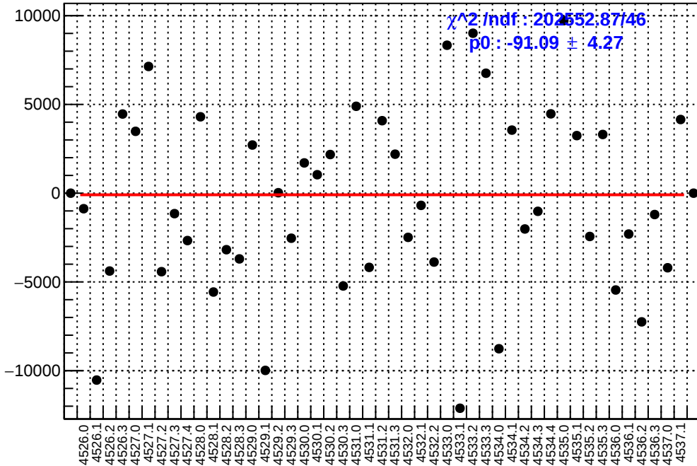
slug65: asym_ds_dd.mean/ppb-reg_asym_ds_dd.mean/ppb
