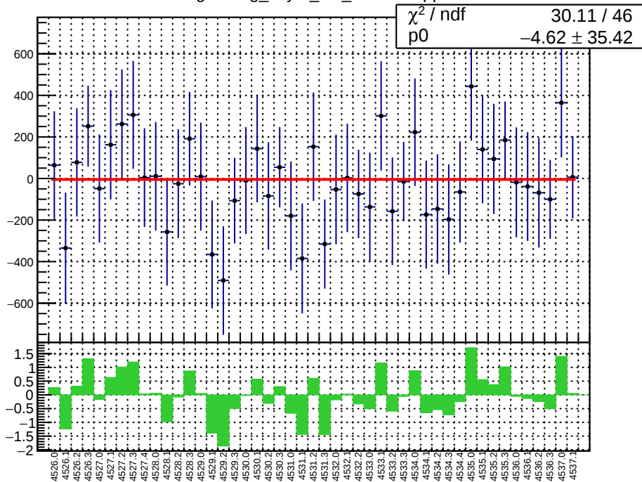
slug65: reg_asym_left_dd.mean/ppb
