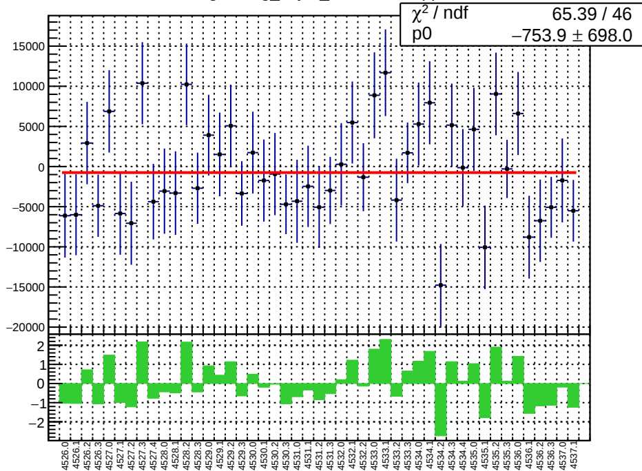
slug65: reg_asym_sam8.mean/ppb
