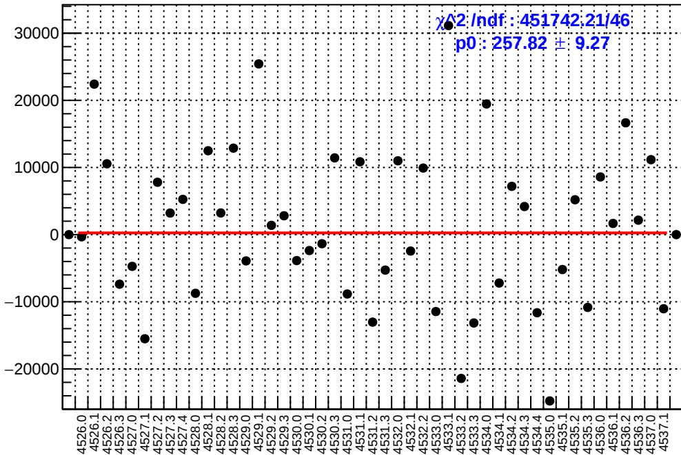
slug65: asym_atl_dd.mean/ppb-reg_asym_atl_dd.mean/ppb
