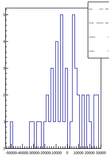
slug65: 1D Corr asym_atl1.mean/ppb-reg_asym_atl1.mean/ppb
