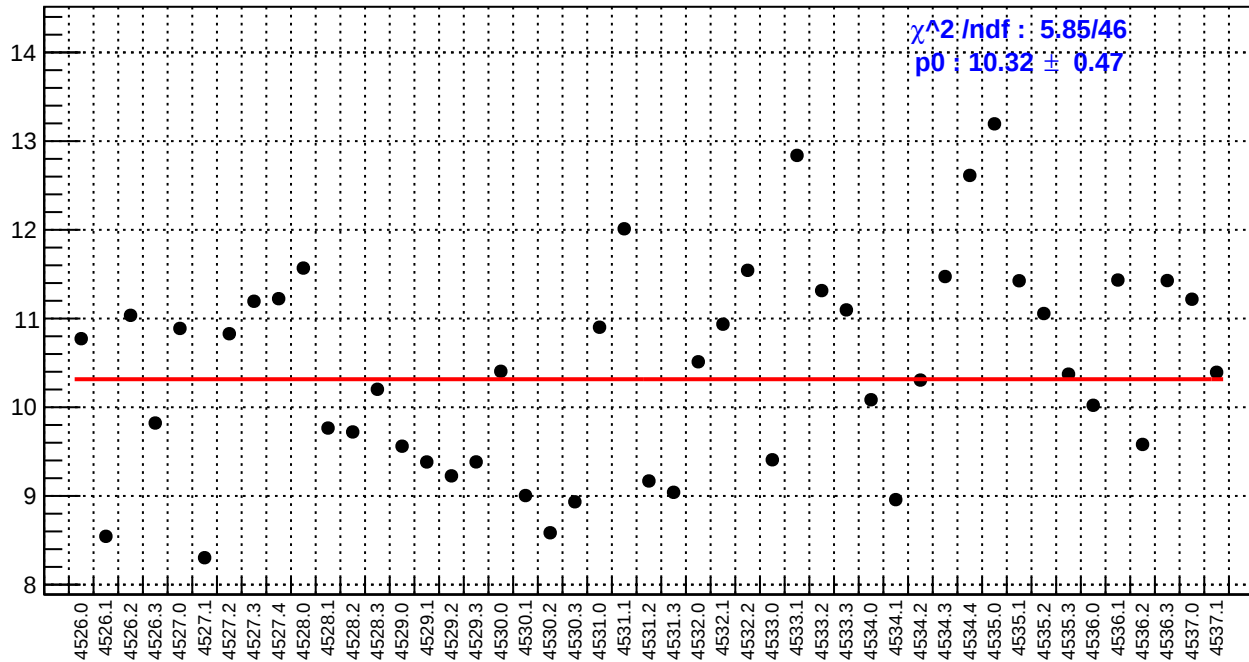
slug65: us_avg_bpm4aY/(ppb/nm)
