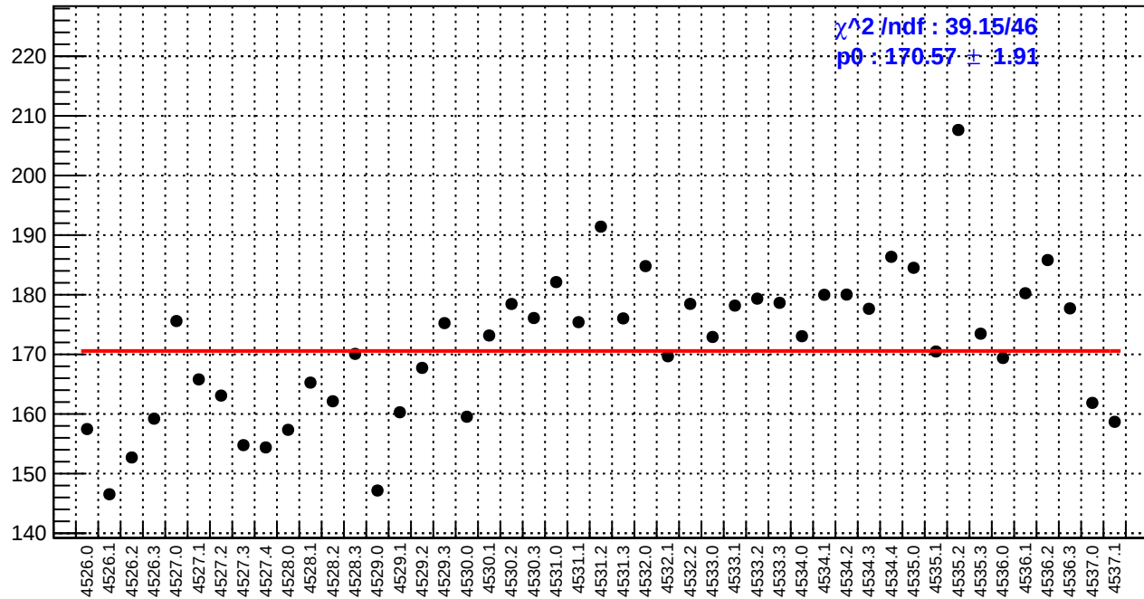
slug65: asym_bcm_an_ds.rms/ppm
