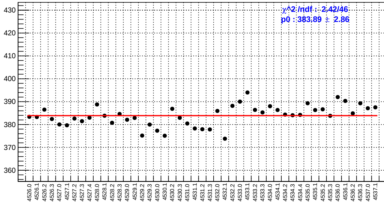
slug65: reg_asym_atl_avg.rms/ppm
