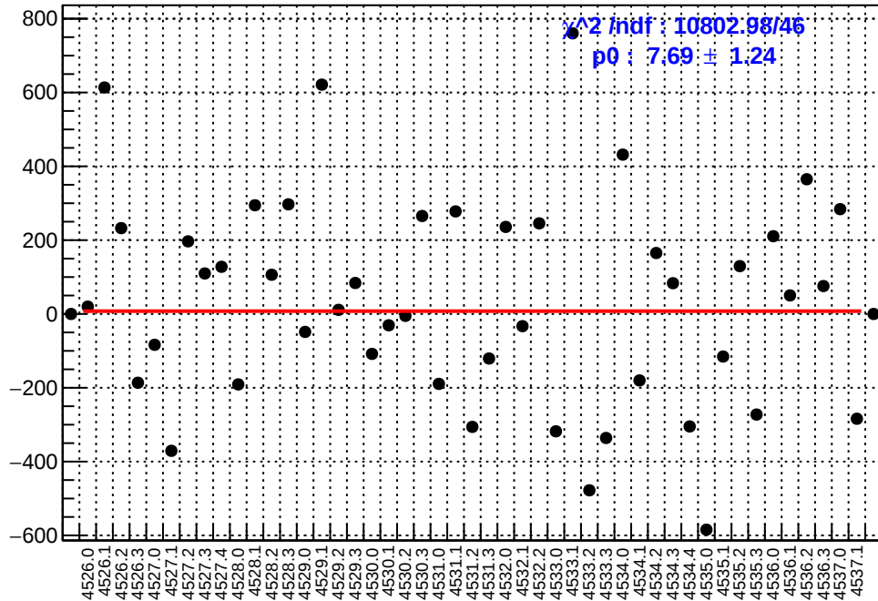
slug65: asym_left_dd.mean/ppb-reg_asym_left_dd.mean/ppb
