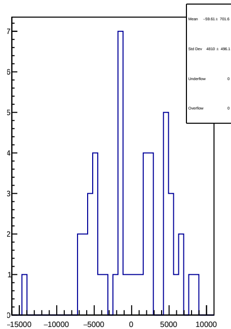
slug65: 1D Corr asym_usr.mean/ppb-reg_asym_usr.mean/ppb
