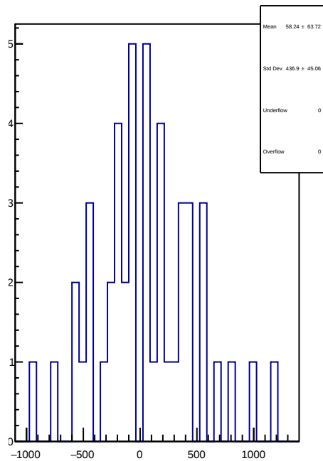
slug65: 1D Corr asym_right_dd.mean/ppb-reg_asym_right_dd.mean/ppb
