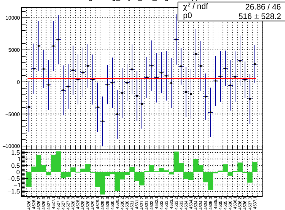
slug65: reg_asym_at1_avg.mean/ppb
