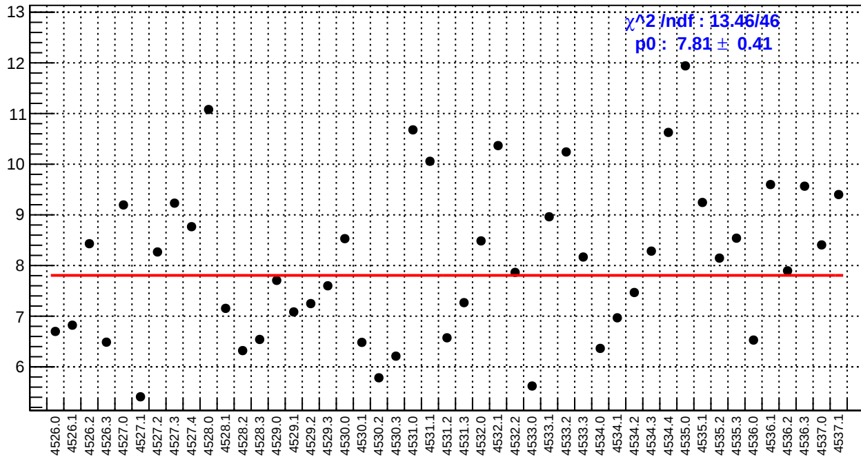
slug65: usl_bpm4aY/(ppb/nm)
