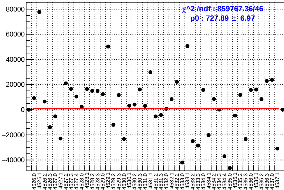
slug65: asym_sam6.mean/ppb-reg_asym_sam6.mean/ppb
