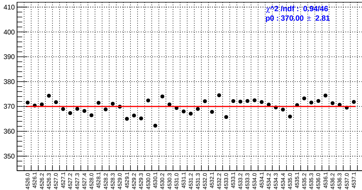
slug65: reg_asym_at1_avg.rms/ppm
