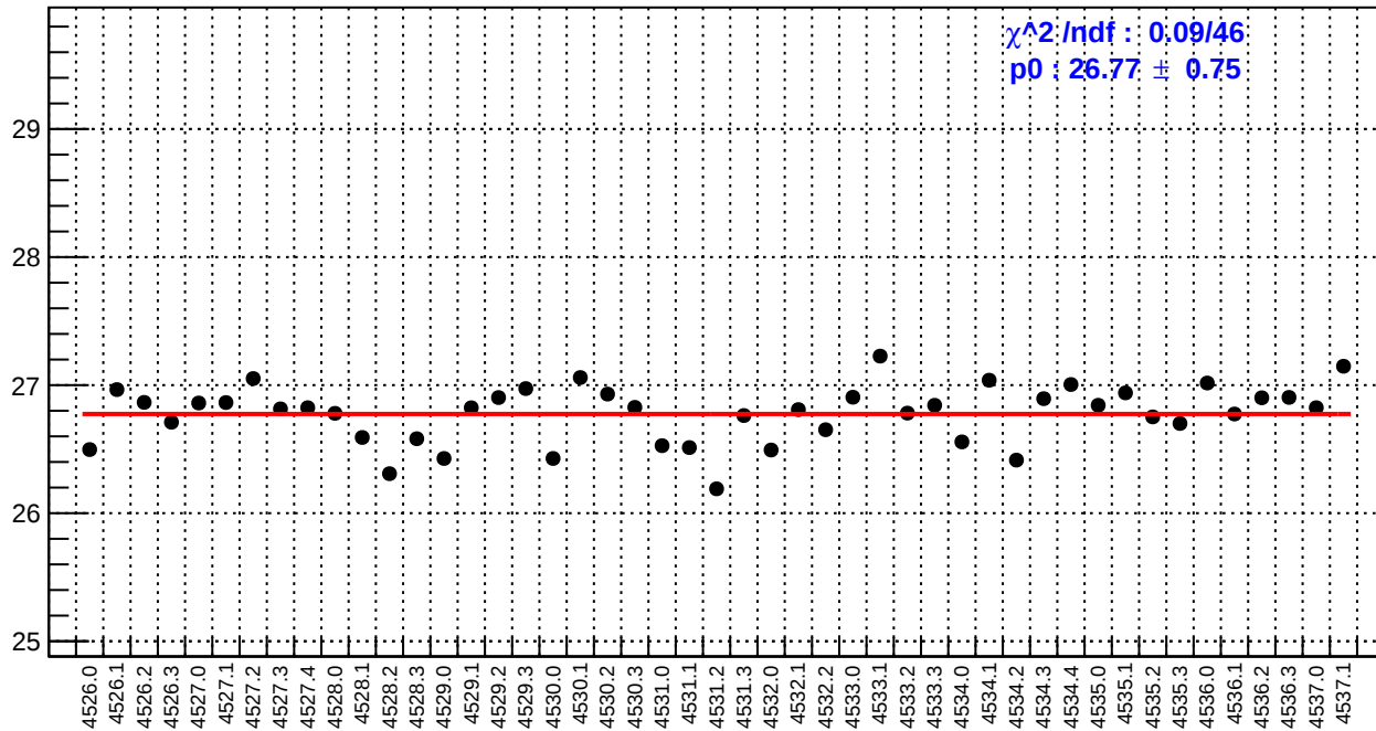
slug65: reg_asym_right_dd.rms/ppm
