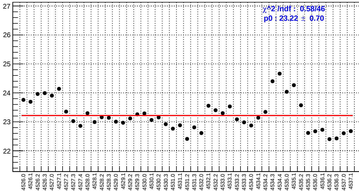
slug65: right_avg_bpm4eX/(ppb/nm)
