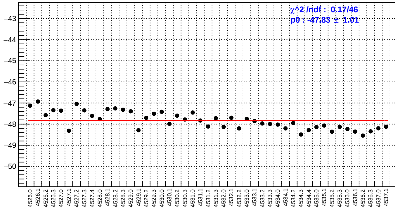
slug65: left_avg_bpm12X/(ppb/nm)
