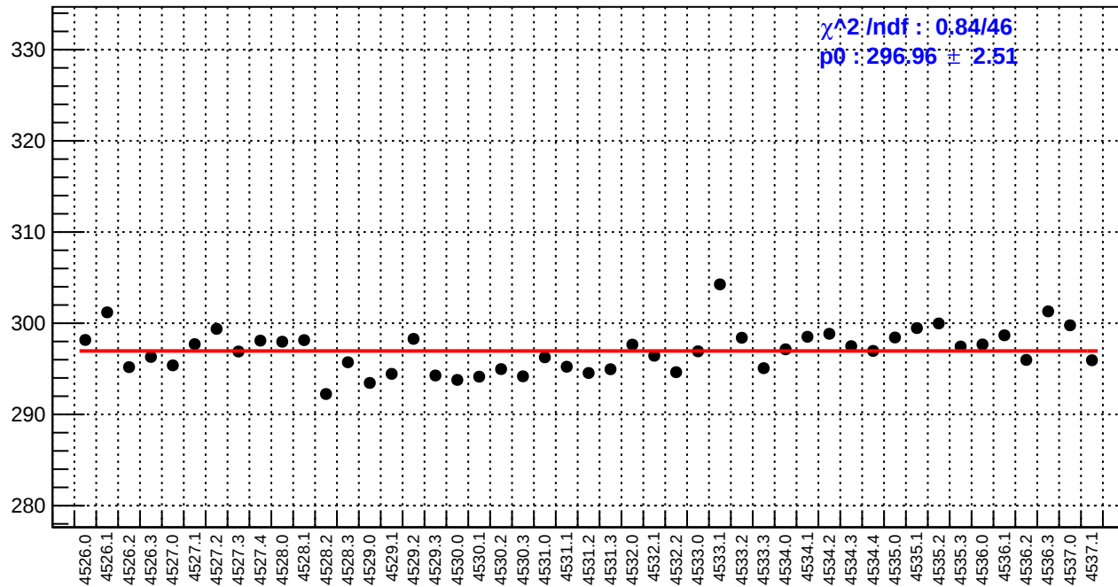
slug65: reg_asym_atr1l2_dd.rms/ppm
