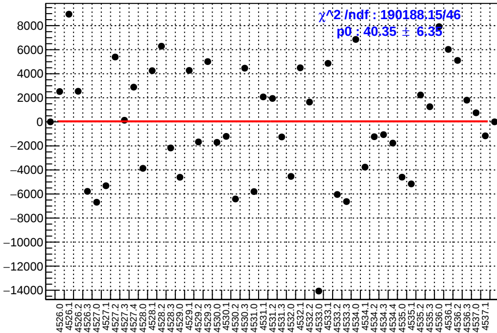
slug65: asym_usr.mean/ppb-reg_asym_usr.mean/ppb
