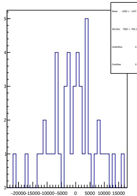
slug65: 1D Corr asym_left_avg.mean/ppb-reg_asym_left_avg.mean/ppb
