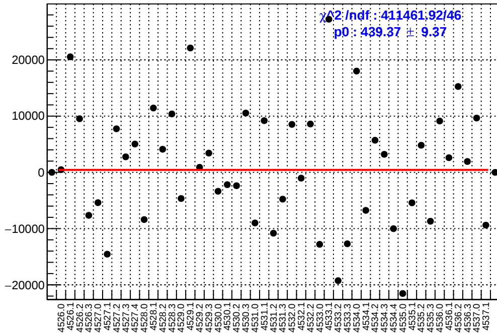
slug65: asym_at2_dd.mean/ppb-reg_asym_at2_dd.mean/ppb
