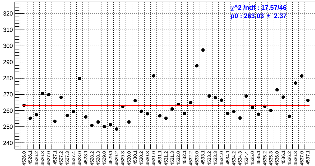
slug65: reg_asym_sam1.rms/ppm
