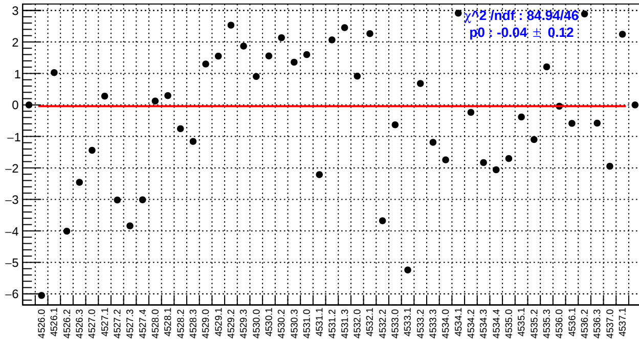
slug65: right_avg_bpm4eY/(ppb/nm)
