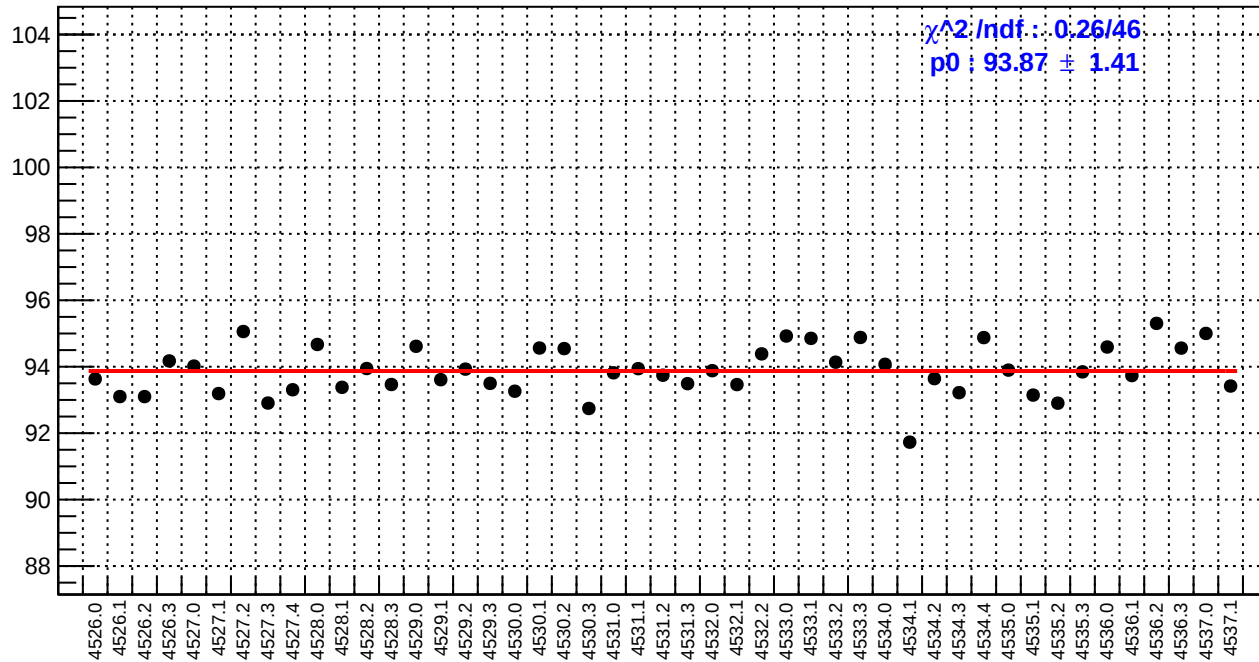
slug65: reg_asym_ds_dd.rms/ppm
