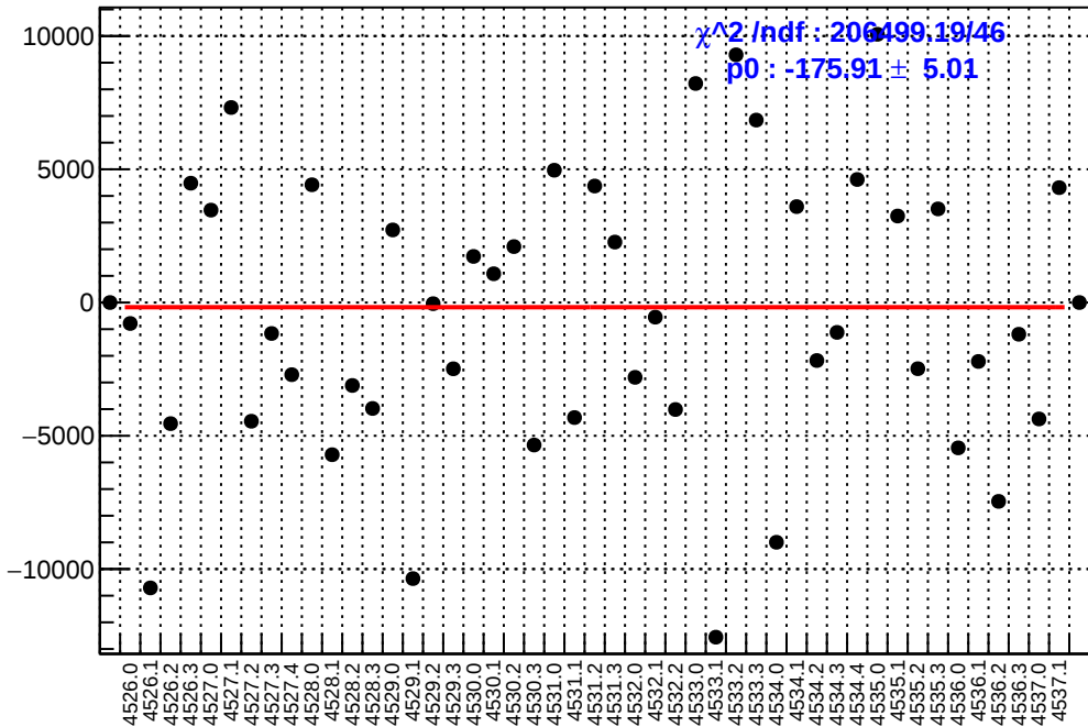
slug65: asym_us_dd.mean/ppb-reg_asym_us_dd.mean/ppb
