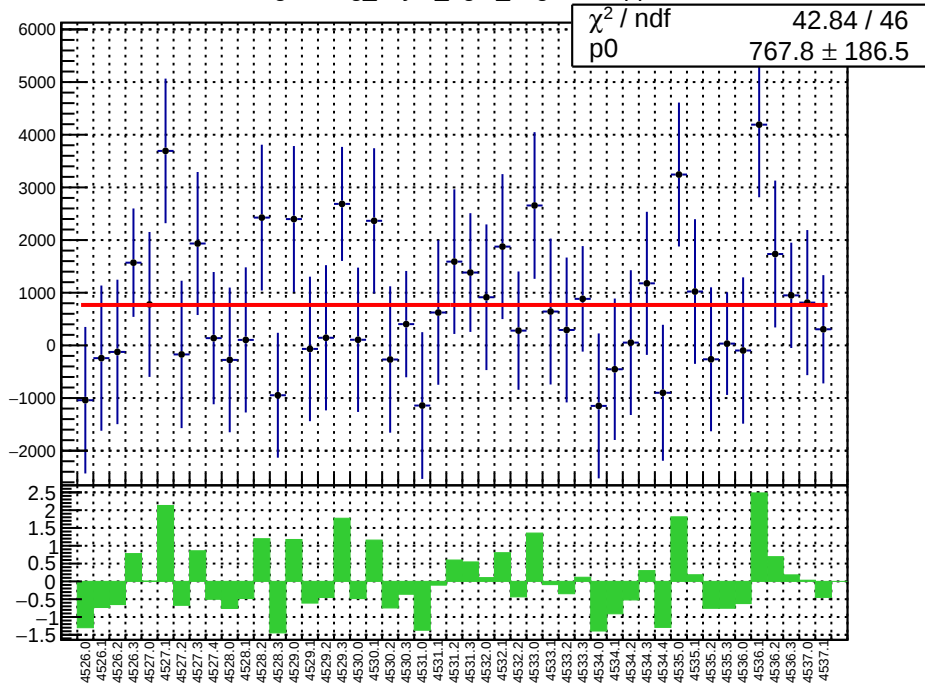
slug65: reg_asym_right_avg.mean/ppb
