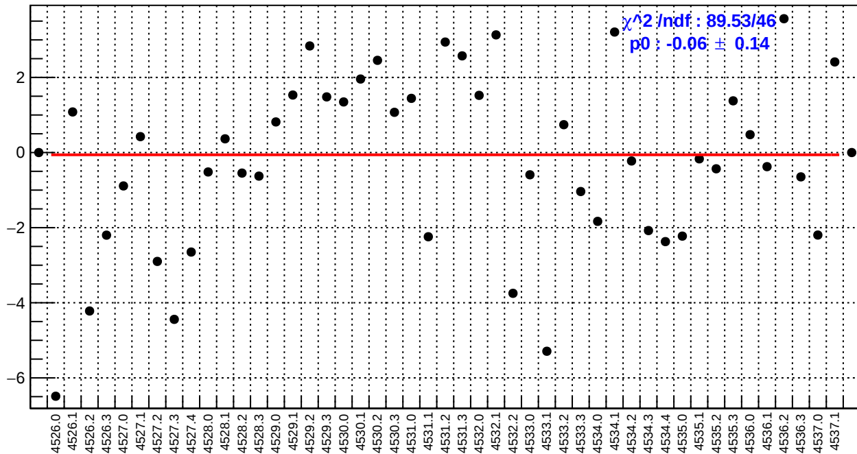
slug65: dsr_bpm4eY/(ppb/nm)
