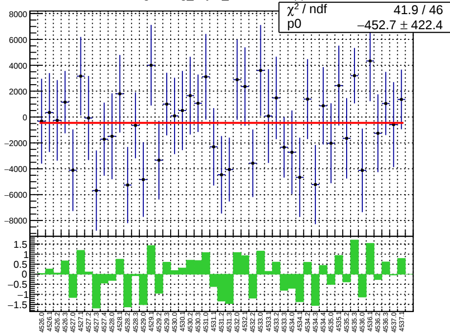
slug65: reg_asym_sam5.mean/ppb
