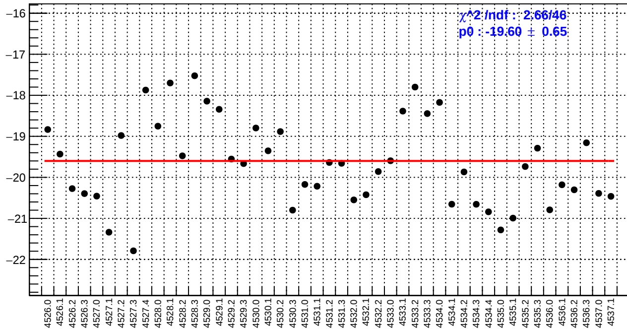
slug65: right_avg_bpm4aX/(ppb/nm)
