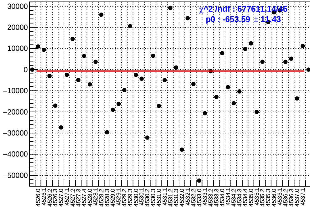
slug65: asym_atr2.mean/ppb-reg_asym_atr2.mean/ppb
