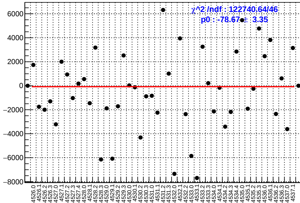
slug65: asym_us_avg.mean/ppb-reg_asym_us_avg.mean/ppb
