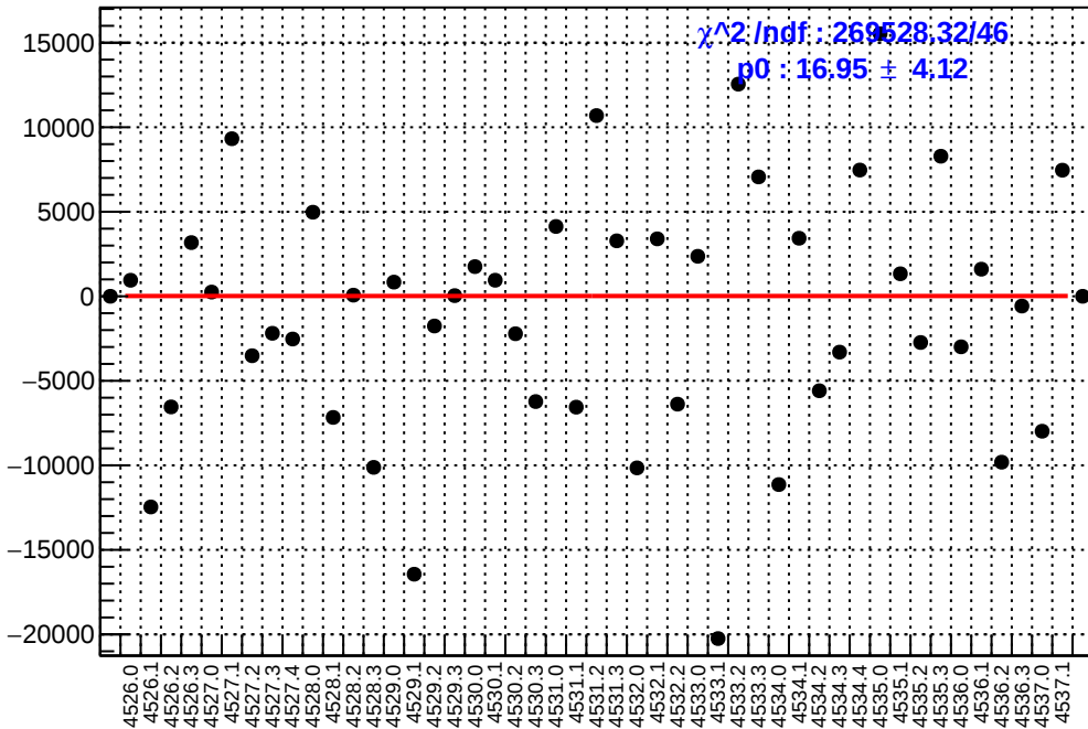
slug65: asym_usl.mean/ppb-reg_asym_usl.mean/ppb
