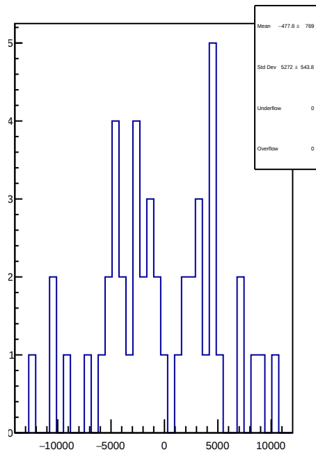
slug65: 1D Corr asym_us_dd.mean/ppb-reg_asym_us_dd.mean/ppb
