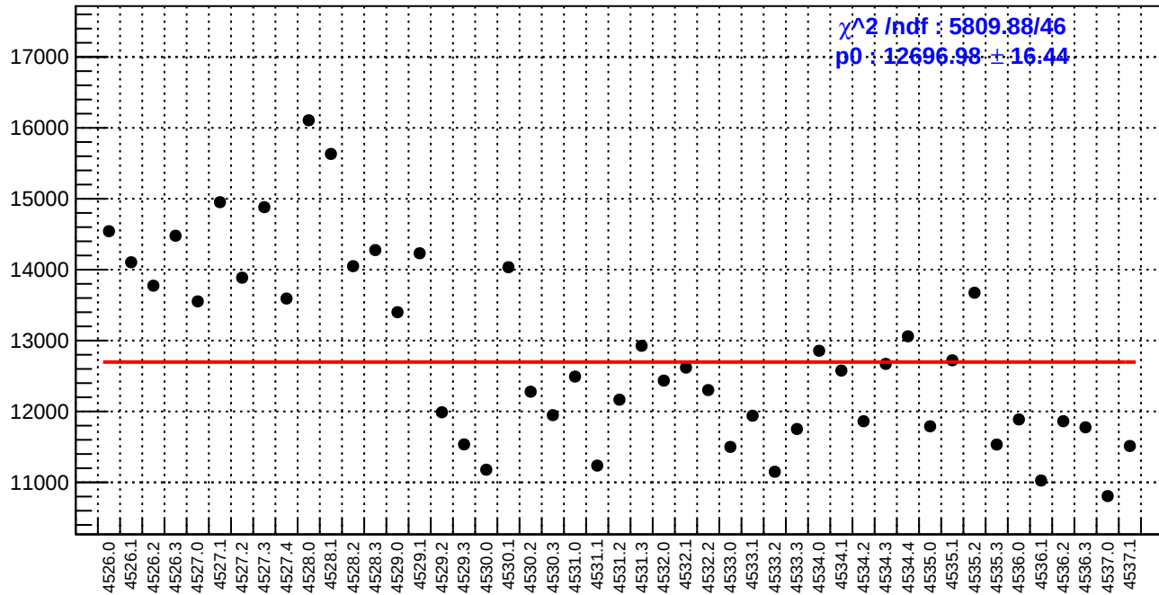
slug65: diff_bpm4eX.rms/nm
