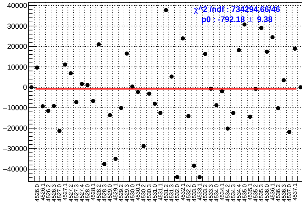
slug65: asym_atl_avg.mean/ppb-reg_asym_atl_avg.mean/ppb
