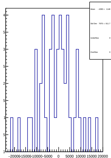
slug65: 1D Corr asym_dsl.mean/ppb-reg_asym_dsl.mean/ppb
