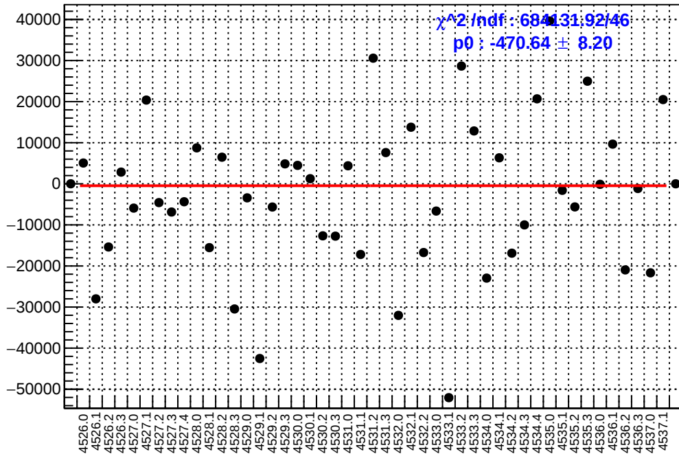
slug65: asym_atr1l2_avg.mean/ppb-reg_asym_atr1l2_avg.mean/ppb
