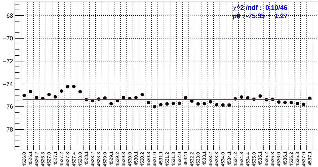
slug65: dsl_bpm4eX/(ppb/nm)
