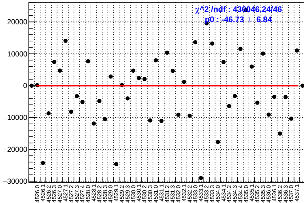
slug65: asym_atr1.mean/ppb-reg_asym_atr1.mean/ppb
