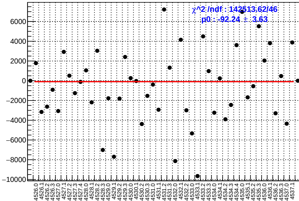
slug65: asym_ds_avg.mean/ppb-reg_asym_ds_avg.mean/ppb
