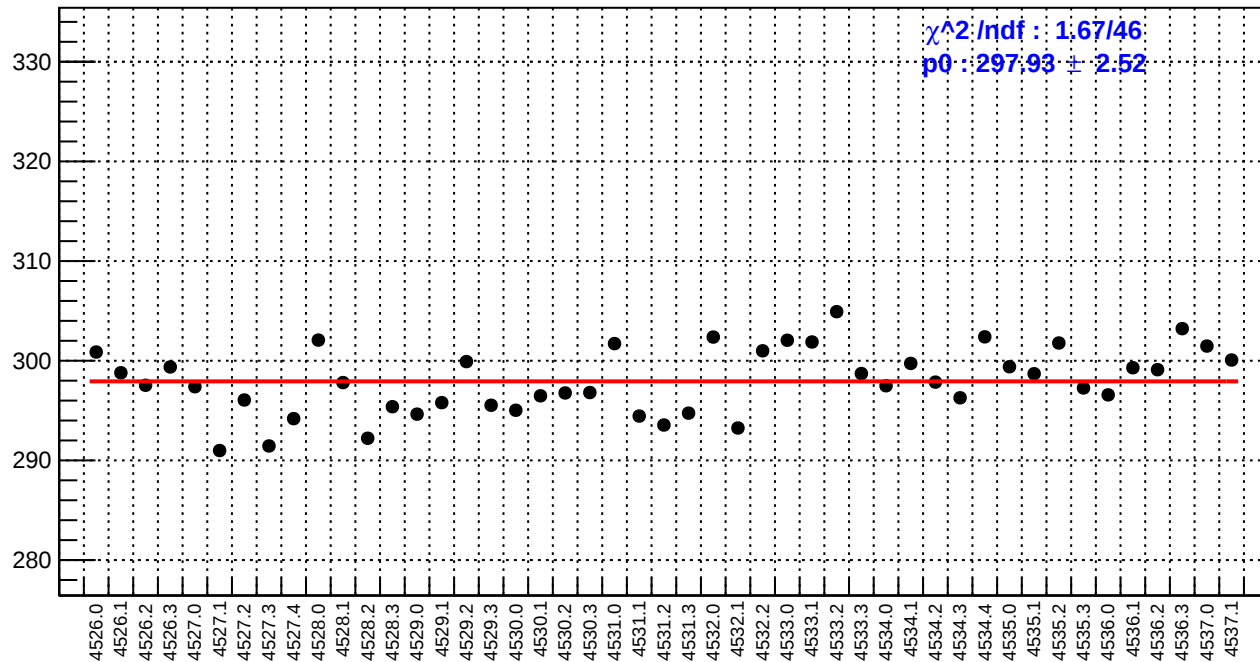
slug65: reg_asym_atr1l2_avg.rms/ppm
