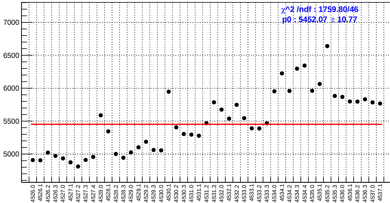
slug65: diff_bpm11X.rms/nm
