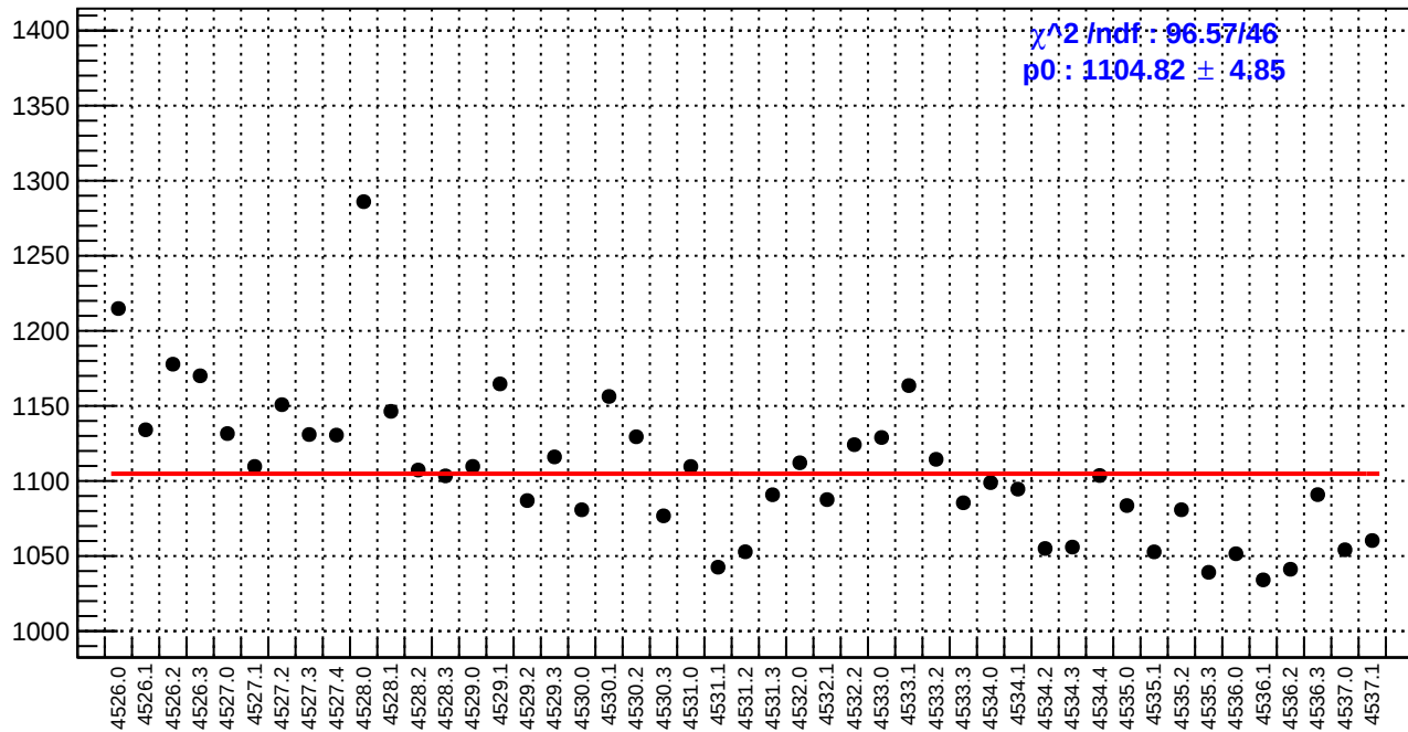
slug65: reg_asym_sam3.rms/ppm
