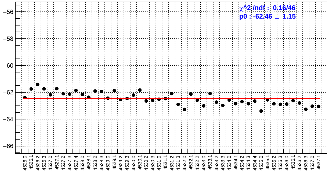
slug65: right_avg_bpm12X/(ppb/nm)
