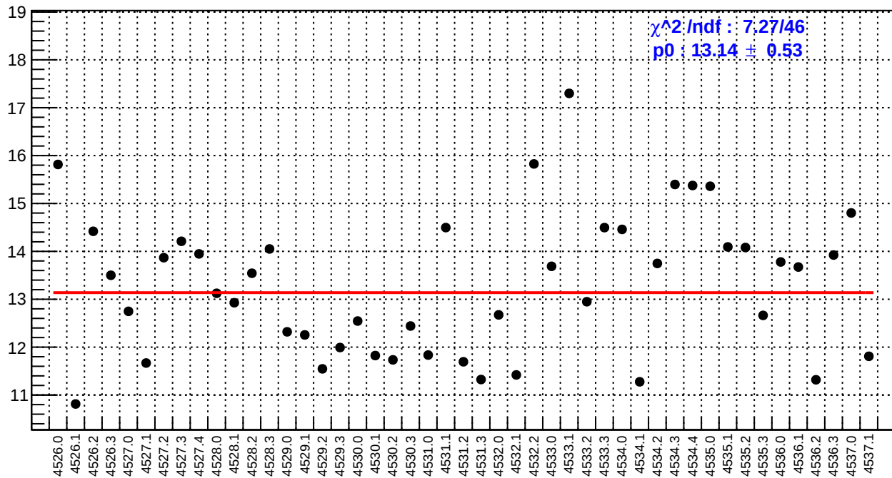
slug65: right_avg_bpm4aY/(ppb/nm)
