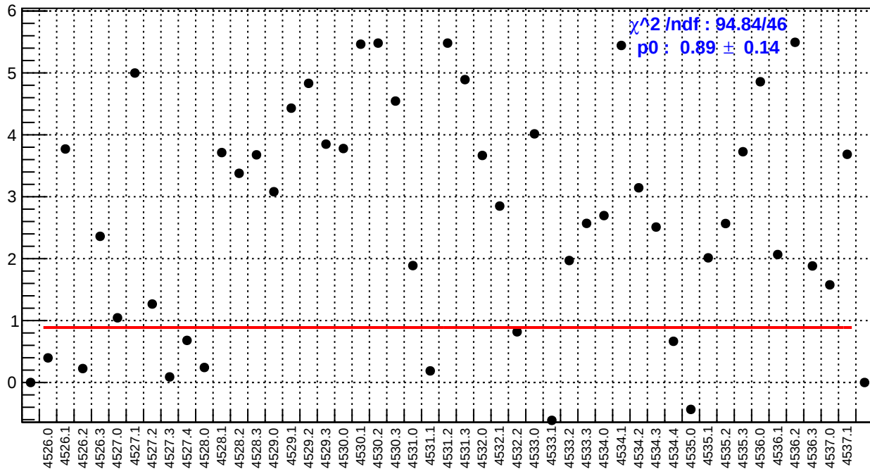
slug65: ds_avg_bpm4eY/(ppb/nm)
