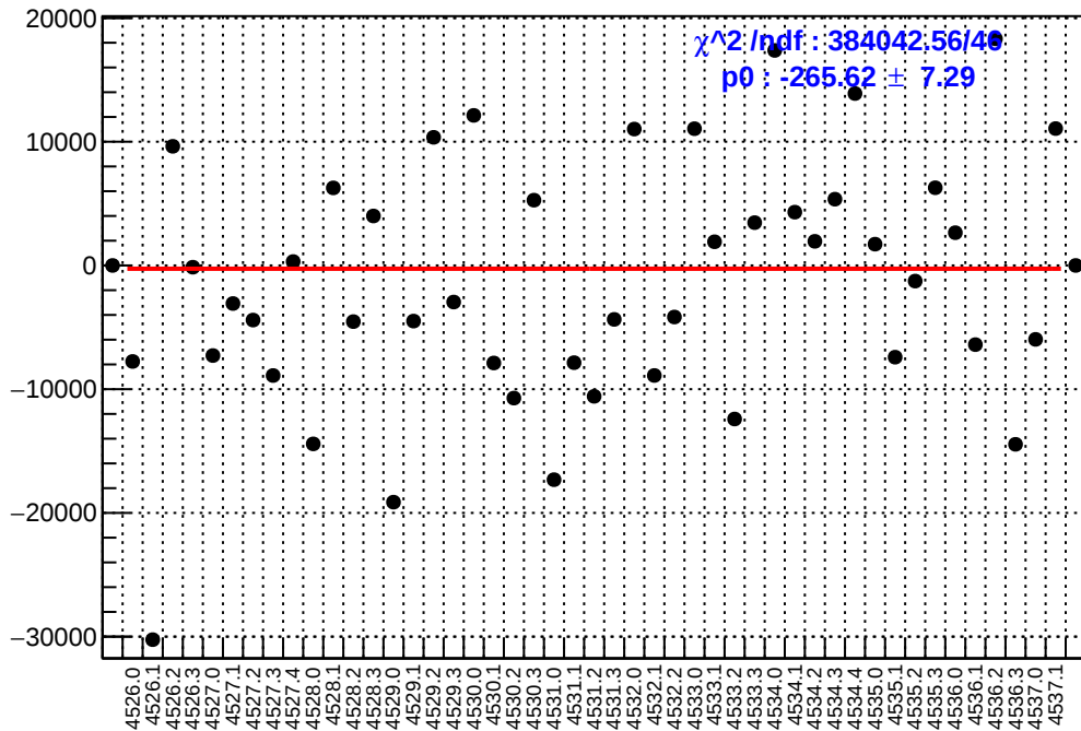
slug65: asym_sam1.mean/ppb-reg_asym_sam1.mean/ppb
