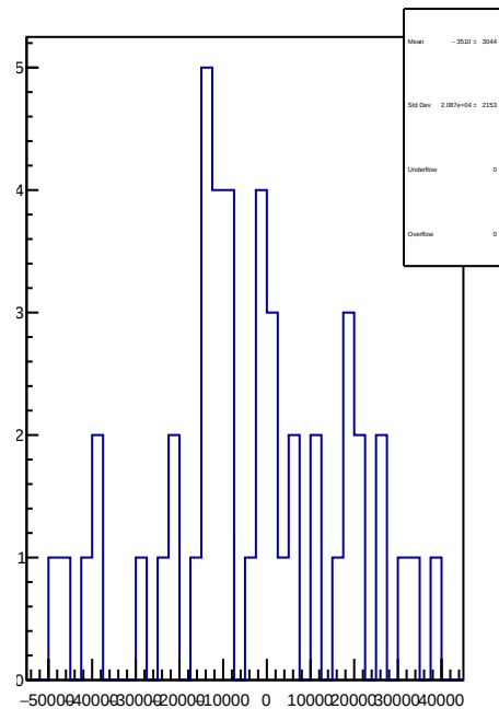
slug65: 1D Corr asym_at2_avg.mean/ppb-reg_asym_at2_avg.mean/ppb
