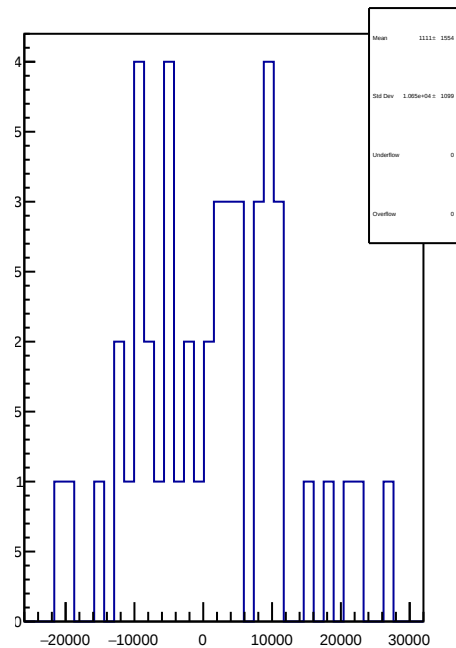
slug65: 1D Corr asym_at2_dd.mean/ppb-reg_asym_at2_dd.mean/ppb
