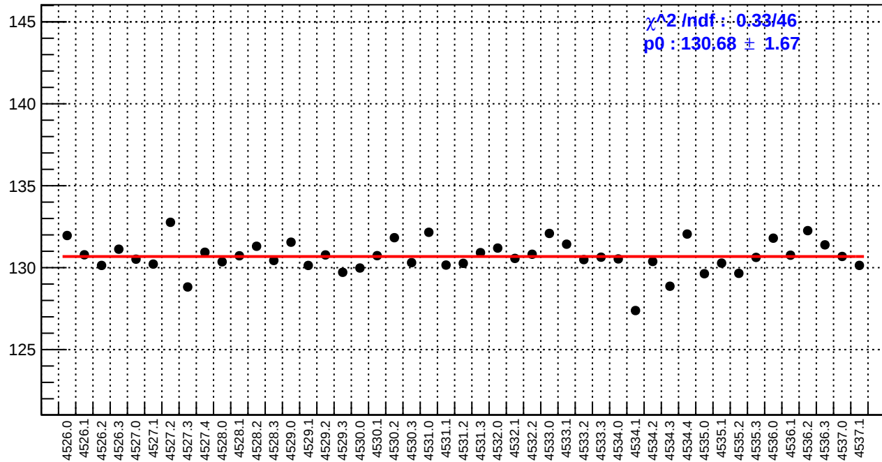
slug65: reg_asym_right_avg.rms/ppm
