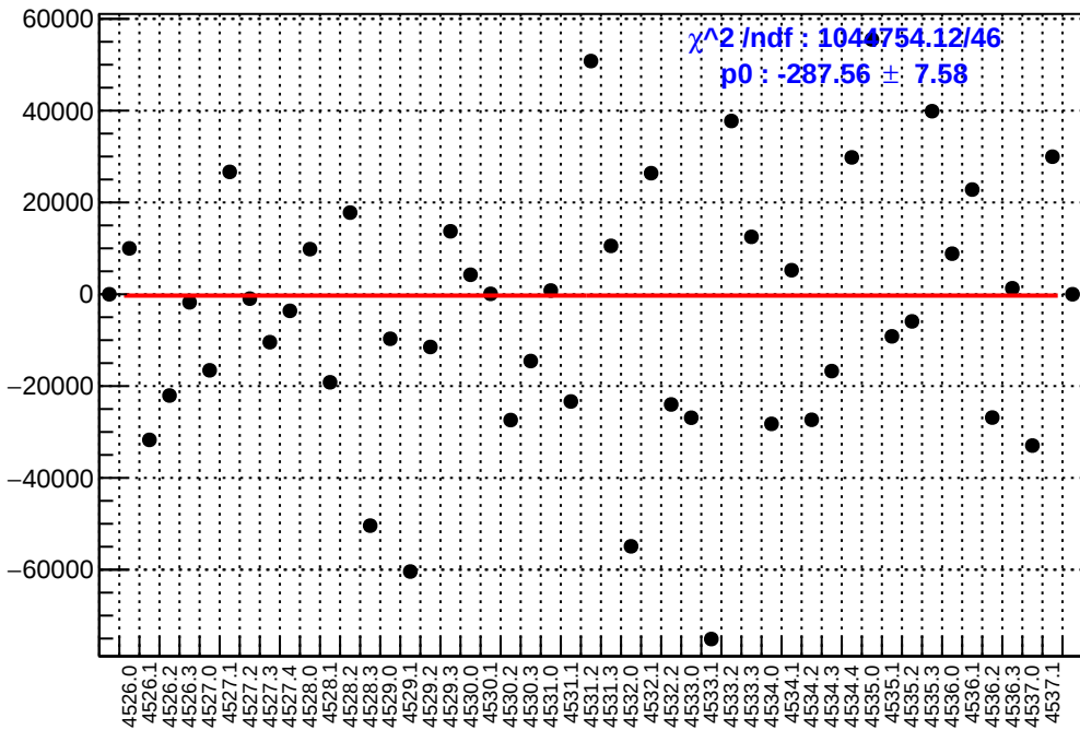
slug65: asym_atl2.mean/ppb-reg_asym_atl2.mean/ppb
