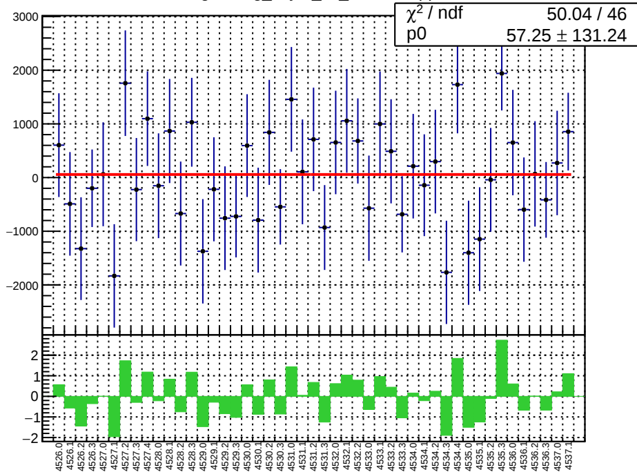
slug65: reg_asym_us_dd.mean/ppb
