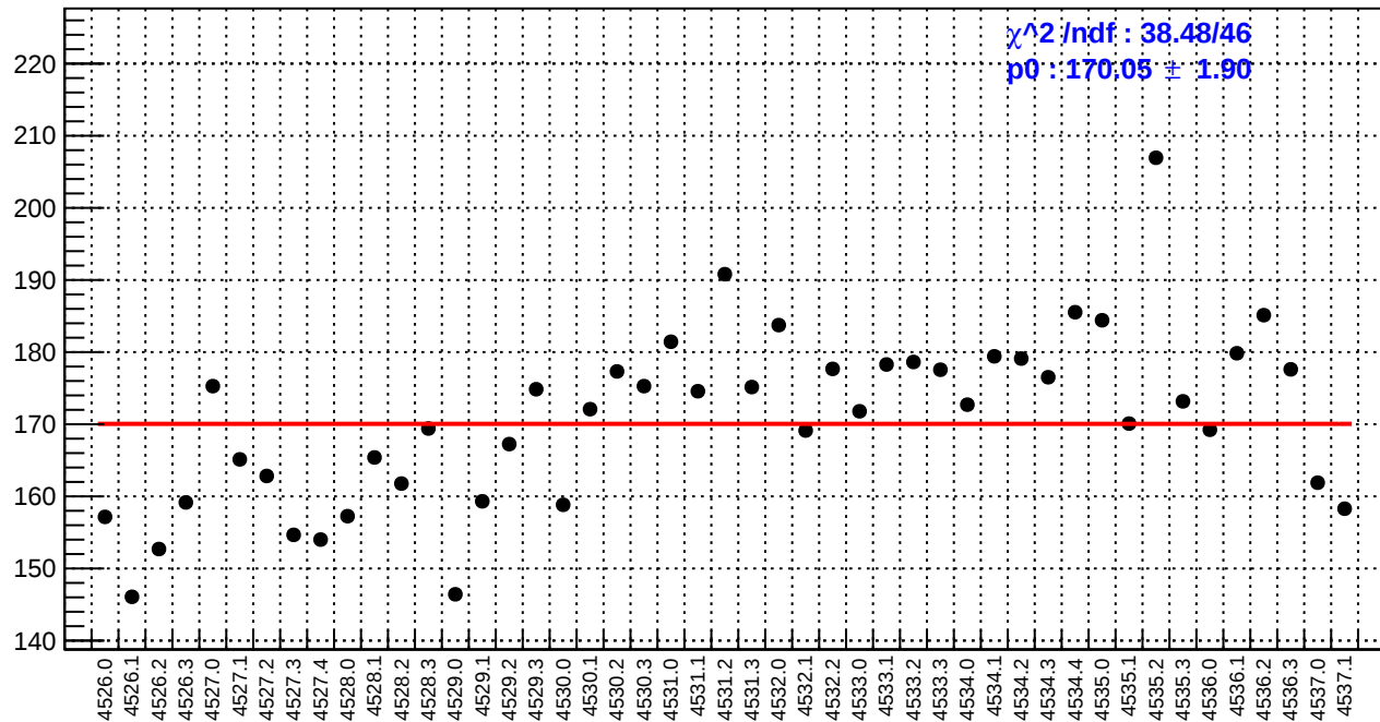
slug65: asym_bcm_an_us.rms/ppm
