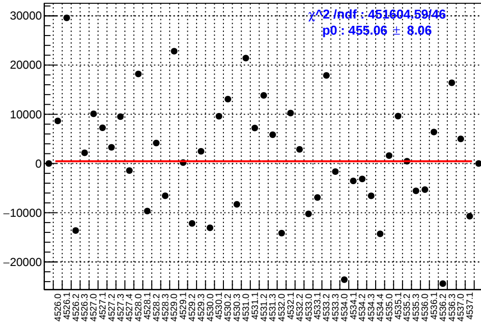
slug65: asym_sam5.mean/ppb-reg_asym_sam5.mean/ppb
