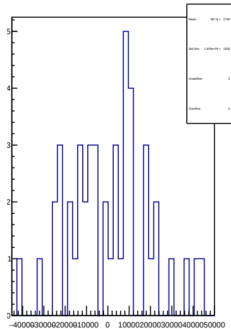
slug65: 1D Corr asym_sam8.mean/ppb-reg_asym_sam8.mean/ppb
