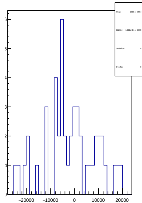
slug65: 1D Corr asym_atr_avg.mean/ppb-reg_asym_atr_avg.mean/ppb
