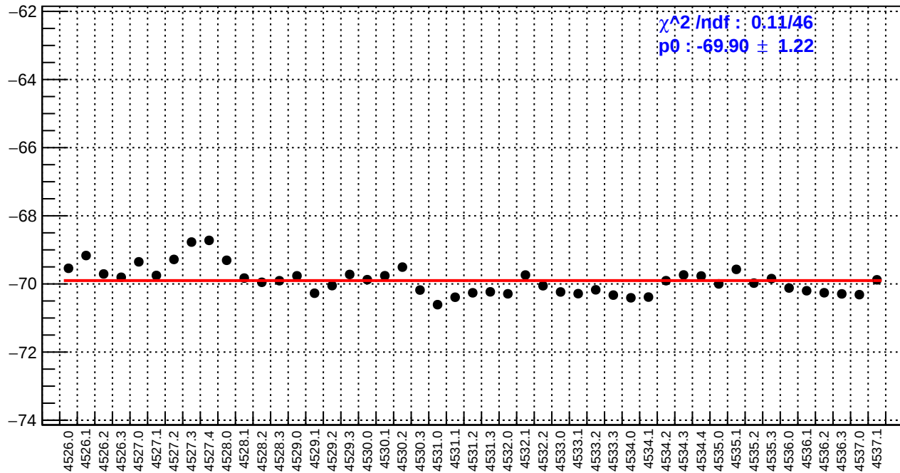
slug65: usl_bpm4eX/(ppb/nm)
