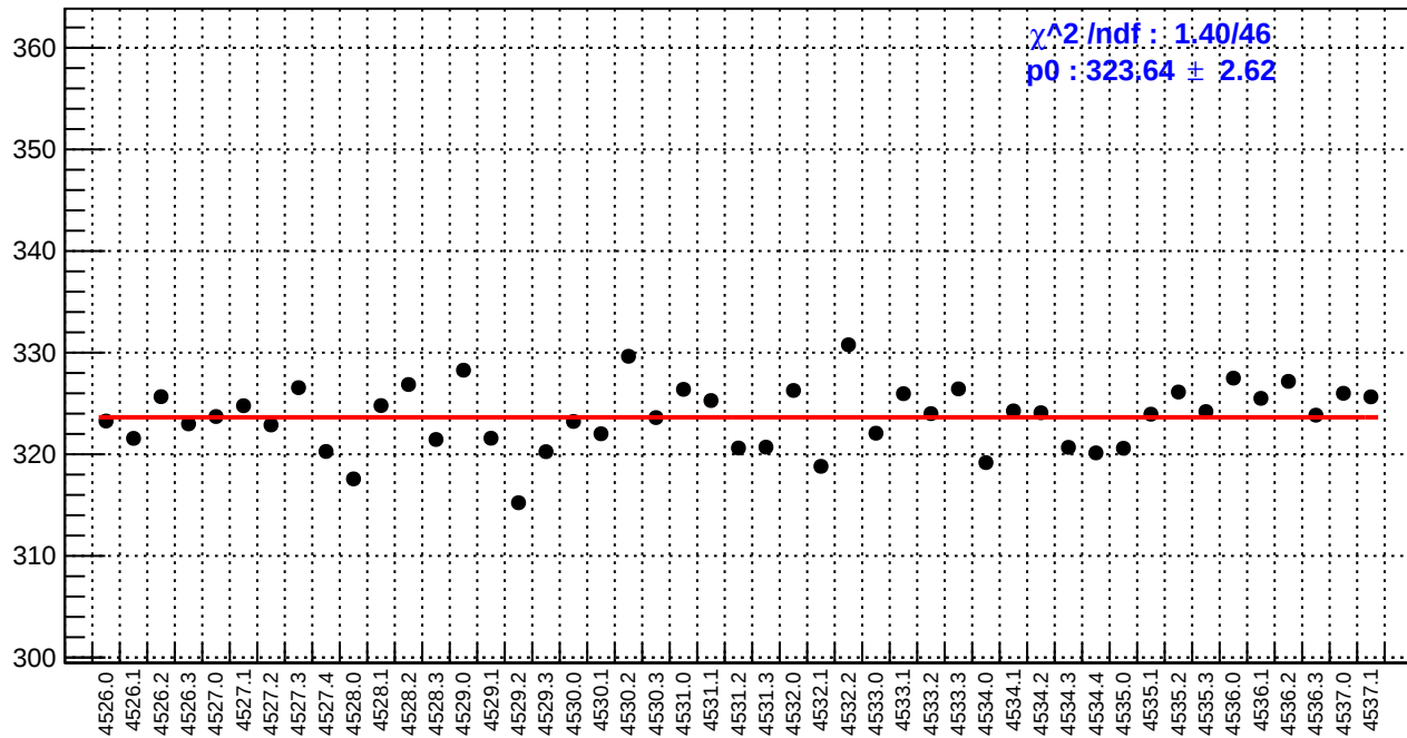
slug65: reg_asym_atl1r2_dd.rms/ppm
