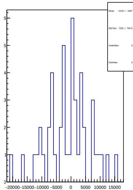
slug65: 1D Corr asym_usl.mean/ppb-reg_asym_usl.mean/ppb
