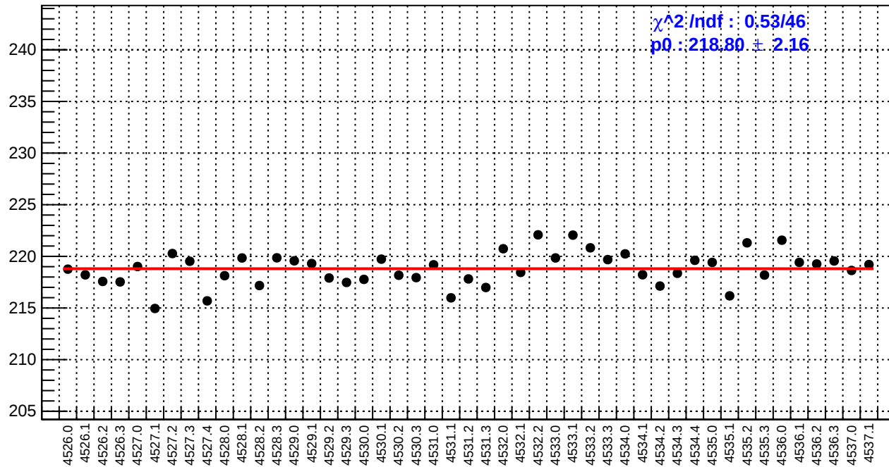
slug65: reg_asym_at2_dd.rms/ppm
