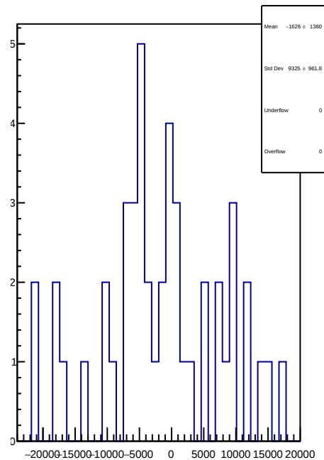
slug65: 1D Corr asym_at1_avg.mean/ppb-reg_asym_at1_avg.mean/ppb
