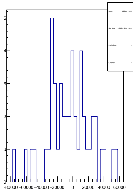
slug65: 1D Corr asym_atl2.mean/ppb-reg_asym_atl2.mean/ppb
