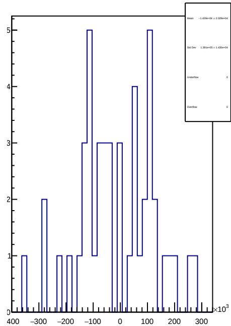
slug65: 1D Corr asym_sam3.mean/ppb-reg_asym_sam3.mean/ppb
