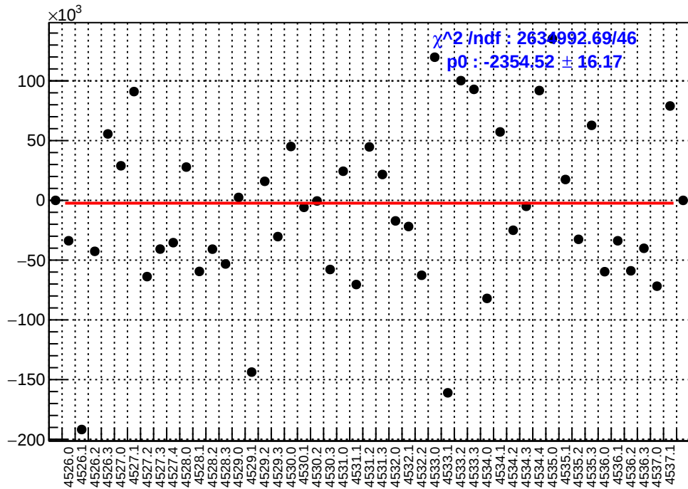
slug65: asym_sam2.mean/ppb-reg_asym_sam2.mean/ppb
