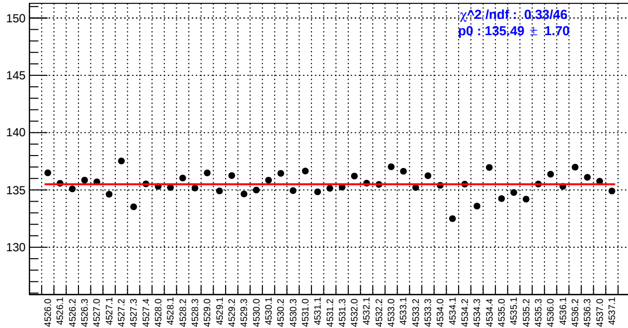
slug65: reg_asym_dsr.rms/ppm
