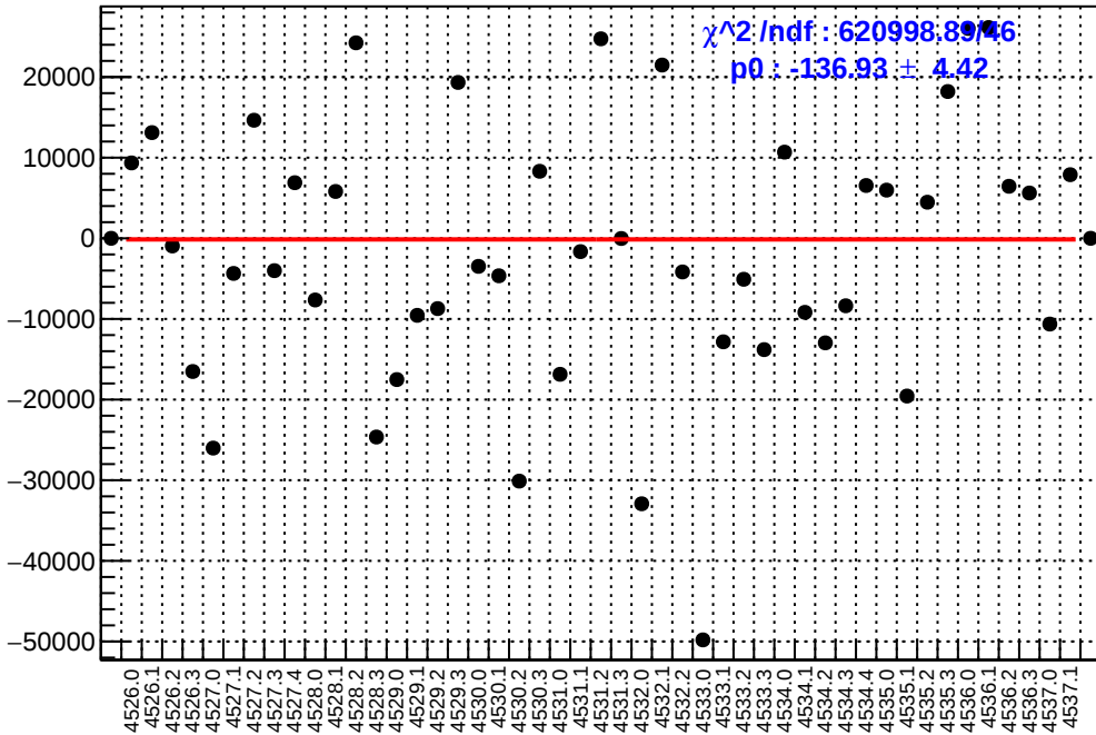
slug65: asym_atl1.mean/ppb-reg_asym_atl1.mean/ppb
