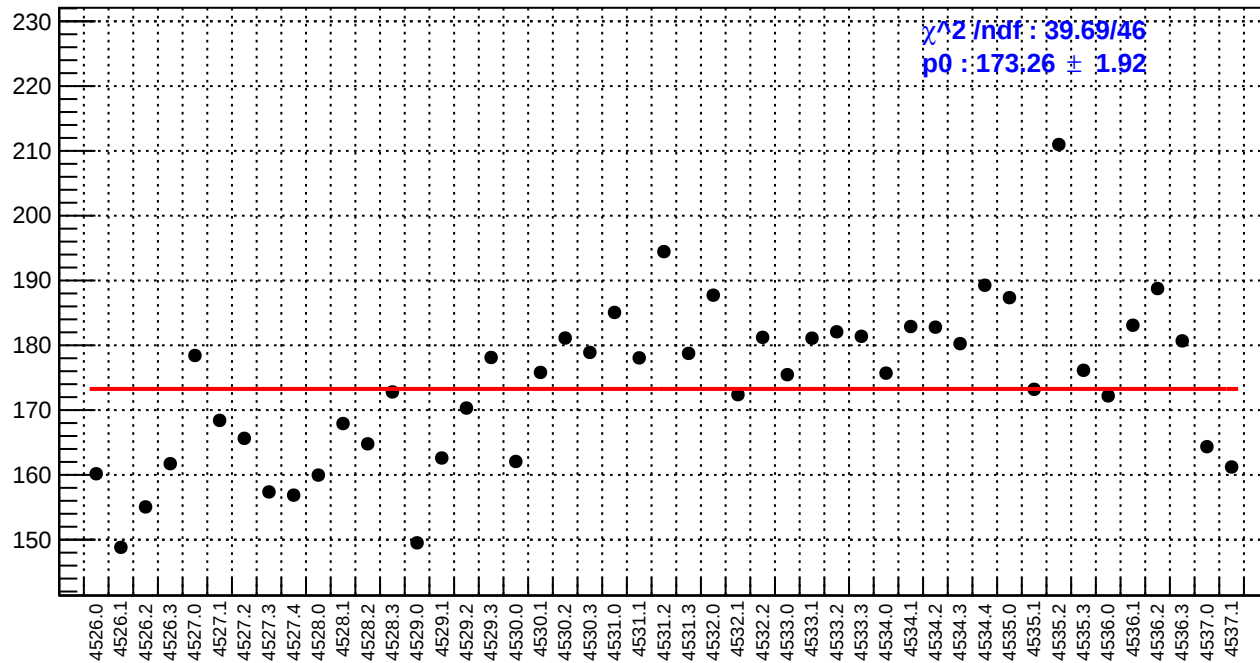
slug65: asym_bcm_an_ds3.rms/ppm
