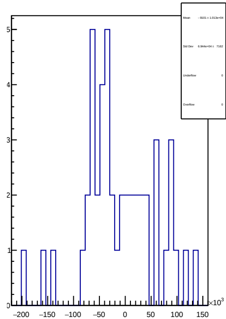
slug65: 1D Corr asym_sam2.mean/ppb-reg_asym_sam2.mean/ppb
