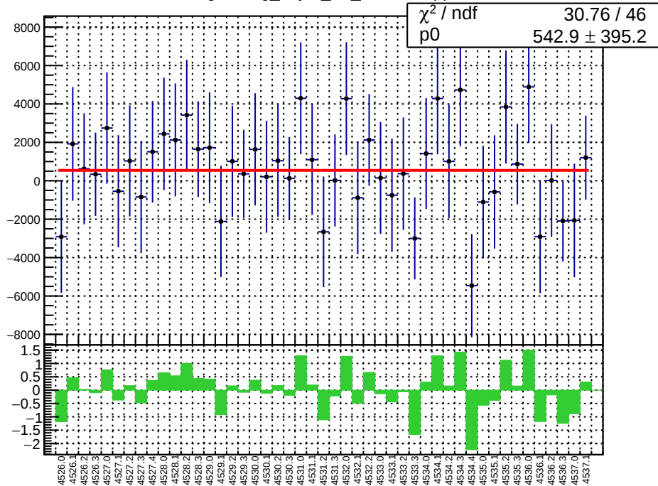
slug65: reg_asym_atr_dd.mean/ppb
