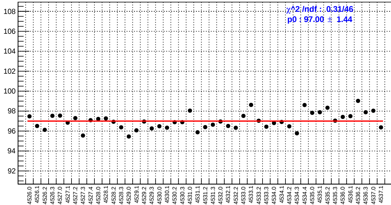
slug65: reg_asym_us_avg.rms/ppm
