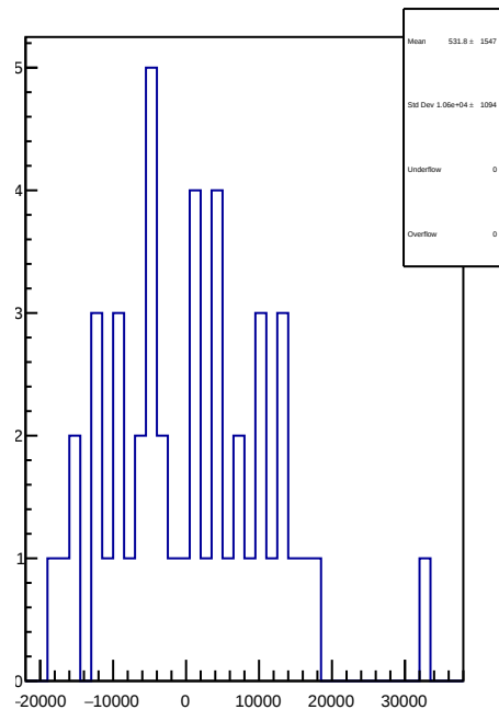
slug65: 1D Corr asym_atr_dd.mean/ppb-reg_asym_atr_dd.mean/ppb
