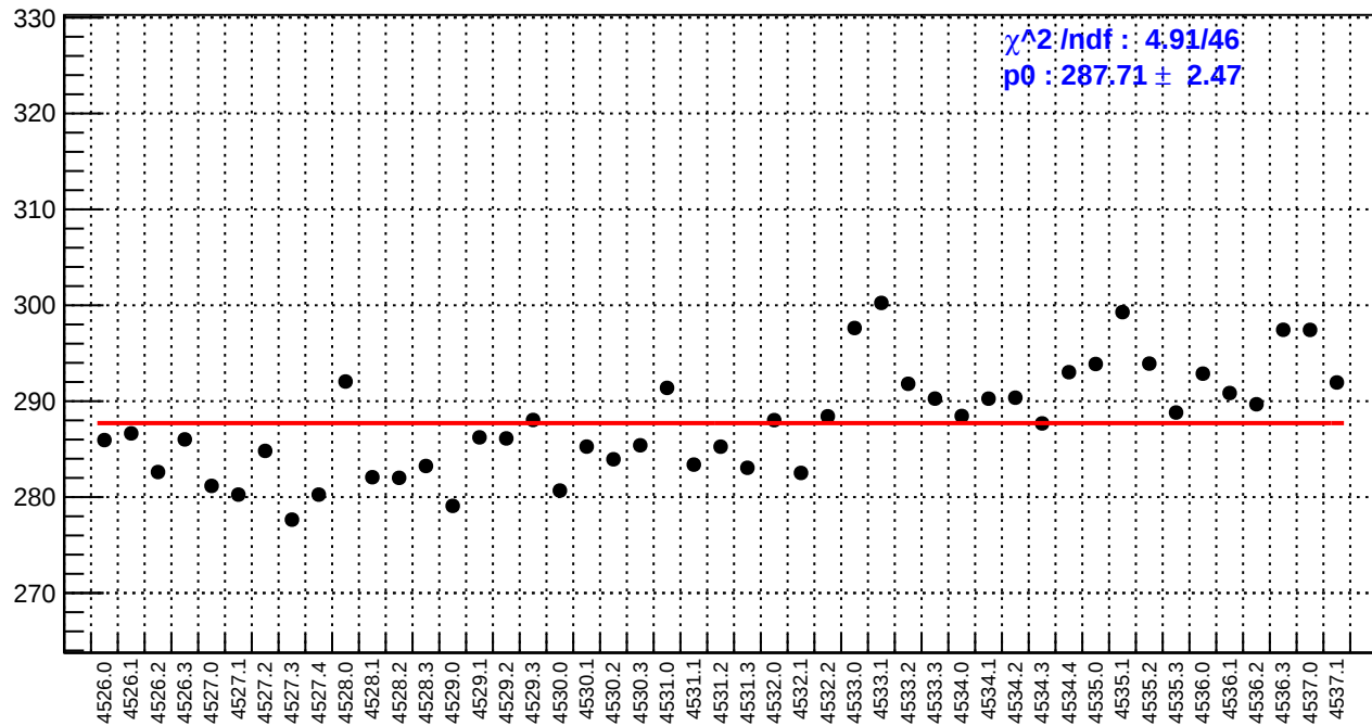
slug65: reg_asym_at2_avg.rms/ppm
