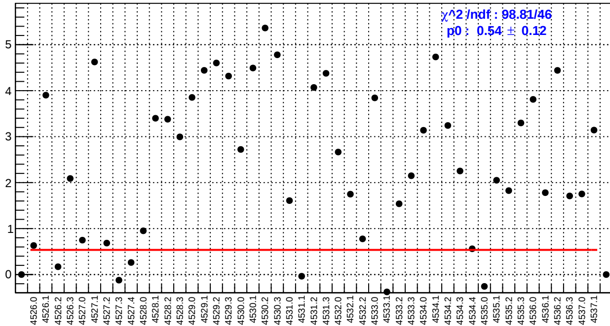
slug65: us_avg_bpm4eY/(ppb/nm)
