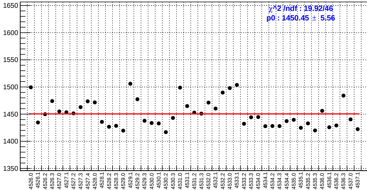
slug65: reg_asym_sam4.rms/ppm
