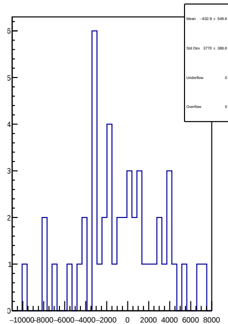
slug65: 1D Corr asym_ds_avg.mean/ppb-reg_asym_ds_avg.mean/ppb
