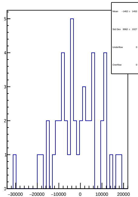
slug65: 1D Corr asym_sam1.mean/ppb-reg_asym_sam1.mean/ppb
