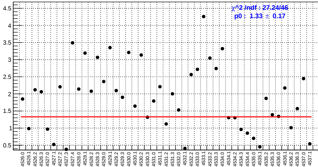
slug65: us_avg_bpm4aX/(ppb/nm)
