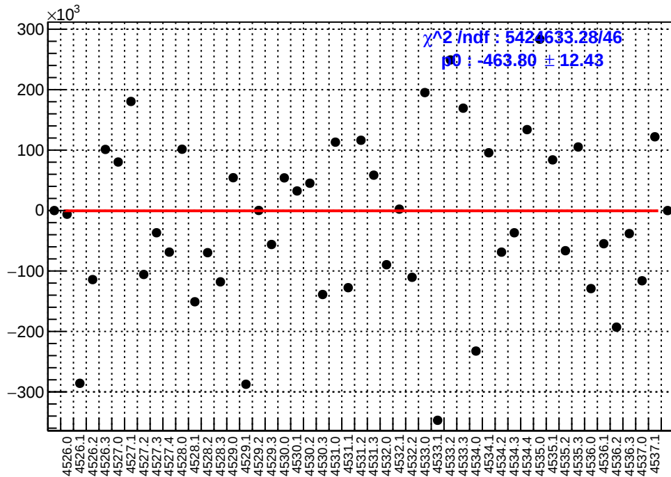
slug65: asym_sam3.mean/ppb-reg_asym_sam3.mean/ppb
