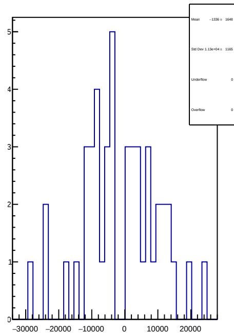
slug65: 1D Corr asym_atr1.mean/ppb-reg_asym_atr1.mean/ppb
