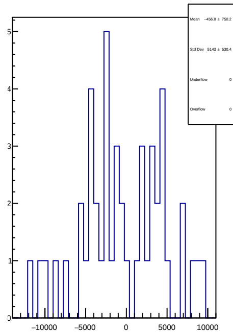
slug65: 1D Corr asym_ds_dd.mean/ppb-reg_asym_ds_dd.mean/ppb
