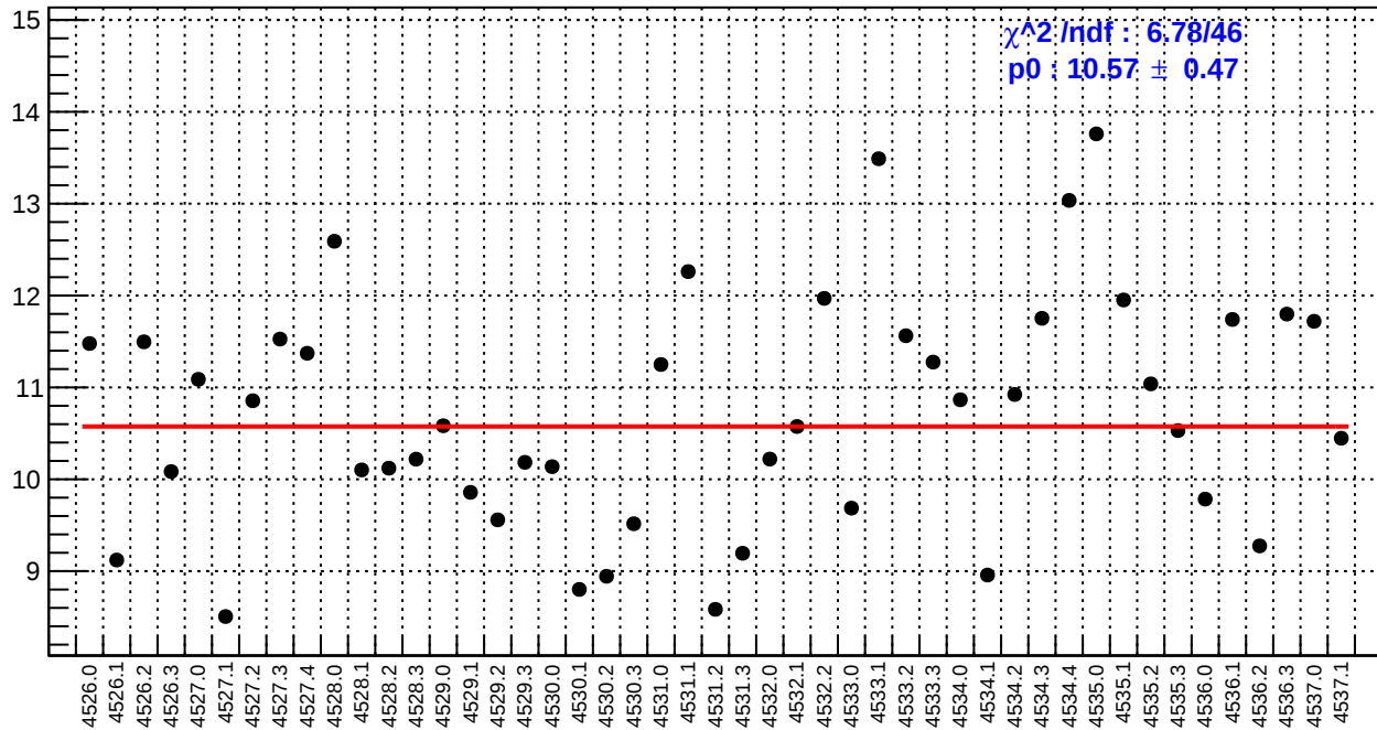
slug65: ds_avg_bpm4aY/(ppb/nm)
