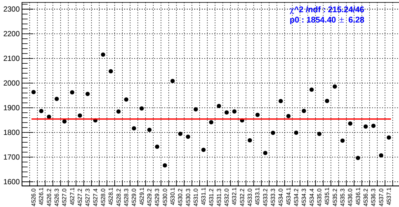
slug65: diff_bpm4aX.rms/nm
