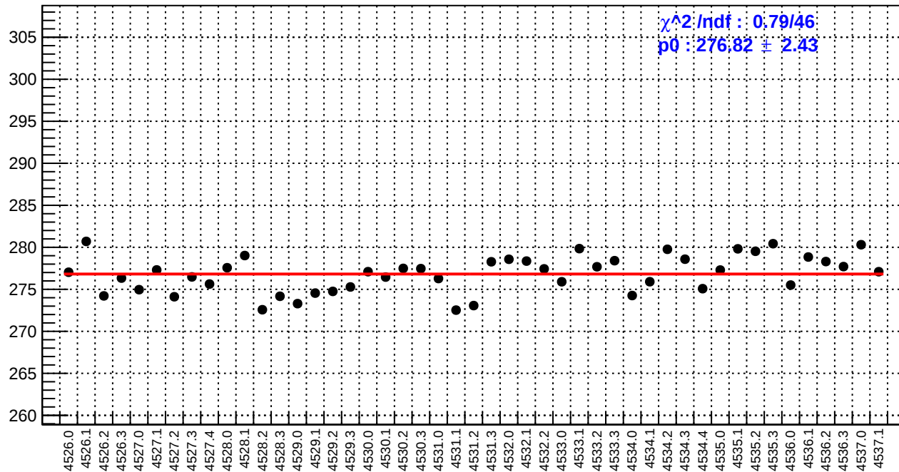
slug65: reg_asym_atr_dd.rms/ppm
