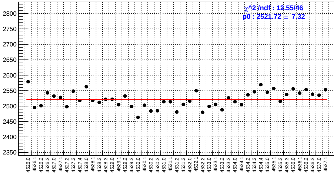
slug65: reg_asym_sam2.rms/ppm
