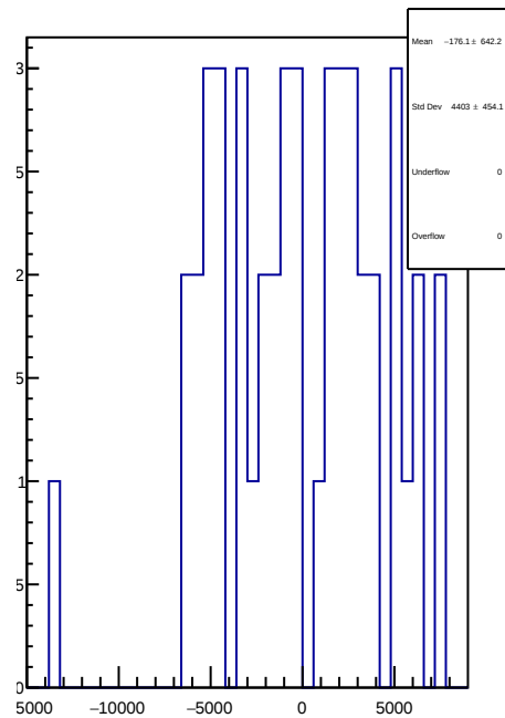
slug65: 1D Corr asym_dsr.mean/ppb-reg_asym_dsr.mean/ppb
