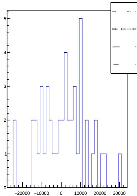
slug65: 1D Corr asym_sam5.mean/ppb-reg_asym_sam5.mean/ppb
