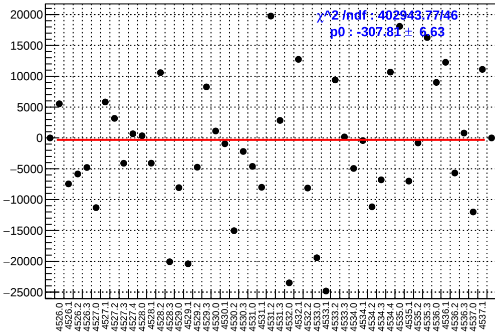
slug65: asym_atr_avg.mean/ppb-reg_asym_atr_avg.mean/ppb
