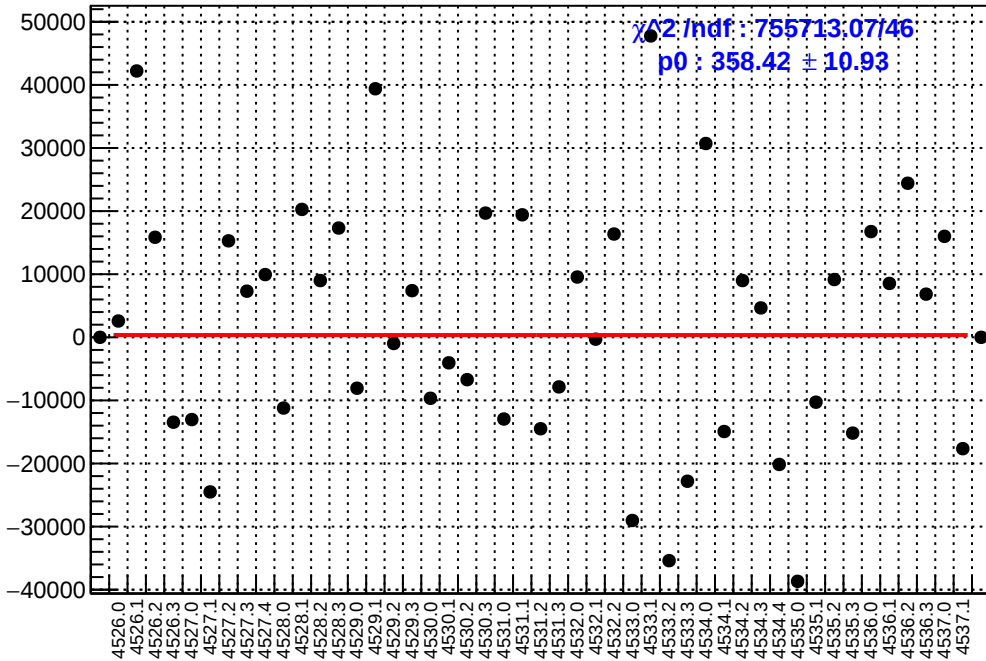
slug65: asym_sam7.mean/ppb-reg_asym_sam7.mean/ppb
