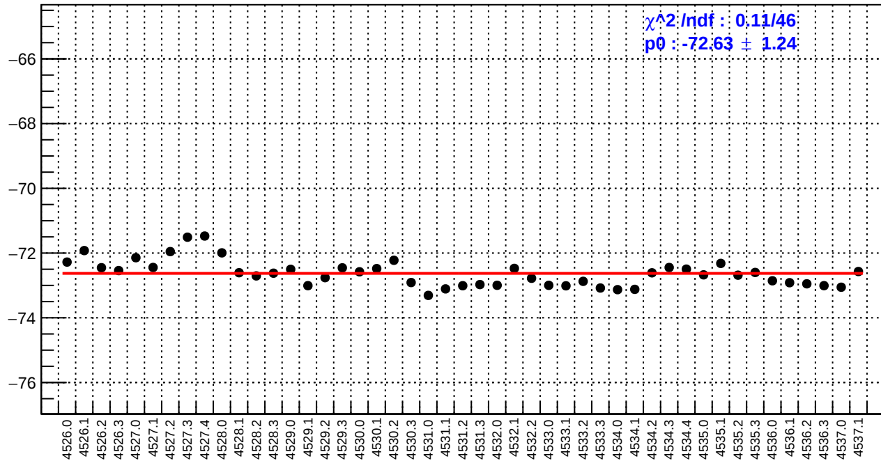
slug65: left_avg_bpm4eX/(ppb/nm)
