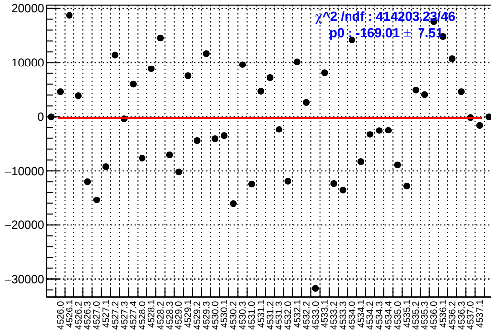
slug65: asym_at1_dd.mean/ppb-reg_asym_at1_dd.mean/ppb
