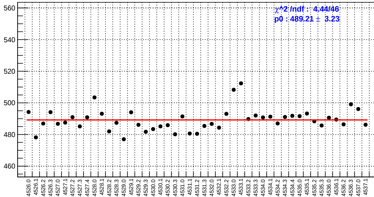
slug65: reg_asym_sam8.rms/ppm
