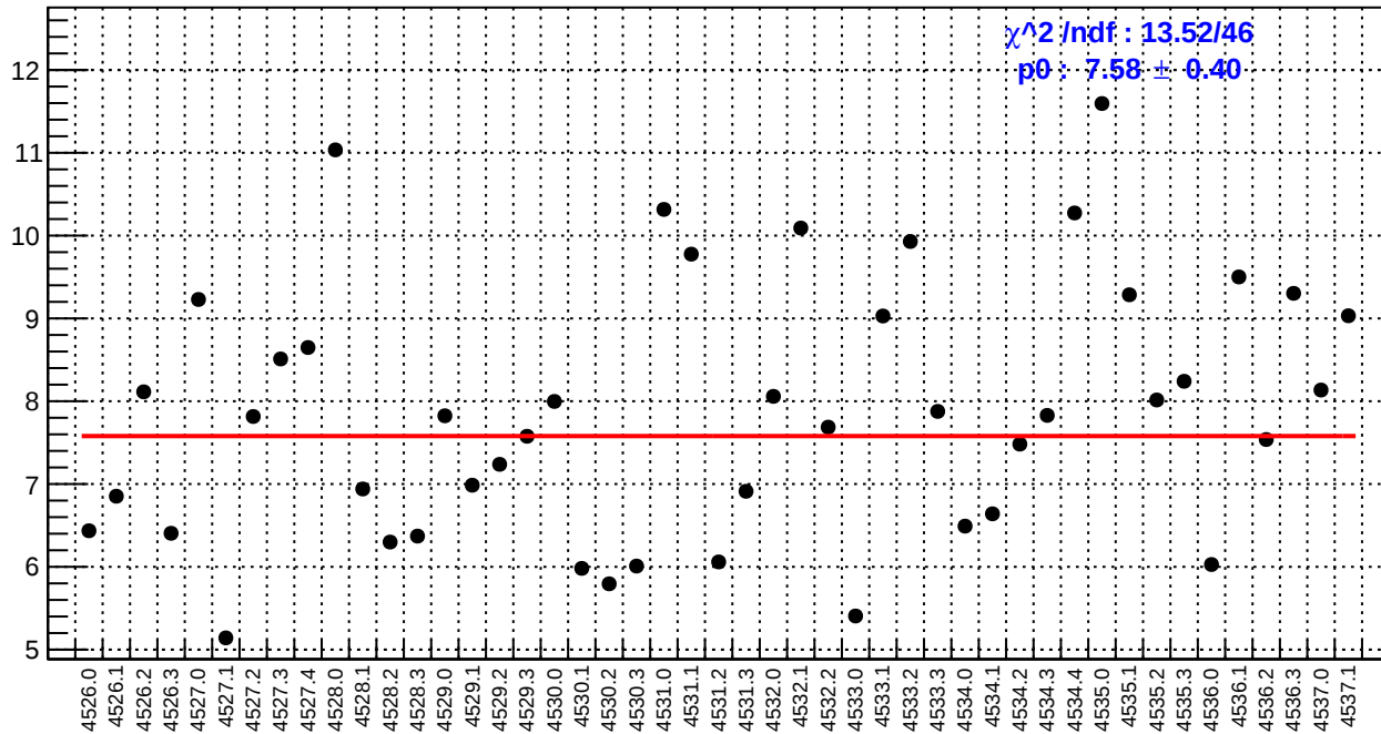
slug65: left_avg_bpm4aY/(ppb/nm)
