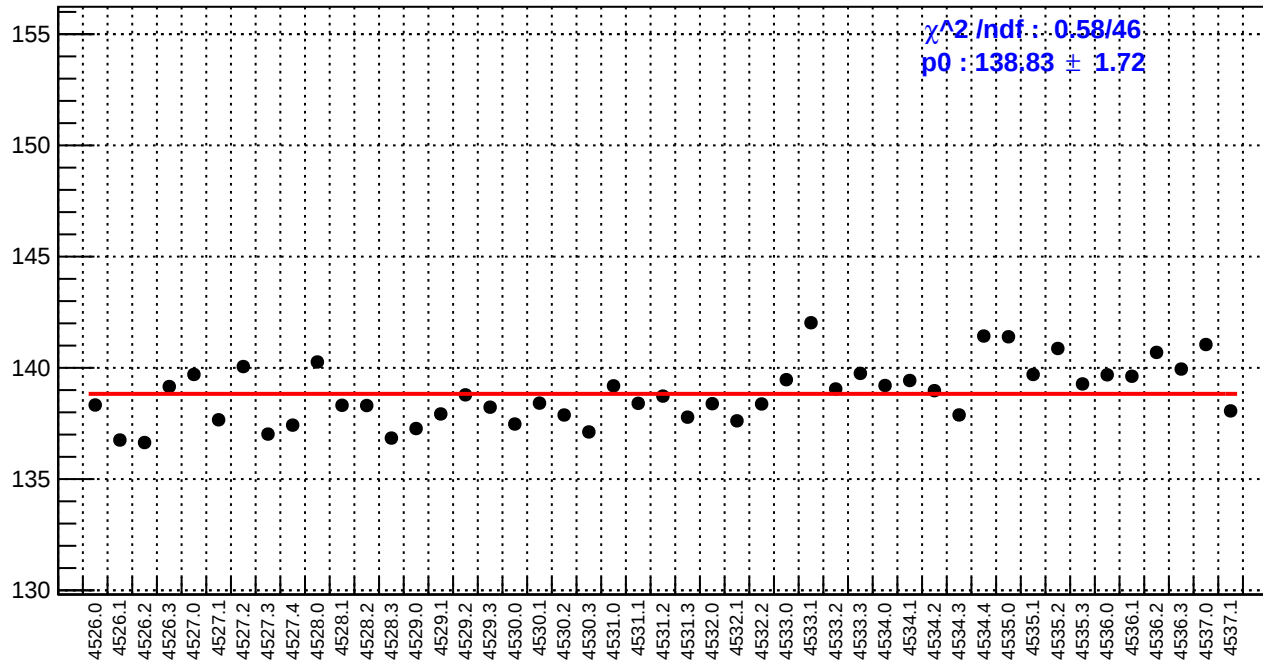
slug65: reg_asym_dsl.rms/ppm
