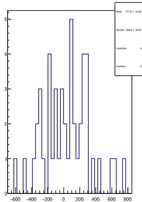
slug65: 1D Corr asym_left_dd.mean/ppb-reg_asym_left_dd.mean/ppb
