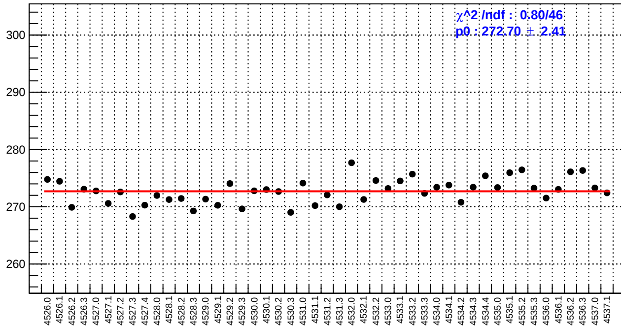
slug65: reg_asym_atr_avg.rms/ppm
