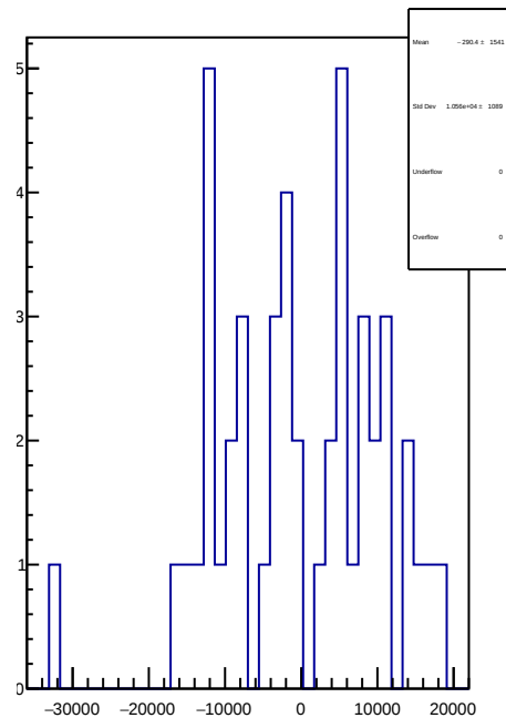
slug65: 1D Corr asym_at1_dd.mean/ppb-reg_asym_at1_dd.mean/ppb
