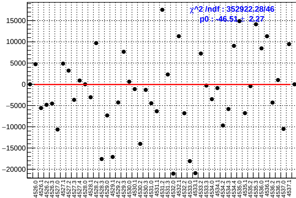
slug65: asym_at1_avg.mean/ppb-reg_asym_at1_avg.mean/ppb
