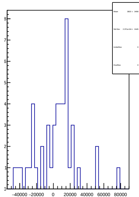
slug65: 1D Corr asym_sam6.mean/ppb-reg_asym_sam6.mean/ppb
