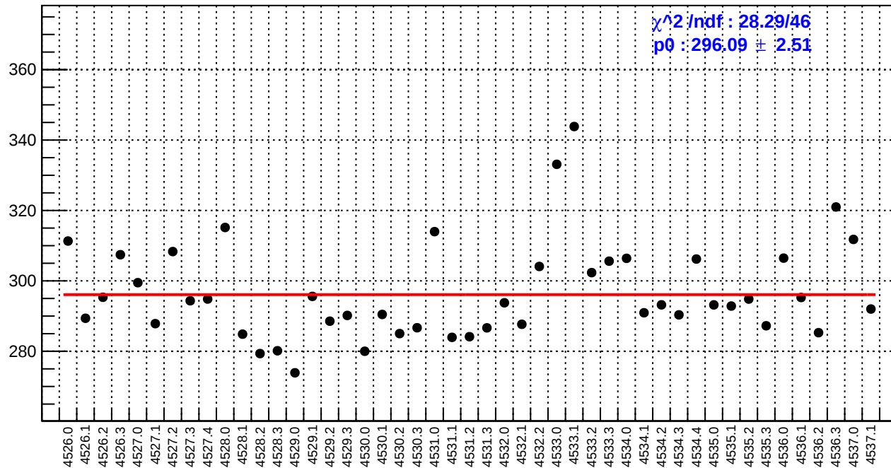
slug65: reg_asym_sam5.rms/ppm
