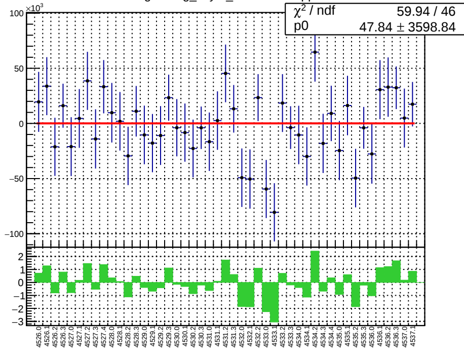
slug65: reg_asym_sam2.mean/ppb
