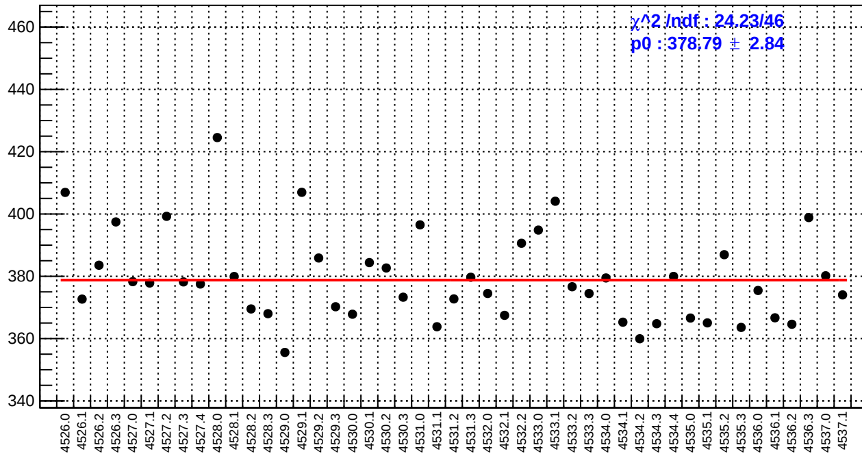
slug65: reg_asym_sam6.rms/ppm
