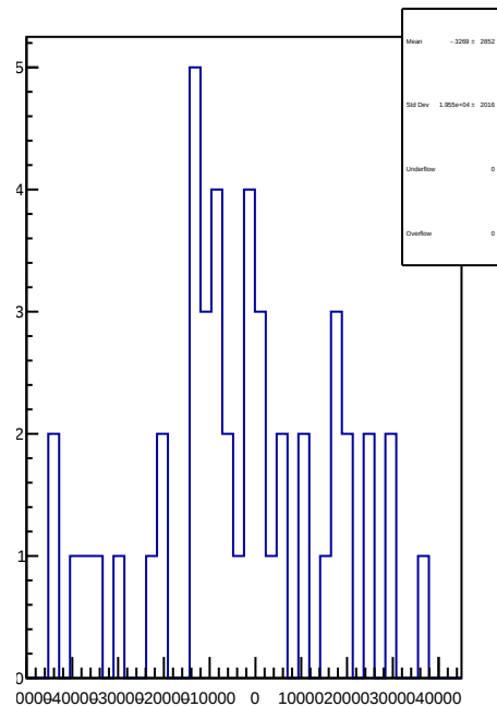
slug65: 1D Corr asym_atl_avg.mean/ppb-reg_asym_atl_avg.mean/ppb
