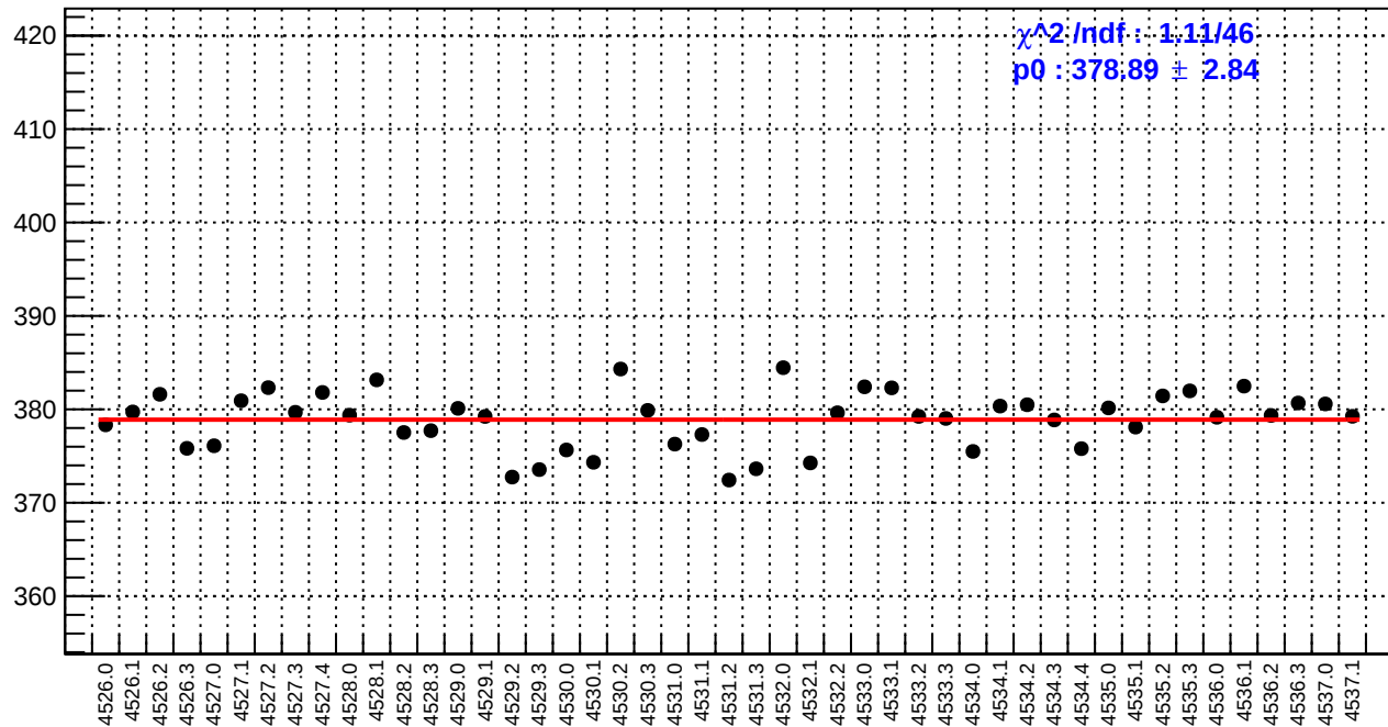
slug65: reg_asym_at1_dd.rms/ppm
