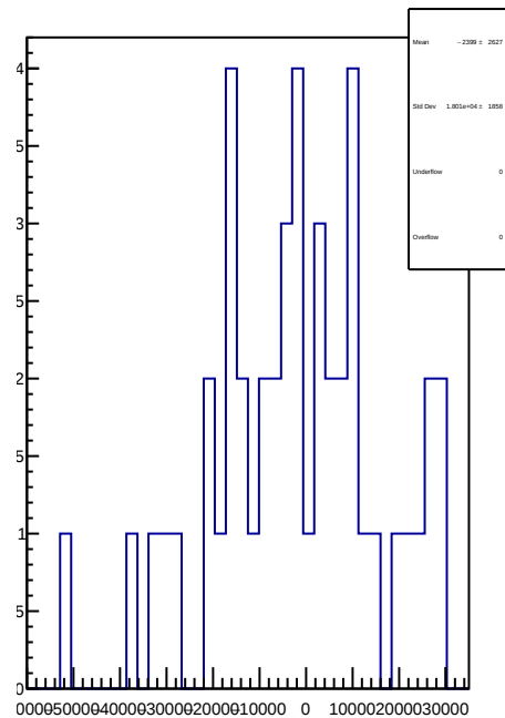
slug65: 1D Corr asym_atr2.mean/ppb-reg_asym_atr2.mean/ppb
