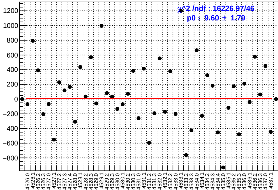
slug65: asym_right_dd.mean/ppb-reg_asym_right_dd.mean/ppb
