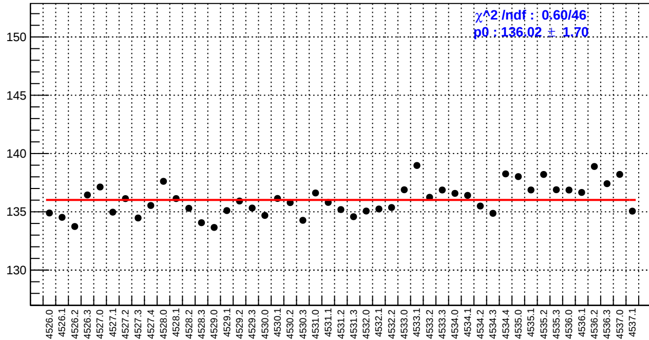
slug65: reg_asym_usl.rms/ppm
