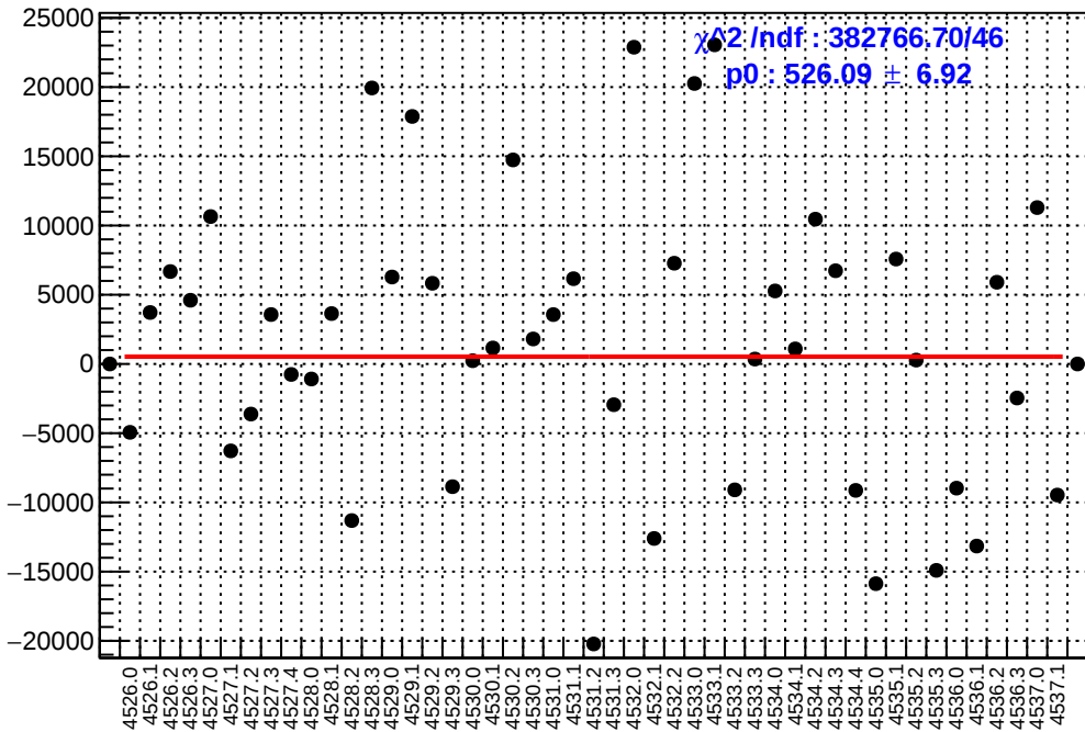
slug65: asym_atr1l2_dd.mean/ppb-reg_asym_atr1l2_dd.mean/ppb
