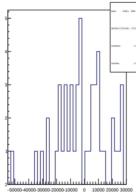
slug65: 1D Corr asym_atl1r2_avg.mean/ppb-reg_asym_atl1r2_avg.mean/ppb
