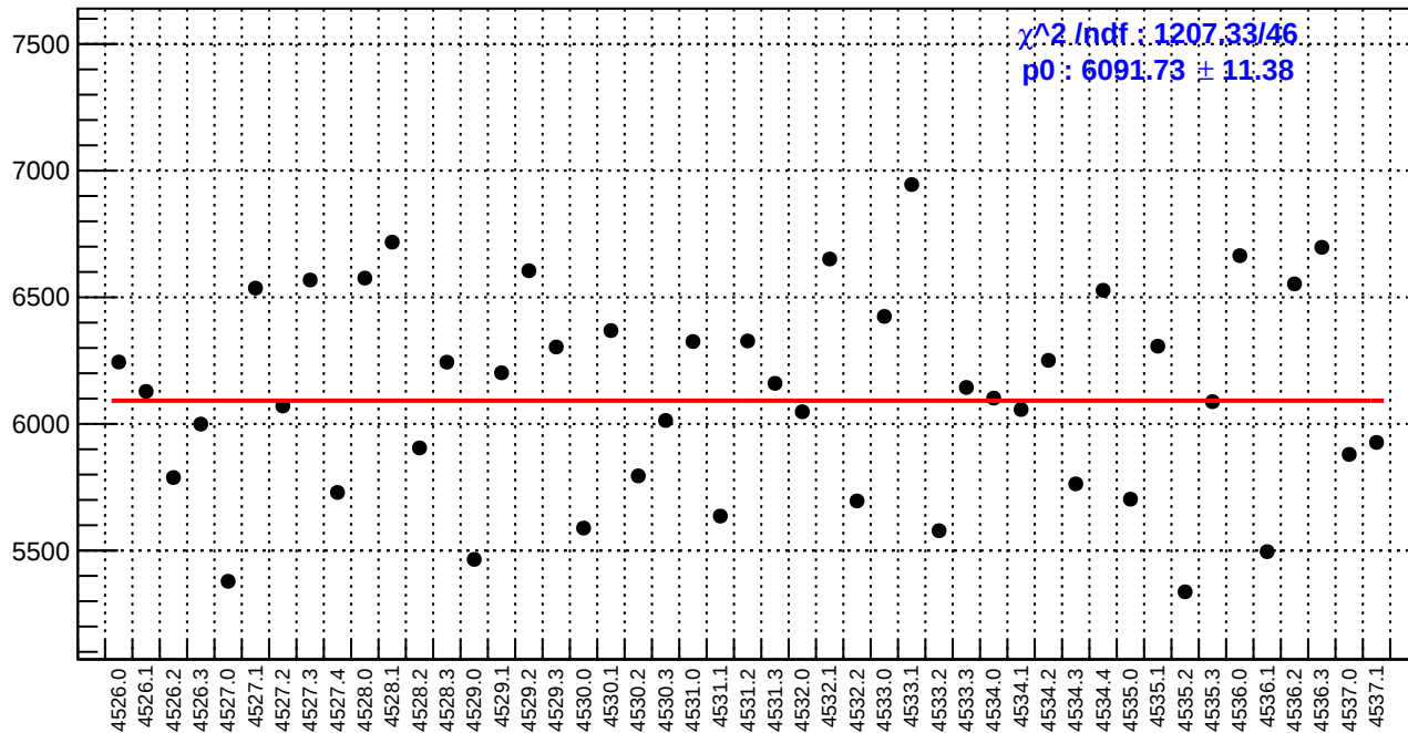
slug65: diff_bpm4eY.rms/nm
