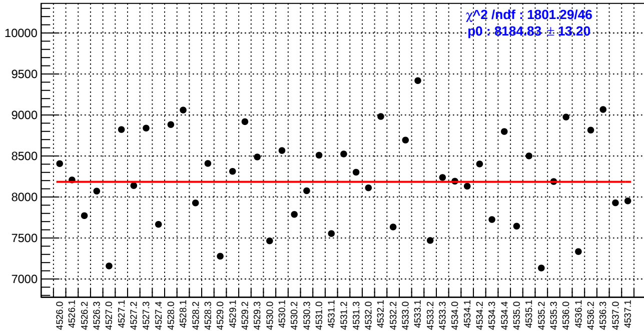
slug65: diff_bpm4aY.rms/nm
