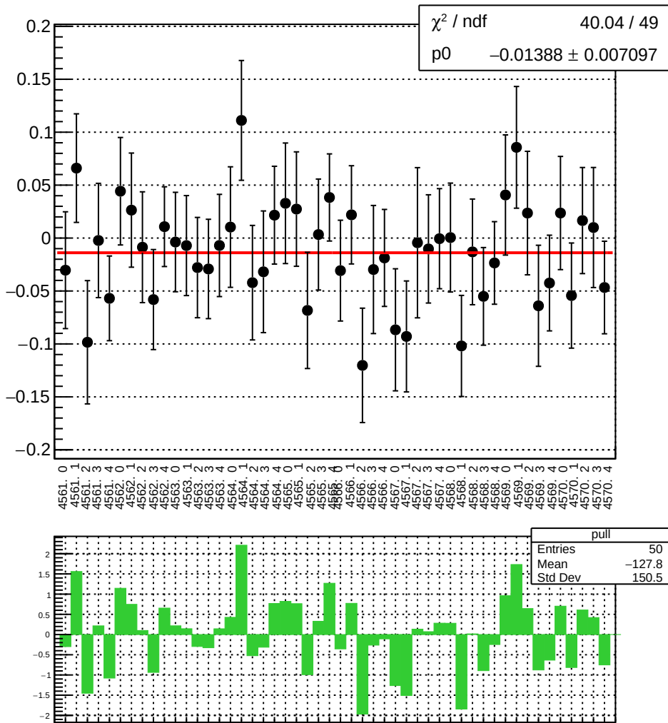
reg_bcm_dg_us_ds_dd_diff_bpm11X_slope vs run
