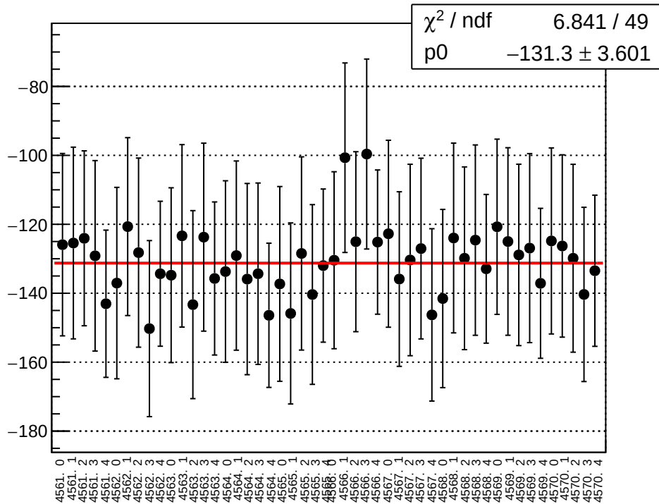
reg_asym_sam8_diff_bpm4eY_slope vs run
