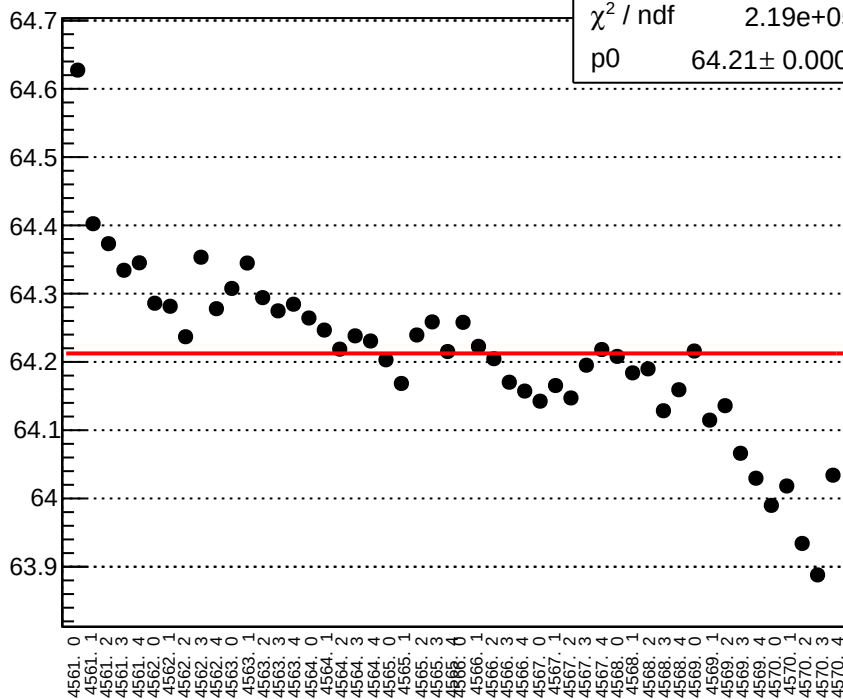
yield_usl_mean vs run
