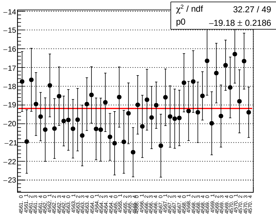
reg asym sam1 diff bpm4eX slope vs run
