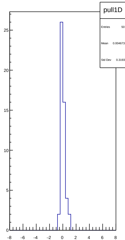
\chi^2 / \text{ndf} 5.098 / 49 p0 36.46 \pm 0.449
