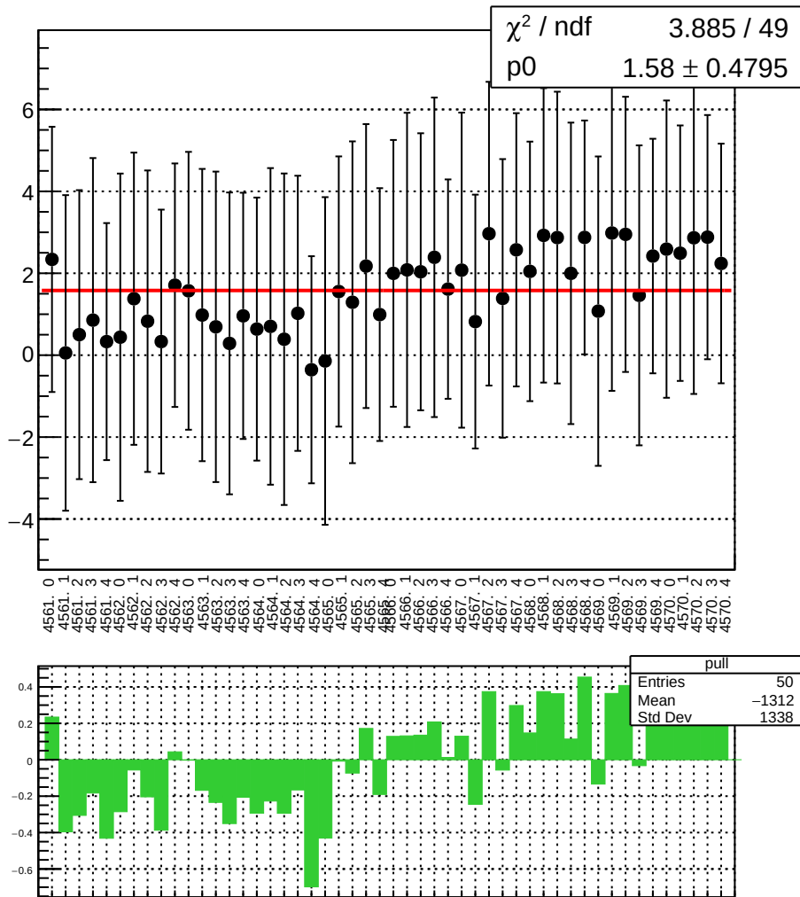
reg_asym_sam_15_dd_diff_bpm11X_slope vs run
