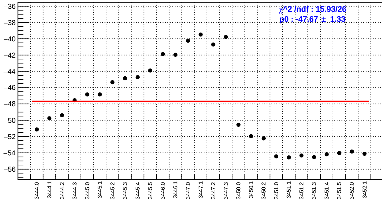
slug7: us_avg_bpm12X/(ppb/nm)
