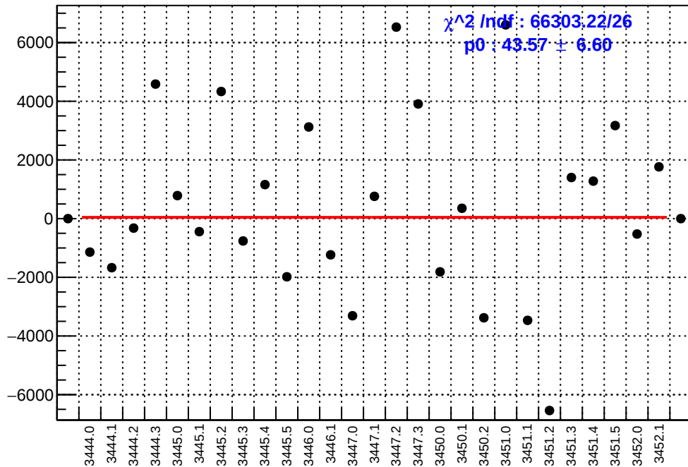
slug7: asym_us_dd.mean/ppb-reg_asym_us_dd.mean/ppb
