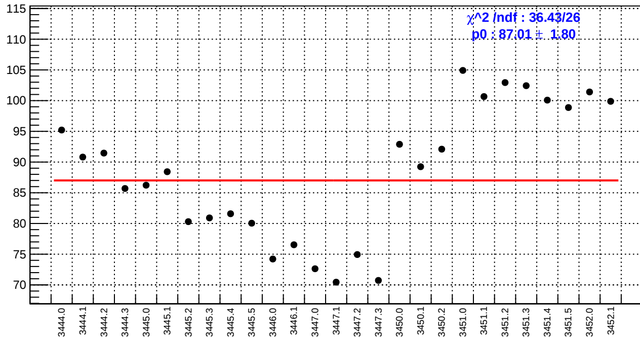
slug7: ds_avg_bpm4aX/(ppb/nm)
