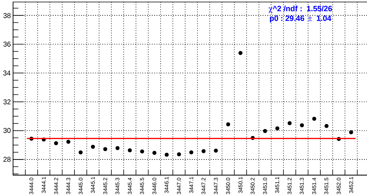
slug7: reg_asym_left_dd.rms/ppm
