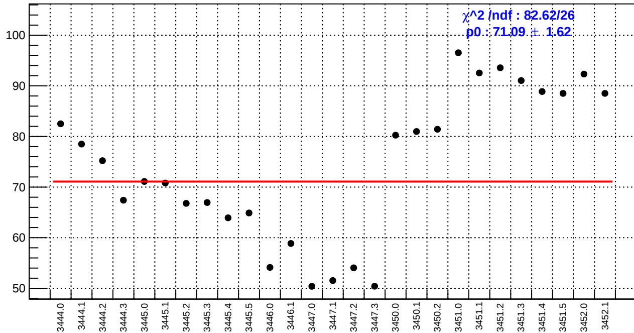
slug7: dsr_bpm4aX/(ppb/nm)
