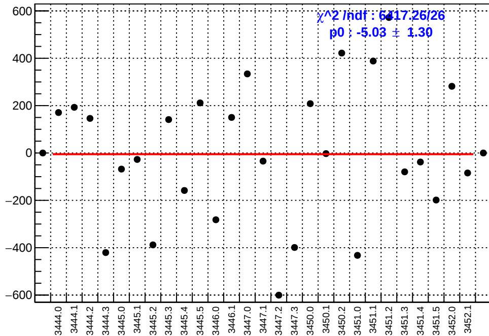
slug7: asym_right_dd.mean/ppb-reg_asym_right_dd.mean/ppb
