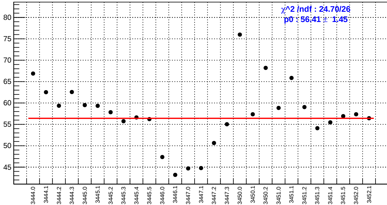
slug7: dsl_bpm4eY/(ppb/nm)
