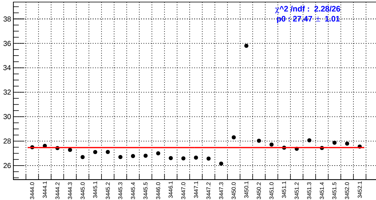
slug7: reg_asym_right_dd.rms/ppm
