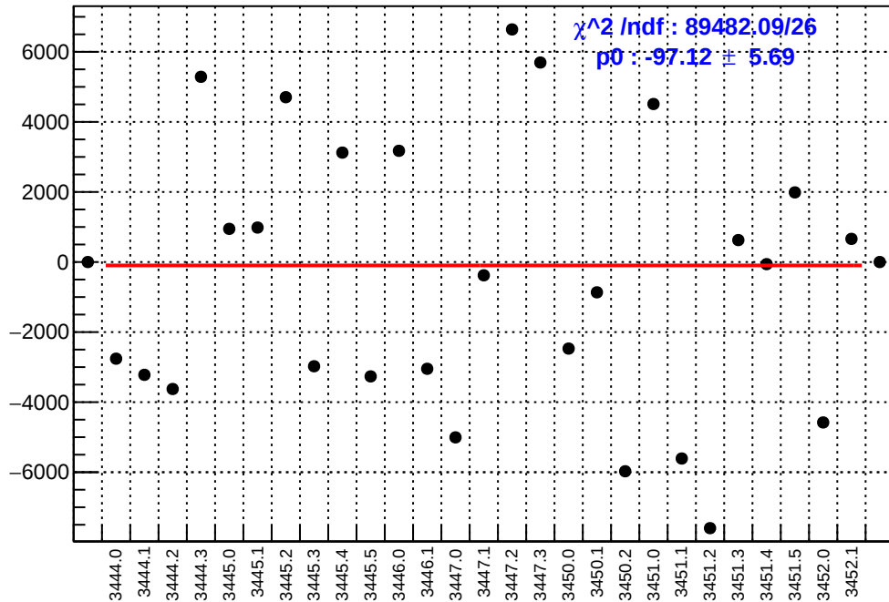
slug7: asym_usl.mean/ppb-reg_asym_usl.mean/ppb
