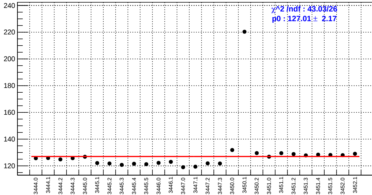
slug7: reg_asym_ds_avg.rms/ppm
