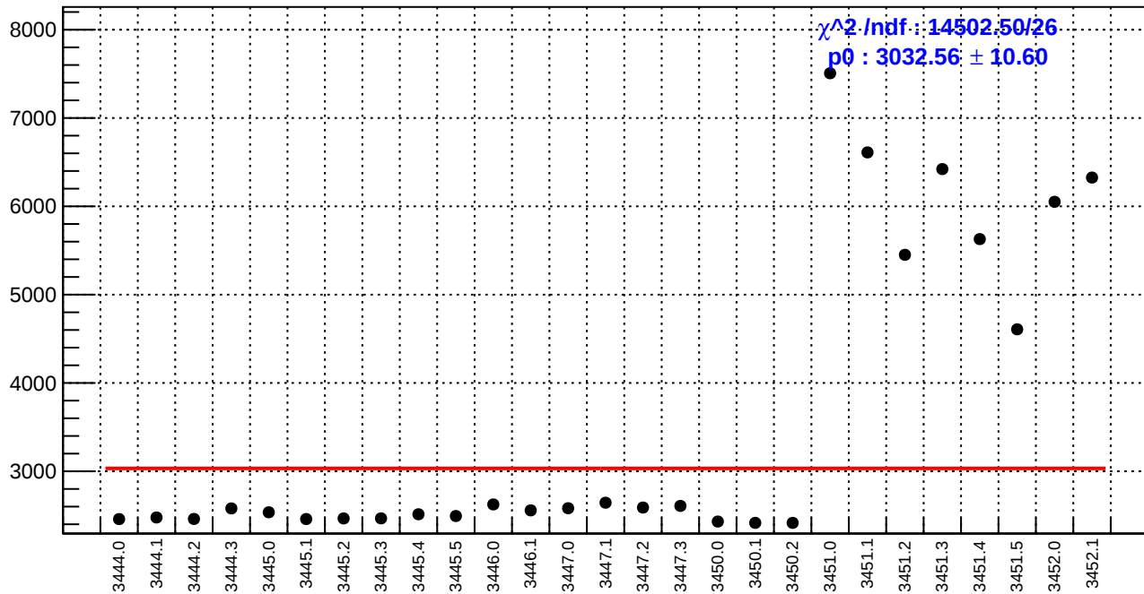
slug7: diff_bpm4aY.rms/nm
