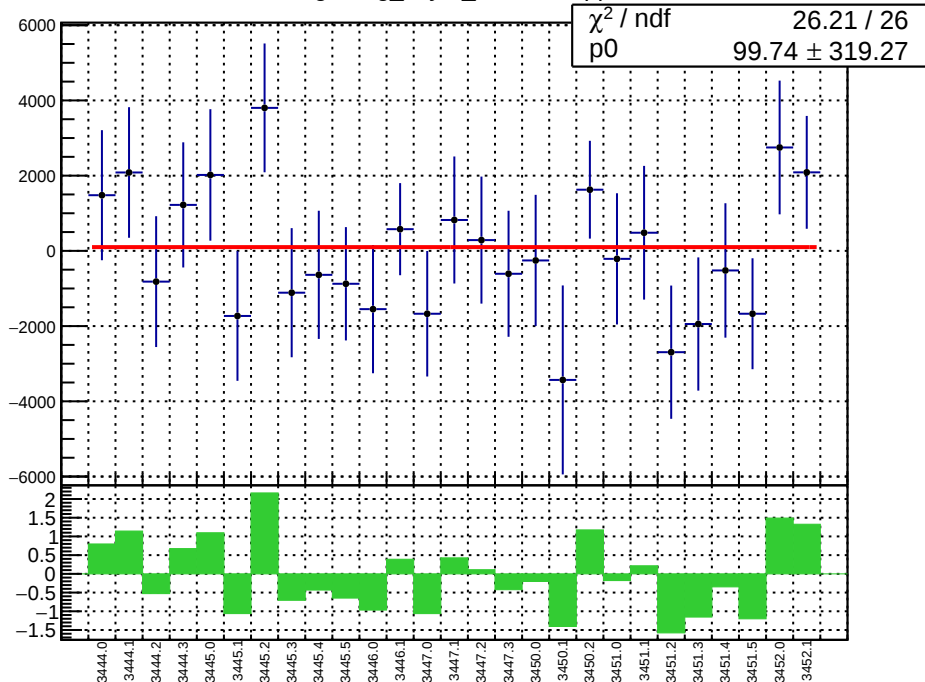
slug7: reg_asym_dsr.mean/ppb
