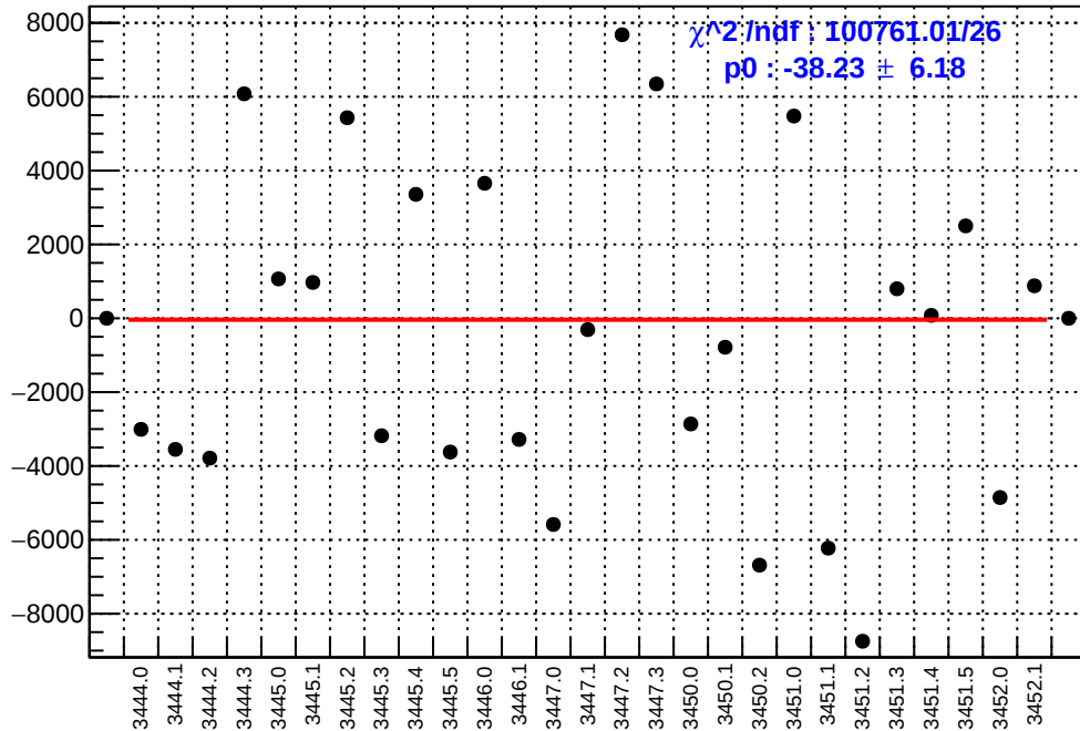
slug7: asym_dsl.mean/ppb-reg_asym_dsl.mean/ppb
