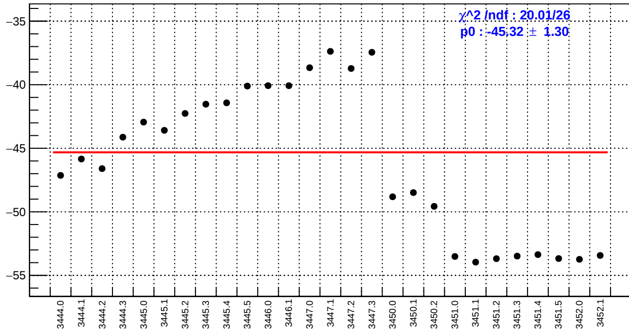
slug7: dsl_bpm12X/(ppb/nm)
