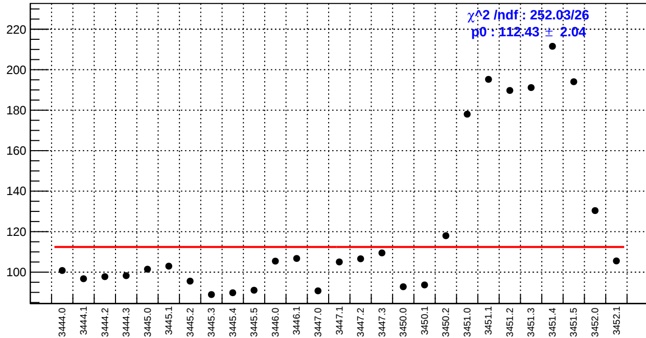
slug7: asym_bcm_an_ds3.rms/ppm
