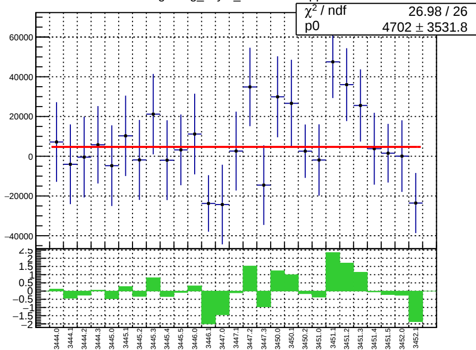
slug7: reg_asym_sam2.mean/ppb
