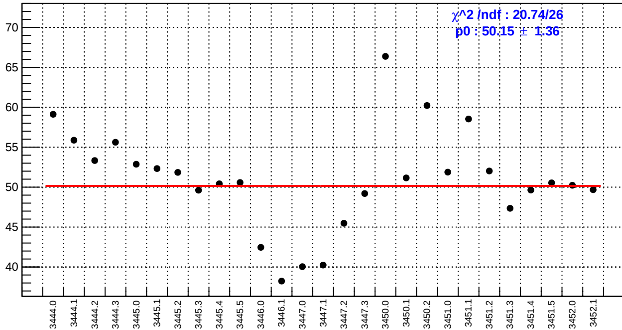
slug7: usl_bpm4eY/(ppb/nm)
