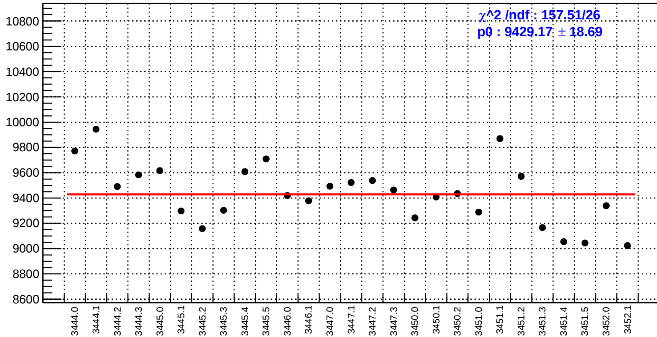
slug7: diff_bpm4eX.rms/nm
