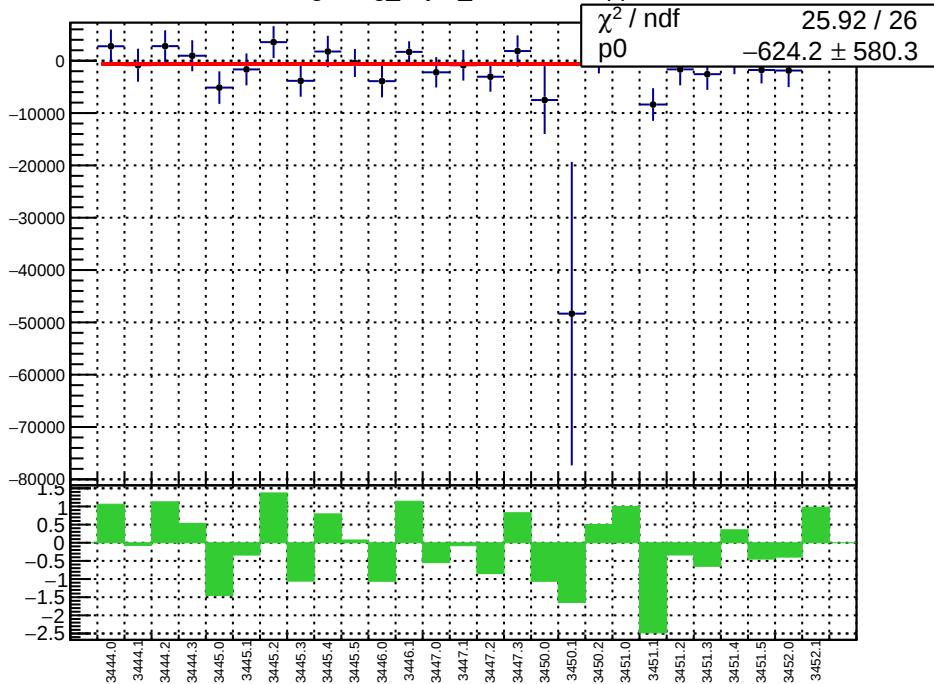
slug7: reg_asym_sam7.mean/ppb
