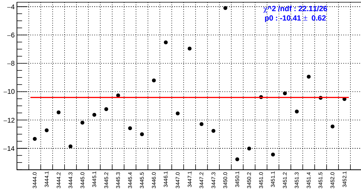
slug7: dsr_bpm4eY/(ppb/nm)
