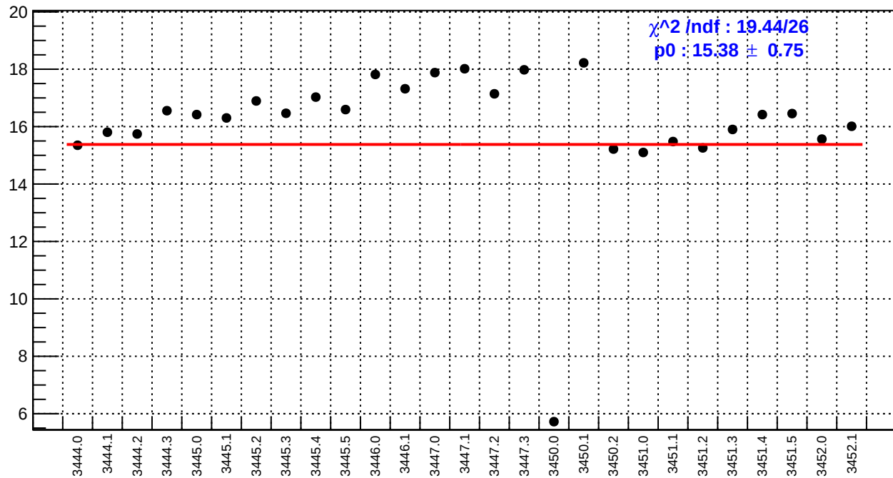
slug7: dsr_bpm4eX/(ppb/nm)
