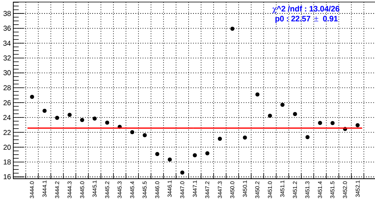
slug7: ds_avg_bpm4eY/(ppb/nm)
