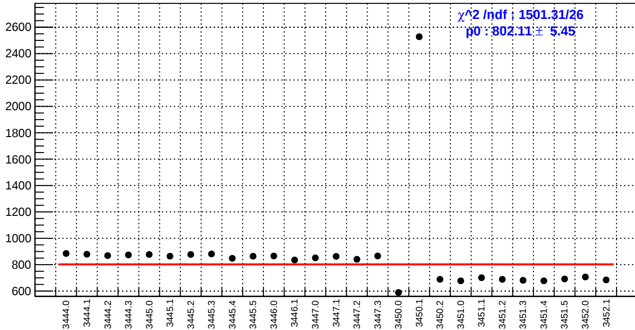
slug7: reg_asym_sam6.rms/ppm
