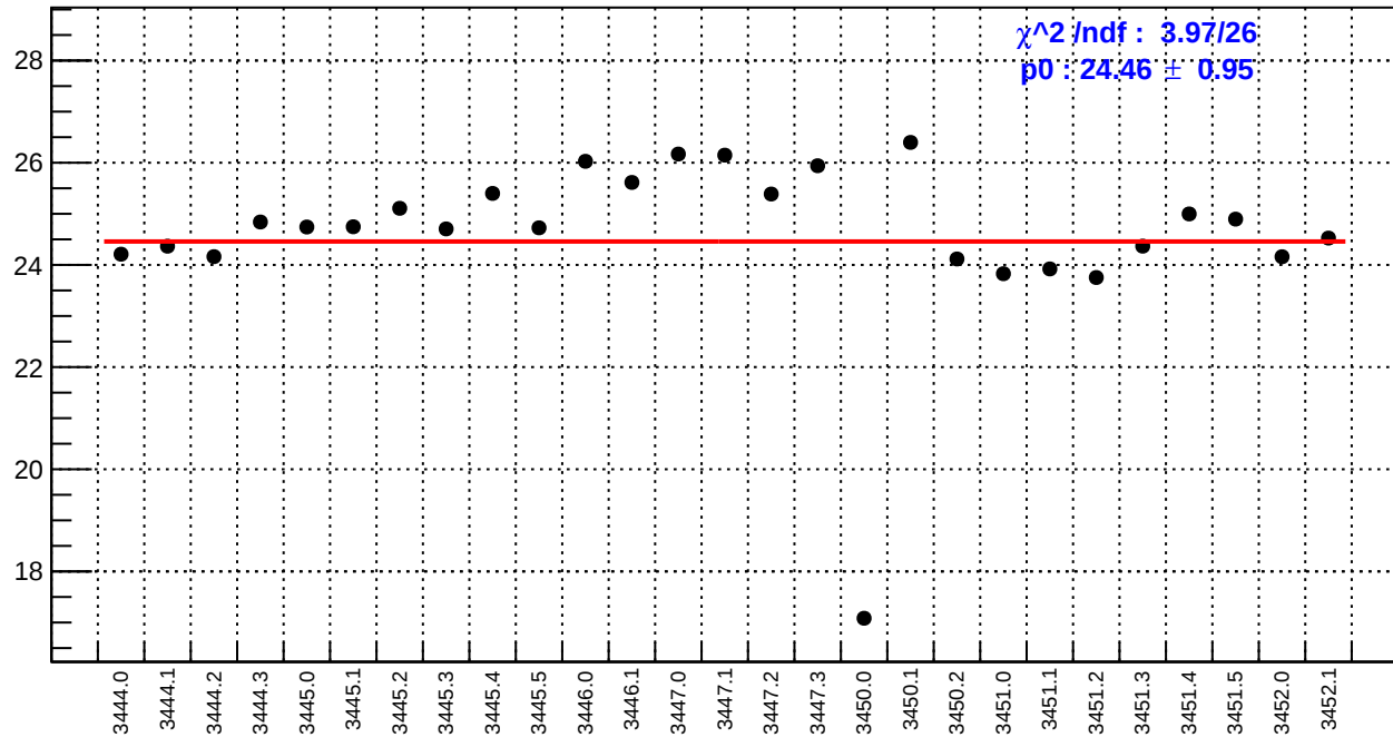
slug7: usr_bpm4eX/(ppb/nm)
