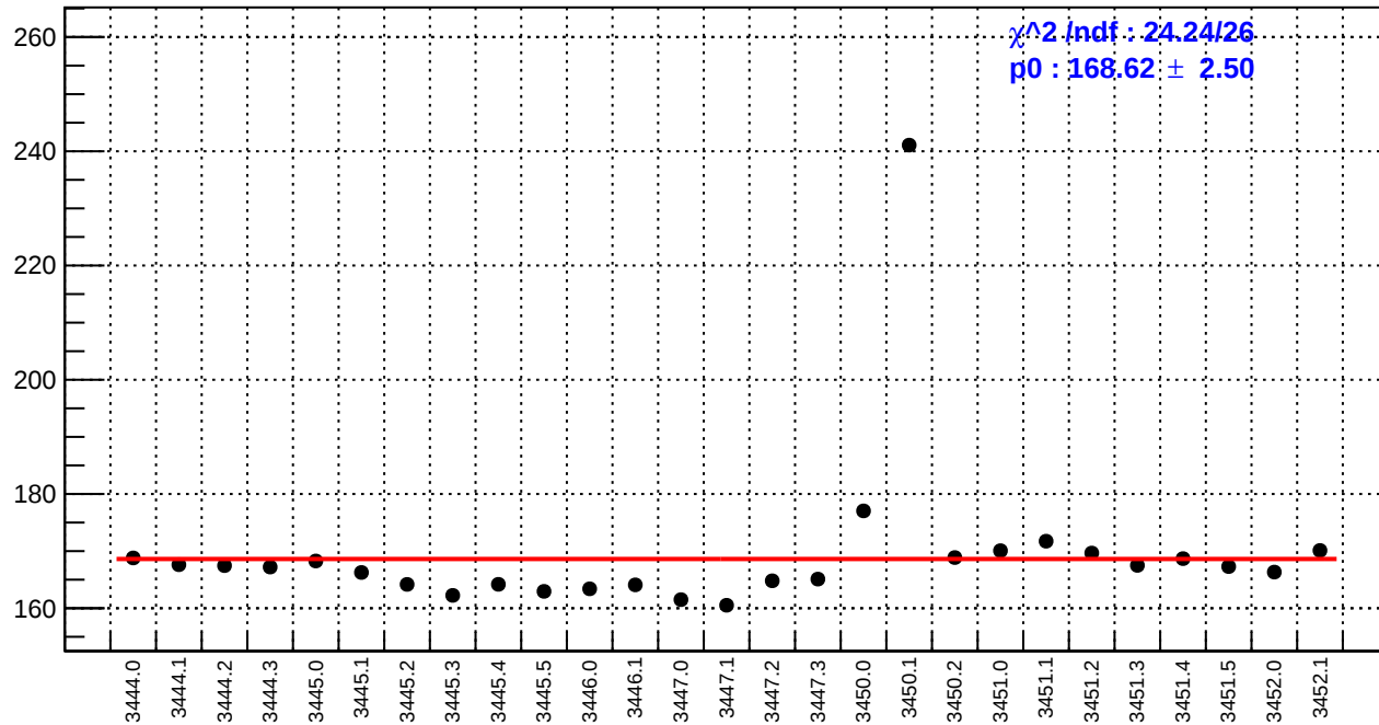
slug7: reg_asym_left_avg.rms/ppm
