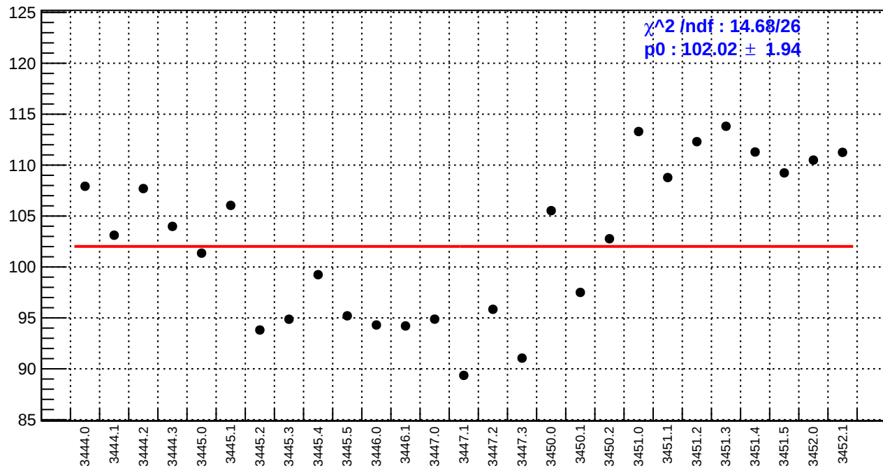
slug7: dsl_bpm4aX/(ppb/nm)
