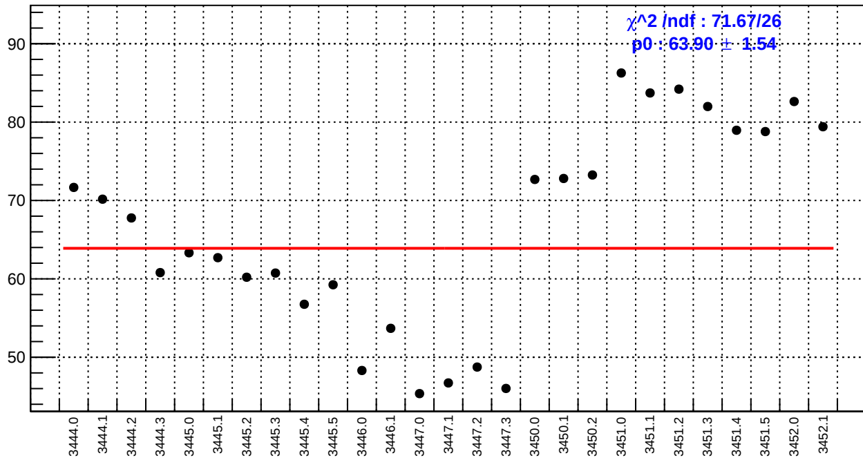
slug7: usr_bpm4aX/(ppb/nm)
