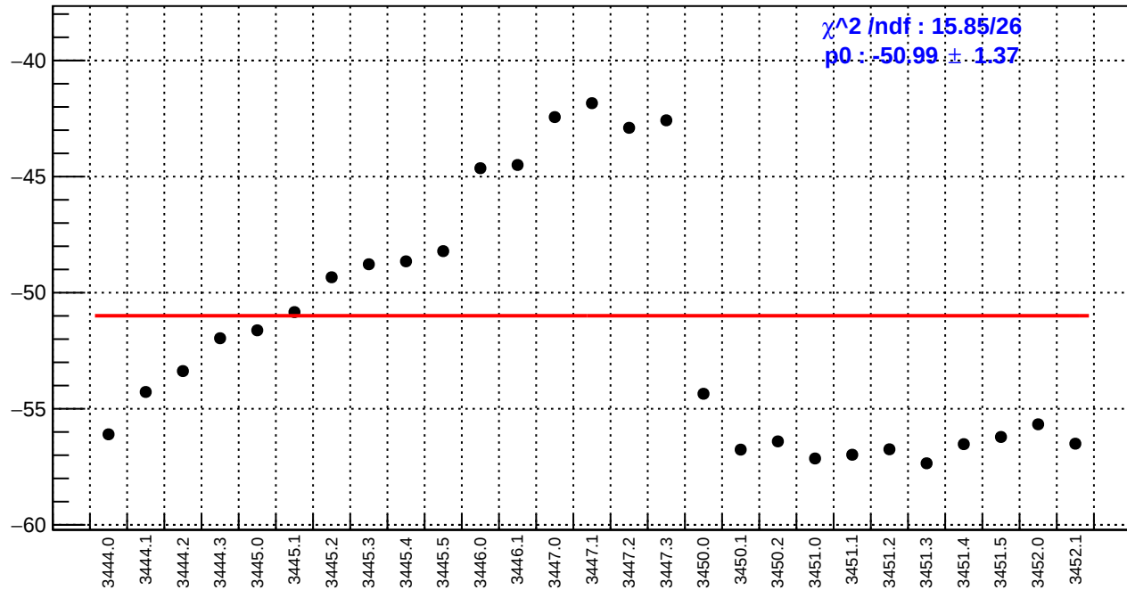
slug7: usr_bpm12X/(ppb/nm)
