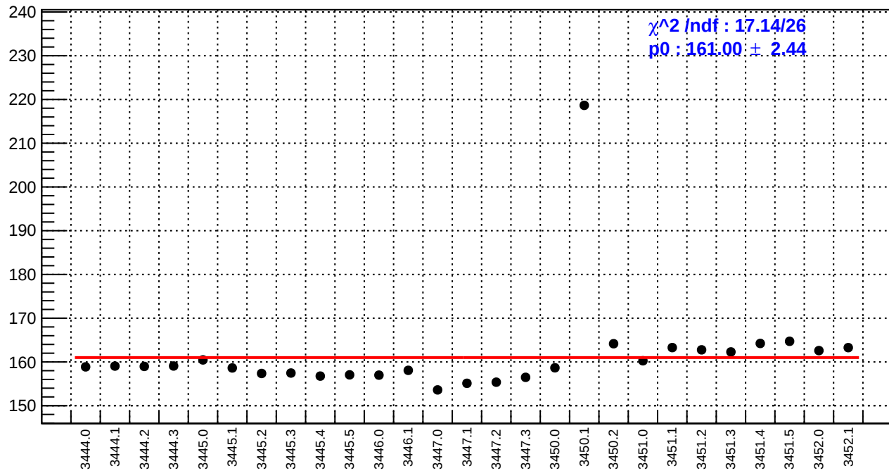
slug7: reg_asym_right_avg.rms/ppm
