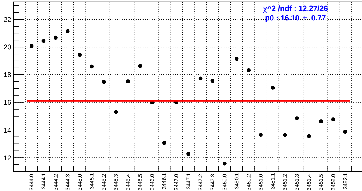
slug7: dsr_bpm4aY/(ppb/nm)
