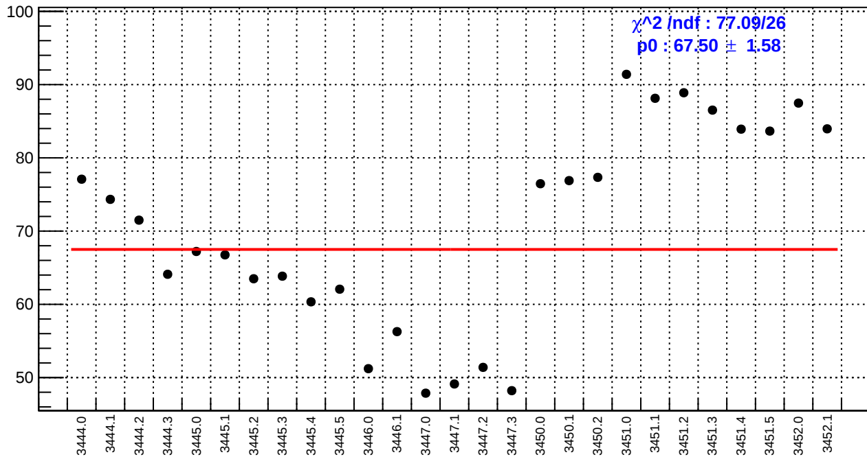
slug7: right_avg_bpm4aX/(ppb/nm)
