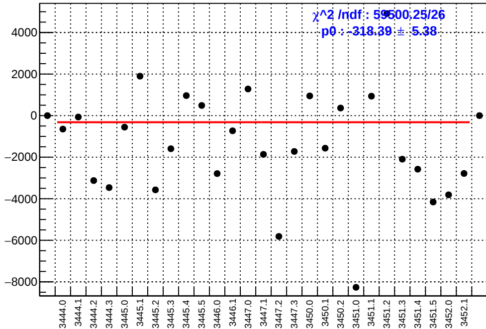
slug7: asym_right_avg.mean/ppb-reg_asym_right_avg.mean/ppb
