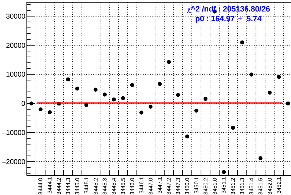
slug7: asym_sam5.mean/ppb-reg_asym_sam5.mean/ppb
