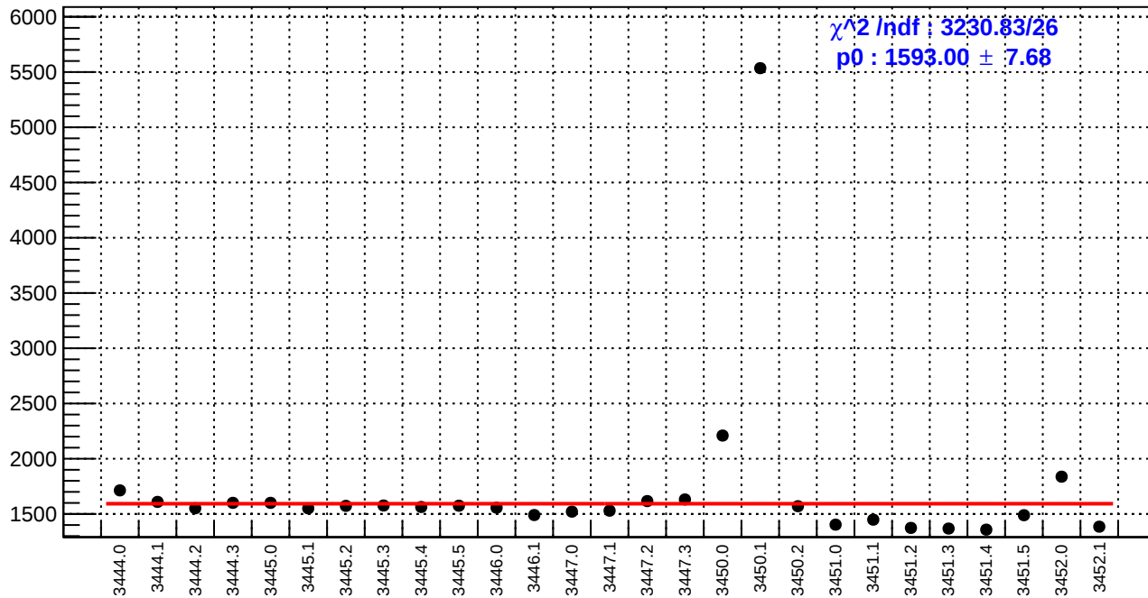
slug7: reg_asym_sam3.rms/ppm
