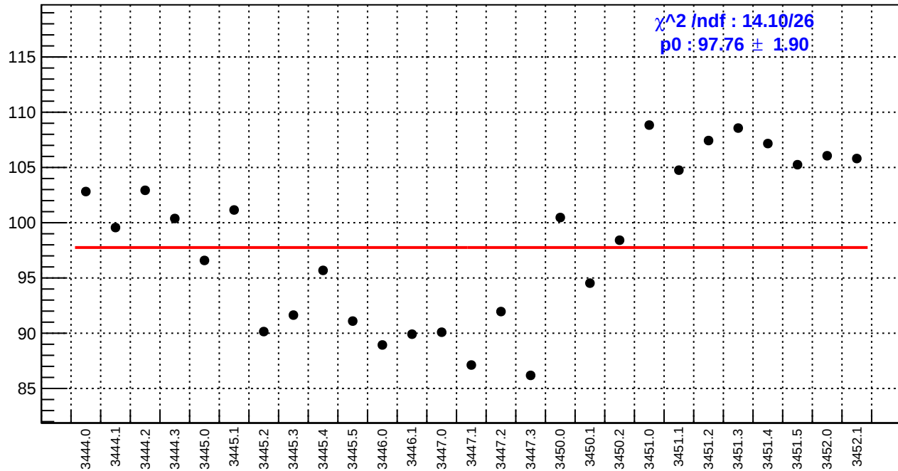
slug7: usl_bpm4aX/(ppb/nm)
