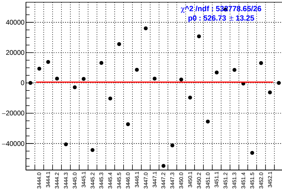
slug7: asym_sam6.mean/ppb-reg_asym_sam6.mean/ppb
