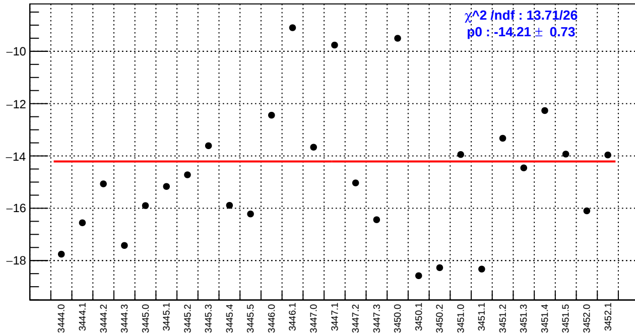
slug7: right_avg_bpm4eY/(ppb/nm)
