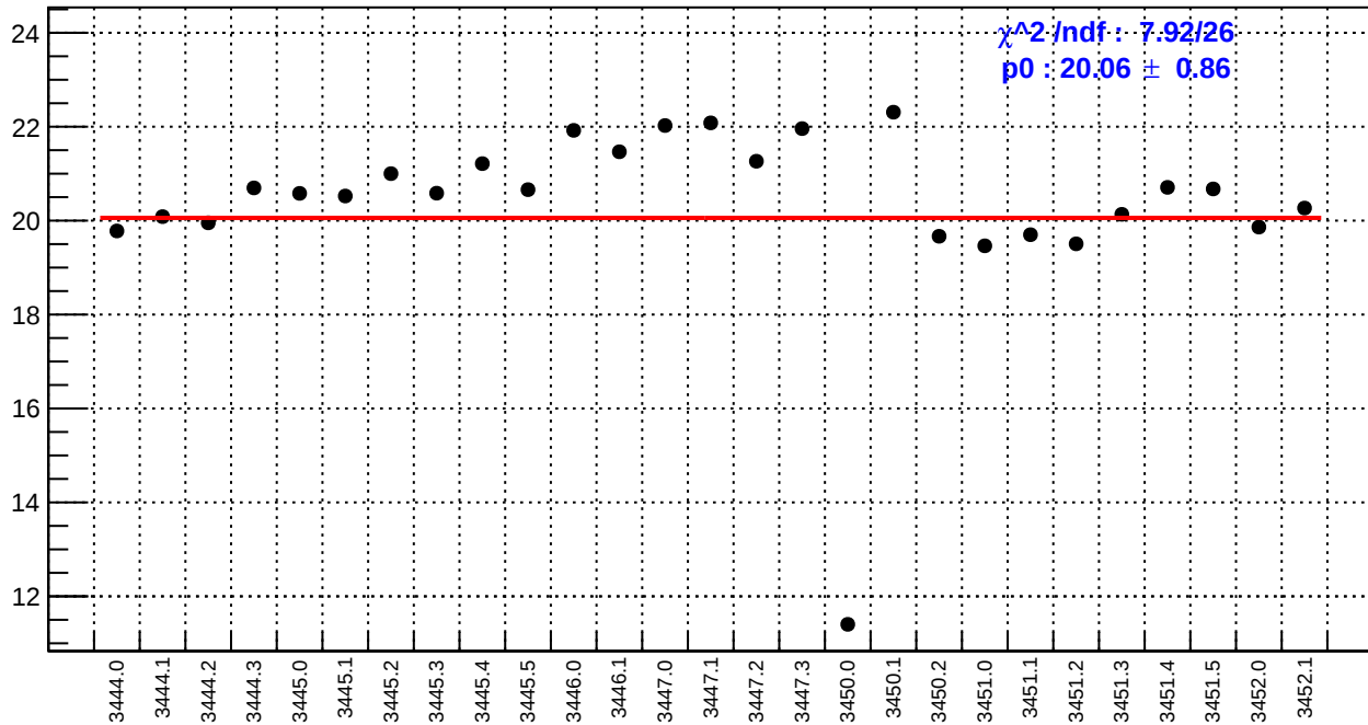
slug7: right_avg_bpm4eX/(ppb/nm)
