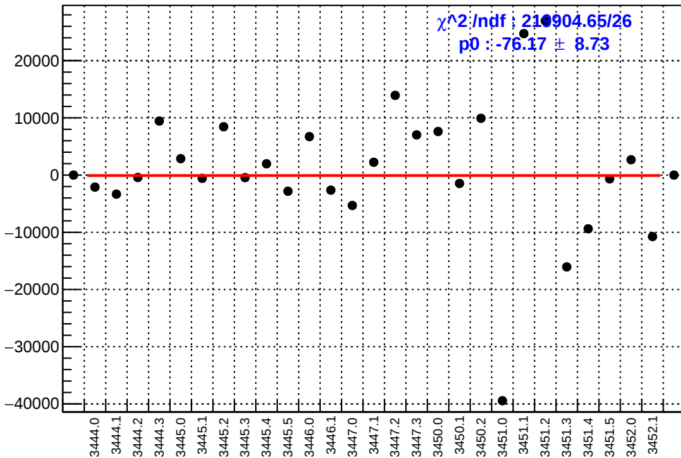
slug7: asym_sam8.mean/ppb-reg_asym_sam8.mean/ppb
