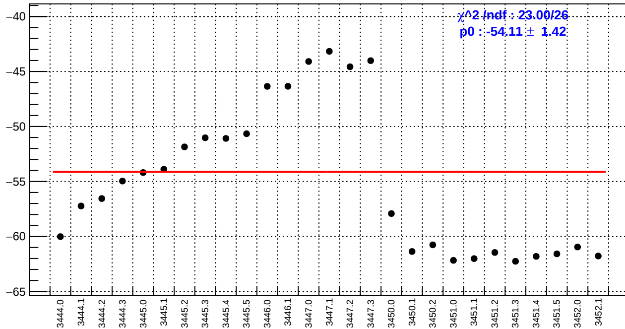
slug7: dsr_bpm12X/(ppb/nm)
