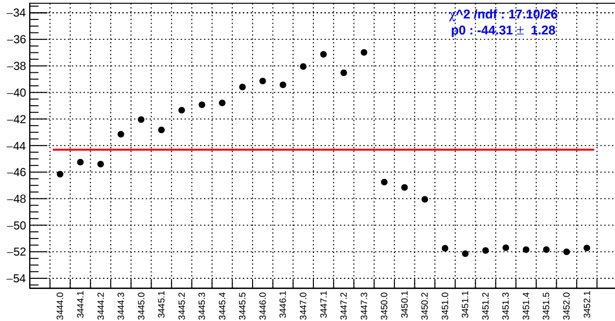
slug7: usl_bpm12X/(ppb/nm)
