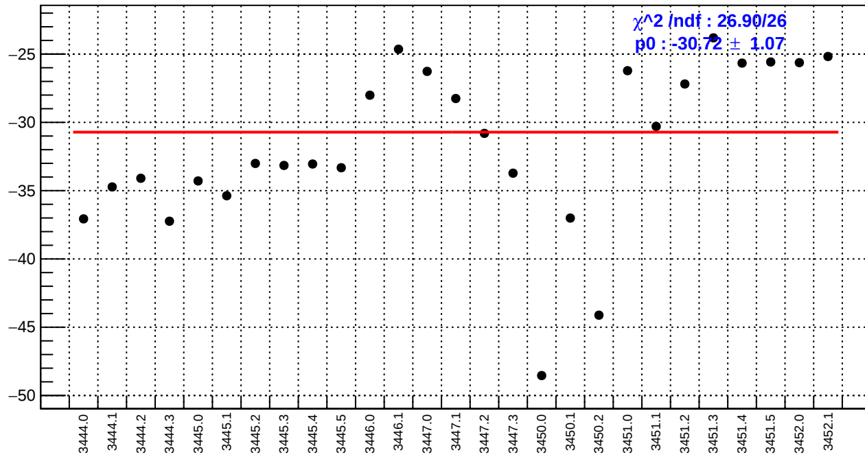
slug7: left_avg_bpm4aY/(ppb/nm)
