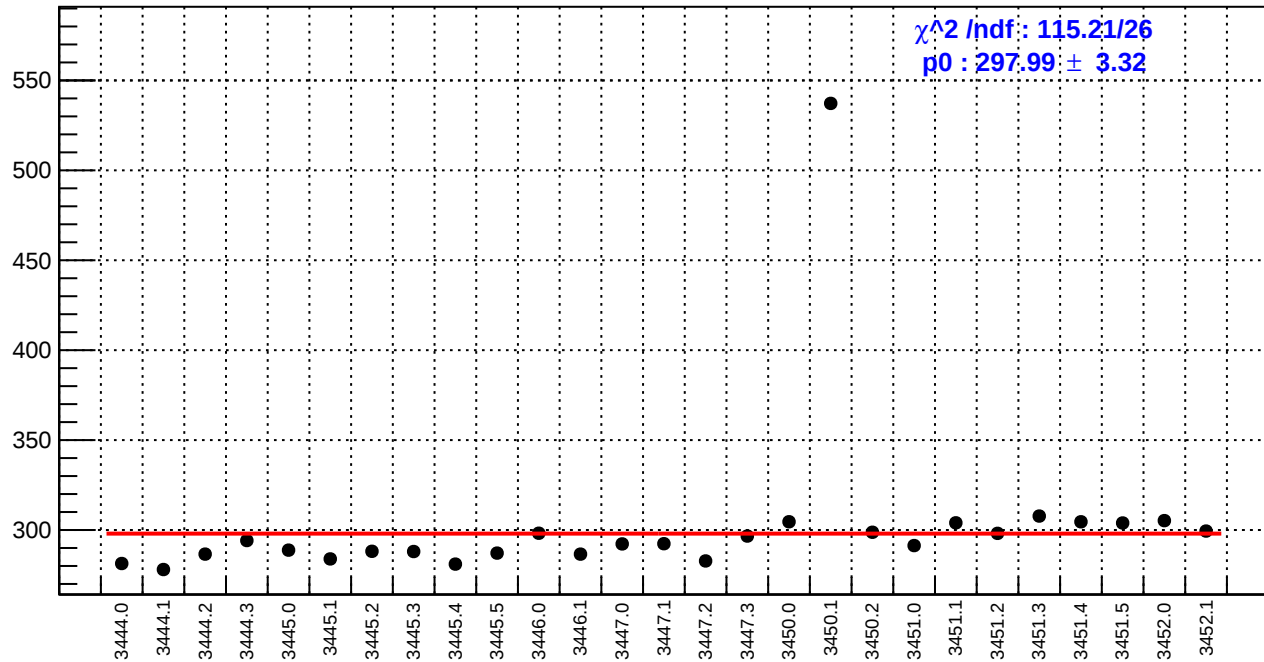
slug7: reg_asym_sam1.rms/ppm
