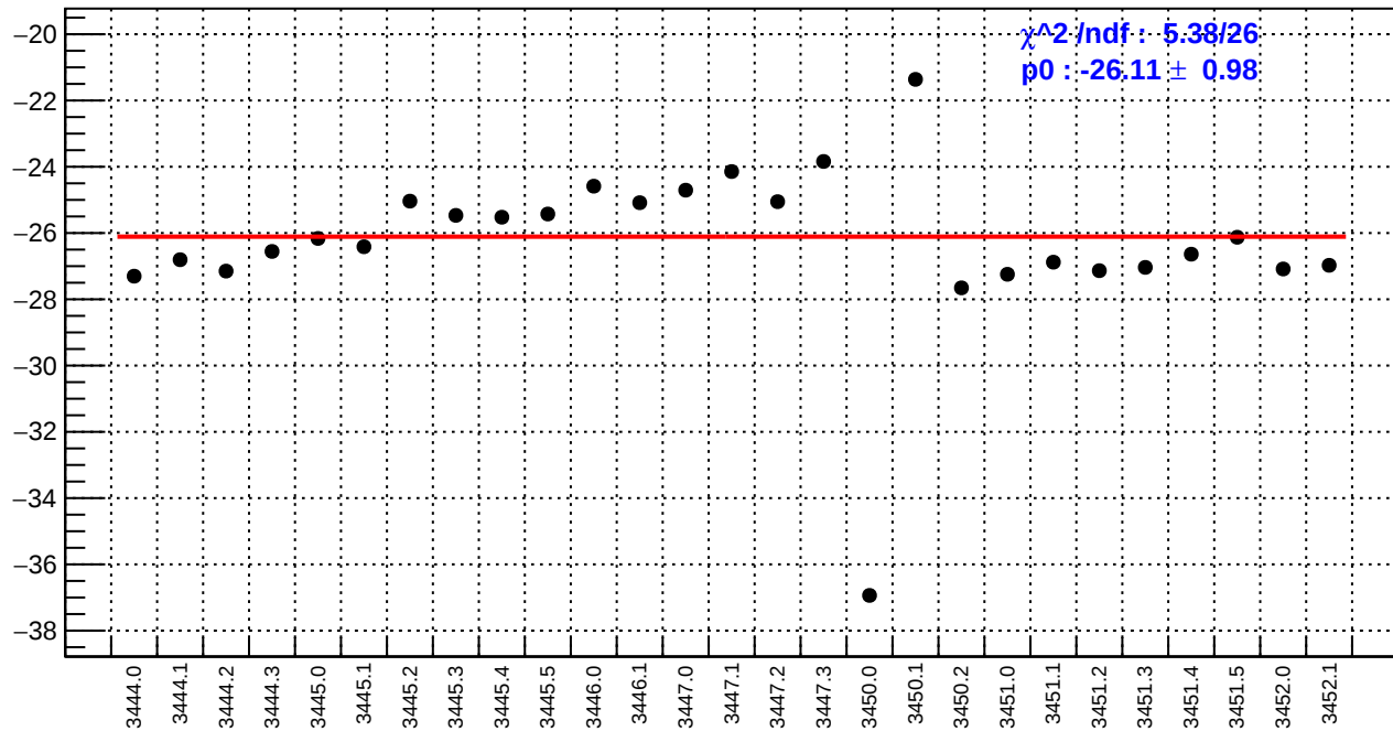
slug7: ds_avg_bpm4eX/(ppb/nm)
