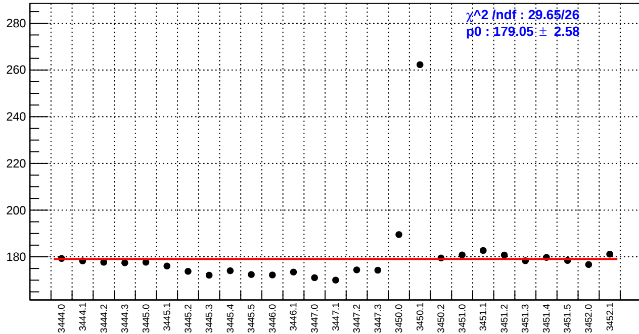
slug7: reg_asym_dsl.rms/ppm
