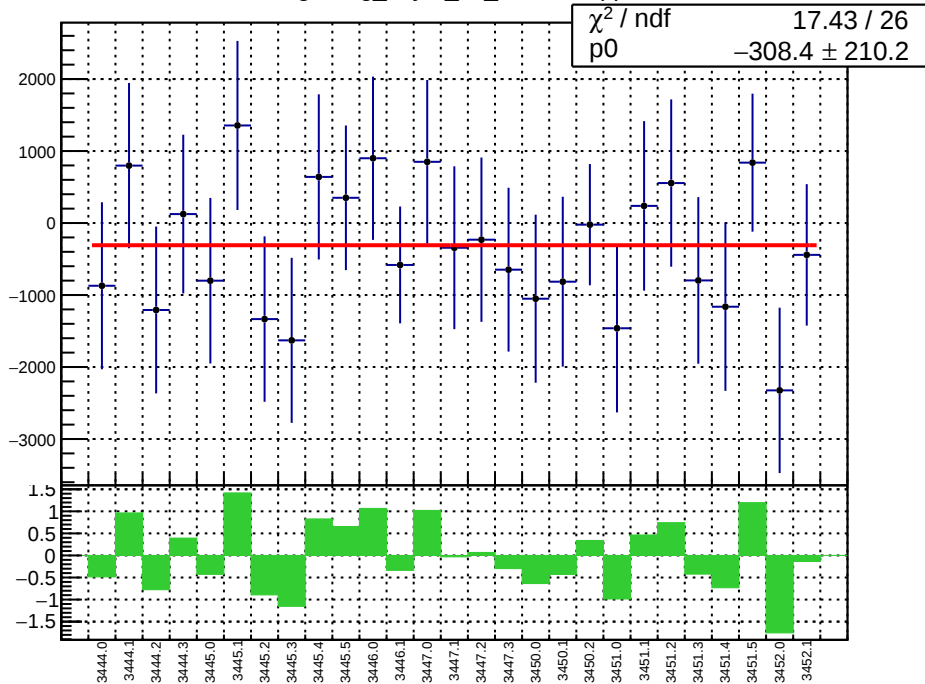
slug7: reg_asym_us_dd.mean/ppb
