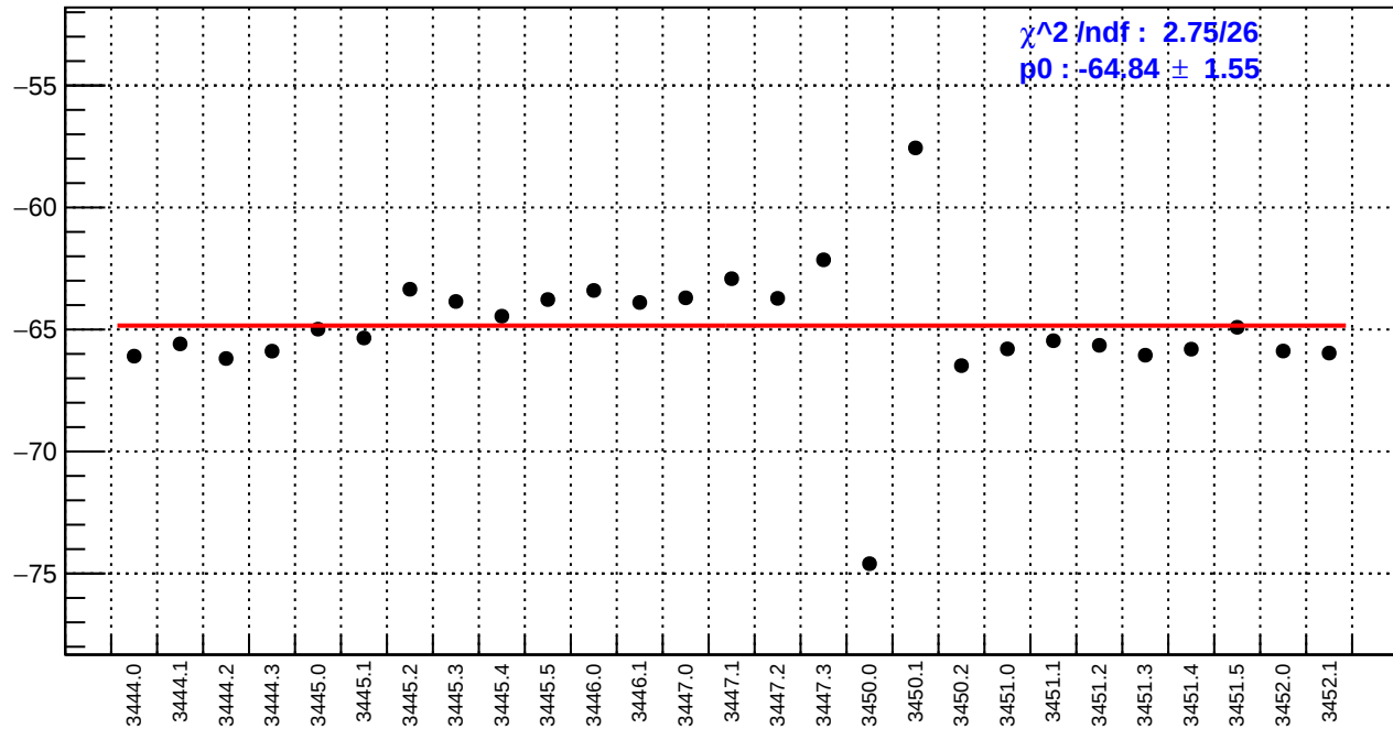
slug7: left_avg_bpm4eX/(ppb/nm)
