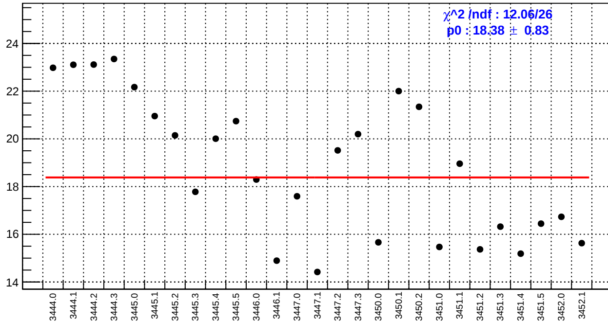
slug7: right_avg_bpm4aY/(ppb/nm)
