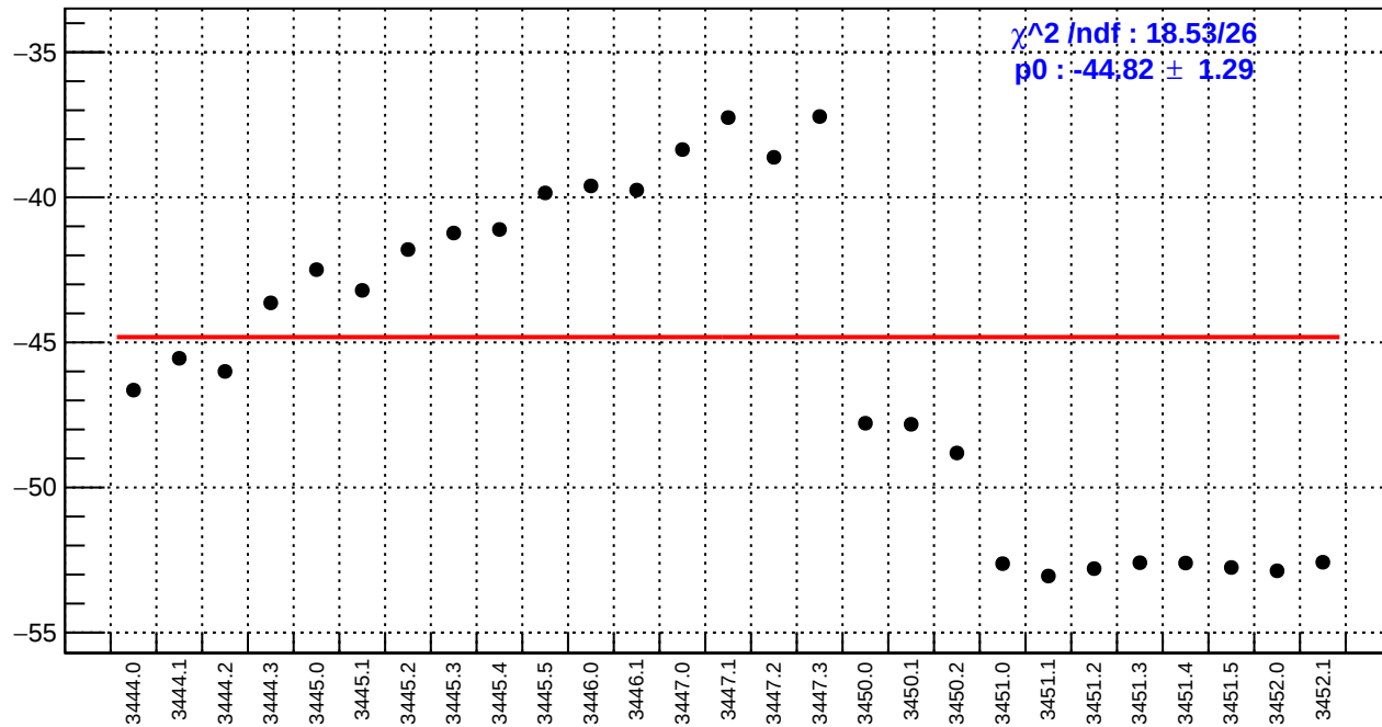
slug7: left_avg_bpm12X/(ppb/nm)
