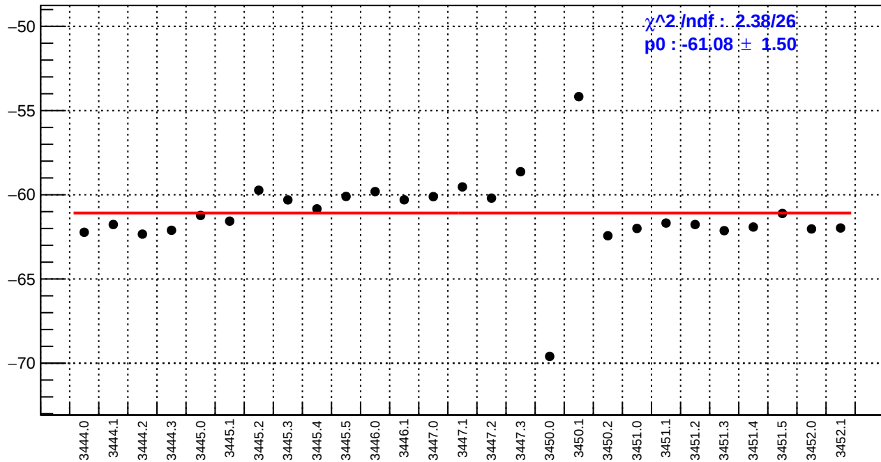
slug7: usl_bpm4eX/(ppb/nm)
