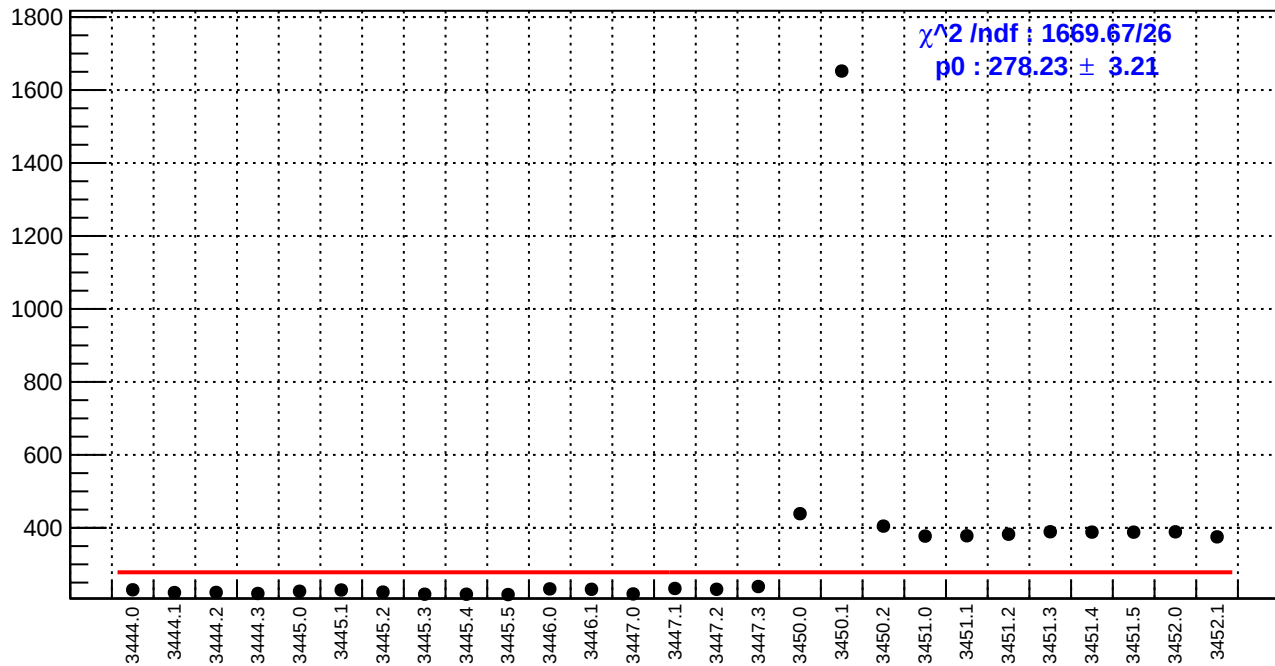
slug7: reg_asym_sam8.rms/ppm
