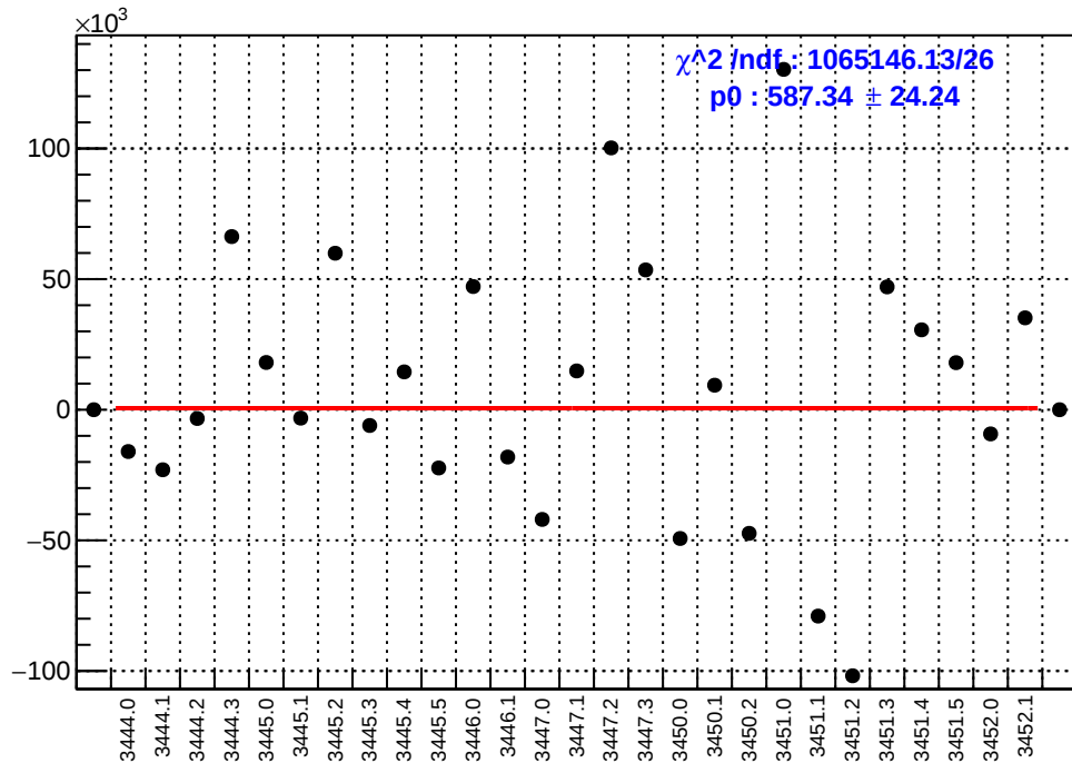
slug7: asym_sam4.mean/ppb-reg_asym_sam4.mean/ppb
