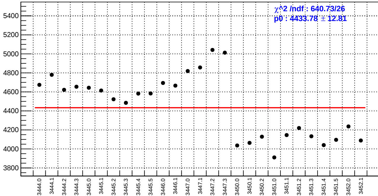
slug7: diff_bpm12X.rms/nm
