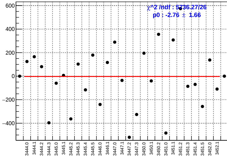
slug7: asym_left_dd.mean/ppb-reg_asym_left_dd.mean/ppb
