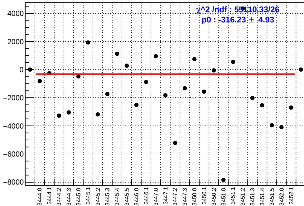
slug7: asym_dsr.mean/ppb-reg_asym_dsr.mean/ppb
