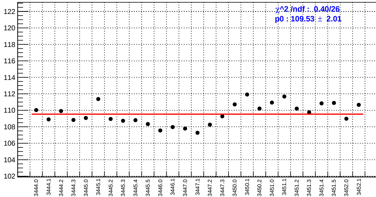
slug7: reg_asym_us_dd.rms/ppm
