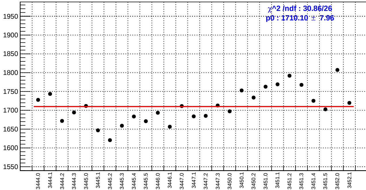
slug7: diff_bpm4aX.rms/nm
