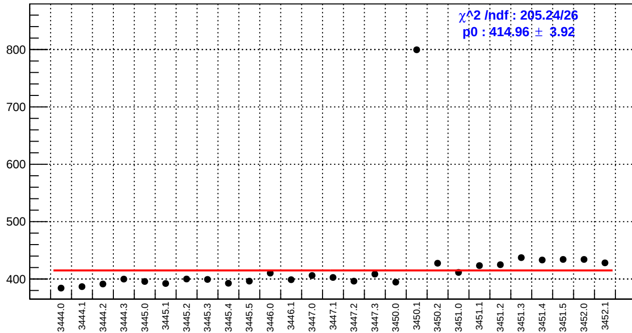
slug7: reg_asym_sam5.rms/ppm
