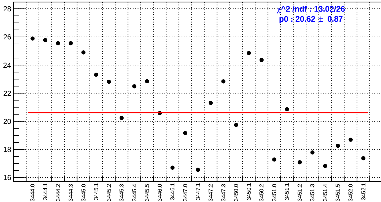
slug7: usr_bpm4aY/(ppb/nm)
