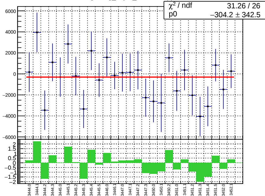
slug7: reg_asym_dsl.mean/ppb
