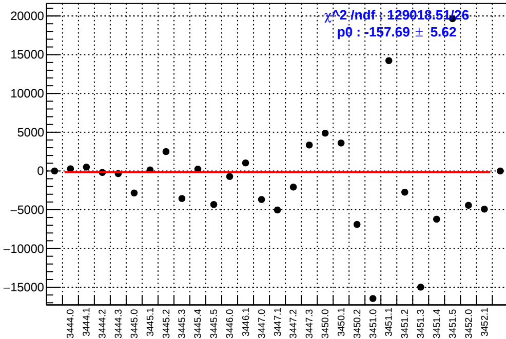
slug7: asym_sam1.mean/ppb-reg_asym_sam1.mean/ppb
