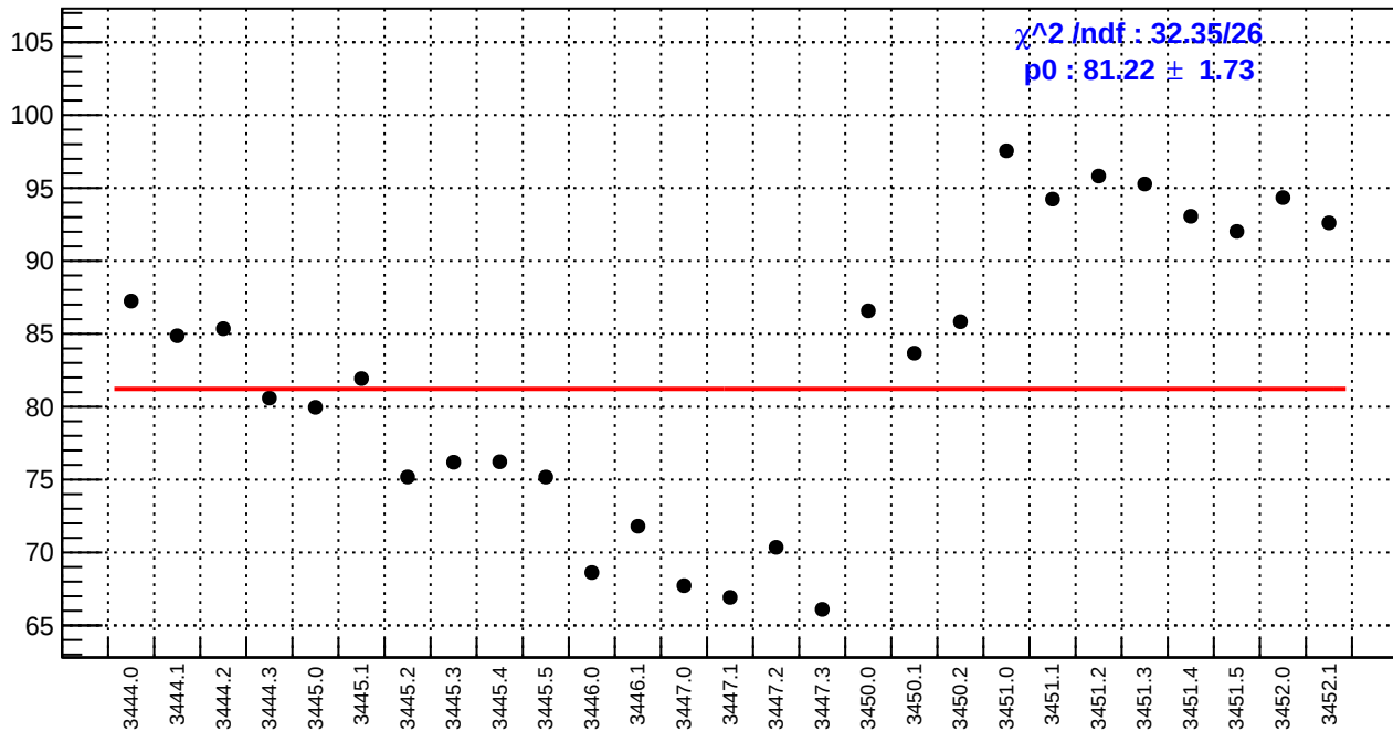
slug7: us_avg_bpm4aX/(ppb/nm)
