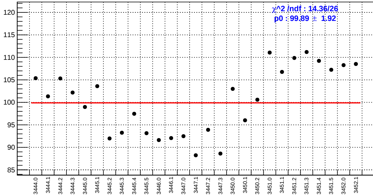
slug7: left_avg_bpm4aX/(ppb/nm)
