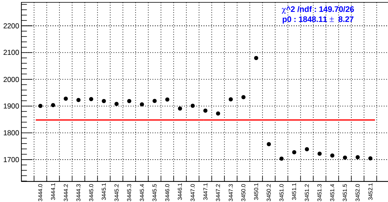
slug7: reg_asym_sam2.rms/ppm
