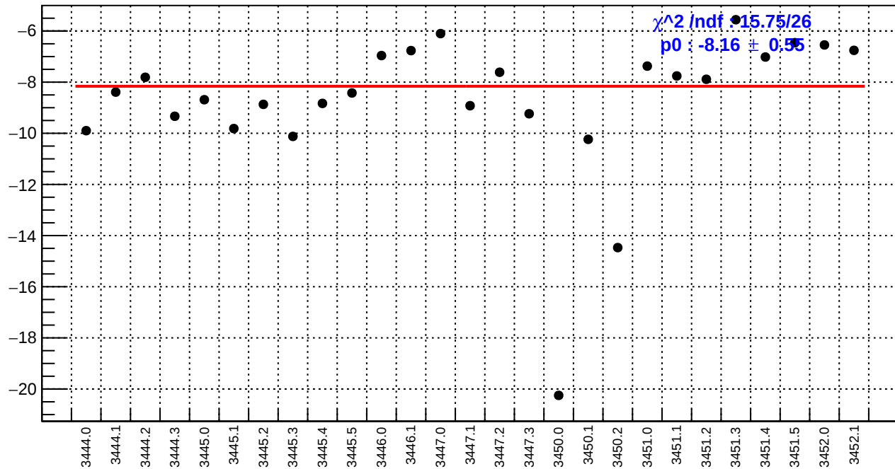
slug7: ds_avg_bpm4aY/(ppb/nm)
