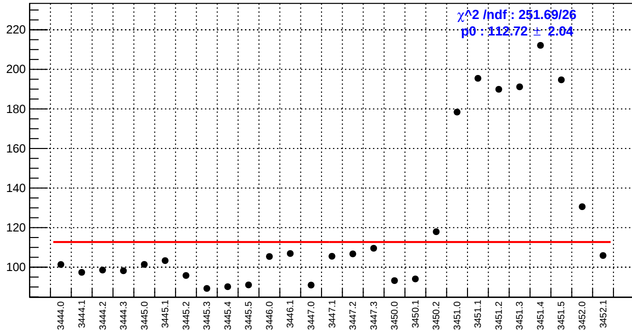
slug7: asym_bcm_an_us.rms/ppm
