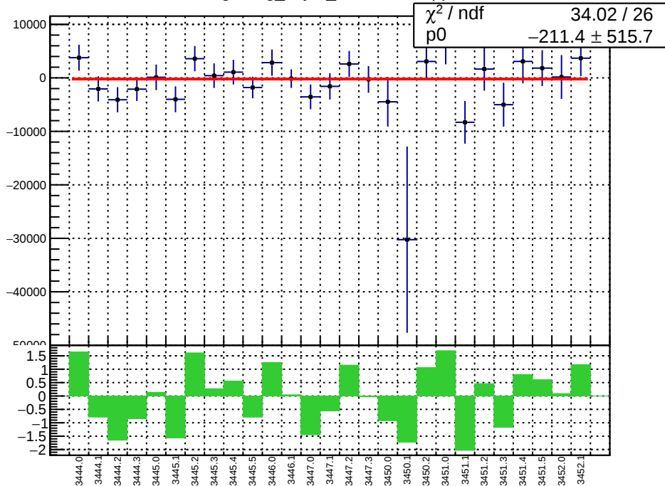
slug7: reg_asym_sam8.mean/ppb
