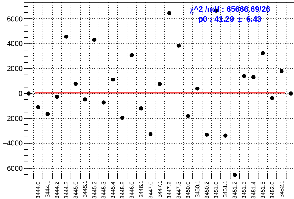
slug7: asym_ds_dd.mean/ppb-reg_asym_ds_dd.mean/ppb
