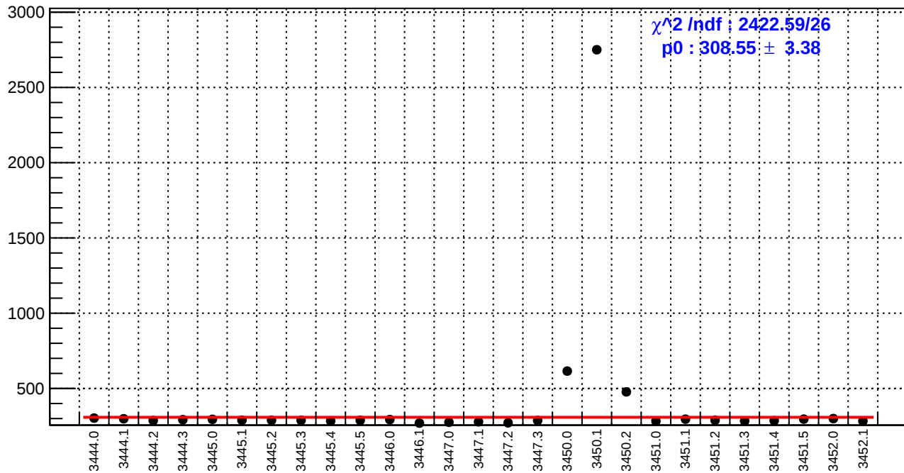
slug7: reg_asym_sam7.rms/ppm
