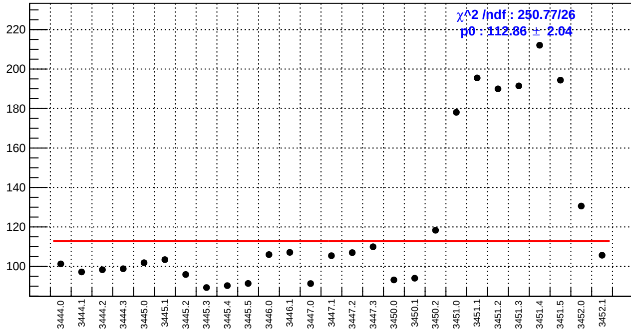
slug7: asym_bcm_an_ds.rms/ppm
