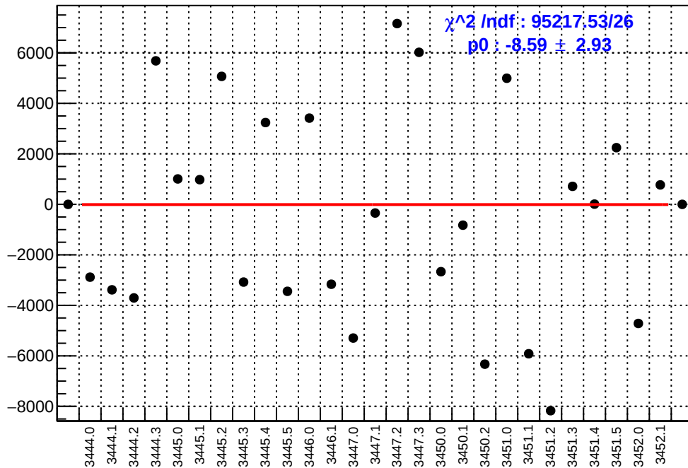
slug7: asym_left_avg.mean/ppb-reg_asym_left_avg.mean/ppb
