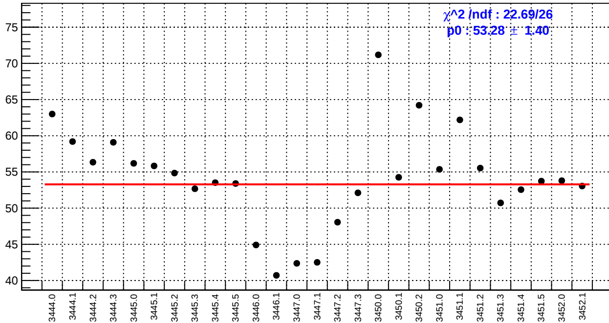
slug7: left_avg_bpm4eY/(ppb/nm)
