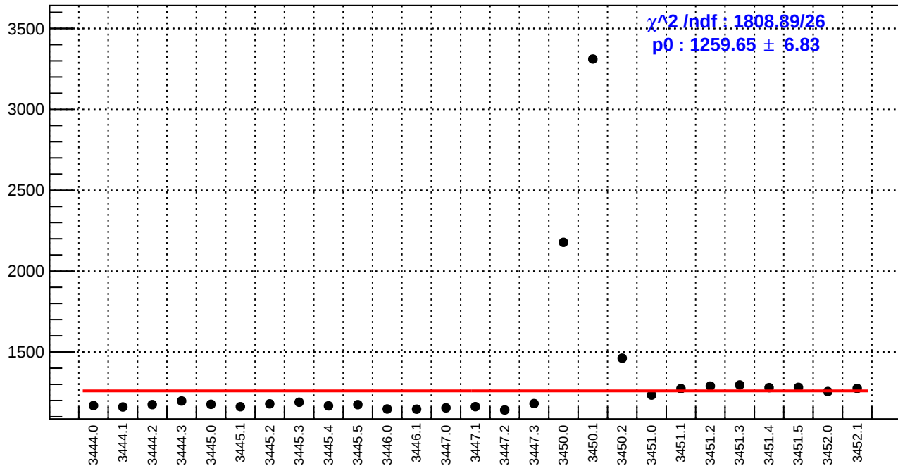
slug7: reg_asym_sam4.rms/ppm
