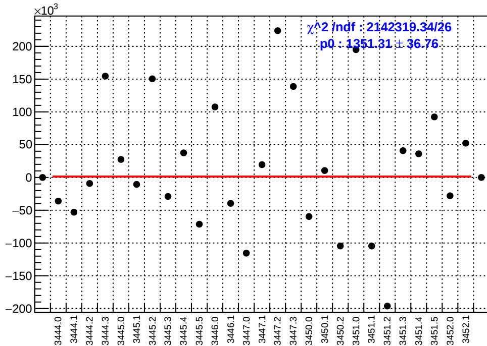
slug7: asym_sam3.mean/ppb-reg_asym_sam3.mean/ppb
