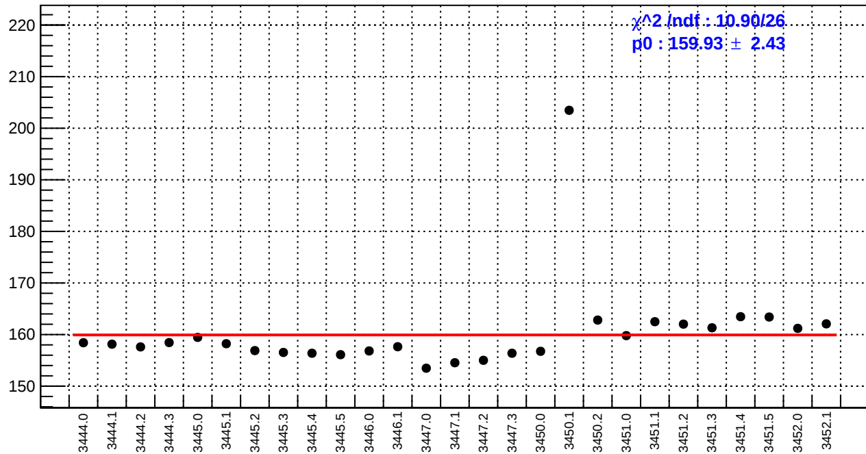
slug7: reg_asym_usr.rms/ppm
