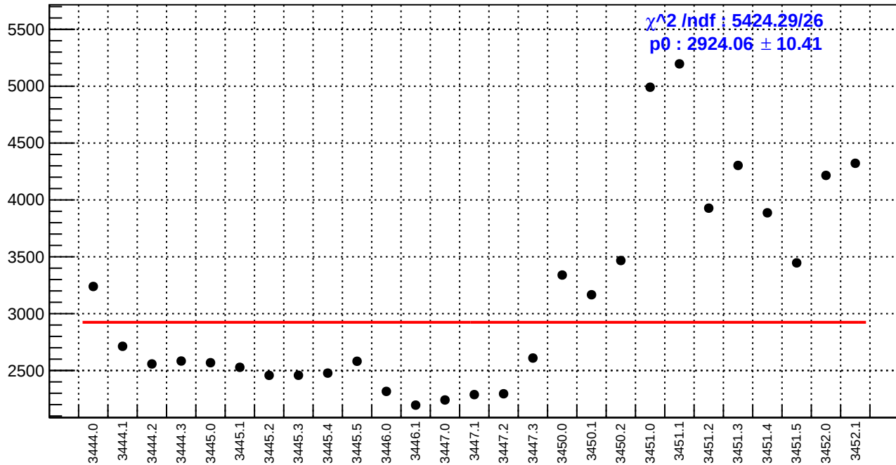
slug7: diff_bpm4eY.rms/nm
