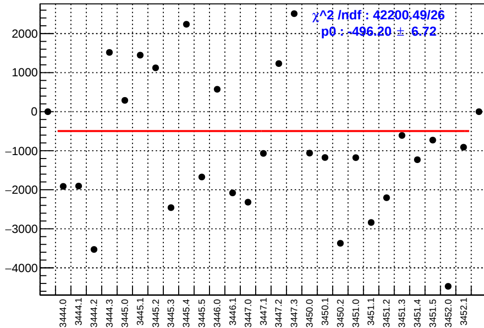
slug7: asym_ds_avg.mean/ppb-reg_asym_ds_avg.mean/ppb
