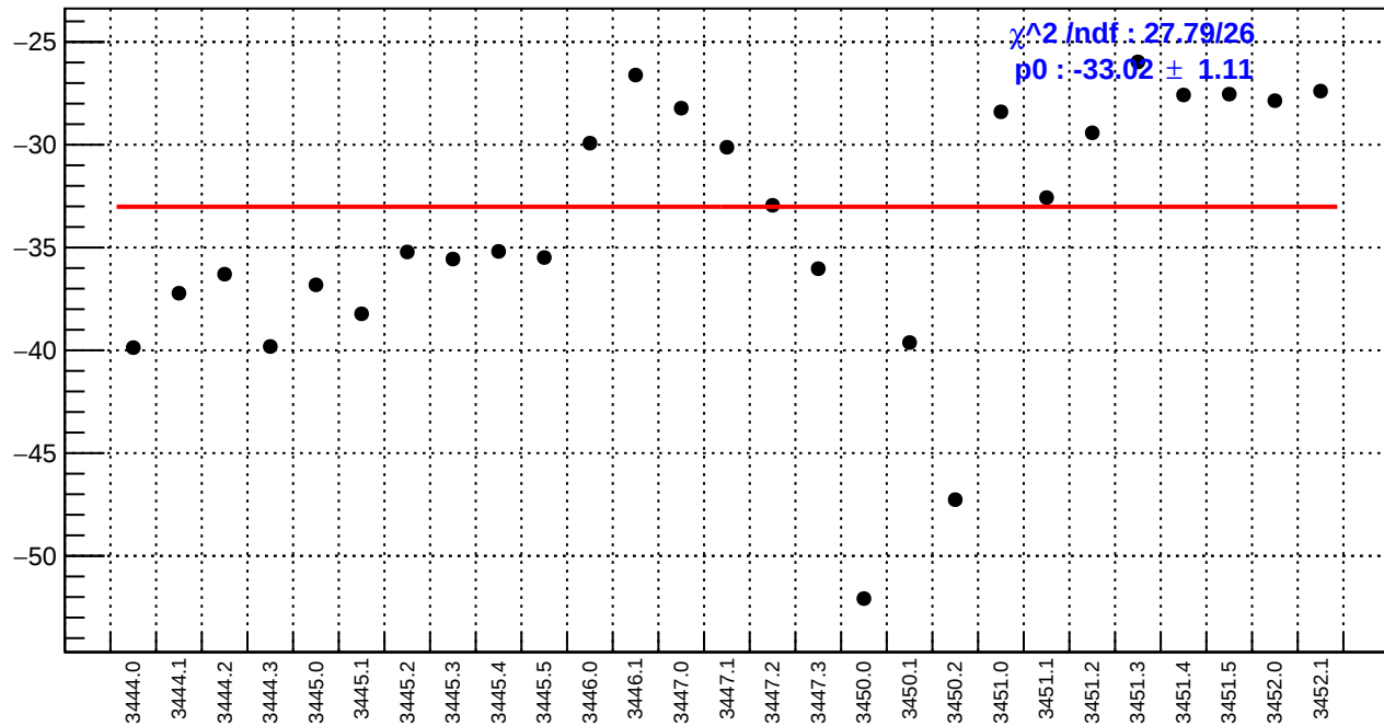
slug7: dsl_bpm4aY/(ppb/nm)
