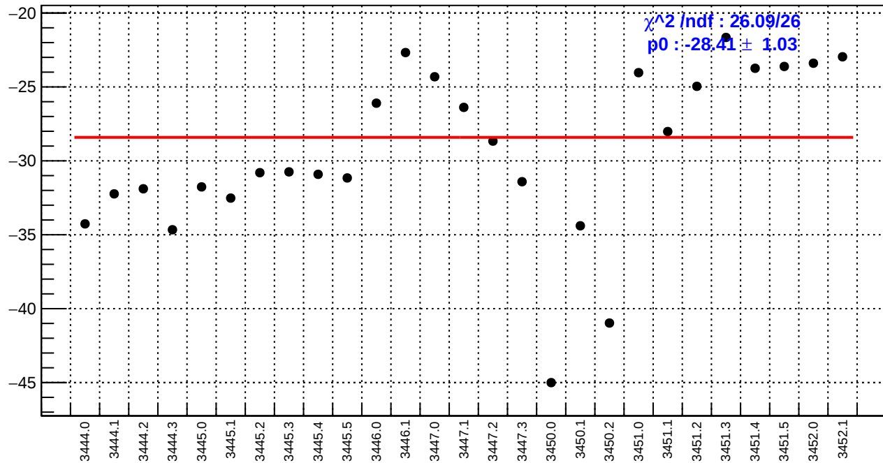
slug7: usl_bpm4aY/(ppb/nm)
