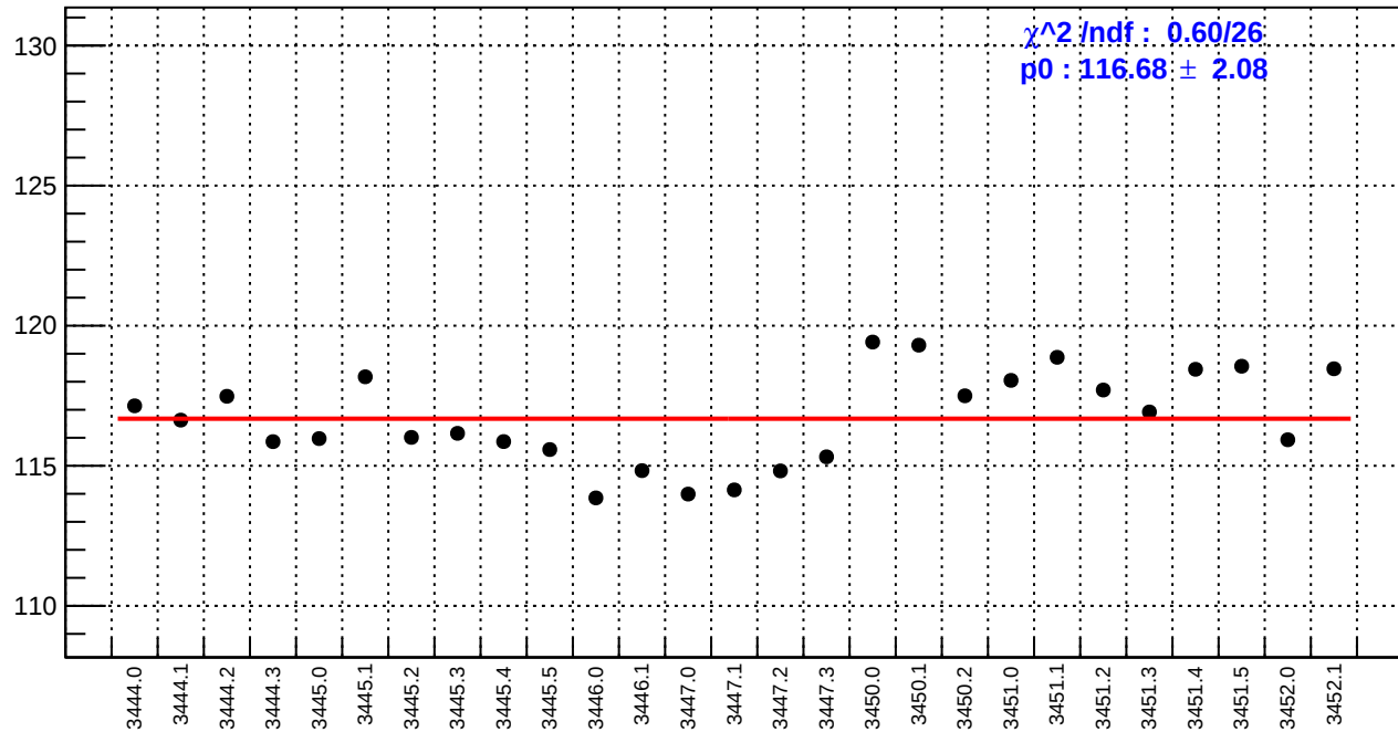
slug7: reg_asym_ds_dd.rms/ppm
