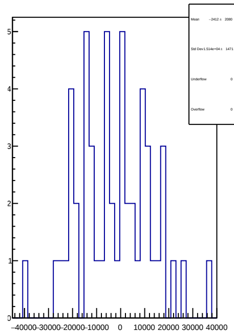
slug70: 1D Corr asym_atr1l2_dd.mean/ppb-reg_asym_atr1l2_dd.mean/ppb
