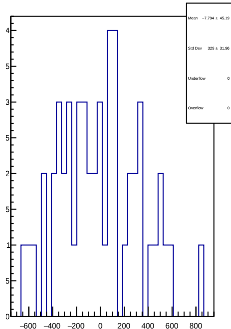
slug70: 1D Corr asym_right_dd.mean/ppb-reg_asym_right_dd.mean/ppb
