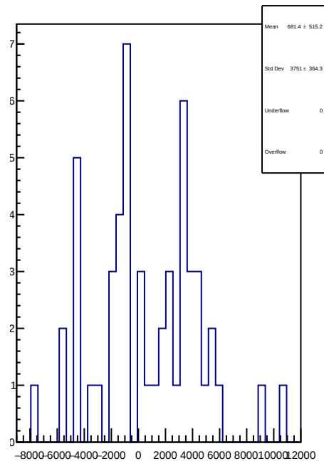
slug70: 1D Corr asym_usr.mean/ppb-reg_asym_usr.mean/ppb
