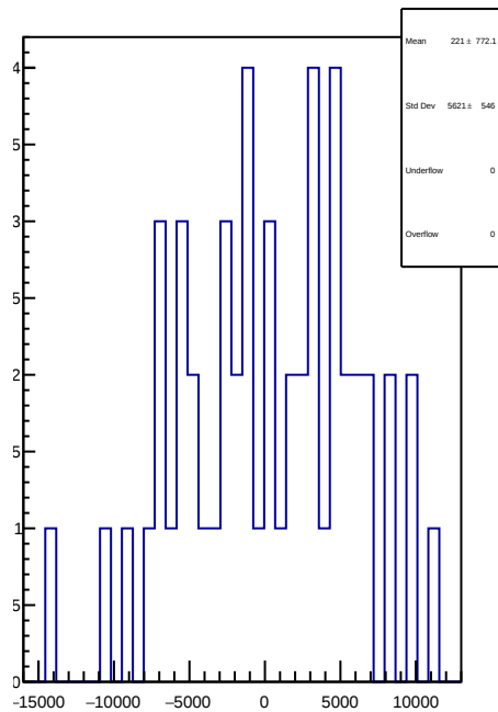
slug70: 1D Corr asym_usl.mean/ppb-reg_asym_usl.mean/ppb
