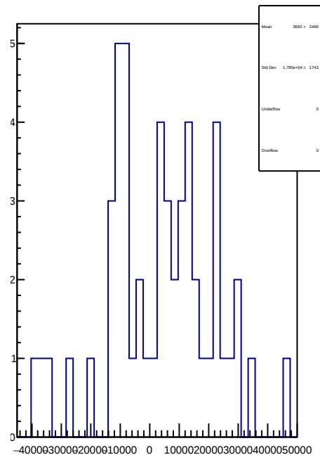
slug70: 1D Corr asym_atr2.mean/ppb-reg_asym_atr2.mean/ppb
