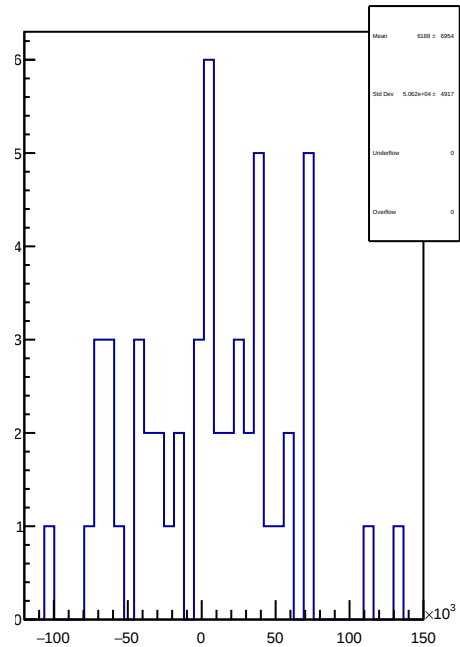
slug70: 1D Corr asym_sam4.mean/ppb-reg_asym_sam4.mean/ppb
