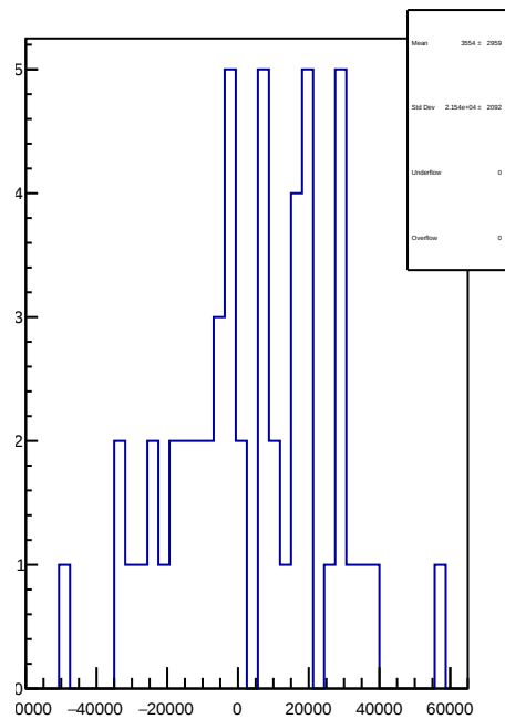
slug70: 1D Corr asym_at2_avg.mean/ppb-reg_asym_at2_avg.mean/ppb
