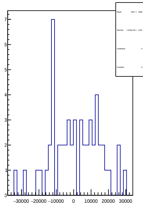
slug70: 1D Corr asym_atr1l2_avg.mean/ppb-reg_asym_atr1l2_avg.mean/ppb
