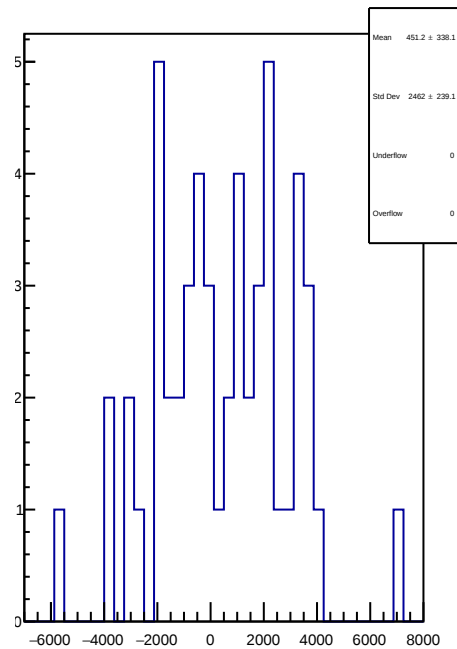
slug70: 1D Corr asym_us_avg.mean/ppb-reg_asym_us_avg.mean/ppb
