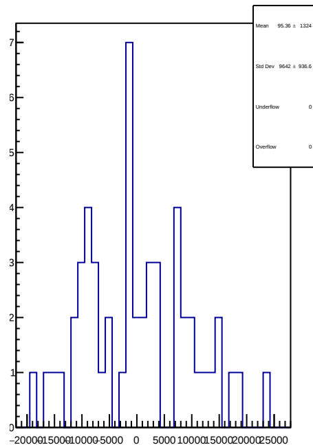
slug70: 1D Corr asym_at2_dd.mean/ppb-reg_asym_at2_dd.mean/ppb
