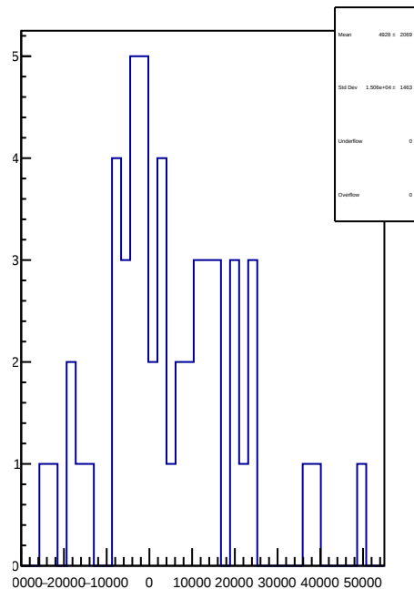
slug70: 1D Corr asym_sam5.mean/ppb-reg_asym_sam5.mean/ppb
