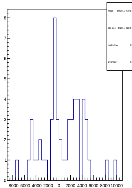
slug70: 1D Corr asym_dsr.mean/ppb-reg_asym_dsr.mean/ppb
