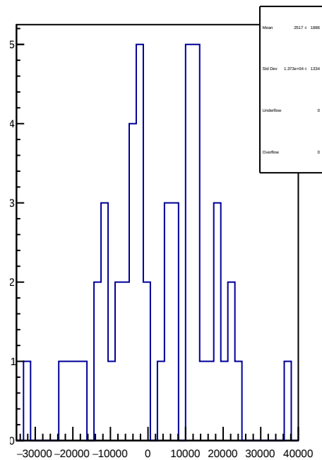
slug70: 1D Corr asym_atl_avg.mean/ppb-reg_asym_atl_avg.mean/ppb
