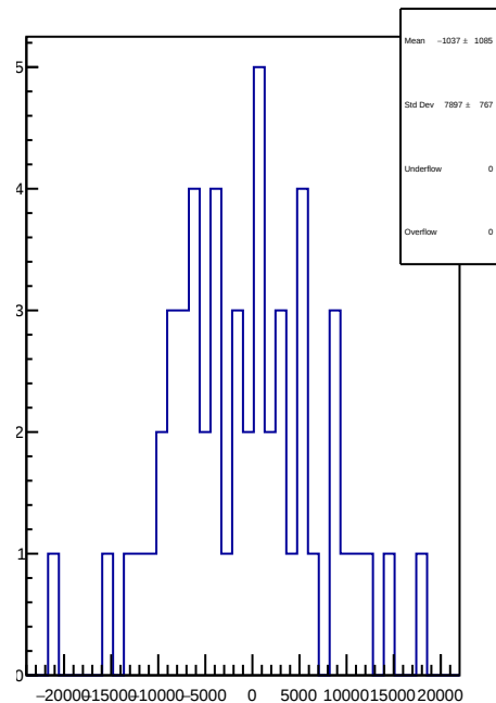
slug70: 1D Corr asym_atl1r2_dd.mean/ppb-reg_asym_atl1r2_dd.mean/ppb
