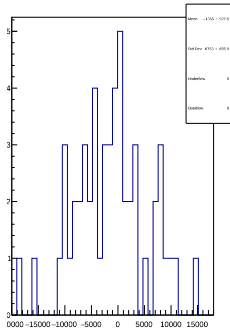
slug70: 1D Corr asym_atr1.mean/ppb-reg_asym_atr1.mean/ppb
