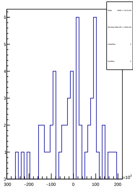
slug70: 1D Corr asym_sam3.mean/ppb-reg_asym_sam3.mean/ppb
