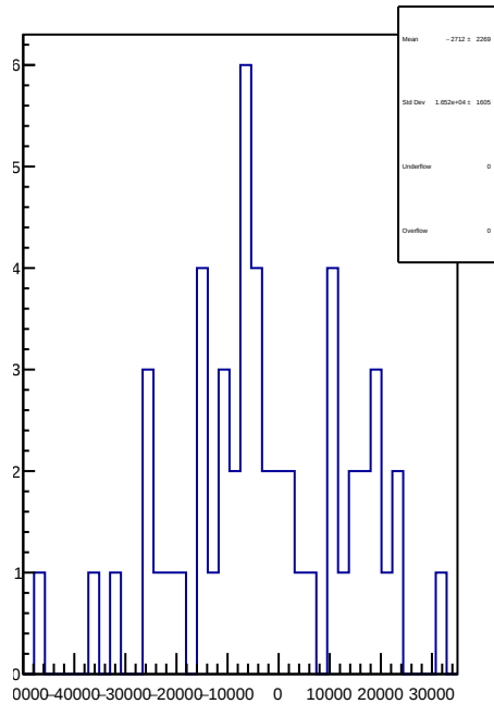
slug70: 1D Corr asym_sam8.mean/ppb-reg_asym_sam8.mean/ppb
