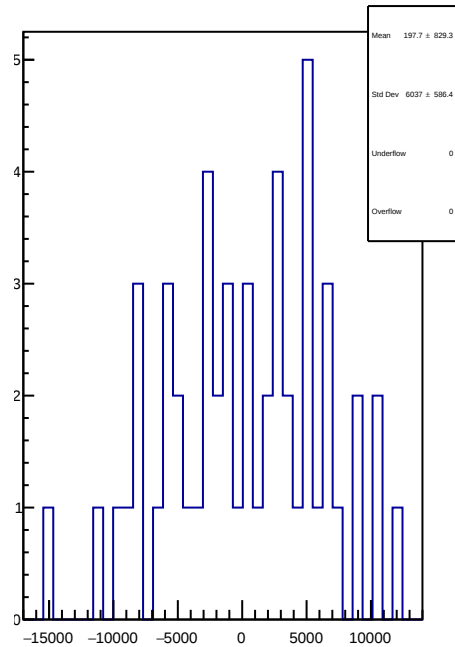
slug70: 1D Corr asym_dsl.mean/ppb-reg_asym_dsl.mean/ppb
