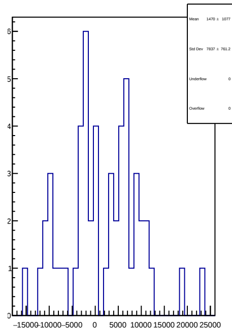
slug70: 1D Corr asym_at1_dd.mean/ppb-reg_asym_at1_dd.mean/ppb
