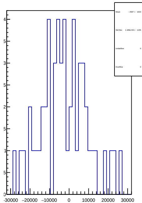
slug70: 1D Corr asym_atr_dd.mean/ppb-reg_asym_atr_dd.mean/ppb
