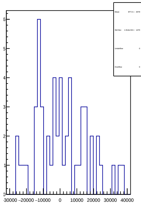
slug70: 1D Corr asym_sam7.mean/ppb-reg_asym_sam7.mean/ppb
