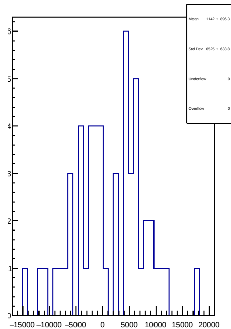
slug70: 1D Corr asym_atr_avg.mean/ppb-reg_asym_atr_avg.mean/ppb
