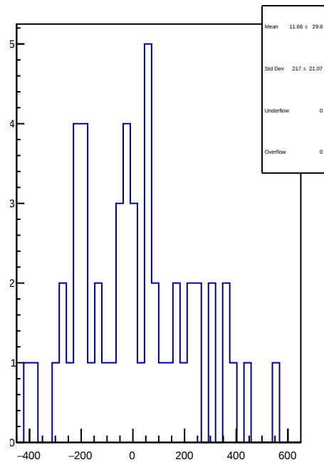
slug70: 1D Corr asym_left_dd.mean/ppb-reg_asym_left_dd.mean/ppb
