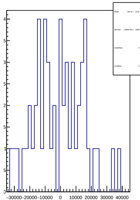
slug70: 1D Corr asym_atl_dd.mean/ppb-reg_asym_atl_dd.mean/ppb
