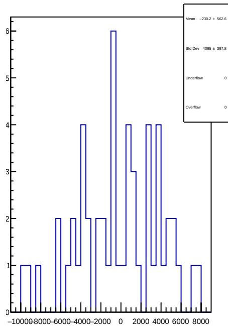
slug70: 1D Corr asym_us_dd.mean/ppb-reg_asym_us_dd.mean/ppb
