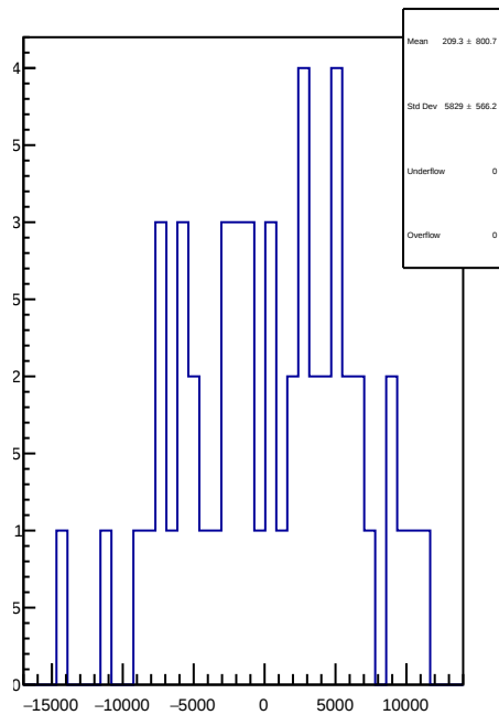
slug70: 1D Corr asym_left_avg.mean/ppb-reg_asym_left_avg.mean/ppb
