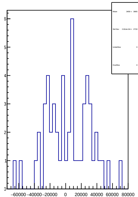
slug70: 1D Corr asym_atl2.mean/ppb-reg_asym_atl2.mean/ppb
