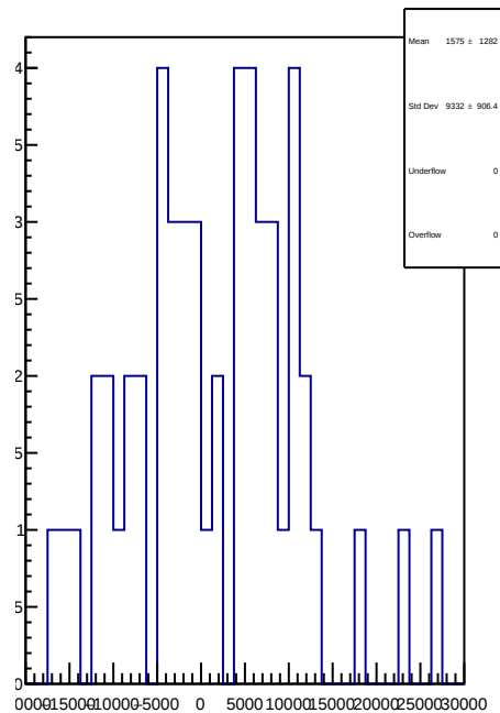
slug70: 1D Corr asym_atl1.mean/ppb-reg_asym_atl1.mean/ppb
