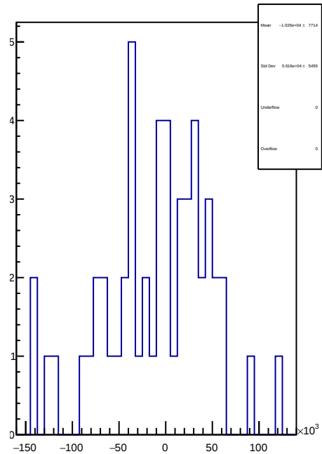
slug70: 1D Corr asym_sam2.mean/ppb-reg_asym_sam2.mean/ppb
