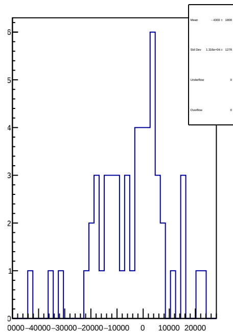
slug70: 1D Corr asym_sam1.mean/ppb-reg_asym_sam1.mean/ppb
