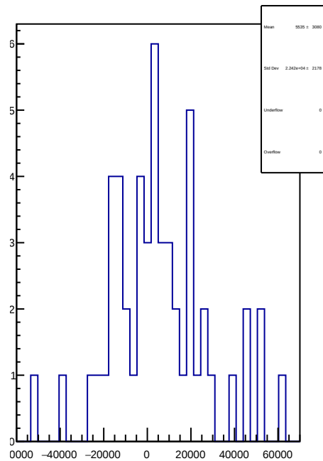
slug70: 1D Corr asym_sam6.mean/ppb-reg_asym_sam6.mean/ppb
