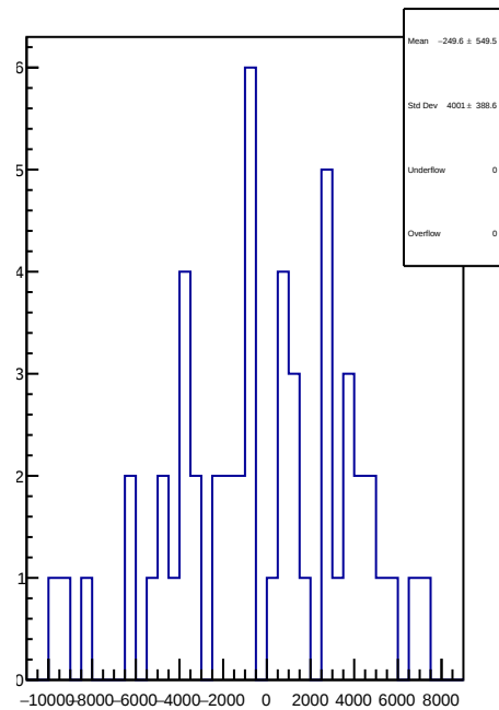
slug70: 1D Corr asym_ds_dd.mean/ppb-reg_asym_ds_dd.mean/ppb
