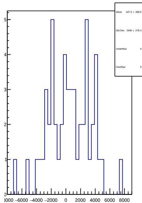
slug70: 1D Corr asym_ds_avg.mean/ppb-reg_asym_ds_avg.mean/ppb
