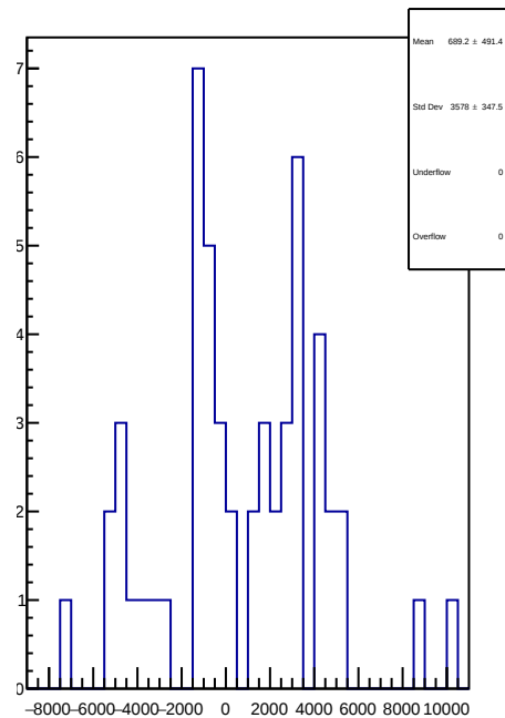
slug70: 1D Corr asym_right_avg.mean/ppb-reg_asym_right_avg.mean/ppb
