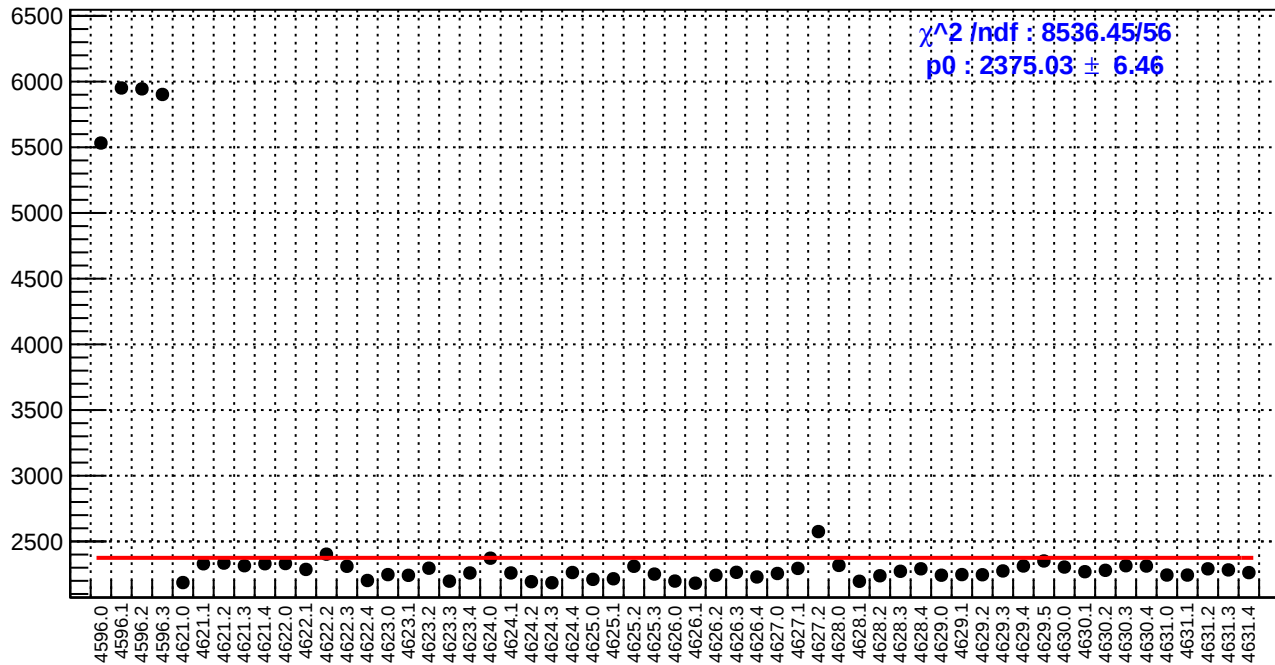
slug71: diff_bpm4eY.rms/nm
