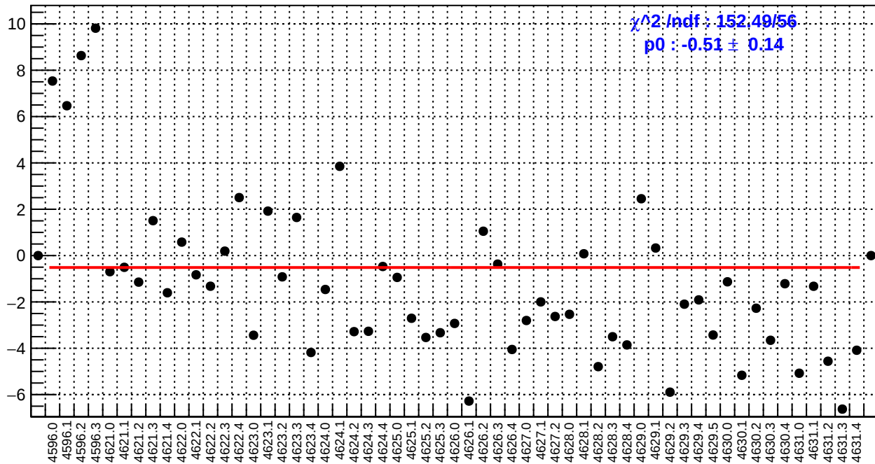
slug71: usr_bpm4aY/(ppb/nm)
