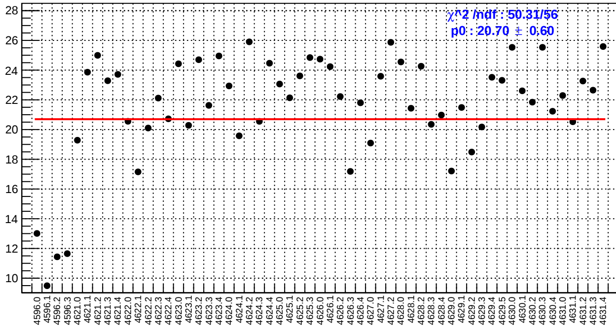
slug71: dsl_bpm4eY/(ppb/nm)
