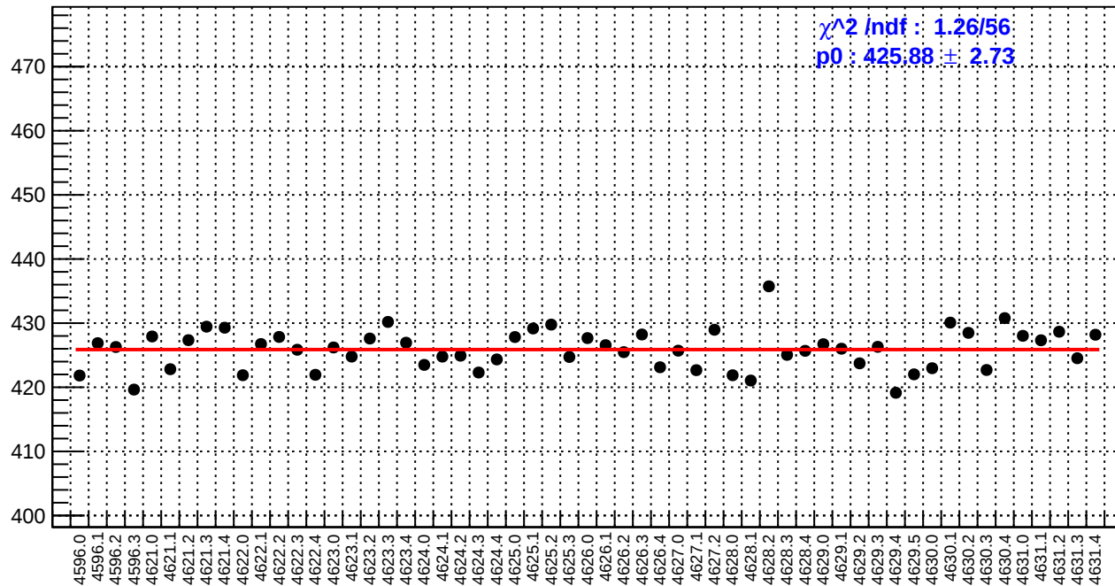
slug71: reg_asym_atl1r2_avg.rms/ppm
