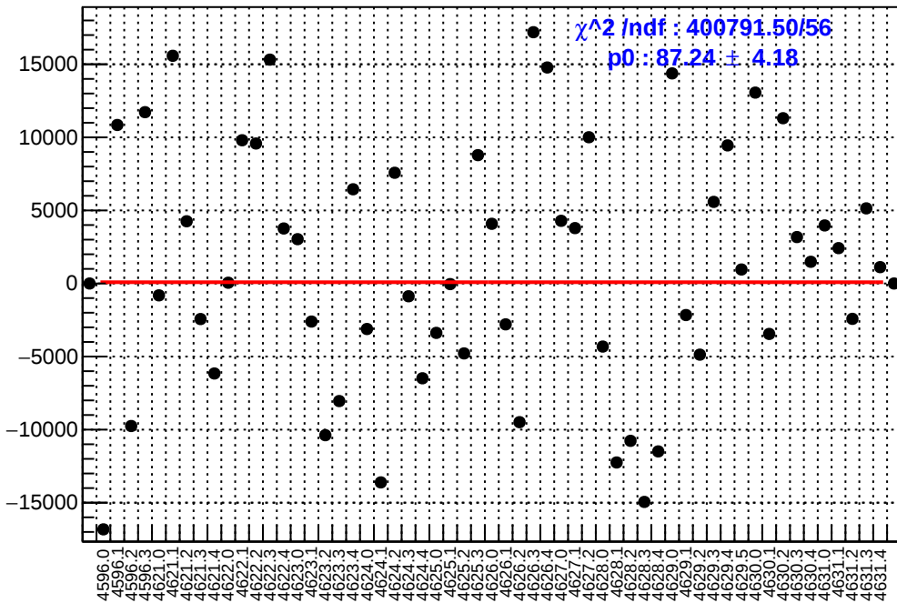
slug71: asym_at2_dd.mean/ppb-reg_asym_at2_dd.mean/ppb
