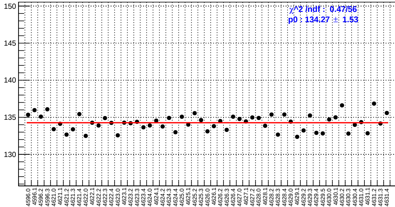
slug71: reg_asym_left_avg.rms/ppm
