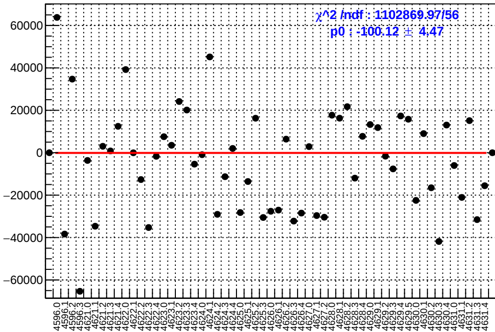
slug71: asym_atl2.mean/ppb-reg_asym_atl2.mean/ppb
