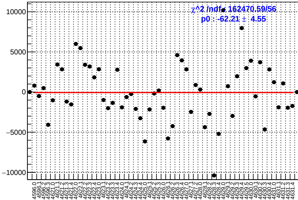
slug71: asym_dsr.mean/ppb-reg_asym_dsr.mean/ppb
