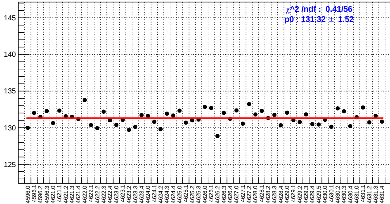
slug71: reg_asym_usr.rms/ppm
