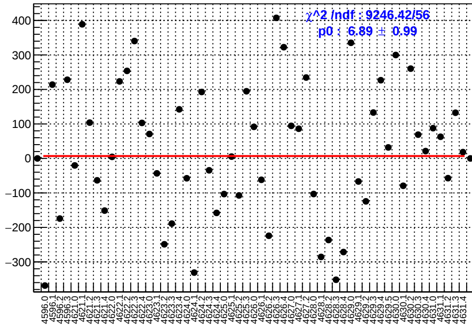
slug71: asym_left_dd.mean/ppb-reg_asym_left_dd.mean/ppb
