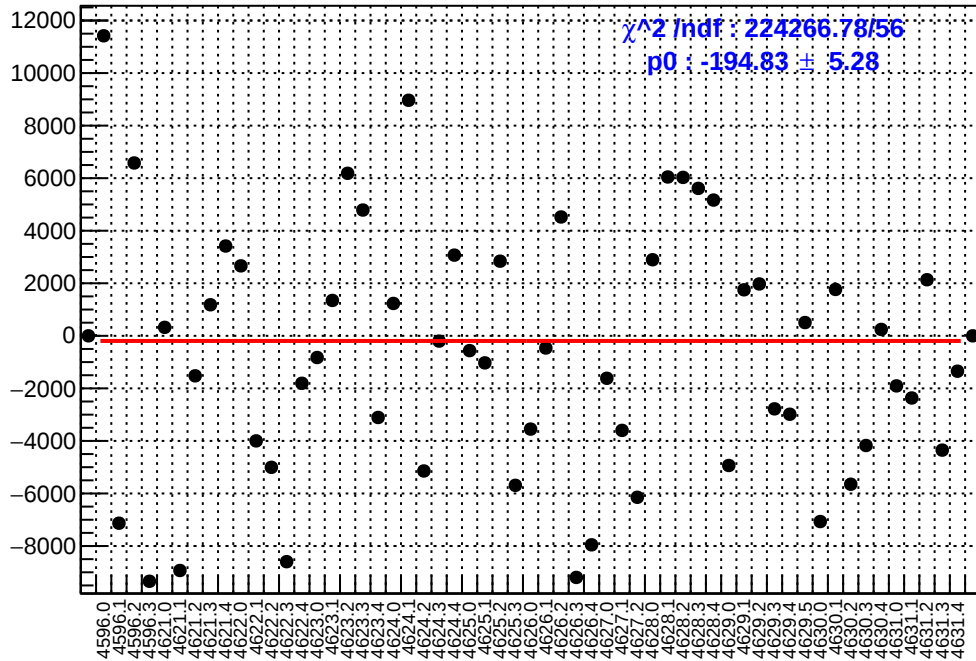
slug71: asym_usl.mean/ppb-reg_asym_usl.mean/ppb
