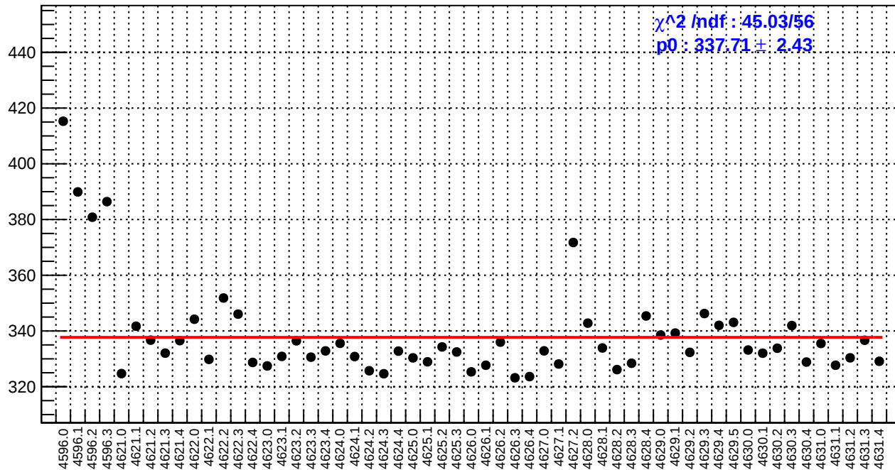
slug71: reg_asym_sam6.rms/ppm
