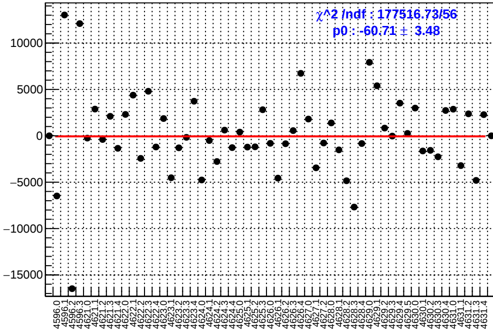
slug71: asym_sam1.mean/ppb-reg_asym_sam1.mean/ppb
