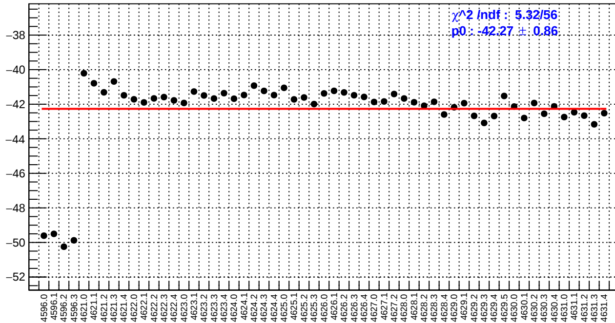
slug71: usl_bpm12X/(ppb/nm)
