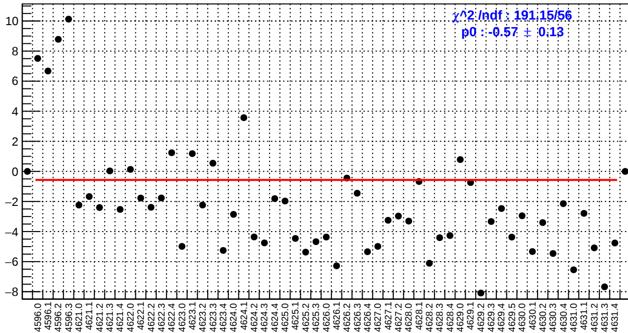
slug71: right_avg_bpm4aY/(ppb/nm)
