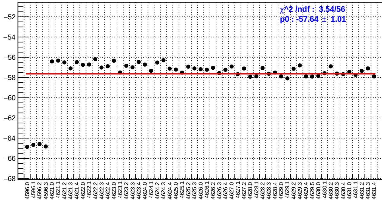
slug71: right_avg_bpm12X/(ppb/nm)
