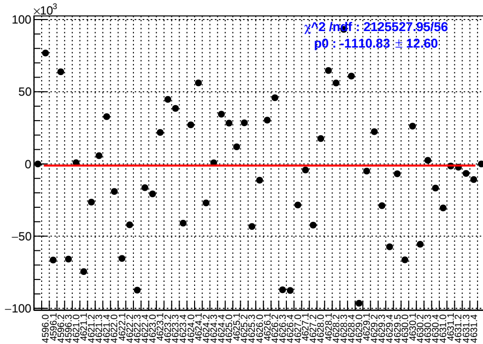
slug71: asym_sam4.mean/ppb-reg_asym_sam4.mean/ppb
