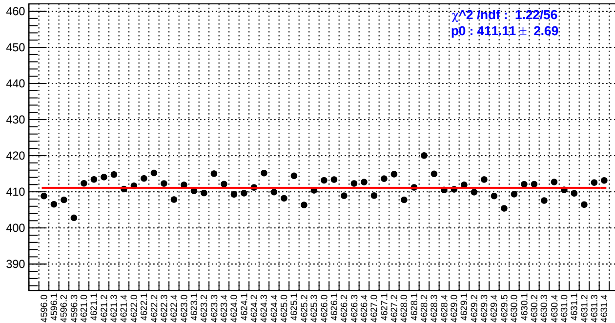
slug71: reg_asym_at1_avg.rms/ppm
