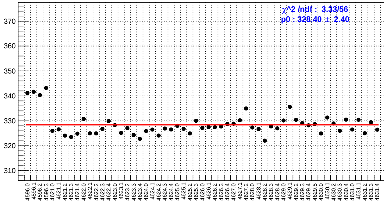
slug71: reg_asym_atr1l2_avg.rms/ppm
