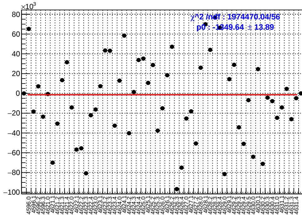
slug71: asym_sam2.mean/ppb-reg_asym_sam2.mean/ppb
