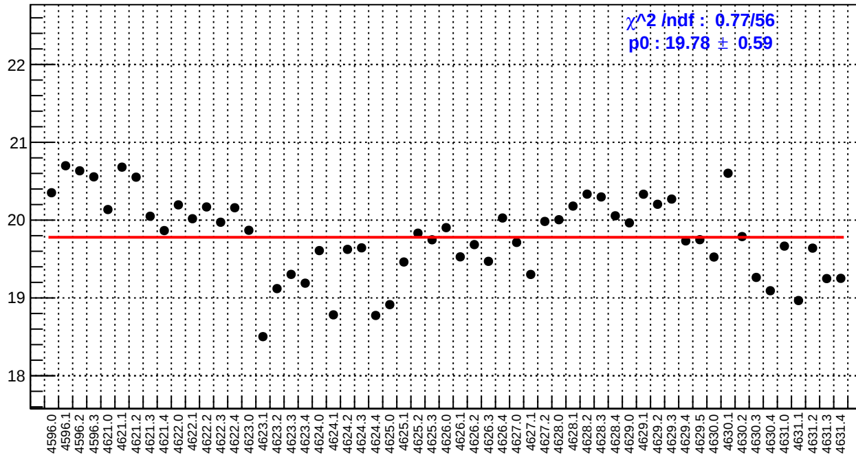
slug71: right_avg_bpm4eX/(ppb/nm)
