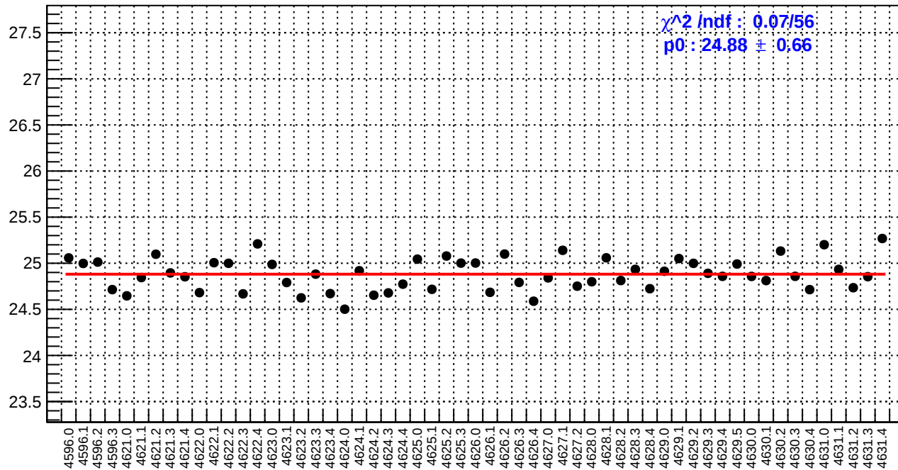
slug71: reg_asym_left_dd.rms/ppm
