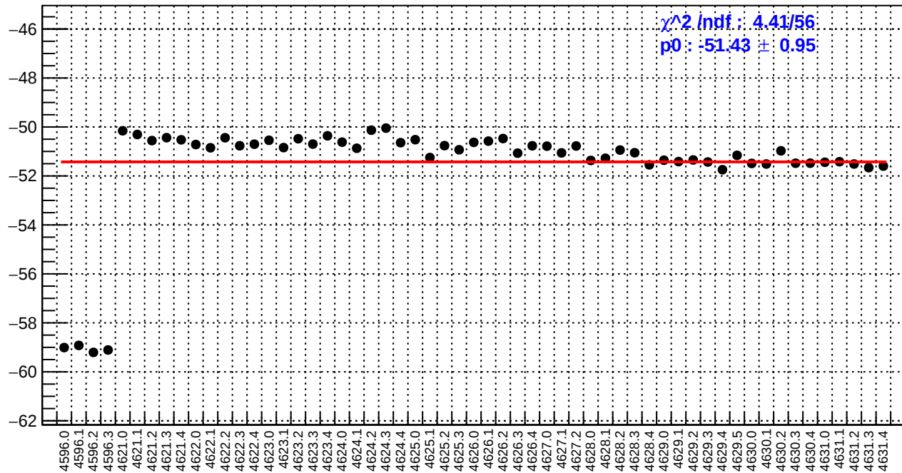
slug71: ds_avg_bpm12X/(ppb/nm)
