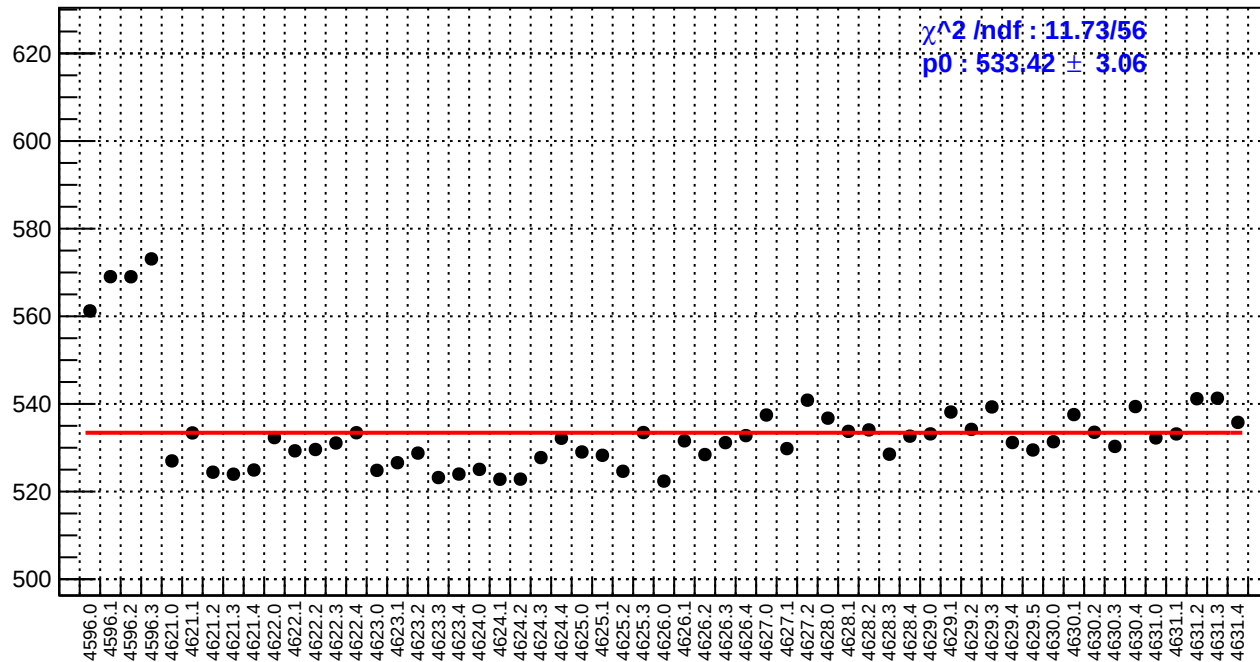
slug71: reg_asym_atl2.rms/ppm
