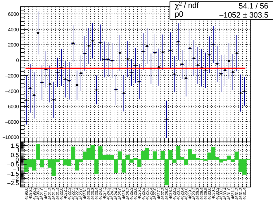
slug71: reg_asym_sam5.mean/ppb
