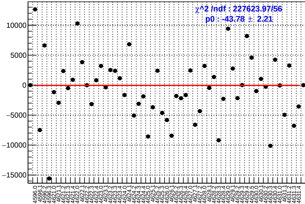
slug71: asym_atr_avg.mean/ppb-reg_asym_atr_avg.mean/ppb
