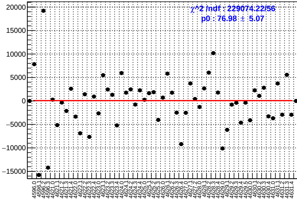
slug71: asym_sam5.mean/ppb-reg_asym_sam5.mean/ppb
