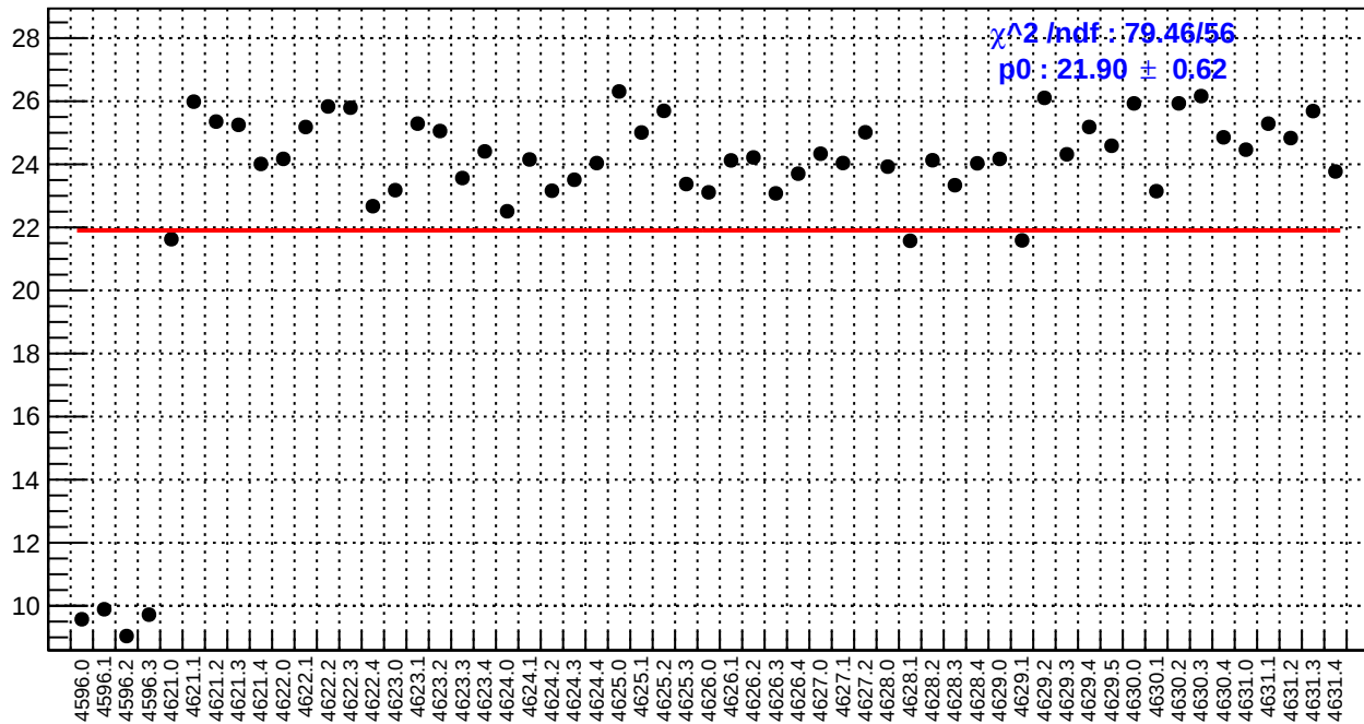
slug71: ds_avg_bpm4aX/(ppb/nm)
