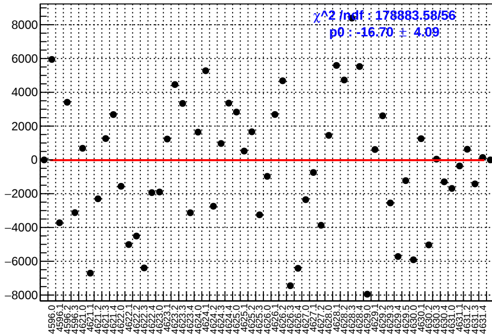
slug71: asym_us_dd.mean/ppb-reg_asym_us_dd.mean/ppb
