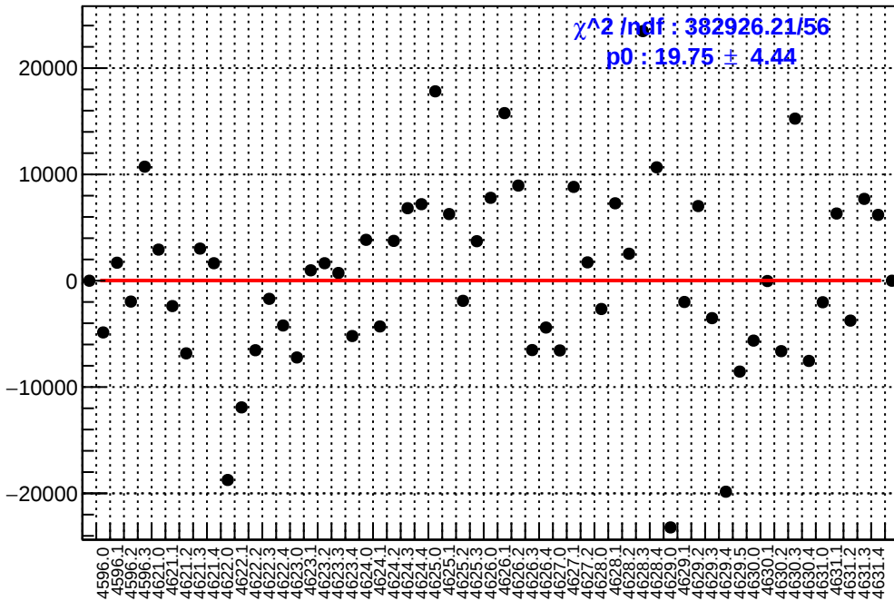
slug71: asym_atr1.mean/ppb-reg_asym_atr1.mean/ppb
