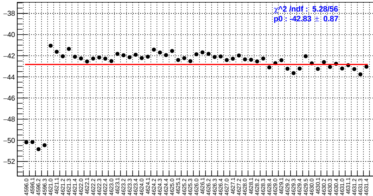
slug71: left_avg_bpm12X/(ppb/nm)
