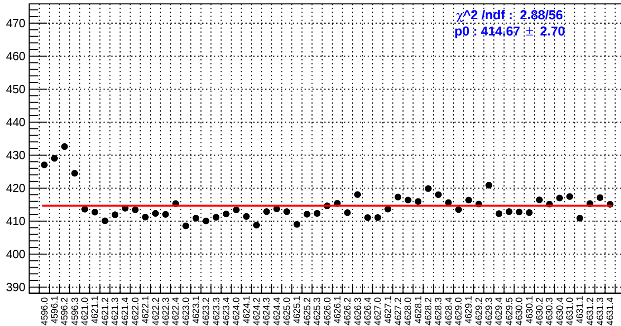
slug71: reg_asym_atl_dd.rms/ppm
