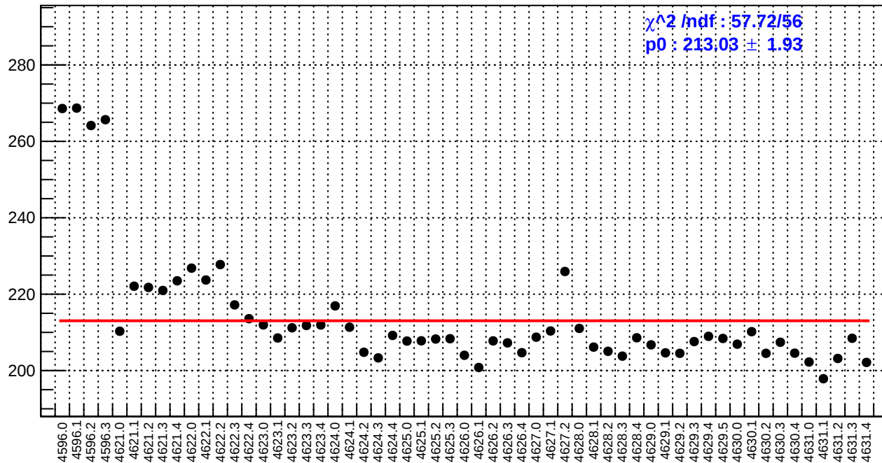
slug71: reg_asym_sam1.rms/ppm
