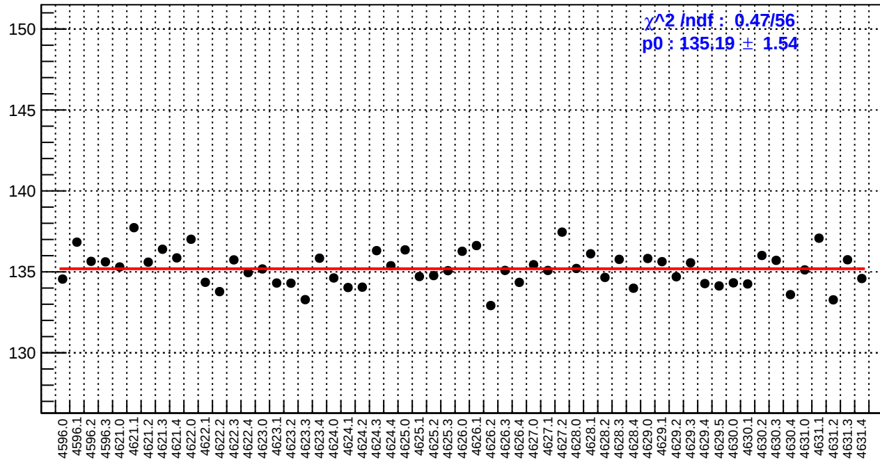
slug71: reg_asym_dsr.rms/ppm
