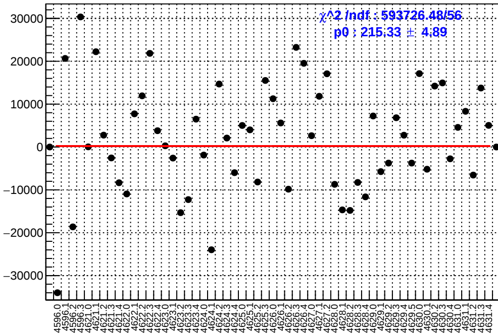
slug71: asym_atl_dd.mean/ppb-reg_asym_atl_dd.mean/ppb
