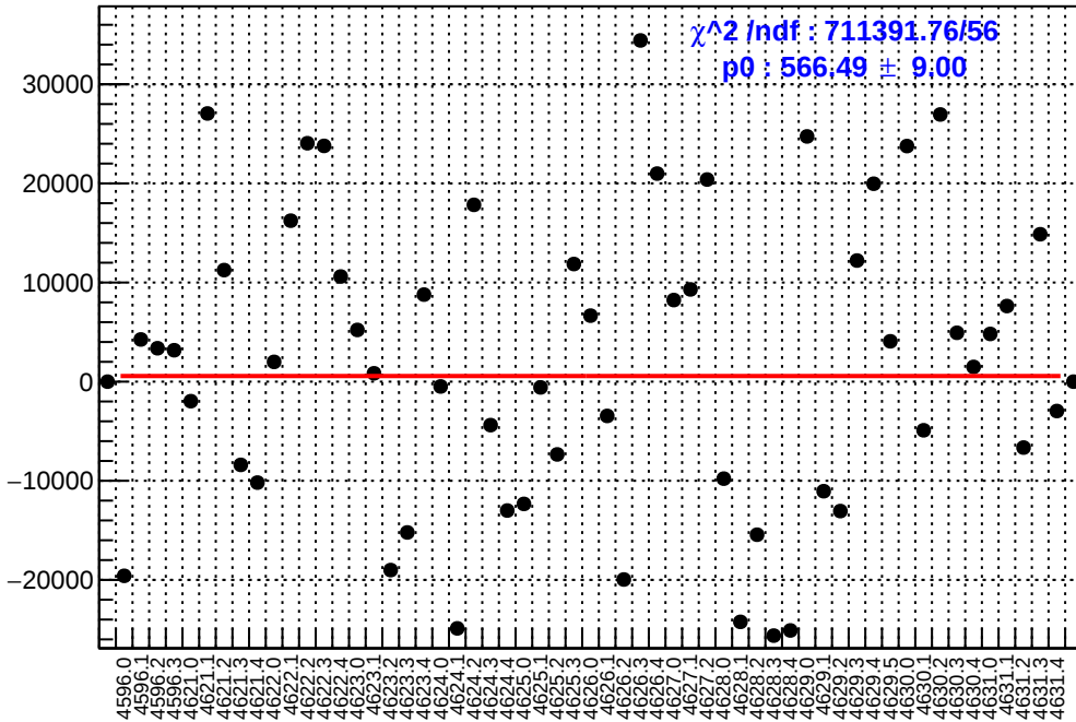
slug71: asym_sam6.mean/ppb-reg_asym_sam6.mean/ppb
