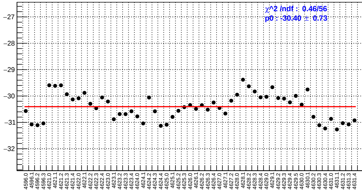
slug71: ds_avg_bpm4eX/(ppb/nm)
