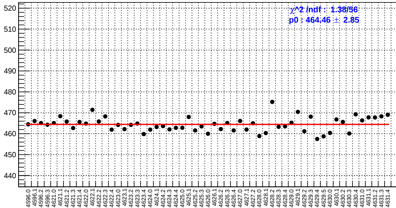
slug71: reg_asym_atl_avg.rms/ppm
