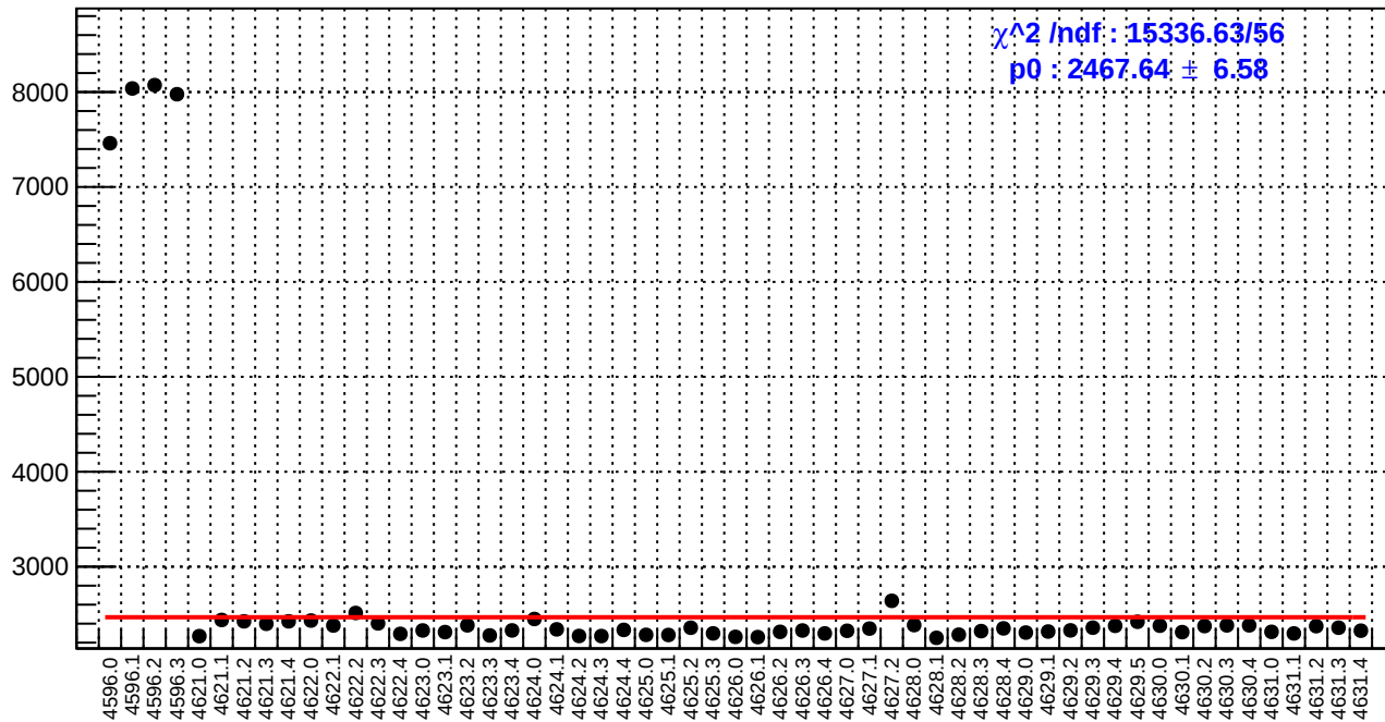
slug71: diff_bpm4aY.rms/nm
