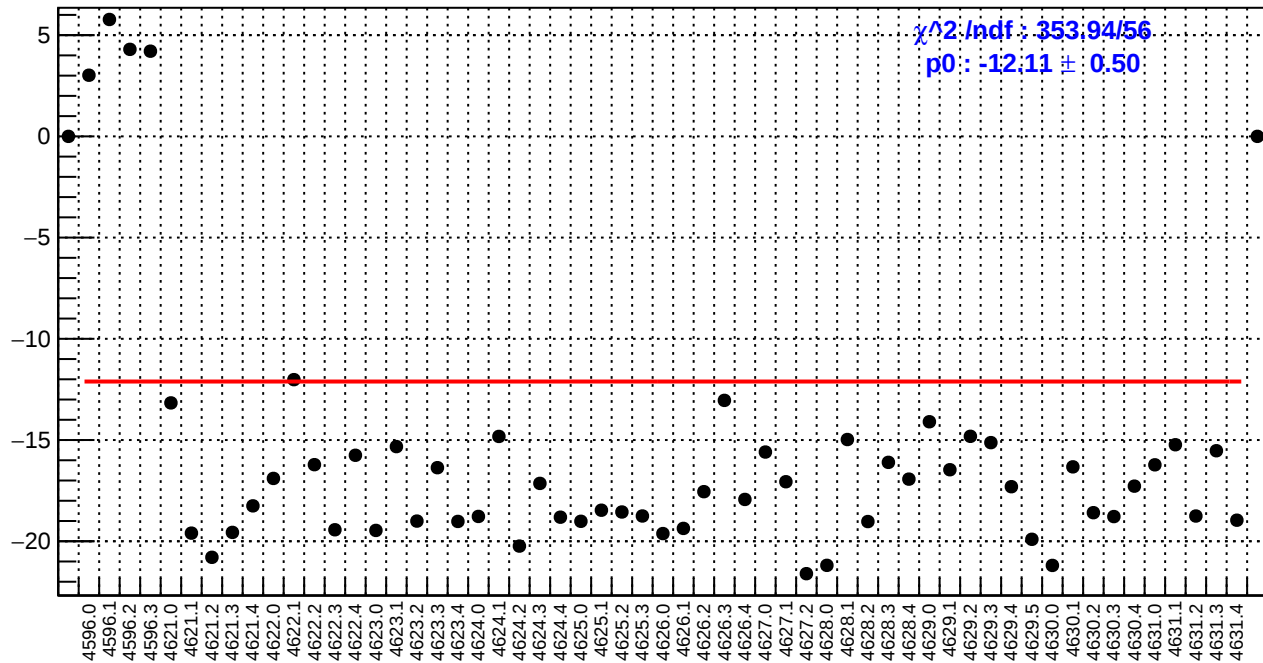
slug71: left_avg_bpm4aY/(ppb/nm)
