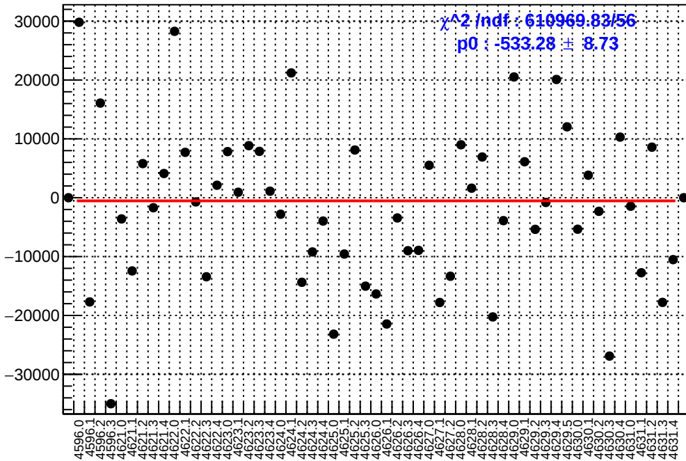
slug71: asym_atl_avg.mean/ppb-reg_asym_atl_avg.mean/ppb
