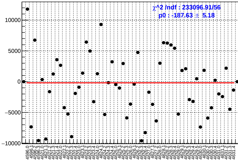
slug71: asym_left_avg.mean/ppb-reg_asym_left_avg.mean/ppb
