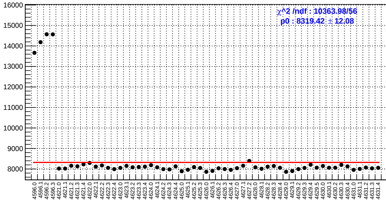
slug71: diff_bpm4eX.rms/nm
