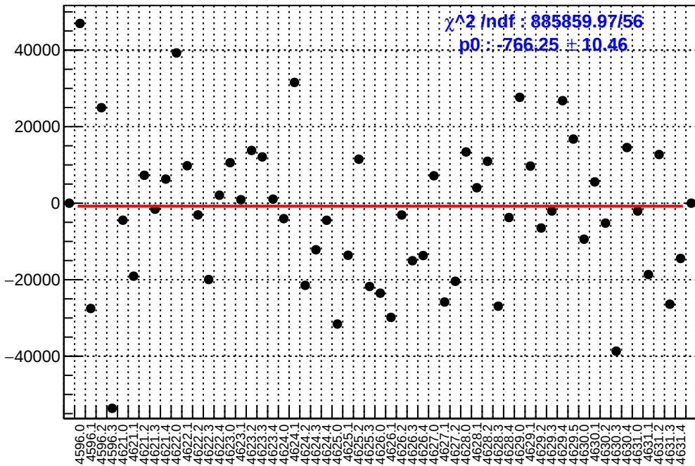
slug71: asym_at2_avg.mean/ppb-reg_asym_at2_avg.mean/ppb
