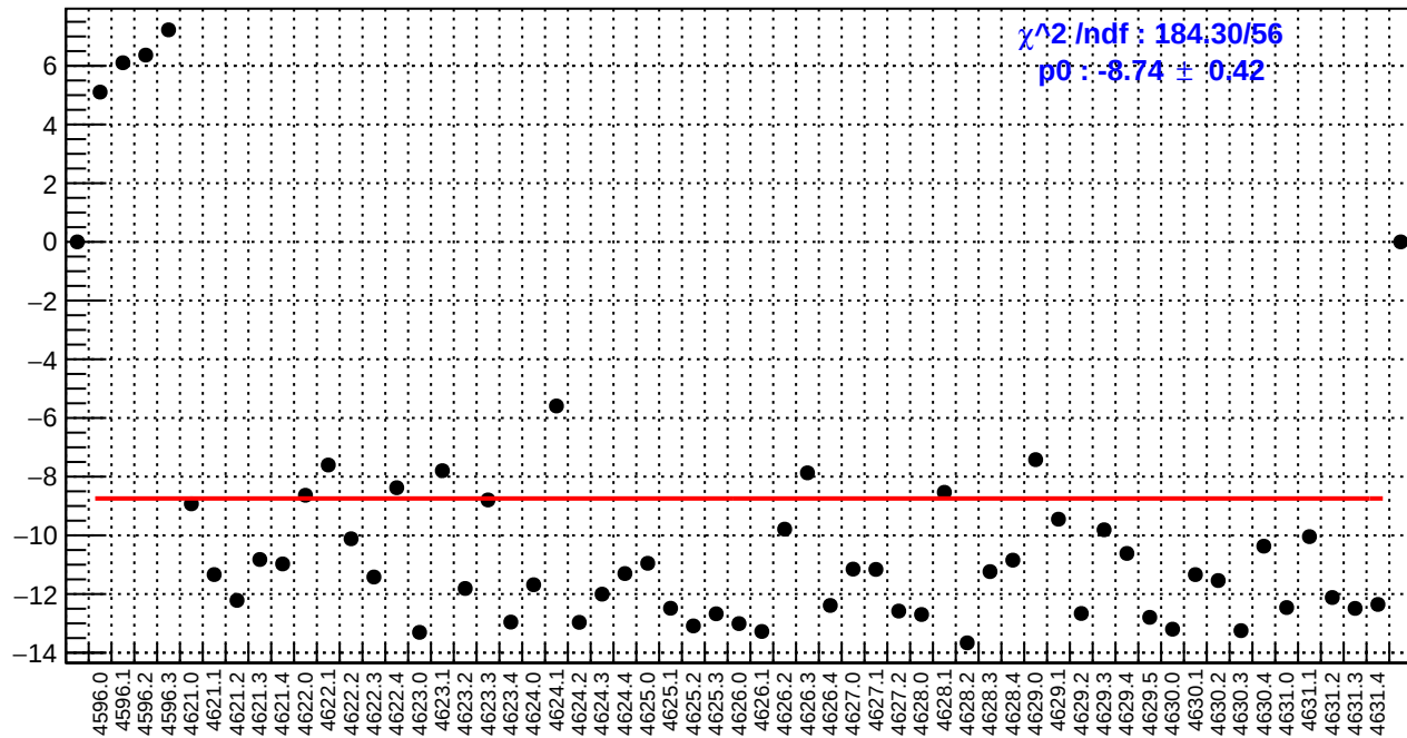
slug71: ds_avg_bpm4aY/(ppb/nm)
