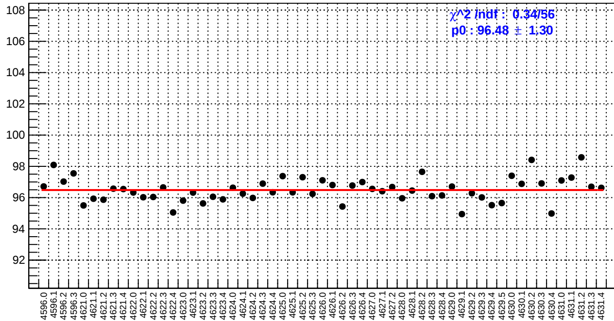
slug71: reg_asym_us_avg.rms/ppm
