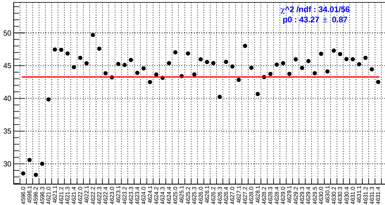
slug71: usl_bpm4aX/(ppb/nm)
