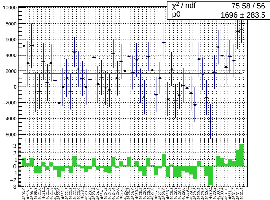
slug71: reg_asym_sam1.mean/ppb
