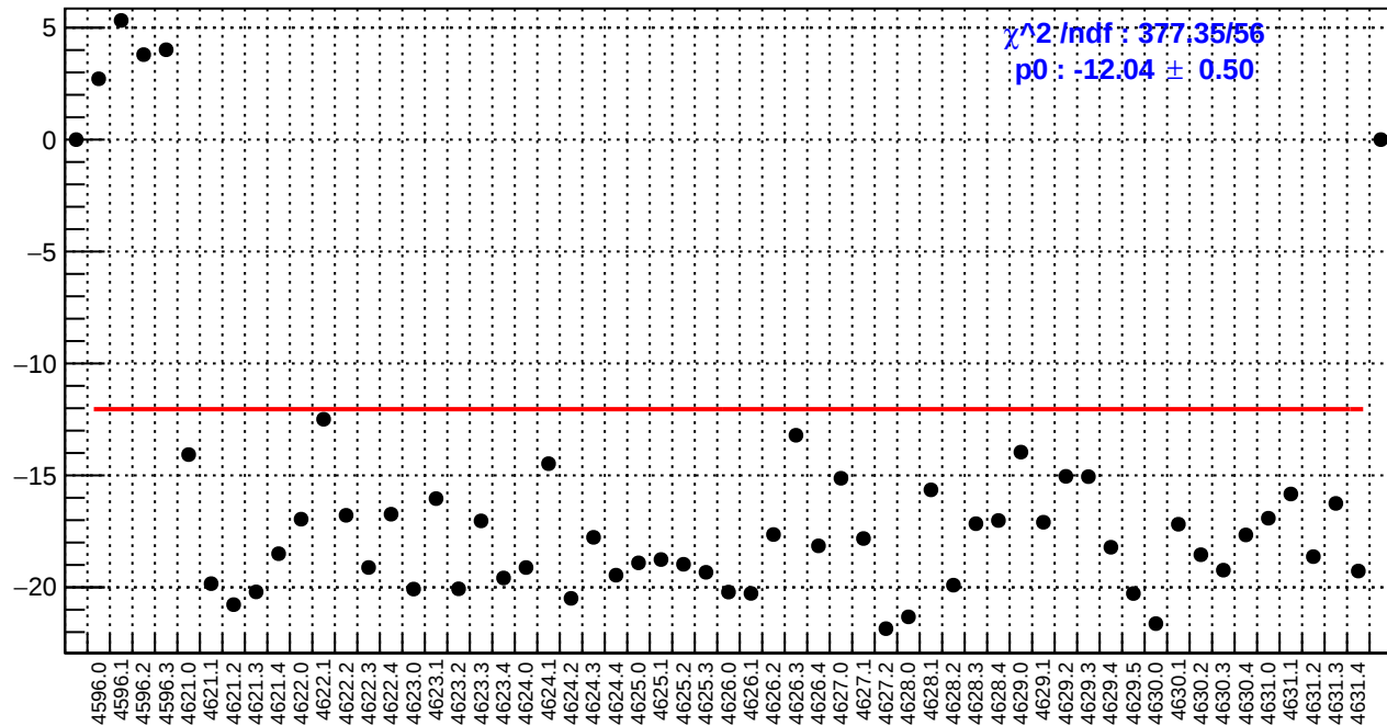
slug71: dsl_bpm4aY/(ppb/nm)
