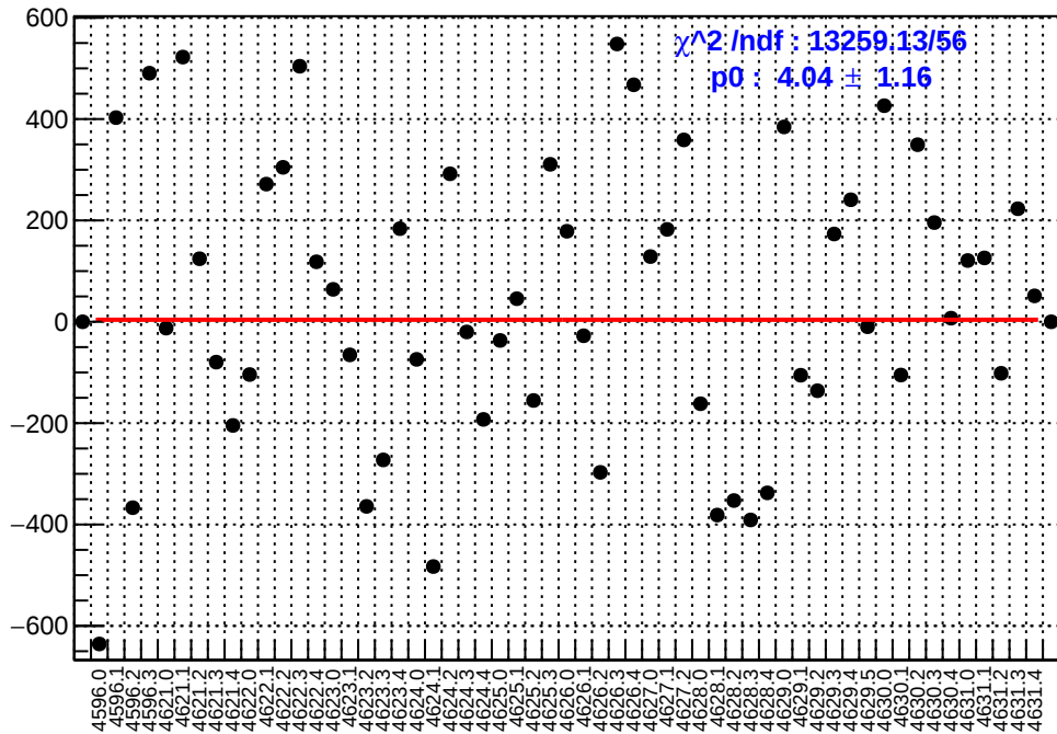
slug71: asym_right_dd.mean/ppb-reg_asym_right_dd.mean/ppb
