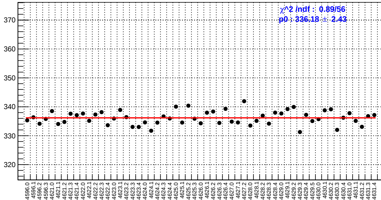
slug71: reg_asym_atr_dd.rms/ppm
