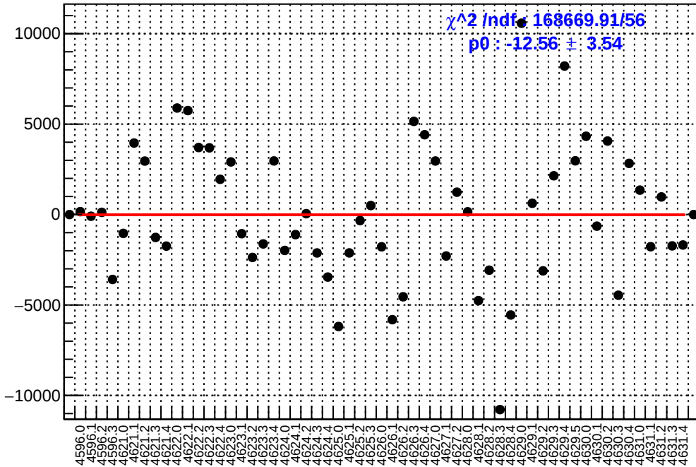
slug71: asym_right_avg.mean/ppb-reg_asym_right_avg.mean/ppb
