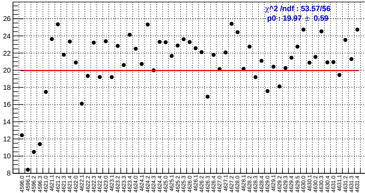
slug71: usl_bpm4eY/(ppb/nm)
