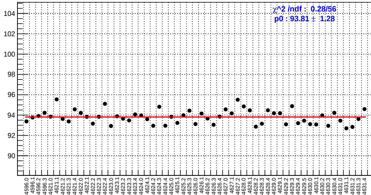
slug71: reg_asym_ds_dd.rms/ppm
