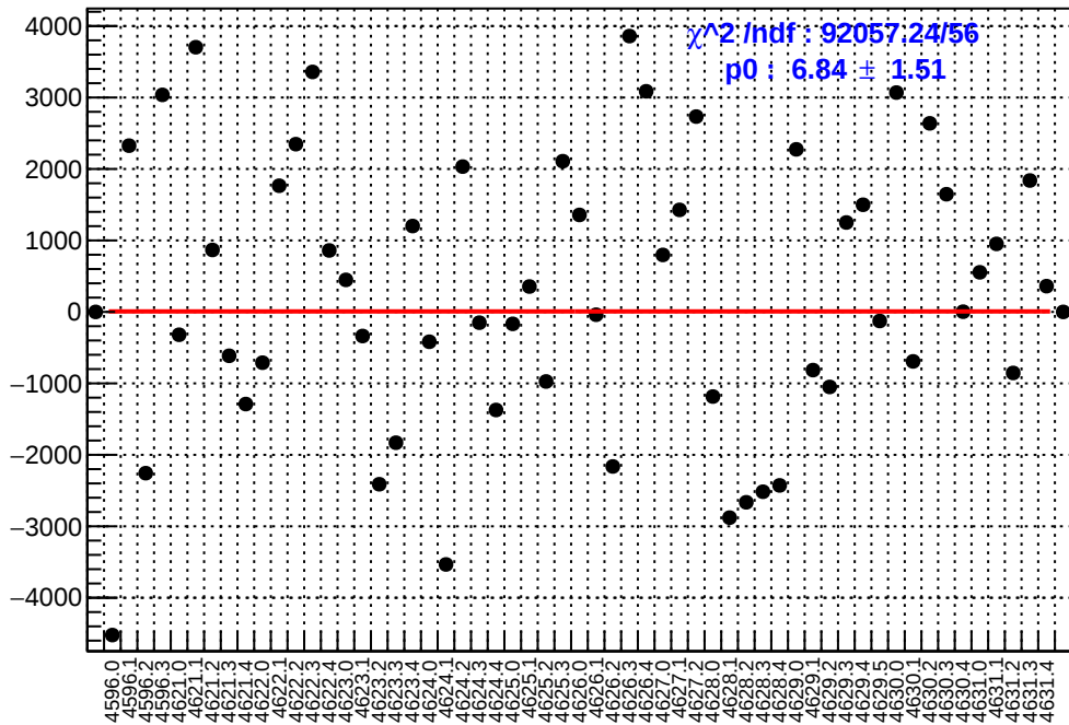
slug71: asym_at1_avg.mean/ppb-reg_asym_at1_avg.mean/ppb
