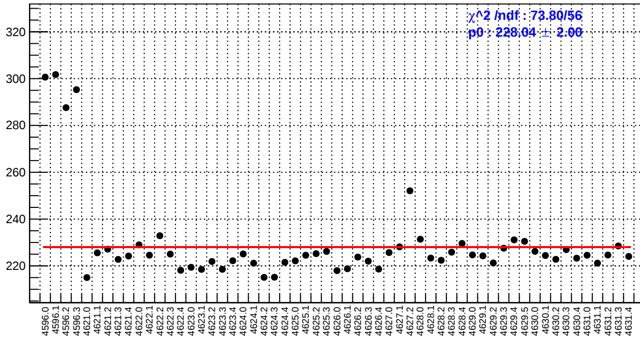
slug71: reg_asym_sam5.rms/ppm
