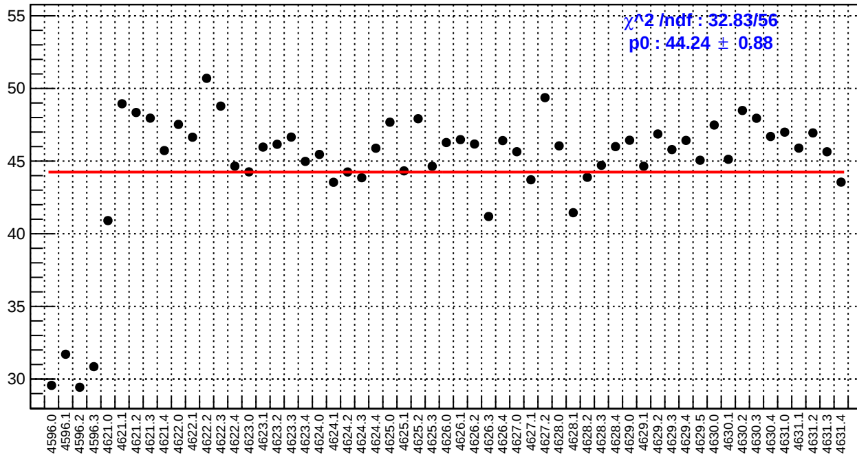
slug71: left_avg_bpm4aX/(ppb/nm)
