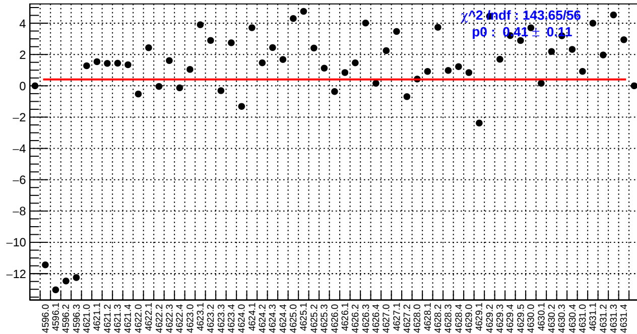
slug71: dsr_bpm4aX/(ppb/nm)
