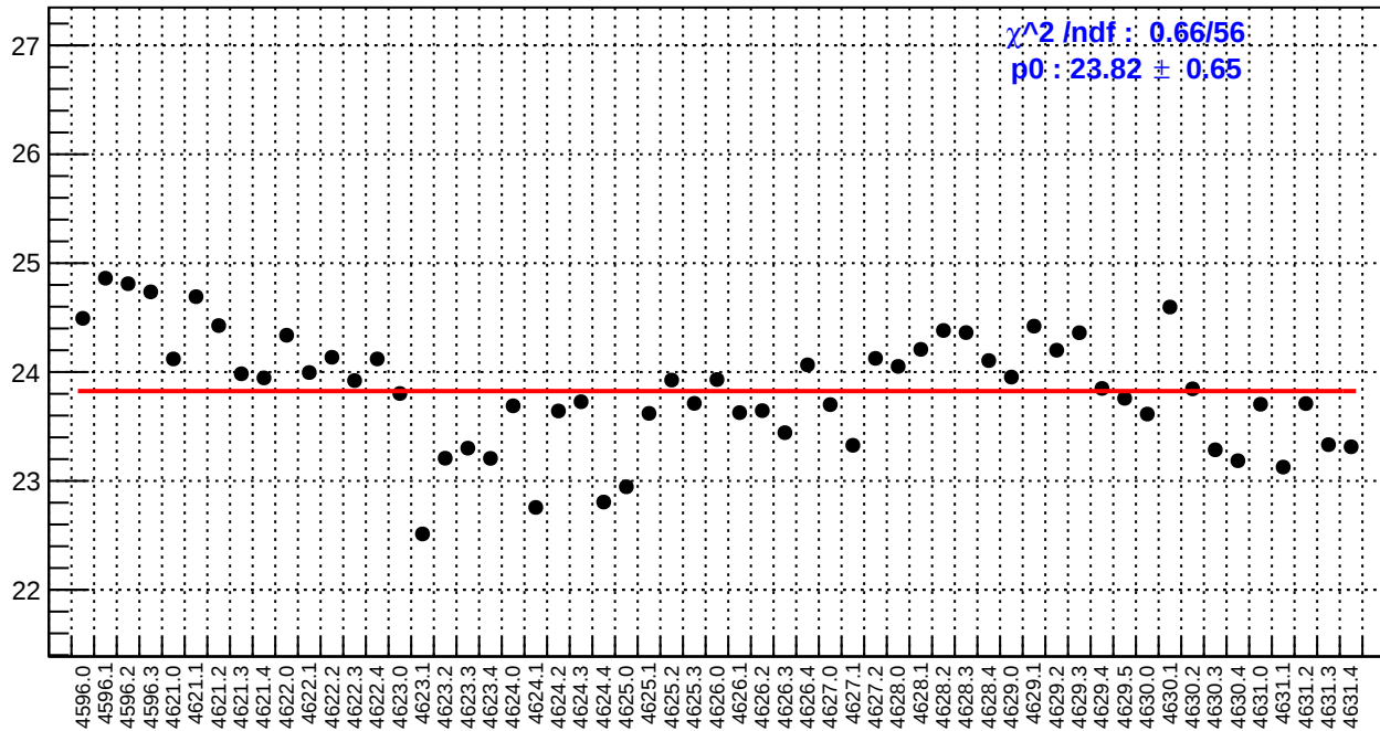
slug71: usr_bpm4eX/(ppb/nm)
