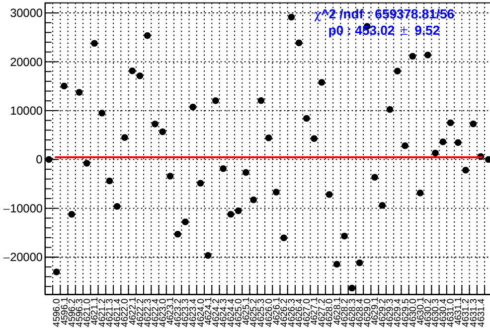
slug71: asym_sam7.mean/ppb-reg_asym_sam7.mean/ppb
