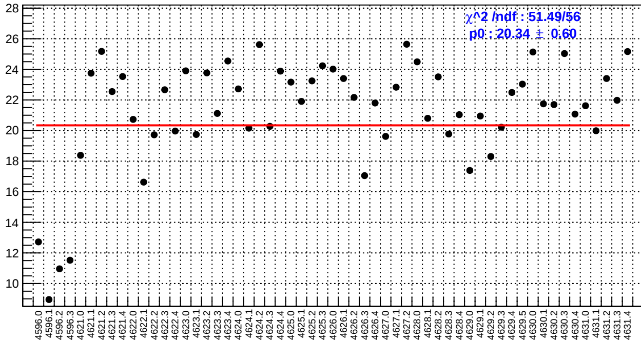
slug71: left_avg_bpm4eY/(ppb/nm)
