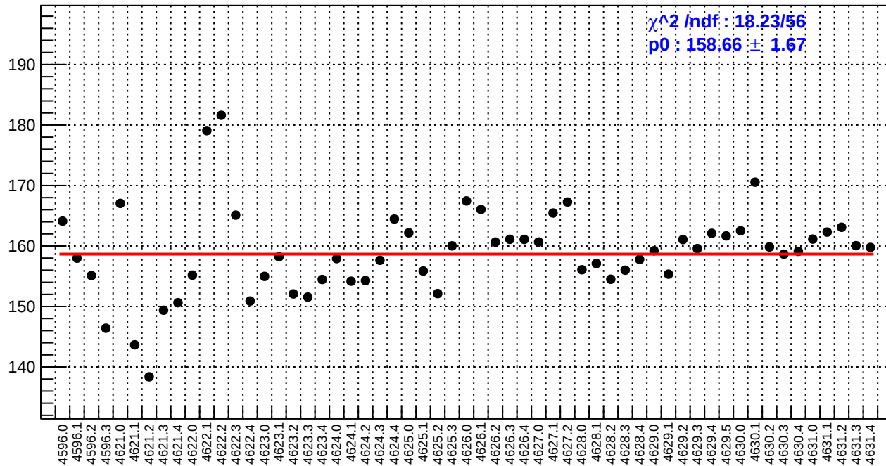
slug71: asym_bcm_an_ds3.rms/ppm
