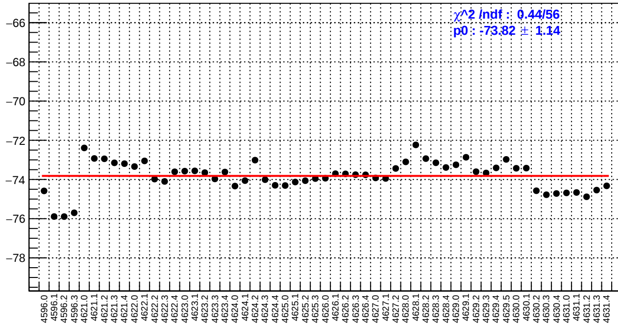
slug71: left_avg_bpm4eX/(ppb/nm)
