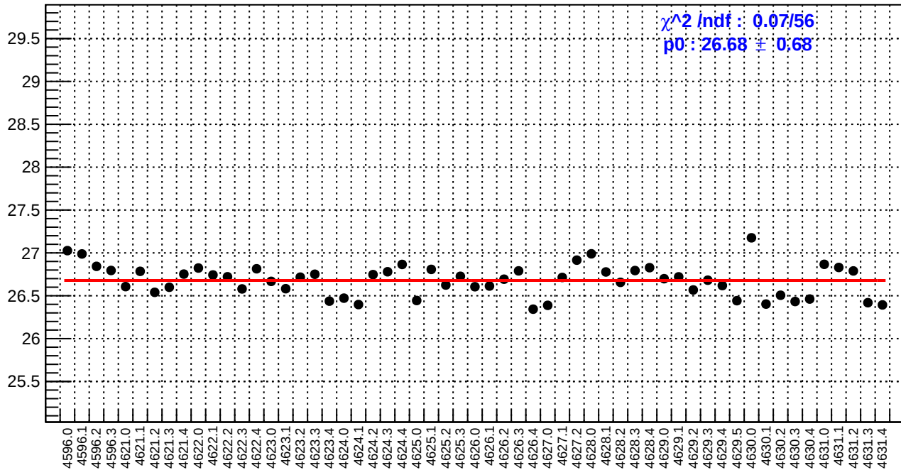
slug71: reg_asym_right_dd.rms/ppm
