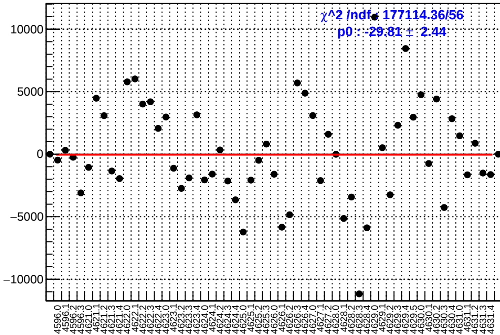
slug71: asym_usr.mean/ppb-reg_asym_usr.mean/ppb
