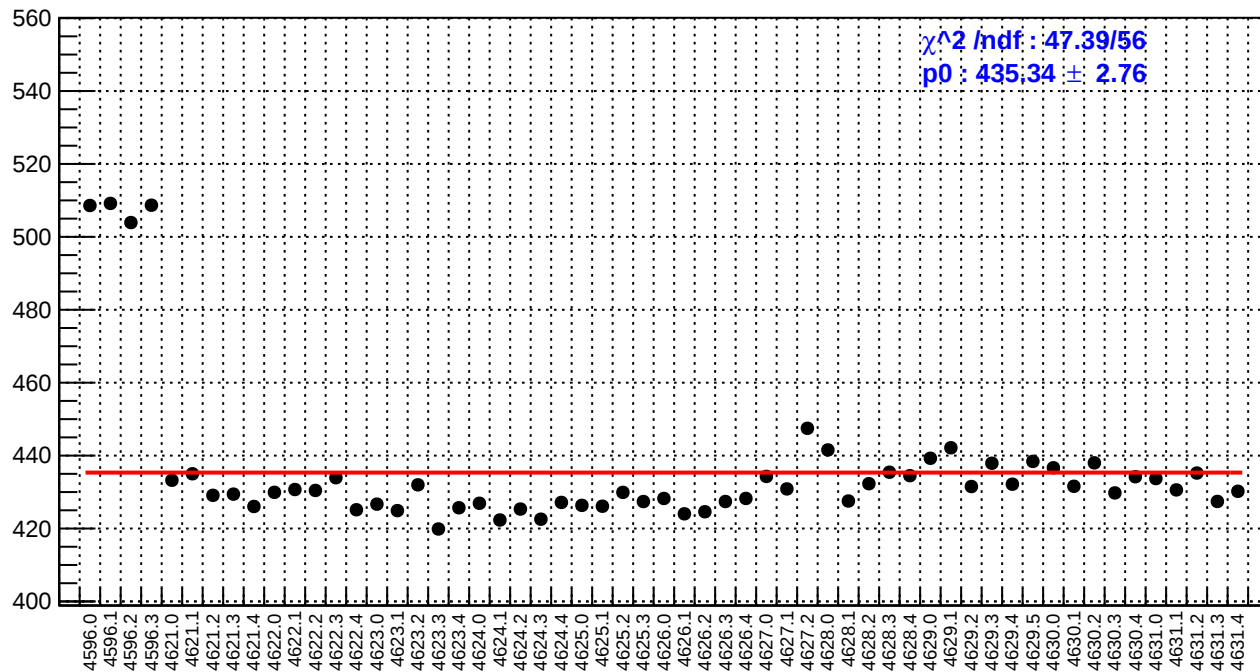
slug71: reg_asym_sam8.rms/ppm
