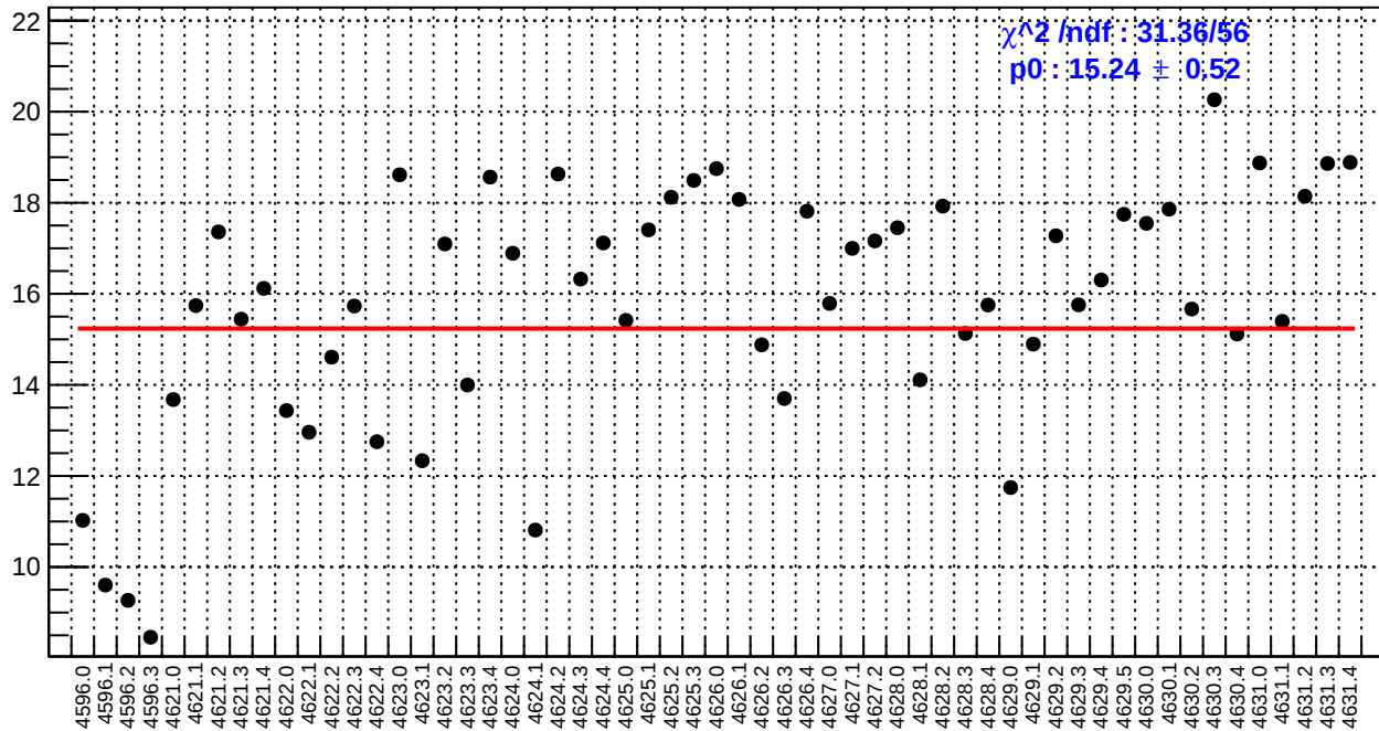
slug71: ds_avg_bpm4eY/(ppb/nm)
