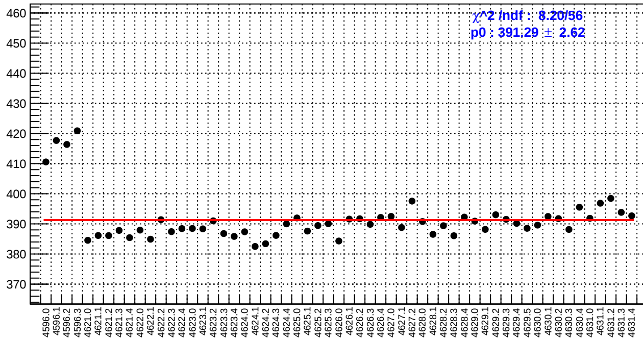
slug71: reg_asym_at2_avg.rms/ppm
