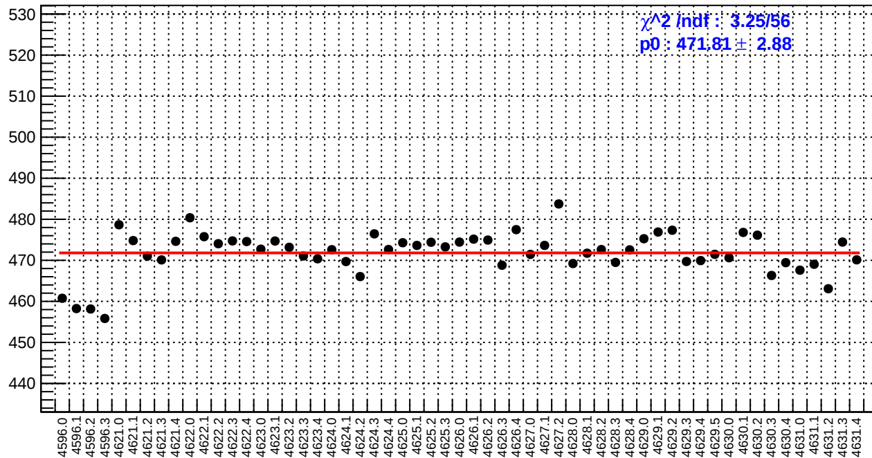
slug71: reg_asym_atr1.rms/ppm
