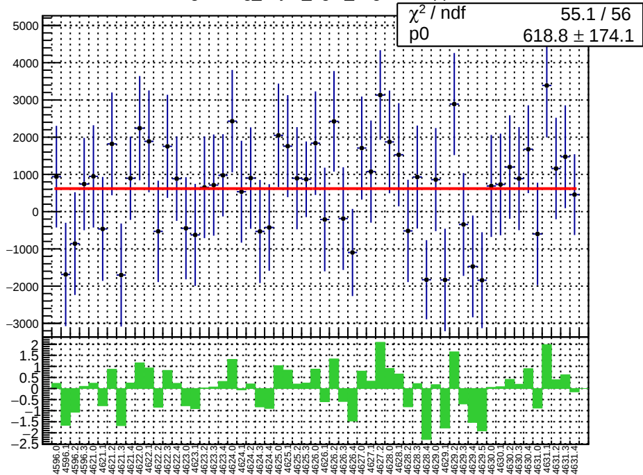
slug71: reg_asym_right_avg.mean/ppb
