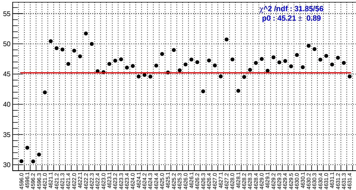
slug71: dsl_bpm4aX/(ppb/nm)
