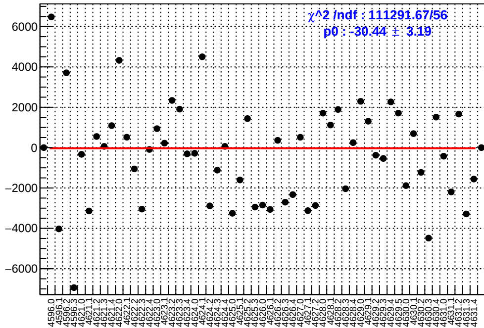
slug71: asym_ds_avg.mean/ppb-reg_asym_ds_avg.mean/ppb
