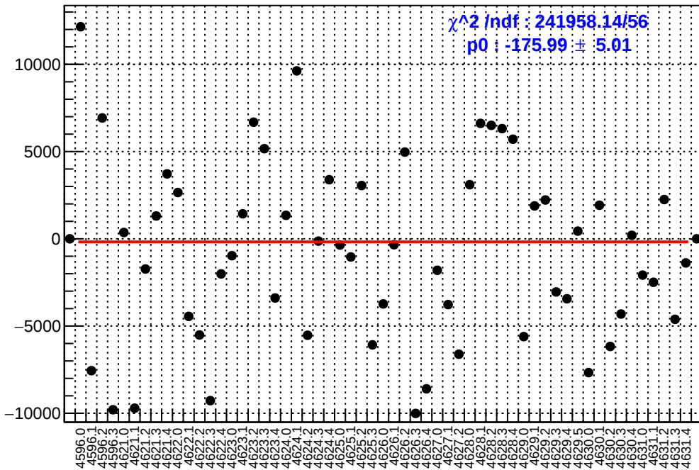
slug71: asym_dsl.mean/ppb-reg_asym_dsl.mean/ppb
