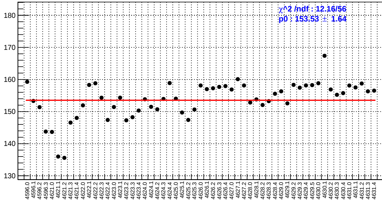
slug71: asym_bcm_an_us.rms/ppm
