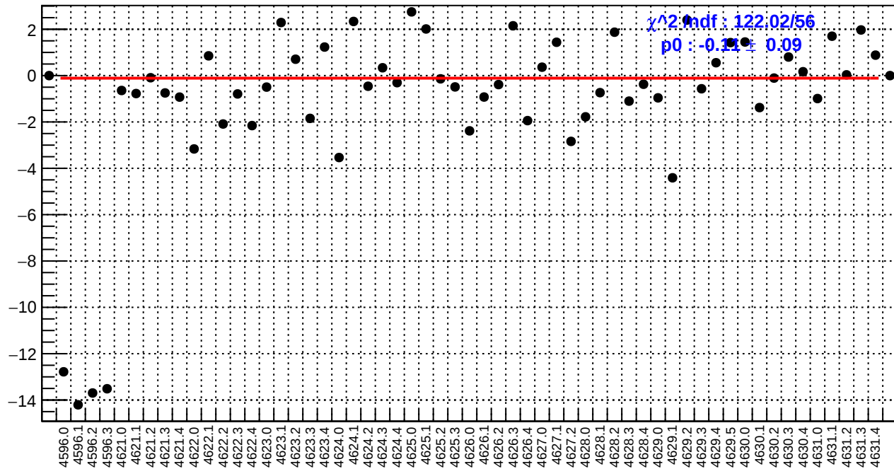
slug71: right_avg_bpm4aX/(ppb/nm)
