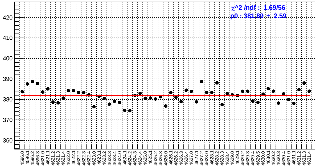
slug71: reg_asym_atr1l2_dd.rms/ppm
