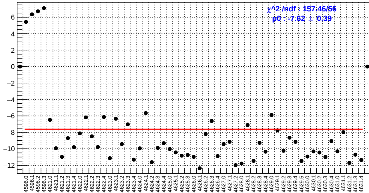
slug71: us_avg_bpm4aY/(ppb/nm)
