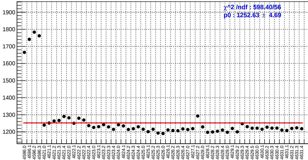
slug71: diff_bpm4aX.rms/nm
