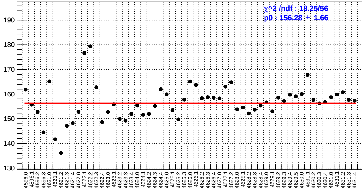
slug71: asym_bcm_an_ds.rms/ppm
