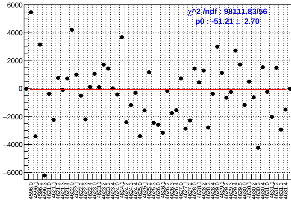
slug71: asym_us_avg.mean/ppb-reg_asym_us_avg.mean/ppb
