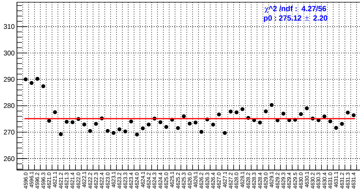
slug71: reg_asym_at2_dd.rms/ppm
