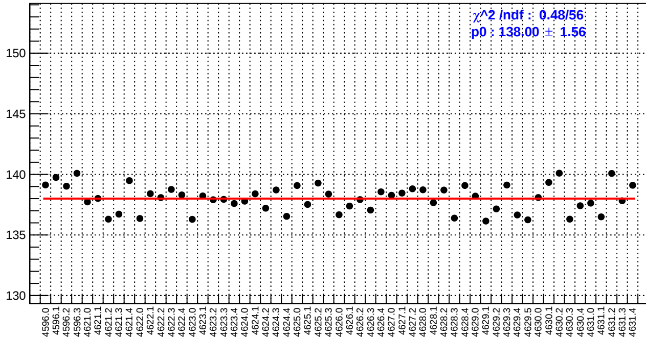
slug71: reg_asym_dsl.rms/ppm
