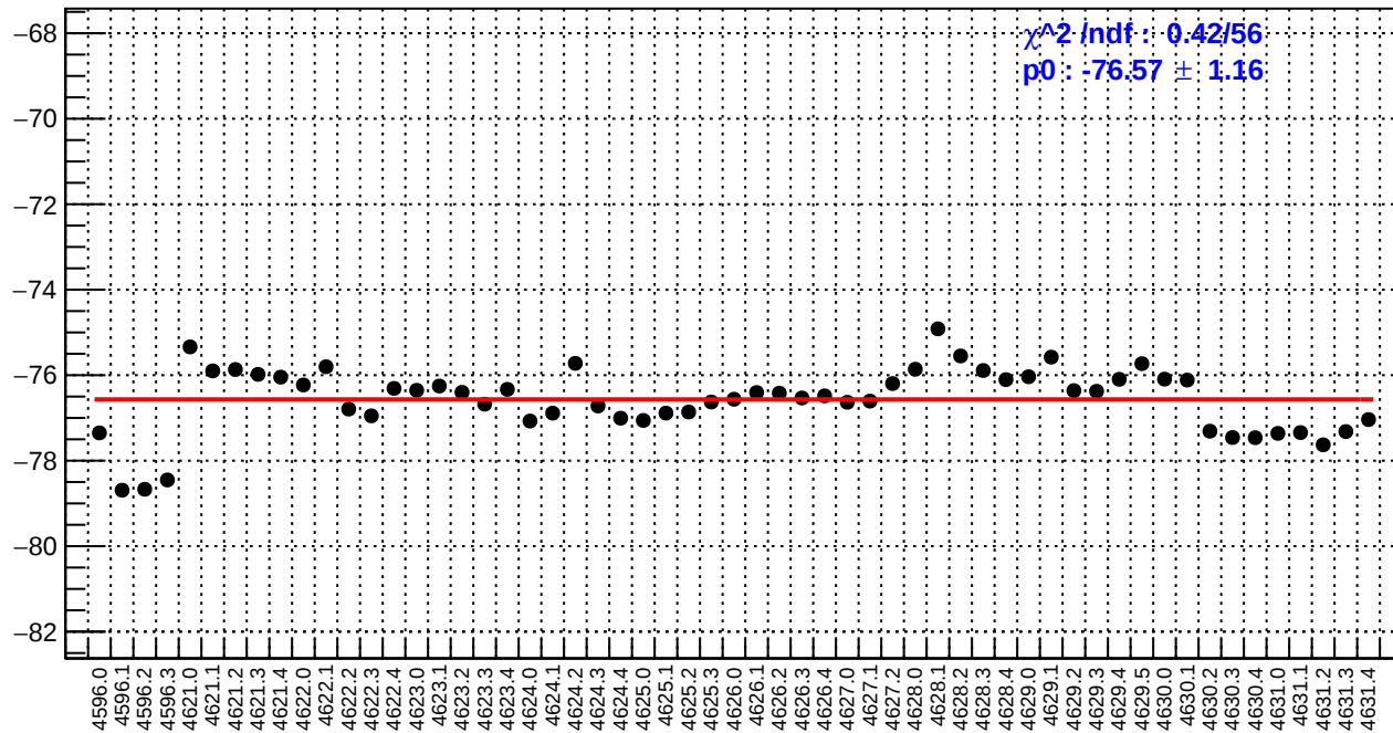
slug71: dsl_bpm4eX/(ppb/nm)
