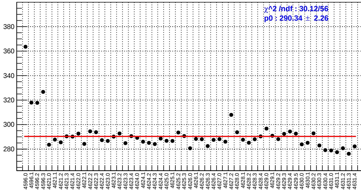
slug71: reg_asym_sam7.rms/ppm
