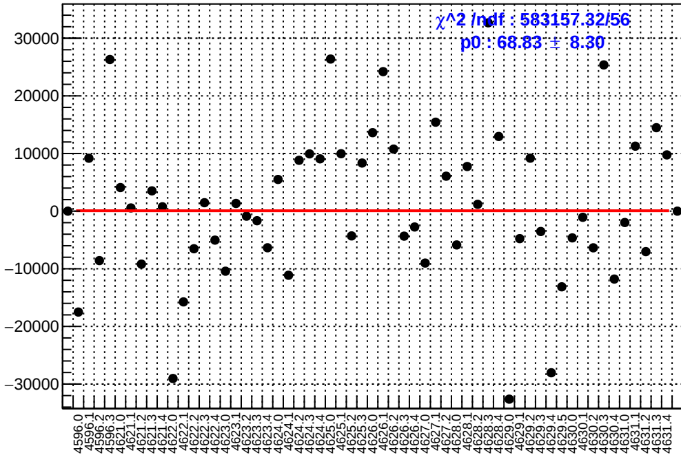
slug71: asym_atr_dd.mean/ppb-reg_asym_atr_dd.mean/ppb
