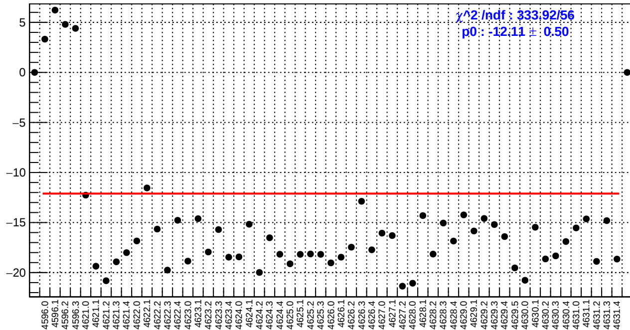
slug71: usl_bpm4aY/(ppb/nm)
