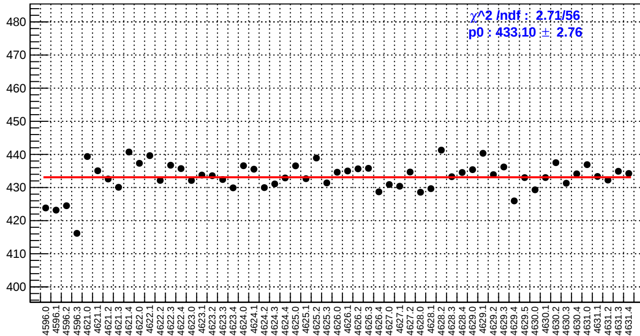
slug71: reg_asym_at1_dd.rms/ppm
