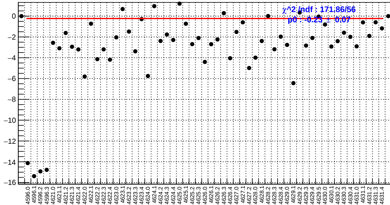
slug71: usr_bpm4aX/(ppb/nm)
