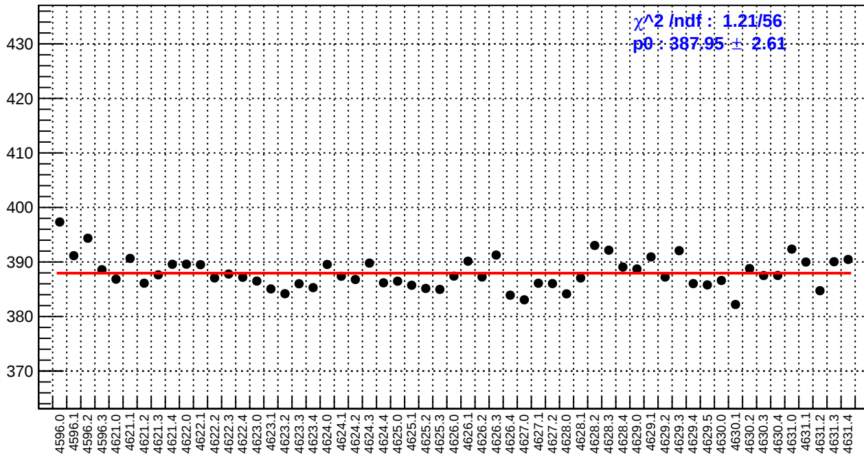
slug71: reg_asym_atl1r2_dd.rms/ppm
