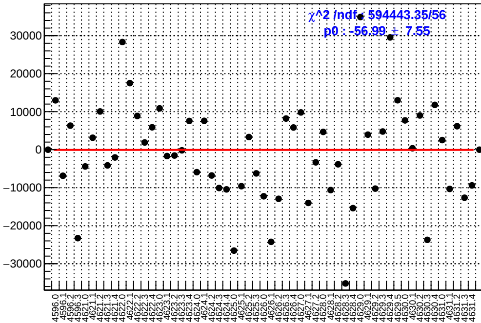
slug71: asym_atl1r2_avg.mean/ppb-reg_asym_atl1r2_avg.mean/ppb
