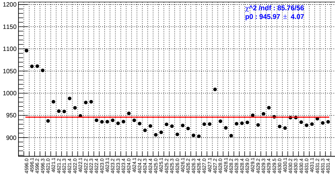
slug71: reg_asym_sam3.rms/ppm
