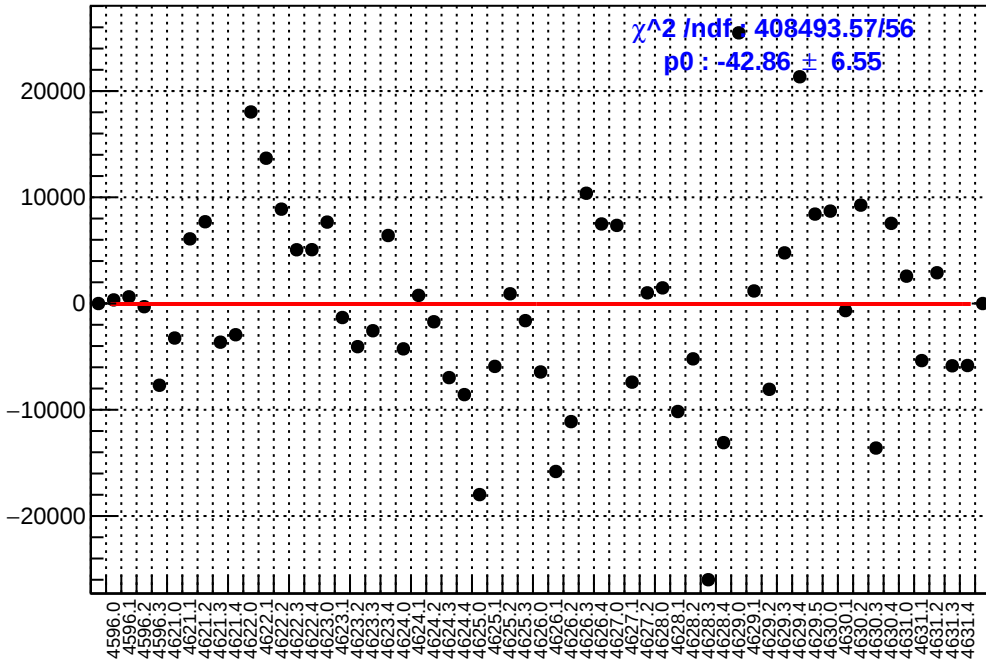
slug71: asym_at1_dd.mean/ppb-reg_asym_at1_dd.mean/ppb
