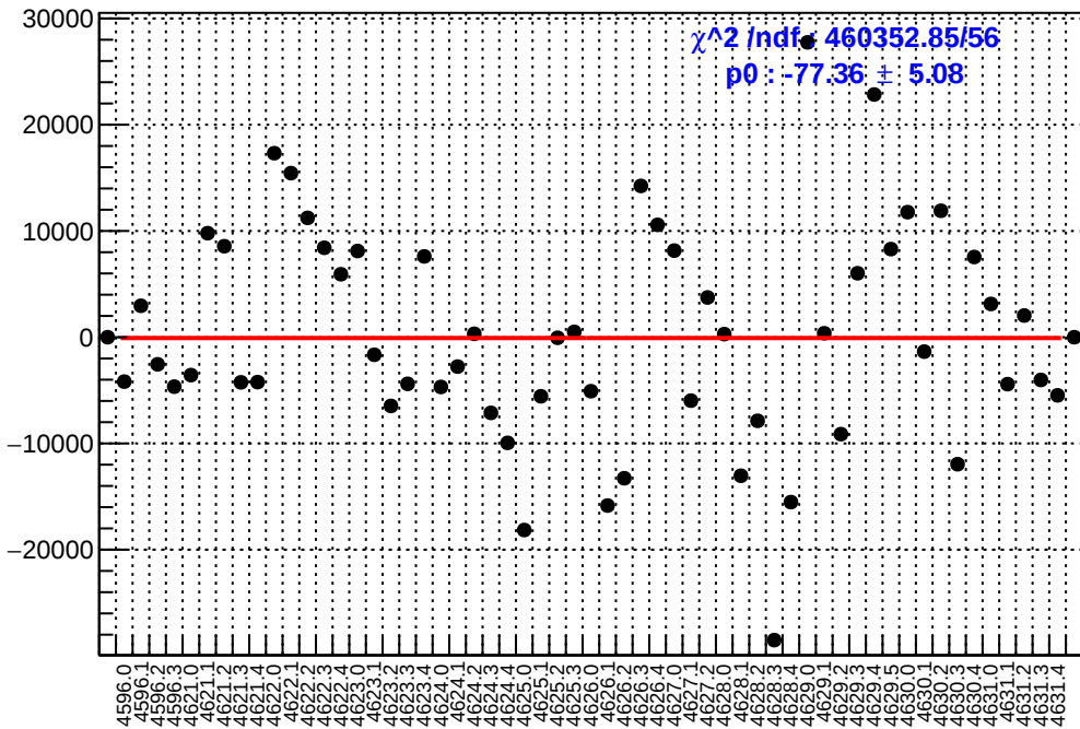
slug71: asym_atl1.mean/ppb-reg_asym_atl1.mean/ppb
