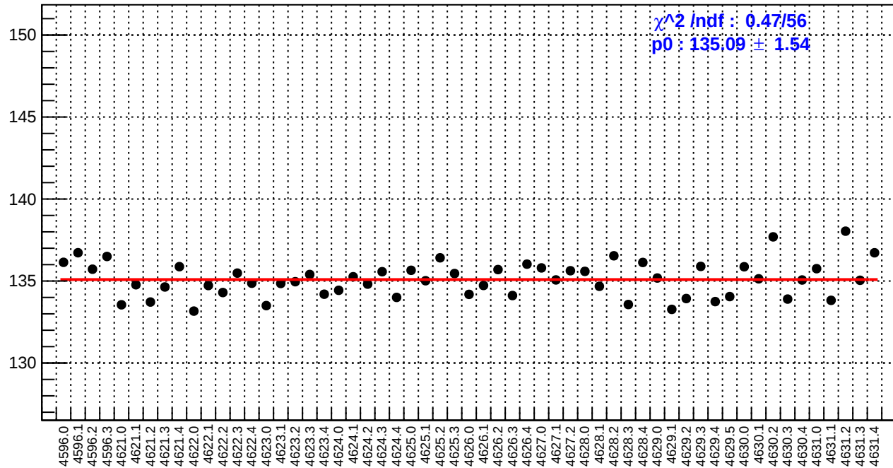
slug71: reg_asym_usl.rms/ppm
