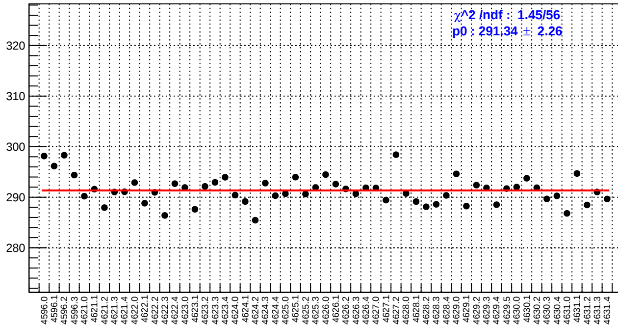
slug71: reg_asym_atr_avg.rms/ppm
