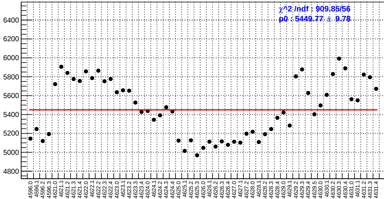
slug71: diff_bpm11X.rms/nm
