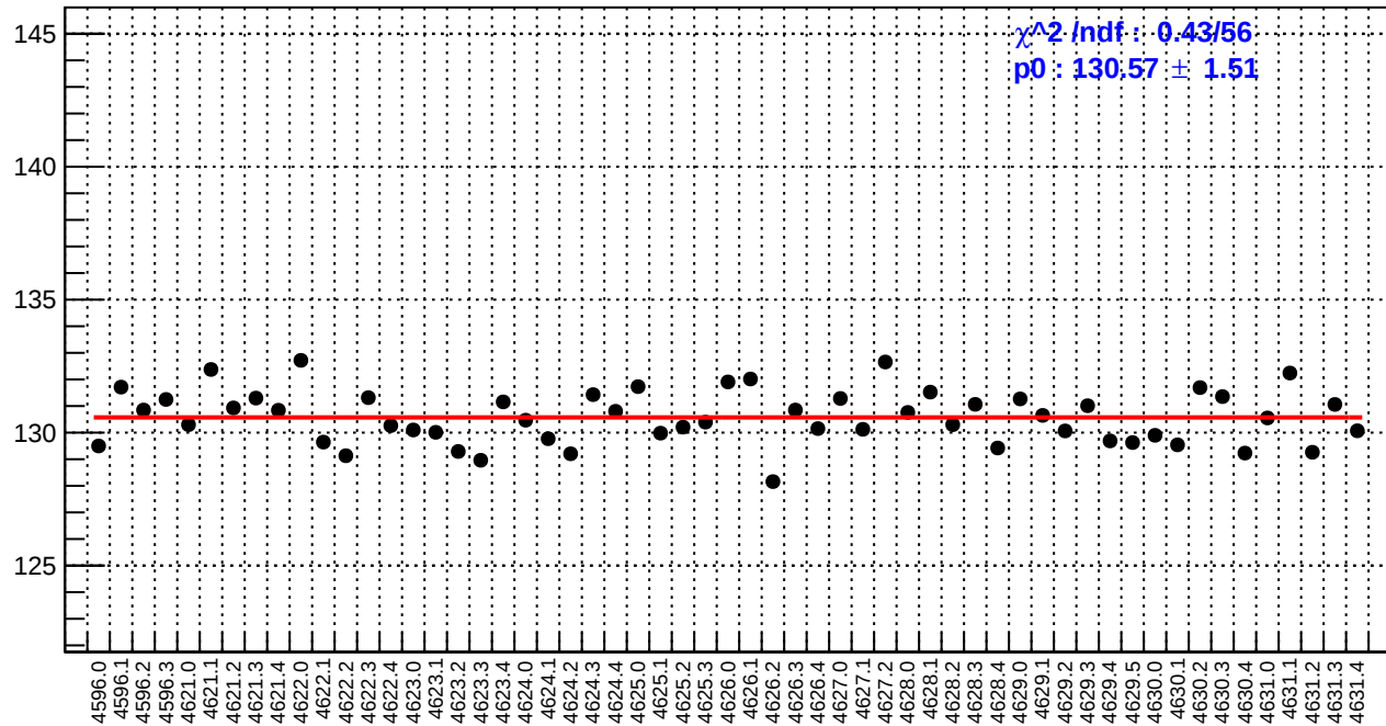
slug71: reg_asym_right_avg.rms/ppm
