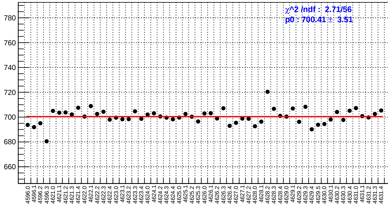
slug71: reg_asym_atl1.rms/ppm
