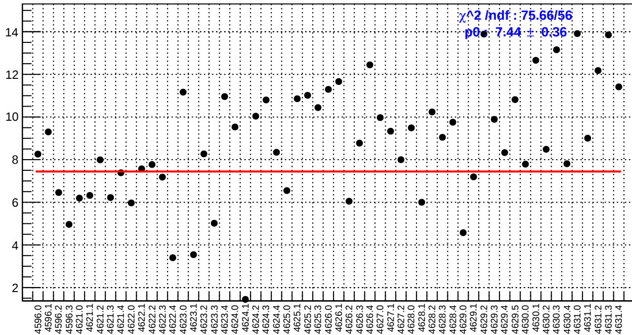
slug71: right_avg_bpm4eY/(ppb/nm)
