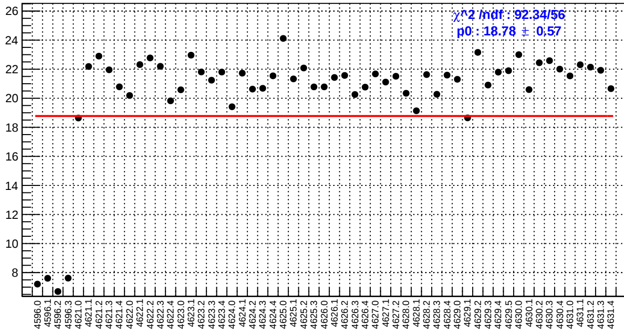
slug71: us_avg_bpm4aX/(ppb/nm)
