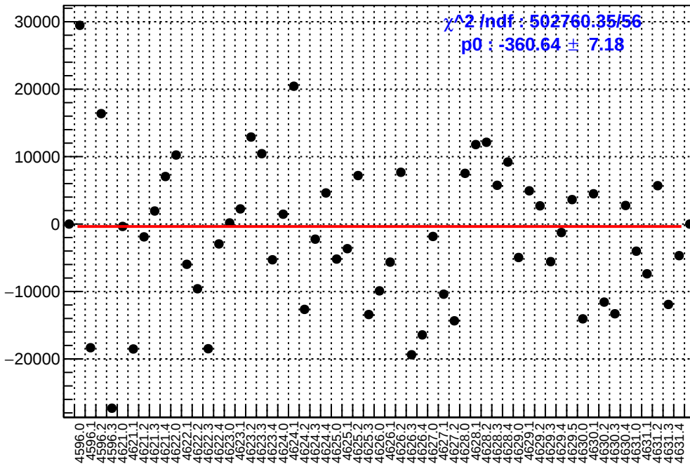
slug71: asym_atr1l2_avg.mean/ppb-reg_asym_atr1l2_avg.mean/ppb
