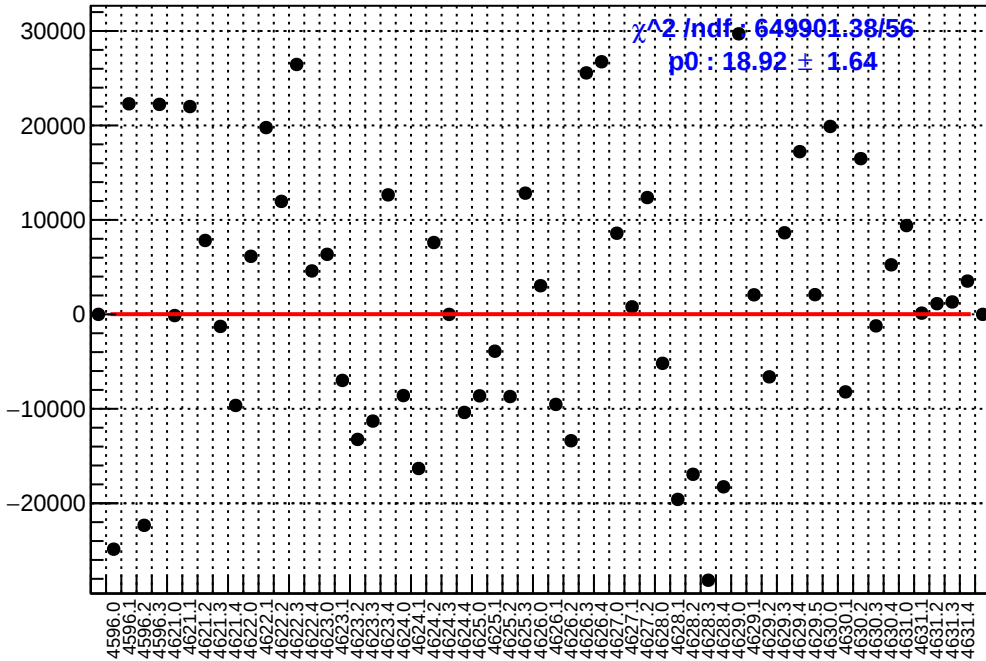
slug71: asym_sam8.mean/ppb-reg_asym_sam8.mean/ppb
