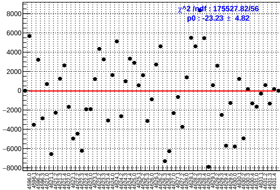
slug71: asym_ds_dd.mean/ppb-reg_asym_ds_dd.mean/ppb
