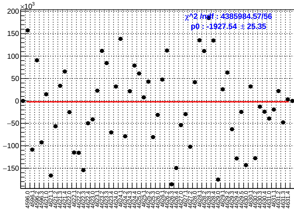
slug71: asym_sam3.mean/ppb-reg_asym_sam3.mean/ppb
