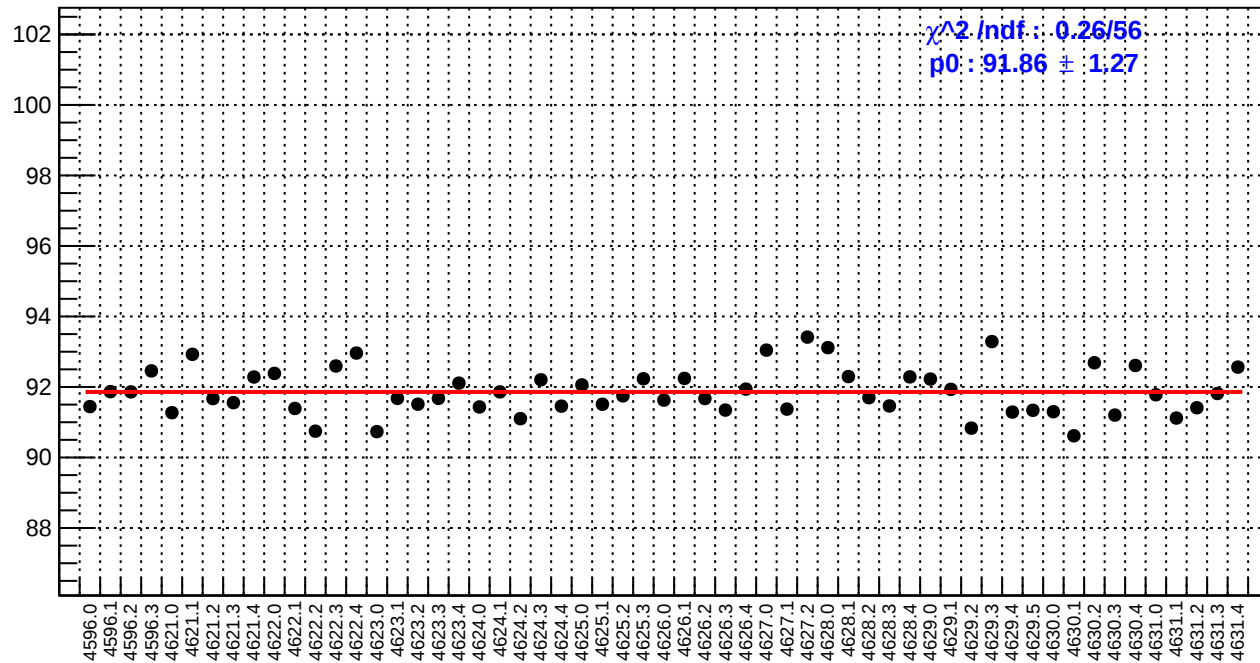
slug71: reg_asym_us_dd.rms/ppm
