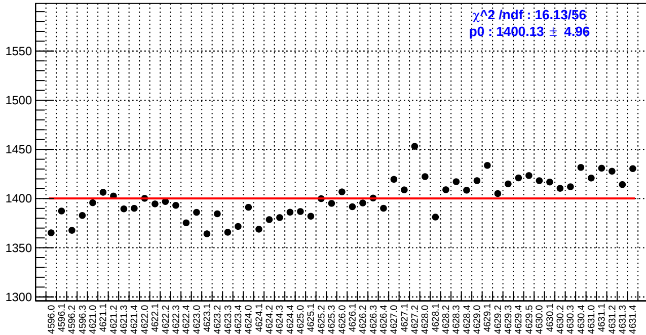
slug71: reg_asym_sam4.rms/ppm
