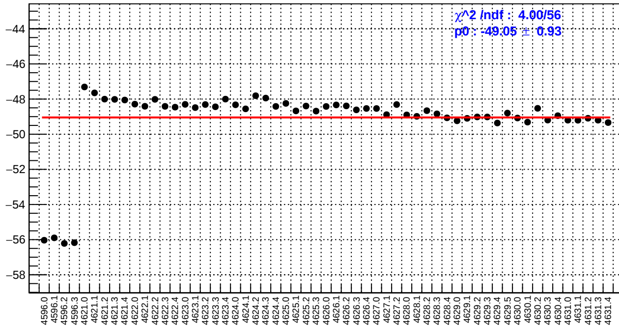
slug71: us_avg_bpm12X/(ppb/nm)
