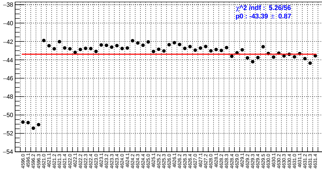
slug71: dsl_bpm12X/(ppb/nm)
