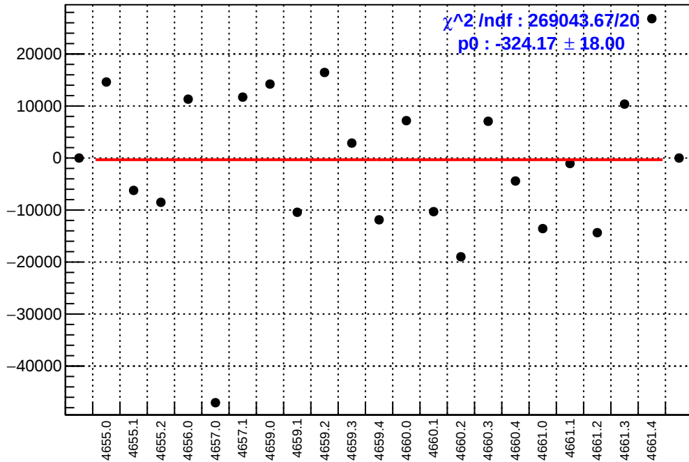
slug72B: asym_atr1.mean/ppb-reg_asym_atr1.mean/ppb
