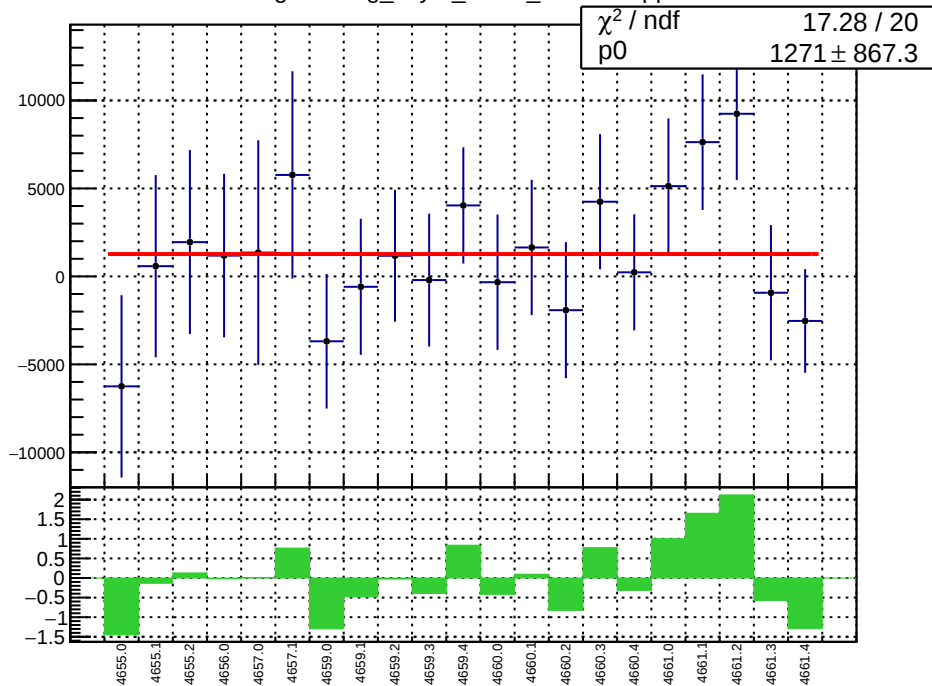
slug72B: reg_asym_atr1l2_dd.mean/ppb
