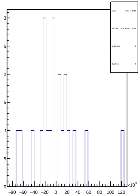
slug72B: 1D Corr asym_sam6.mean/ppb-reg_asym_sam6.mean/ppb
