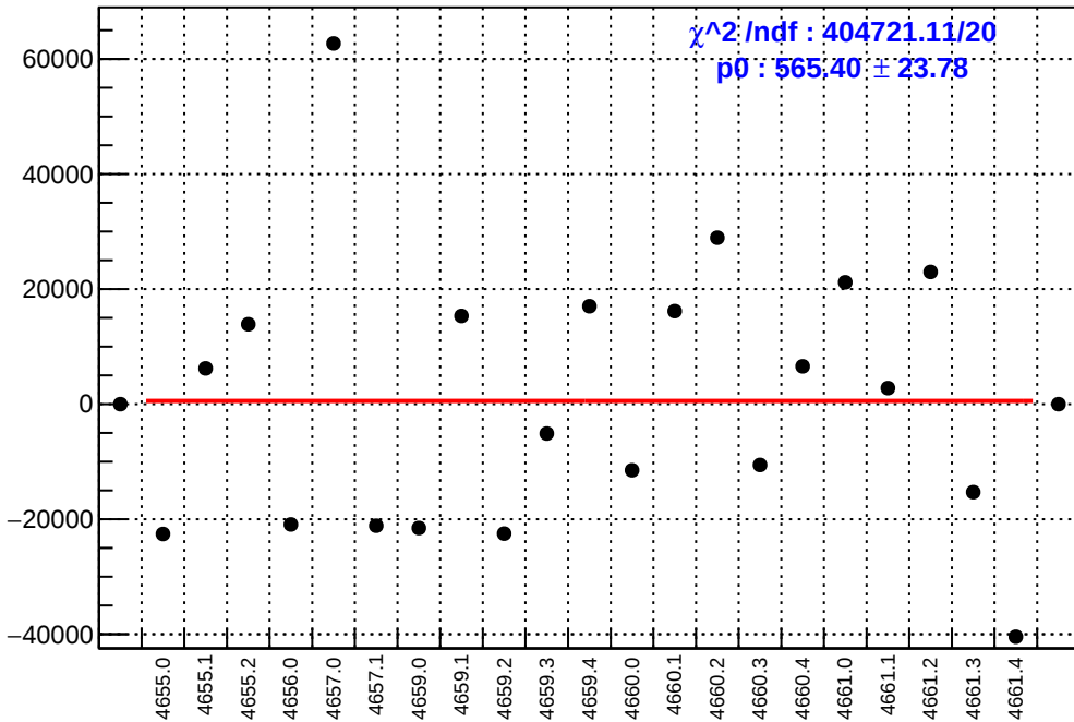
slug72B: asym_atl1r2_avg.mean/ppb-reg_asym_atl1r2_avg.mean/ppb
