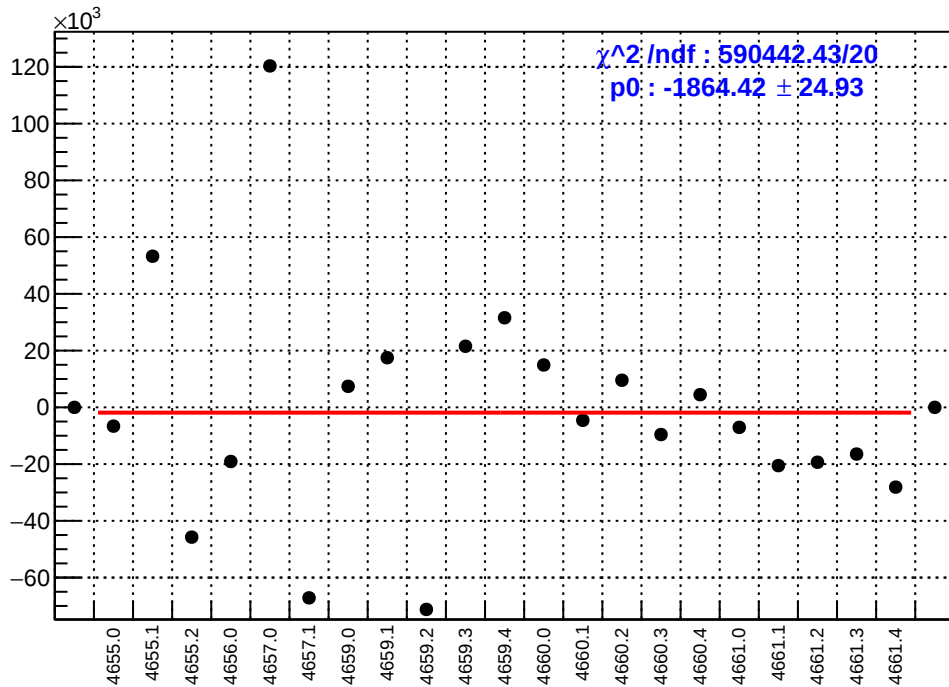
slug72B: asym_sam6.mean/ppb-reg_asym_sam6.mean/ppb
