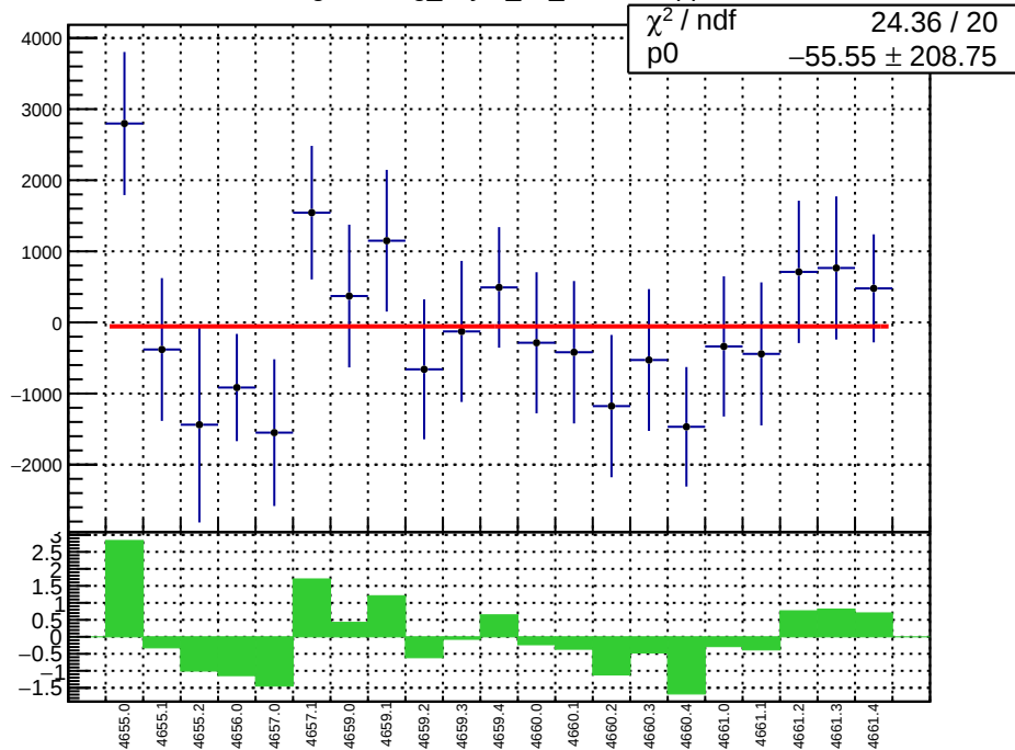
slug72B: reg_asym_ds_dd.mean/ppb
