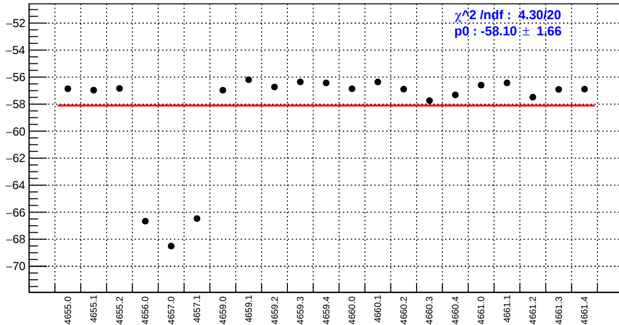
slug72B: right_avg_bpm12X/(ppb/nm)
