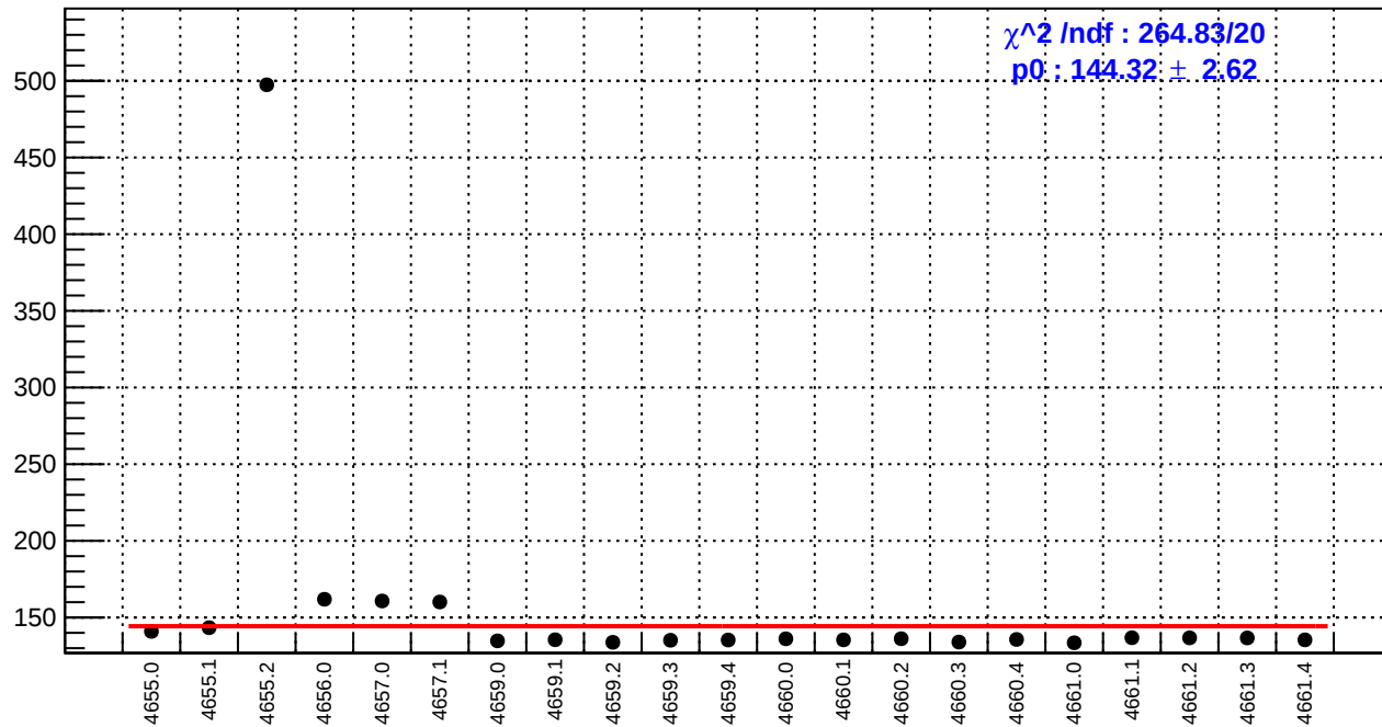
slug72B: reg_asym_usl.rms/ppm
