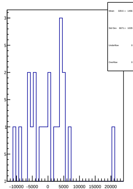
slug72B: 1D Corr asym_dsr.mean/ppb-reg_asym_dsr.mean/ppb
