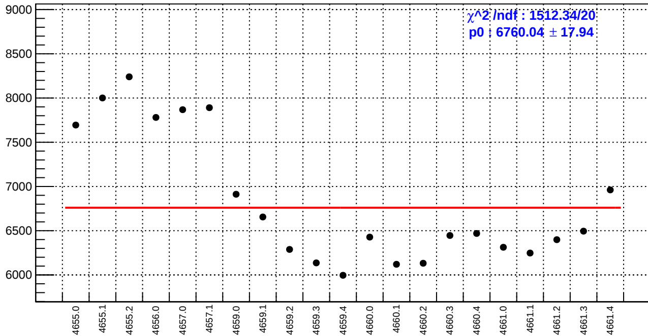
slug72B: diff_bpm11X.rms/nm
