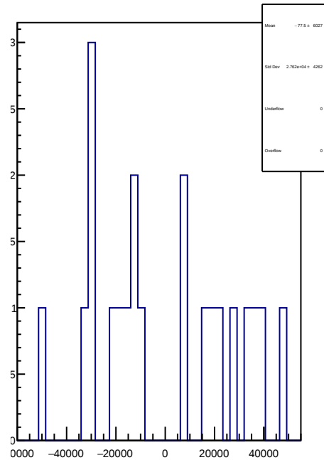
slug72B: 1D Corr asym_atr2.mean/ppb-reg_asym_atr2.mean/ppb
