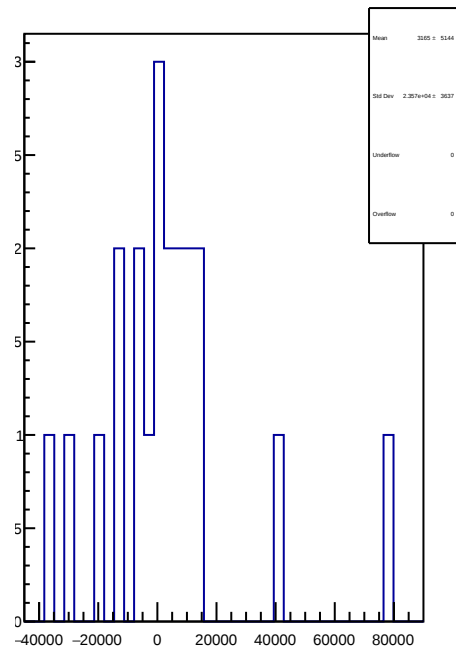
slug72B: 1D Corr asym_atl_dd.mean/ppb-reg_asym_atl_dd.mean/ppb
