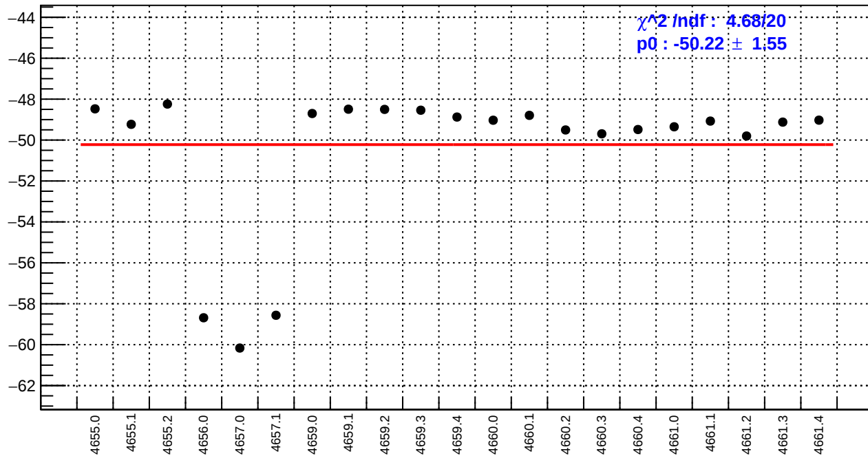
slug72B: us_avg_bpm12X/(ppb/nm)
