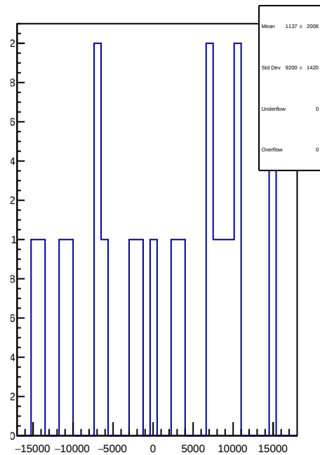
slug72B: 1D Corr asym_atl1r2_dd.mean/ppb-reg_asym_atl1r2_dd.mean/ppb
