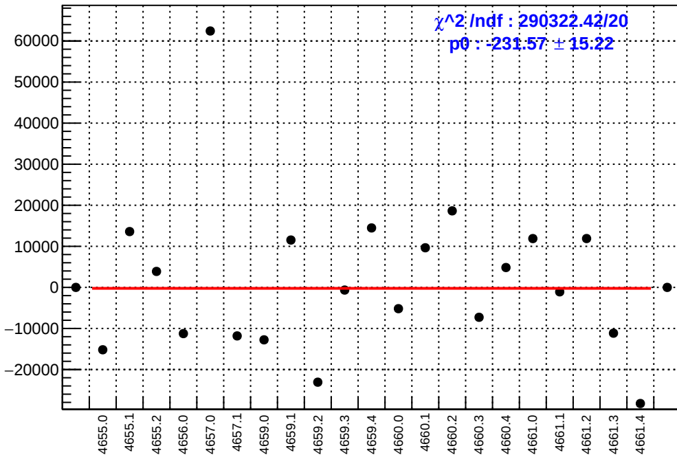
slug72B: asym_at1_dd.mean/ppb-reg_asym_at1_dd.mean/ppb
