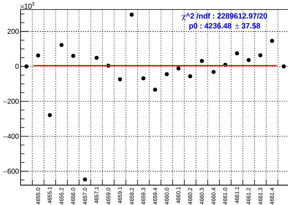
slug72B: asym_sam3.mean/ppb-reg_asym_sam3.mean/ppb
