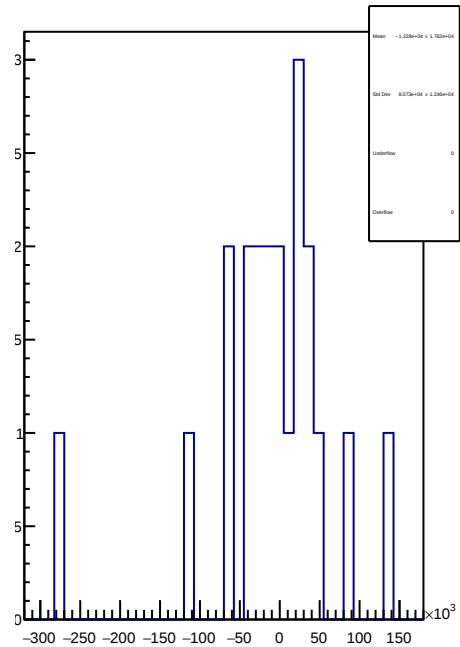
slug72B: 1D Corr asym_sam4.mean/ppb-reg_asym_sam4.mean/ppb
