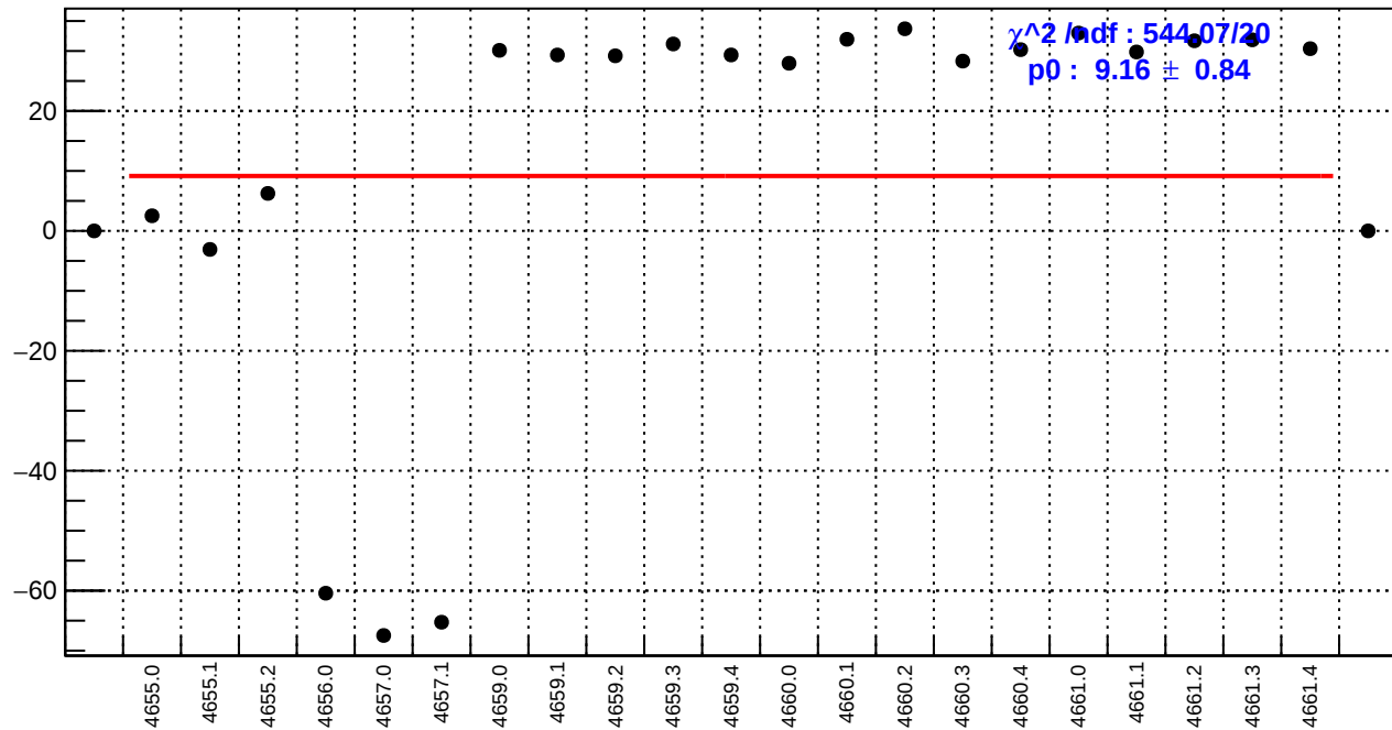
slug72B: left_avg_bpm4aX/(ppb/nm)
