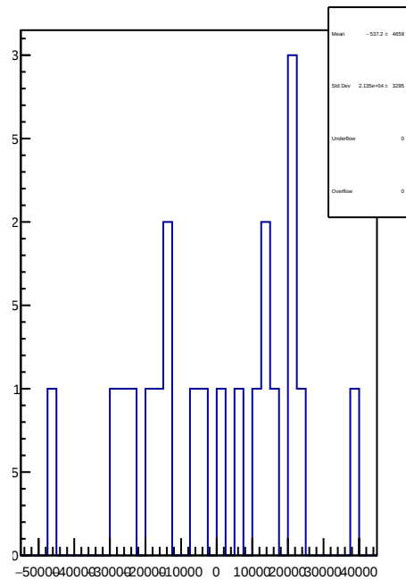
slug72B: 1D Corr asym_atr_dd.mean/ppb-reg_asym_atr_dd.mean/ppb
