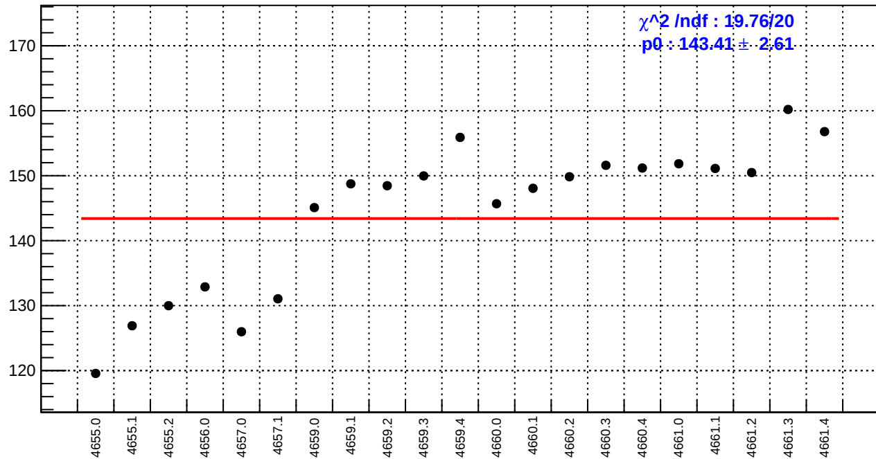
slug72B: asym_bcm_an_us.rms/ppm
