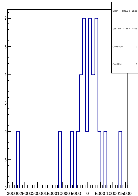
slug72B: 1D Corr asym_us_dd.mean/ppb-reg_asym_us_dd.mean/ppb
