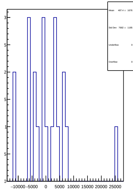
slug72B: 1D Corr asym_usr.mean/ppb-reg_asym_usr.mean/ppb
