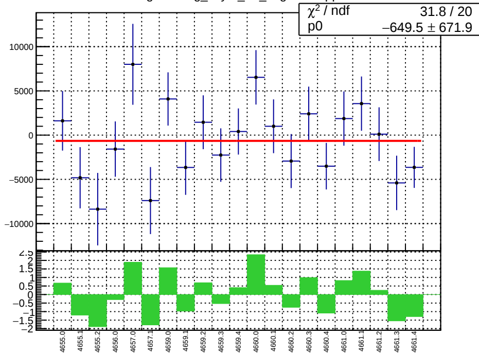
slug72B: reg_asym_atr_avg.mean/ppb
