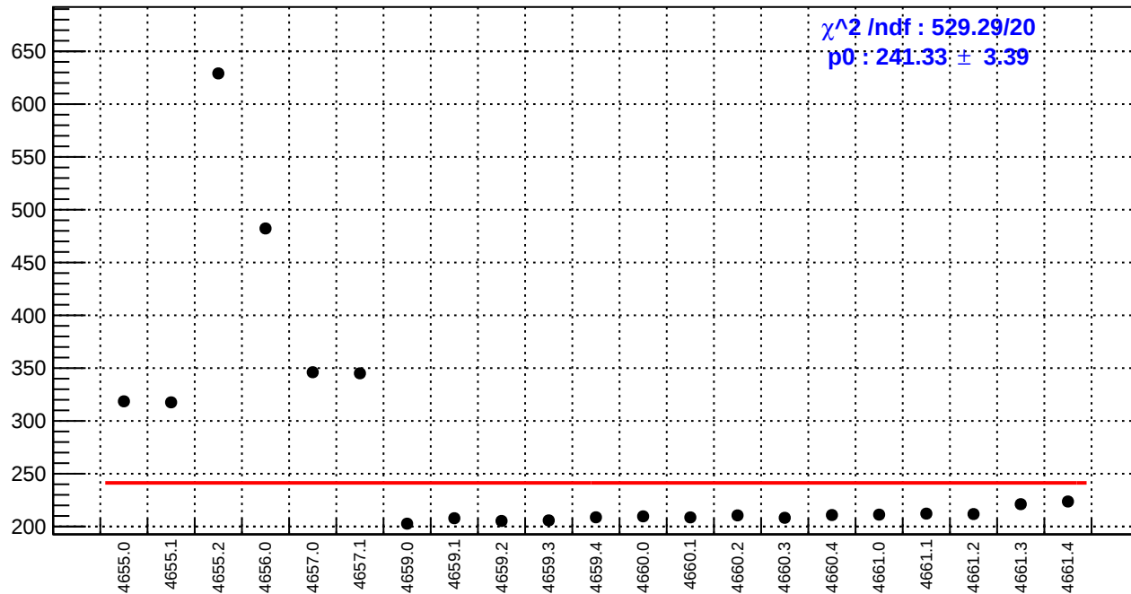
slug72B: reg_asym_sam5.rms/ppm
