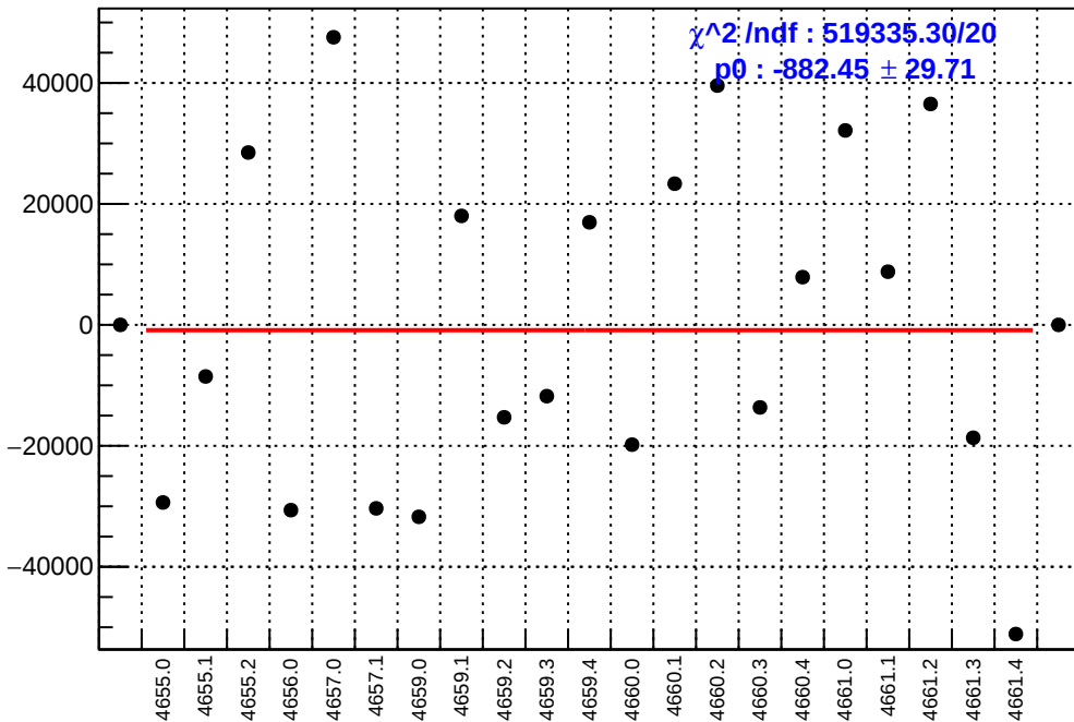
slug72B: asym_atr2.mean/ppb-reg_asym_atr2.mean/ppb
