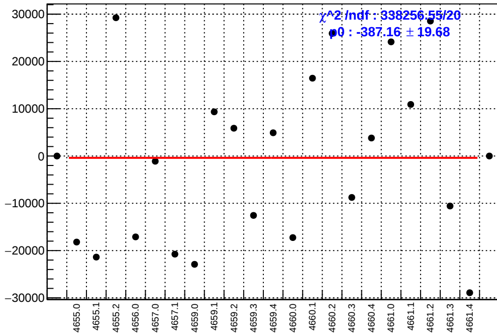
slug72B: asym_atl_avg.mean/ppb-reg_asym_atl_avg.mean/ppb
