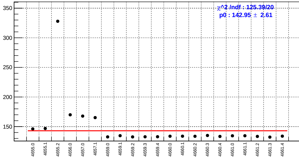
slug72B: reg_asym_dsr.rms/ppm
