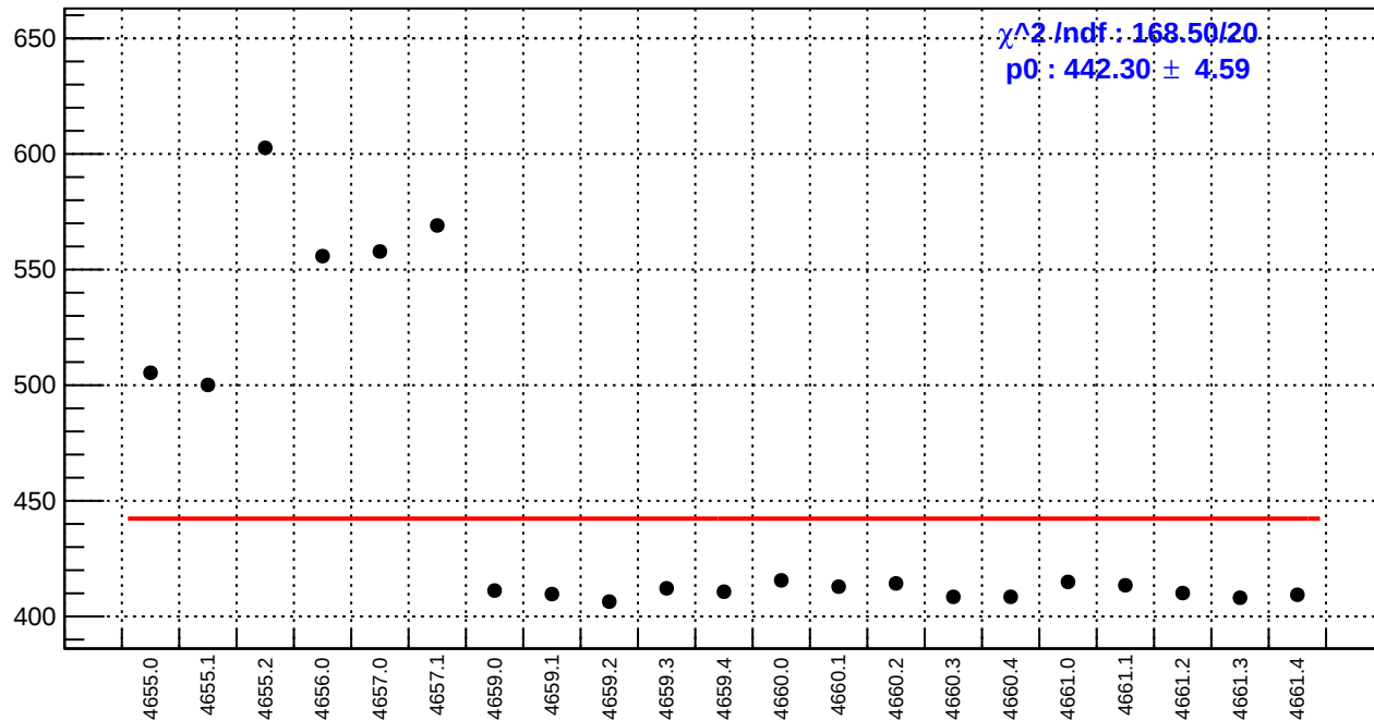
slug72B: reg_asym_atl1r2_avg.rms/ppm
