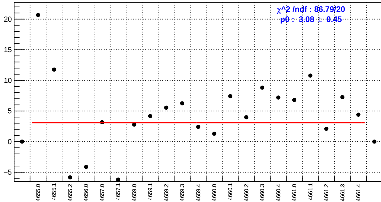
slug72B: dsl_bpm4eY/(ppb/nm)
