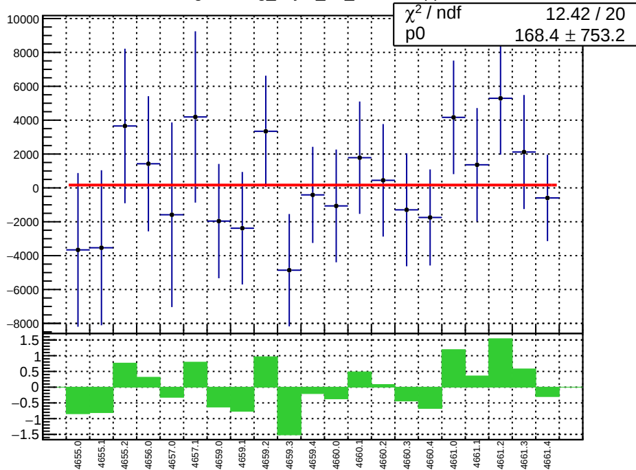
slug72B: reg_asym_atr_dd.mean/ppb
