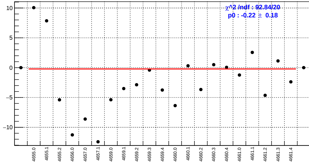
slug72B: us_avg_bpm4eY/(ppb/nm)
