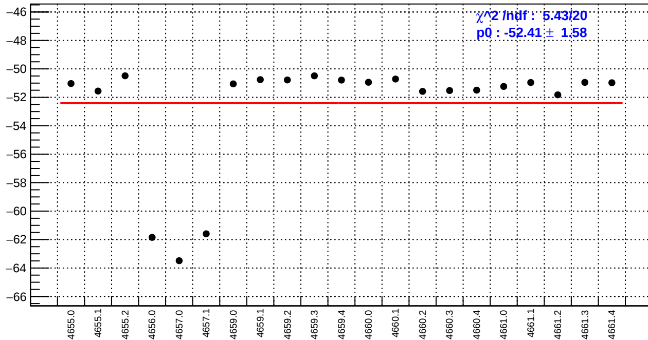
slug72B: ds_avg_bpm12X/(ppb/nm)
