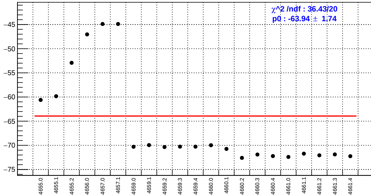
slug72B: dsl_bpm4eX/(ppb/nm)
