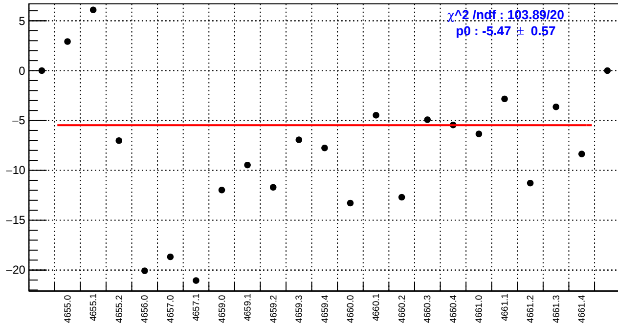
slug72B: dsr_bpm4eY/(ppb/nm)
