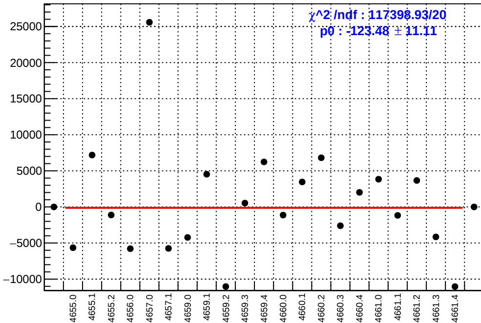
slug72B: asym_usr.mean/ppb-reg_asym_usr.mean/ppb
