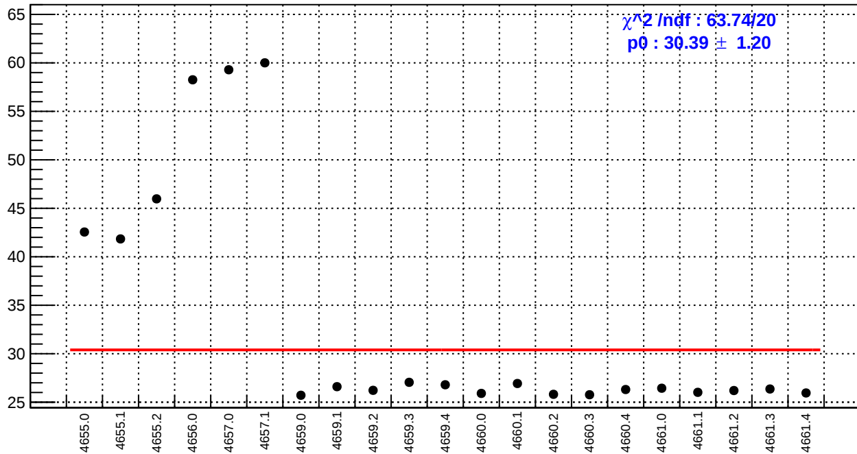
slug72B: right_avg_bpm4eX/(ppb/nm)
