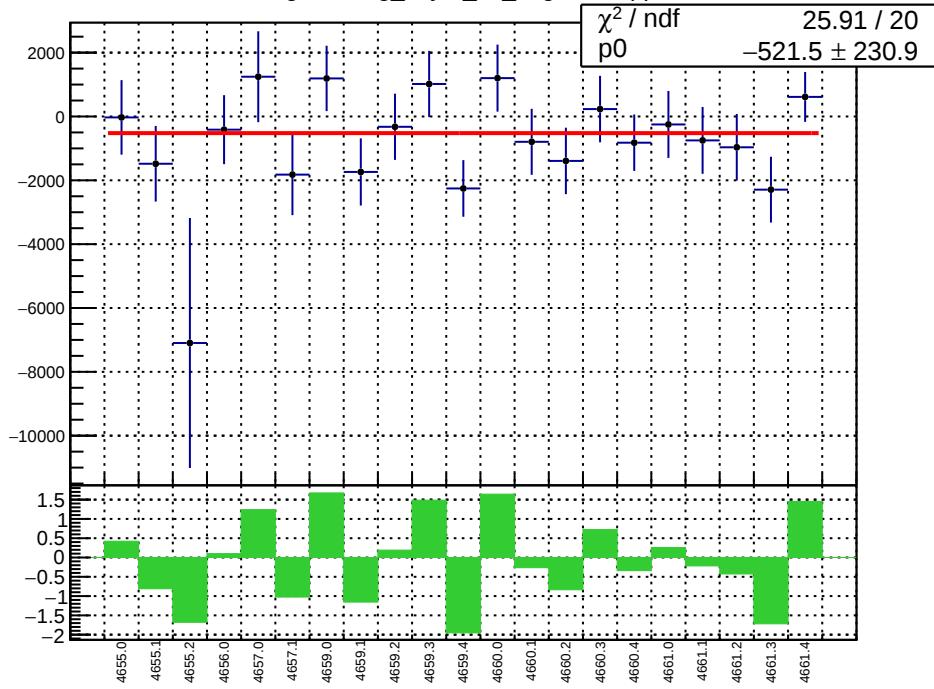
slug72B: reg_asym_ds_avg.mean/ppb
