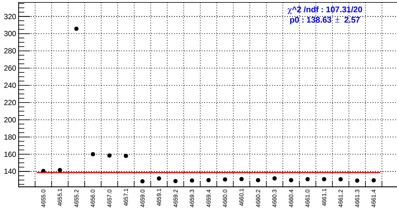
slug72B: reg_asym_usr.rms/ppm
