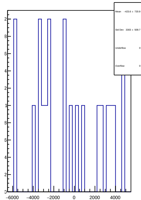
slug72B: 1D Corr asym_ds_avg.mean/ppb-reg_asym_ds_avg.mean/ppb
