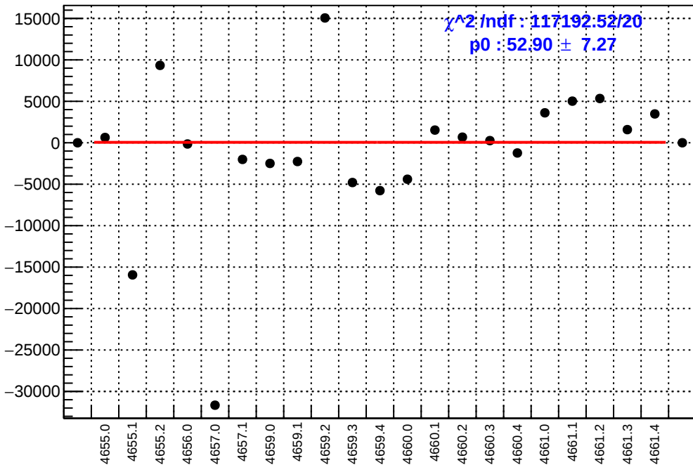
slug72B: asym_left_avg.mean/ppb-reg_asym_left_avg.mean/ppb
