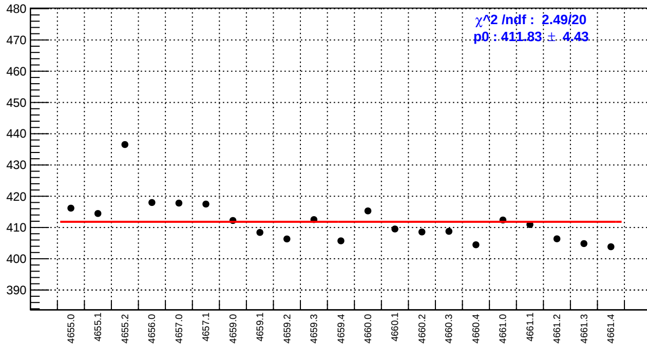
slug72B: reg_asym_at1_avg.rms/ppm
