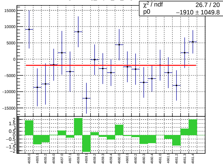
slug72B: reg_asym_atl_avg.mean/ppb
