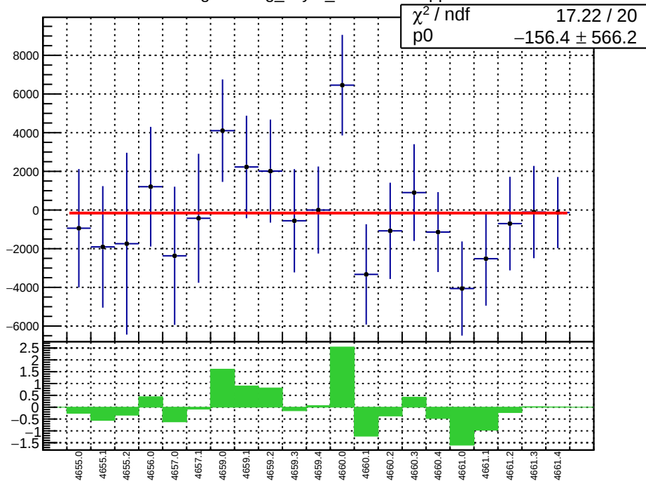
slug72B: reg_asym_sam1.mean/ppb
