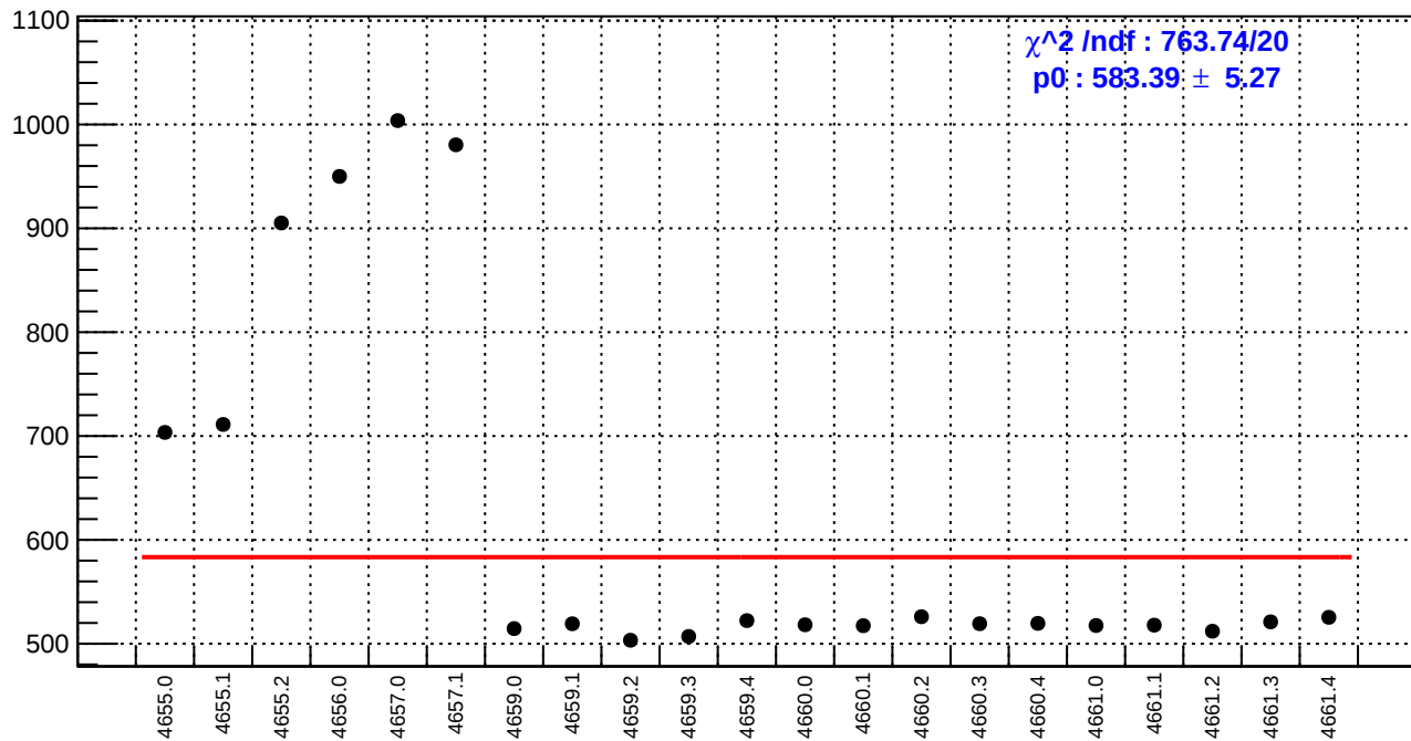
slug72B: reg_asym_atl2.rms/ppm
