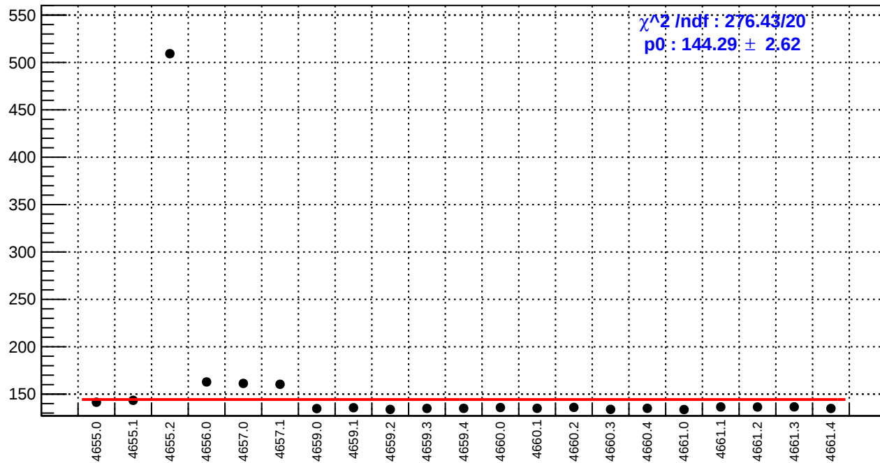
slug72B: reg_asym_left_avg.rms/ppm
