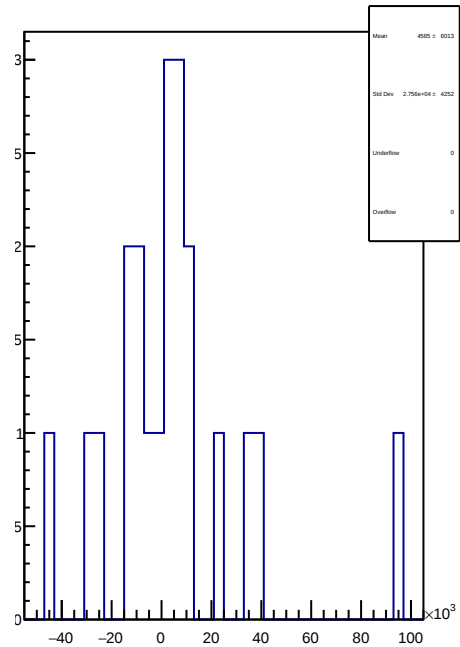
slug72B: 1D Corr asym_sam8.mean/ppb-reg_asym_sam8.mean/ppb
