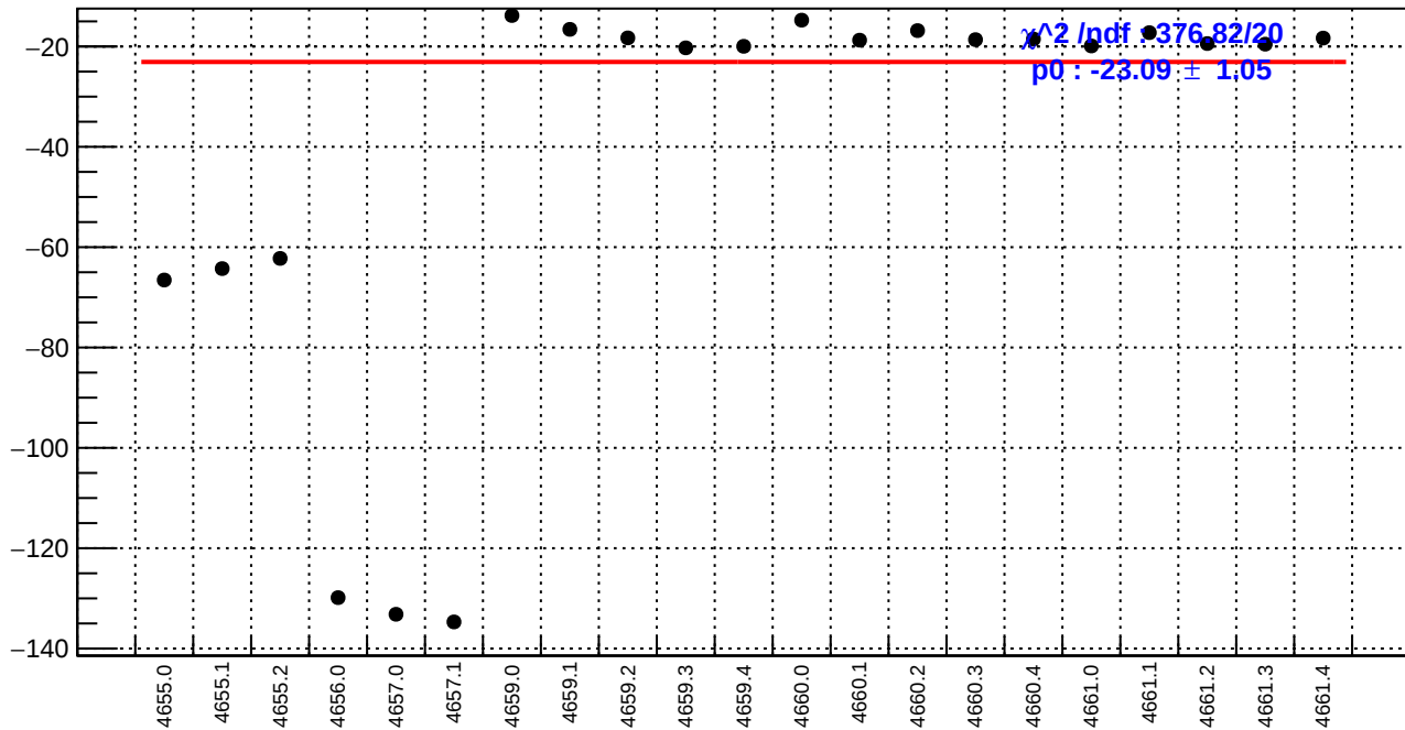
slug72B: right_avg_bpm4aX/(ppb/nm)
