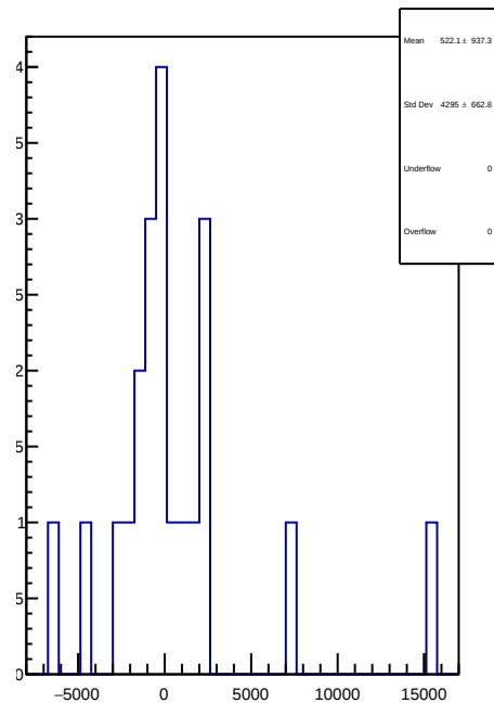
slug72B: 1D Corr asym_at1_avg.mean/ppb-reg_asym_at1_avg.mean/ppb
