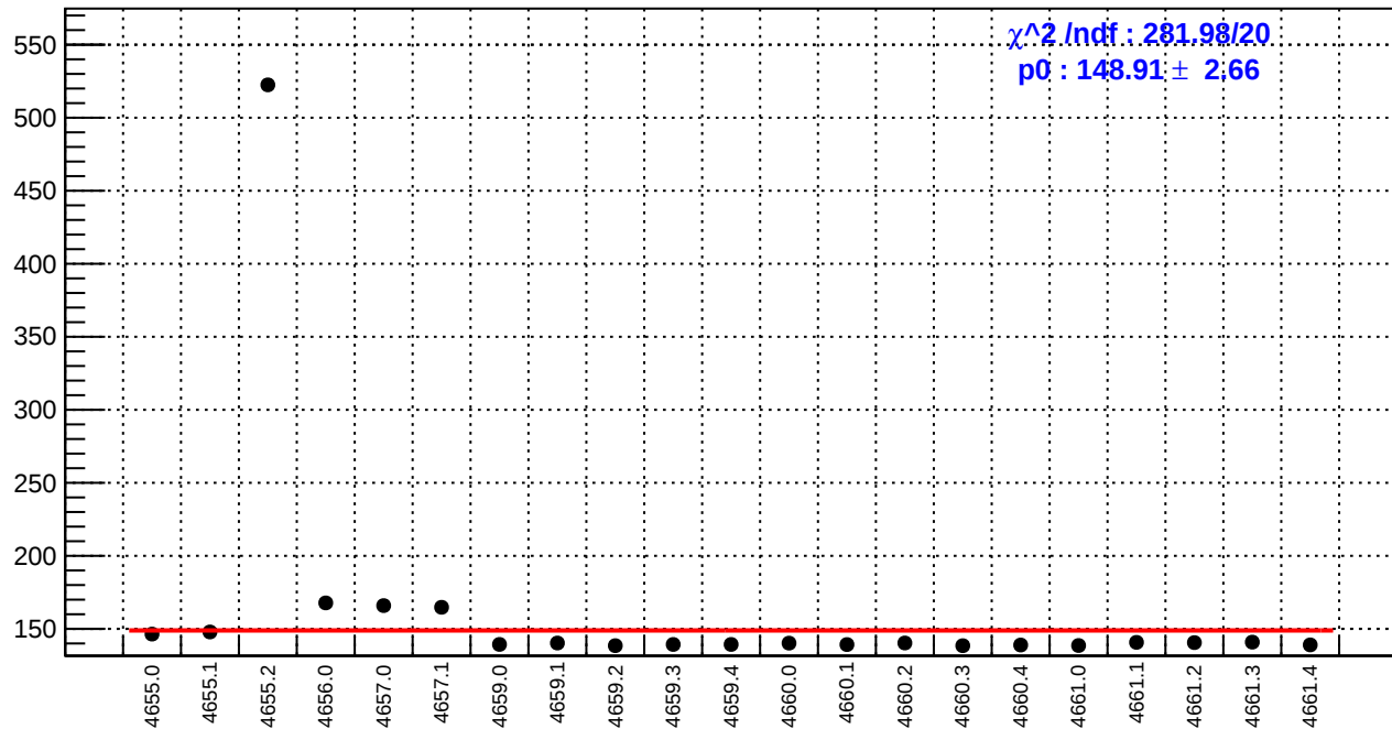
slug72B: reg_asym_dsl.rms/ppm
