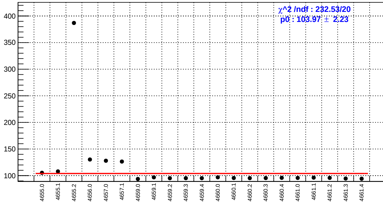
slug72B: reg_asym_us_avg.rms/ppm
