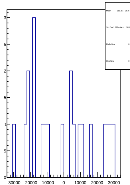
slug72B: 1D Corr asym_atl_avg.mean/ppb-reg_asym_atl_avg.mean/ppb
