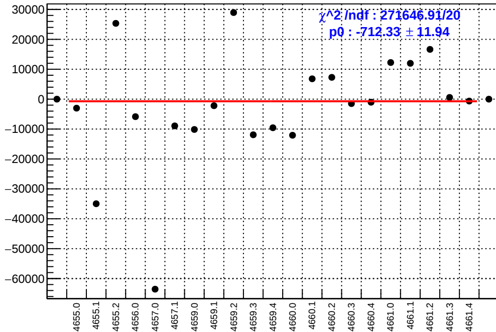
slug72B: asym_atr1l2_avg.mean/ppb-reg_asym_atr1l2_avg.mean/ppb
