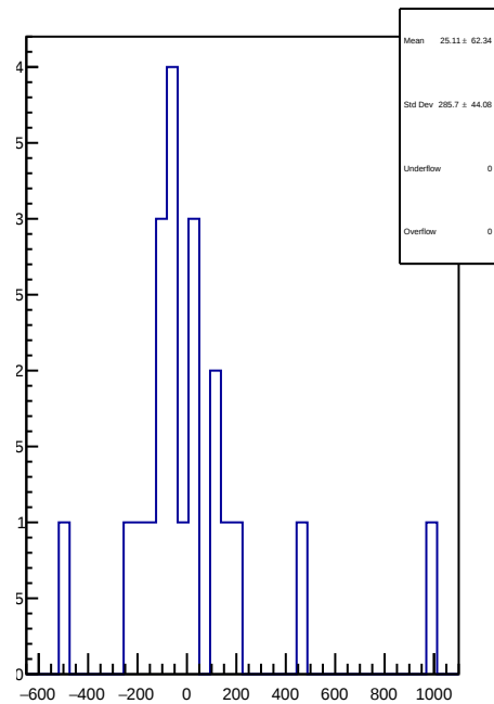
slug72B: 1D Corr asym_left_dd.mean/ppb-reg_asym_left_dd.mean/ppb
