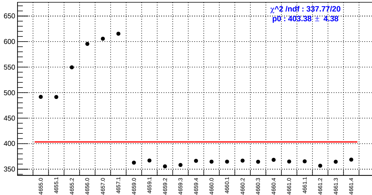
slug72B: reg_asym_atr1l2_dd.rms/ppm
