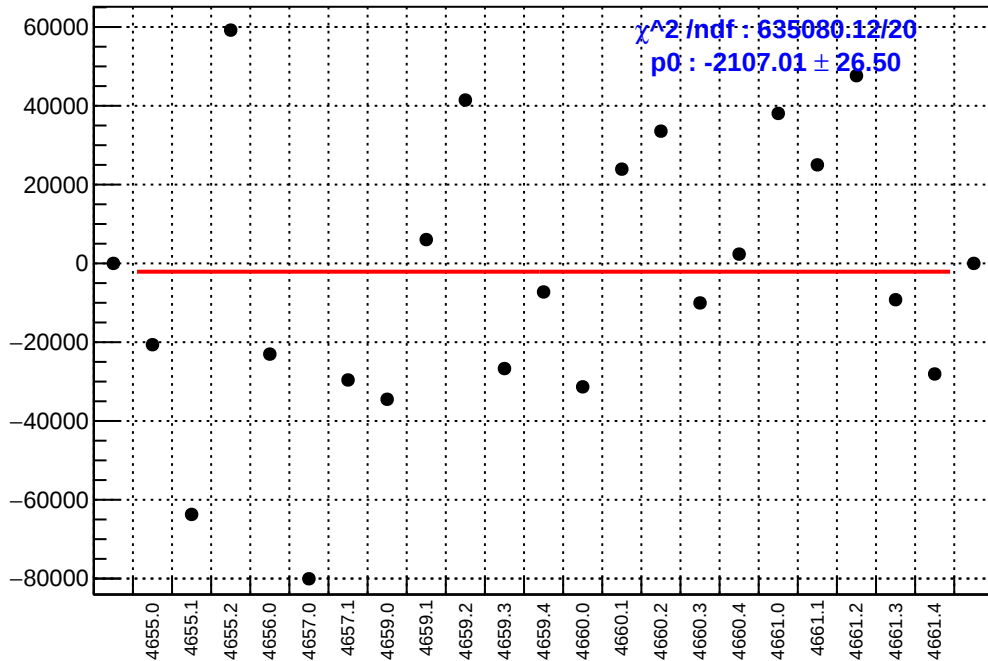
slug72B: asym_atl2.mean/ppb-reg_asym_atl2.mean/ppb
