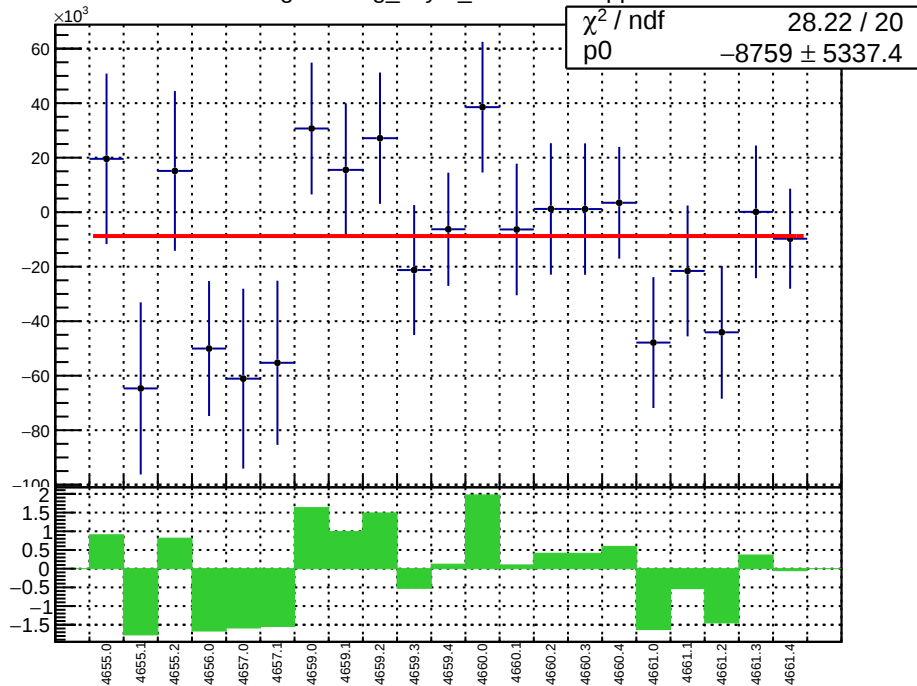
slug72B: reg_asym_sam2.mean/ppb
