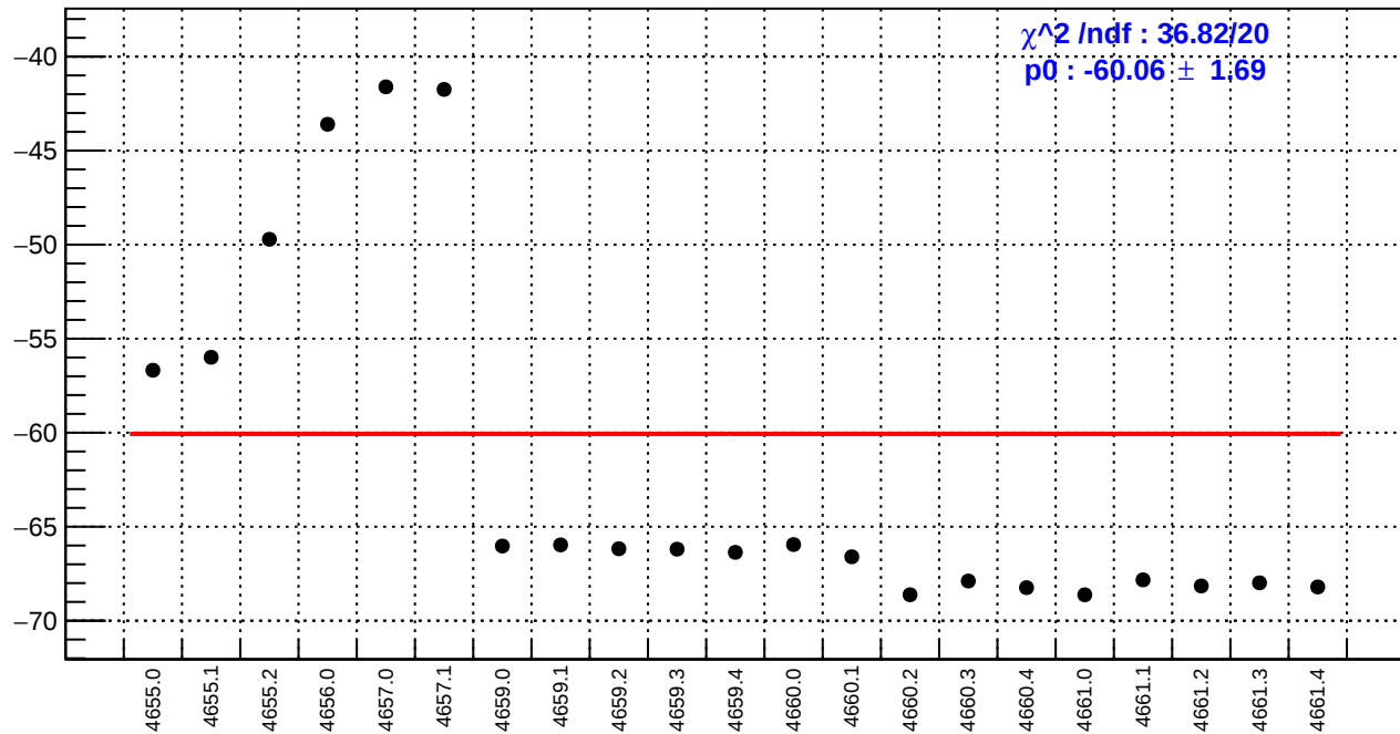
slug72B: usl_bpm4eX/(ppb/nm)
