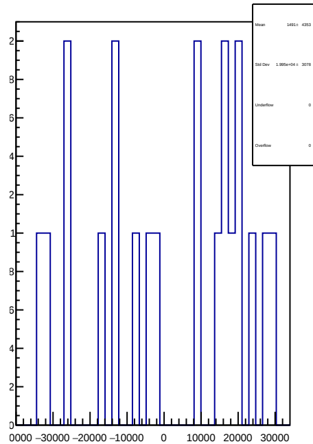
slug72B: 1D Corr asym_atr1i2_dd.mean/ppb-reg_asym_atr1i2_dd.mean/ppb
