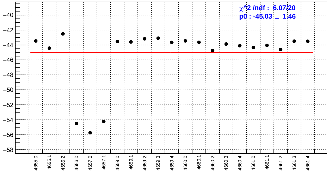
slug72B: dsl_bpm12X/(ppb/nm)
