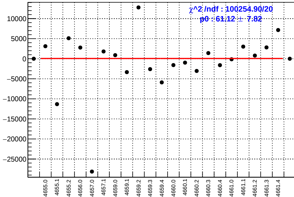
slug72B: asym_us_dd.mean/ppb-reg_asym_us_dd.mean/ppb
