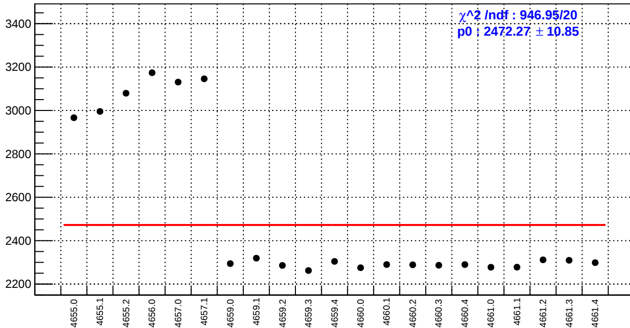
slug72B: reg_asym_sam2.rms/ppm
