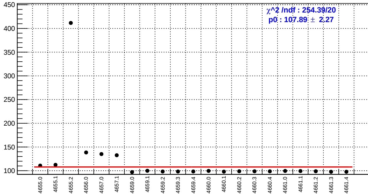
slug72B: reg_asym_ds_avg.rms/ppm
