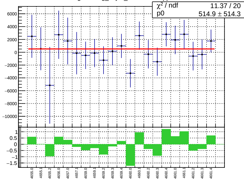
slug72B: reg_asym_sam5.mean/ppb
