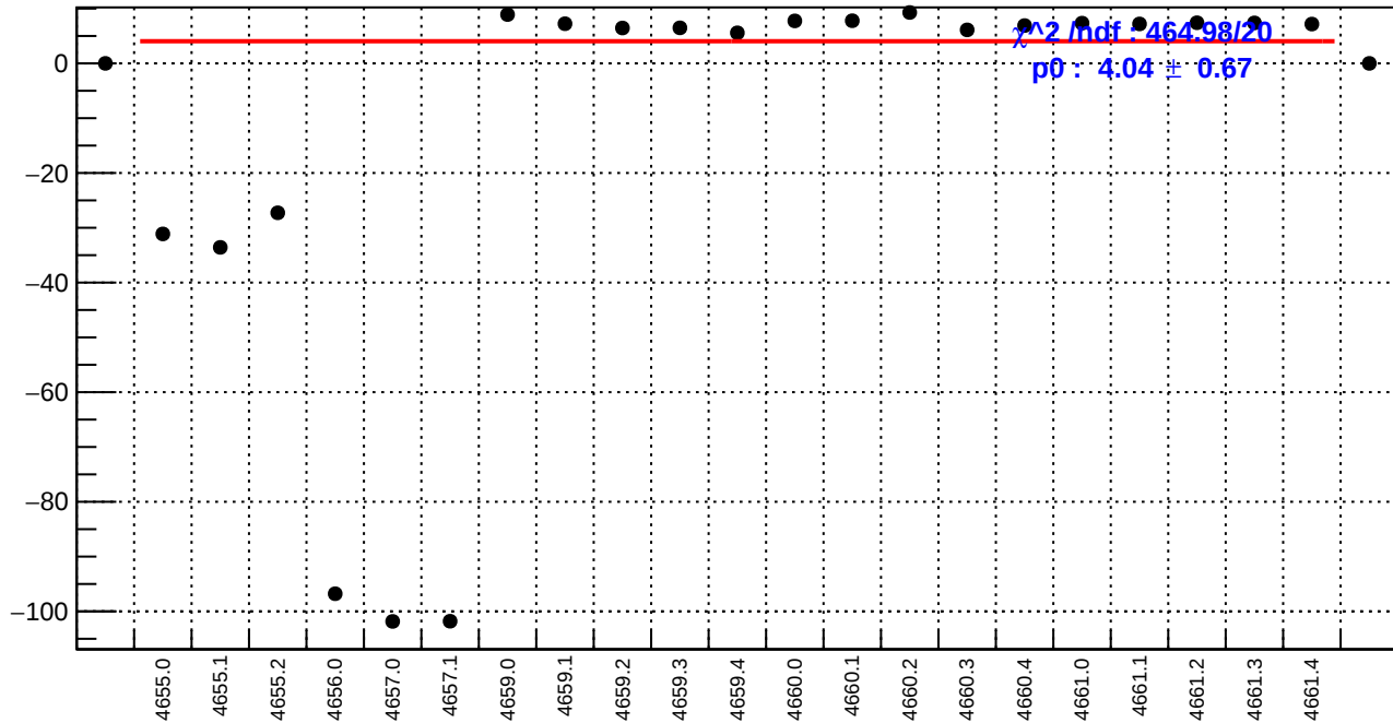
slug72B: ds_avg_bpm4aX/(ppb/nm)
