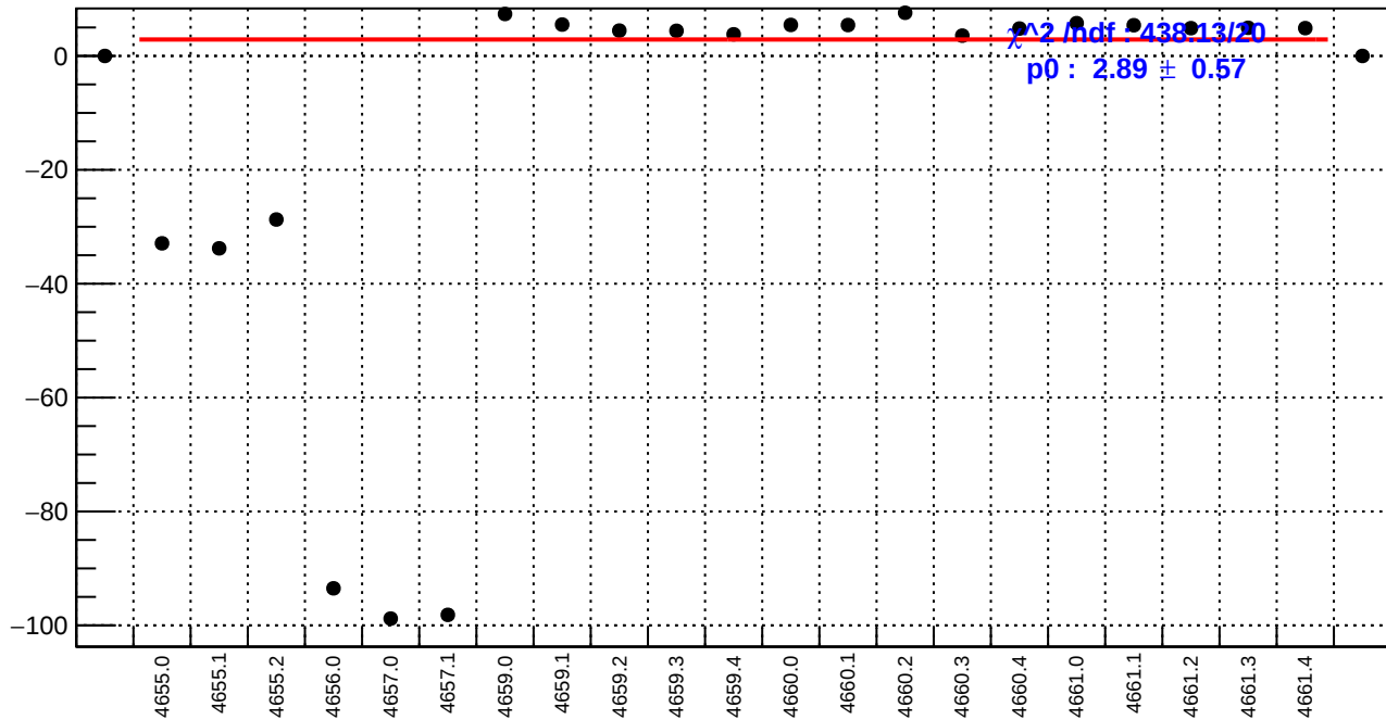
slug72B: us_avg_bpm4aX/(ppb/nm)
