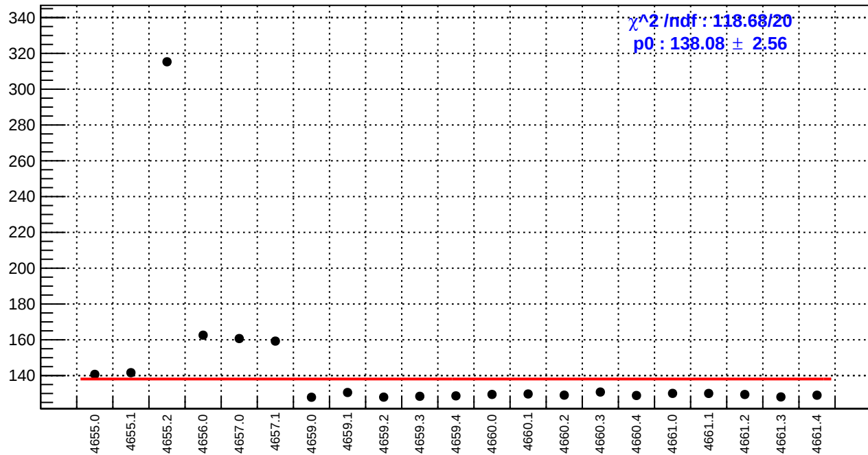
slug72B: reg_asym_right_avg.rms/ppm
