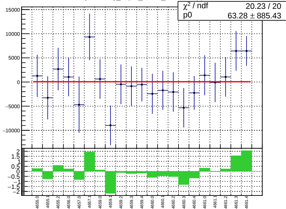
slug72B: reg_asym_atl1r2_dd.mean/ppb
