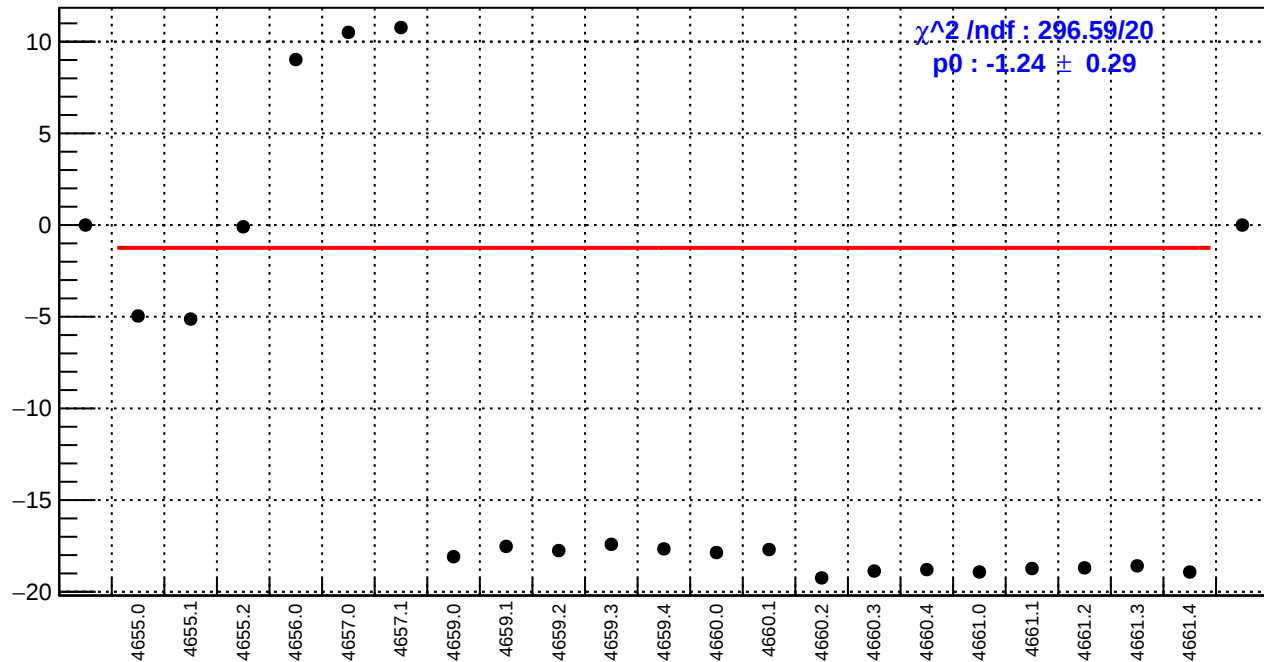
slug72B: us_avg_bpm4eX/(ppb/nm)
