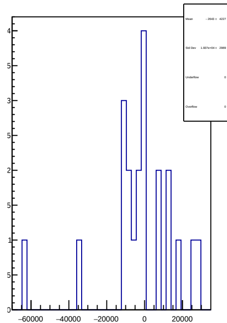
slug72B: 1D Corr asym_atr1l2_avg.mean/ppb-reg_asym_atr1l2_avg.mean/ppb
