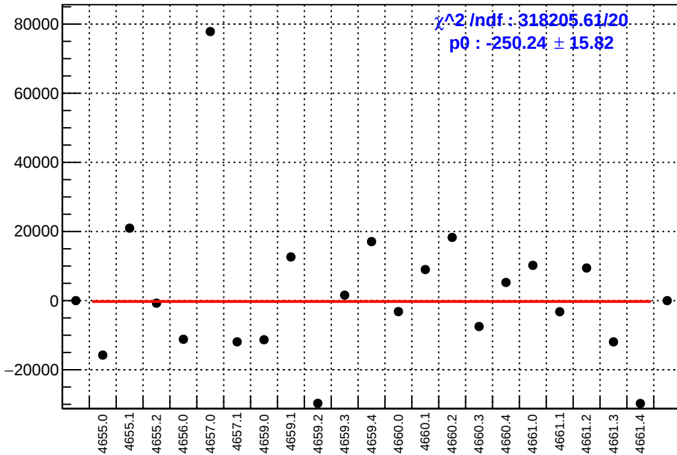
slug72B: asym_atl1.mean/ppb-reg_asym_atl1.mean/ppb
