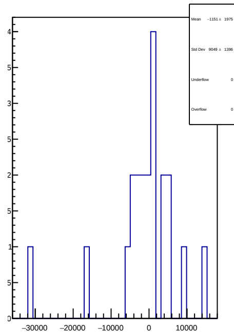
slug72B: 1D Corr asym_left_avg.mean/ppb-reg_asym_left_avg.mean/ppb
