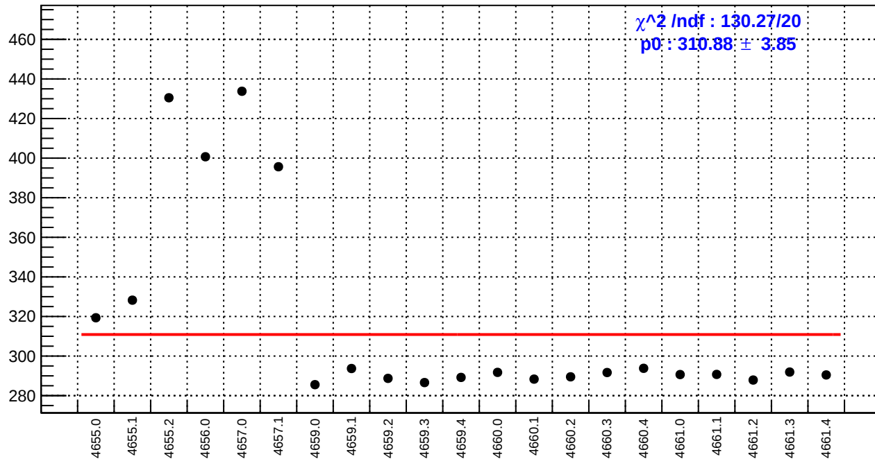
slug72B: reg_asym_atr_avg.rms/ppm
