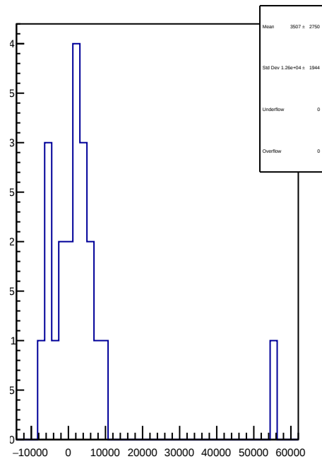
slug72B: 1D Corr asym_sam1.mean/ppb-reg_asym_sam1.mean/ppb
