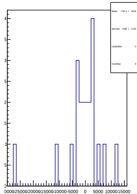
slug72B: 1D Corr asym_ds_dd.mean/ppb-reg_asym_ds_dd.mean/ppb
