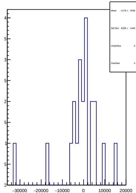
slug72B: 1D Corr asym_dsl.mean/ppb-reg_asym_dsl.mean/ppb
