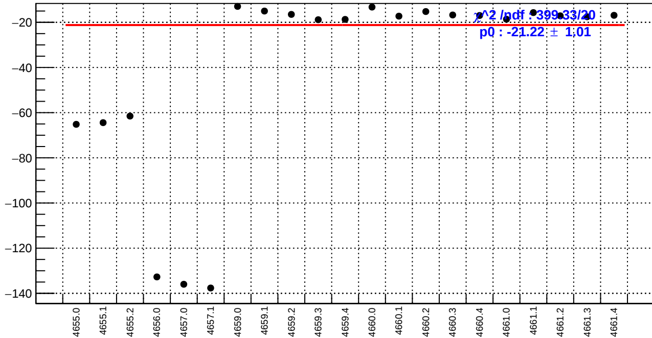
slug72B: dsr_bpm4aX/(ppb/nm)
