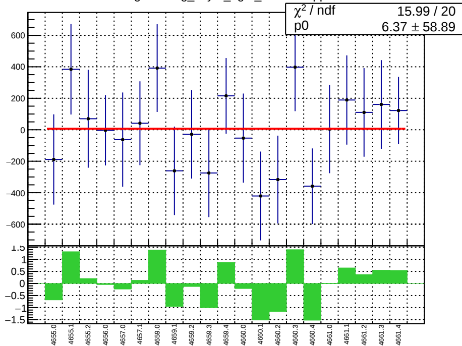
slug72B: reg_asym_right_dd.mean/ppb
