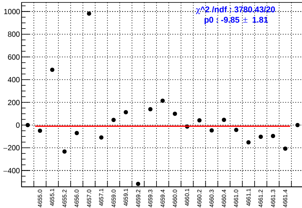
slug72B: asym_left_dd.mean/ppb-reg_asym_left_dd.mean/ppb
