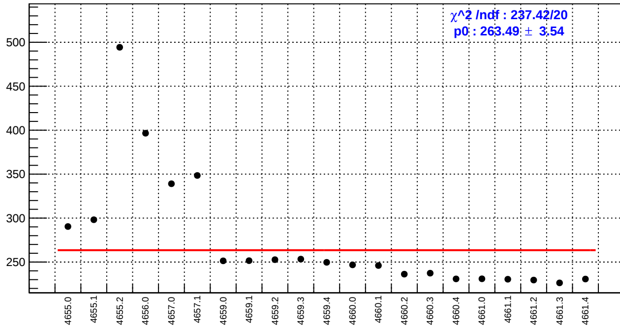
slug72B: reg_asym_sam1.rms/ppm
