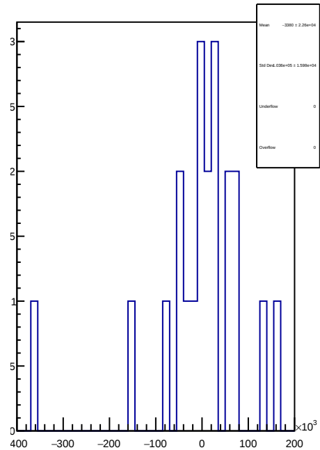
slug72B: 1D Corr asym_sam2.mean/ppb-reg_asym_sam2.mean/ppb
