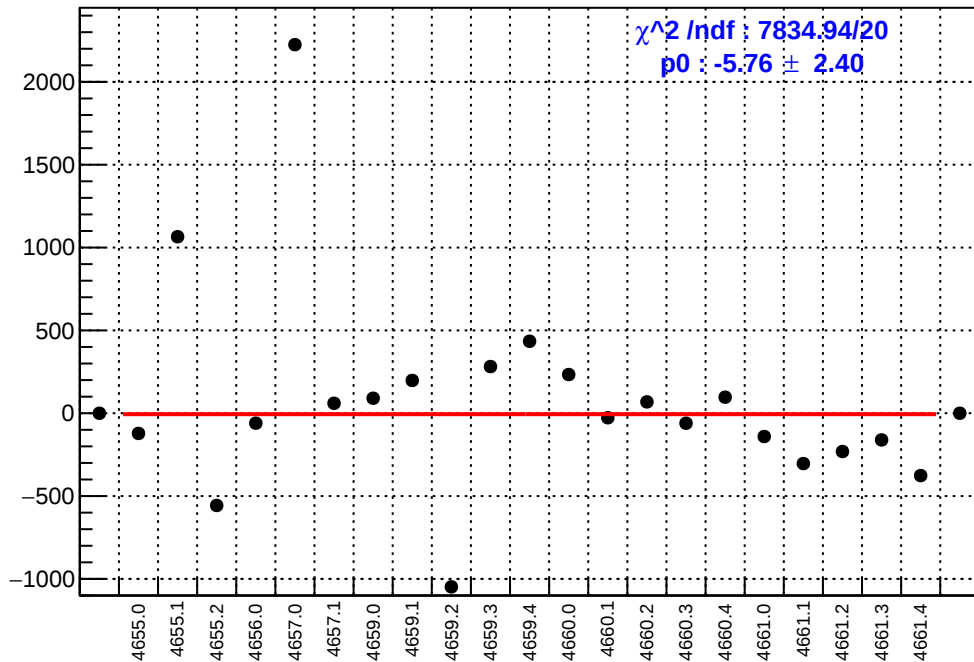
slug72B: asym_right_dd.mean/ppb-reg_asym_right_dd.mean/ppb
