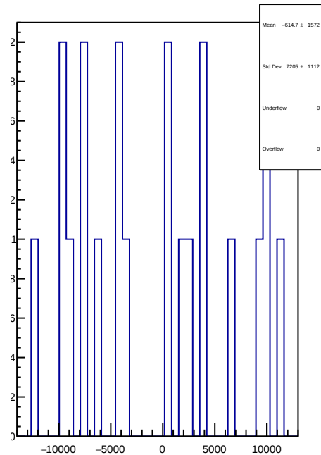
slug72B: 1D Corr asym_atr_avg.mean/ppb-reg_asym_atr_avg.mean/ppb
