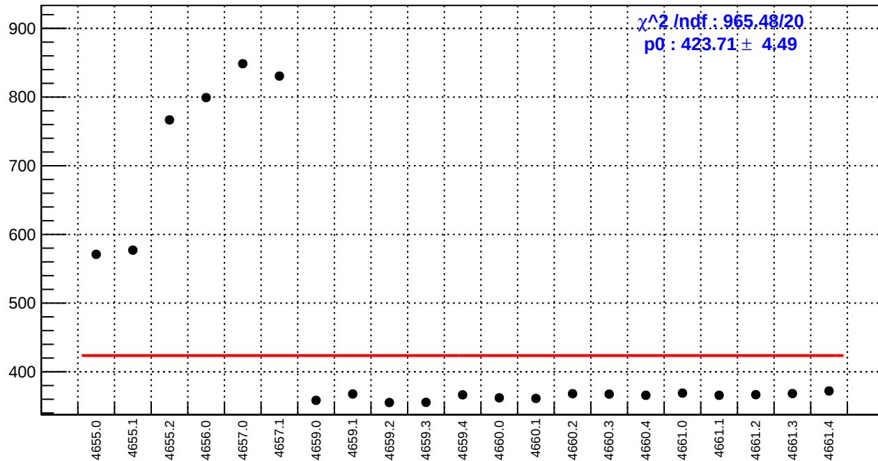
slug72B: reg_asym_at2_avg.rms/ppm
