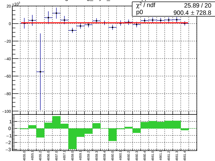
slug72B: reg_asym_sam7.mean/ppb
