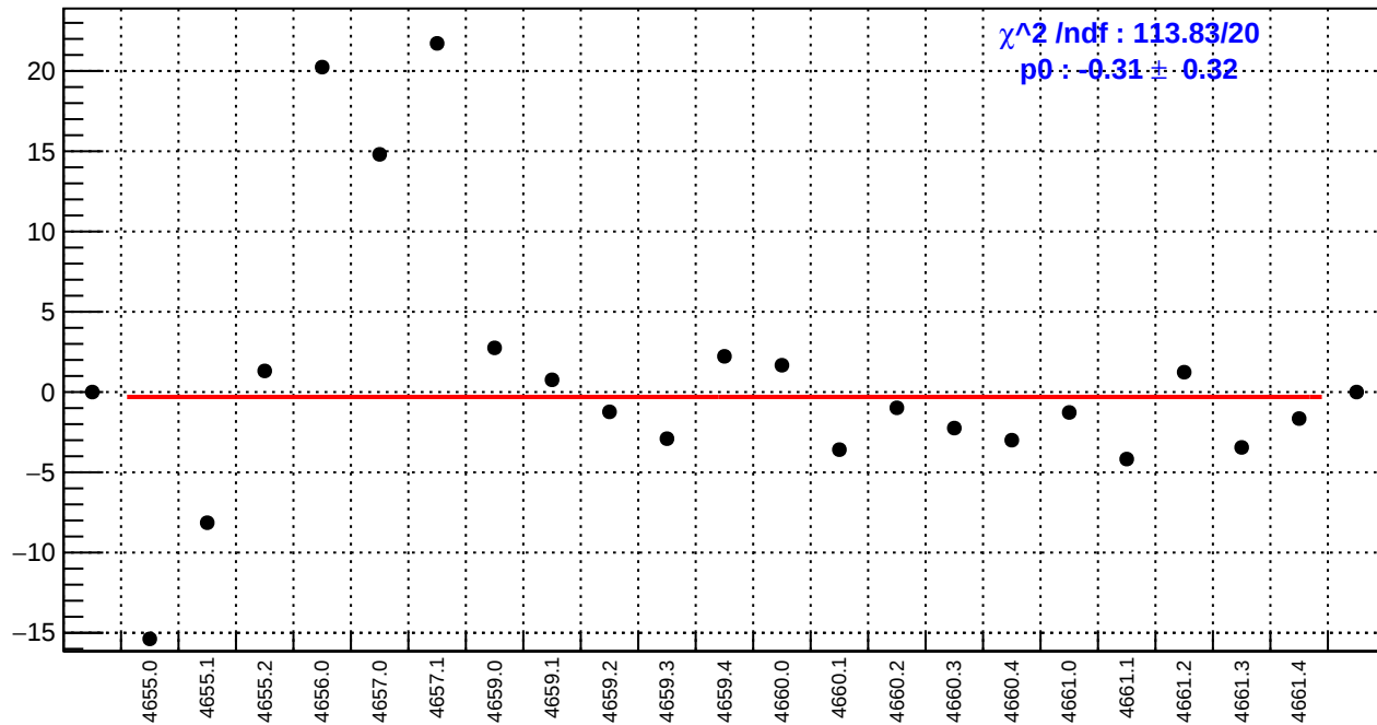
slug72B: left_avg_bpm4aY/(ppb/nm)
