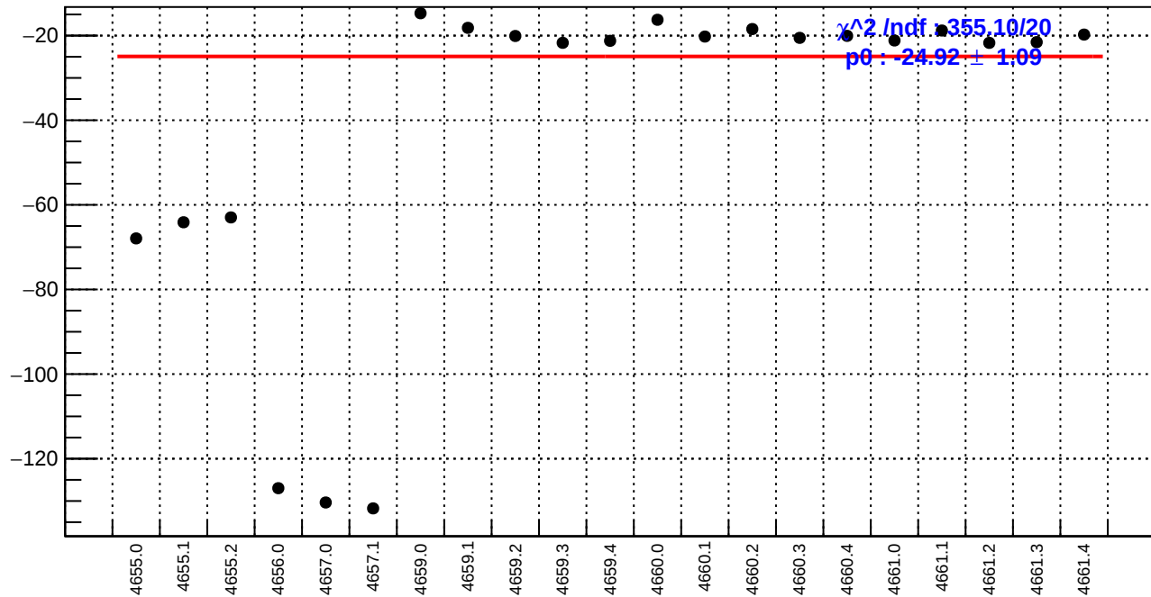
slug72B: usr_bpm4aX/(ppb/nm)
