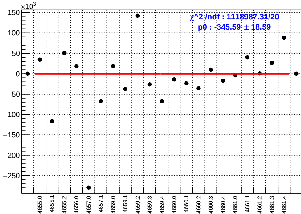
slug72B: asym_sam4.mean/ppb-reg_asym_sam4.mean/ppb
