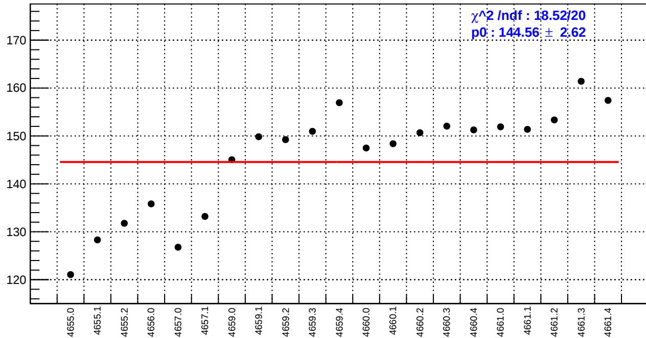
slug72B: asym_bcm_an_ds.rms/ppm
