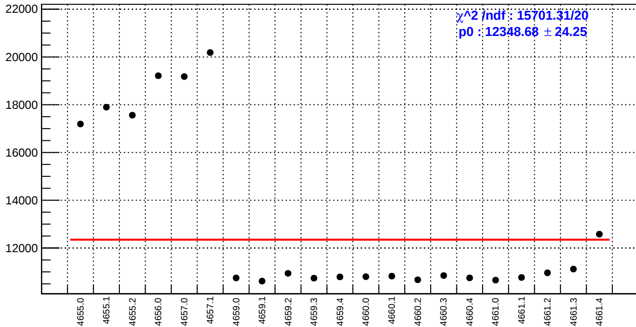
slug72B: diff_bpm4eX.rms/nm
