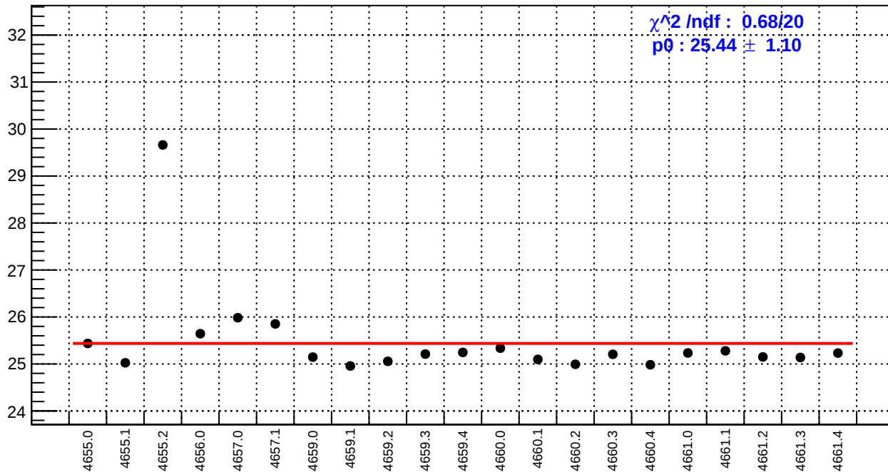
slug72B: reg_asym_left_dd.rms/ppm
