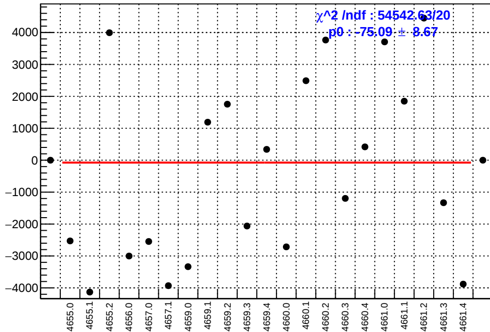
slug72B: asym_us_avg.mean/ppb-reg_asym_us_avg.mean/ppb
