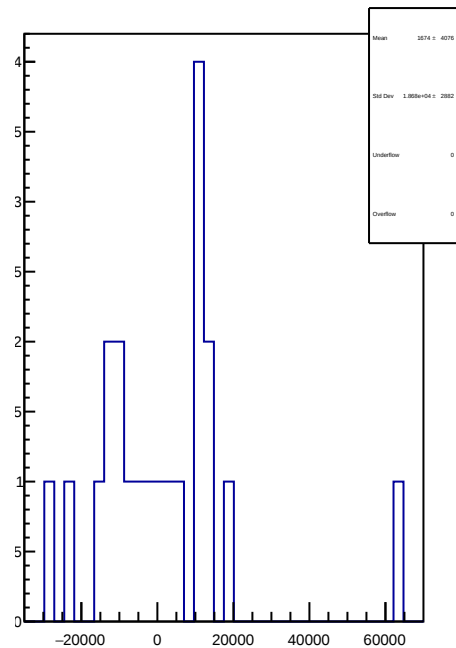
slug72B: 1D Corr asym_at1_dd.mean/ppb-reg_asym_at1_dd.mean/ppb
