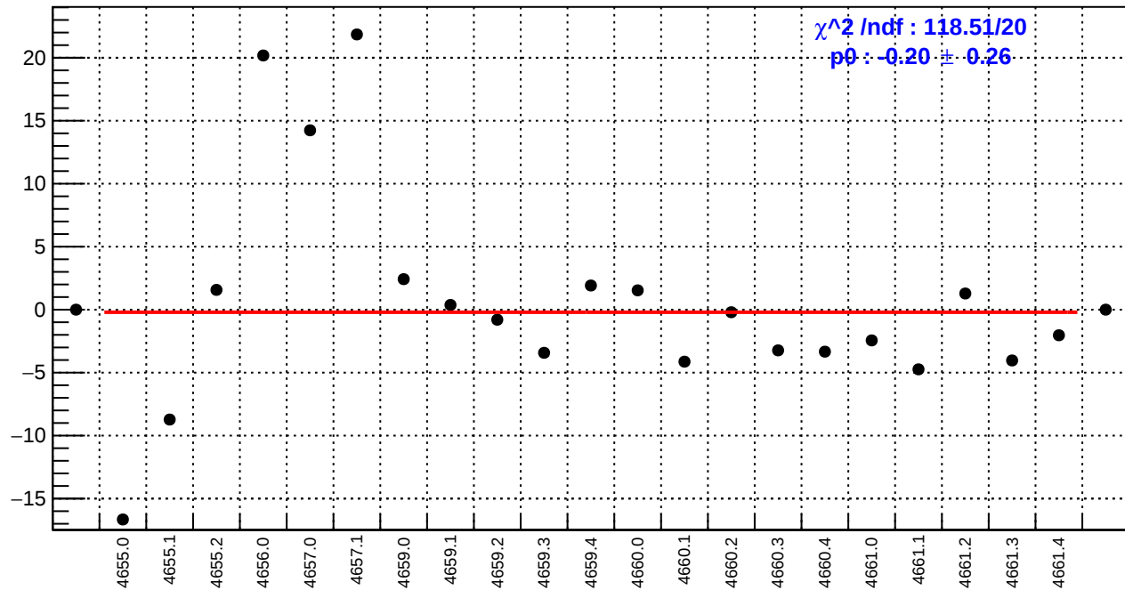
slug72B: dsl_bpm4aY/(ppb/nm)
