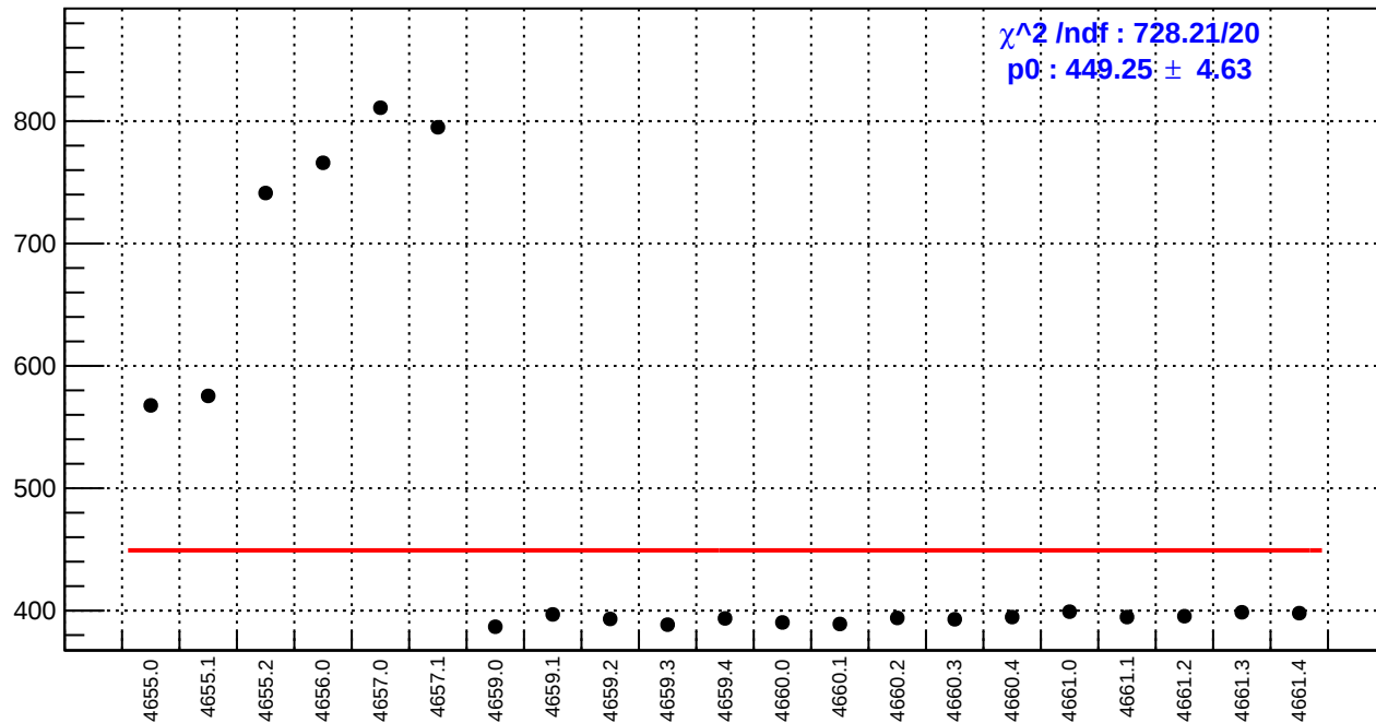
slug72B: reg_asym_atr2.rms/ppm
