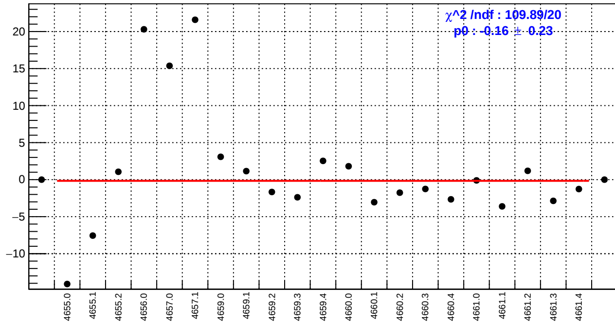
slug72B: usl_bpm4aY/(ppb/nm)
