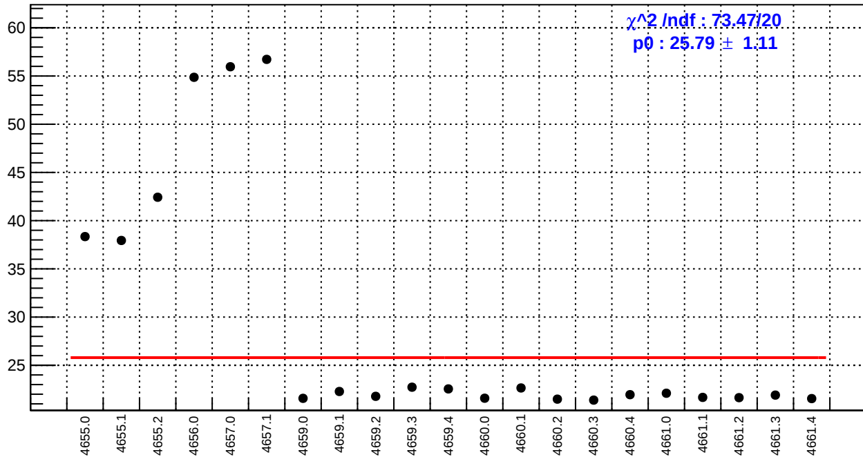
slug72B: dsr_bpm4eX/(ppb/nm)
