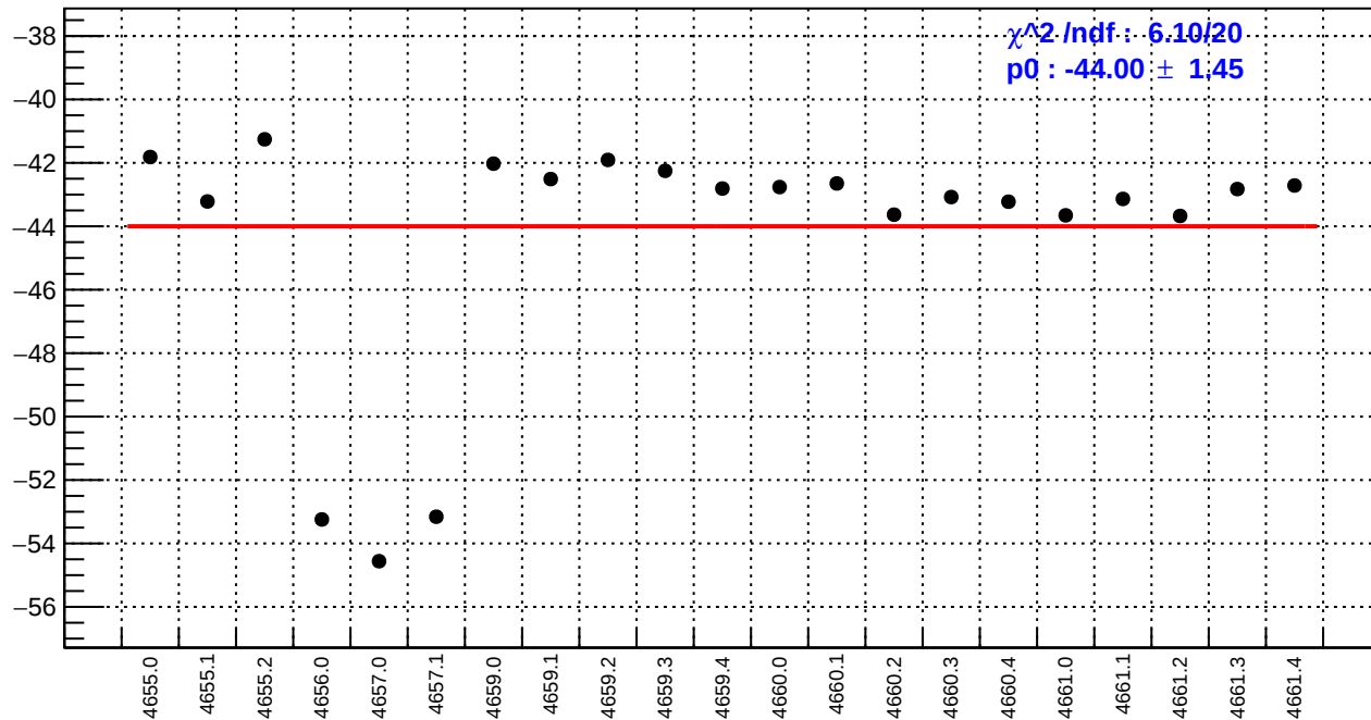
slug72B: usl_bpm12X/(ppb/nm)
