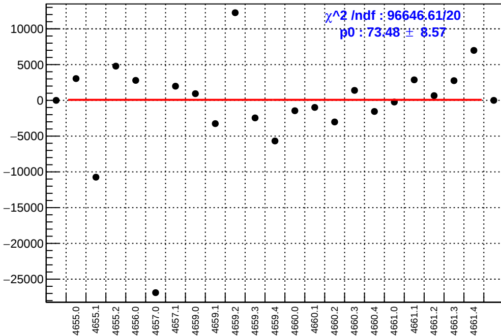
slug72B: asym_ds_dd.mean/ppb-reg_asym_ds_dd.mean/ppb
