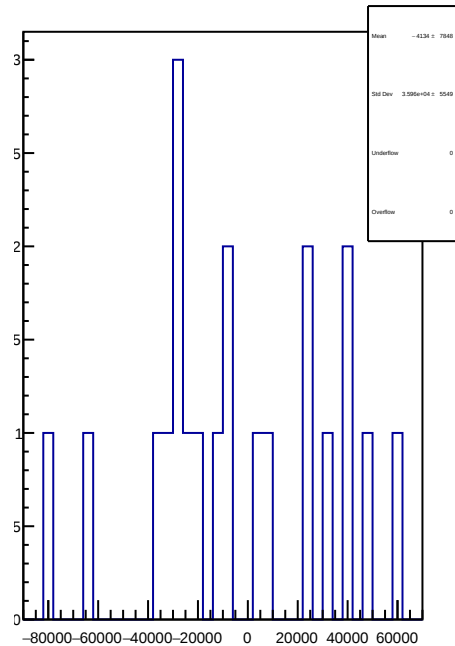
slug72B: 1D Corr asym_atl2.mean/ppb-reg_asym_atl2.mean/ppb
