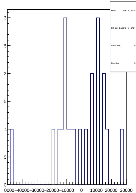
slug72B: 1D Corr asym_atr1.mean/ppb-reg_asym_atr1.mean/ppb
