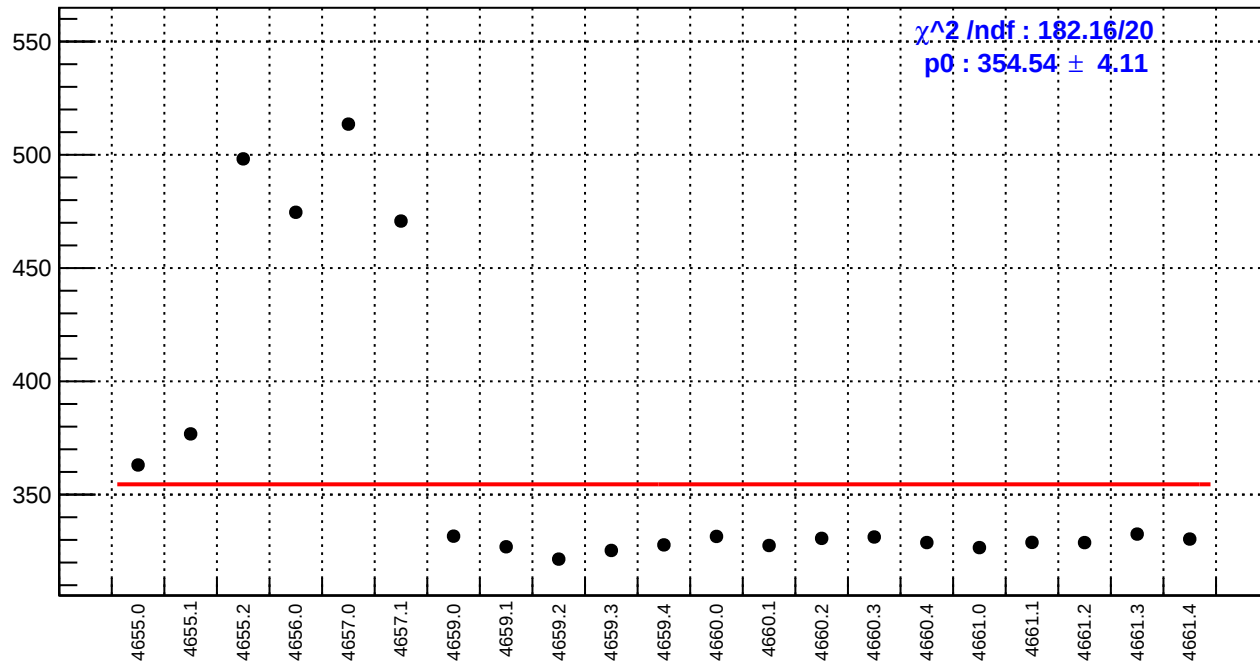
slug72B: reg_asym_atr1l2_avg.rms/ppm
