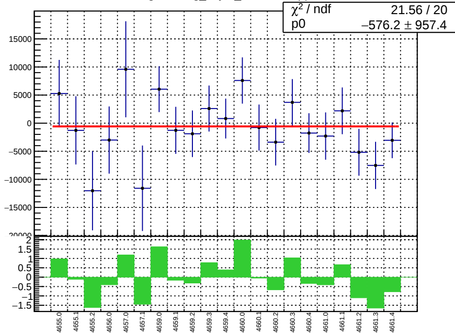
slug72B: reg_asym_atr2.mean/ppb
