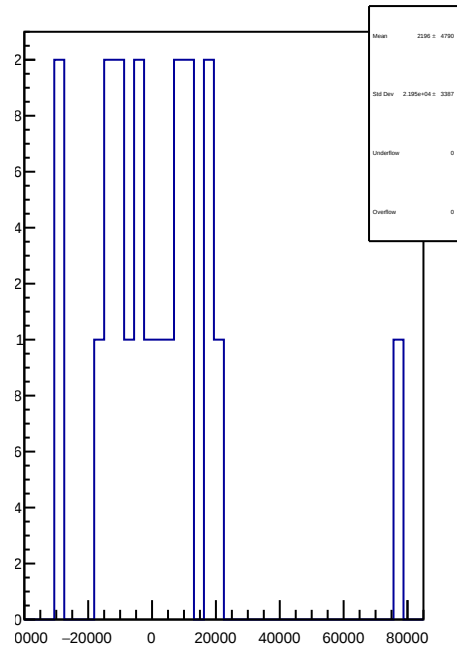
slug72B: 1D Corr asym_atl1.mean/ppb-reg_asym_atl1.mean/ppb
