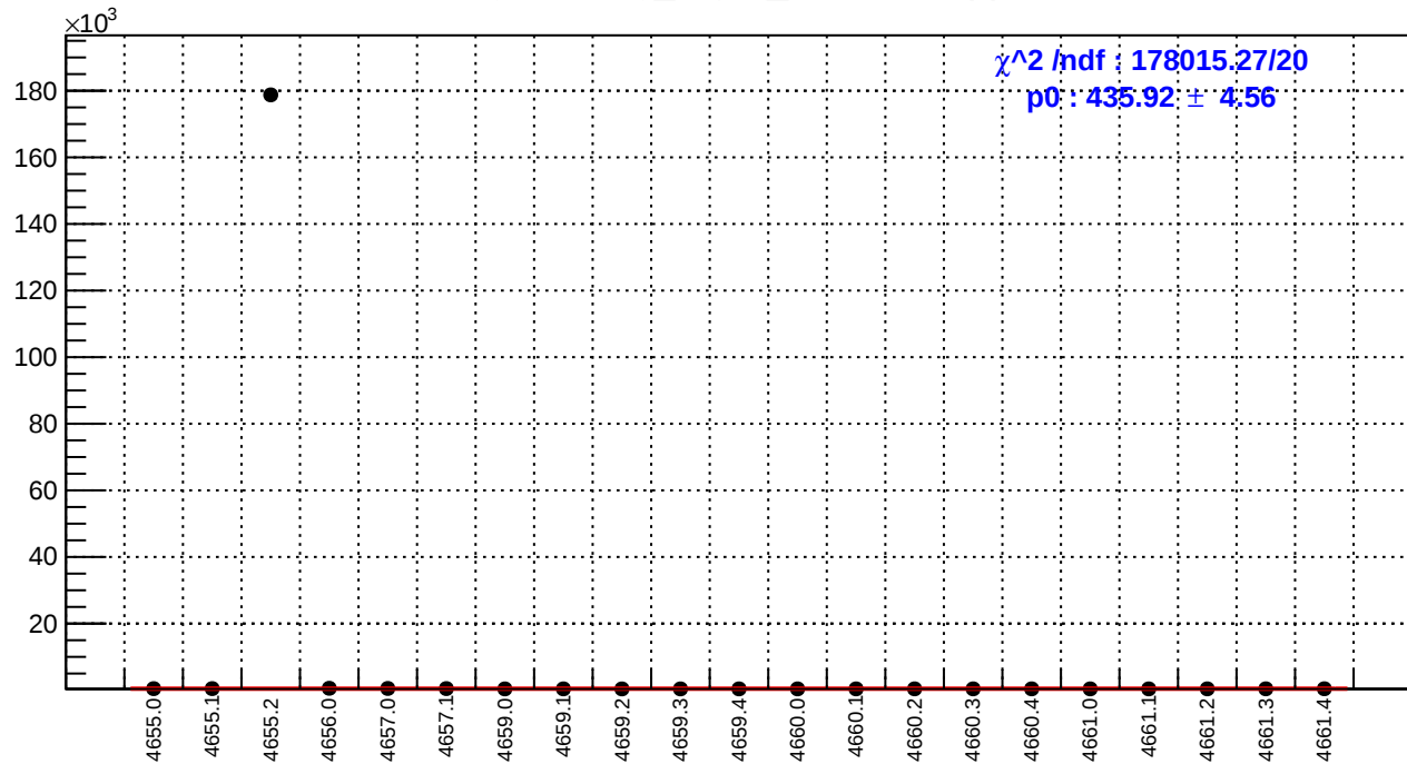
slug72B: reg_asym_sam6.rms/ppm
