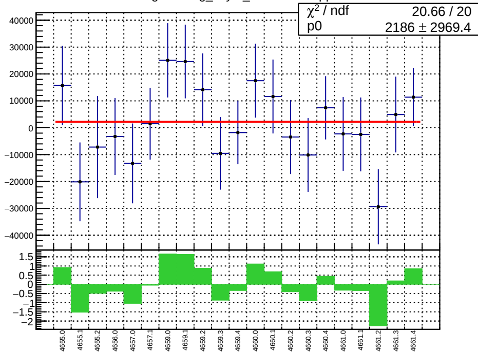
slug72B: reg_asym_sam4.mean/ppb
