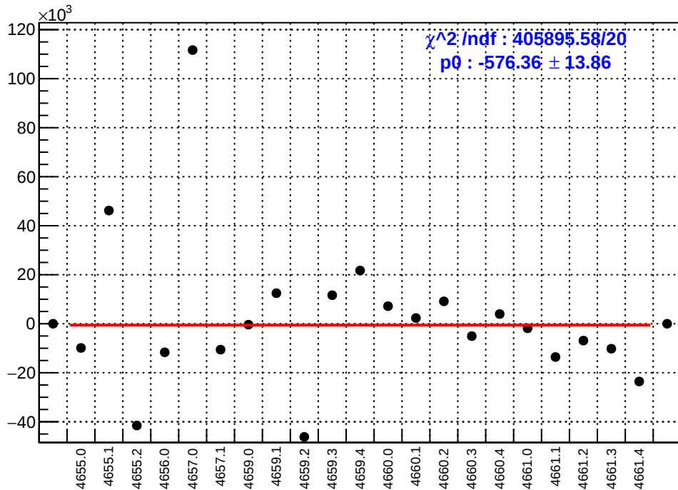
slug72B: asym_sam7.mean/ppb-reg_asym_sam7.mean/ppb
