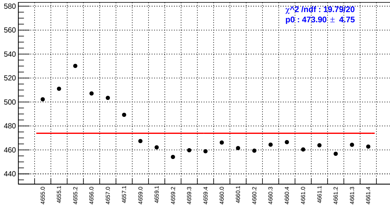
slug72B: reg_asym_atr1.rms/ppm
