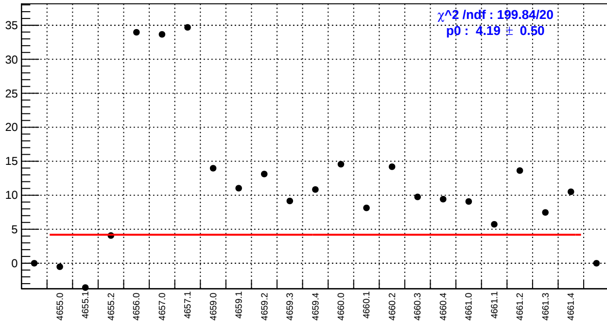
slug72B: right_avg_bpm4aY/(ppb/nm)
