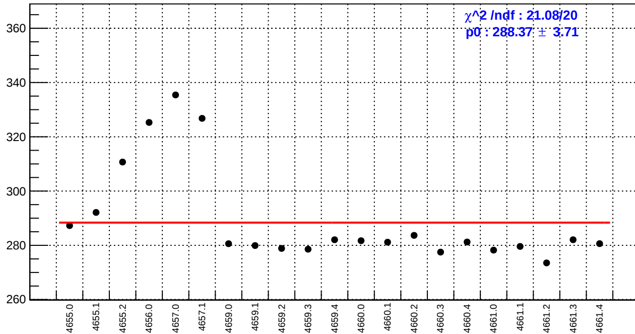
slug72B: reg_asym_at2_dd.rms/ppm
