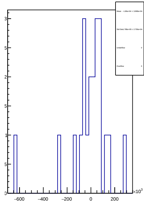
slug72B: 1D Corr asym_sam3.mean/ppb-reg_asym_sam3.mean/ppb
