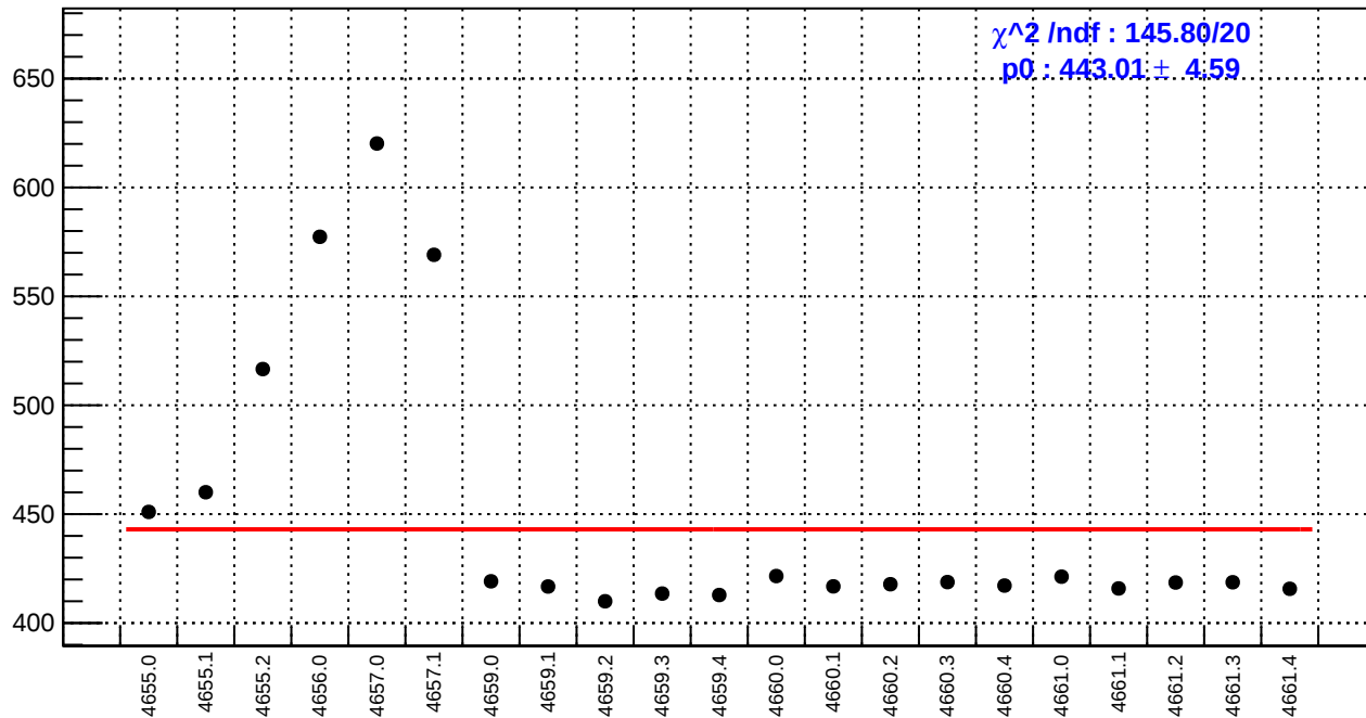
slug72B: reg_asym_atl_dd.rms/ppm
