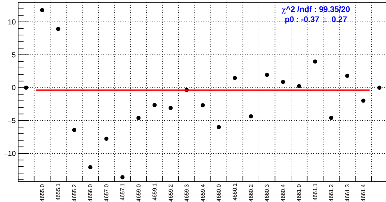
slug72B: ds_avg_bpm4eY/(ppb/nm)
