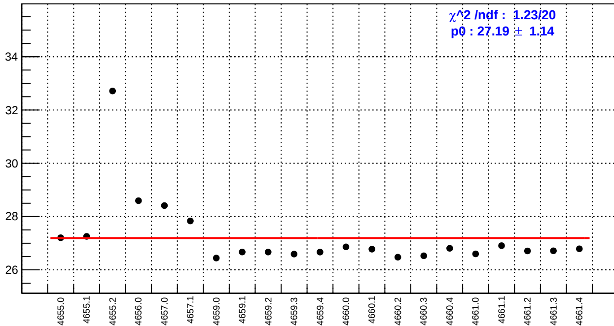
slug72B: reg_asym_right_dd.rms/ppm
