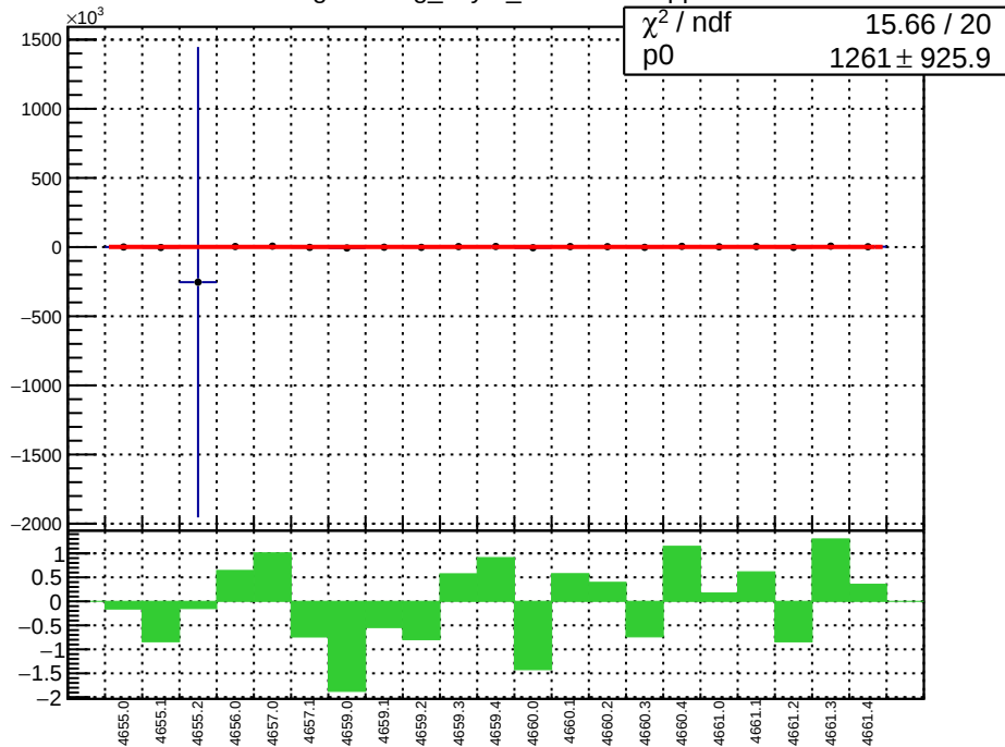
slug72B: reg_asym_sam6.mean/ppb
