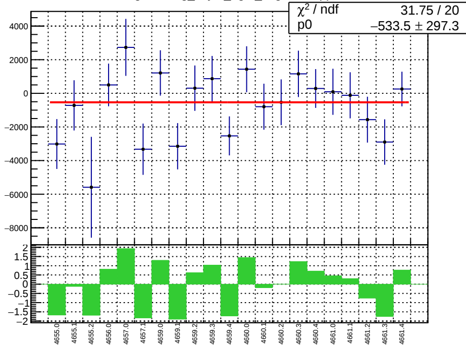
slug72B: reg_asym_right_avg.mean/ppb
