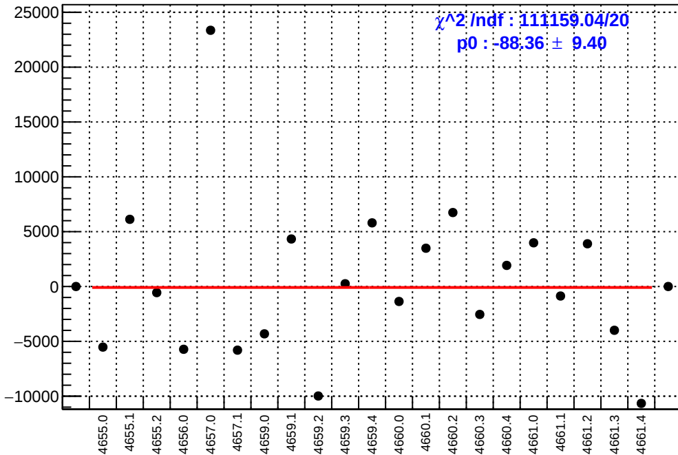
slug72B: asym_right_avg.mean/ppb-reg_asym_right_avg.mean/ppb
