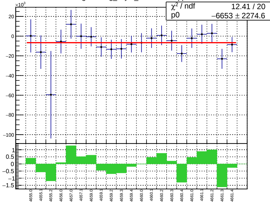
slug72B: reg_asym_sam3.mean/ppb
