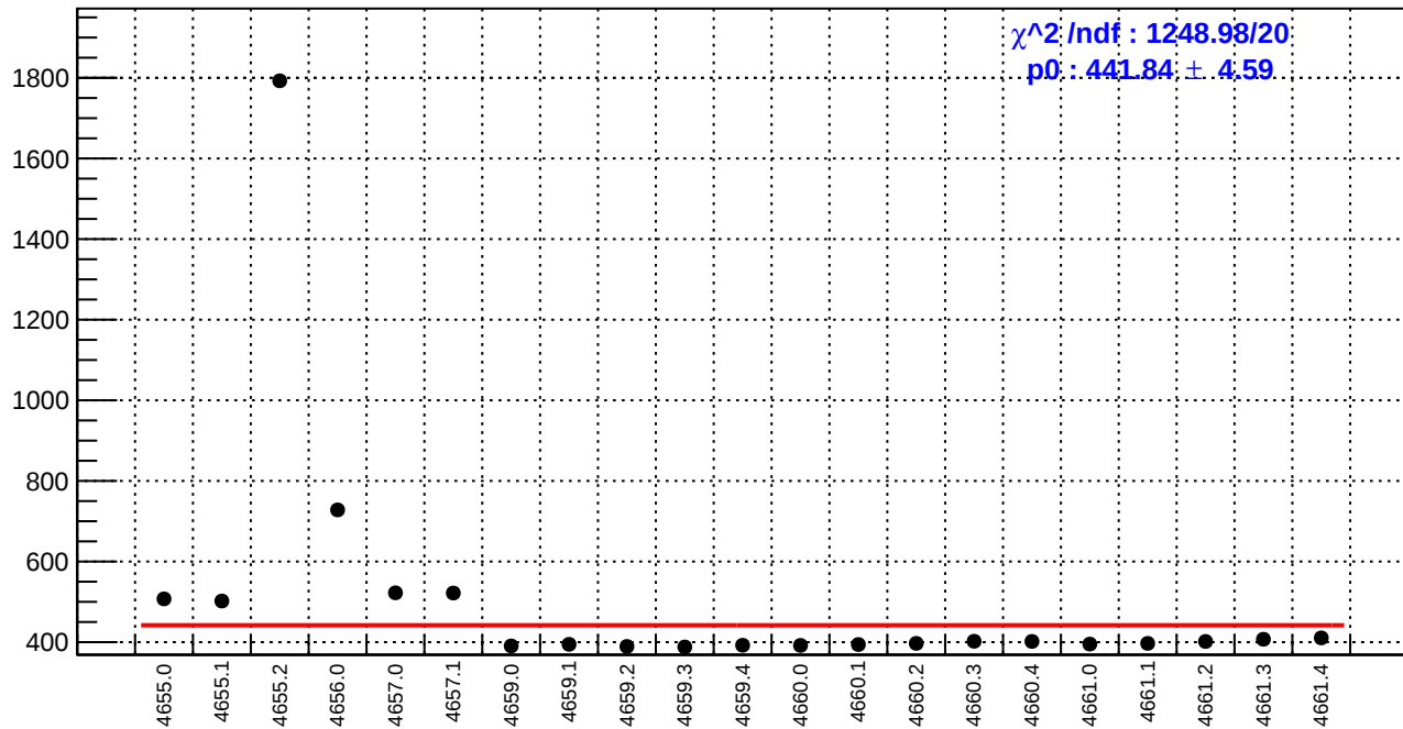
slug72B: reg_asym_sam8.rms/ppm
