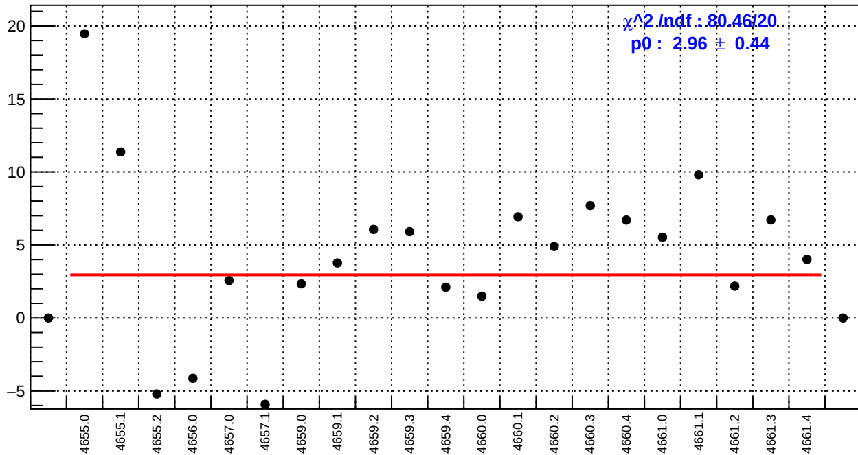
slug72B: left_avg_bpm4eY/(ppb/nm)
