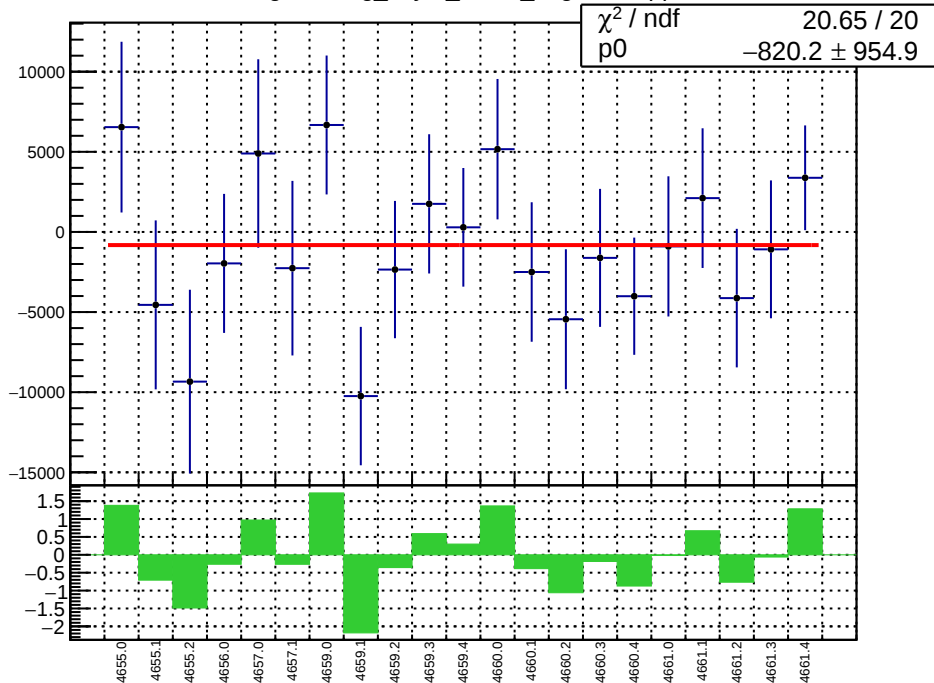
slug72B: reg_asym_atl1r2_avg.mean/ppb
