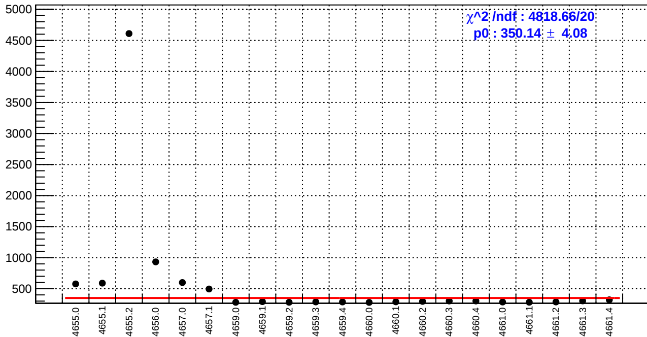
slug72B: reg_asym_sam7.rms/ppm
