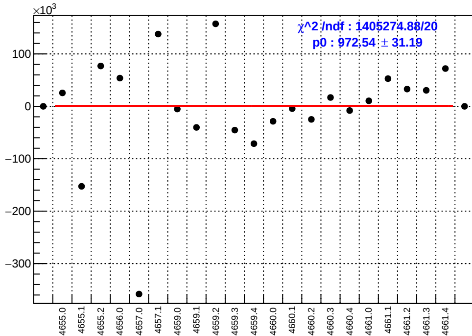
slug72B: asym_sam2.mean/ppb-reg_asym_sam2.mean/ppb
