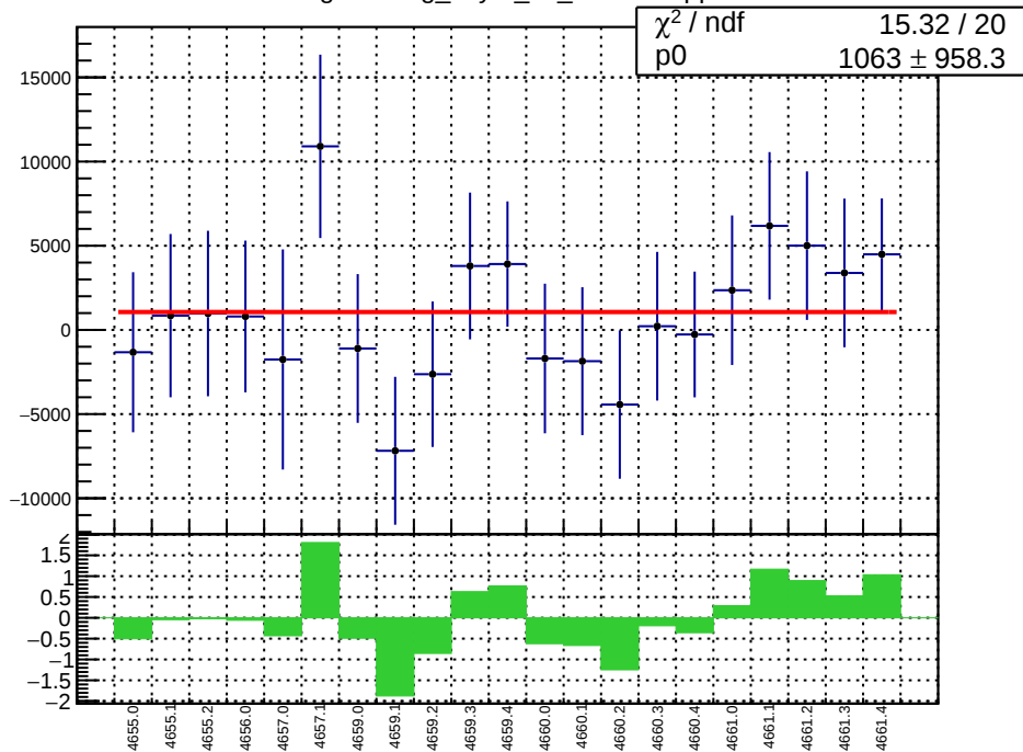
slug72B: reg_asym_atl_dd.mean/ppb
