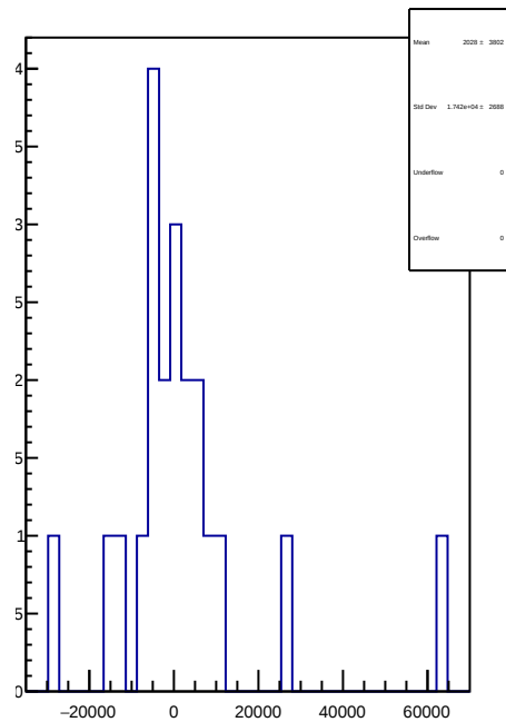
slug72B: 1D Corr asym_at2_dd.mean/ppb-reg_asym_at2_dd.mean/ppb
