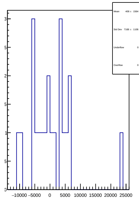
slug72B: 1D Corr asym_right_avg.mean/ppb-reg_asym_right_avg.mean/ppb
