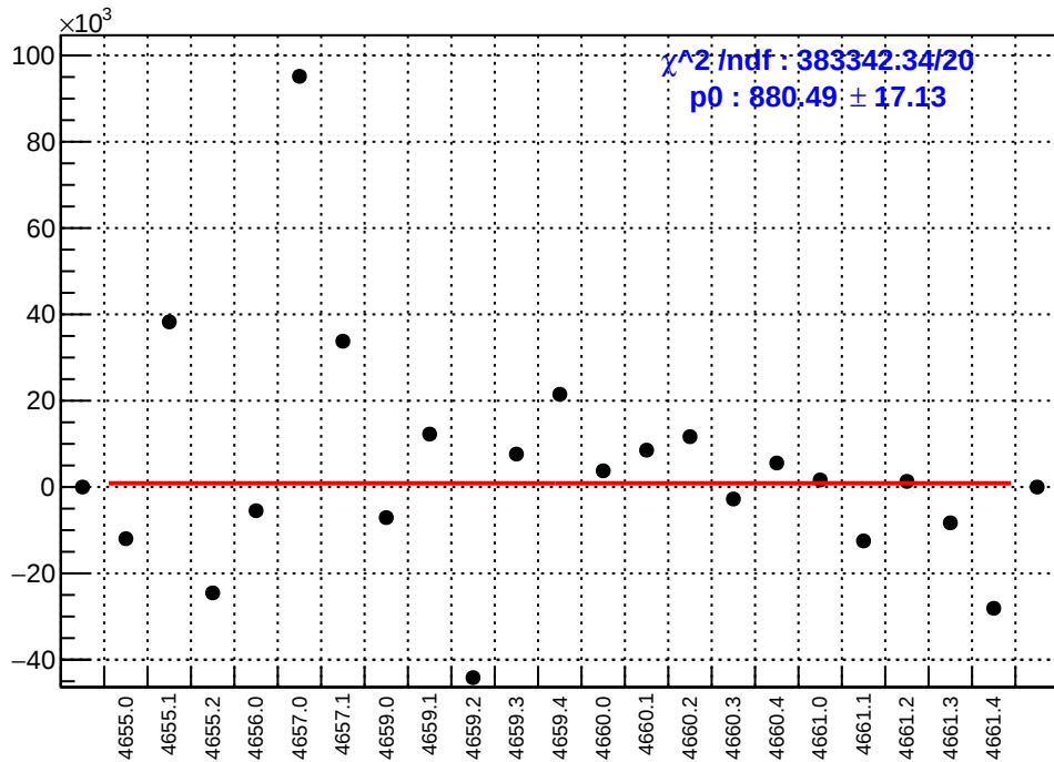
slug72B: asym_sam8.mean/ppb-reg_asym_sam8.mean/ppb
