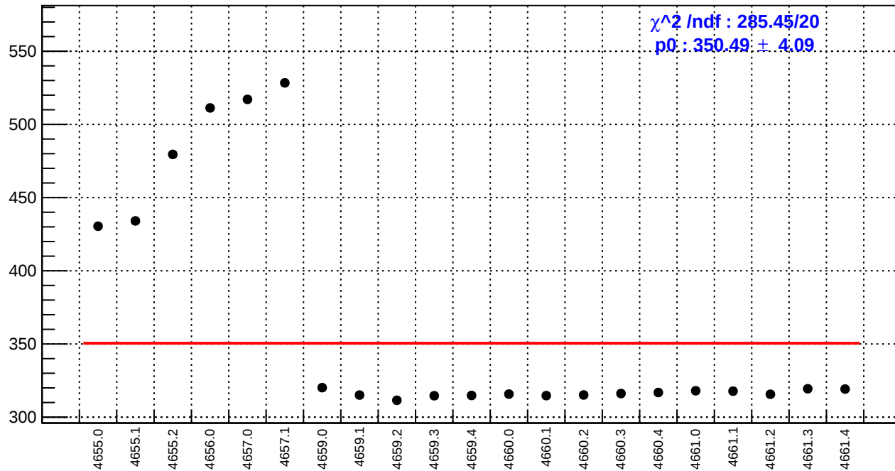
slug72B: reg_asym_atr_dd.rms/ppm
