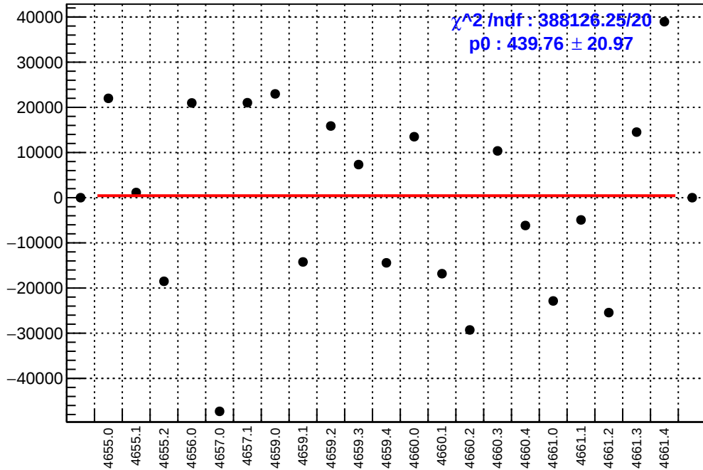
slug72B: asym_atr_dd.mean/ppb-reg_asym_atr_dd.mean/ppb
