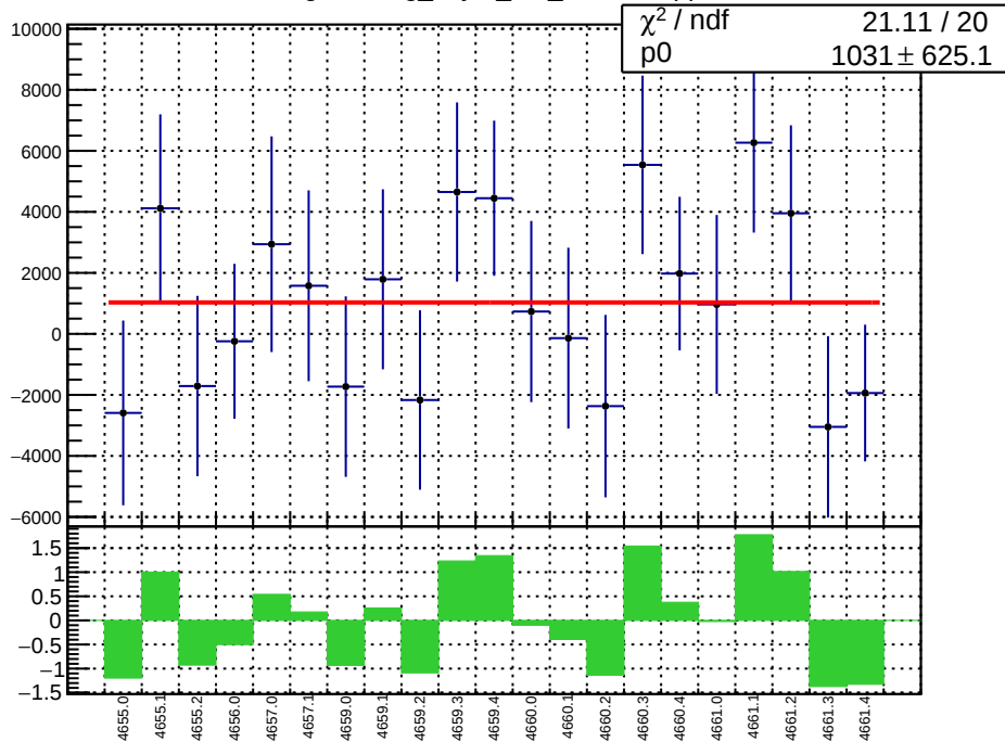
slug72B: reg_asym_at2_dd.mean/ppb
