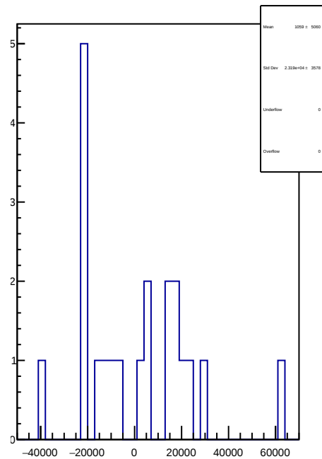
slug72B: 1D Corr asym_atl1r2_avg.mean/ppb-reg_asym_atl1r2_avg.mean/ppb
