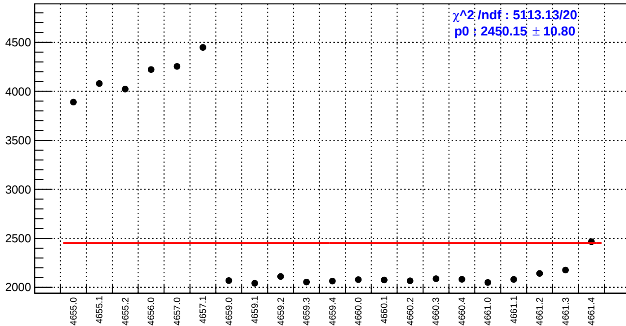
slug72B: diff_bpm4aX.rms/nm
