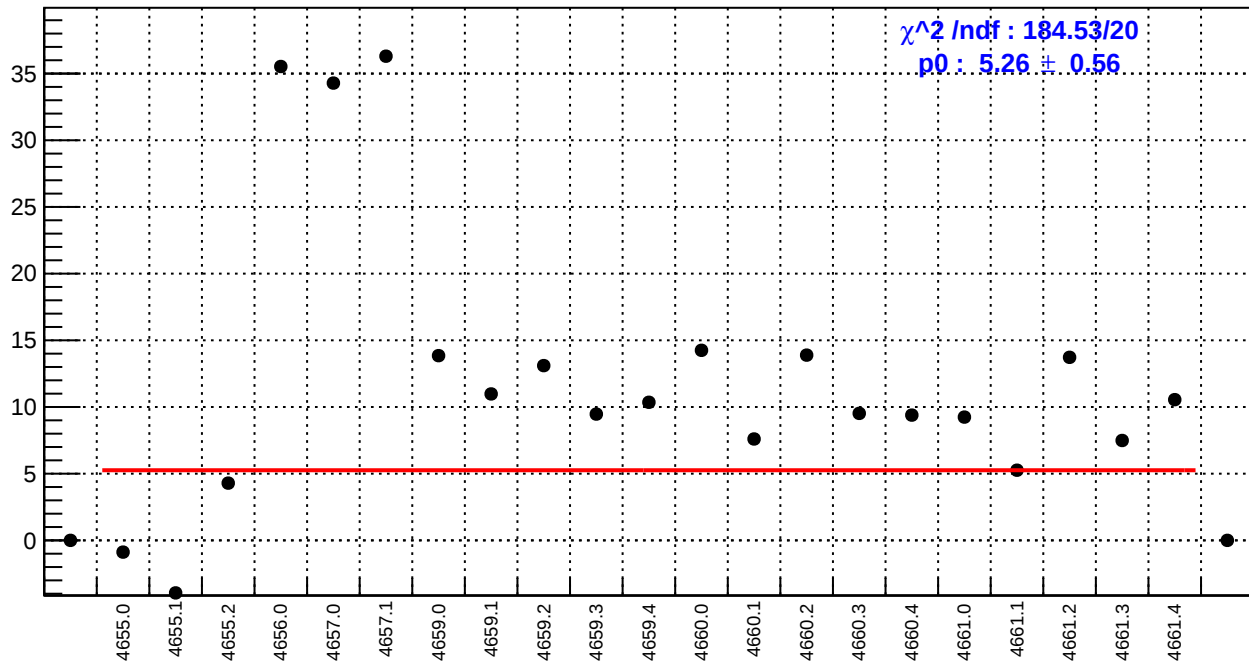
slug72B: dsr_bpm4aY/(ppb/nm)
