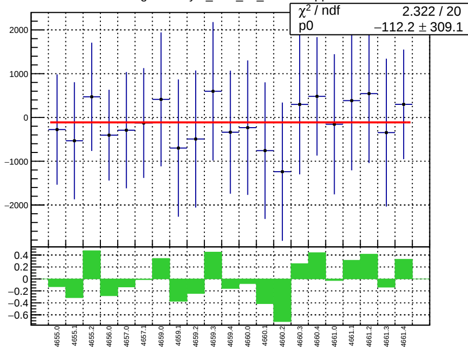
slug72B: asym_bcm_an_us.mean/ppb
