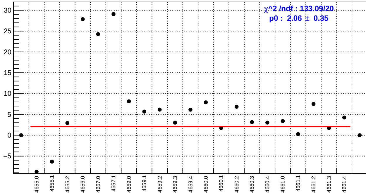
slug72B: ds_avg_bpm4aY/(ppb/nm)
