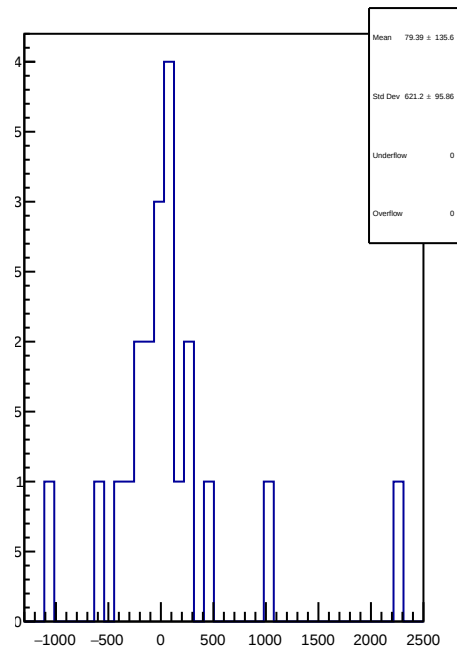
slug72B: 1D Corr asym_right_dd.mean/ppb-reg_asym_right_dd.mean/ppb
