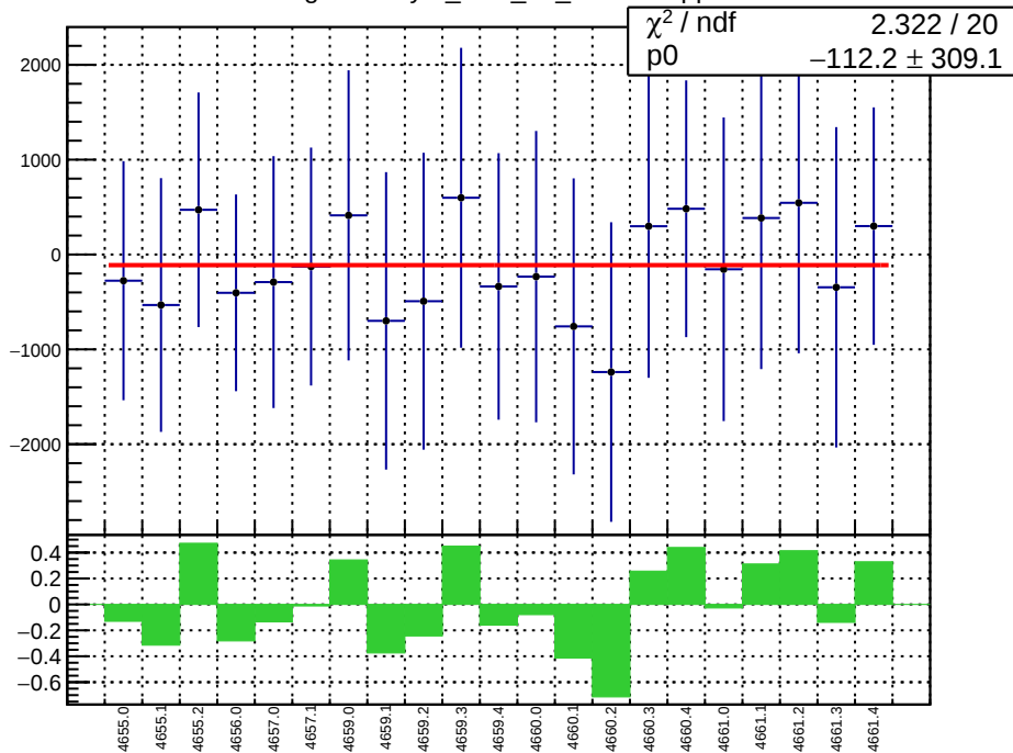
slug72B: asym_bcm_an_us.mean/ppb
