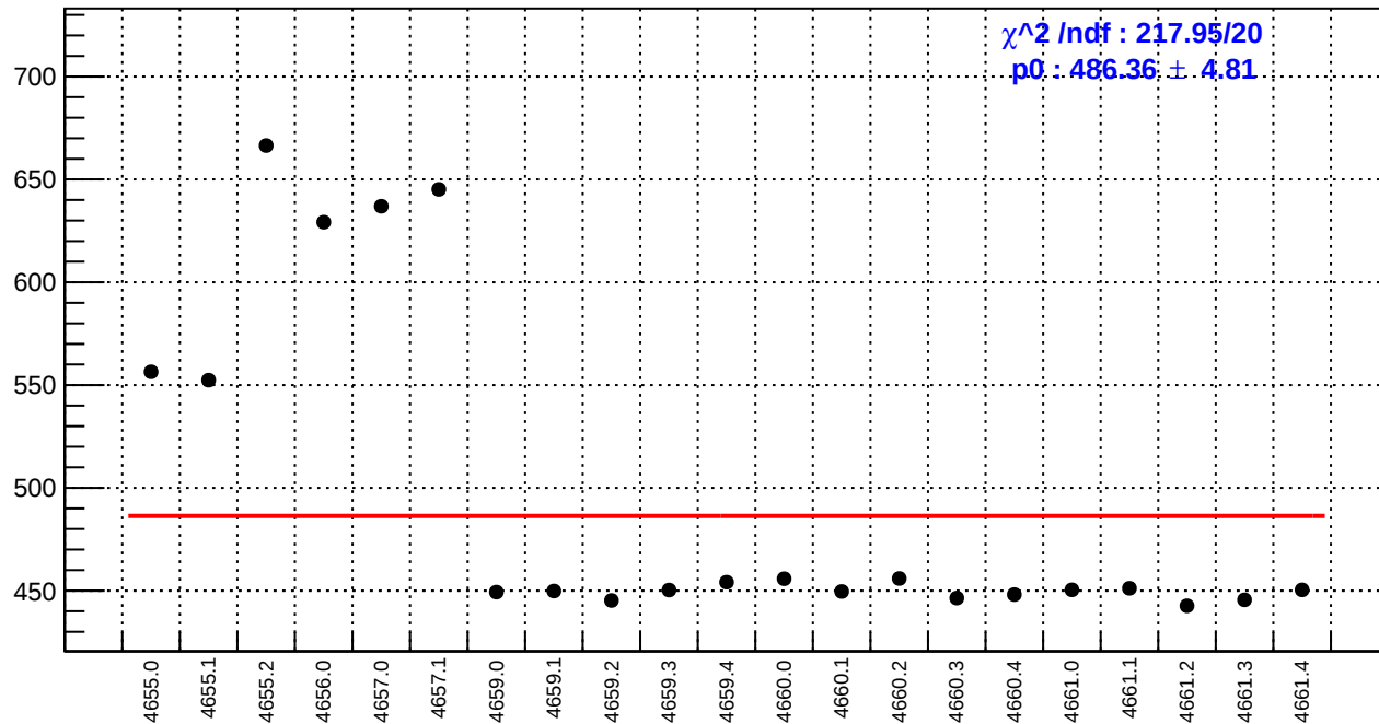
slug72B: reg_asym_atl_avg.rms/ppm
