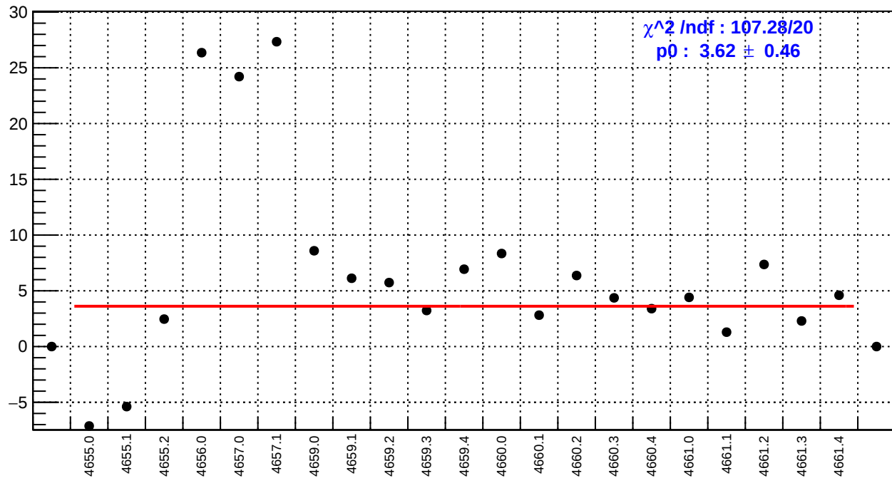
slug72B: us_avg_bpm4aY/(ppb/nm)
