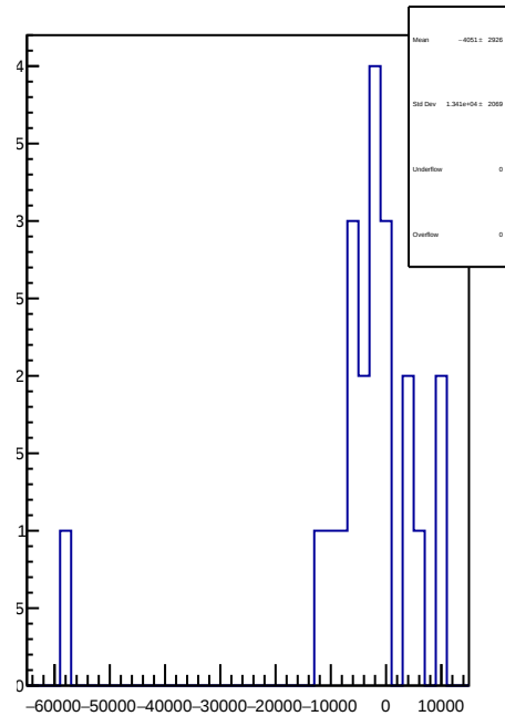
slug72B: 1D Corr asym_sam5.mean/ppb-reg_asym_sam5.mean/ppb
