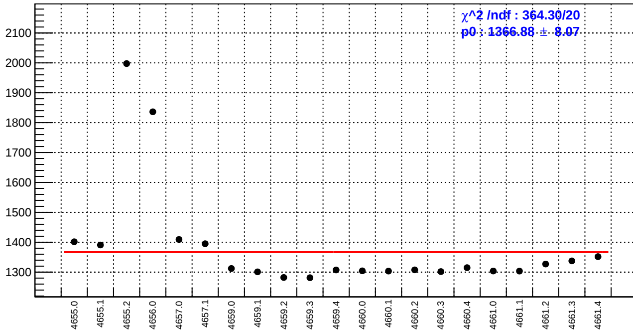
slug72B: reg_asym_sam4.rms/ppm
