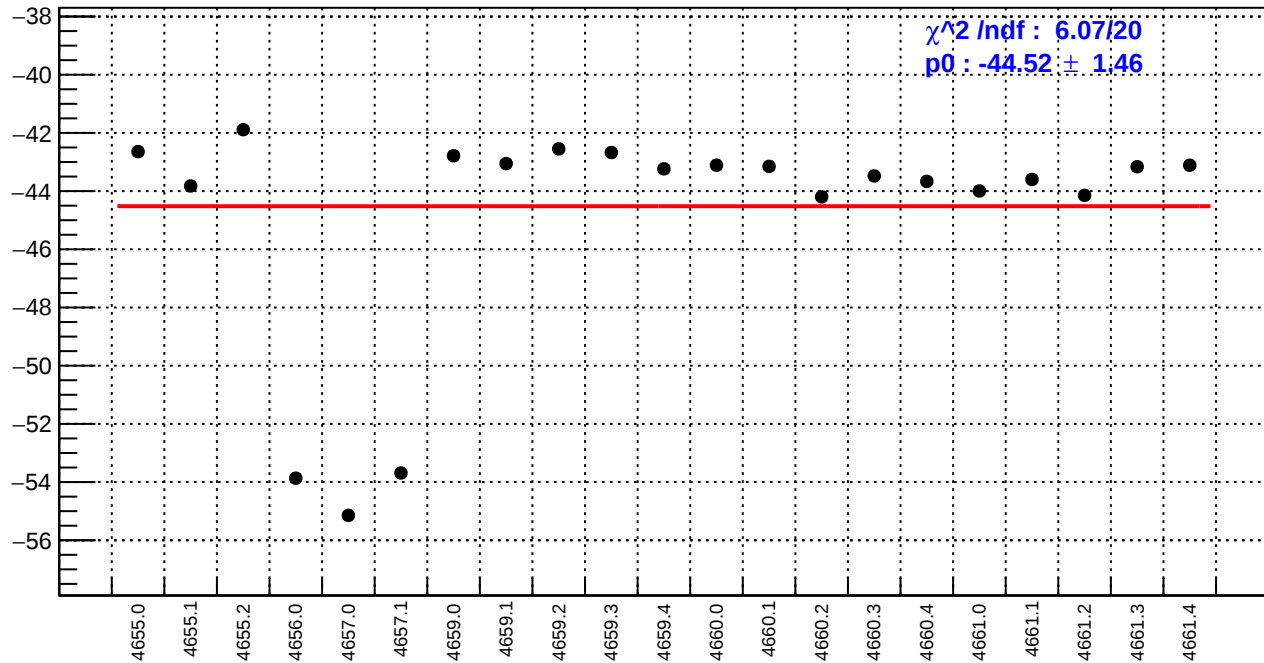
slug72B: left_avg_bpm12X/(ppb/nm)
