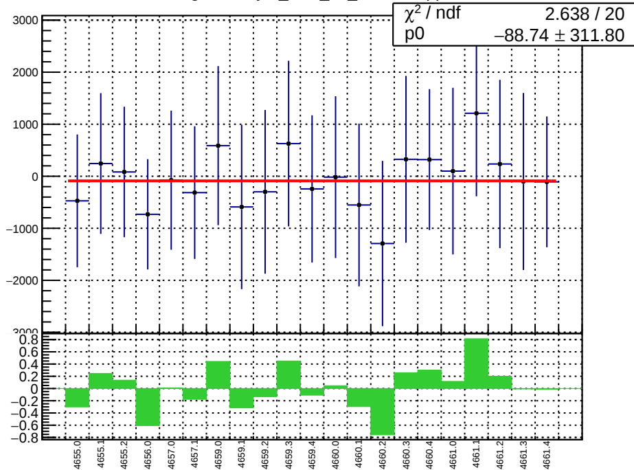
slug72B: asym_bcm_an_ds.mean/ppb
