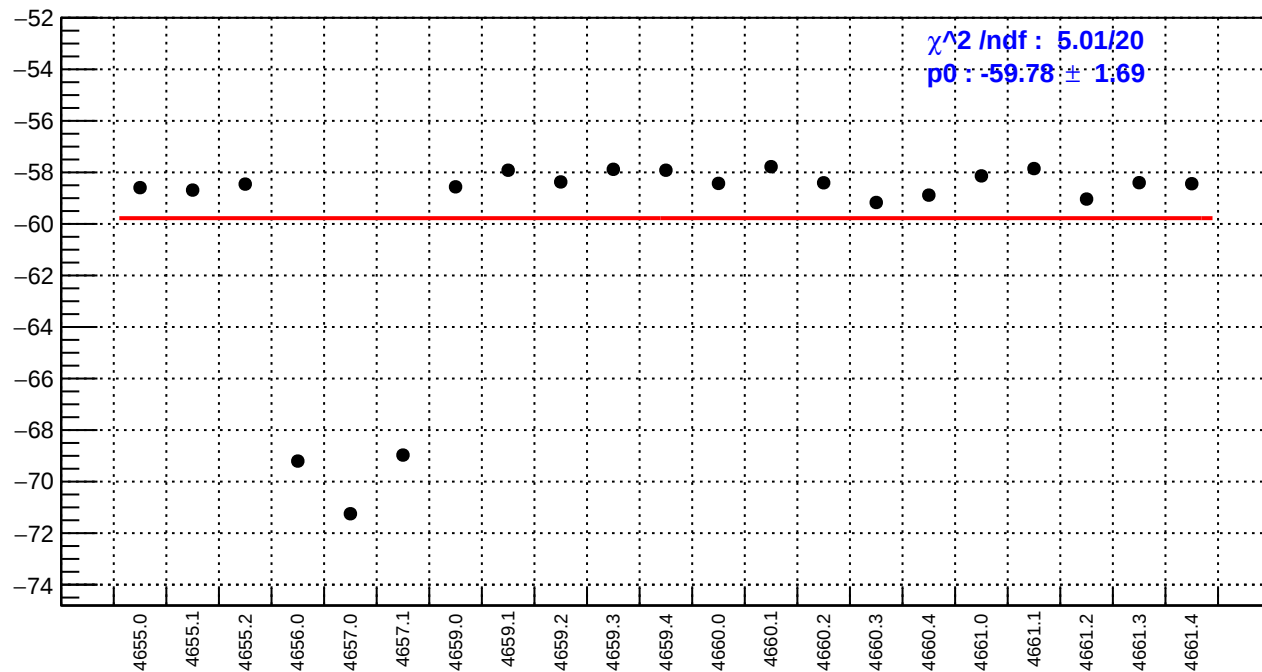
slug72B: dsr_bpm12X/(ppb/nm)
