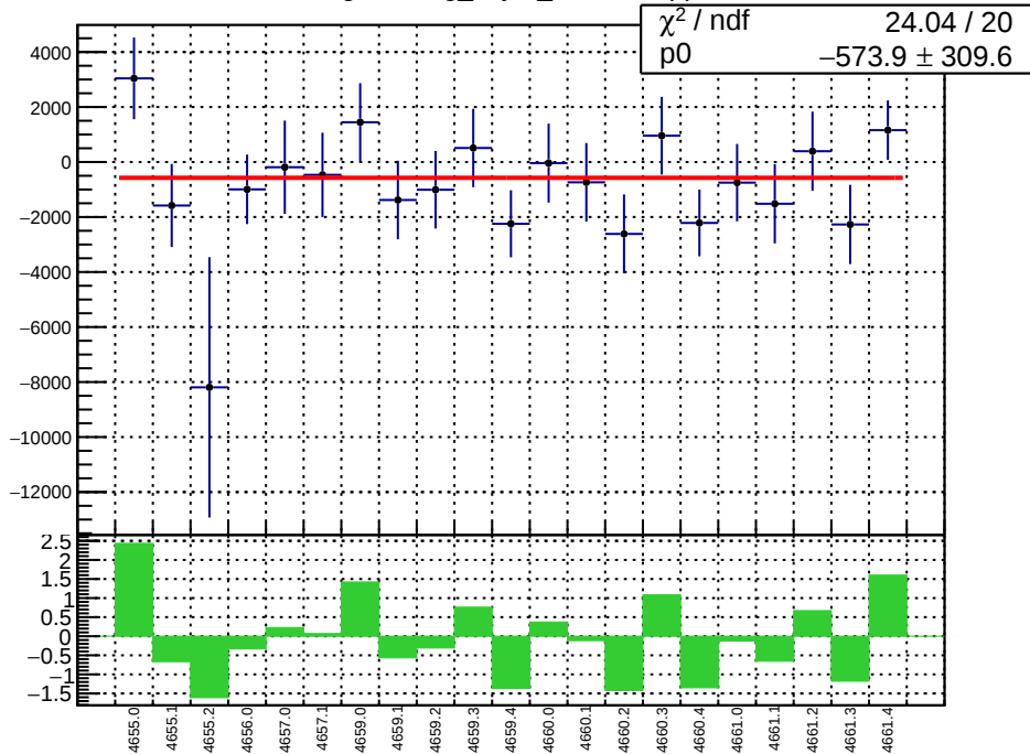
slug72B: reg_asym_usl.mean/ppb
