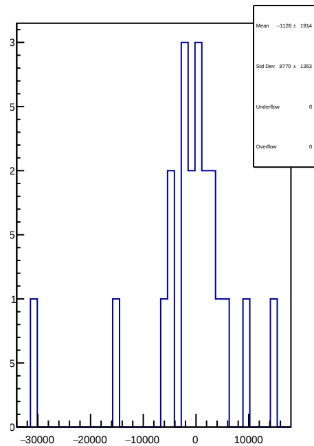
slug72B: 1D Corr asym_usl.mean/ppb-reg_asym_usl.mean/ppb
