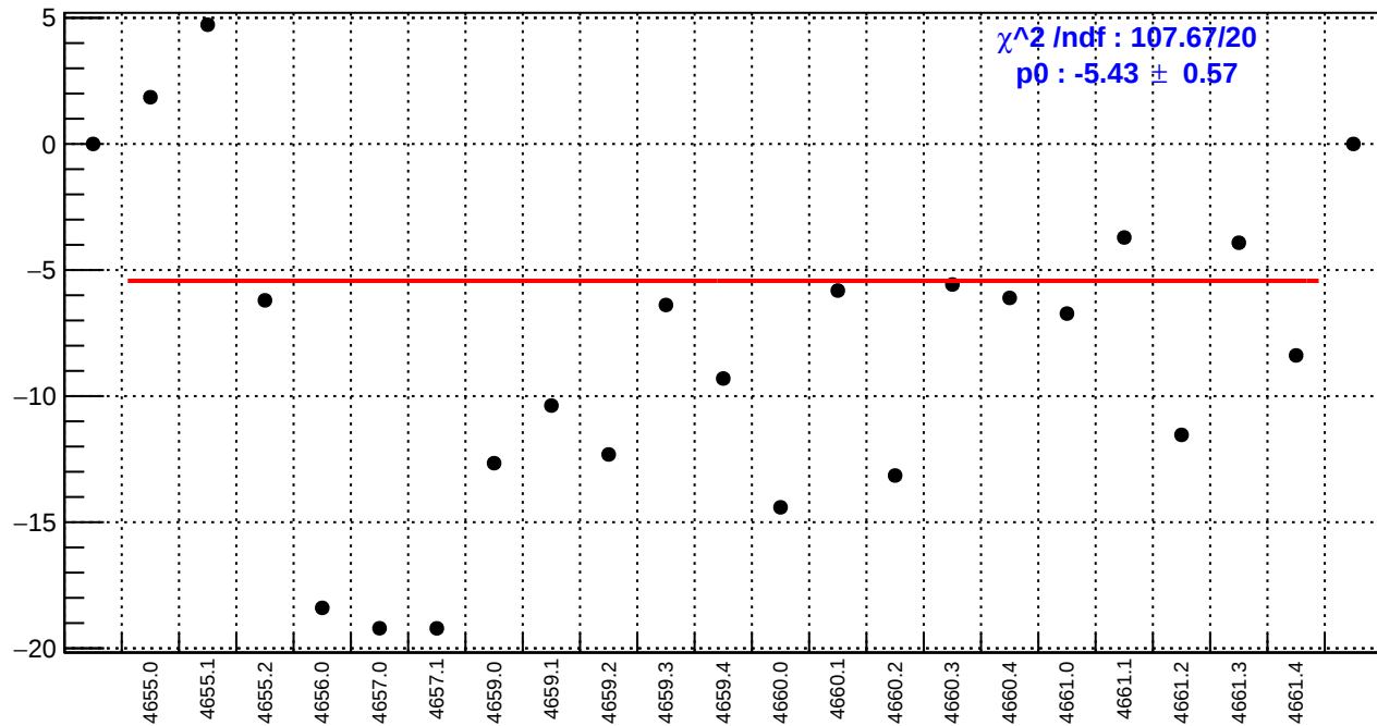
slug72B: usr_bpm4eY/(ppb/nm)
