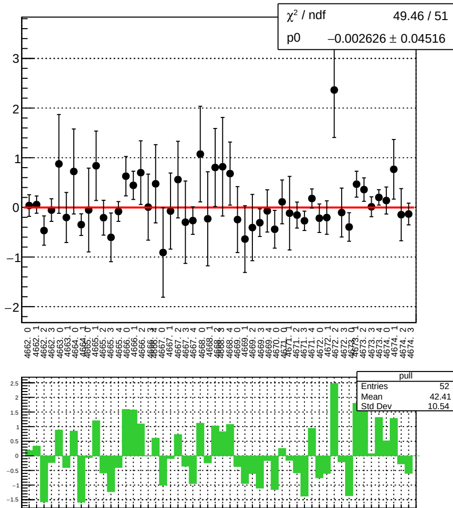
reg_bcm_an_us_ds_dd_diff_bpm4aX_slope vs run
