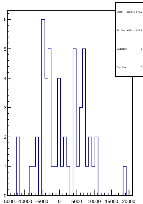
slug73: 1D Corr asym_dsl.mean/ppb-reg_asym_dsl.mean/ppb
