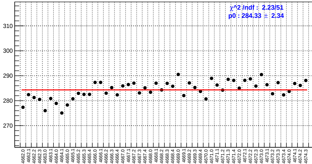
slug73: reg_asym_at2_dd.rms/ppm
