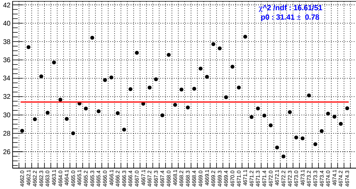
slug73: left_avg_bpm4aX/(ppb/nm)
