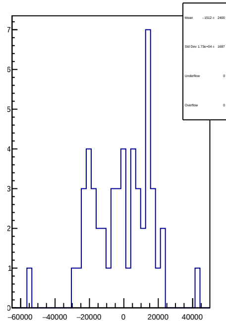
slug73: 1D Corr asym_atl_dd.mean/ppb-reg_asym_atl_dd.mean/ppb
