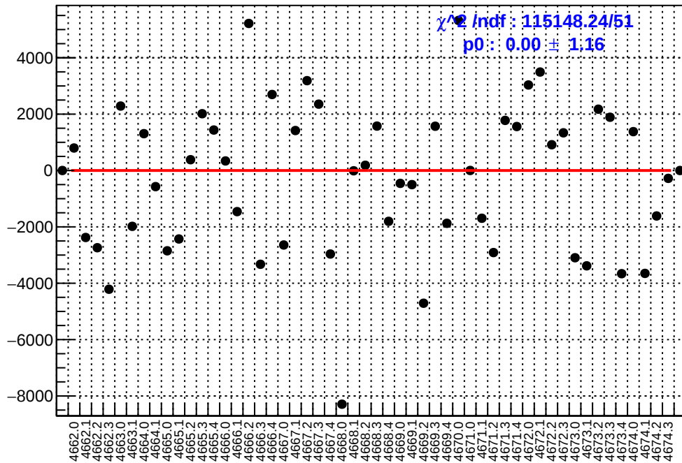
slug73: asym_at1_avg.mean/ppb-reg_asym_at1_avg.mean/ppb
