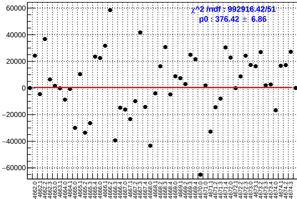
slug73: asym_atr_dd.mean/ppb-reg_asym_atr_dd.mean/ppb
