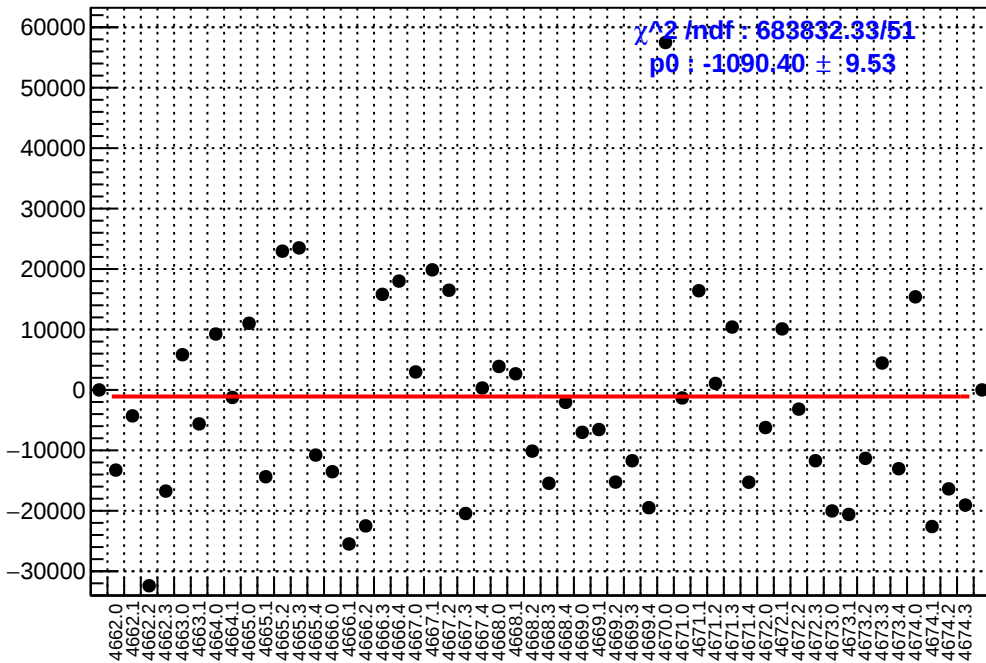
slug73: asym_atl1.mean/ppb-reg_asym_atl1.mean/ppb
