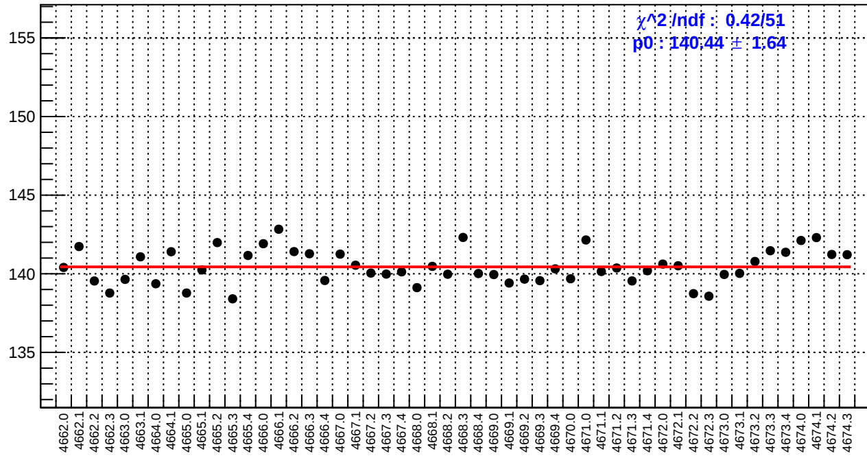
slug73: reg_asym_dsl.rms/ppm
