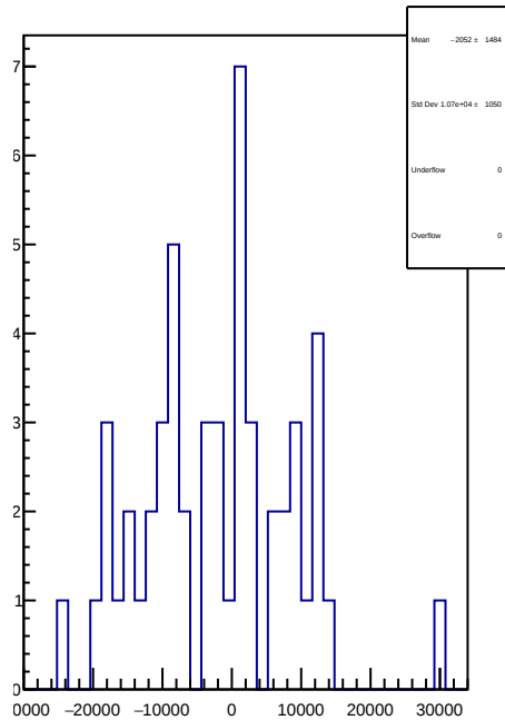
slug73: 1D Corr asym at2 dd.mean/ppb-reg asym at2 dd.mean/ppb
