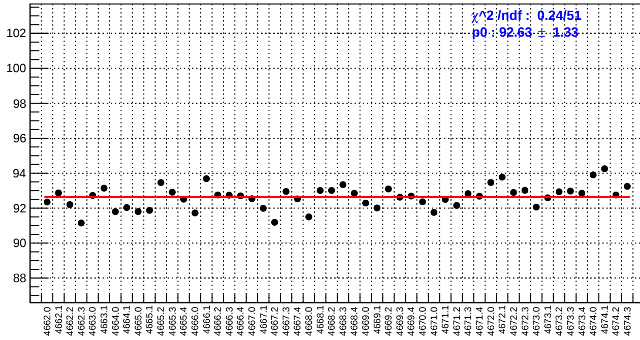
slug73: reg_asym_us_dd.rms/ppm
