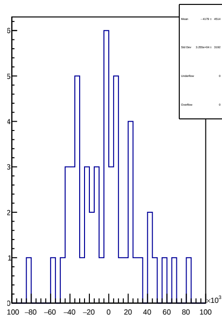
slug73: 1D Corr asym_atr2.mean/ppb-reg_asym_atr2.mean/ppb
