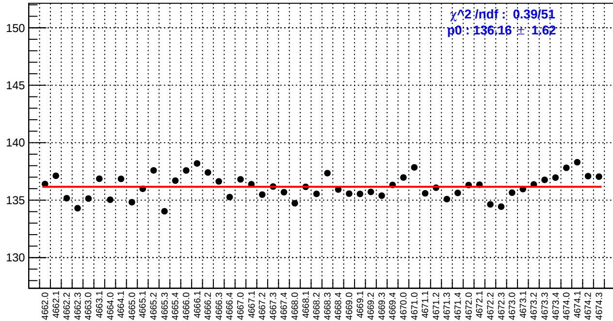
slug73: reg_asym_left_avg.rms/ppm
