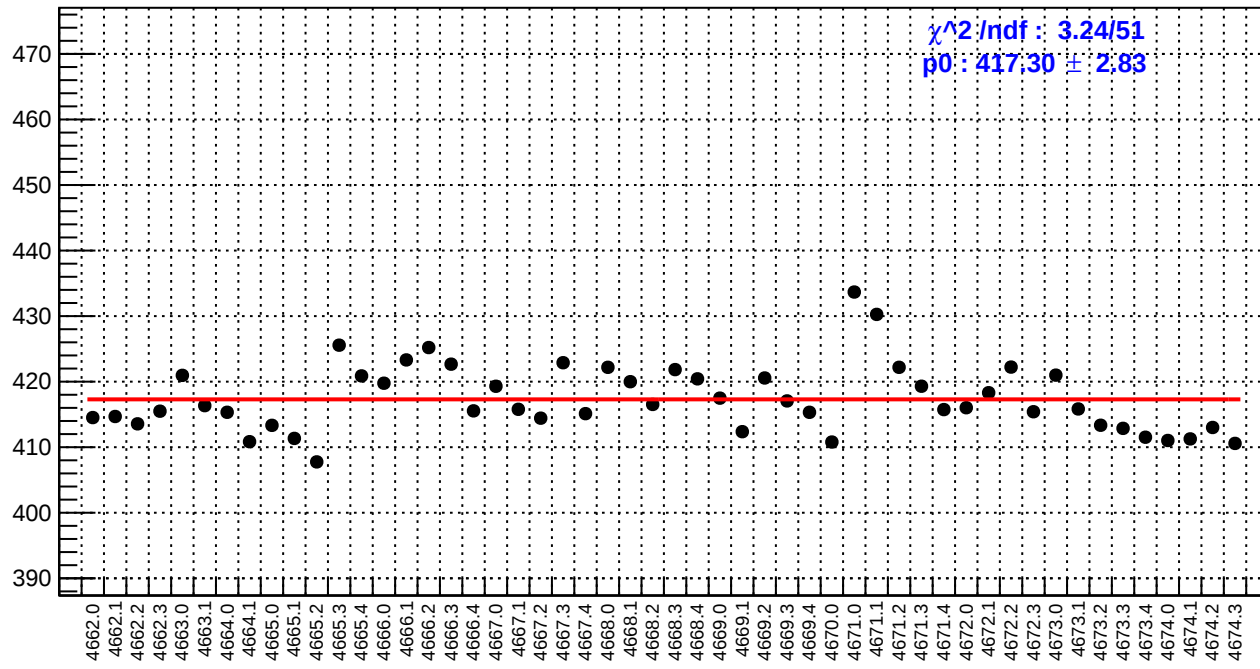
slug73: reg_asym_atl1r2_avg.rms/ppm
