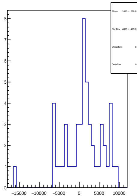
slug73: 1D Corr asym_us_dd.mean/ppb-reg_asym_us_dd.mean/ppb
