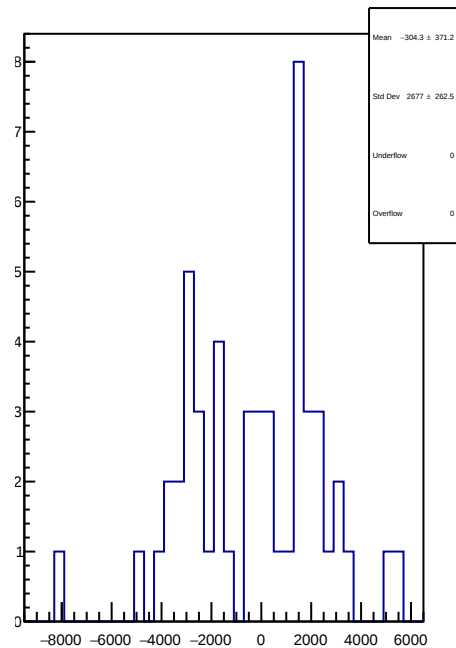
slug73: 1D Corr asym_at1_avg.mean/ppb-reg_asym_at1_avg.mean/ppb
