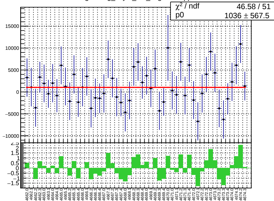
slug73: reg_asym_at1_avg.mean/ppb
