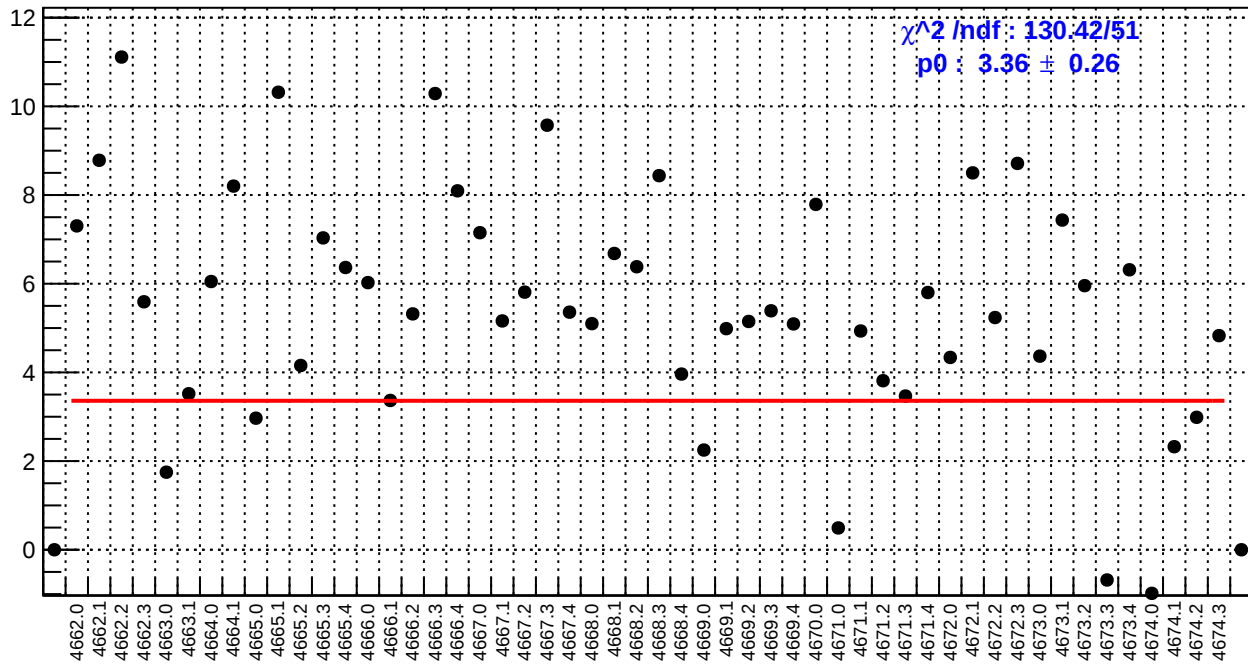
slug73: left_avg_bpm4eY/(ppb/nm)
