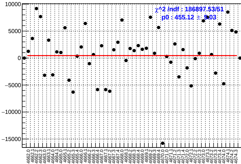
slug73: asym_ds_dd.mean/ppb-reg_asym_ds_dd.mean/ppb
