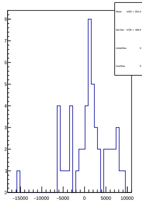
slug73: 1D Corr asym_ds_dd.mean/ppb-reg_asym_ds_dd.mean/ppb
