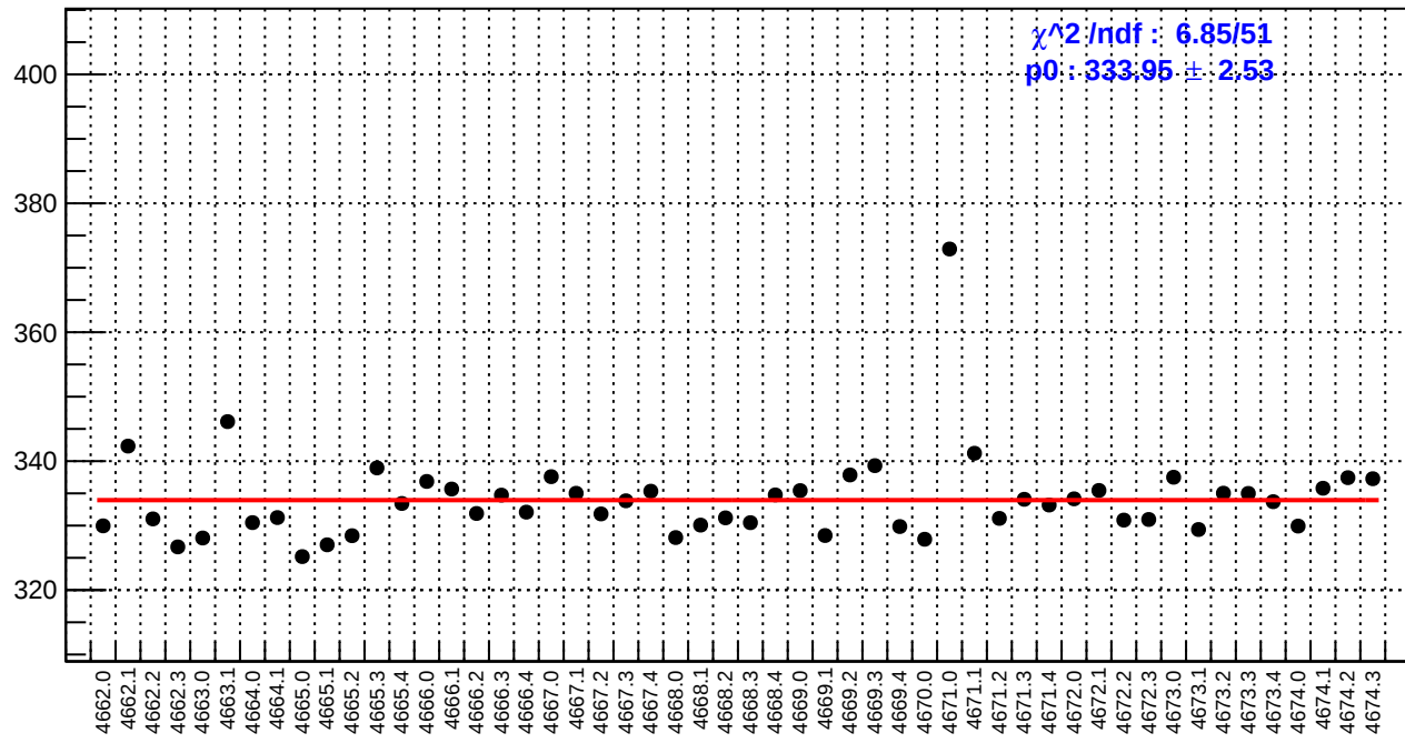
slug73: reg_asym_atr1l2_avg.rms/ppm
