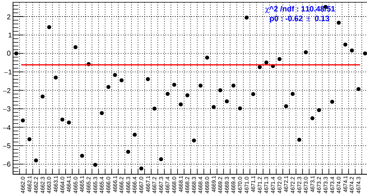
slug73: dsl_bpm4aY/(ppb/nm)
