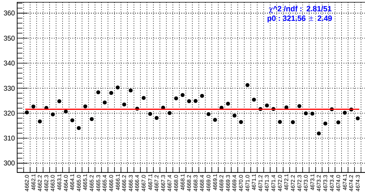
slug73: reg_asym_atr_dd.rms/ppm
