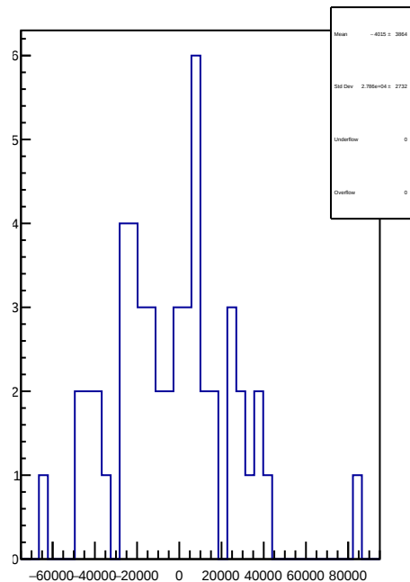
slug73: 1D Corr asym_sam6.mean/ppb-reg_asym_sam6.mean/ppb
