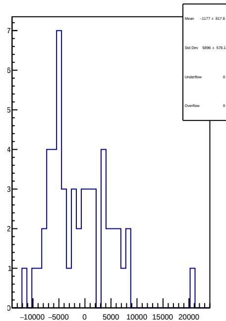
slug73: 1D Corr asym_right_avg.mean/ppb-reg_asym_right_avg.mean/ppb
