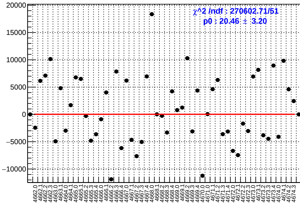
slug73: asym_left_avg.mean/ppb-reg_asym_left_avg.mean/ppb
