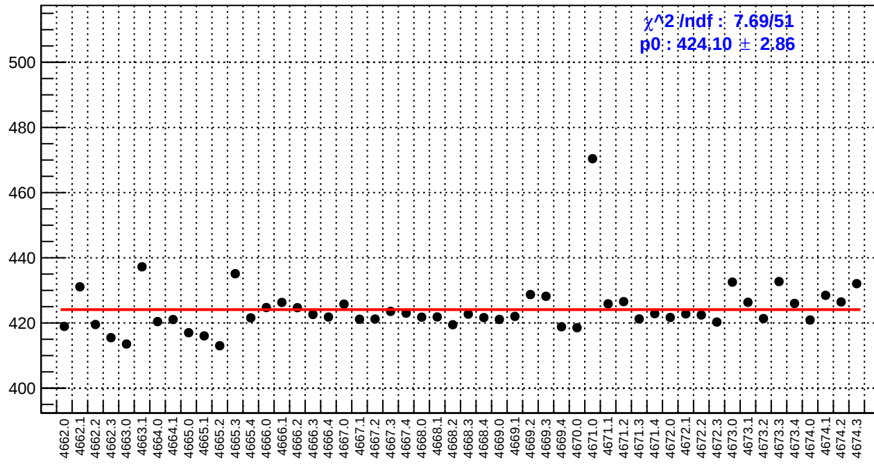
slug73: reg_asym_atl_dd.rms/ppm
