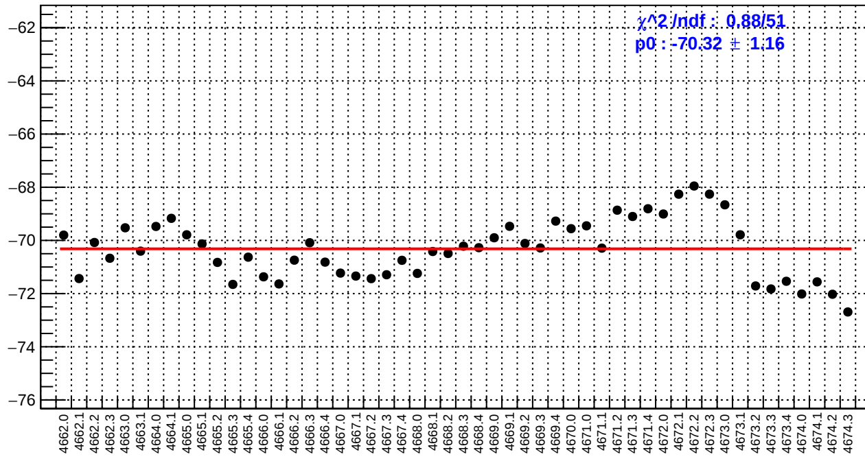
slug73: left_avg_bpm4eX/(ppb/nm)
