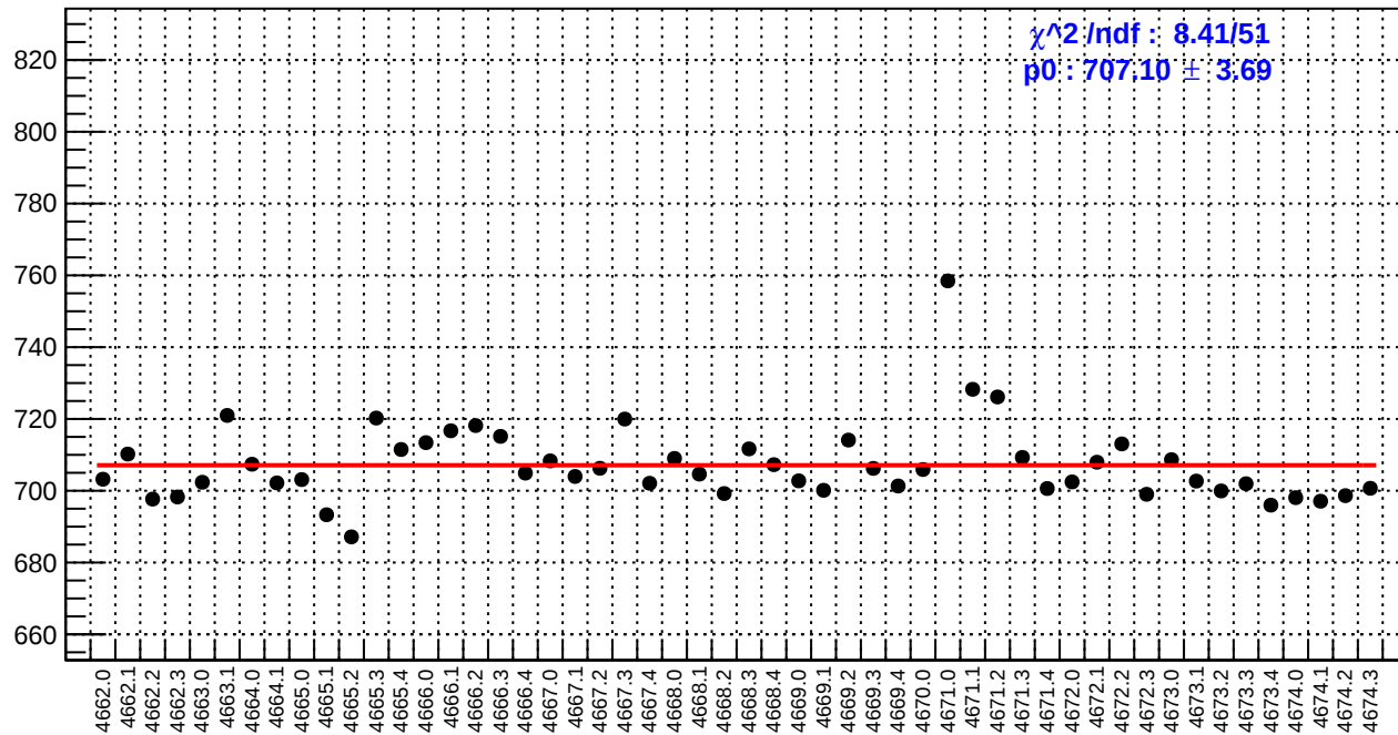
slug73: reg_asym_atl1.rms/ppm
