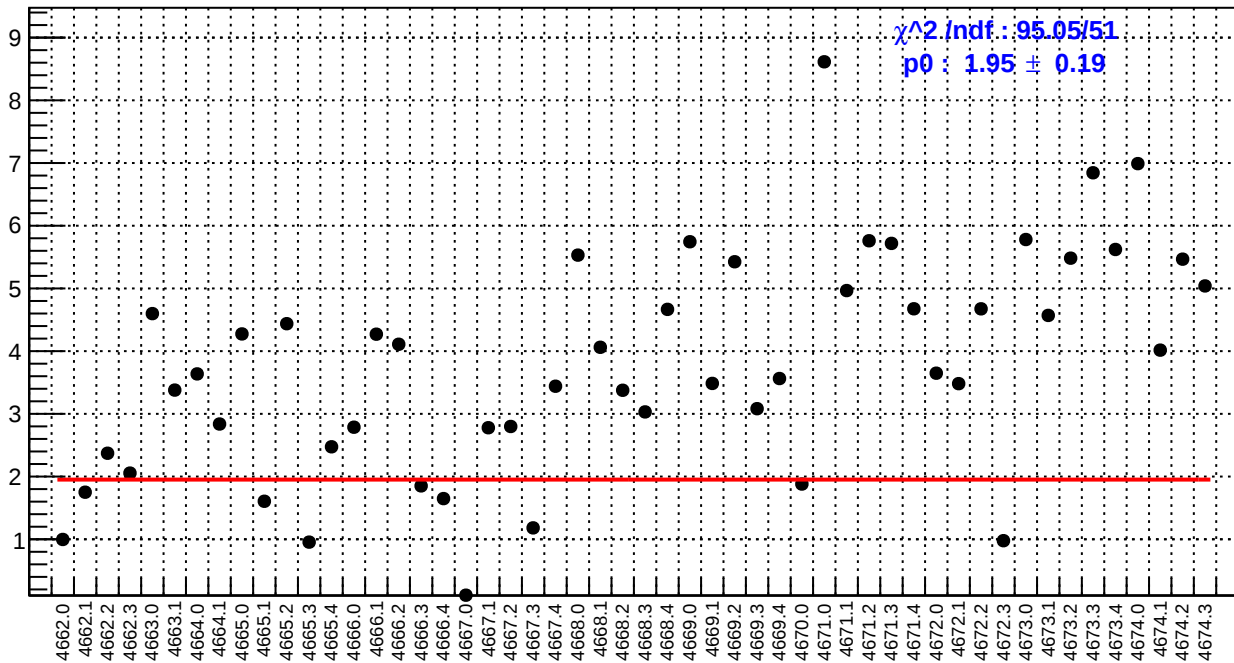
slug73: ds_avg_bpm4aY/(ppb/nm)
