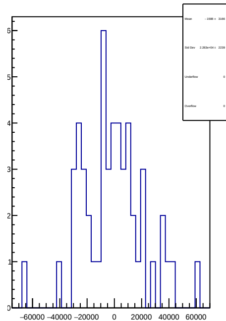
slug73: 1D Corr asym_atl_avg.mean/ppb-reg_asym_atl_avg.mean/ppb
