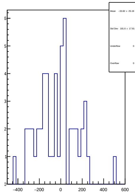
slug73: 1D Corr asym_left_dd.mean/ppb-reg_asym_left_dd.mean/ppb
