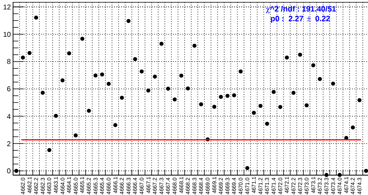
slug73: dsl_bpm4eY/(ppb/nm)
