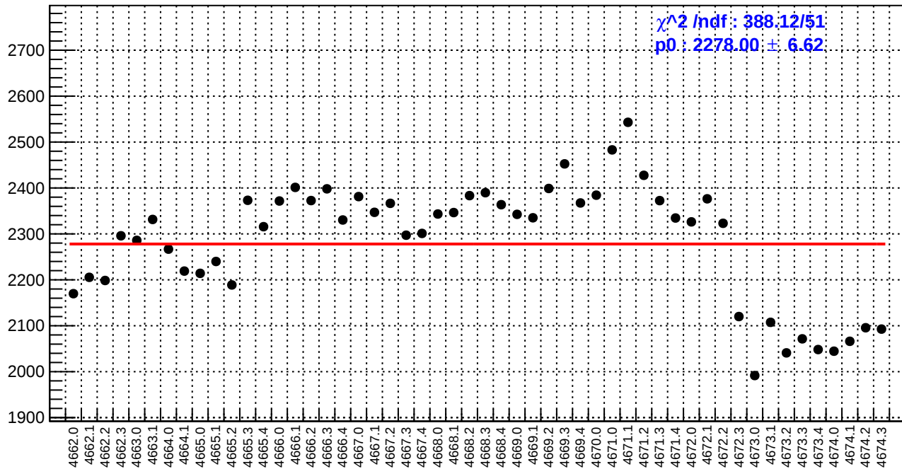
slug73: diff_bpm4eY.rms/nm
