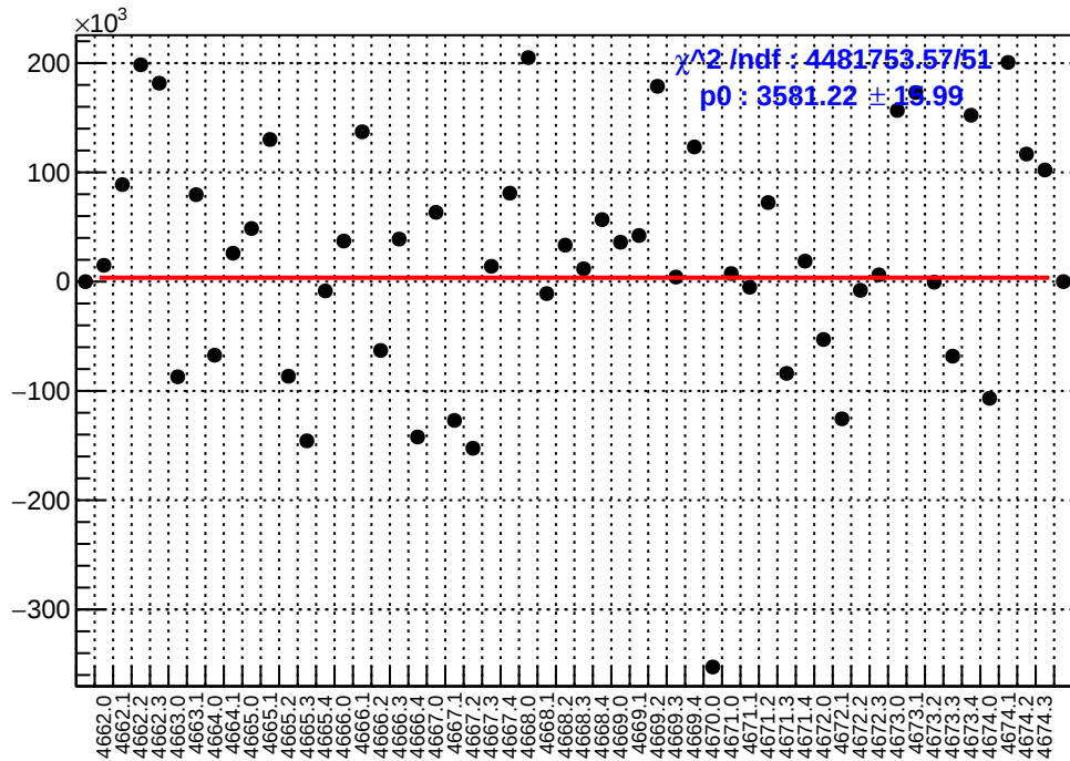
slug73: asym_sam3.mean/ppb-reg_asym_sam3.mean/ppb
