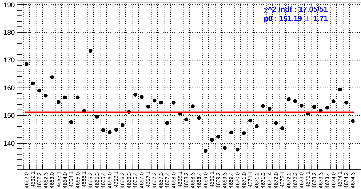
slug73: asym_bcm_an_us.rms/ppm
