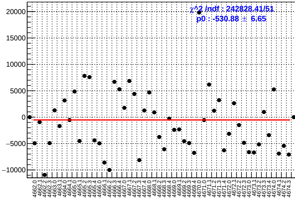
slug73: asym_dsr.mean/ppb-reg_asym_dsr.mean/ppb
