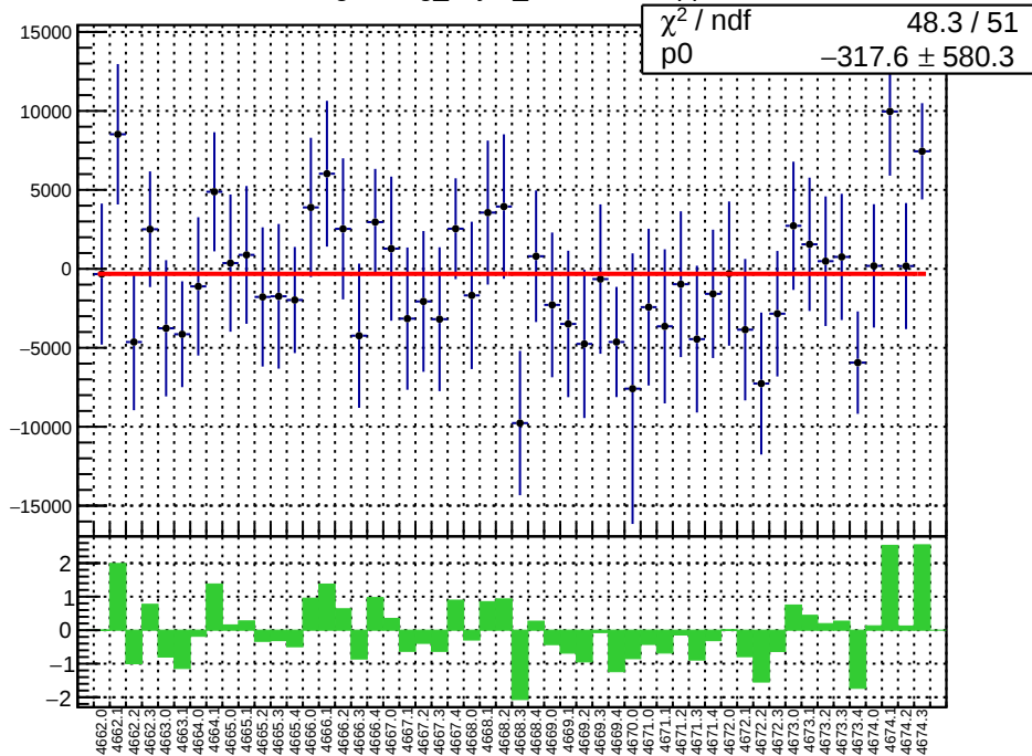
slug73: reg_asym_sam6.mean/ppb
