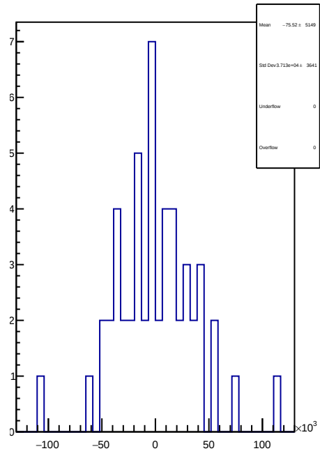
slug73: 1D Corr asym_atl2.mean/ppb-reg_asym_atl2.mean/ppb
