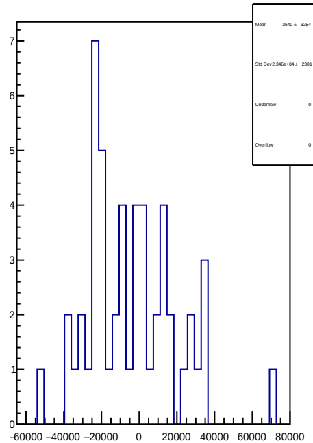
slug73: 1D Corr asym_atl1r2_avg.mean/ppb-reg_asym_atl1r2_avg.mean/ppb
