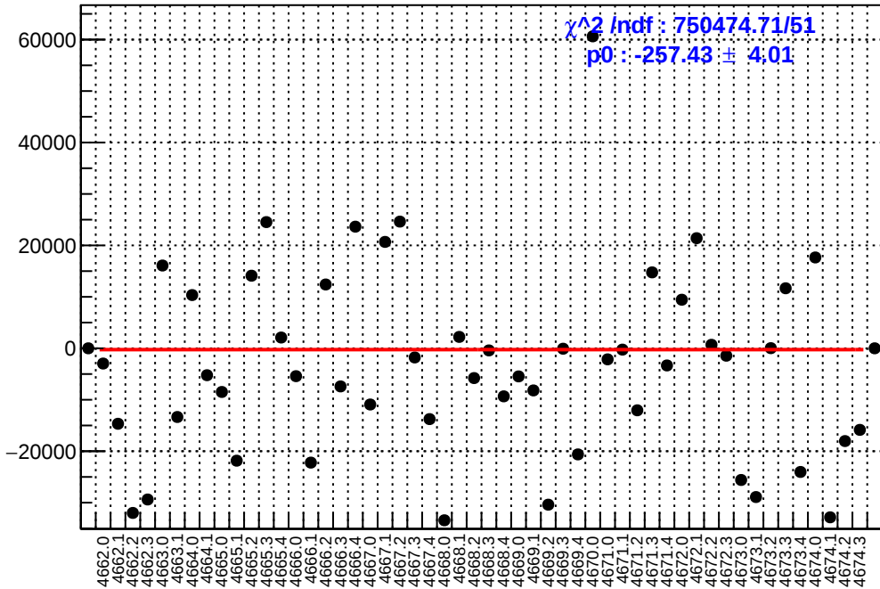
slug73: asym_sam7.mean/ppb-reg_asym_sam7.mean/ppb
