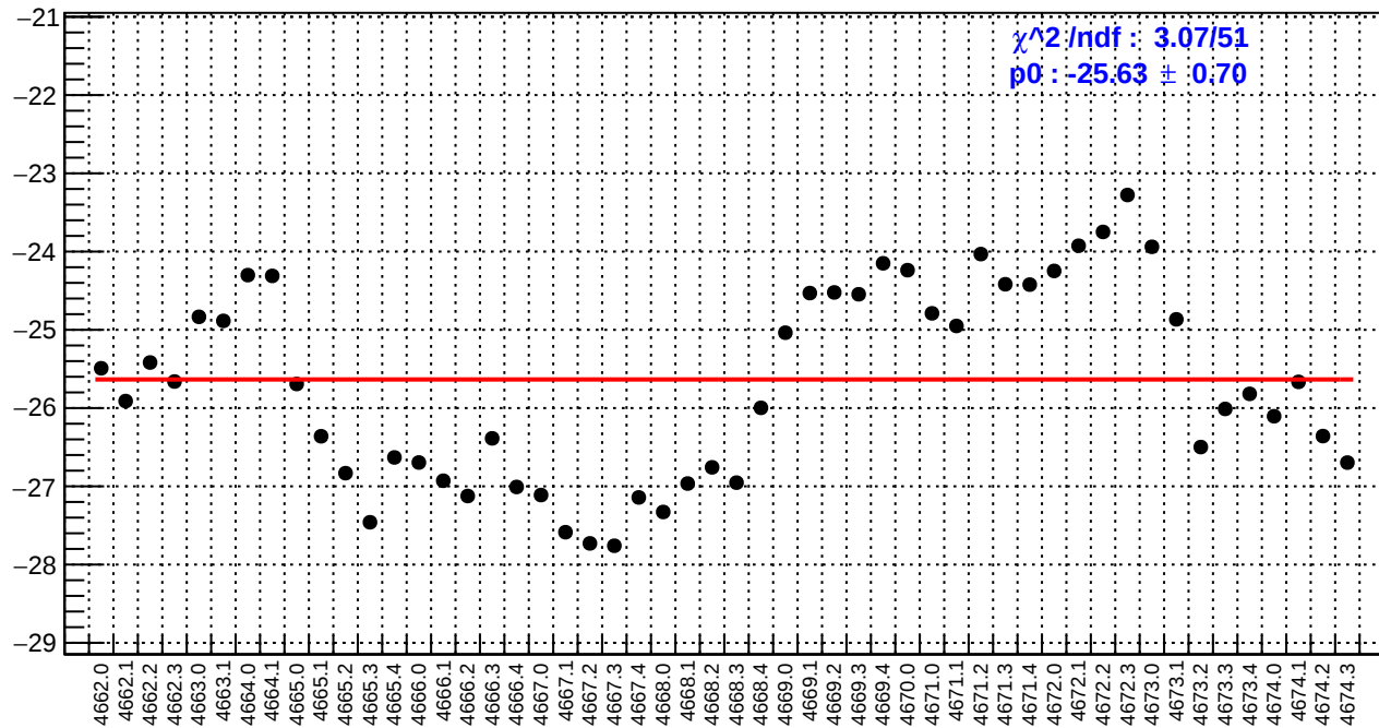
slug73: ds_avg_bpm4eX/(ppb/nm)
