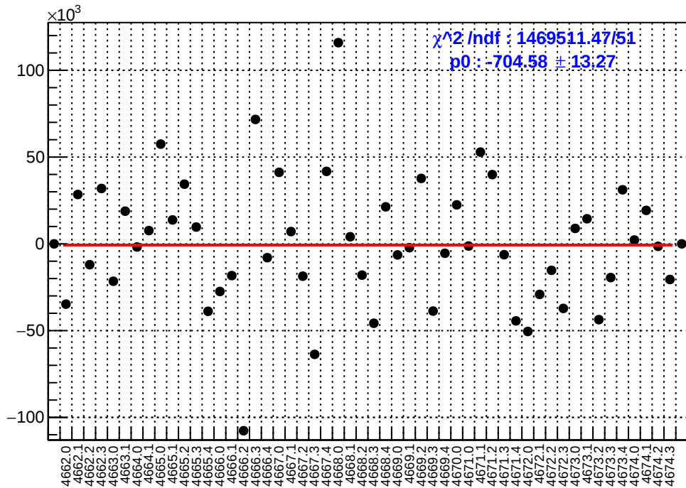
slug73: asym_atl2.mean/ppb-reg_asym_atl2.mean/ppb
