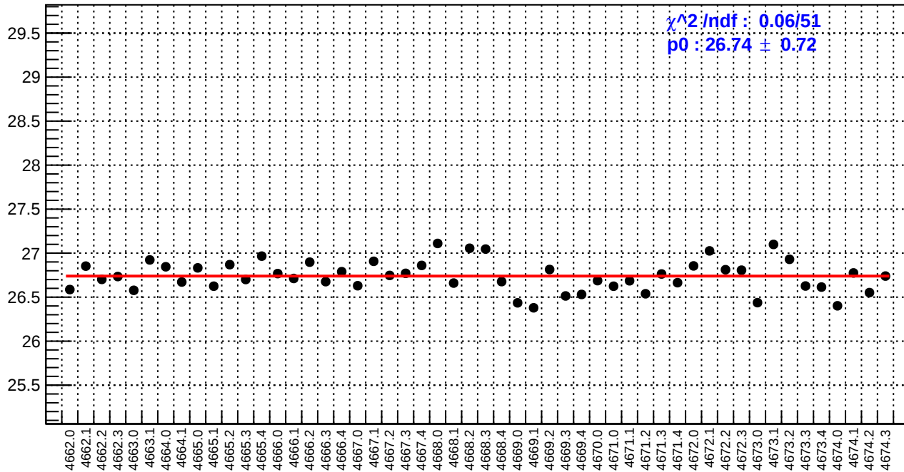
slug73: reg_asym_right_dd.rms/ppm
