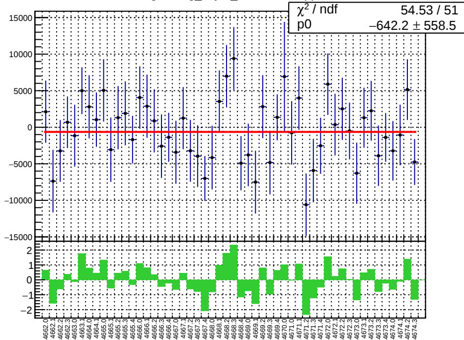
slug73: reg_asym_sam8.mean/ppb
