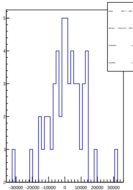
slug73: 1D Corr asym_atl1r2_dd.mean/ppb-reg_asym_atl1r2_dd.mean/ppb
