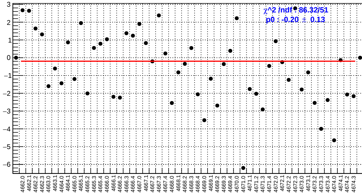
slug73: ds_avg_bpm4eY/(ppb/nm)
