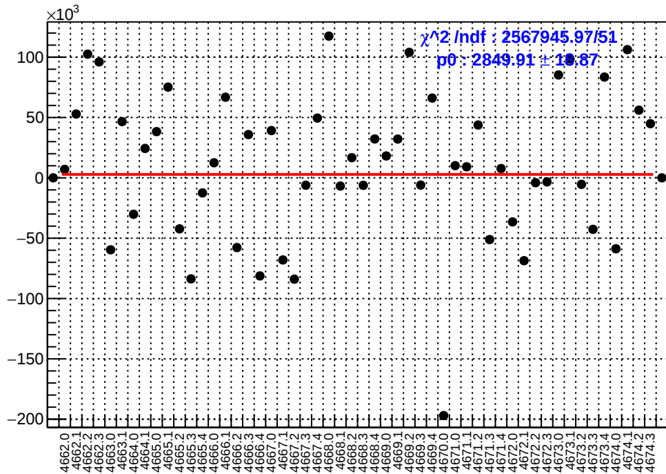
slug73: asym_sam2.mean/ppb-reg_asym_sam2.mean/ppb
