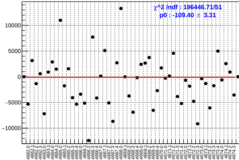
slug73: asym_sam1.mean/ppb-reg_asym_sam1.mean/ppb
