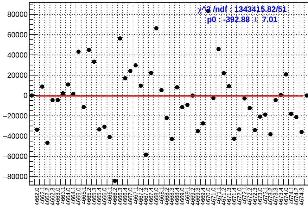
slug73: asym_atr2.mean/ppb-reg_asym_atr2.mean/ppb
