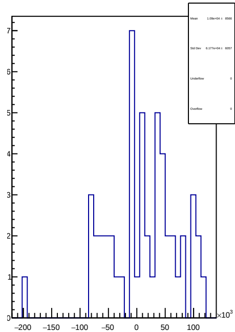
slug73: 1D Corr asym_sam2.mean/ppb-reg_asym_sam2.mean/ppb
