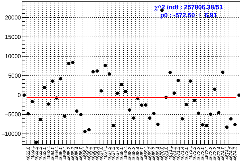
slug73: asym_usr.mean/ppb-reg_asym_usr.mean/ppb
