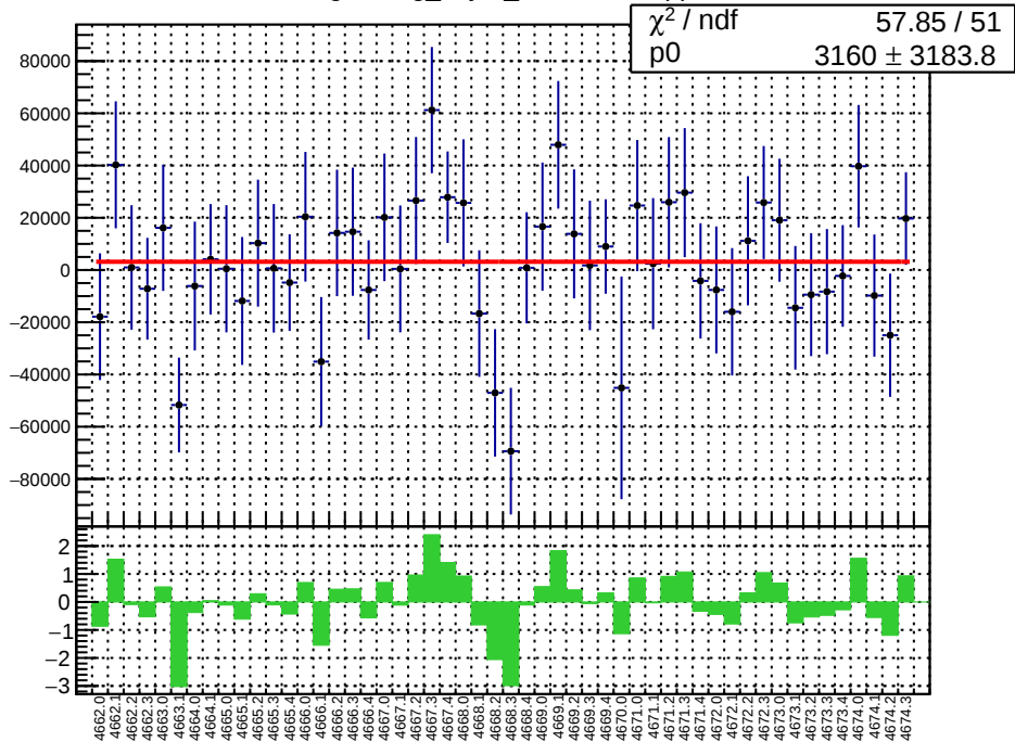
slug73: reg_asym_sam2.mean/ppb
