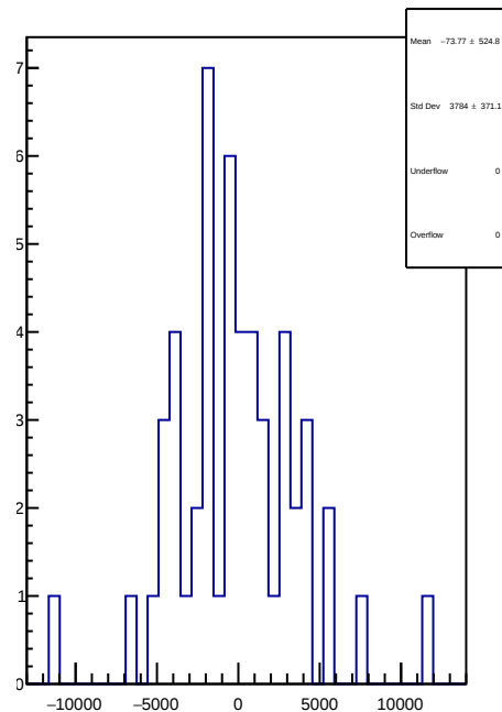
slug73: 1D Corr asym_ds_avg.mean/ppb-reg_asym_ds_avg.mean/ppb
