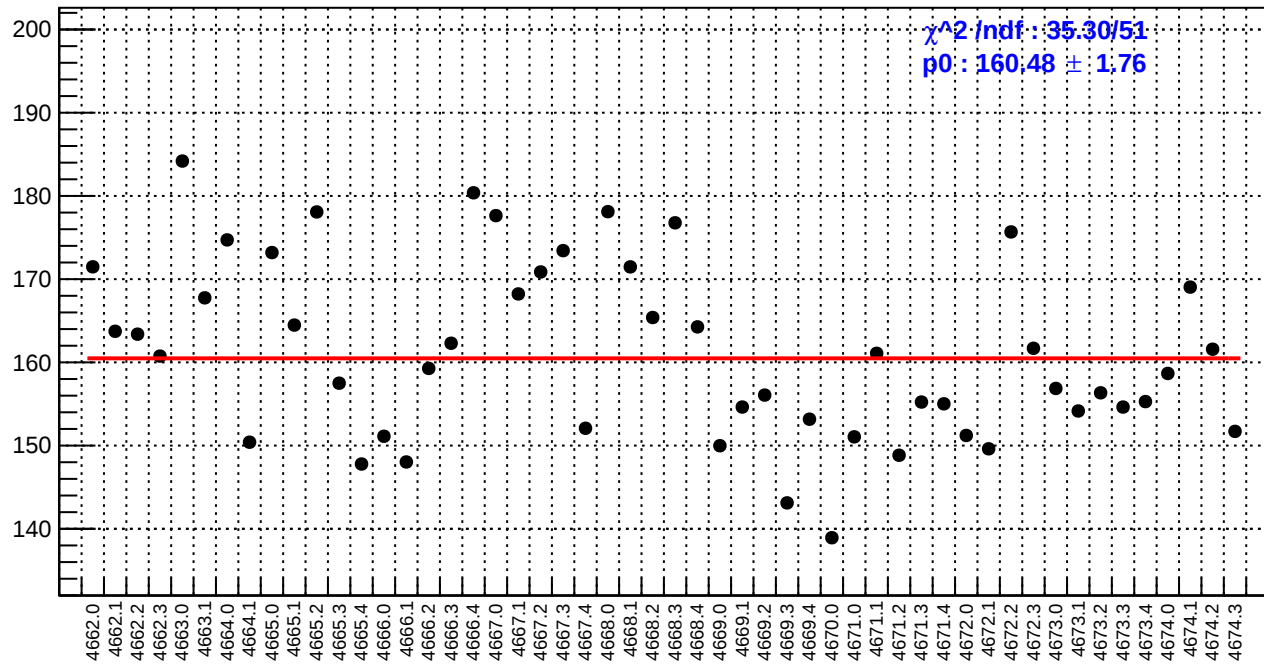
slug73: asym_bcm_an_ds3.rms/ppm
