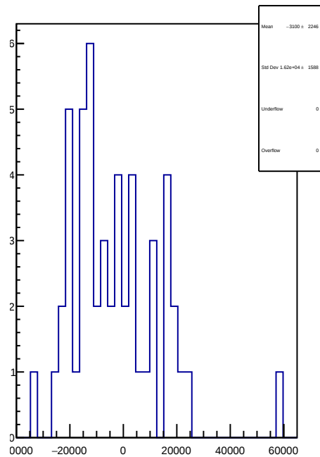
slug73: 1D Corr asym_atl1.mean/ppb-reg_asym_atl1.mean/ppb
