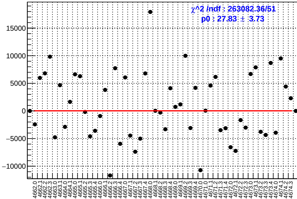
slug73: asym_usl.mean/ppb-reg_asym_usl.mean/ppb
