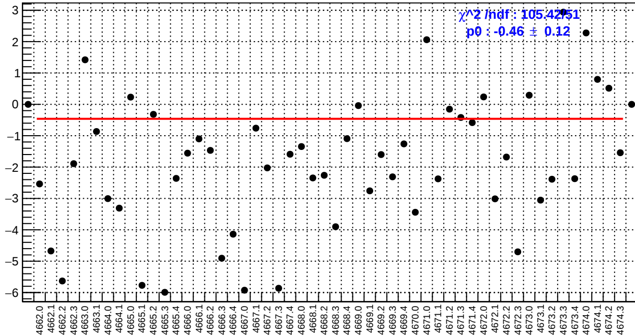
slug73: left_avg_bpm4aY/(ppb/nm)
