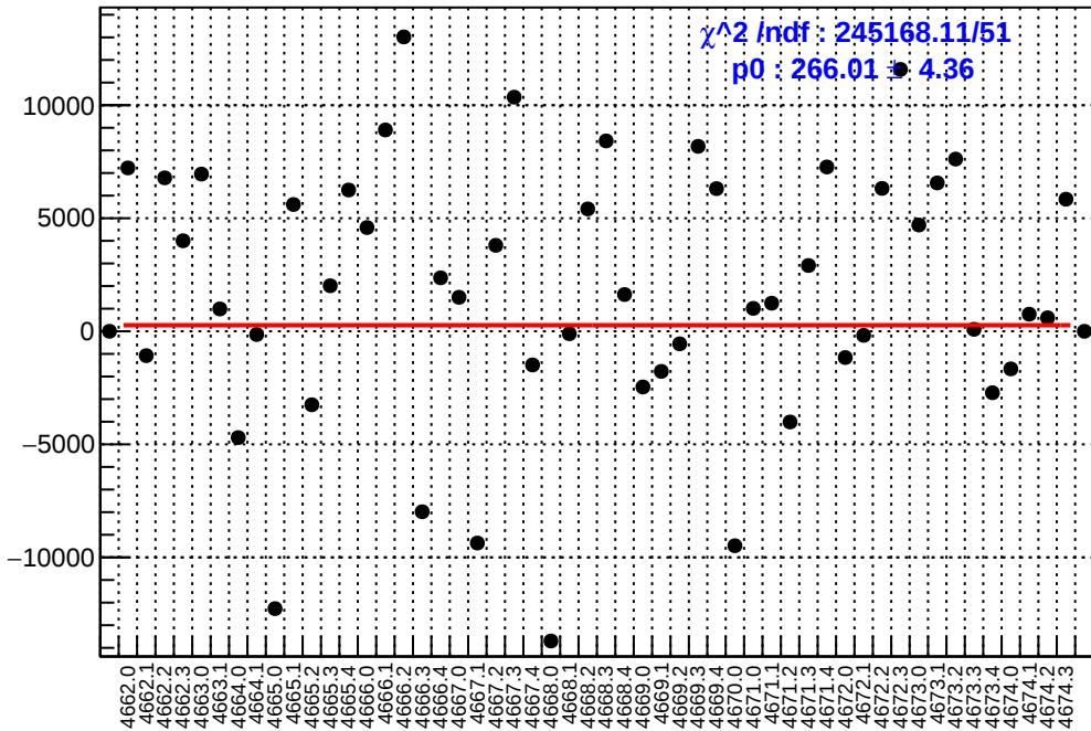
slug73: asym_sam5.mean/ppb-reg_asym_sam5.mean/ppb
