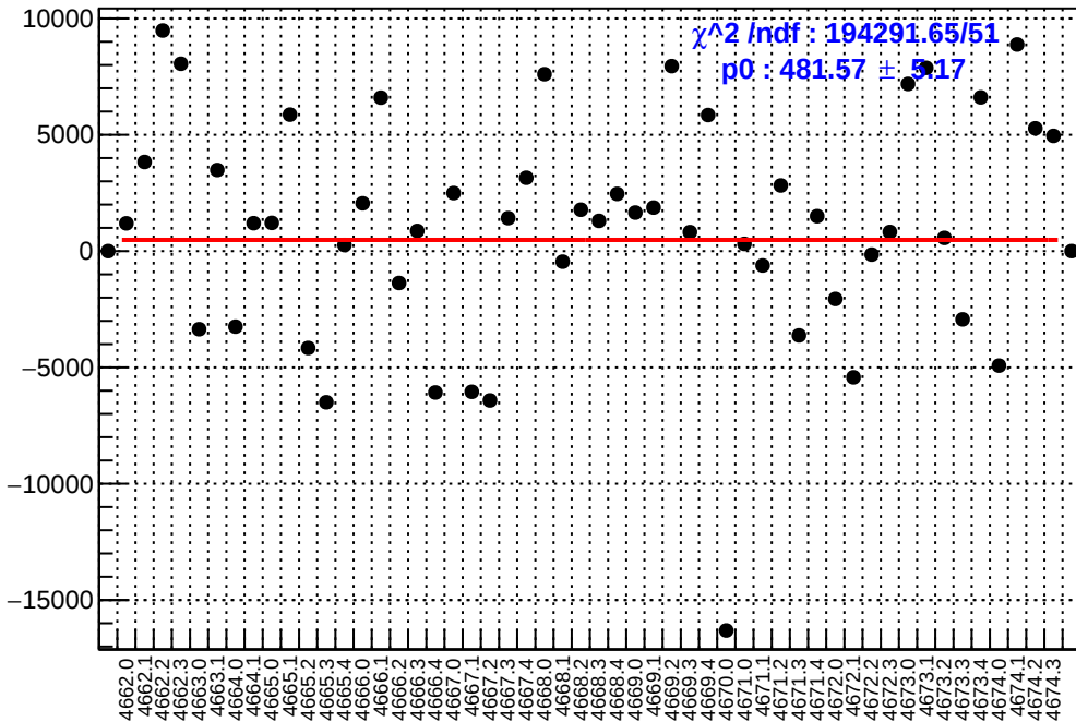
slug73: asym_us_dd.mean/ppb-reg_asym_us_dd.mean/ppb
