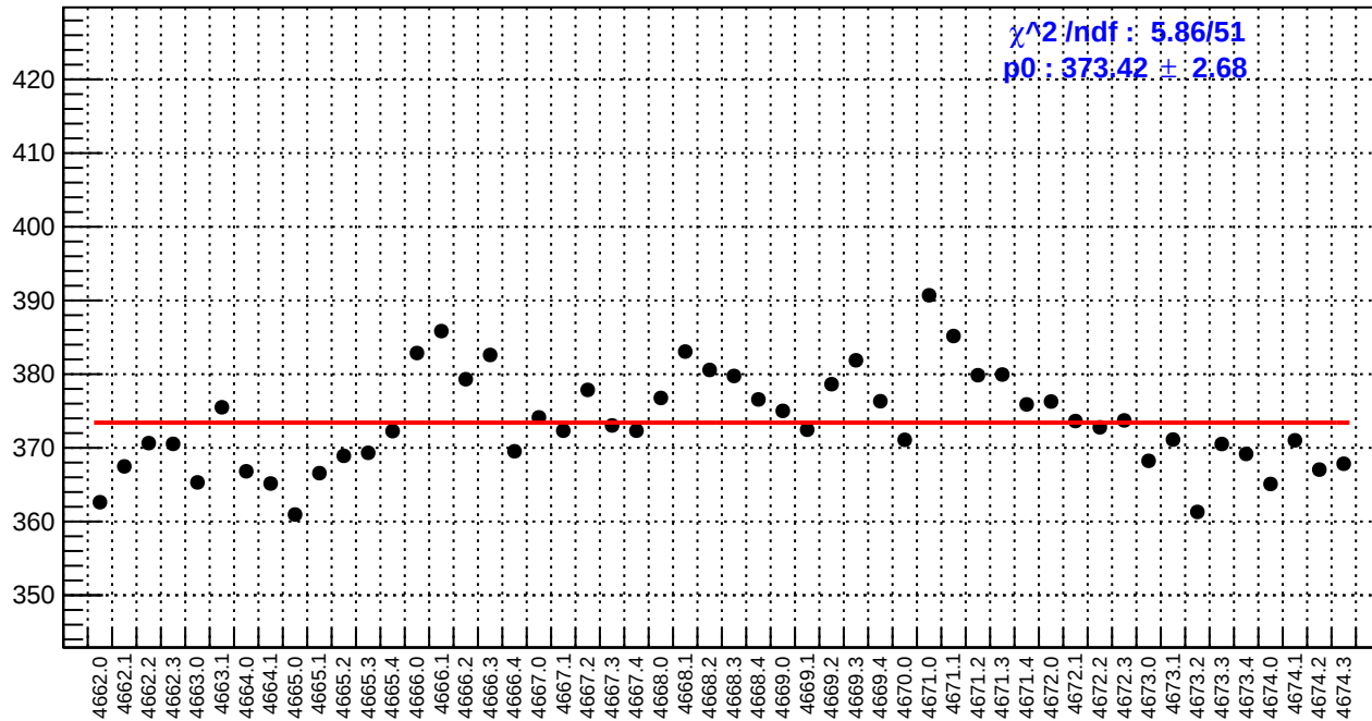
slug73: reg_asym_atr1l2_dd.rms/ppm
