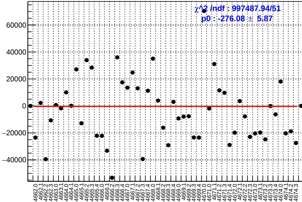
slug73: asym_atl1r2_avg.mean/ppb-reg_asym_atl1r2_avg.mean/ppb
