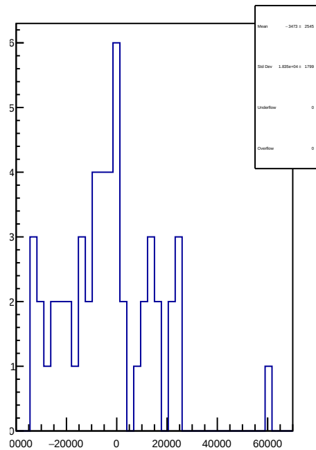
slug73: 1D Corr asym_sam7.mean/ppb-reg_asym_sam7.mean/ppb
