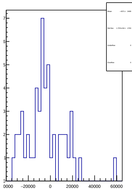
slug73: 1D Corr asym_sam8.mean/ppb-reg_asym_sam8.mean/ppb
