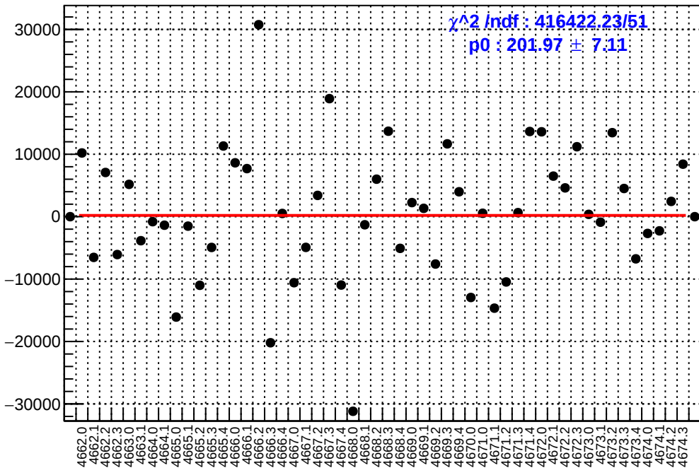
slug73: asym_atl1r2_dd.mean/ppb-reg_asym_atl1r2_dd.mean/ppb
