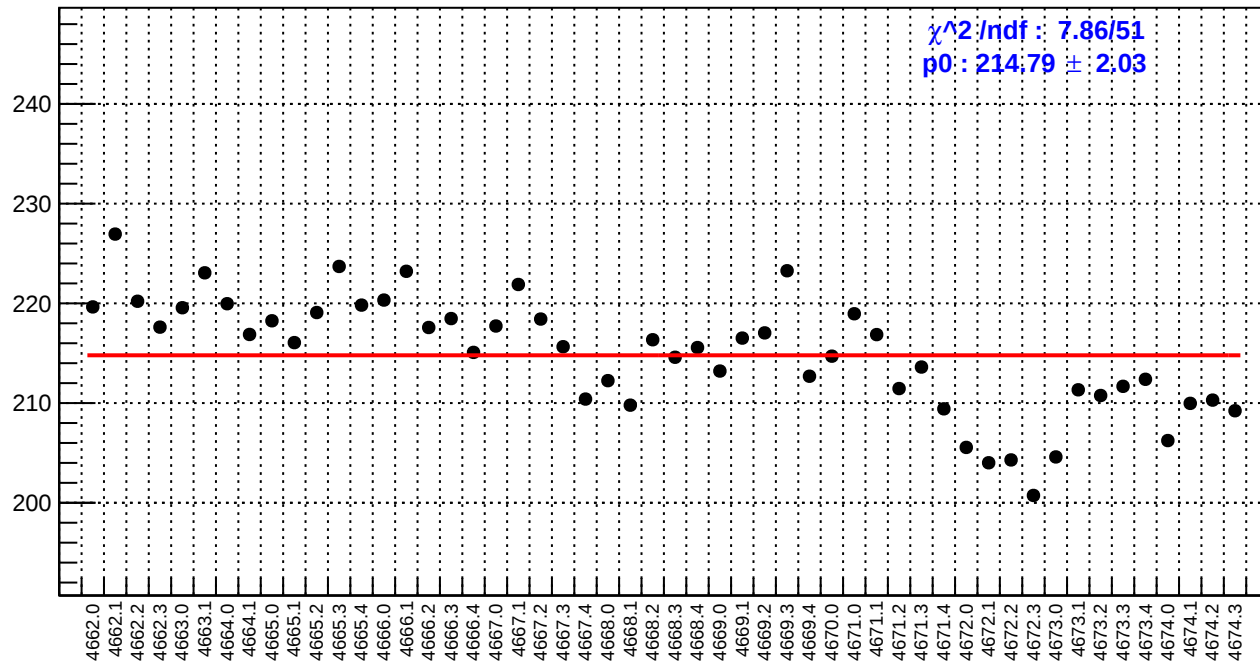
slug73: reg_asym_sam1.rms/ppm
