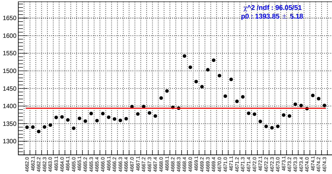
slug73: reg_asym_sam4.rms/ppm
