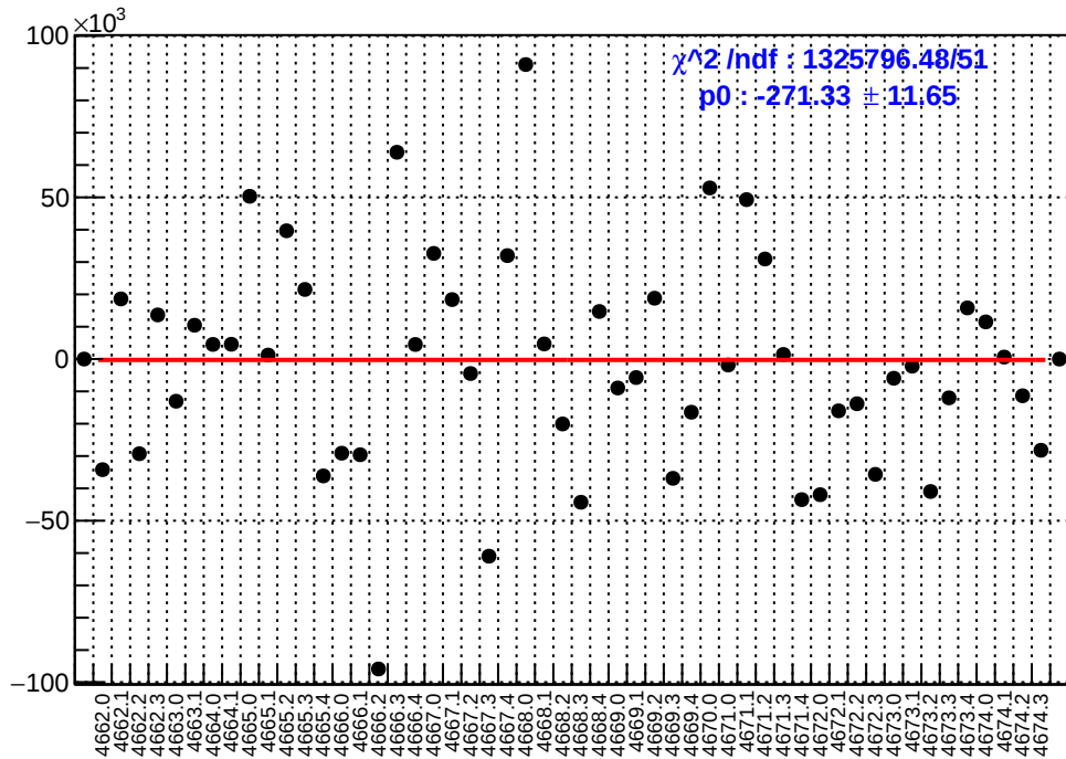
slug73: asym_at2_avg.mean/ppb-reg_asym_at2_avg.mean/ppb
