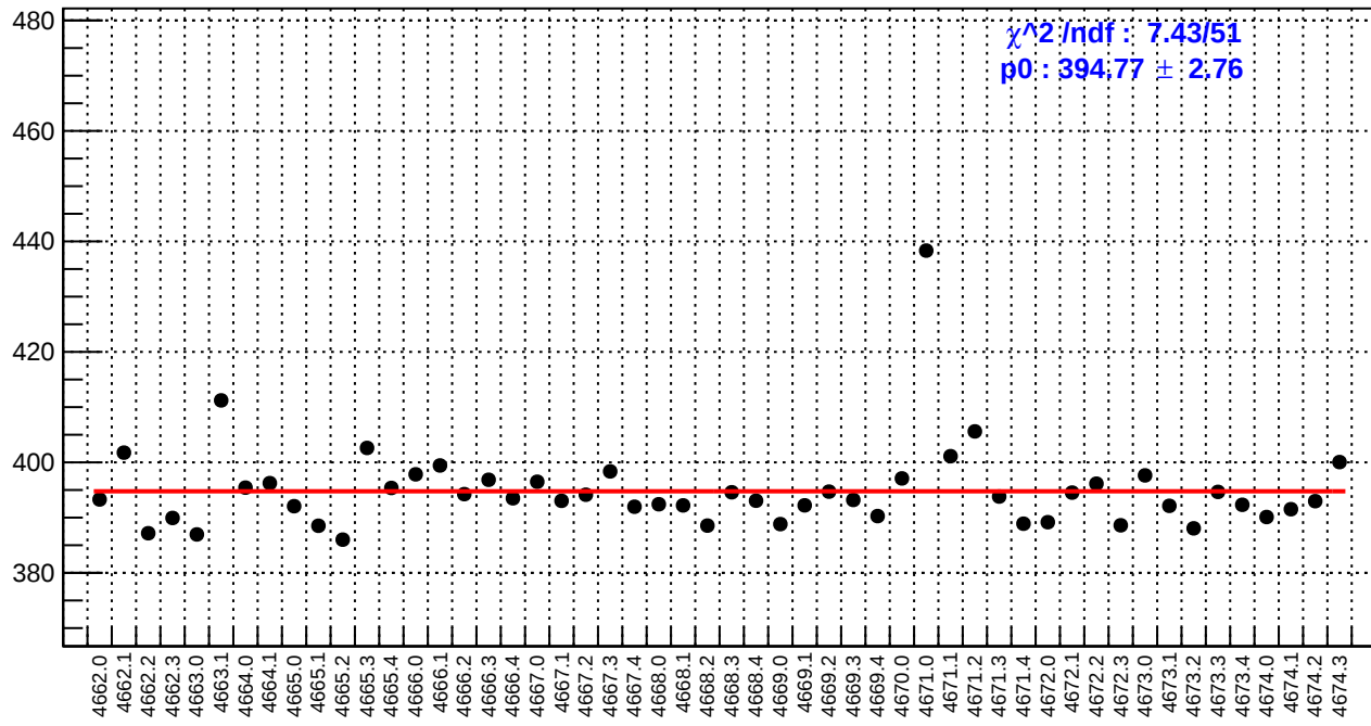
slug73: reg_asym_atl1r2_dd.rms/ppm
