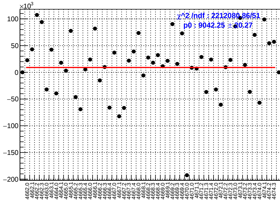
slug73: asym_sam4.mean/ppb-reg_asym_sam4.mean/ppb
