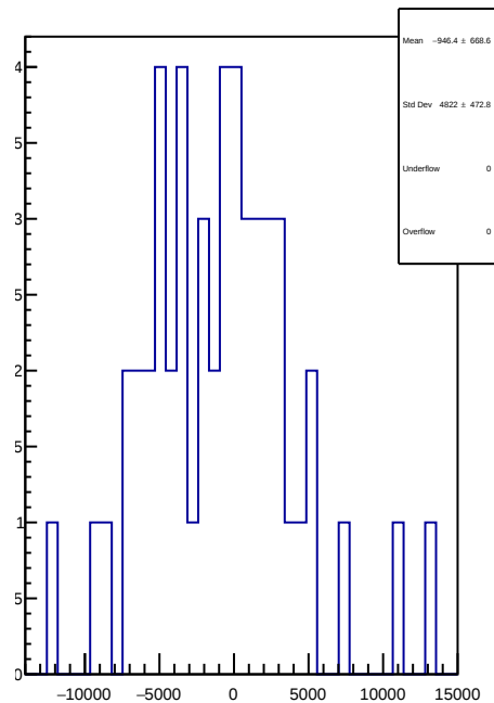
slug73: 1D Corr asym_sam1.mean/ppb-reg_asym_sam1.mean/ppb
