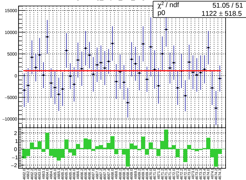
slug73: reg_asym_at2_avg.mean/ppb
