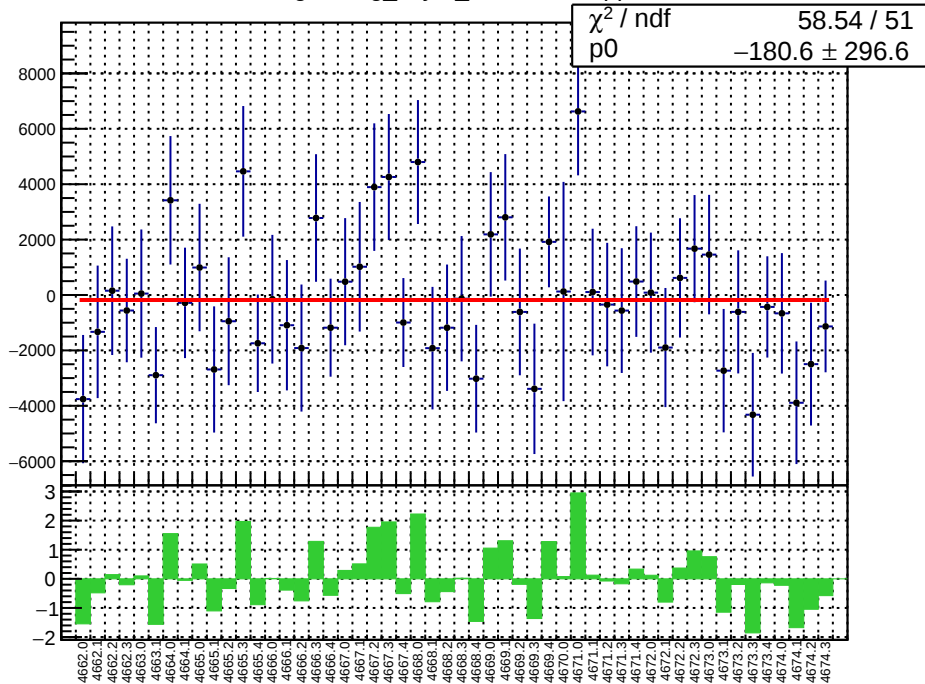
slug73: reg_asym_sam1.mean/ppb
