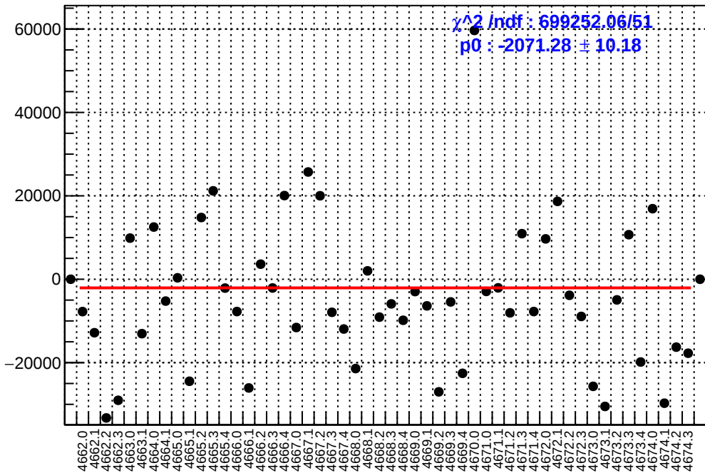
slug73: asym_sam8.mean/ppb-reg_asym_sam8.mean/ppb
