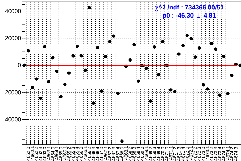
slug73: asym_atl_dd.mean/ppb-reg_asym_atl_dd.mean/ppb
