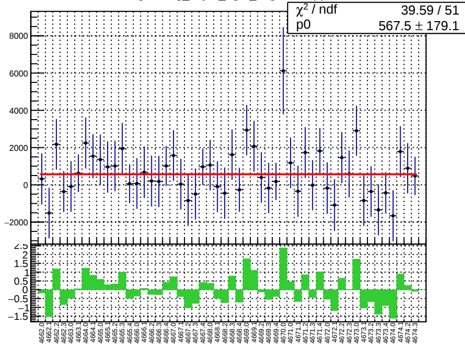
slug73: reg_asym_right_avg.mean/ppb
