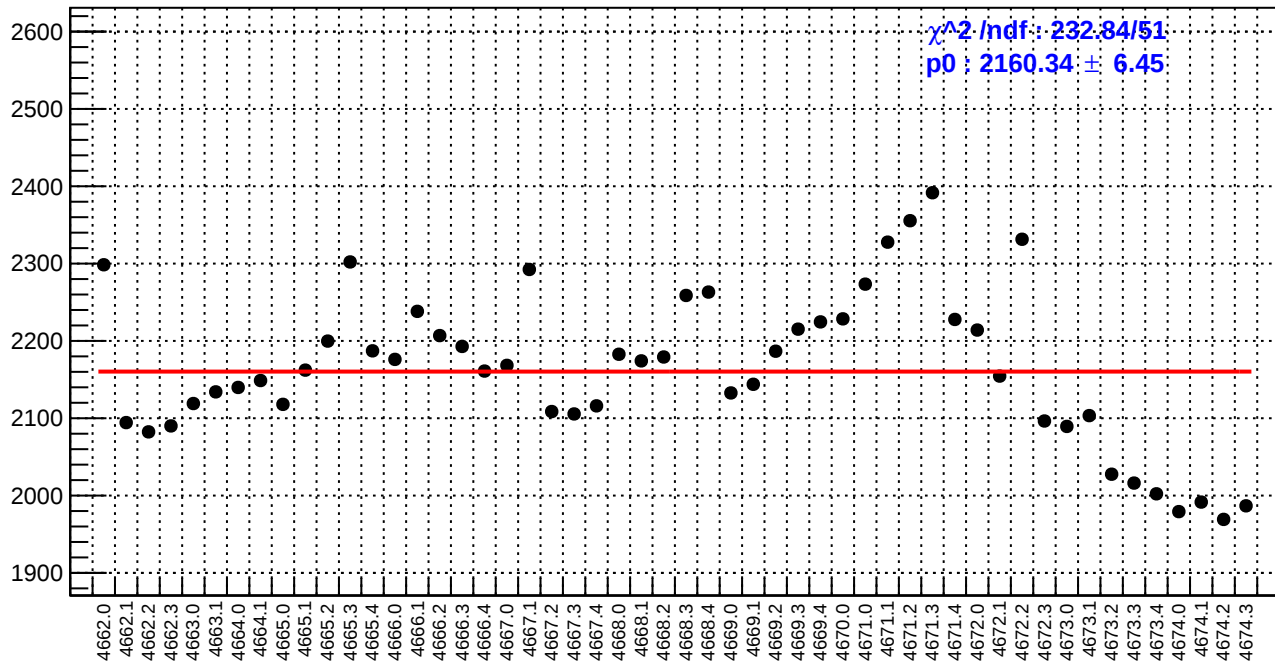
slug73: diff_bpm4aX.rms/nm
