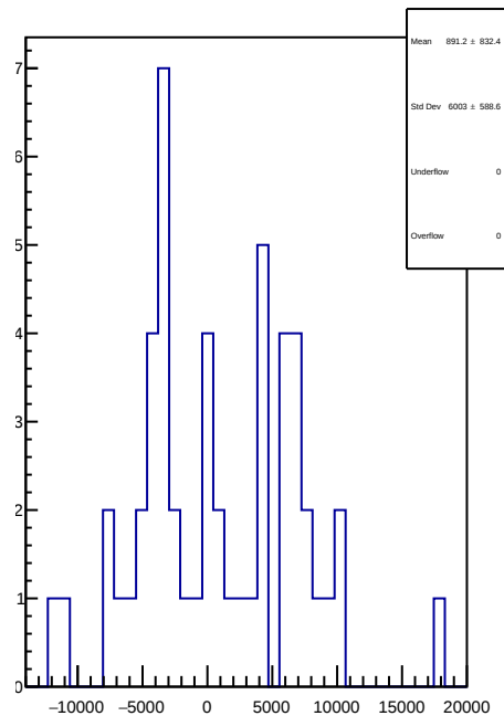
slug73: 1D Corr asym_usl.mean/ppb-reg_asym_usl.mean/ppb
