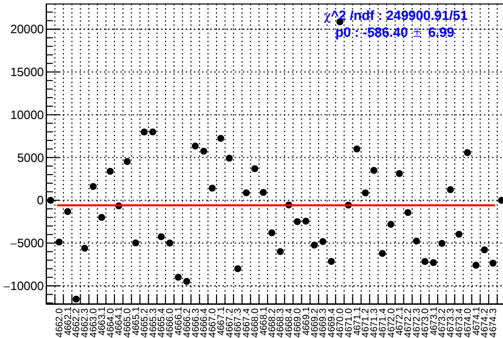
slug73: asym_right_avg.mean/ppb-reg_asym_right_avg.mean/ppb
