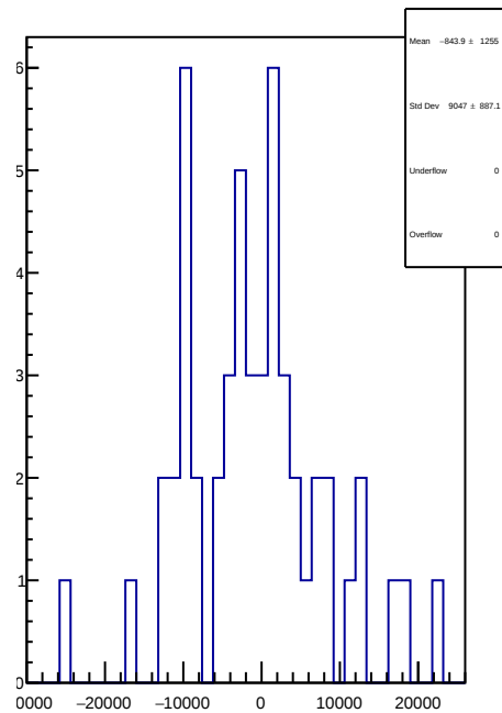
slug73: 1D Corr asym_atr_avg.mean/ppb-reg_asym_atr_avg.mean/ppb
