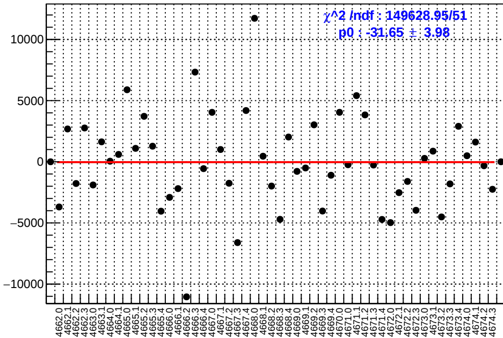
slug73: asym_ds_avg.mean/ppb-reg_asym_ds_avg.mean/ppb
