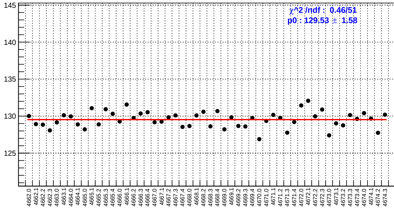
slug73: reg_asym_right_avg.rms/ppm
