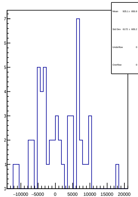
slug73: 1D Corr asym_left_avg.mean/ppb-reg_asym_left_avg.mean/ppb
