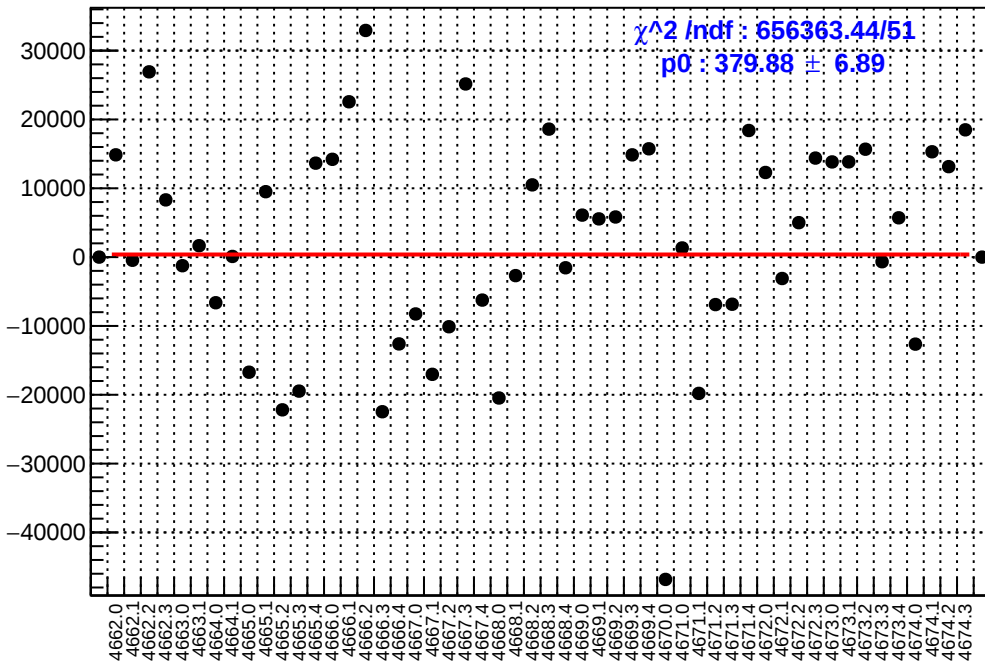
slug73: asym_atr1.mean/ppb-reg_asym_atr1.mean/ppb
