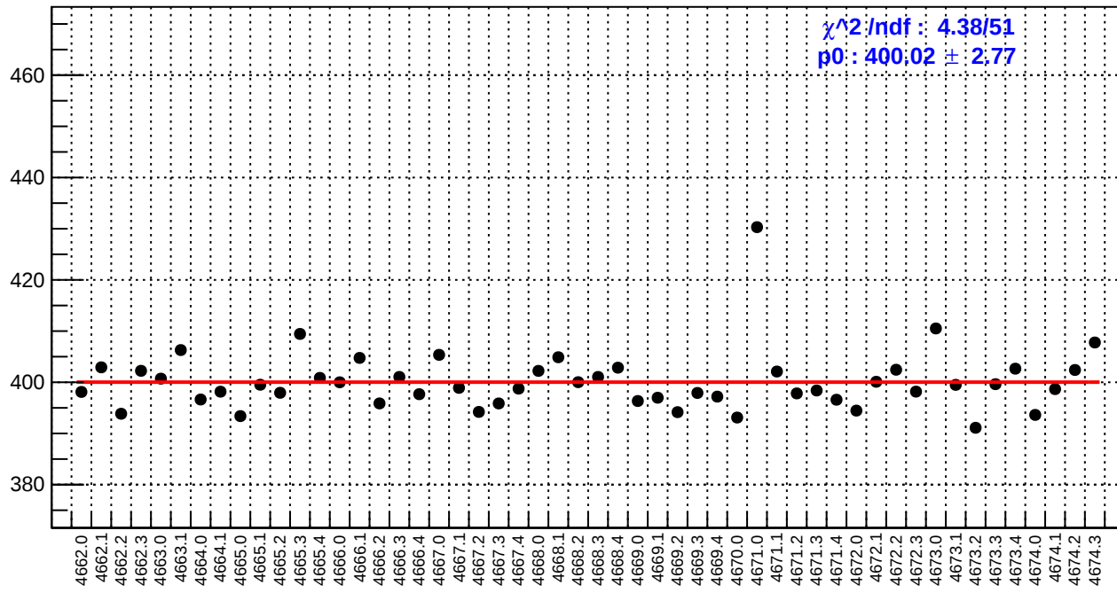
slug73: reg_asym_atr2.rms/ppm
