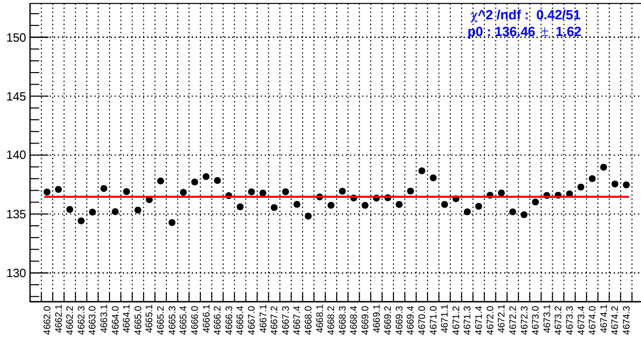
slug73: reg_asym_usl.rms/ppm
