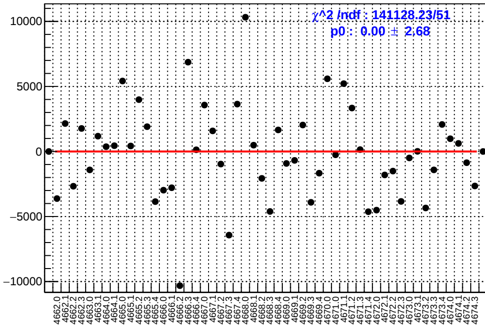
slug73: asym_us_avg.mean/ppb-reg_asym_us_avg.mean/ppb
