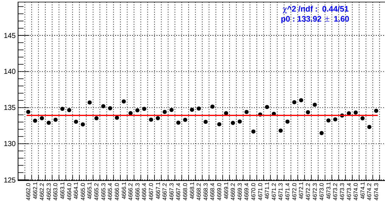
slug73: reg_asym_dsr.rms/ppm
