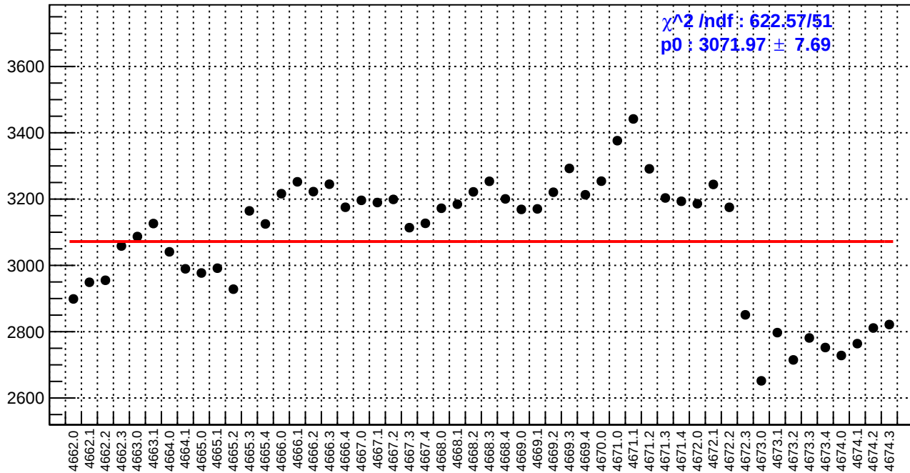
slug73: diff_bpm4aY.rms/nm
