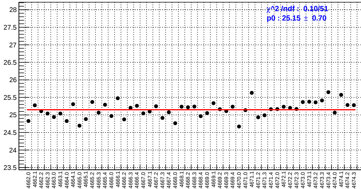
slug73: reg_asym_left_dd.rms/ppm
