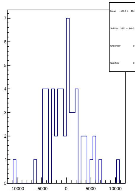
slug73: 1D Corr asym_us_avg.mean/ppb-reg_asym_us_avg.mean/ppb
