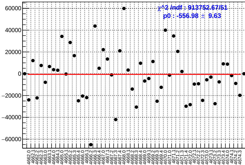
slug73: asym_atl_avg.mean/ppb-reg_asym_atl_avg.mean/ppb
