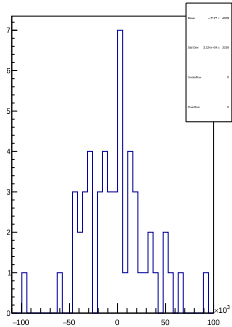
slug73: 1D Corr asym_at2_avg.mean/ppb-reg_asym_at2_avg.mean/ppb
