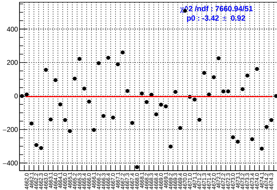
slug73: asym_left_dd.mean/ppb-reg_asym_left_dd.mean/ppb
