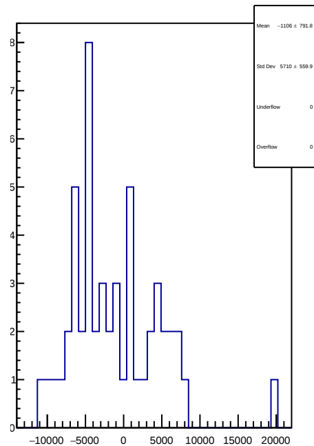
slug73: 1D Corr asym_dsr.mean/ppb-reg_asym_dsr.mean/ppb
