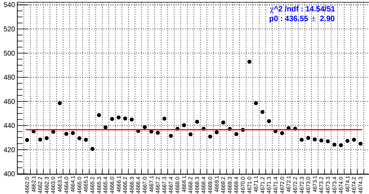
slug73: reg_asym_at1_dd.rms/ppm
