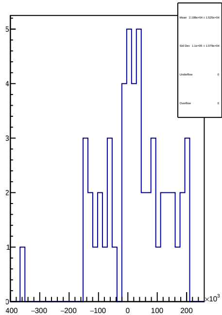
slug73: 1D Corr asym_sam3.mean/ppb-reg_asym_sam3.mean/ppb
