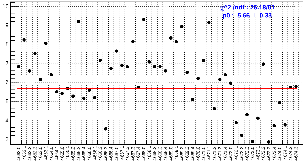
slug73: us_avg_bpm4aX/(ppb/nm)
