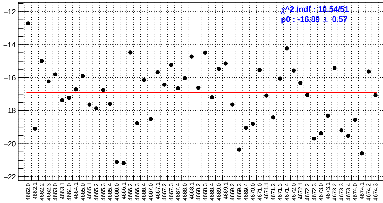
slug73: right_avg_bpm4aX/(ppb/nm)
