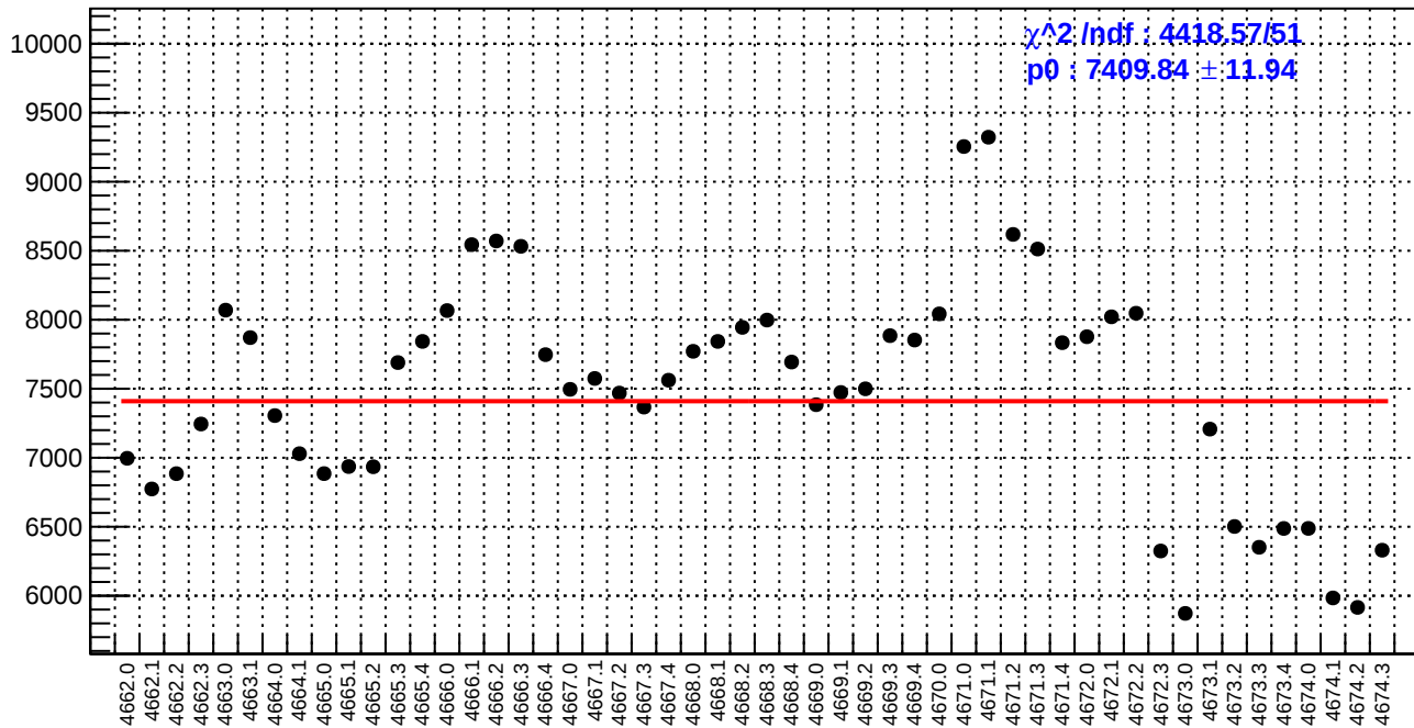
slug73: diff_bpm11X.rms/nm
