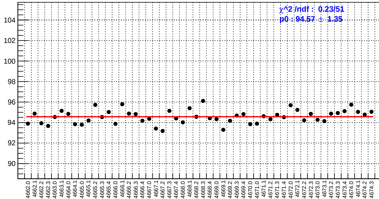
slug73: reg_asym_ds_dd.rms/ppm
