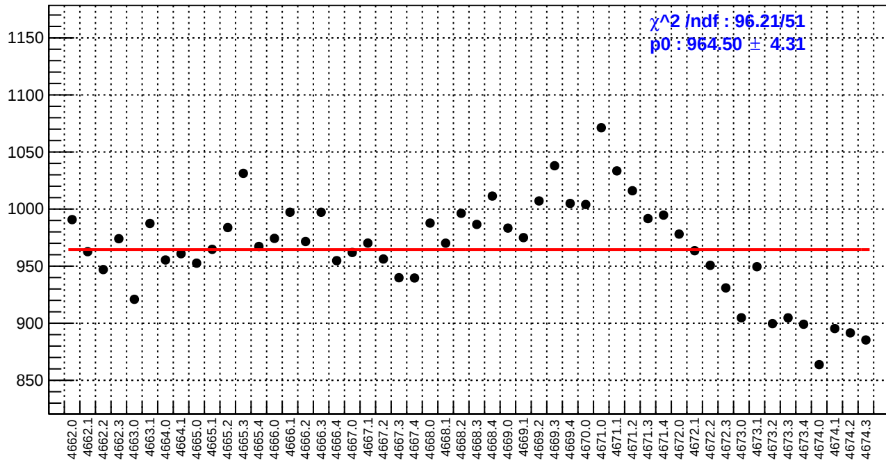
slug73: reg_asym_sam3.rms/ppm
