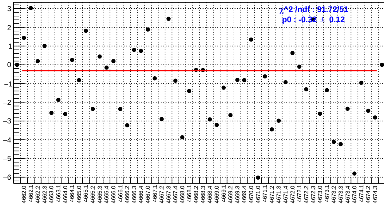
slug73: us_avg_bpm4eY/(ppb/nm)
