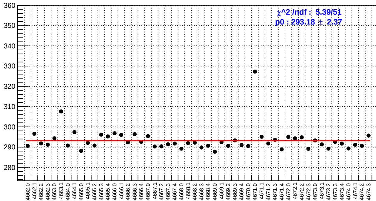
slug73: reg_asym_atr_avg.rms/ppm
