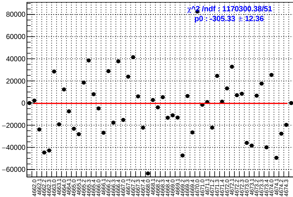
slug73: asym_sam6.mean/ppb-reg_asym_sam6.mean/ppb
