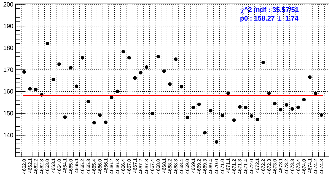
slug73: asym_bcm_an_ds.rms/ppm
