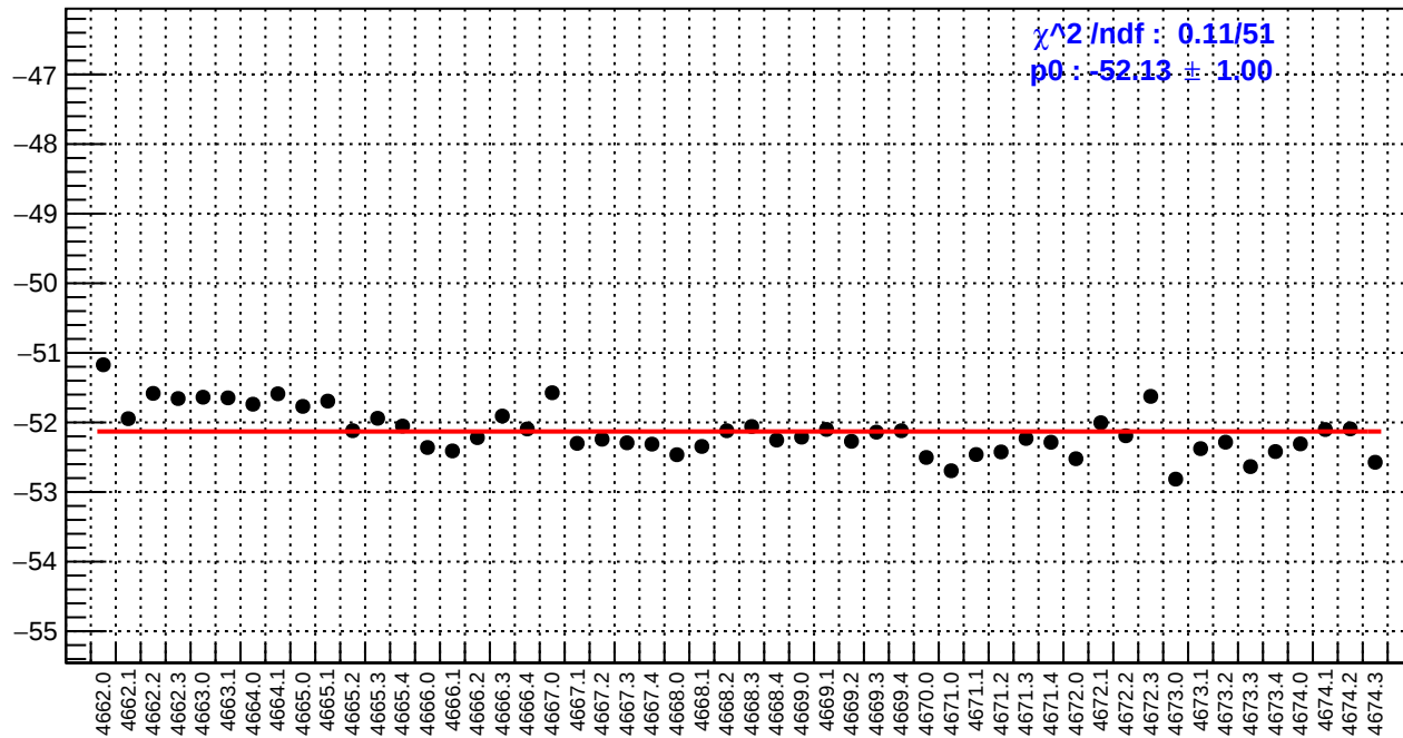
slug73: ds_avg_bpm12X/(ppb/nm)
