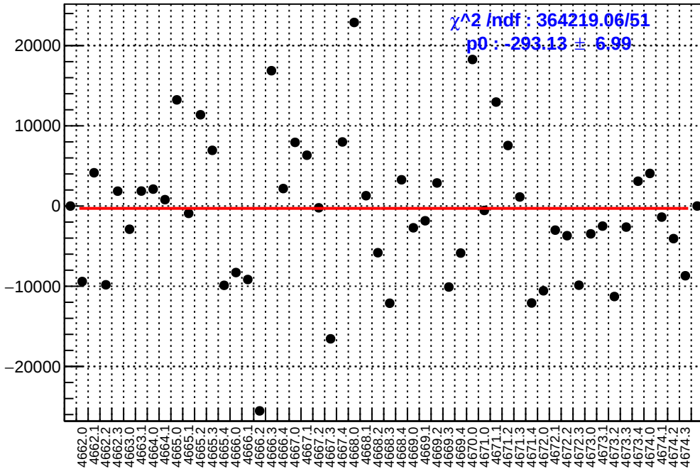
slug73: asym_atr_avg.mean/ppb-reg_asym_atr_avg.mean/ppb
