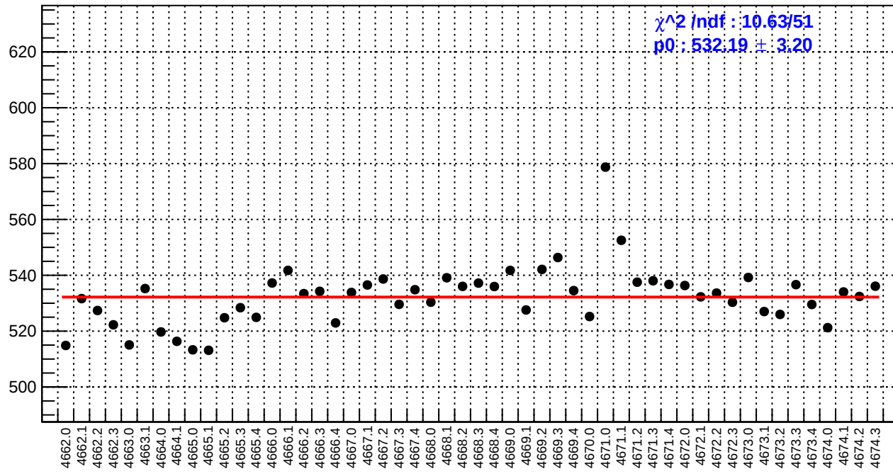
slug73: reg_asym_atl2.rms/ppm
