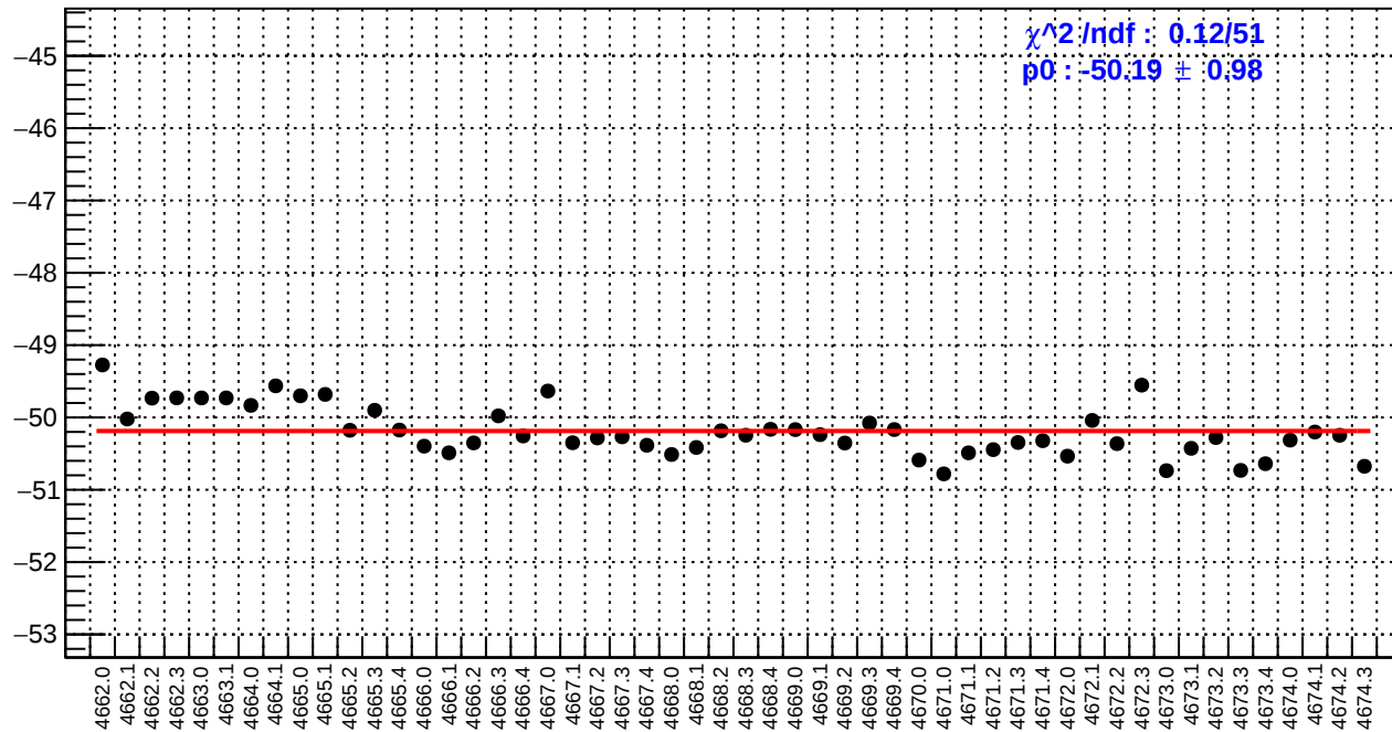
slug73: us_avg_bpm12X/(ppb/nm)
