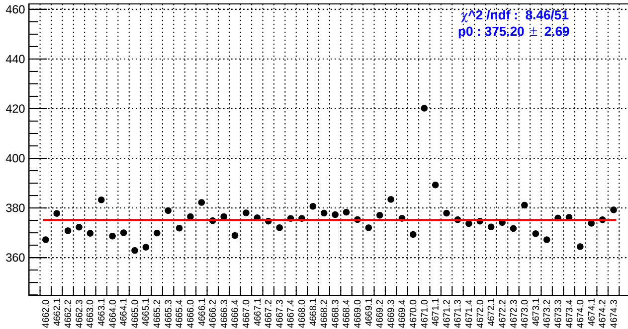
slug73: reg_asym_at2_avg.rms/ppm
