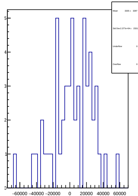
slug73: 1D Corr asym_atr_dd.mean/ppb-reg_asym_atr_dd.mean/ppb
