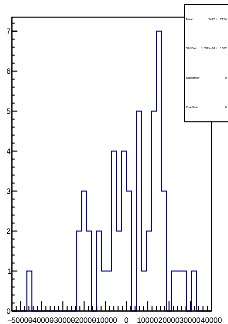
slug73: 1D Corr asym_atr1.mean/ppb-reg_asym_atr1.mean/ppb
