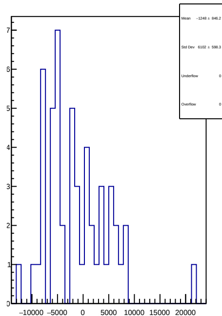
slug73: 1D Corr asym_usr.mean/ppb-reg_asym_usr.mean/ppb
