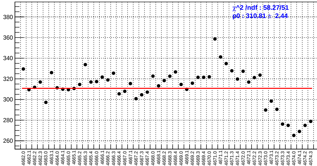
slug73: reg_asym_sam7.rms/ppm
