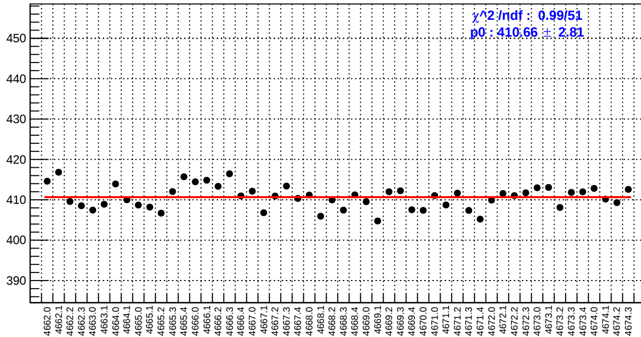
slug73: reg_asym_at1_avg.rms/ppm
