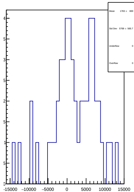
slug73: 1D Corr asym_sam5.mean/ppb-reg_asym_sam5.mean/ppb
