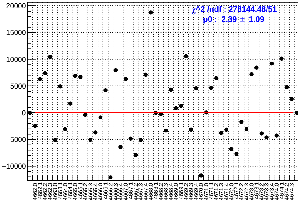
slug73: asym_dsl.mean/ppb-reg_asym_dsl.mean/ppb
