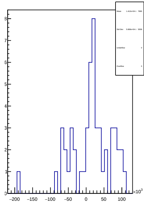
slug73: 1D Corr asym_sam4.mean/ppb-reg_asym_sam4.mean/ppb
