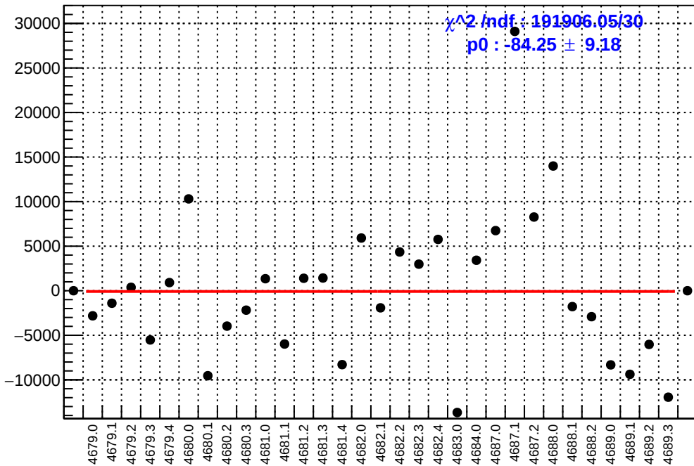
slug74-Left: asym_usl.mean/ppb-reg_asym_usl.mean/ppb
