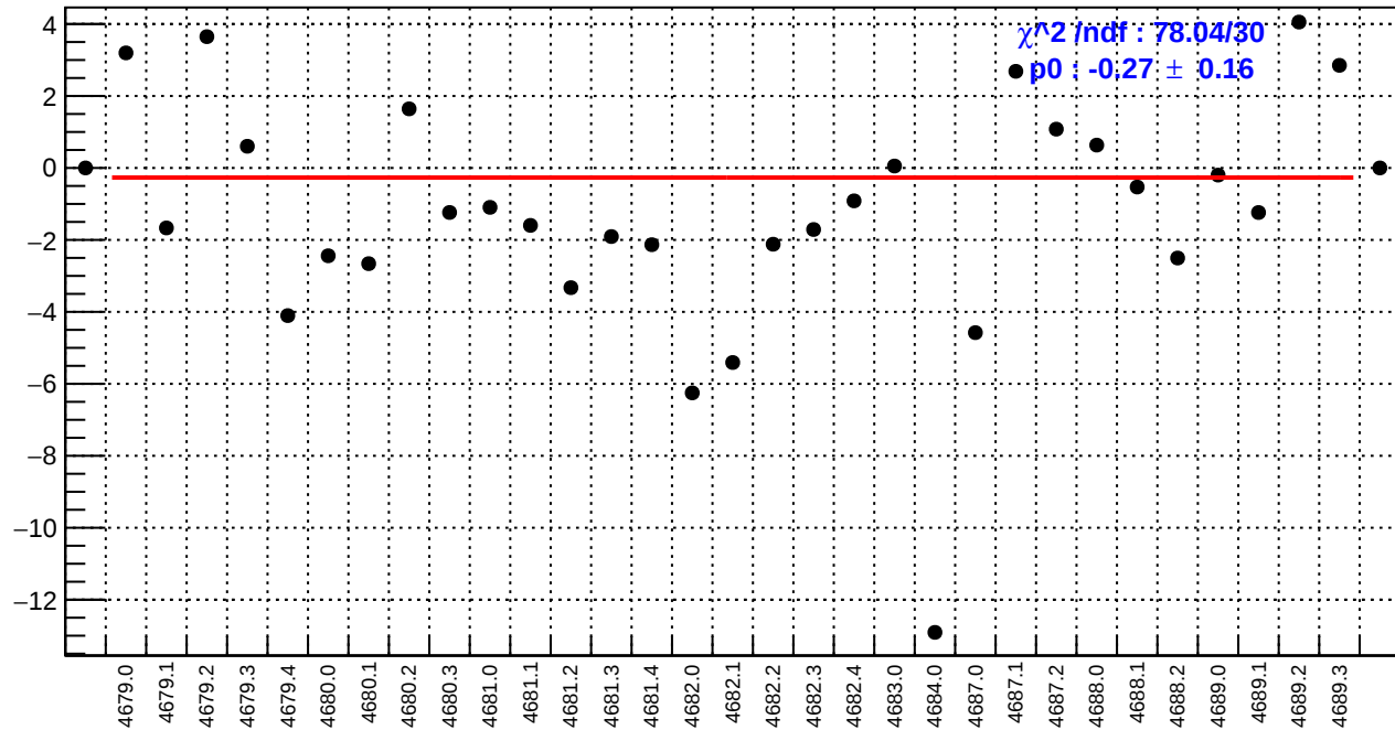
slug74-Left: ds_avg_bpm4eY/(ppb/nm)
