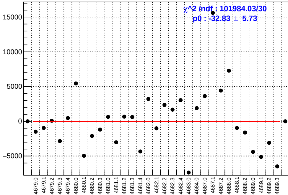
slug74-Left: asym_ds_avg.mean/ppb-reg_asym_ds_avg.mean/ppb
