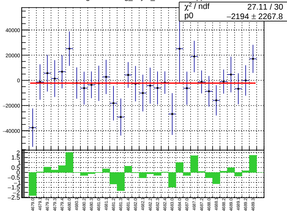
slug74-Left: reg_asym_sam3.mean/ppb
