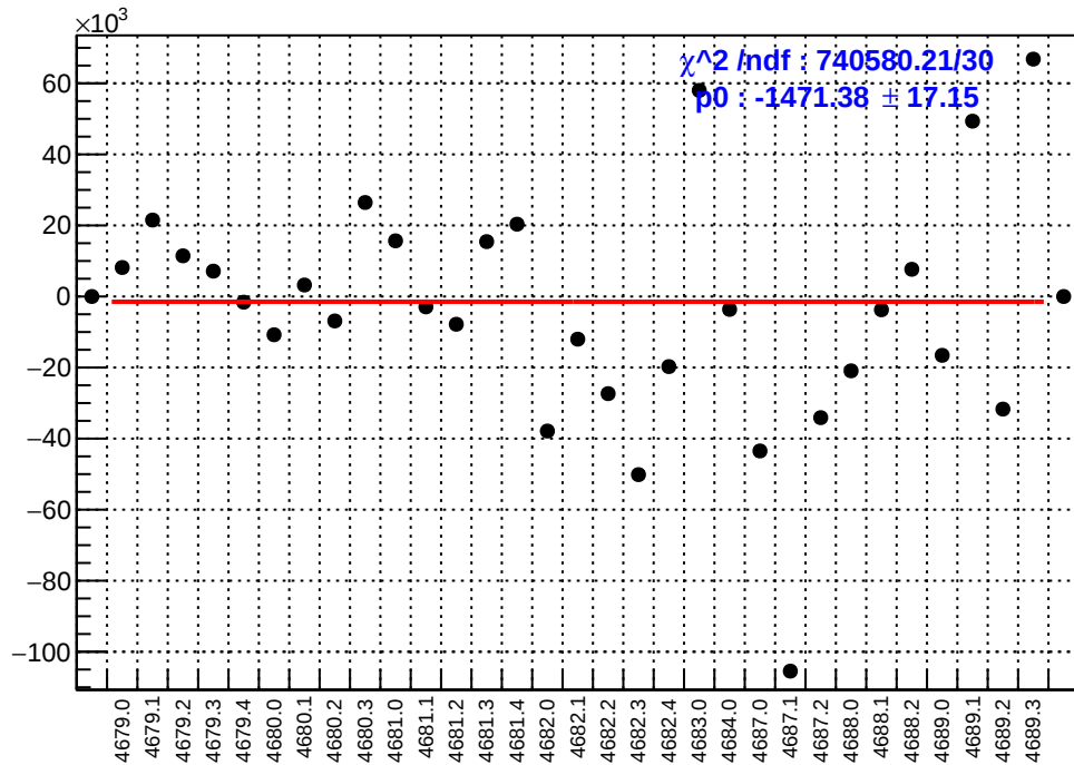
slug74-Left: asym_sam6.mean/ppb-reg_asym_sam6.mean/ppb
