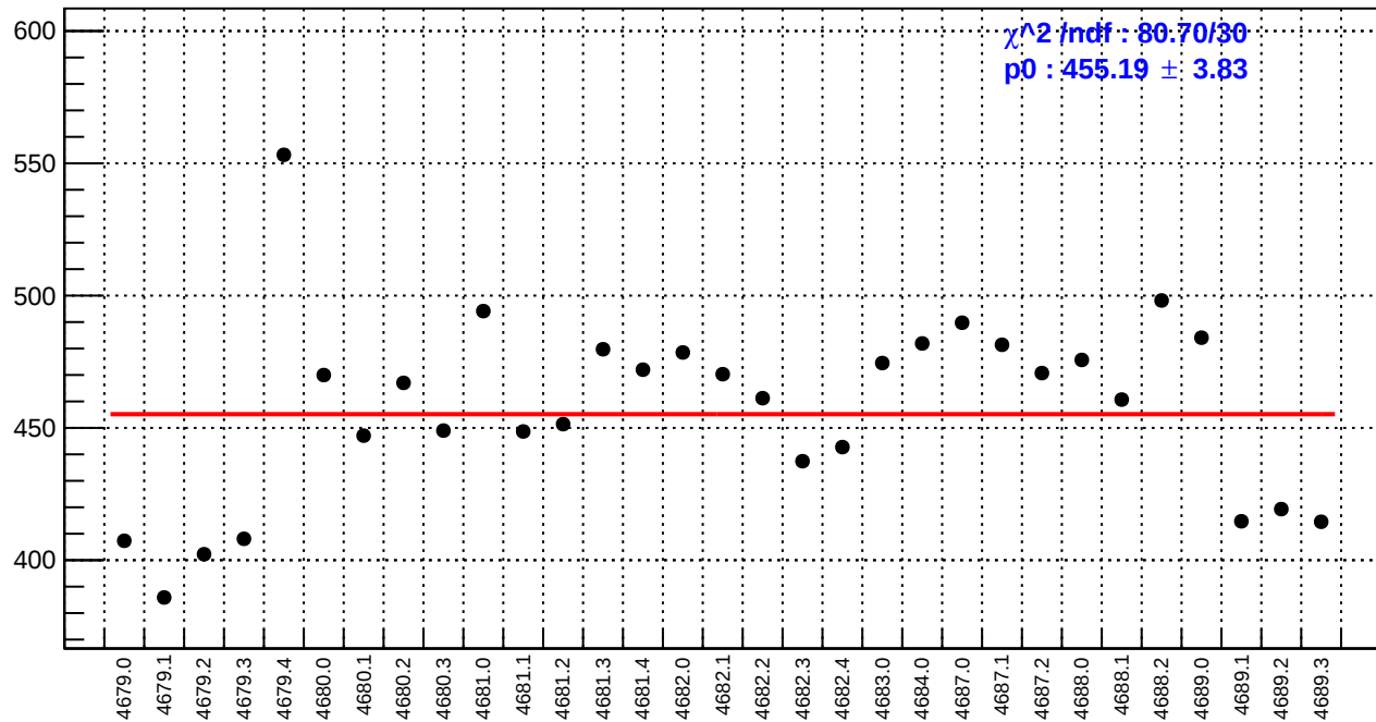
slug74-Left: reg_asym_sam6.rms/ppm
