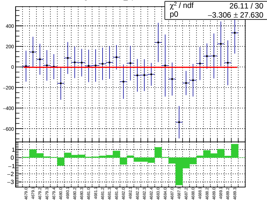
slug74-Left: diff_bpm4eX.mean/nm
