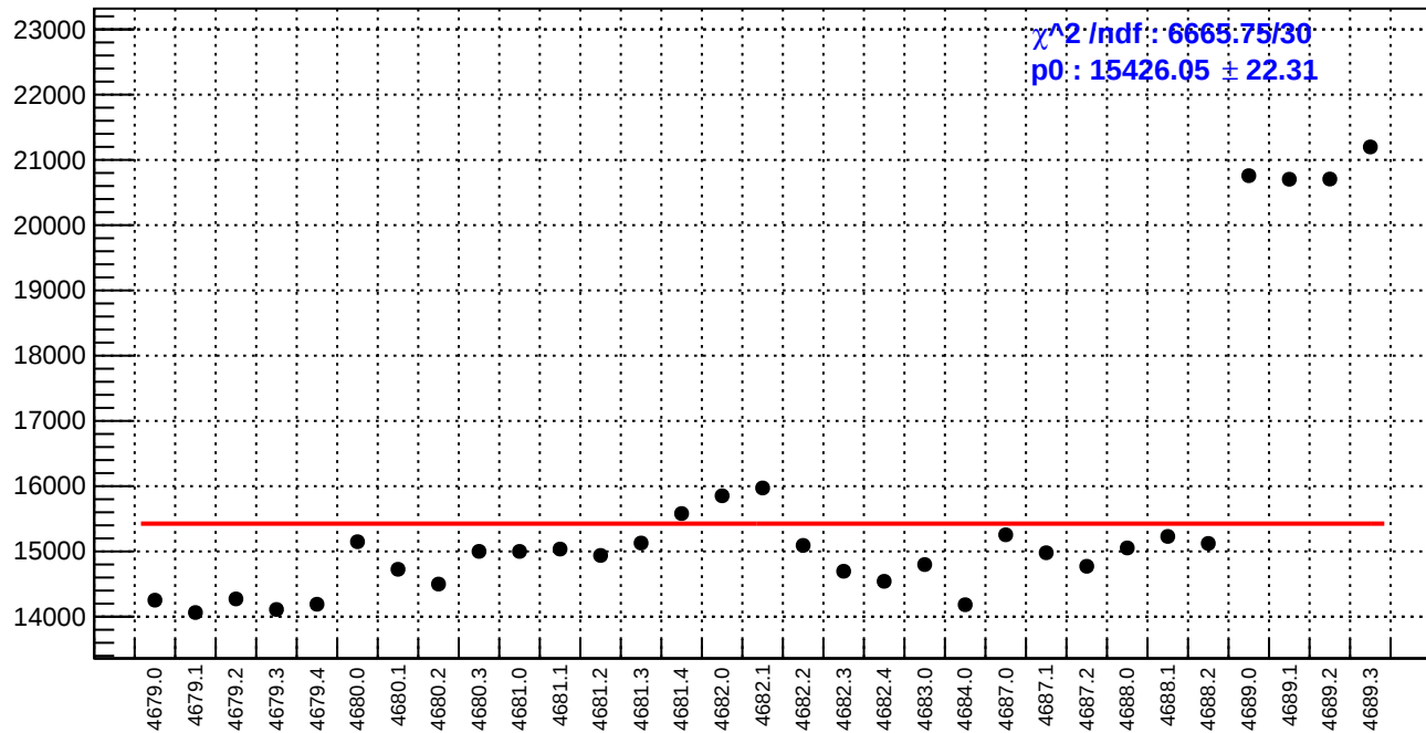
slug74-Left: diff_bpm4eX.rms/nm
