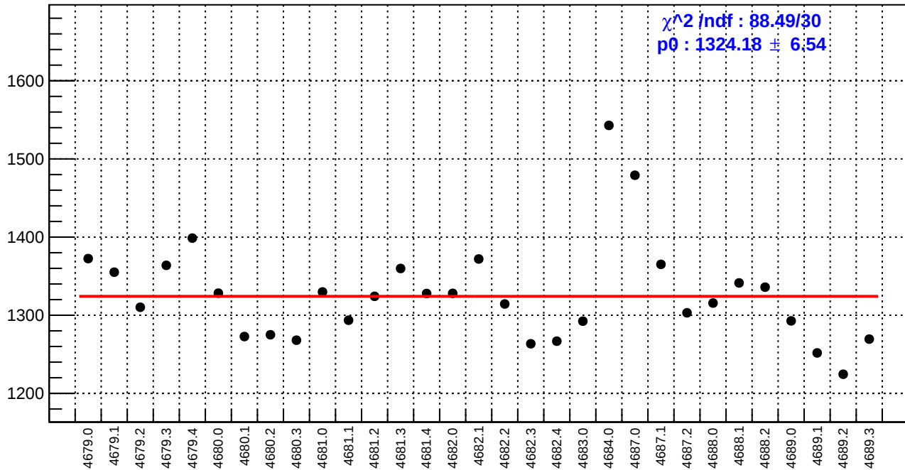
slug74-Left: reg_asym_sam4.rms/ppm
