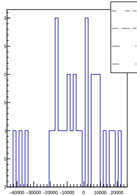
slug74-Left: 1D Corr asym_sam5.mean/ppb-reg_asym_sam5.mean/ppb
