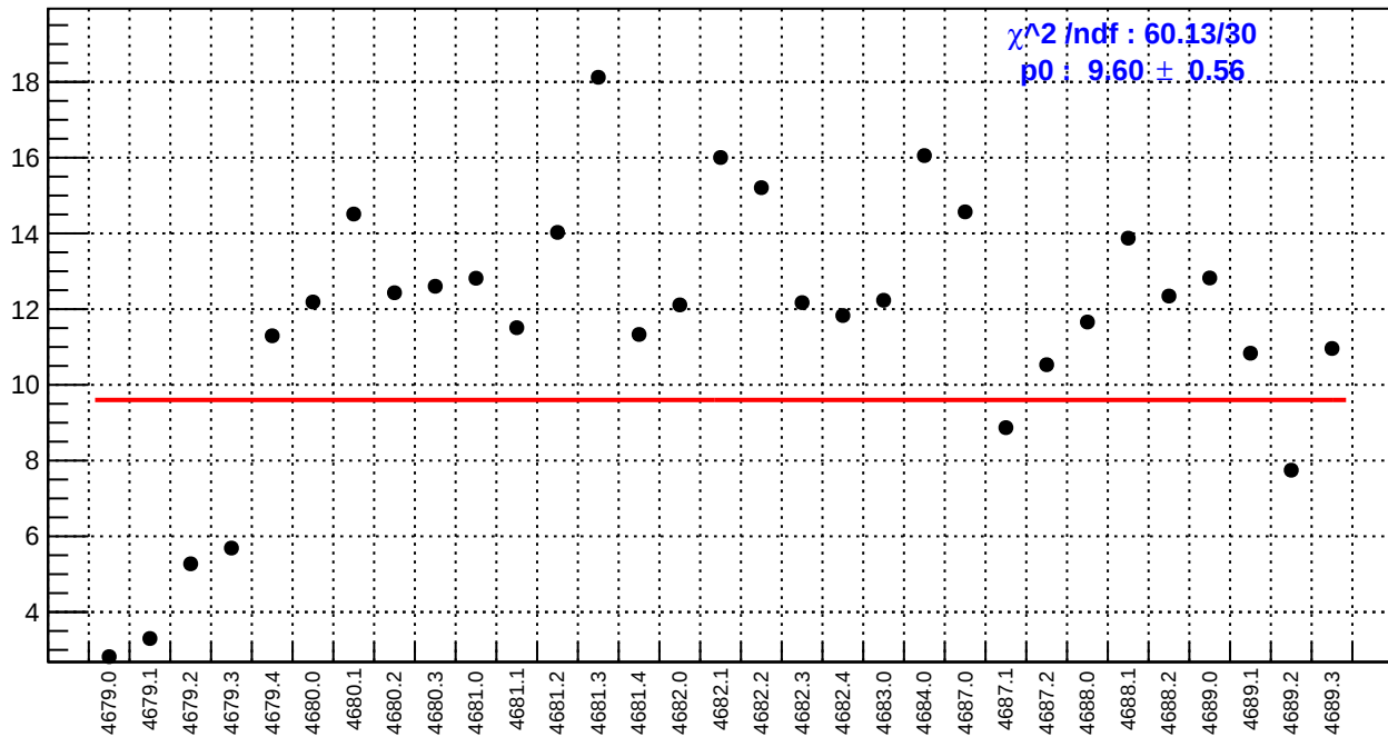
slug74-Left: usl_bpm4aY/(ppb/nm)
