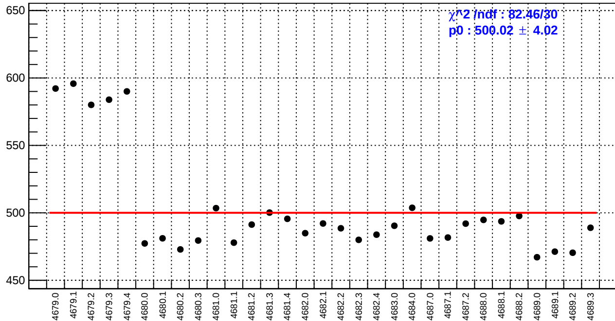
slug74-Left: reg_asym_atl2.rms/ppm
