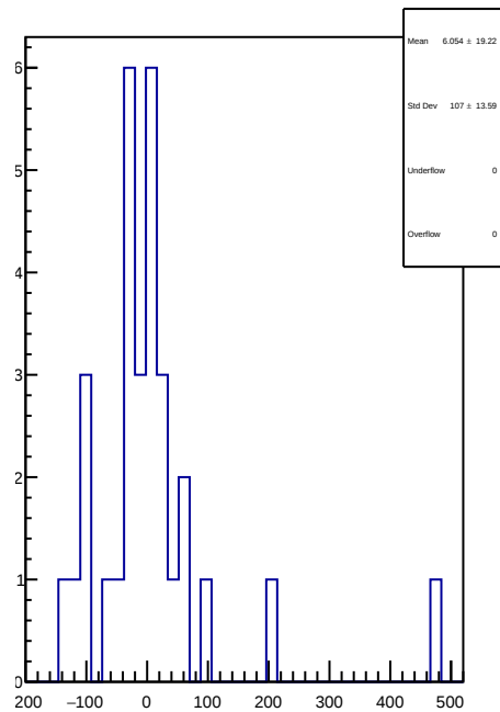
slug74-Left: 1D Corr asym_right_avg.mean/ppb-reg_asym_right_avg.mean/ppb
