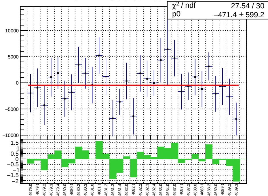
slug74-Left: reg_asym_atl1r2_dd.mean/ppb
