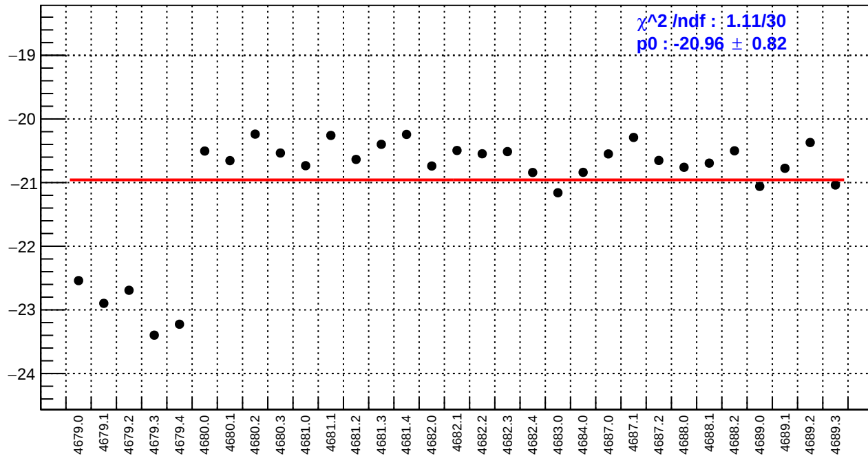
slug74-Left: ds_avg_bpm12X/(ppb/nm)
