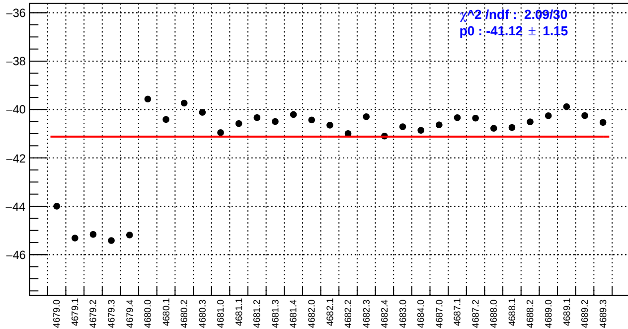
slug74-Left: usl_bpm12X/(ppb/nm)
