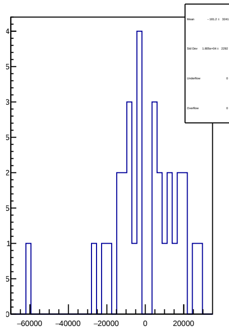
slug74-Left: 1D Corr asym_atl_dd.mean/ppb-reg_asym_atl_dd.mean/ppb
