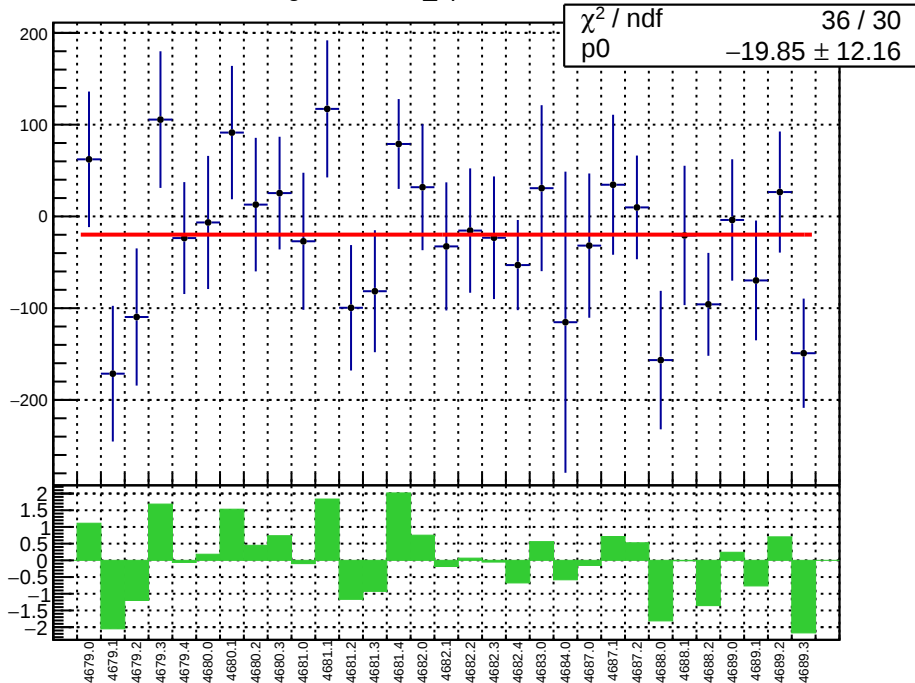
slug74-Left: diff_bpm11X.mean/nm
