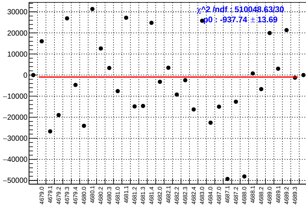
slug74-Left: asym_at2_dd.mean/ppb-reg_asym_at2_dd.mean/ppb
