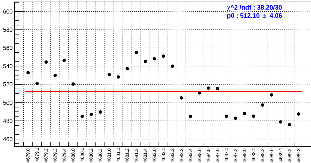
slug74-Left: reg_asym_sam8.rms/ppm
