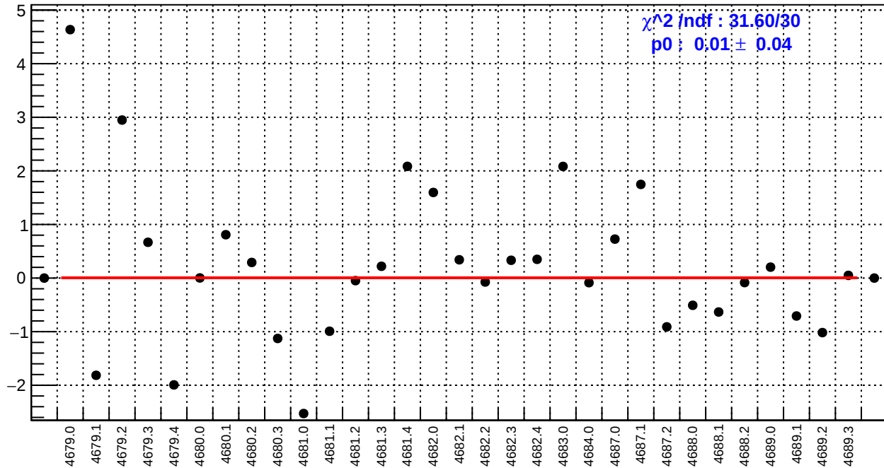
slug74-Left: usr_bpm4eX/(ppb/nm)
