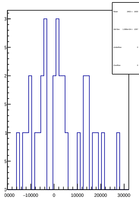
slug74-Left: 1D Corr asym_atl1r2_avg.mean/ppb-reg_asym_atl1r2_avg.mean/ppb
