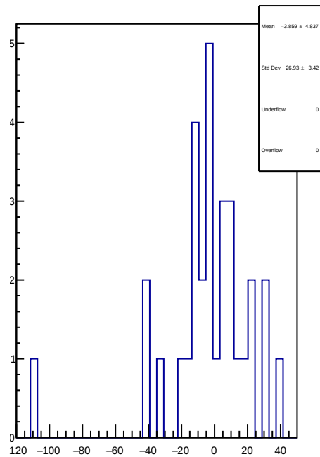
slug74-Left: 1D Corr asym_atr_avg.mean/ppb-reg_asym_atr_avg.mean/ppb
