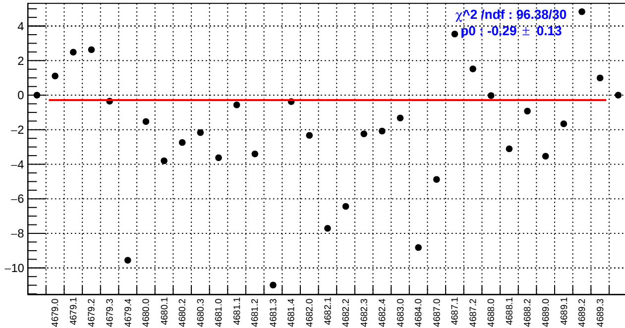
slug74-Left: dsl_bpm4eY/(ppb/nm)
