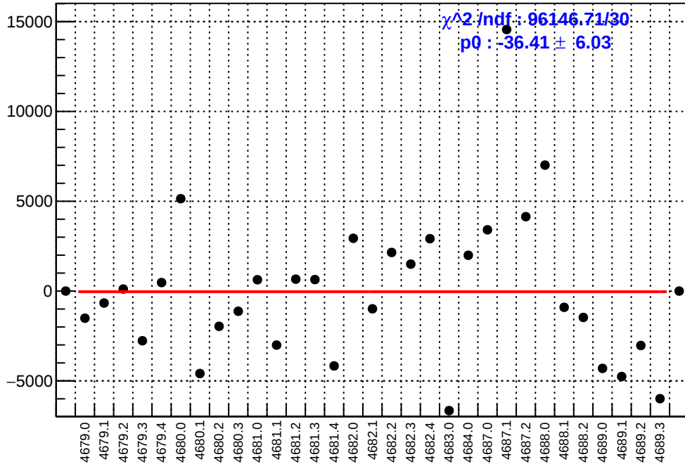
slug74-Left: asym_us_avg.mean/ppb-reg_asym_us_avg.mean/ppb
