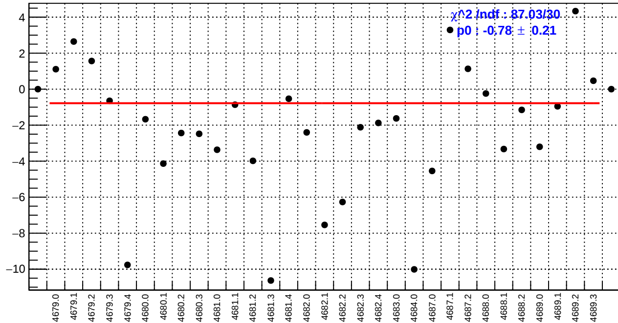
slug74-Left: left_avg_bpm4eY/(ppb/nm)
