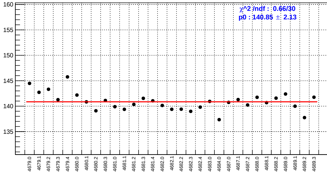
slug74-Left: reg_asym_dsl.rms/ppm
