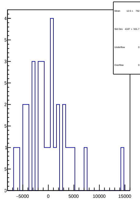
slug74-Left: 1D Corr asym_us_avg.mean/ppb-reg_asym_us_avg.mean/ppb
