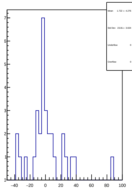
slug74-Left: 1D Corr asym_atr_dd.mean/ppb-reg_asym_atr_dd.mean/ppb
