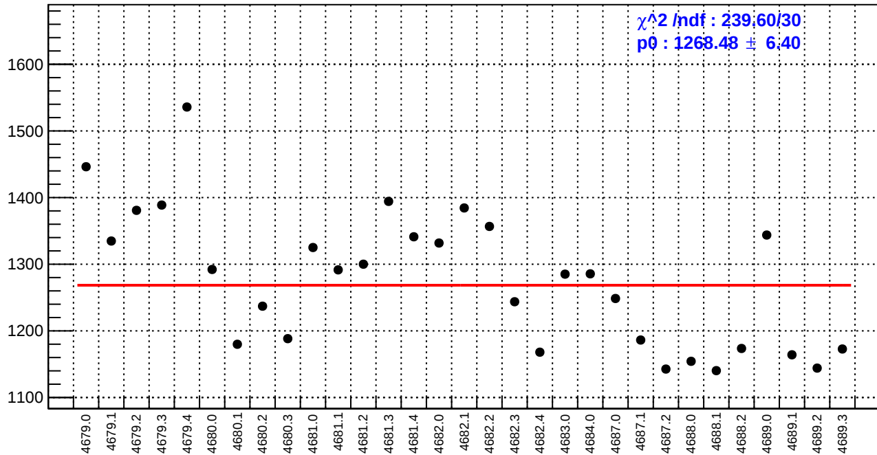
slug74-Left: reg_asym_sam3.rms/ppm
