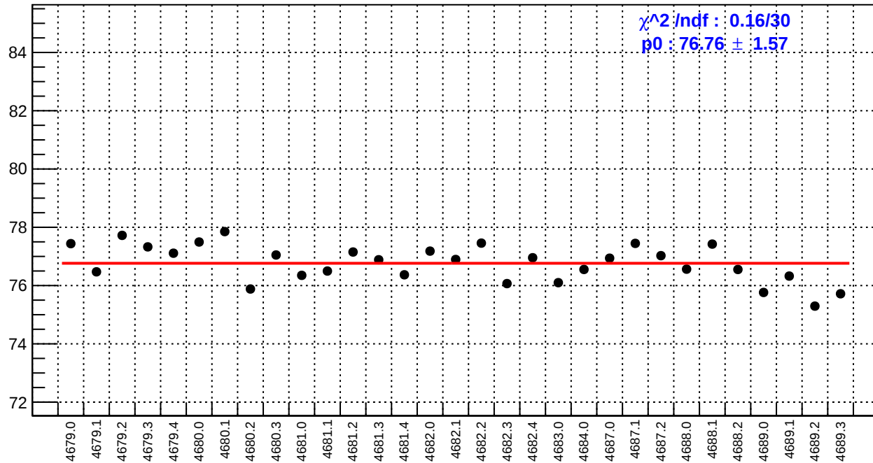
slug74-Left: reg_asym_atr_dd.rms/ppm
