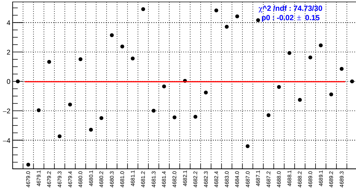
slug74-Left: dsr_bpm4aX/(ppb/nm)
