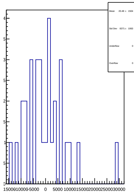
slug74-Left: 1D Corr asym_usl.mean/ppb-reg_asym_usl.mean/ppb
