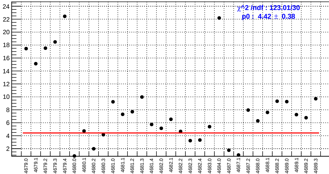
slug74-Left: dsl_bpm4aX/(ppb/nm)
