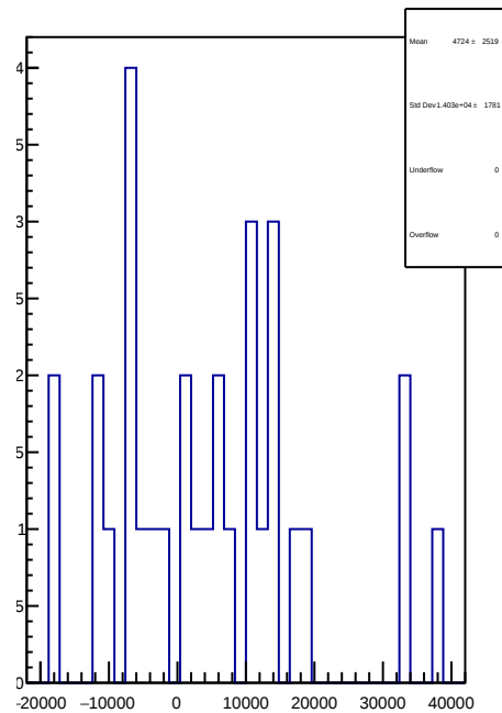
slug74-Left: 1D Corr asym_sam1.mean/ppb-reg_asym_sam1.mean/ppb
