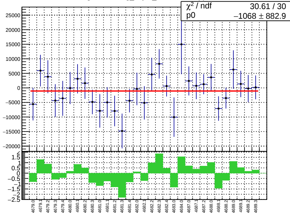
slug74-Left: reg_asym_sam7.mean/ppb
