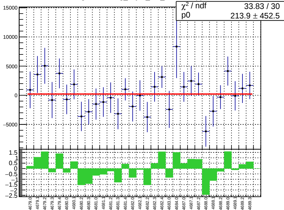
slug74-Left: reg_asym_at2_dd.mean/ppb
