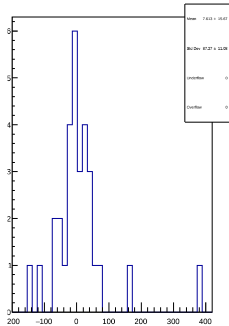
slug74-Left: 1D Corr asym_dsr.mean/ppb-reg_asym_dsr.mean/ppb
