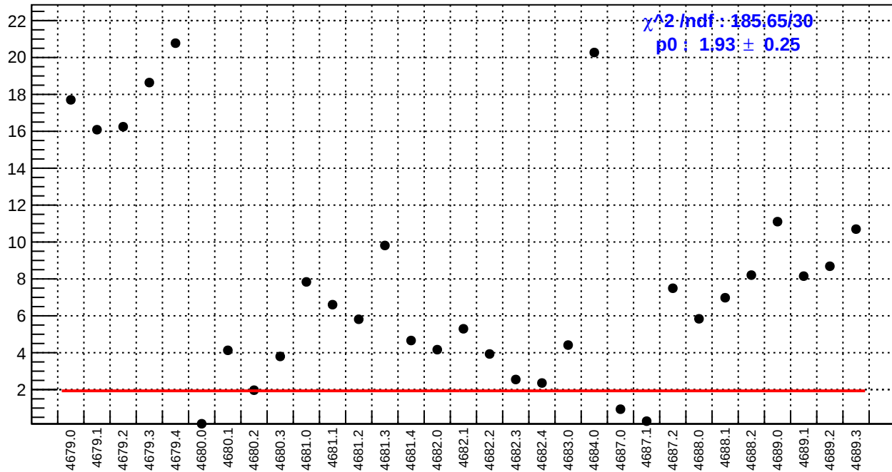
slug74-Left: usl_bpm4aX/(ppb/nm)
