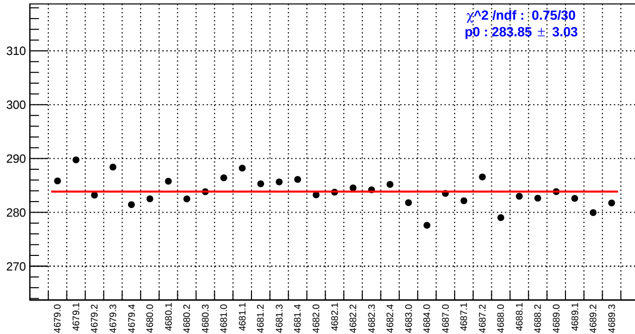
slug74-Left: reg_asym_right_dd.rms/ppm
