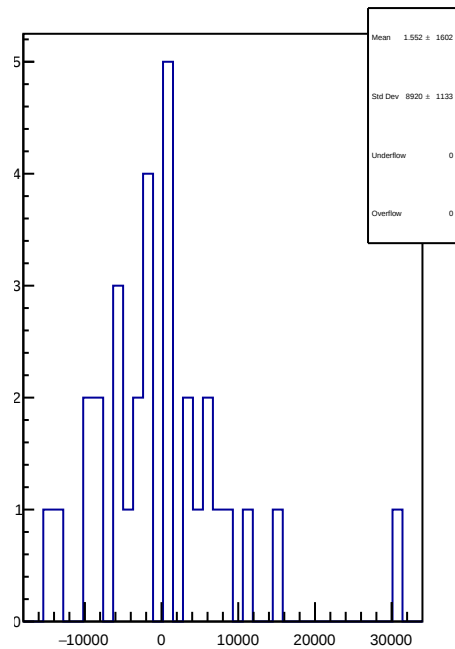
slug74-Left: 1D Corr asym_dsl.mean/ppb-reg_asym_dsl.mean/ppb
