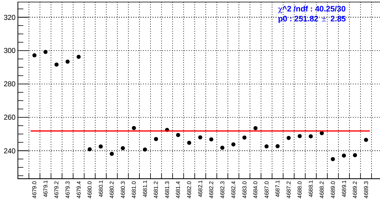
slug74-Left: reg_asym_at2_avg.rms/ppm
