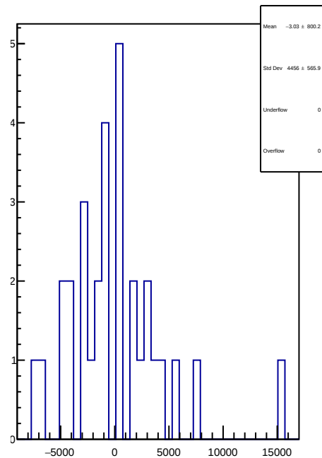
slug74-Left: 1D Corr asym_ds_dd.mean/ppb-reg_asym_ds_dd.mean/ppb
