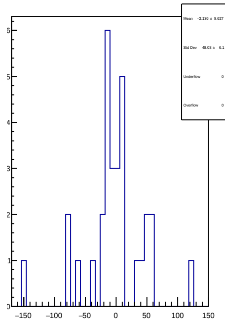
slug74-Left: 1D Corr asym_atr1.mean/ppb-reg_asym_atr1.mean/ppb
