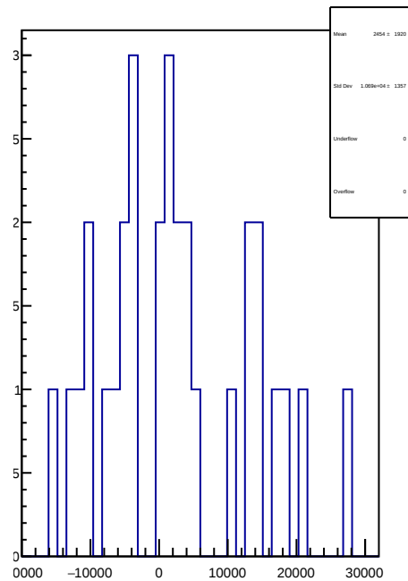
slug74-Left: 1D Corr asym_at1_avg.mean/ppb-reg_asym_at1_avg.mean/ppb
