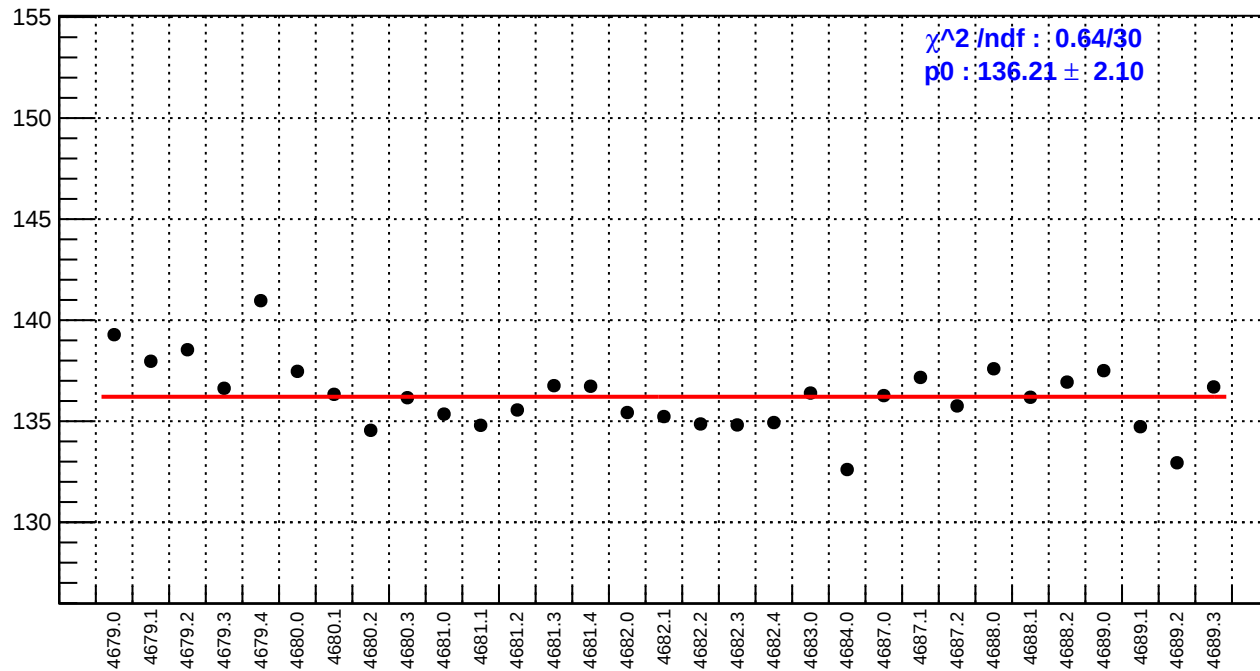
slug74-Left: reg_asym_left_avg.rms/ppm
