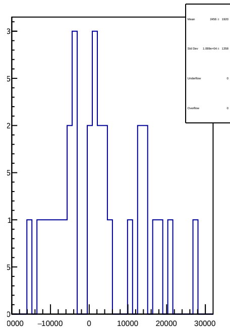
slug74-Left: 1D Corr asym_at1_dd.mean/ppb-reg_asym_at1_dd.mean/ppb
