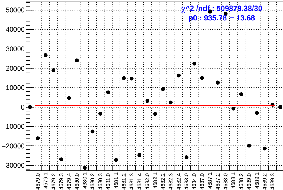
slug74-Left: asym_atr1l2_avg.mean/ppb-reg_asym_atr1l2_avg.mean/ppb
