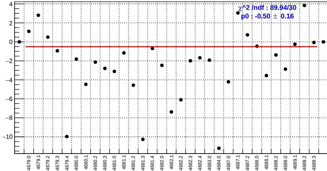
slug74-Left: usl_bpm4eY/(ppb/nm)
