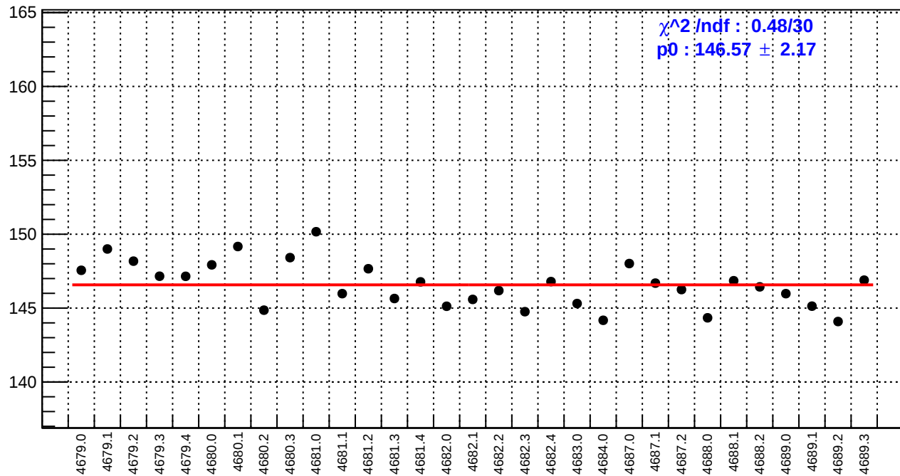
slug74-Left: reg_asym_ds_dd.rms/ppm
