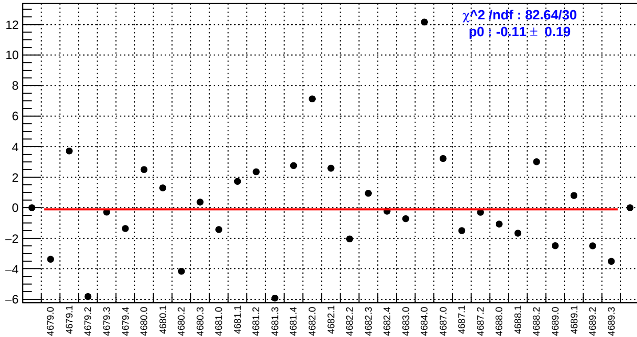
slug74-Left: dsr_bpm4aY/(ppb/nm)
