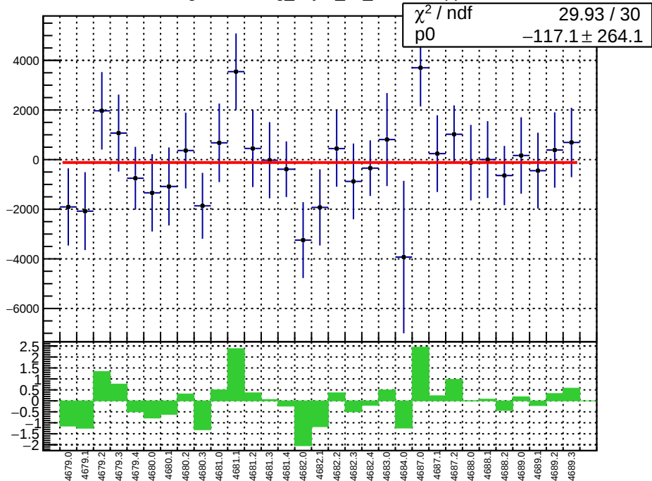
slug74-Left: reg_asym_ds_dd.mean/ppb
