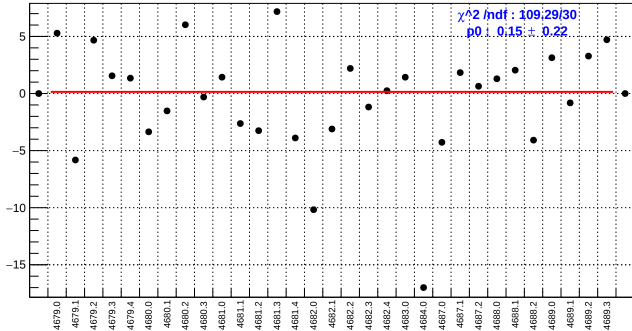
slug74-Left: dsr_bpm4eY/(ppb/nm)
