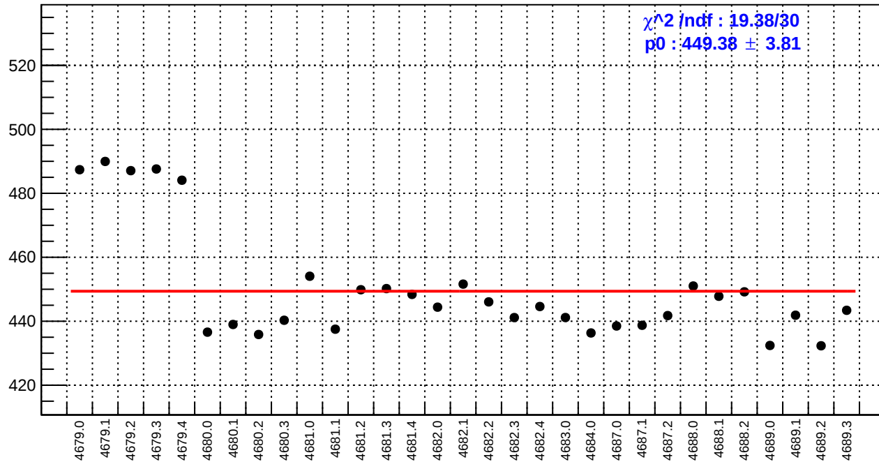
slug74-Left: reg_asym_atl_avg.rms/ppm
