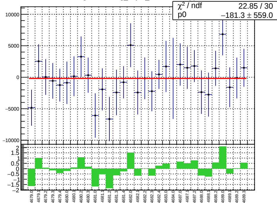
slug74-Left: reg_asym_sam5.mean/ppb
