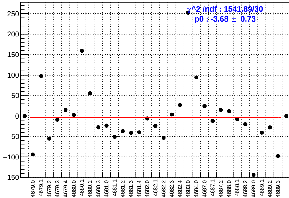
slug74-Left: asym_right_dd.mean/ppb-reg_asym_right_dd.mean/ppb
