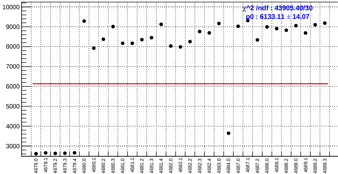
slug74-Left: diff_bpm4eY.rms/nm
