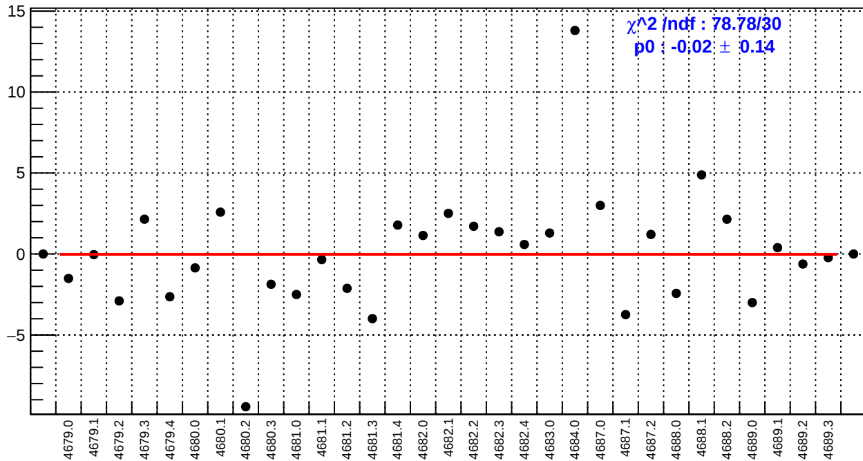
slug74-Left: right_avg_bpm4aY/(ppb/nm)
