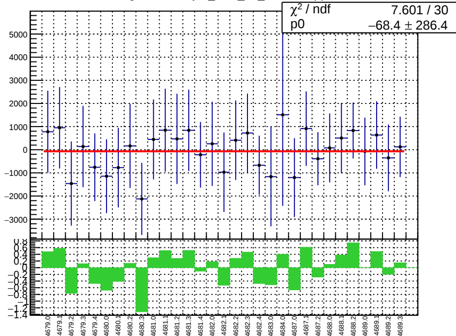
slug74-Left: asym_bcm_an_ds.mean/ppb
