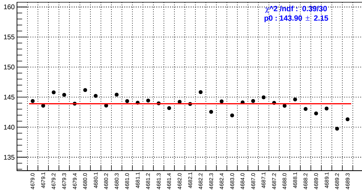
slug74-Left: reg_asym_atr1.rms/ppm
