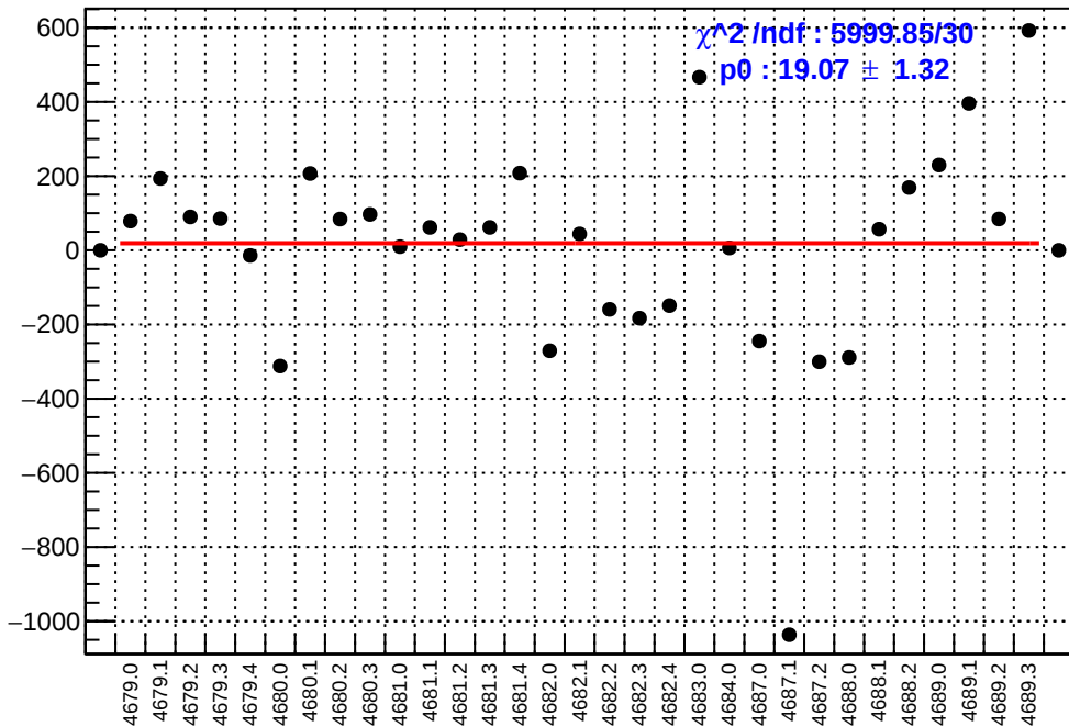
slug74-Left: asym_left_dd.mean/ppb-reg_asym_left_dd.mean/ppb
