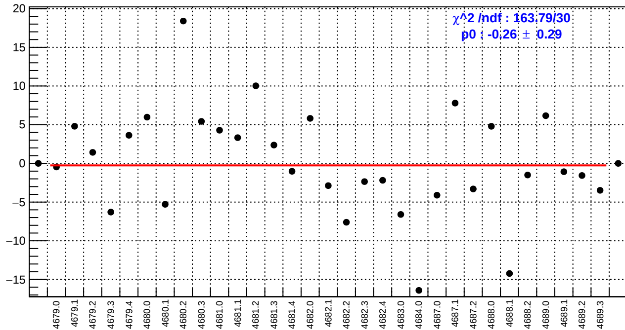
slug74-Left: usr_bpm4eY/(ppb/nm)
