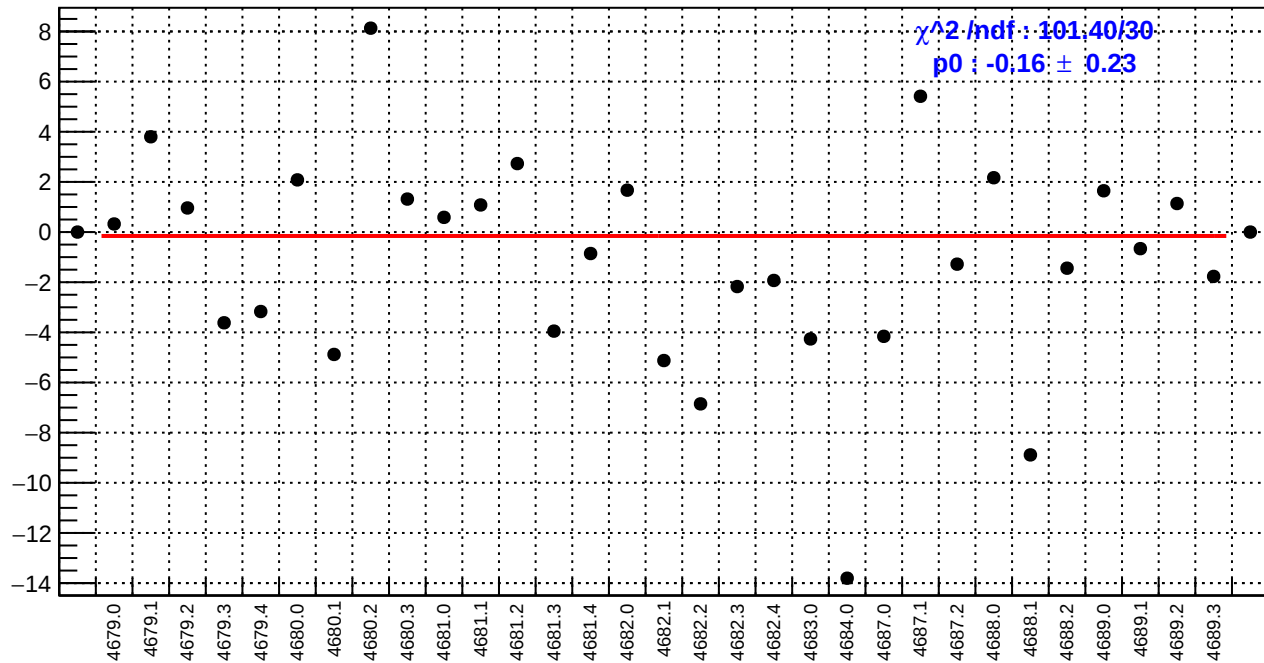
slug74-Left: us_avg_bpm4eY/(ppb/nm)
