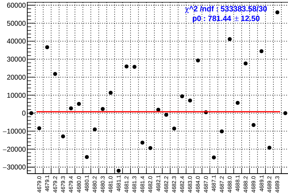
slug74-Left: asym_atl1.mean/ppb-reg_asym_atl1.mean/ppb
