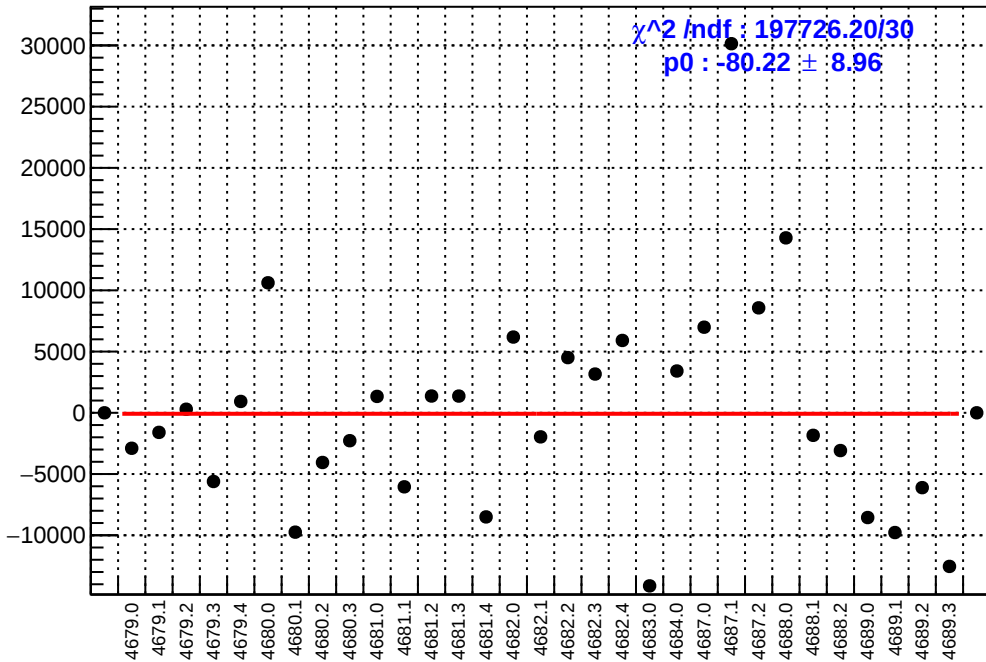
slug74-Left: asym_left_avg.mean/ppb-reg_asym_left_avg.mean/ppb
