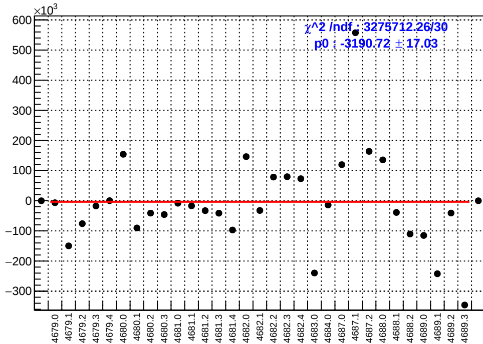
slug74-Left: asym_sam3.mean/ppb-reg_asym_sam3.mean/ppb
