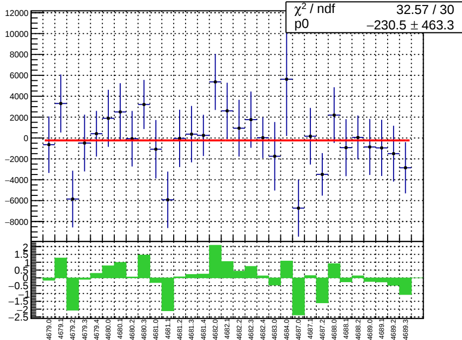
slug74-Left: reg_asym_dsr.mean/ppb
