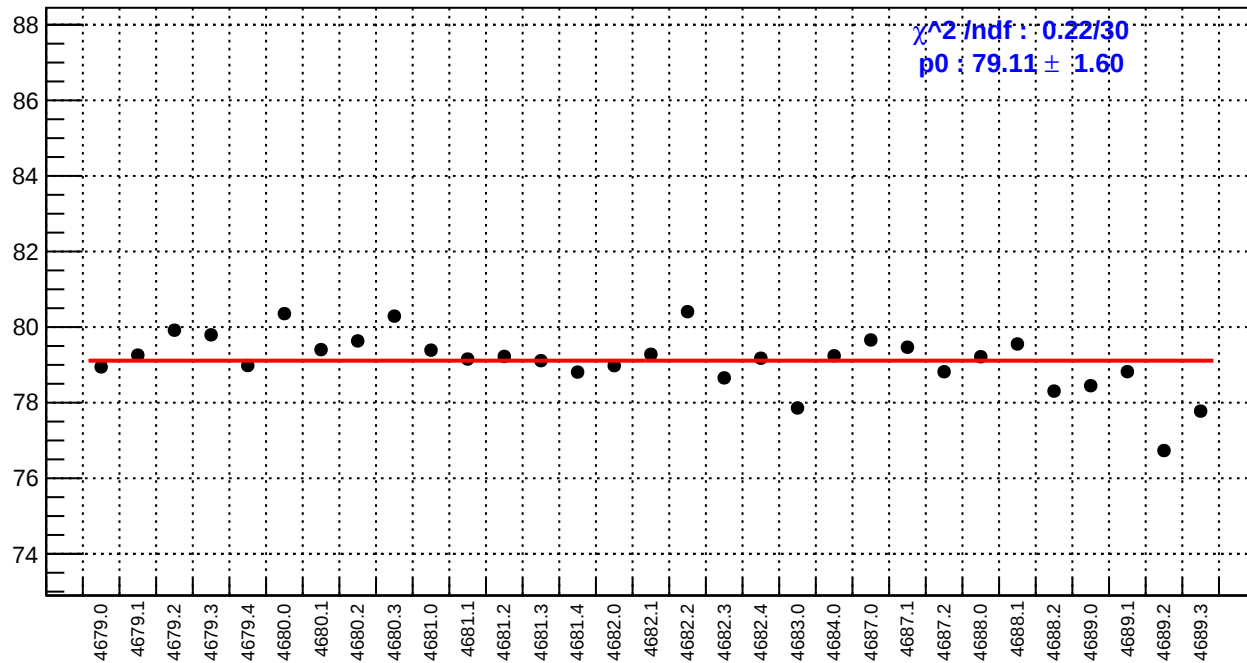
slug74-Left: reg_asym_atr_avg.rms/ppm
