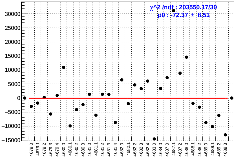
slug74-Left: asym_dsl.mean/ppb-reg_asym_dsl.mean/ppb
