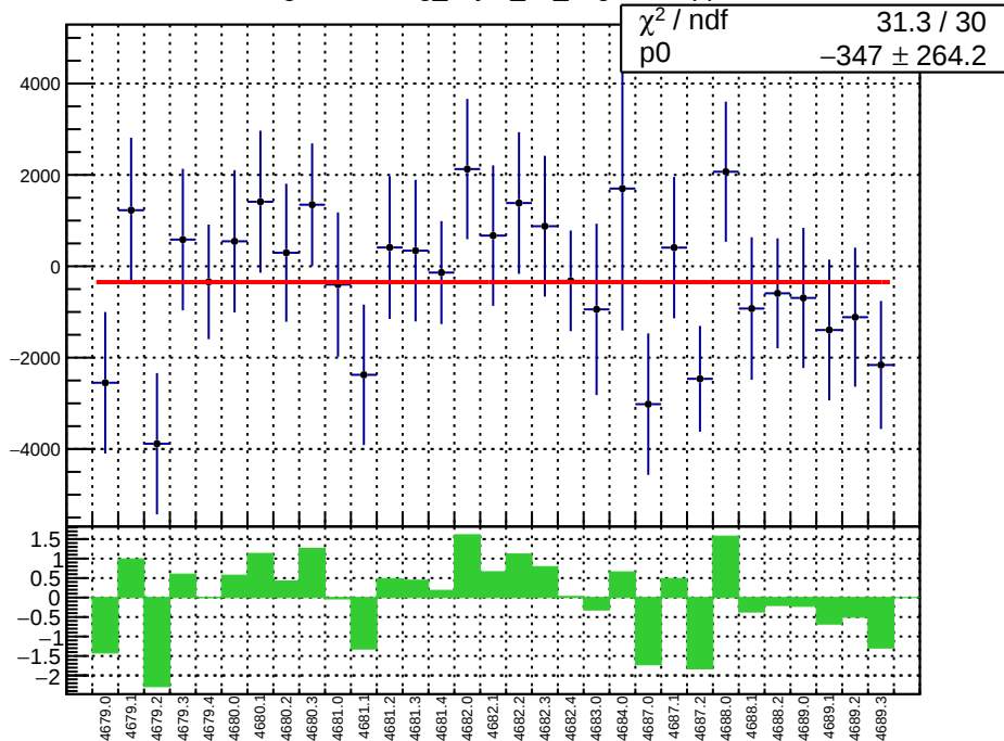
slug74-Left: reg_asym_ds_avg.mean/ppb
