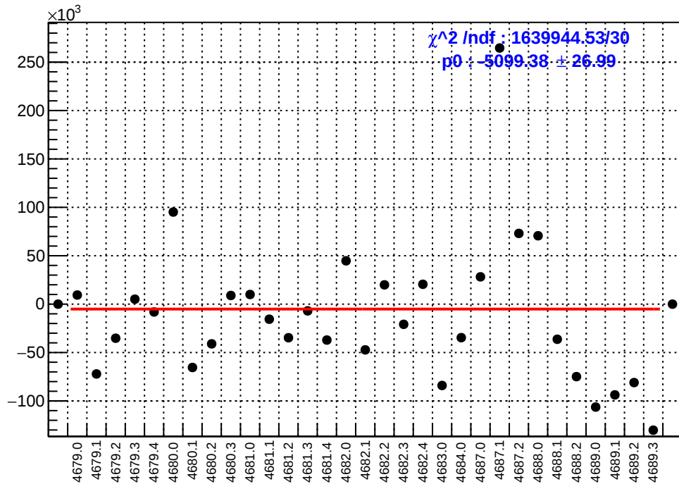
slug74-Left: asym_sam4.mean/ppb-reg_asym_sam4.mean/ppb
