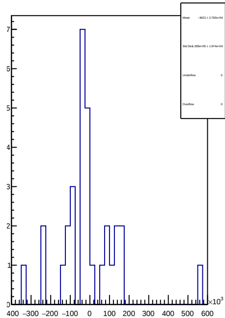
slug74-Left: 1D Corr asym_sam3.mean/ppb-reg_asym_sam3.mean/ppb
