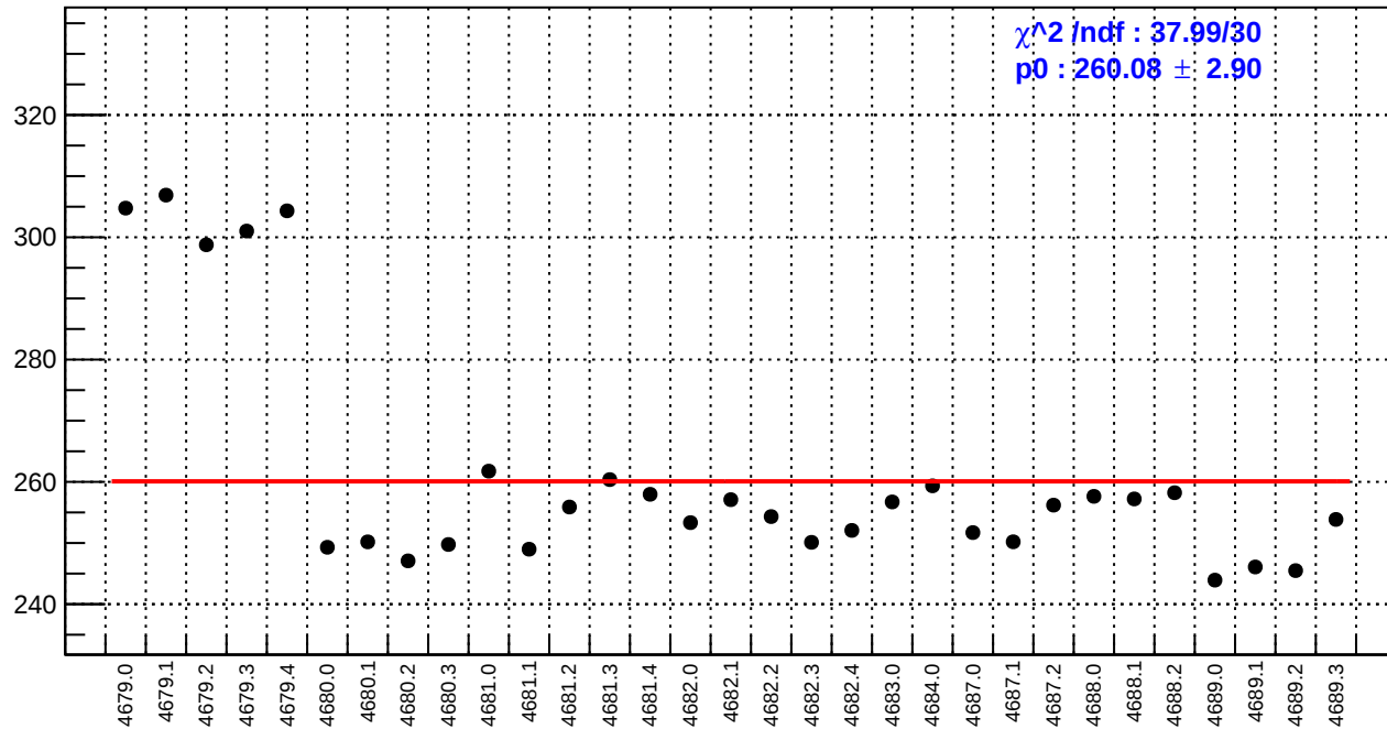
slug74-Left: reg_asym_atr1l2_avg.rms/ppm
