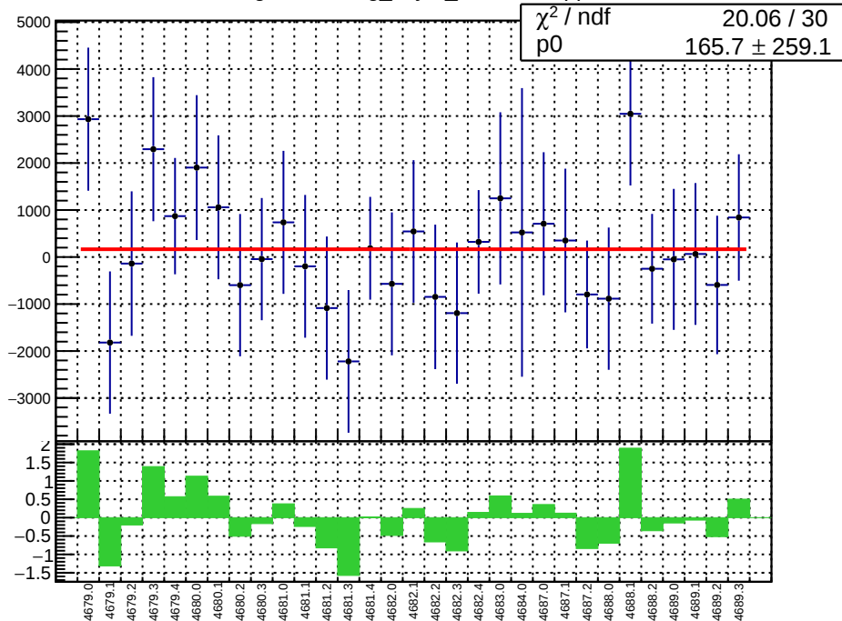
slug74-Left: reg_asym_atr1.mean/ppb
