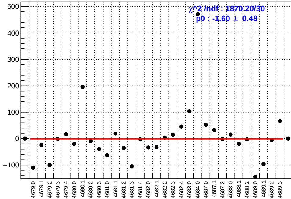
slug74-Left: asym_right_avg.mean/ppb-reg_asym_right_avg.mean/ppb
