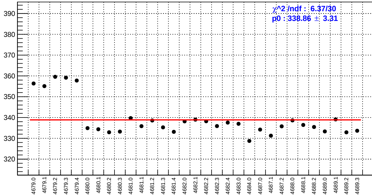
slug74-Left: reg_asym_at1_dd.rms/ppm
