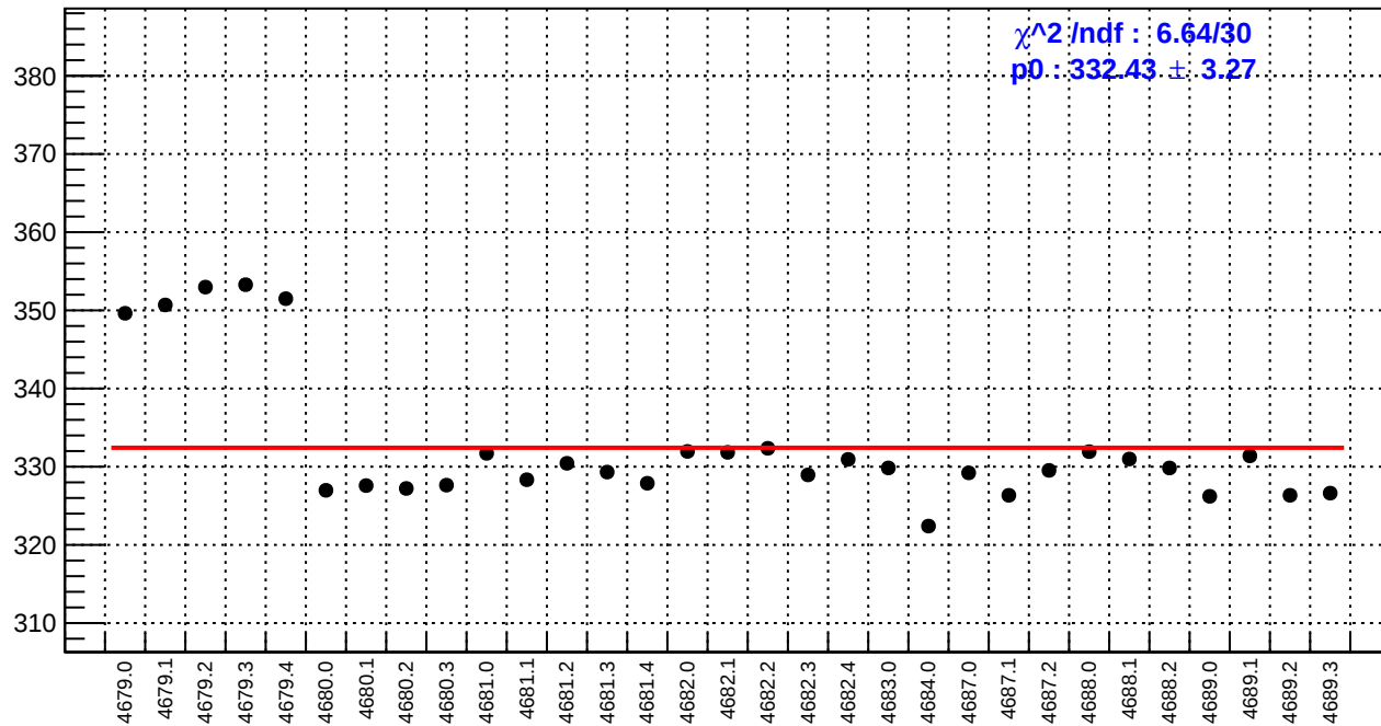
slug74-Left: reg_asym_atl1r2_avg.rms/ppm
