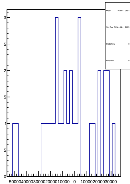
slug74-Left: 1D Corr asym_at2_dd.mean/ppb-reg_asym_at2_dd.mean/ppb
