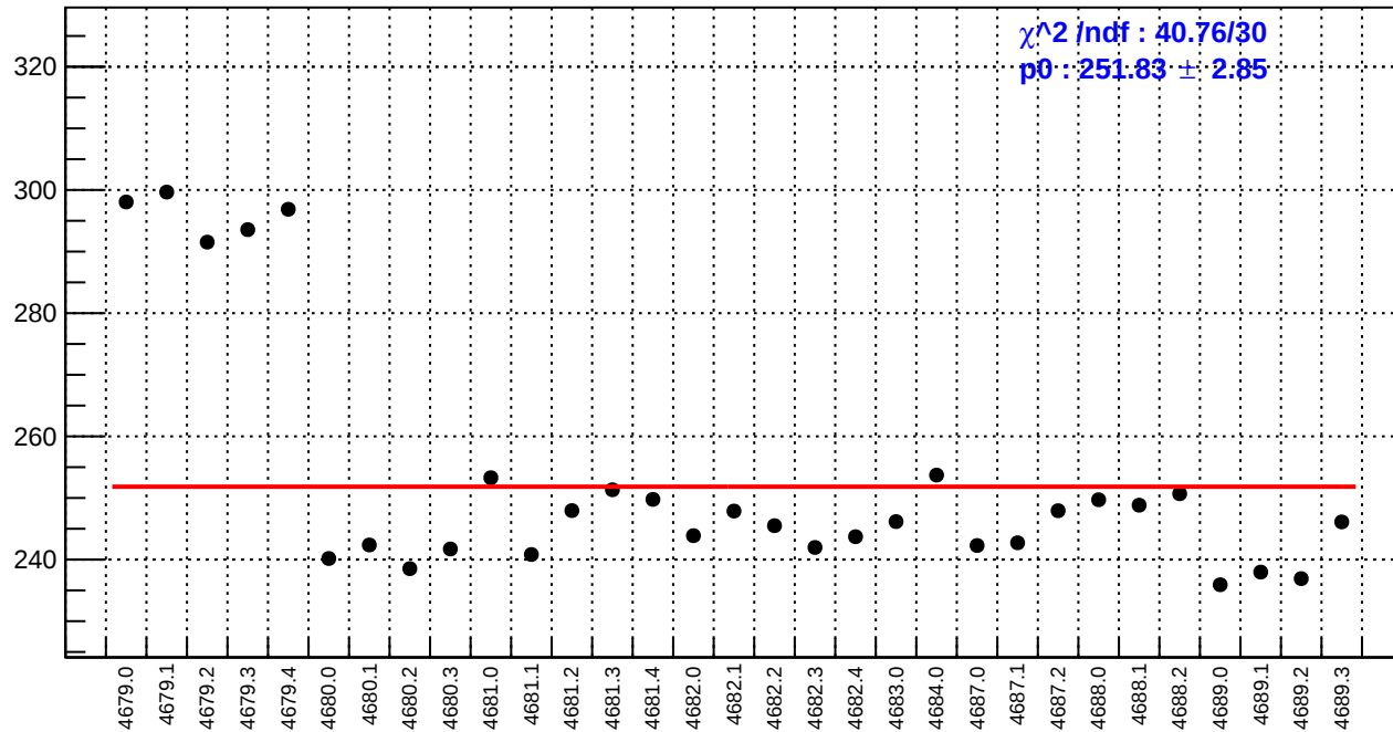
slug74-Left: reg_asym_at2_dd.rms/ppm
