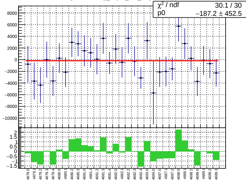
slug74-Left: reg_asym_at2_avg.mean/ppb
