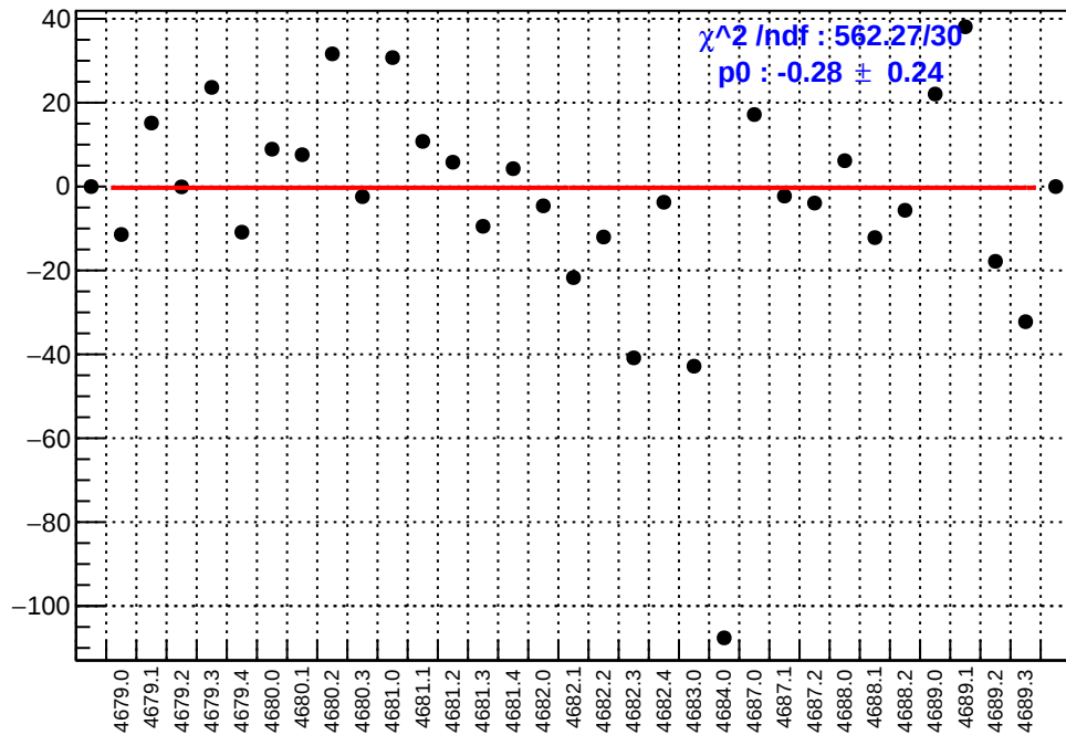
slug74-Left: asym_atr_avg.mean/ppb-reg_asym_atr_avg.mean/ppb
