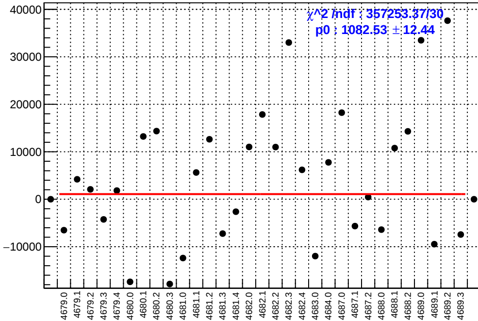
slug74-Left: asym_sam1.mean/ppb-reg_asym_sam1.mean/ppb
