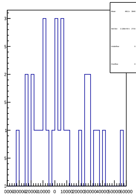
slug74-Left: 1D Corr asym_atl1.mean/ppb-reg_asym_atl1.mean/ppb
