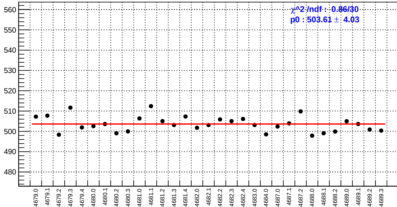
slug74-Left: reg_asym_usr.rms/ppm
