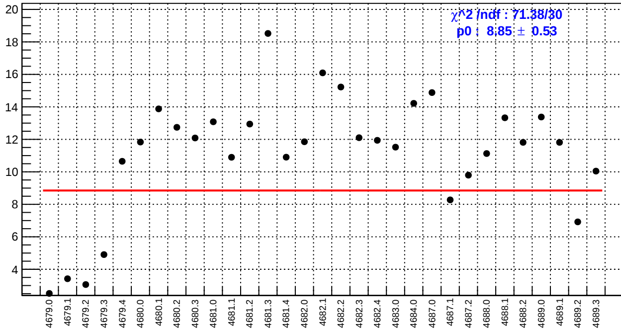
slug74-Left: dsl_bpm4aY/(ppb/nm)
