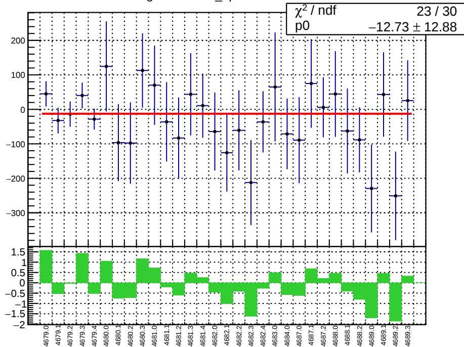
slug74-Left: diff_bpm4aY.mean/nm
