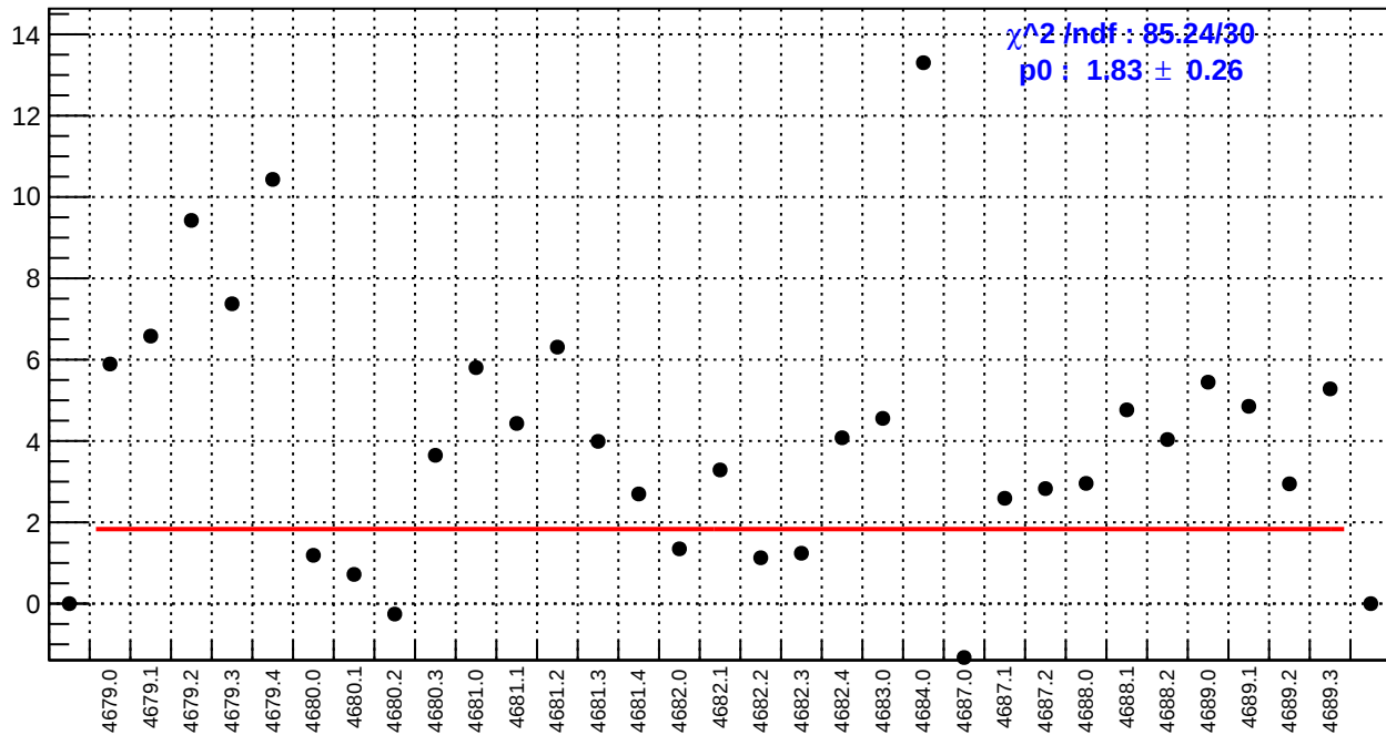
slug74-Left: ds_avg_bpm4aX/(ppb/nm)
