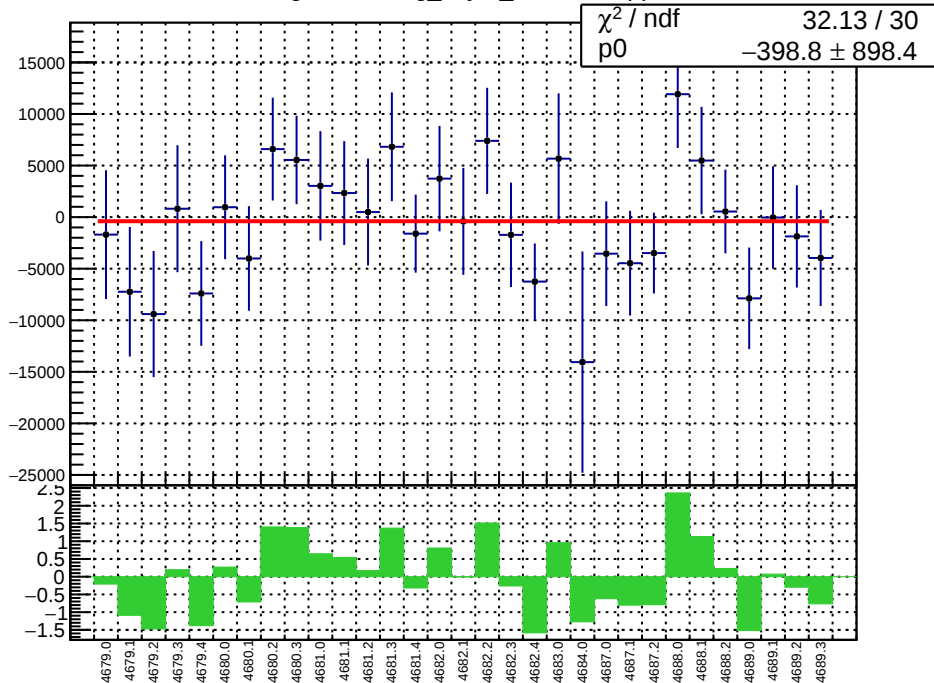
slug74-Left: reg_asym_atl2.mean/ppb
