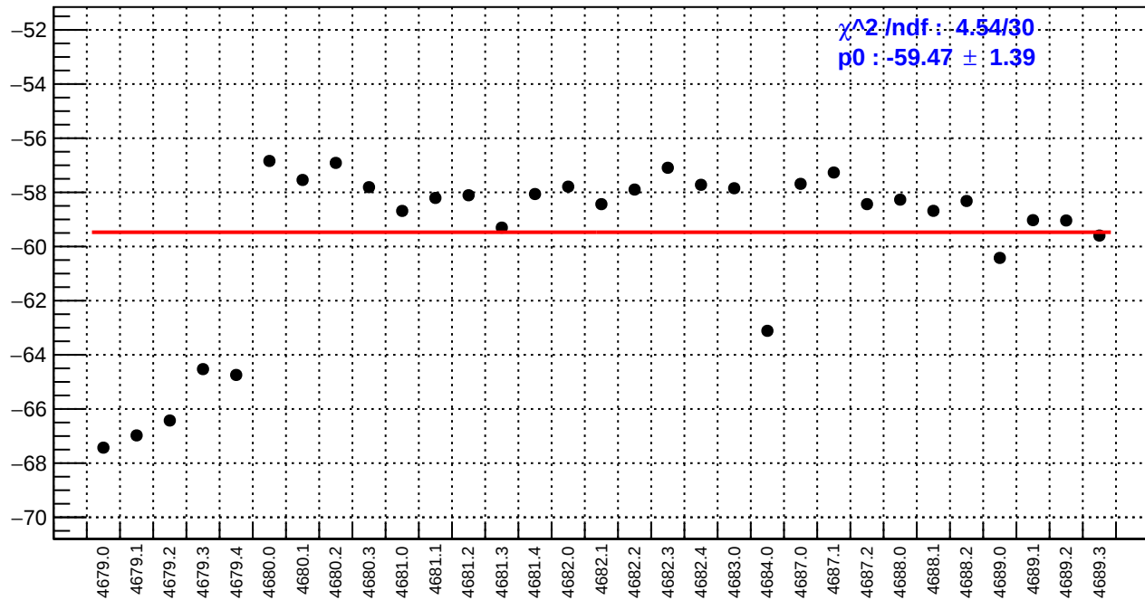
slug74-Left: left_avg_bpm4eX/(ppb/nm)
