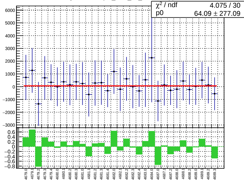
slug74-Left: asym_bcm_an_us.mean/ppb
