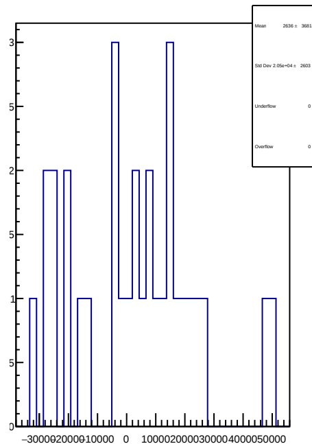
slug74-Left: 1D Corr asym_atr1l2_avg.mean/ppb-reg_asym_atr1l2_avg.mean/ppb
