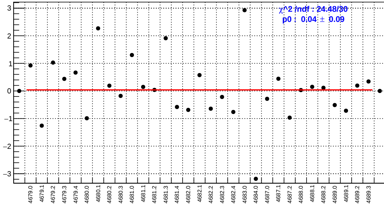
slug74-Left: usr_bpm12X/(ppb/nm)
