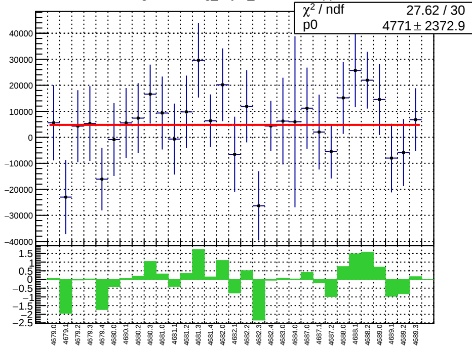
slug74-Left: reg_asym_sam4.mean/ppb
