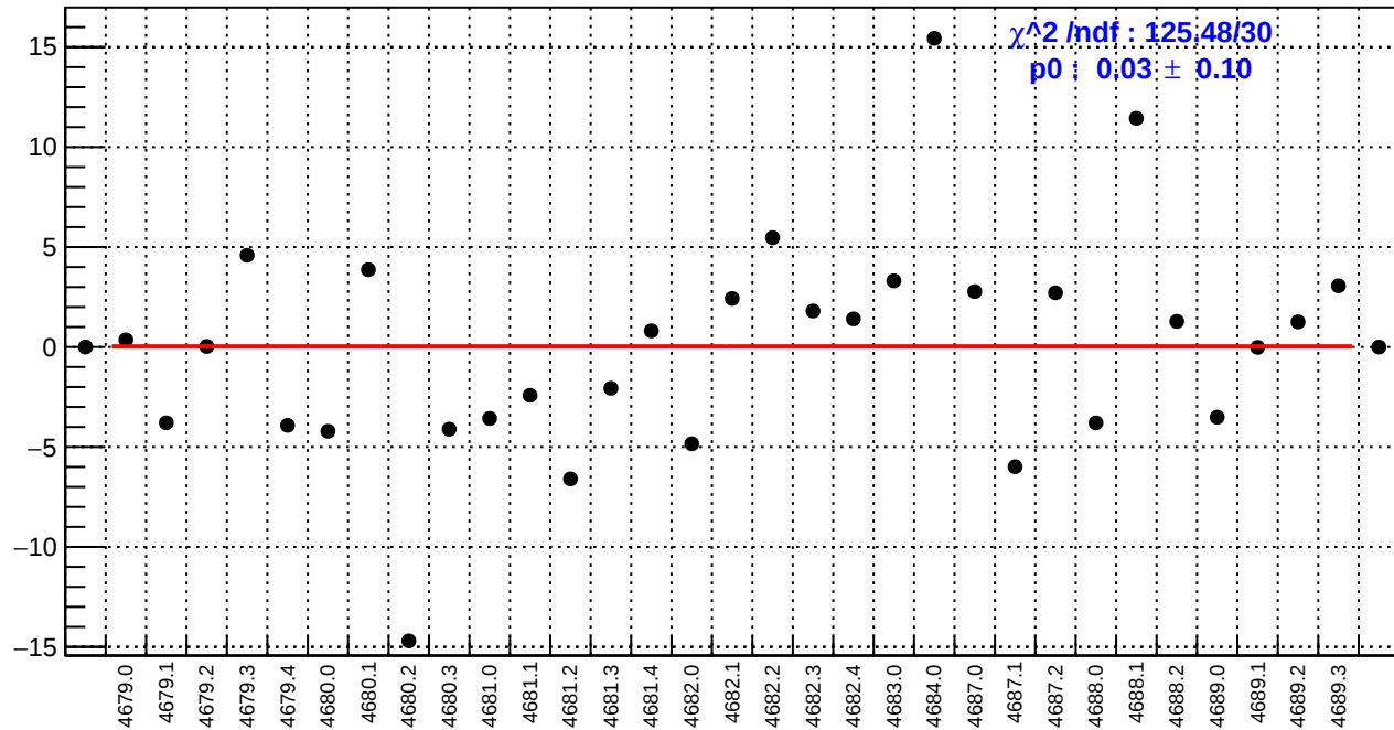
slug74-Left: usr_bpm4aY/(ppb/nm)
