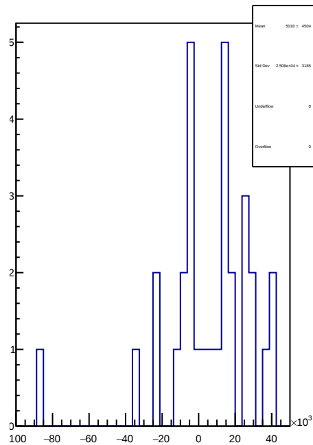
slug74-Left: 1D Corr asym_sam8.mean/ppb-reg_asym_sam8.mean/ppb
