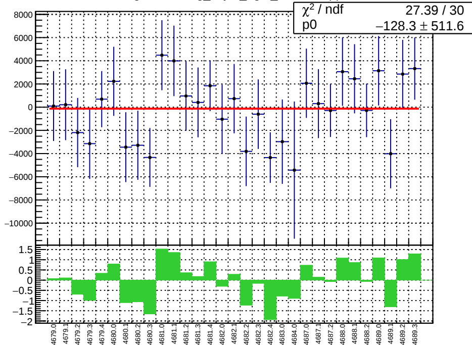
slug74-Left: reg_asym_right_dd.mean/ppb
