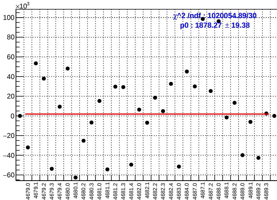
slug74-Left: asym_atl2.mean/ppb-reg_asym_atl2.mean/ppb
