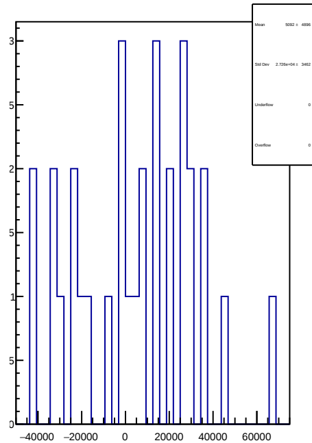
slug74-Left: 1D Corr asym_atl_avg.mean/ppb-reg_asym_atl_avg.mean/ppb
