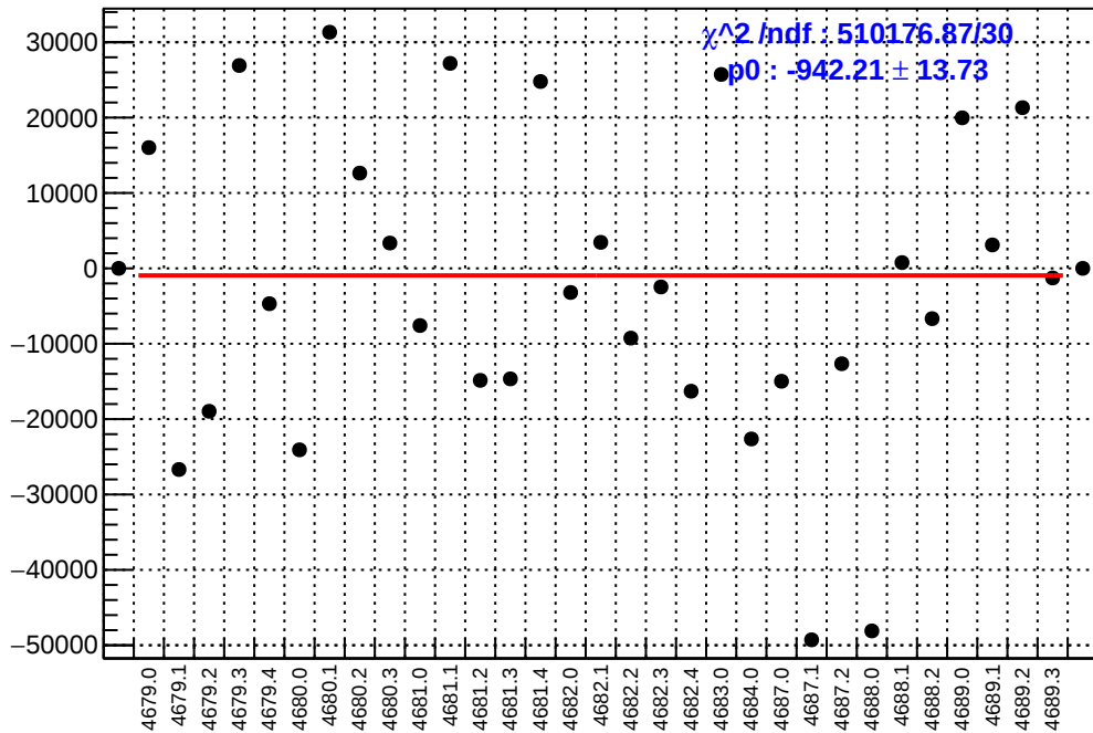
slug74-Left: asym_atr1l2_dd.mean/ppb-reg_asym_atr1l2_dd.mean/ppb
