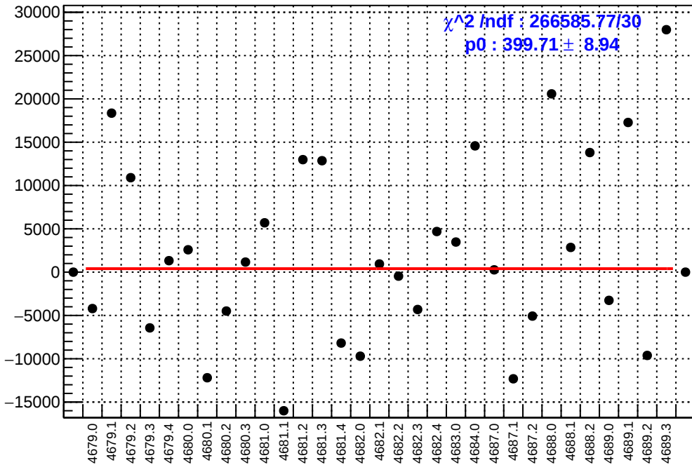
slug74-Left: asym_at1_avg.mean/ppb-reg_asym_at1_avg.mean/ppb
