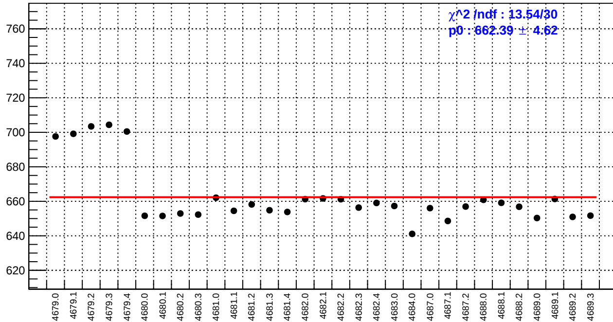
slug74-Left: reg_asym_atl1.rms/ppm
