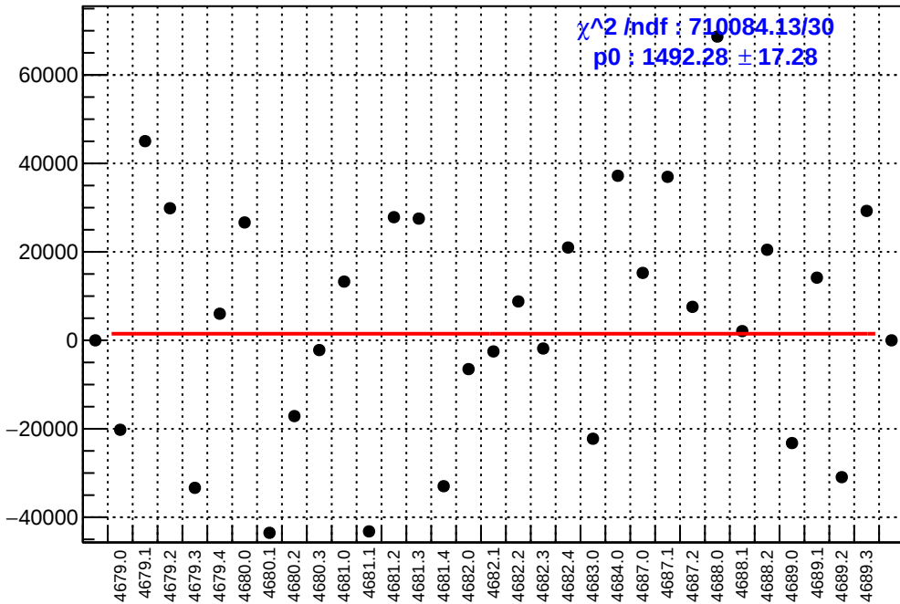
slug74-Left: asym_atl_avg.mean/ppb-reg_asym_atl_avg.mean/ppb
