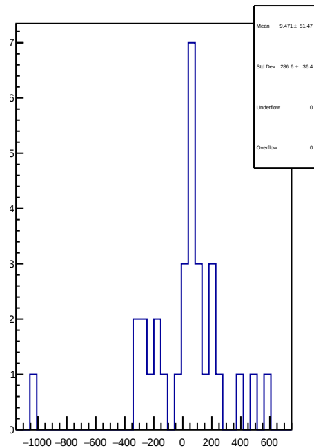
slug74-Left: 1D Corr asym_left_dd.mean/ppb-reg_asym_left_dd.mean/ppb
