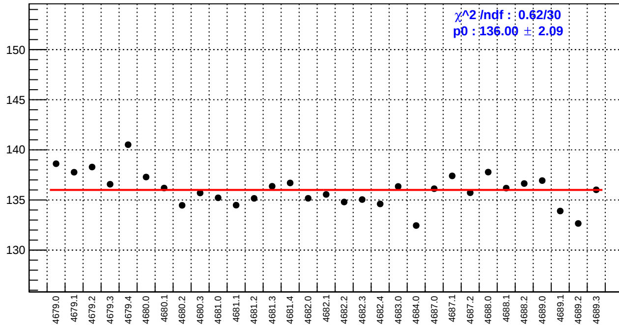
slug74-Left: reg_asym_usl.rms/ppm
