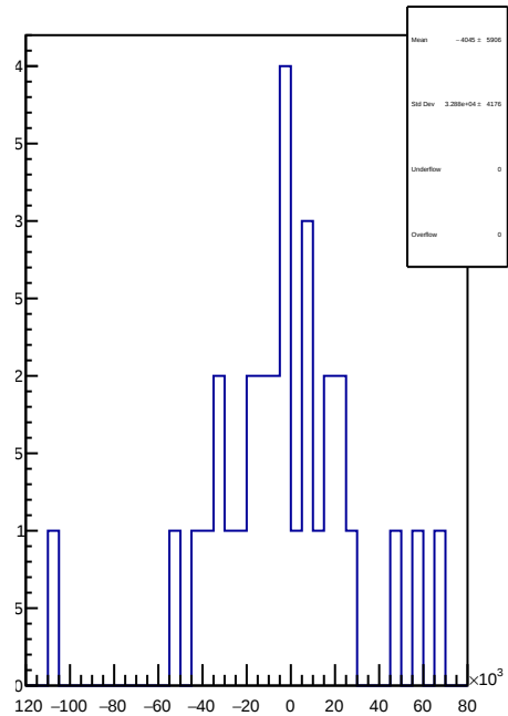
slug74-Left: 1D Corr asym_sam6.mean/ppb-reg_asym_sam6.mean/ppb
