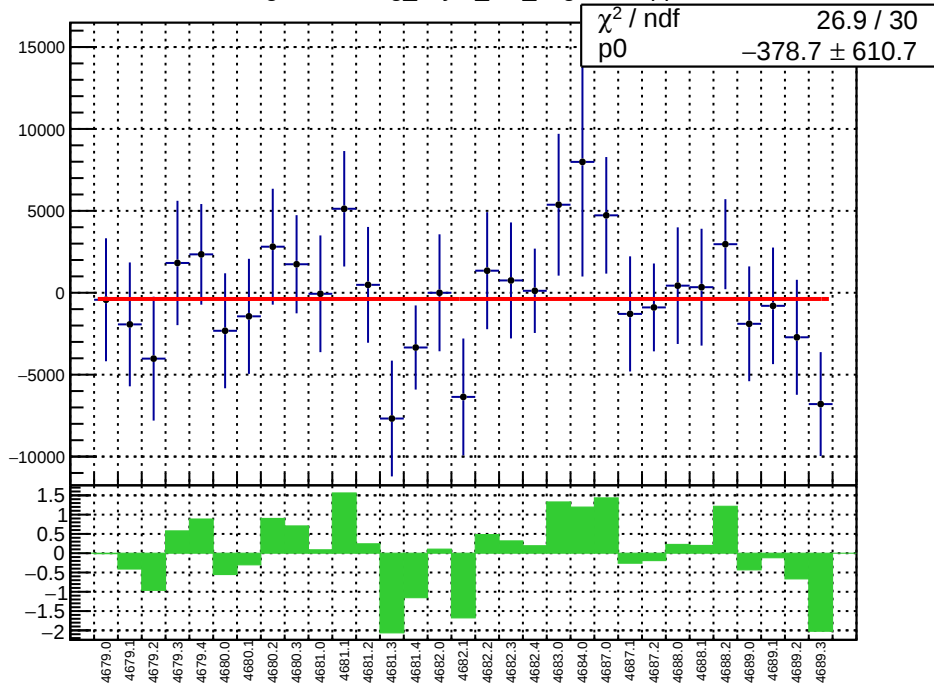
slug74-Left: reg_asym_at1_avg.mean/ppb
