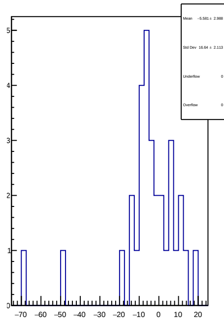
slug74-Left: 1D Corr asym_atr2.mean/ppb-reg_asym_atr2.mean/ppb
