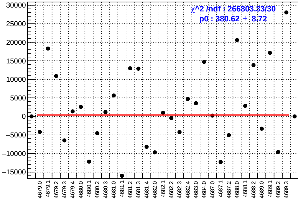
slug74-Left: asym_at1_dd.mean/ppb-reg_asym_at1_dd.mean/ppb
