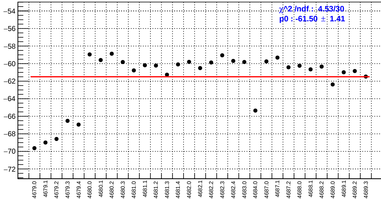
slug74-Left: dsl_bpm4eX/(ppb/nm)
