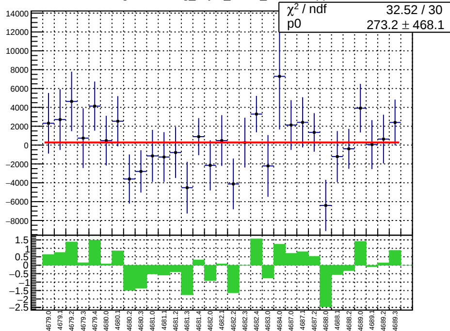
slug74-Left: reg_asym_atr1l2_dd.mean/ppb
