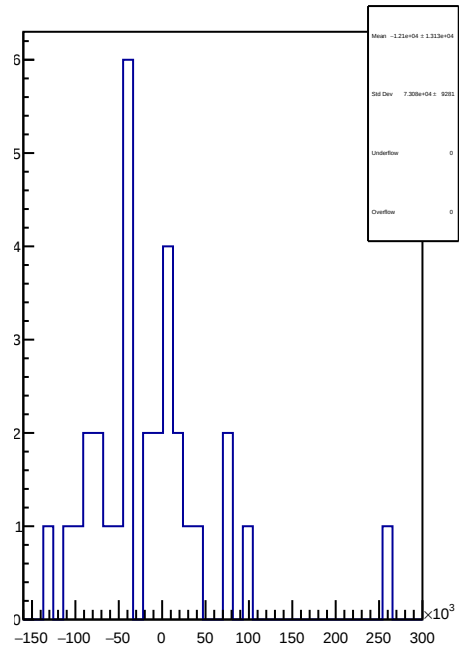
slug74-Left: 1D Corr asym_sam4.mean/ppb-reg_asym_sam4.mean/ppb
