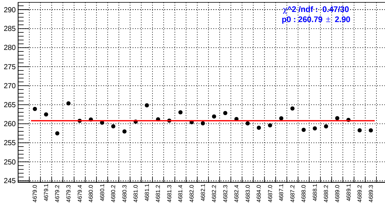
slug74-Left: reg_asym_us_avg.rms/ppm
