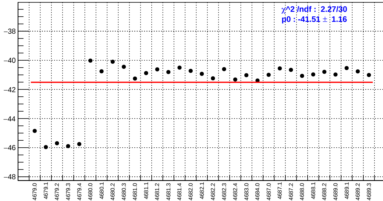
slug74-Left: left_avg_bpm12X/(ppb/nm)
