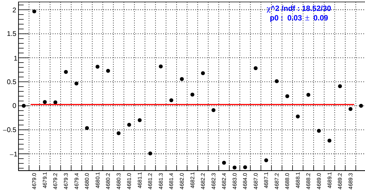
slug74-Left: dsr_bpm4eX/(ppb/nm)
