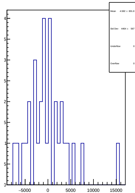
slug74-Left: 1D Corr asym_ds_avg.mean/ppb-reg_asym_ds_avg.mean/ppb
