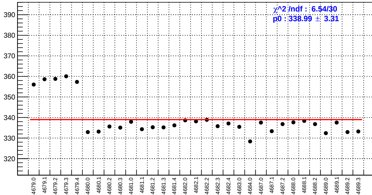
slug74-Left: reg_asym_at1_avg.rms/ppm
