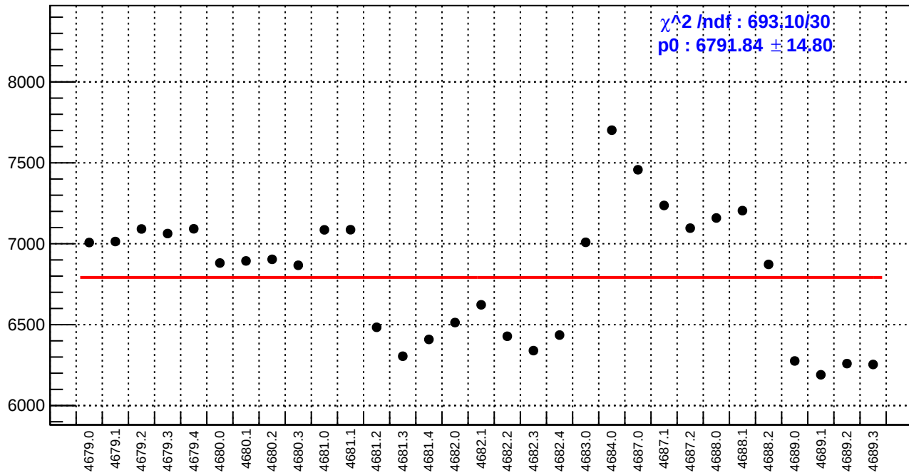
slug74-Left: diff_bpm11X.rms/nm
