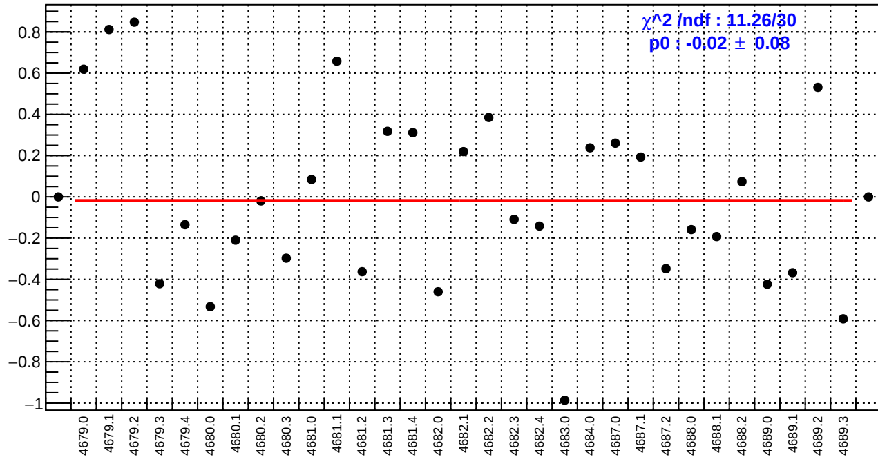
slug74-Left: dsr_bpm12X/(ppb/nm)
