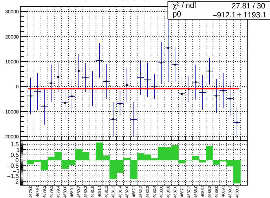
slug74-Left: reg_asym_atl1.mean/ppb
