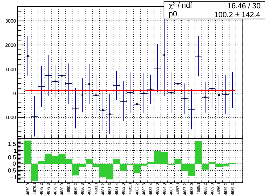
slug74-Left: reg_asym_atr_avg.mean/ppb
