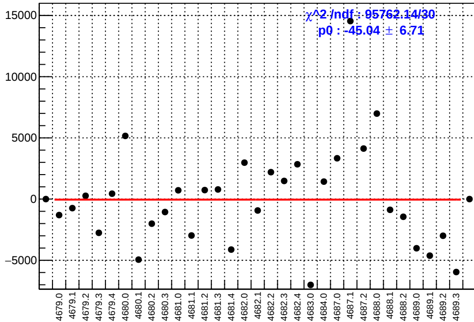
slug74-Left: asym_us_dd.mean/ppb-reg_asym_us_dd.mean/ppb
