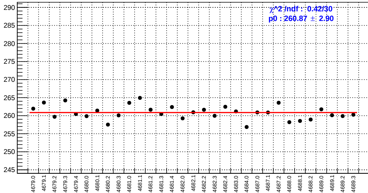
slug74-Left: reg_asym_us_dd.rms/ppm
