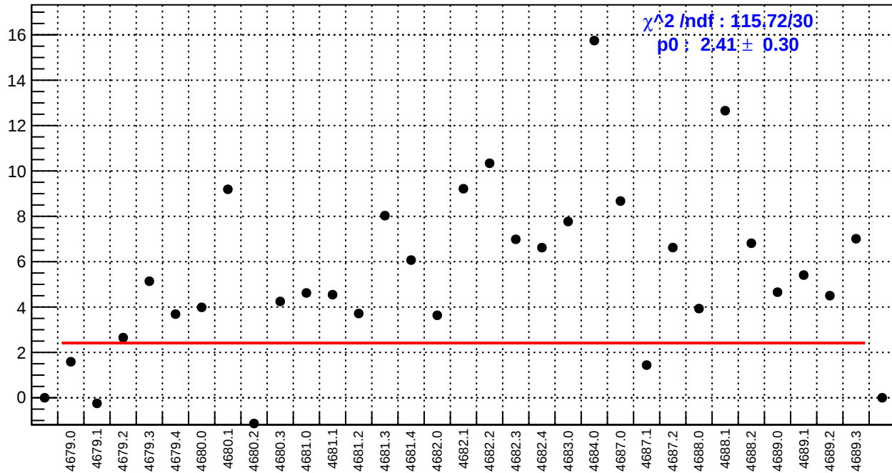
slug74-Left: us_avg_bpm4aY/(ppb/nm)
