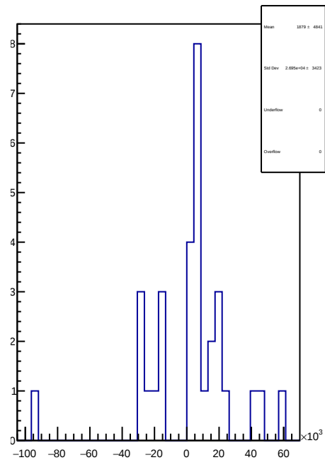
slug74-Left: 1D Corr asym_sam7.mean/ppb-reg_asym_sam7.mean/ppb
