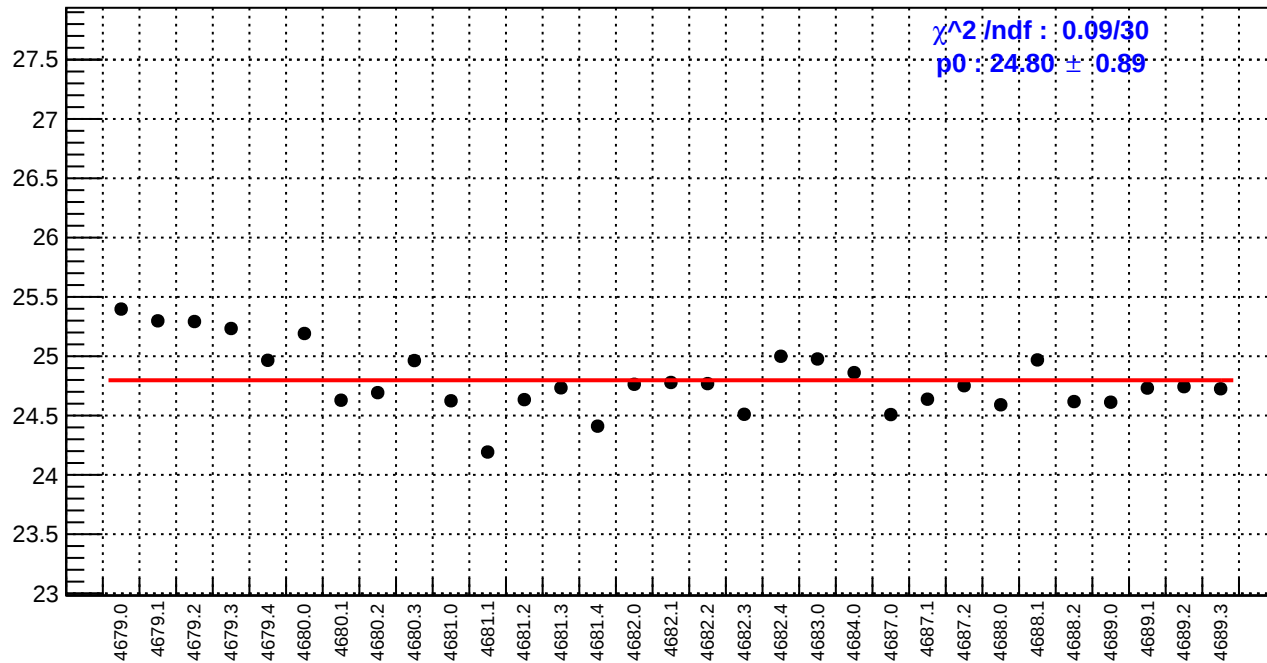
slug74-Left: reg_asym_left_dd.rms/ppm
