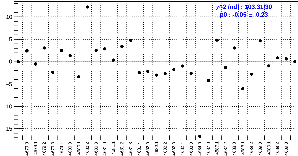
slug74-Left: right_avg_bpm4eY/(ppb/nm)
