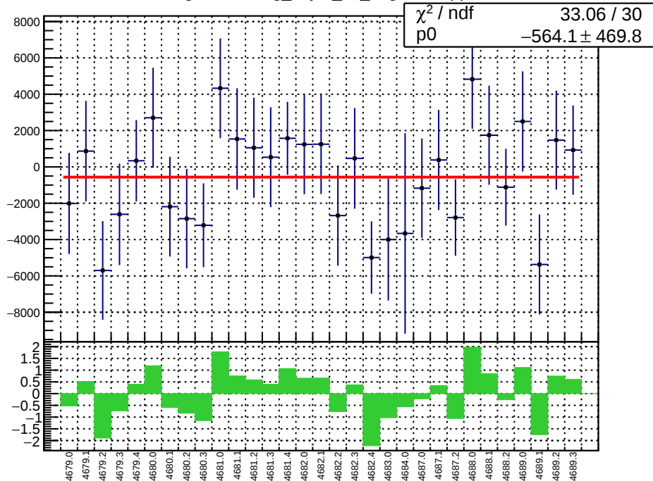
slug74-Left: reg_asym_us_avg.mean/ppb
