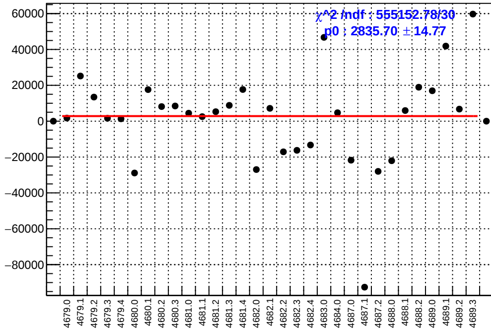
slug74-Left: asym_sam7.mean/ppb-reg_asym_sam7.mean/ppb
