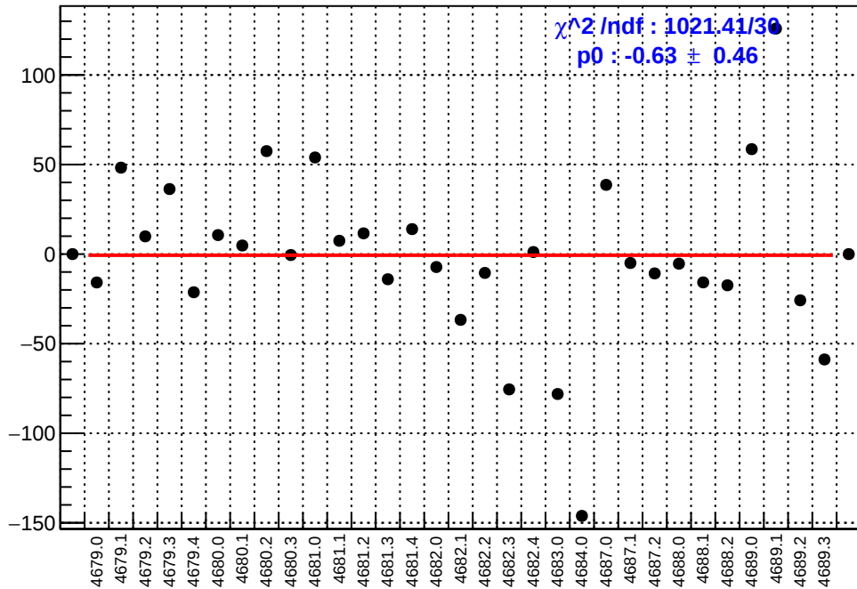
slug74-Left: asym_atr1.mean/ppb-reg_asym_atr1.mean/ppb
