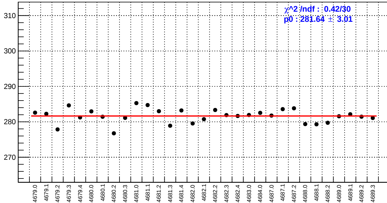
slug74-Left: reg_asym_right_avg.rms/ppm
