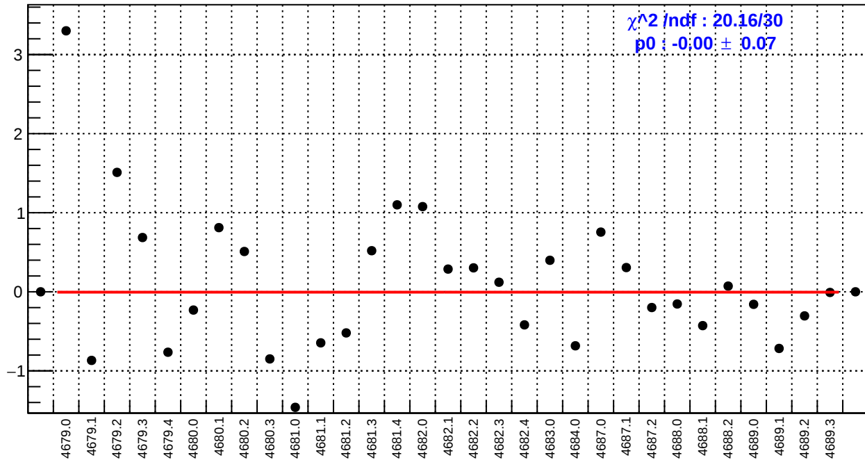
slug74-Left: right_avg_bpm4eX/(ppb/nm)
