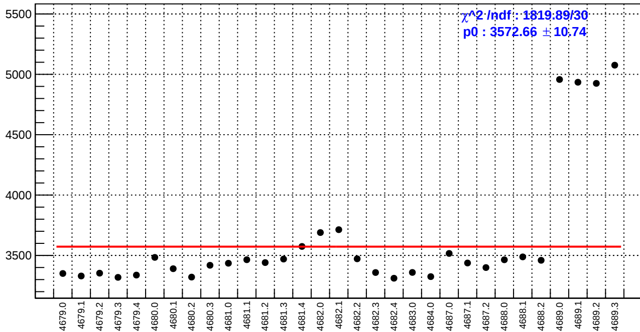
slug74-Left: diff_bpm4aX.rms/nm
