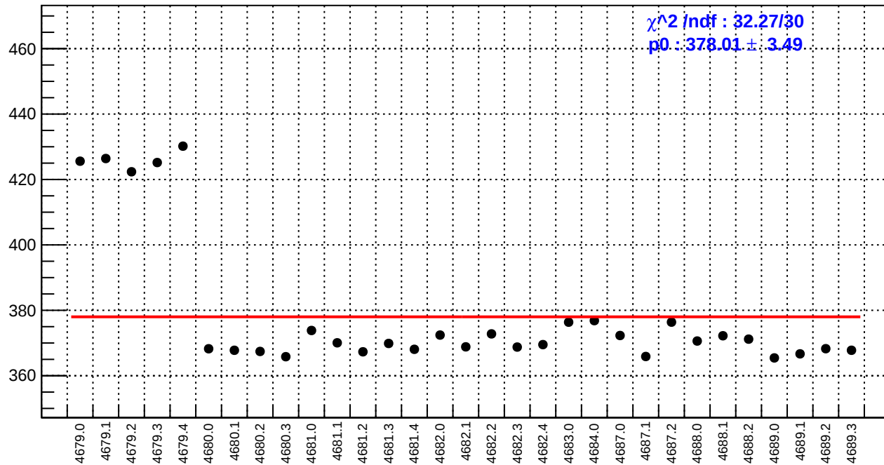
slug74-Left: reg_asym_atl_dd.rms/ppm
