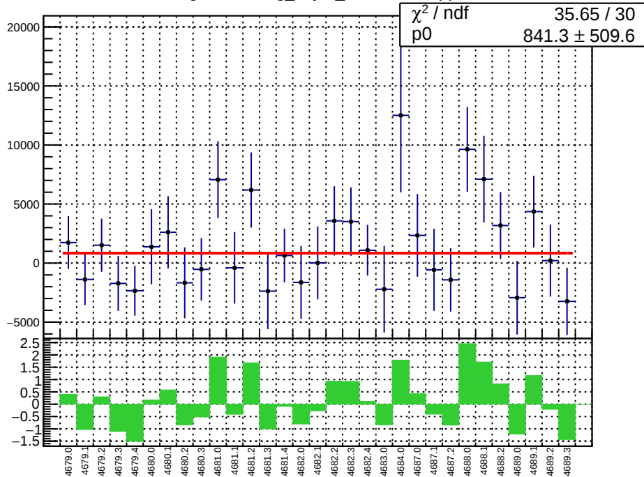
slug74-Left: reg_asym_sam1.mean/ppb
