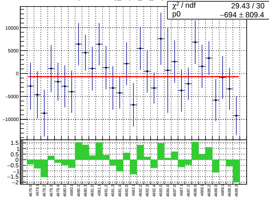
slug74-Left: reg_asym_atl_avg.mean/ppb
