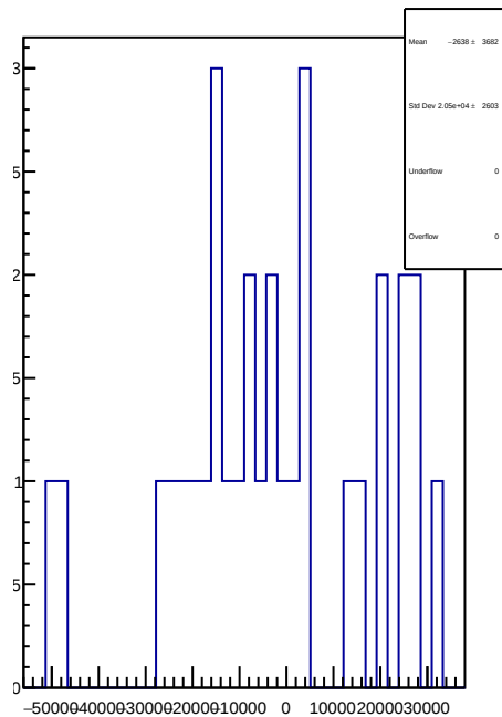
slug74-Left: 1D Corr asym_atr1l2_dd.mean/ppb-reg_asym_atr1l2_dd.mean/ppb
