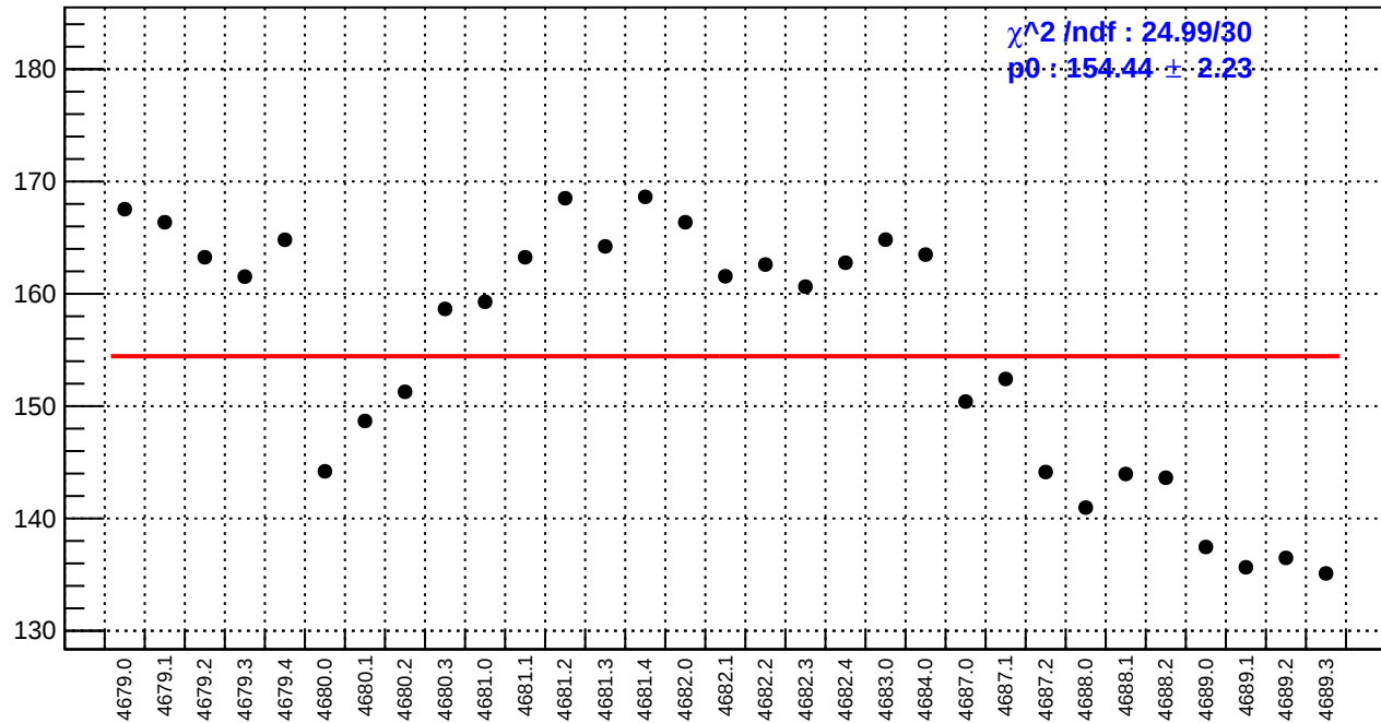
slug74-Left: asym_bcm_an_us.rms/ppm
