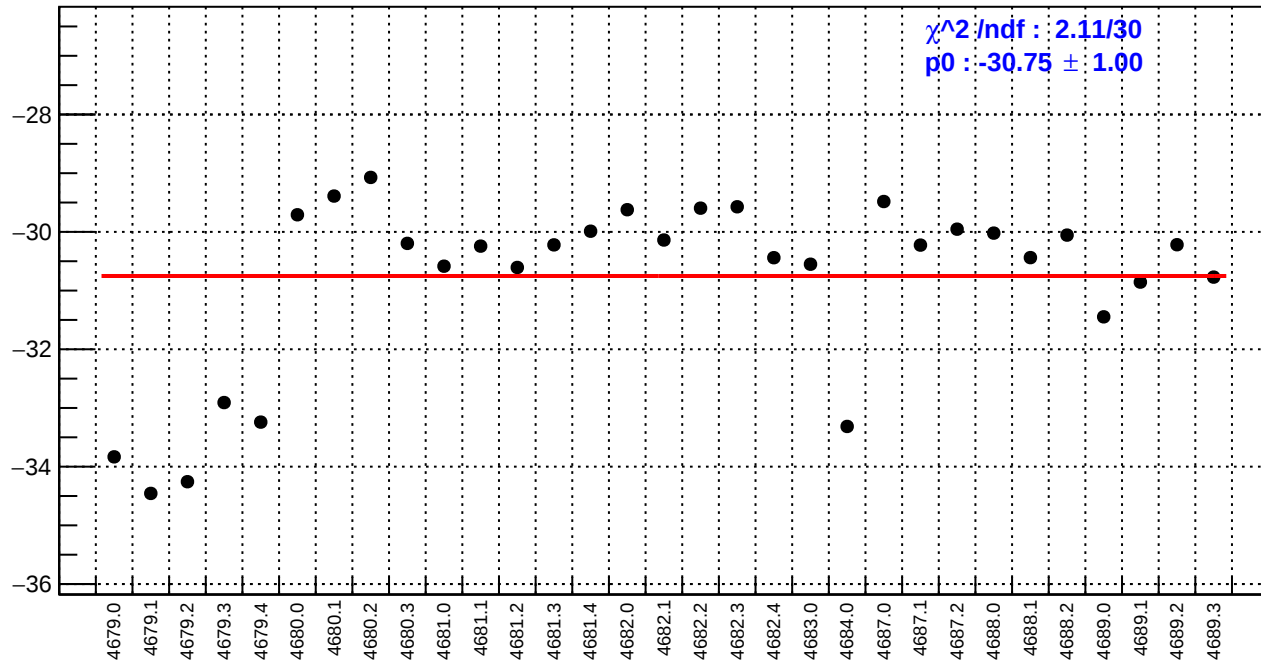
slug74-Left: ds_avg_bpm4eX/(ppb/nm)
