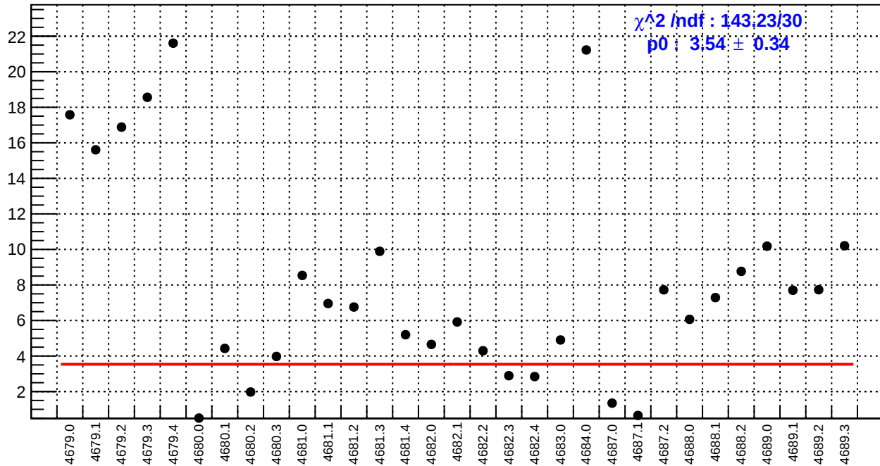
slug74-Left: left_avg_bpm4aX/(ppb/nm)
