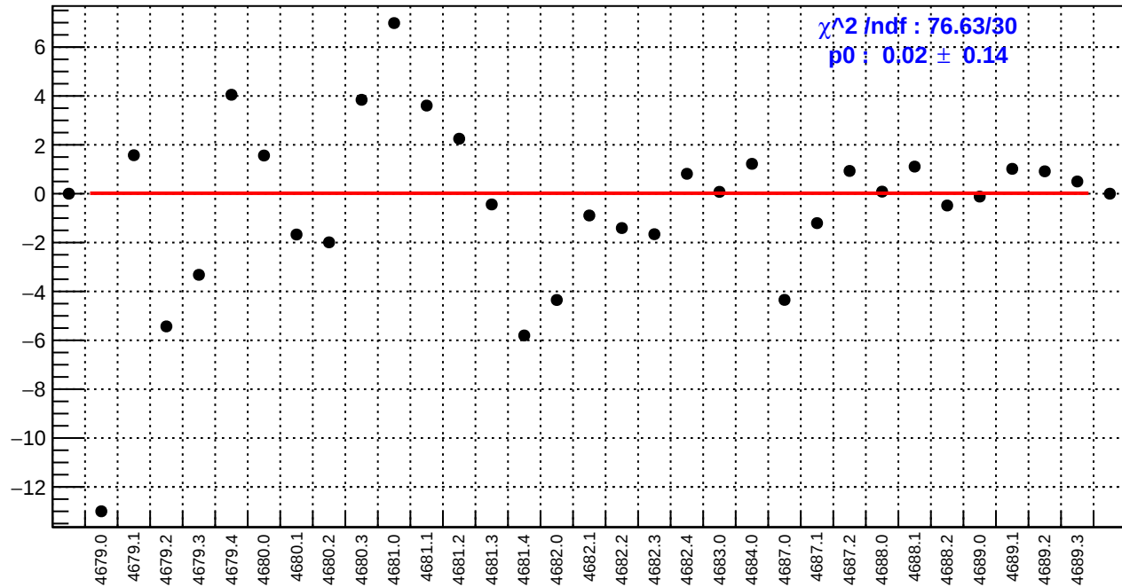
slug74-Left: right_avg_bpm4aX/(ppb/nm)
