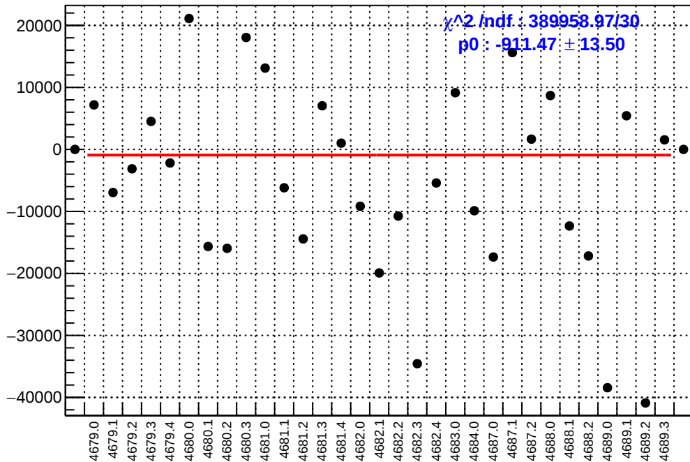
slug74-Left: asym_sam5.mean/ppb-reg_asym_sam5.mean/ppb
