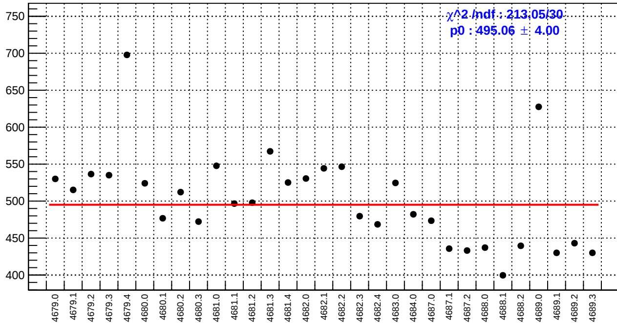
slug74-Left: reg_asym_sam7.rms/ppm
