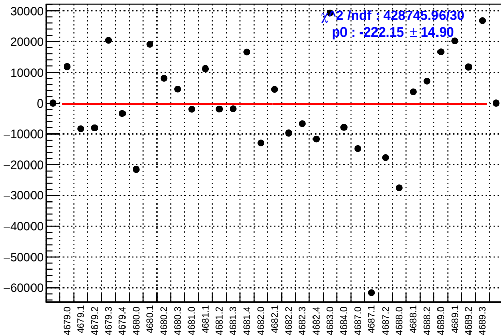
slug74-Left: asym_atl_dd.mean/ppb-reg_asym_atl_dd.mean/ppb
