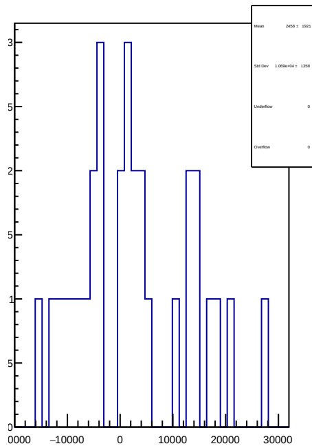
slug74-Left: 1D Corr asym_atl1r2_dd.mean/ppb-reg_asym_atl1r2_dd.mean/ppb
