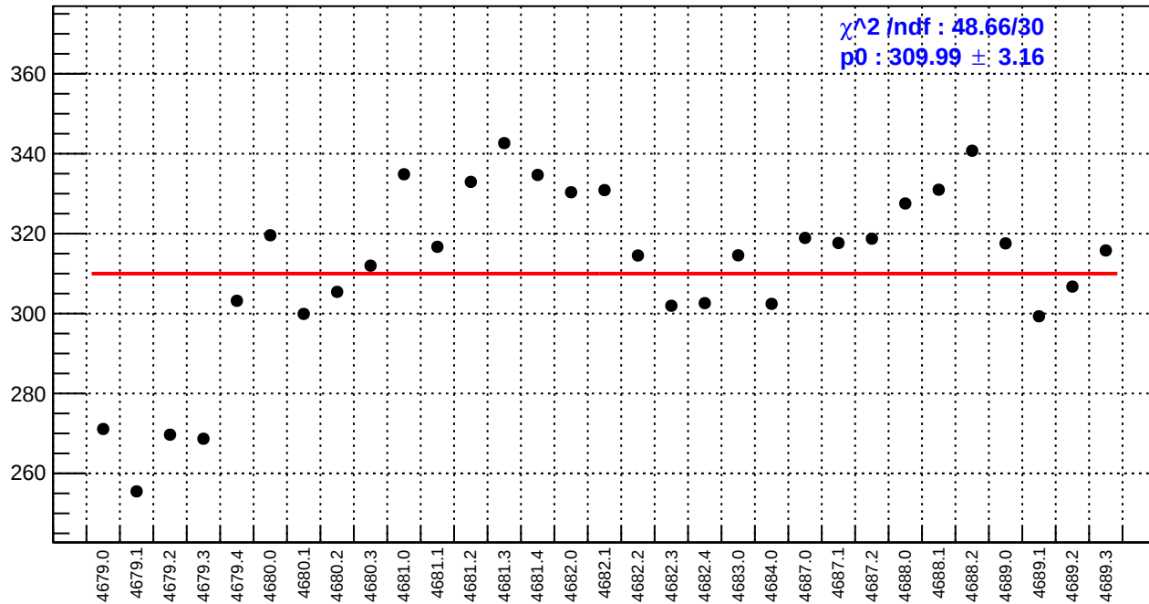
slug74-Left: reg_asym_sam5.rms/ppm
