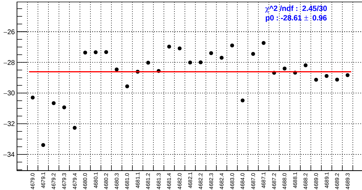
slug74-Left: us_avg_bpm4eX/(ppb/nm)
