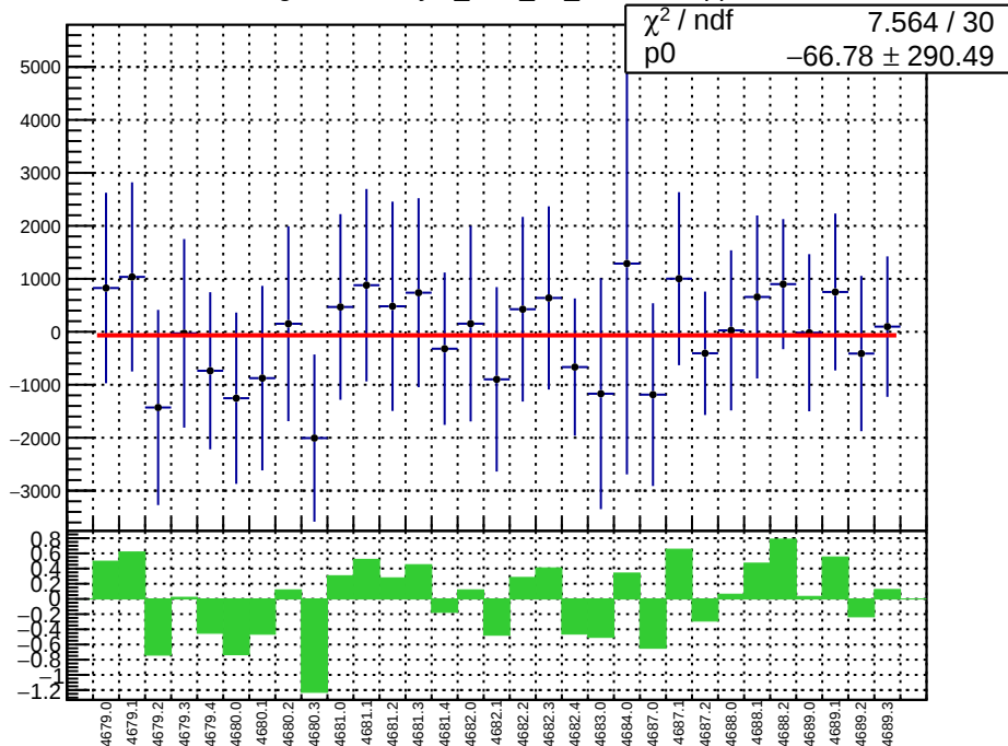
slug74-Left: asym_bcm_an_ds3.mean/ppb
