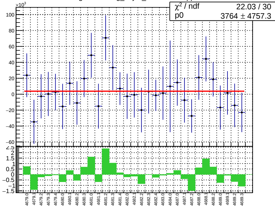
slug74-Left: reg_asym_sam2.mean/ppb
