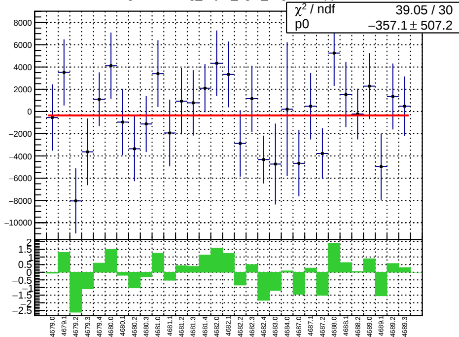
slug74-Left: reg_asym_right_avg.mean/ppb
