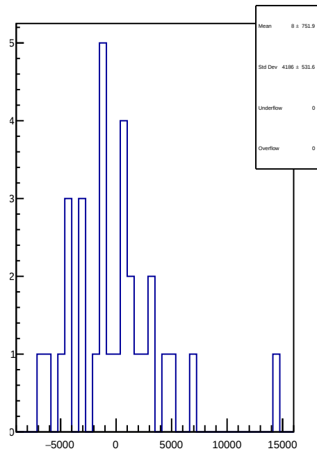
slug74-Left: 1D Corr asym_us_dd.mean/ppb-reg_asym_us_dd.mean/ppb
