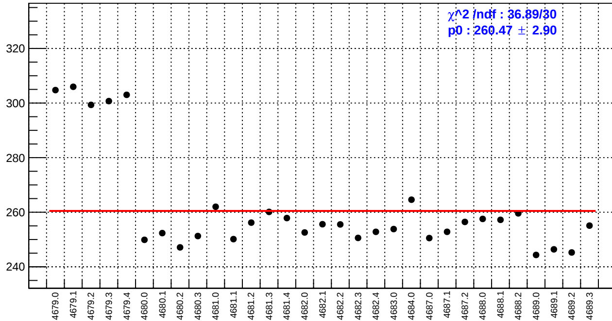
slug74-Left: reg_asym_atr1l2_dd.rms/ppm
