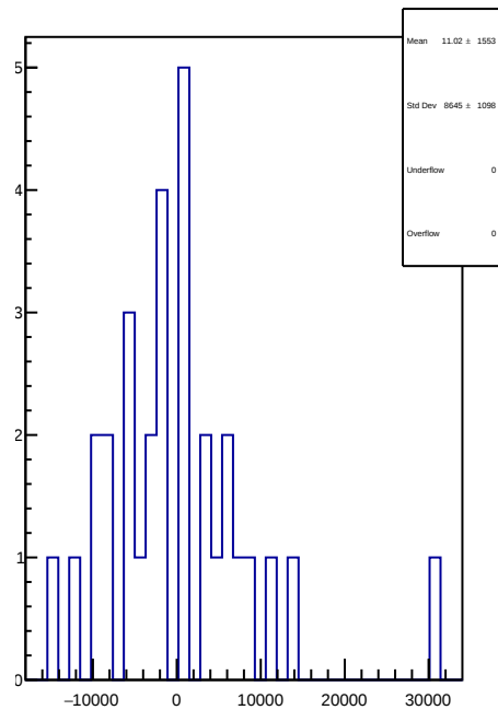
slug74-Left: 1D Corr asym_left_avg.mean/ppb-reg_asym_left_avg.mean/ppb
