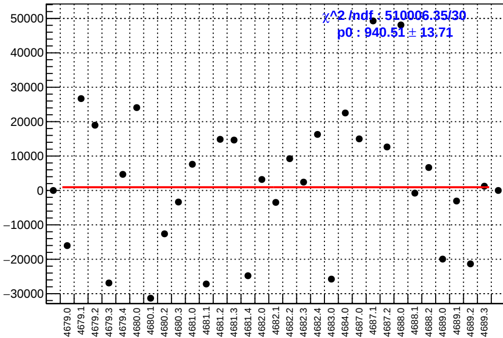
slug74-Left: asym_at2_avg.mean/ppb-reg_asym_at2_avg.mean/ppb
