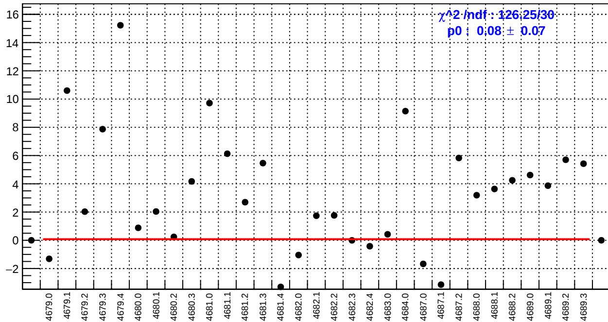
slug74-Left: us_avg_bpm4aX/(ppb/nm)
