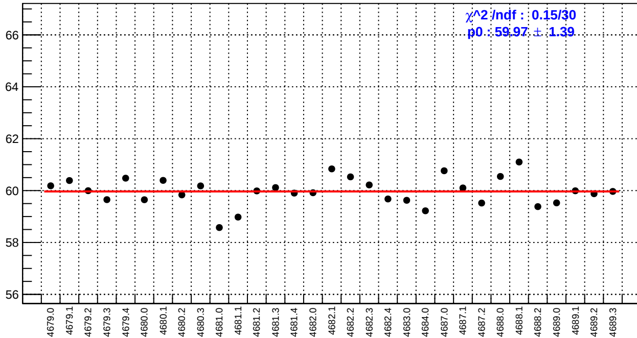
slug74-Left: reg_asym_atr2.rms/ppm
