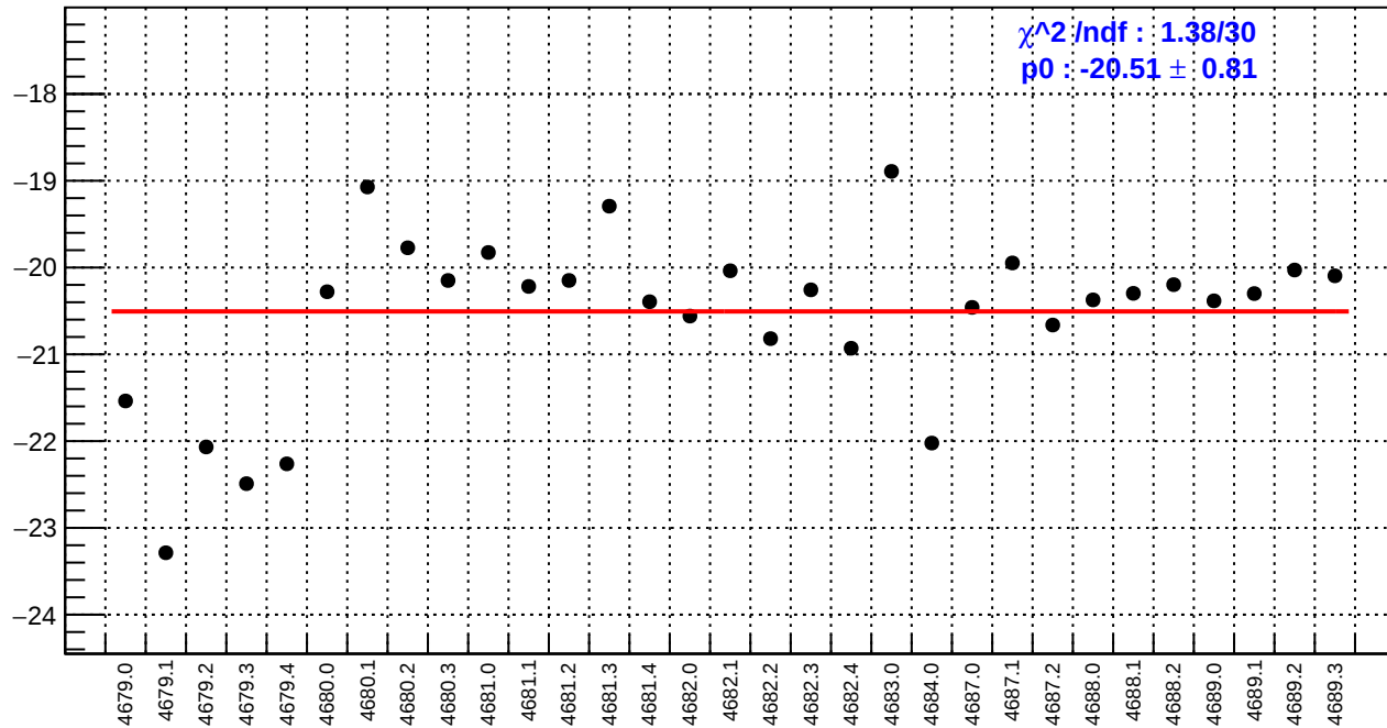
slug74-Left: us_avg_bpm12X/(ppb/nm)
