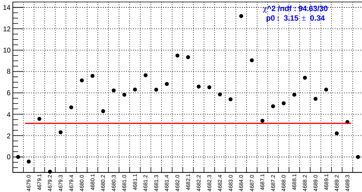
slug74-Left: ds_avg_bpm4aY/(ppb/nm)
