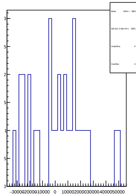
slug74-Left: 1D Corr asym_at2_avg.mean/ppb-reg_asym_at2_avg.mean/ppb
