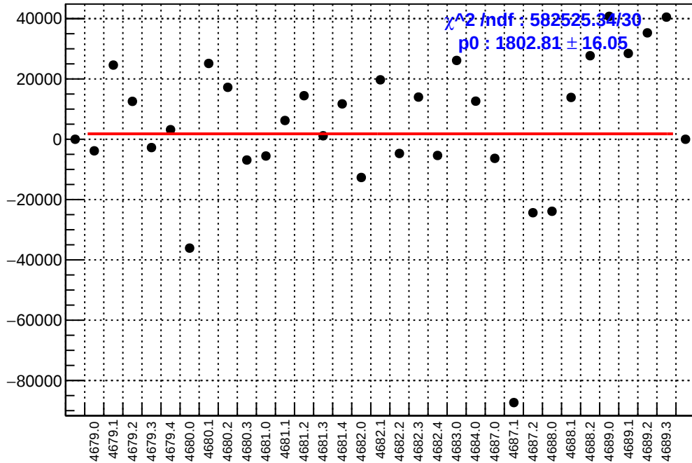
slug74-Left: asym_sam8.mean/ppb-reg_asym_sam8.mean/ppb
