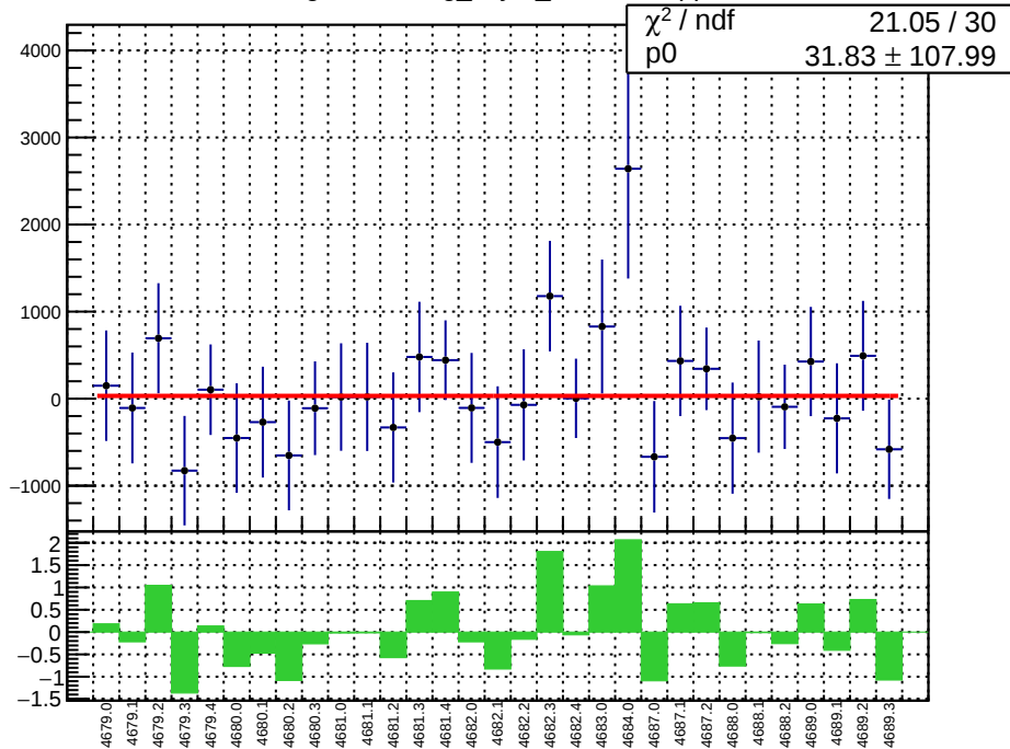
slug74-Left: reg_asym_atr2.mean/ppb
