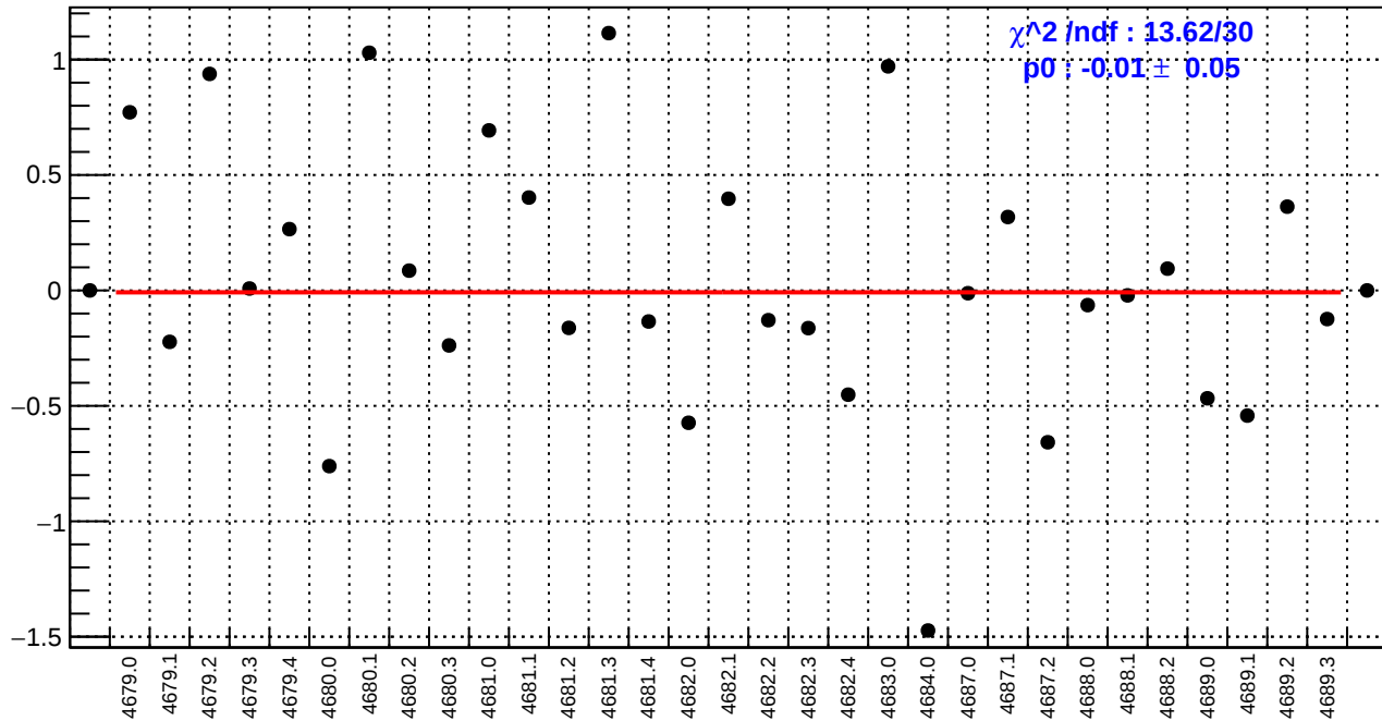
slug74-Left: right_avg_bpm12X/(ppb/nm)
