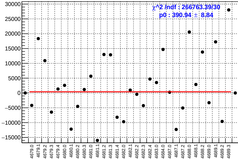
slug74-Left: asym_atl1r2_dd.mean/ppb-reg_asym_atl1r2_dd.mean/ppb
