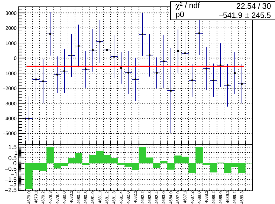
slug74-Left: reg_asym_left_avg.mean/ppb
