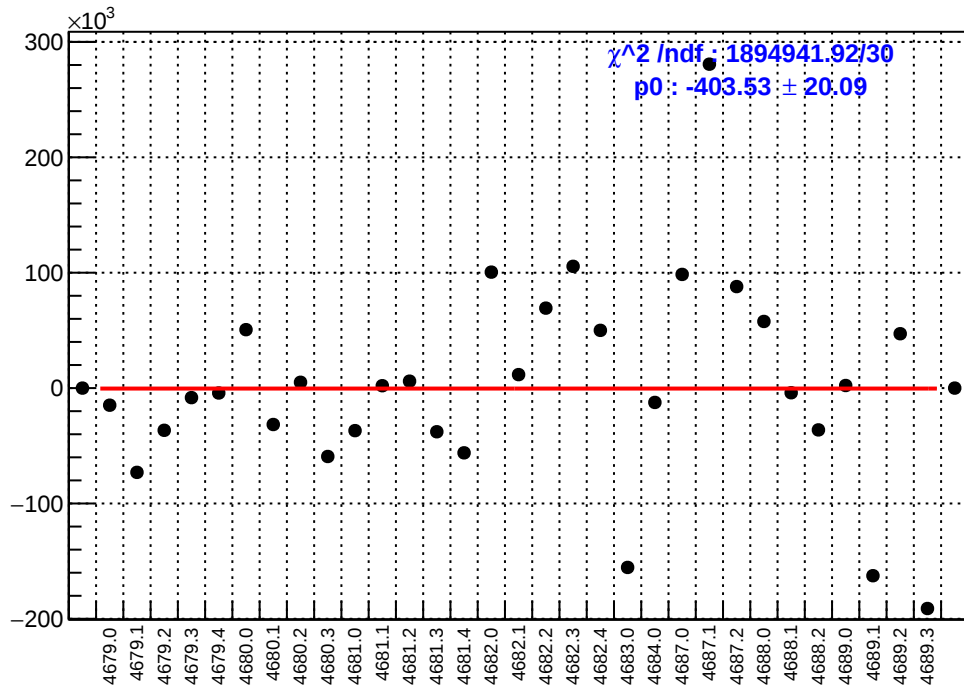
slug74-Left: asym_sam2.mean/ppb-reg_asym_sam2.mean/ppb
