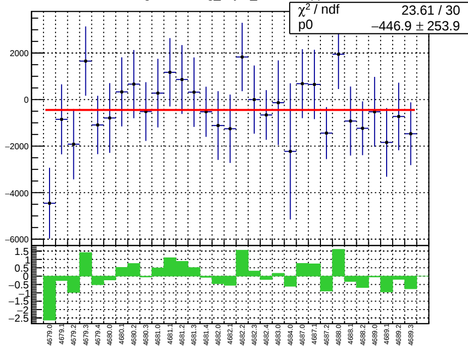
slug74-Left: reg_asym_dsl.mean/ppb
