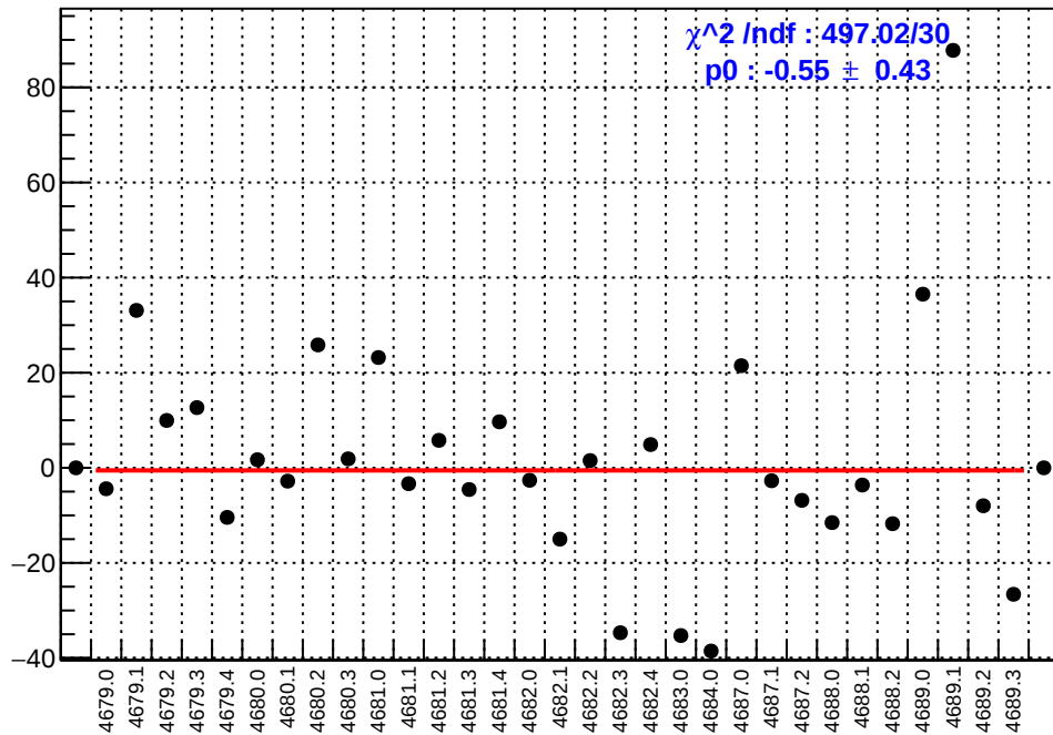
slug74-Left: asym_atr_dd.mean/ppb-reg_asym_atr_dd.mean/ppb
