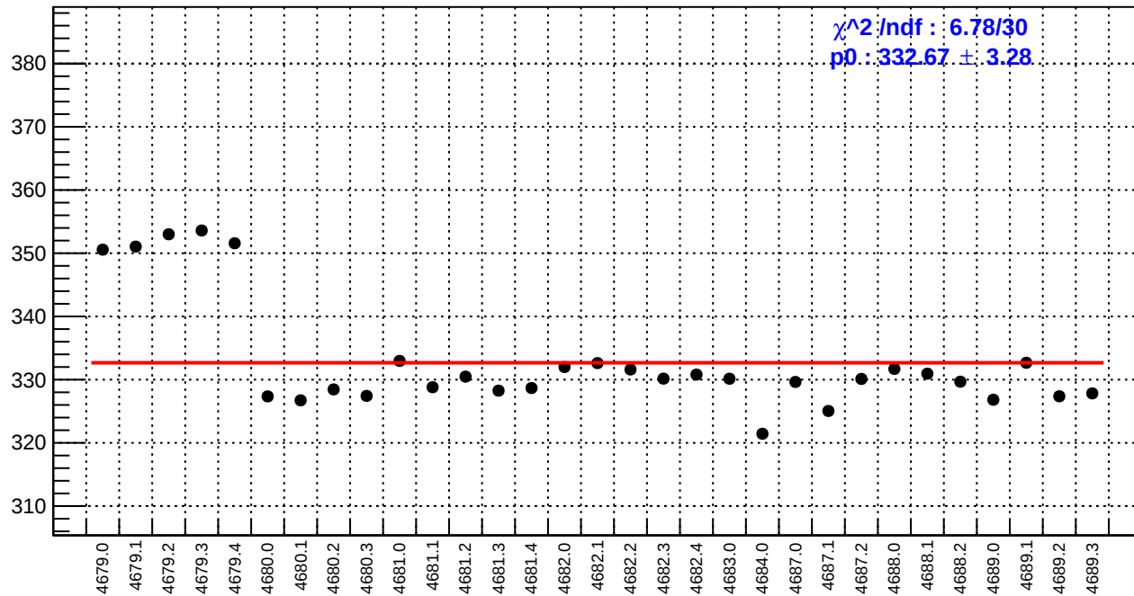
slug74-Left: reg_asym_atl1r2_dd.rms/ppm
