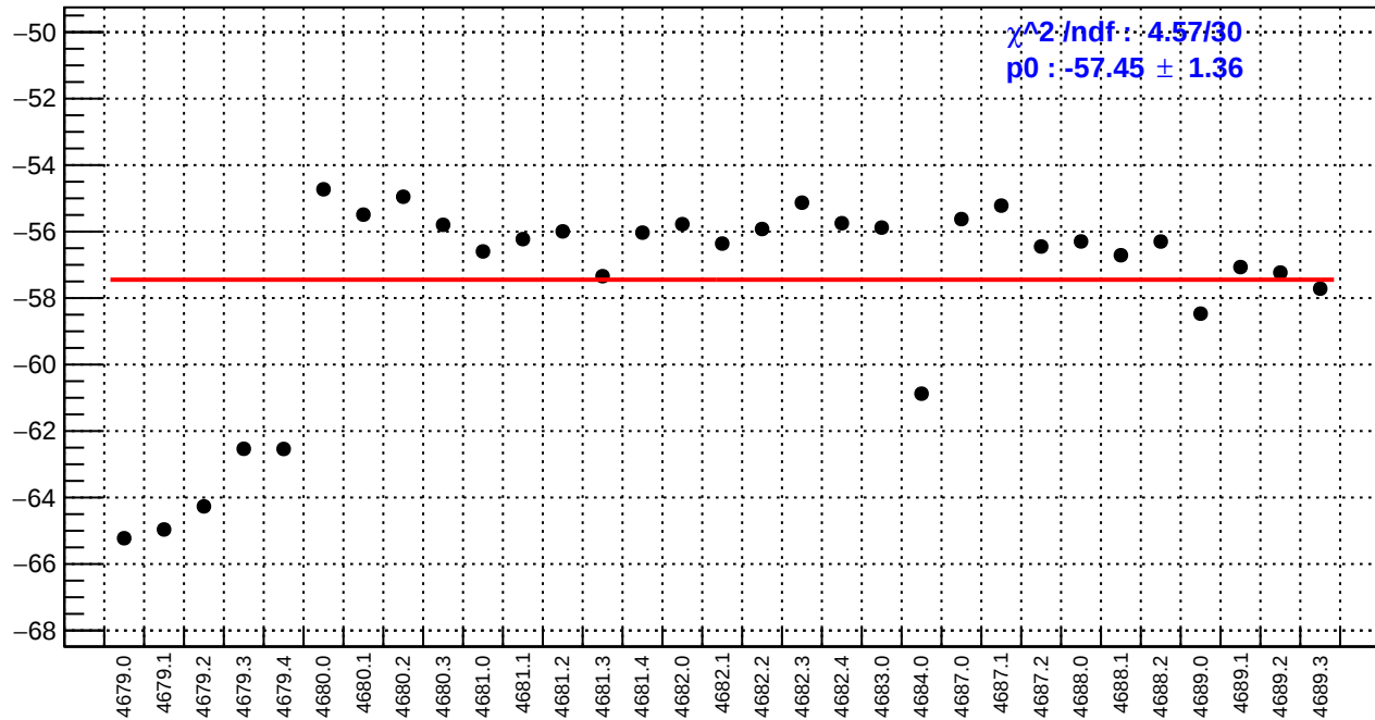
slug74-Left: usl_bpm4eX/(ppb/nm)
