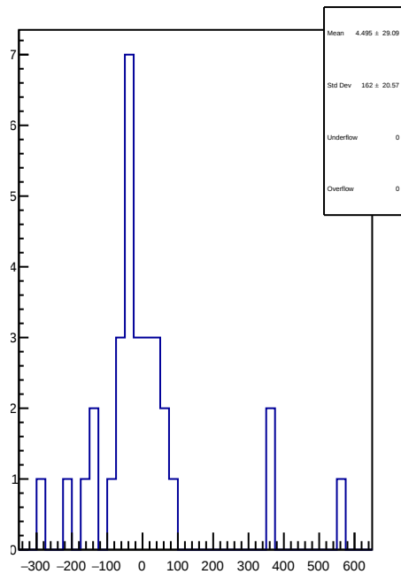
slug74-Left: 1D Corr asym_usr.mean/ppb-reg_asym_usr.mean/ppb
