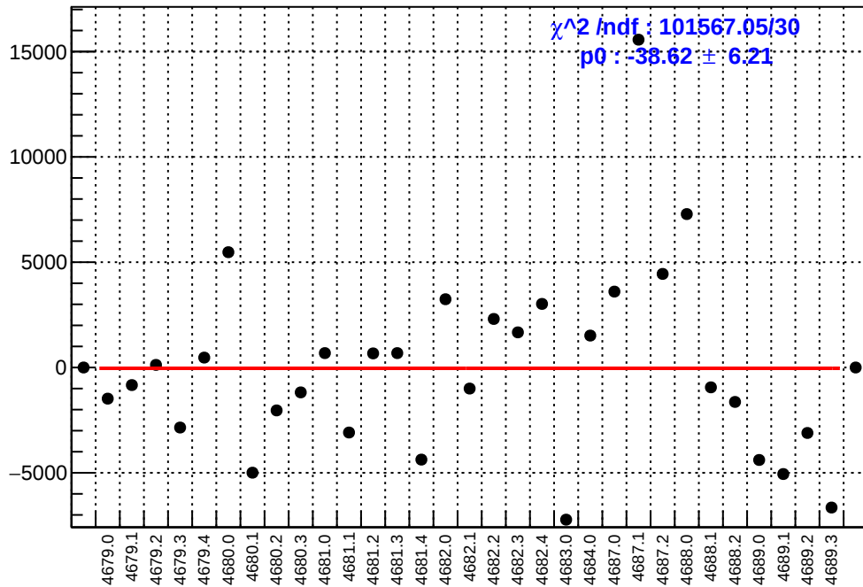
slug74-Left: asym_ds_dd.mean/ppb-reg_asym_ds_dd.mean/ppb
