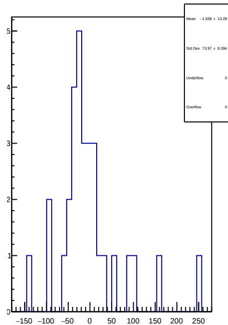
slug74-Left: 1D Corr asym_right_dd.mean/ppb-reg_asym_right_dd.mean/ppb
