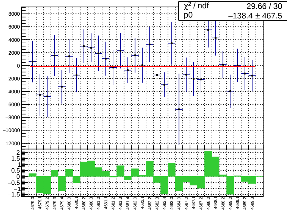
slug74-Left: reg_asym_atr1l2_avg.mean/ppb
