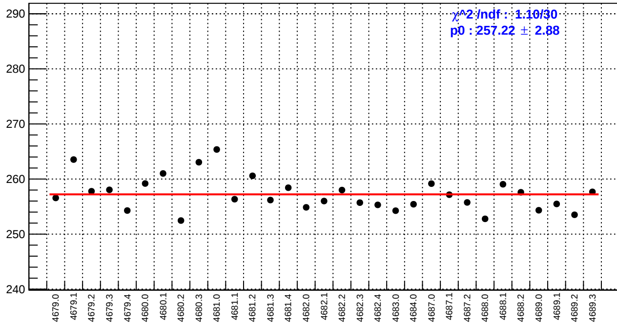
slug74-Left: reg_asym_dsr.rms/ppm
