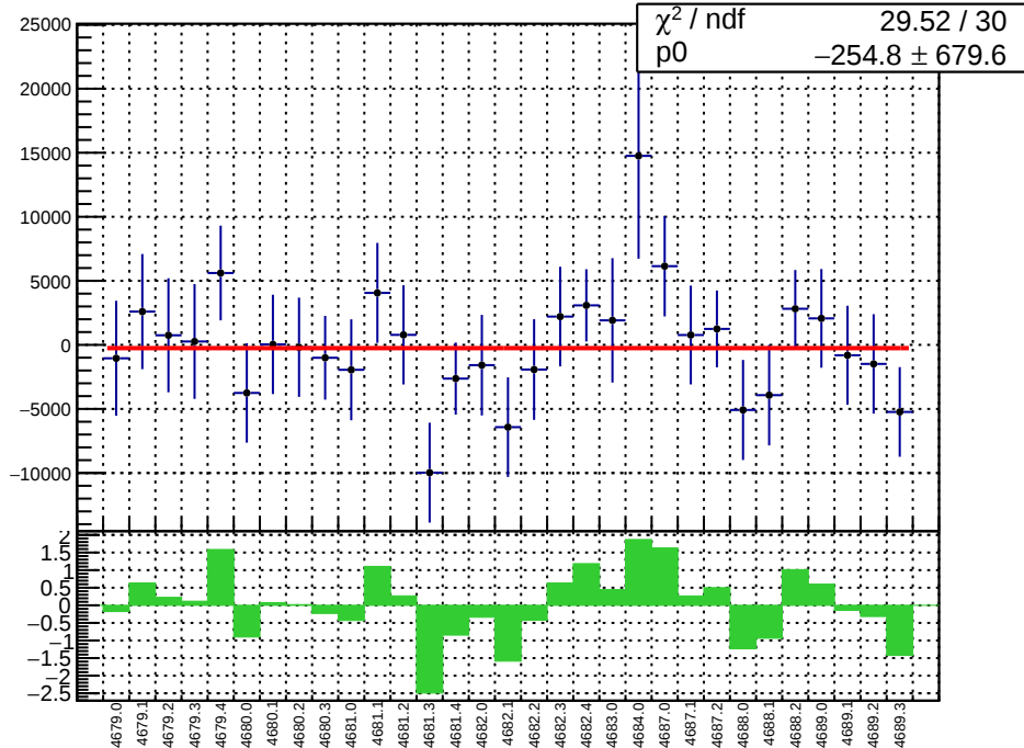
slug74-Left: reg_asym_atl_dd.mean/ppb
