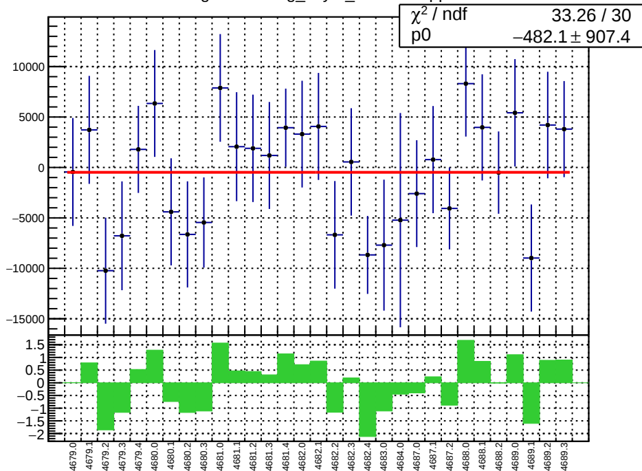
slug74-Left: reg_asym_usr.mean/ppb
