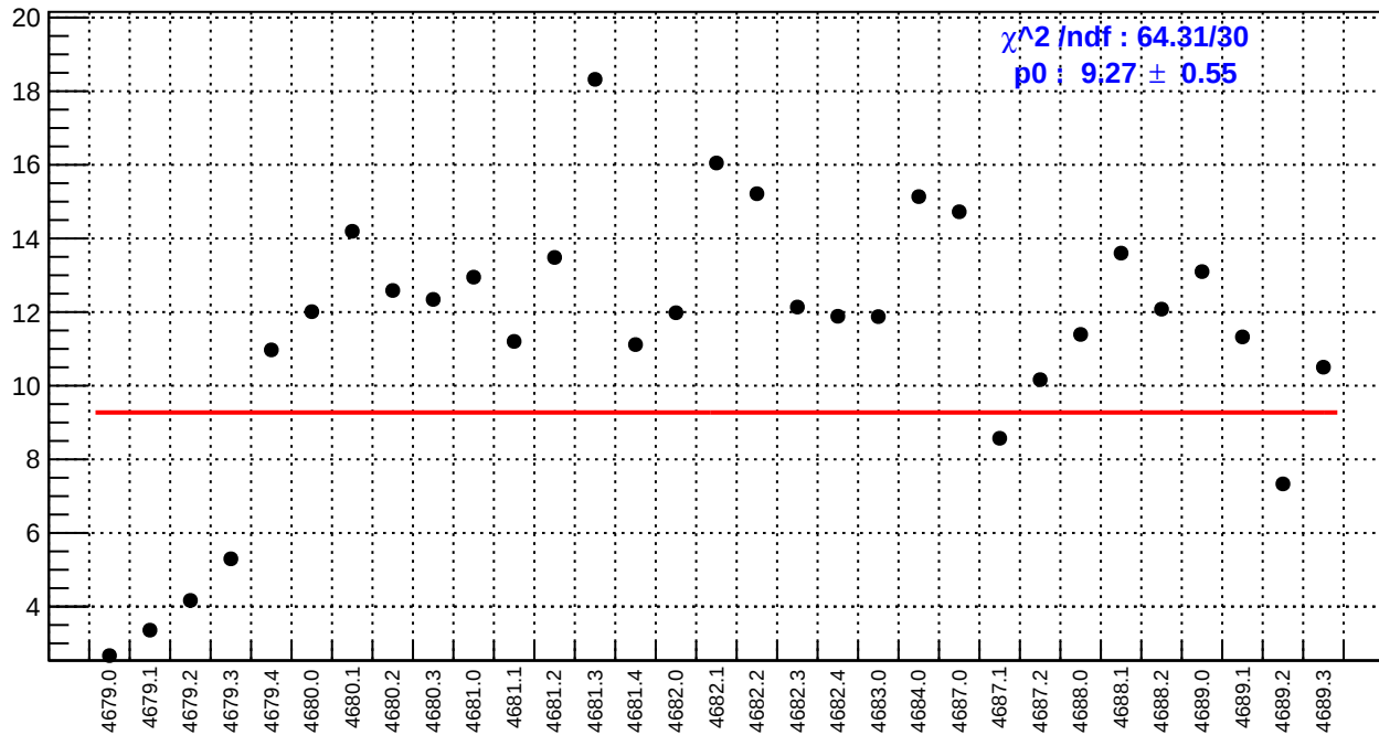
slug74-Left: left_avg_bpm4aY/(ppb/nm)
