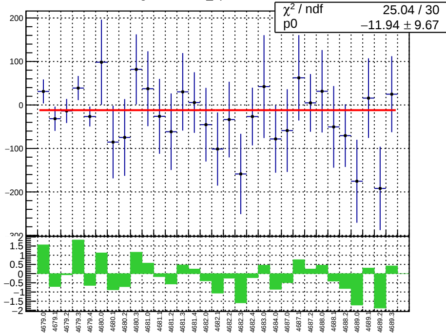
slug74-Left: diff_bpm4eY.mean/nm
