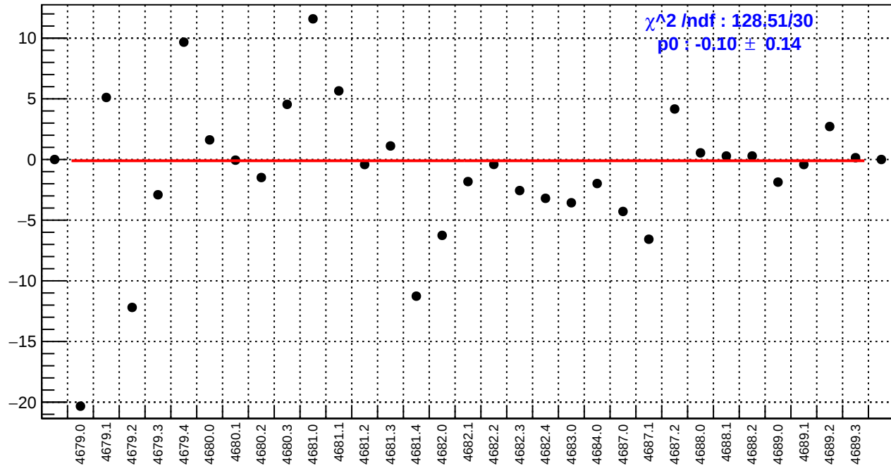
slug74-Left: usr_bpm4aX/(ppb/nm)
