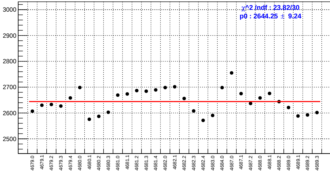
slug74-Left: reg_asym_sam2.rms/ppm
