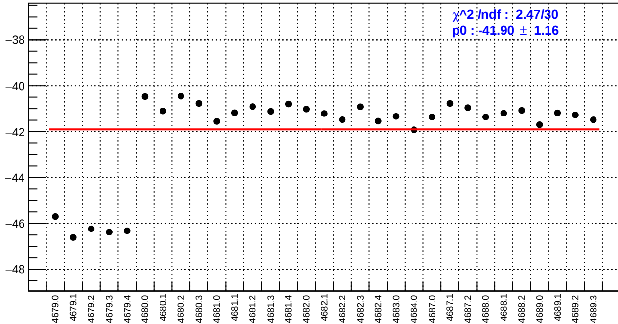
slug74-Left: dsl_bpm12X/(ppb/nm)
