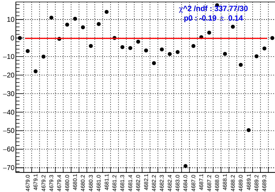
slug74-Left: asym_atr2.mean/ppb-reg_asym_atr2.mean/ppb
