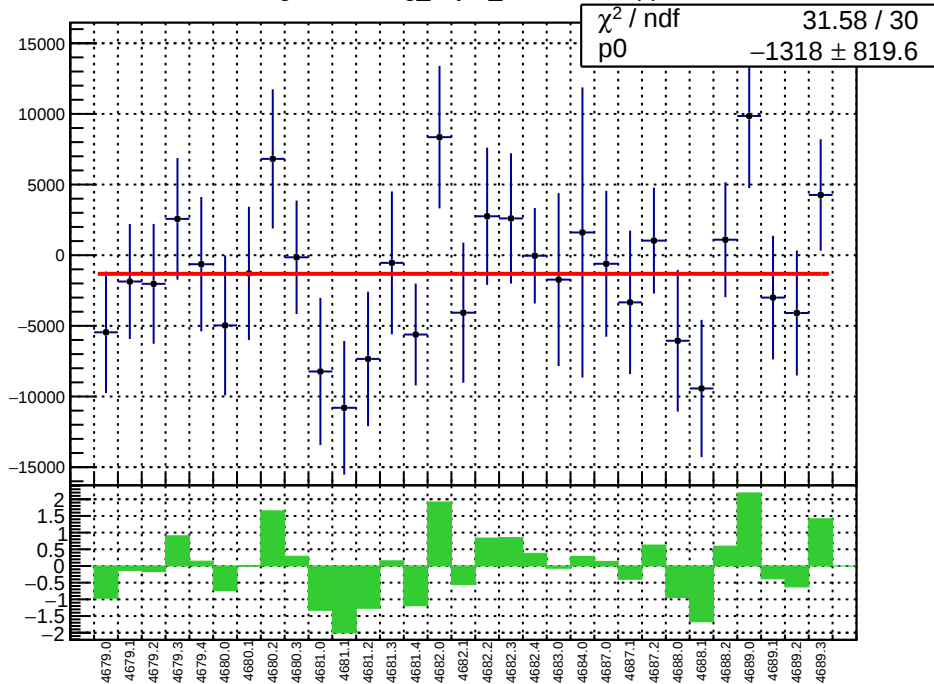
slug74-Left: reg_asym_sam6.mean/ppb
