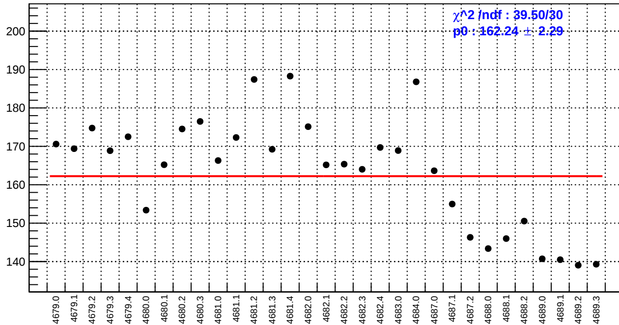
slug74-Left: asym_bcm_an_ds3.rms/ppm
