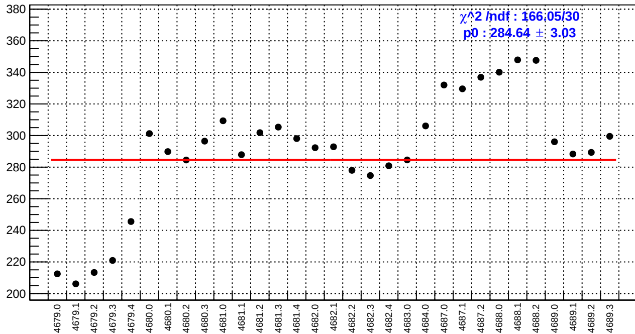
slug74-Left: reg_asym_sam1.rms/ppm
