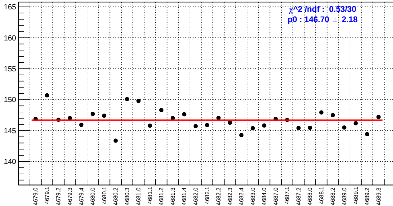
slug74-Left: reg_asym_ds_avg.rms/ppm
