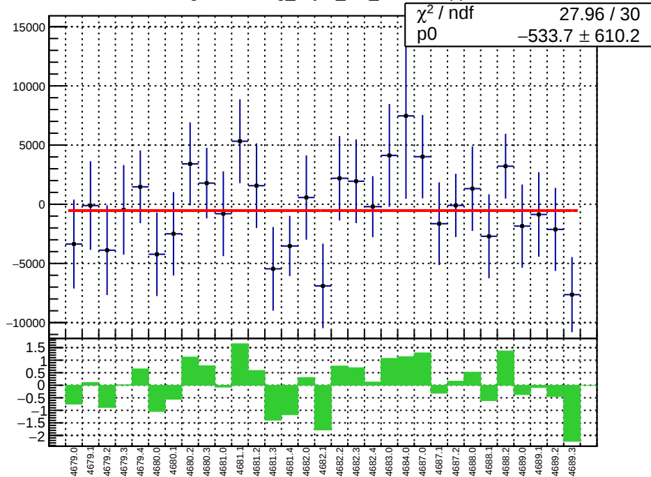
slug74-Left: reg_asym_at1_dd.mean/ppb
