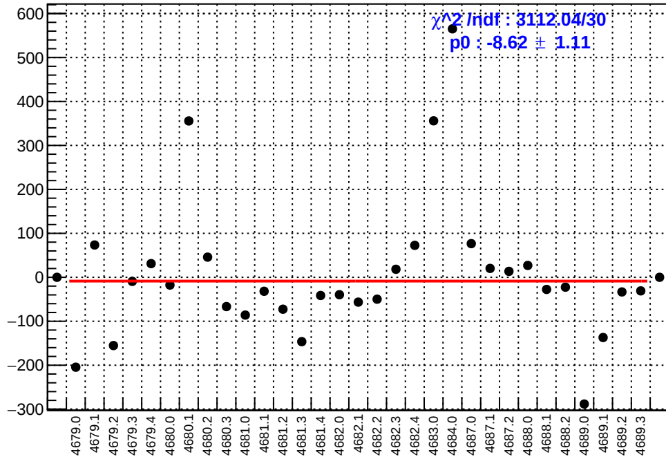
slug74-Left: asym_usr.mean/ppb-reg_asym_usr.mean/ppb
