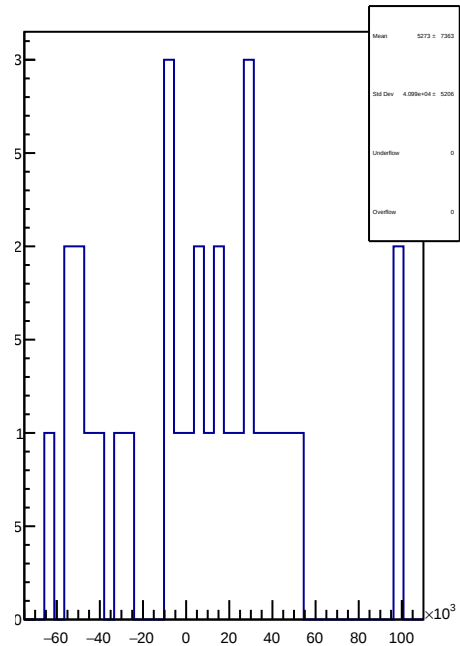
slug74-Left: 1D Corr asym_atl2.mean/ppb-reg_asym_atl2.mean/ppb
