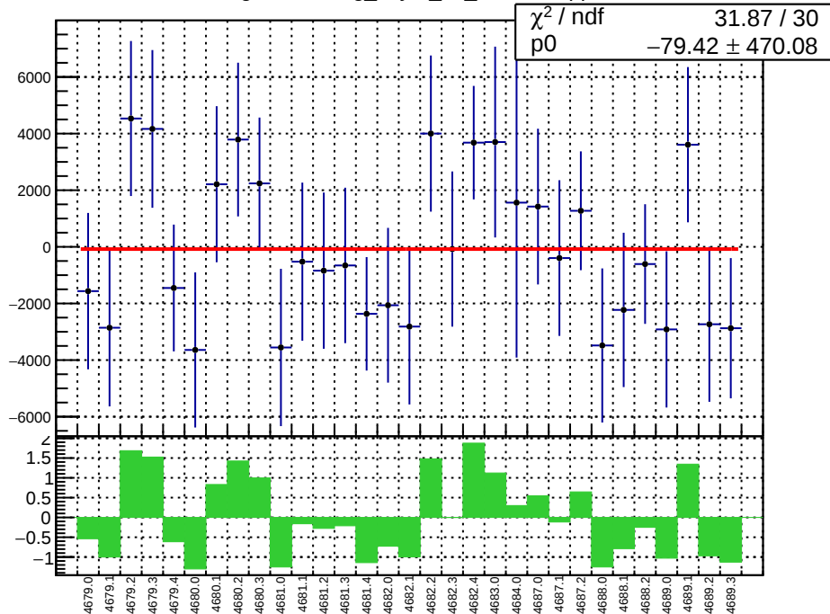
slug74-Left: reg_asym_us_dd.mean/ppb
