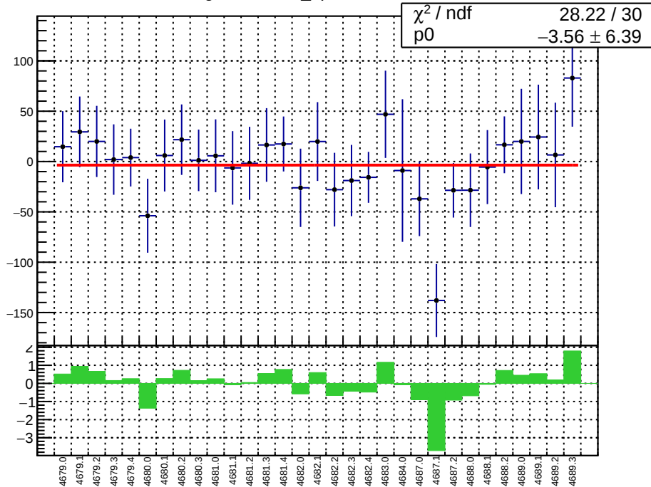
slug74-Left: diff_bpm4aX.mean/nm
