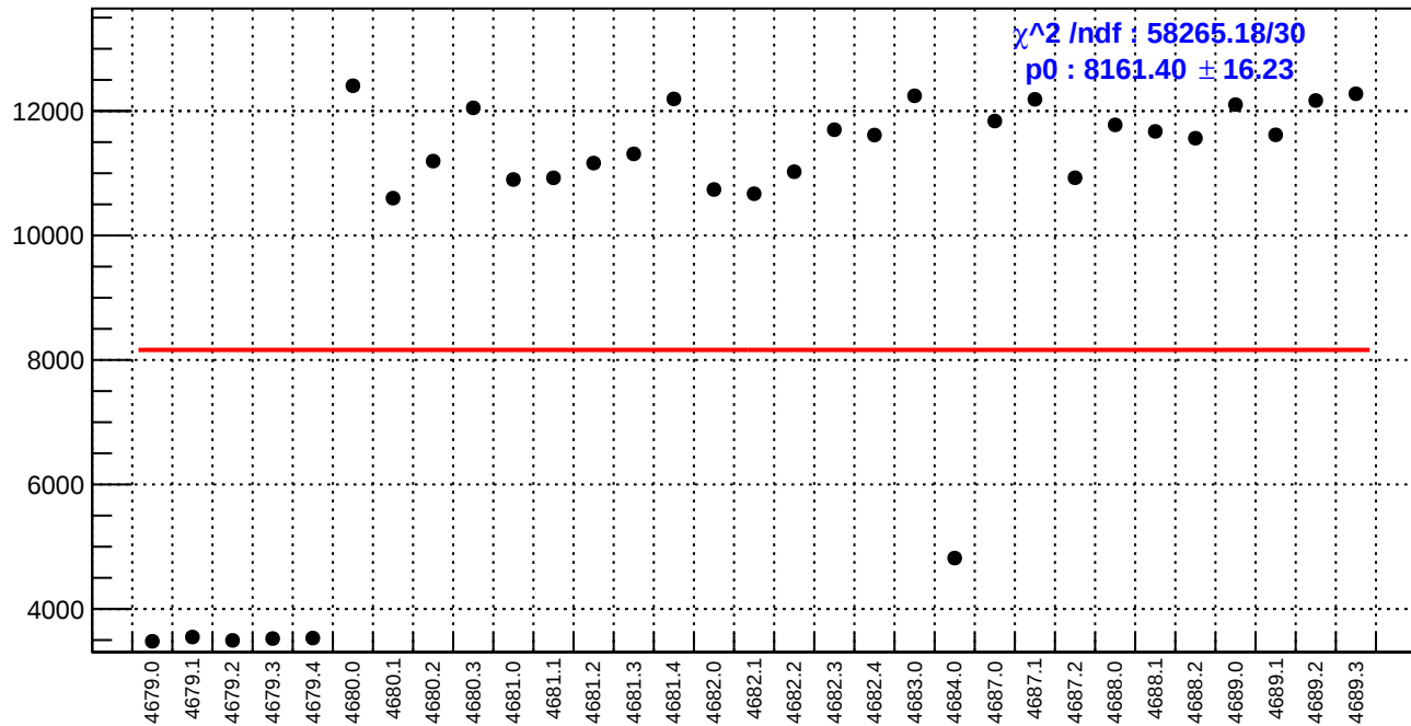
slug74-Left: diff_bpm4aY.rms/nm
