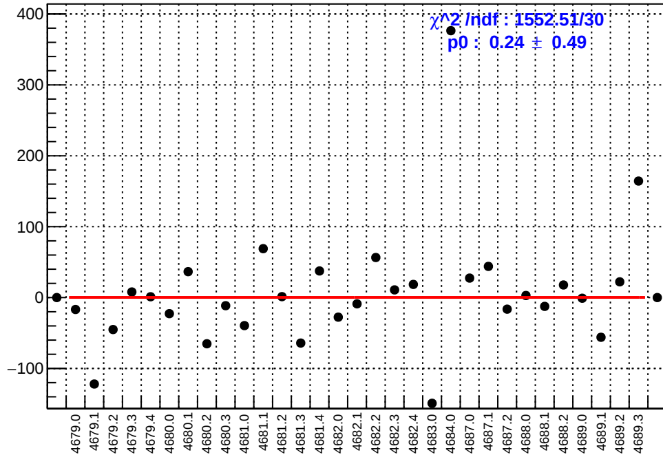
slug74-Left: asym_dsr.mean/ppb-reg_asym_dsr.mean/ppb
