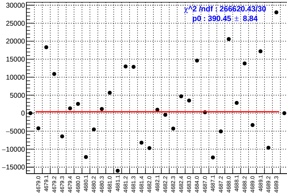
slug74-Left: asym_atl1r2_avg.mean/ppb-reg_asym_atl1r2_avg.mean/ppb
