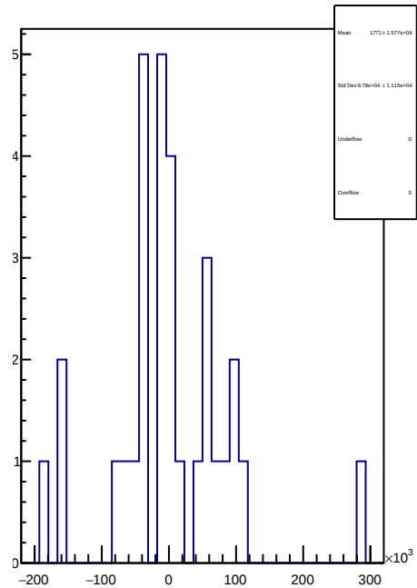
slug74-Left: 1D Corr asym_sam2.mean/ppb-reg_asym_sam2.mean/ppb
