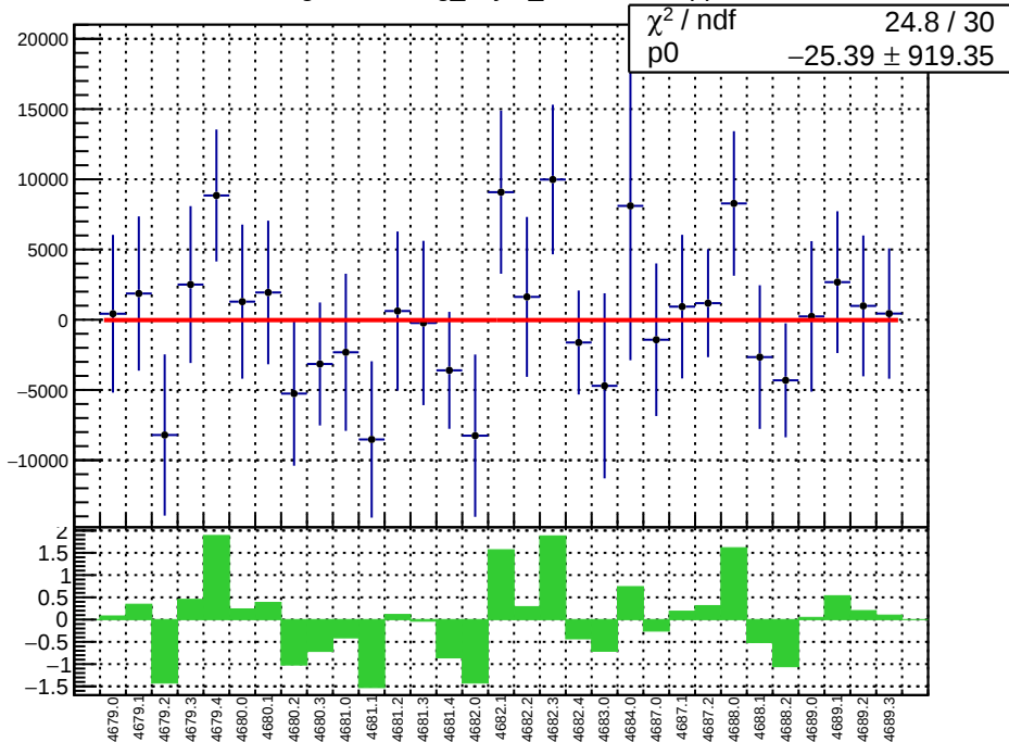
slug74-Left: reg_asym_sam8.mean/ppb
