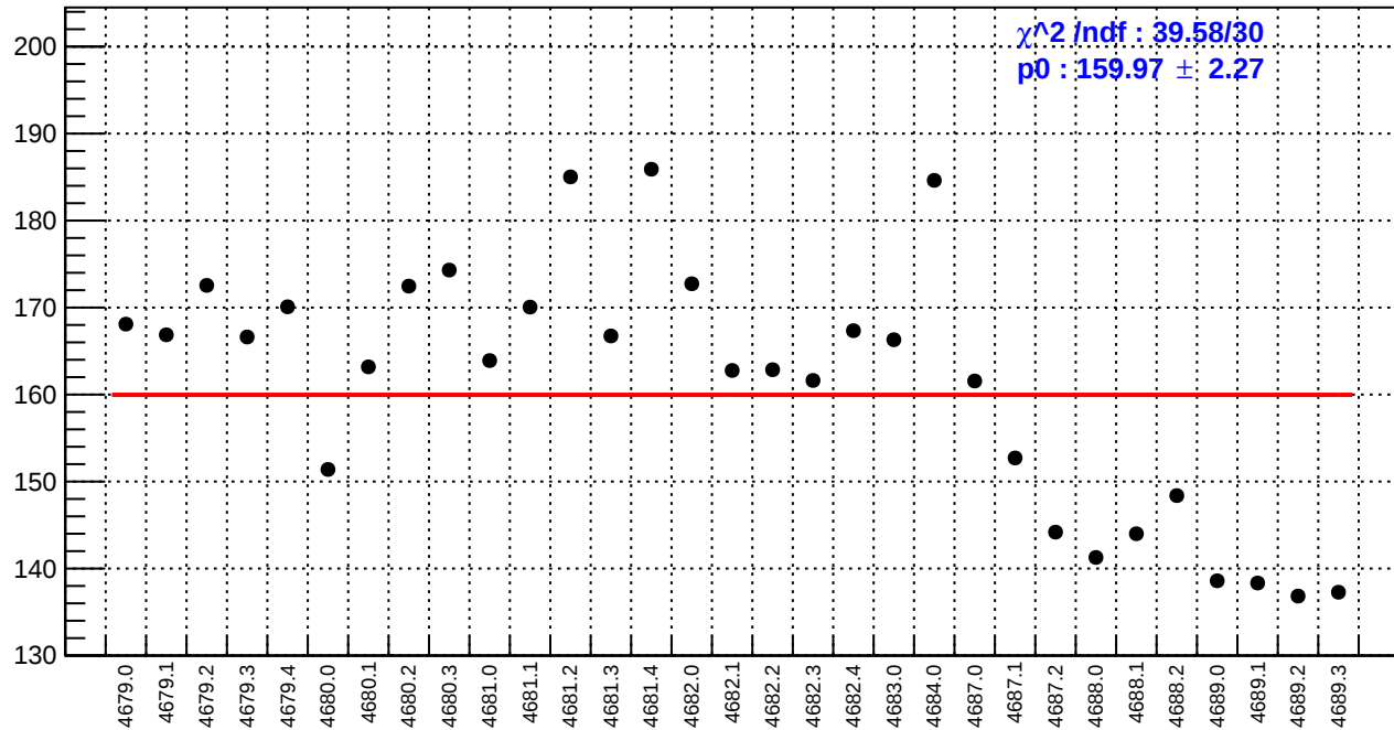
slug74-Left: asym_bcm_an_ds.rms/ppm
