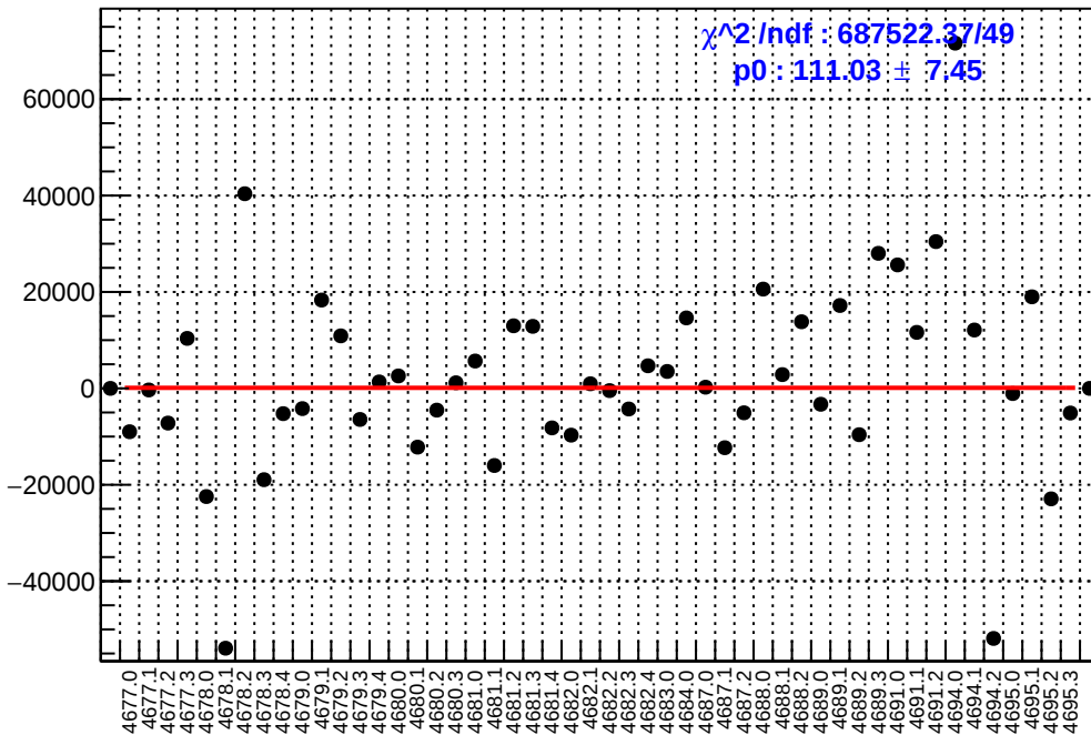
slug74: asym_atl1r2_avg.mean/ppb-reg_asym_atl1r2_avg.mean/ppb
