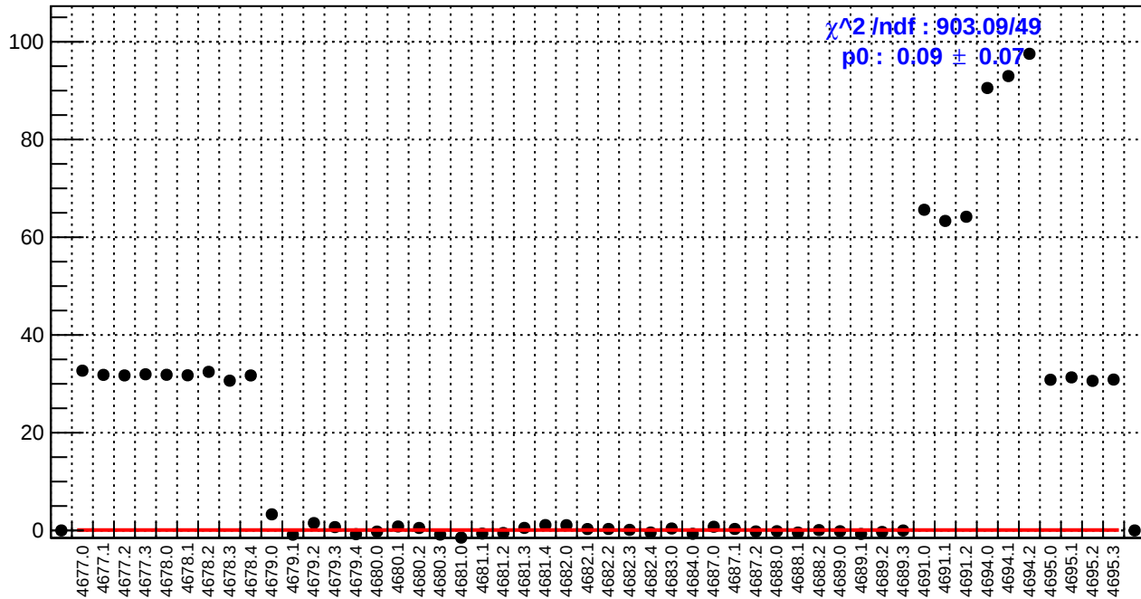
slug74: right_avg_bpm4eX/(ppb/nm)
