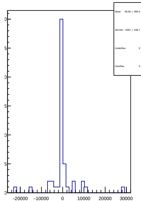
slug74: 1D Corr asym_dsr.mean/ppb-reg_asym_dsr.mean/ppb
