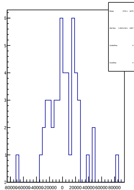
slug74: 1D Corr asym_atr1l2_avg.mean/ppb-reg_asym_atr1l2_avg.mean/ppb
