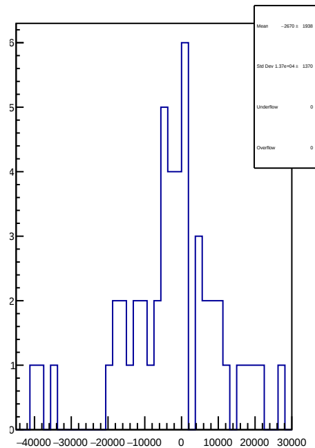
slug74: 1D Corr asym_sam5.mean/ppb-reg_asym_sam5.mean/ppb
