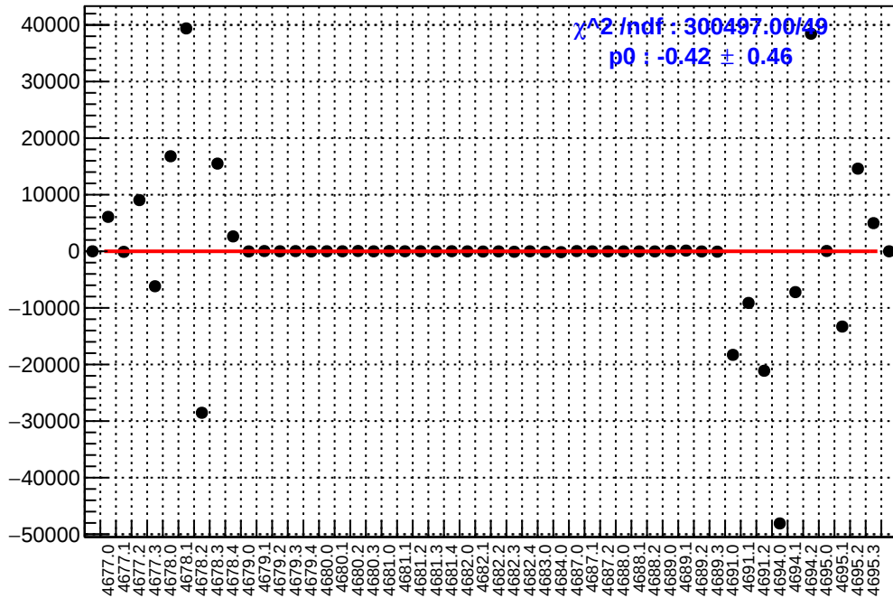
slug74: asym_atr1.mean/ppb-reg_asym_atr1.mean/ppb
