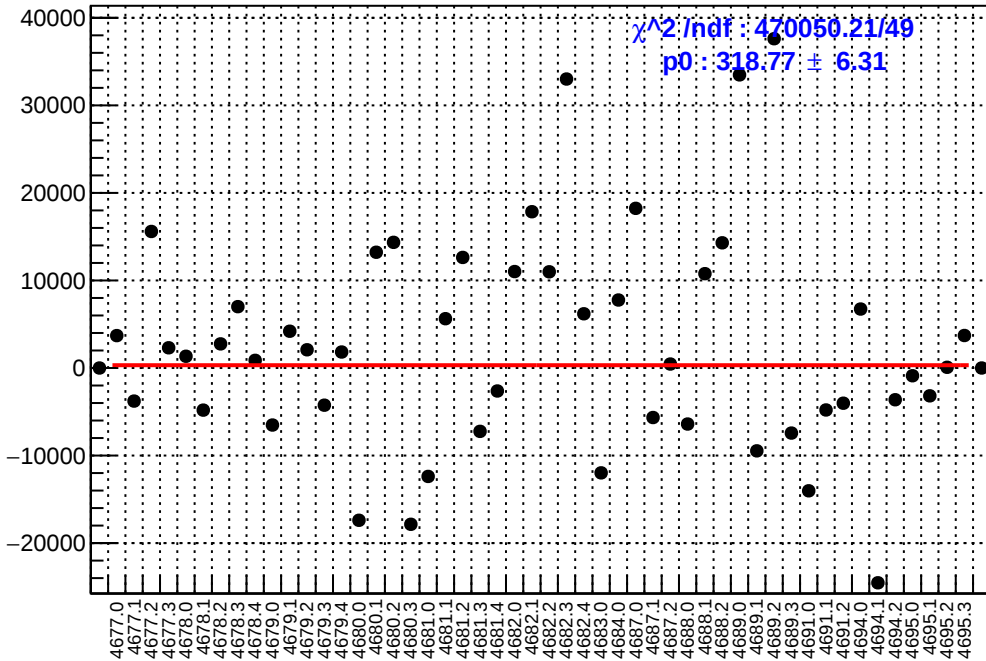
slug74: asym_sam1.mean/ppb-reg_asym_sam1.mean/ppb
