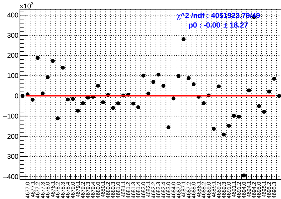
slug74: asym_sam2.mean/ppb-reg_asym_sam2.mean/ppb
