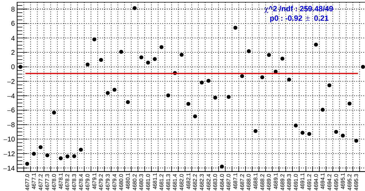
slug74: us_avg_bpm4eY/(ppb/nm)
