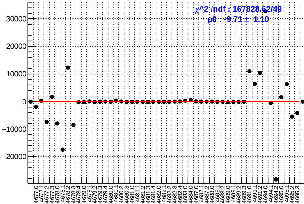
slug74: asym_usr.mean/ppb-reg_asym_usr.mean/ppb
