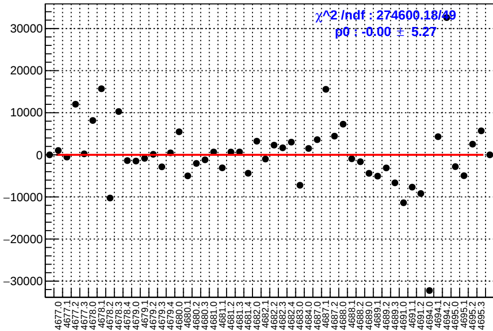
slug74: asym_ds_dd.mean/ppb-reg_asym_ds_dd.mean/ppb
