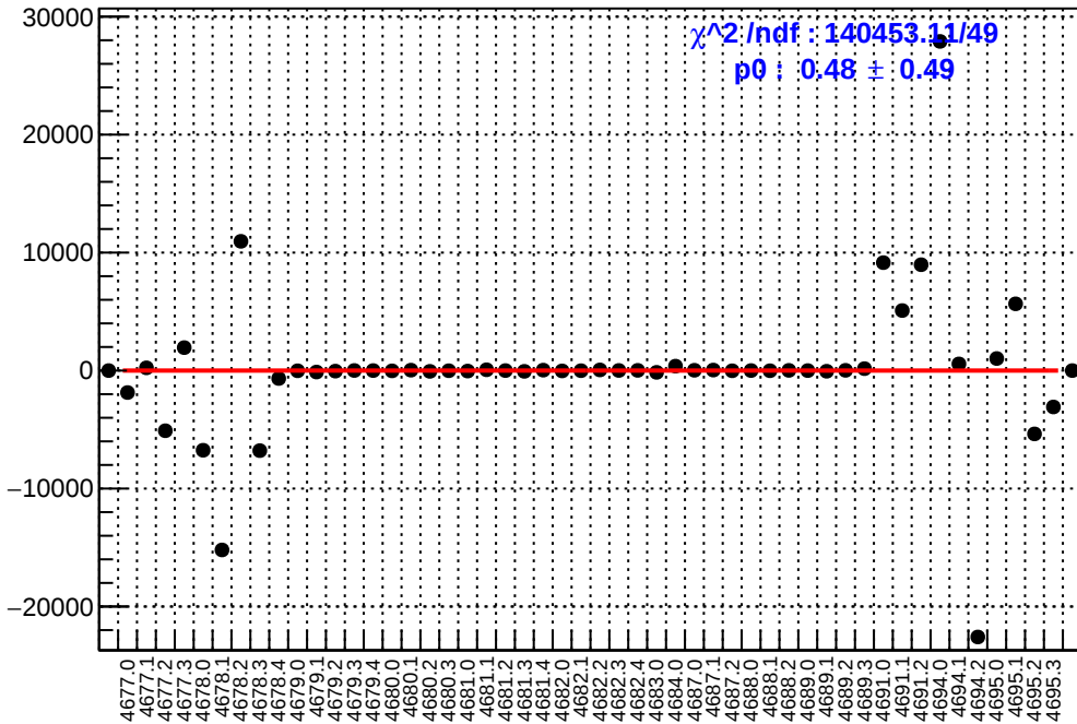
slug74: asym_dsr.mean/ppb-reg_asym_dsr.mean/ppb
