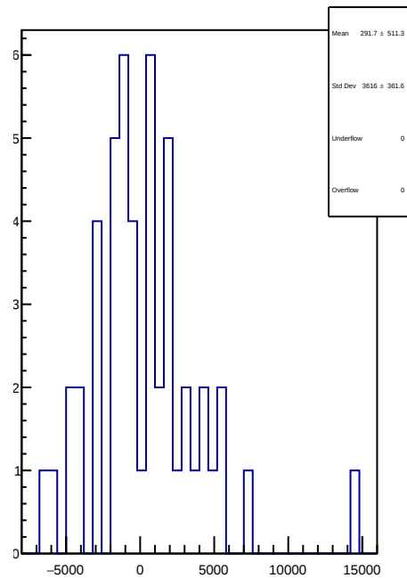
slug74: 1D Corr asym_us_avg.mean/ppb-reg_asym_us_avg.mean/ppb
