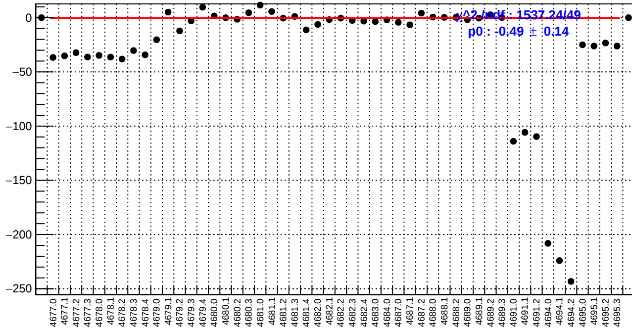
slug74: usr_bpm4aX/(ppb/nm)
