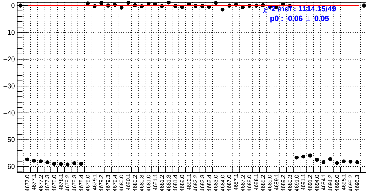
slug74: right_avg_bpm12X/(ppb/nm)
