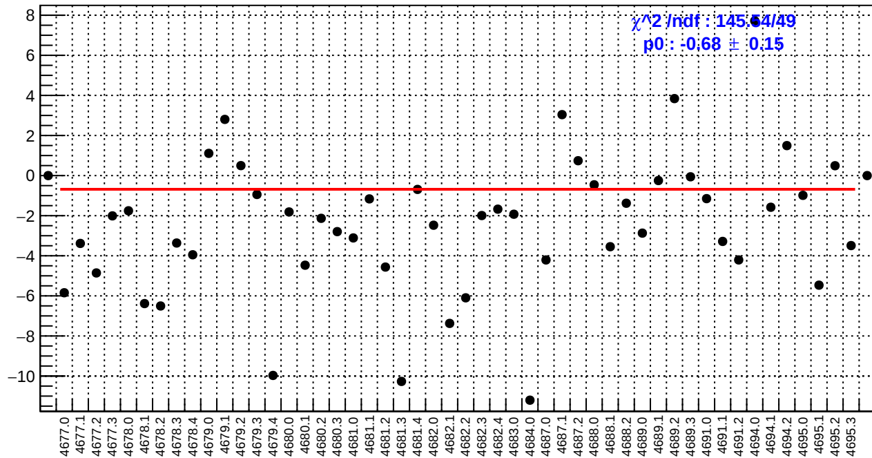
slug74: usl_bpm4eY/(ppb/nm)
