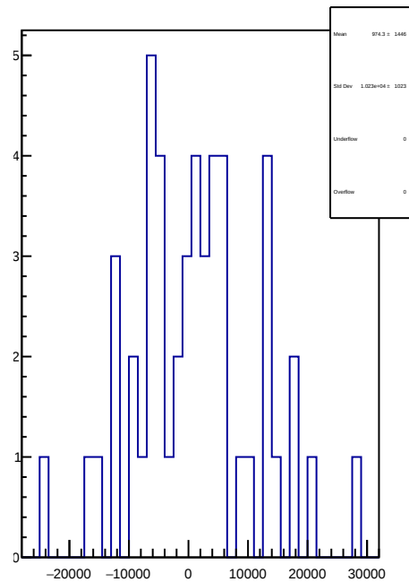
slug74: 1D Corr asym_atl1r2_dd.mean/ppb-reg_asym_atl1r2_dd.mean/ppb
