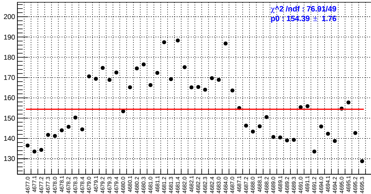
slug74: asym_bcm_an_ds3.rms/ppm
