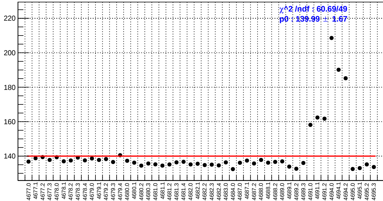
slug74: reg_asym_usl.rms/ppm
