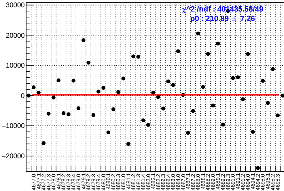
slug74: asym_atl1r2_dd.mean/ppb-reg_asym_atl1r2_dd.mean/ppb
