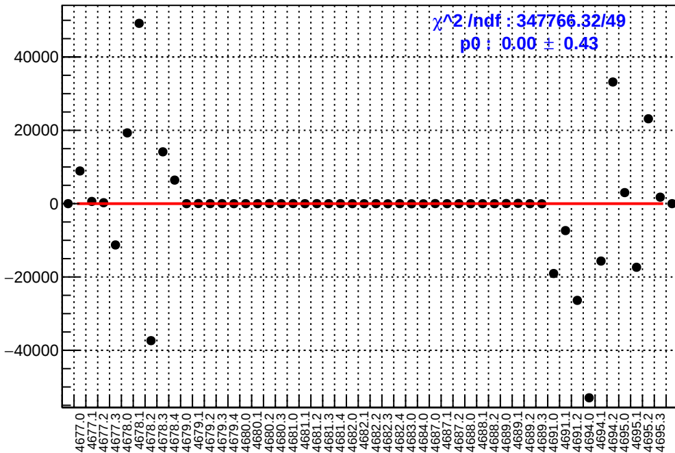
slug74: asym_atr_dd.mean/ppb-reg_asym_atr_dd.mean/ppb
