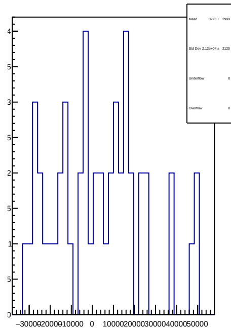
slug74: 1D Corr asym_at2_avg.mean/ppb-reg_asym_at2_avg.mean/ppb
