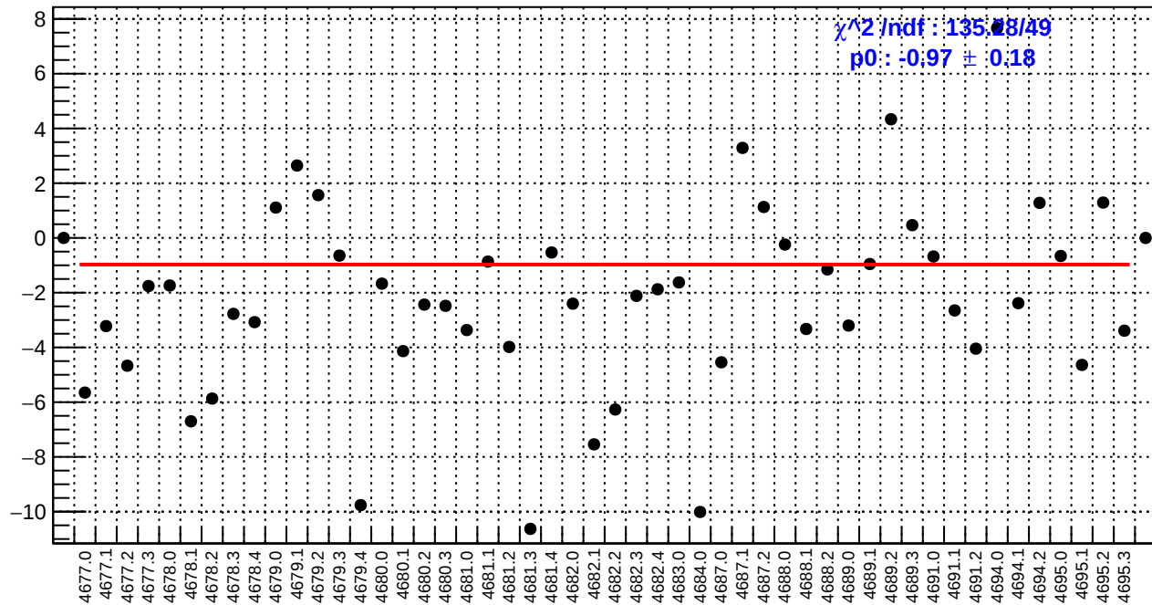
slug74: left_avg_bpm4eY/(ppb/nm)
