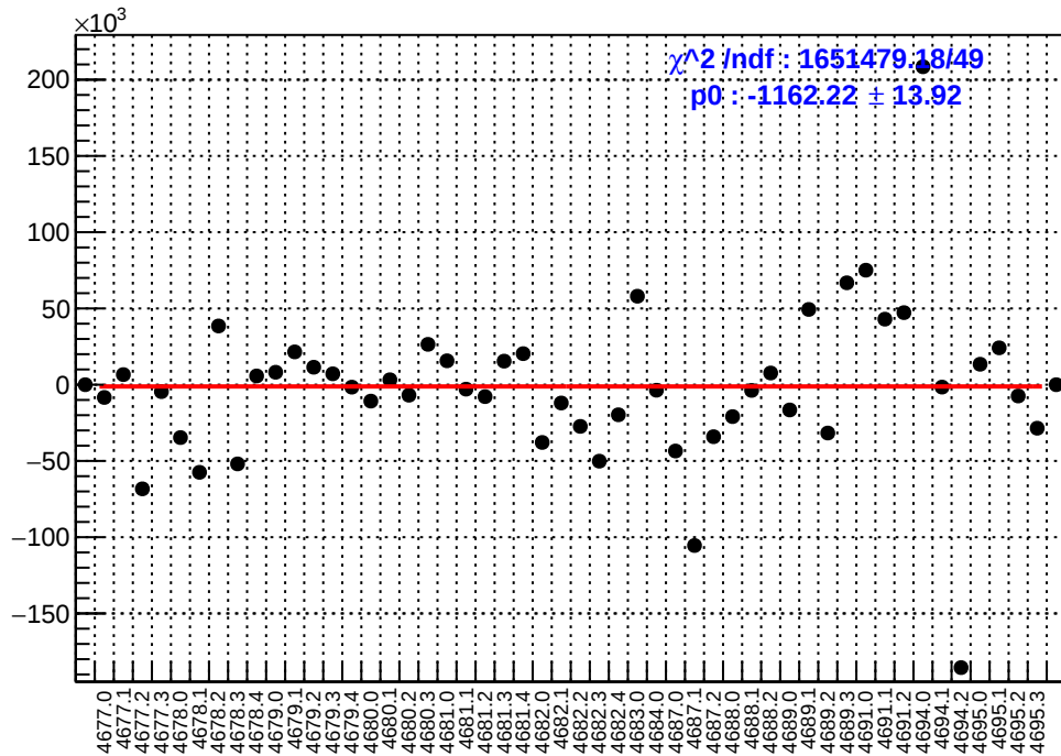
slug74: asym_sam6.mean/ppb-reg_asym_sam6.mean/ppb
