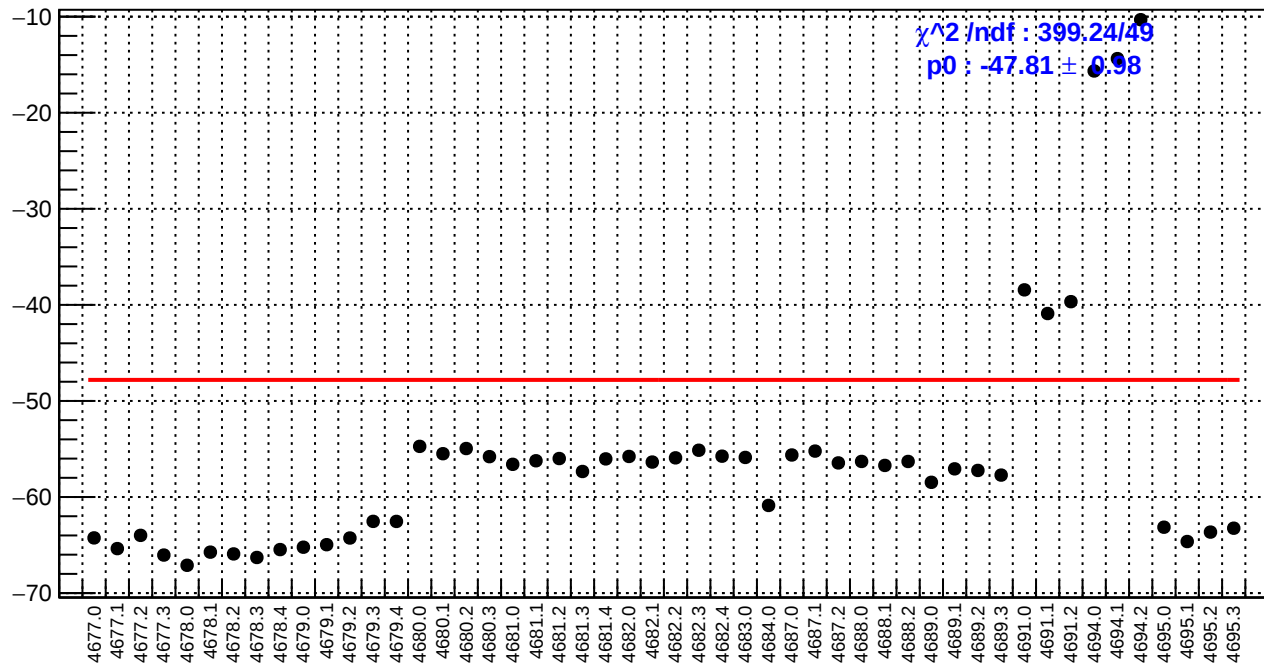
slug74: usl_bpm4eX/(ppb/nm)
