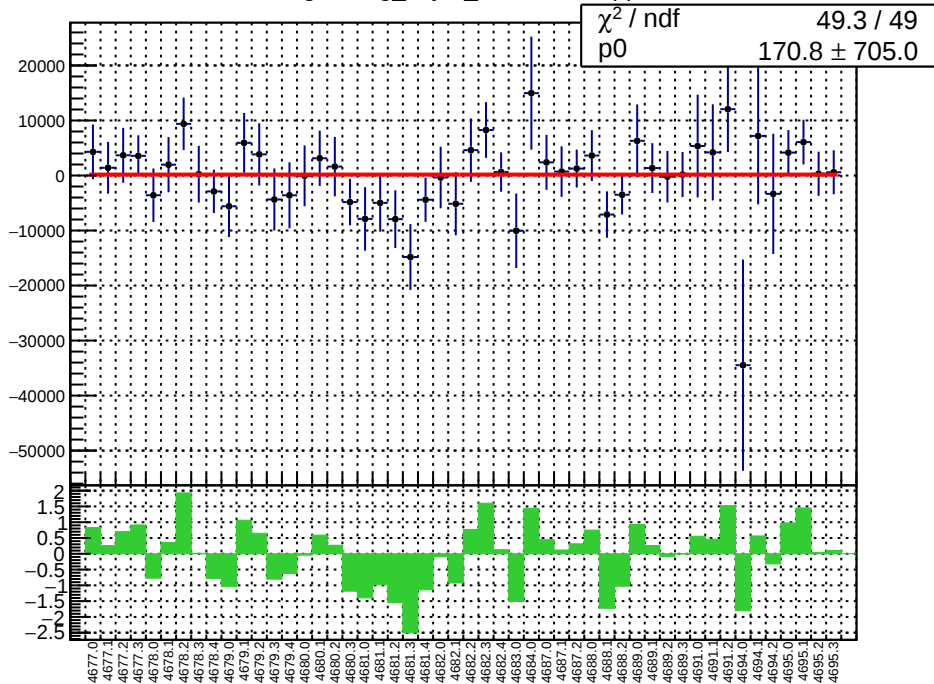
slug74: reg_asym_sam7.mean/ppb
