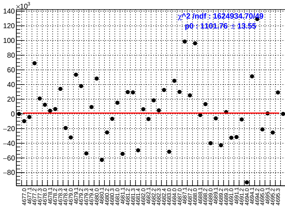
slug74: asym_atl2.mean/ppb-reg_asym_atl2.mean/ppb
