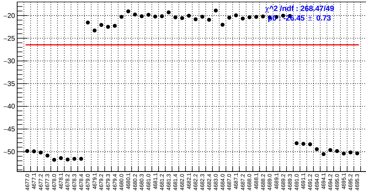
slug74: us_avg_bpm12X/(ppb/nm)
