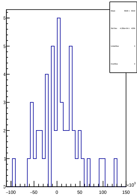
slug74: 1D Corr asym_atl2.mean/ppb-reg_asym_atl2.mean/ppb
