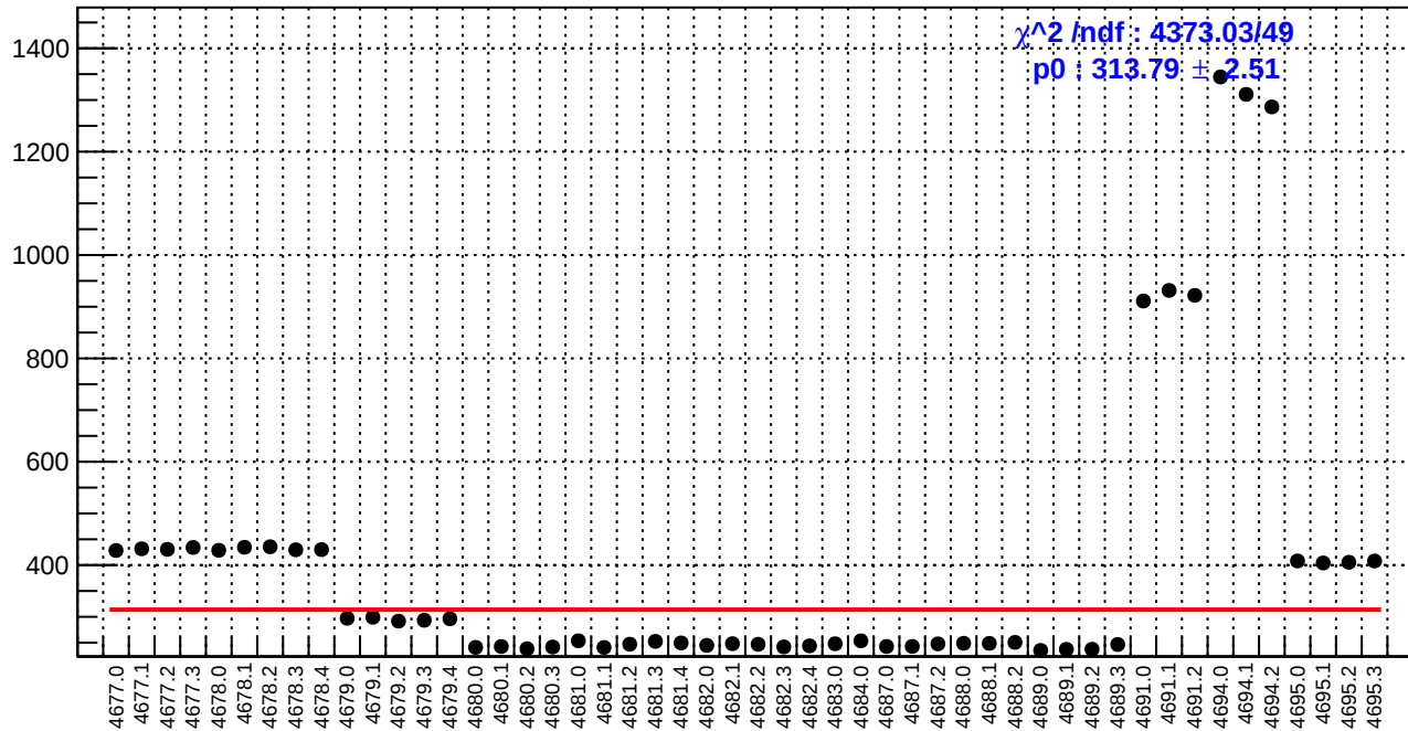
slug74: reg_asym_at2_avg.rms/ppm
