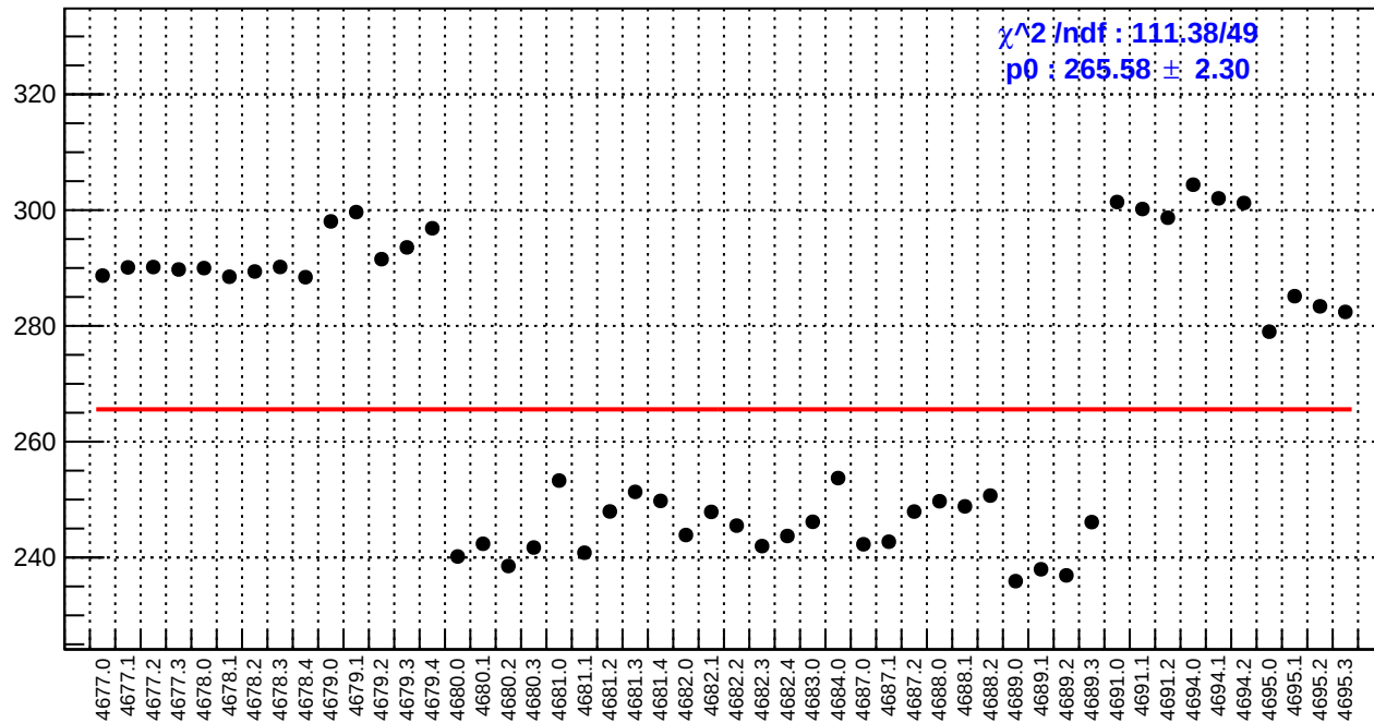
slug74: reg_asym_at2_dd.rms/ppm
