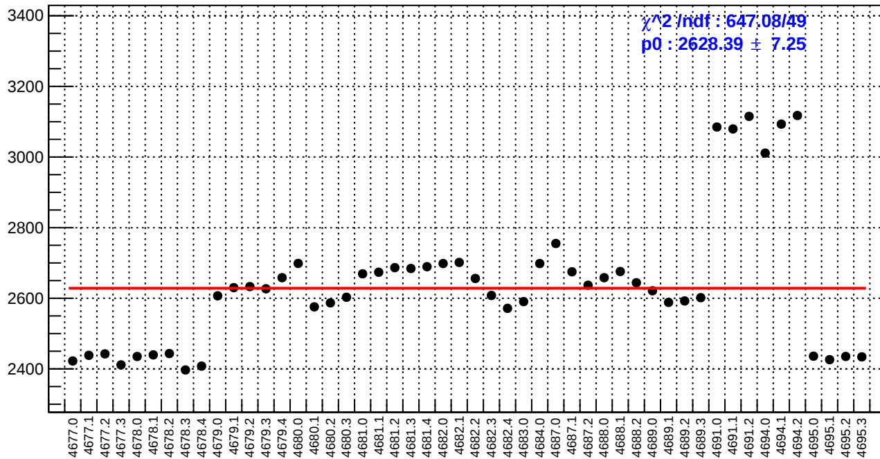
slug74: reg_asym_sam2.rms/ppm
