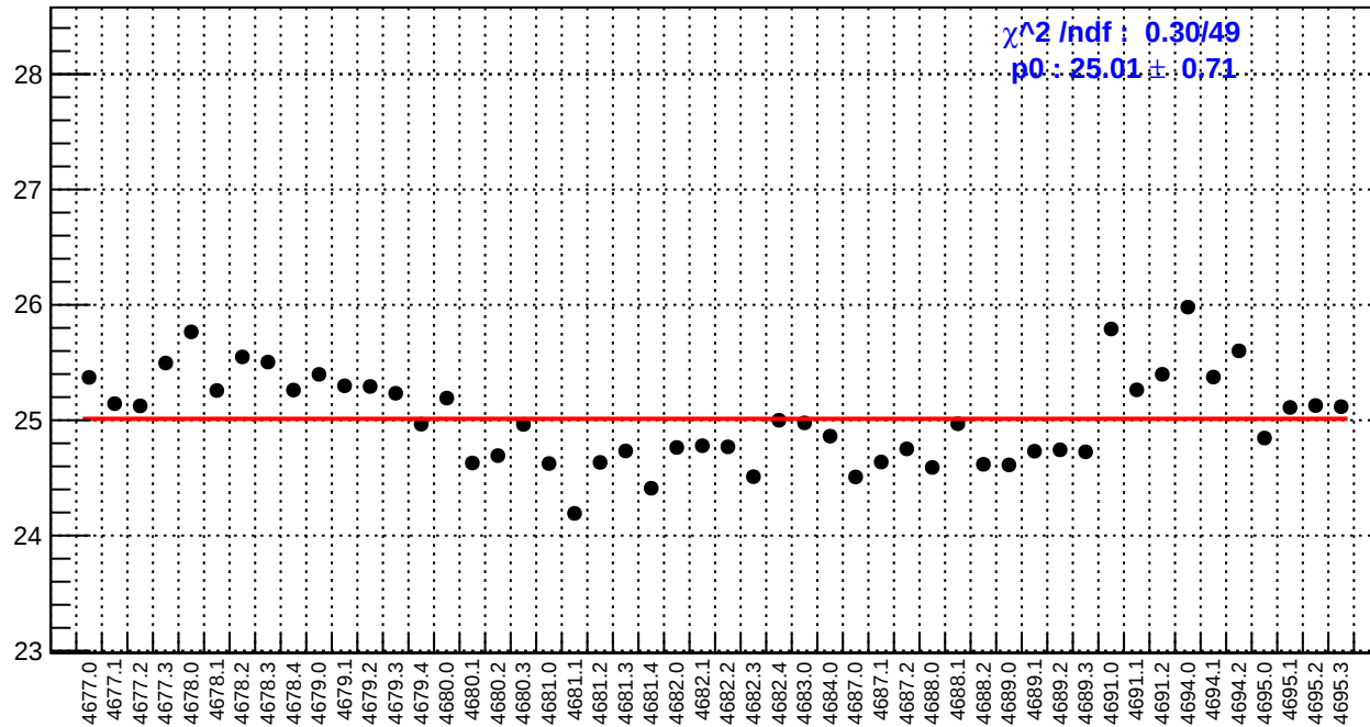
slug74: reg_asym_left_dd.rms/ppm
