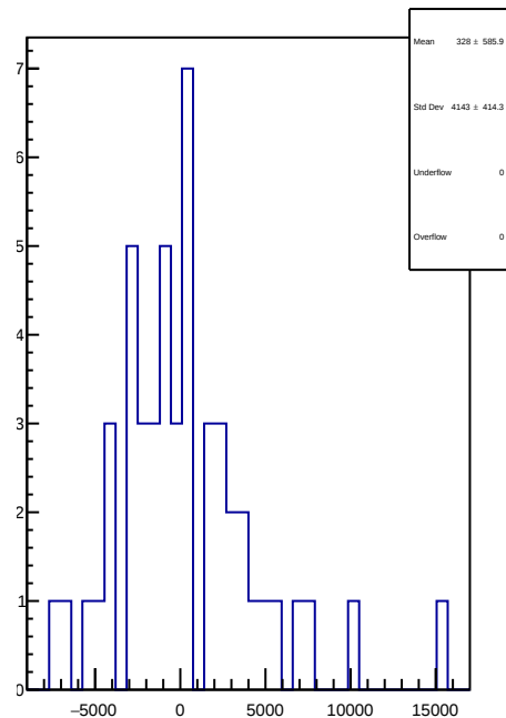
slug74: 1D Corr asym_ds_avg.mean/ppb-reg_asym_ds_avg.mean/ppb
