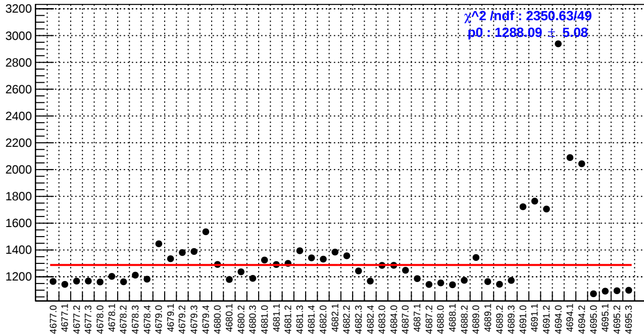
slug74: reg_asym_sam3.rms/ppm
