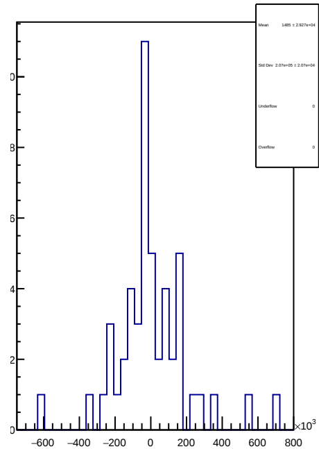
slug74: 1D Corr asym_sam3.mean/ppb-reg_asym_sam3.mean/ppb
