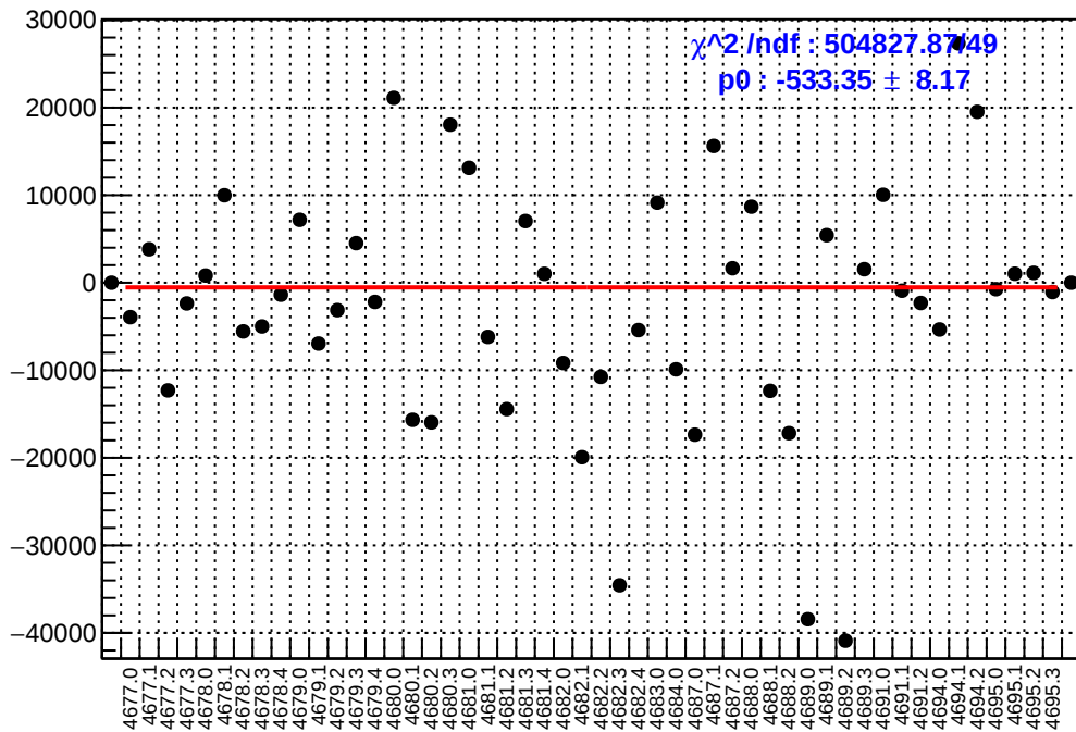
slug74: asym_sam5.mean/ppb-reg_asym_sam5.mean/ppb
