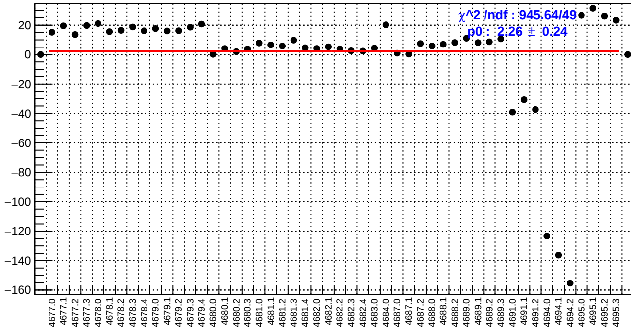
slug74: usl_bpm4aX/(ppb/nm)
