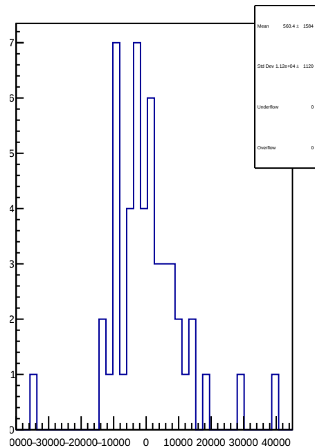
slug74: 1D Corr asym_usl.mean/ppb-reg_asym_usl.mean/ppb
