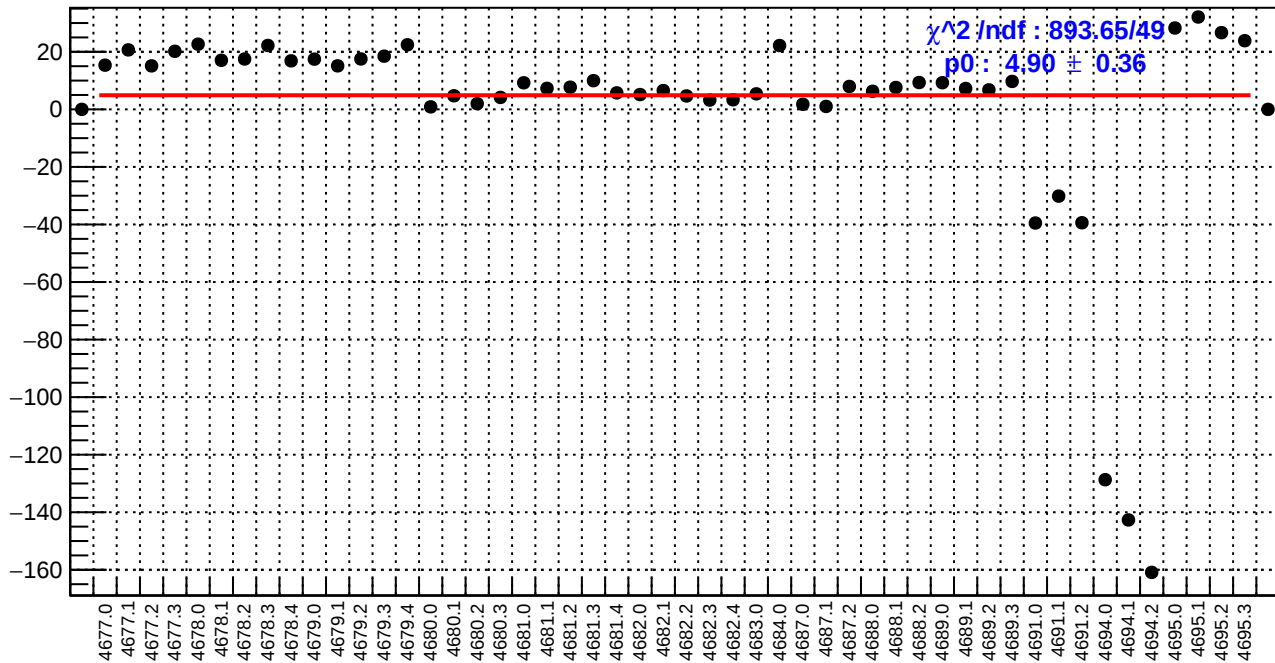
slug74: dsl_bpm4aX/(ppb/nm)
