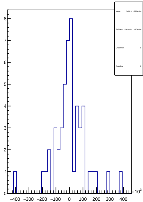
slug74: 1D Corr asym_sam2.mean/ppb-reg_asym_sam2.mean/ppb
