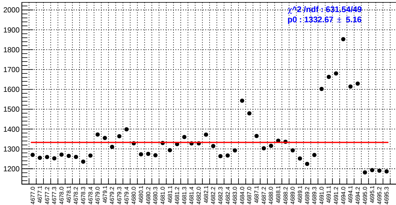
slug74: reg_asym_sam4.rms/ppm
