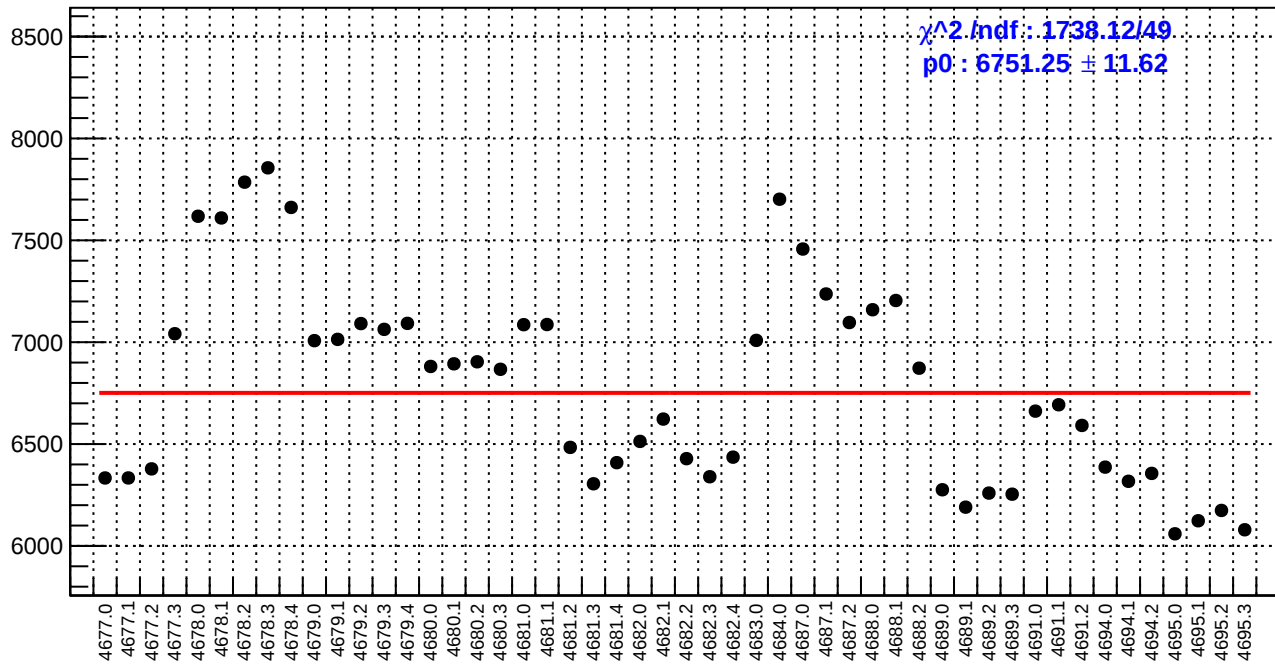
slug74: diff_bpm11X.rms/nm
