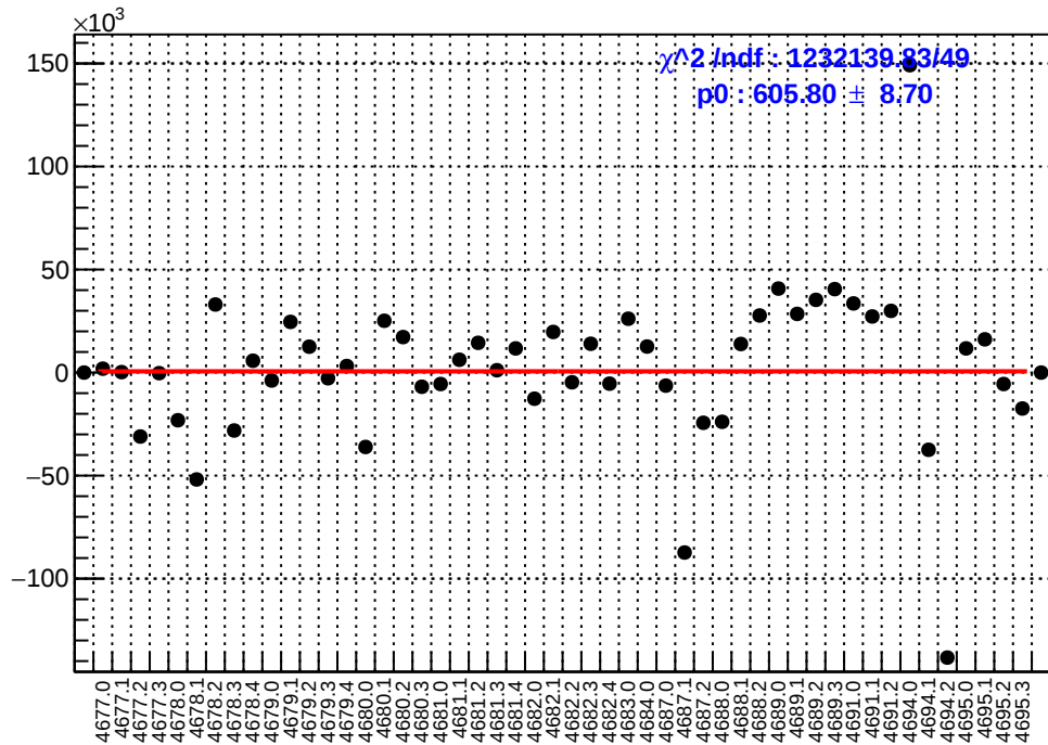
slug74: asym_sam8.mean/ppb-reg_asym_sam8.mean/ppb
