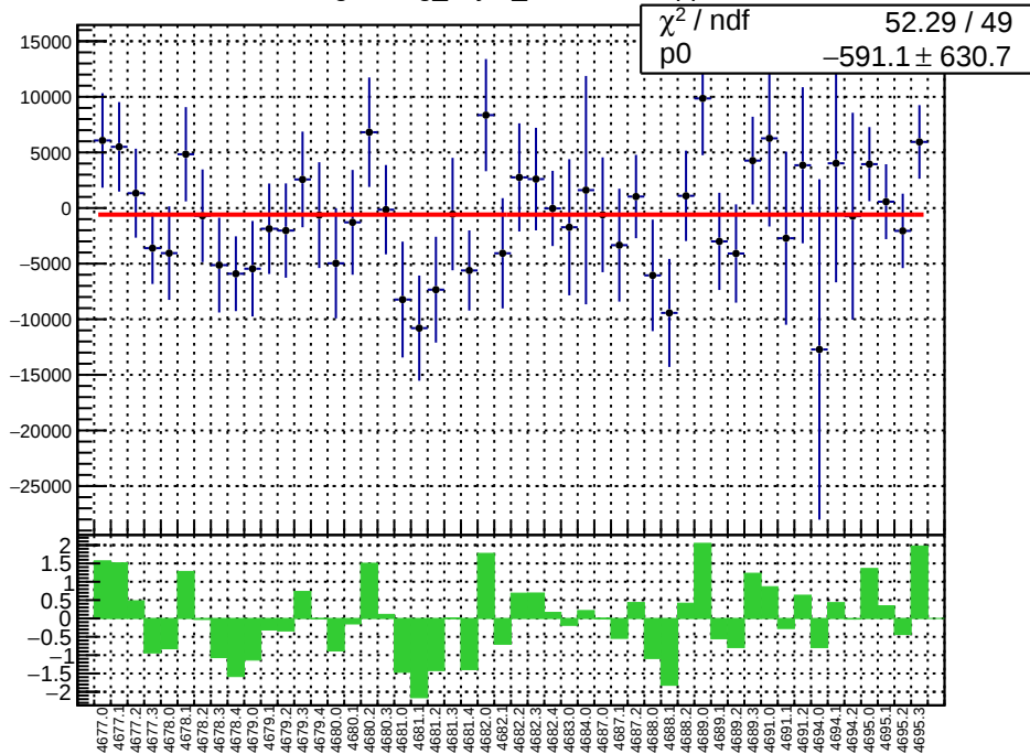
slug74: reg_asym_sam6.mean/ppb
