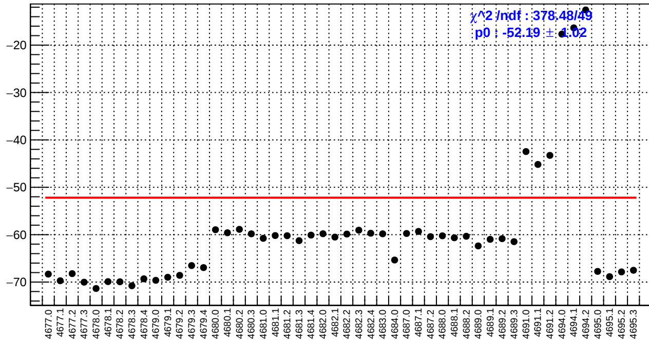
slug74: dsl_bpm4eX/(ppb/nm)
