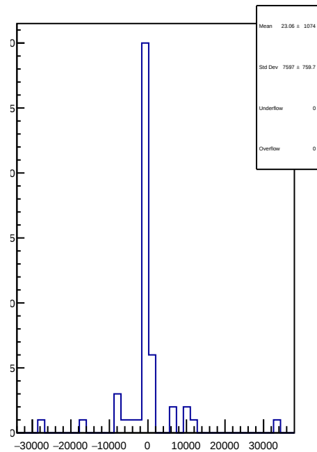
slug74: 1D Corr asym_usr.mean/ppb-reg_asym_usr.mean/ppb
