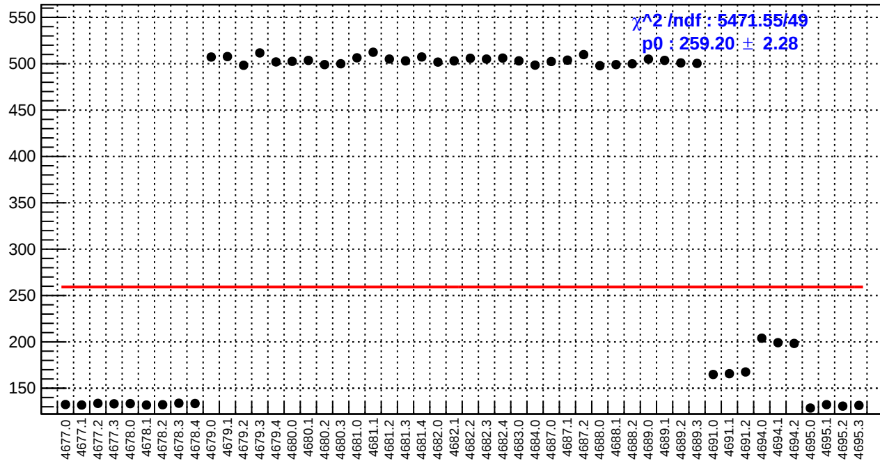
slug74: reg_asym_usr.rms/ppm
