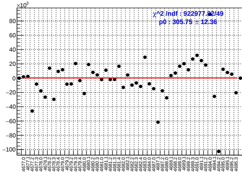
slug74: asym_atl_dd.mean/ppb-reg_asym_atl_dd.mean/ppb
