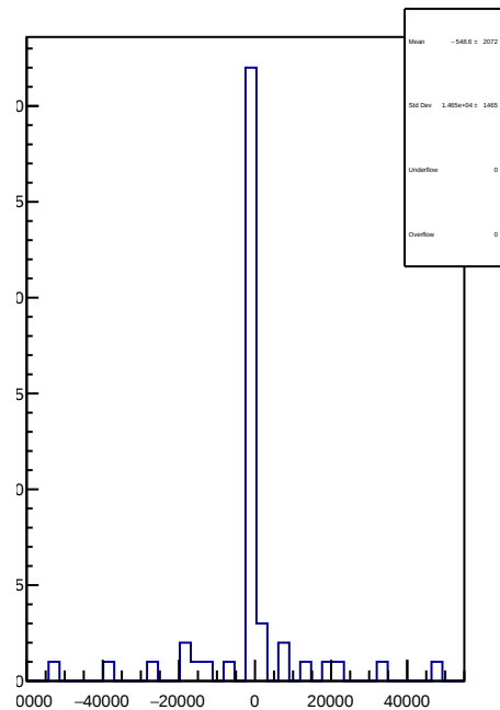
slug74: 1D Corr asym_atr_dd.mean/ppb-reg_asym_atr_dd.mean/ppb
