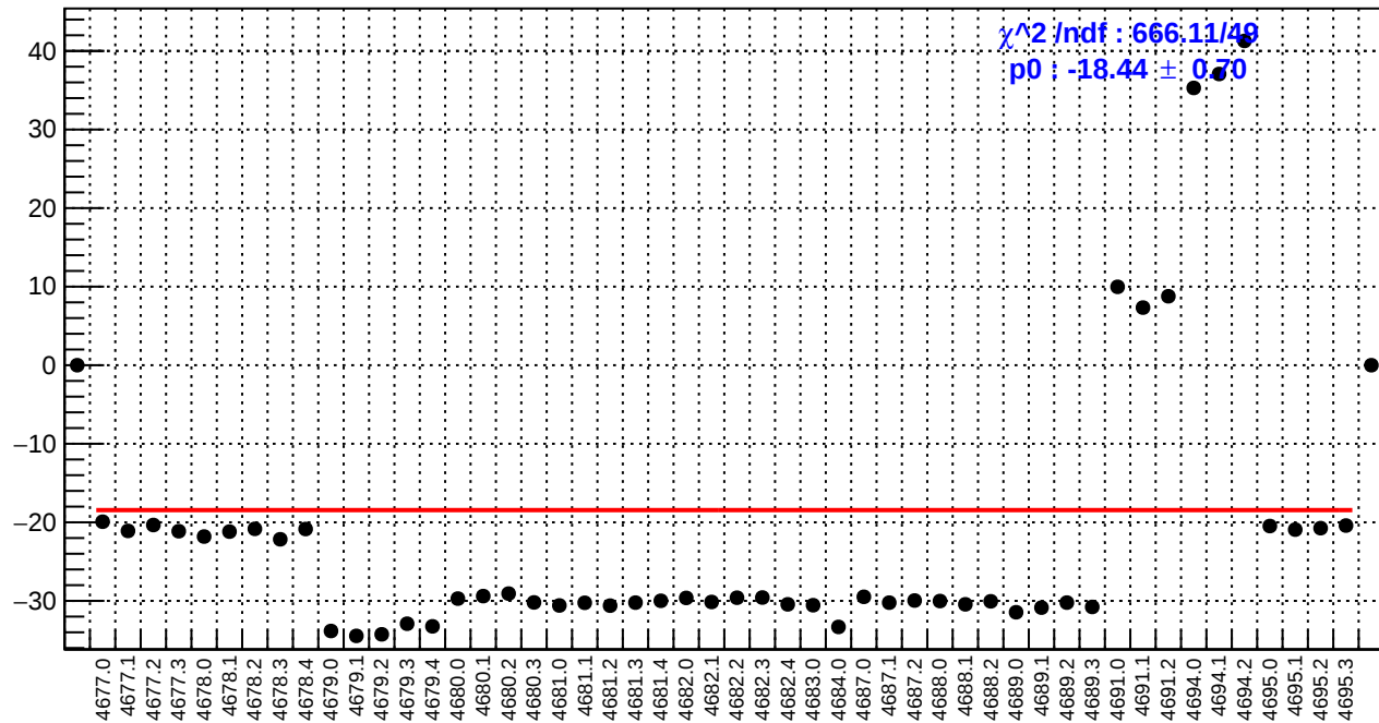
slug74: ds_avg_bpm4eX/(ppb/nm)
