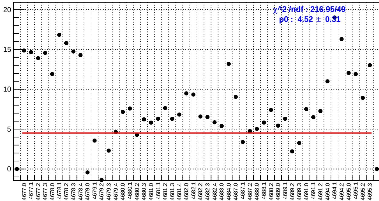
slug74: ds_avg_bpm4aY/(ppb/nm)
