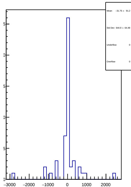
slug74: 1D Corr asym_right_dd.mean/ppb-reg_asym_right_dd.mean/ppb
