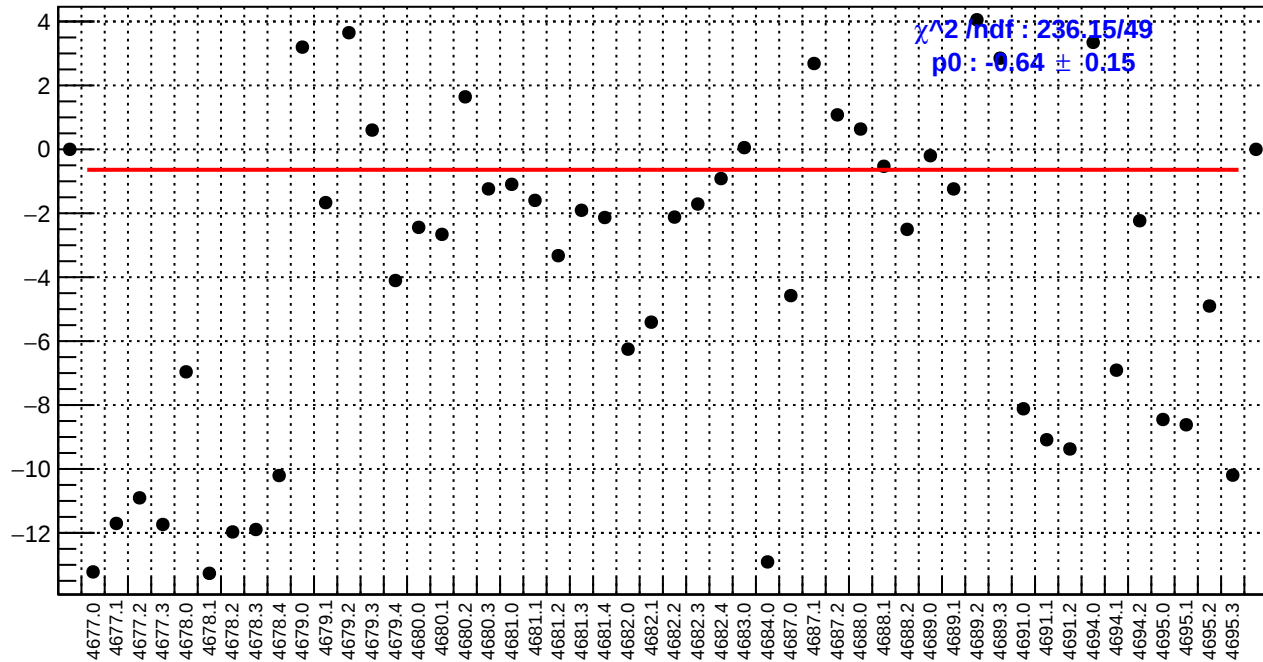
slug74: ds_avg_bpm4eY/(ppb/nm)
