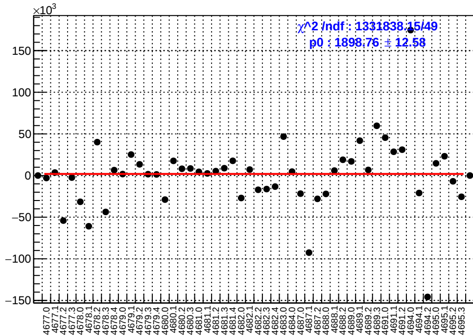
slug74: asym_sam7.mean/ppb-reg_asym_sam7.mean/ppb
