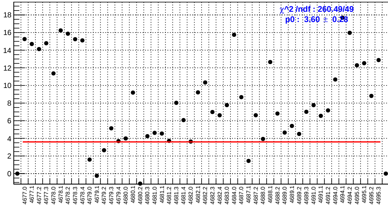
slug74: us_avg_bpm4aY/(ppb/nm)
