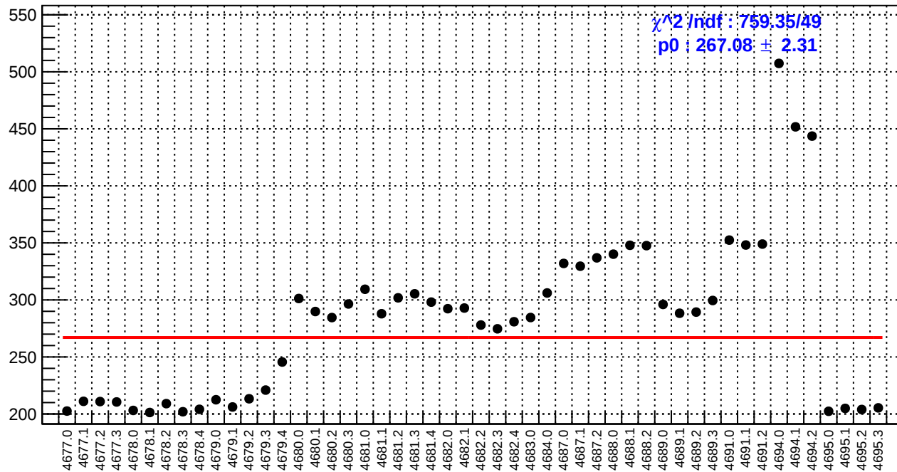
slug74: reg_asym_sam1.rms/ppm
