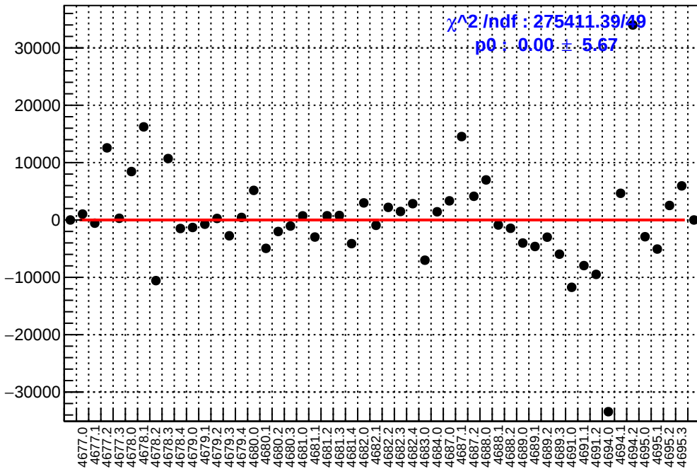
slug74: asym_us_dd.mean/ppb-reg_asym_us_dd.mean/ppb
