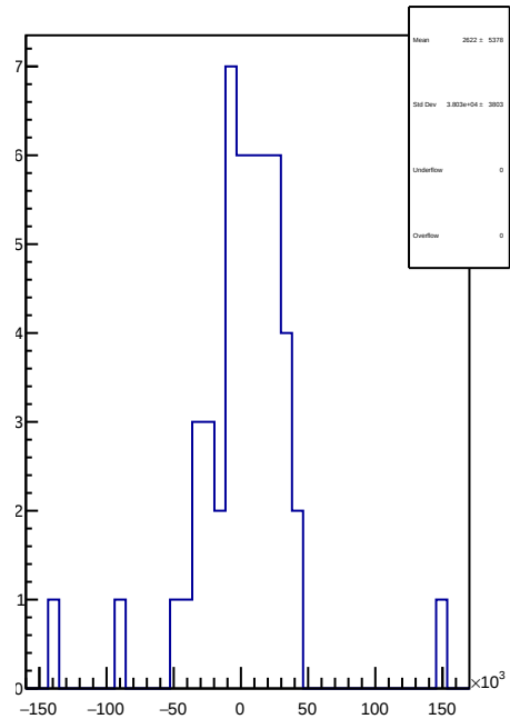
slug74: 1D Corr asym_sam8.mean/ppb-reg_asym_sam8.mean/ppb
