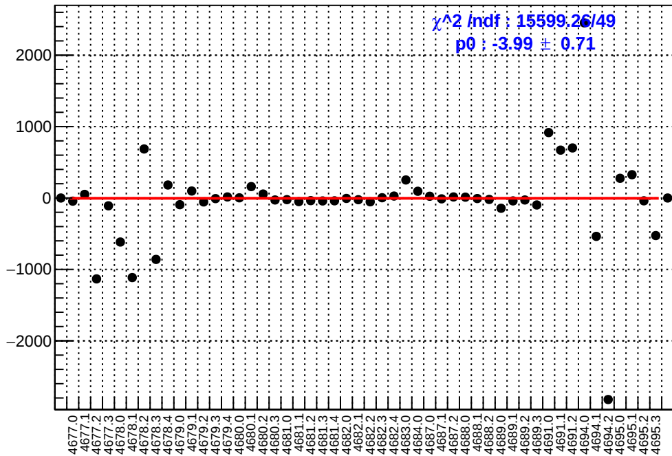
slug74: asym_right_dd.mean/ppb-reg_asym_right_dd.mean/ppb
