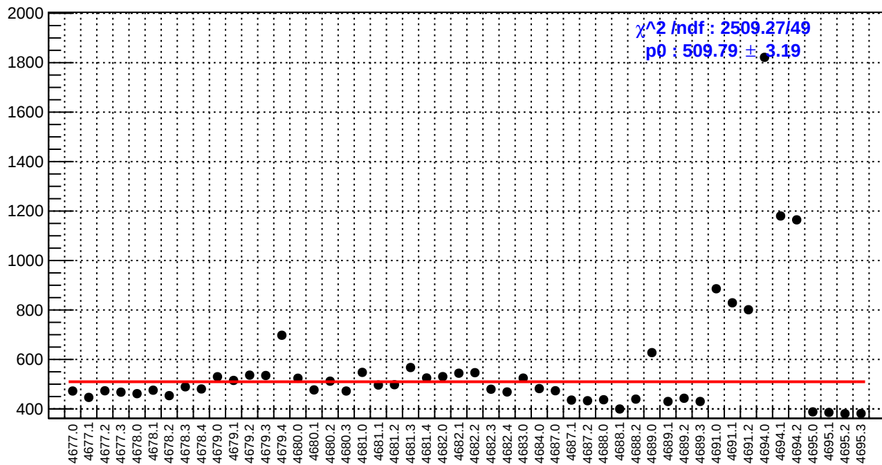
slug74: reg_asym_sam7.rms/ppm
