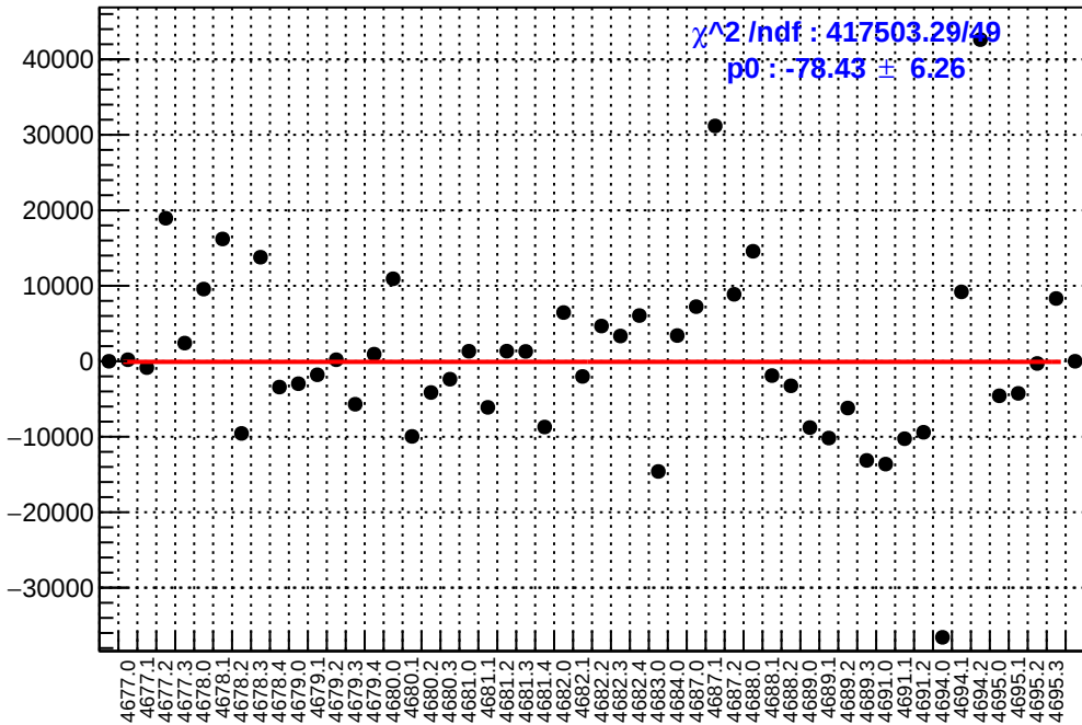
slug74: asym_dsl.mean/ppb-reg_asym_dsl.mean/ppb
