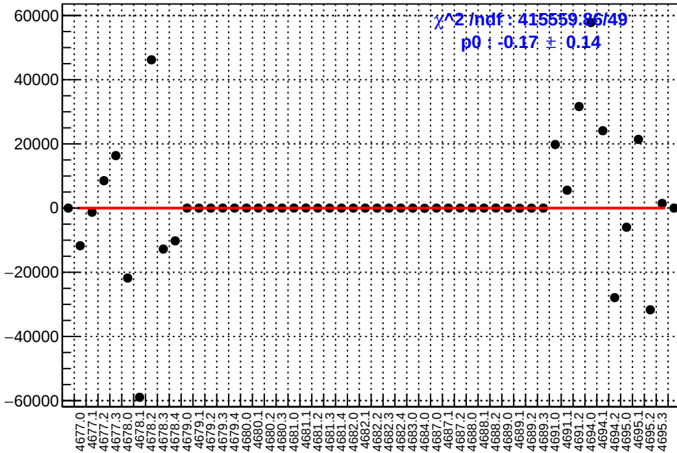
slug74: asym_atr2.mean/ppb-reg_asym_atr2.mean/ppb
