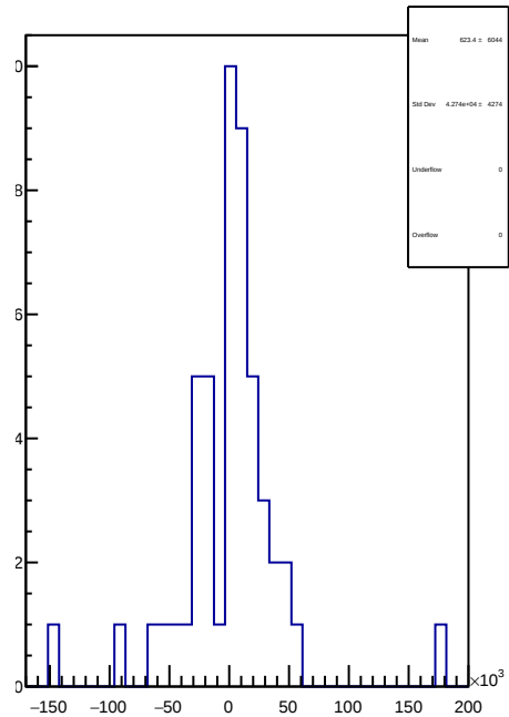
slug74: 1D Corr asym_sam7.mean/ppb-reg_asym_sam7.mean/ppb
