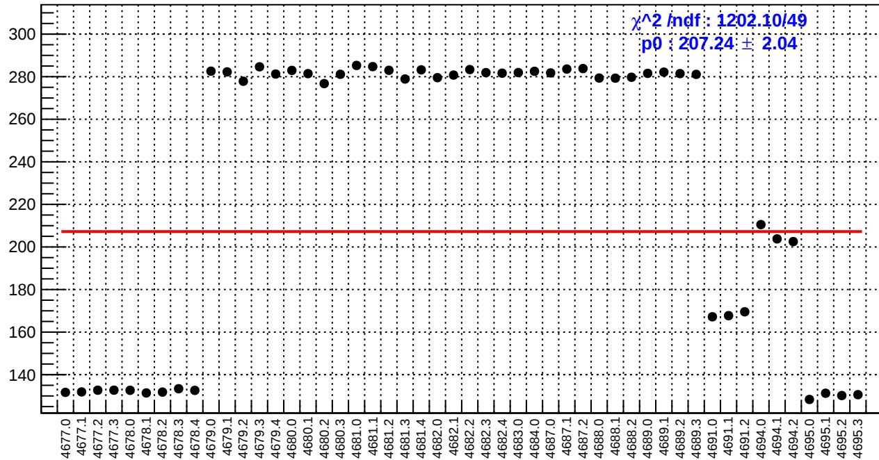
slug74: reg_asym_right_avg.rms/ppm
