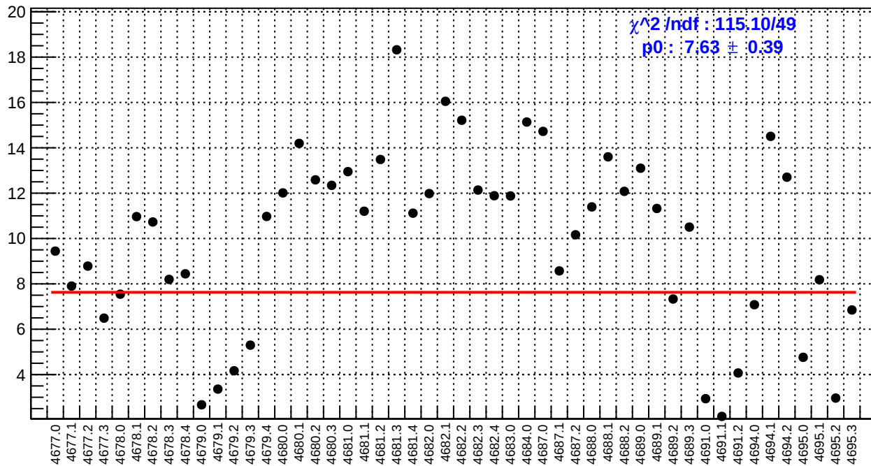
slug74: left_avg_bpm4aY/(ppb/nm)
