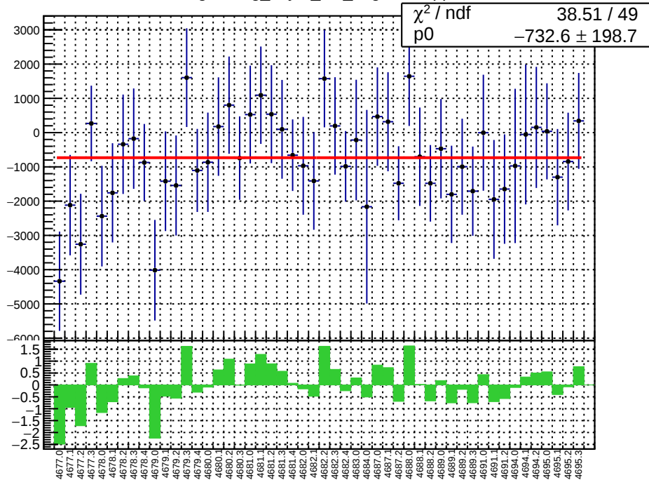
slug74: reg_asym_left_avg.mean/ppb
