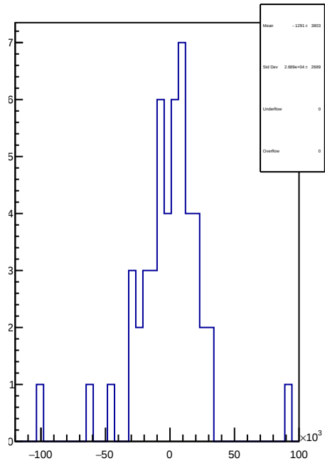
slug74: 1D Corr asym_atl_dd.mean/ppb-reg_asym_atl_dd.mean/ppb
