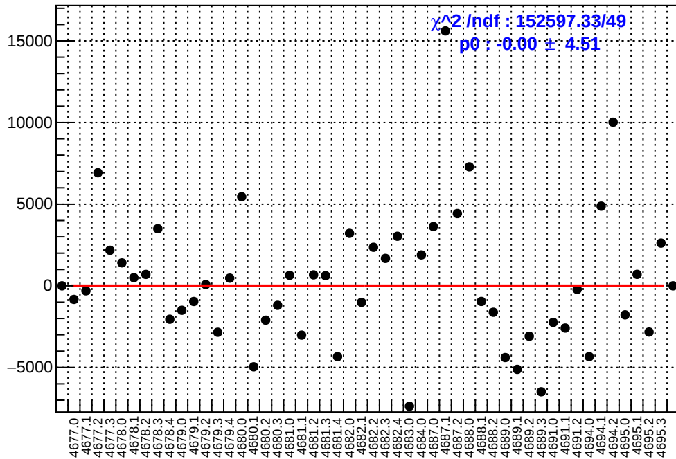
slug74: asym_ds_avg.mean/ppb-reg_asym_ds_avg.mean/ppb
