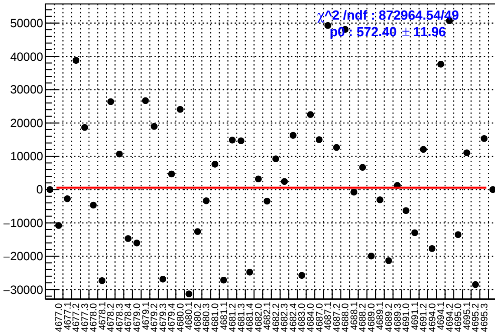
slug74: asym_at2_avg.mean/ppb-reg_asym_at2_avg.mean/ppb
