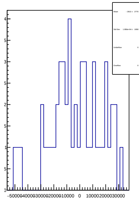
slug74: 1D Corr asym_atr1l2_dd.mean/ppb-reg_asym_atr1l2_dd.mean/ppb
