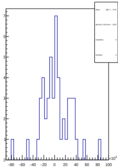
slug74: 1D Corr asym_atl1.mean/ppb-reg_asym_atl1.mean/ppb
