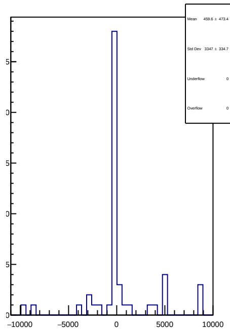
slug74: 1D Corr asym_atr_avg.mean/ppb-reg_asym_atr_avg.mean/ppb
