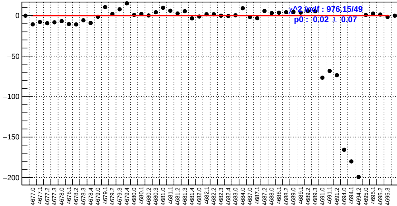
slug74: us_avg_bpm4aX/(ppb/nm)
