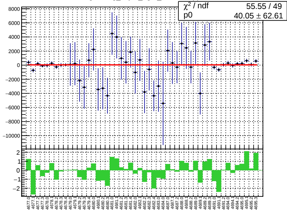
slug74: reg_asym_right_dd.mean/ppb
