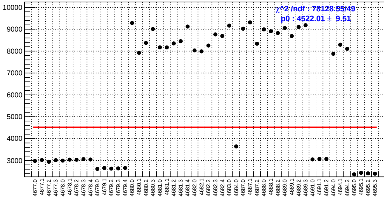
slug74: diff_bpm4eY.rms/nm
