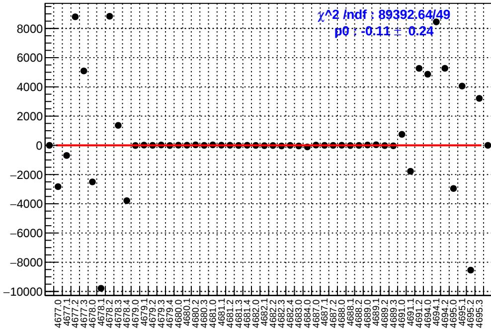
slug74: asym_atr_avg.mean/ppb-reg_asym_atr_avg.mean/ppb
