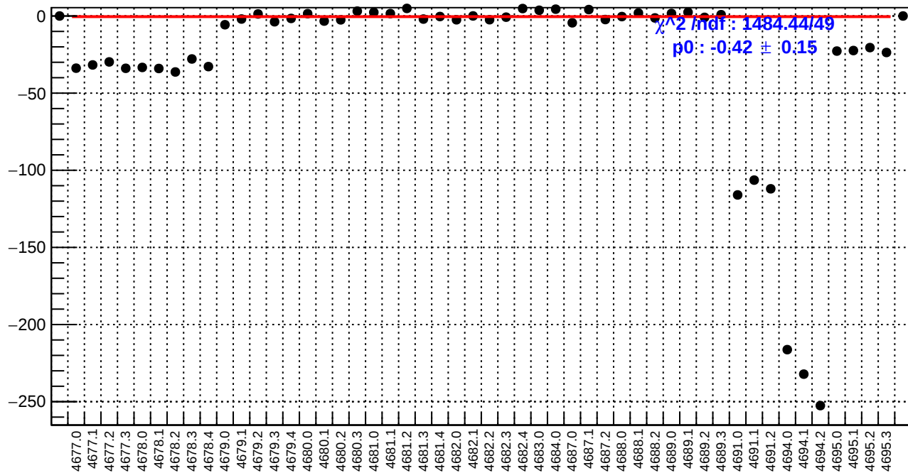
slug74: dsr_bpm4aX/(ppb/nm)
