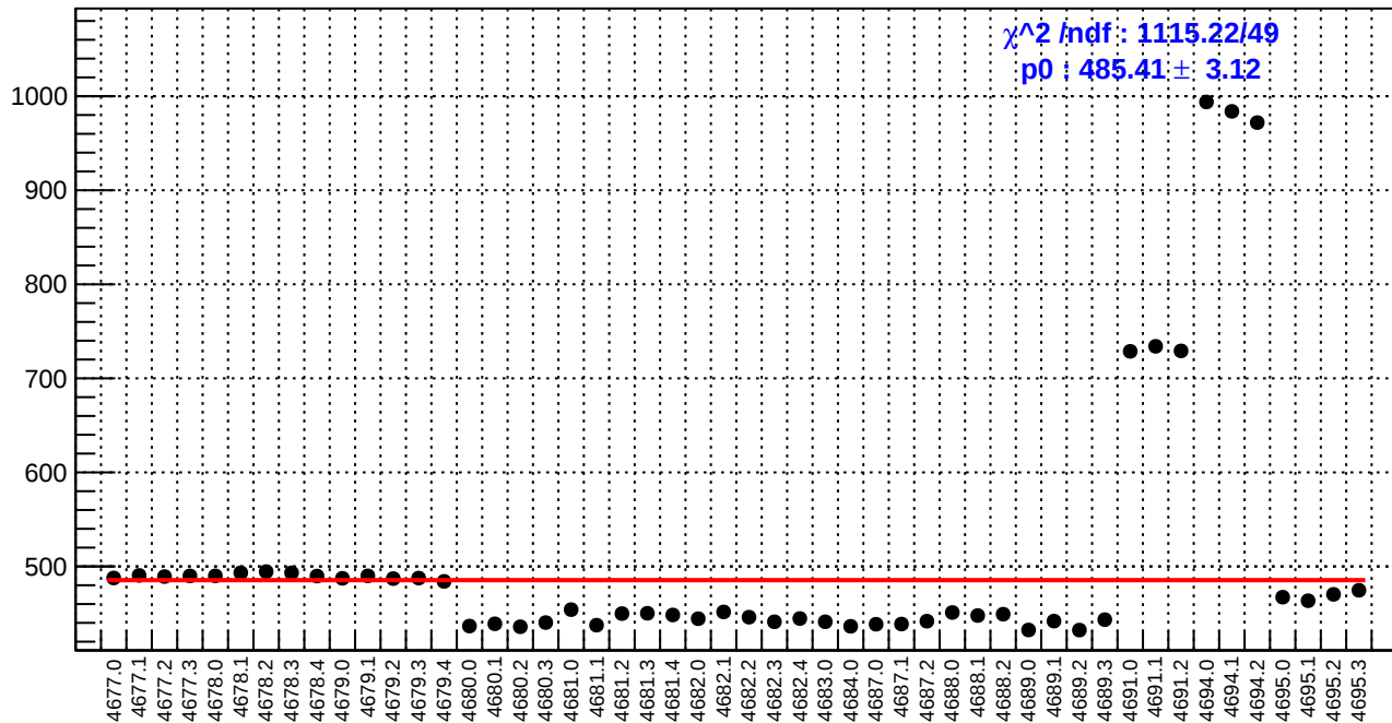
slug74: reg_asym_atl_avg.rms/ppm
