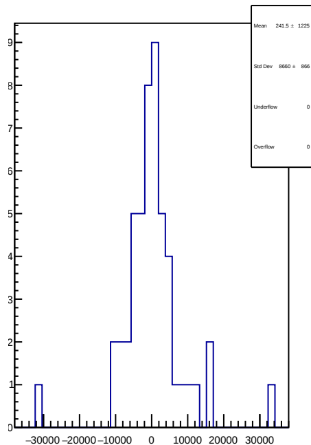
slug74: 1D Corr asym_ds_dd.mean/ppb-reg_asym_ds_dd.mean/ppb
