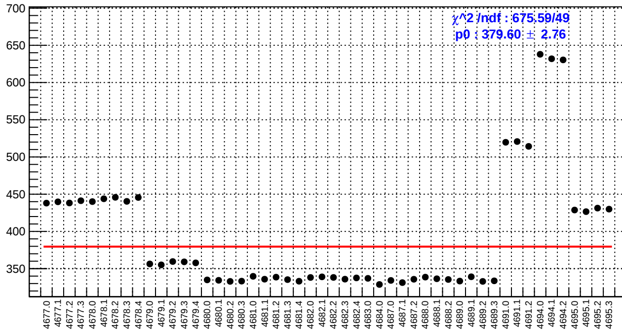
slug74: reg_asym_at1_dd.rms/ppm
