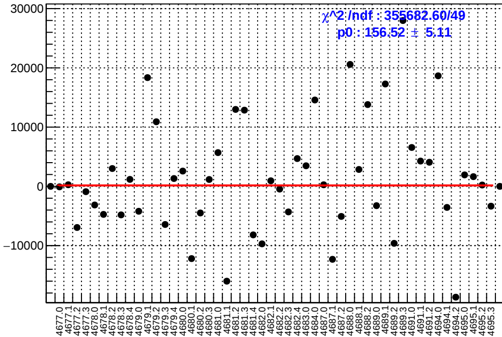
slug74: asym_at1_avg.mean/ppb-reg_asym_at1_avg.mean/ppb
