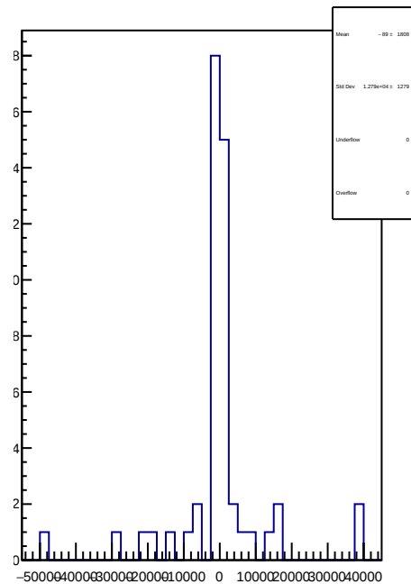
slug74: 1D Corr asym_atr1.mean/ppb-reg_asym_atr1.mean/ppb
