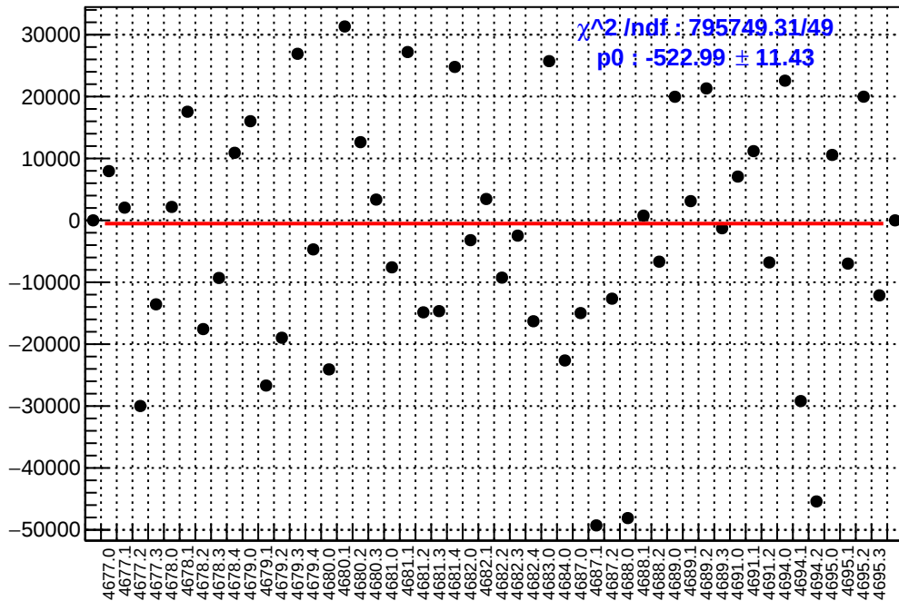
slug74: asym_atr1l2_dd.mean/ppb-reg_asym_atr1l2_dd.mean/ppb
