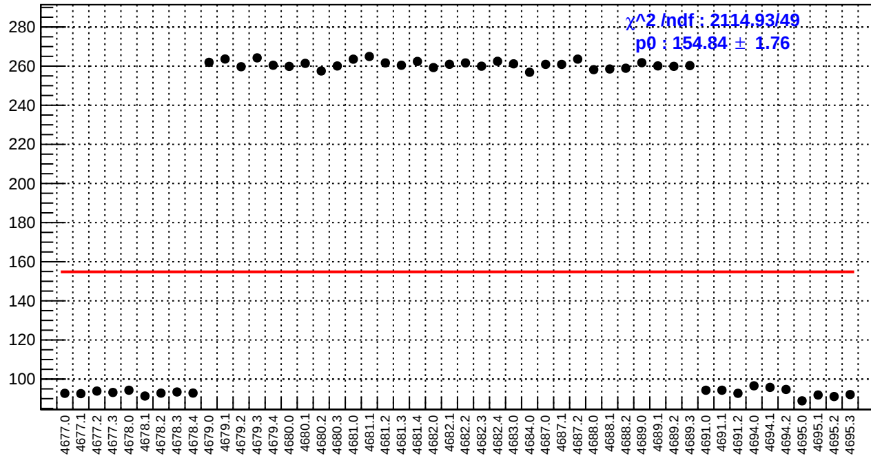
slug74: reg_asym_us_dd.rms/ppm
