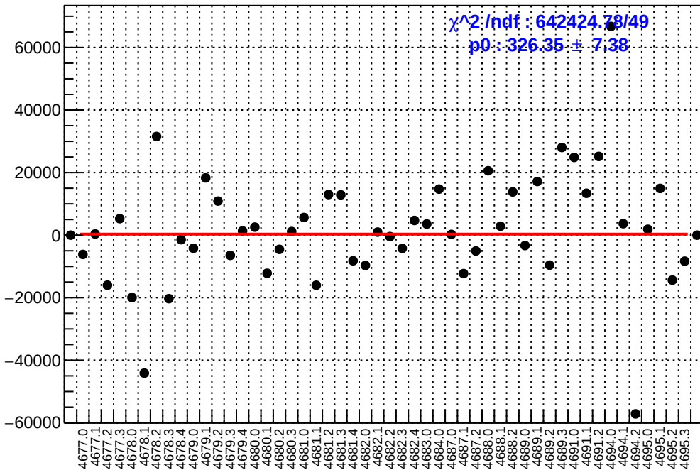
slug74: asym_at1_dd.mean/ppb-reg_asym_at1_dd.mean/ppb
