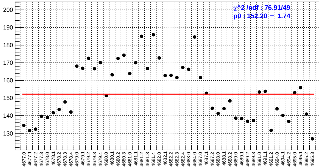
slug74: asym_bcm_an_ds.rms/ppm
