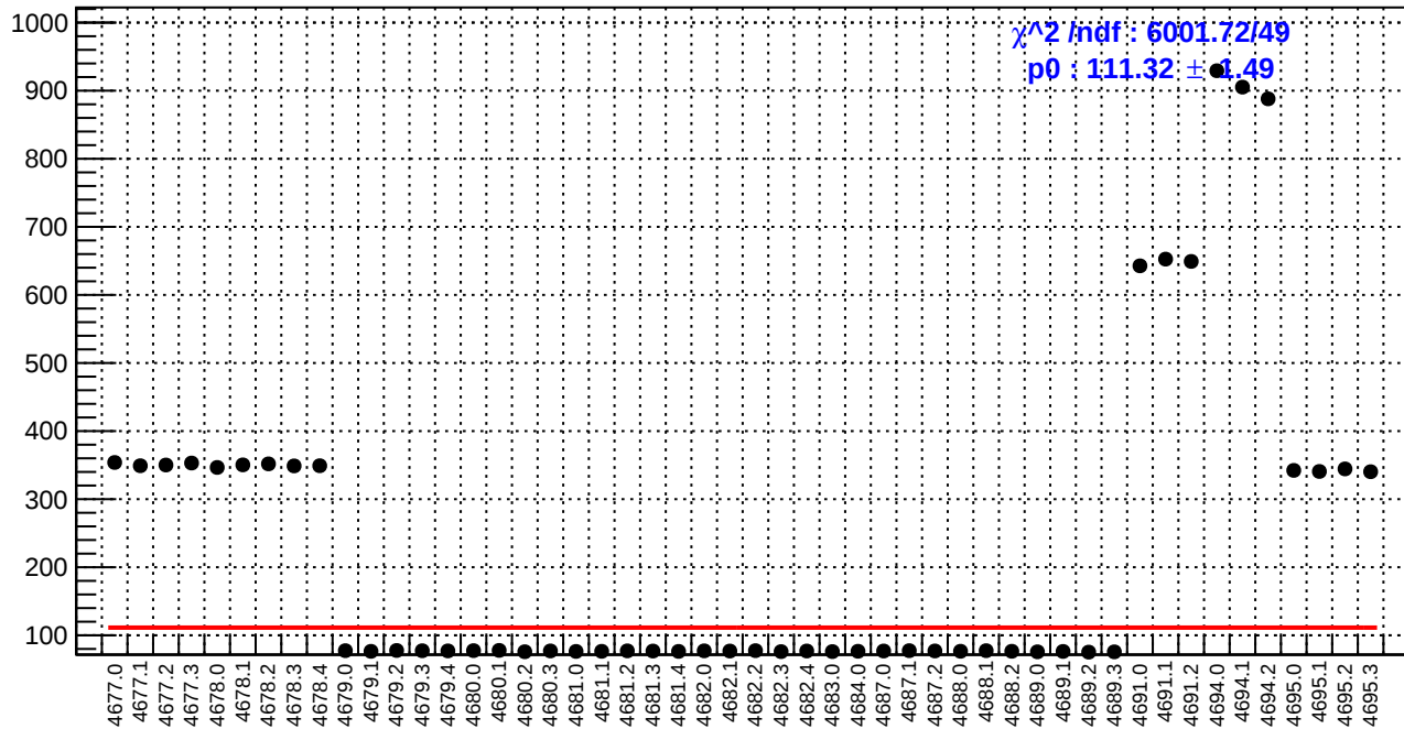
slug74: reg_asym_atr_dd.rms/ppm
