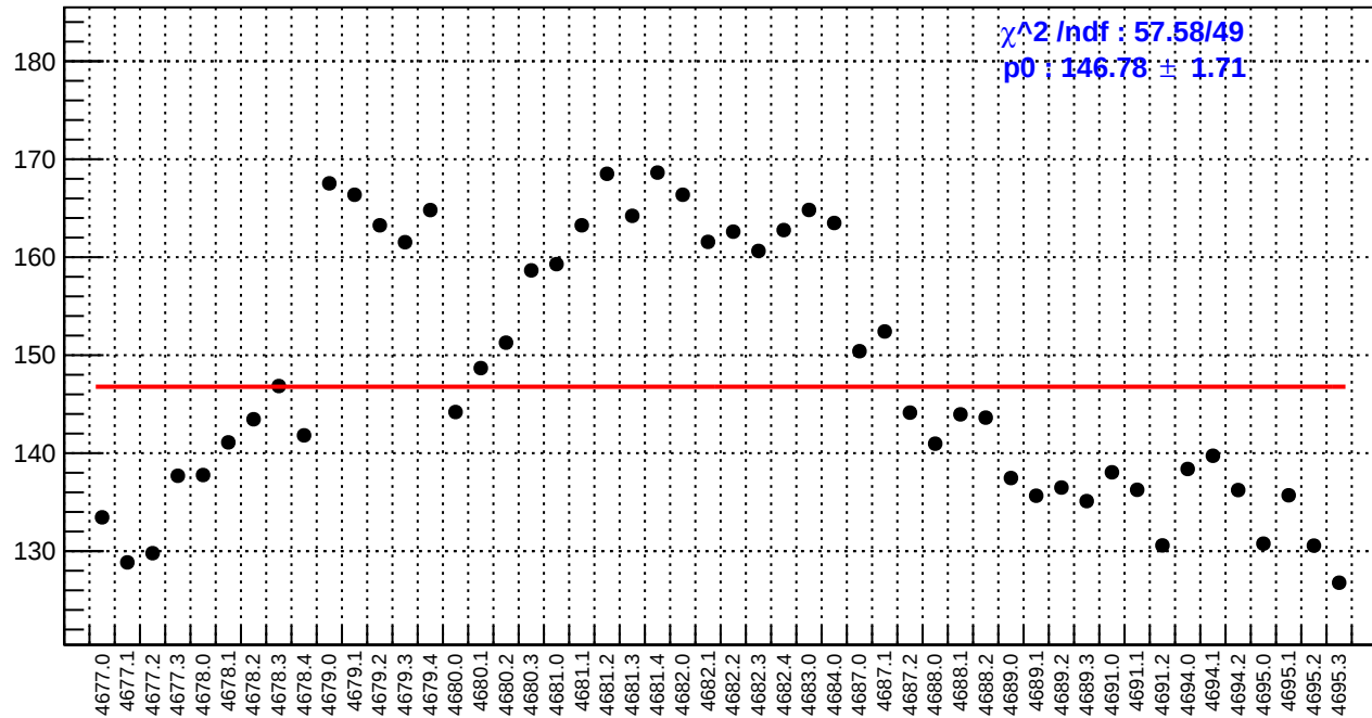
slug74: asym_bcm_an_us.rms/ppm
