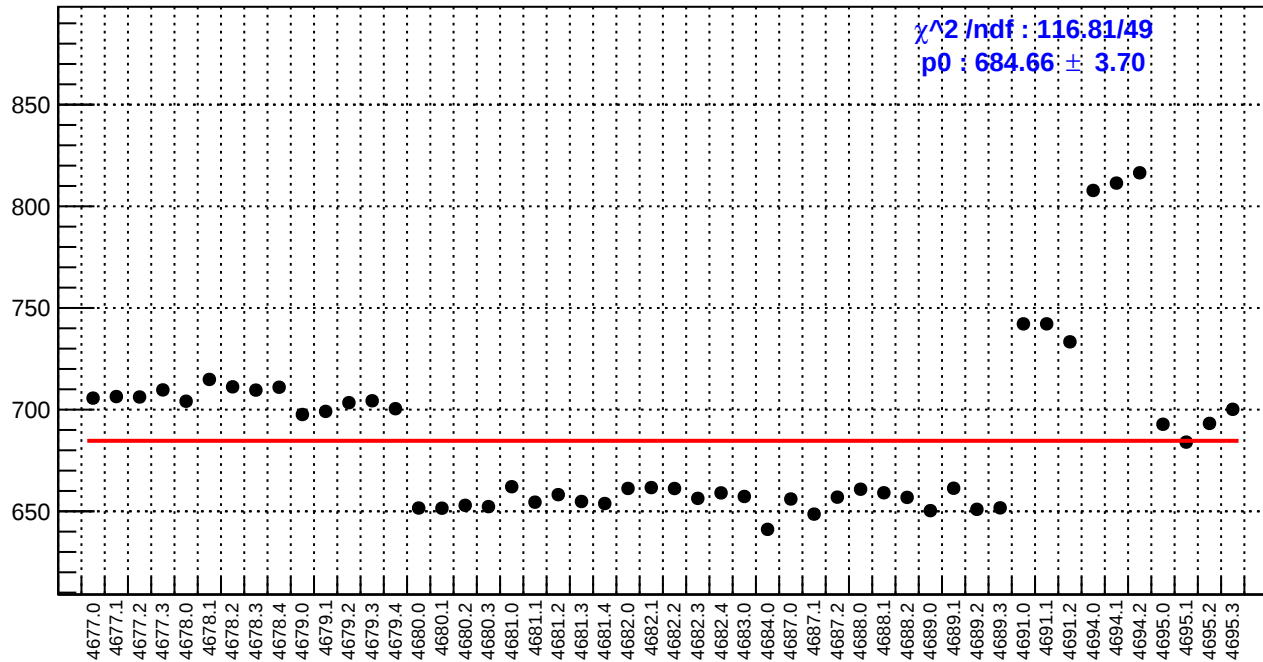
slug74: reg_asym_atl1.rms/ppm
