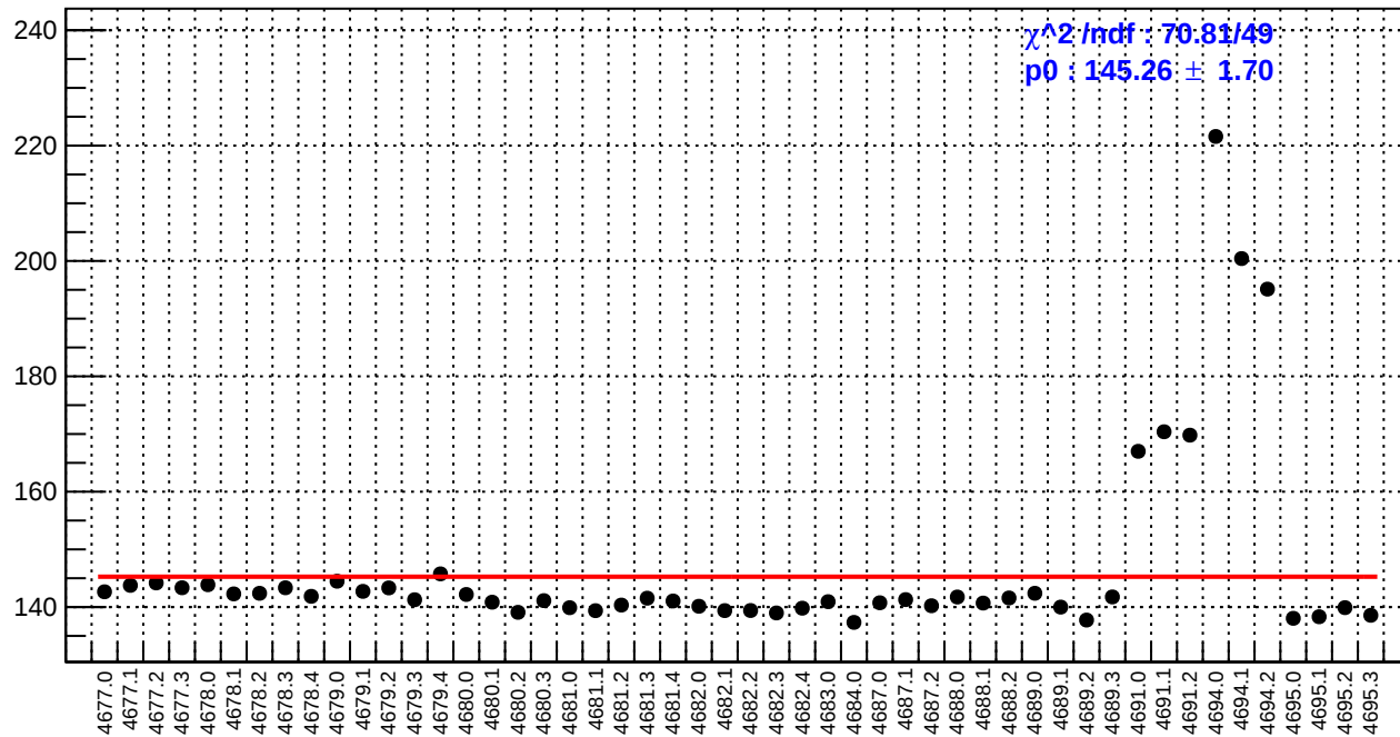
slug74: reg_asym_dsl.rms/ppm
