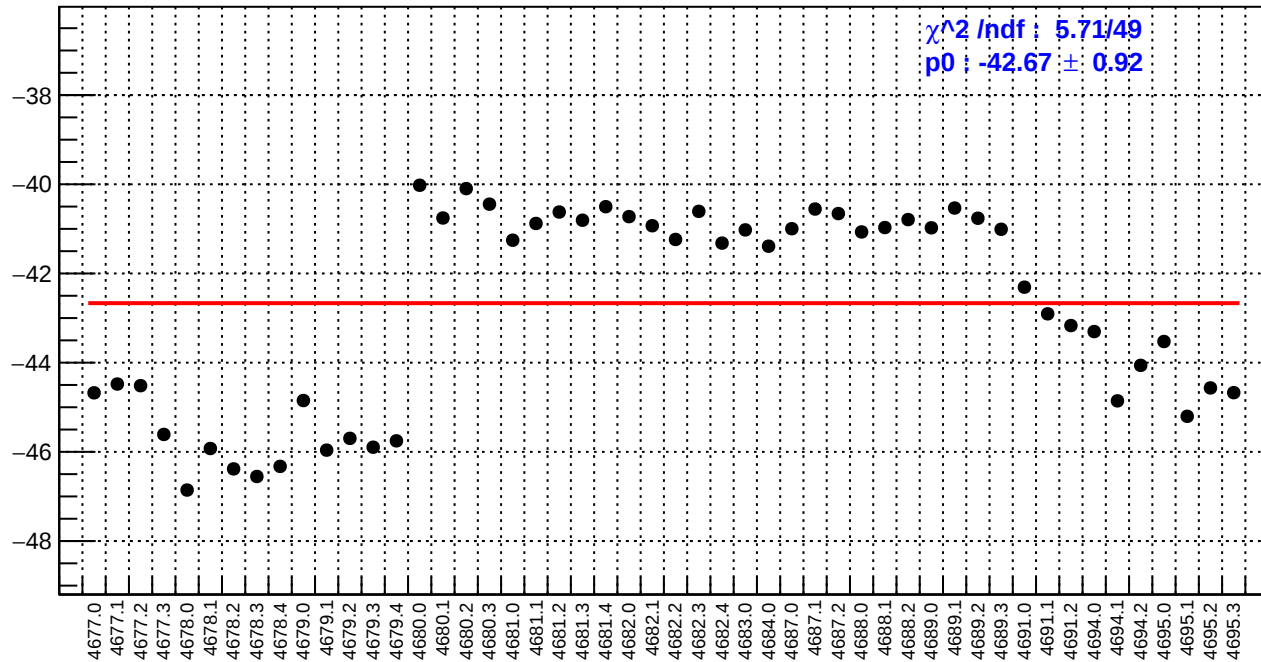
slug74: left_avg_bpm12X/(ppb/nm)
