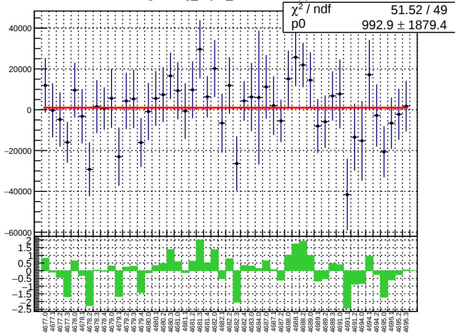
slug74: reg_asym_sam4.mean/ppb
