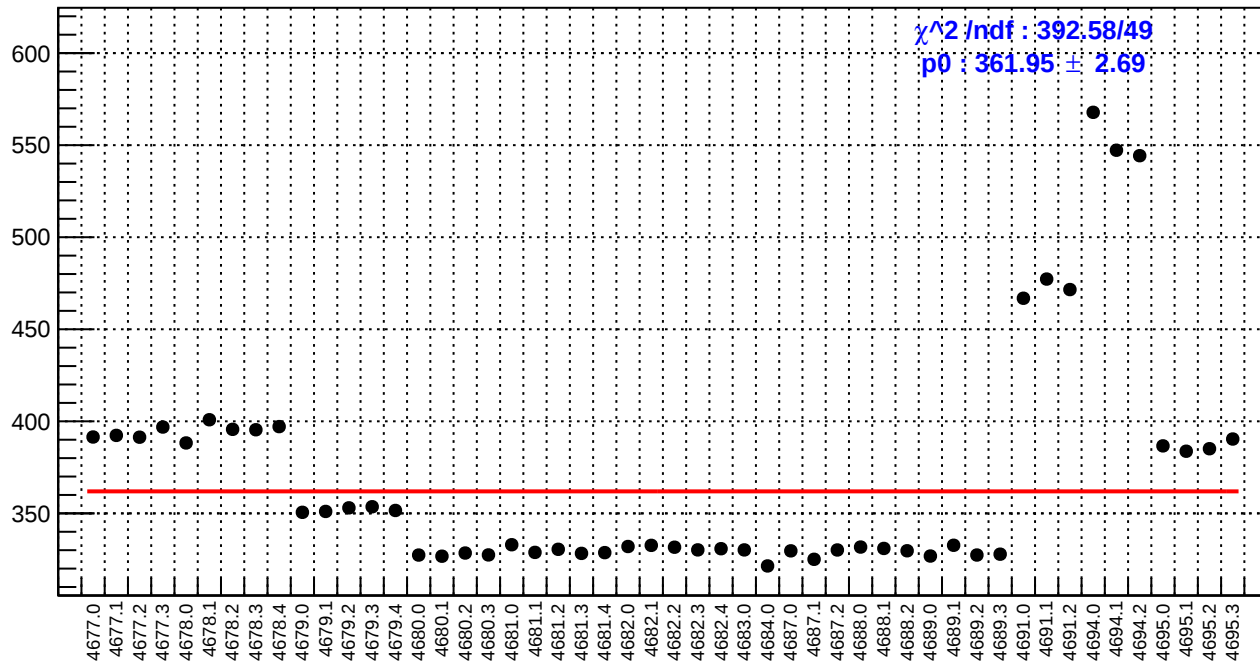
slug74: reg_asym_atl1r2_dd.rms/ppm
