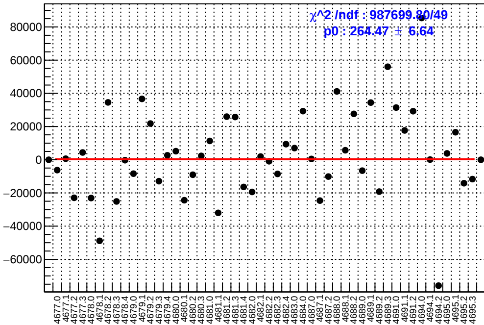
slug74: asym_atl1.mean/ppb-reg_asym_atl1.mean/ppb
