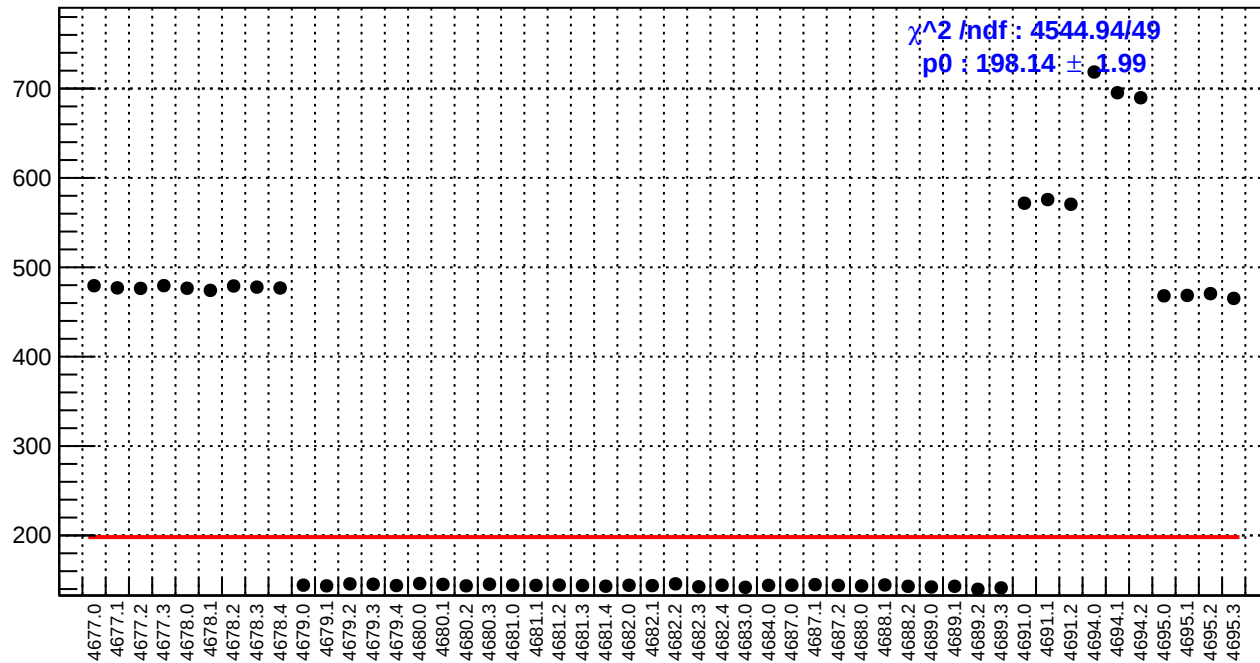
slug74: reg_asym_atr1.rms/ppm
