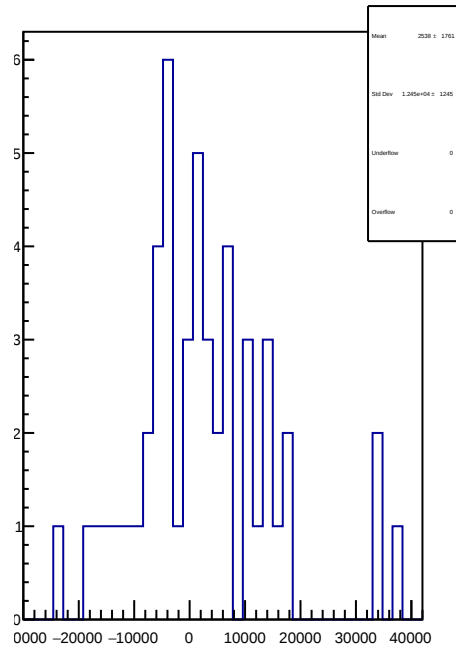
slug74: 1D Corr asym_sam1.mean/ppb-reg_asym_sam1.mean/ppb
