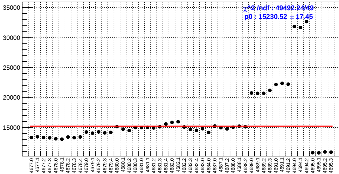
slug74: diff_bpm4eX.rms/nm
