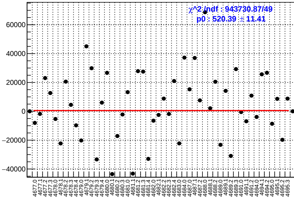
slug74: asym_atl_avg.mean/ppb-reg_asym_atl_avg.mean/ppb
