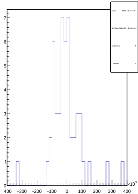
slug74: 1D Corr asym_sam4.mean/ppb-reg_asym_sam4.mean/ppb
