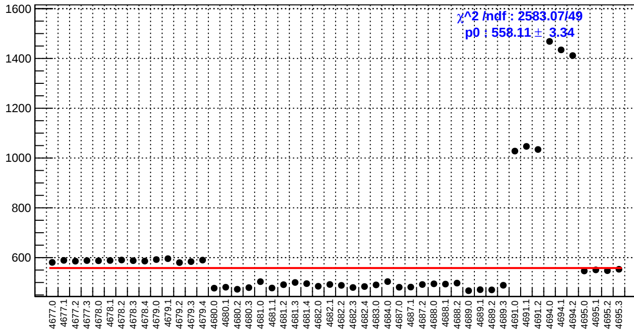
slug74: reg_asym_atl2.rms/ppm
