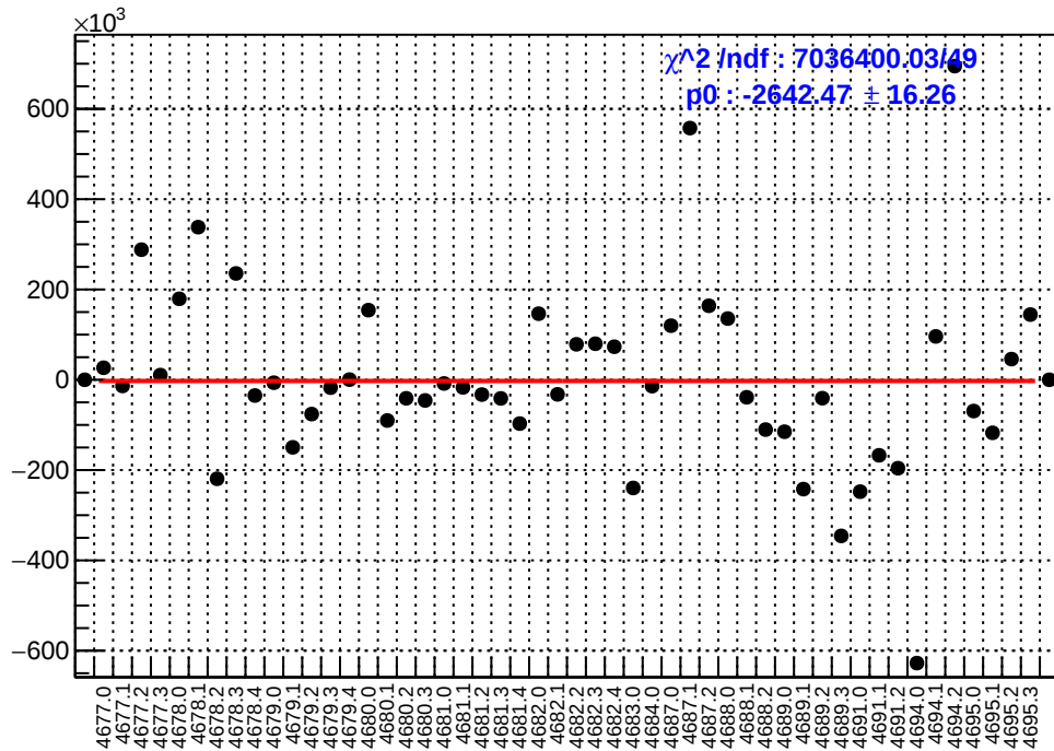
slug74: asym_sam3.mean/ppb-reg_asym_sam3.mean/ppb
