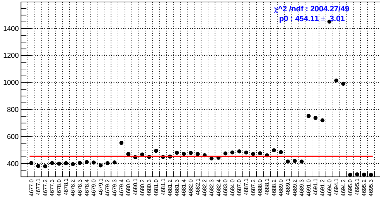
slug74: reg_asym_sam6.rms/ppm
