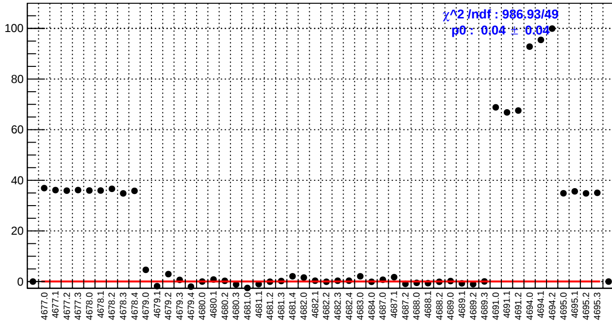
slug74: usr_bpm4eX/(ppb/nm)
