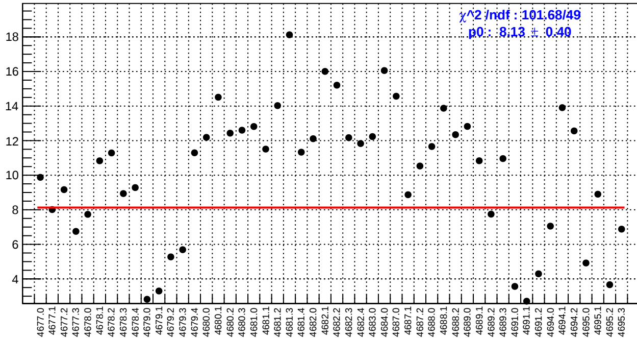
slug74: usl_bpm4aY/(ppb/nm)
