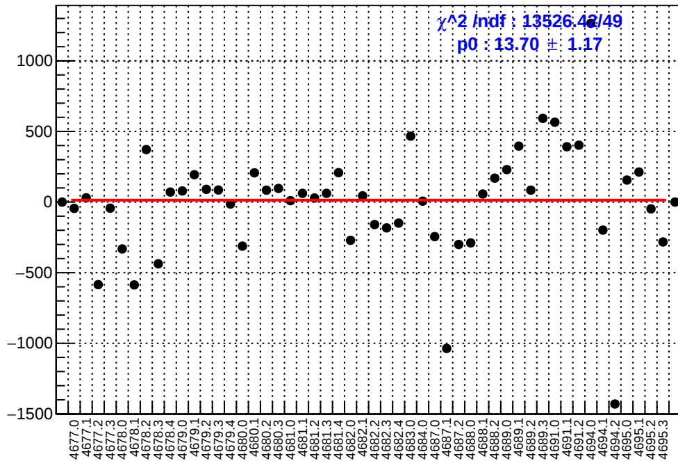
slug74: asym_left_dd.mean/ppb-reg_asym_left_dd.mean/ppb
