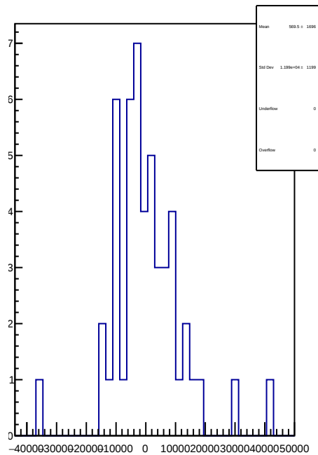
slug74: 1D Corr asym_dsl.mean/ppb-reg_asym_dsl.mean/ppb
