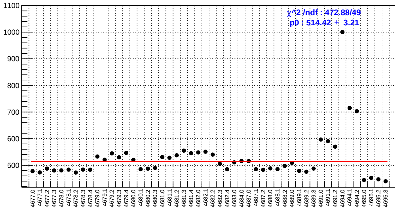
slug74: reg_asym_sam8.rms/ppm
