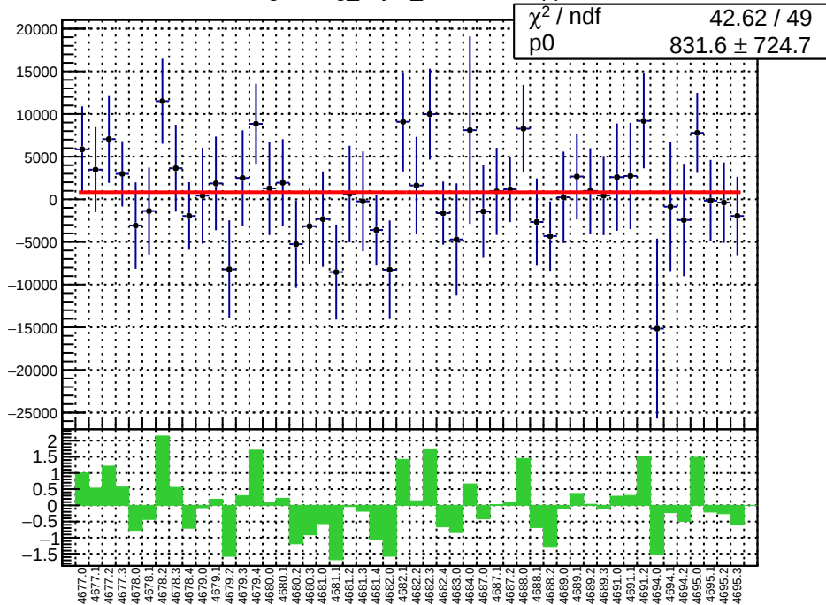
slug74: reg_asym_sam8.mean/ppb
