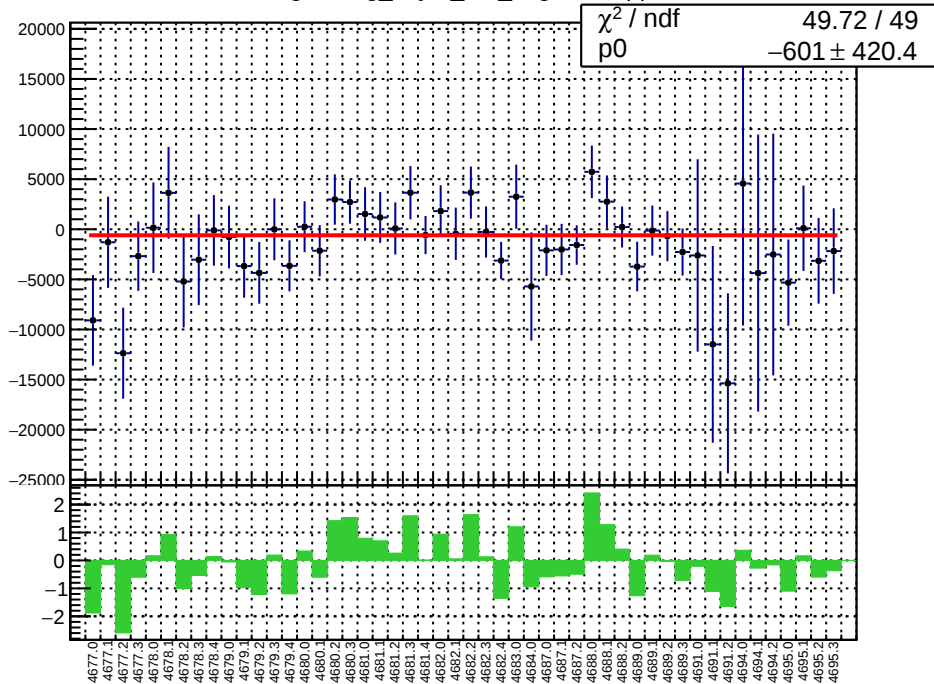
slug74: reg_asym_at2_avg.mean/ppb
