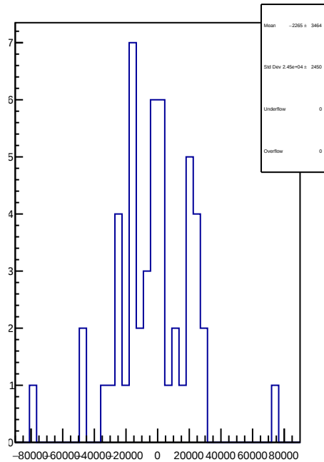
slug74: 1D Corr asym_at2_dd.mean/ppb-reg_asym_at2_dd.mean/ppb
