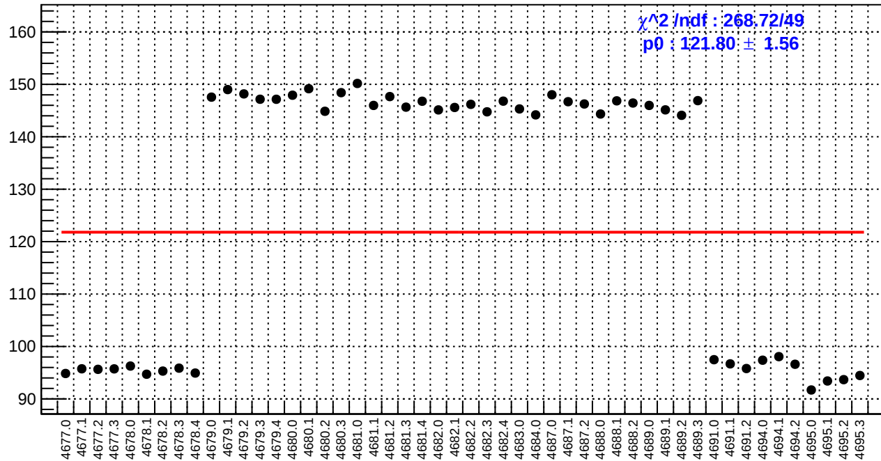
slug74: reg_asym_ds_dd.rms/ppm
