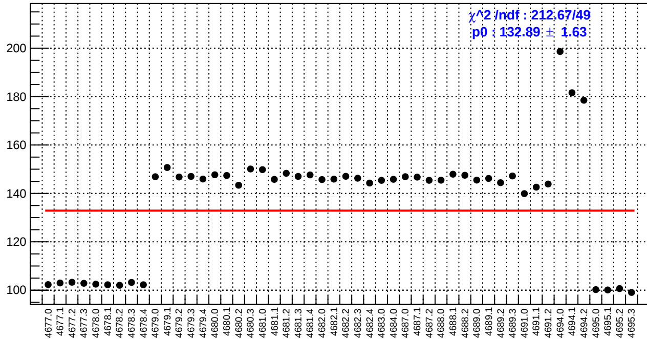
slug74: reg_asym_ds_avg.rms/ppm
