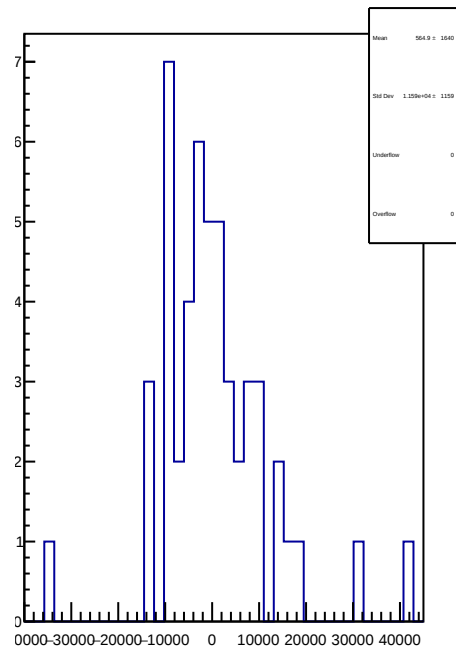
slug74: 1D Corr asym_left_avg.mean/ppb-reg_asym_left_avg.mean/ppb
