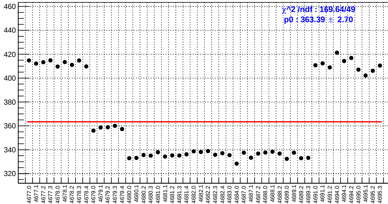
slug74: reg_asym_at1_avg.rms/ppm
