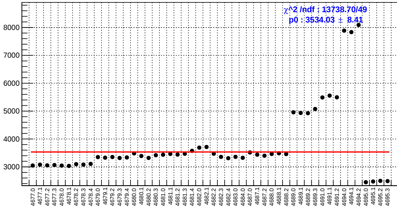
slug74: diff_bpm4aX.rms/nm
