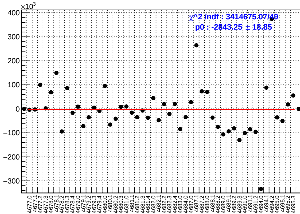
slug74: asym_sam4.mean/ppb-reg_asym_sam4.mean/ppb
