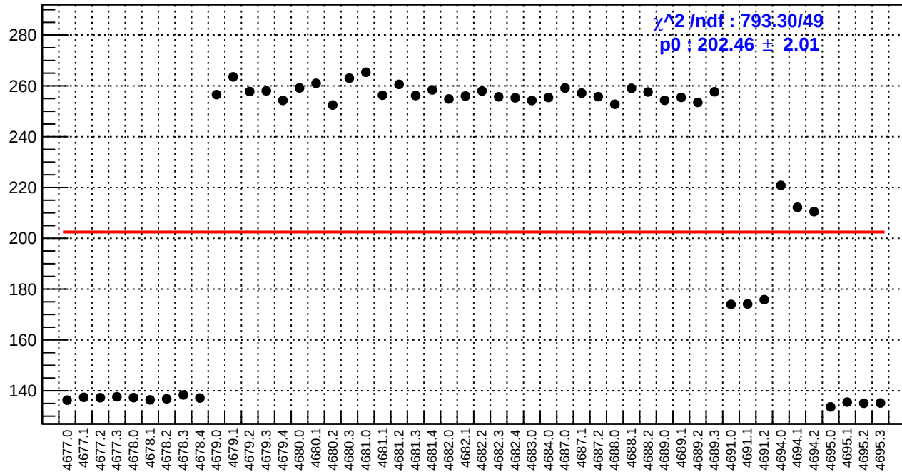
slug74: reg_asym_dsr.rms/ppm
