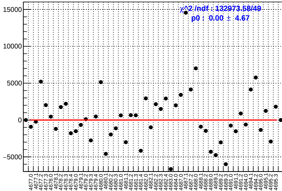
slug74: asym_us_avg.mean/ppb-reg_asym_us_avg.mean/ppb
