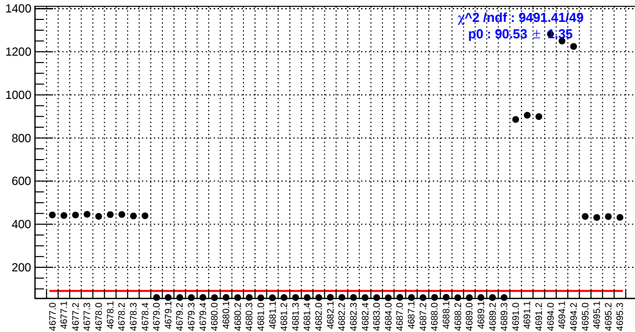
slug74: reg_asym_atr2.rms/ppm
