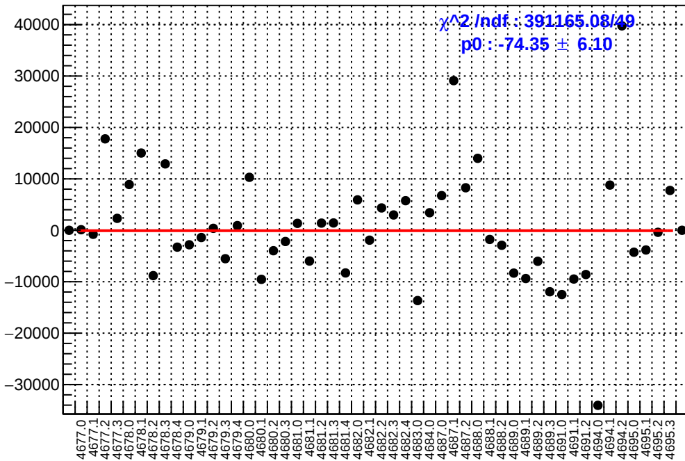
slug74: asym_usl.mean/ppb-reg_asym_usl.mean/ppb
