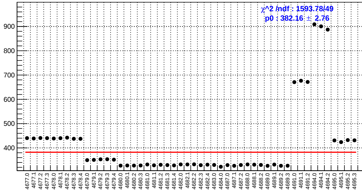
slug74: reg_asym_atl1r2_avg.rms/ppm
