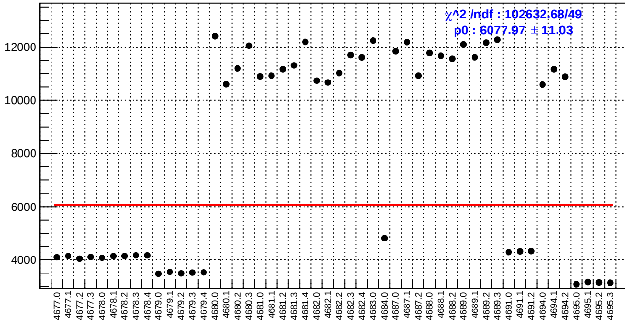
slug74: diff_bpm4aY.rms/nm
