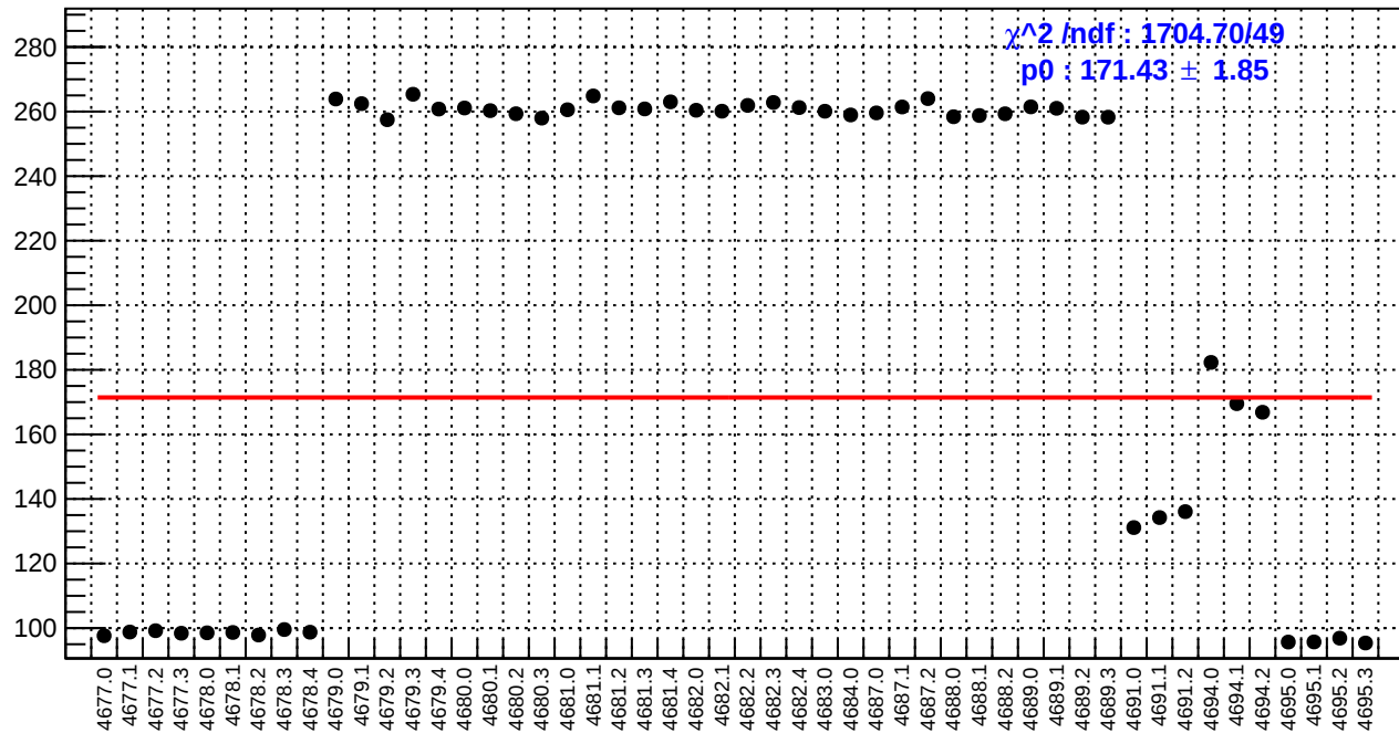
slug74: reg_asym_us_avg.rms/ppm
