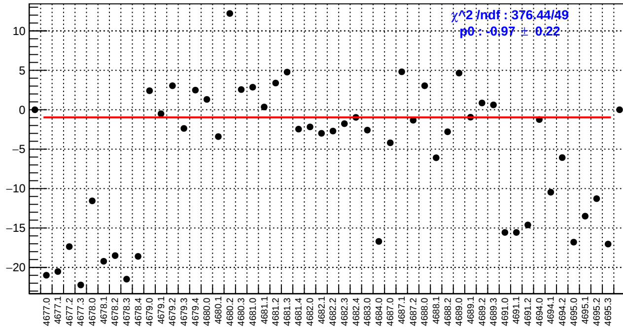
slug74: right_avg_bpm4eY/(ppb/nm)
