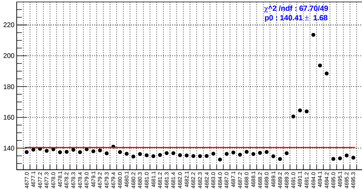
slug74: reg_asym_left_avg.rms/ppm
