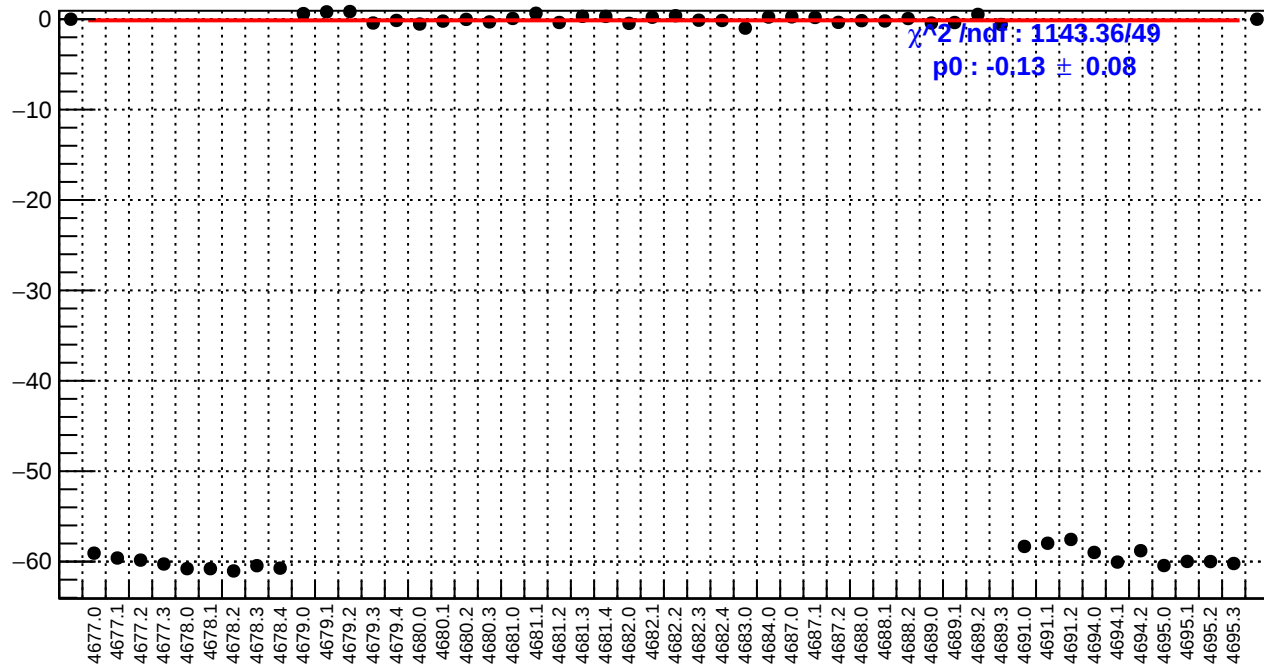
slug74: dsr_bpm12X/(ppb/nm)
