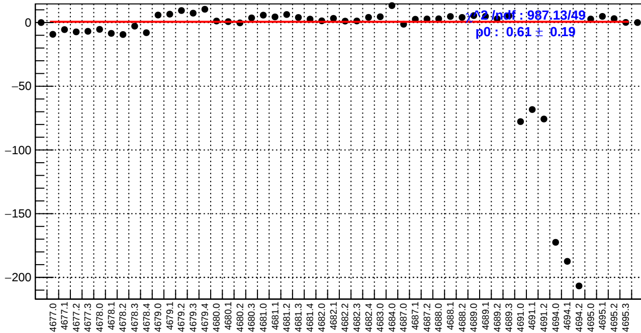
slug74: ds_avg_bpm4aX/(ppb/nm)
