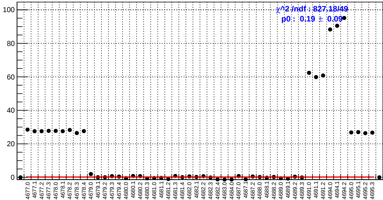
slug74: dsr_bpm4eX/(ppb/nm)
