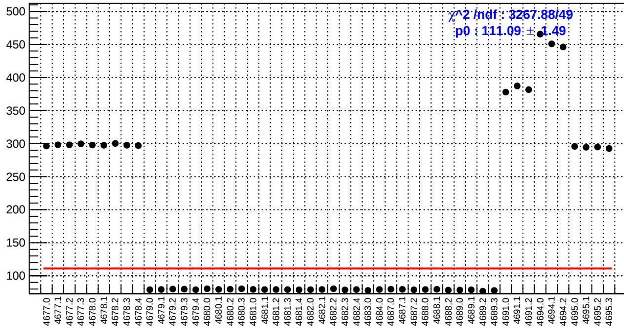
slug74: reg_asym_atr_avg.rms/ppm
