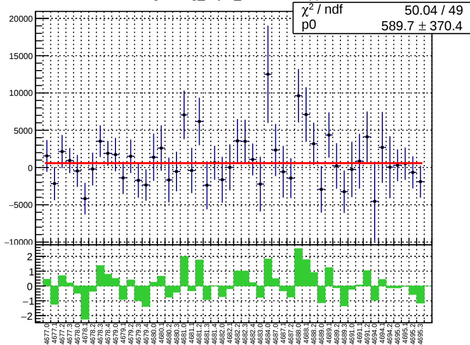
slug74: reg_asym_sam1.mean/ppb
