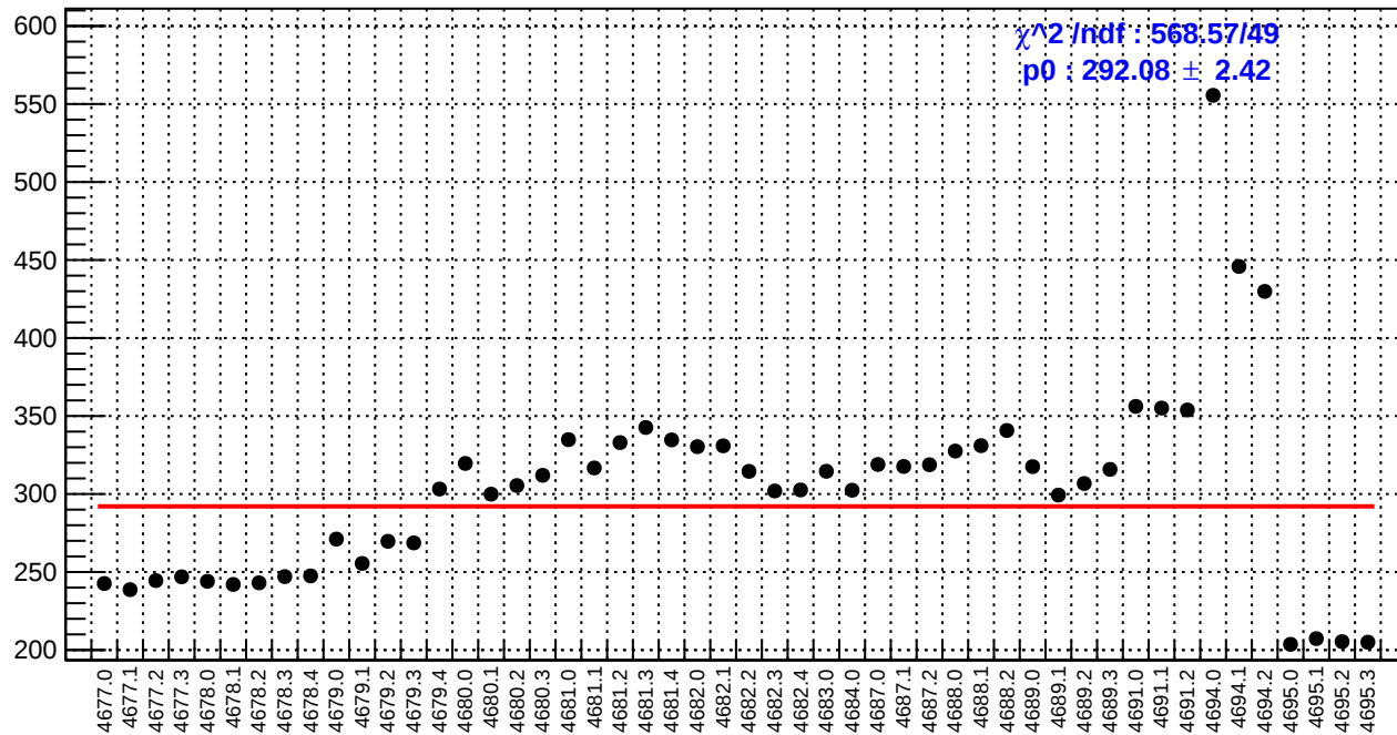
slug74: reg_asym_sam5.rms/ppm
