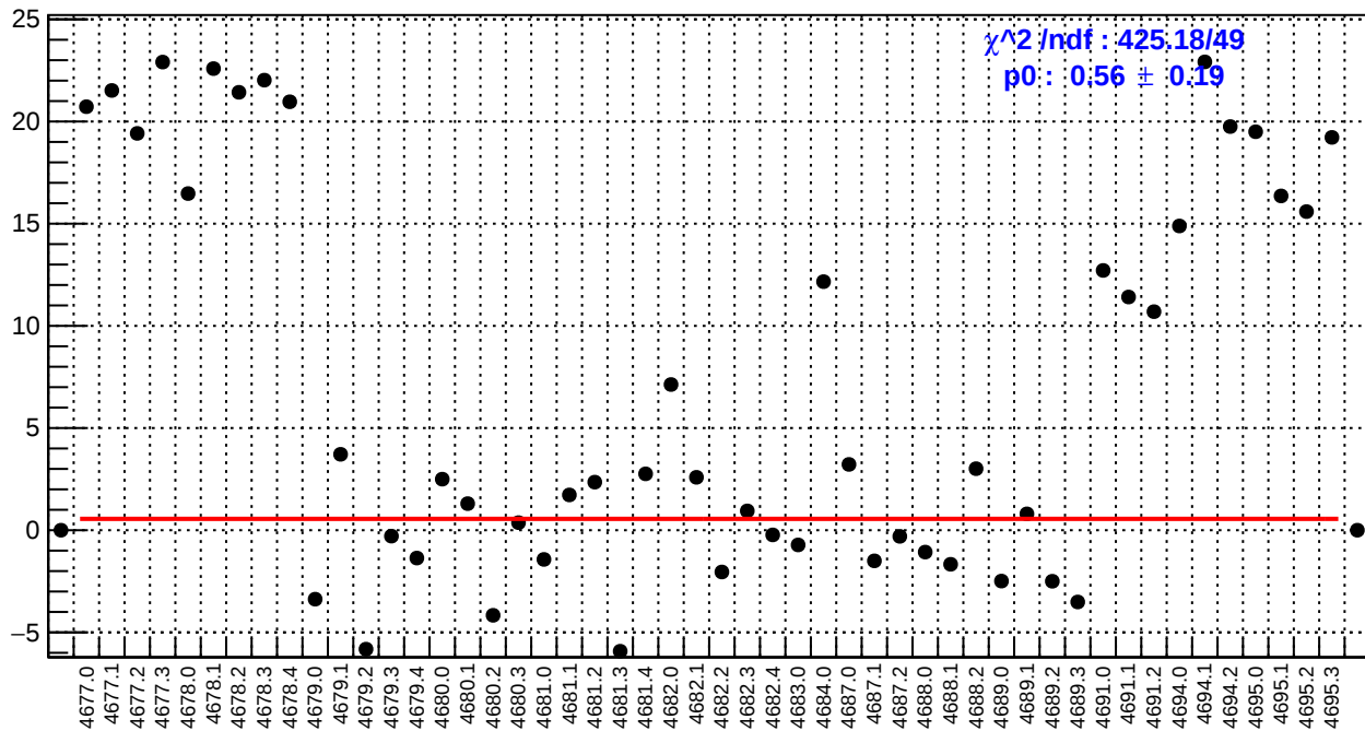
slug74: dsr_bpm4aY/(ppb/nm)
