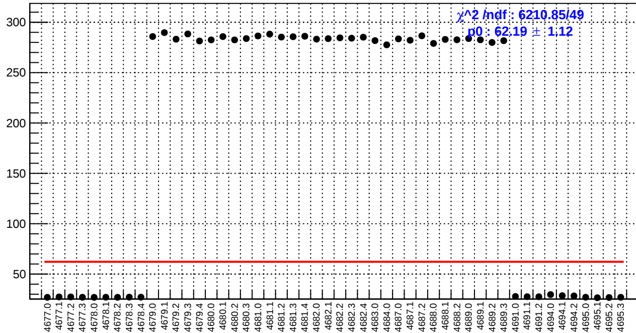
slug74: reg_asym_right_dd.rms/ppm
