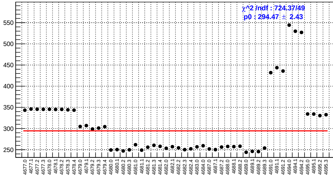
slug74: reg_asym_atr1l2_avg.rms/ppm
