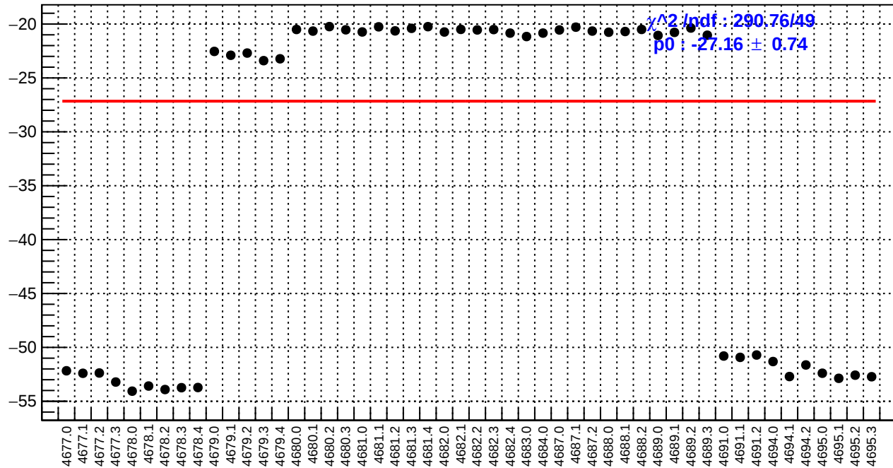
slug74: ds_avg_bpm12X/(ppb/nm)
