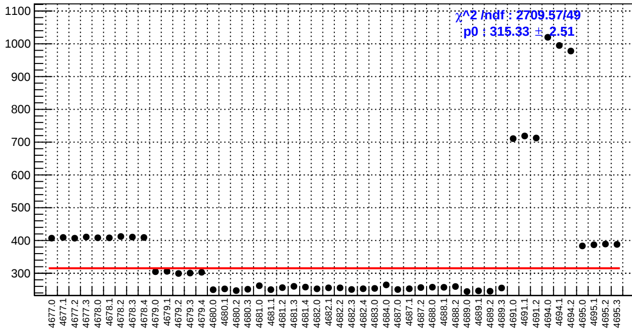
slug74: reg_asym_atr1l2_dd.rms/ppm
