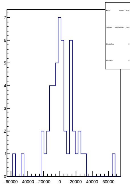
slug74: 1D Corr asym_at1_dd.mean/ppb-reg_asym_at1_dd.mean/ppb
