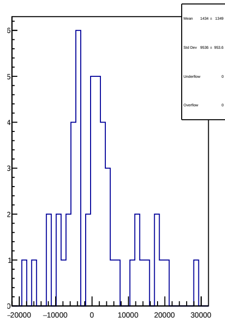
slug74: 1D Corr asym_at1_avg.mean/ppb-reg_asym_at1_avg.mean/ppb
