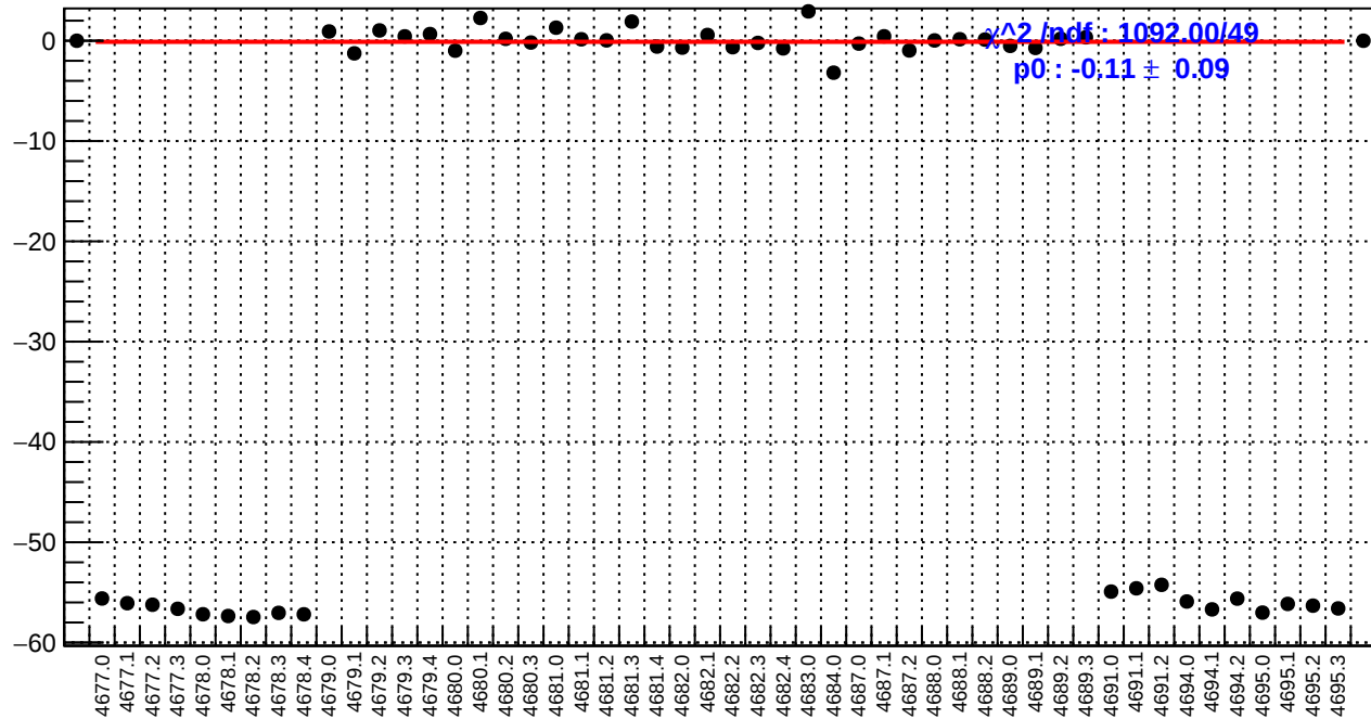
slug74: usr_bpm12X/(ppb/nm)
