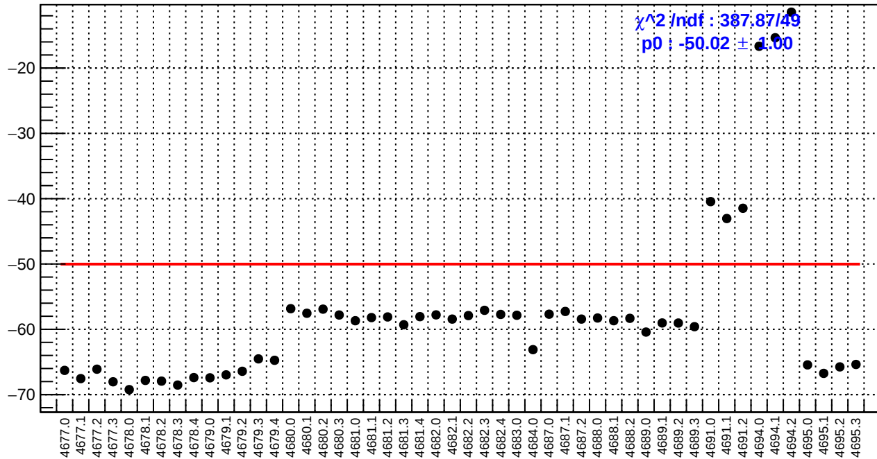
slug74: left_avg_bpm4eX/(ppb/nm)
