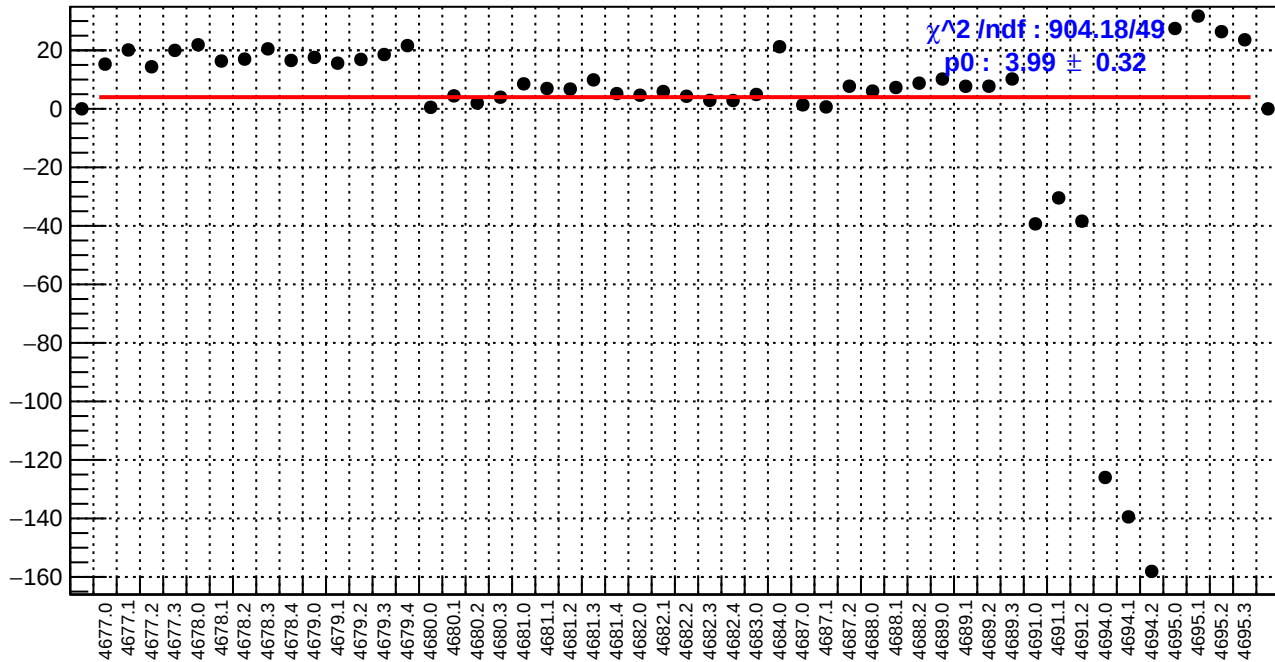
slug74: left_avg_bpm4aX/(ppb/nm)
