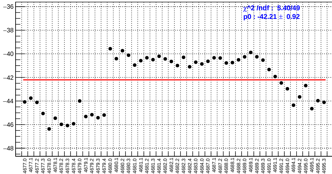
slug74: usl_bpm12X/(ppb/nm)
