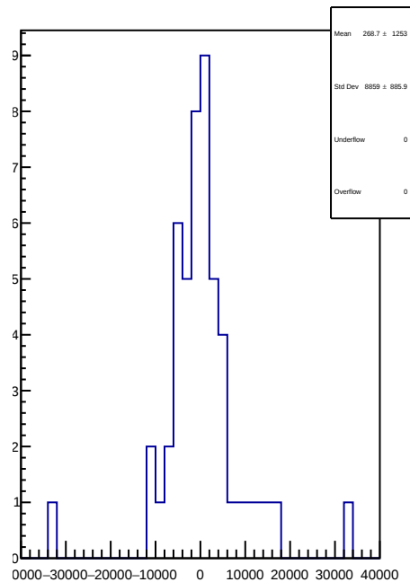
slug74: 1D Corr asym_us_dd.mean/ppb-reg_asym_us_dd.mean/ppb
