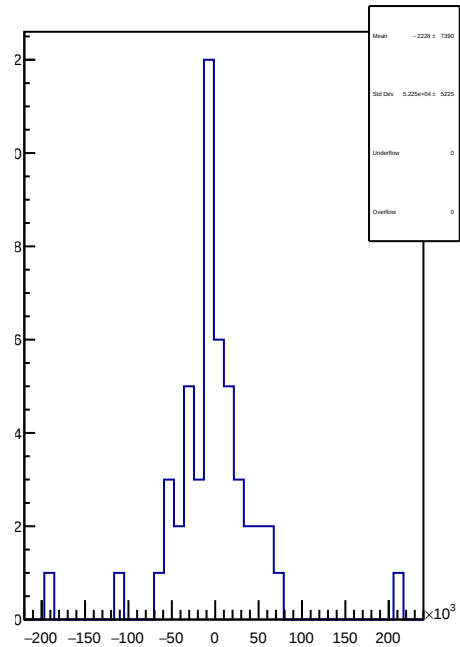
slug74: 1D Corr asym_sam6.mean/ppb-reg_asym_sam6.mean/ppb
