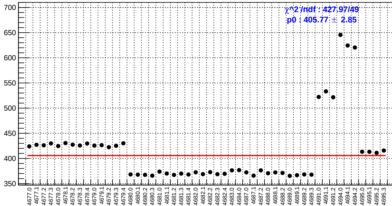
slug74: reg_asym_atl_dd.rms/ppm
