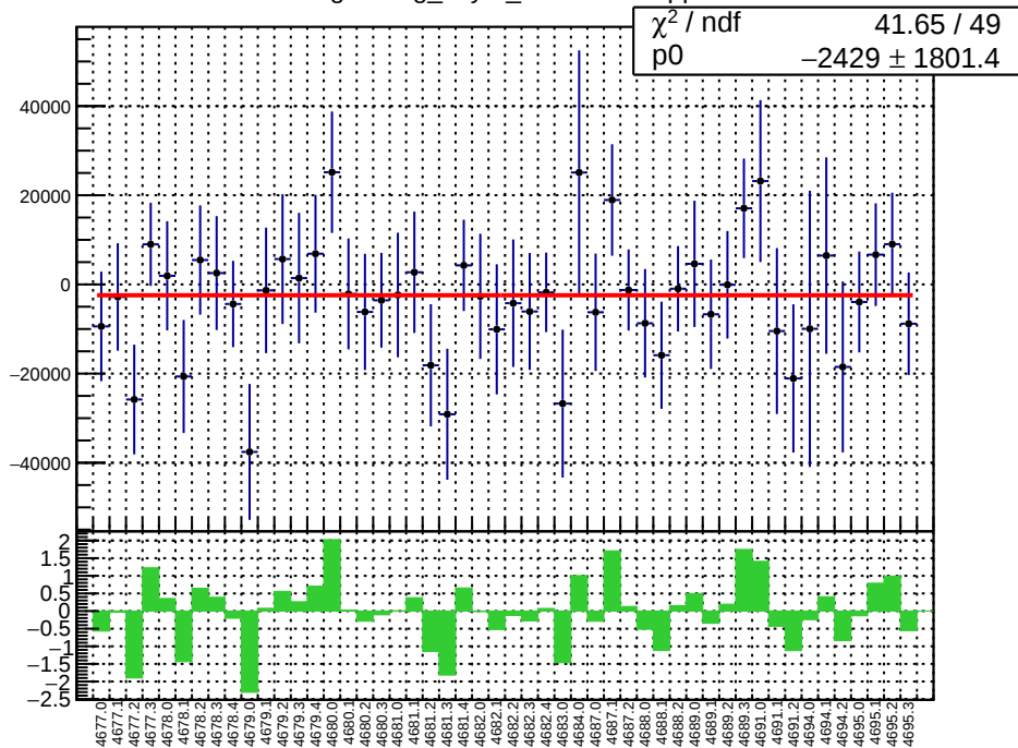
slug74: reg_asym_sam3.mean/ppb
