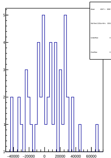
slug74: 1D Corr asym_atl_avg.mean/ppb-reg_asym_atl_avg.mean/ppb
