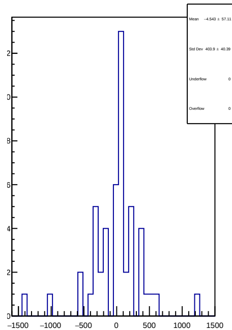
slug74: 1D Corr asym_left_dd.mean/ppb-reg_asym_left_dd.mean/ppb
