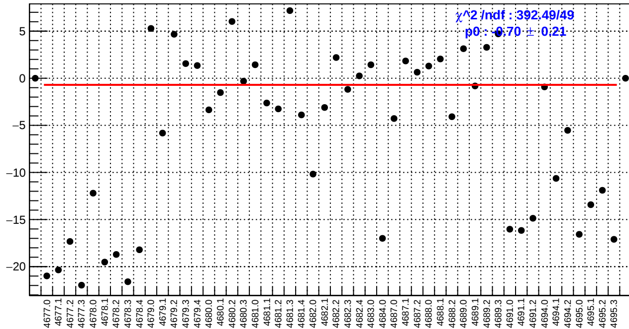
slug74: dsr_bpm4eY/(ppb/nm)
