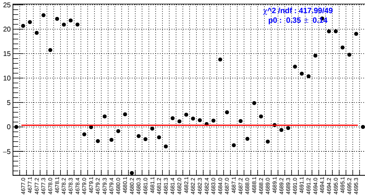
slug74: right_avg_bpm4aY/(ppb/nm)
