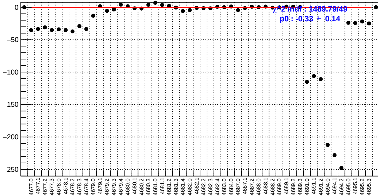
slug74: right_avg_bpm4aX/(ppb/nm)
