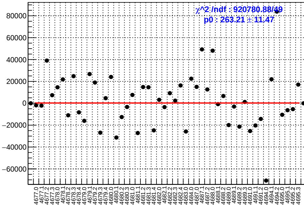
slug74: asym_atr1l2_avg.mean/ppb-reg_asym_atr1l2_avg.mean/ppb
