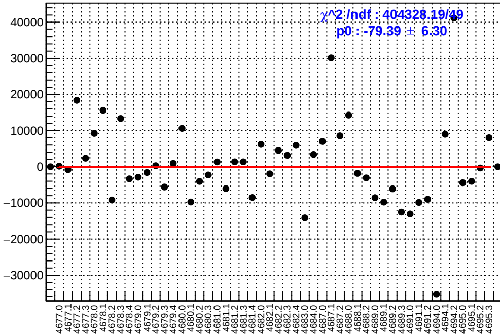
slug74: asym_left_avg.mean/ppb-reg_asym_left_avg.mean/ppb
