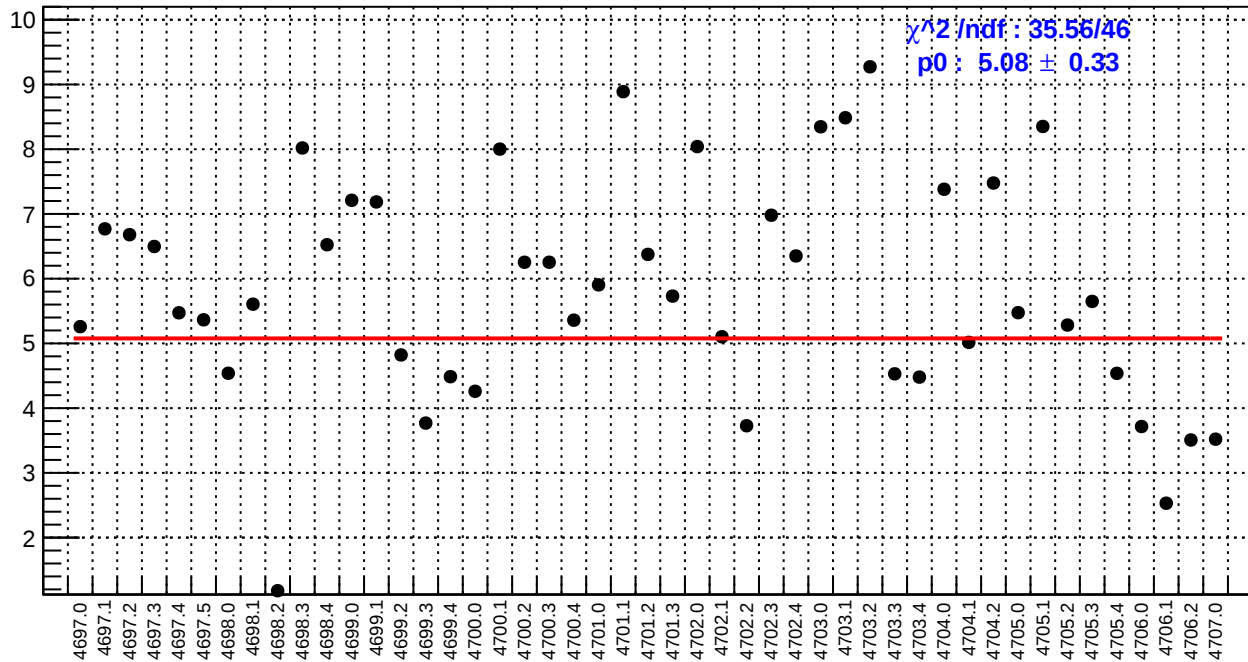
slug75: left_avg_bpm4aY/(ppb/nm)
