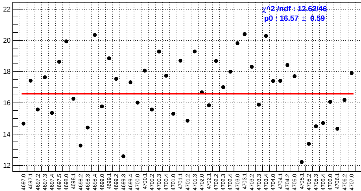
slug75: dsr_bpm4aY/(ppb/nm)
