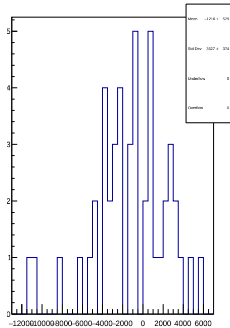
slug75: 1D Corr asym_sam1.mean/ppb-reg_asym_sam1.mean/ppb
