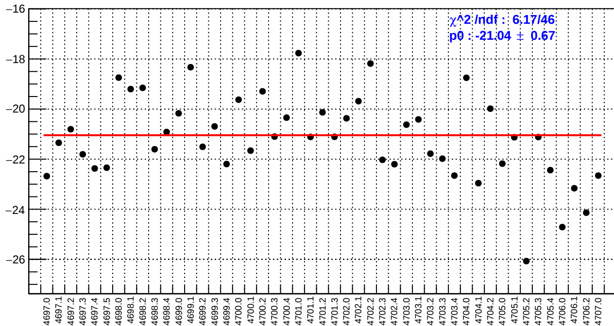
slug75: dsr_bpm4aX/(ppb/nm)
