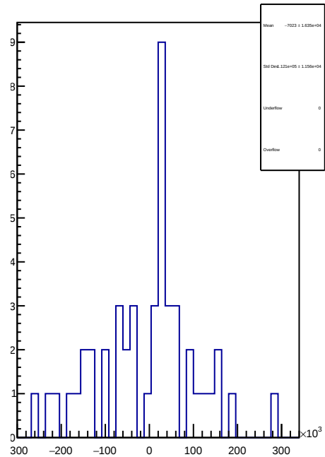
slug75: 1D Corr asym_sam3.mean/ppb-reg_asym_sam3.mean/ppb
