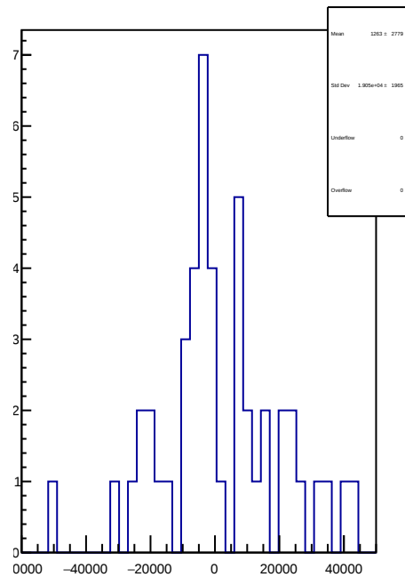
slug75: 1D Corr asym_sam7.mean/ppb-reg_asym_sam7.mean/ppb
