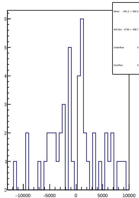
slug75: 1D Corr asym_dsr.mean/ppb-reg_asym_dsr.mean/ppb
