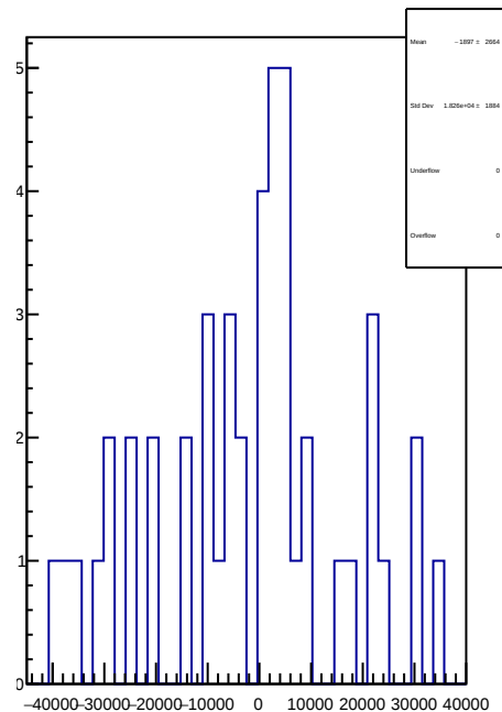
slug75: 1D Corr asym_atl1r2_avg.mean/ppb-reg_asym_atl1r2_avg.mean/ppb
