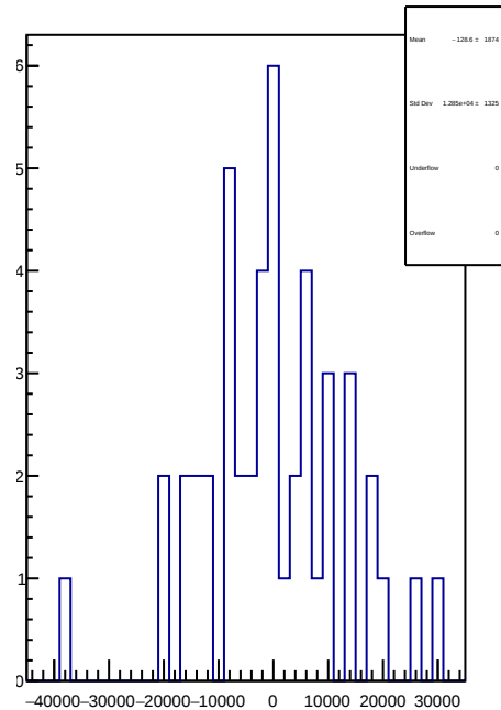
slug75: 1D Corr asym_sam8.mean/ppb-reg_asym_sam8.mean/ppb
