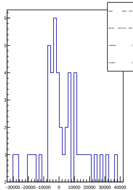
slug75: 1D Corr asym_atl_dd.mean/ppb-reg_asym_atl_dd.mean/ppb
