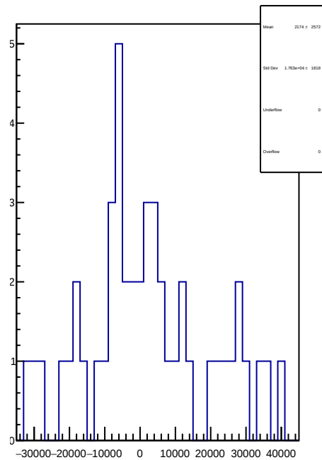
slug75: 1D Corr asym_atr_dd.mean/ppb-reg_asym_atr_dd.mean/ppb
