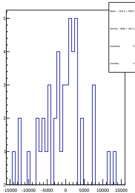
slug75: 1D Corr asym_dsl.mean/ppb-reg_asym_dsl.mean/ppb
