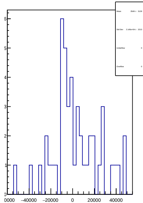
slug75: 1D Corr asym_sam6.mean/ppb-reg_asym_sam6.mean/ppb
