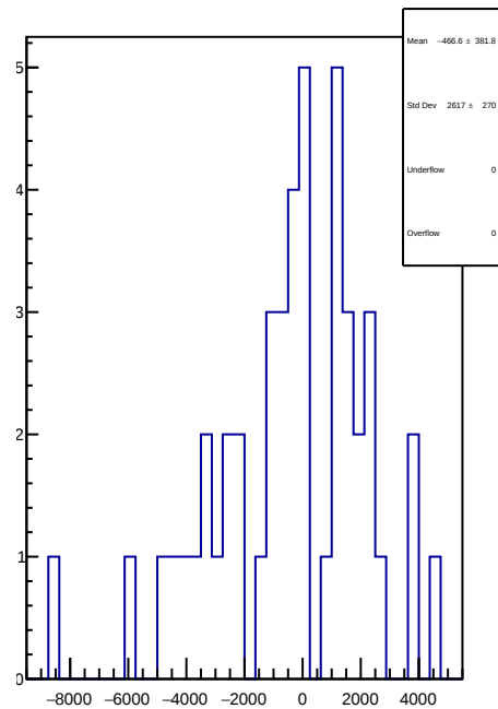
slug75: 1D Corr asym_ds_avg.mean/ppb-reg_asym_ds_avg.mean/ppb
