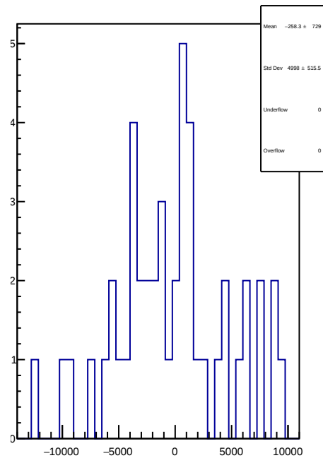
slug75: 1D Corr asym_right_avg.mean/ppb-reg_asym_right_avg.mean/ppb
