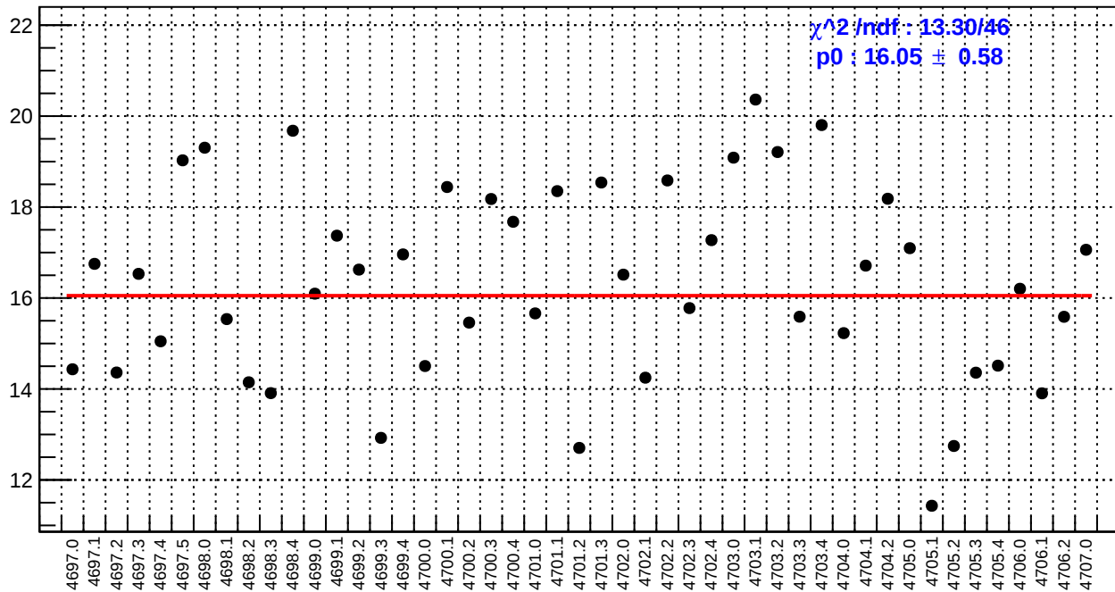
slug75: usr_bpm4aY/(ppb/nm)
