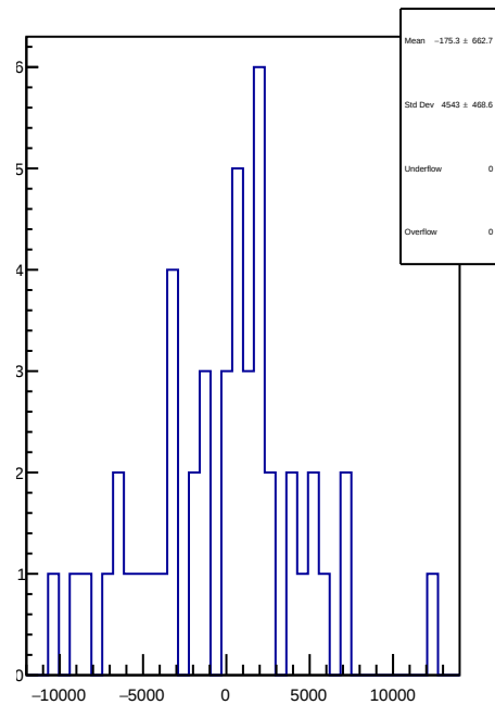
slug75: 1D Corr asym_ds_dd.mean/ppb-reg_asym_ds_dd.mean/ppb
