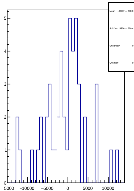
slug75: 1D Corr asym_usl.mean/ppb-reg_asym_usl.mean/ppb
