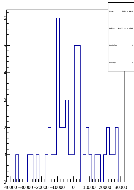
slug75: 1D Corr asym_atl1.mean/ppb-reg_asym_atl1.mean/ppb
