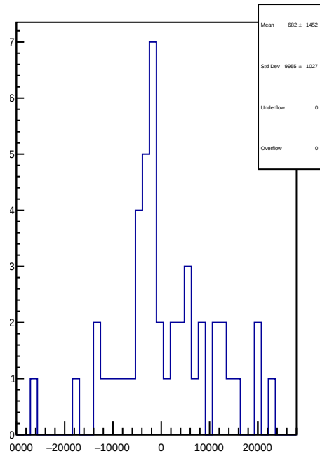
slug75: 1D Corr asym_at2_dd.mean/ppb-reg_asym_at2_dd.mean/ppb
