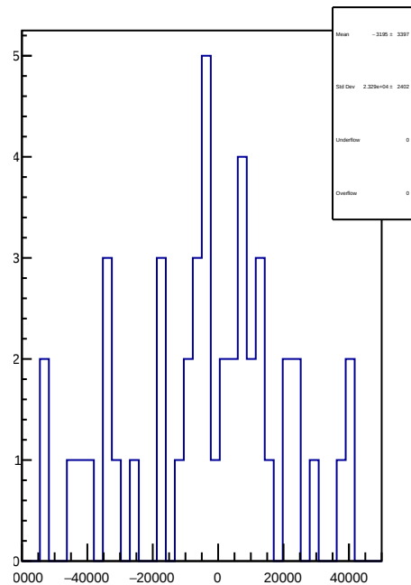
slug75: 1D Corr asym_atr2.mean/ppb-reg_asym_atr2.mean/ppb
