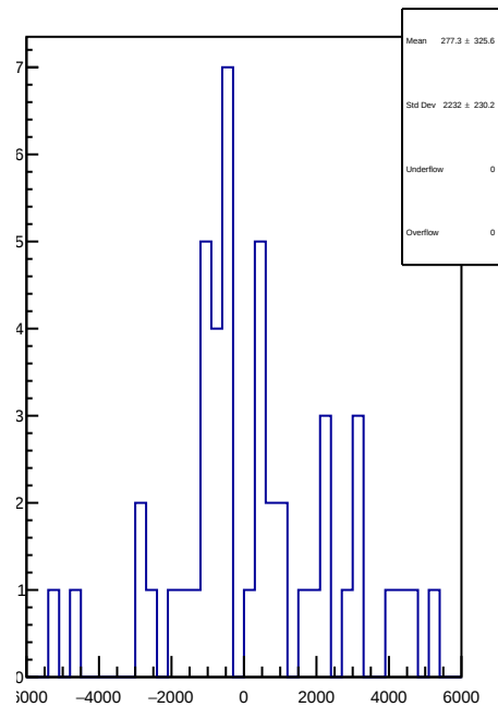
slug75: 1D Corr asym_at1_avg.mean/ppb-reg_asym_at1_avg.mean/ppb
