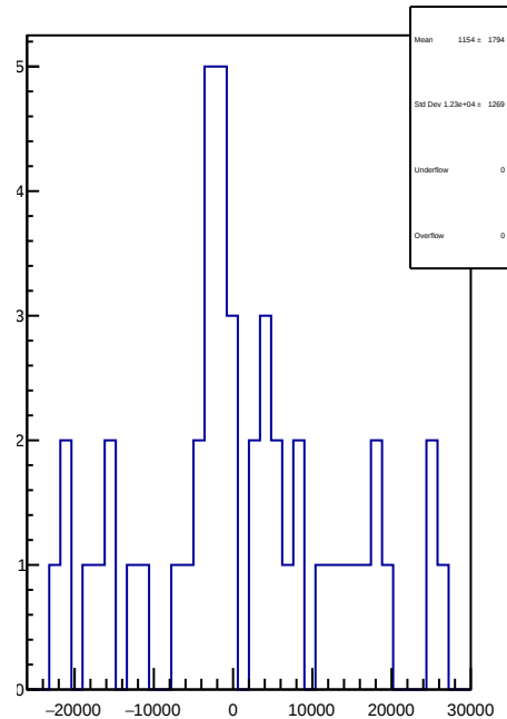
slug75: 1D Corr asym_atr1.mean/ppb-reg_asym_atr1.mean/ppb
