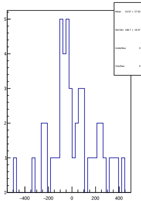
slug75: 1D Corr asym_left_dd.mean/ppb-reg_asym_left_dd.mean/ppb
