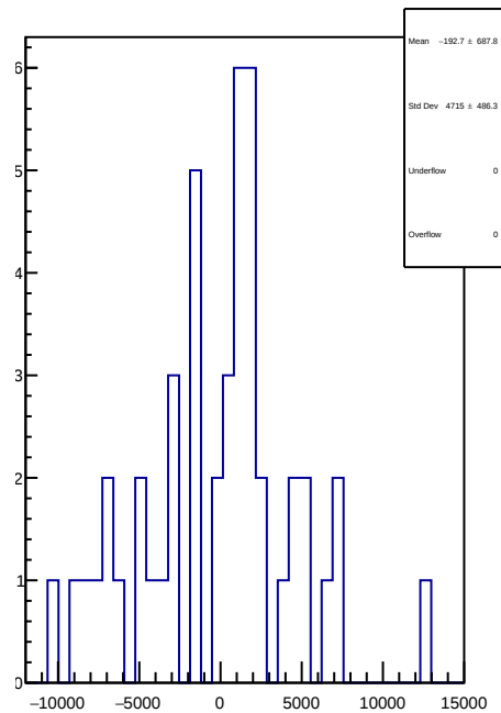
slug75: 1D Corr asym_us_dd.mean/ppb-reg_asym_us_dd.mean/ppb
