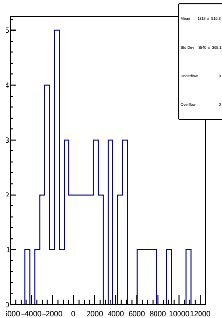
slug75: 1D Corr asym_sam5.mean/ppb-reg_asym_sam5.mean/ppb
