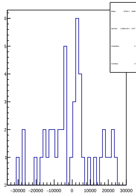
slug75: 1D Corr asym_at1_dd.mean/ppb-reg_asym_at1_dd.mean/ppb
