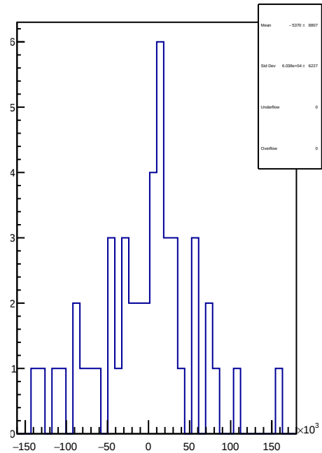
slug75: 1D Corr asym_sam2.mean/ppb-reg_asym_sam2.mean/ppb
