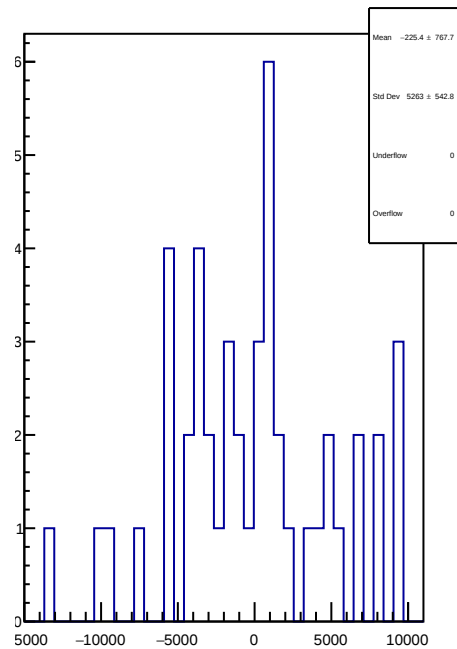
slug75: 1D Corr asym_usr.mean/ppb-reg_asym_usr.mean/ppb
