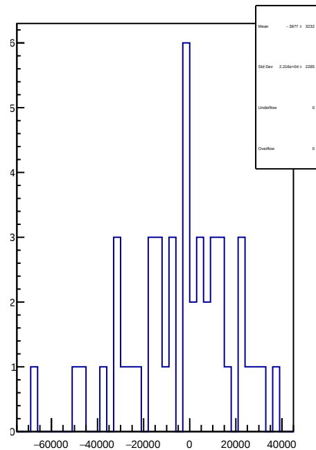
slug75: 1D Corr asym_at2_avg.mean/ppb-reg_asym_at2_avg.mean/ppb
