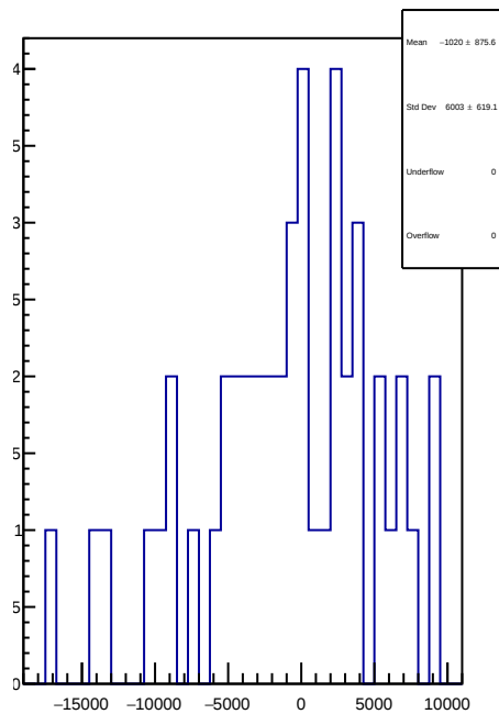
slug75: 1D Corr asym_atr_avg.mean/ppb-reg_asym_atr_avg.mean/ppb
