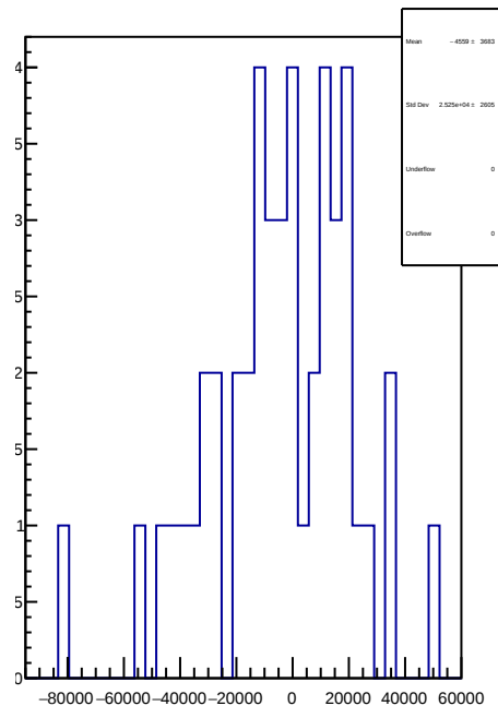
slug75: 1D Corr asym_atl2.mean/ppb-reg_asym_atl2.mean/ppb
