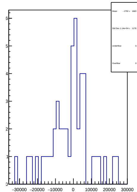
slug75: 1D Corr asym_atr1l2_avg.mean/ppb-reg_asym_atr1l2_avg.mean/ppb
