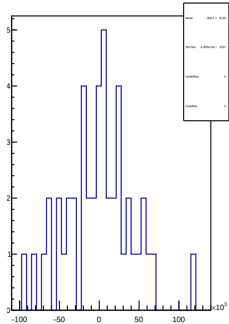
slug75: 1D Corr asym_sam4.mean/ppb-reg_asym_sam4.mean/ppb
