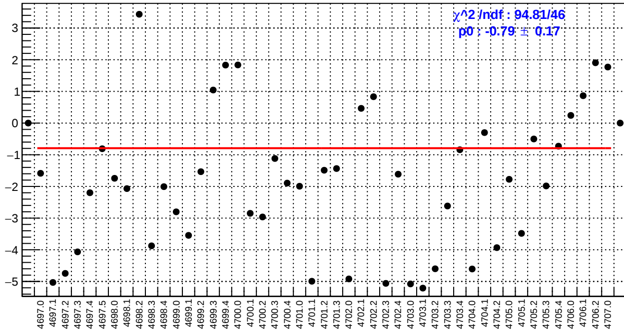
slug75: left_avg_bpm4eY/(ppb/nm)
