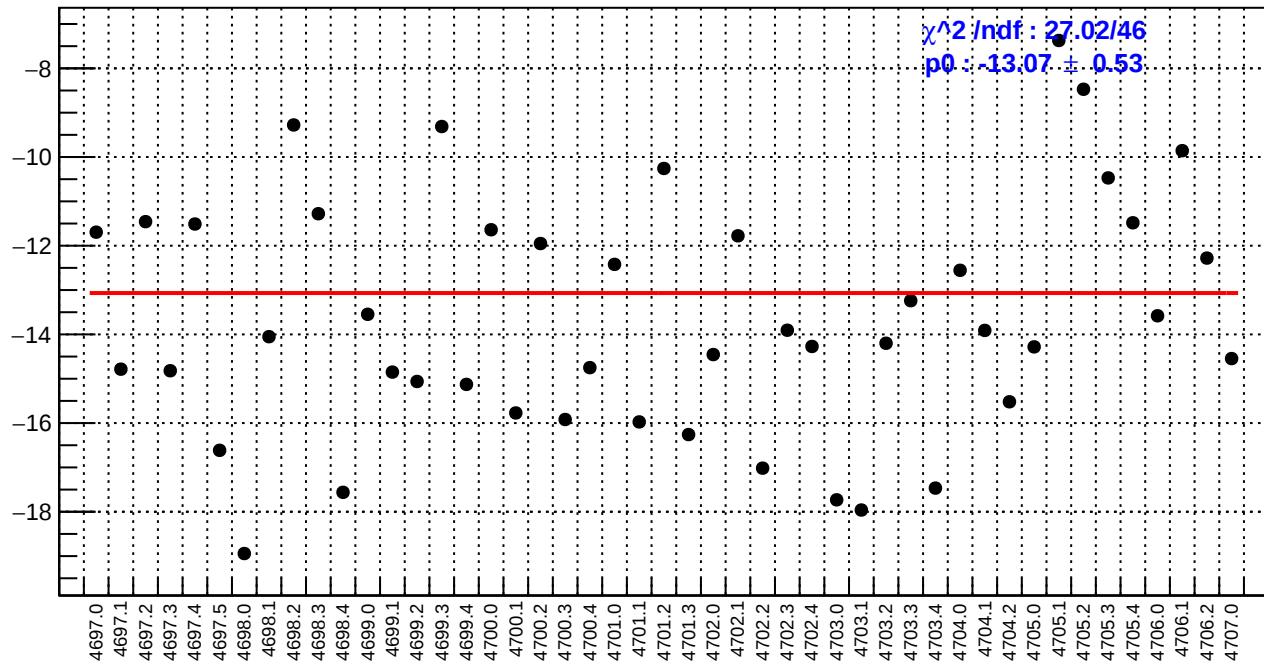
slug75: right_avg_bpm4eY/(ppb/nm)
