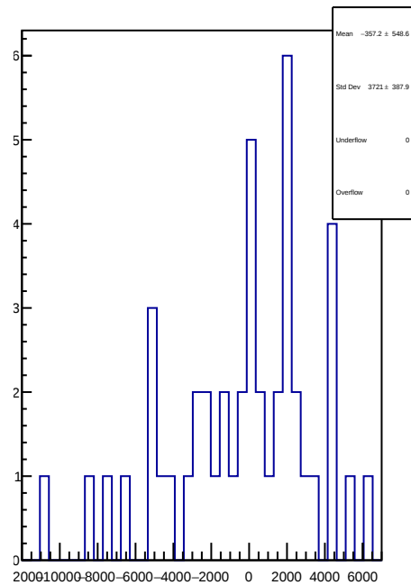
slug78: 1D Corr asym_sam5.mean/ppb-reg_asym_sam5.mean/ppb
