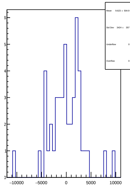
slug78: 1D Corr asym_atl1.mean/ppb-reg_asym_atl1.mean/ppb
