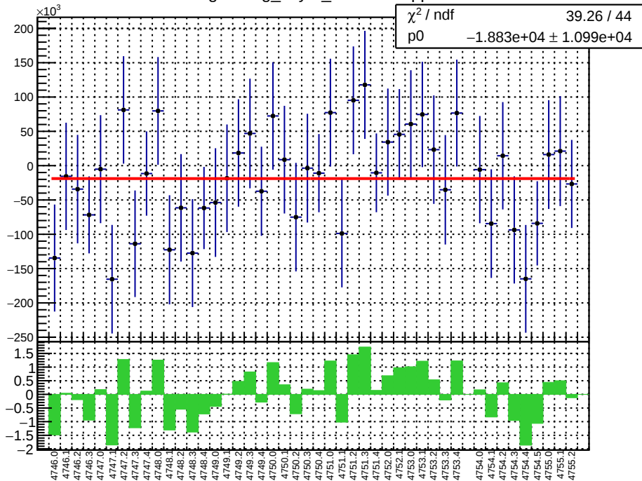
slug78: reg_asym_atl2.mean/ppb
