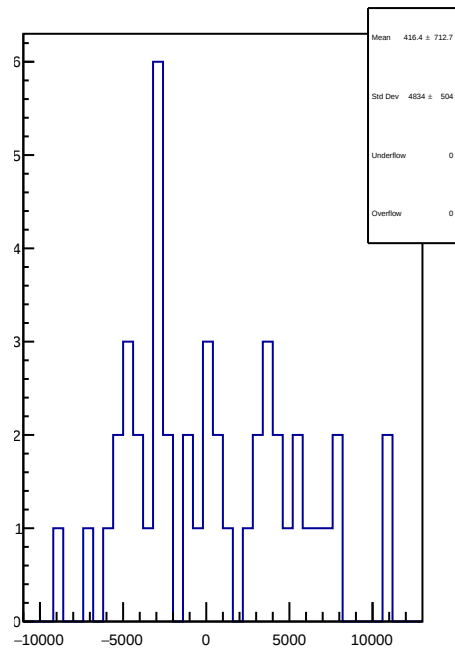
slug78: 1D Corr asym_usr.mean/ppb-reg_asym_usr.mean/ppb
