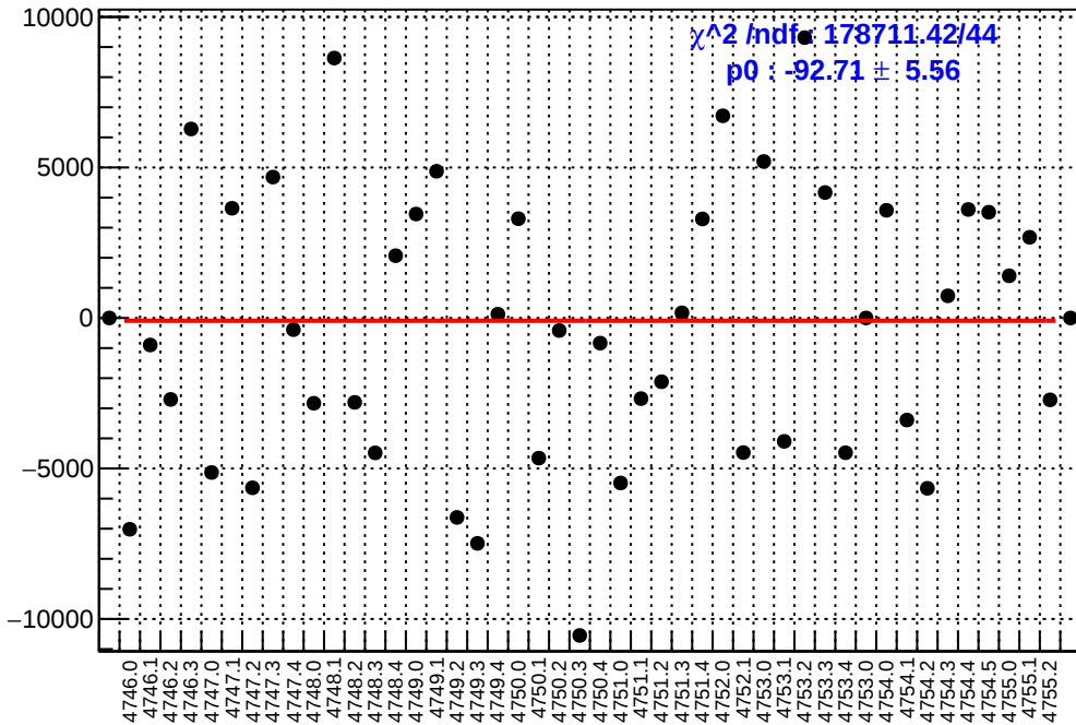
slug78: asym_us_dd.mean/ppb-reg_asym_us_dd.mean/ppb
