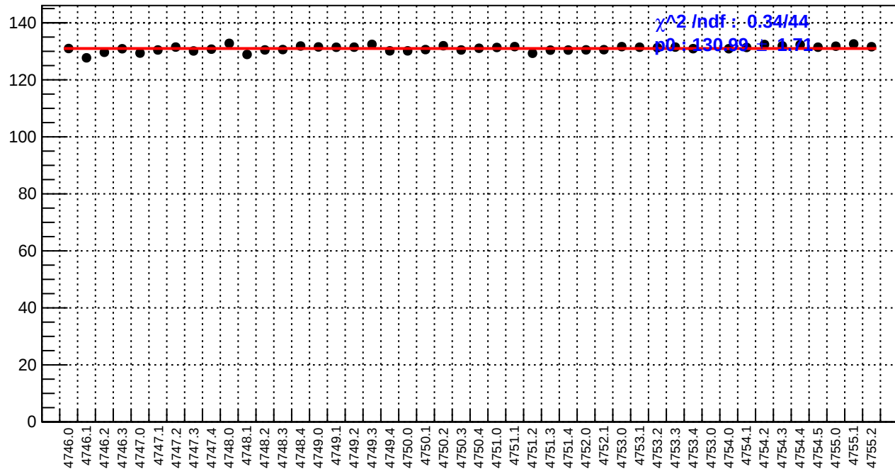
slug78: reg_asym_usr.rms/ppm
