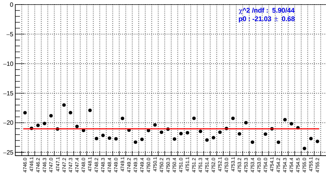
slug78: dsr_bpm4aX/(ppb/nm)
