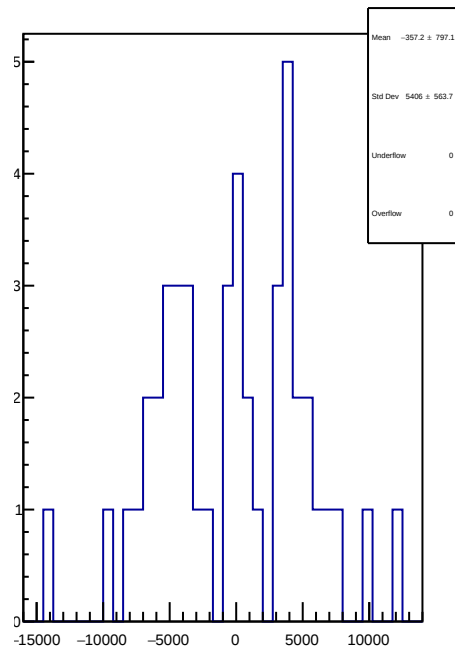
slug78: 1D Corr asym_atl1r2_dd.mean/ppb-reg_asym_atl1r2_dd.mean/ppb
