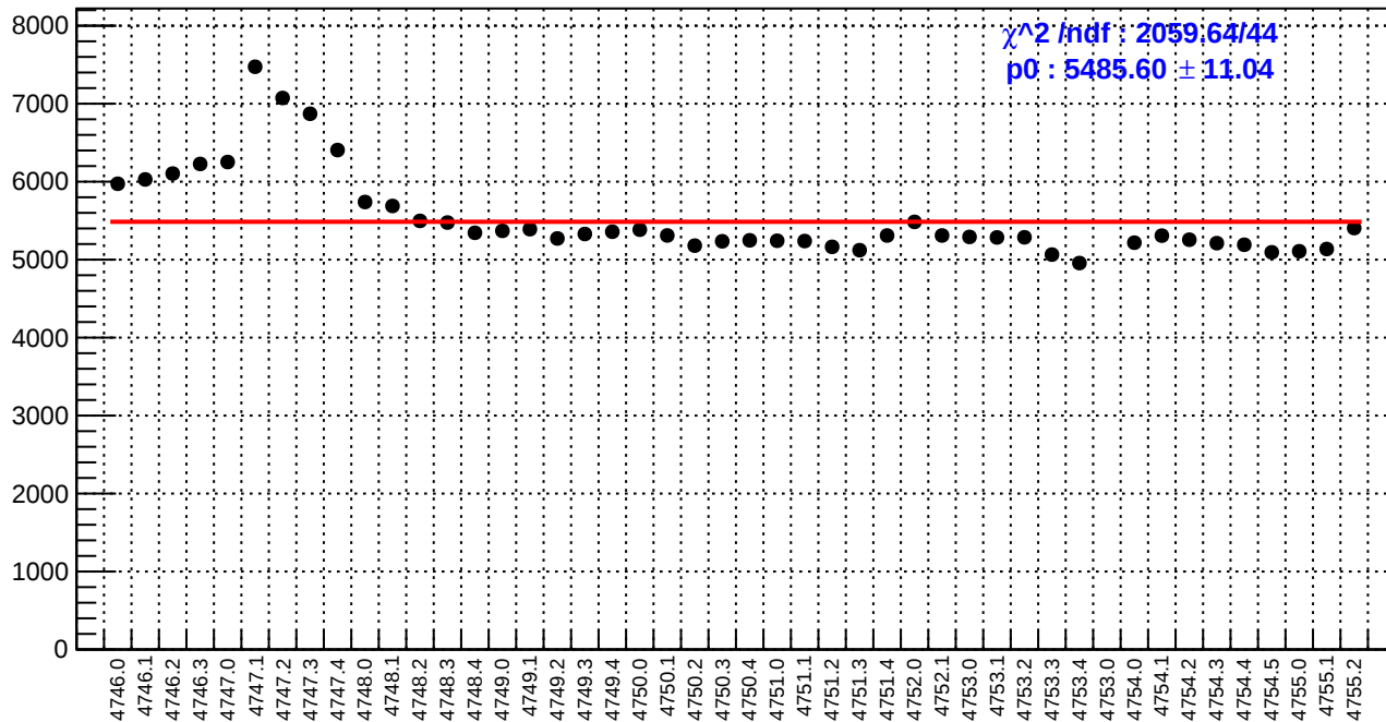
slug78: diff_bpm11X.rms/nm
