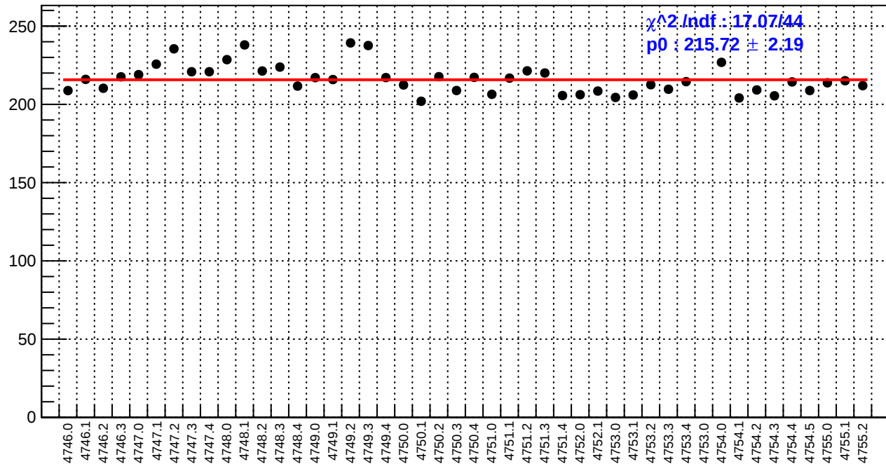
slug78: reg_asym_sam5.rms/ppm
