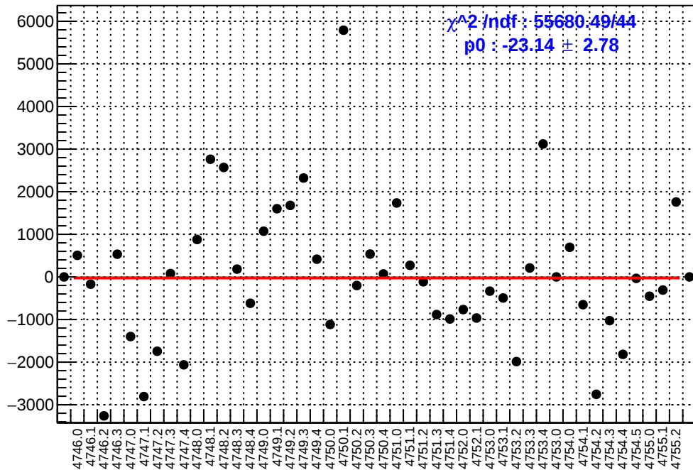
slug78: asym_at2_avg.mean/ppb-reg_asym_at2_avg.mean/ppb
