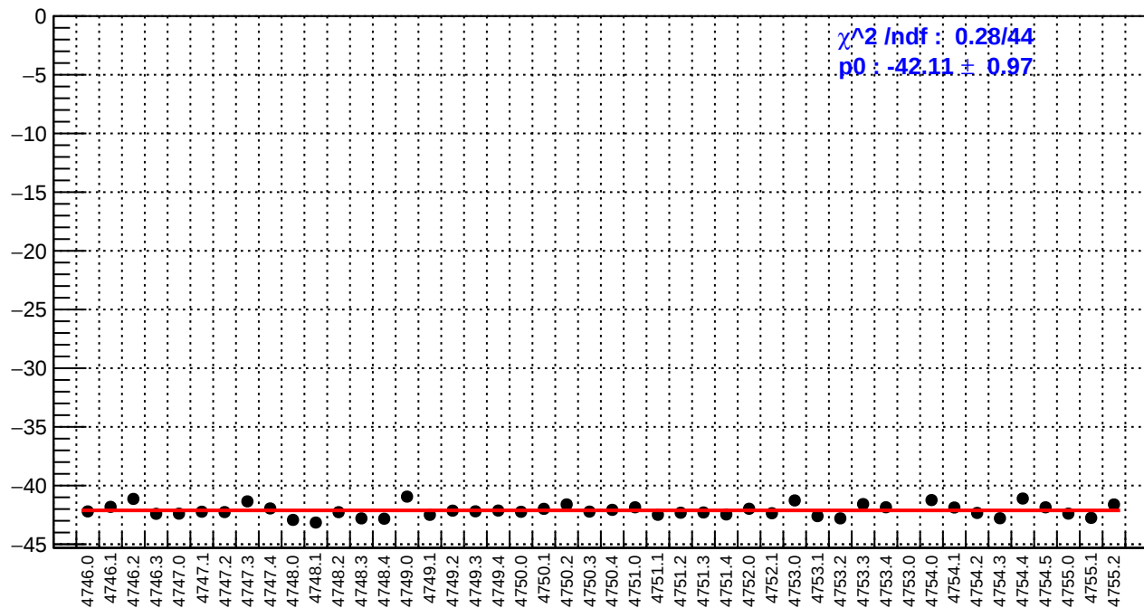
slug78: dsl_bpm12X/(ppb/nm)
