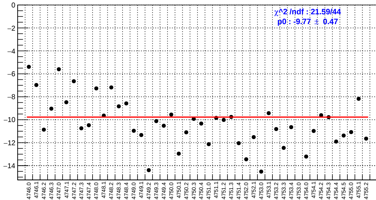
slug78: usl_bpm4aY/(ppb/nm)
