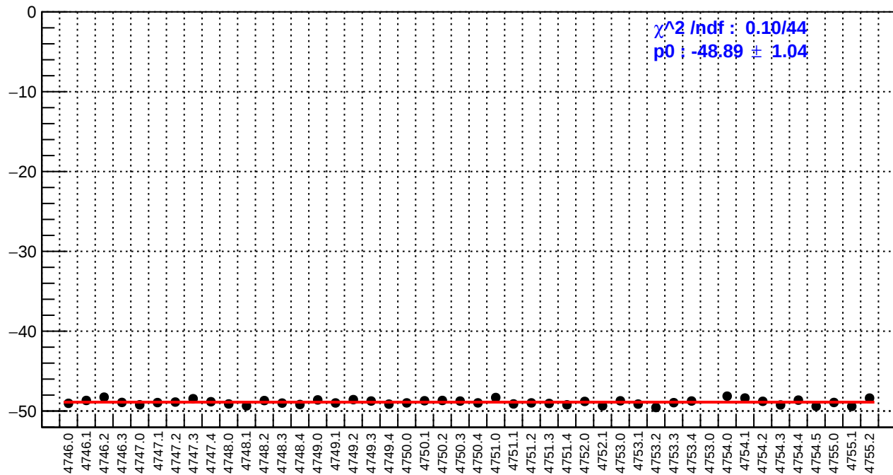
slug78: us_avg_bpm12X/(ppb/nm)
