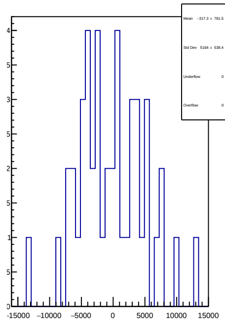
slug78: 1D Corr asym_atl_avg.mean/ppb-reg_asym_atl_avg.mean/ppb
