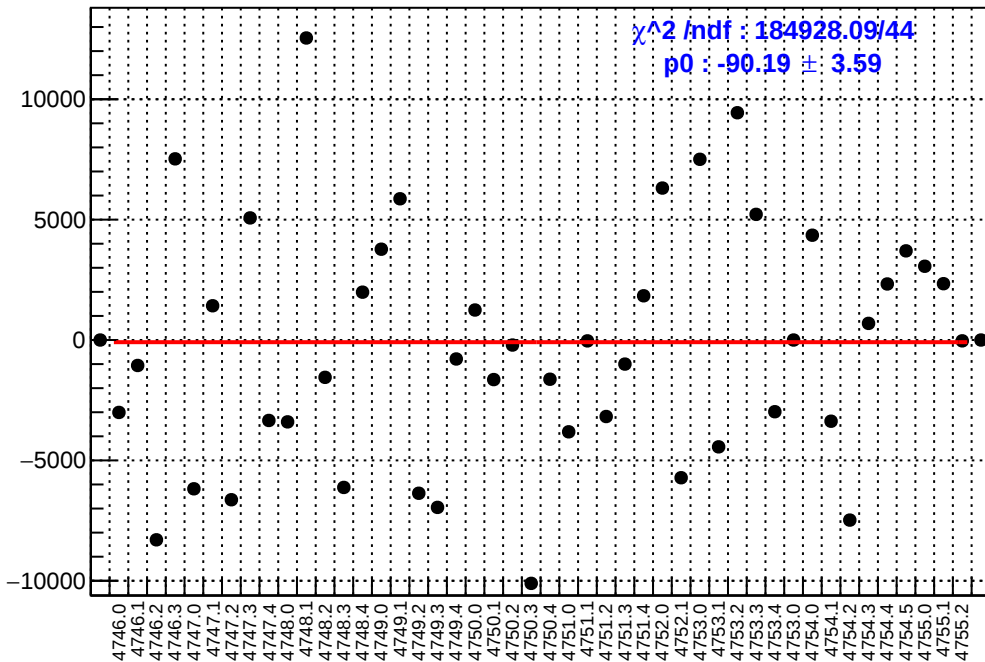
slug78: asym_usl.mean/ppb-reg_asym_usl.mean/ppb
