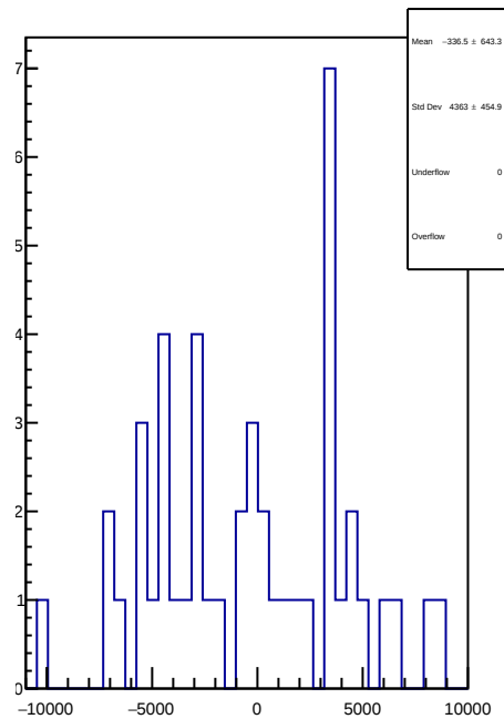
slug78: 1D Corr asym_ds_dd.mean/ppb-reg_asym_ds_dd.mean/ppb
