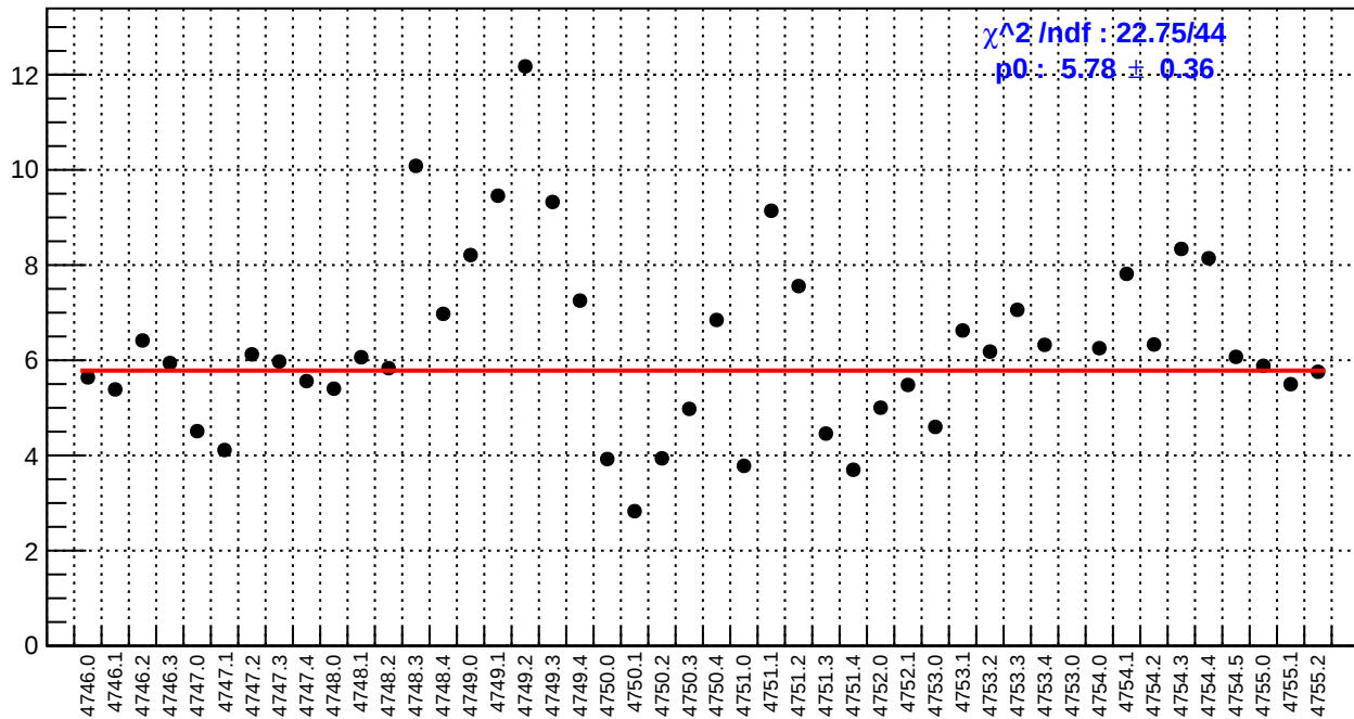
slug78: ds_avg_bpm4aX/(ppb/nm)
