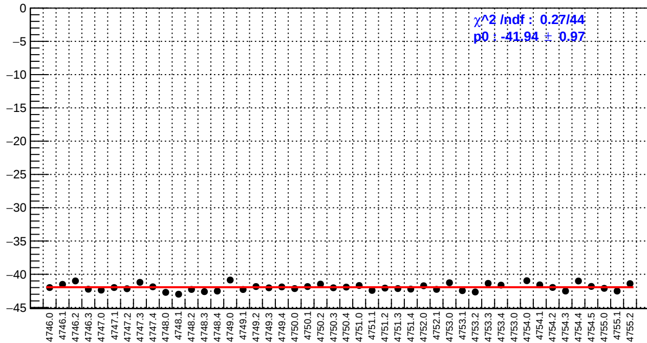
slug78: left_avg_bpm12X/(ppb/nm)
