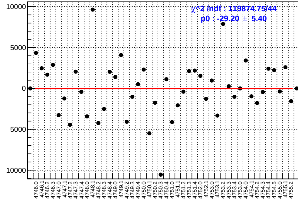
slug78: asym_atl1.mean/ppb-reg_asym_atl1.mean/ppb
