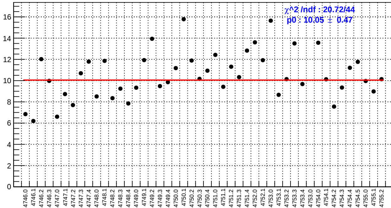
slug78: left_avg_bpm4eY/(ppb/nm)
