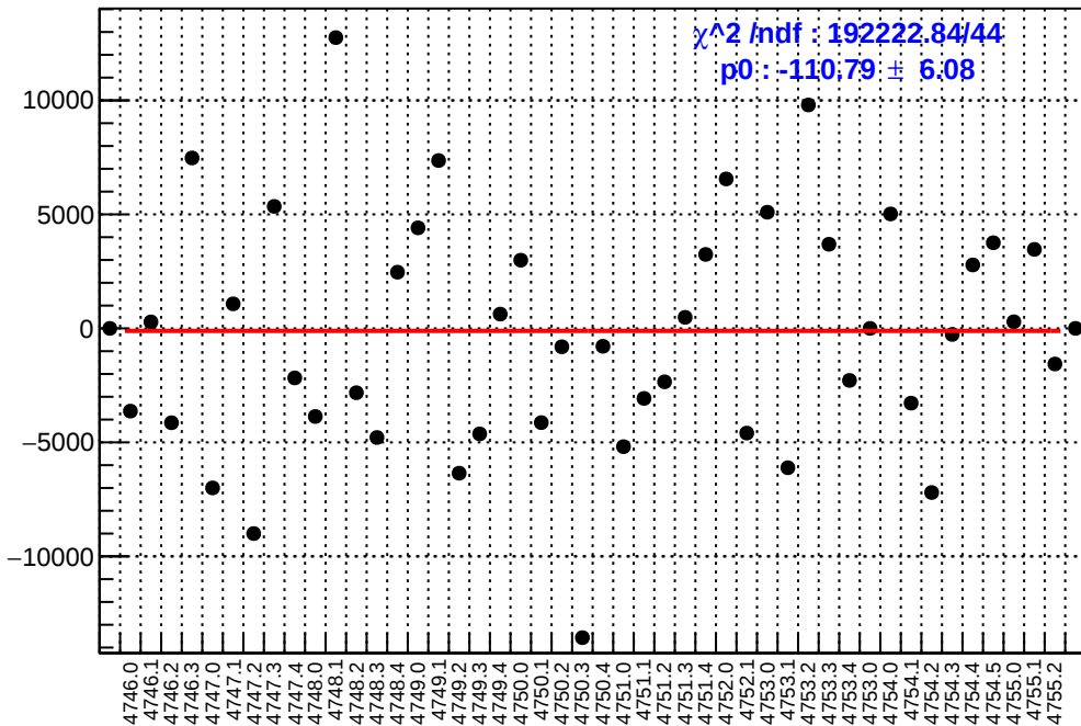
slug78: asym_atl_avg.mean/ppb-reg_asym_atl_avg.mean/ppb
