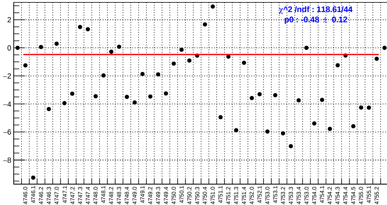
slug78: usr_bpm4eY/(ppb/nm)
