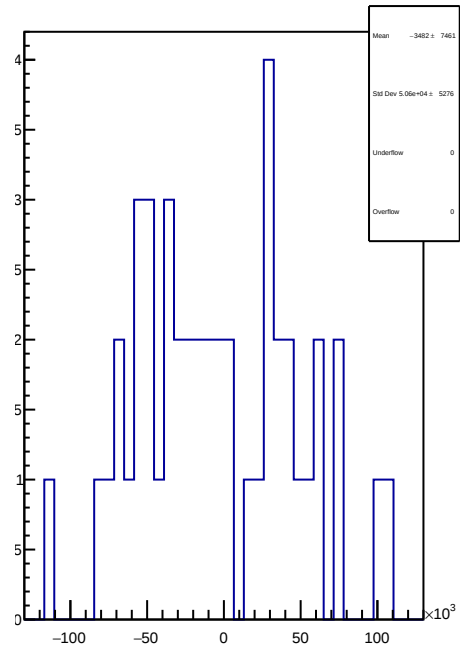
slug78: 1D Corr asym_sam2.mean/ppb-reg_asym_sam2.mean/ppb
