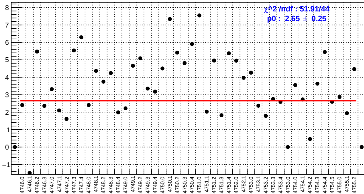
slug78: us_avg_bpm4eY/(ppb/nm)
