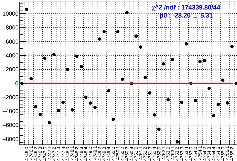
slug78: asym_right_avg.mean/ppb-reg_asym_right_avg.mean/ppb
