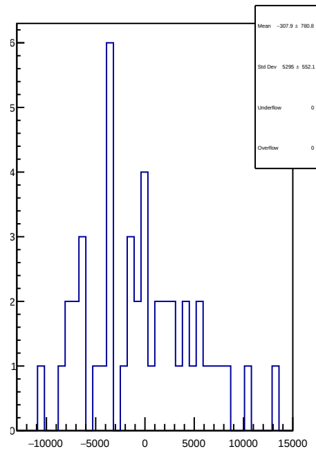
slug78: 1D Corr asym_dsl.mean/ppb-reg_asym_dsl.mean/ppb
