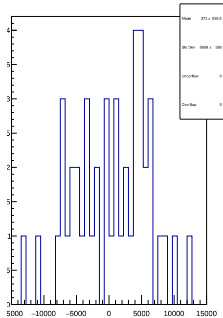
slug78: 1D Corr asym_atr1l2_dd.mean/ppb-reg_asym_atr1l2_dd.mean/ppb
