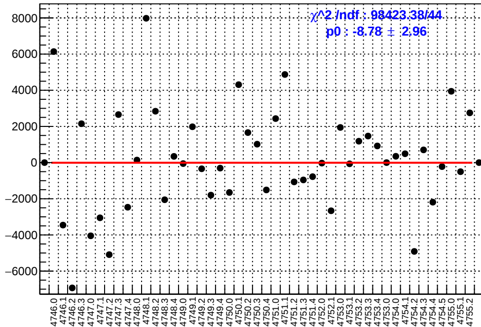
slug78: asym_sam1.mean/ppb-reg_asym_sam1.mean/ppb
