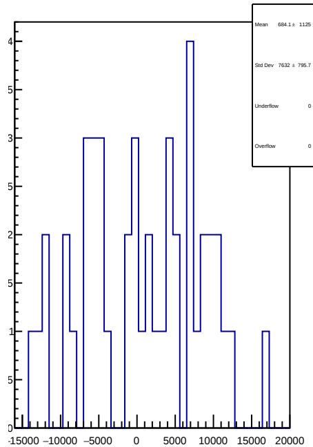
slug78: 1D Corr asym_at2_dd.mean/ppb-reg_asym_at2_dd.mean/ppb
