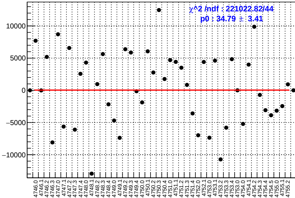
slug78: asym_atr1l2_dd.mean/ppb-reg_asym_atr1l2_dd.mean/ppb
