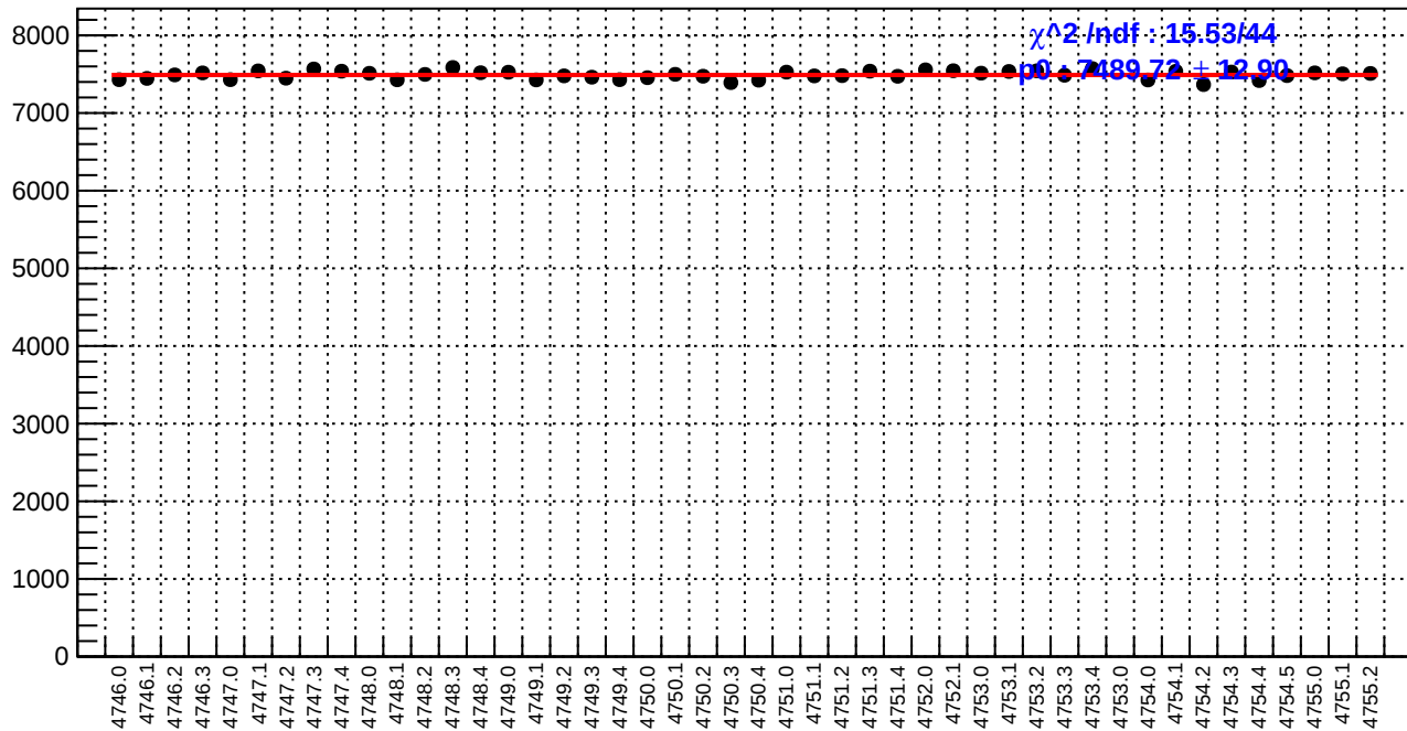
slug78: reg_asym_atr2.rms/ppm
