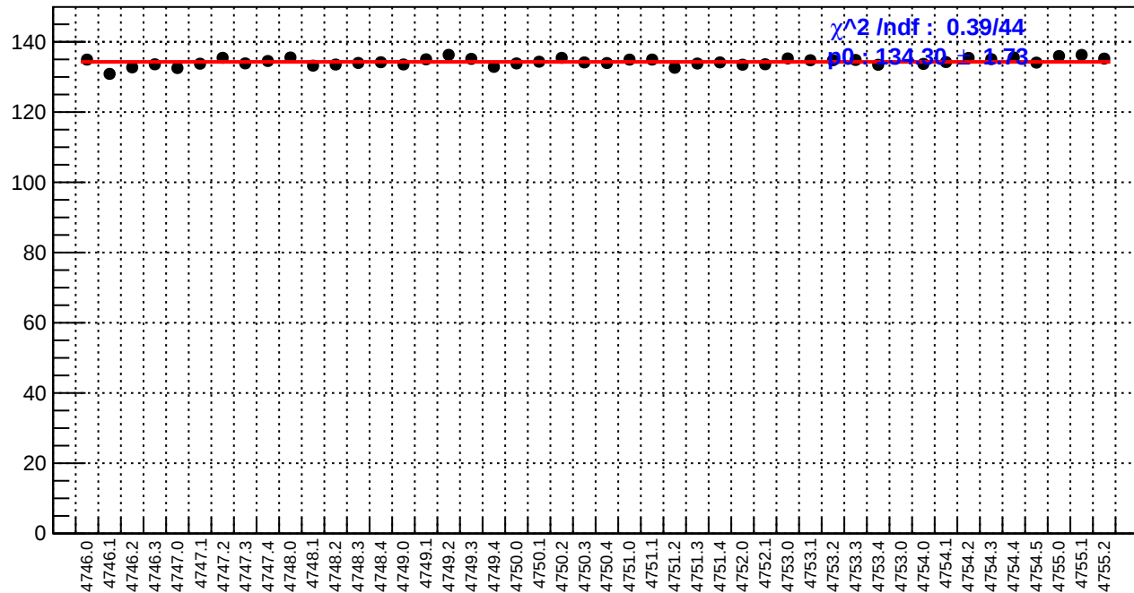
slug78: reg_asym_dsr.rms/ppm
