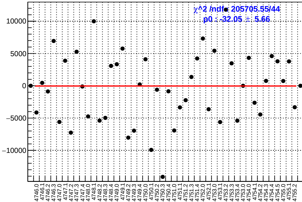
slug78: asym_atl1r2_dd.mean/ppb-reg_asym_atl1r2_dd.mean/ppb
