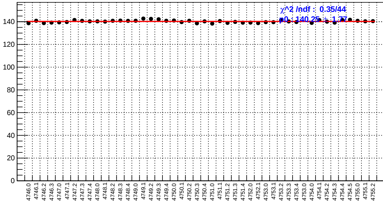
slug78: reg_asym_dsl.rms/ppm
