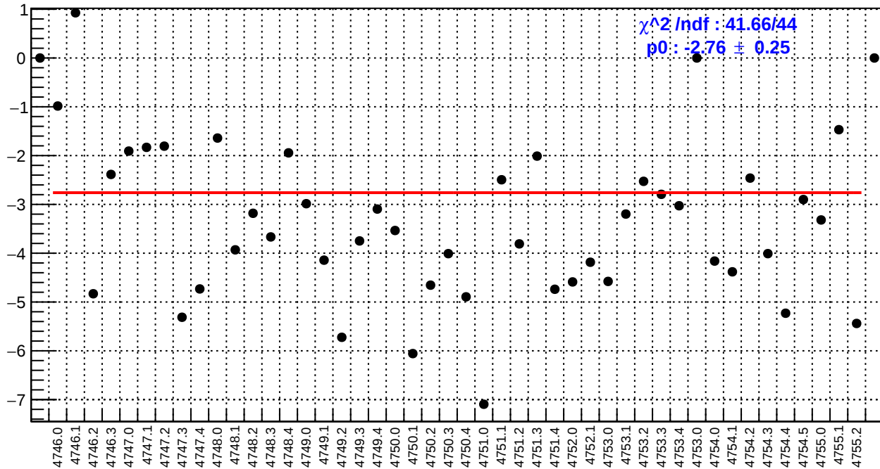
slug78: us_avg_bpm4aY/(ppb/nm)
