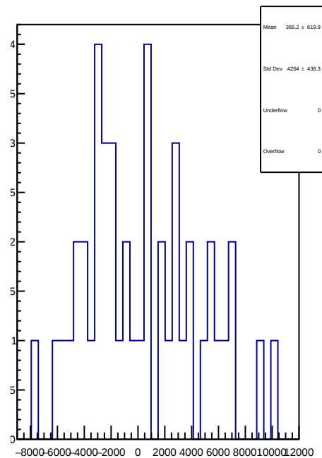
slug78: 1D Corr asym_dsr.mean/ppb-reg_asym_dsr.mean/ppb
