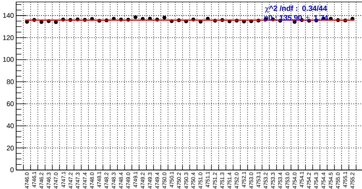
slug78: reg_asym_usl.rms/ppm
