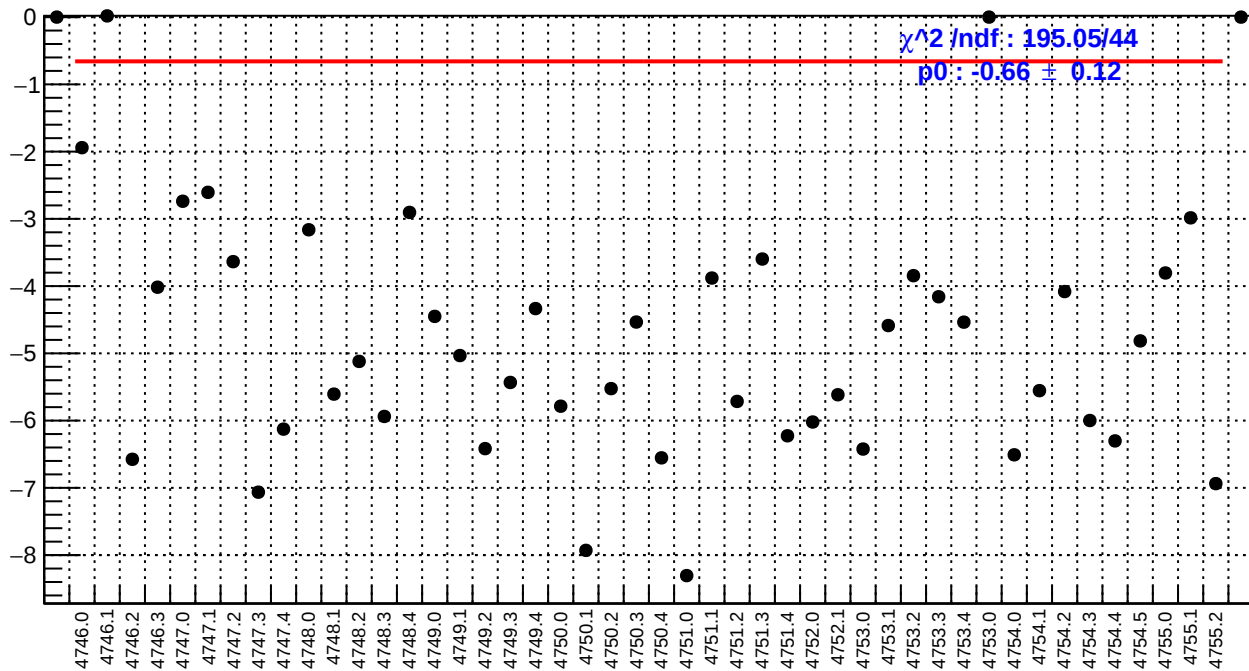
slug78: ds_avg_bpm4aY/(ppb/nm)
