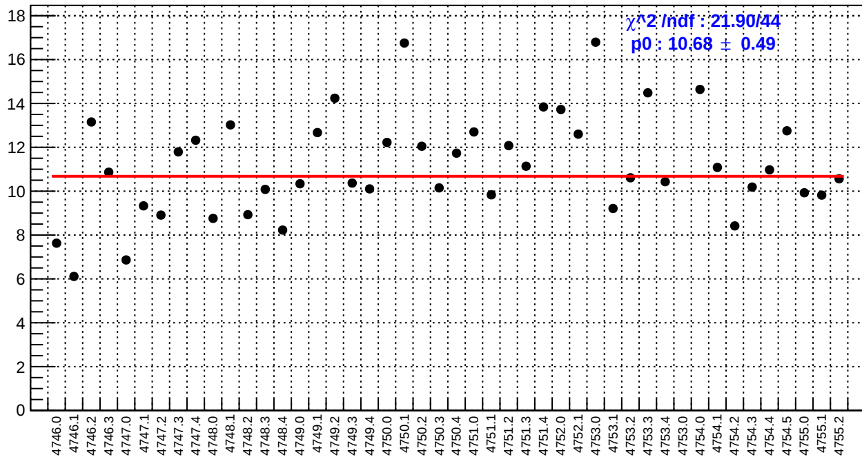
slug78: dsl_bpm4eY/(ppb/nm)
