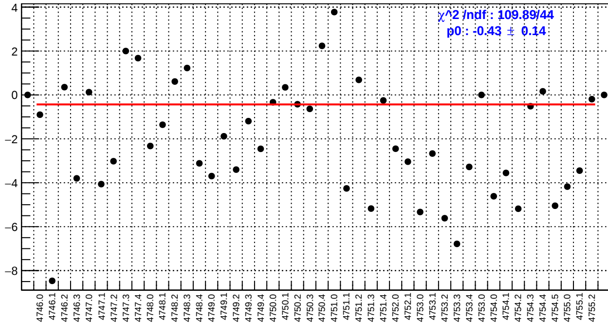
slug78: right_avg_bpm4eY/(ppb/nm)
