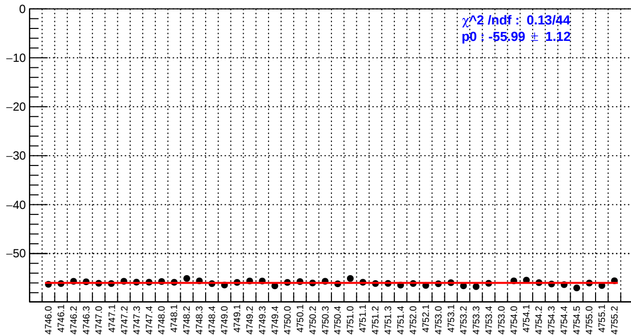
slug78: usr_bpm12X/(ppb/nm)
