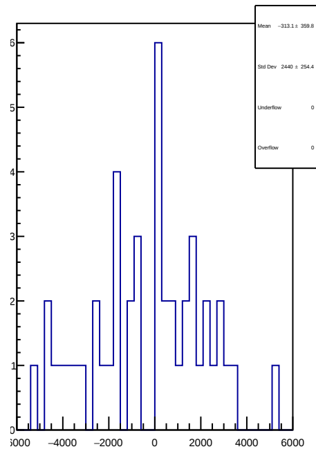
slug78: 1D Corr asym_atr_dd.mean/ppb-reg_asym_atr_dd.mean/ppb
