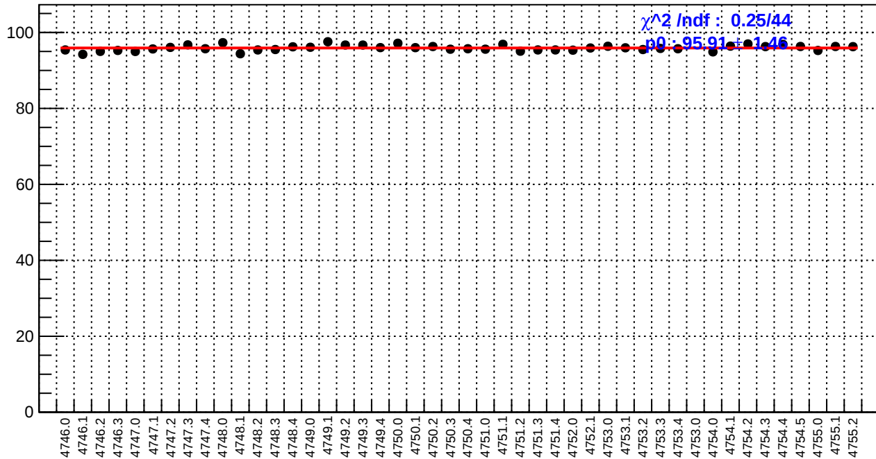
slug78: reg_asym_us_avg.rms/ppm
