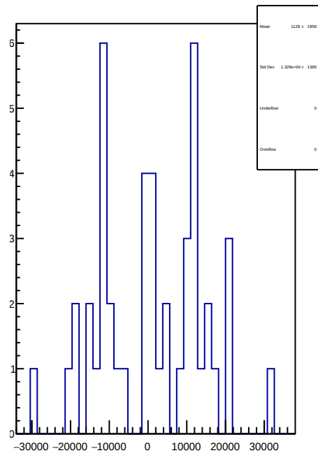
slug78: 1D Corr asym_sam8.mean/ppb-reg_asym_sam8.mean/ppb
