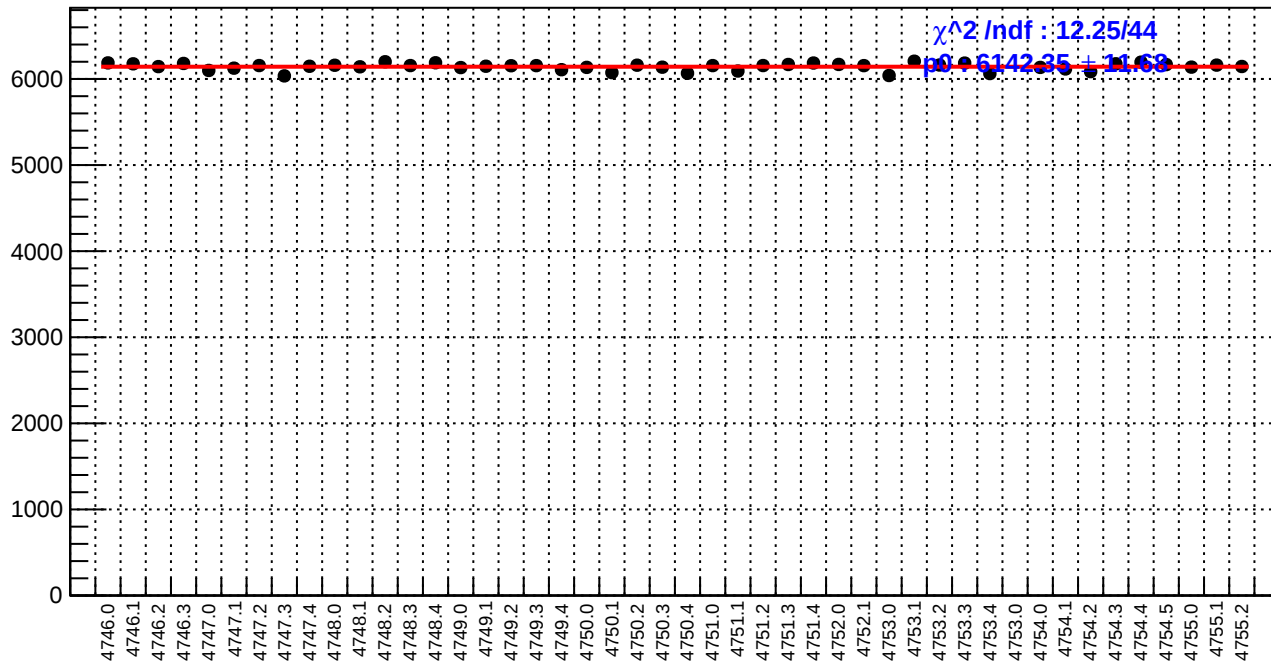
slug78: reg_asym_at1_avg.rms/ppm
