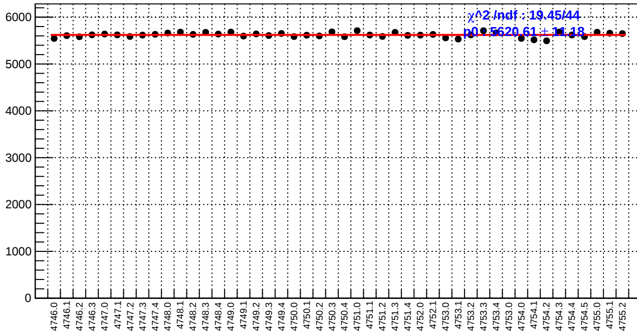
slug78: reg_asym_atl_dd.rms/ppm
