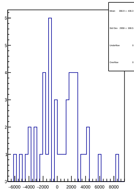
slug78: 1D Corr asym_atl1r2_avg.mean/ppb-reg_asym_atl1r2_avg.mean/ppb
