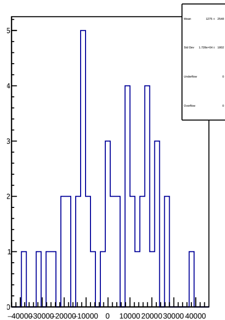
slug78: 1D Corr asym_sam7.mean/ppb-reg_asym_sam7.mean/ppb
