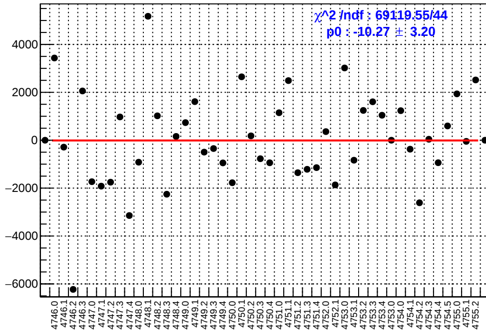
slug78: asym_ds_avg.mean/ppb-reg_asym_ds_avg.mean/ppb
