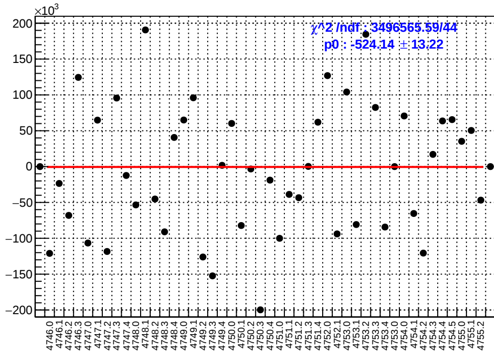
slug78: asym_sam3.mean/ppb-reg_asym_sam3.mean/ppb
