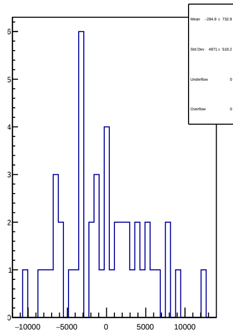
slug78: 1D Corr asym_usl.mean/ppb-reg_asym_usl.mean/ppb
