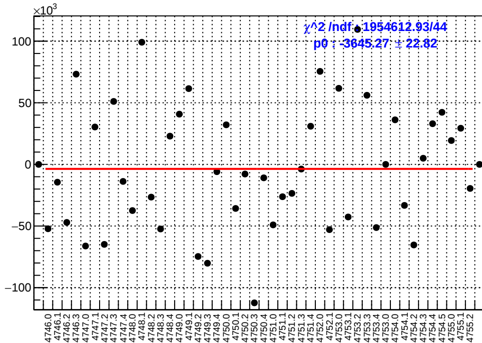
slug78: asym_sam2.mean/ppb-reg_asym_sam2.mean/ppb
