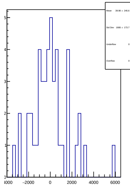
slug78: 1D Corr asym_at2_avg.mean/ppb-reg_asym_at2_avg.mean/ppb
