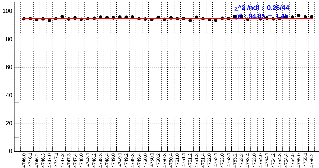
slug78: reg_asym_ds_dd.rms/ppm
