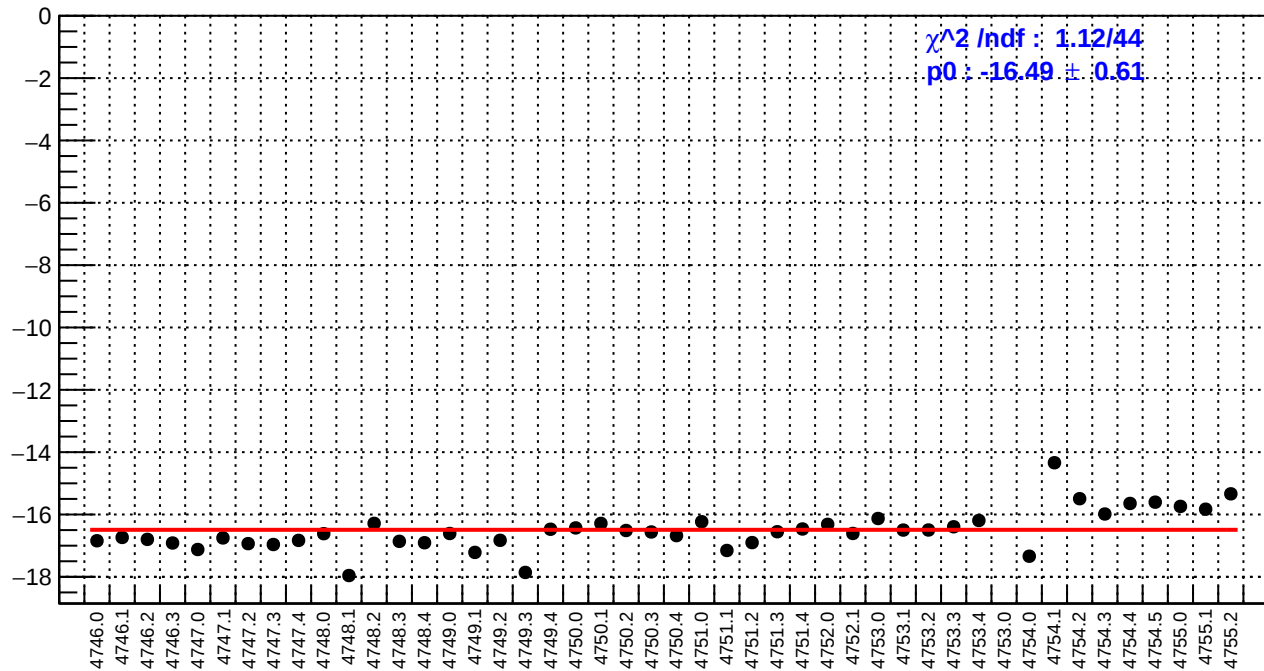
slug78: us_avg_bpm4eX/(ppb/nm)
