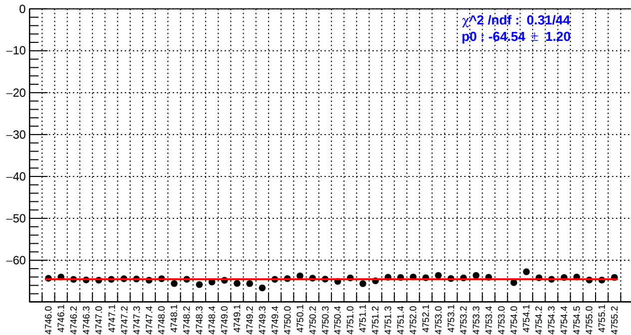
slug78: usl_bpm4eX/(ppb/nm)
