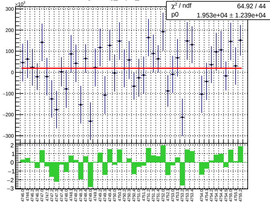
slug78: reg_asym_atl1.mean/ppb
