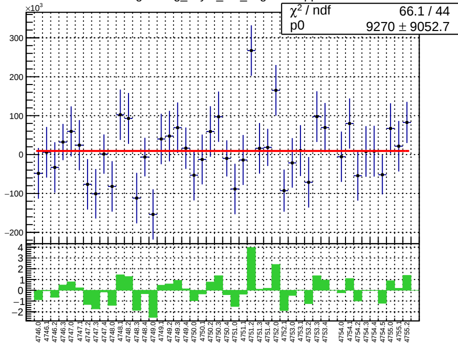
slug78: reg_asym_at1_avg.mean/ppb
