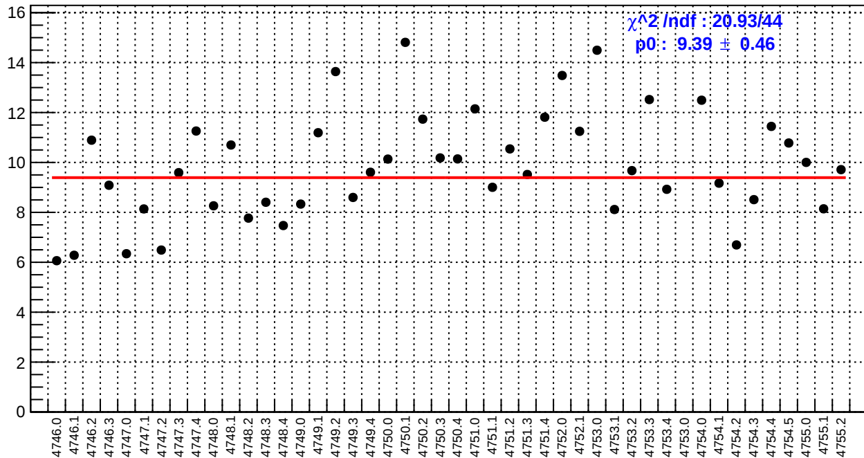
slug78: usl_bpm4eY/(ppb/nm)
