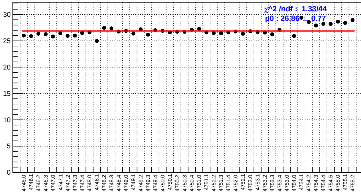
slug78: right_avg_bpm4eX/(ppb/nm)
