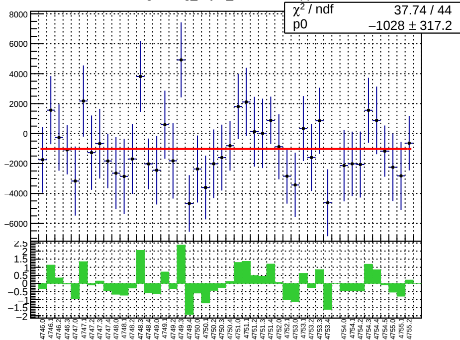
slug78: reg_asym_sam5.mean/ppb
