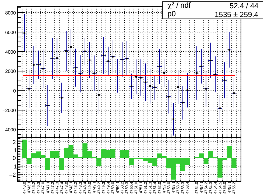
slug78: reg_asym_sam1.mean/ppb
