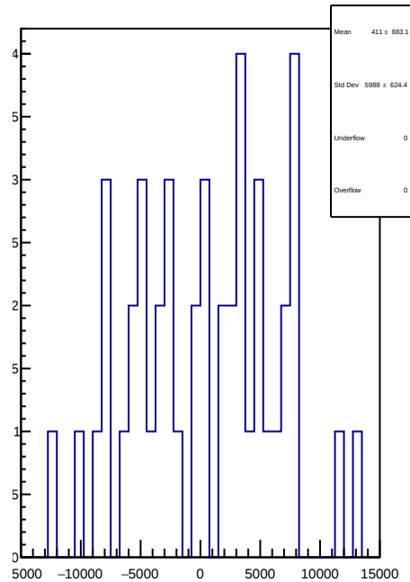
slug78: 1D Corr asym_atr_avg.mean/ppb-reg_asym_atr_avg.mean/ppb
