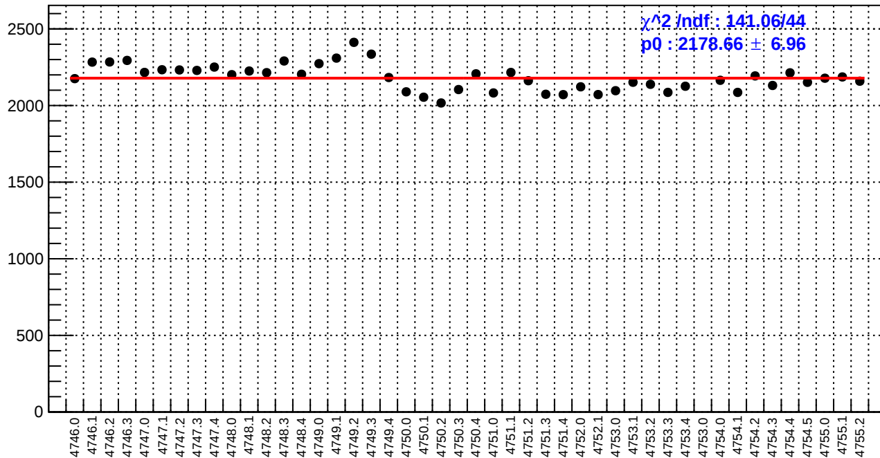
slug78: diff_bpm4eY.rms/nm
