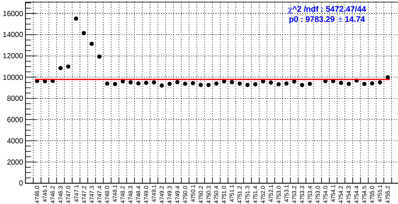
slug78: diff_bpm4eX.rms/nm
