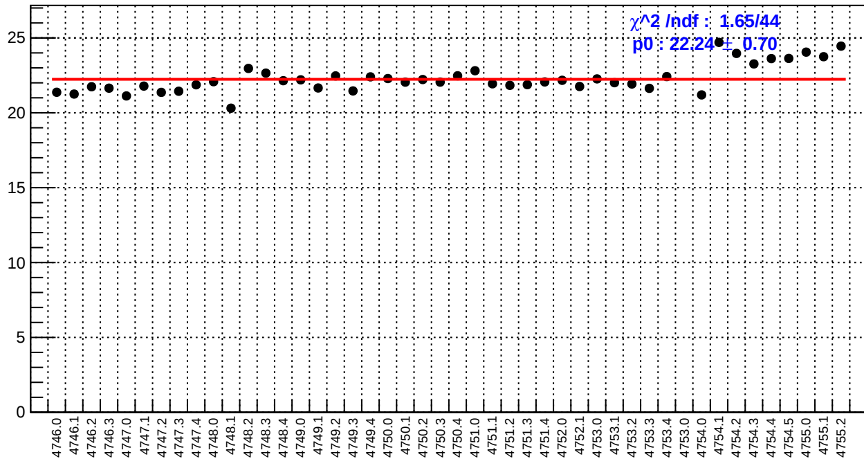
slug78: dsr_bpm4eX/(ppb/nm)
