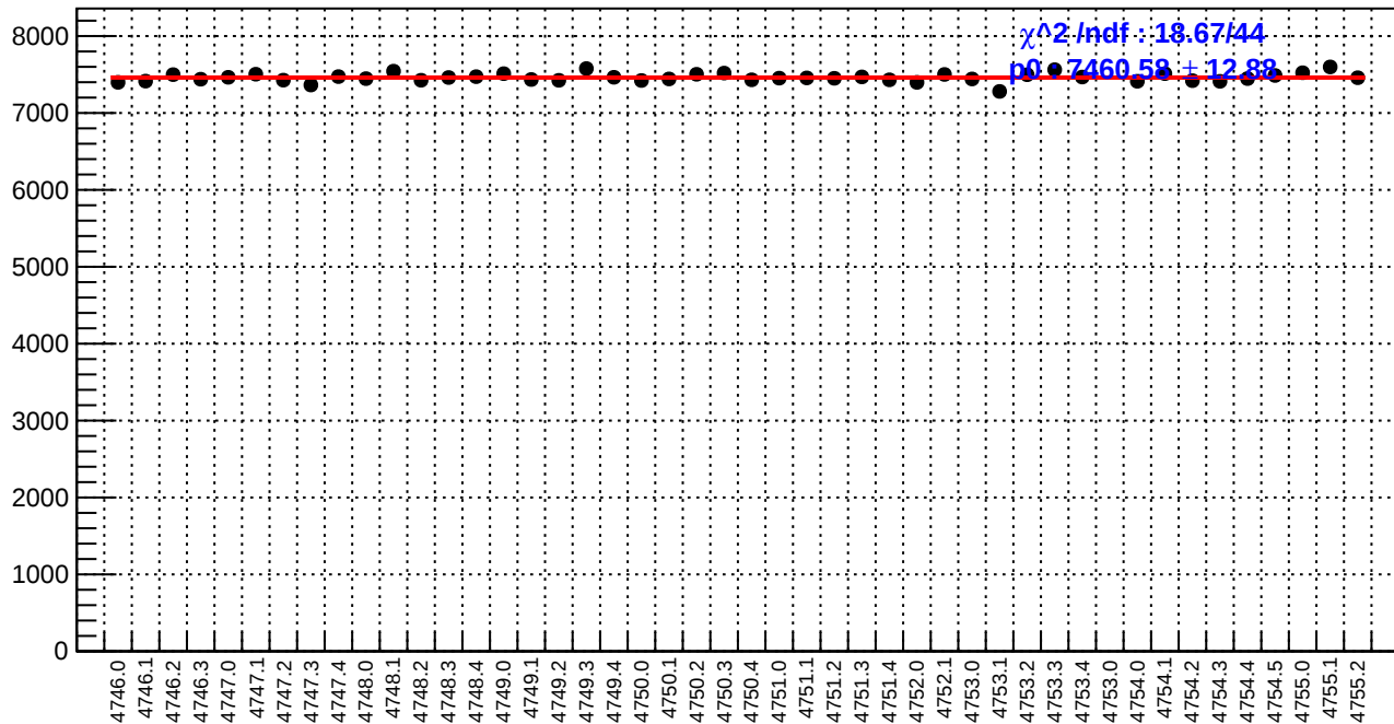
slug78: reg_asym_atl2.rms/ppm
