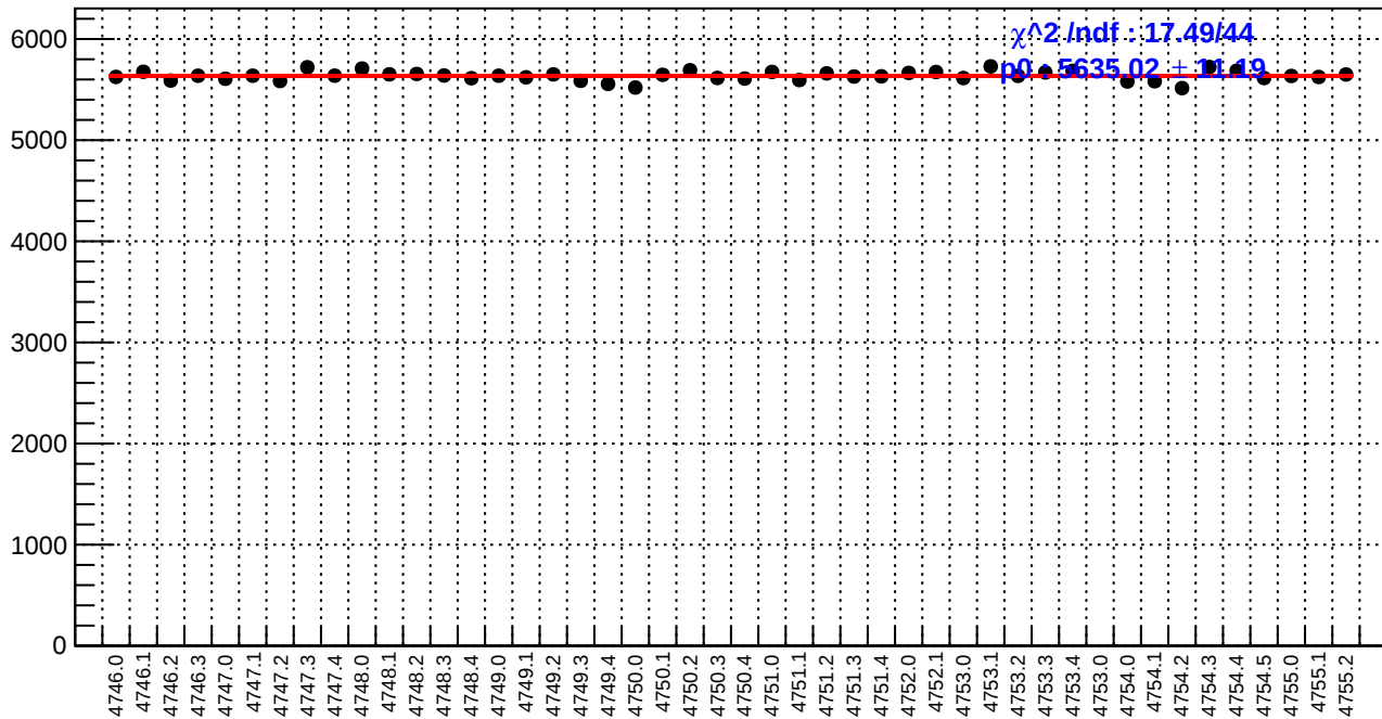
slug78: reg_asym_atl1r2_dd.rms/ppm
