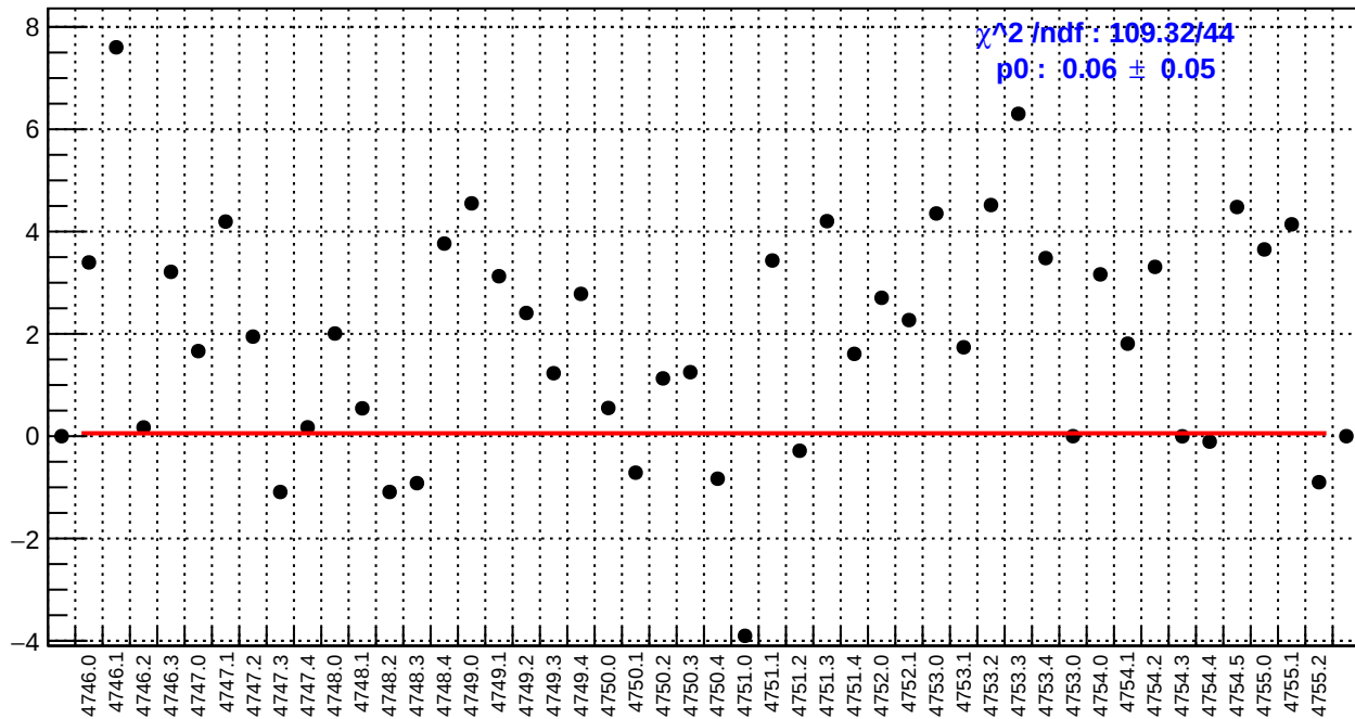
slug78: dsr_bpm4aY/(ppb/nm)
