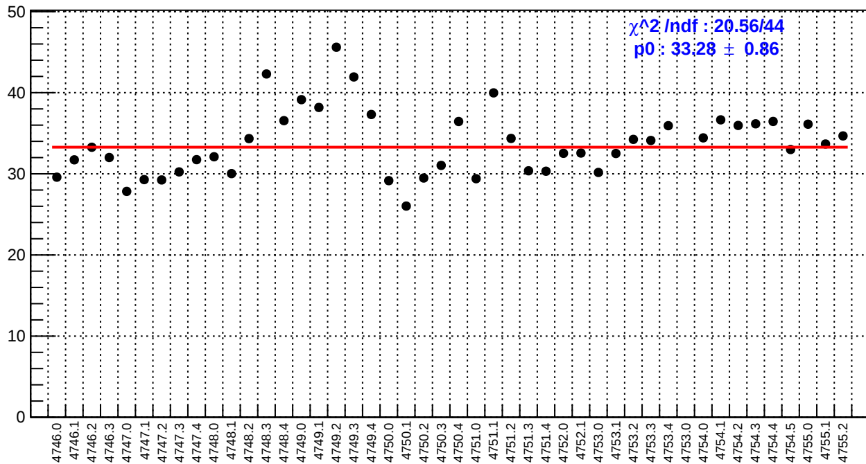
slug78: dsl_bpm4aX/(ppb/nm)
