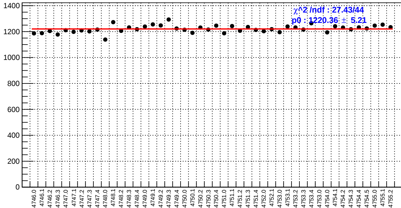
slug78: reg_asym_sam4.rms/ppm
