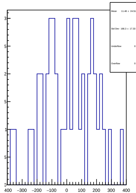
slug78: 1D Corr asym_left_dd.mean/ppb-reg_asym_left_dd.mean/ppb
