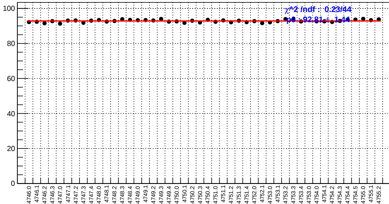
slug78: reg_asym_us_dd.rms/ppm
