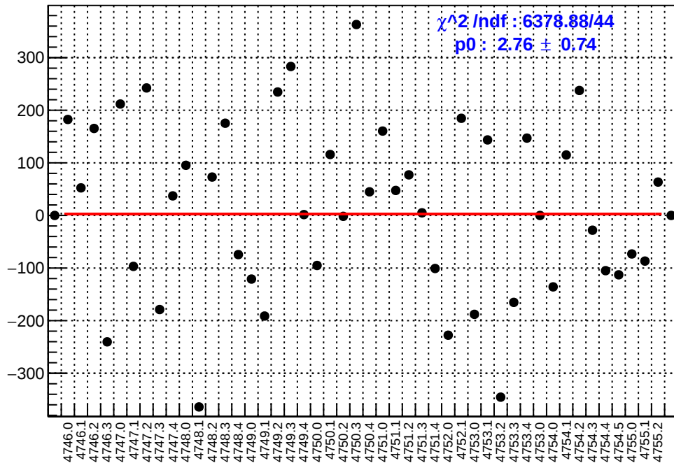
slug78: asym_left_dd.mean/ppb-reg_asym_left_dd.mean/ppb
