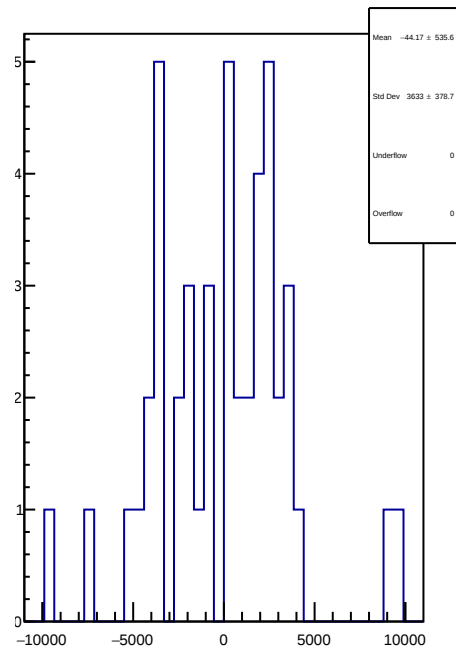
slug78: 1D Corr asym_at1_dd.mean/ppb-reg_asym_at1_dd.mean/ppb
