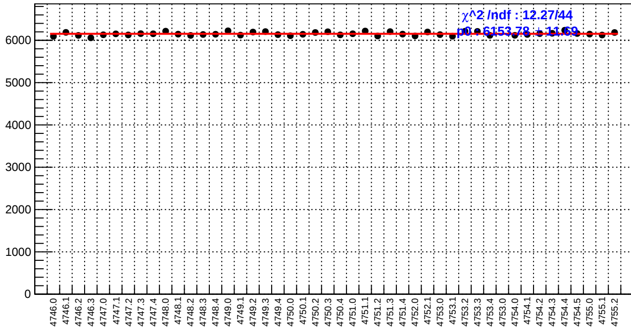
slug78: reg_asym_at1_dd.rms/ppm
