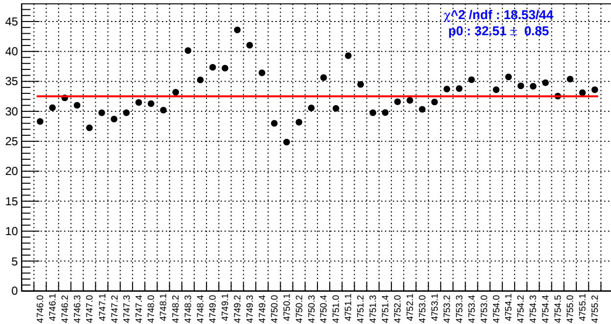
slug78: usl_bpm4aX/(ppb/nm)
