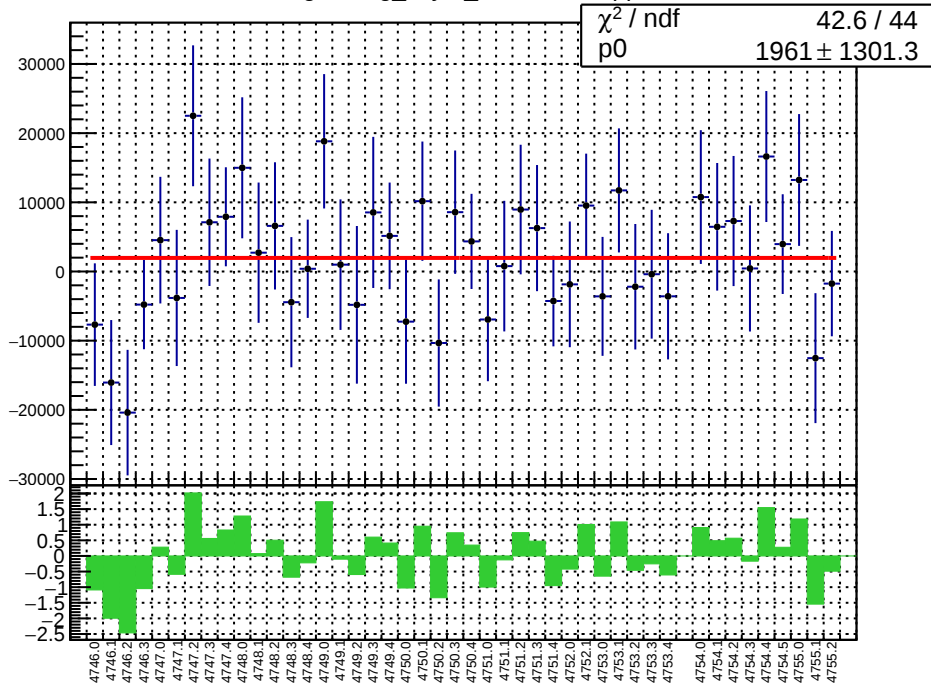
slug78: reg_asym_sam3.mean/ppb
