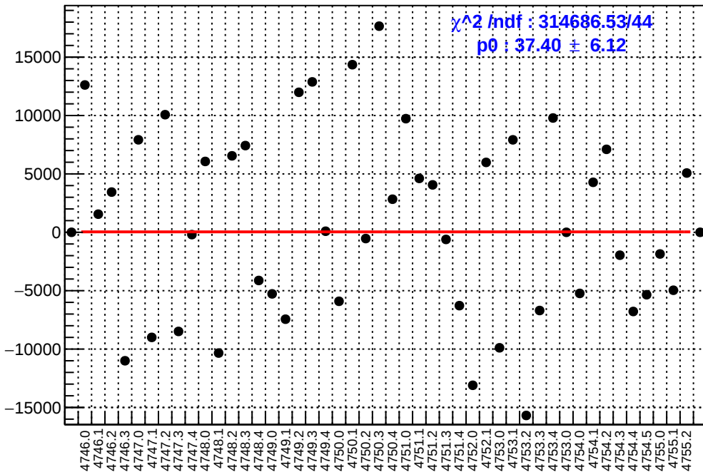
slug78: asym_atr2.mean/ppb-reg_asym_atr2.mean/ppb
