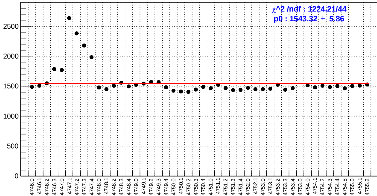
slug78: diff_bpm4aX.rms/nm
