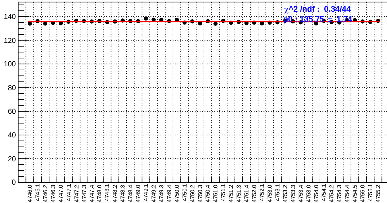
slug78: reg_asym_left_avg.rms/ppm
