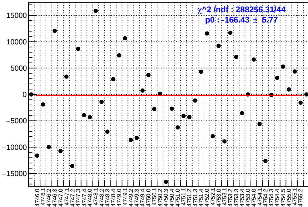
slug78: asym_atl2.mean/ppb-reg_asym_atl2.mean/ppb
