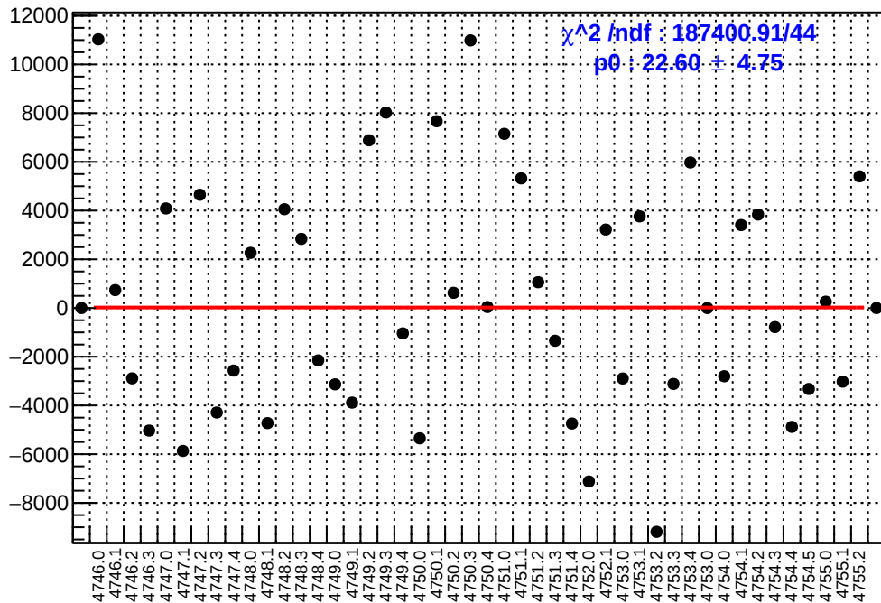
slug78: asym_usr.mean/ppb-reg_asym_usr.mean/ppb
