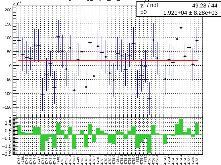
slug78: reg_asym_atl_dd.mean/ppb
