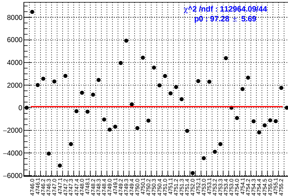
slug78: asym_atl1r2_avg.mean/ppb-reg_asym_atl1r2_avg.mean/ppb
