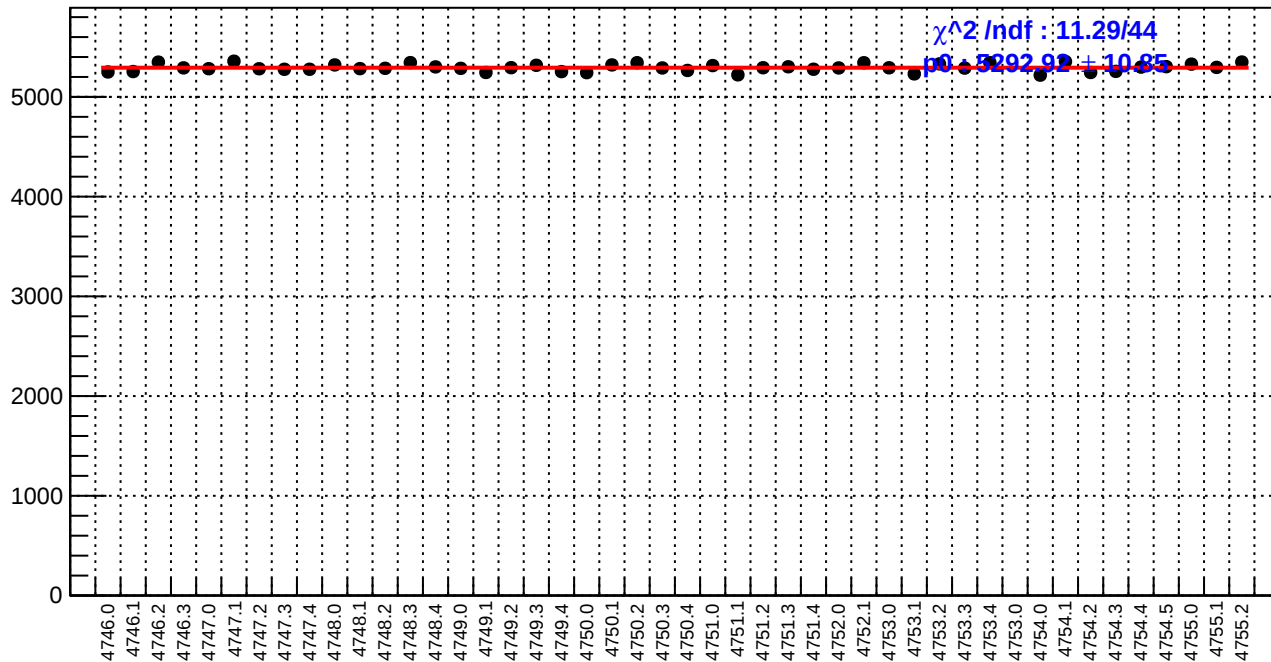
slug78: reg_asym_at2_dd.rms/ppm
