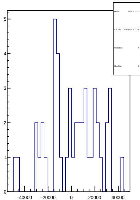
slug78: 1D Corr asym_sam6.mean/ppb-reg_asym_sam6.mean/ppb
