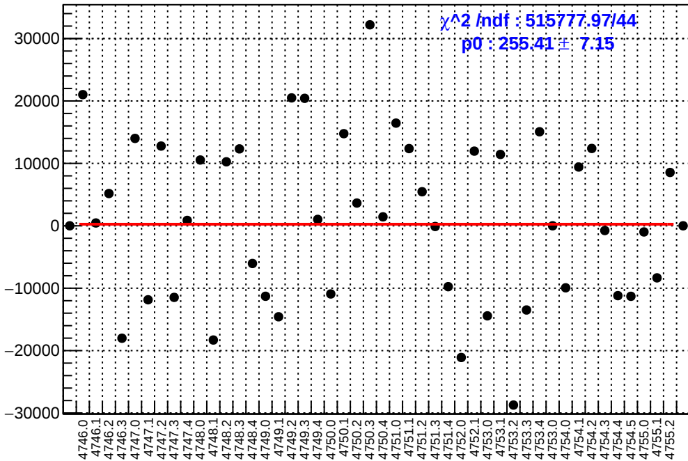
slug78: asym_sam8.mean/ppb-reg_asym_sam8.mean/ppb
