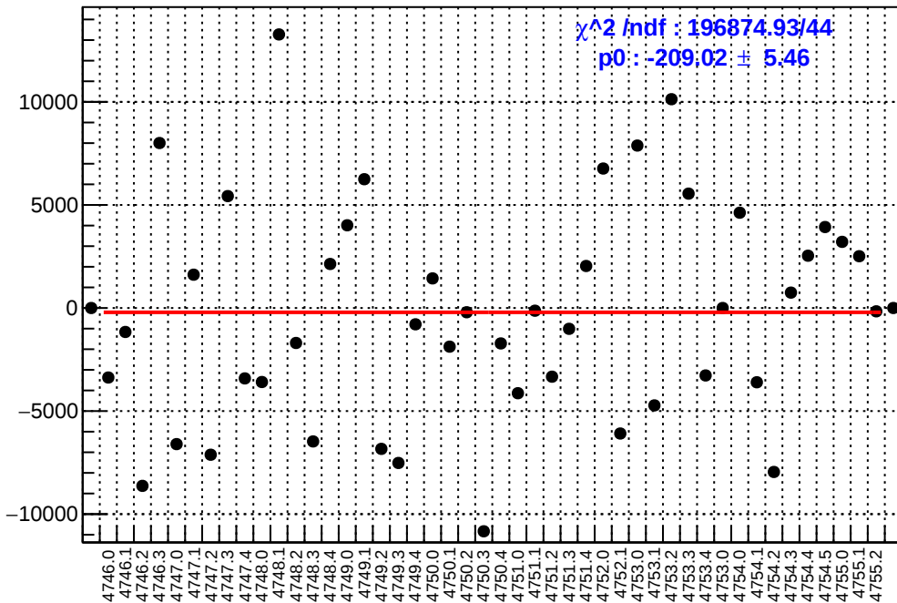
slug78: asym_dsl.mean/ppb-reg_asym_dsl.mean/ppb
