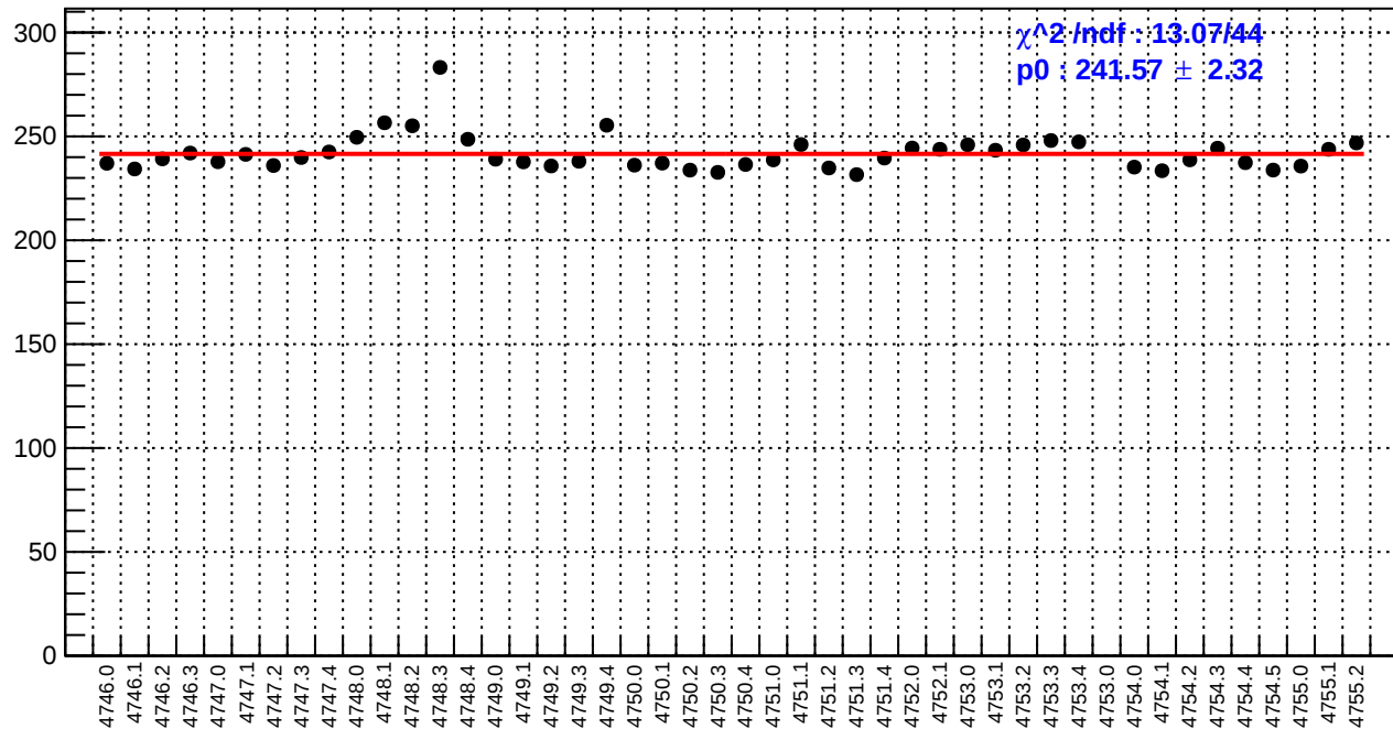
slug78: asym_bcm_an_us.rms/ppm
