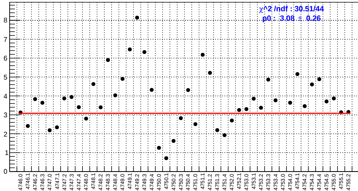
slug78: us_avg_bpm4aX/(ppb/nm)
