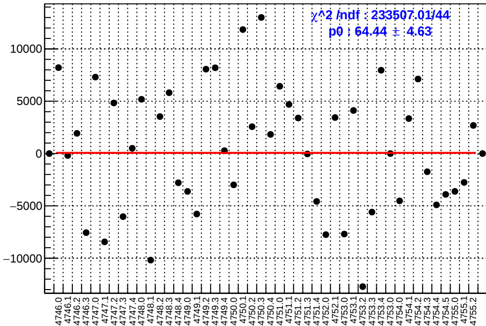
slug78: asym_atr_avg.mean/ppb-reg_asym_atr_avg.mean/ppb
