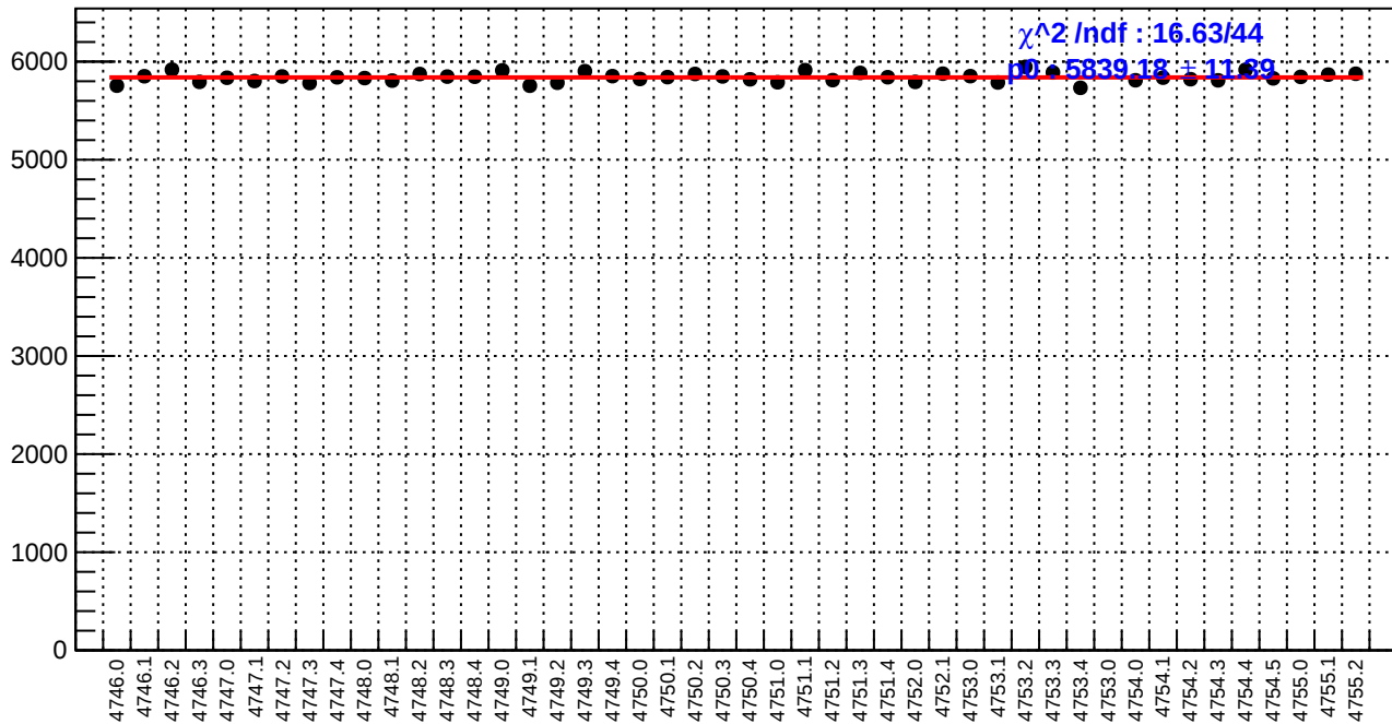
slug78: reg_asym_atr1l2_dd.rms/ppm
