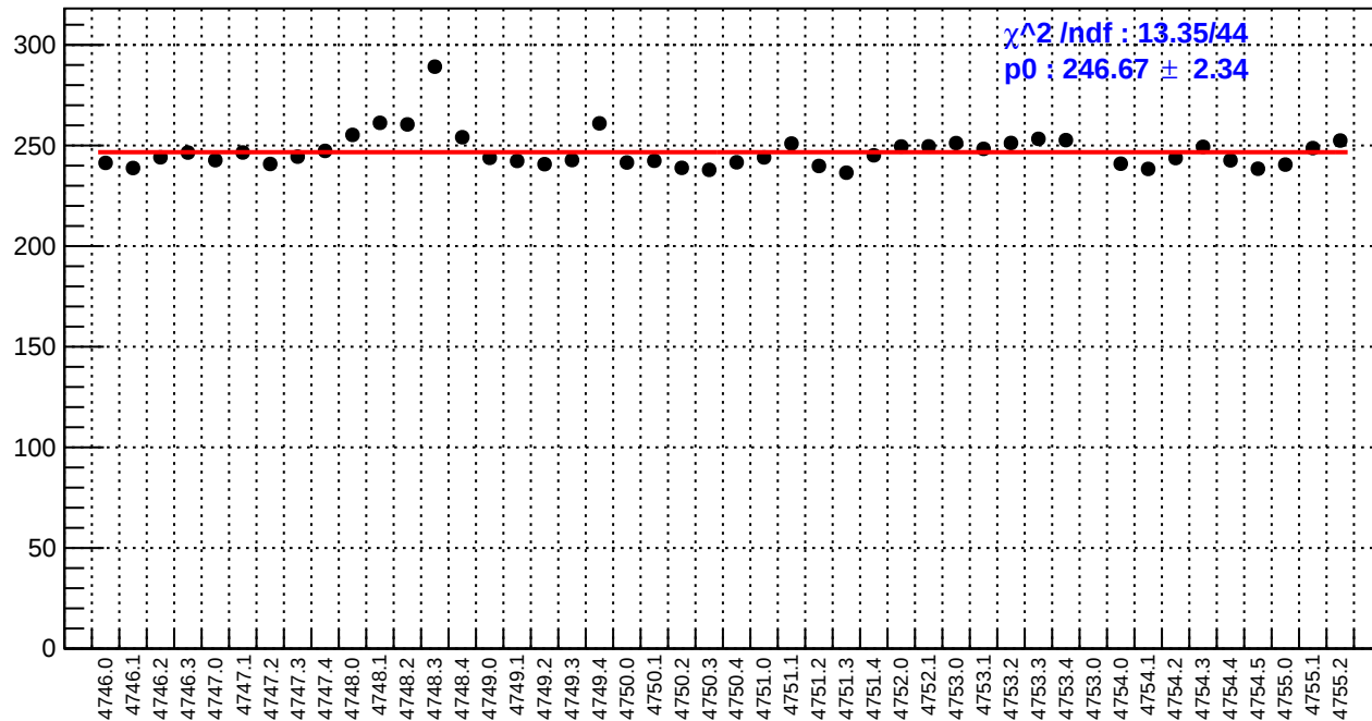
slug78: asym_bcm_an_ds3.rms/ppm
