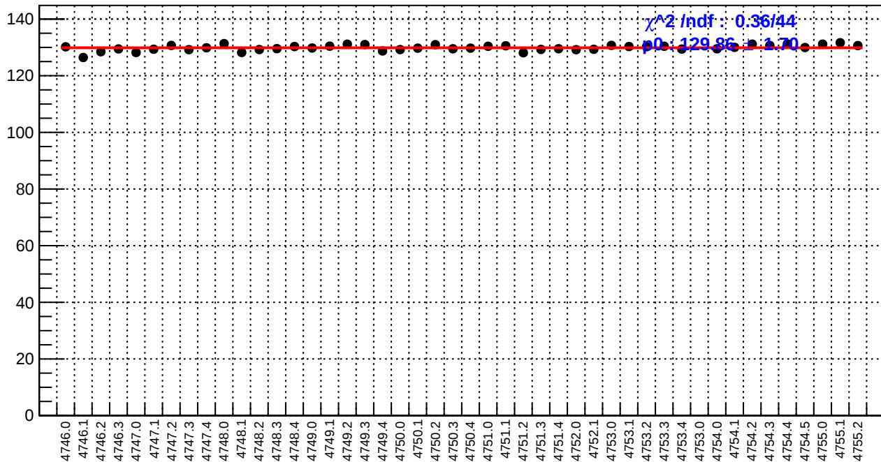
slug78: reg_asym_right_avg.rms/ppm
