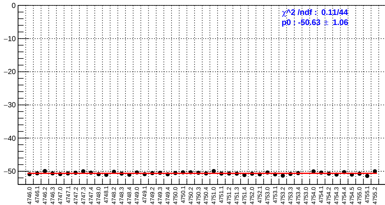
slug78: ds_avg_bpm12X/(ppb/nm)
