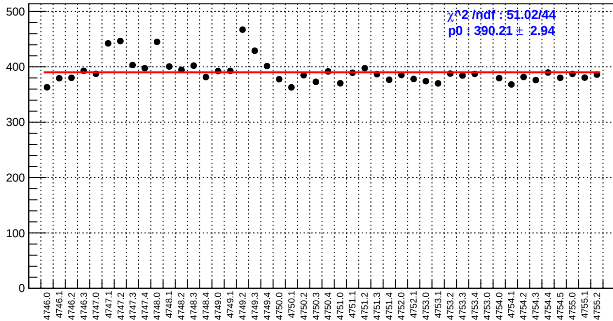
slug78: reg_asym_sam6.rms/ppm
