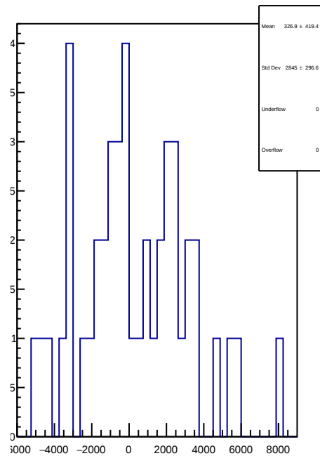
slug78: 1D Corr asym_atl_dd.mean/ppb-reg_asym_atl_dd.mean/ppb
