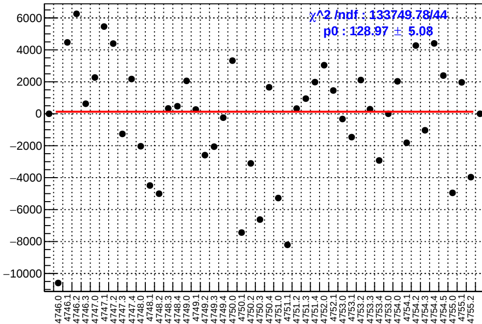
slug78: asym_sam5.mean/ppb-reg_asym_sam5.mean/ppb
