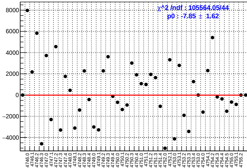
slug78: asym_atl_dd.mean/ppb-reg_asym_atl_dd.mean/ppb
