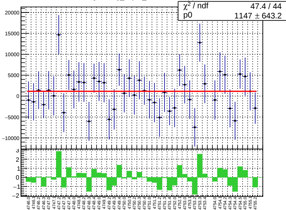
slug78: reg_asym_sam8.mean/ppb
