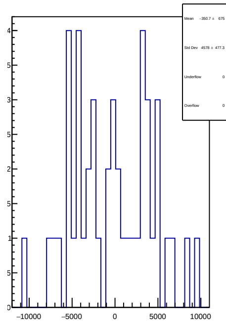
slug78: 1D Corr asym_us_dd.mean/ppb-reg_asym_us_dd.mean/ppb
