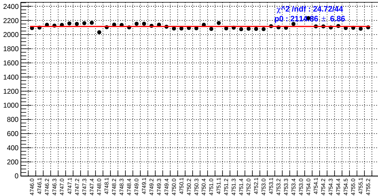
slug78: reg_asym_sam2.rms/ppm
