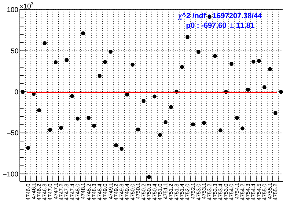
slug78: asym_sam4.mean/ppb-reg_asym_sam4.mean/ppb
