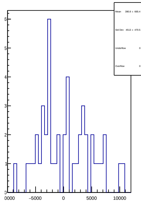
slug78: 1D Corr asym_right_avg.mean/ppb-reg_asym_right_avg.mean/ppb
