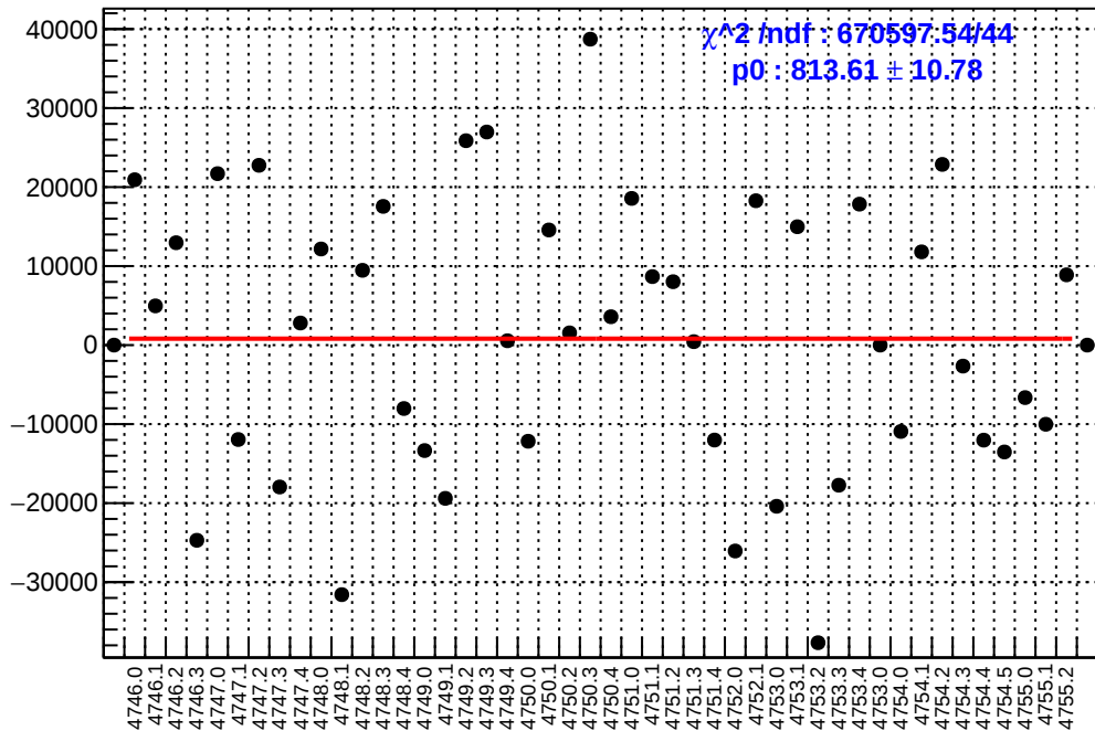
slug78: asym_sam7.mean/ppb-reg_asym_sam7.mean/ppb
