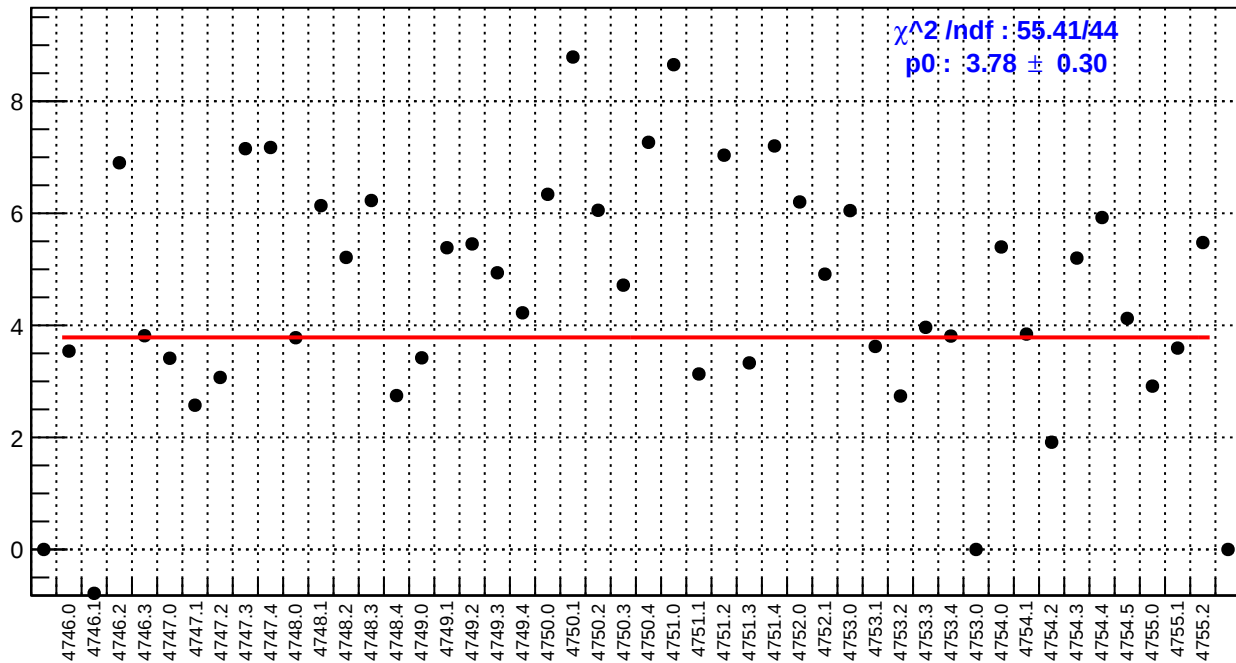
slug78: ds_avg_bpm4eY/(ppb/nm)
