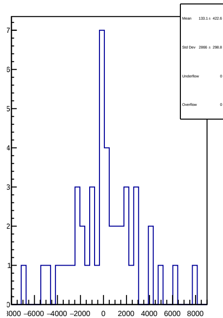
slug78: 1D Corr asym_sam1.mean/ppb-reg_asym_sam1.mean/ppb
