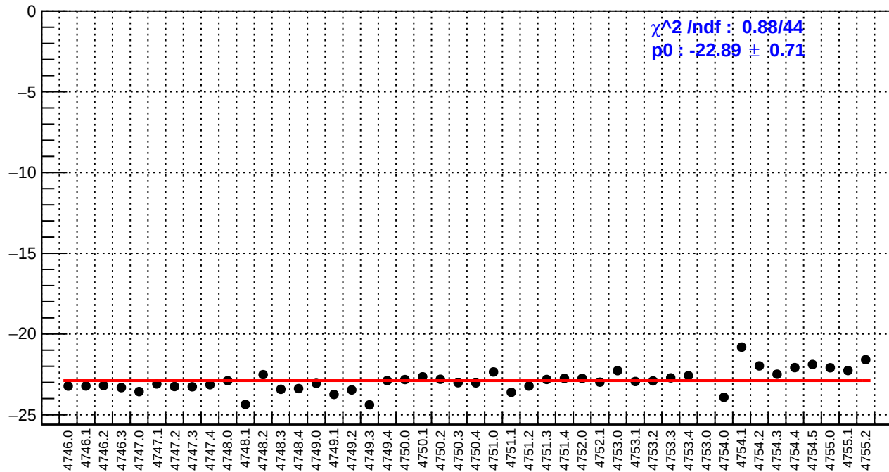
slug78: ds_avg_bpm4eX/(ppb/nm)
