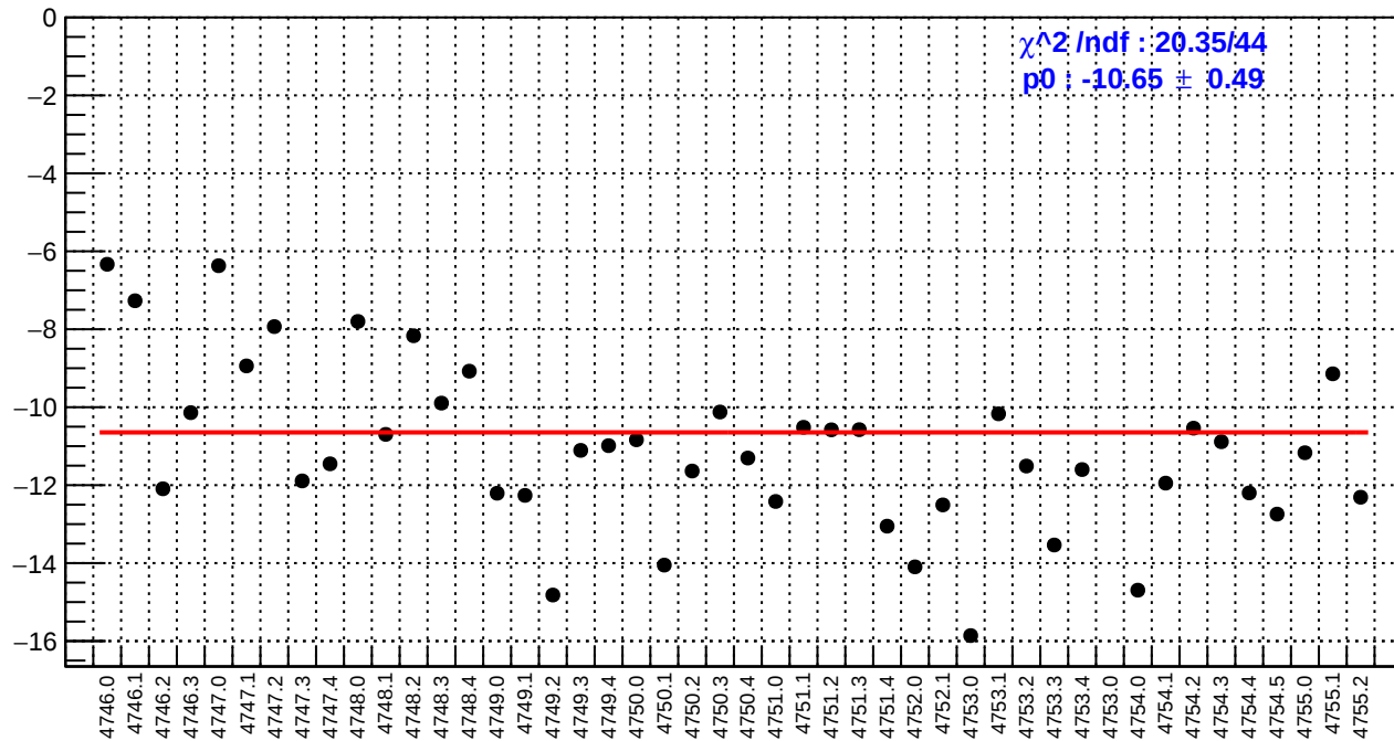
slug78: left_avg_bpm4aY/(ppb/nm)
