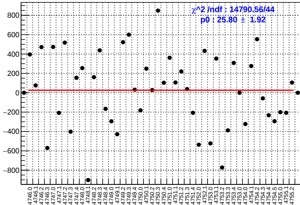
slug78: asym_right_dd.mean/ppb-reg_asym_right_dd.mean/ppb
