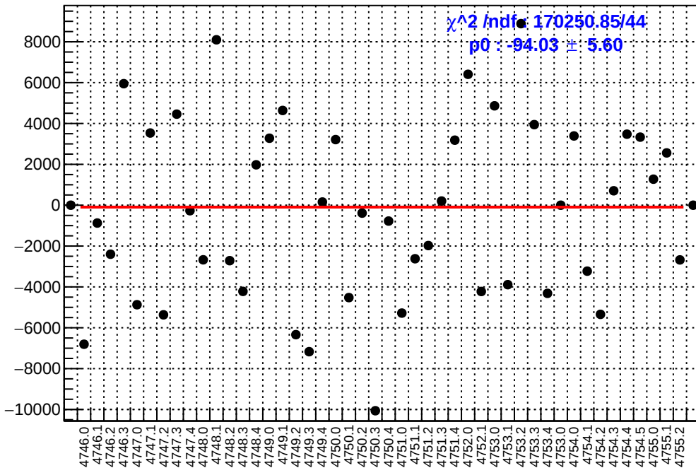
slug78: asym_ds_dd.mean/ppb-reg_asym_ds_dd.mean/ppb
