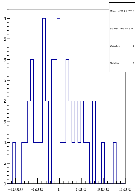
slug78: 1D Corr asym_left_avg.mean/ppb-reg_asym_left_avg.mean/ppb
