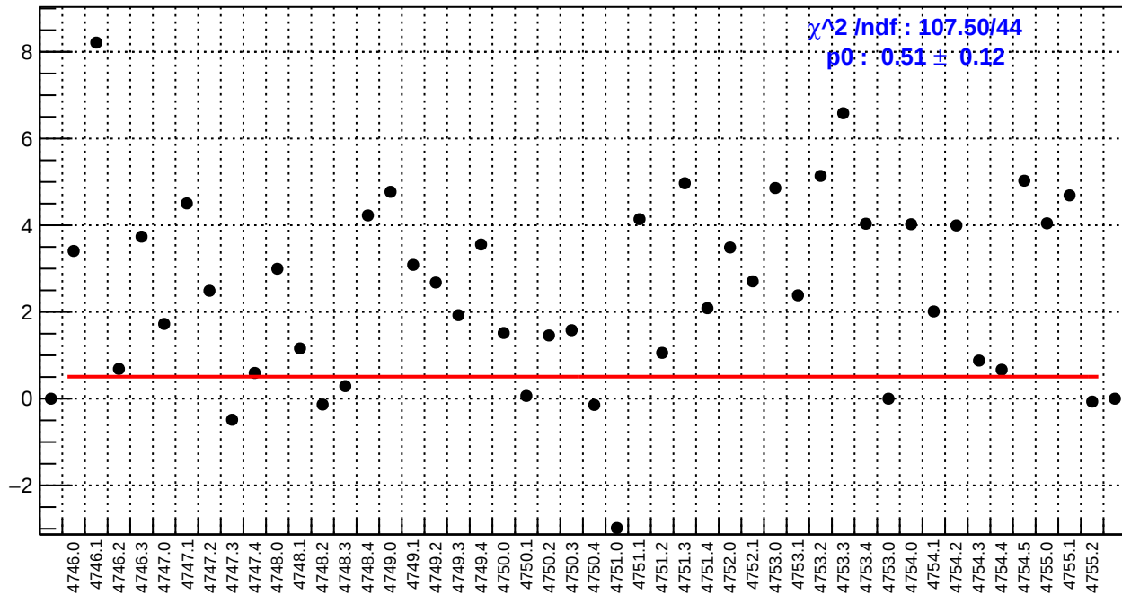
slug78: right_avg_bpm4aY/(ppb/nm)
