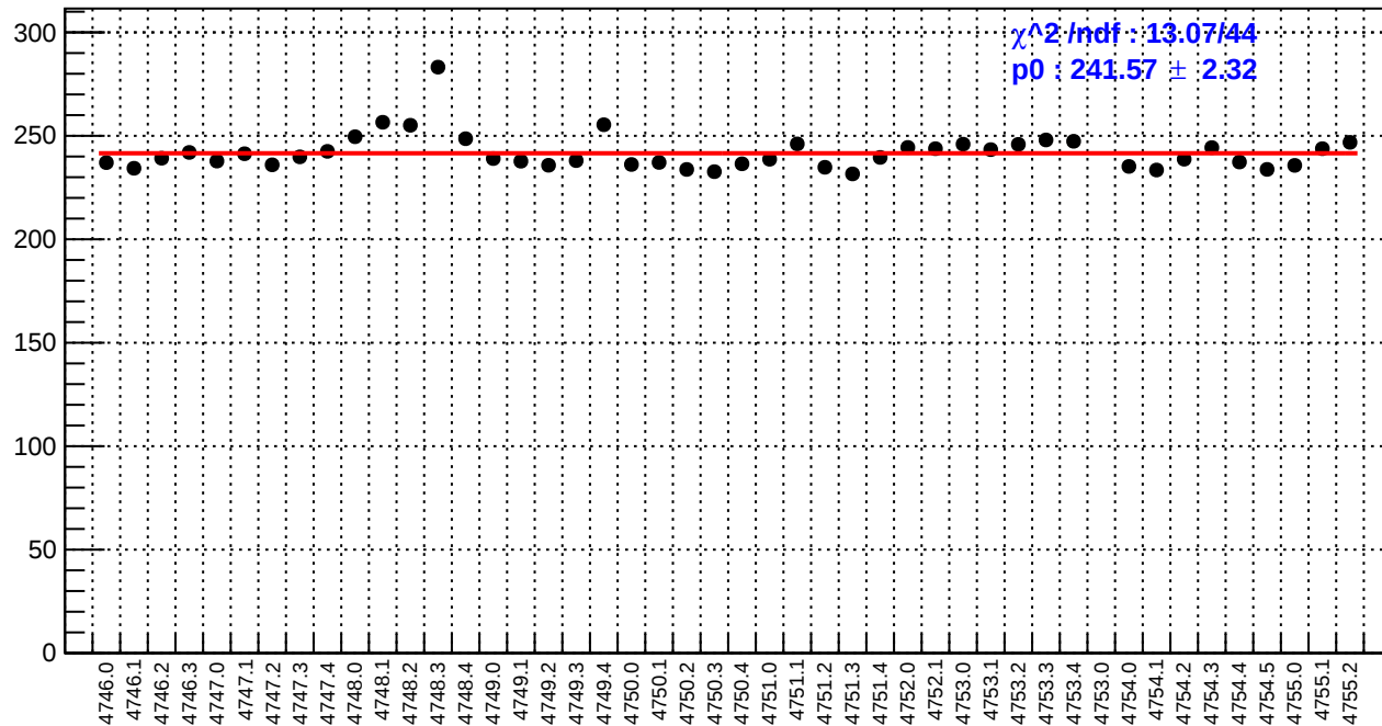
slug78: asym_bcm_an_us.rms/ppm
