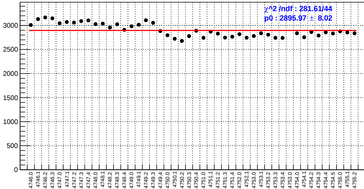
slug78: diff_bpm4aY.rms/nm
