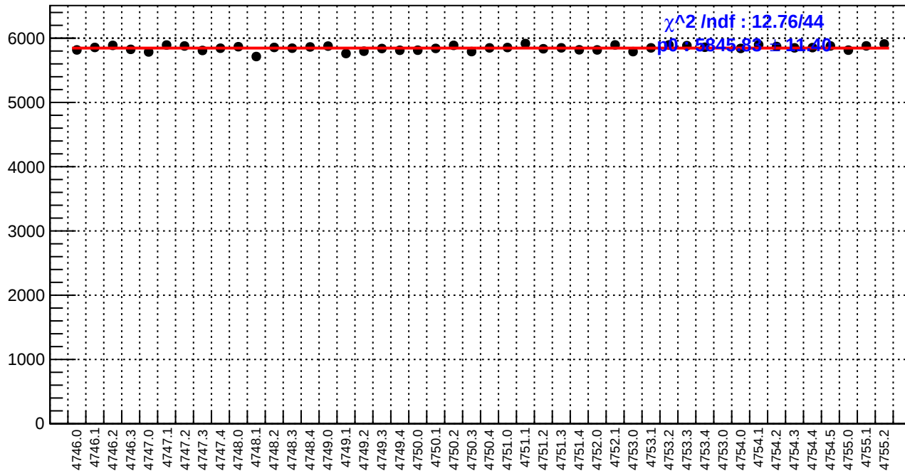
slug78: reg_asym_atr_dd.rms/ppm
