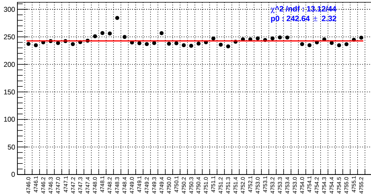
slug78: asym_bcm_an_ds.rms/ppm
