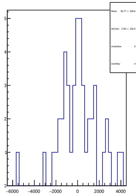
slug78: 1D Corr asym_us_avg.mean/ppb-reg_asym_us_avg.mean/ppb
