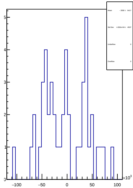
slug78: 1D Corr asym_sam4.mean/ppb-reg_asym_sam4.mean/ppb
