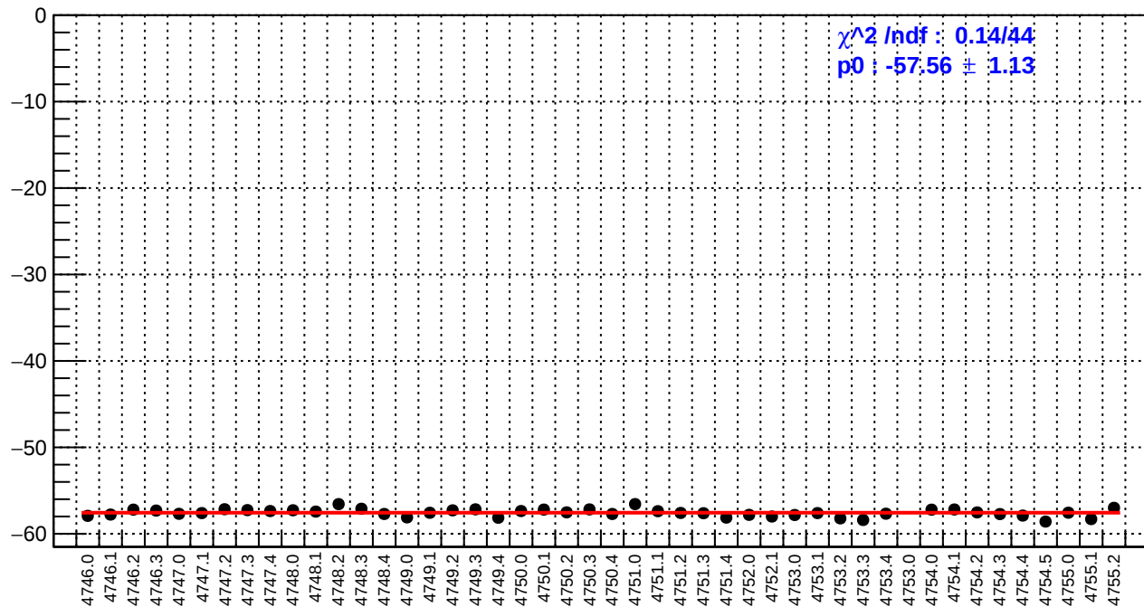
slug78: right_avg_bpm12X/(ppb/nm)
