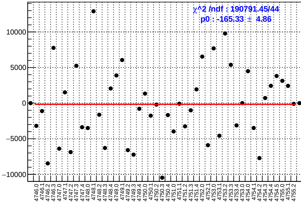
slug78: asym_left_avg.mean/ppb-reg_asym_left_avg.mean/ppb
