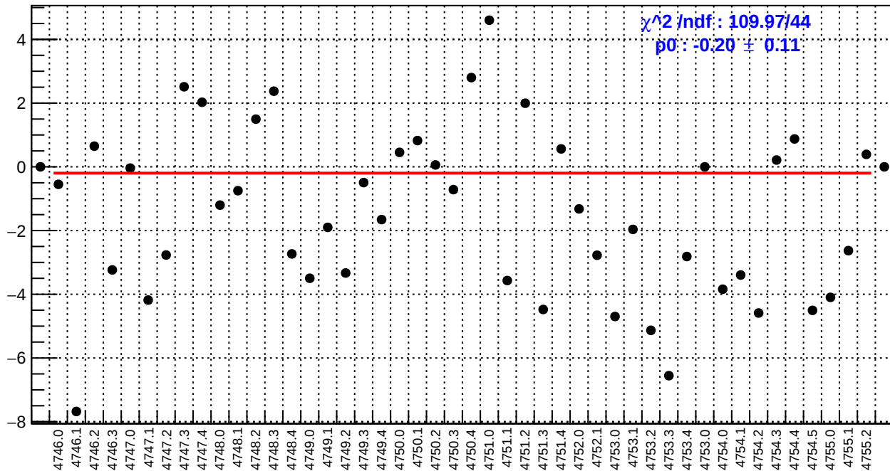
slug78: dsr_bpm4eY/(ppb/nm)
