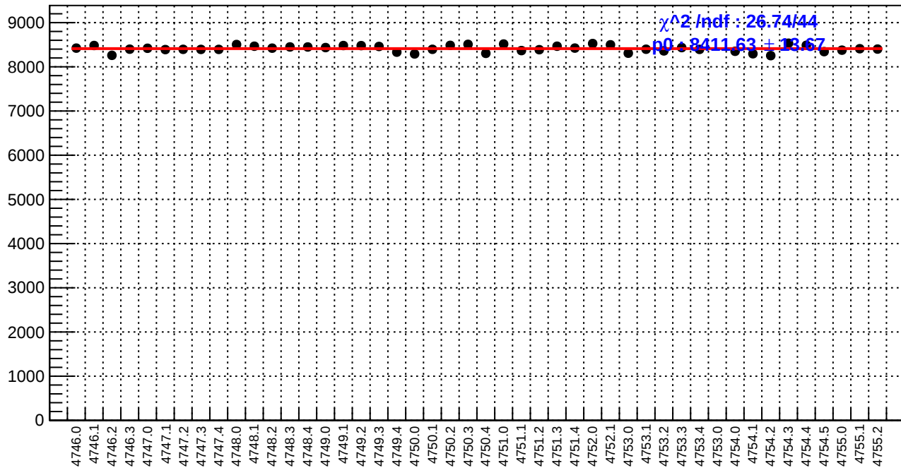
slug78: reg_asym_atl1.rms/ppm
