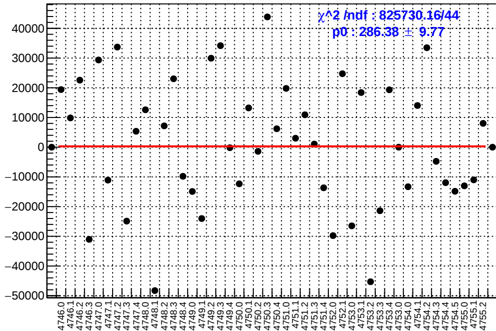
slug78: asym_sam6.mean/ppb-reg_asym_sam6.mean/ppb
