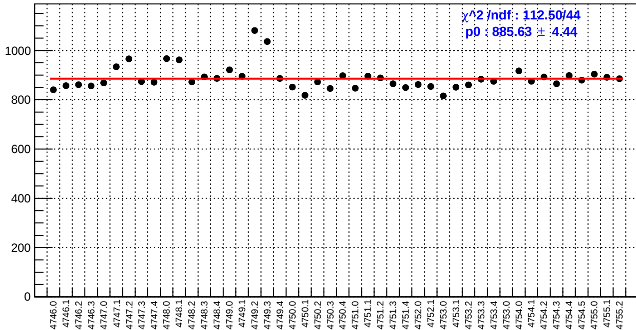
slug78: reg_asym_sam3.rms/ppm
