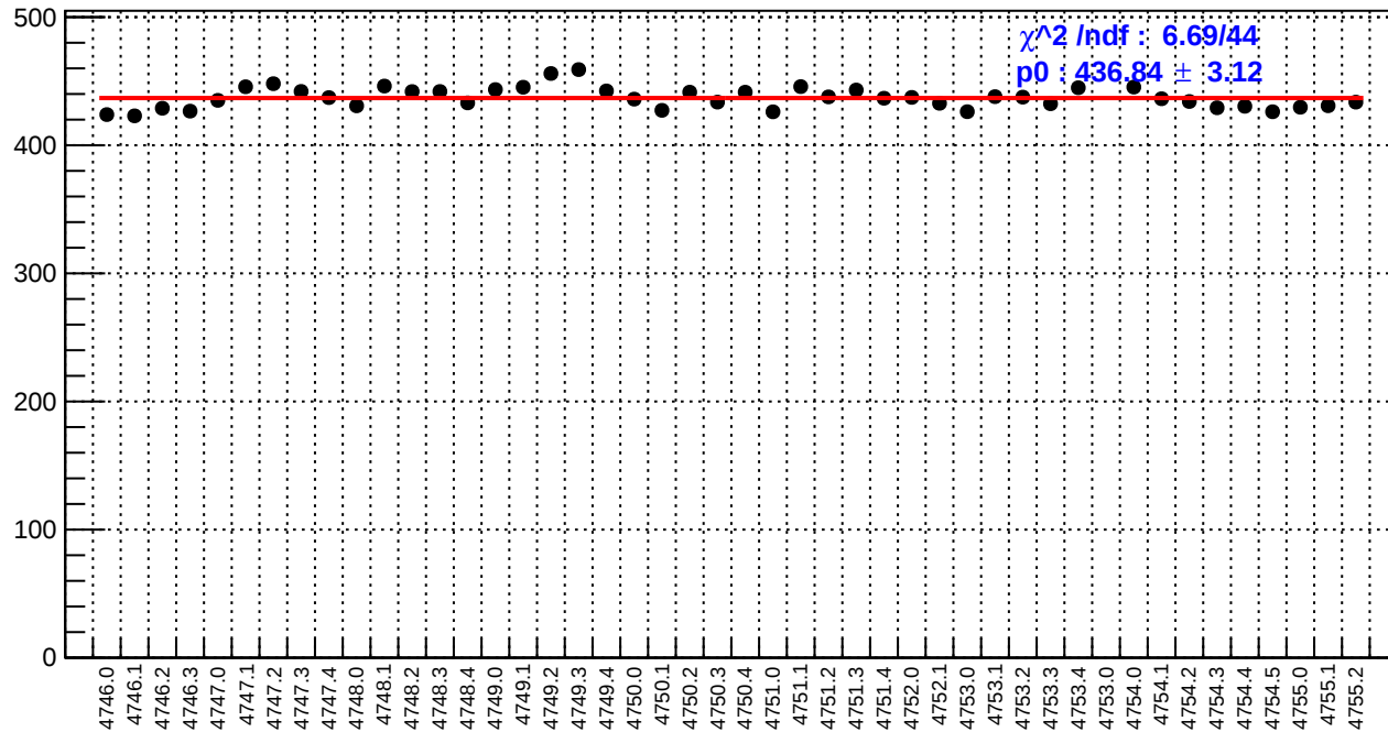
slug78: reg_asym_sam8.rms/ppm
