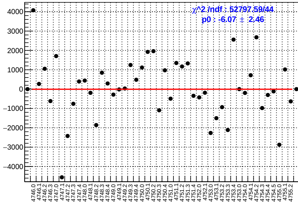
slug78: asym_at1_avg.mean/ppb-reg_asym_at1_avg.mean/ppb
