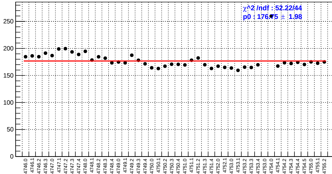
slug78: reg_asym_sam1.rms/ppm
