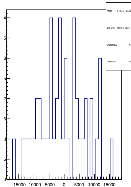
slug78: 1D Corr asym_atl2.mean/ppb-reg_asym_atl2.mean/ppb
