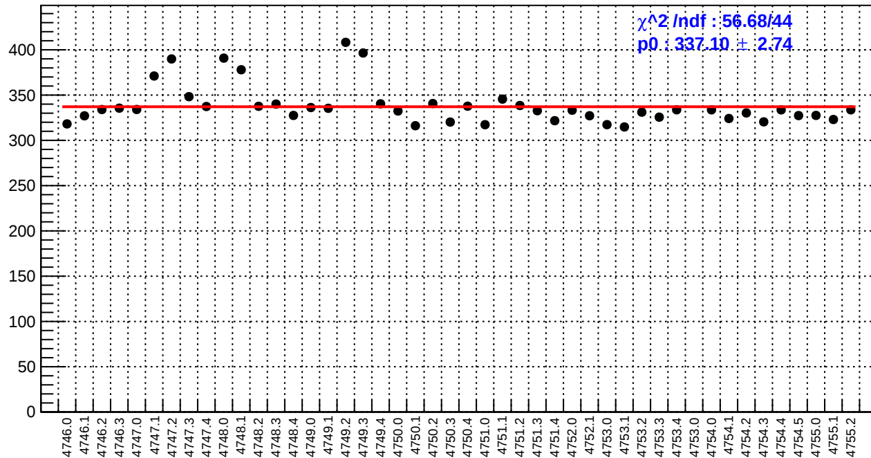
slug78: reg_asym_sam7.rms/ppm
