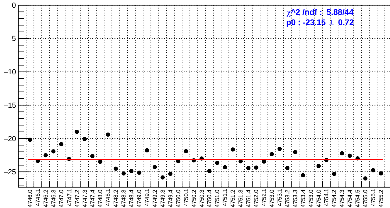
slug78: right_avg_bpm4aX/(ppb/nm)
