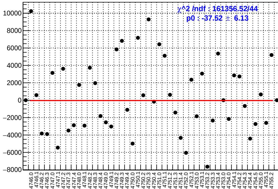
slug78: asym_dsr.mean/ppb-reg_asym_dsr.mean/ppb
