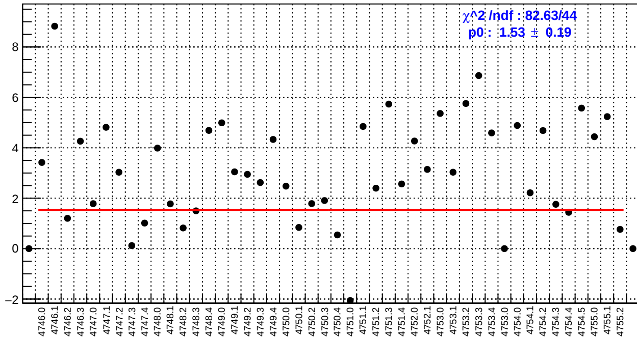
slug78: usr_bpm4aY/(ppb/nm)
