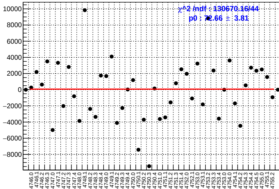
slug78: asym_at1_dd.mean/ppb-reg_asym_at1_dd.mean/ppb
