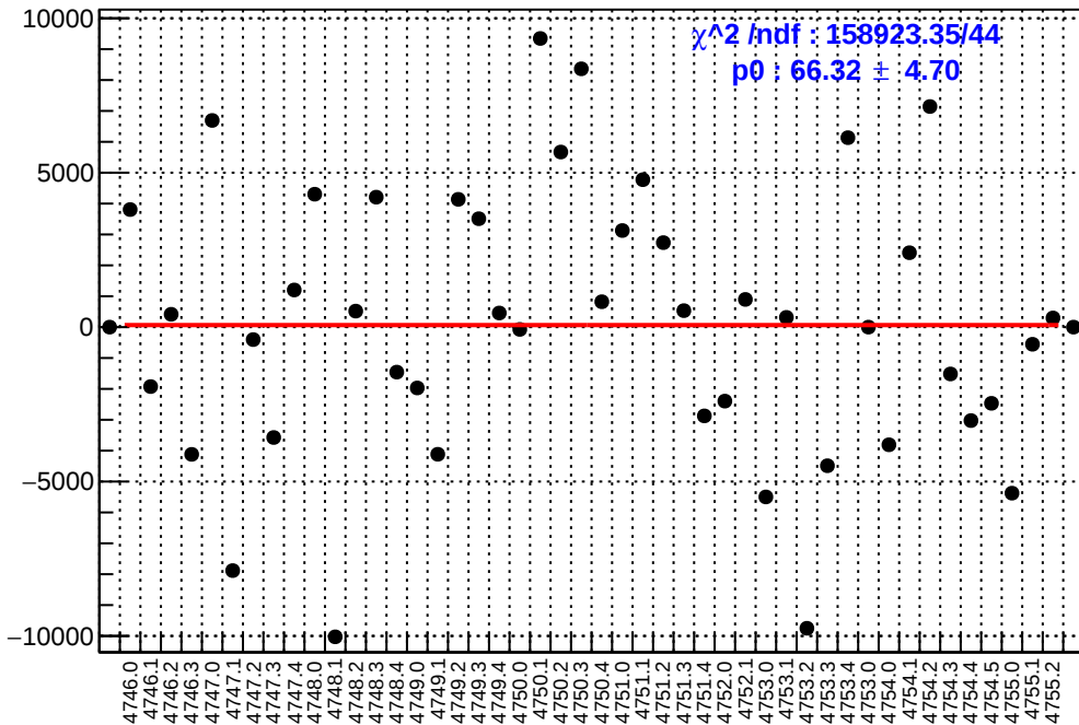
slug78: asym_atr1.mean/ppb-reg_asym_atr1.mean/ppb
