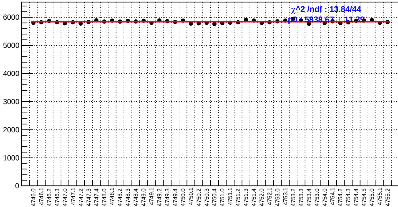
slug78: reg_asym_atr_avg.rms/ppm
