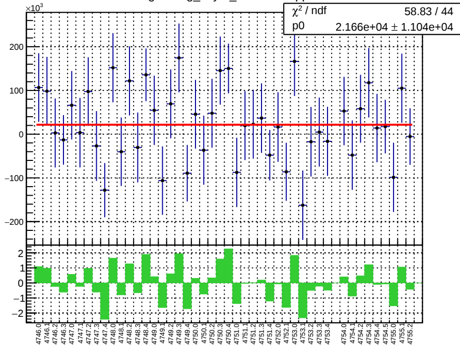
slug78: reg_asym_atr2.mean/ppb
