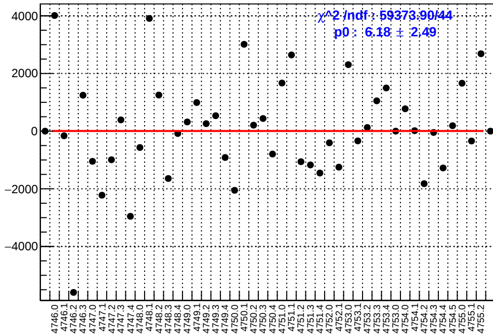
slug78: asym_us_avg.mean/ppb-reg_asym_us_avg.mean/ppb
