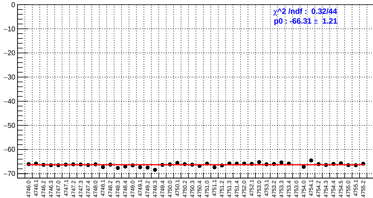
slug78: left_avg_bpm4eX/(ppb/nm)
