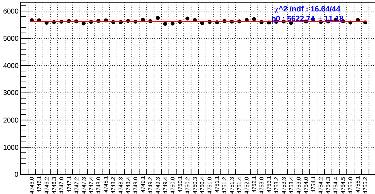
slug78: reg_asym_atl_avg.rms/ppm
