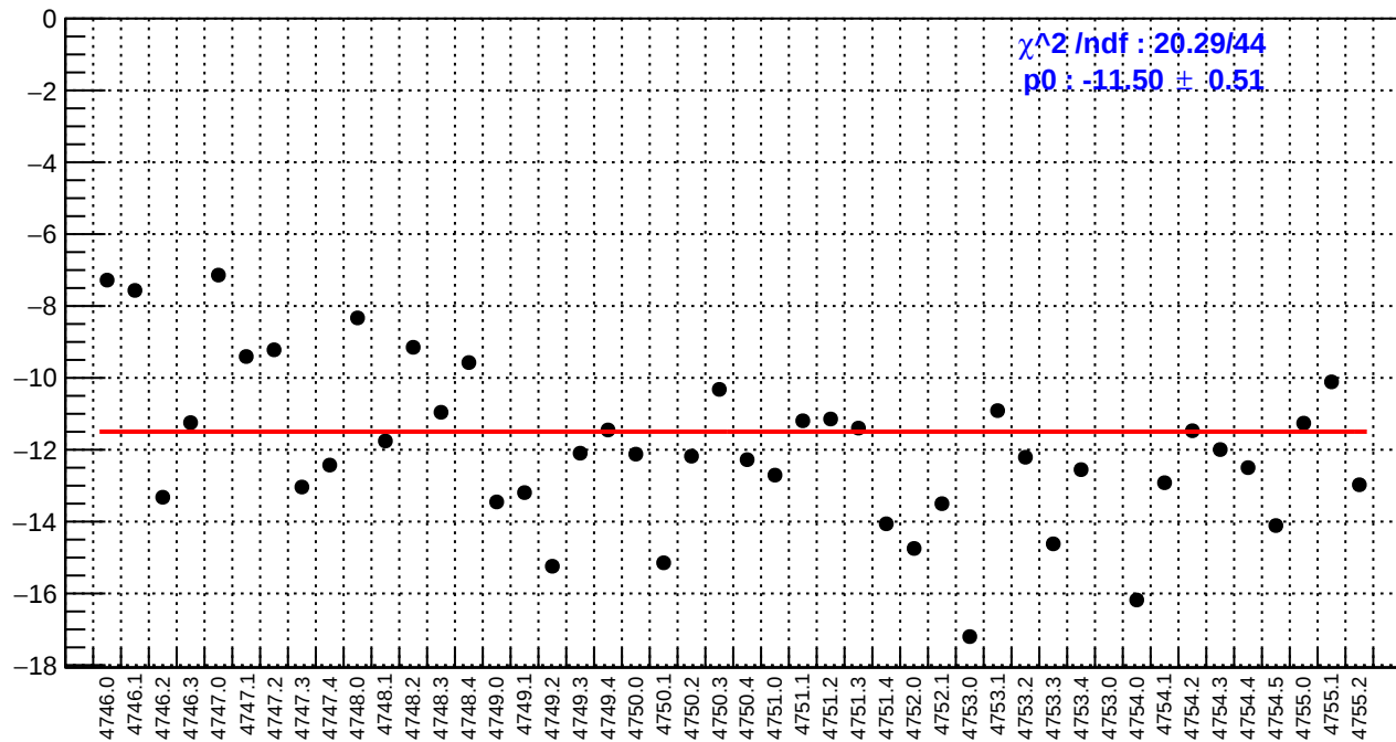
slug78: dsl_bpm4aY/(ppb/nm)
