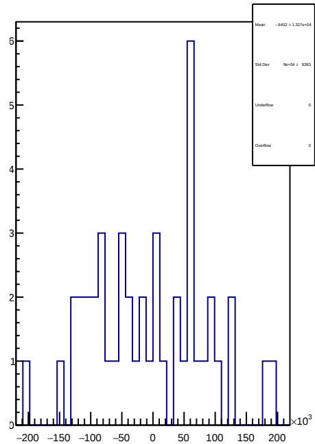
slug78: 1D Corr asym_sam3.mean/ppb-reg_asym_sam3.mean/ppb
