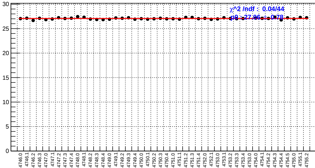
slug78: reg_asym_right_dd.rms/ppm
