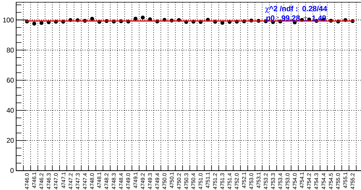
slug78: reg_asym_ds_avg.rms/ppm
