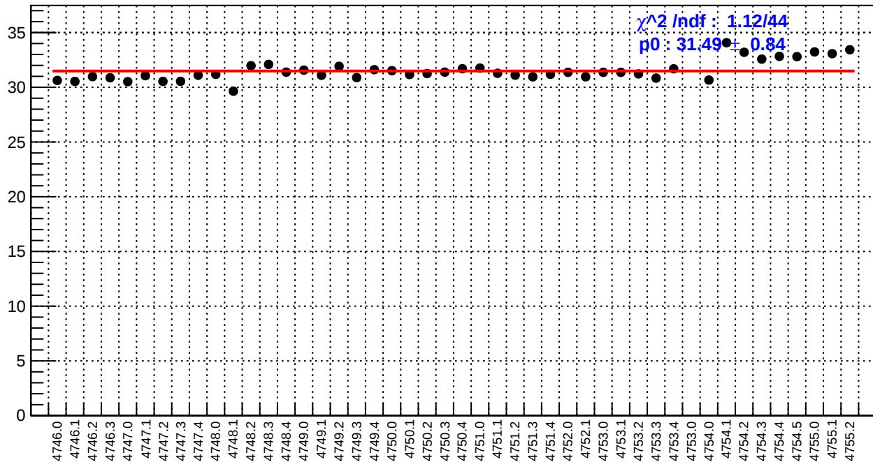
slug78: usr_bpm4eX/(ppb/nm)
