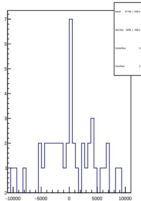
slug78: 1D Corr asym_atr1.mean/ppb-reg_asym_atr1.mean/ppb
