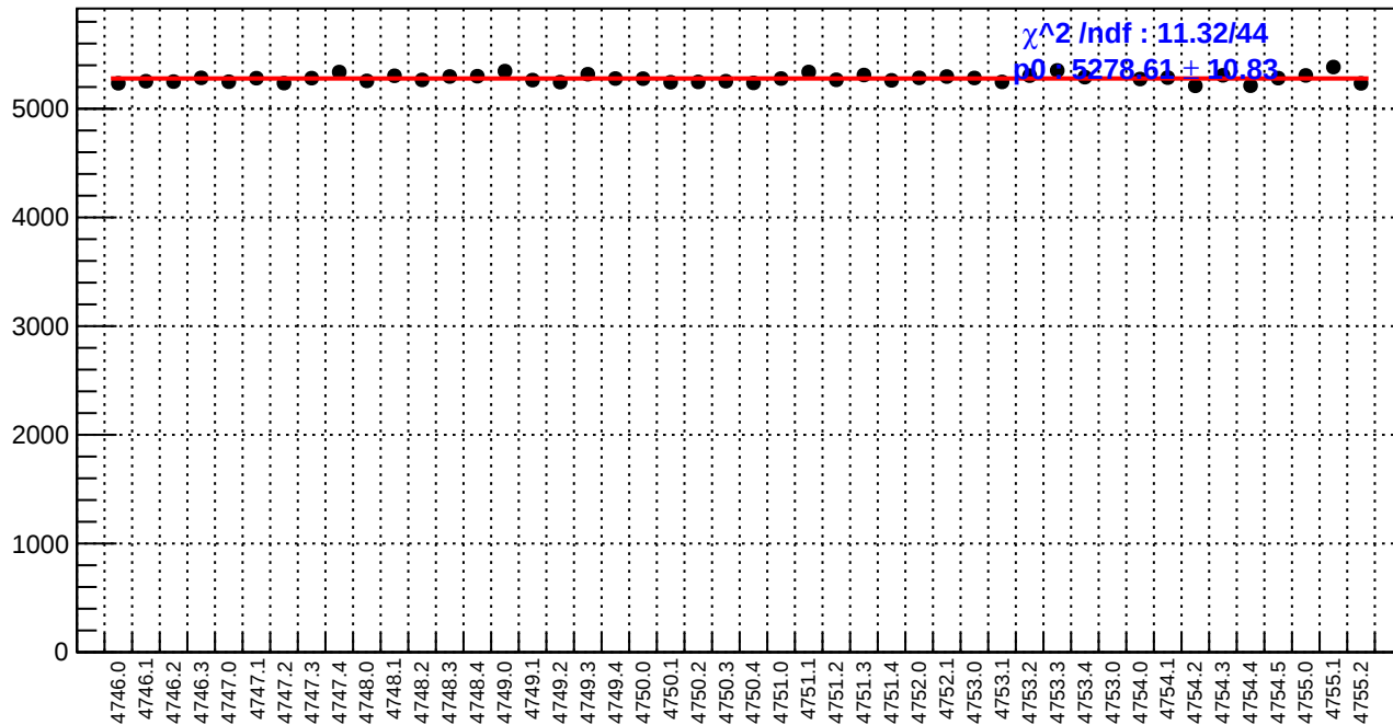
slug78: reg_asym_at2_avg.rms/ppm
