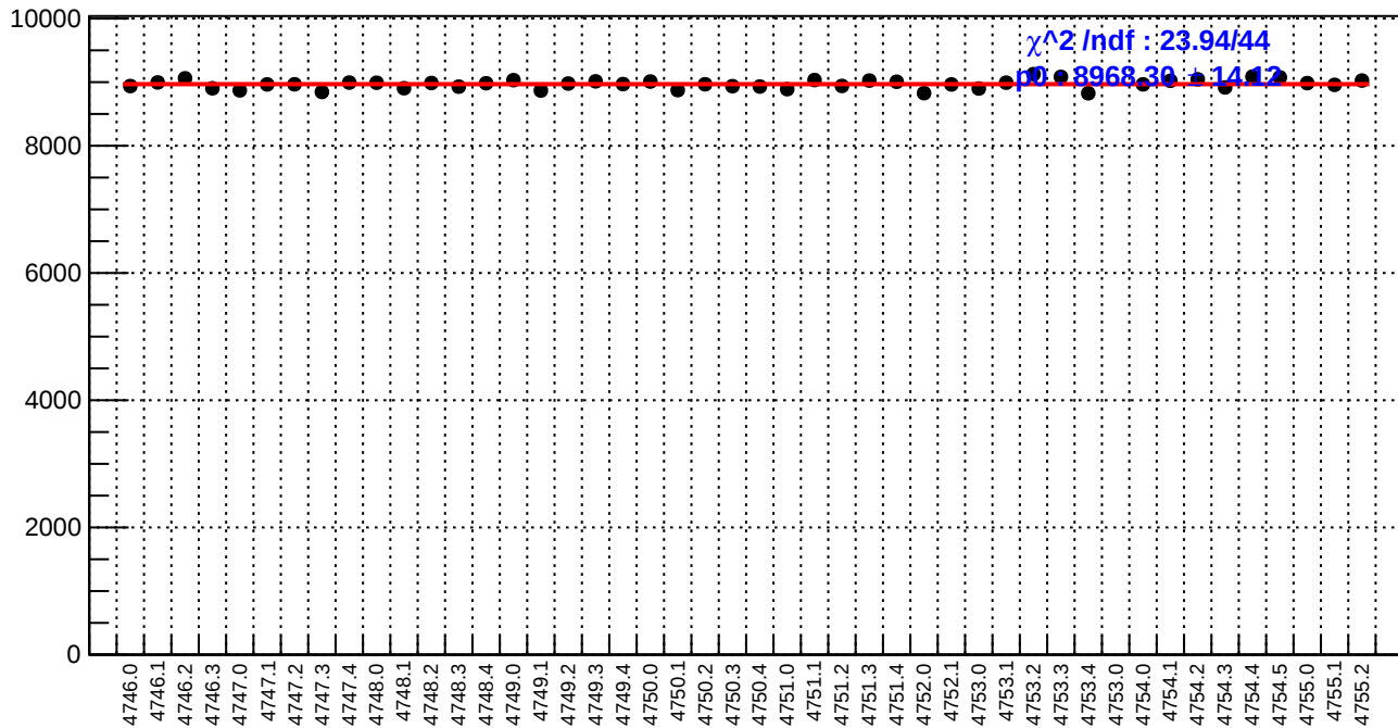
slug78: reg_asym_atr1.rms/ppm
