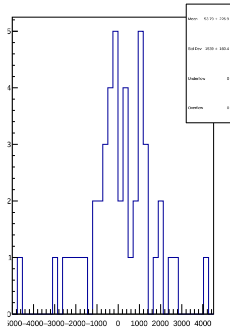
slug78: 1D Corr asym_at1_avg.mean/ppb-reg_asym_at1_avg.mean/ppb
