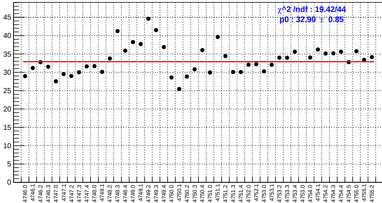
slug78: left_avg_bpm4aX/(ppb/nm)
