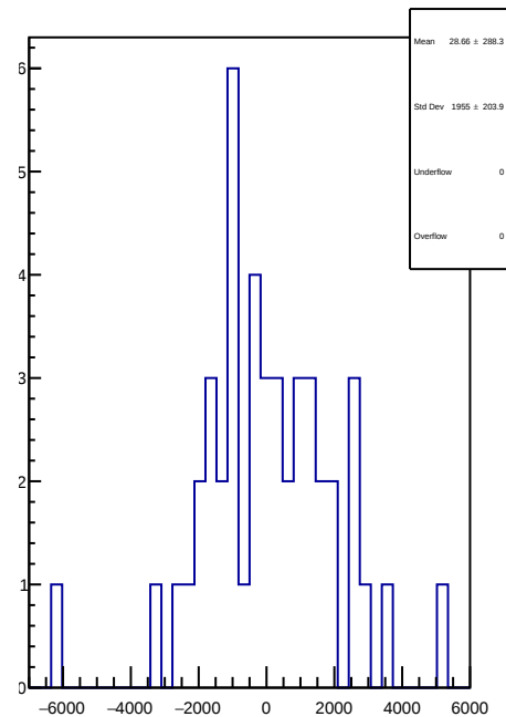
slug78: 1D Corr asym_ds_avg.mean/ppb-reg_asym_ds_avg.mean/ppb
