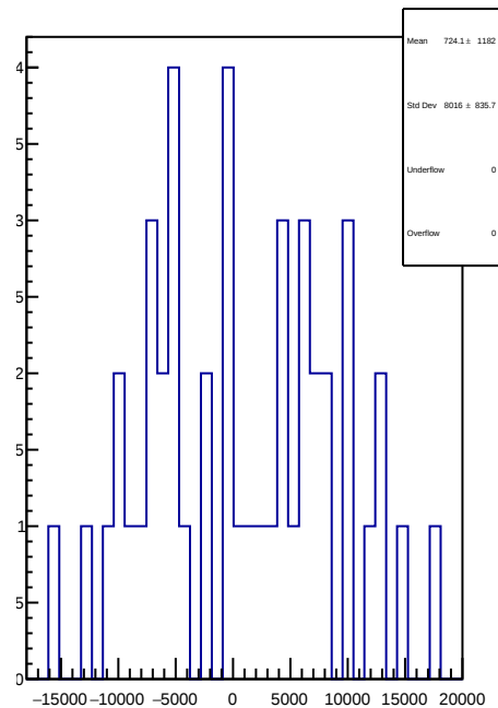
slug78: 1D Corr asym_atr2.mean/ppb-reg_asym_atr2.mean/ppb
