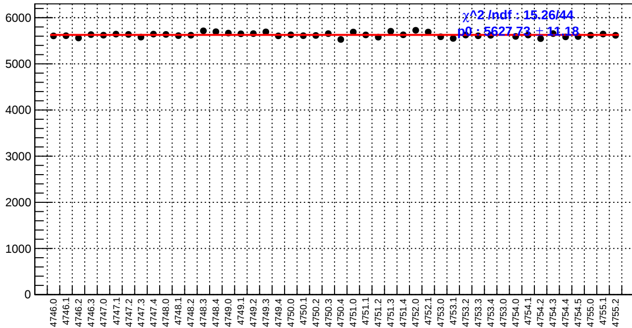
slug78: reg_asym_atl1r2_avg.rms/ppm
