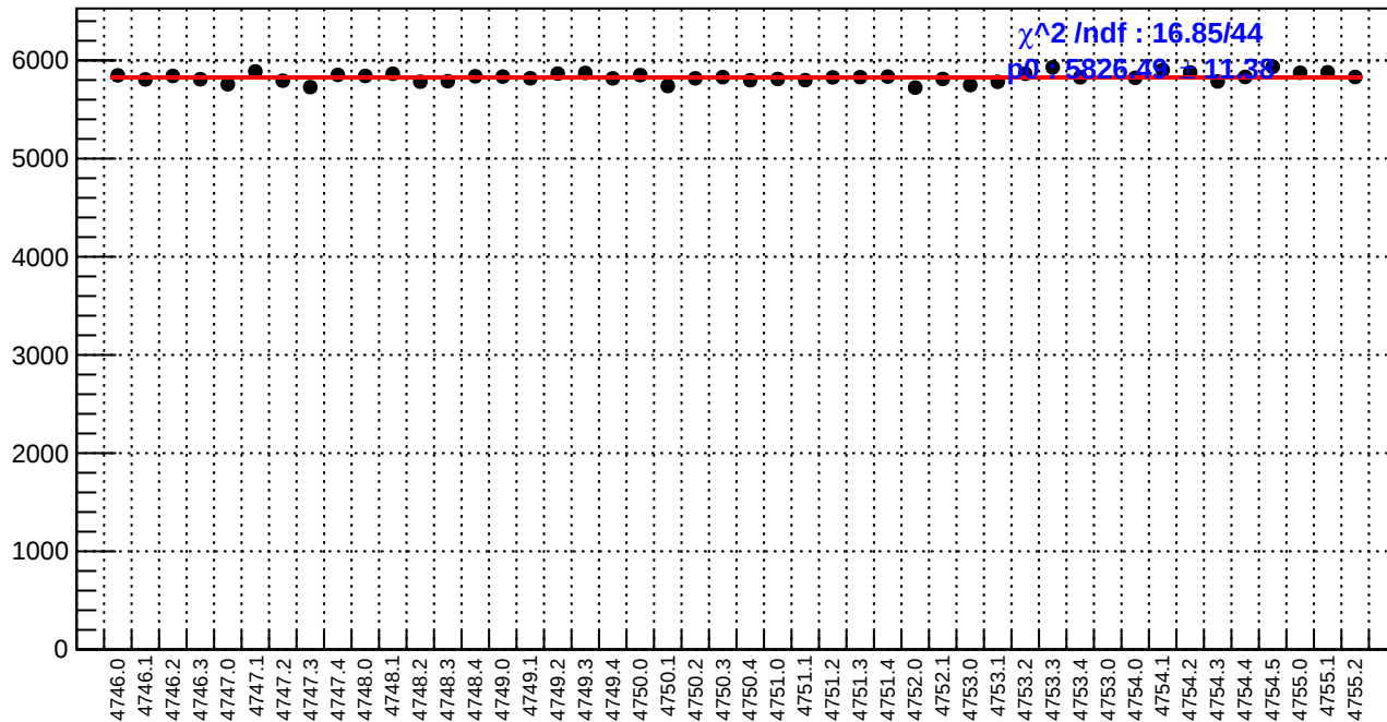
slug78: reg_asym_atr1l2_avg.rms/ppm
