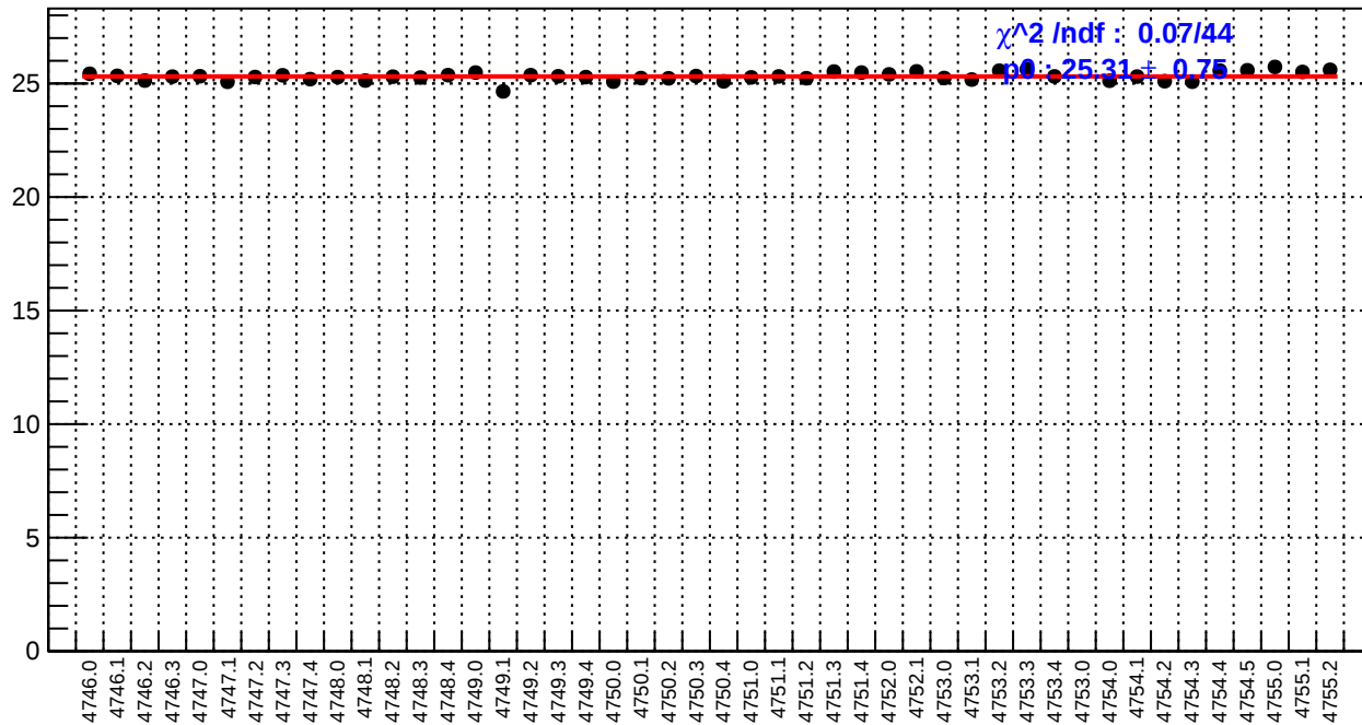
slug78: reg_asym_left_dd.rms/ppm
