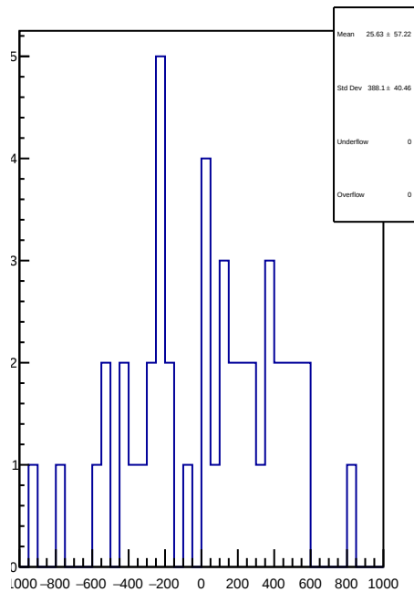
slug78: 1D Corr asym_right_dd.mean/ppb-reg_asym_right_dd.mean/ppb
