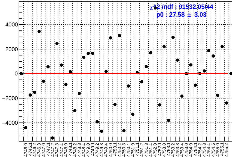
slug78: asym_atr_dd.mean/ppb-reg_asym_atr_dd.mean/ppb
