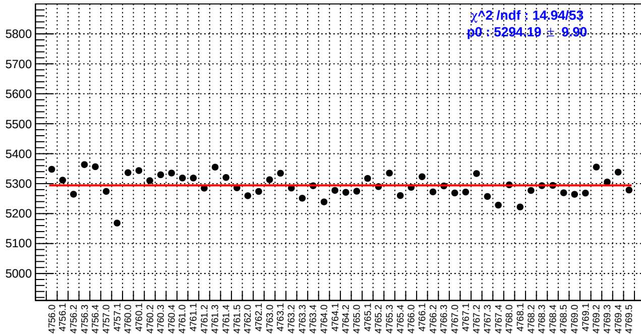
slug79: reg_asym_at2_dd.rms/ppm
