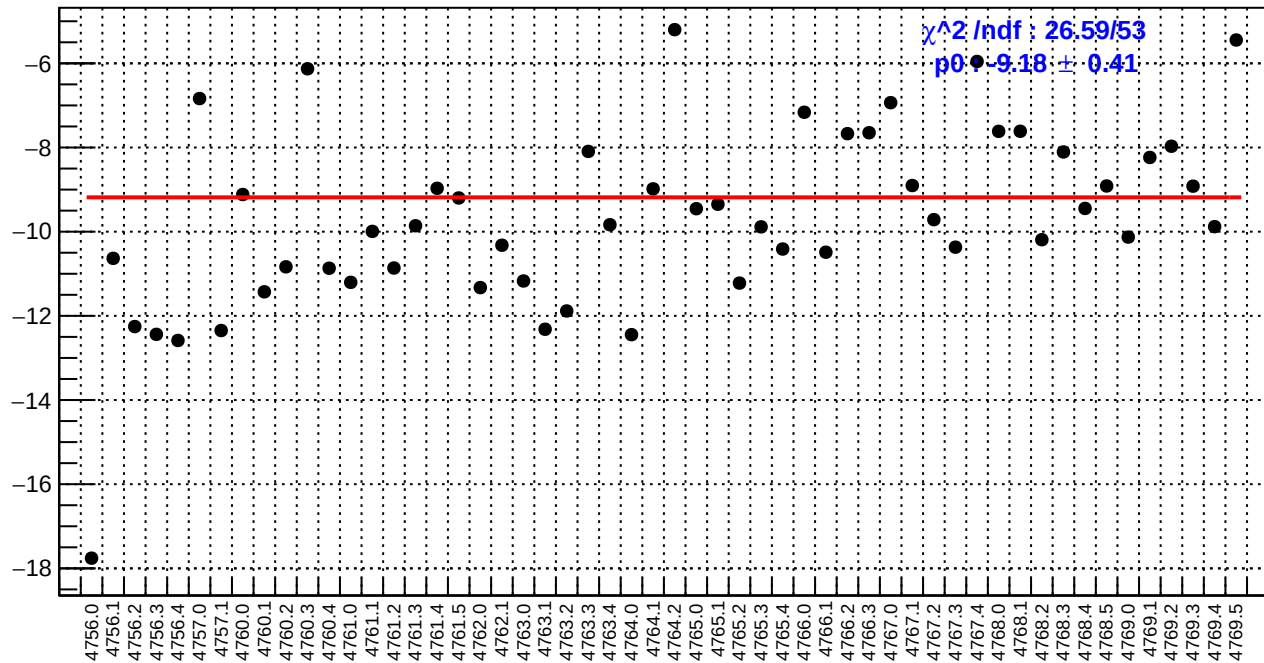
slug79: dsl_bpm4aY/(ppb/nm)
