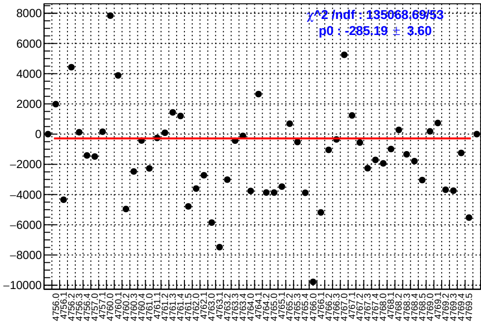
slug79: asym_atl_dd.mean/ppb-reg_asym_atl_dd.mean/ppb
