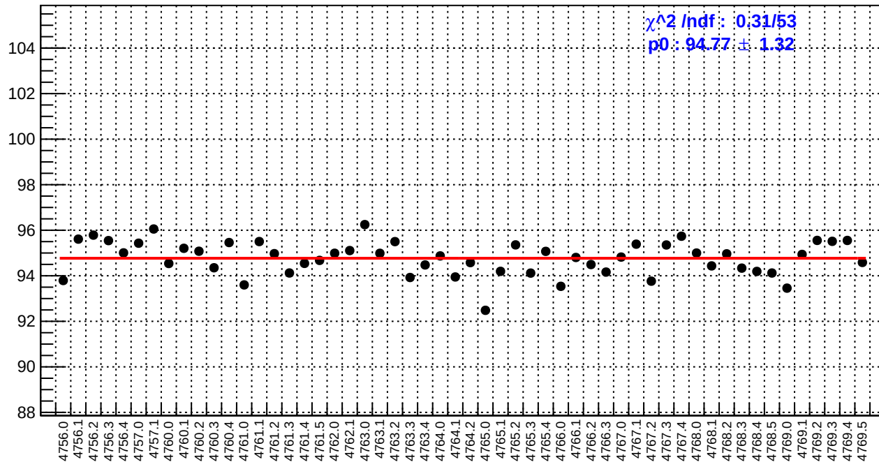
slug79: reg_asym_ds_dd.rms/ppm
