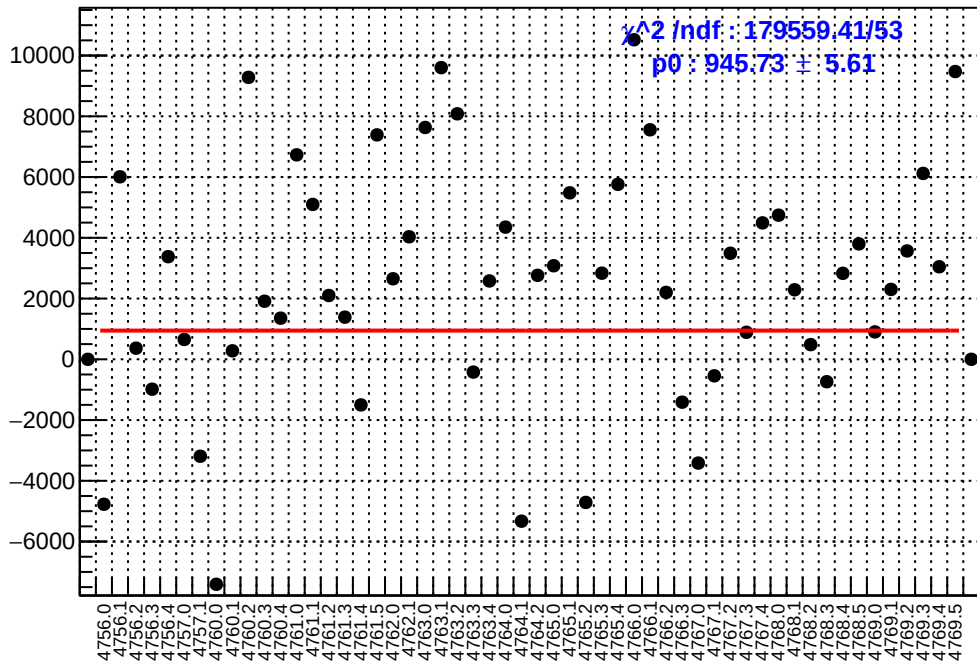
slug79: asym_ds_dd.mean/ppb-reg_asym_ds_dd.mean/ppb
