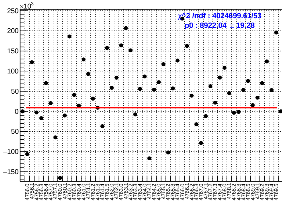
slug79: asym_sam3.mean/ppb-reg_asym_sam3.mean/ppb
