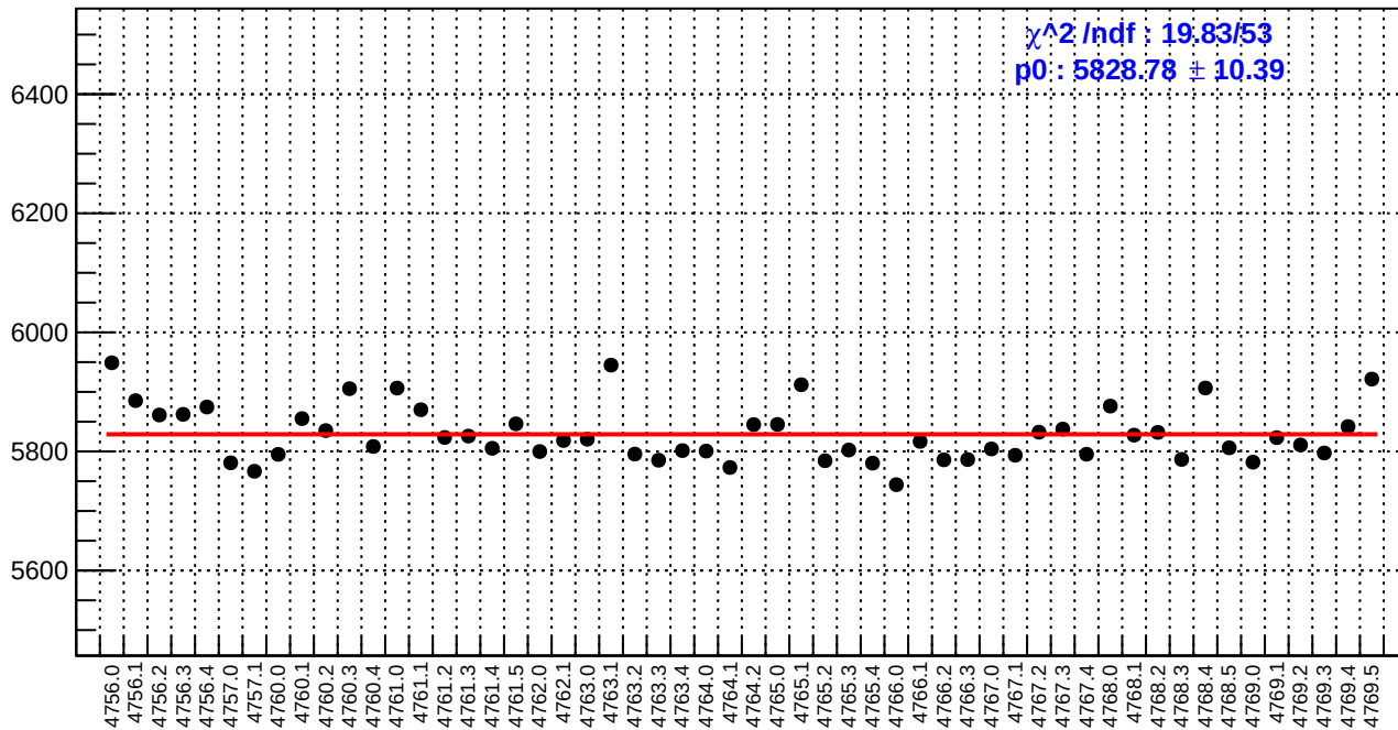
slug79: reg_asym_atr1l2_dd.rms/ppm
