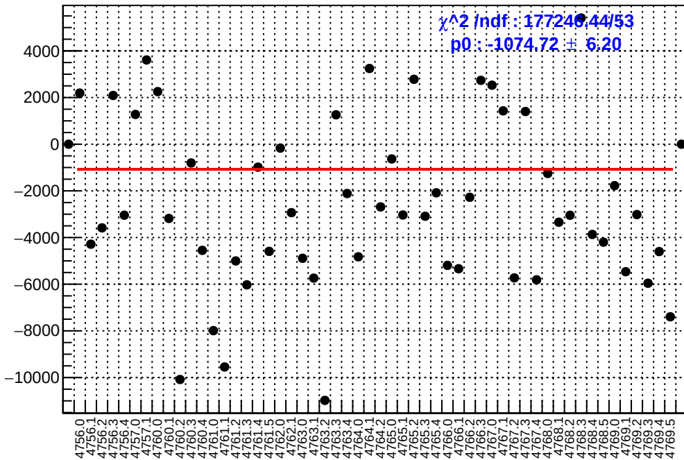
slug79: asym_dsr.mean/ppb-reg_asym_dsr.mean/ppb
