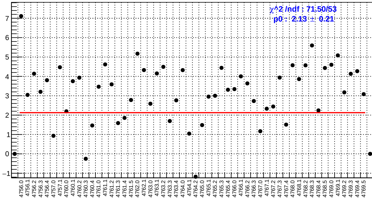
slug79: ds_avg_bpm4eY/(ppb/nm)
