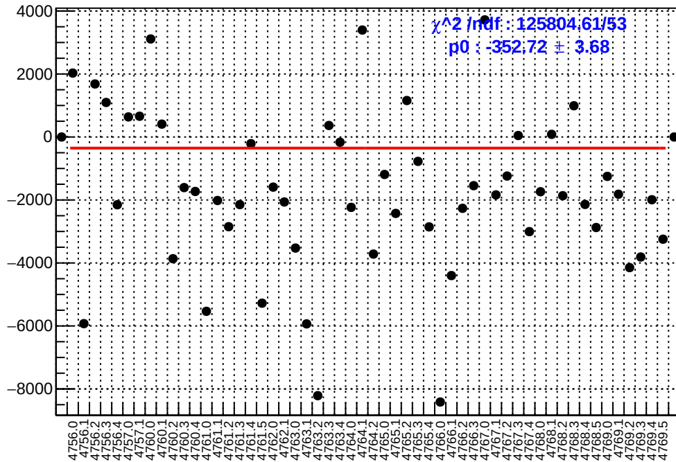
slug79: asym_atl1r2_avg.mean/ppb-reg_asym_atl1r2_avg.mean/ppb
