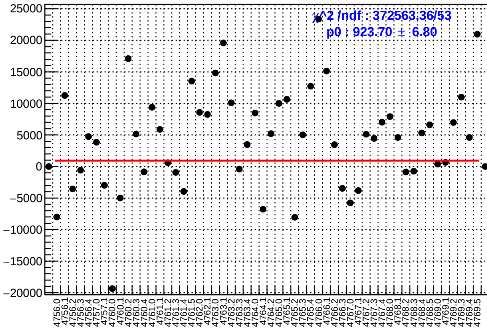
slug79: asym_atl2.mean/ppb-reg_asym_atl2.mean/ppb
