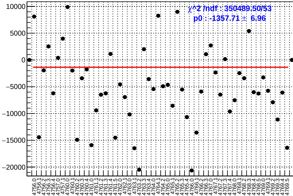
slug79: asym_atr2.mean/ppb-reg_asym_atr2.mean/ppb
