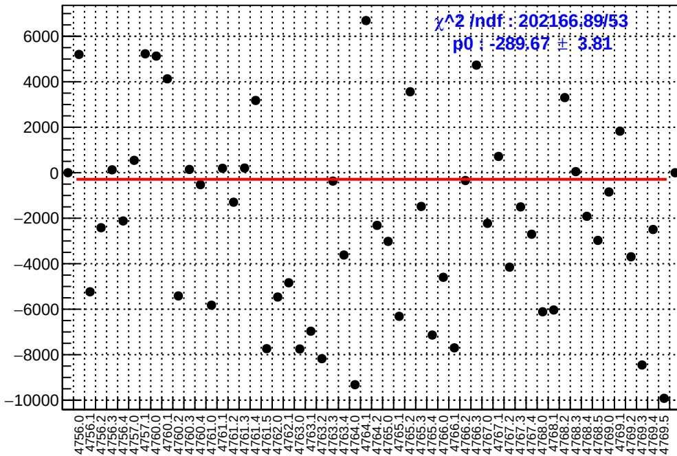
slug79: asym_atr1.mean/ppb-reg_asym_atr1.mean/ppb
