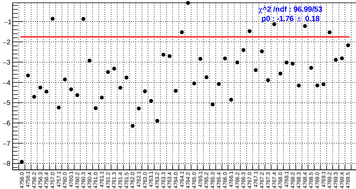
slug79: ds_avg_bpm4aY/(ppb/nm)
