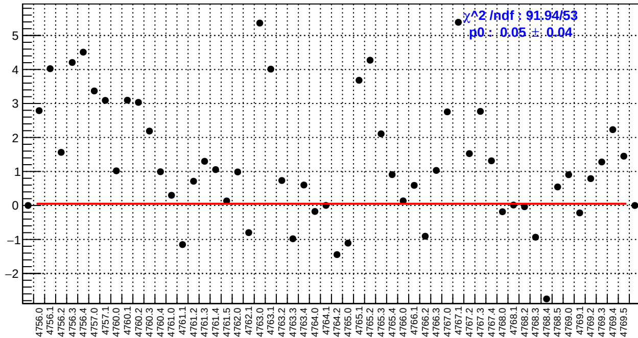
slug79: us_avg_bpm4aX/(ppb/nm)
