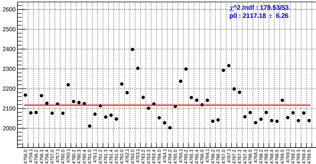
slug79: diff_bpm4eY.rms/nm
