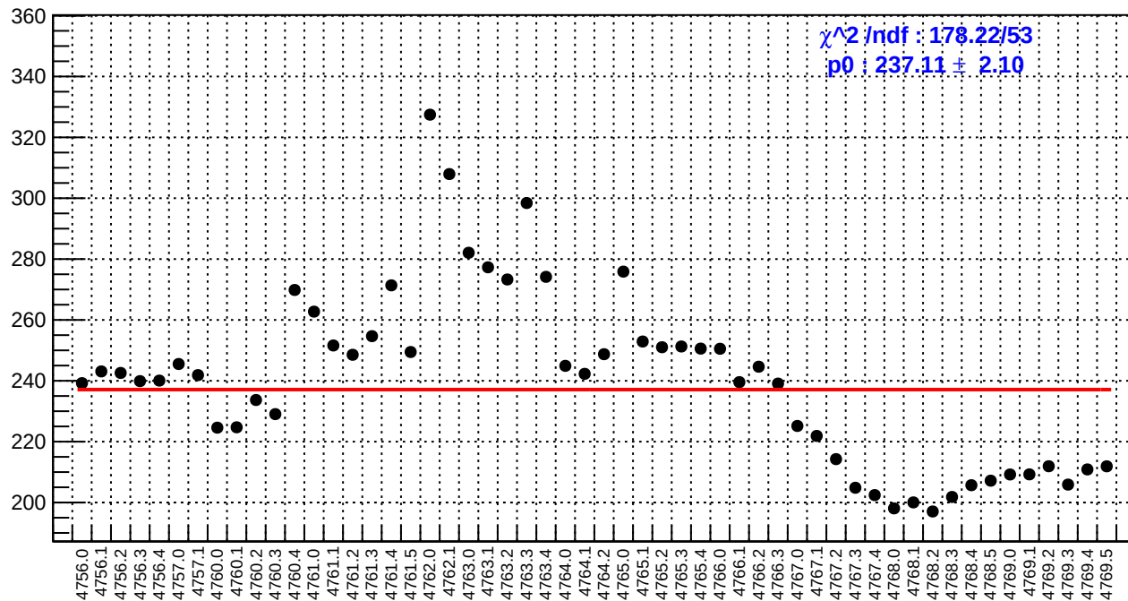
slug79: asym_bcm_an_ds.rms/ppm
