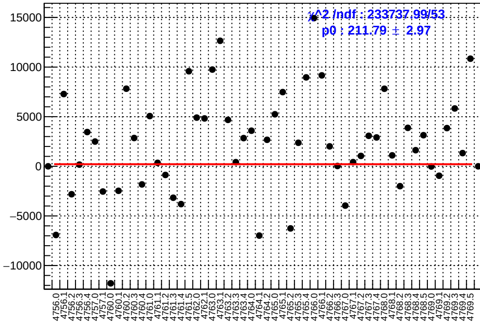
slug79: asym_usl.mean/ppb-reg_asym_usl.mean/ppb
