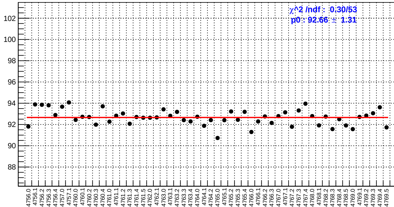
slug79: reg_asym_us_dd.rms/ppm
