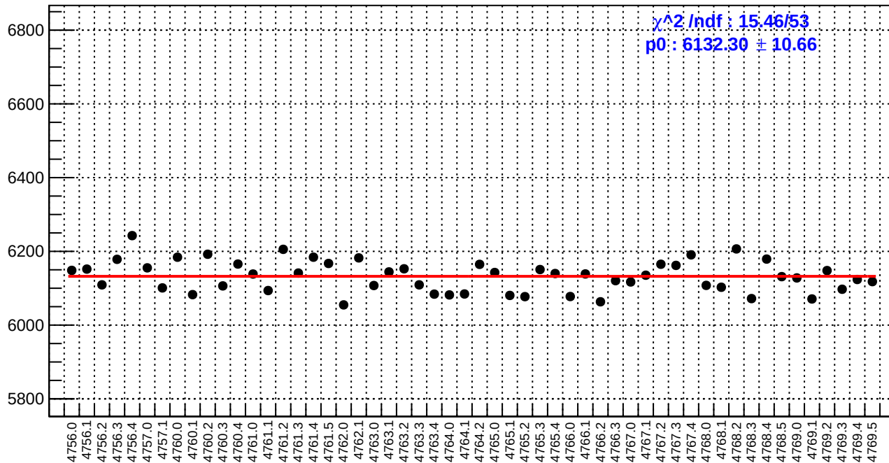
slug79: reg_asym_at1_dd.rms/ppm
