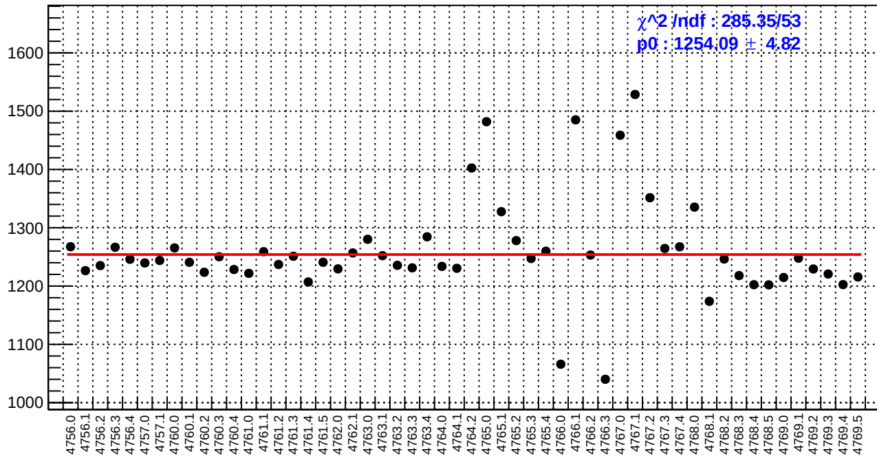
slug79: reg_asym_sam4.rms/ppm
