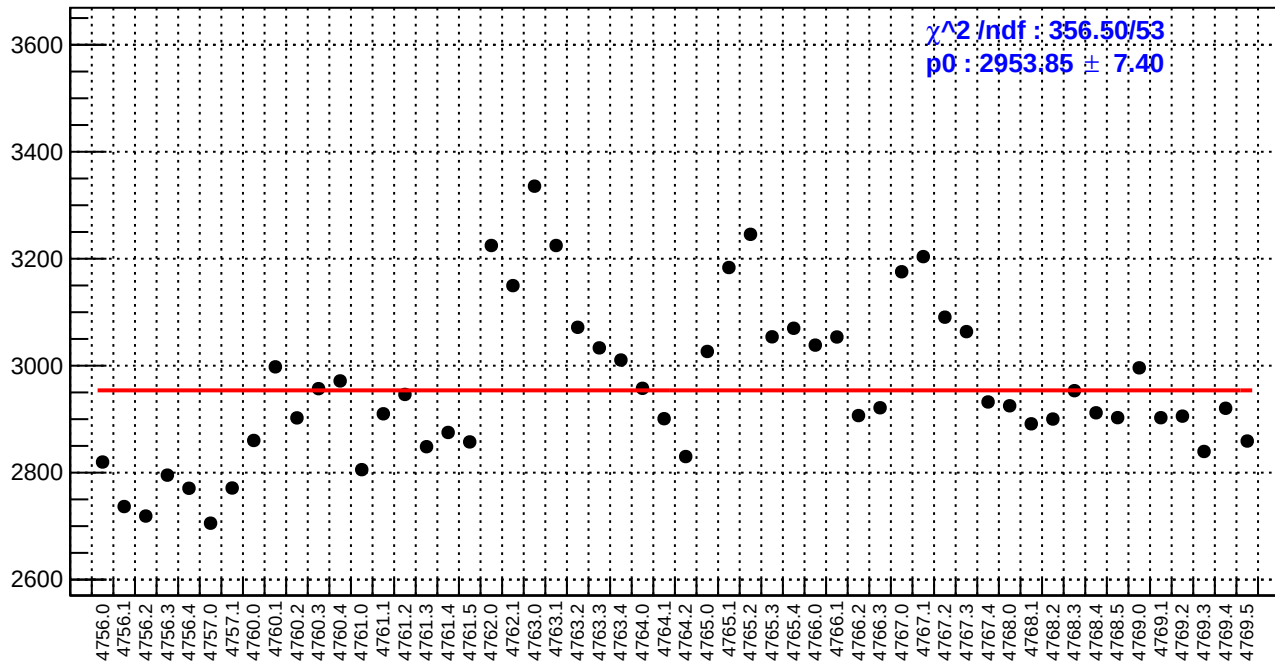
slug79: diff_bpm4aY.rms/nm
