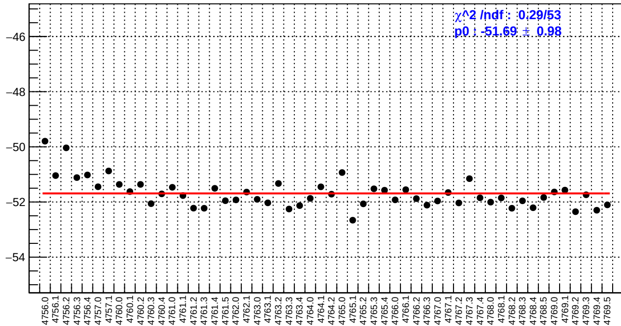
slug79: ds_avg_bpm12X/(ppb/nm)
