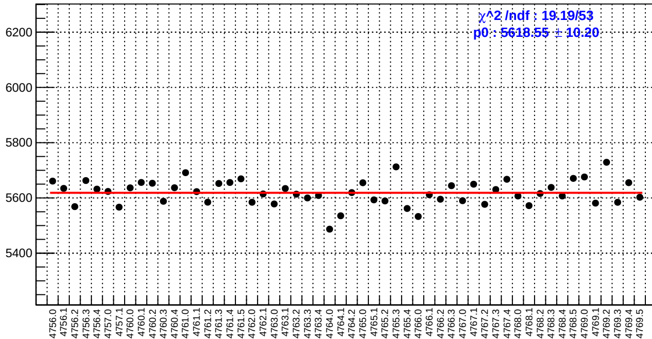
slug79: reg_asym_atl_dd.rms/ppm
