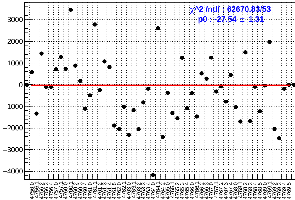
slug79: asym_at1_avg.mean/ppb-reg_asym_at1_avg.mean/ppb
