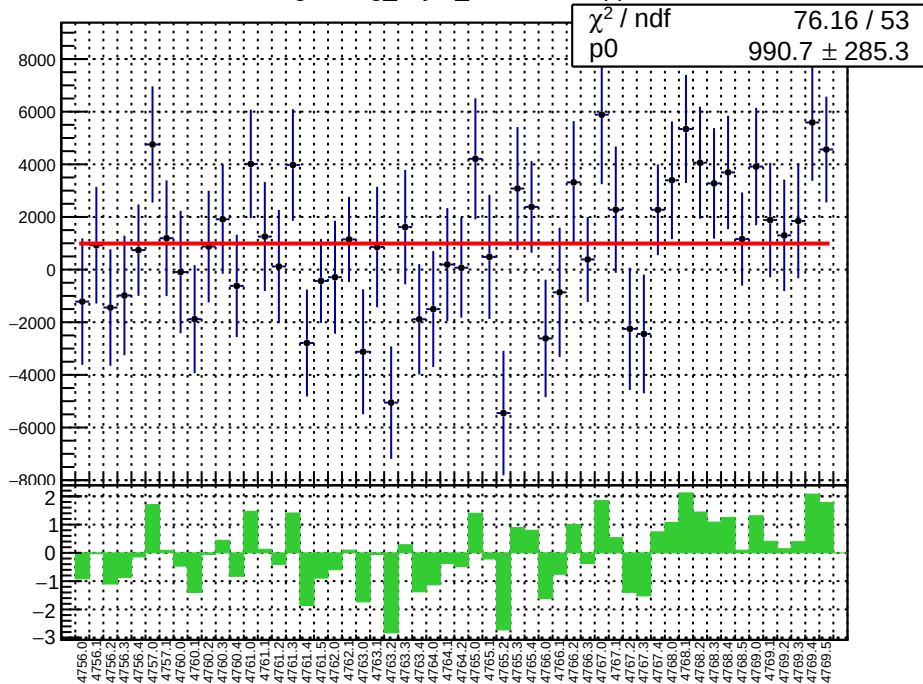
slug79: reg_asym_sam5.mean/ppb
