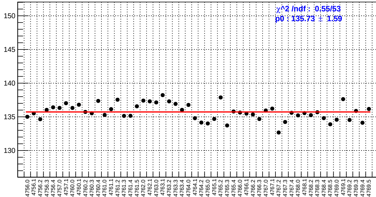
slug79: reg_asym_left_avg.rms/ppm
