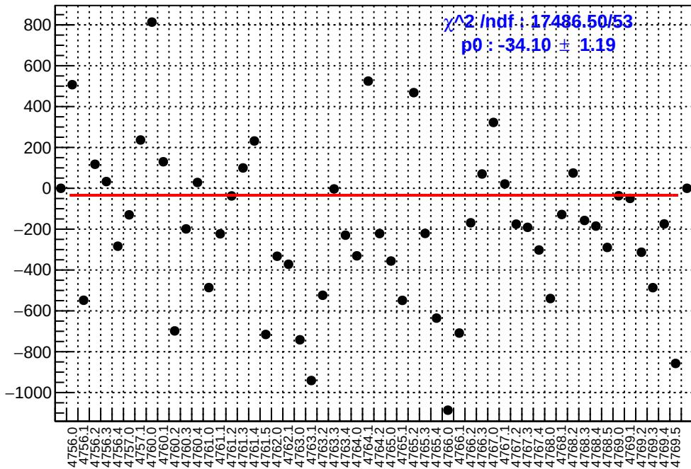
slug79: asym_right_dd.mean/ppb-reg_asym_right_dd.mean/ppb
