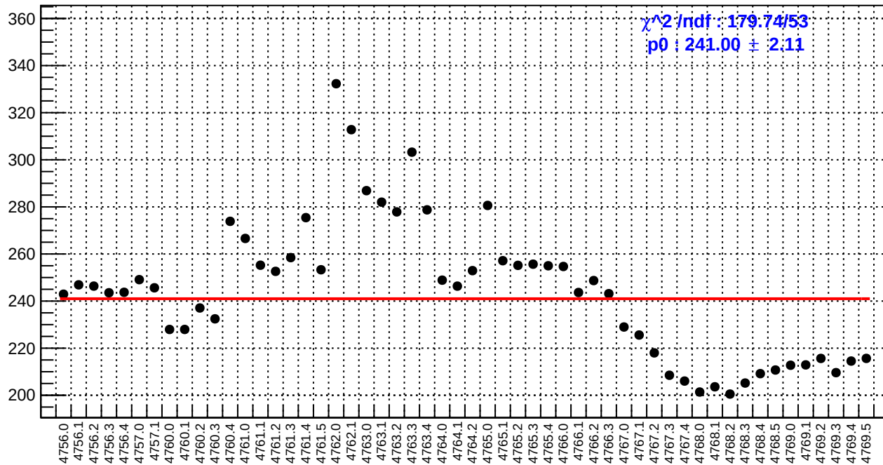
slug79: asym_bcm_an_ds3.rms/ppm
