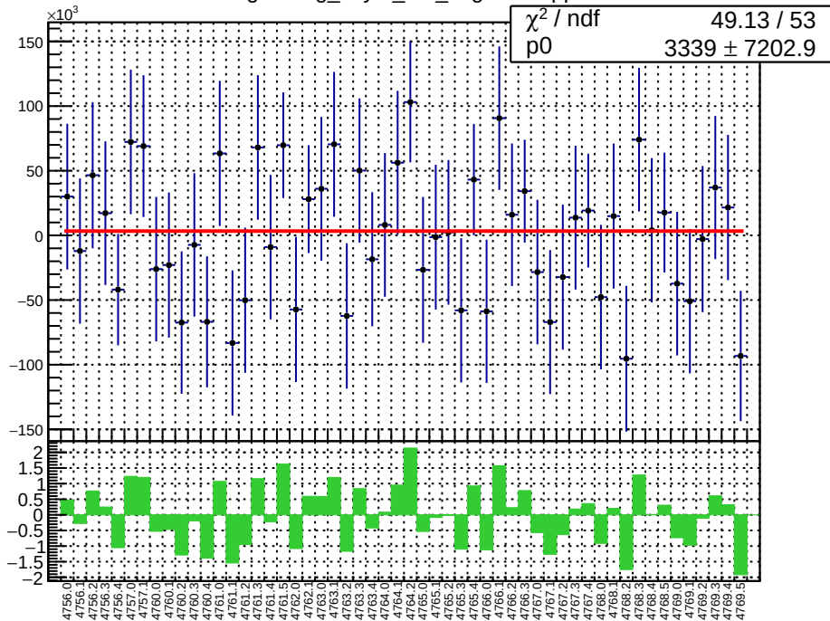
slug79: reg_asym_at2_avg.mean/ppb
