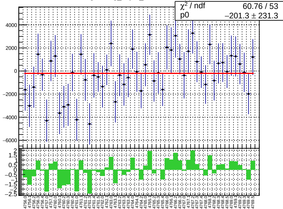
slug79: reg_asym_sam1.mean/ppb
