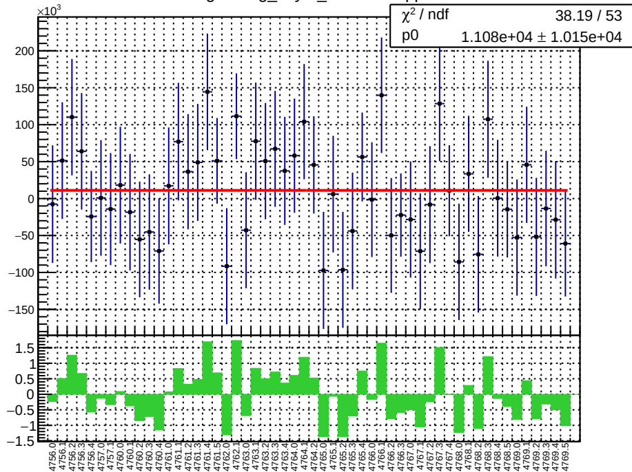
slug79: reg_asym_atl2.mean/ppb
