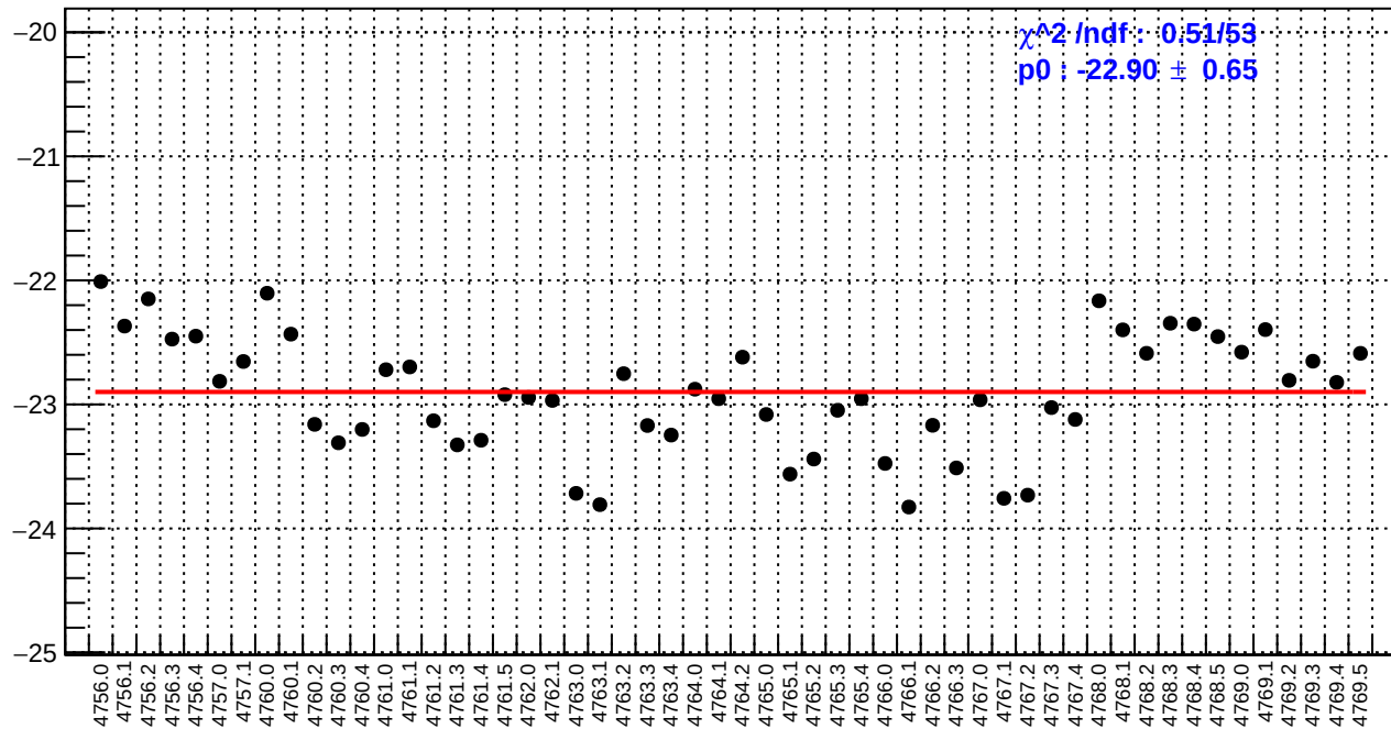
slug79: ds_avg_bpm4eX/(ppb/nm)
