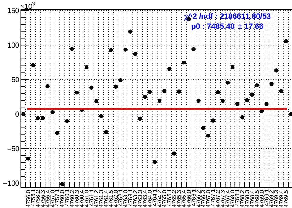
slug79: asym_sam2.mean/ppb-reg_asym_sam2.mean/ppb
