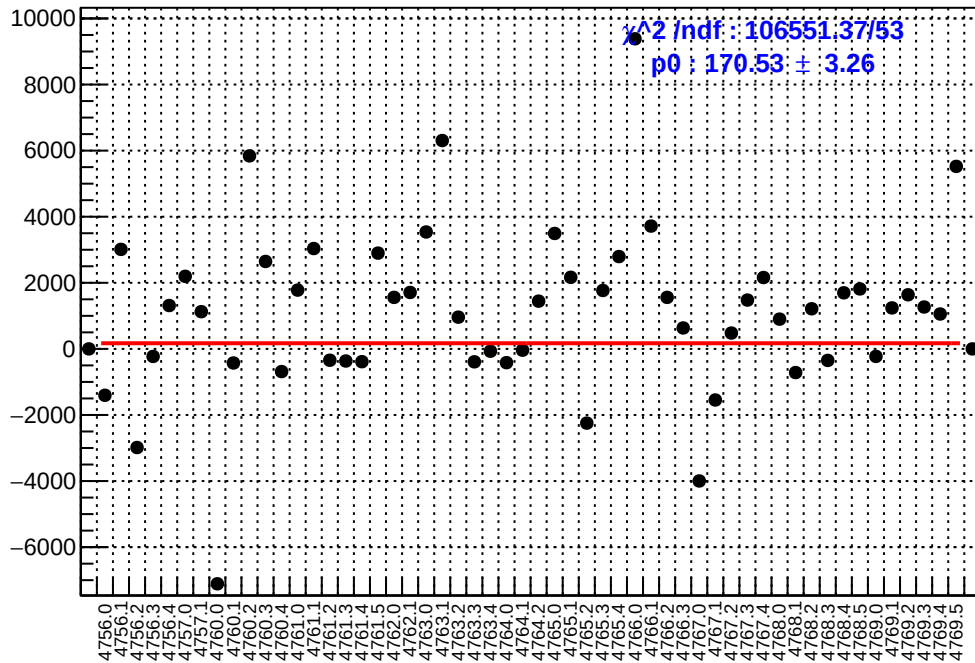
slug79: asym_atr1l2_avg.mean/ppb-reg_asym_atr1l2_avg.mean/ppb
