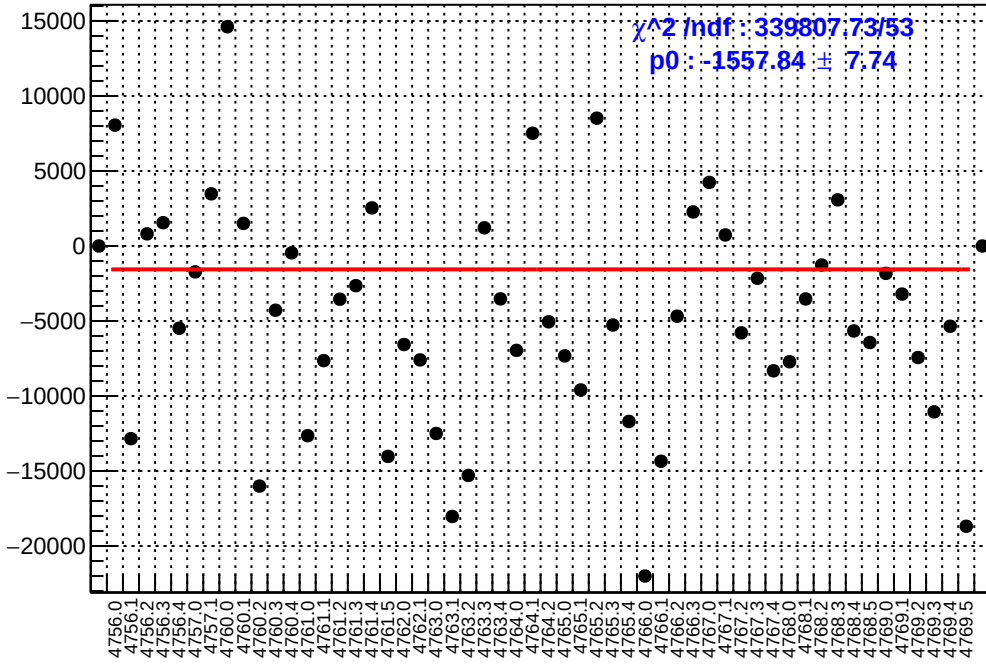
slug79: asym_at2_dd.mean/ppb-reg_asym_at2_dd.mean/ppb
