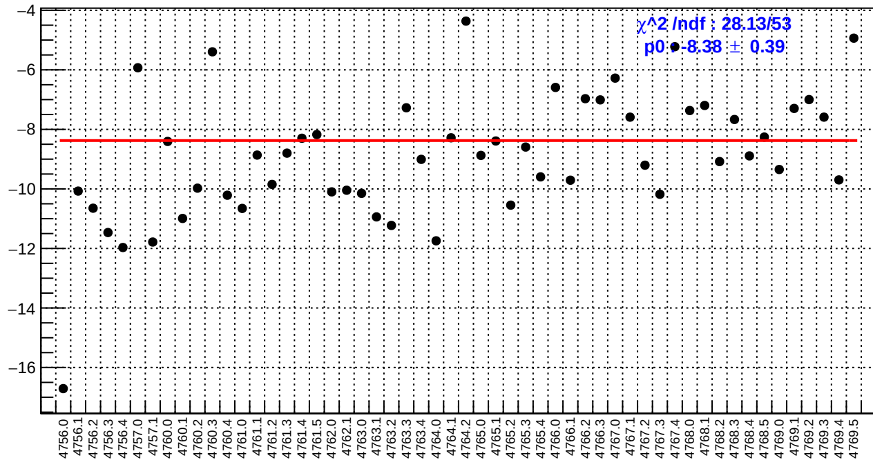
slug79: left_avg_bpm4aY/(ppb/nm)
