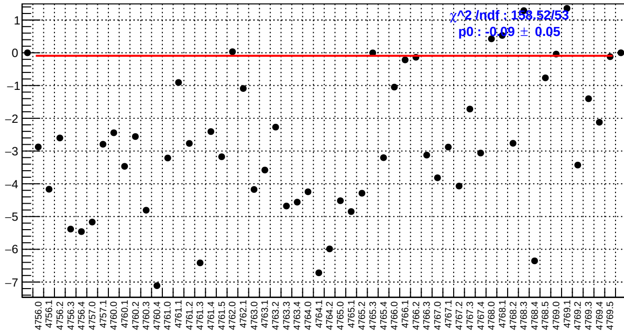
slug79: right_avg_bpm4eY/(ppb/nm)
