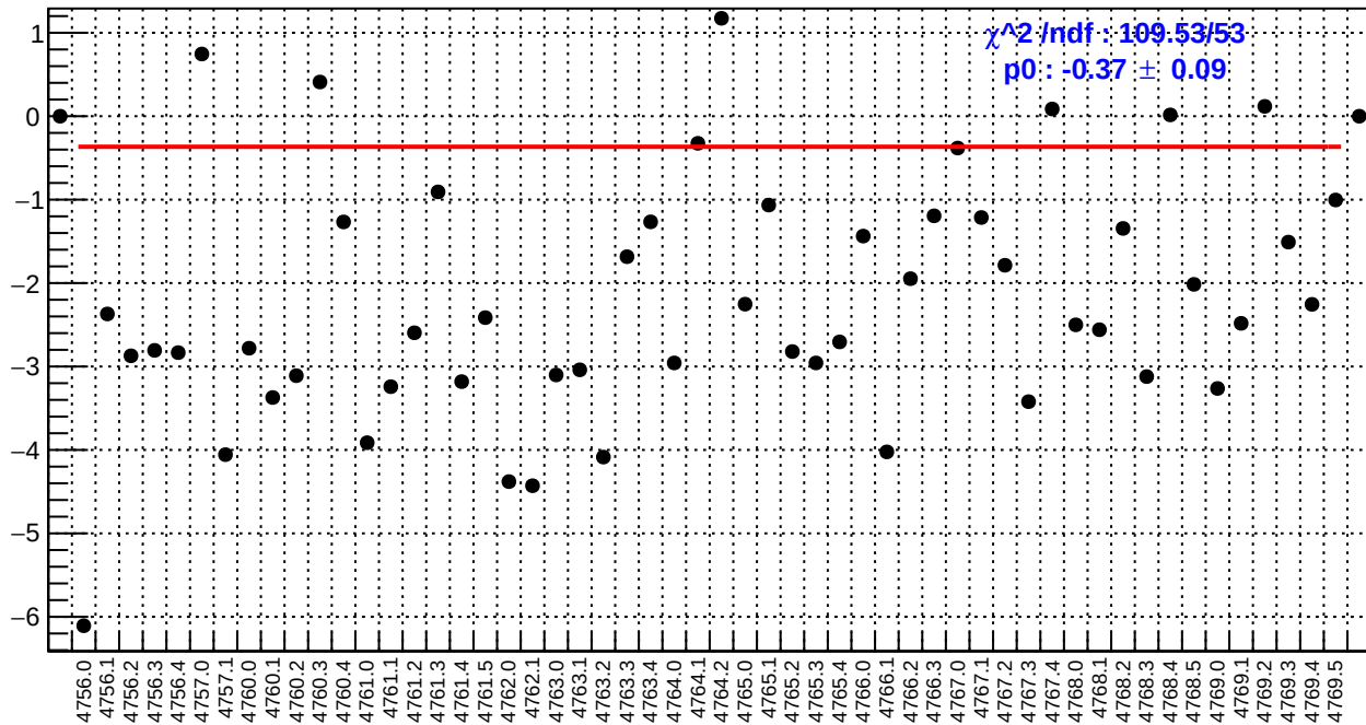
slug79: us_avg_bpm4aY/(ppb/nm)
