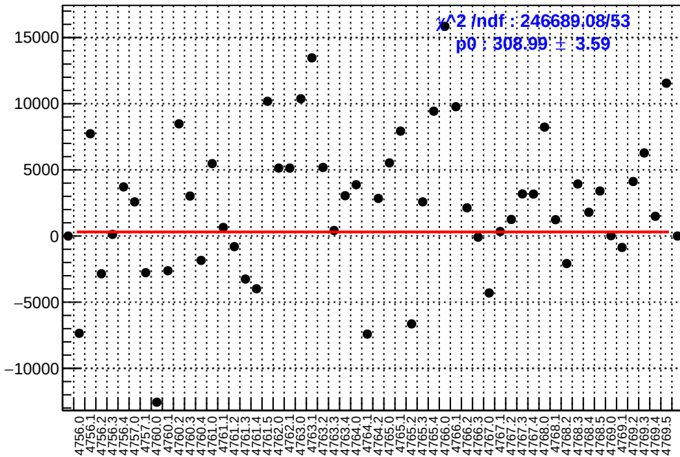
slug79: asym_dsl.mean/ppb-reg_asym_dsl.mean/ppb
