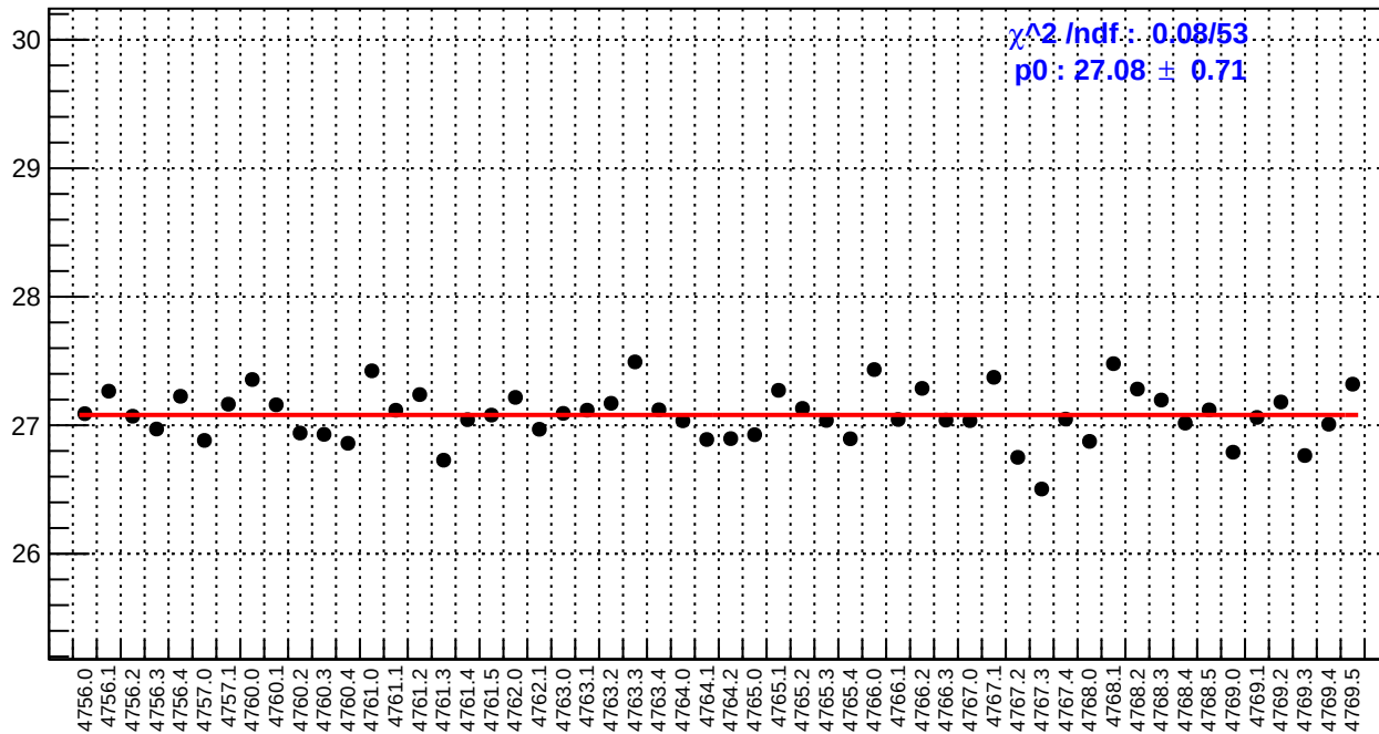
slug79: reg_asym_right_dd.rms/ppm
