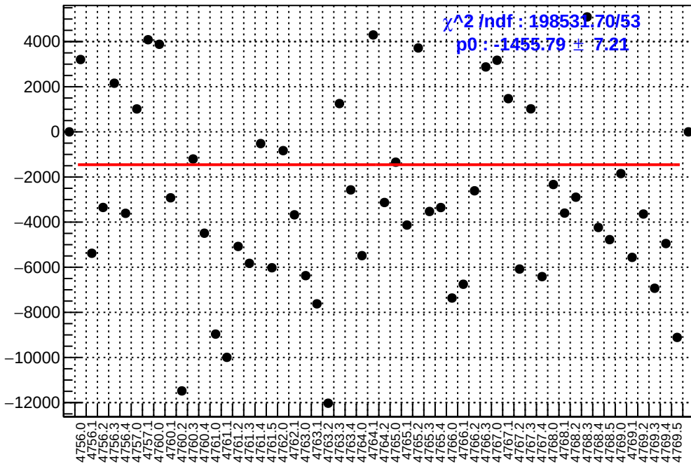
slug79: asym_usr.mean/ppb-reg_asym_usr.mean/ppb
