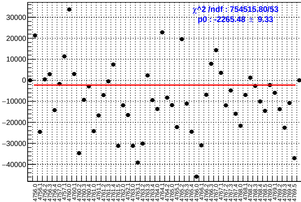
slug79: asym_sam7.mean/ppb-reg_asym_sam7.mean/ppb
