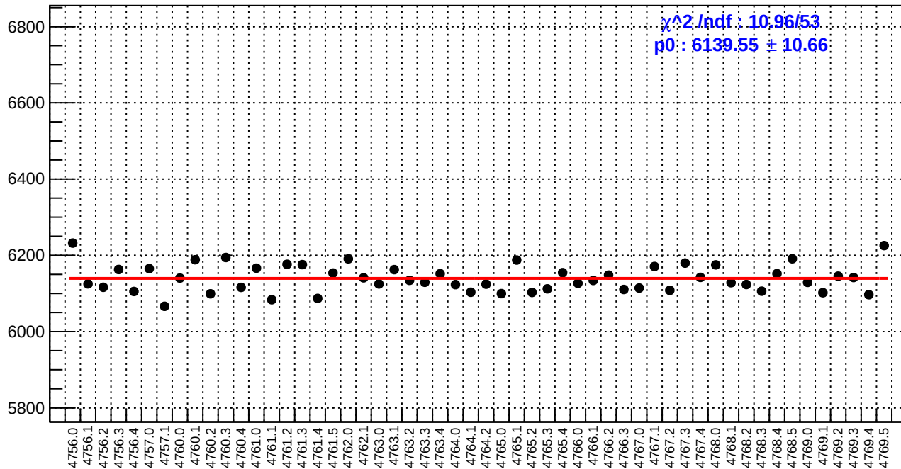
slug79: reg_asym_at1_avg.rms/ppm
