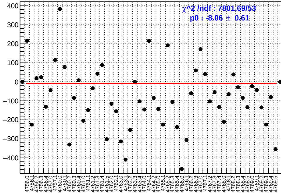
slug79: asym_left_dd.mean/ppb-reg_asym_left_dd.mean/ppb
