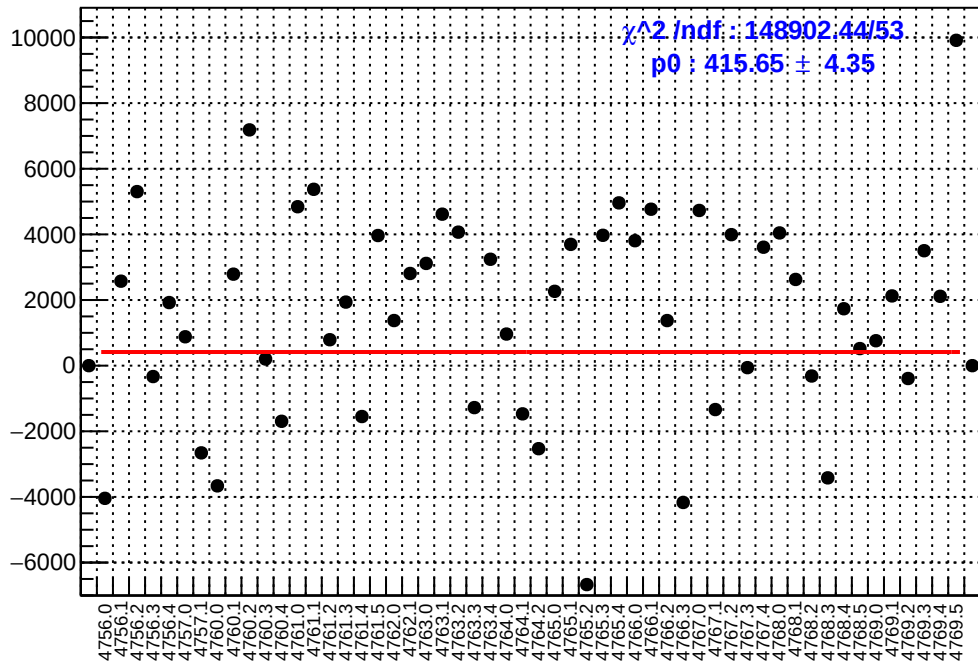
slug79: asym_atl1.mean/ppb-reg_asym_atl1.mean/ppb
