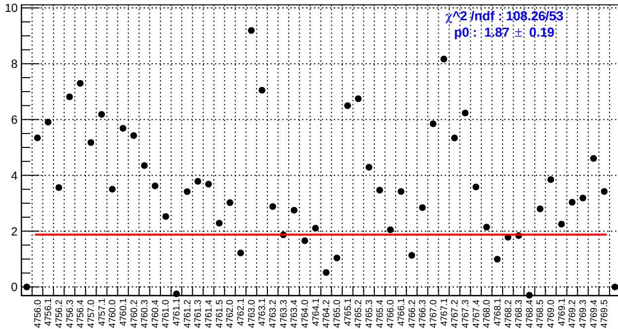
slug79: ds_avg_bpm4aX/(ppb/nm)
