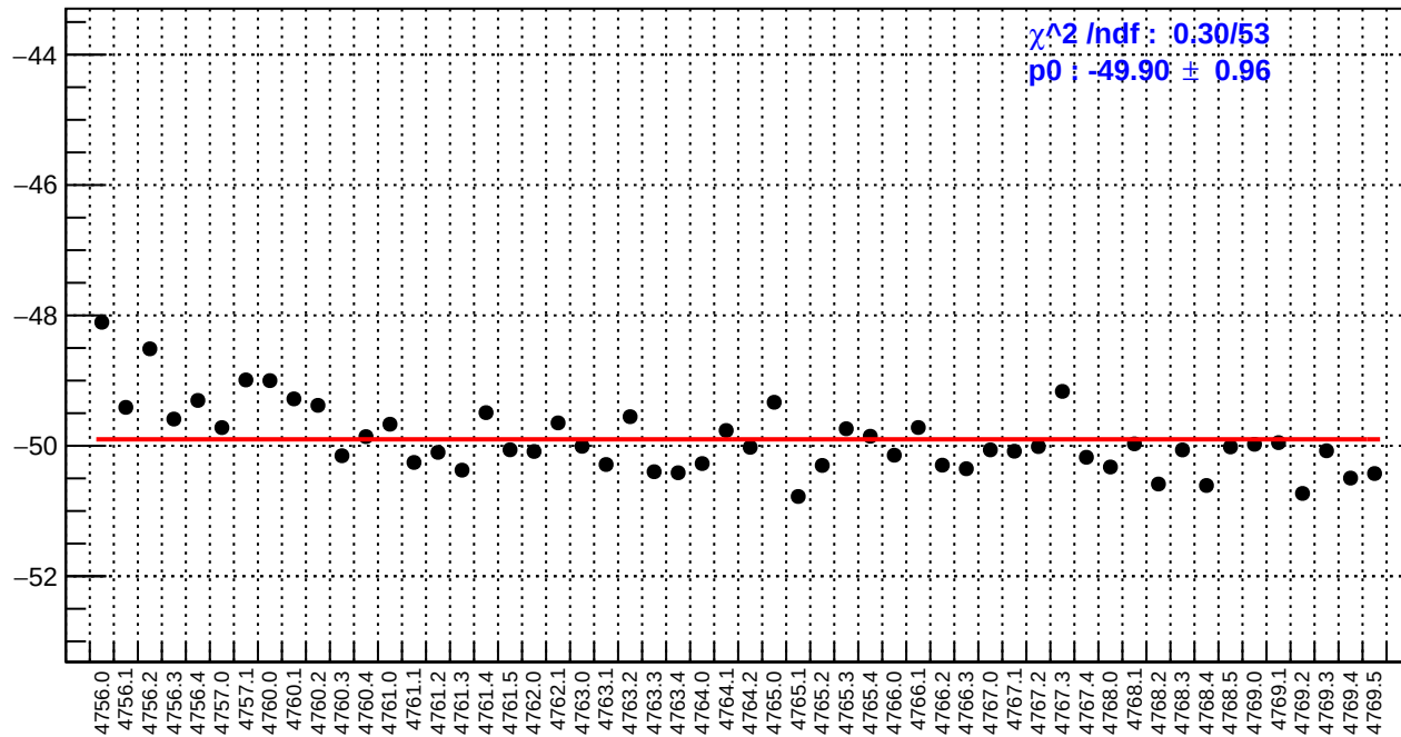
slug79: us_avg_bpm12X/(ppb/nm)
