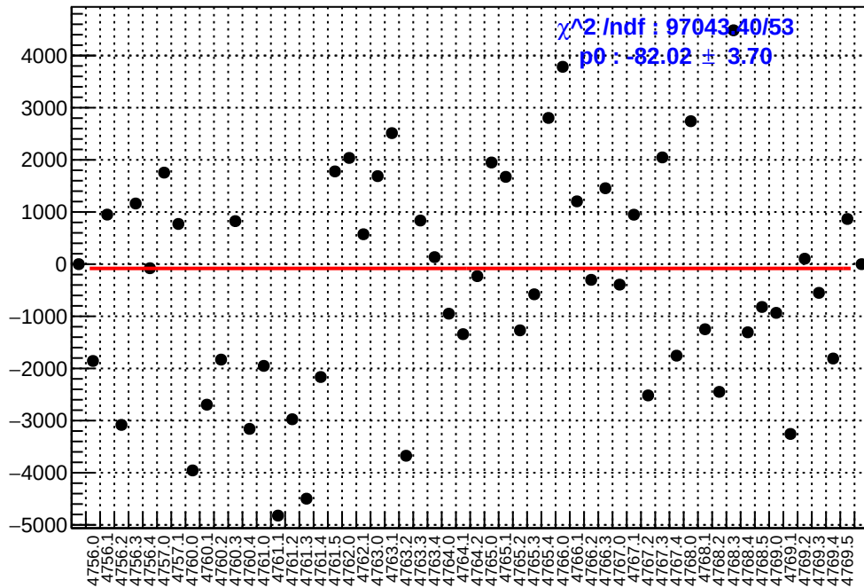
slug79: asym_us_avg.mean/ppb-reg_asym_us_avg.mean/ppb
