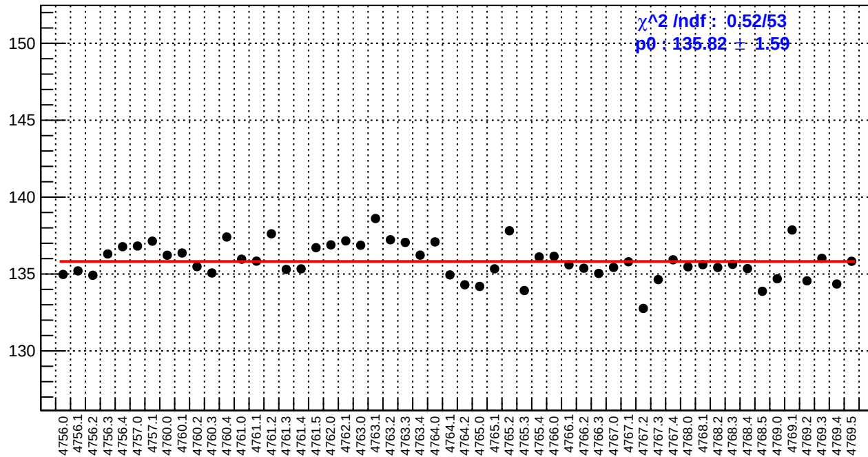
slug79: reg_asym_usl.rms/ppm
