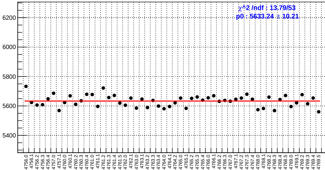
slug79: reg_asym_atl1r2_dd.rms/ppm
