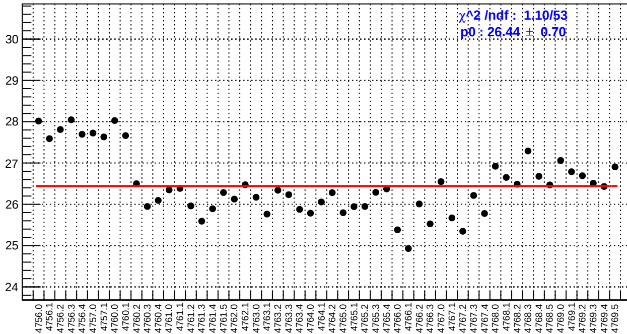
slug79: right_avg_bpm4eX/(ppb/nm)
