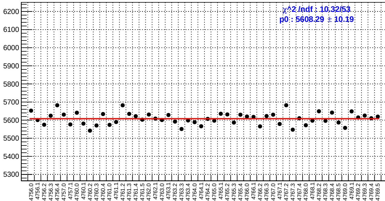
slug79: reg_asym_atl_avg.rms/ppm
