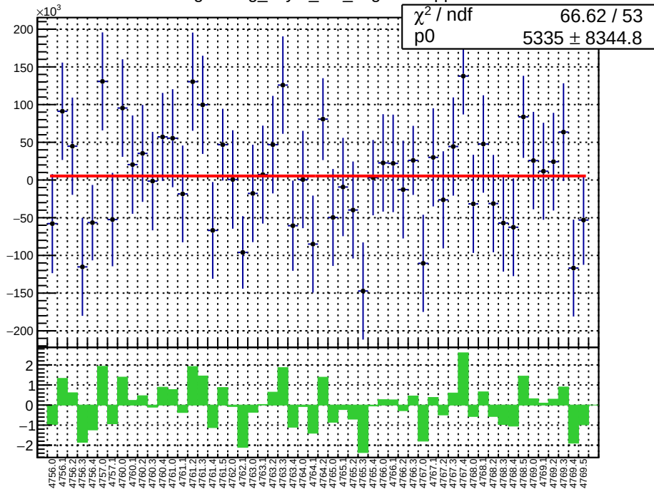
slug79: reg_asym_at1_avg.mean/ppb
