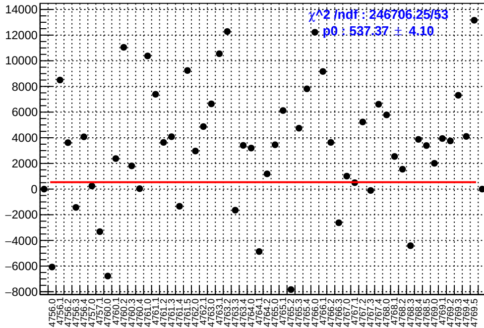
slug79: asym_atl1r2_dd.mean/ppb-reg_asym_atl1r2_dd.mean/ppb
