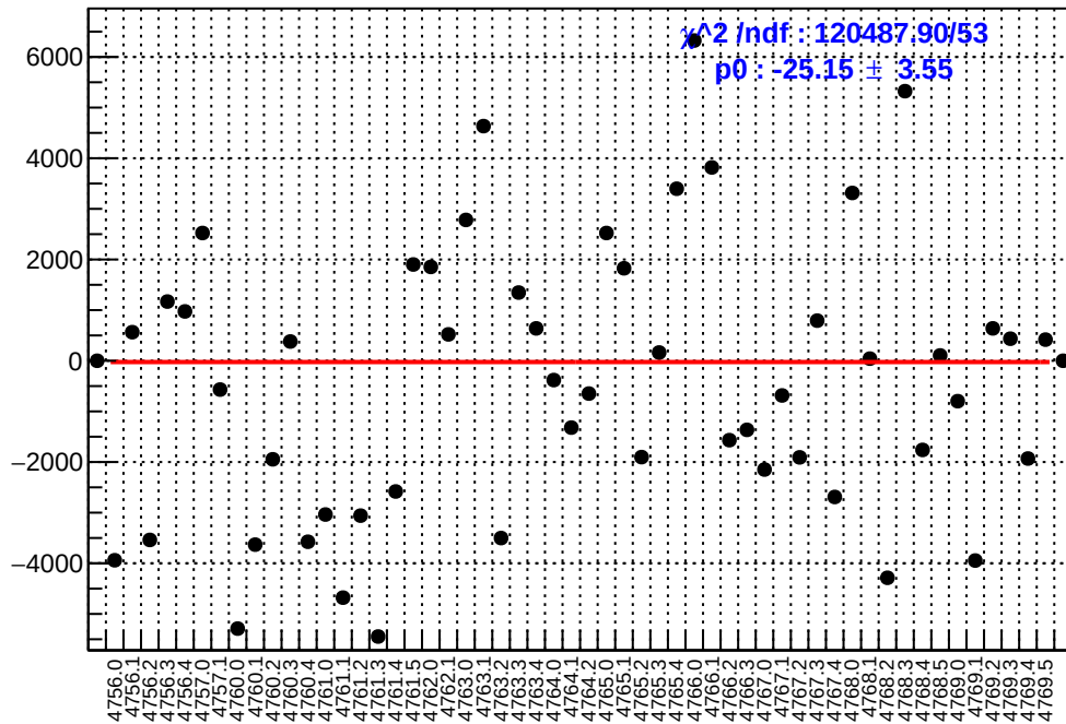
slug79: asym_sam1.mean/ppb-reg_asym_sam1.mean/ppb
