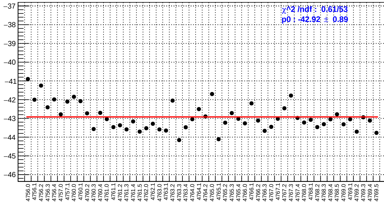
slug79: left_avg_bpm12X/(ppb/nm)
