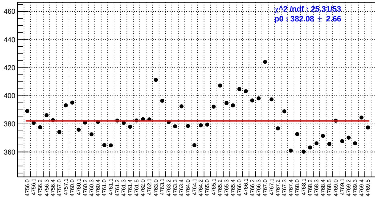
slug79: reg_asym_sam6.rms/ppm
