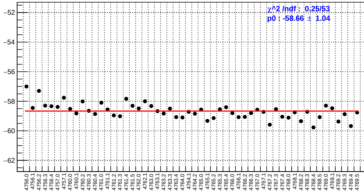
slug79: right_avg_bpm12X/(ppb/nm)
