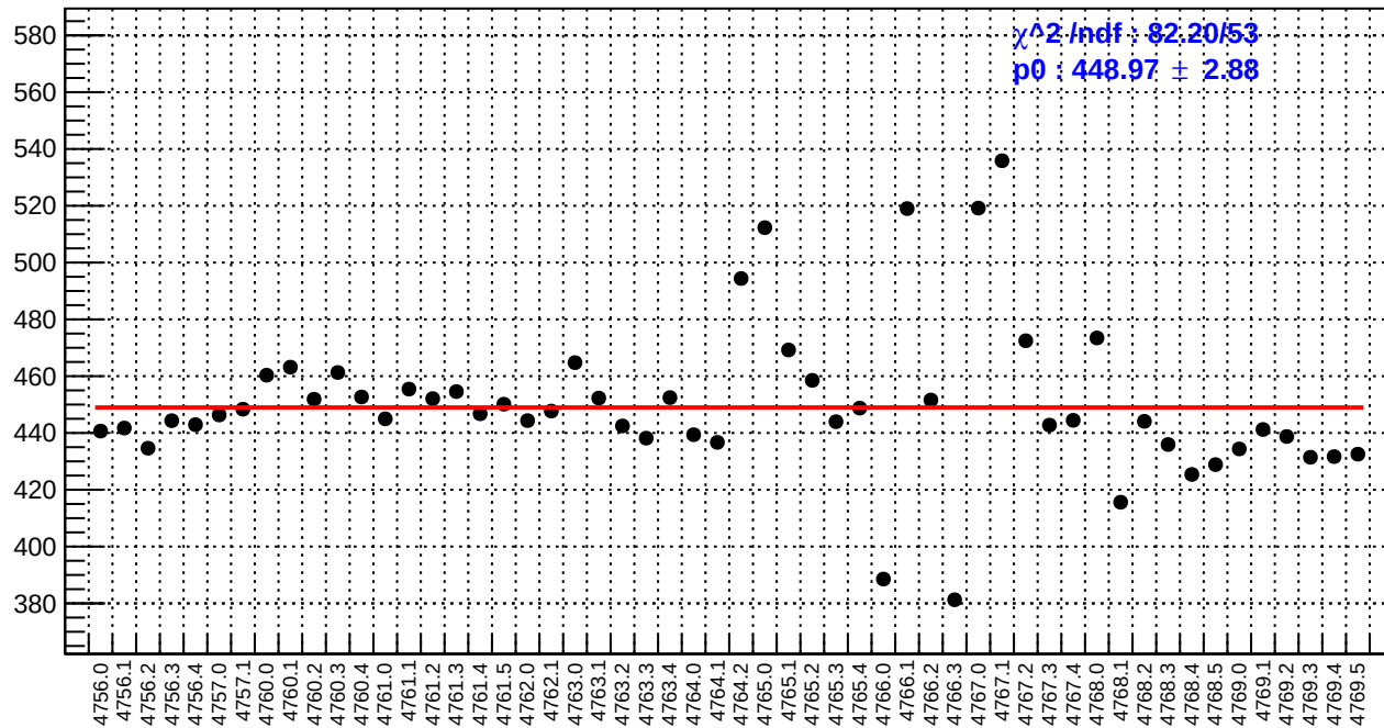
slug79: reg_asym_sam8.rms/ppm
