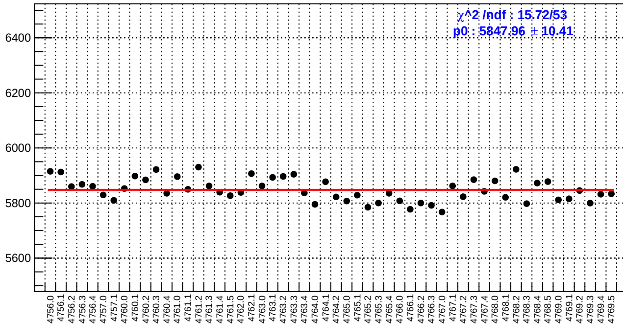
slug79: reg_asym_atr_dd.rms/ppm
