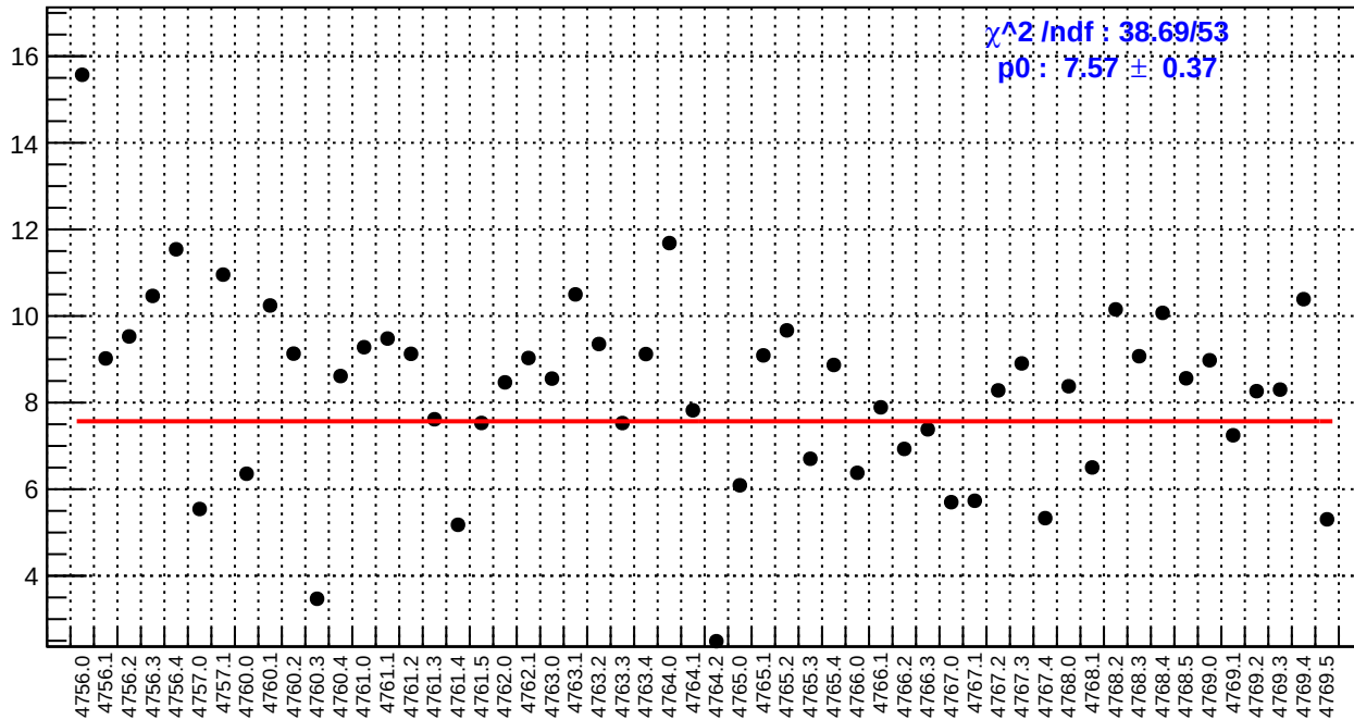
slug79: left_avg_bpm4eY/(ppb/nm)
