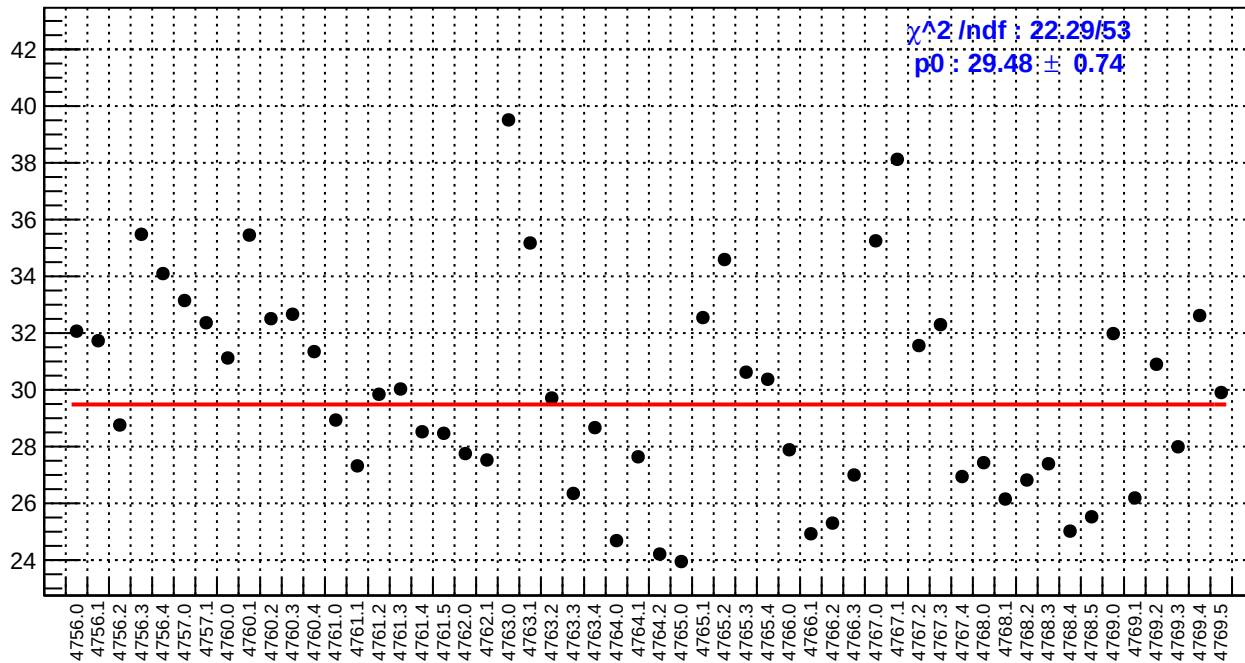
slug79: left_avg_bpm4aX/(ppb/nm)
