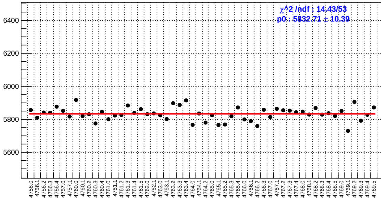
slug79: reg_asym_atr1l2_avg.rms/ppm
