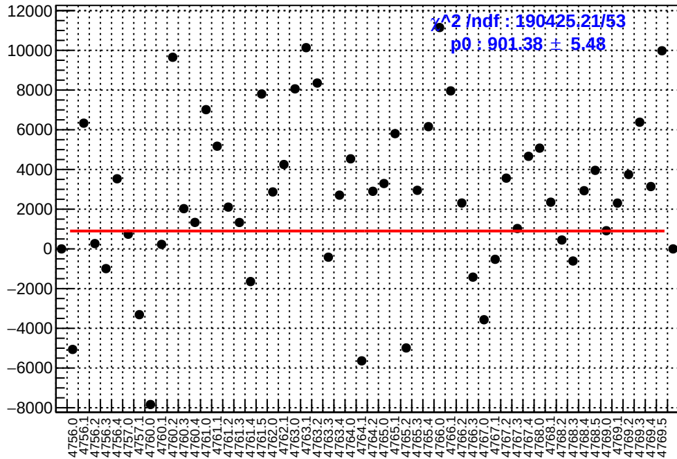
slug79: asym_us_dd.mean/ppb-reg_asym_us_dd.mean/ppb
