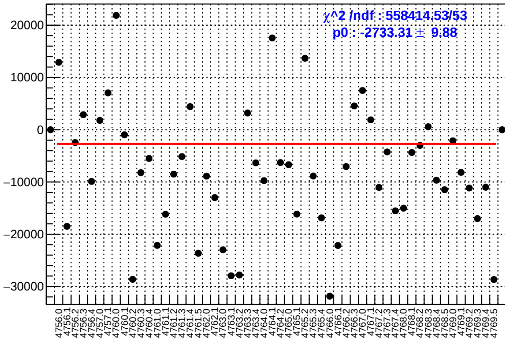
slug79: asym_sam8.mean/ppb-reg_asym_sam8.mean/ppb
