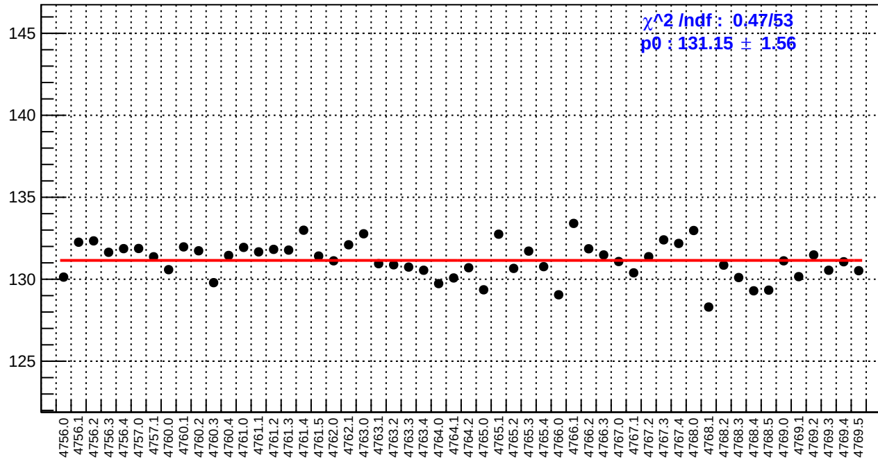
slug79: reg_asym_usr.rms/ppm
