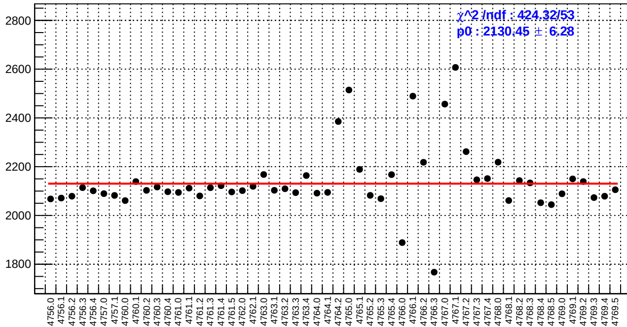
slug79: reg_asym_sam2.rms/ppm
