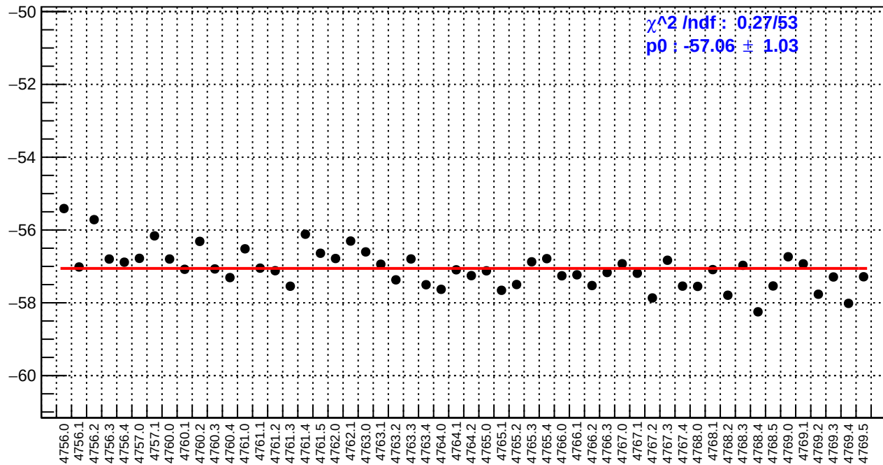
slug79: usr_bpm12X/(ppb/nm)
