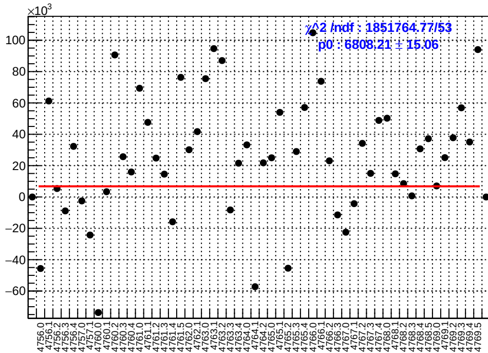
slug79: asym_sam4.mean/ppb-reg_asym_sam4.mean/ppb
