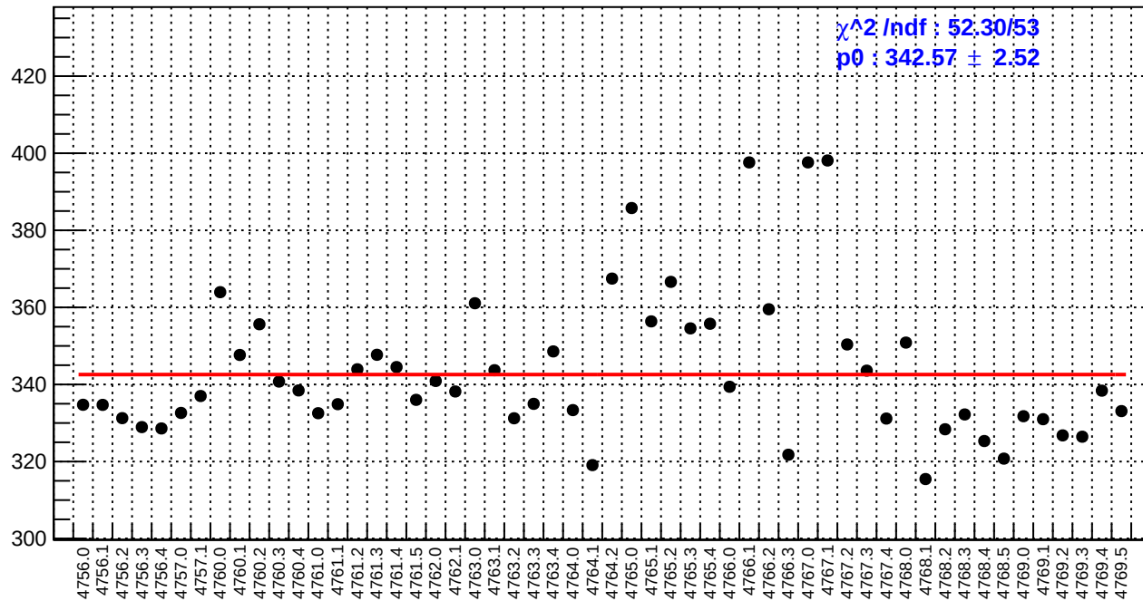
slug79: reg_asym_sam7.rms/ppm
