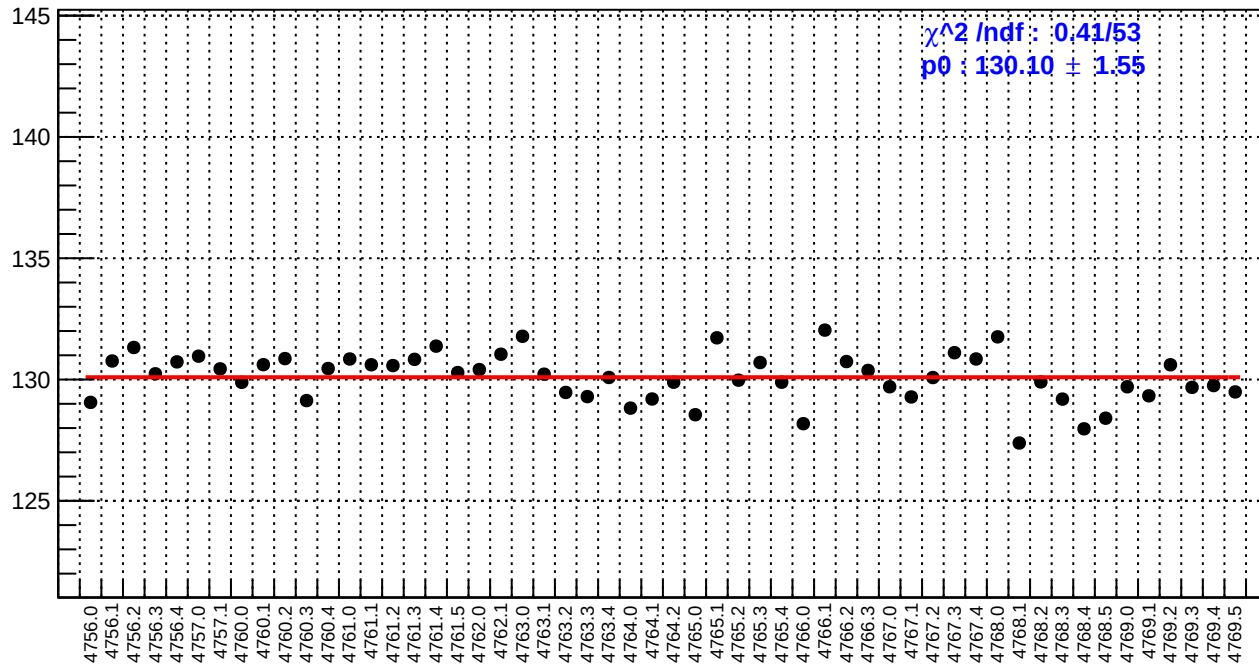
slug79: reg_asym_right_avg.rms/ppm
