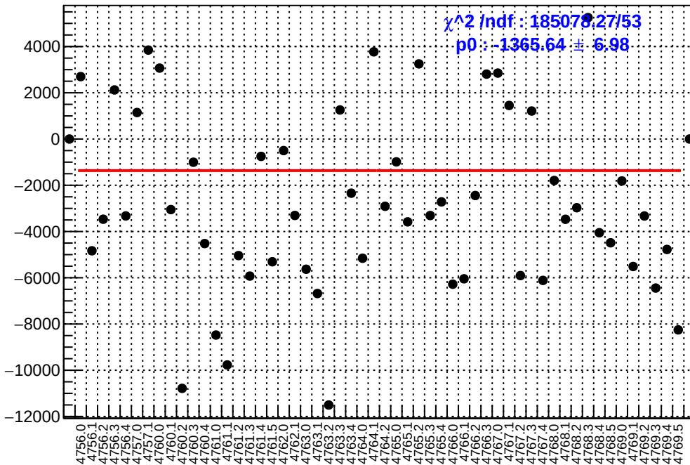
slug79: asym_right_avg.mean/ppb-reg_asym_right_avg.mean/ppb
