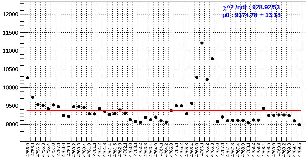
slug79: diff_bpm4eX.rms/nm
