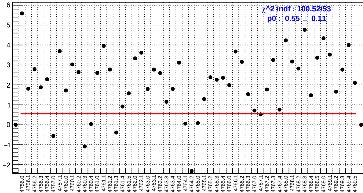
slug79: us_avg_bpm4eY/(ppb/nm)
