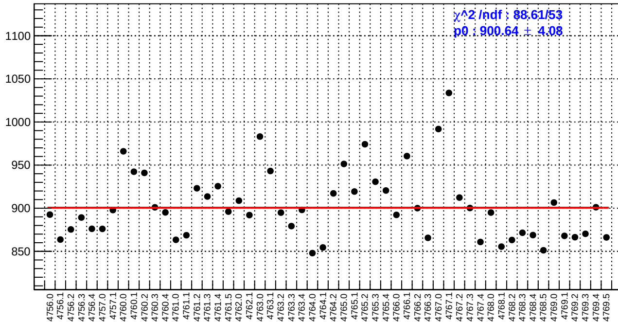
slug79: reg_asym_sam3.rms/ppm
