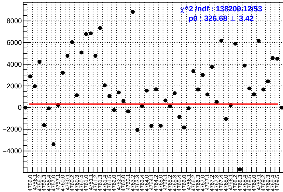
slug79: asym_sam5.mean/ppb-reg_asym_sam5.mean/ppb
