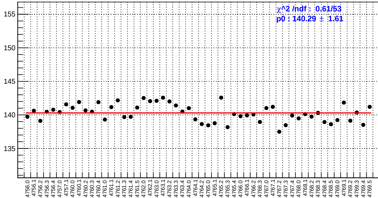
slug79: reg_asym_dsl.rms/ppm
