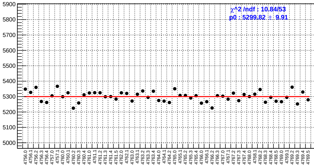
slug79: reg_asym_at2_avg.rms/ppm
