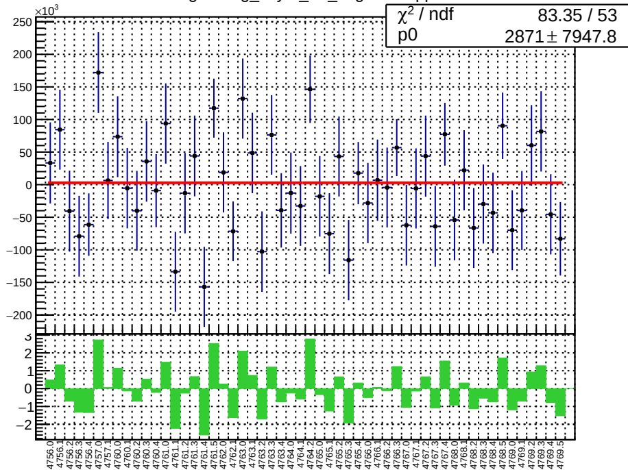
slug79: reg_asym_atr_avg.mean/ppb
