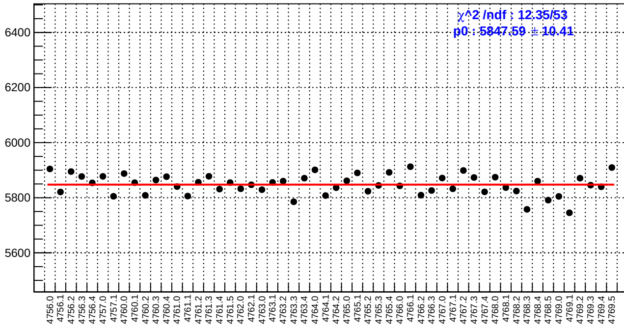
slug79: reg_asym_atr_avg.rms/ppm
