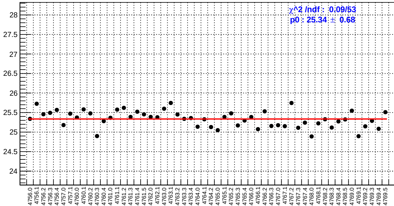
slug79: reg_asym_left_dd.rms/ppm
