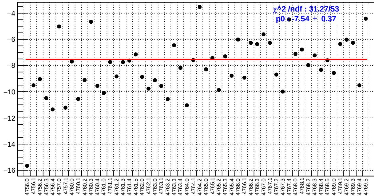
slug79: usl_bpm4aY/(ppb/nm)
