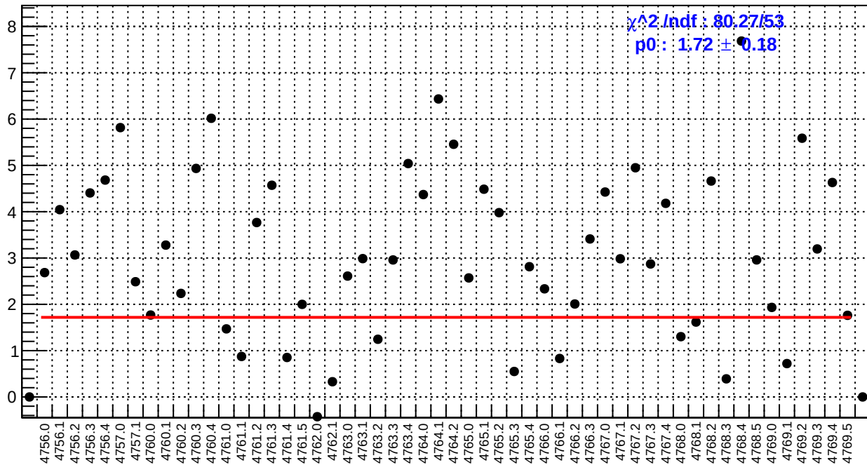
slug79: right_avg_bpm4aY/(ppb/nm)
