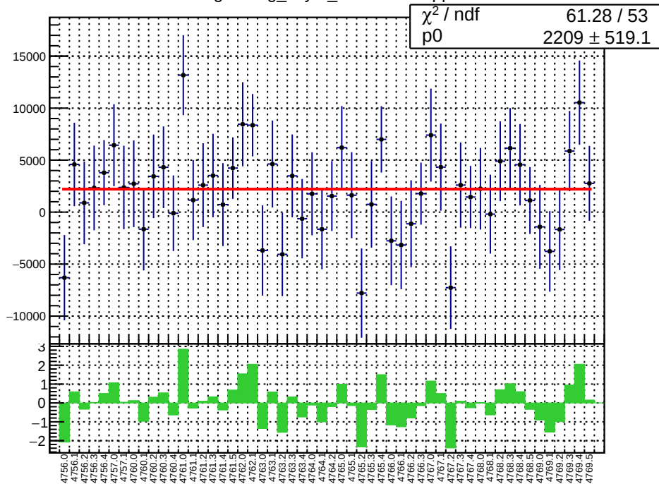
slug79: reg_asym_sam6.mean/ppb
