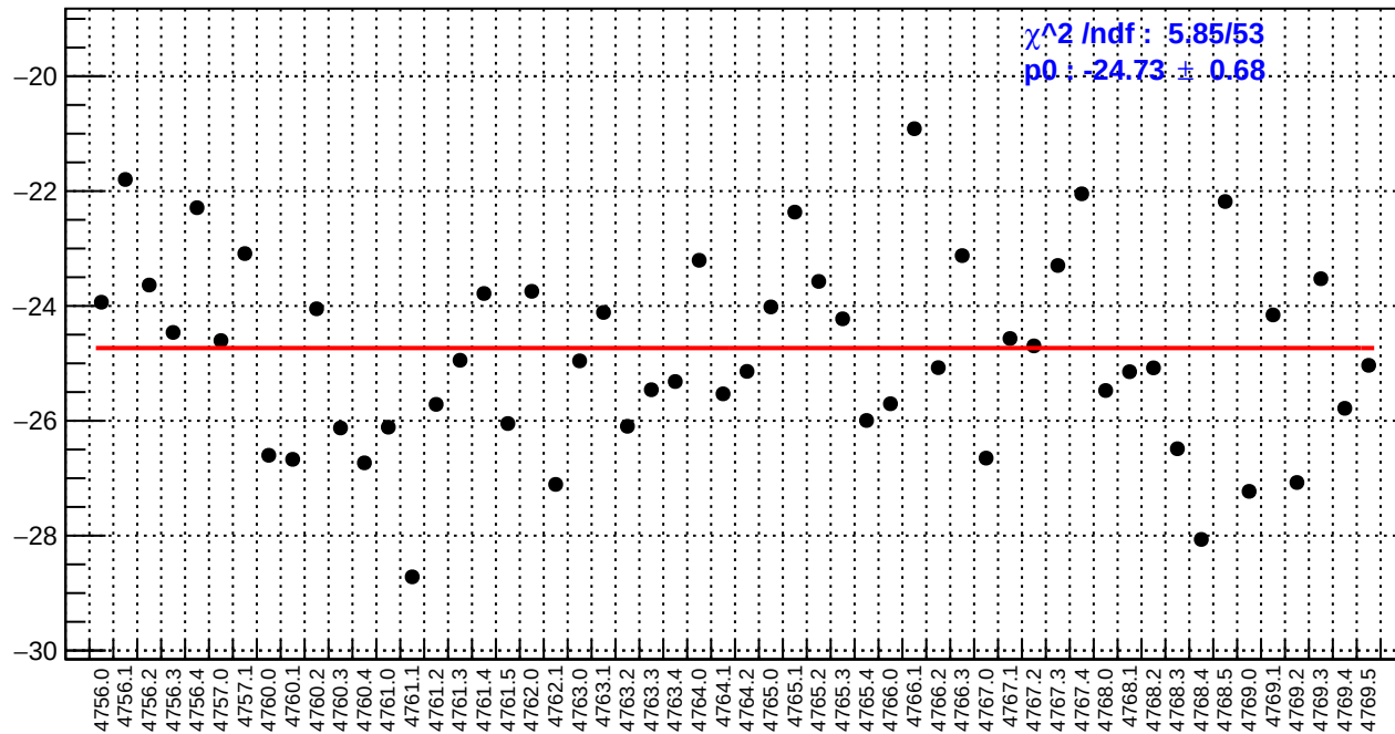
slug79: right_avg_bpm4aX/(ppb/nm)
