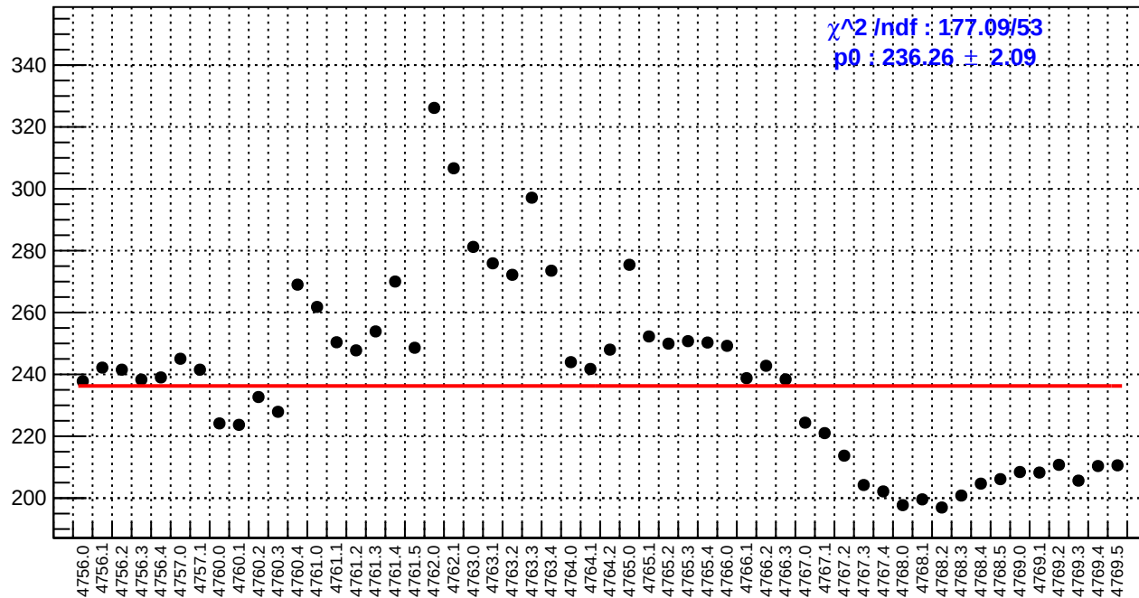
slug79: asym_bcm_an_us.rms/ppm
