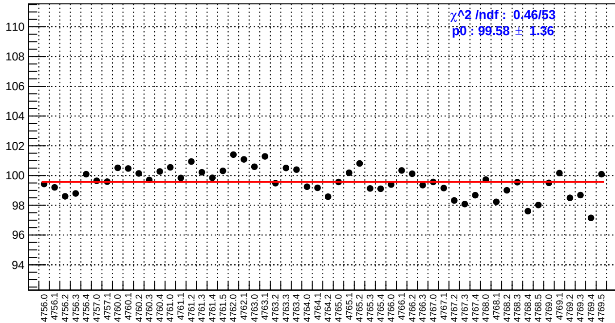
slug79: reg_asym_ds_avg.rms/ppm
