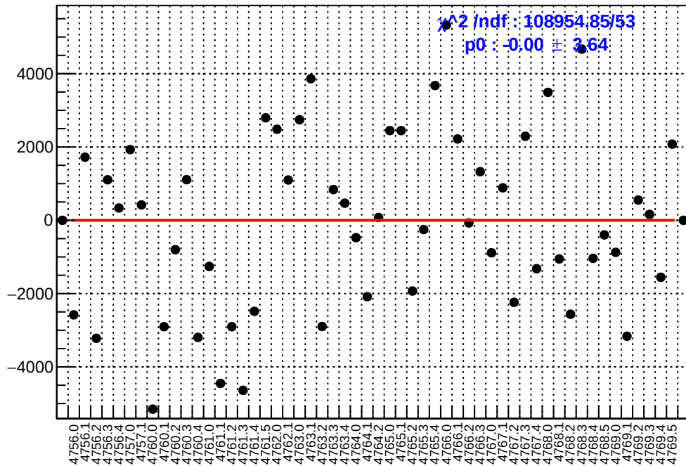
slug79: asym_ds_avg.mean/ppb-reg_asym_ds_avg.mean/ppb
