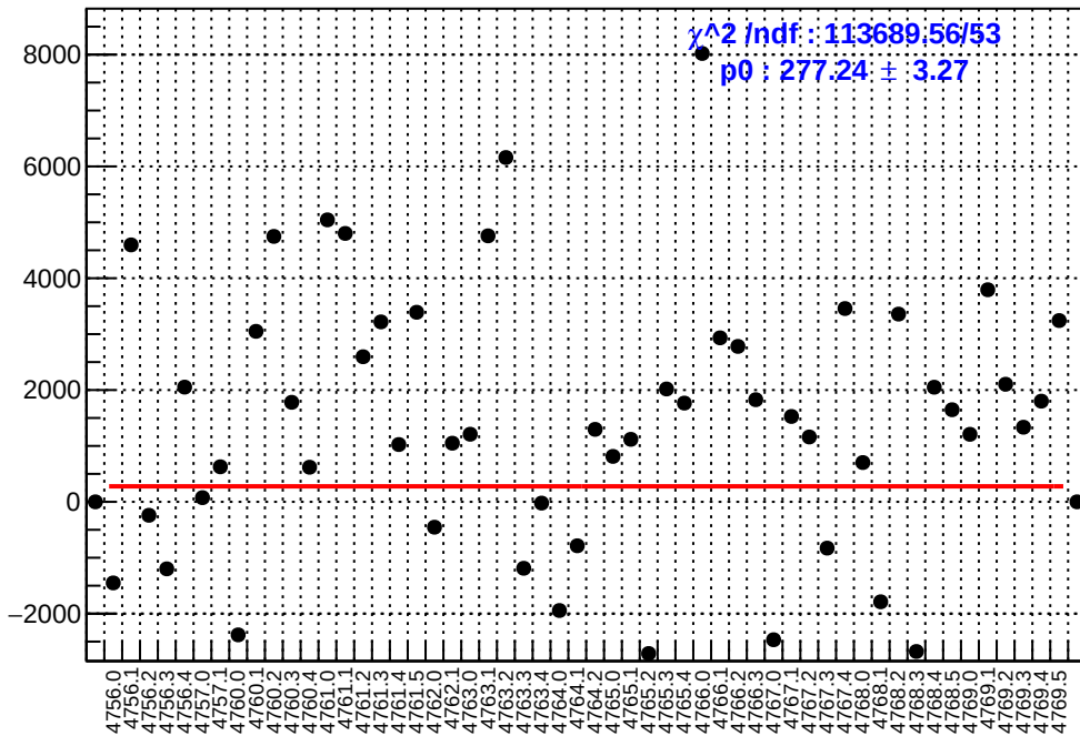
slug79: asym_atr_dd.mean/ppb-reg_asym_atr_dd.mean/ppb
