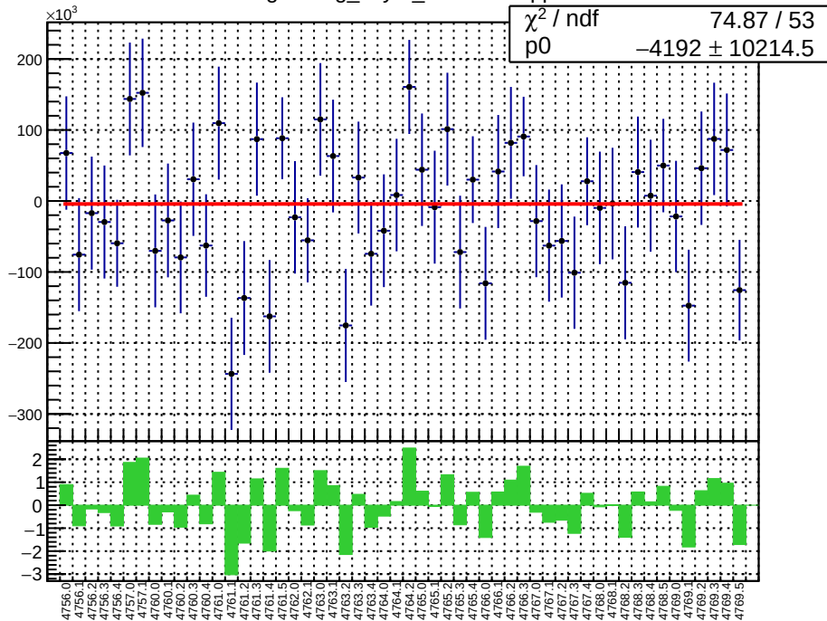
slug79: reg_asym_atr2.mean/ppb
