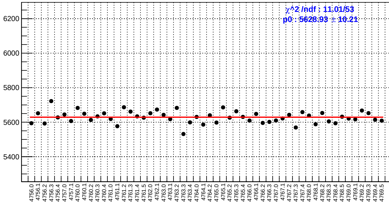
slug79: reg_asym_atl1r2_avg.rms/ppm
