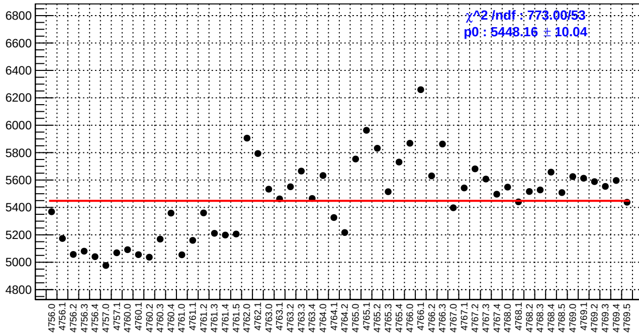
slug79: diff_bpm11X.rms/nm
