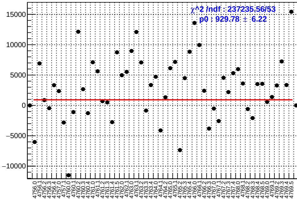
slug79: asym_atl_avg.mean/ppb-reg_asym_atl_avg.mean/ppb
