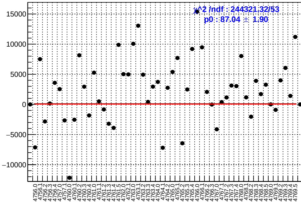
slug79: asym_left_avg.mean/ppb-reg_asym_left_avg.mean/ppb
