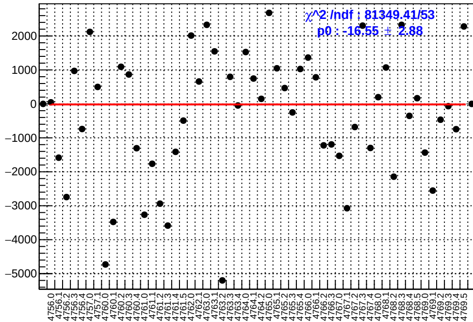
slug79: asym_at2_avg.mean/ppb-reg_asym_at2_avg.mean/ppb
