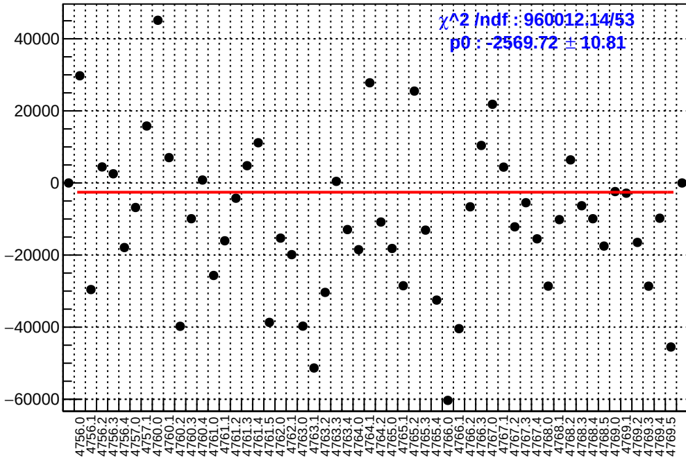
slug79: asym_sam6.mean/ppb-reg_asym_sam6.mean/ppb
