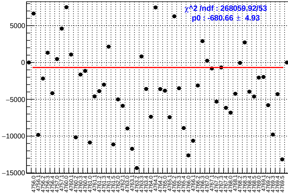
slug79: asym_atr_avg.mean/ppb-reg_asym_atr_avg.mean/ppb
