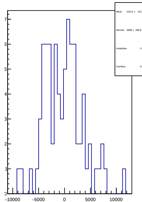
slug8: 1D Corr asym_sam1.mean/ppb-reg_asym_sam1.mean/ppb
