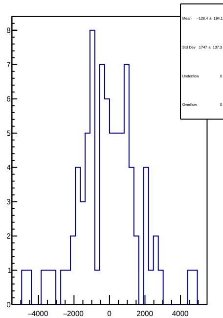
slug8: 1D Corr asym_right_avg.mean/ppb-reg_asym_right_avg.mean/ppb
