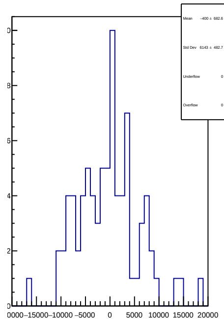
slug8: 1D Corr asym_dsl.mean/ppb-reg_asym_dsl.mean/ppb
