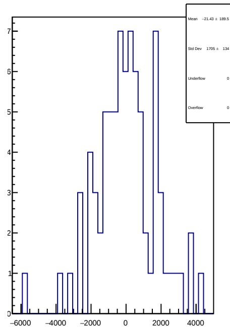
slug8: 1D Corr asym_ds_dd.mean/ppb-reg_asym_ds_dd.mean/ppb
