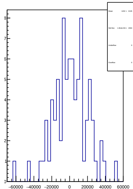
slug8: 1D Corr asym_sam8.mean/ppb-reg_asym_sam8.mean/ppb
