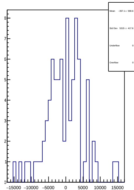
slug8: 1D Corr asym_dsr.mean/ppb-reg_asym_dsr.mean/ppb
