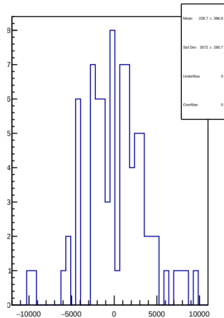
slug8: 1D Corr asym_right_dd.mean/ppb-reg_asym_right_dd.mean/ppb
