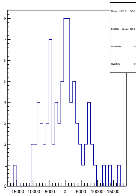
slug8: 1D Corr asym_usl.mean/ppb-reg_asym_usl.mean/ppb
