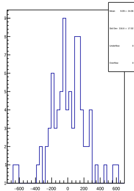
slug8: 1D Corr asym_left_dd.mean/ppb-reg_asym_left_dd.mean/ppb
