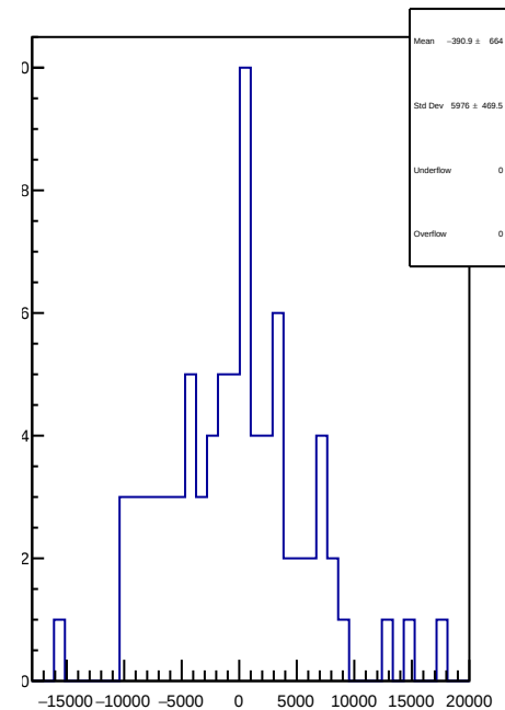
slug8: 1D Corr asym_left_avg.mean/ppb-reg_asym_left_avg.mean/ppb
