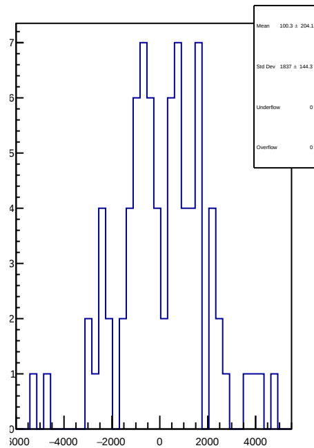
slug8: 1D Corr asym_usr.mean/ppb-reg_asym_usr.mean/ppb
