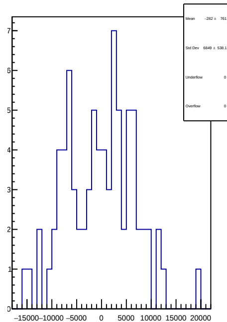
slug8: 1D Corr asym_sam5.mean/ppb-reg_asym_sam5.mean/ppb
