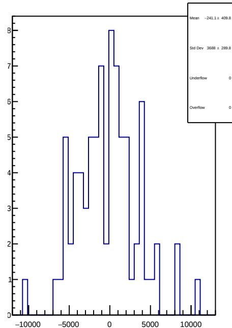
slug8: 1D Corr asym_us_dd.mean/ppb-reg_asym_us_dd.mean/ppb
