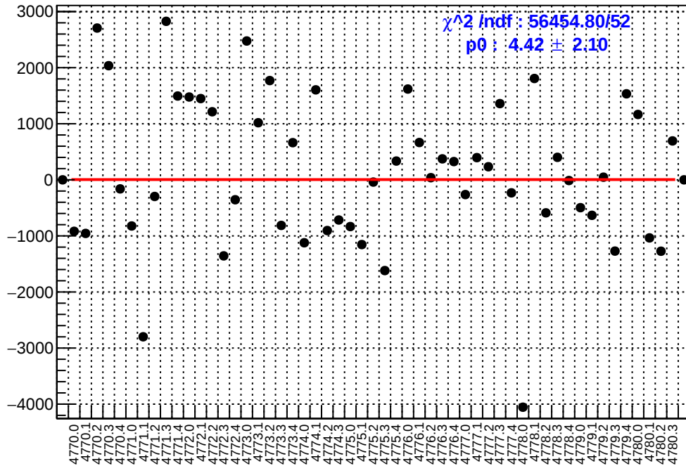
slug80: asym_at1_avg.mean/ppb-reg_asym_at1_avg.mean/ppb
