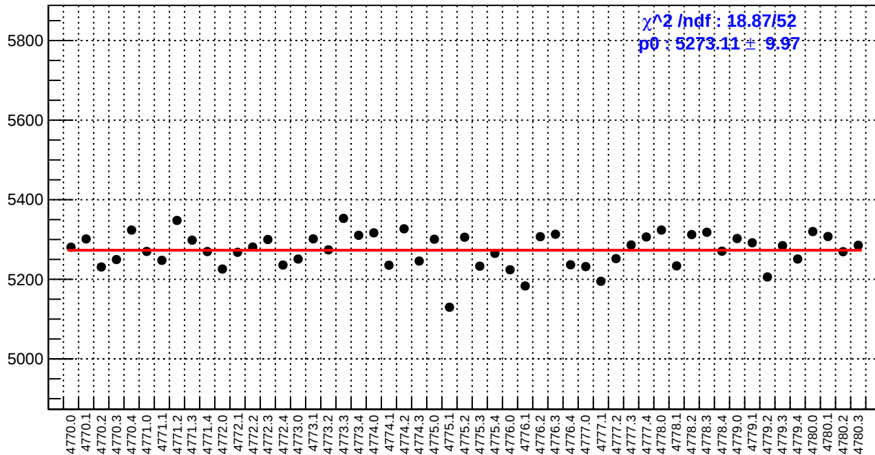
slug80: reg_asym_at2_avg.rms/ppm
