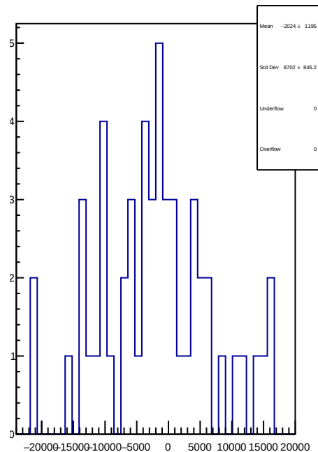
slug80: 1D Corr asym_atl2.mean/ppb-reg_asym_atl2.mean/ppb
