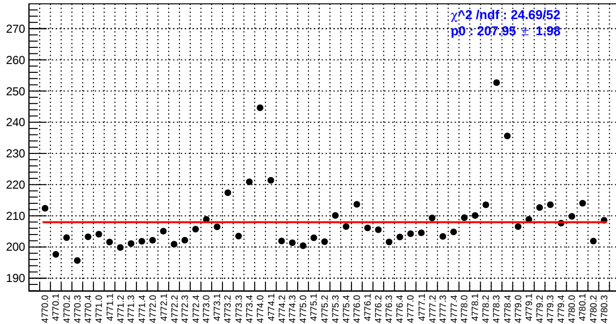
slug80: reg_asym_sam5.rms/ppm
