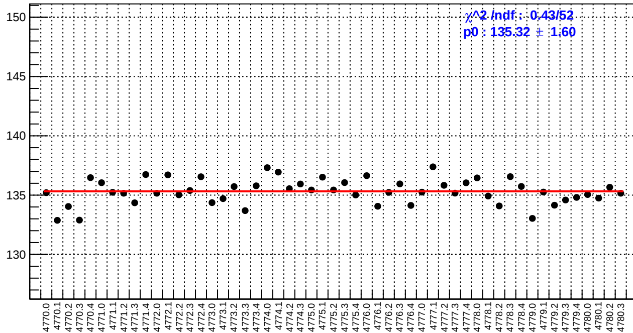
slug80: reg_asym_usl.rms/ppm
