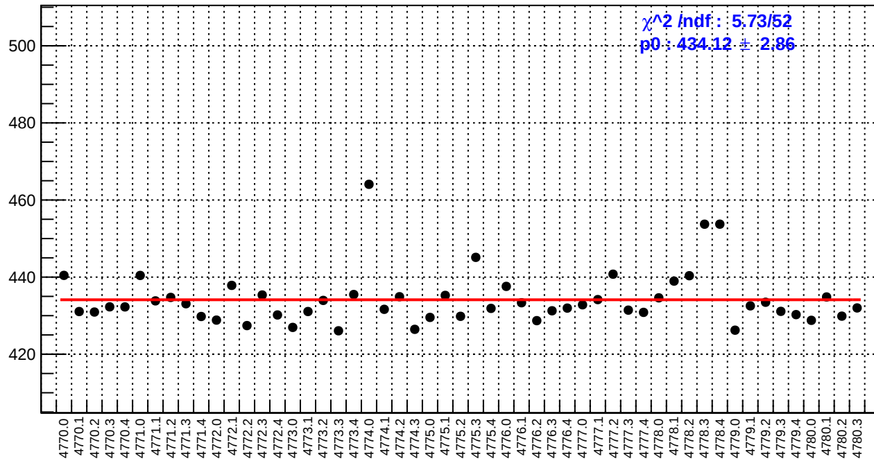
slug80: reg_asym_sam8.rms/ppm
