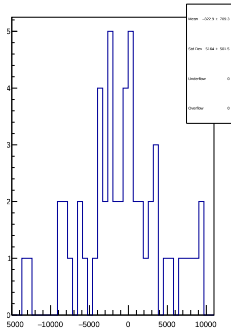
slug80: 1D Corr asym_usl.mean/ppb-reg_asym_usl.mean/ppb
