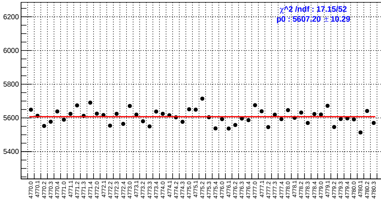
slug80: reg_asym_atl1r2_avg.rms/ppm
