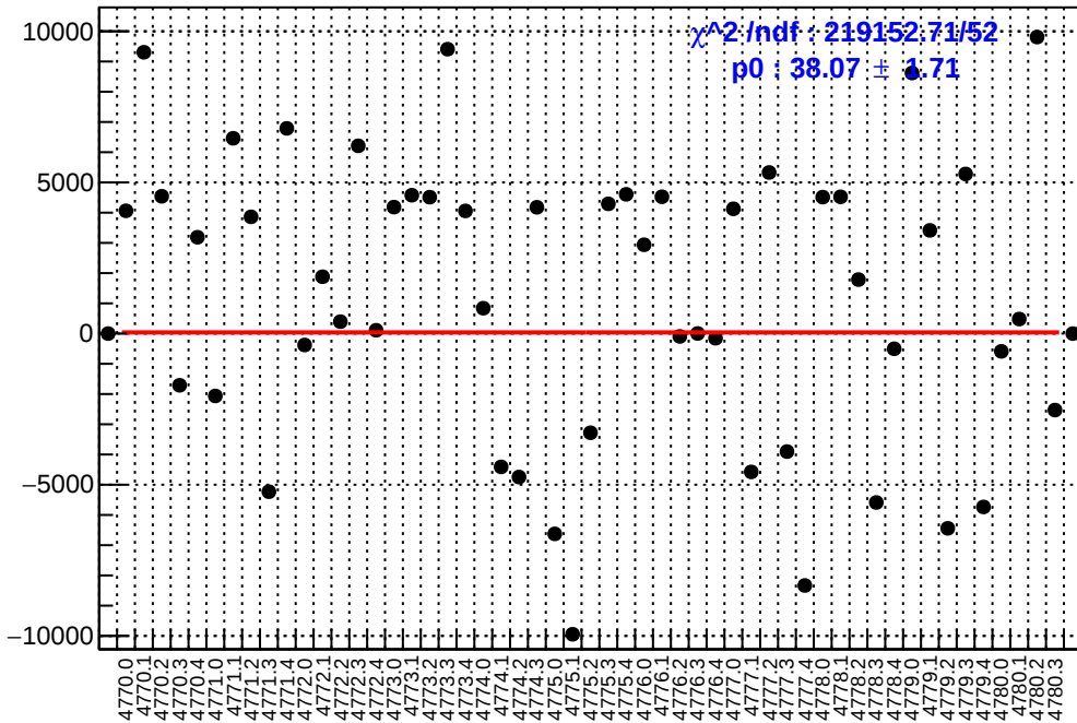
slug80: asym_dsr.mean/ppb-reg_asym_dsr.mean/ppb
