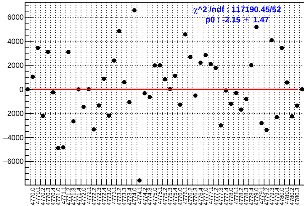
slug80: asym_sam1.mean/ppb-reg_asym_sam1.mean/ppb
