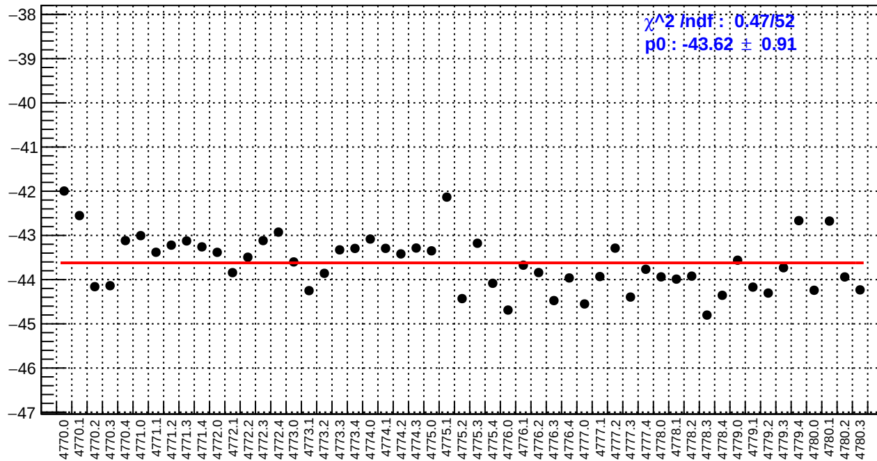
slug80: left_avg_bpm12X/(ppb/nm)
