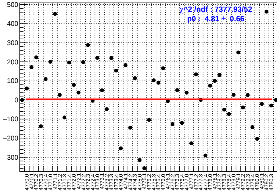
slug80: asym_left_dd.mean/ppb-reg_asym_left_dd.mean/ppb
