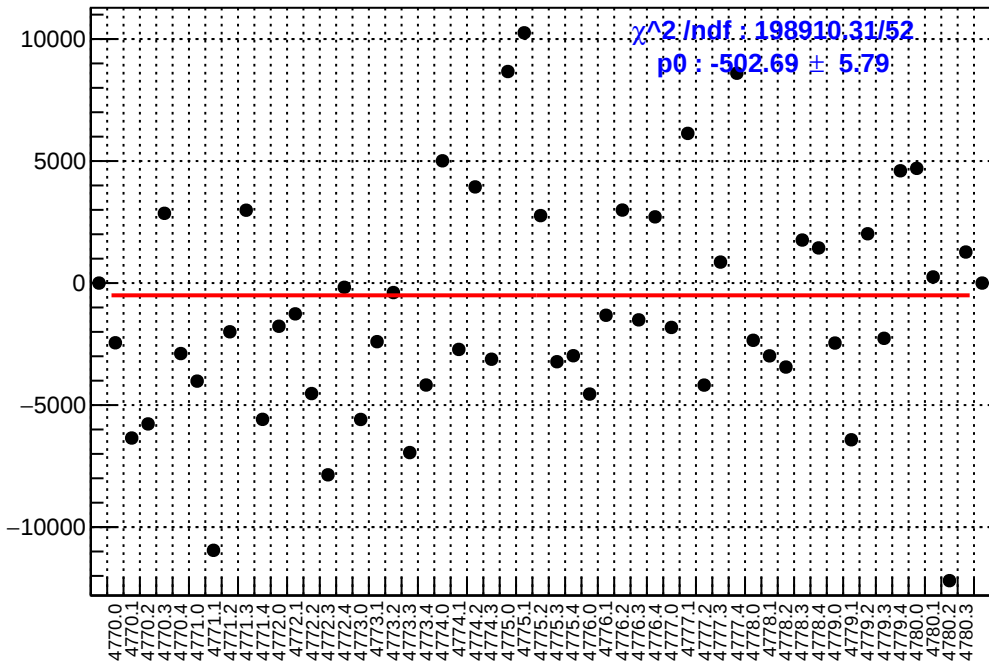
slug80: asym_us_dd.mean/ppb-reg_asym_us_dd.mean/ppb
