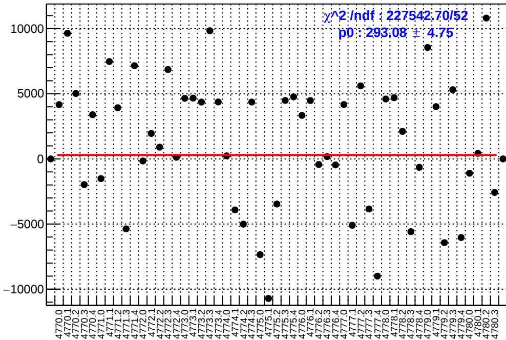
slug80: asym_right_avg.mean/ppb-reg_asym_right_avg.mean/ppb
