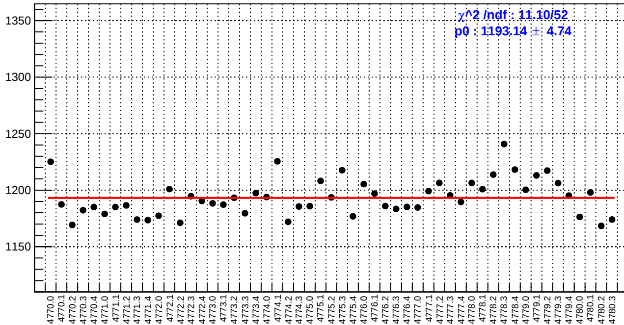
slug80: reg_asym_sam4.rms/ppm
