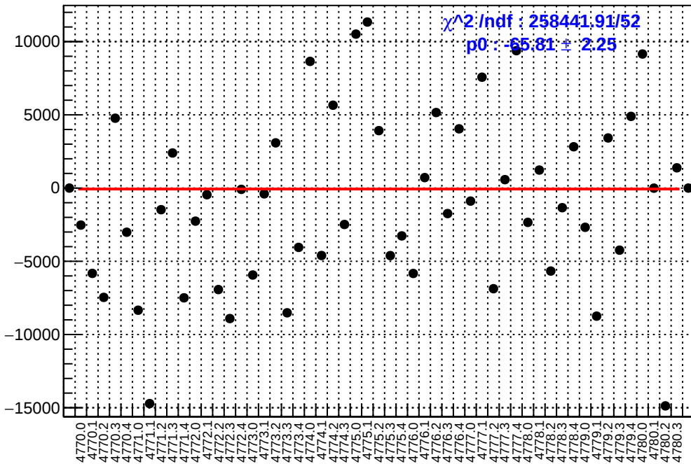
slug80: asym_atl_avg.mean/ppb-reg_asym_atl_avg.mean/ppb
