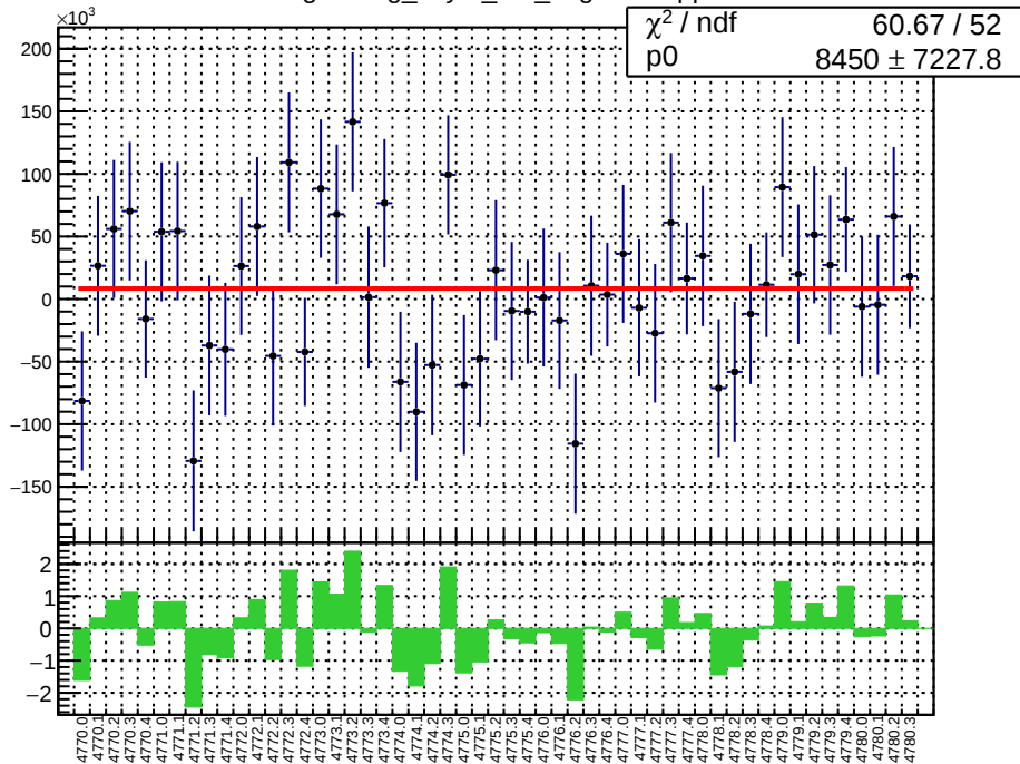
slug80: reg_asym_at2_avg.mean/ppb
