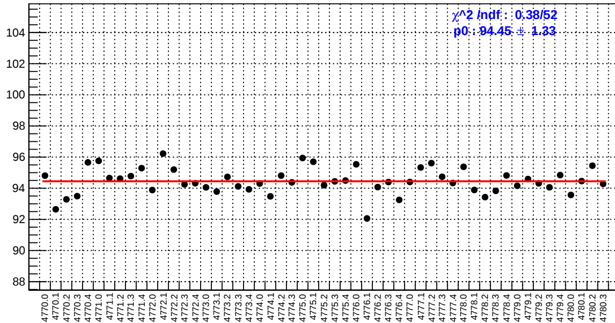
slug80: reg_asym_ds_dd.rms/ppm
