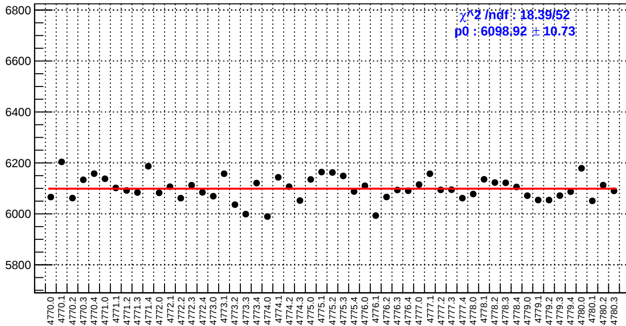
slug80: reg_asym_at1_avg.rms/ppm
