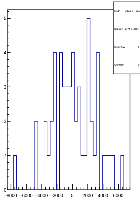
slug80: 1D Corr asym_sam1.mean/ppb-reg_asym_sam1.mean/ppb
