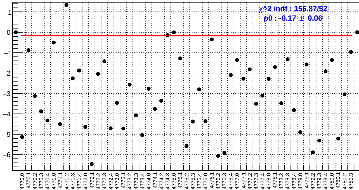
slug80: right_avg_bpm4eY/(ppb/nm)
