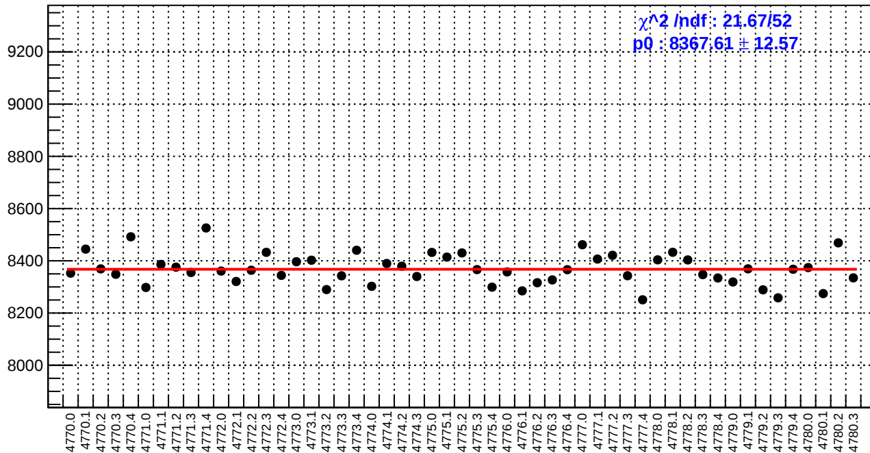
slug80: reg_asym_atl1.rms/ppm
