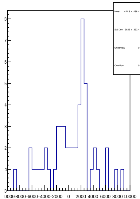
slug80: 1D Corr asym_atr1.mean/ppb-reg_asym_atr1.mean/ppb
