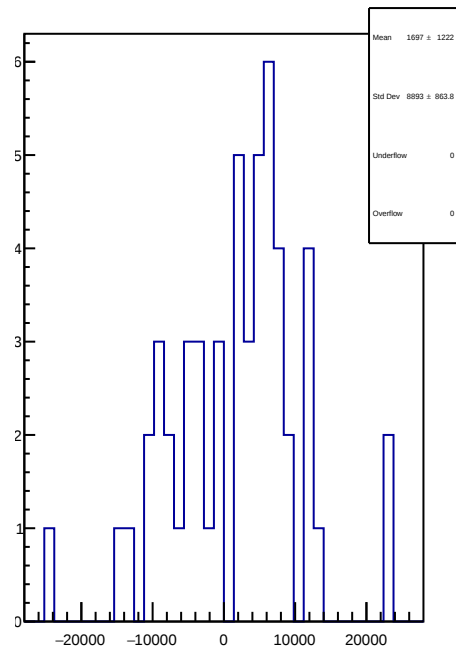
slug80: 1D Corr asym_atr2.mean/ppb-reg_asym_atr2.mean/ppb
