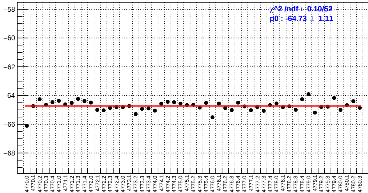
slug80: usl_bpm4eX/(ppb/nm)
