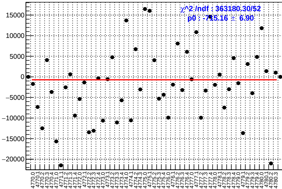
slug80: asym_atl2.mean/ppb-reg_asym_atl2.mean/ppb
