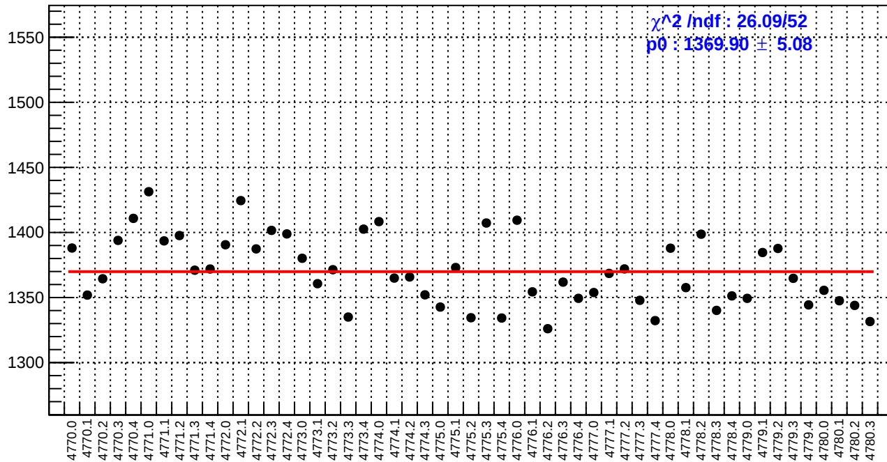
slug80: diff_bpm4aX.rms/nm
