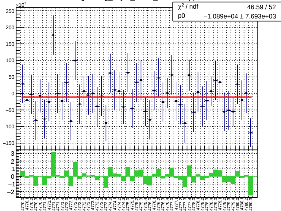
slug80: reg_asym_atl1r2_dd.mean/ppb
