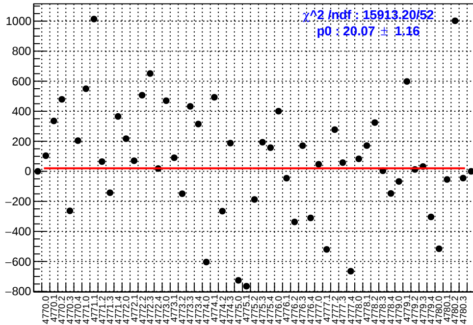
slug80: asym_right_dd.mean/ppb-reg_asym_right_dd.mean/ppb
