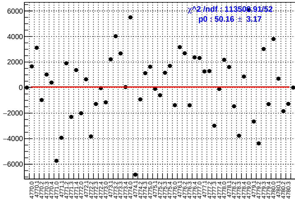
slug80: asym_ds_avg.mean/ppb-reg_asym_ds_avg.mean/ppb
