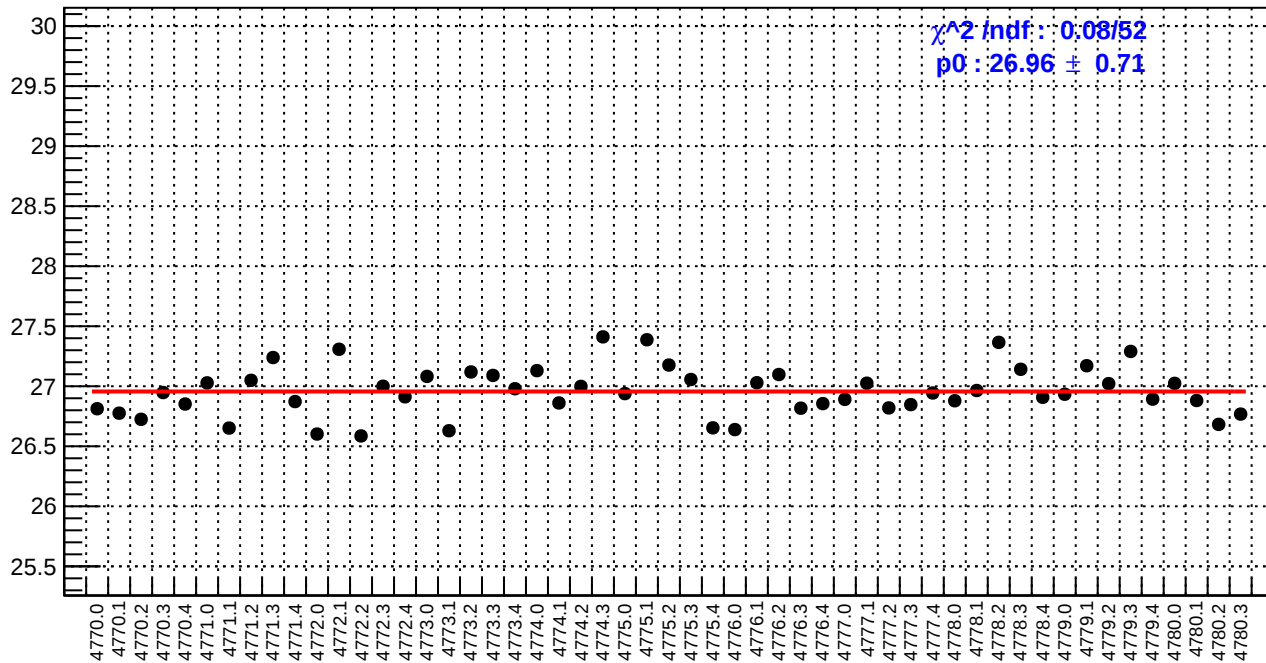
slug80: reg_asym_right_dd.rms/ppm
