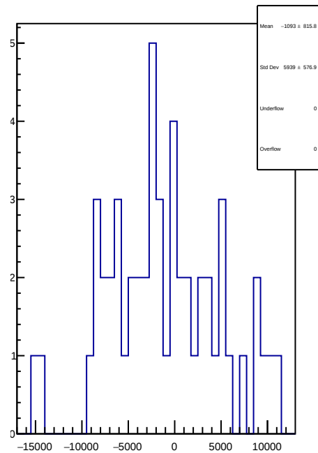
slug80: 1D Corr asym_atl_avg.mean/ppb-reg_asym_atl_avg.mean/ppb
