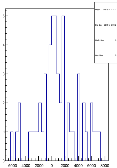
slug80: 1D Corr asym_atl_dd.mean/ppb-reg_asym_atl_dd.mean/ppb
