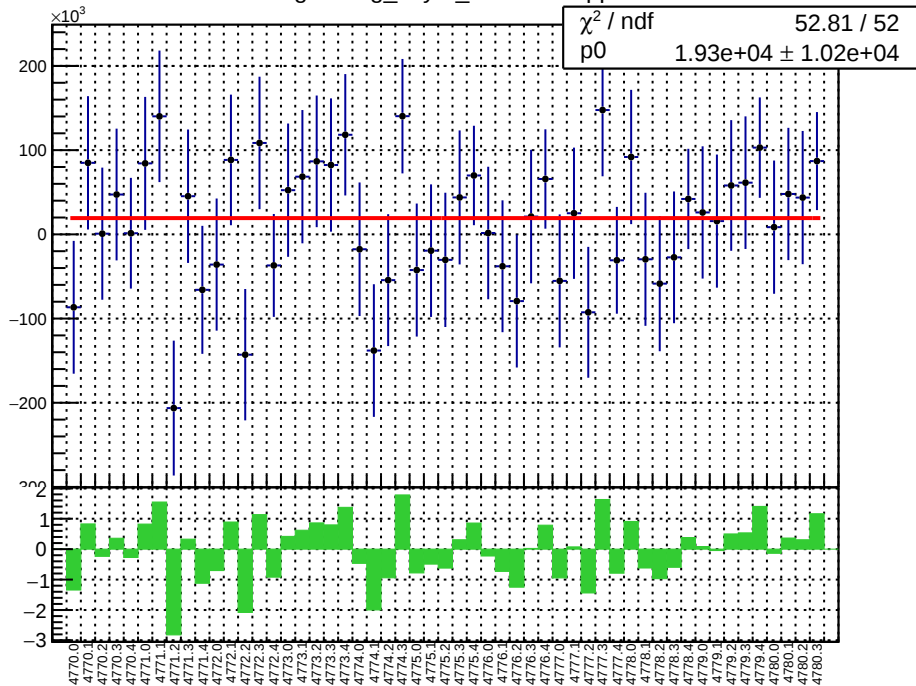
slug80: reg_asym_atr2.mean/ppb
