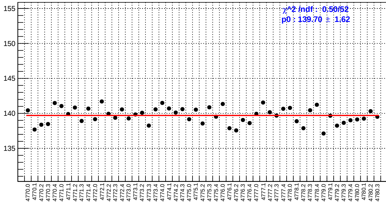
slug80: reg_asym_dsl.rms/ppm
