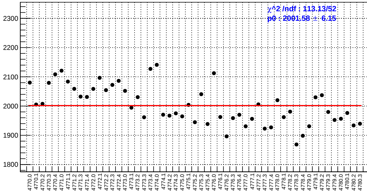
slug80: diff_bpm4eY.rms/nm
