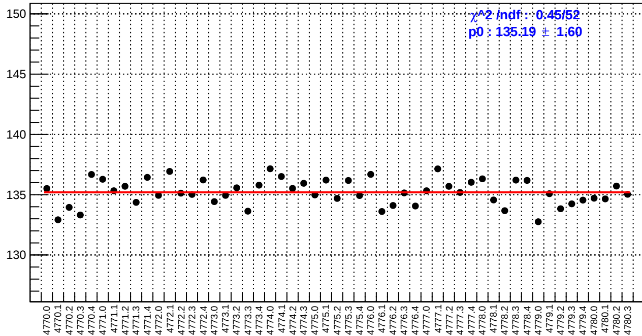
slug80: reg_asym_left_avg.rms/ppm
