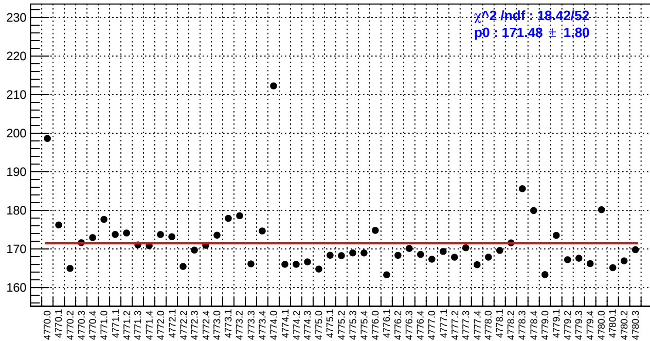
slug80: reg_asym_sam1.rms/ppm
