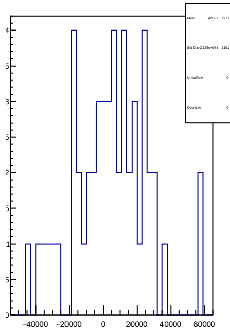
slug80: 1D Corr asym_sam6.mean/ppb-reg_asym_sam6.mean/ppb
