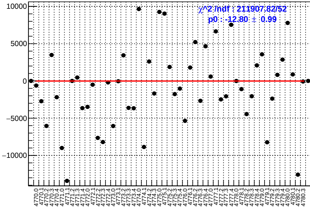
slug80: asym_usl.mean/ppb-reg_asym_usl.mean/ppb
