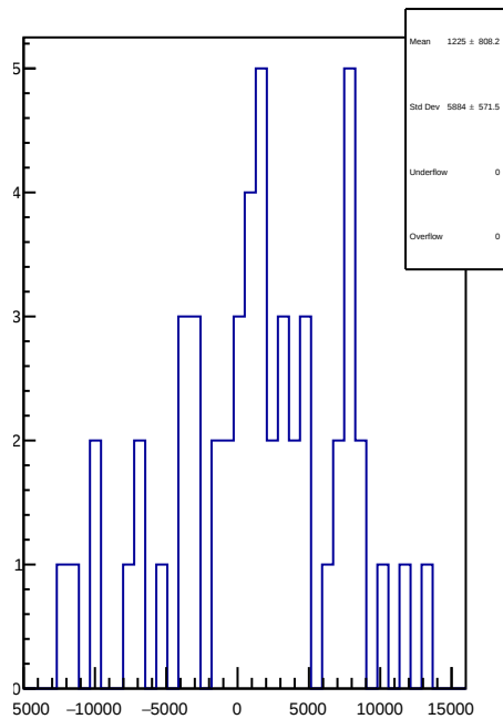
slug80: 1D Corr asym_atr1l2_dd.mean/ppb-reg_asym_atr1l2_dd.mean/ppb
