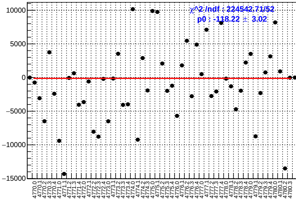
slug80: asym_dsl.mean/ppb-reg_asym_dsl.mean/ppb
