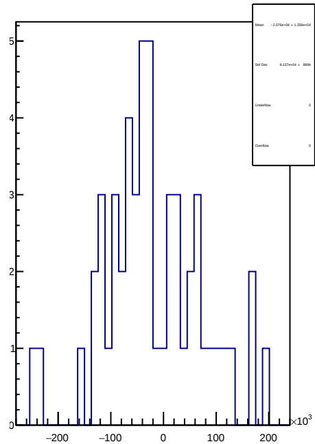
slug80: 1D Corr asym_sam3.mean/ppb-reg_asym_sam3.mean/ppb
