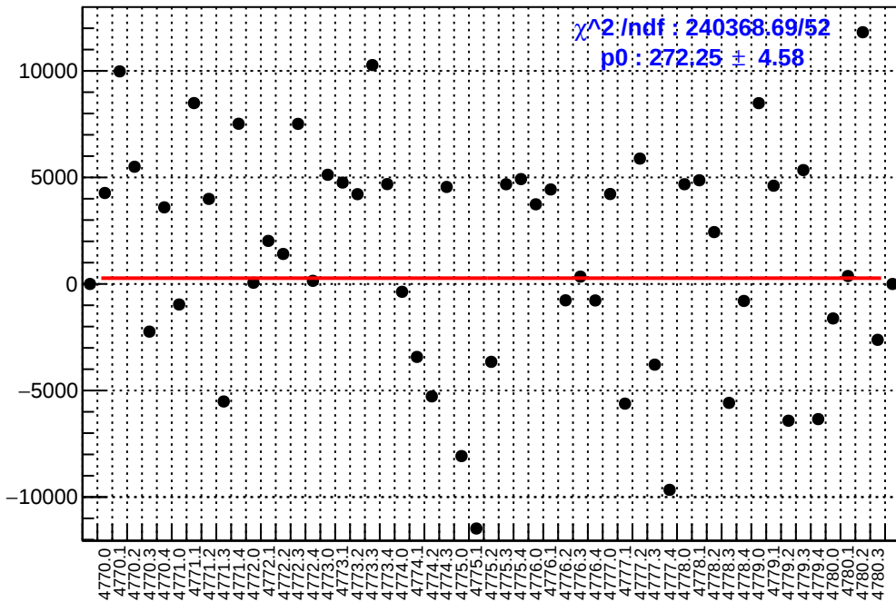
slug80: asym_usr.mean/ppb-reg_asym_usr.mean/ppb
