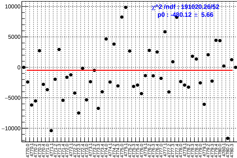
slug80: asym_ds_dd.mean/ppb-reg_asym_ds_dd.mean/ppb
