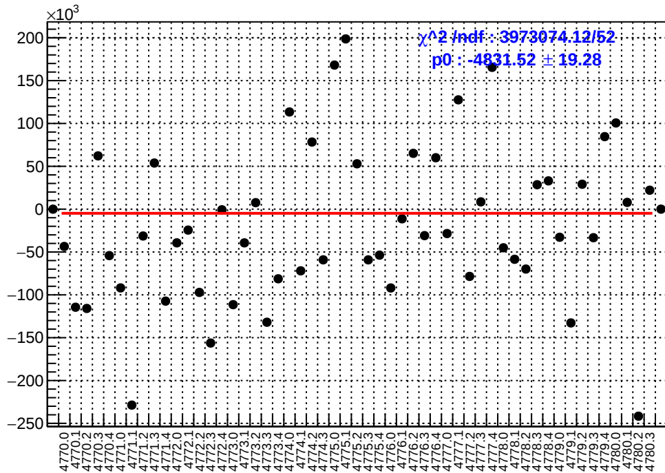
slug80: asym_sam3.mean/ppb-reg_asym_sam3.mean/ppb
