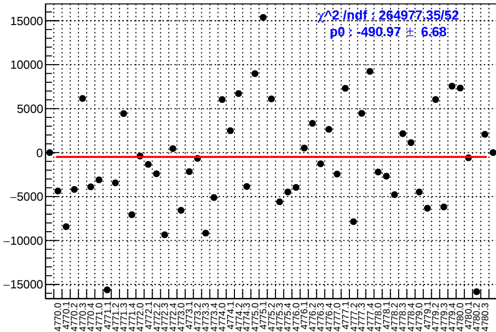
slug80: asym_atl1r2_dd.mean/ppb-reg_asym_atl1r2_dd.mean/ppb
