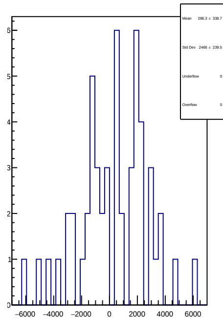
slug80: 1D Corr asym_us_avg.mean/ppb-reg_asym_us_avg.mean/ppb
