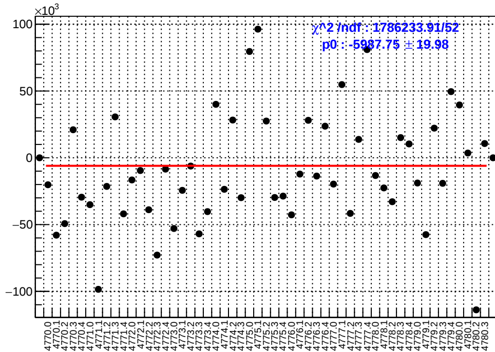
slug80: asym_sam4.mean/ppb-reg_asym_sam4.mean/ppb
