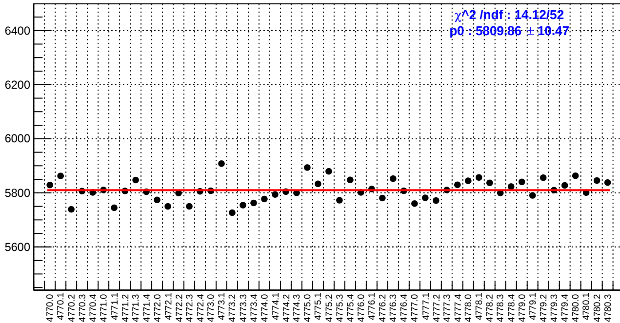
slug80: reg_asym_atr_avg.rms/ppm
