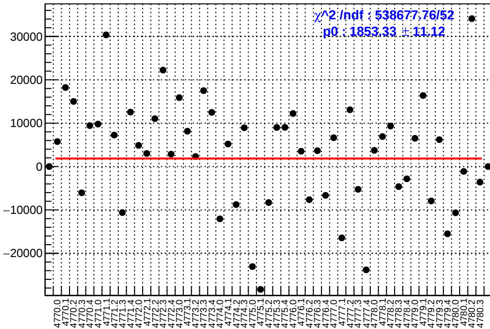
slug80: asym_sam8.mean/ppb-reg_asym_sam8.mean/ppb
