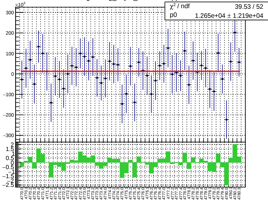
slug80: reg_asym_atr1.mean/ppb
