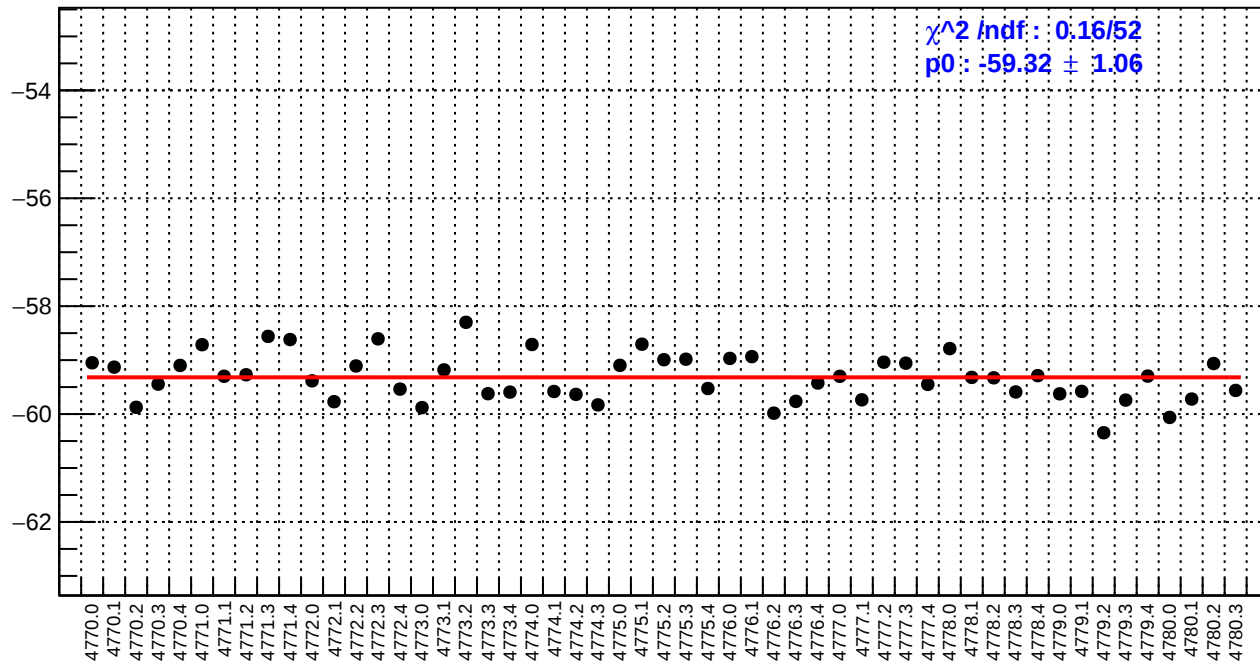
slug80: right_avg_bpm12X/(ppb/nm)
