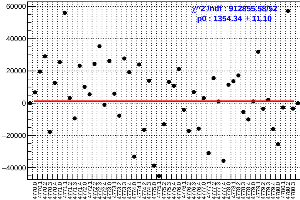
slug80: asym_sam6.mean/ppb-reg_asym_sam6.mean/ppb
