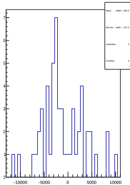
slug80: 1D Corr asym_ds_dd.mean/ppb-reg_asym_ds_dd.mean/ppb
