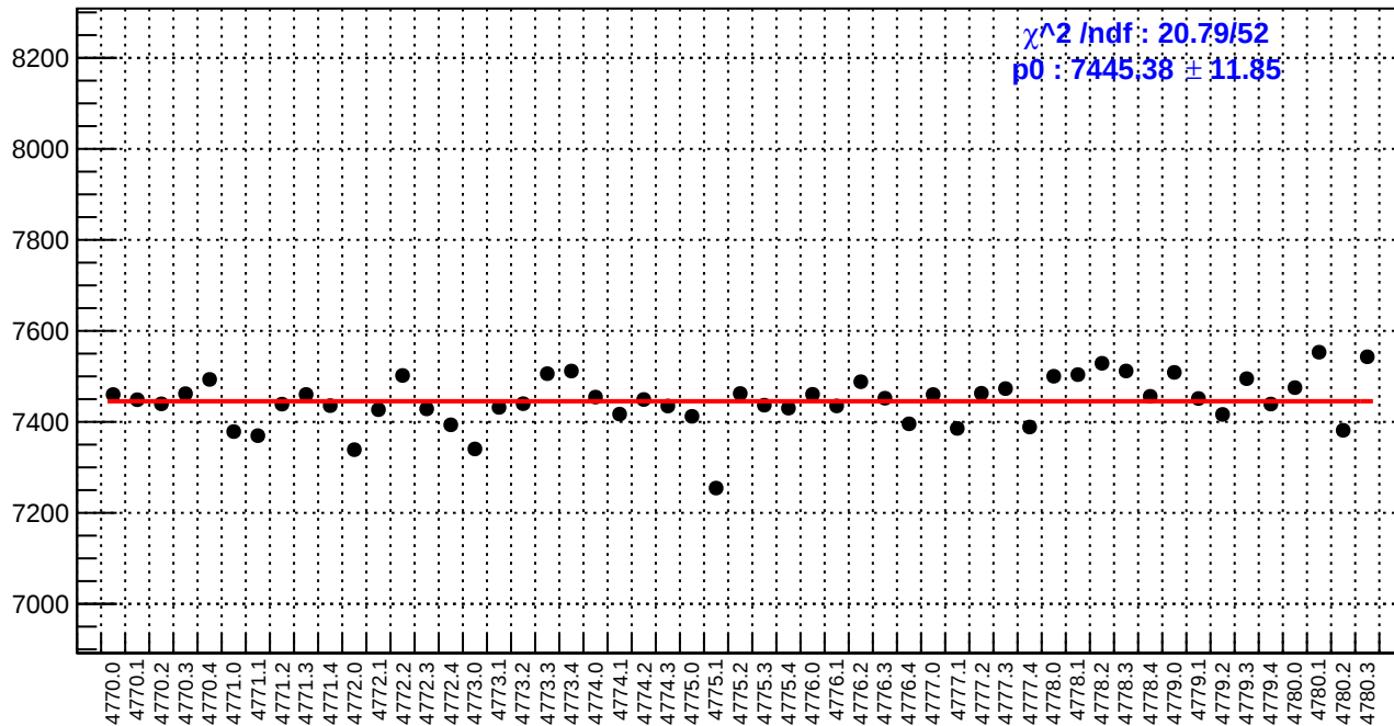
slug80: reg_asym_atl2.rms/ppm
