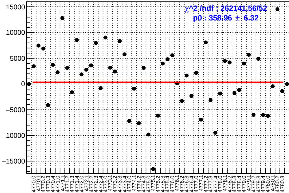
slug80: asym_atr_avg.mean/ppb-reg_asym_atr_avg.mean/ppb
