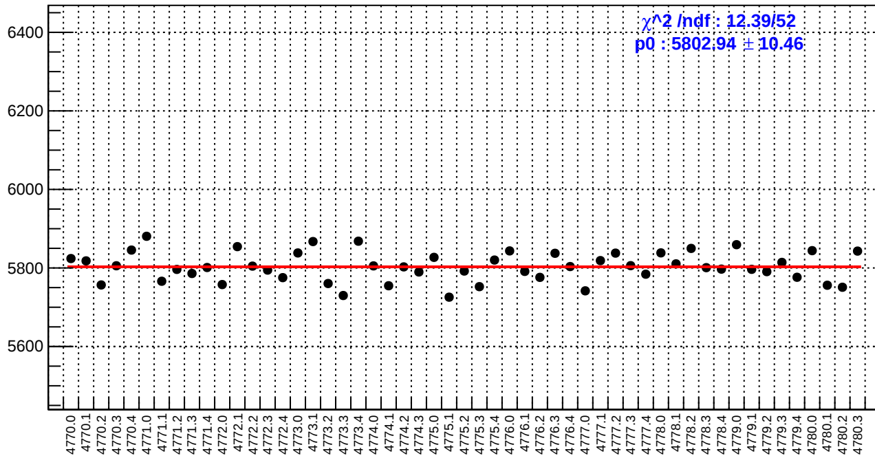
slug80: reg_asym_atr1l2_dd.rms/ppm
