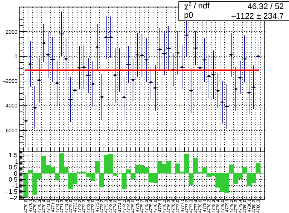
slug80: reg_asym_sam1.mean/ppb
