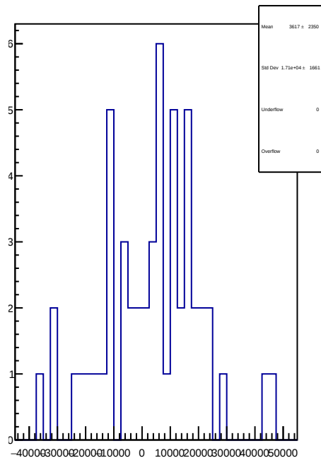
slug80: 1D Corr asym_sam7.mean/ppb-reg_asym_sam7.mean/ppb
