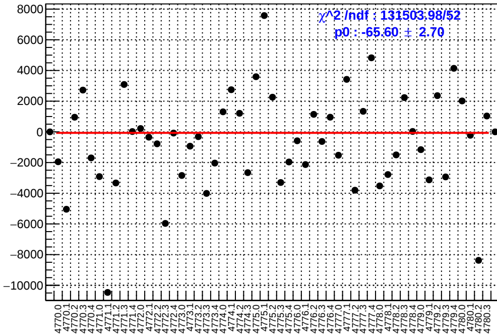
slug80: asym_atr_dd.mean/ppb-reg_asym_atr_dd.mean/ppb
