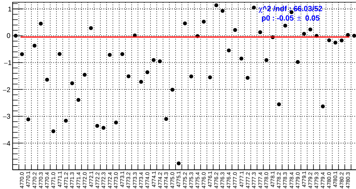
slug80: ds_avg_bpm4aY/(ppb/nm)
