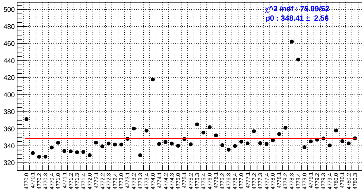
slug80: reg_asym_sam7.rms/ppm
