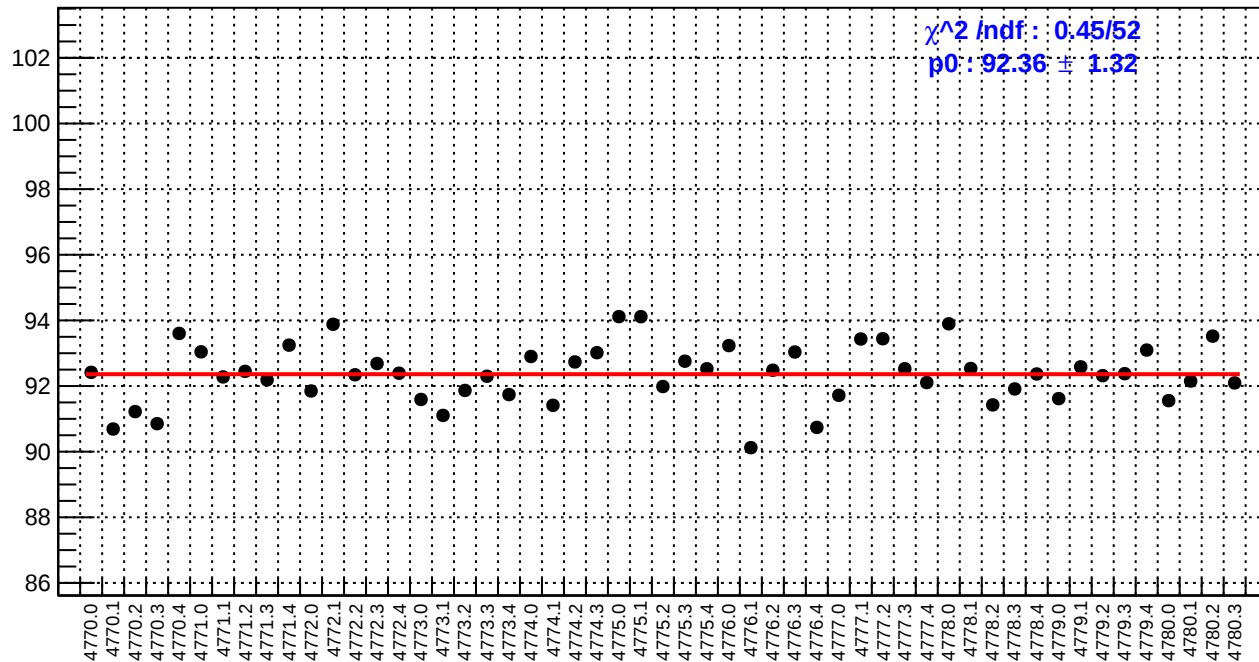
slug80: reg_asym_us_dd.rms/ppm
