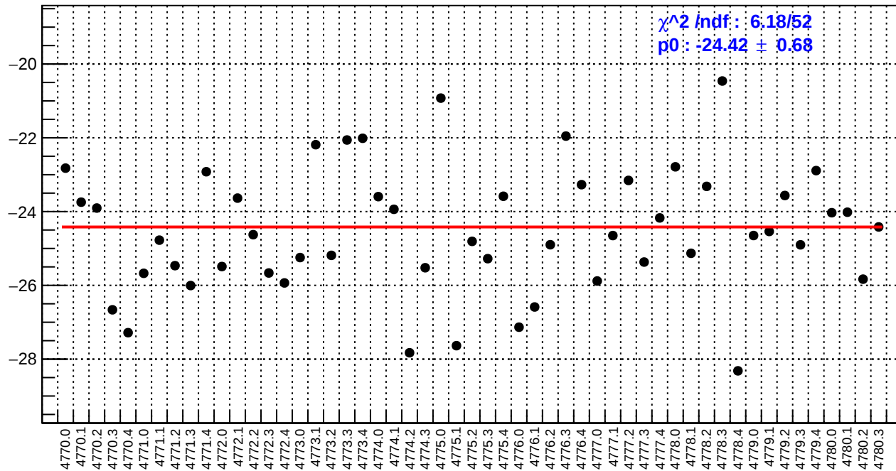
slug80: right_avg_bpm4aX/(ppb/nm)
