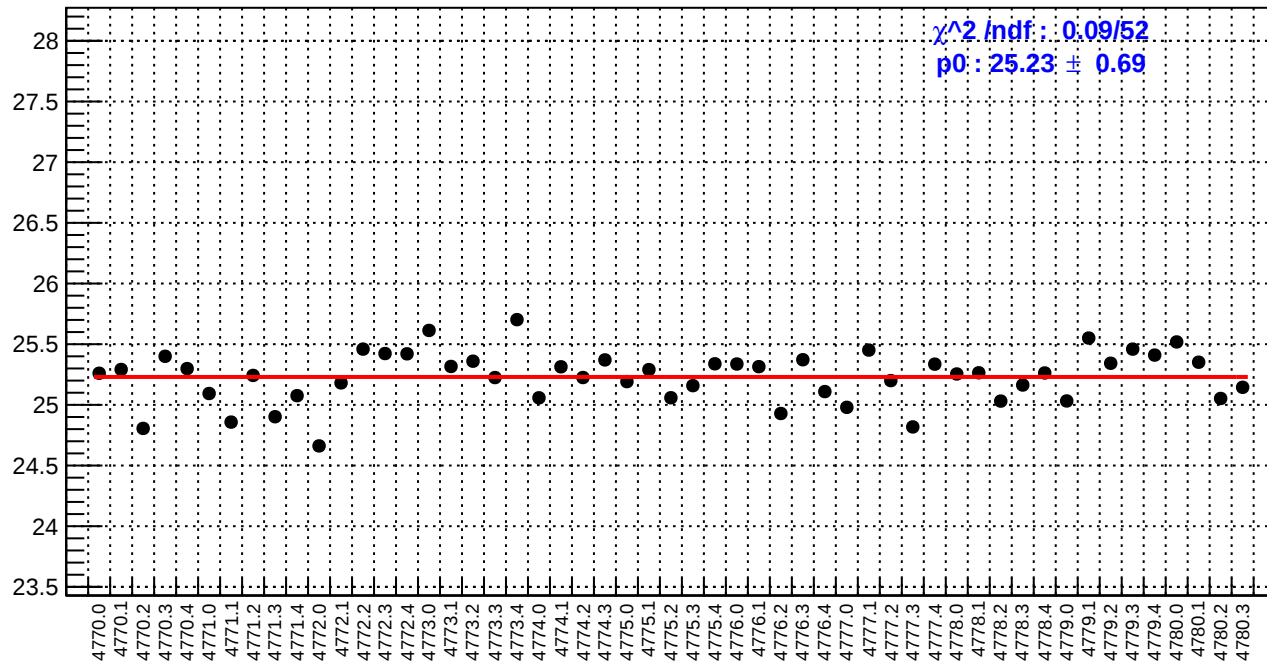
slug80: reg_asym_left_dd.rms/ppm
