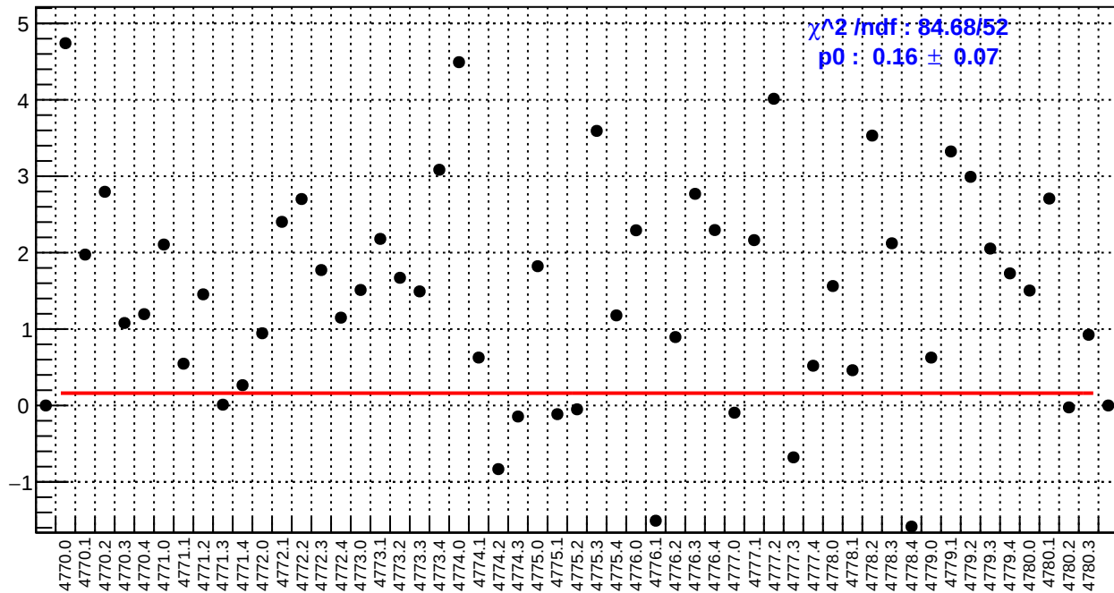
slug80: us_avg_bpm4aX/(ppb/nm)
