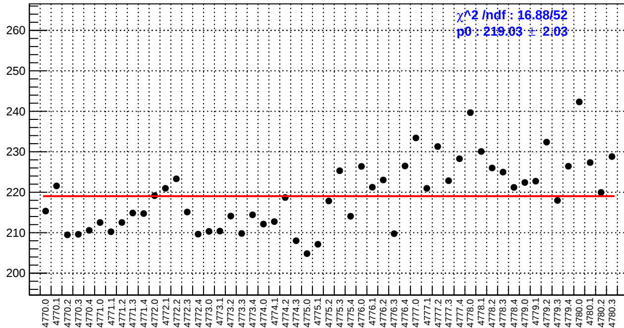
slug80: asym_bcm_an_ds.rms/ppm
