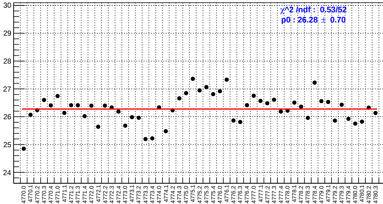
slug80: right_avg_bpm4eX/(ppb/nm)
