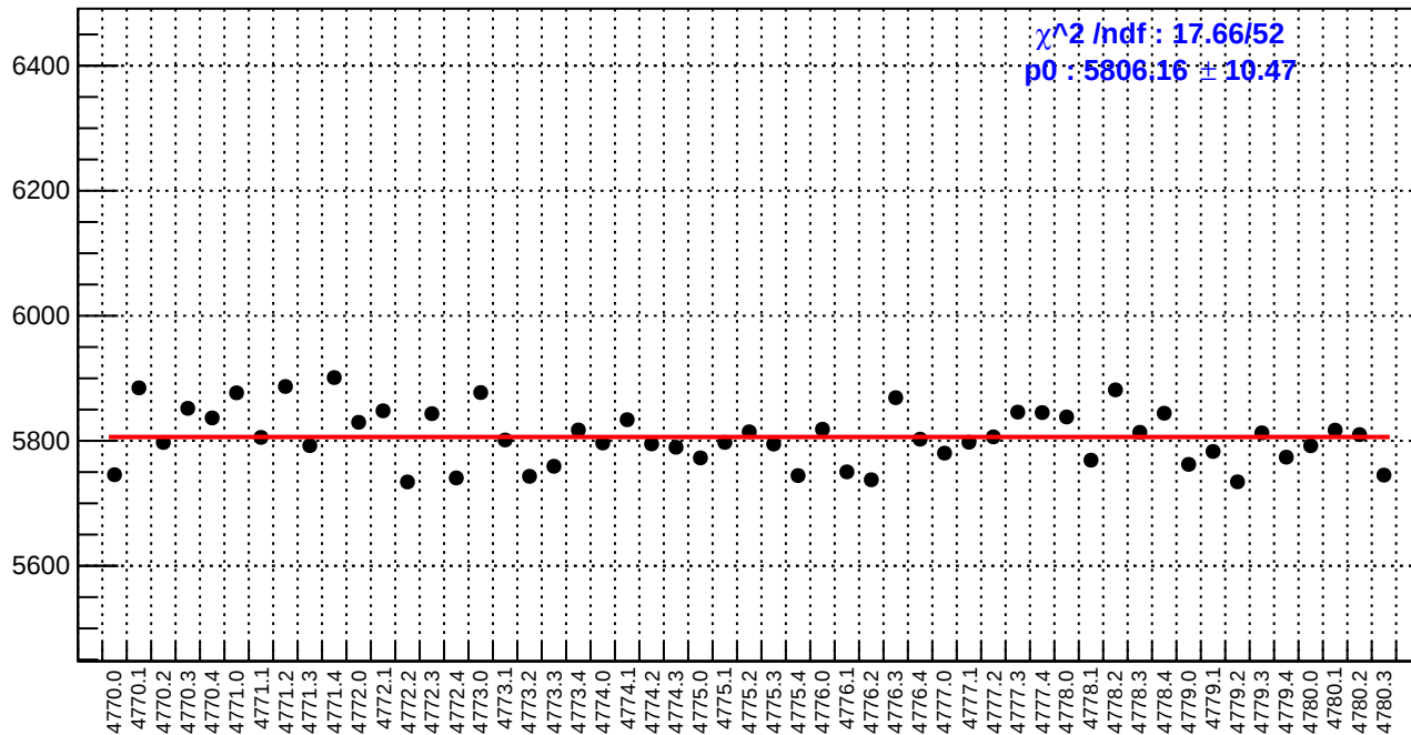
slug80: reg_asym_atr_dd.rms/ppm
