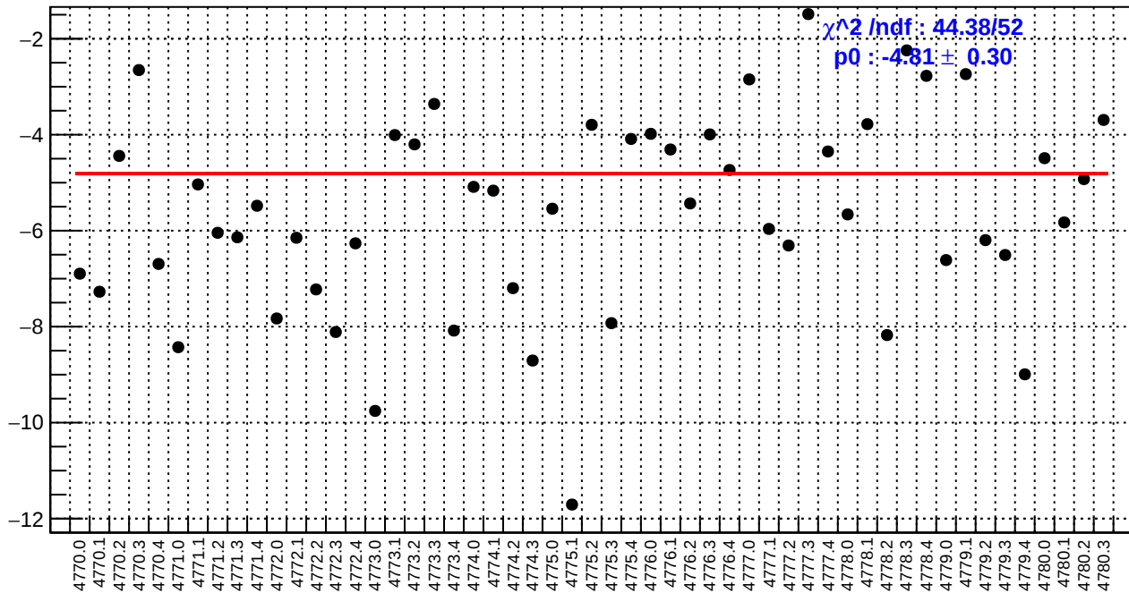
slug80: left_avg_bpm4aY/(ppb/nm)
