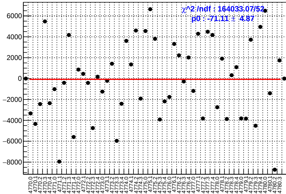
slug80: asym_atl1.mean/ppb-reg_asym_atl1.mean/ppb
