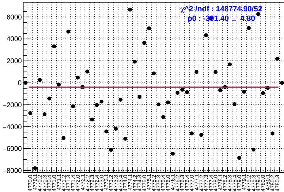
slug80: asym_sam5.mean/ppb-reg_asym_sam5.mean/ppb
