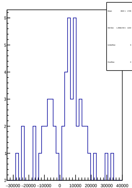
slug80: 1D Corr asym_sam8.mean/ppb-reg_asym_sam8.mean/ppb
