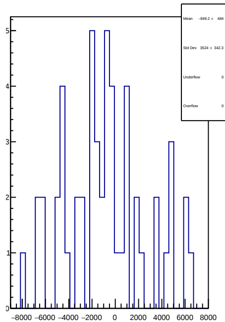
slug80: 1D Corr asym_sam5.mean/ppb-reg_asym_sam5.mean/ppb
