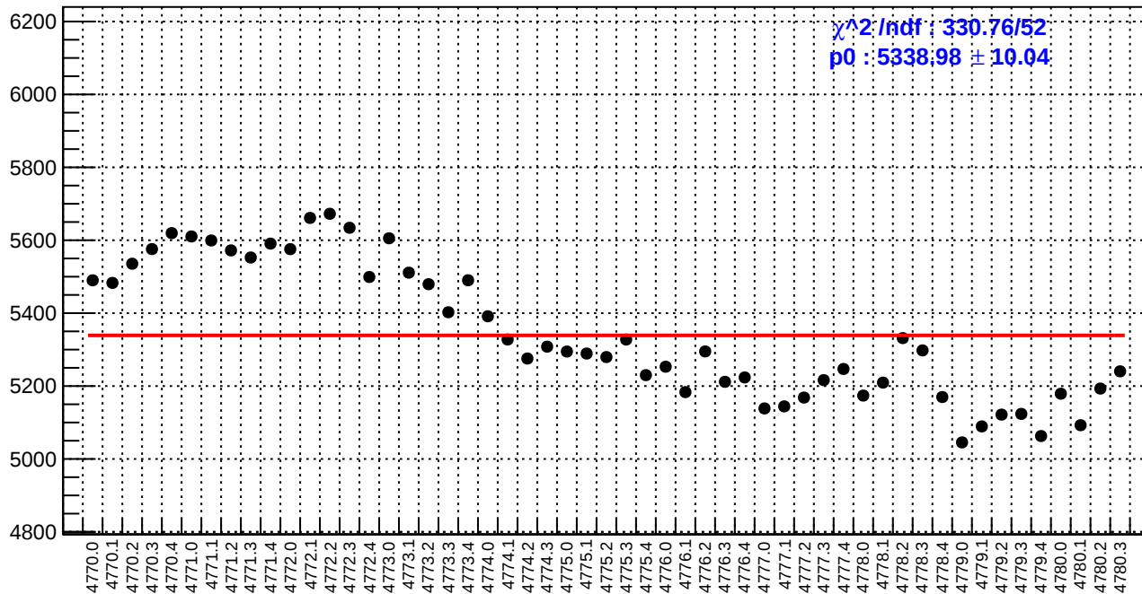
slug80: diff_bpm11X.rms/nm
