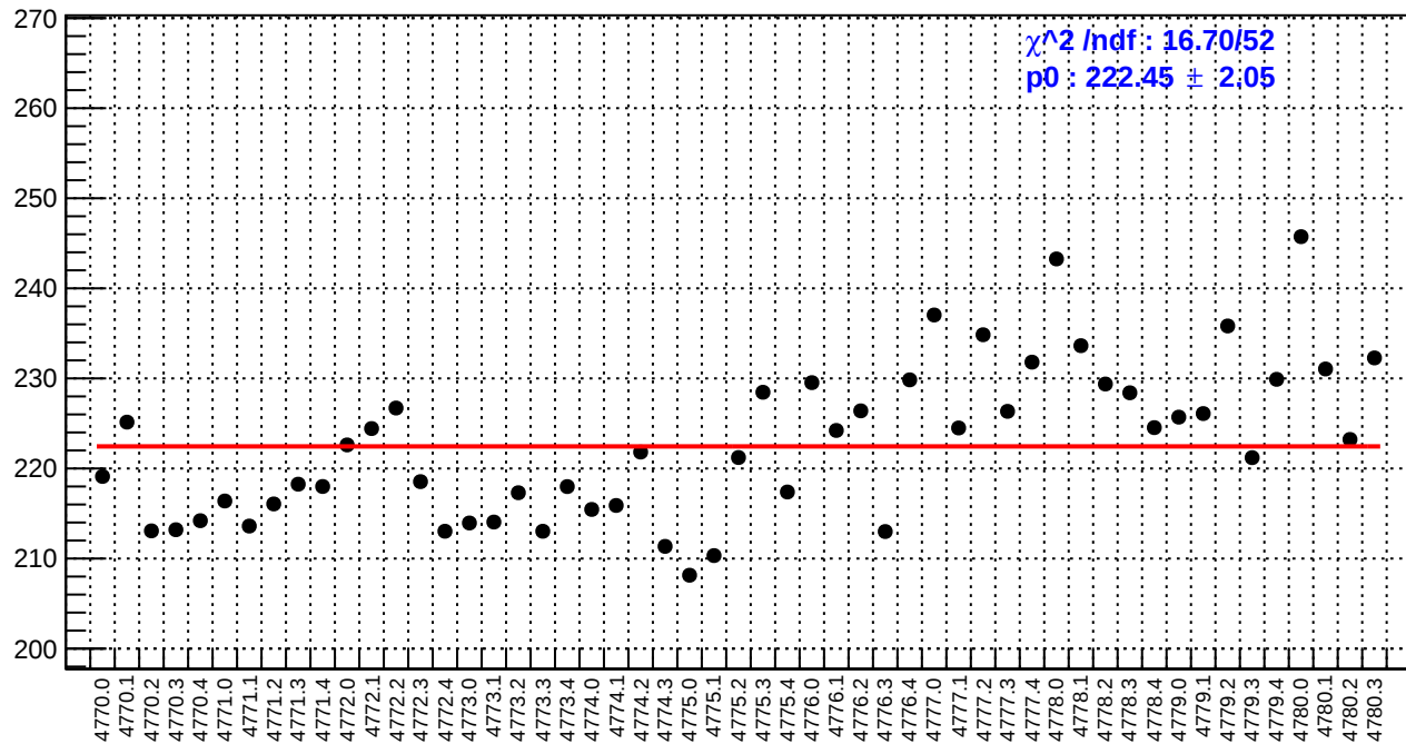
slug80: asym_bcm_an_ds3.rms/ppm
