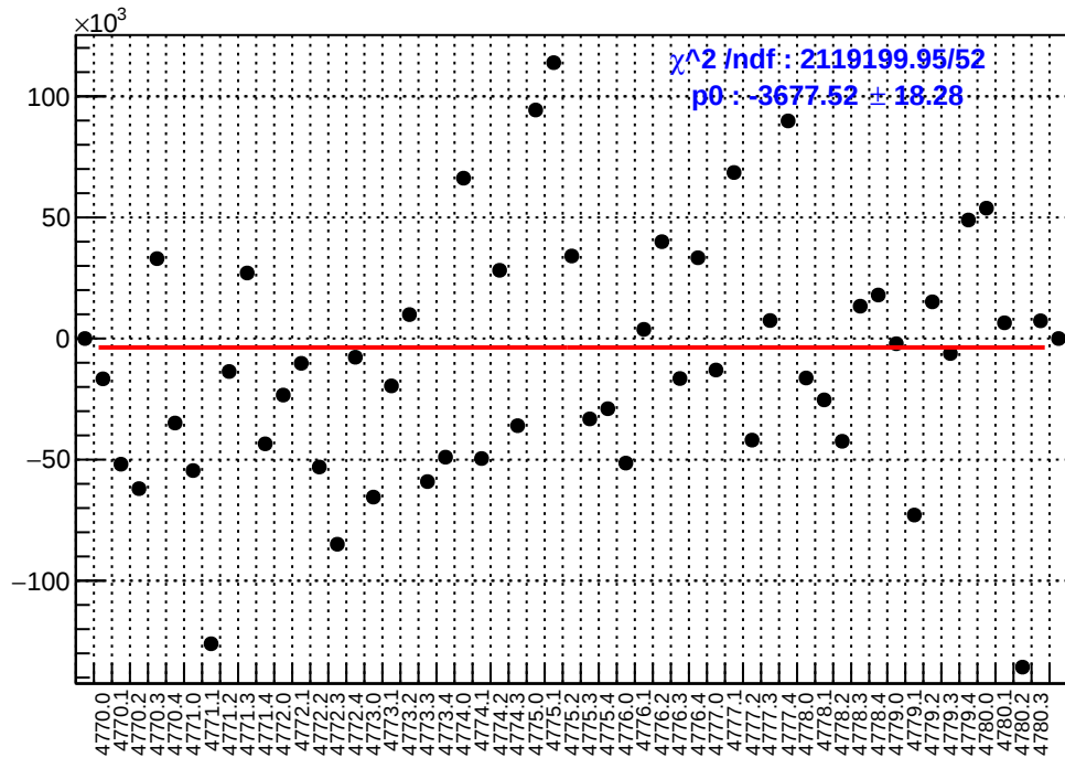
slug80: asym_sam2.mean/ppb-reg_asym_sam2.mean/ppb
