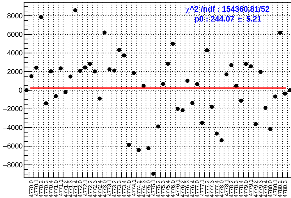
slug80: asym_atr1.mean/ppb-reg_asym_atr1.mean/ppb
