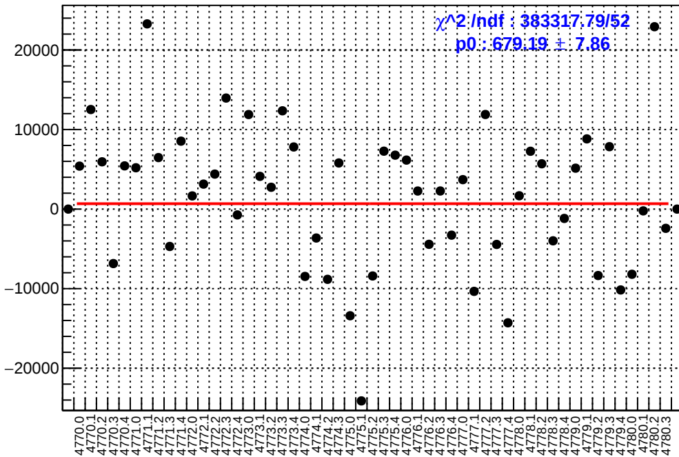
slug80: asym_atr2.mean/ppb-reg_asym_atr2.mean/ppb
