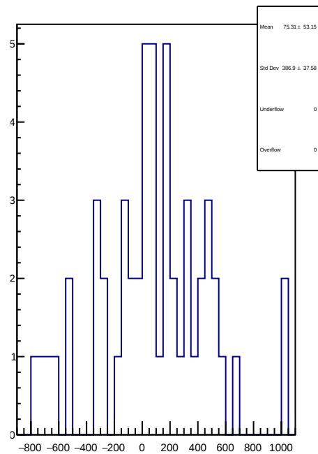
slug80: 1D Corr asym_right_dd.mean/ppb-reg_asym_right_dd.mean/ppb
