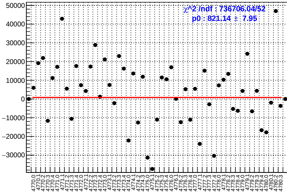
slug80: asym_sam7.mean/ppb-reg_asym_sam7.mean/ppb
