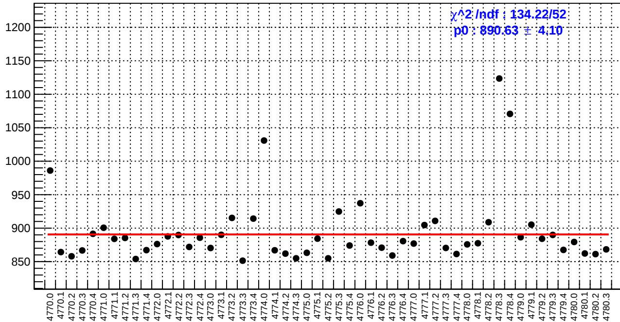
slug80: reg_asym_sam3.rms/ppm
