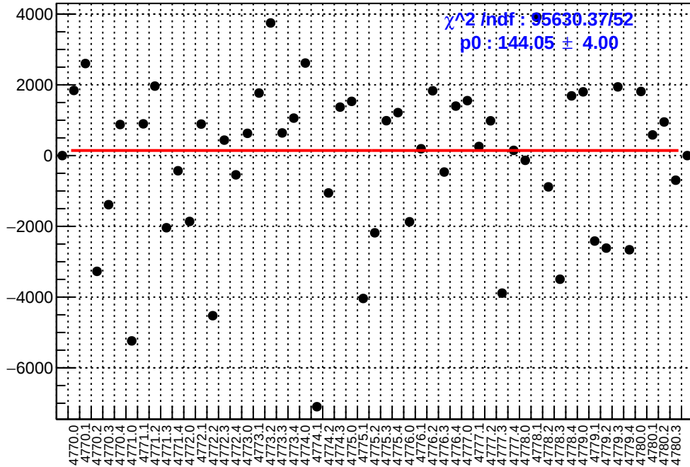
slug80: asym_at2_avg.mean/ppb-reg_asym_at2_avg.mean/ppb
