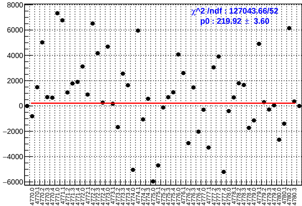
slug80: asym_atl_dd.mean/ppb-reg_asym_atl_dd.mean/ppb
