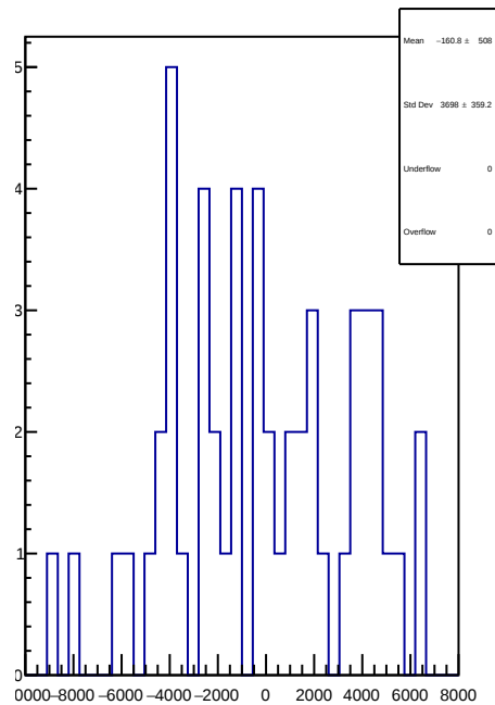
slug80: 1D Corr asym_atl1.mean/ppb-reg_asym_atl1.mean/ppb
