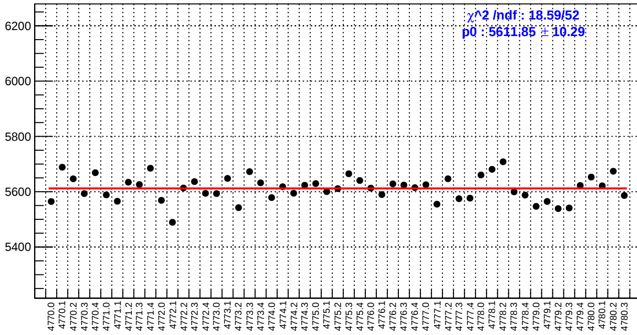
slug80: reg_asym_atl1r2_dd.rms/ppm
