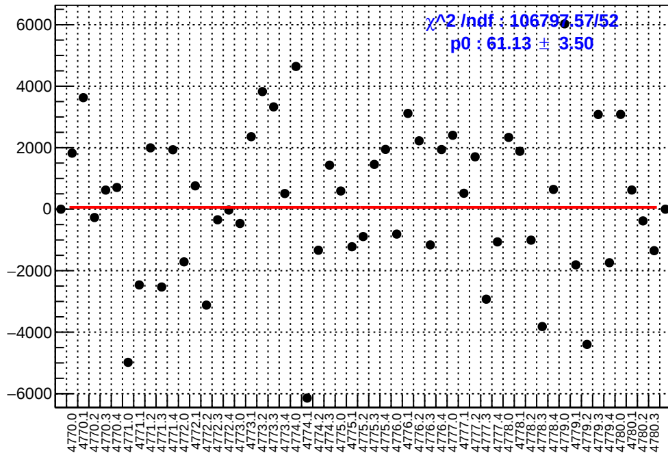
slug80: asym_us_avg.mean/ppb-reg_asym_us_avg.mean/ppb
