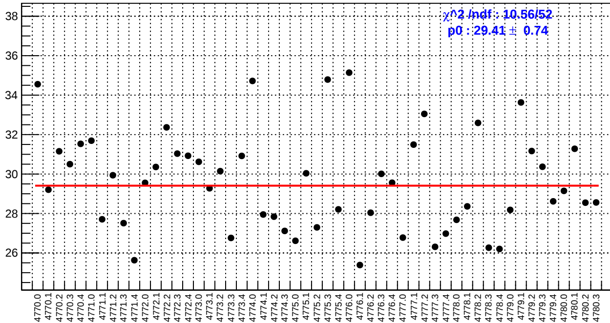
slug80: left_avg_bpm4aX/(ppb/nm)
