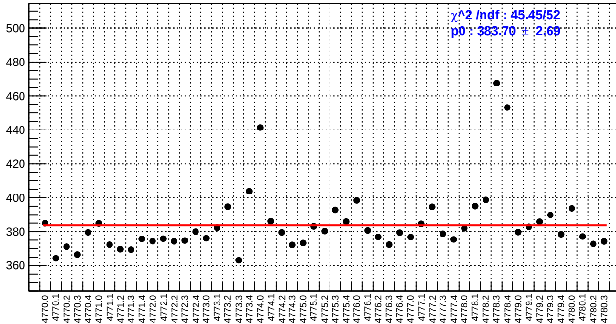
slug80: reg_asym_sam6.rms/ppm
