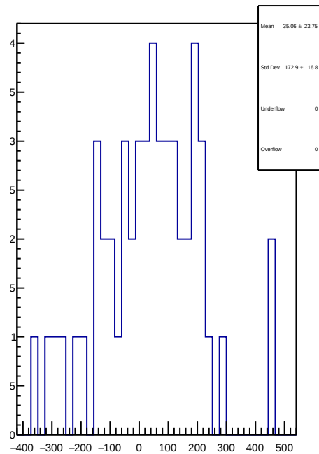
slug80: 1D Corr asym_left_dd.mean/ppb-reg_asym_left_dd.mean/ppb
