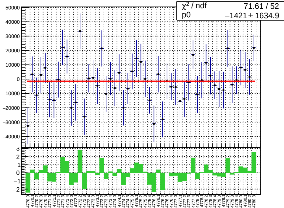
slug80: reg_asym_sam4.mean/ppb
