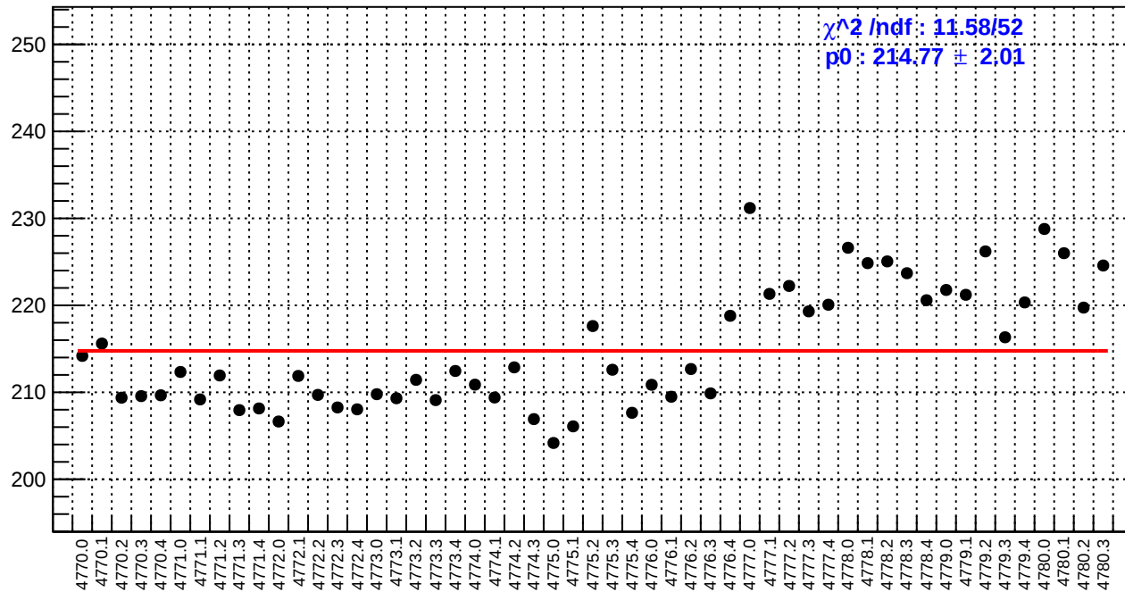
slug80: asym_bcm_an_us.rms/ppm
