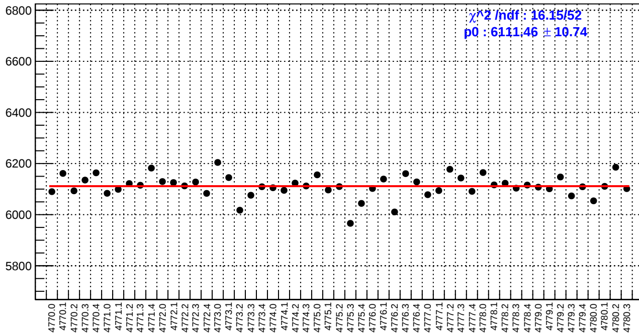
slug80: reg_asym_at1_dd.rms/ppm
