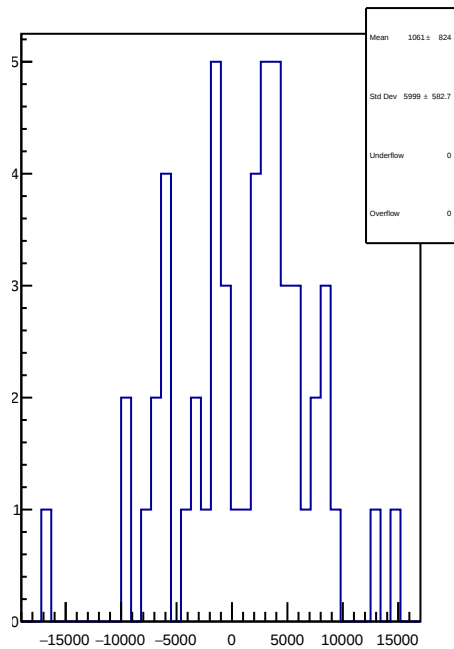
slug80: 1D Corr asym_atr_avg.mean/ppb-reg_asym_atr_avg.mean/ppb
