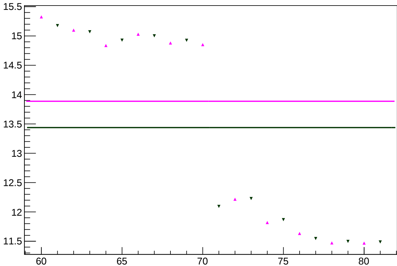
yield_sam7_mean vs slug
