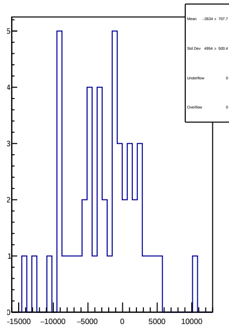
slug81: 1D Corr asym_usr.mean/ppb-reg_asym_usr.mean/ppb
