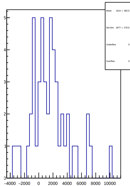
slug81: 1D Corr asym_atr_dd.mean/ppb-reg_asym_atr_dd.mean/ppb
