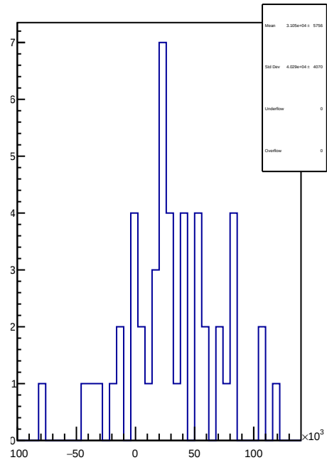
slug81: 1D Corr asym_sam2.mean/ppb-reg_asym_sam2.mean/ppb
