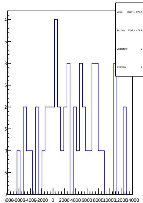
slug81: 1D Corr asym_left_avg.mean/ppb-reg_asym_left_avg.mean/ppb
