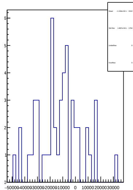
slug81: 1D Corr asym_sam6.mean/ppb-reg_asym_sam6.mean/ppb
