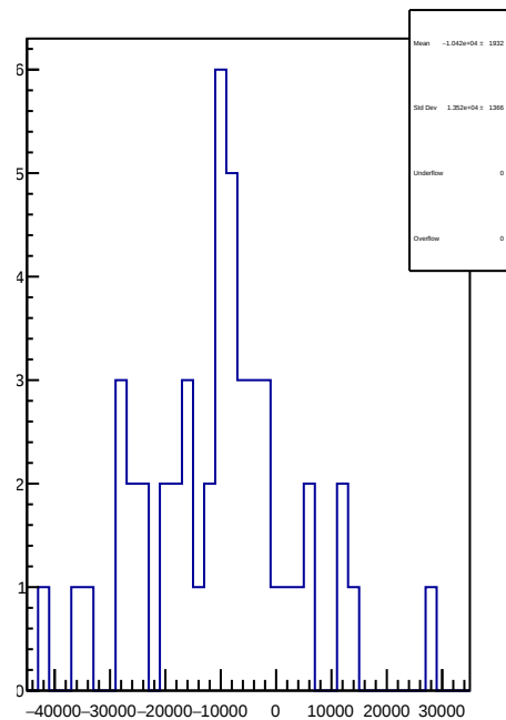
slug81: 1D Corr asym_sam7.mean/ppb-reg_asym_sam7.mean/ppb
