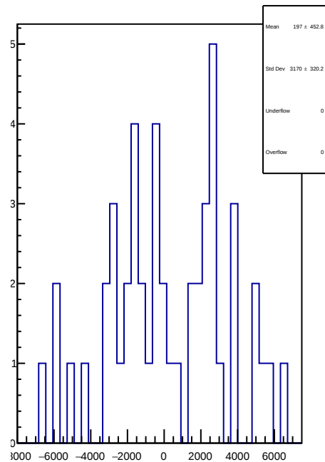
slug81: 1D Corr asym_us_avg.mean/ppb-reg_asym_us_avg.mean/ppb
