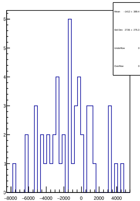
slug81: 1D Corr asym_atl_dd.mean/ppb-reg_asym_atl_dd.mean/ppb
