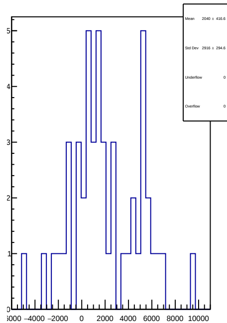
slug81: 1D Corr asym_at1_dd.mean/ppb-reg_asym_at1_dd.mean/ppb
