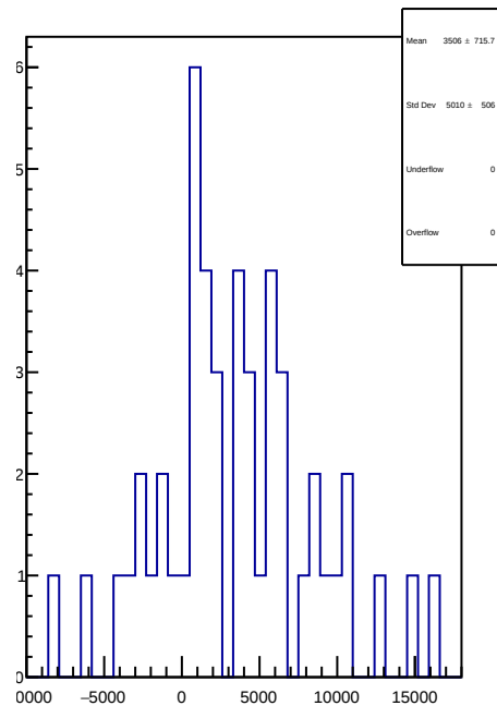
slug81: 1D Corr asym_atl_avg.mean/ppb-reg_asym_atl_avg.mean/ppb
