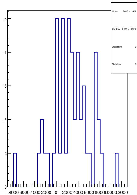
slug81: 1D Corr asym_ds_dd.mean/ppb-reg_asym_ds_dd.mean/ppb
