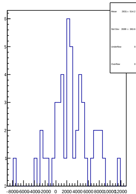
slug81: 1D Corr asym_us_dd.mean/ppb-reg_asym_us_dd.mean/ppb
