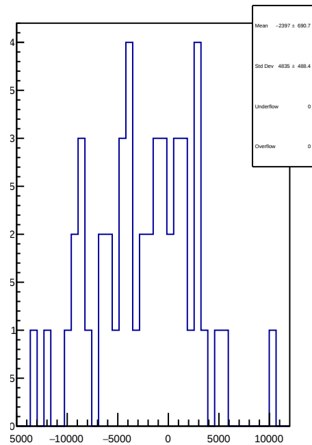
slug81: 1D Corr asym_right_avg.mean/ppb-reg_asym_right_avg.mean/ppb
