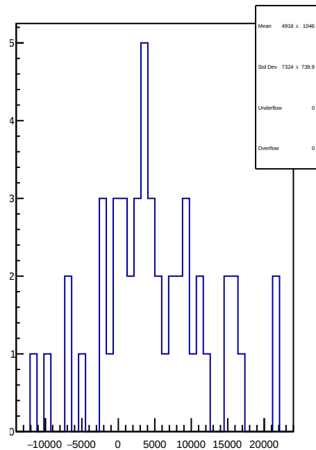
slug81: 1D Corr asym_atl2.mean/ppb-reg_asym_atl2.mean/ppb
