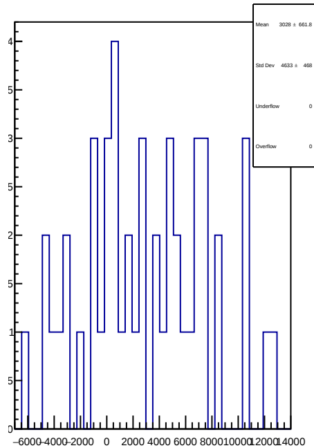
slug81: 1D Corr asym_usl.mean/ppb-reg_asym_usl.mean/ppb
