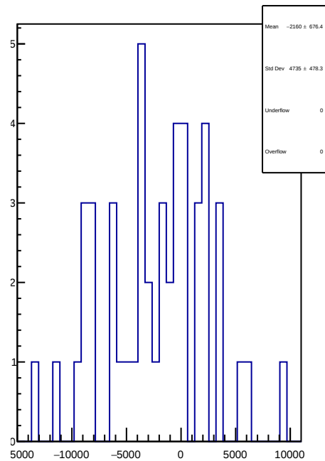
slug81: 1D Corr asym_dsr.mean/ppb-reg_asym_dsr.mean/ppb
