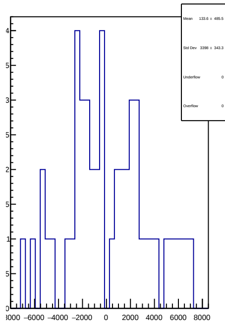
slug81: 1D Corr asym_sam1.mean/ppb-reg_asym_sam1.mean/ppb
