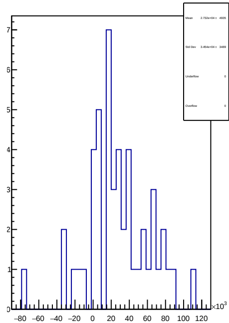
slug81: 1D Corr asym_sam4.mean/ppb-reg_asym_sam4.mean/ppb
