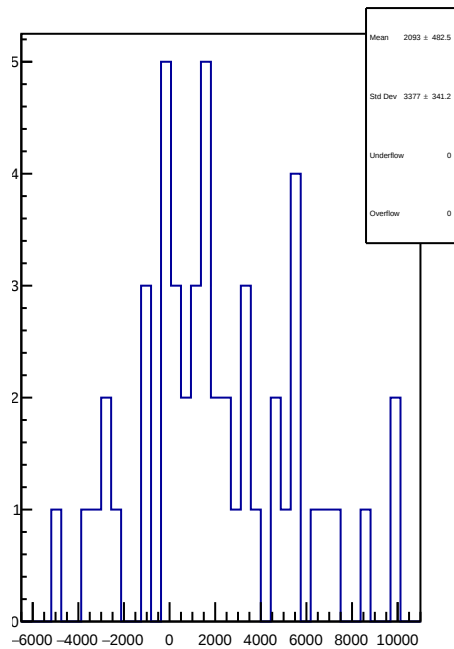
slug81: 1D Corr asym_atl1.mean/ppb-reg_asym_atl1.mean/ppb
