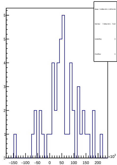
slug81: 1D Corr asym_sam3.mean/ppb-reg_asym_sam3.mean/ppb
