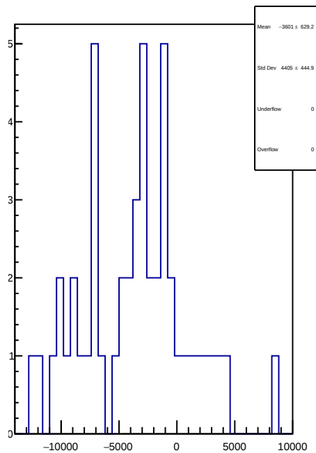
slug81: 1D Corr asym_atr_avg.mean/ppb-reg_asym_atr_avg.mean/ppb
