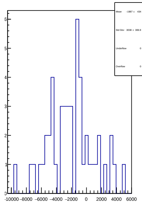
slug81: 1D Corr asym_atr1.mean/ppb-reg_asym_atr1.mean/ppb
