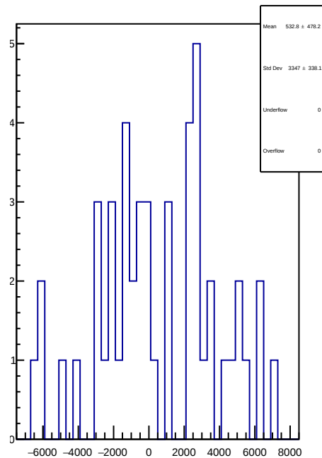
slug81: 1D Corr asym_ds_avg.mean/ppb-reg_asym_ds_avg.mean/ppb
