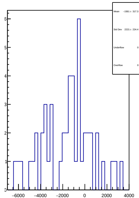
slug81: 1D Corr asym_atl1r2_avg.mean/ppb-reg_asym_atl1r2_avg.mean/ppb
