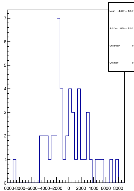
slug81: 1D Corr asym_at2_avg.mean/ppb-reg_asym_at2_avg.mean/ppb
