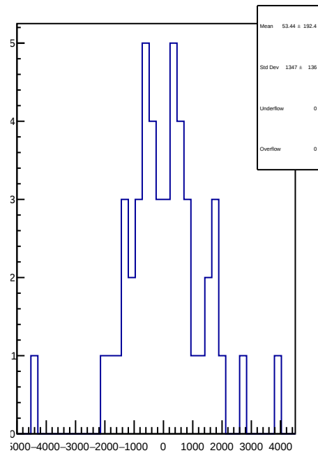
slug81: 1D Corr asym_at1_avg.mean/ppb-reg_asym_at1_avg.mean/ppb
