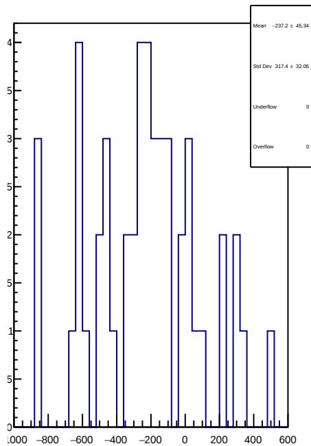
slug81: 1D Corr asym_right_dd.mean/ppb-reg_asym_right_dd.mean/ppb
