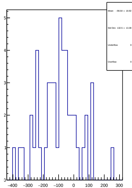
slug81: 1D Corr asym_left_dd.mean/ppb-reg_asym_left_dd.mean/ppb
