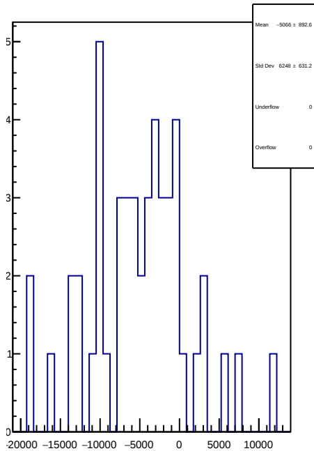
slug81: 1D Corr asym_at2_dd.mean/ppb-reg_asym_at2_dd.mean/ppb
