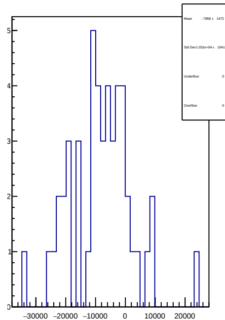
slug81: 1D Corr asym_sam8.mean/ppb-reg_asym_sam8.mean/ppb
