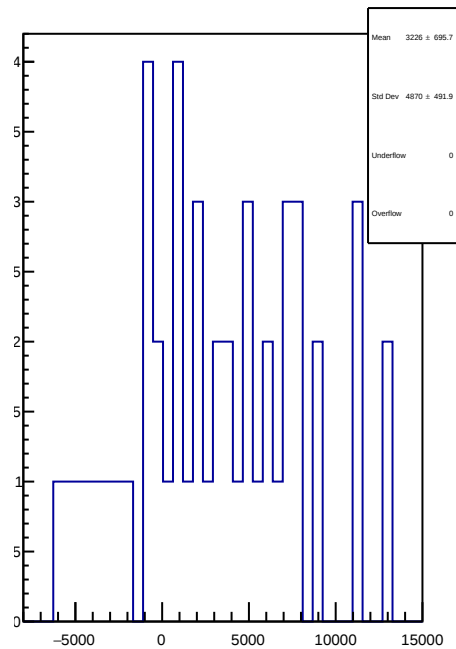
slug81: 1D Corr asym_dsl.mean/ppb-reg_asym_dsl.mean/ppb
