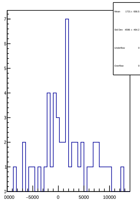
slug81: 1D Corr asym_sam5.mean/ppb-reg_asym_sam5.mean/ppb
