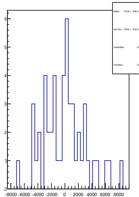
slug82: 1D Corr asym_atl_dd.mean/ppb-reg_asym_atl_dd.mean/ppb
