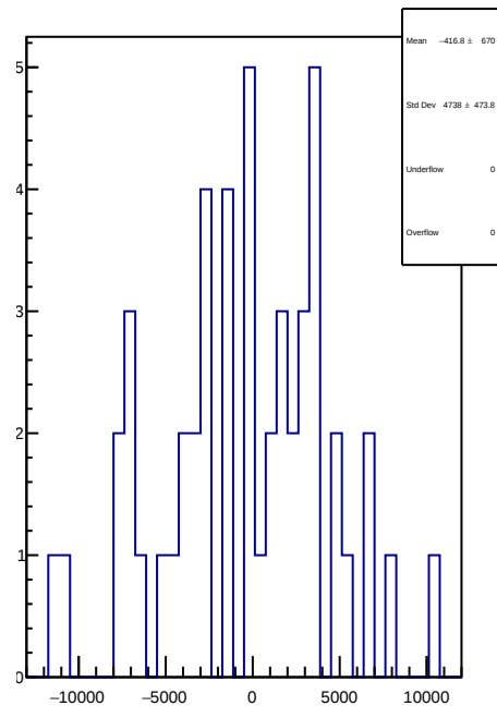
slug82: 1D Corr asym_right_avg.mean/ppb-reg_asym_right_avg.mean/ppb
