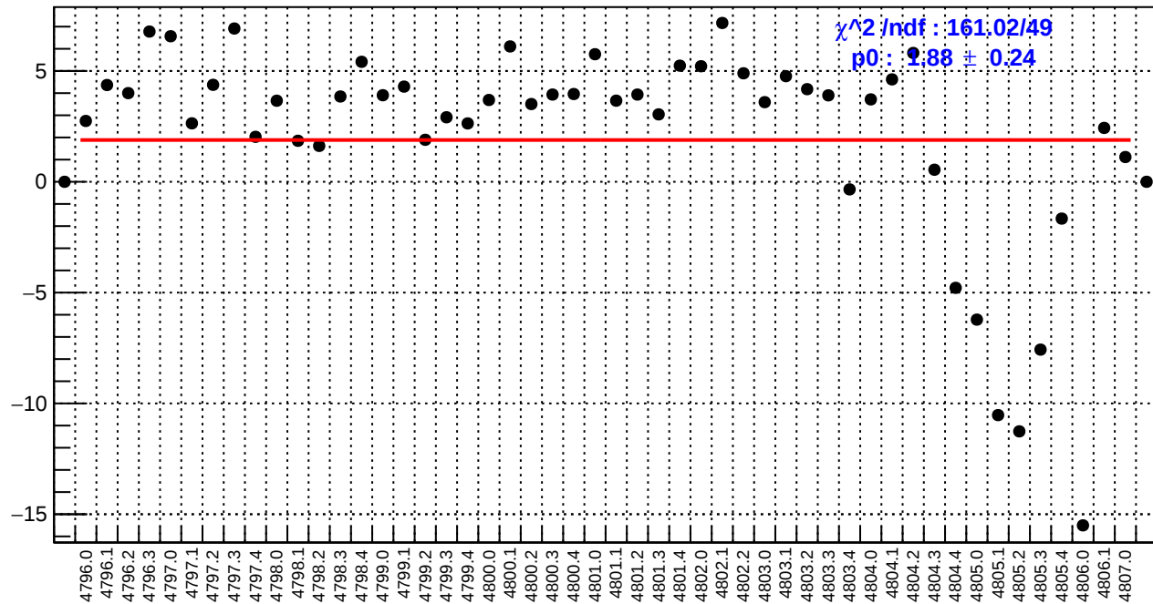
slug82: dsr_bpm4aY/(ppb/nm)
