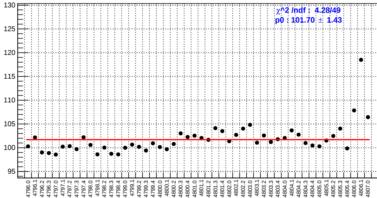
slug82: reg_asym_ds_avg.rms/ppm
