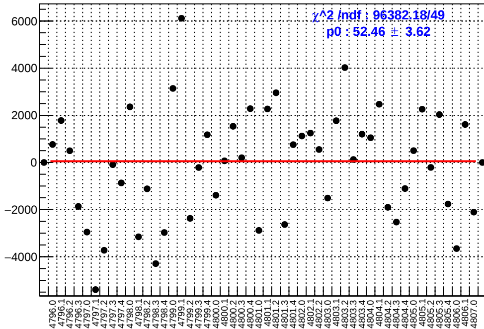
slug82: asym_at2_avg.mean/ppb-reg_asym_at2_avg.mean/ppb
