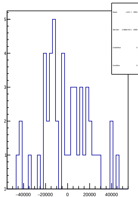
slug82: 1D Corr asym_sam6.mean/ppb-reg_asym_sam6.mean/ppb
