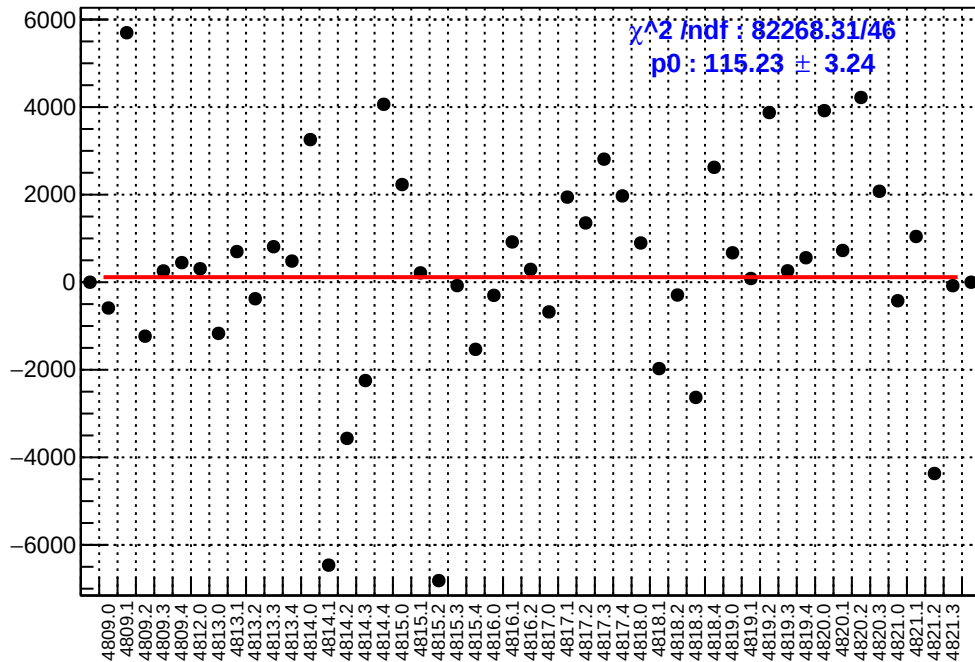
slug83: asym_at2_avg.mean/ppb-reg_asym_at2_avg.mean/ppb
