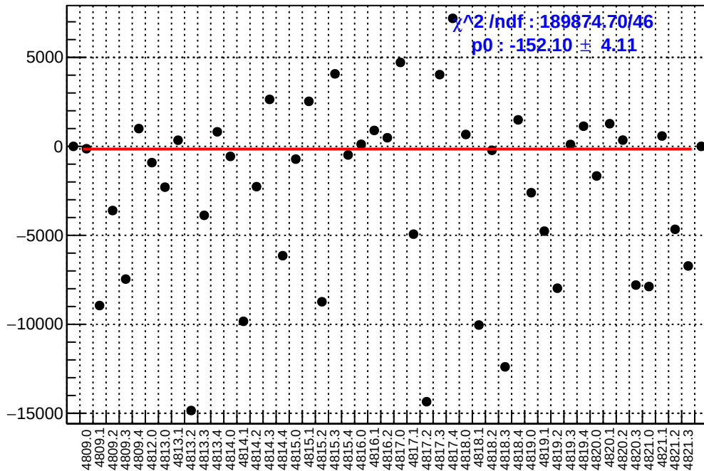
slug83: asym_atr2.mean/ppb-reg_asym_atr2.mean/ppb
