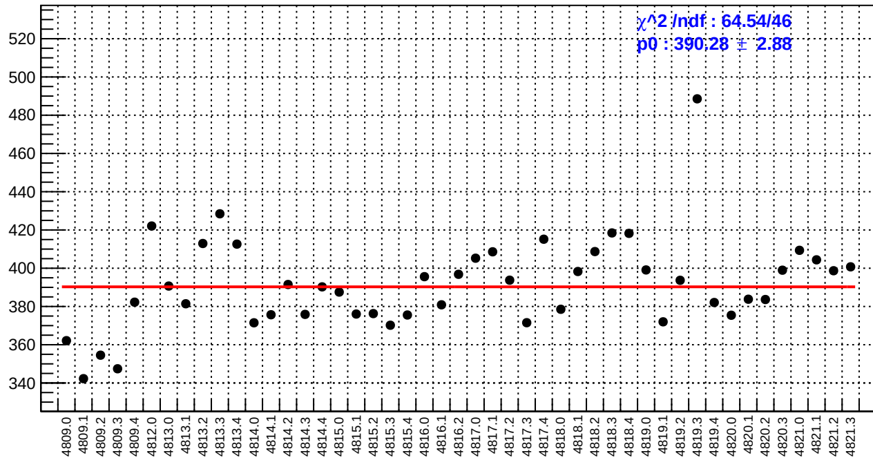
slug83: reg_asym_sam7.rms/ppm
