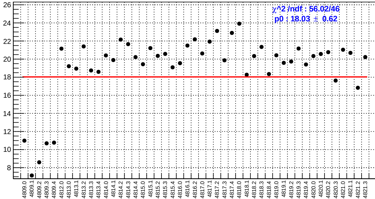
slug83: ds_avg_bpm4aX/(ppb/nm)
