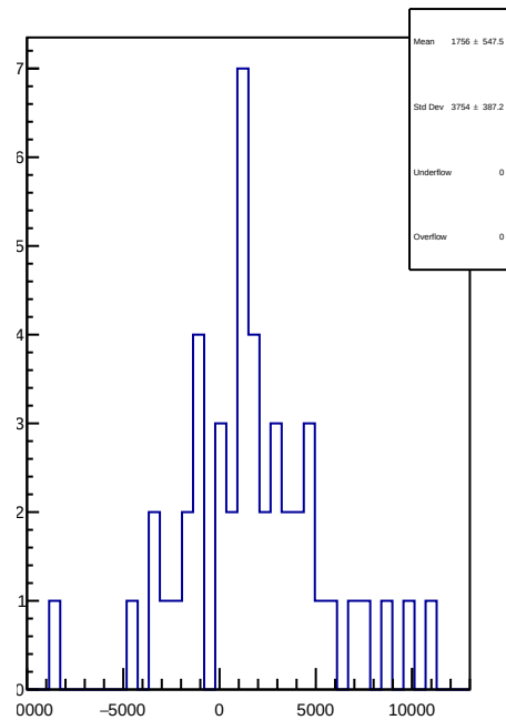
slug83: 1D Corr asym_sam5.mean/ppb-reg_asym_sam5.mean/ppb
