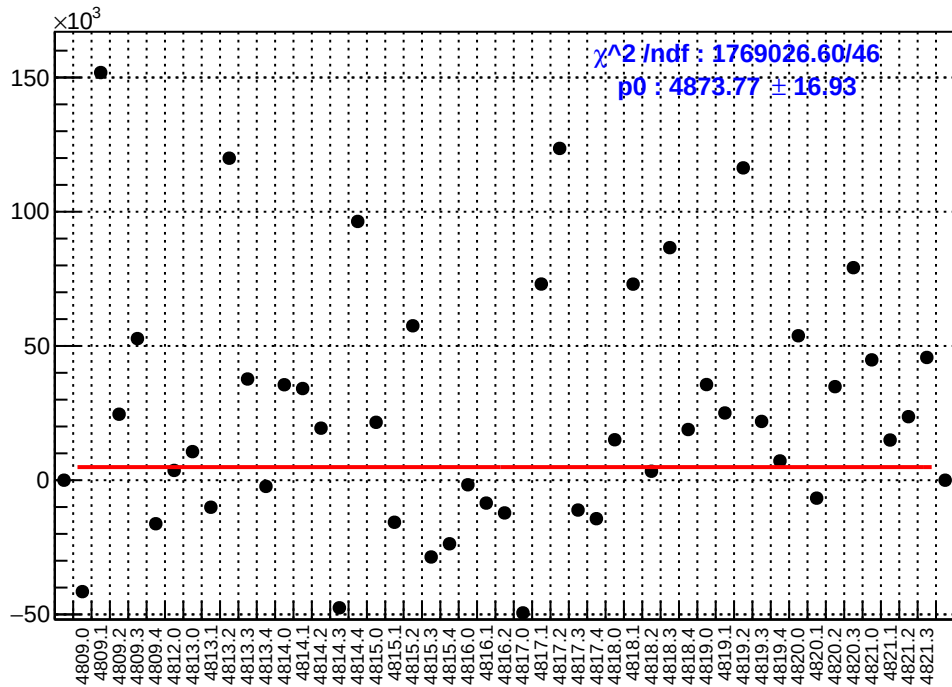
slug83: asym_sam2.mean/ppb-reg_asym_sam2.mean/ppb
