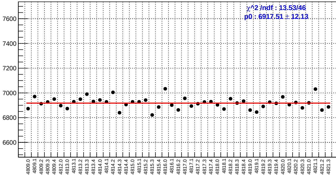
slug83: reg_asym_atr1l2_avg.rms/ppm
