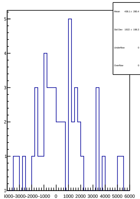
slug83: 1D Corr asym_atr_dd.mean/ppb-reg_asym_atr_dd.mean/ppb
