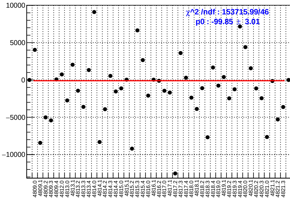
slug83: asym_usr.mean/ppb-reg_asym_usr.mean/ppb
