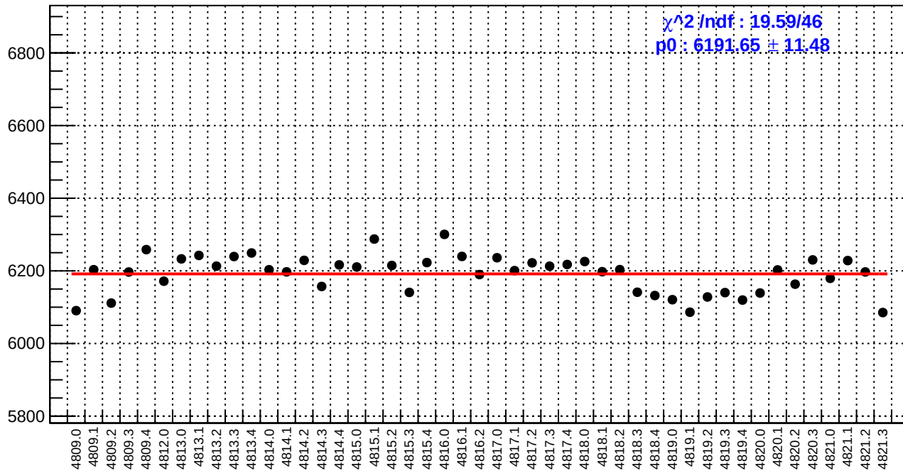
slug83: reg_asym_at1_avg.rms/ppm
