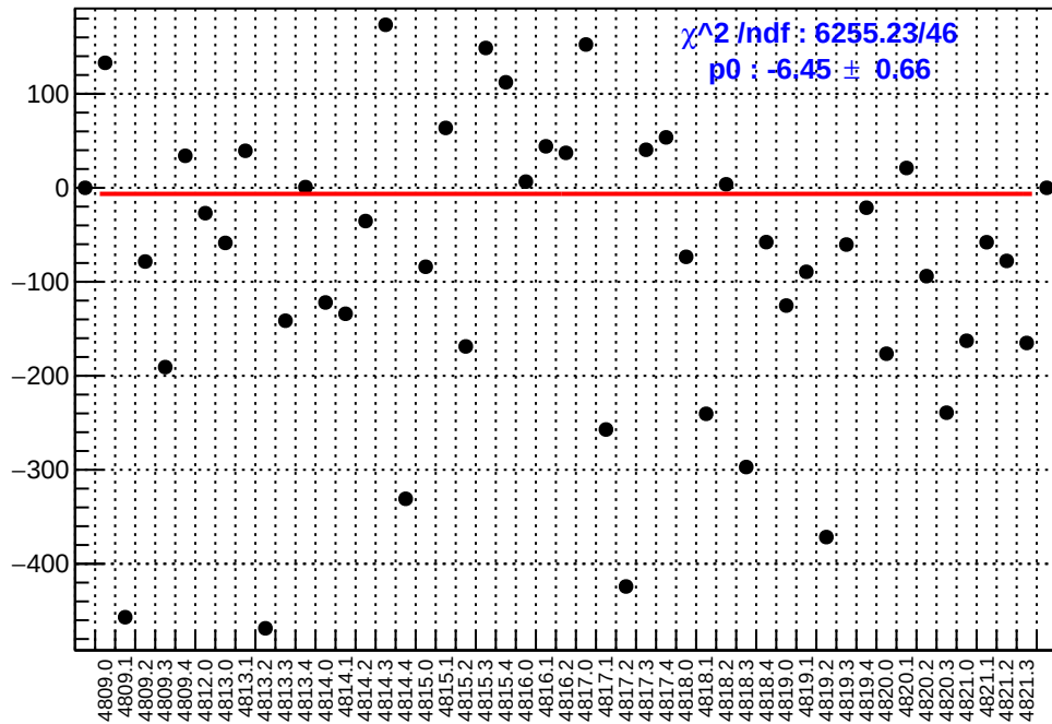
slug83: asym_left_dd.mean/ppb-reg_asym_left_dd.mean/ppb
