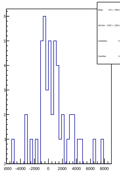
slug83: 1D Corr asym_atr1l2_avg.mean/ppb-reg_asym_atr1l2_avg.mean/ppb
