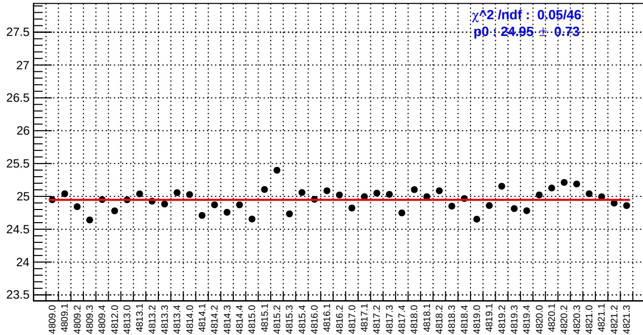
slug83: reg_asym_left_dd.rms/ppm
