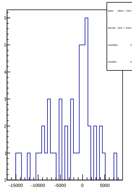
slug83: 1D Corr asym_atr2.mean/ppb-reg_asym_atr2.mean/ppb
