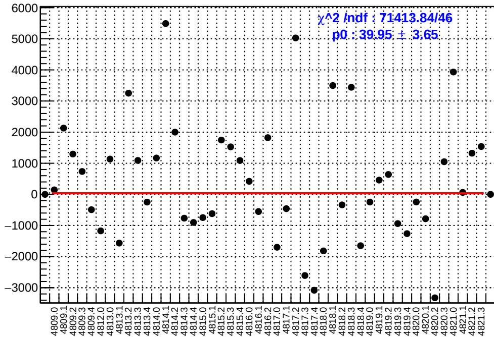
slug83: asym_atr_dd.mean/ppb-reg_asym_atr_dd.mean/ppb
