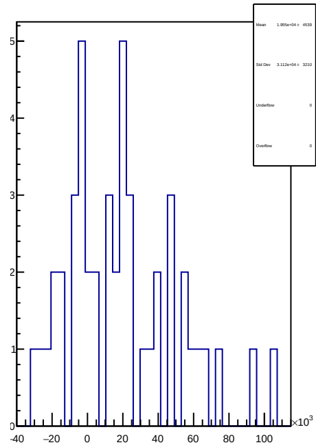
slug83: 1D Corr asym_sam4.mean/ppb-reg_asym_sam4.mean/ppb
