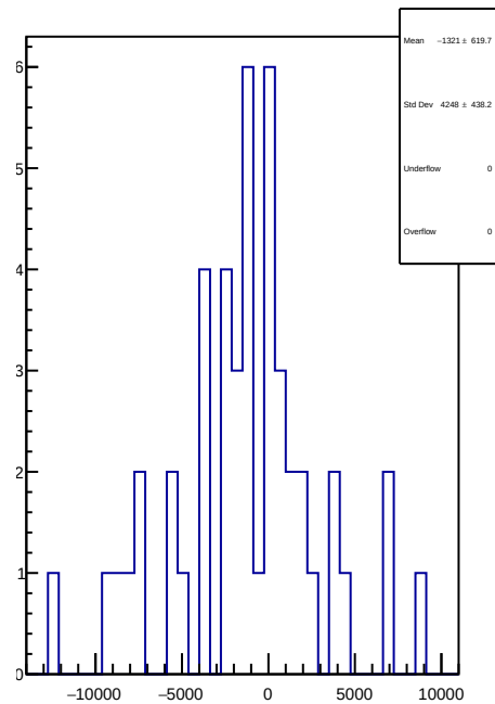
slug83: 1D Corr asym_usr.mean/ppb-reg_asym_usr.mean/ppb
