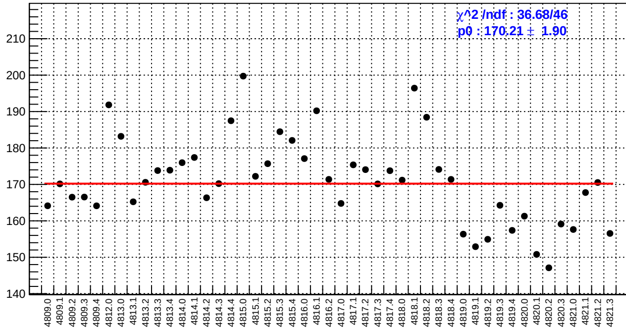
slug83: asym_bcm_an_ds.rms/ppm
