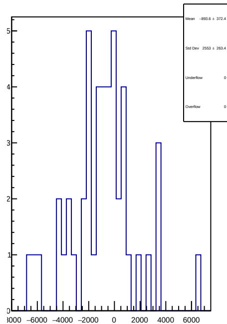
slug83: 1D Corr asym_atl_dd.mean/ppb-reg_asym_atl_dd.mean/ppb
