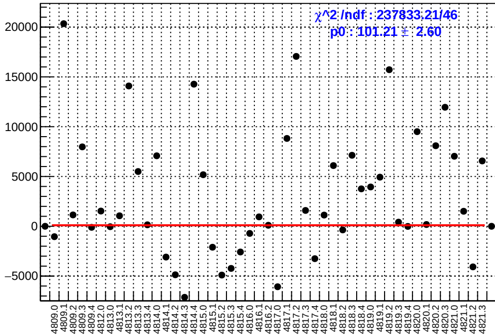
slug83: asym_atl2.mean/ppb-reg_asym_atl2.mean/ppb
