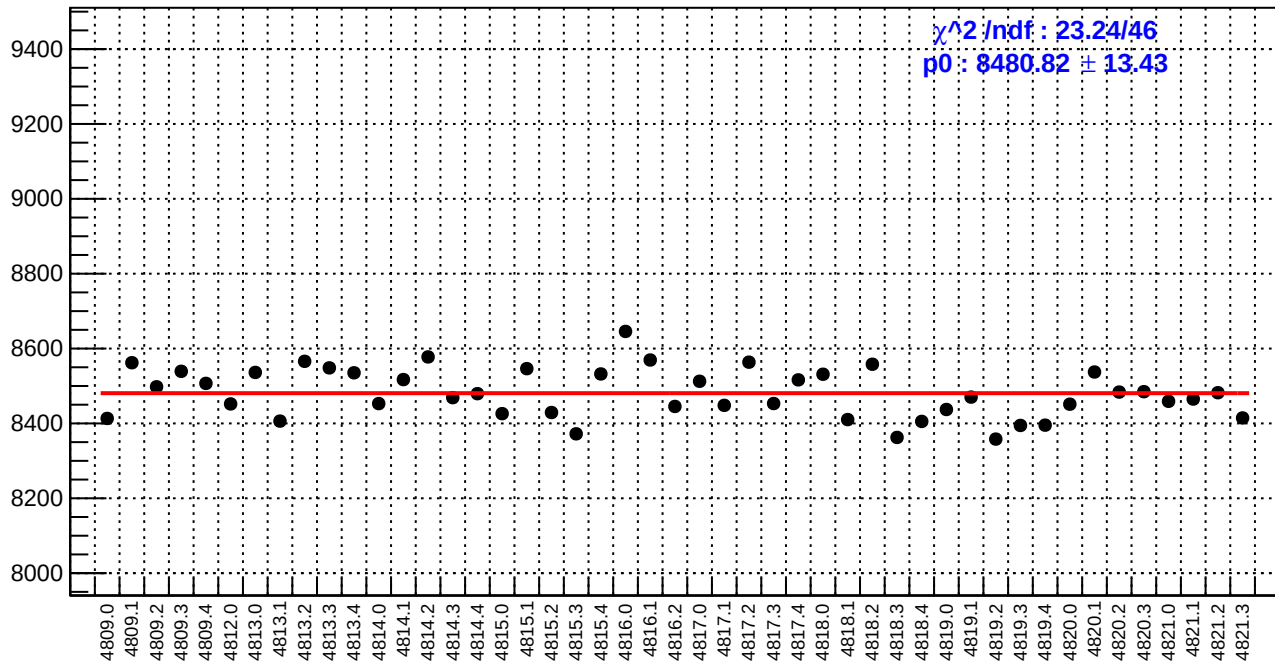
slug83: reg_asym_atl1.rms/ppm
