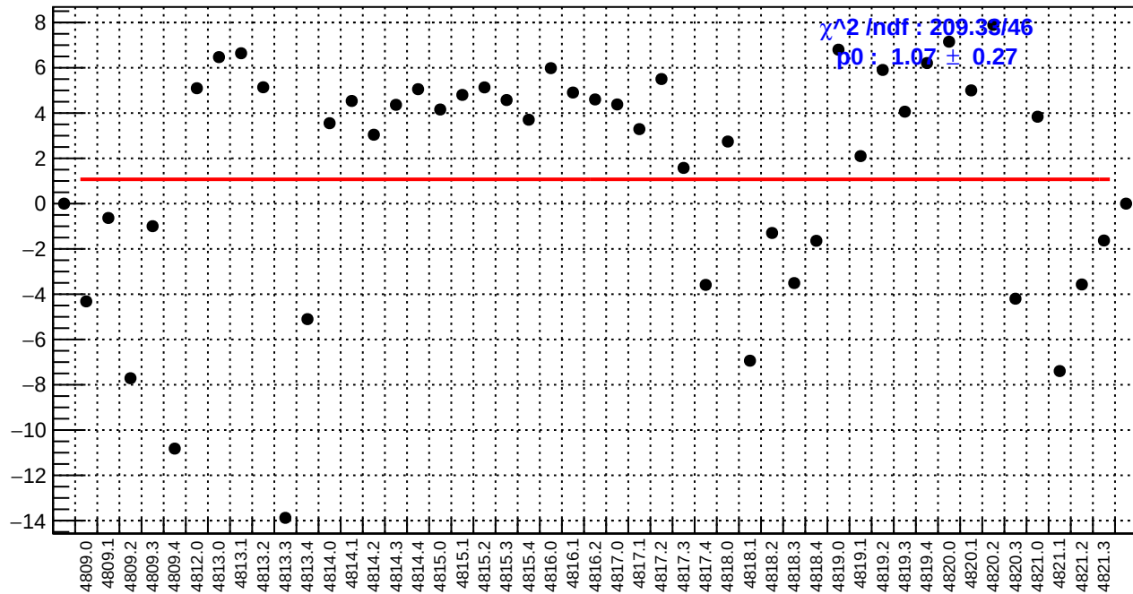
slug83: us_avg_bpm4eY/(ppb/nm)
