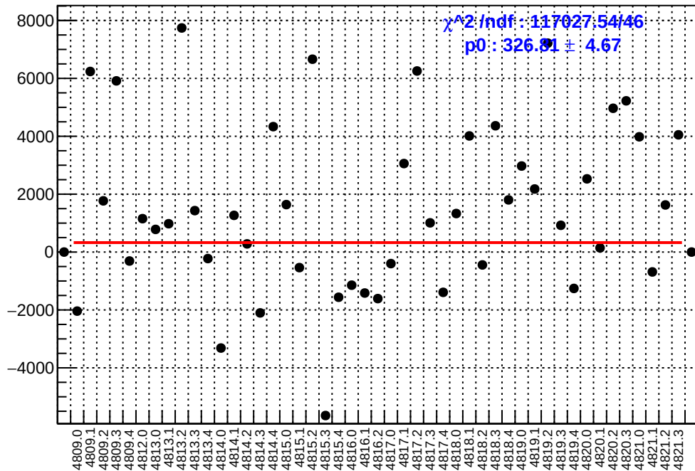
slug83: asym_at1_dd.mean/ppb-reg_asym_at1_dd.mean/ppb
