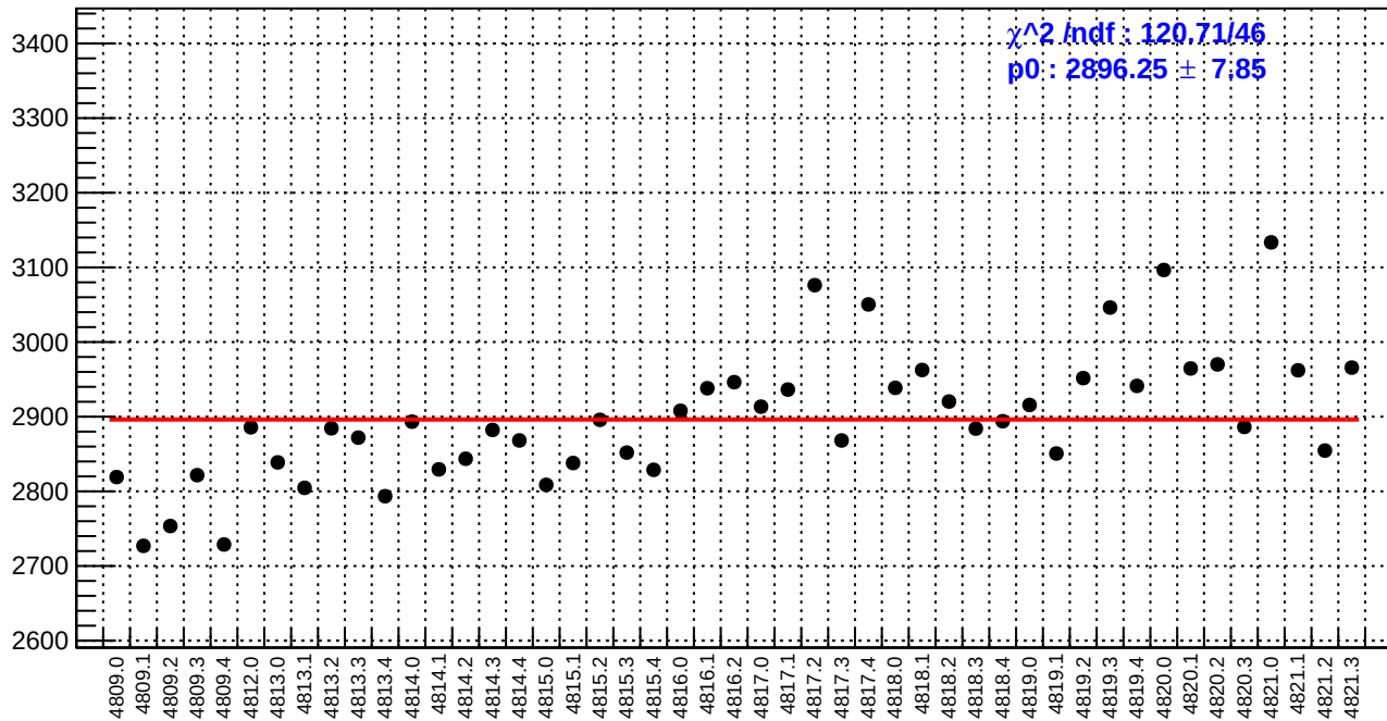
slug83: diff_bpm4aY.rms/nm
