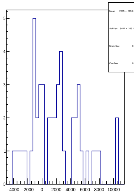
slug83: 1D Corr asym_us_dd.mean/ppb-reg_asym_us_dd.mean/ppb
