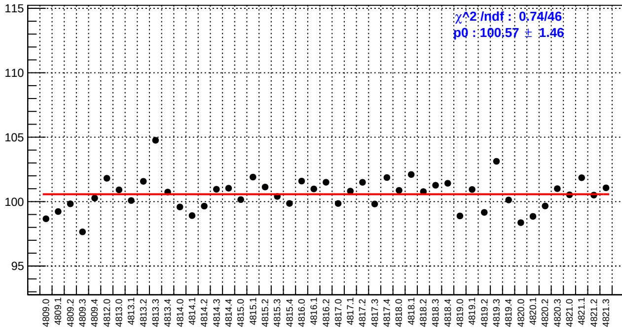
slug83: reg_asym_ds_avg.rms/ppm
