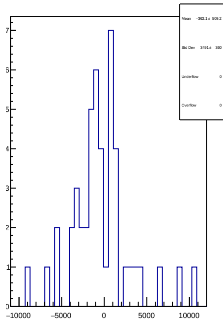
slug83: 1D Corr asym_sam1.mean/ppb-reg_asym_sam1.mean/ppb
