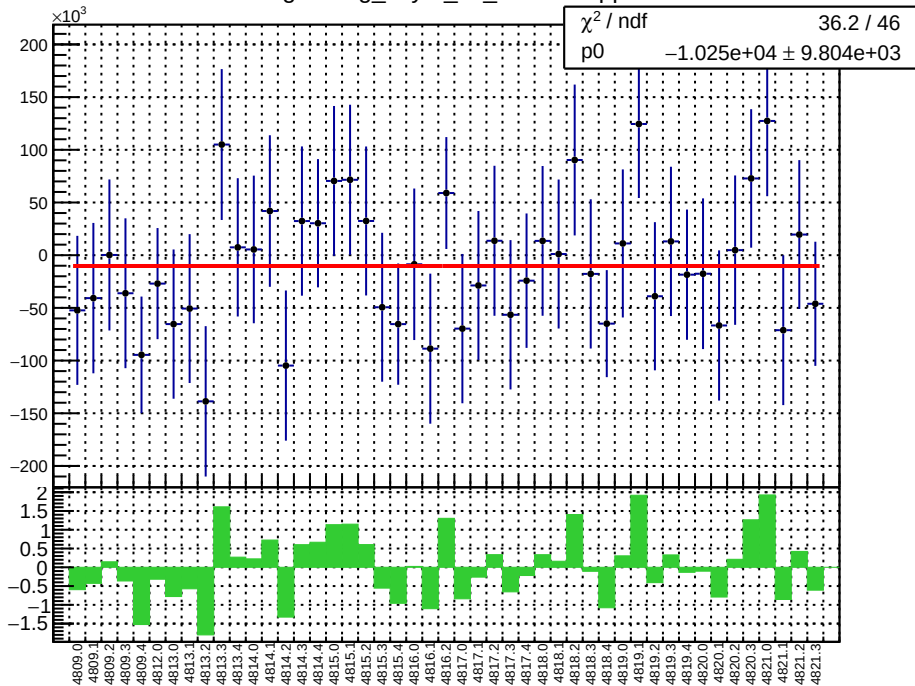
slug83: reg_asym_atl_dd.mean/ppb
