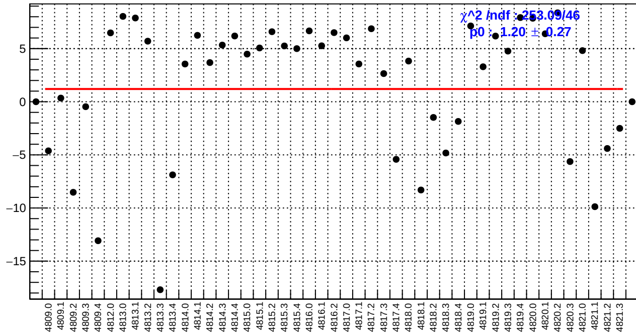
slug83: ds_avg_bpm4eY/(ppb/nm)
