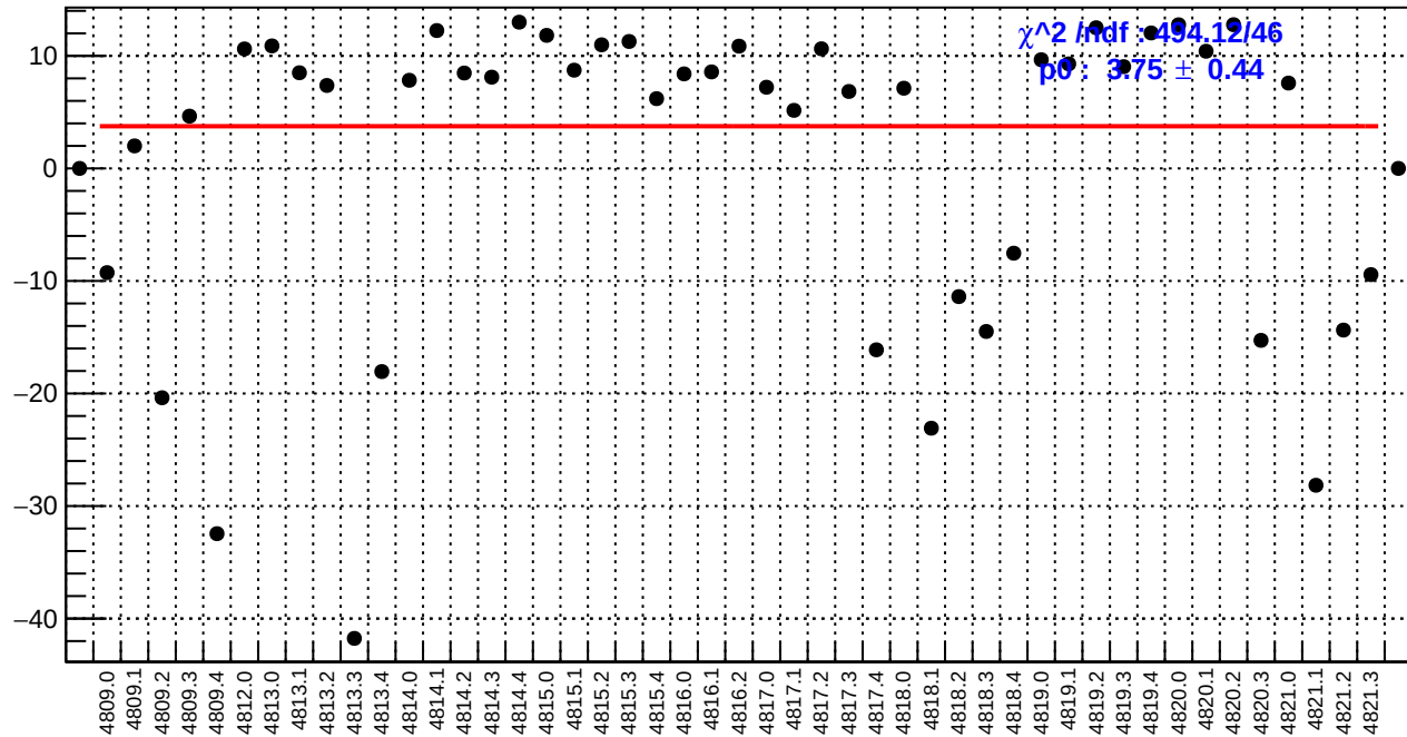
slug83: left_avg_bpm4eY/(ppb/nm)
