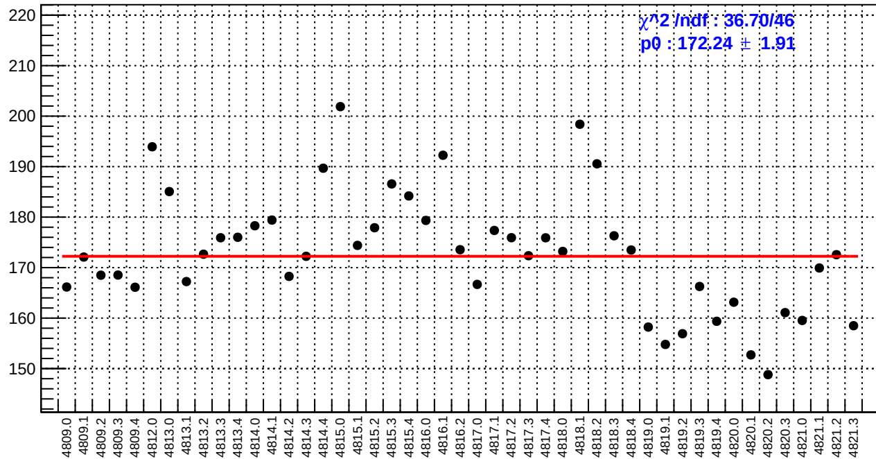
slug83: asym_bcm_an_ds3.rms/ppm
