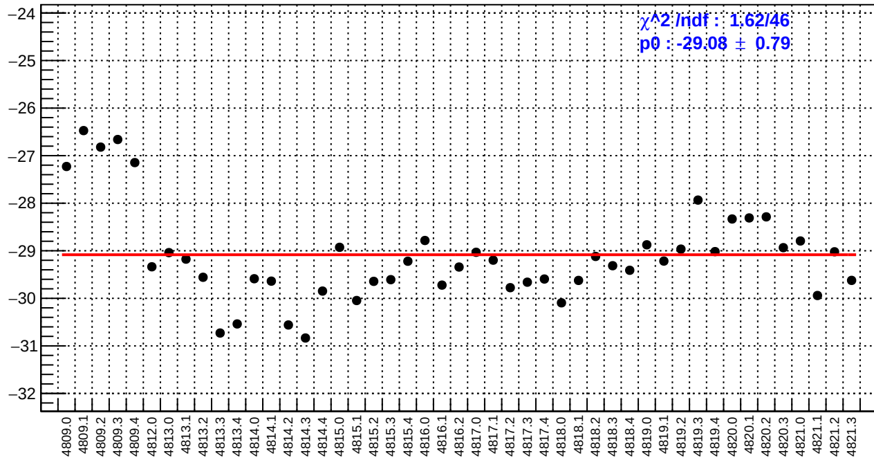
slug83: ds_avg_bpm4eX/(ppb/nm)
