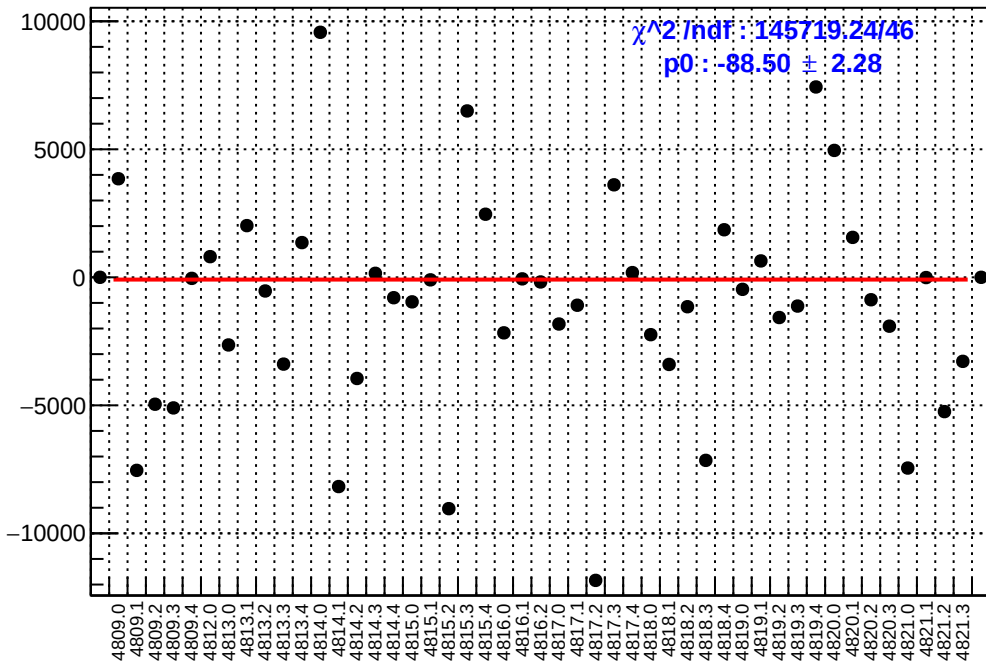
slug83: asym_right_avg.mean/ppb-reg_asym_right_avg.mean/ppb
