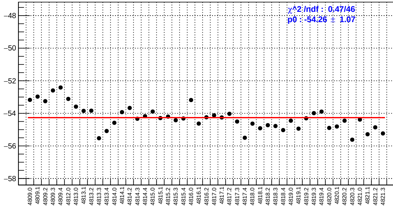
slug83: ds_avg_bpm12X/(ppb/nm)
