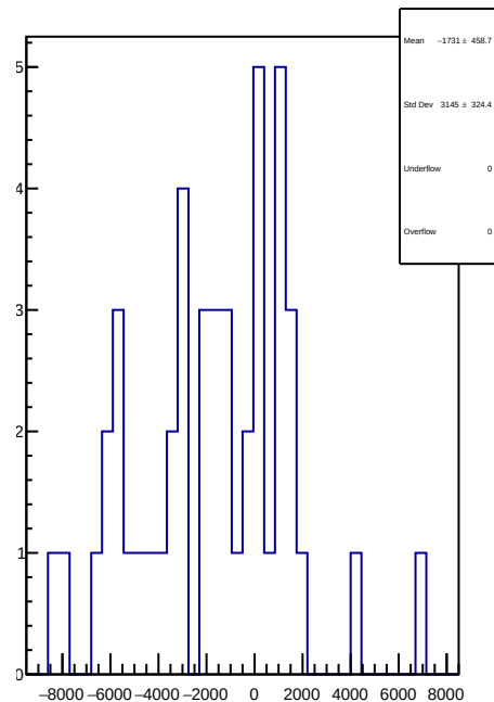
slug83: 1D Corr asym_atr1.mean/ppb-reg_asym_atr1.mean/ppb
