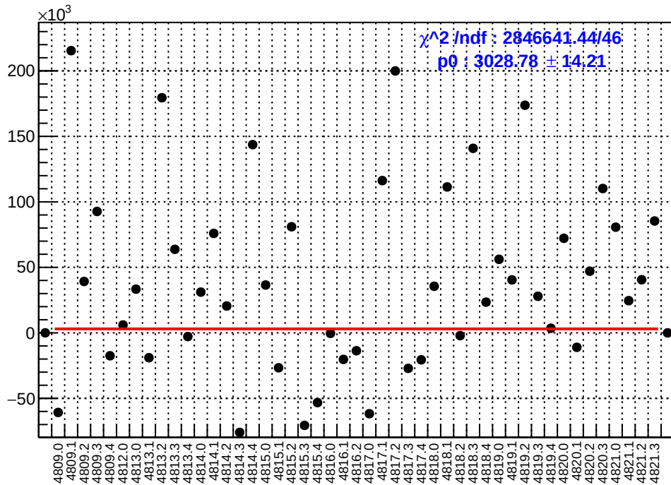
slug83: asym_sam3.mean/ppb-reg_asym_sam3.mean/ppb
