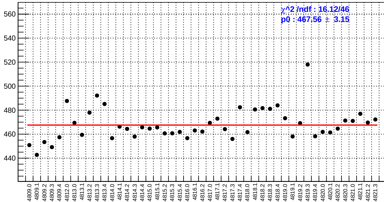
slug83: reg_asym_sam8.rms/ppm
