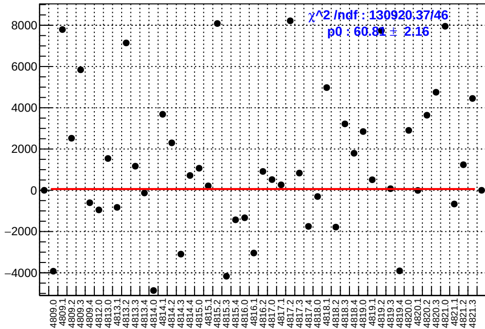
slug83: asym_atl1.mean/ppb-reg_asym_atl1.mean/ppb
