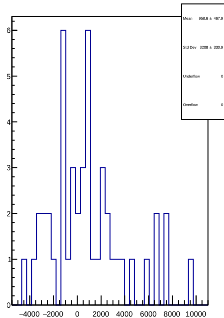
slug83: 1D Corr asym_ds_avg.mean/ppb-reg_asym_ds_avg.mean/ppb
