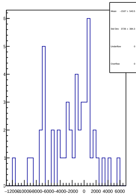
slug83: 1D Corr asym_atr_avg.mean/ppb-reg_asym_atr_avg.mean/ppb
