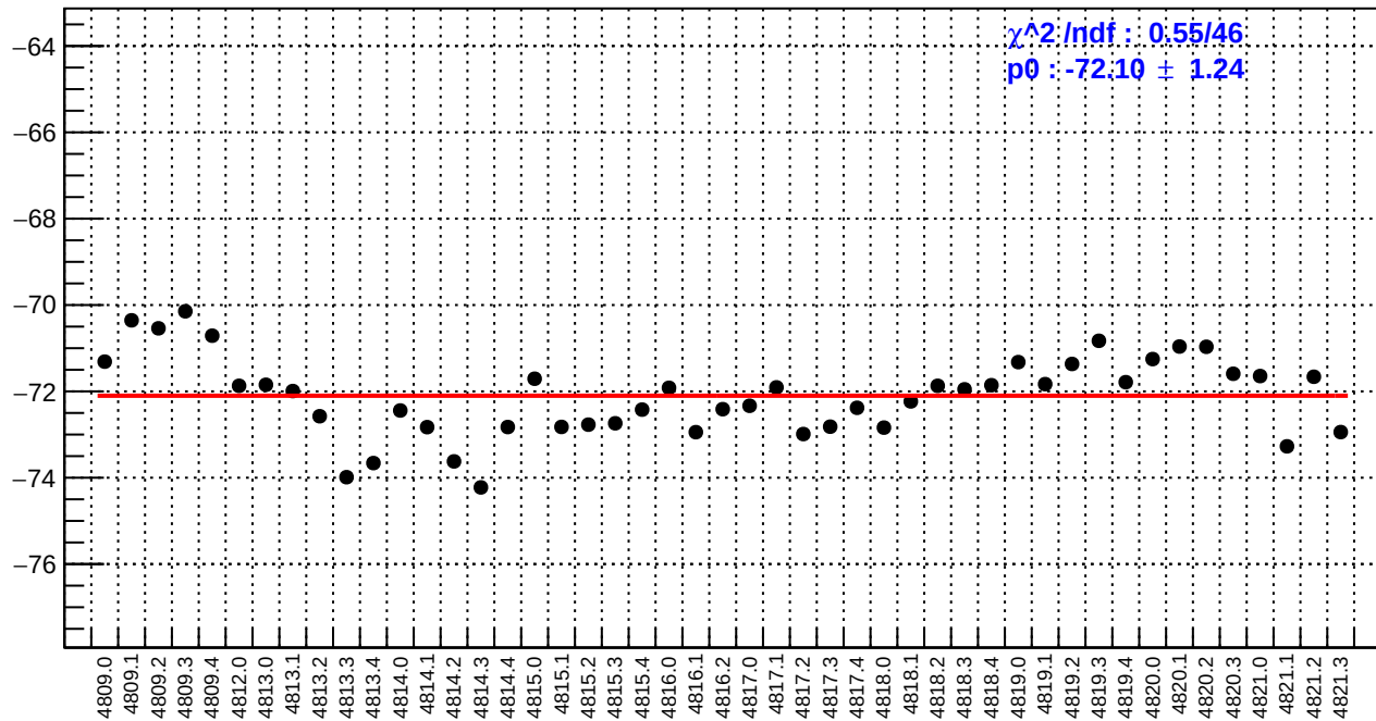
slug83: left_avg_bpm4eX/(ppb/nm)
