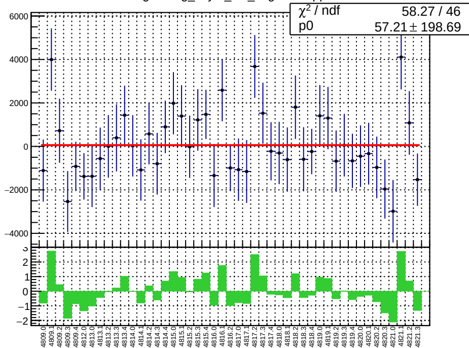
slug83: reg_asym_left_avg.mean/ppb
