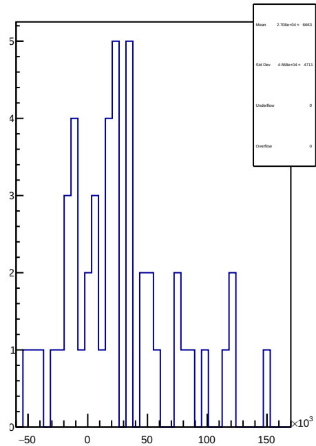
slug83: 1D Corr asym_sam2.mean/ppb-reg_asym_sam2.mean/ppb
