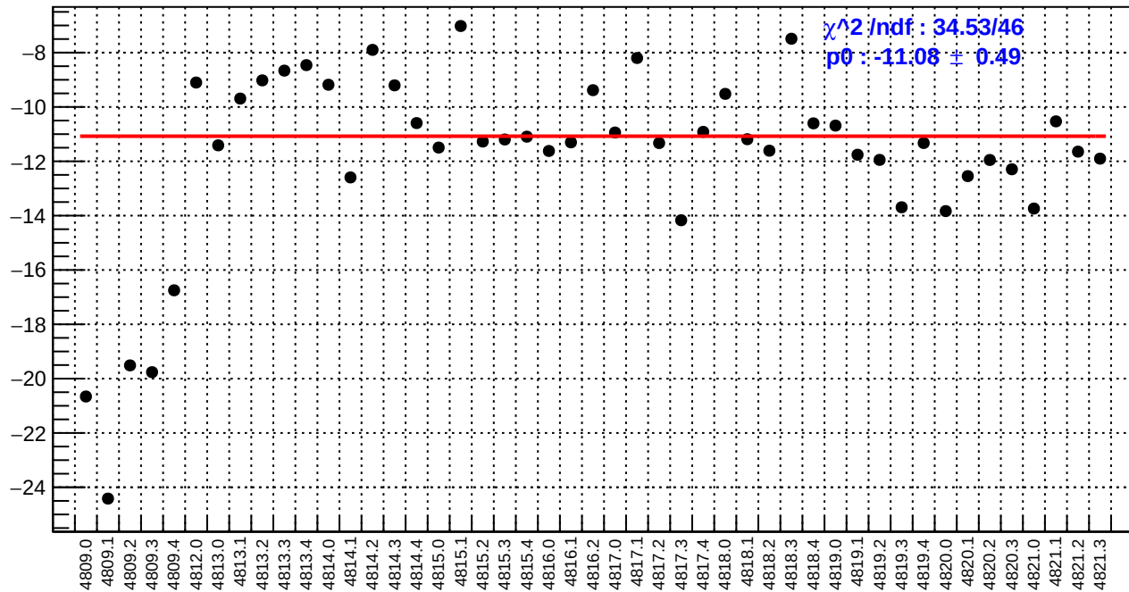
slug83: right_avg_bpm4aX/(ppb/nm)
