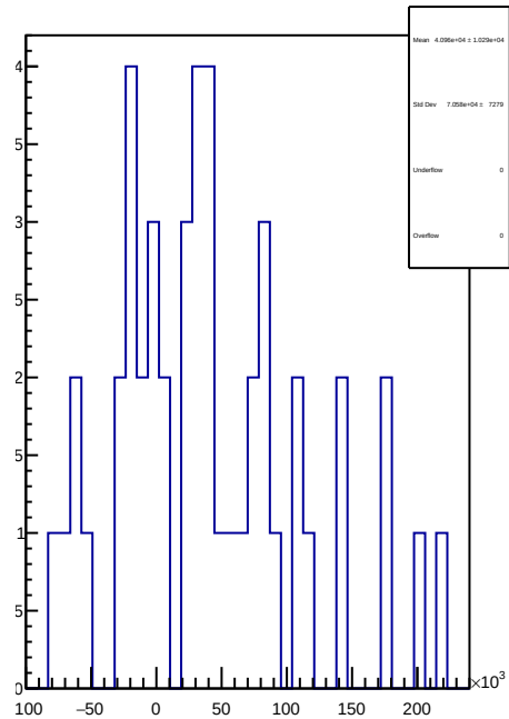
slug83: 1D Corr asym_sam3.mean/ppb-reg_asym_sam3.mean/ppb
