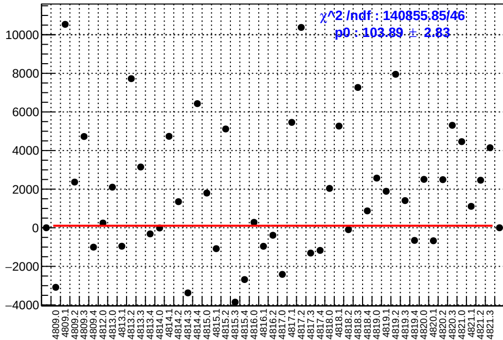
slug83: asym_us_dd.mean/ppb-reg_asym_us_dd.mean/ppb
