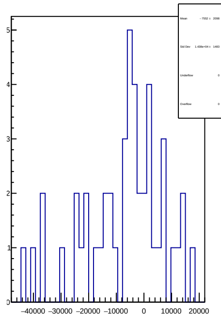
slug83: 1D Corr asym_sam6.mean/ppb-reg_asym_sam6.mean/ppb
