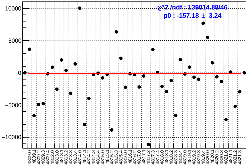
slug83: asym_dsr.mean/ppb-reg_asym_dsr.mean/ppb
