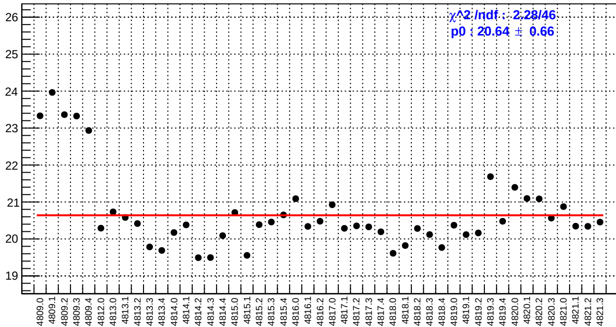
slug83: right_avg_bpm4eX/(ppb/nm)
