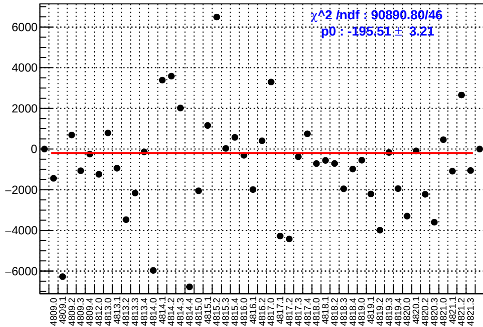
slug83: asym_atl_dd.mean/ppb-reg_asym_atl_dd.mean/ppb
