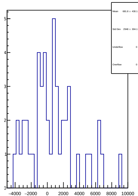
slug83: 1D Corr asym_us_avg.mean/ppb-reg_asym_us_avg.mean/ppb
