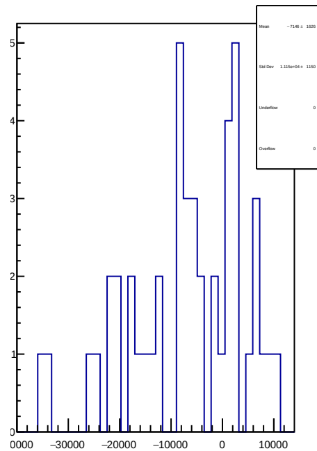
slug83: 1D Corr asym_sam8.mean/ppb-reg_asym_sam8.mean/ppb
