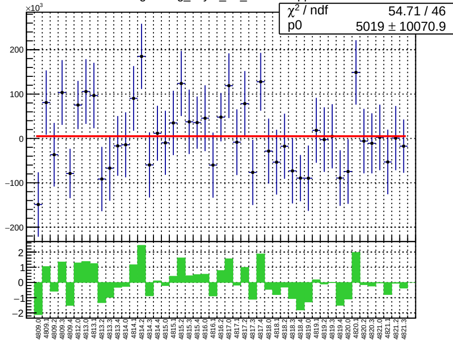
slug83: reg_asym_atr_dd.mean/ppb
