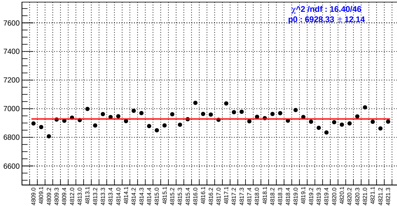
slug83: reg_asym_atr_dd.rms/ppm
