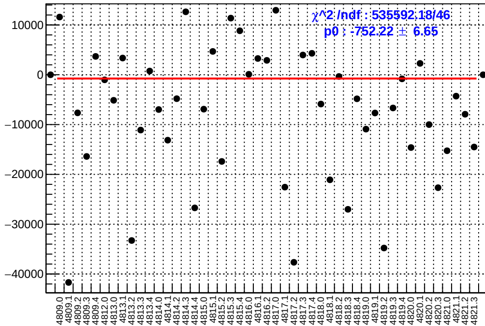
slug83: asym_sam7.mean/ppb-reg_asym_sam7.mean/ppb
