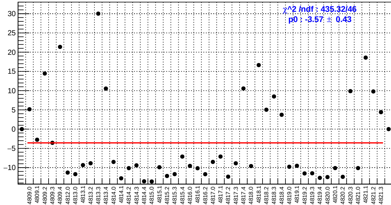
slug83: left_avg_bpm4aY/(ppb/nm)
