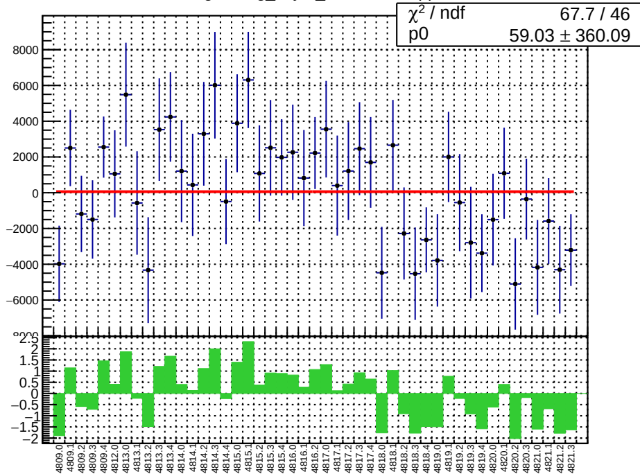
slug83: reg_asym_sam1.mean/ppb
