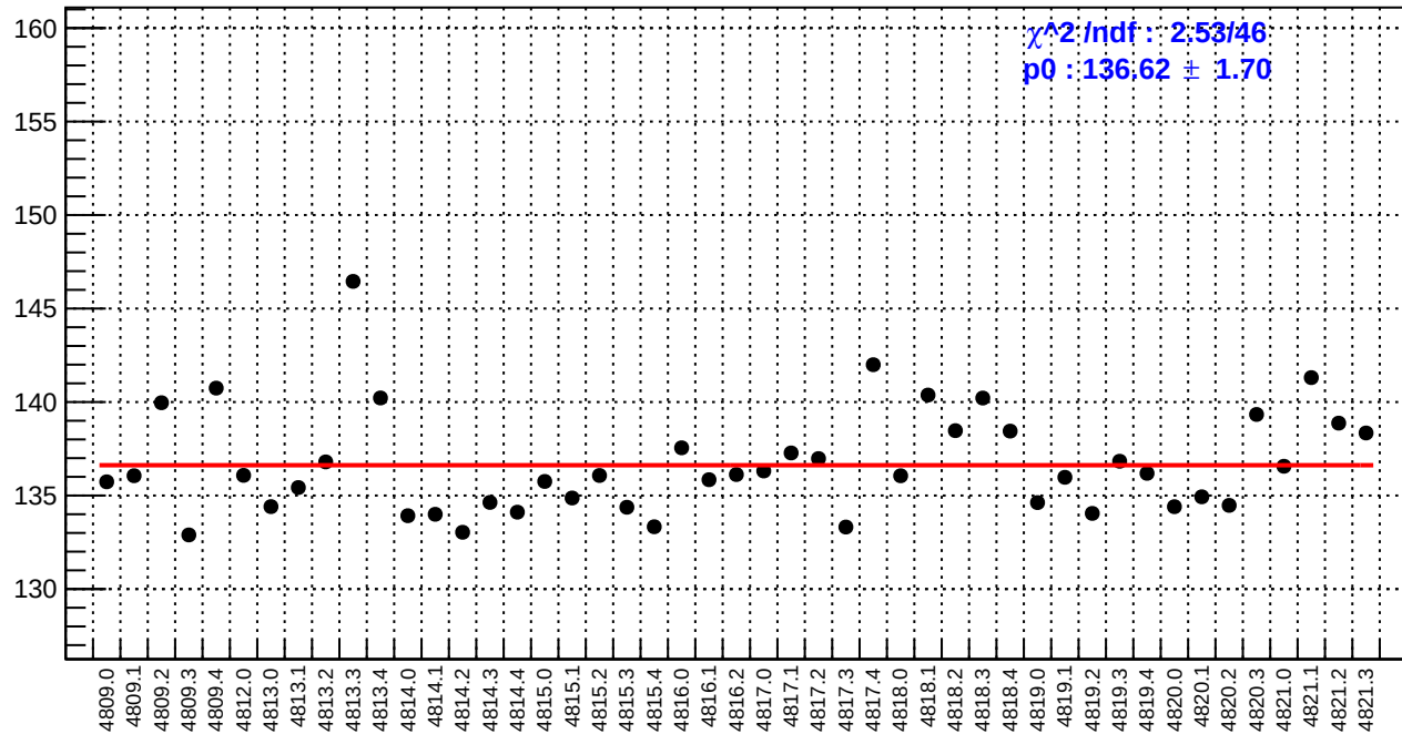
slug83: reg_asym_left_avg.rms/ppm
