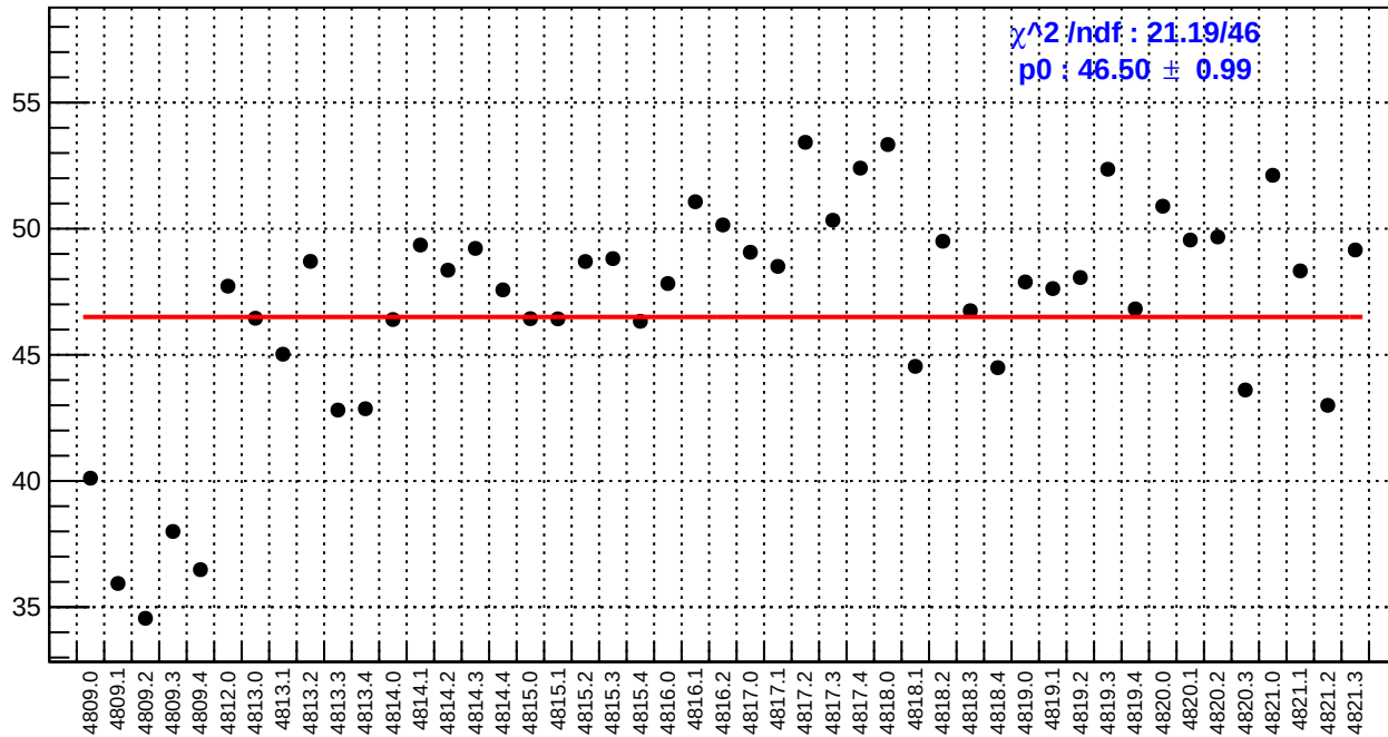
slug83: left_avg_bpm4aX/(ppb/nm)
