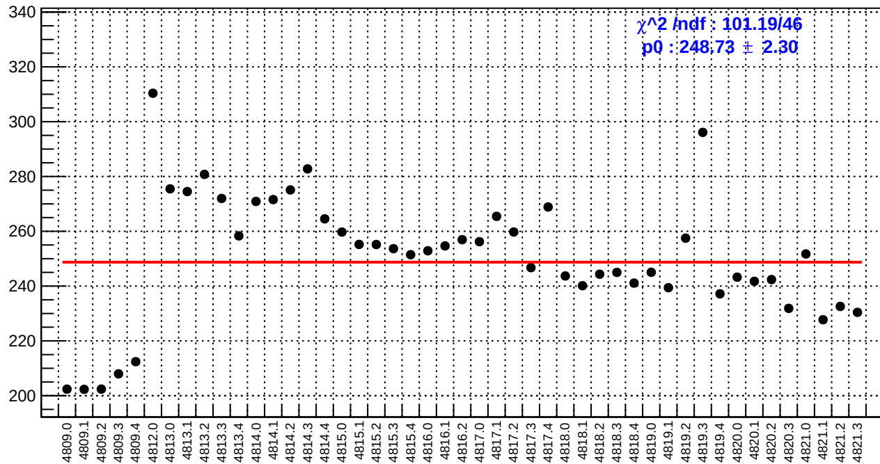
slug83: reg_asym_sam1.rms/ppm
