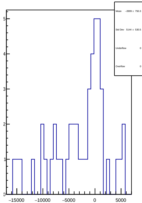
slug83: 1D Corr asym_at2_dd.mean/ppb-reg_asym_at2_dd.mean/ppb
