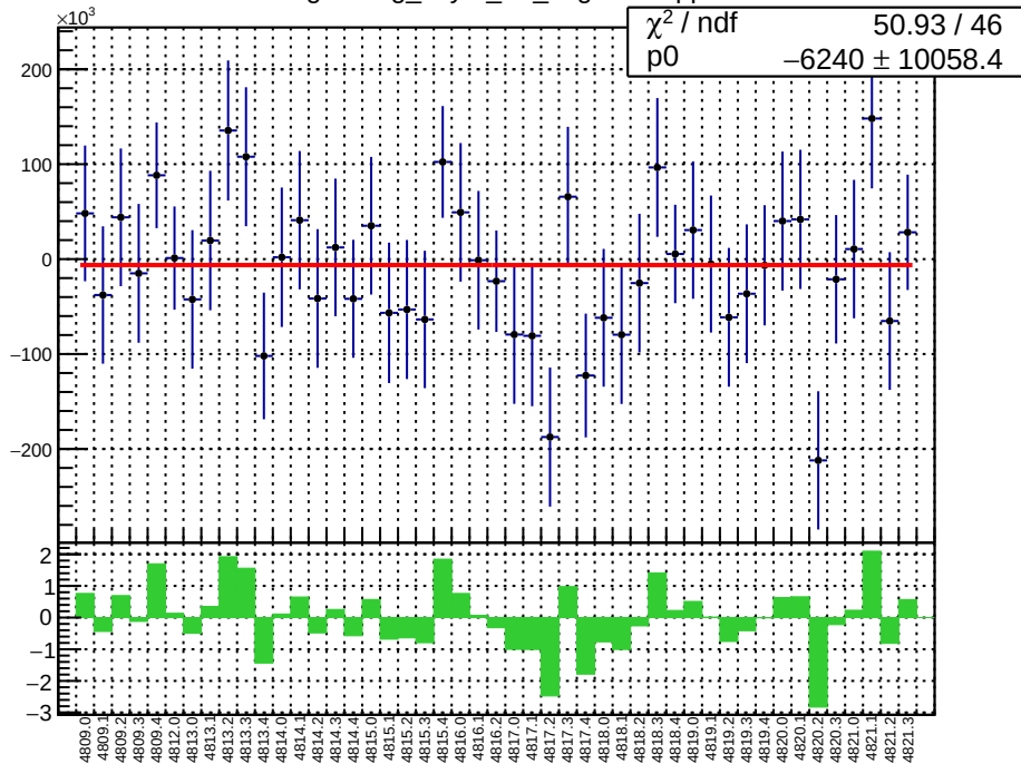
slug83: reg_asym_atr_avg.mean/ppb
