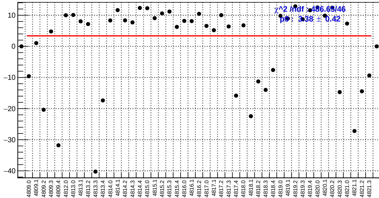
slug83: usl_bpm4eY/(ppb/nm)
