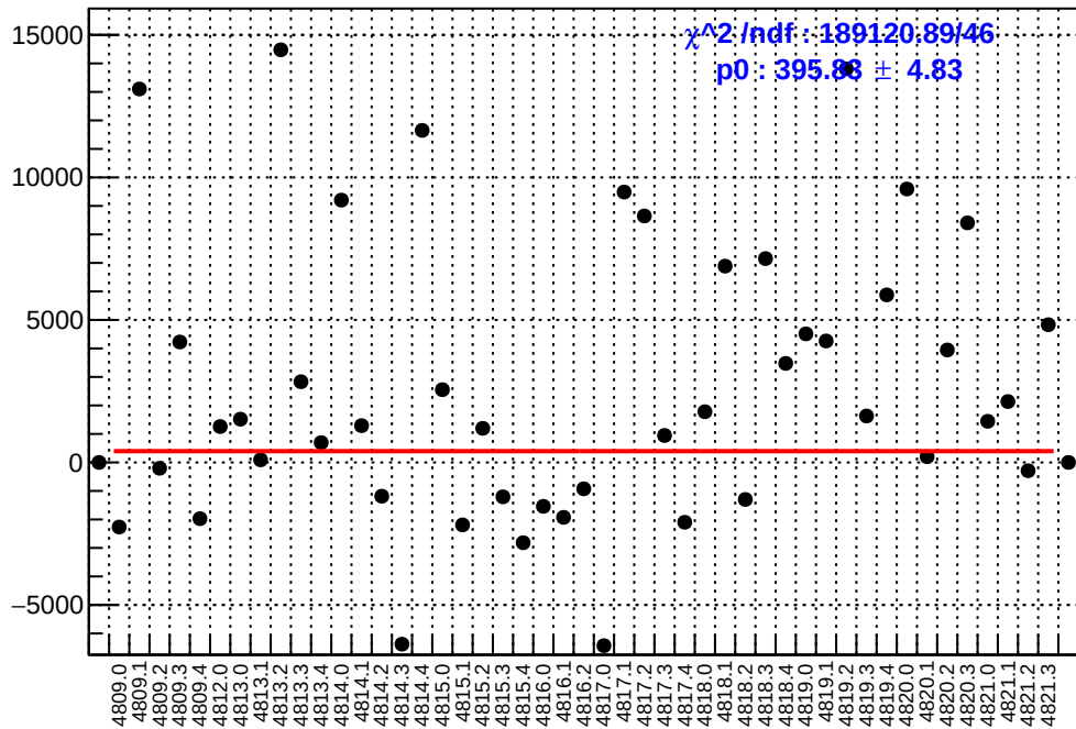
slug83: asym_left_avg.mean/ppb-reg_asym_left_avg.mean/ppb
