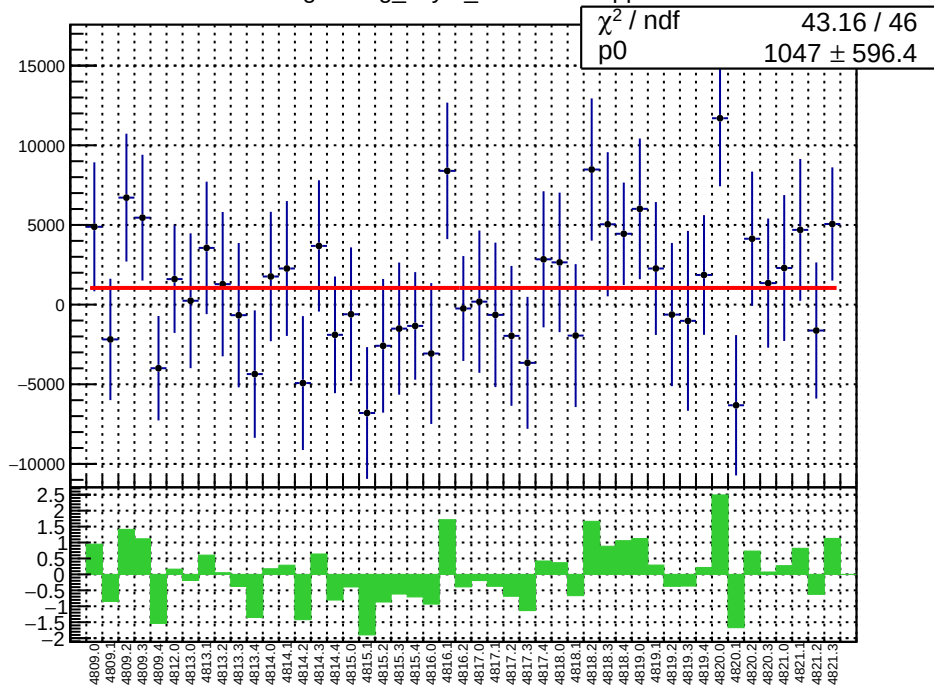
slug83: reg_asym_sam6.mean/ppb
