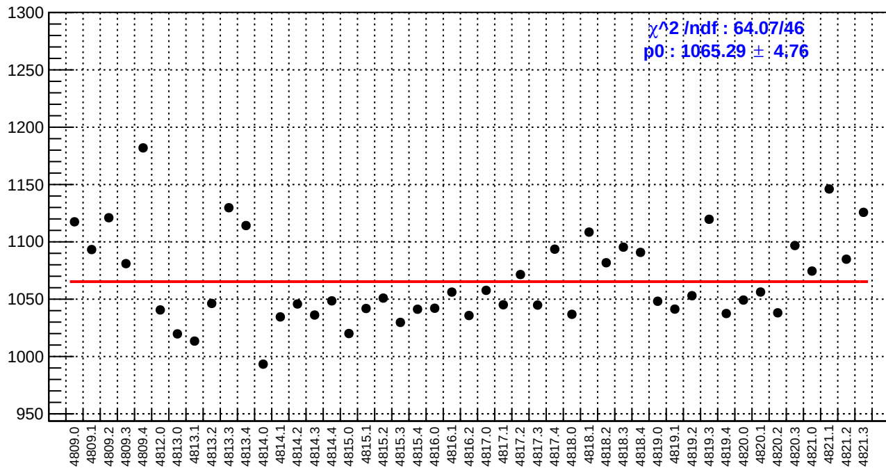
slug83: reg_asym_sam4.rms/ppm
