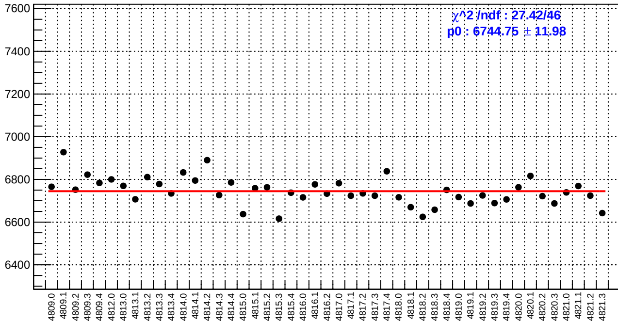
slug83: reg_asym_atl_avg.rms/ppm
