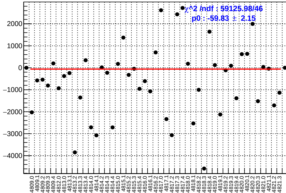
slug83: asym_atl1r2_avg.mean/ppb-reg_asym_atl1r2_avg.mean/ppb
