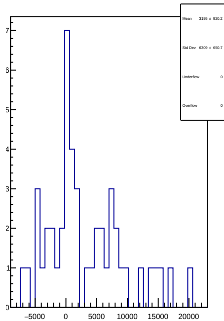
slug83: 1D Corr asym_atl2.mean/ppb-reg_asym_atl2.mean/ppb
