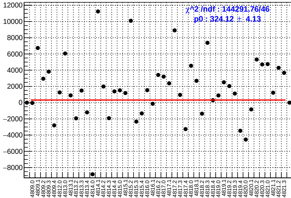
slug83: asym_sam5.mean/ppb-reg_asym_sam5.mean/ppb
