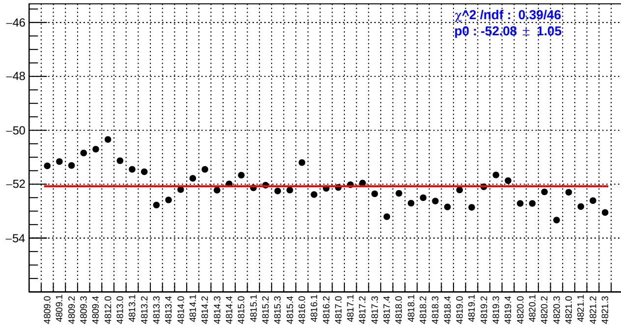
slug83: us_avg_bpm12X/(ppb/nm)
