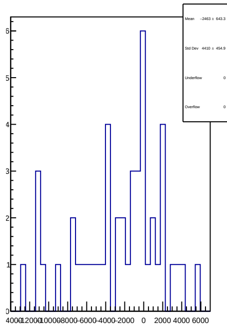
slug83: 1D Corr asym_atr1l2_dd.mean/ppb-reg_asym_atr1l2_dd.mean/ppb
