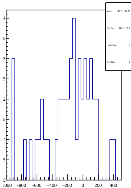
slug83: 1D Corr asym_right_dd.mean/ppb-reg_asym_right_dd.mean/ppb
