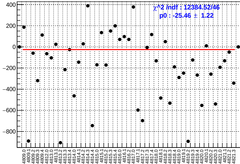
slug83: asym_right_dd.mean/ppb-reg_asym_right_dd.mean/ppb
