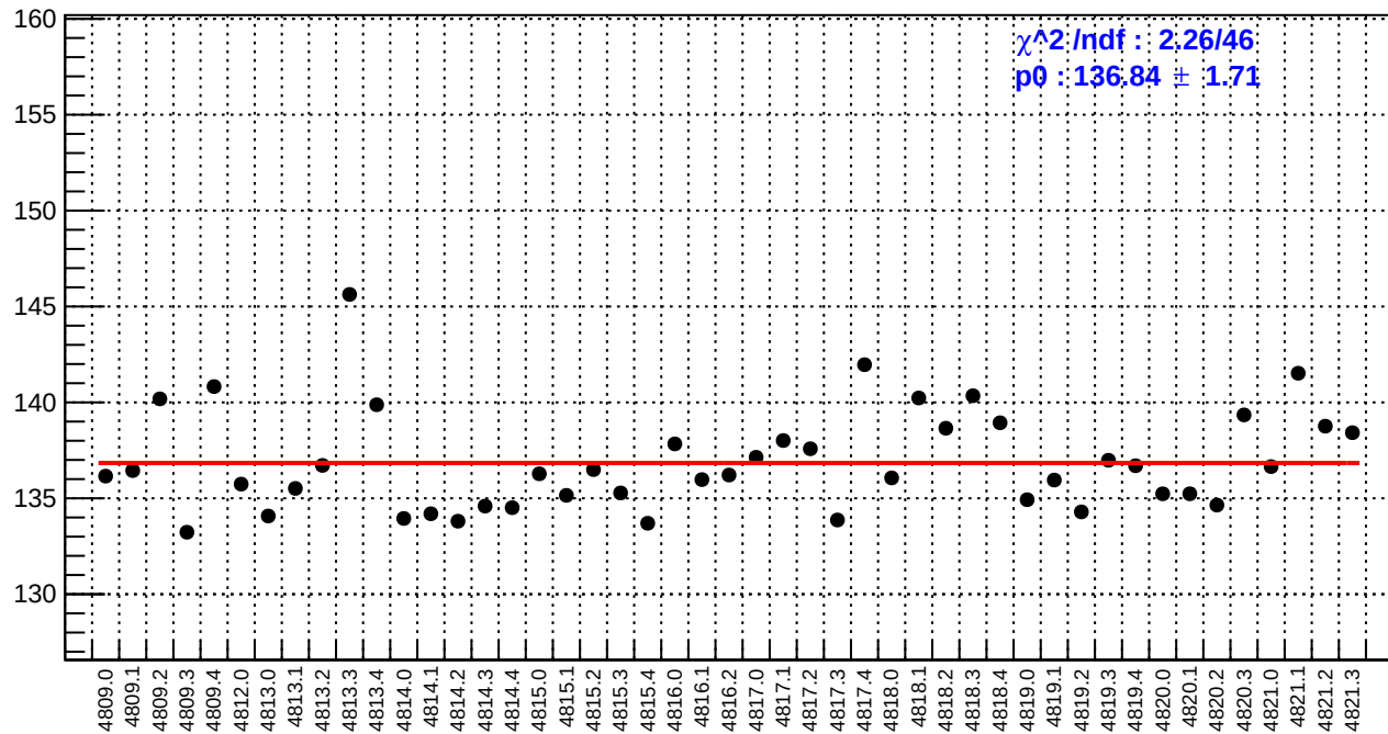
slug83: reg_asym_usl.rms/ppm
