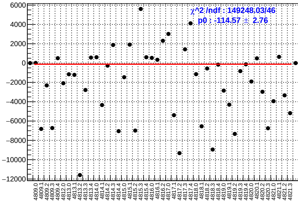
slug83: asym_atr_avg.mean/ppb-reg_asym_atr_avg.mean/ppb
