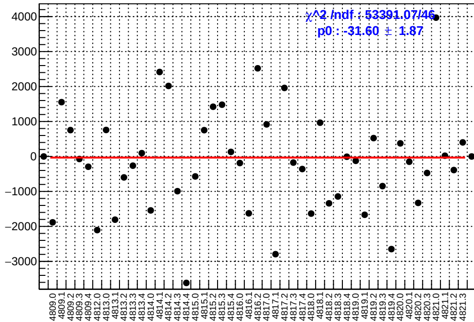
slug83: asym_at1_avg.mean/ppb-reg_asym_at1_avg.mean/ppb
