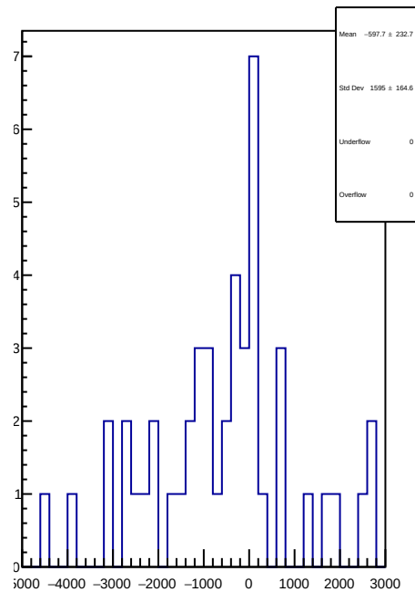
slug83: 1D Corr asym_atl1r2_avg.mean/ppb-reg_asym_atl1r2_avg.mean/ppb
