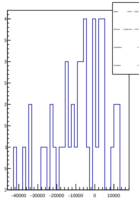
slug83: 1D Corr asym_sam7.mean/ppb-reg_asym_sam7.mean/ppb
