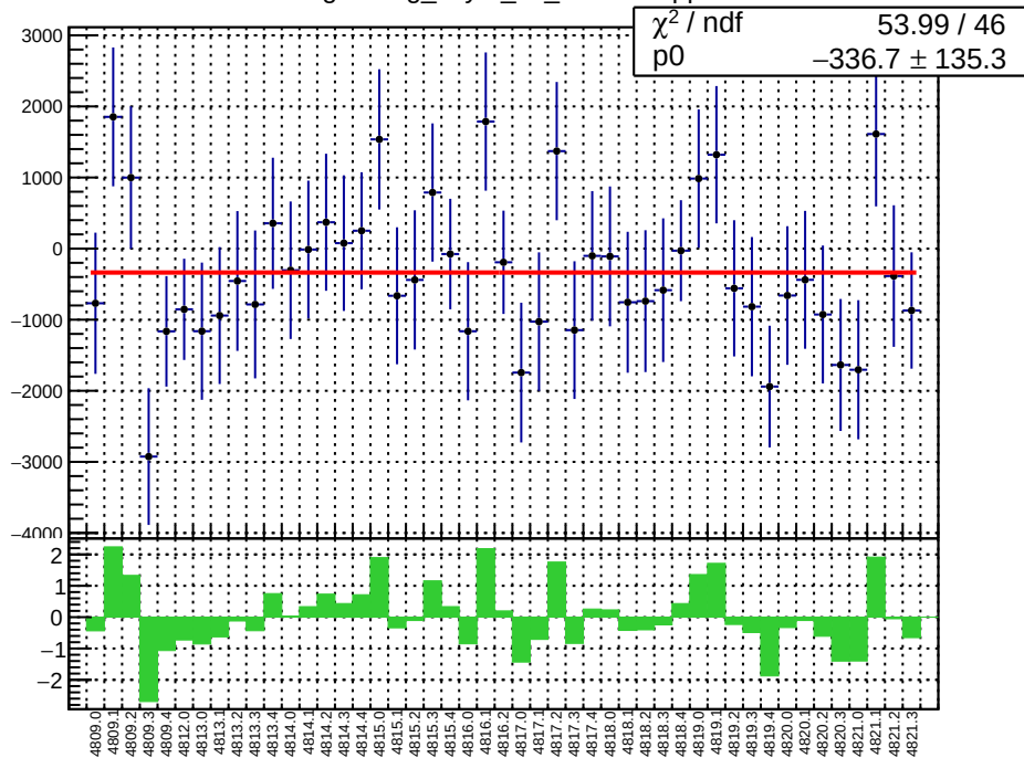
slug83: reg_asym_us_dd.mean/ppb
