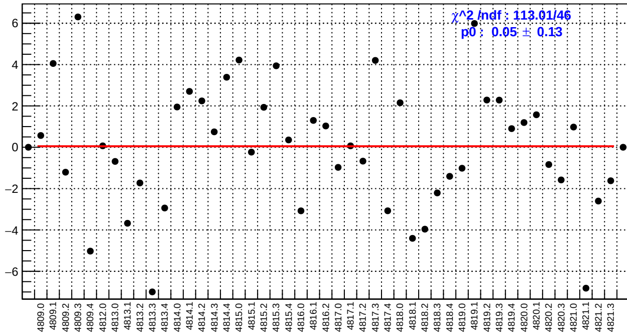
slug83: right_avg_bpm4aY/(ppb/nm)
