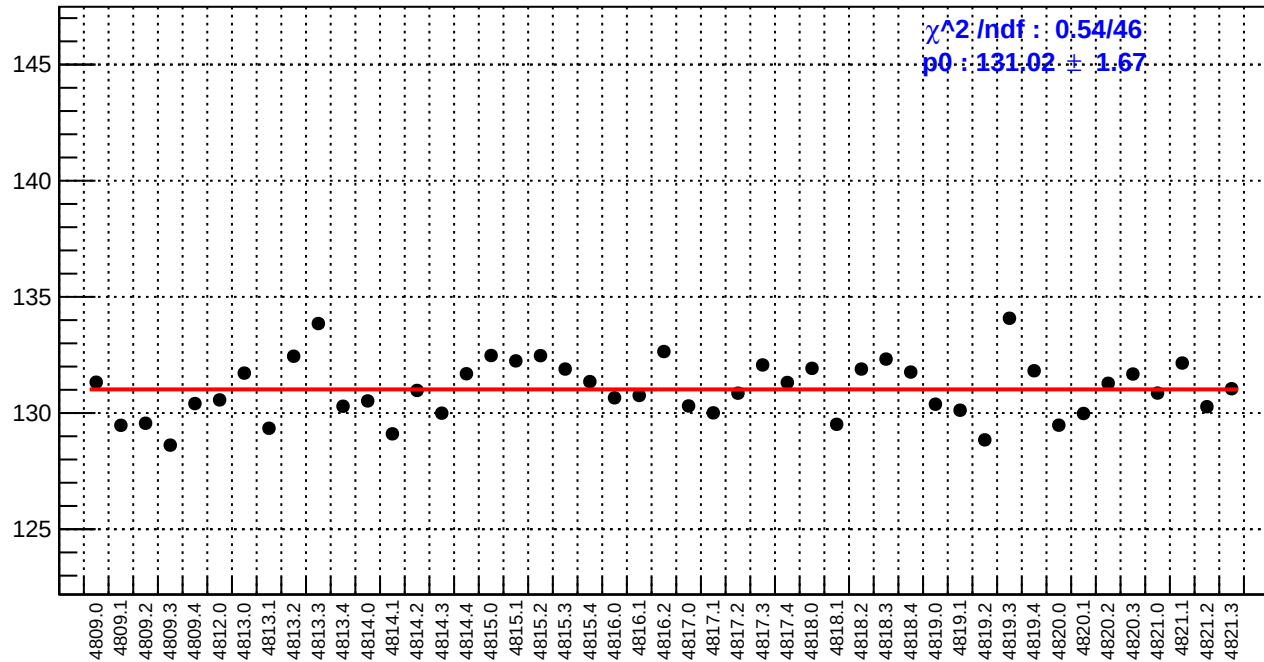
slug83: reg_asym_right_avg.rms/ppm
