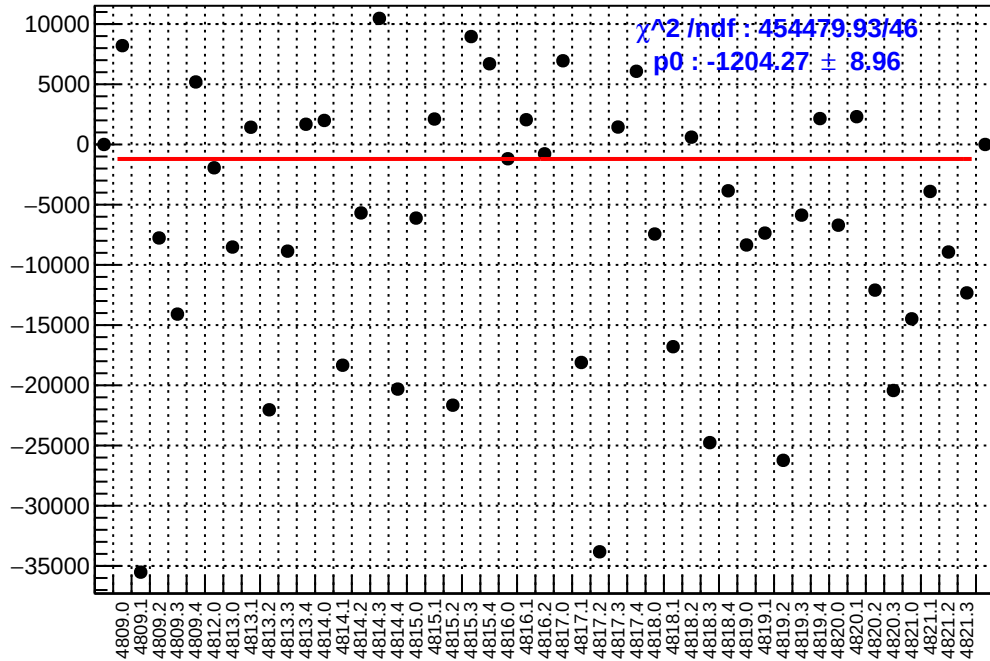
slug83: asym_sam8.mean/ppb-reg_asym_sam8.mean/ppb
