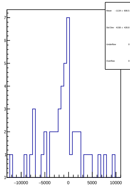
slug83: 1D Corr asym_right_avg.mean/ppb-reg_asym_right_avg.mean/ppb
