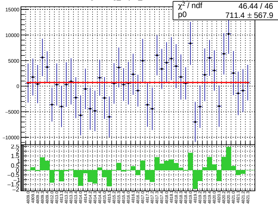
slug83: reg_asym_sam7.mean/ppb
