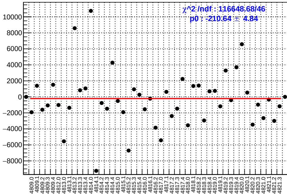
slug83: asym_sam1.mean/ppb-reg_asym_sam1.mean/ppb
