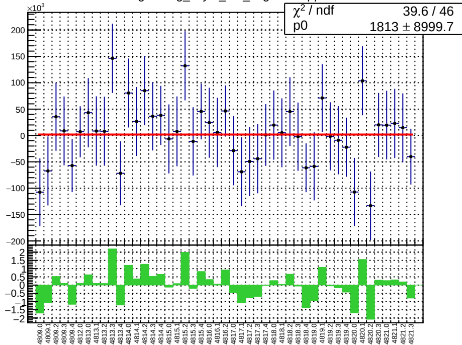
slug83: reg_asym_at1_avg.mean/ppb
