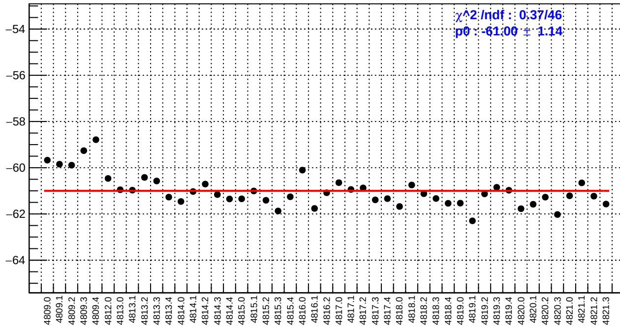
slug83: right_avg_bpm12X/(ppb/nm)
