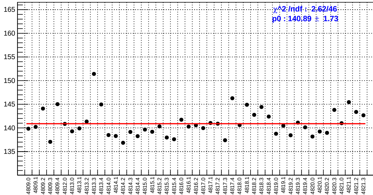
slug83: reg_asym_dsl.rms/ppm
