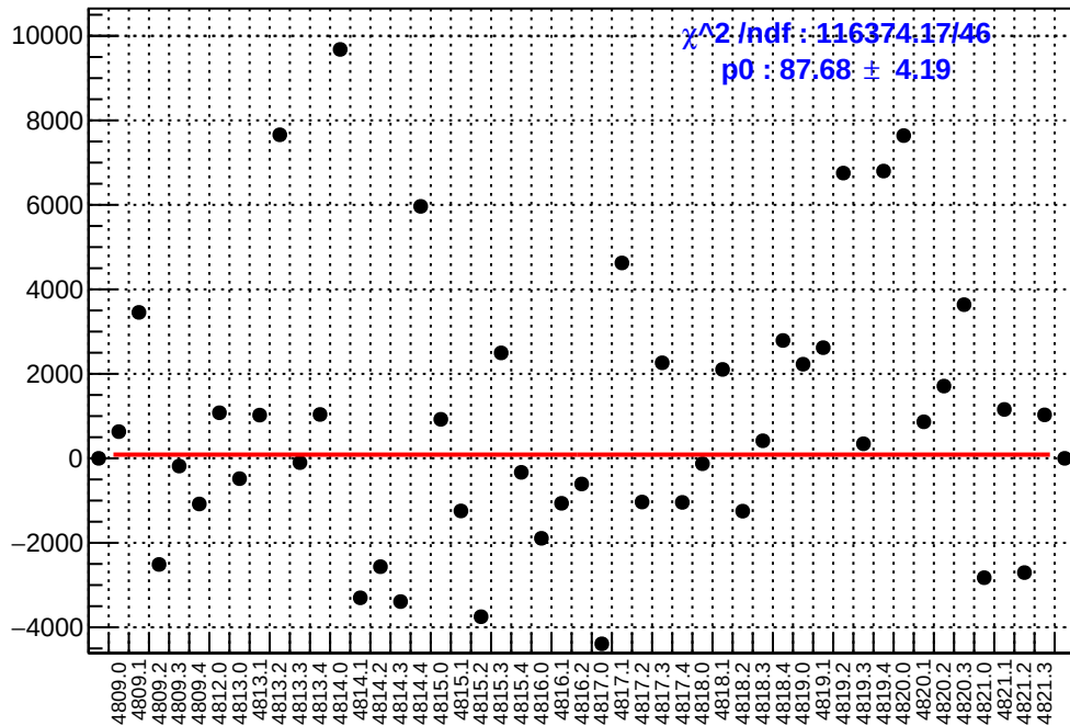
slug83: asym_ds_avg.mean/ppb-reg_asym_ds_avg.mean/ppb
