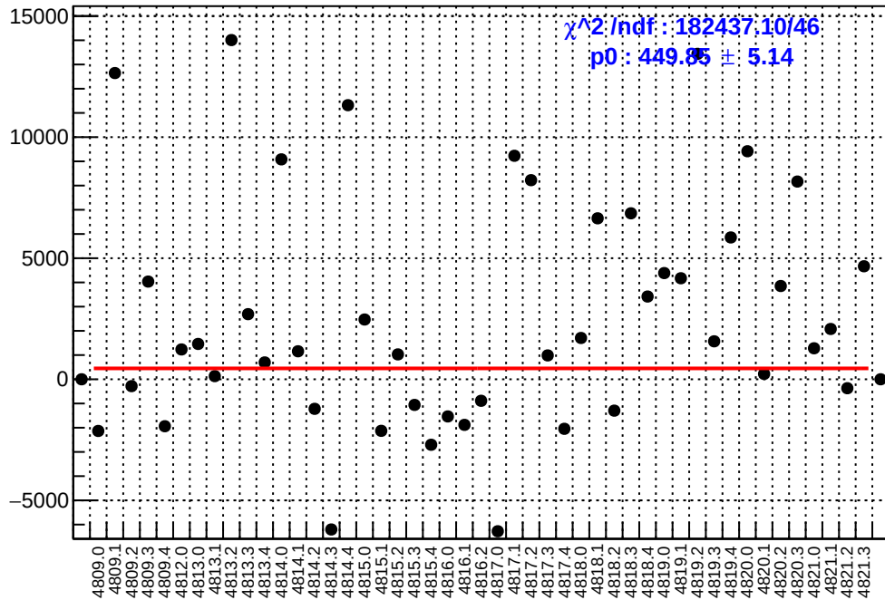
slug83: asym_usl.mean/ppb-reg_asym_usl.mean/ppb
