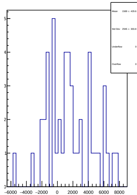
slug83: 1D Corr asym_at1_dd.mean/ppb-reg_asym_at1_dd.mean/ppb
