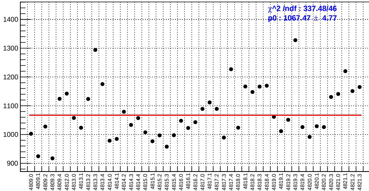
slug83: reg_asym_sam3.rms/ppm
