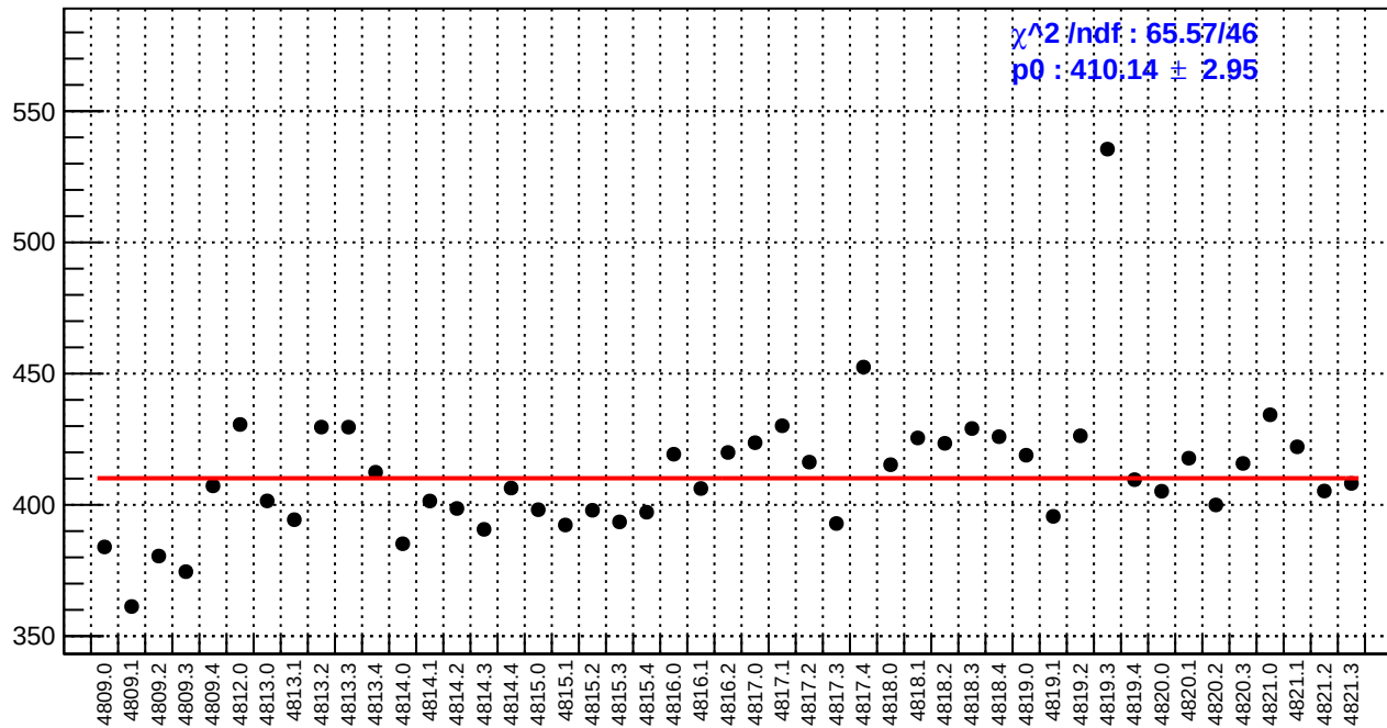
slug83: reg_asym_sam6.rms/ppm
