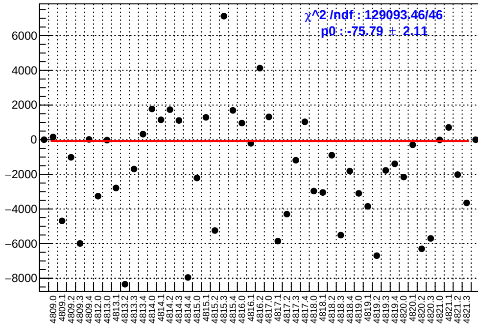
slug83: asym_atr1.mean/ppb-reg_asym_atr1.mean/ppb
