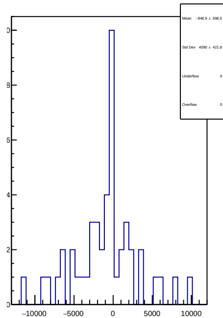
slug83: 1D Corr asym_dsr.mean/ppb-reg_asym_dsr.mean/ppb
