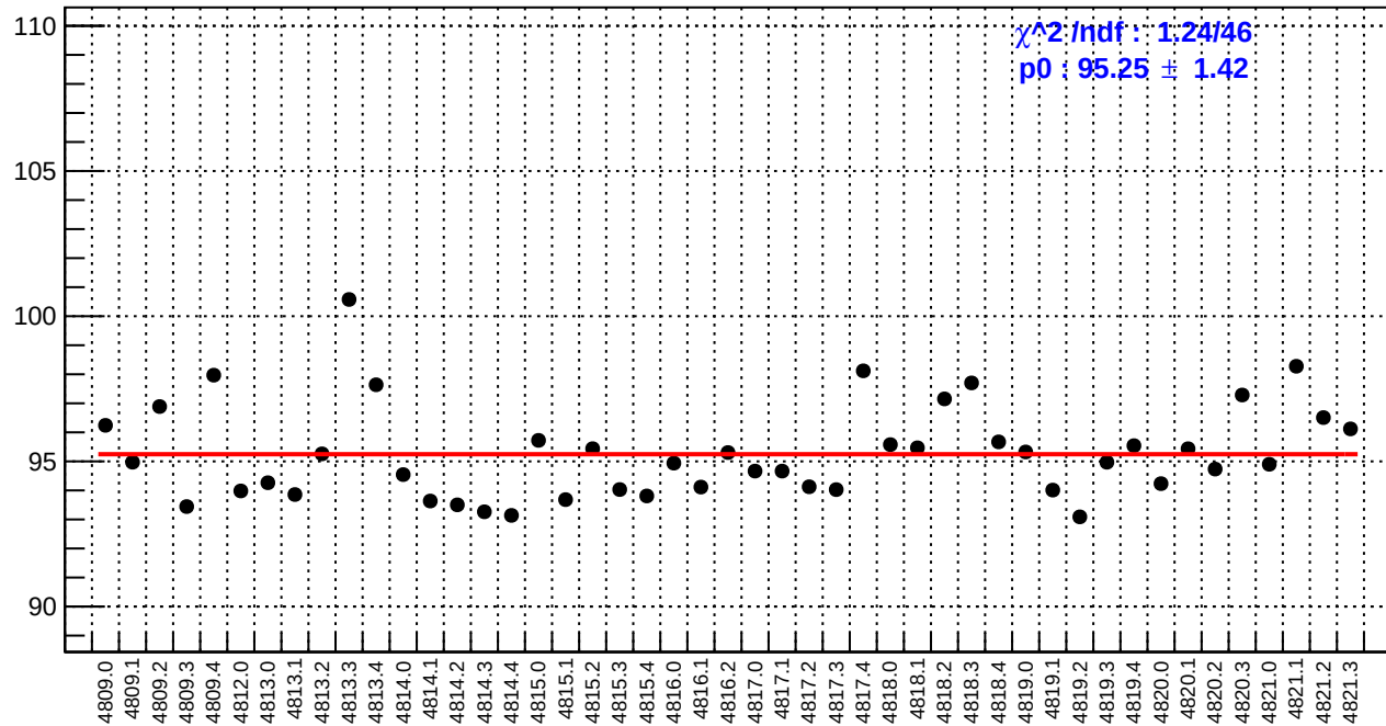
slug83: reg_asym_ds_dd.rms/ppm
