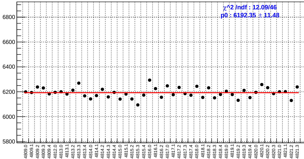
slug83: reg_asym_at1_dd.rms/ppm
