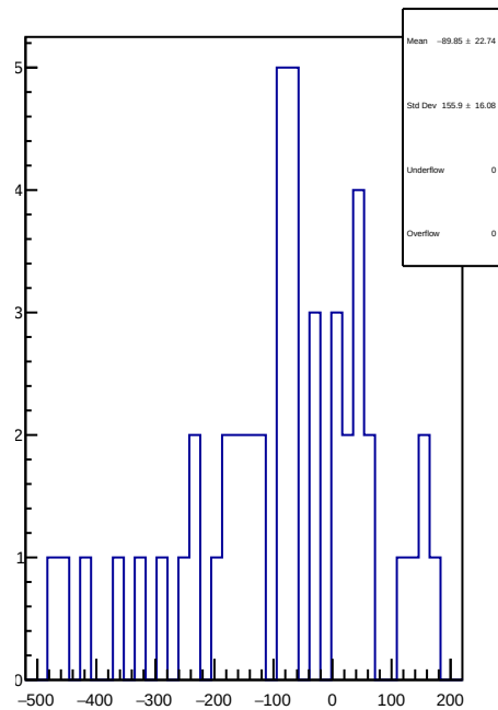
slug83: 1D Corr asym_left_dd.mean/ppb-reg_asym_left_dd.mean/ppb
