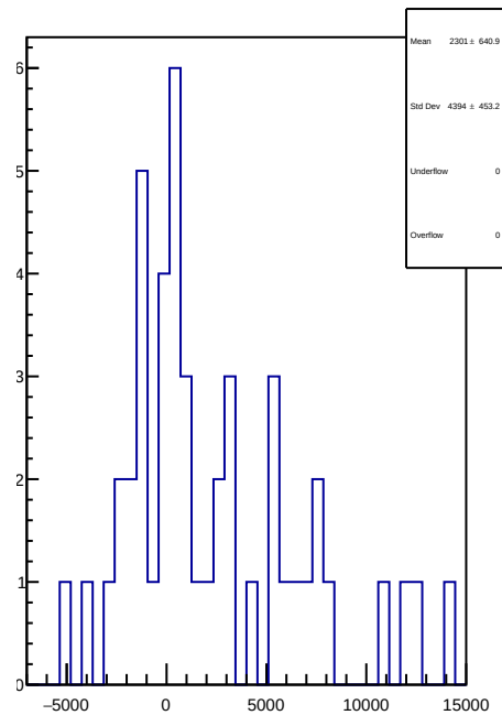
slug83: 1D Corr asym_atl_avg.mean/ppb-reg_asym_atl_avg.mean/ppb
