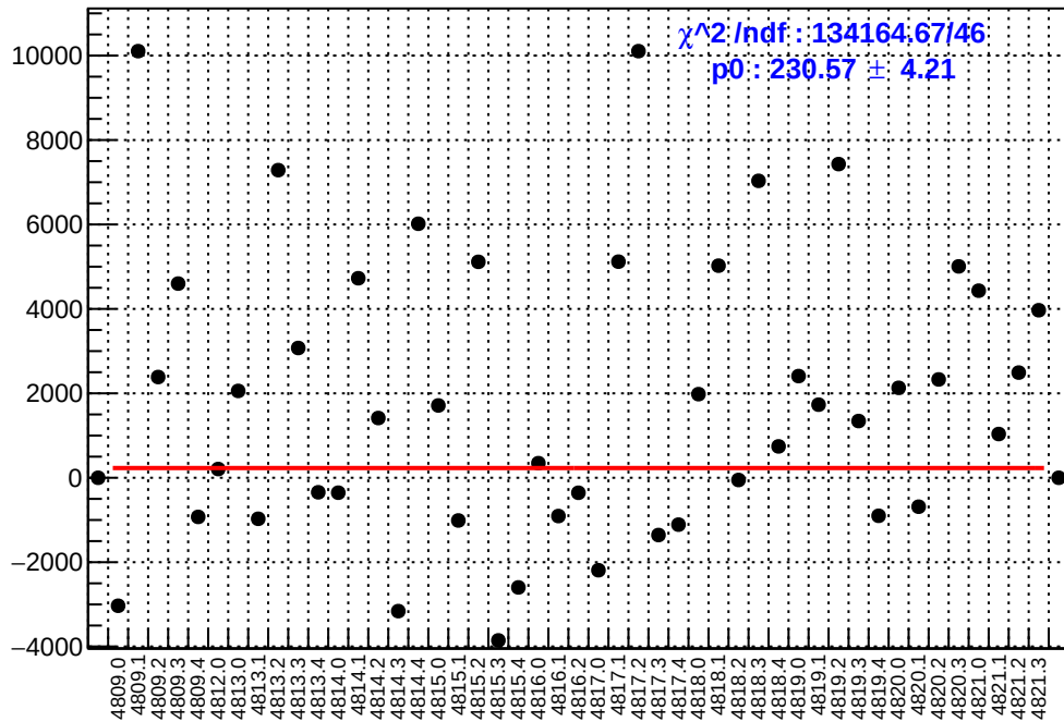
slug83: asym_ds_dd.mean/ppb-reg_asym_ds_dd.mean/ppb
