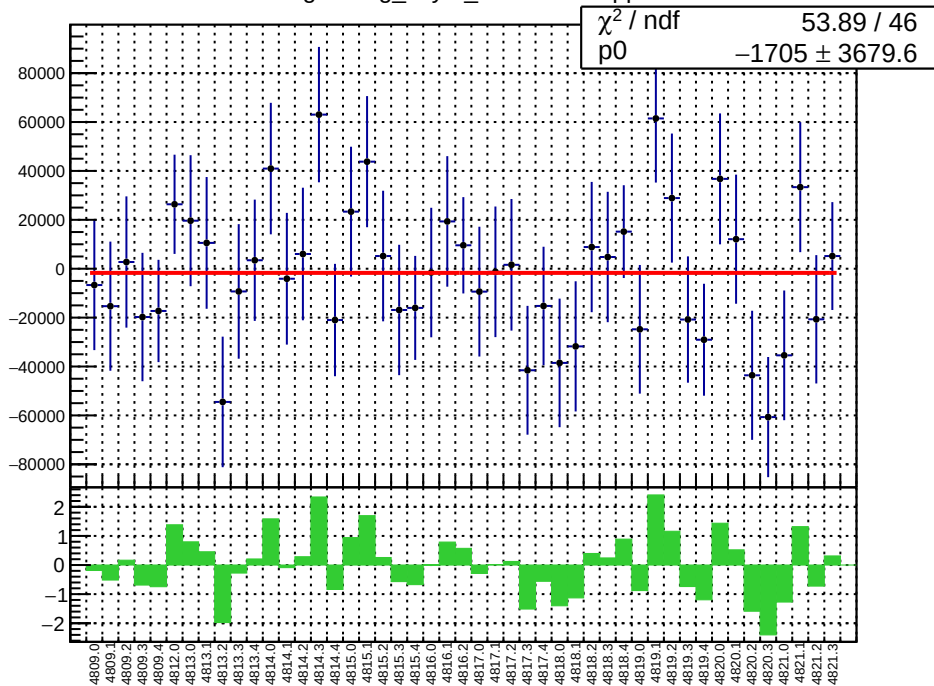
slug83: reg_asym_sam2.mean/ppb
