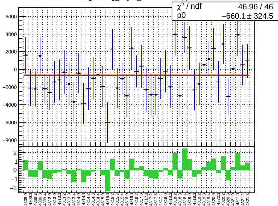
slug83: reg_asym_sam5.mean/ppb
