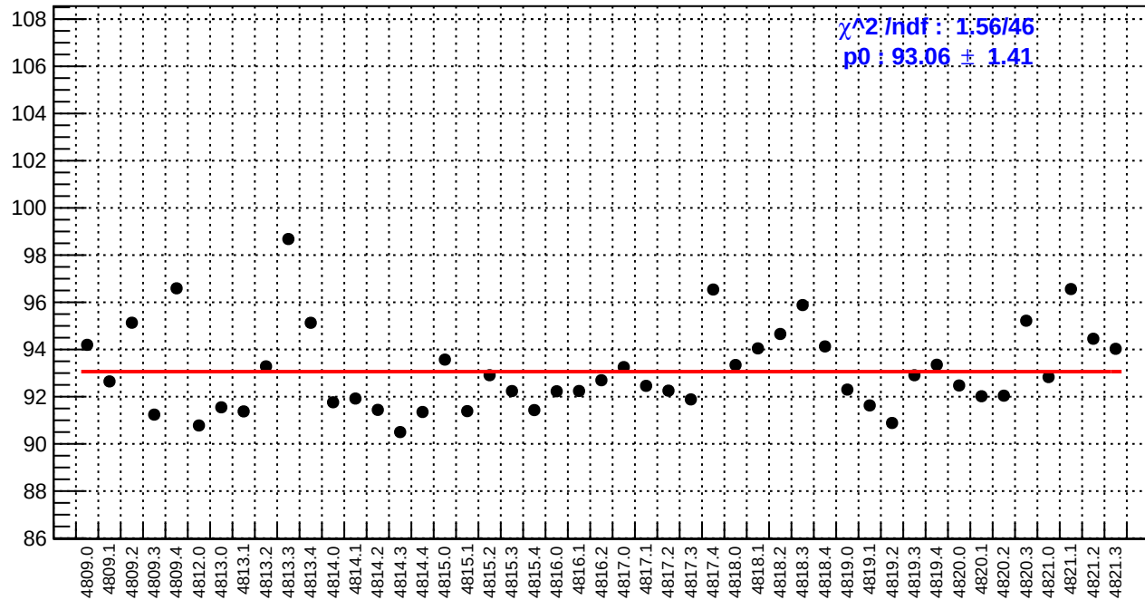
slug83: reg_asym_us_dd.rms/ppm
