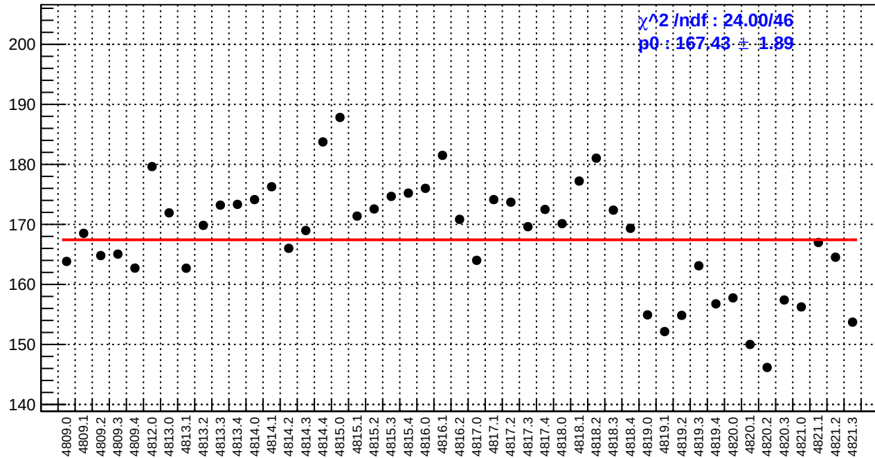
slug83: asym_bcm_an_us.rms/ppm
