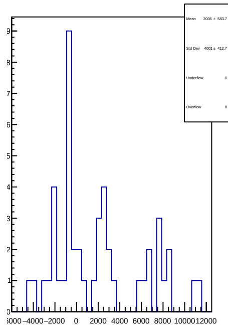
slug83: 1D Corr asym_atl1r2_dd.mean/ppb-reg_asym_atl1r2_dd.mean/ppb
