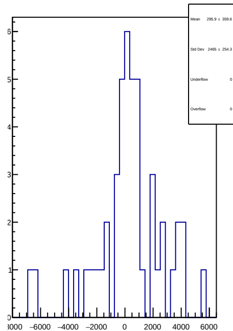
slug83: 1D Corr asym_at2_avg.mean/ppb-reg_asym_at2_avg.mean/ppb
