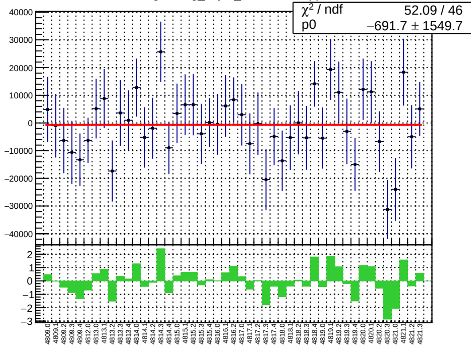
slug83: reg_asym_sam4.mean/ppb
