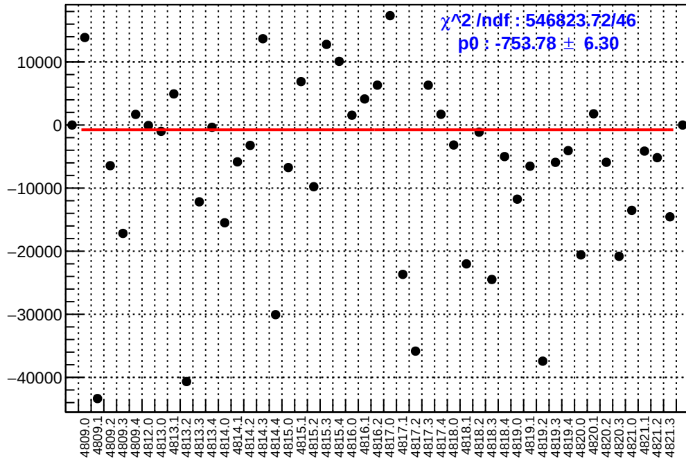
slug83: asym_sam6.mean/ppb-reg_asym_sam6.mean/ppb
