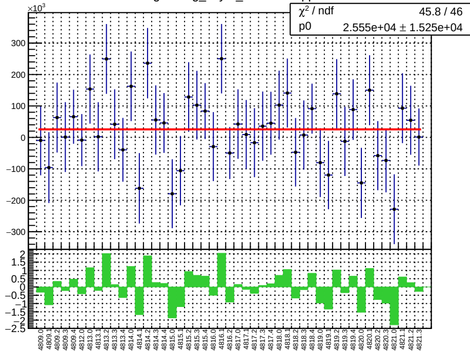
slug83: reg_asym_atl2.mean/ppb
