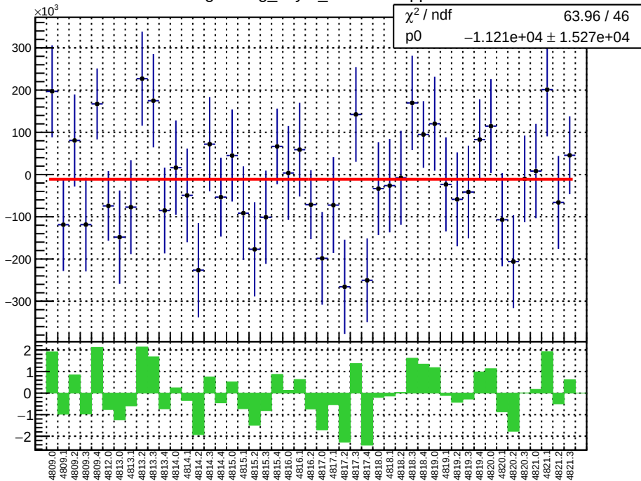
slug83: reg_asym_atr2.mean/ppb
