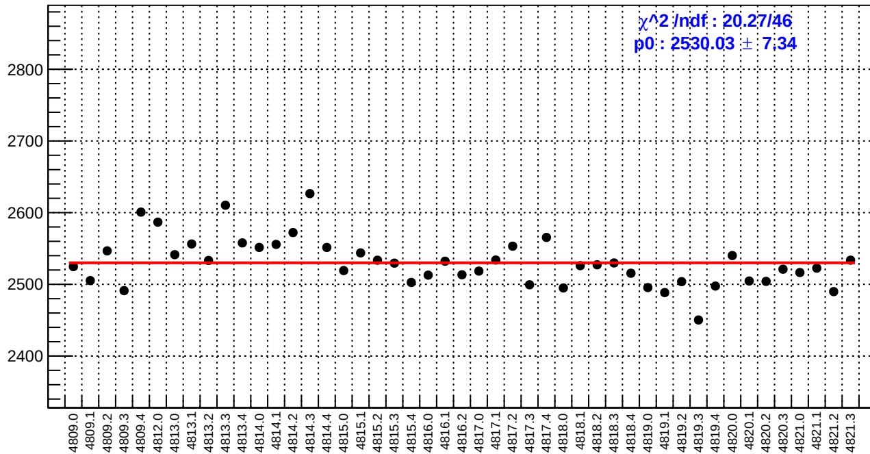
slug83: reg_asym_sam2.rms/ppm
