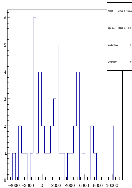
slug83: 1D Corr asym_ds_dd.mean/ppb-reg_asym_ds_dd.mean/ppb
