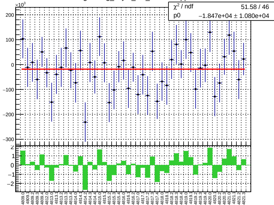
slug83: reg_asym_at2_dd.mean/ppb
