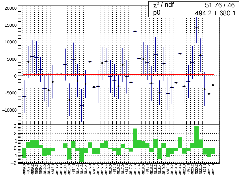
slug83: reg_asym_sam8.mean/ppb
