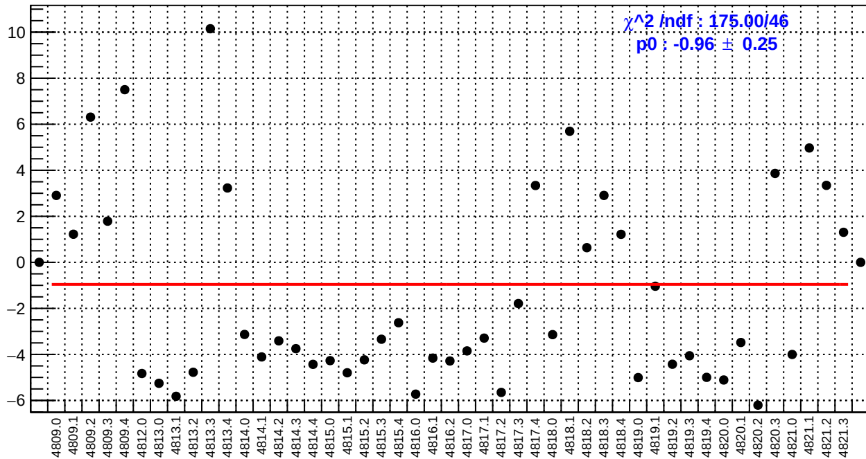
slug83: us_avg_bpm4aY/(ppb/nm)
