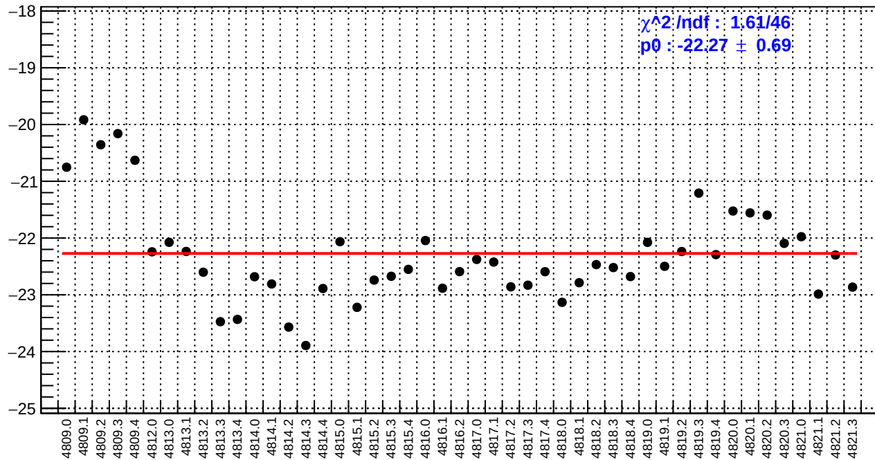
slug83: us_avg_bpm4eX/(ppb/nm)
