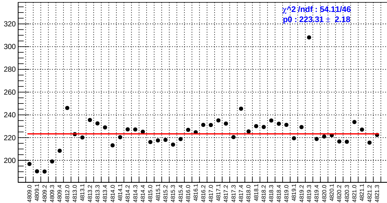
slug83: reg_asym_sam5.rms/ppm
