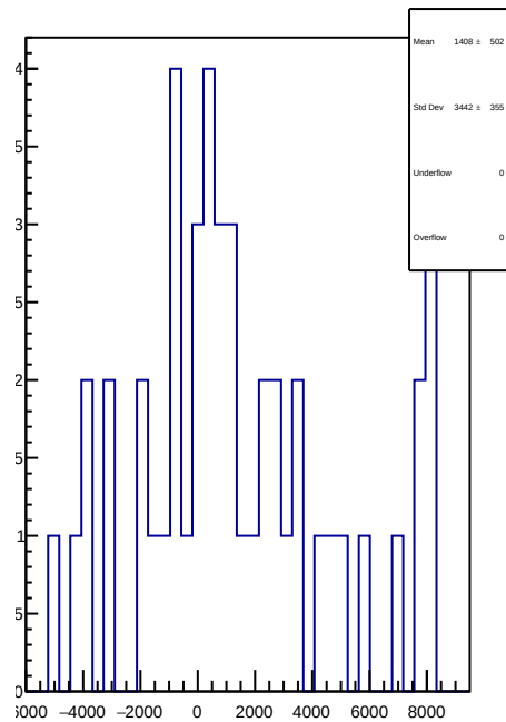
slug83: 1D Corr asym_atl1.mean/ppb-reg_asym_atl1.mean/ppb
