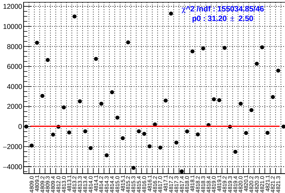
slug83: asym_atl1r2_dd.mean/ppb-reg_asym_atl1r2_dd.mean/ppb
