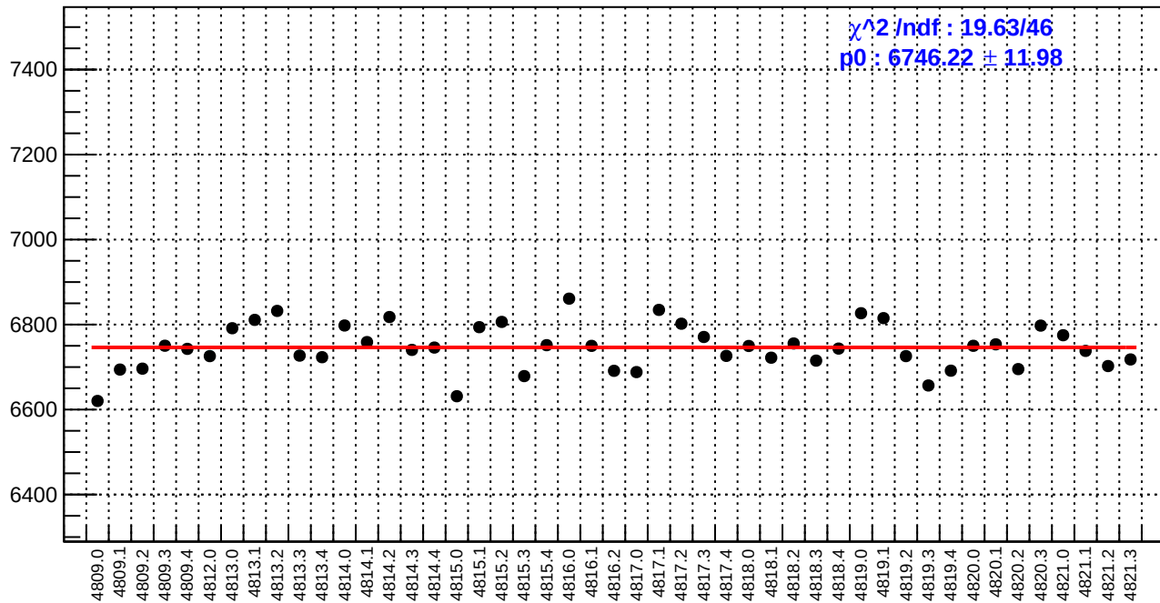
slug83: reg_asym_atl1r2_avg.rms/ppm
