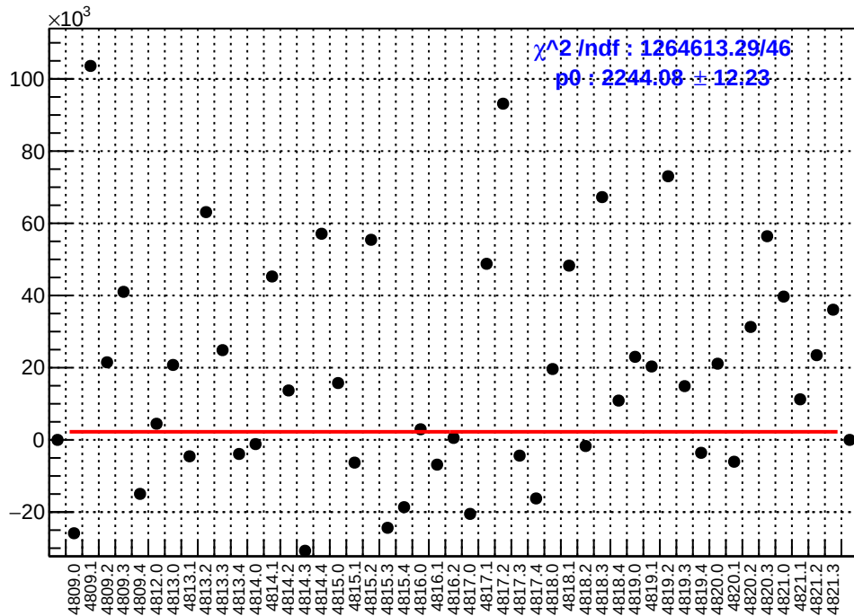
slug83: asym_sam4.mean/ppb-reg_asym_sam4.mean/ppb
