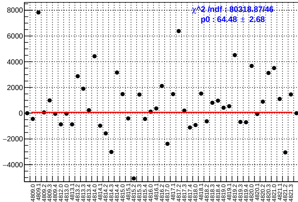
slug83: asym_atr1l2_avg.mean/ppb-reg_asym_atr1l2_avg.mean/ppb
