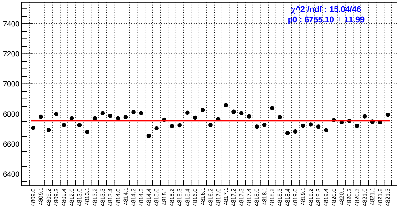
slug83: reg_asym_atl1r2_dd.rms/ppm
