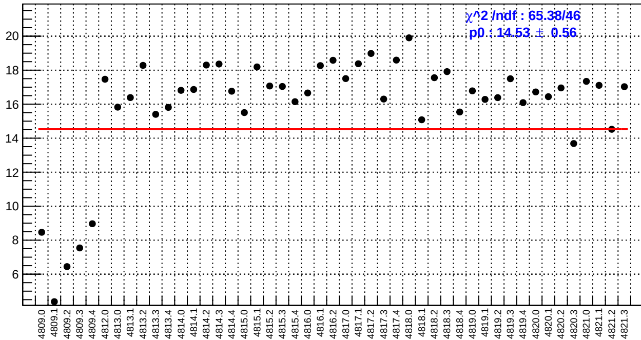
slug83: us_avg_bpm4aX/(ppb/nm)
