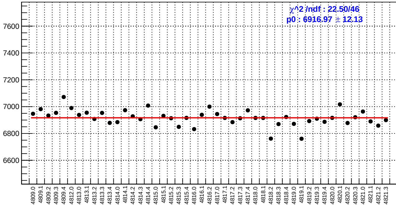
slug83: reg_asym_atr1l2_dd.rms/ppm
