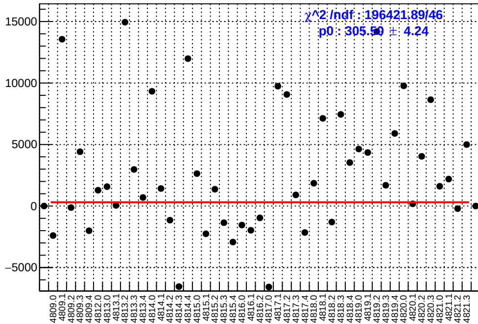
slug83: asym_dsl.mean/ppb-reg_asym_dsl.mean/ppb
