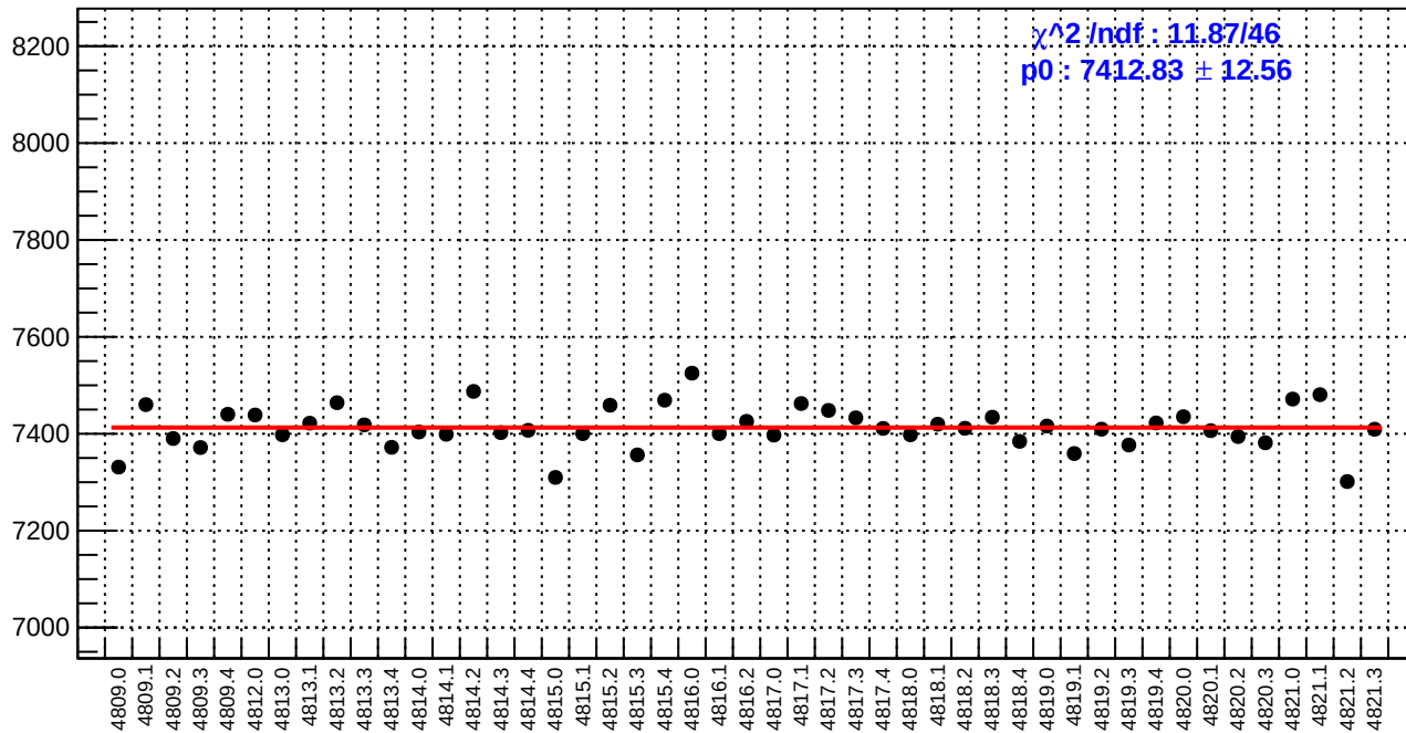
slug83: reg_asym_at2_avg.rms/ppm
