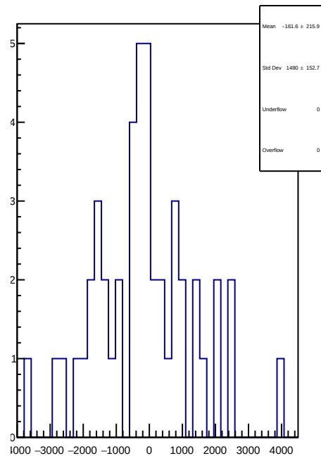
slug83: 1D Corr asym_at1_avg.mean/ppb-reg_asym_at1_avg.mean/ppb
