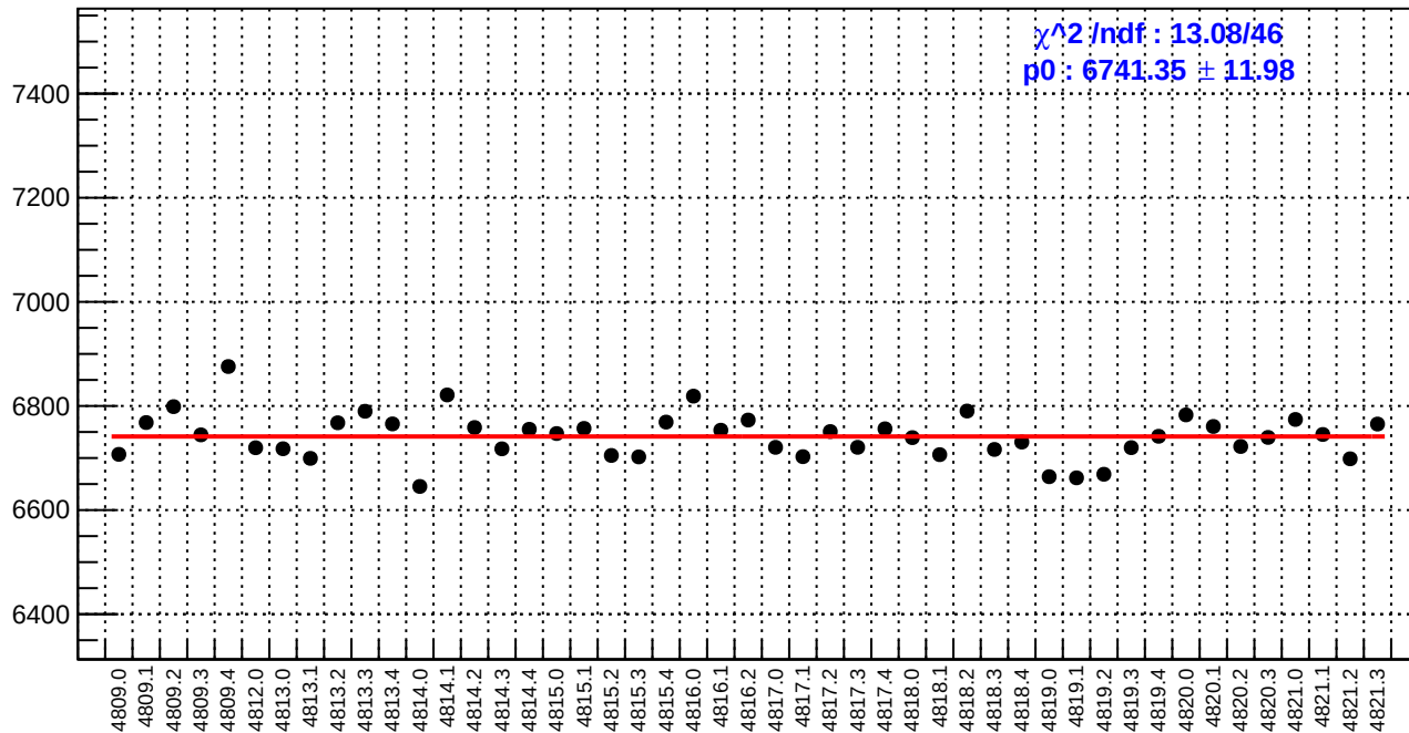
slug83: reg_asym_atl_dd.rms/ppm
