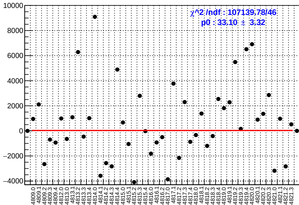
slug83: asym_us_avg.mean/ppb-reg_asym_us_avg.mean/ppb
