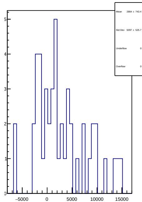
slug83: 1D Corr asym_dsl.mean/ppb-reg_asym_dsl.mean/ppb
