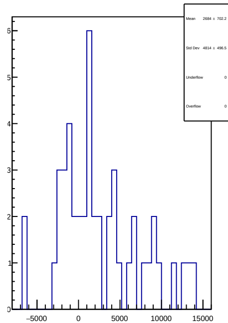
slug83: 1D Corr asym_usl.mean/ppb-reg_asym_usl.mean/ppb
