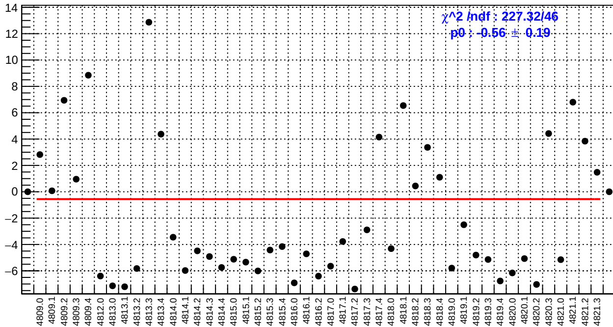
slug83: ds_avg_bpm4aY/(ppb/nm)
