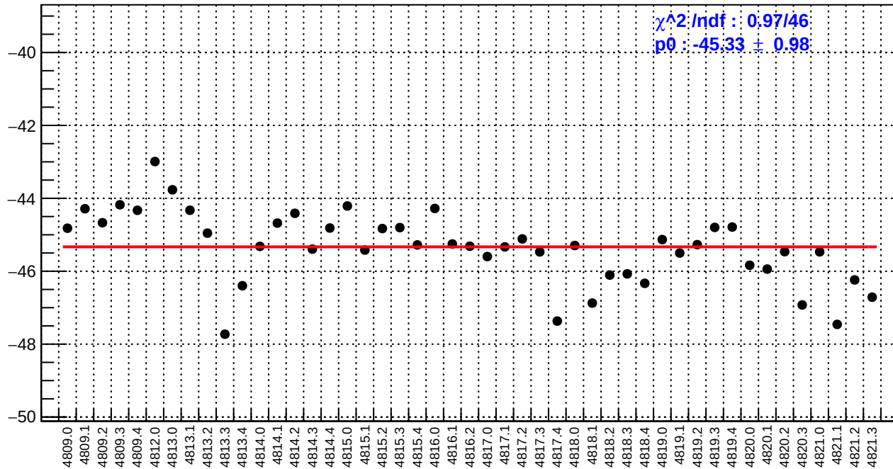
slug83: left_avg_bpm12X/(ppb/nm)
