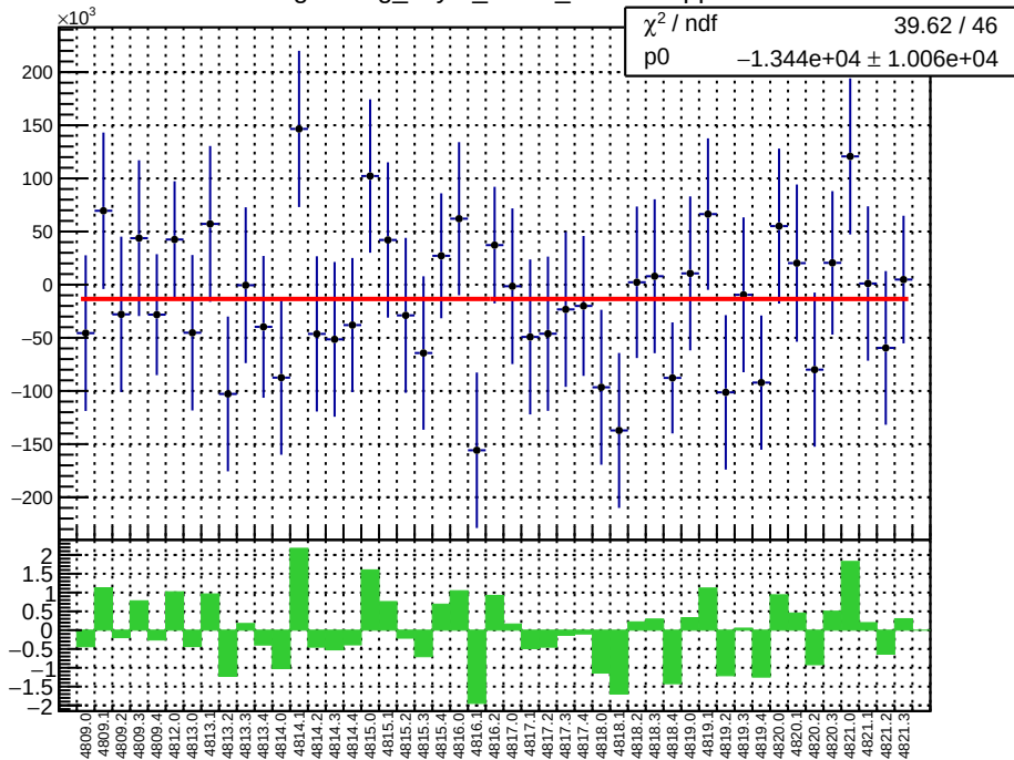
slug83: reg_asym_atr1l2_dd.mean/ppb
