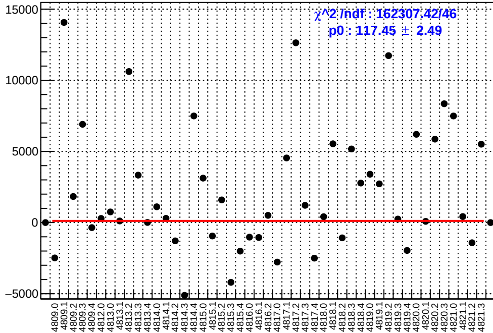
slug83: asym_atl_avg.mean/ppb-reg_asym_atl_avg.mean/ppb
