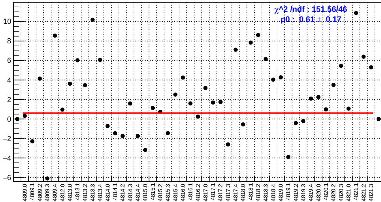
slug83: right_avg_bpm4eY/(ppb/nm)
