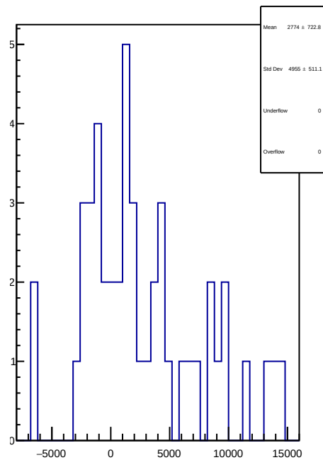
slug83: 1D Corr asym_left_avg.mean/ppb-reg_asym_left_avg.mean/ppb
