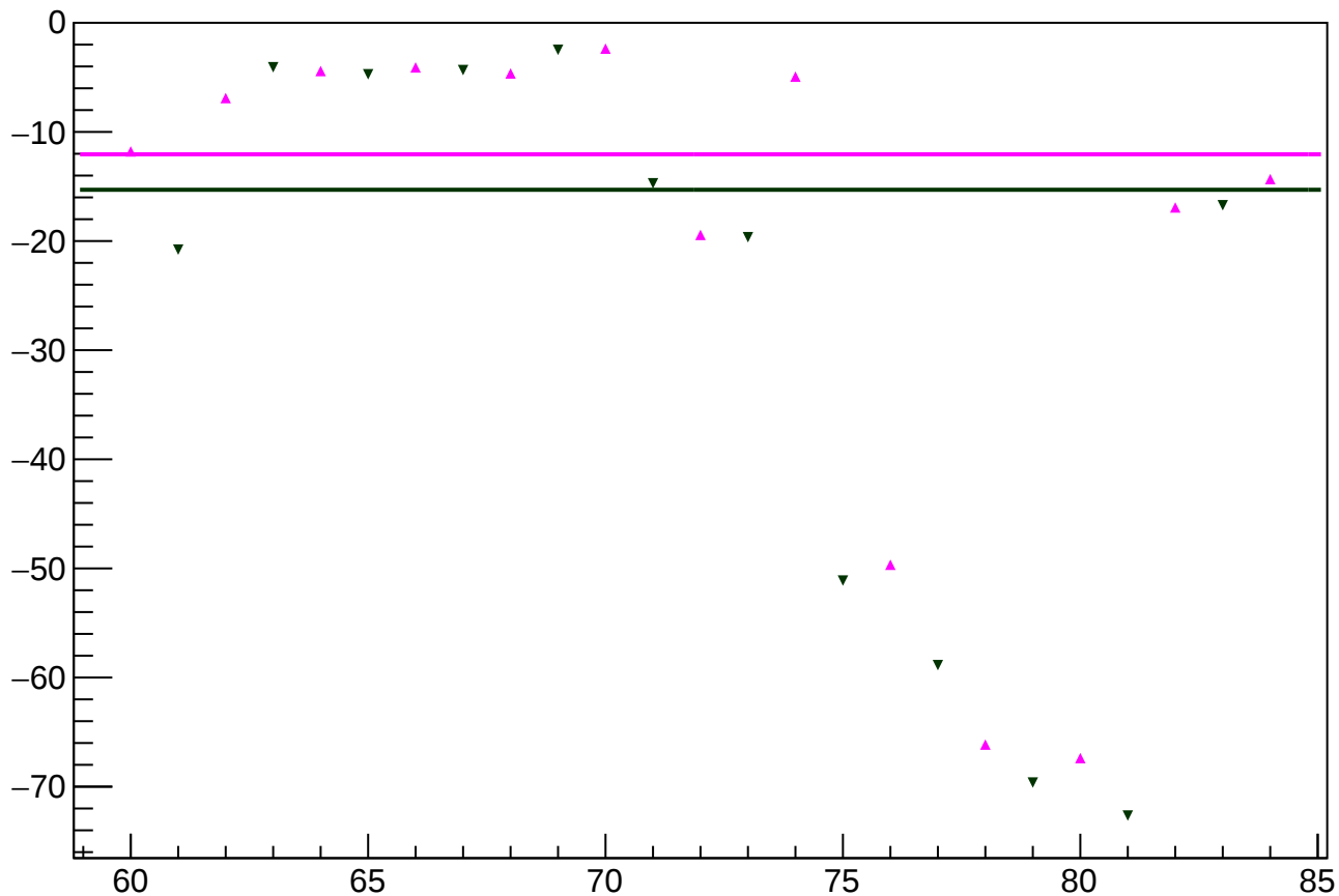
reg_asym_bcm_an_ds_diff_bpm4aX_slope vs slug
