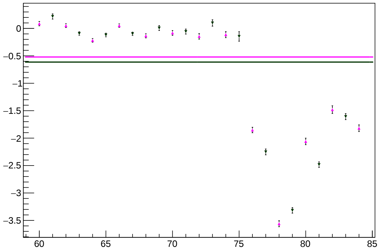
reg_bcm_dg_us_ds_dd_diff_bpm4eY_slope vs slug
