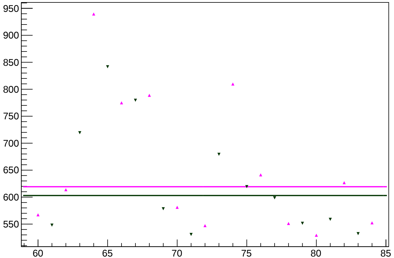
asym_left_agg_avg_rms vs slug
