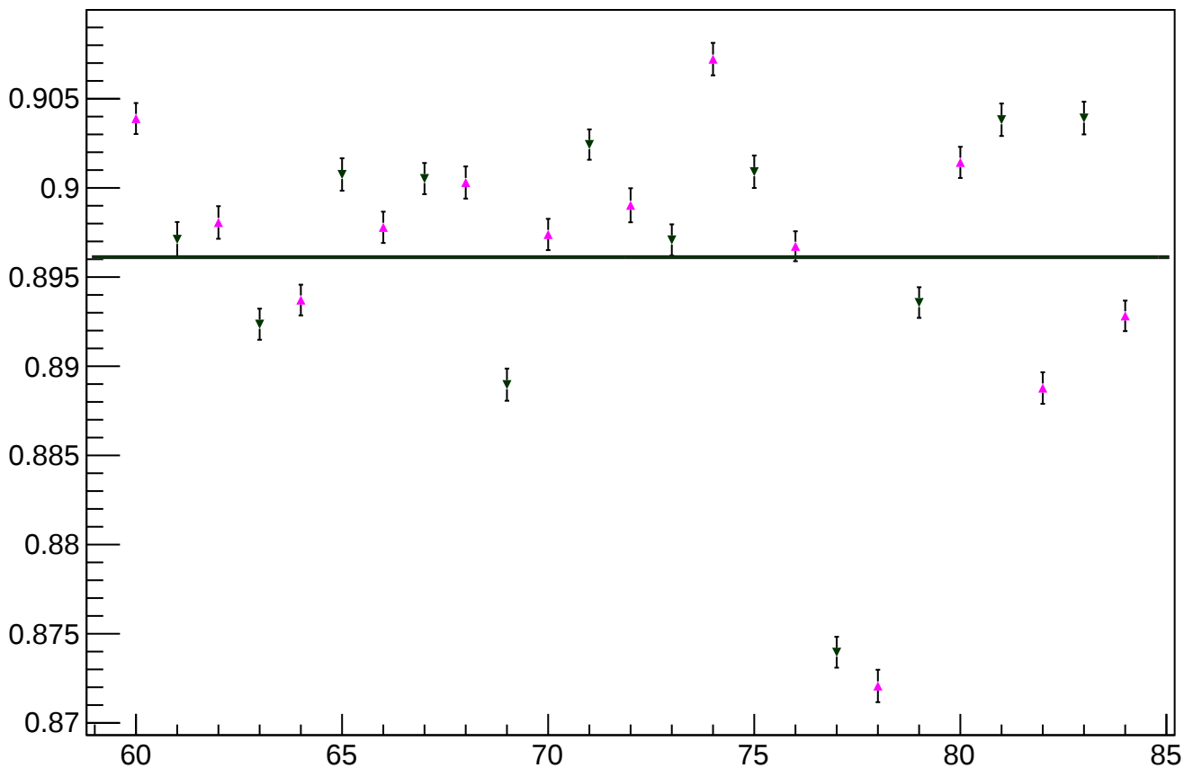
asym_cav4dQ_rms vs slug
