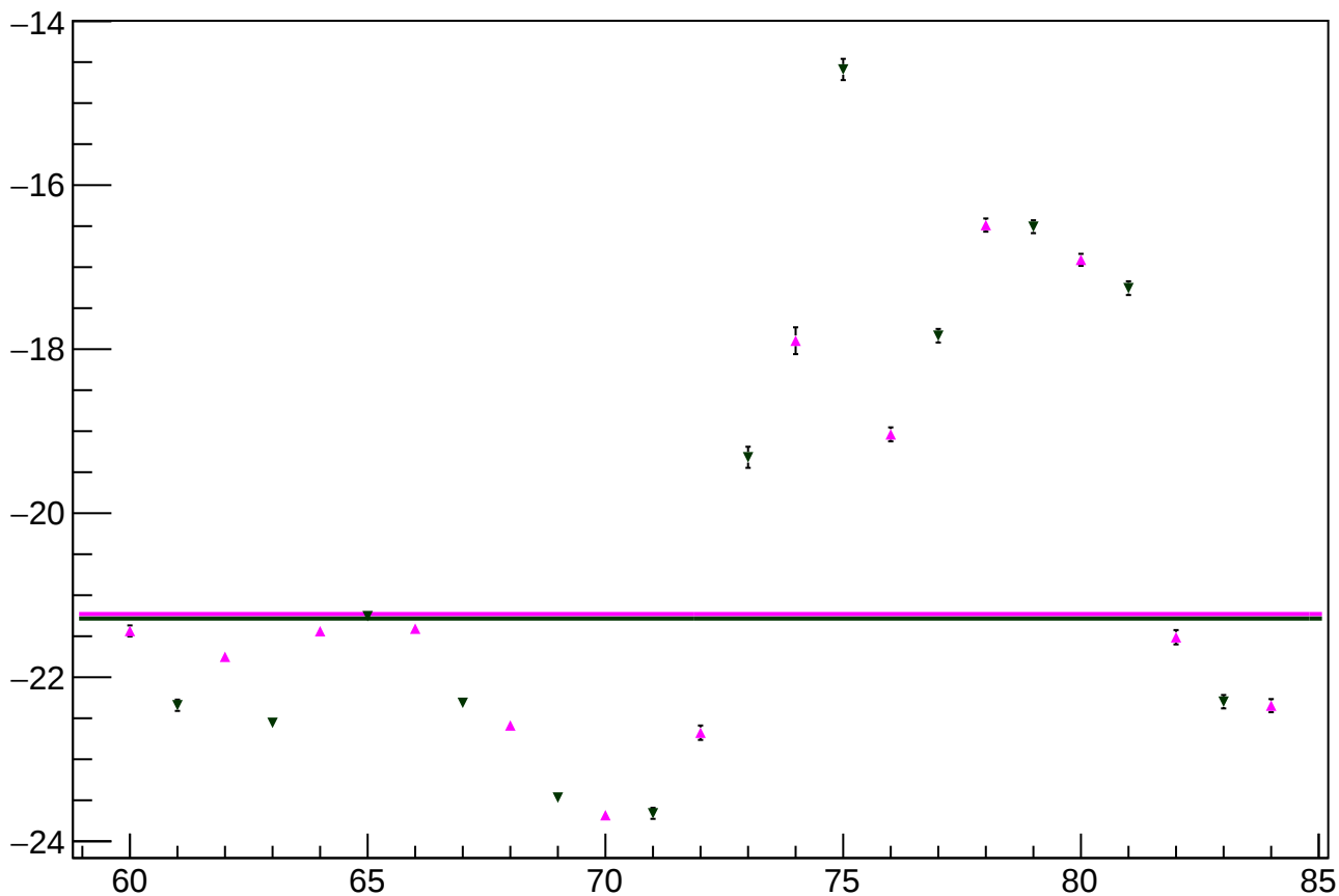
reg_asym_us_avg_diff_bpm4eX_slope vs slug
