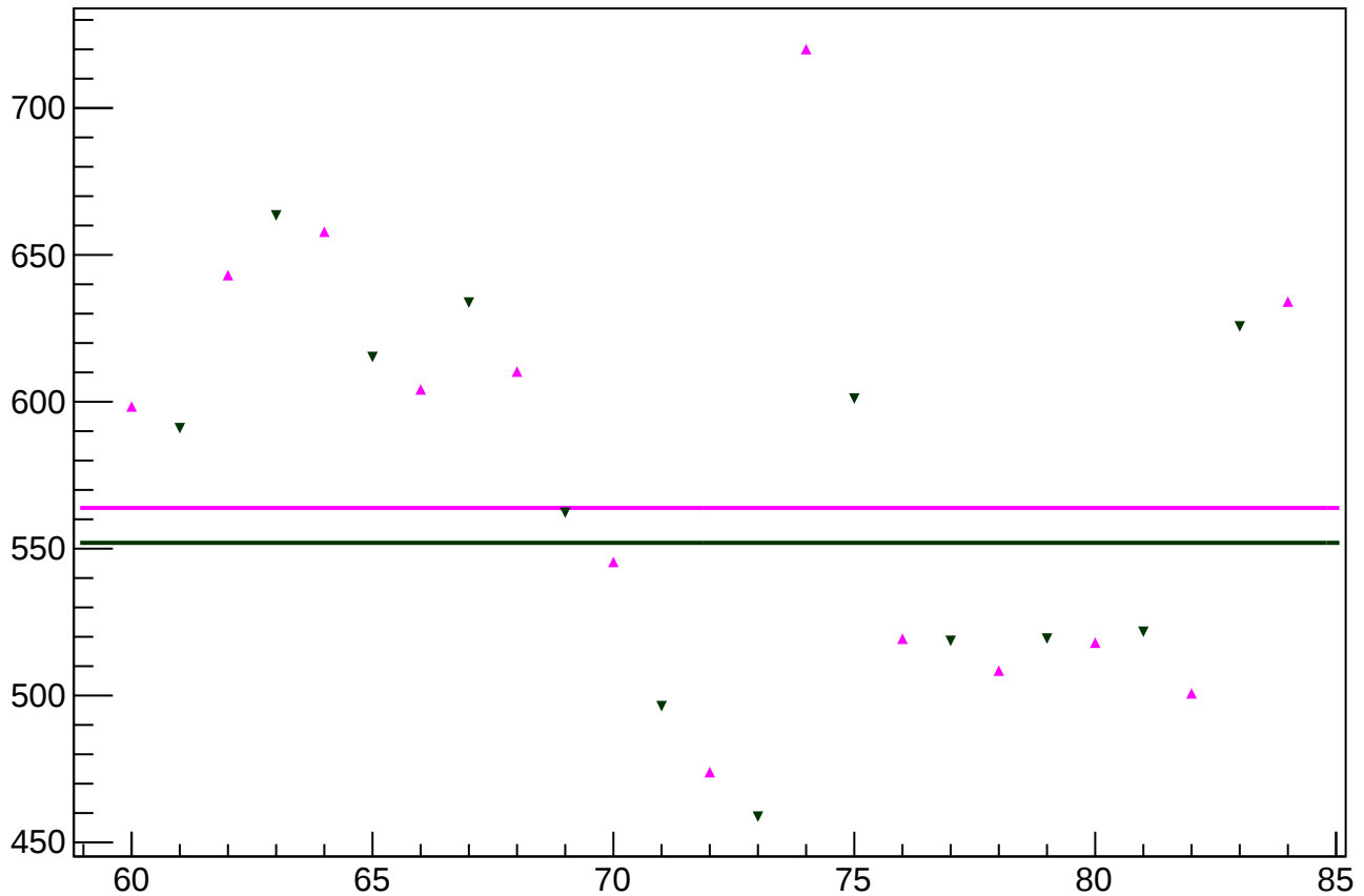
reg_asym_sam_37_avg_rms vs slug
