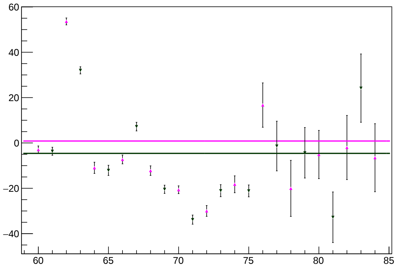
reg_asym_at2_dd_diff_bpm4eY_slope vs slug
