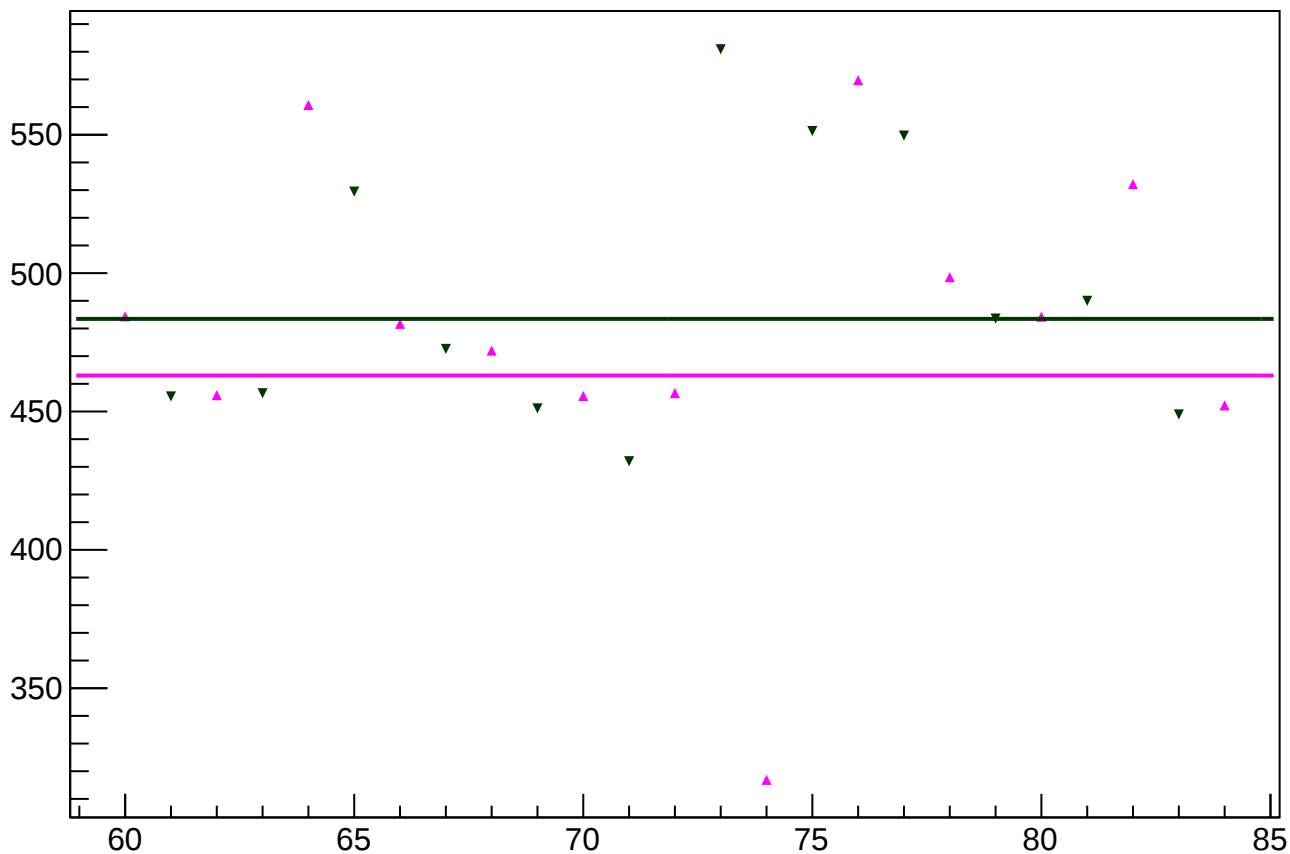
asym_right_agg_avg_rms vs slug
