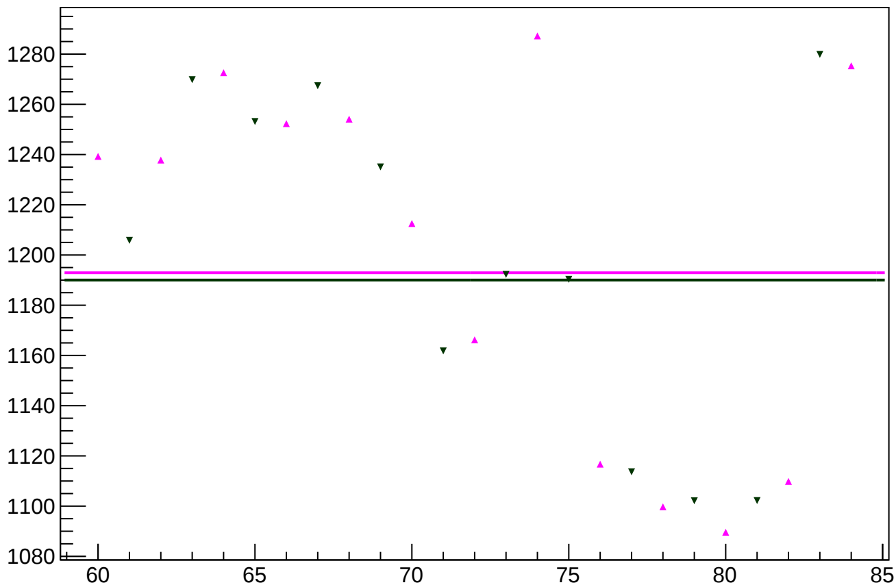
reg_asym_sam_26_avg_rms vs slug
