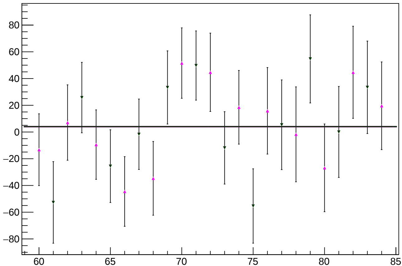
bcm_dg_us_dg_ds_dd_mean vs slug
