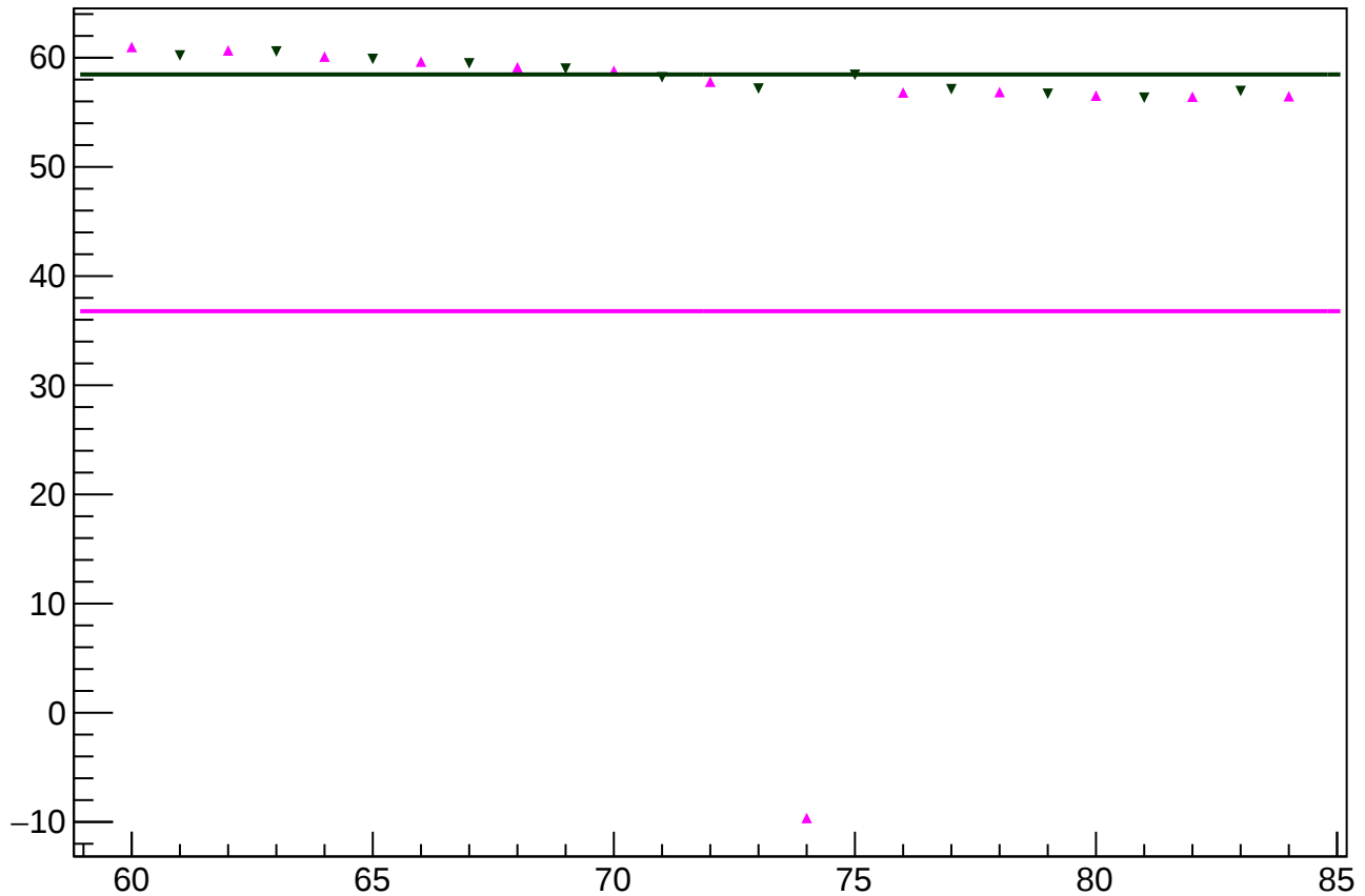
yield_usr_mean vs slug
