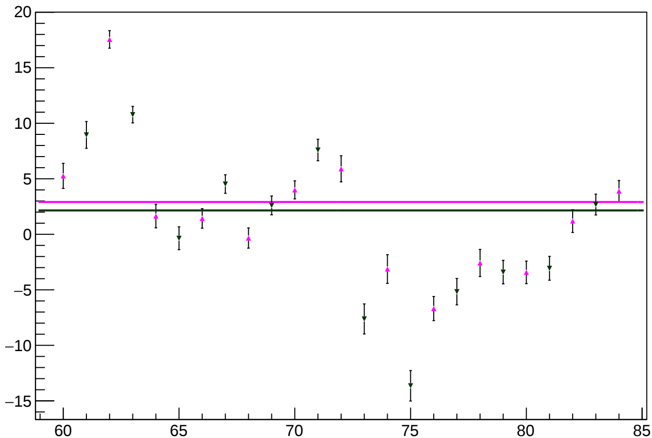
reg_asym_usr_diff_bpm4eY_slope vs slug
