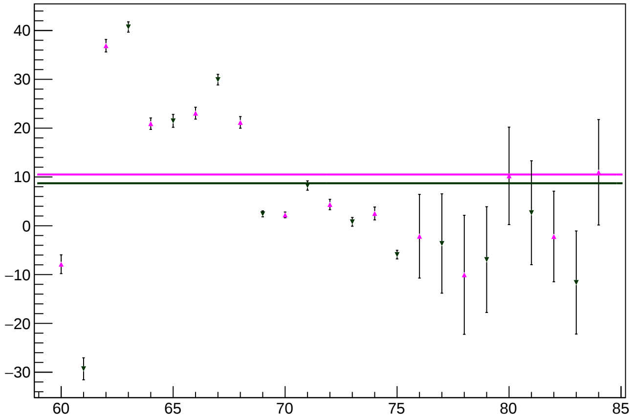
reg_asym_at1_avg_diff_bpm4aY_slope vs slug
