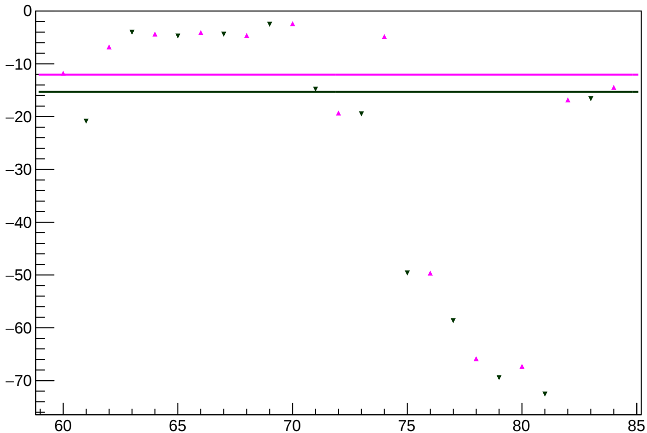
reg_asym_bcm_an_us_diff_bpm4aX_slope vs slug
