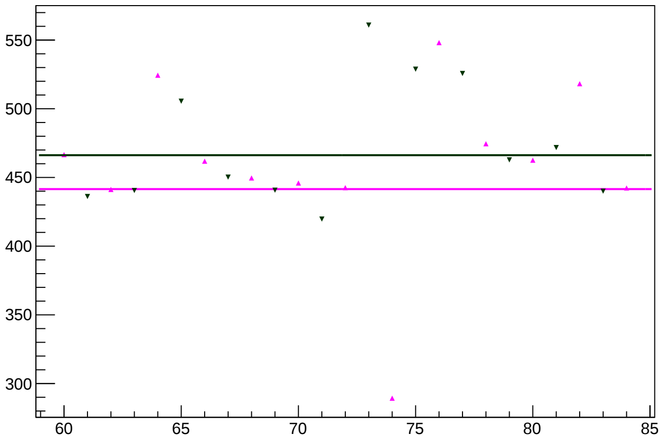
asym_dsr_rms vs slug
