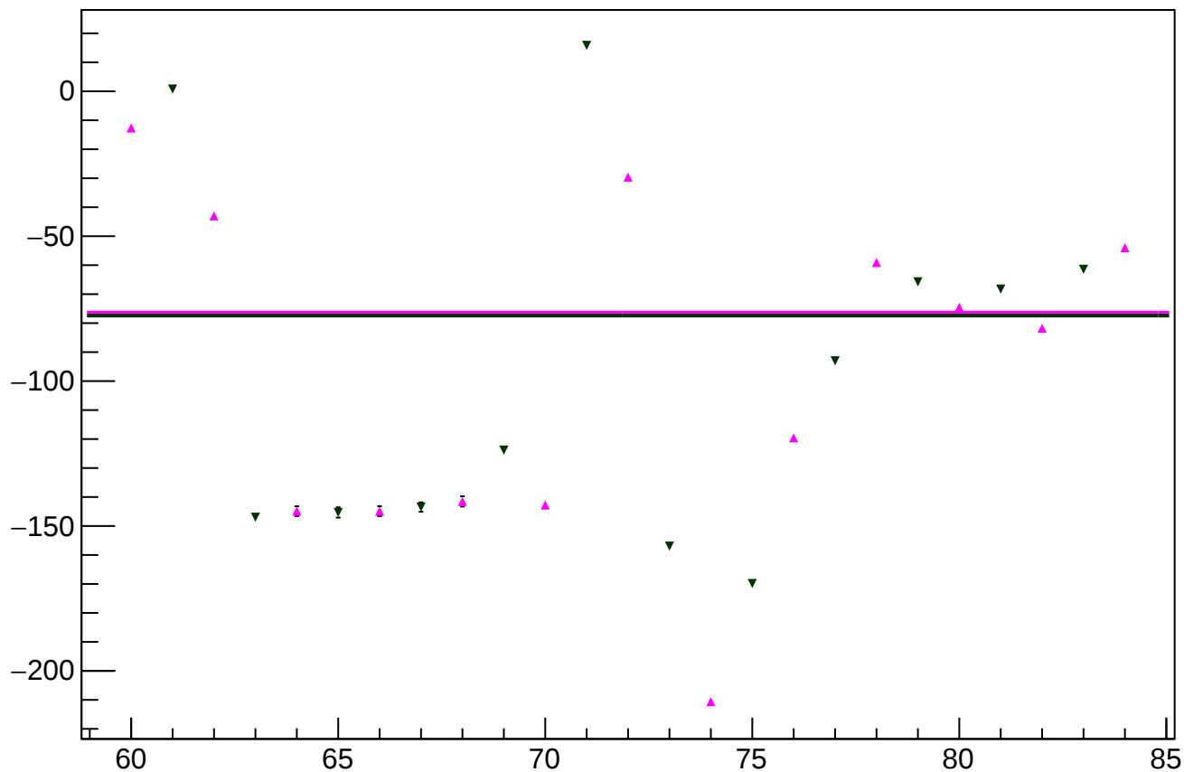
reg_asym_sam1_diff_bpm4aY_slope vs slug
