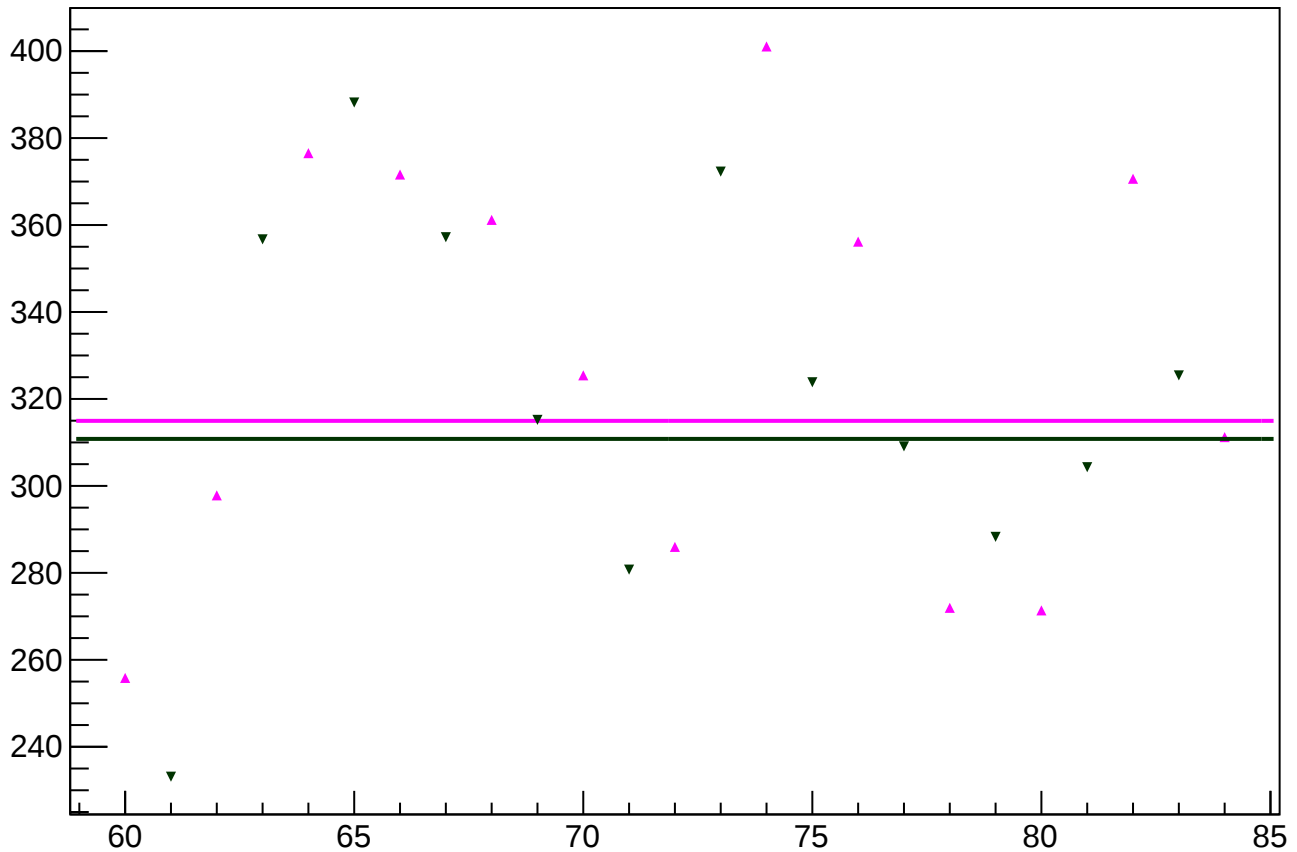
asym_ds_agg_av_rms vs slug
