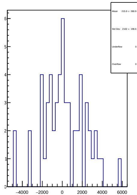
slug84: 1D Corr asym_atl1r2_avg.mean/ppb-reg_asym_atl1r2_avg.mean/ppb
