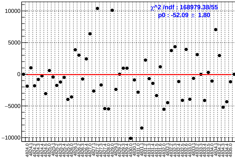
slug84: asym_ds_avg.mean/ppb-reg_asym_ds_avg.mean/ppb
