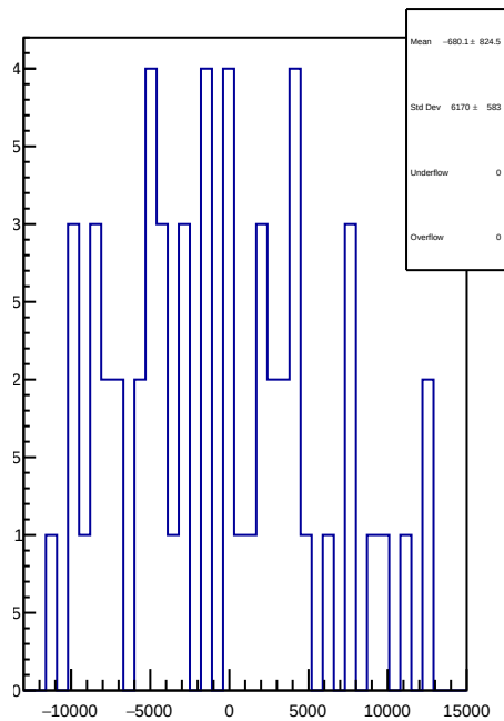
slug84: 1D Corr asym_dsl.mean/ppb-reg_asym_dsl.mean/ppb
