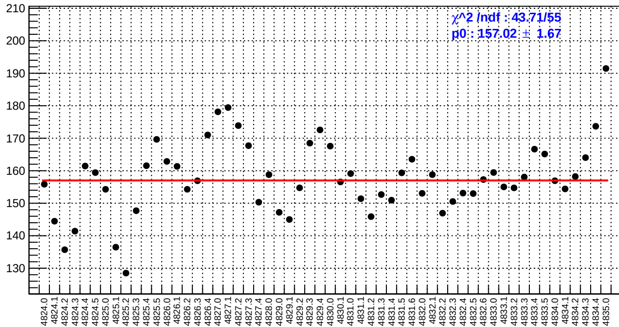
slug84: asym_bcm_an_us.rms/ppm
