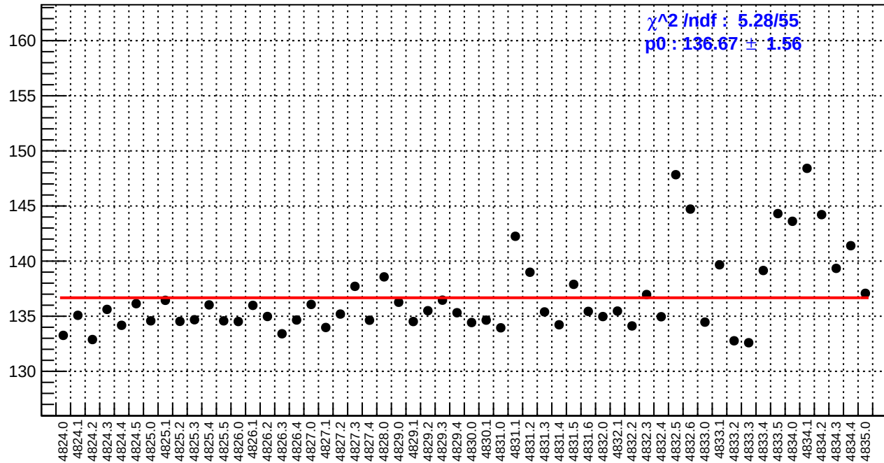
slug84: reg_asym_left_avg.rms/ppm
