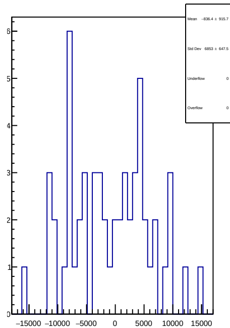
slug84: 1D Corr asym_atl2.mean/ppb-reg_asym_atl2.mean/ppb
