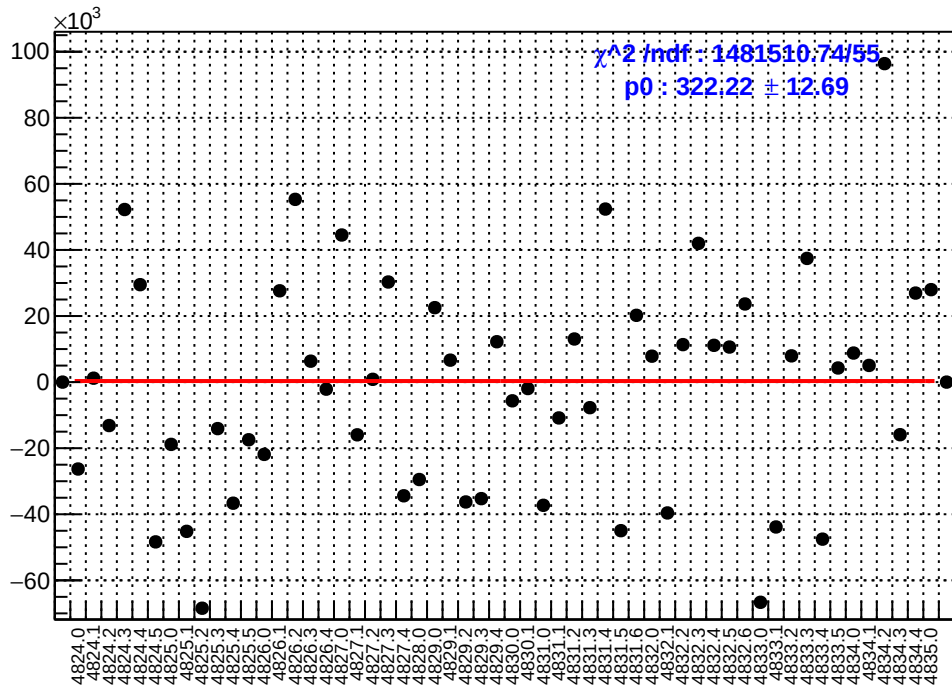
slug84: asym_sam4.mean/ppb-reg_asym_sam4.mean/ppb
