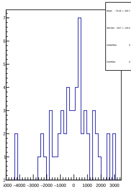
slug84: 1D Corr asym_at1_avg.mean/ppb-reg_asym_at1_avg.mean/ppb
