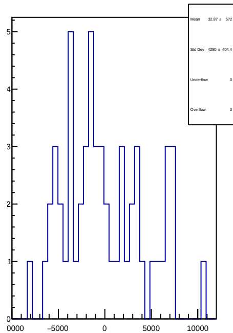
slug84: 1D Corr asym_sam5.mean/ppb-reg_asym_sam5.mean/ppb
