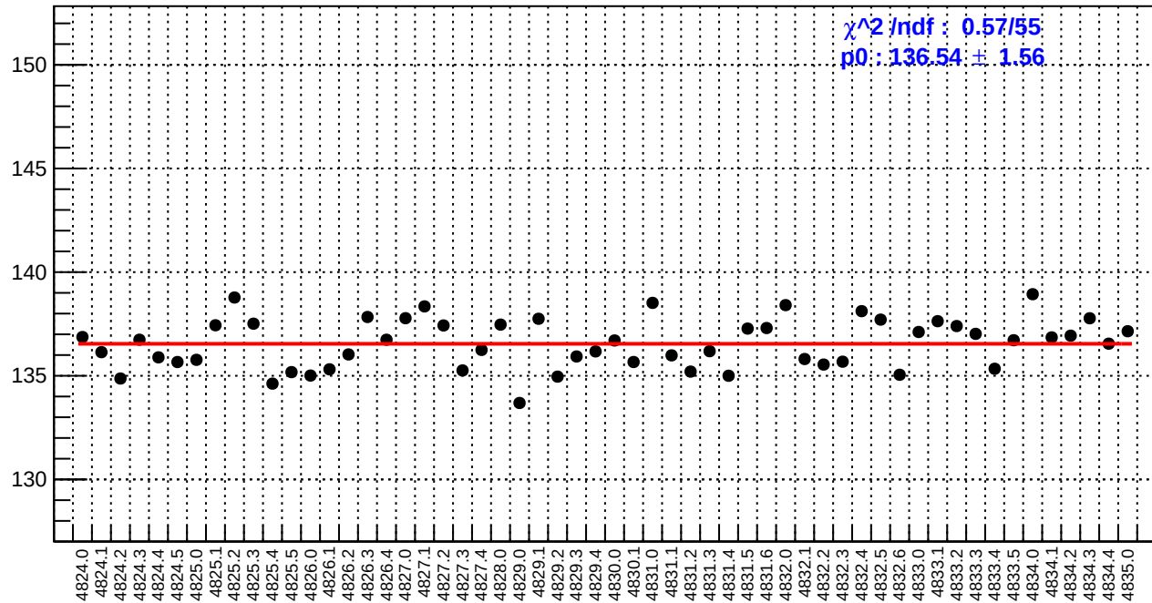
slug84: reg_asym_dsr.rms/ppm
