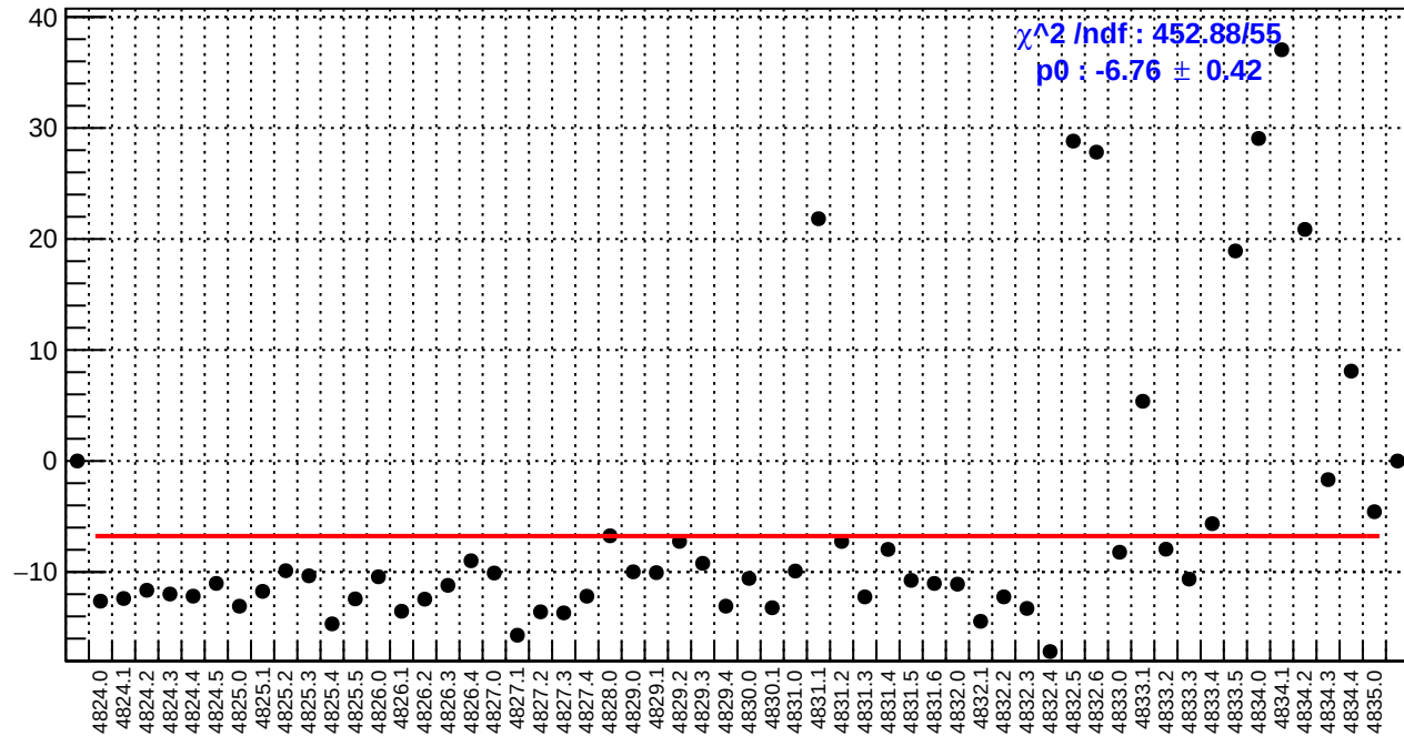
slug84: usl_bpm4aY/(ppb/nm)
