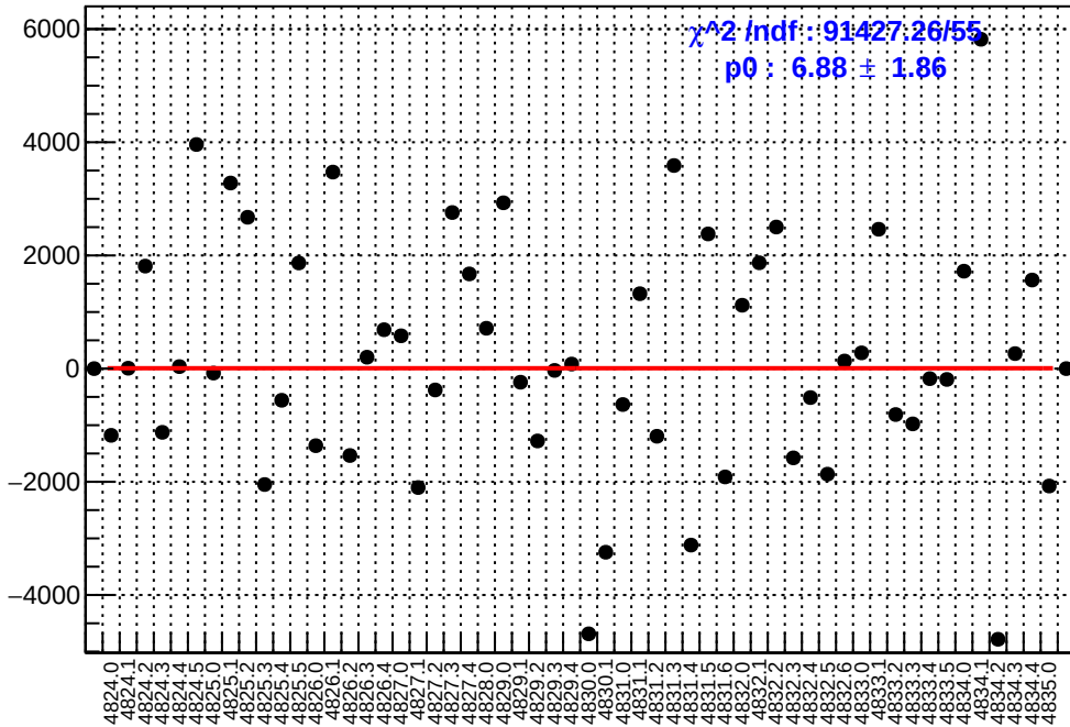
slug84: asym_atl1r2_avg.mean/ppb-reg_asym_atl1r2_avg.mean/ppb
