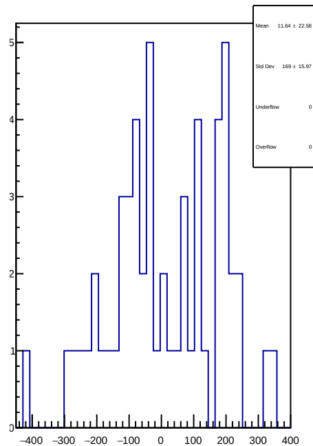
slug84: 1D Corr asym_left_dd.mean/ppb-reg_asym_left_dd.mean/ppb
