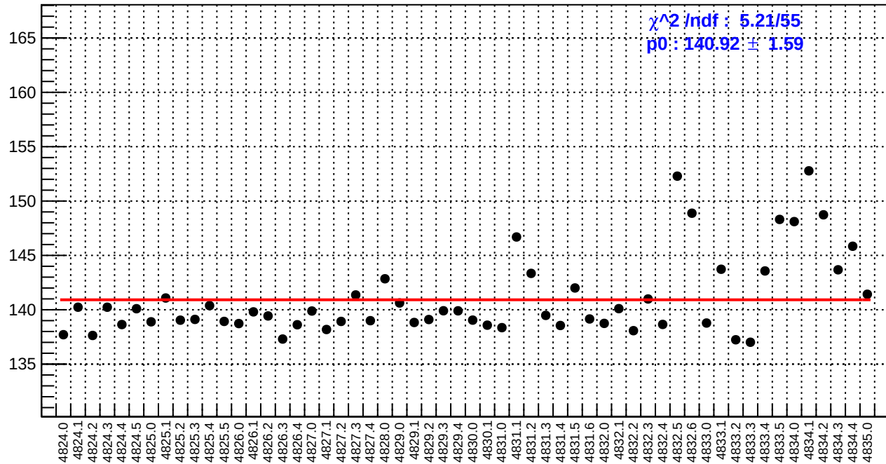
slug84: reg_asym_dsl.rms/ppm
