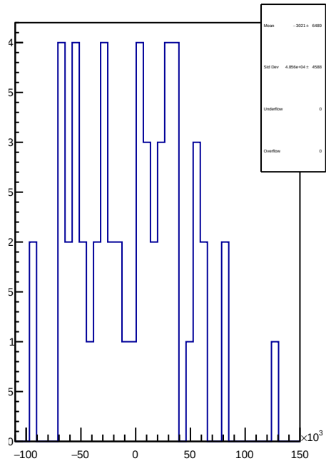
slug84: 1D Corr asym_sam2.mean/ppb-reg_asym_sam2.mean/ppb
