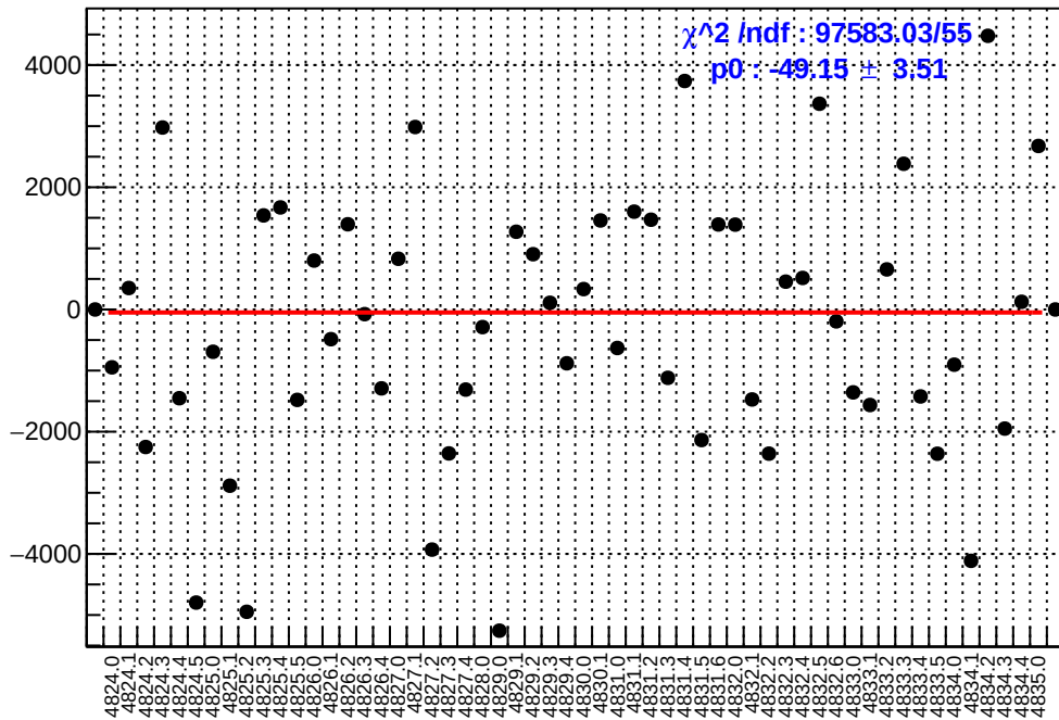
slug84: asym_atr_dd.mean/ppb-reg_asym_atr_dd.mean/ppb
