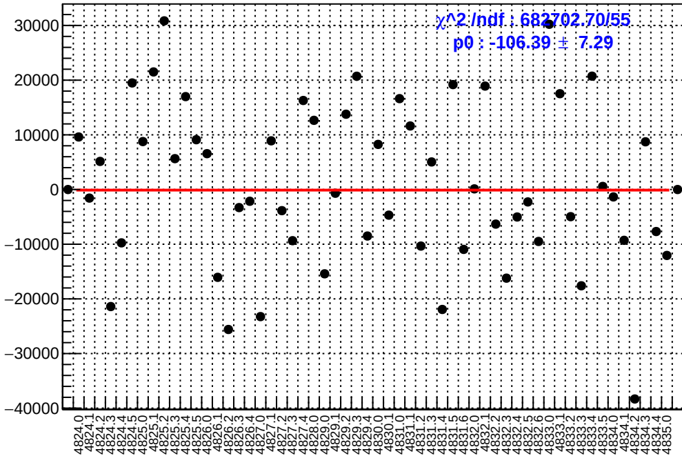
slug84: asym_sam7.mean/ppb-reg_asym_sam7.mean/ppb
