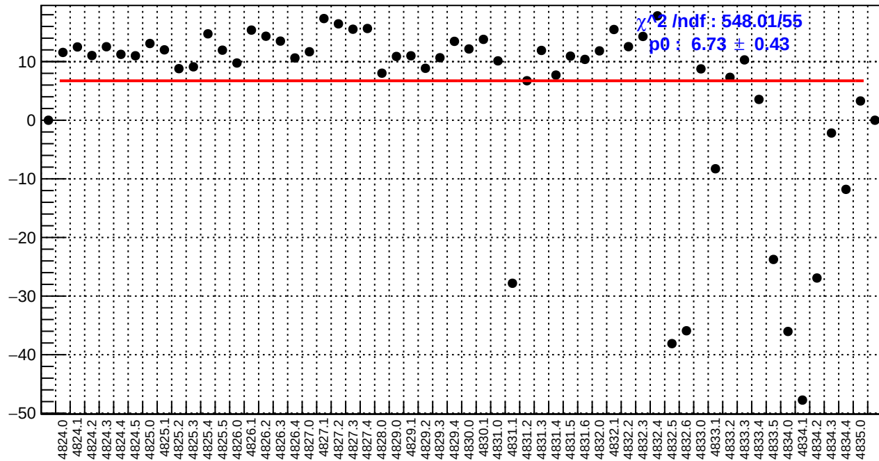
slug84: usl_bpm4eY/(ppb/nm)
