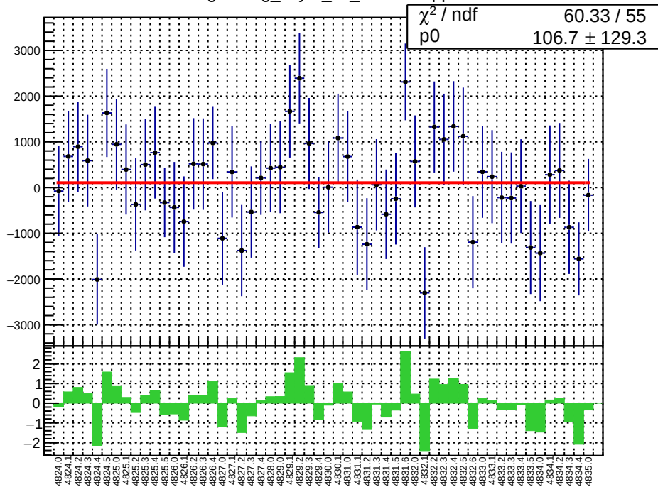
slug84: reg_asym_ds_dd.mean/ppb
