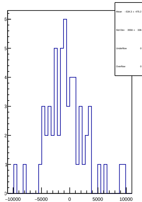
slug84: 1D Corr asym_us_avg.mean/ppb-reg_asym_us_avg.mean/ppb
