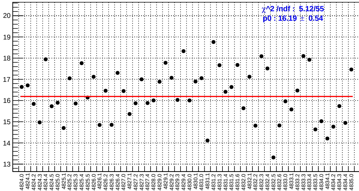
slug84: us_avg_bpm4aX/(ppb/nm)
