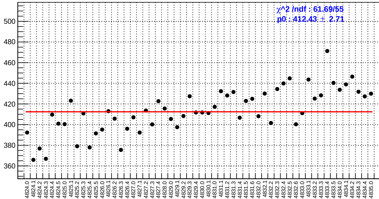
slug84: reg_asym_sam6.rms/ppm
