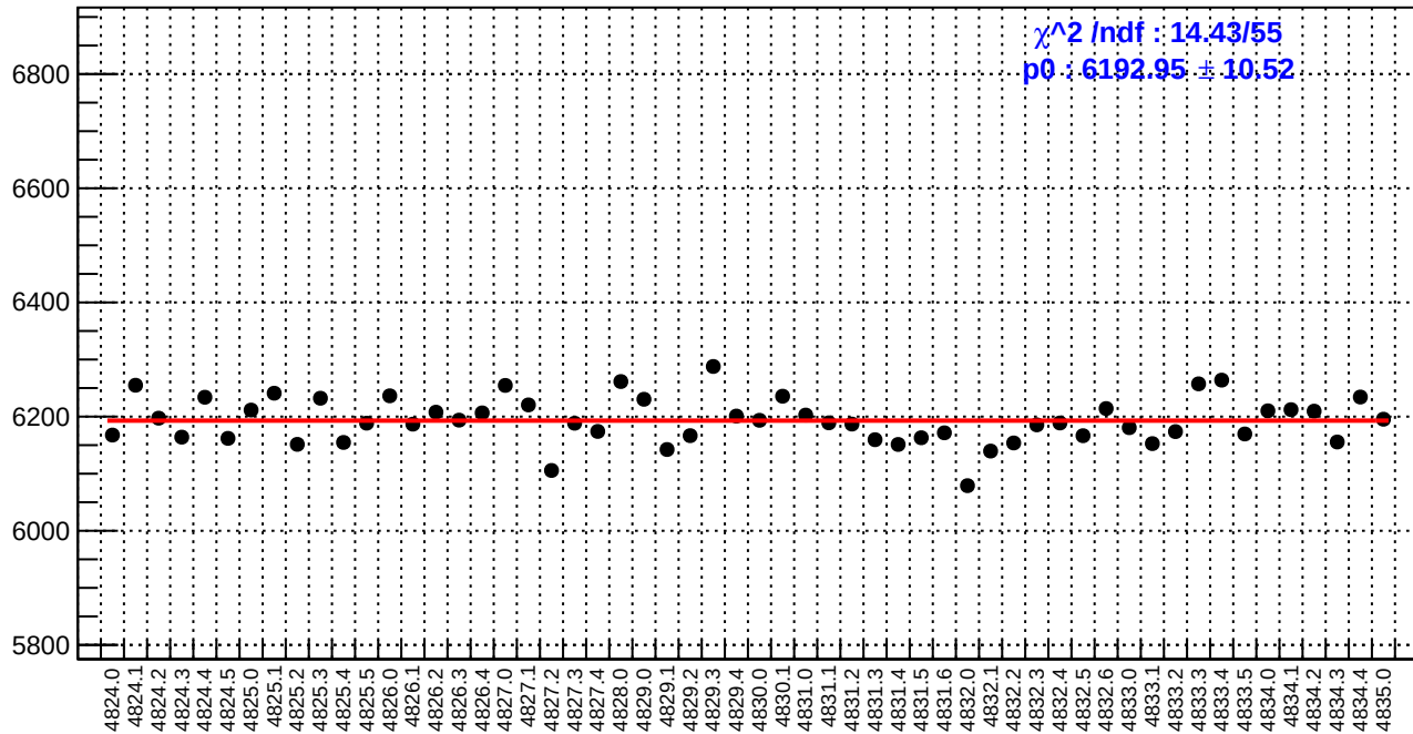
slug84: reg_asym_at1_dd.rms/ppm
