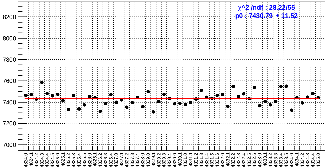
slug84: reg_asym_at2_dd.rms/ppm
