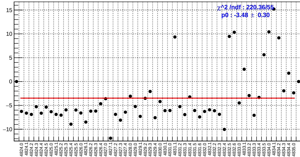
slug84: ds_avg_bpm4aY/(ppb/nm)
