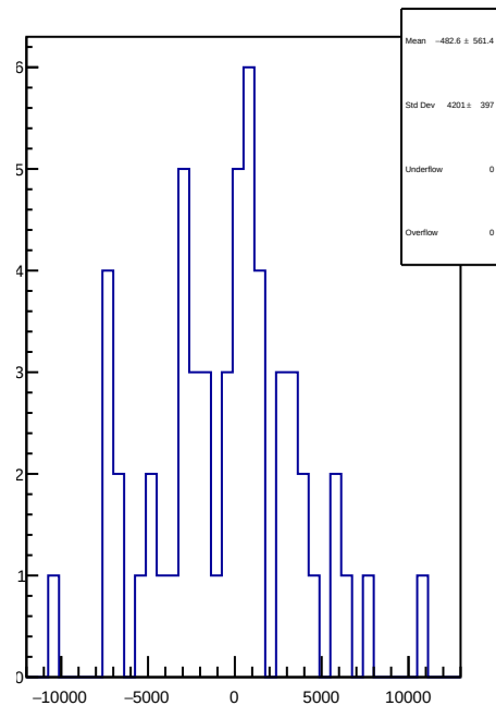
slug84: 1D Corr asym_dsr.mean/ppb-reg_asym_dsr.mean/ppb
