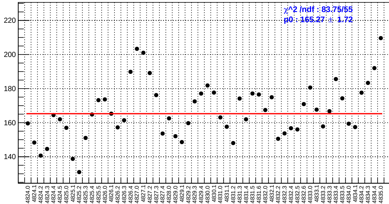
slug84: asym_bcm_an_ds3.rms/ppm
