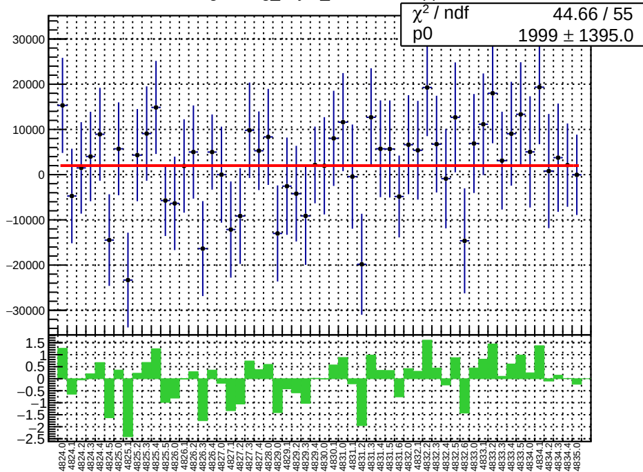
slug84: reg_asym_sam4.mean/ppb
