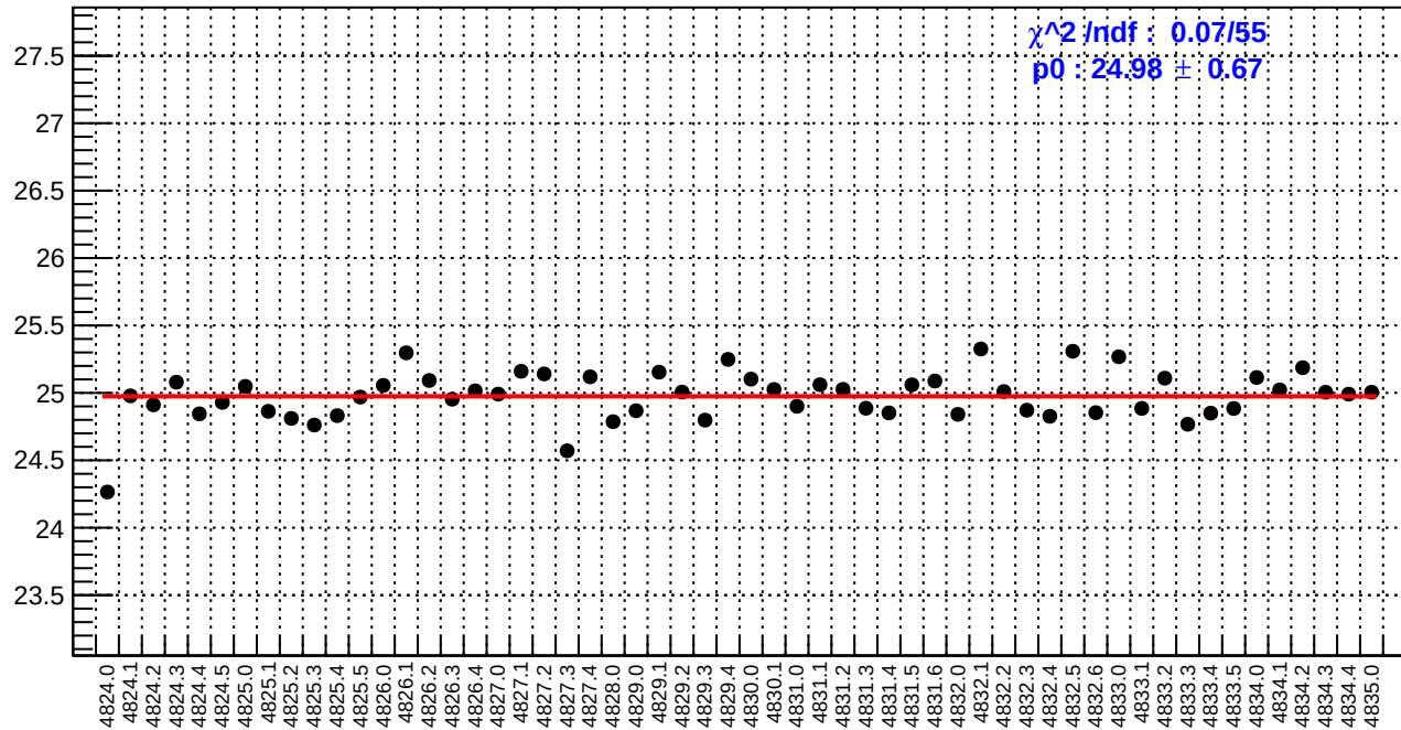
slug84: reg_asym_left_dd.rms/ppm
