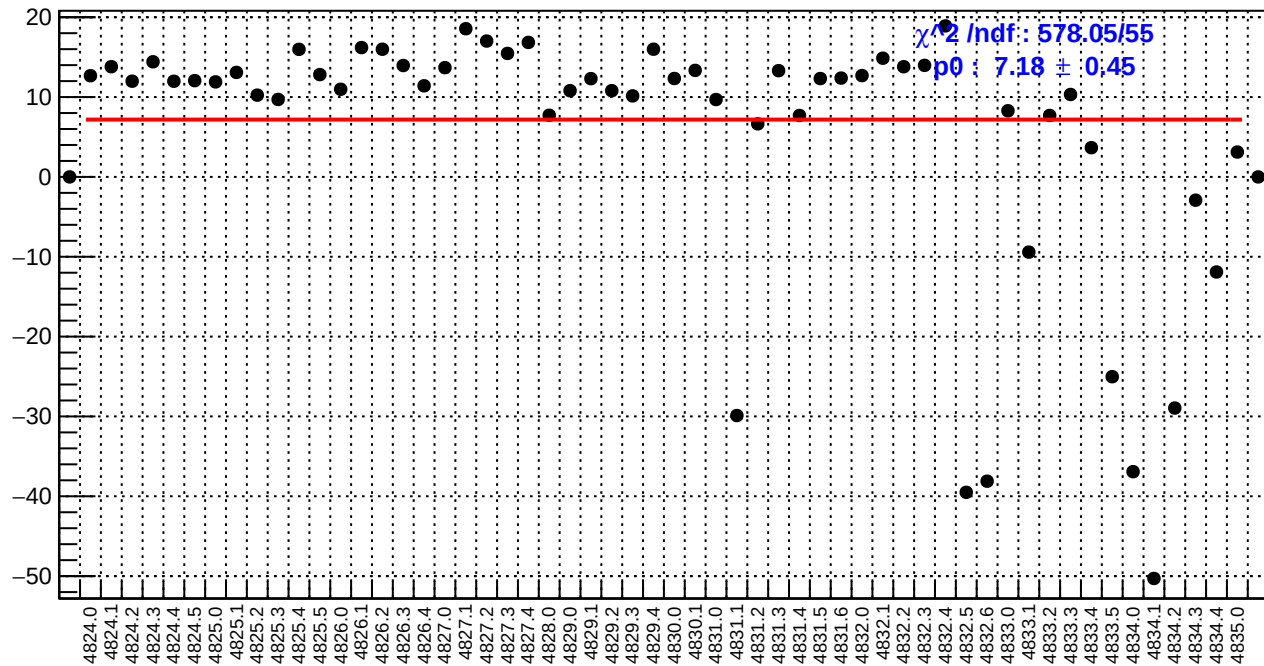
slug84: dsl_bpm4eY/(ppb/nm)
