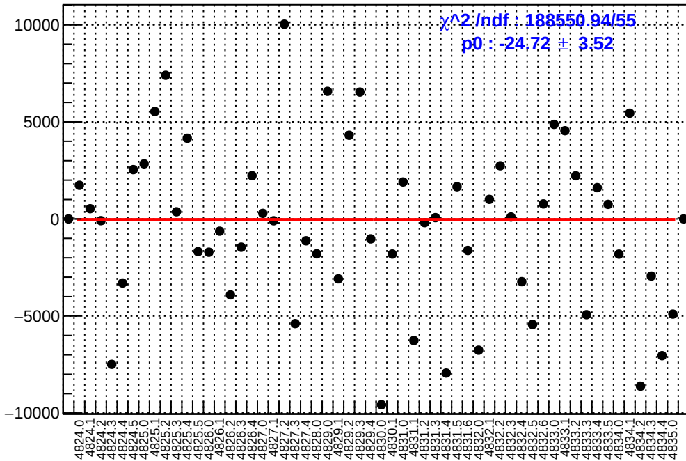
slug84: asym_usr.mean/ppb-reg_asym_usr.mean/ppb
