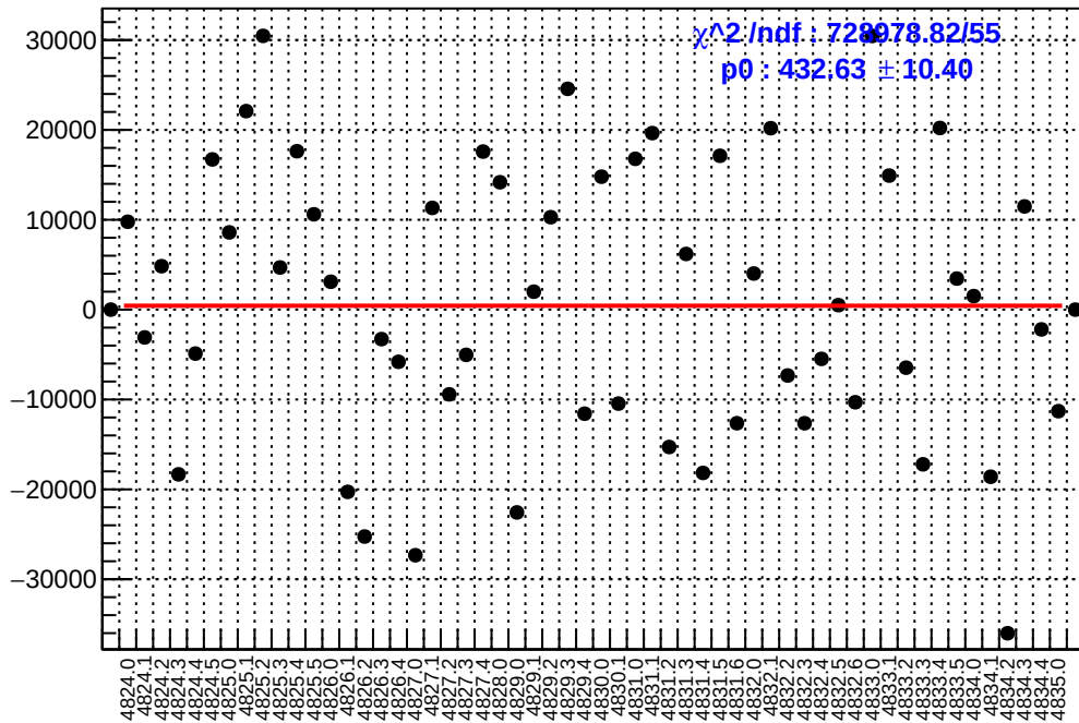
slug84: asym_sam6.mean/ppb-reg_asym_sam6.mean/ppb
