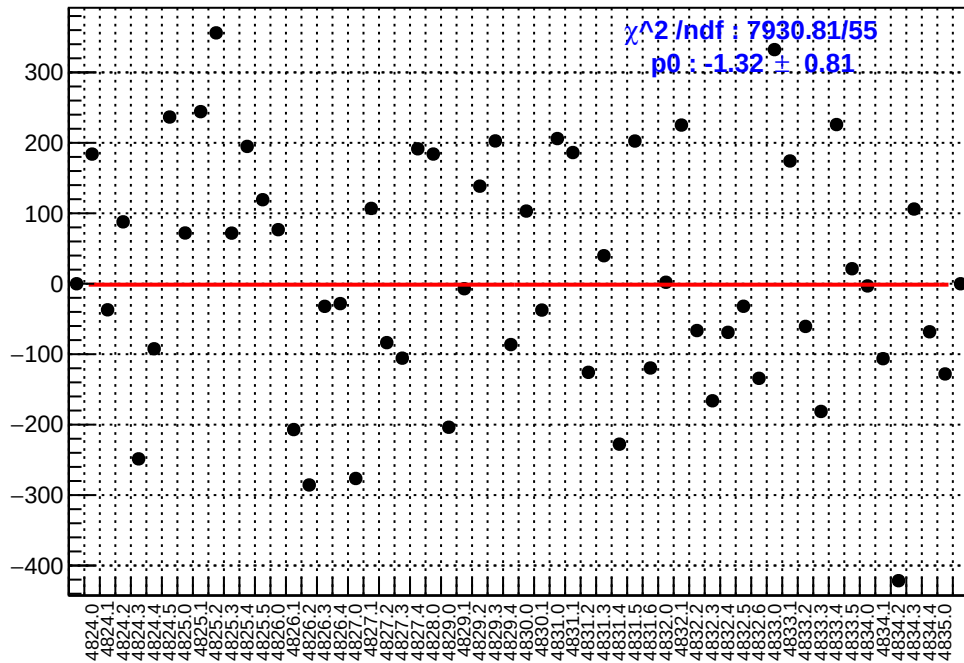
slug84: asym_left_dd.mean/ppb-reg_asym_left_dd.mean/ppb
