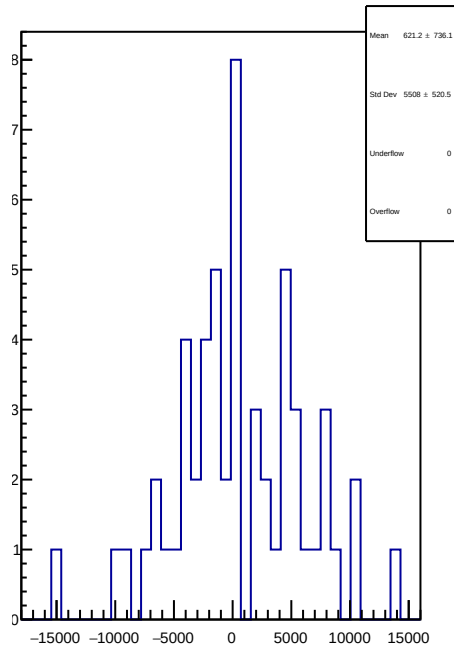
slug84: 1D Corr asym_at2_dd.mean/ppb-reg_asym_at2_dd.mean/ppb
