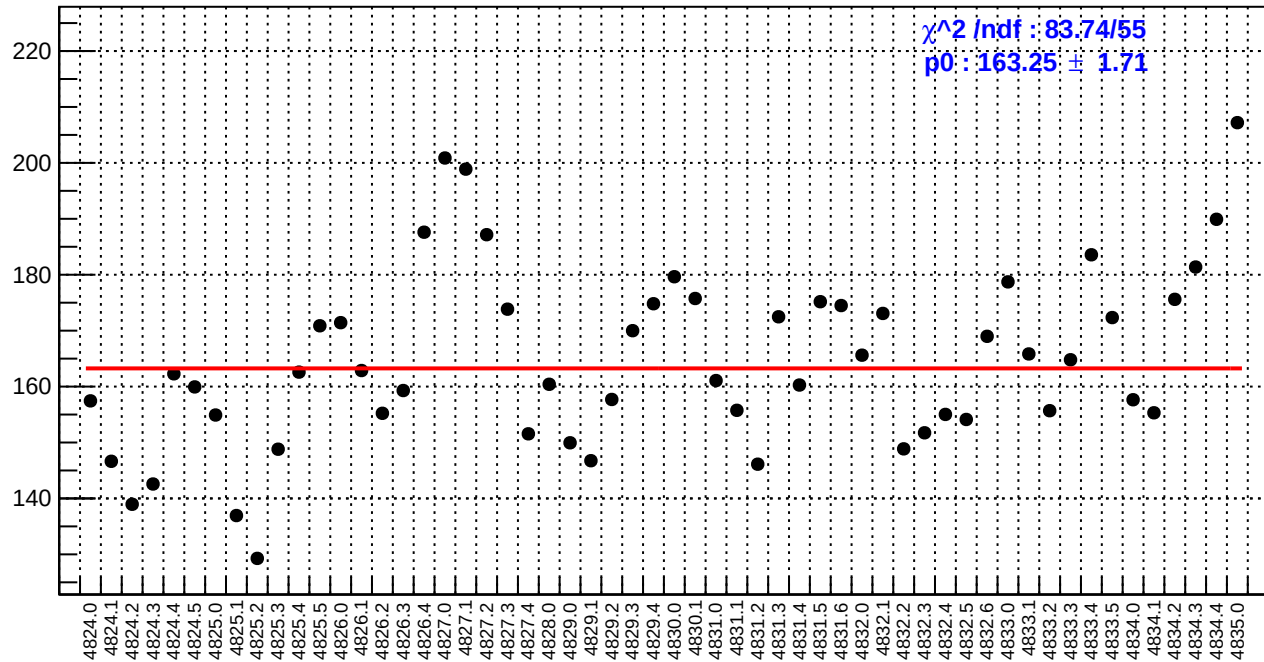
slug84: asym_bcm_an_ds.rms/ppm
