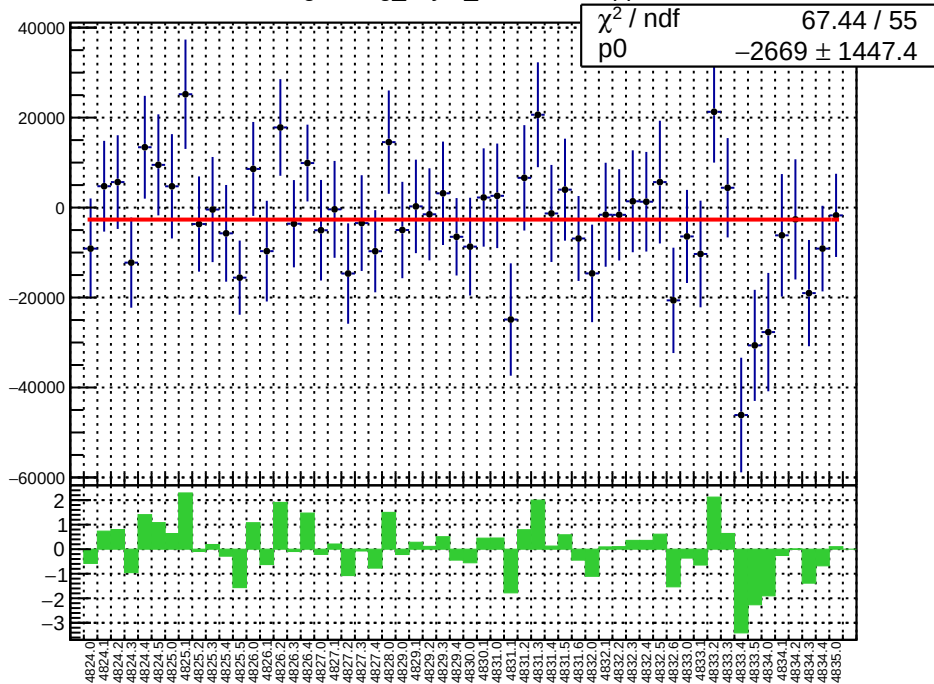
slug84: reg_asym_sam3.mean/ppb
