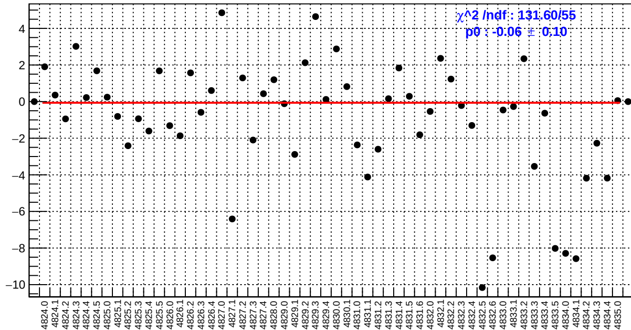
slug84: dsr_bpm4aY/(ppb/nm)
