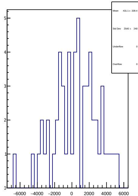
slug84: 1D Corr asym_atl_dd.mean/ppb-reg_asym_atl_dd.mean/ppb
