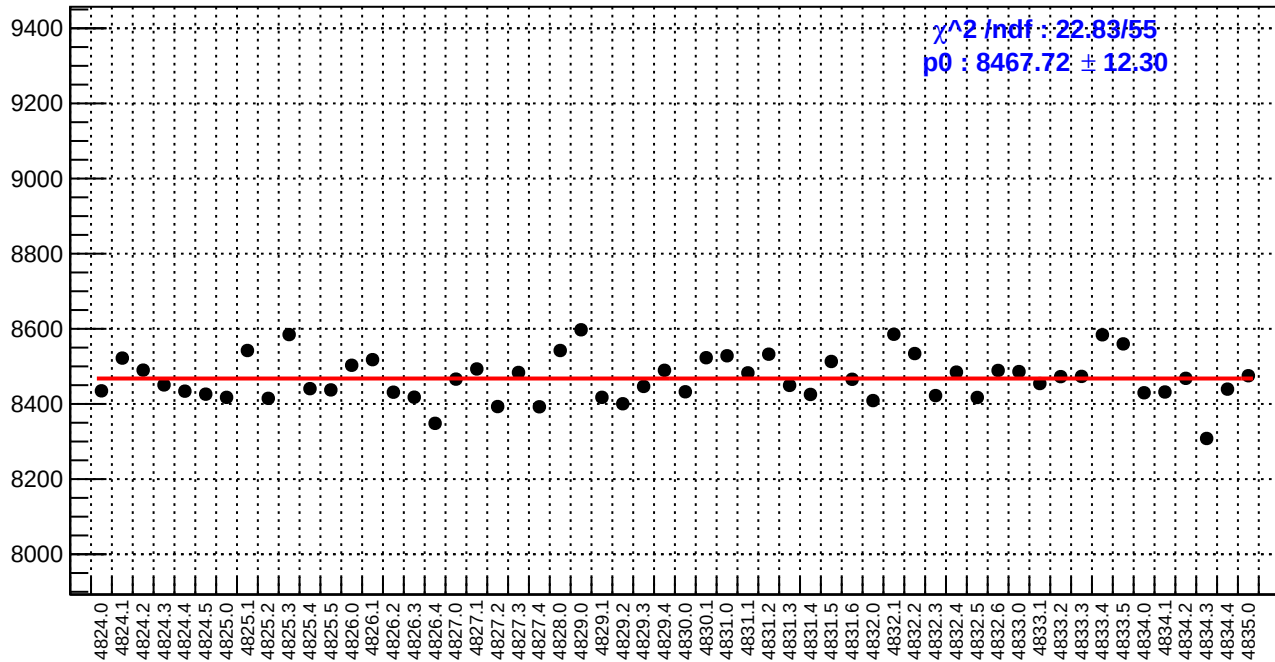
slug84: reg_asym_atl1.rms/ppm
