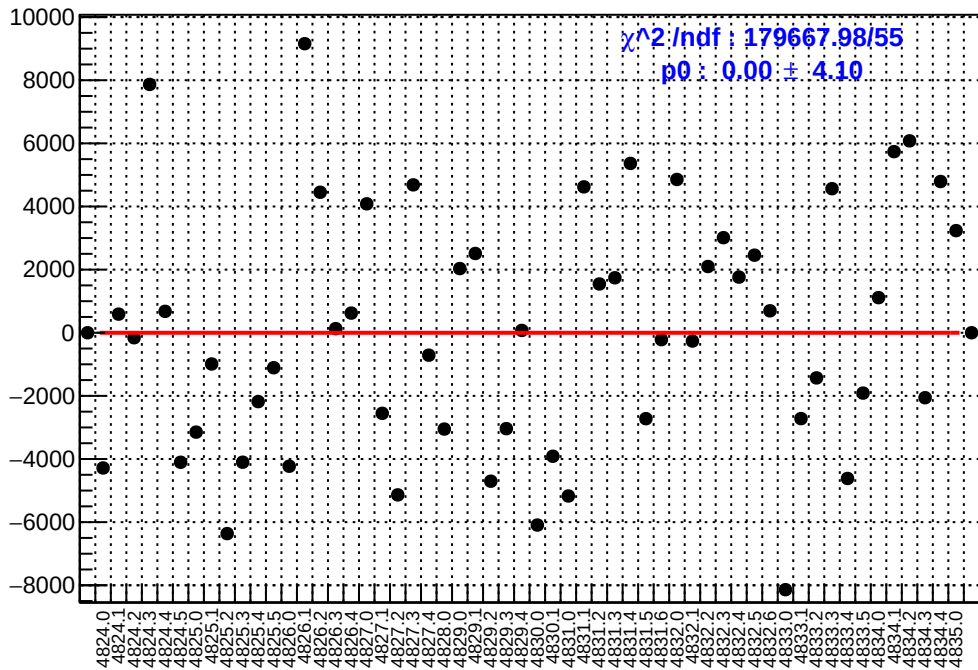
slug84: asym_atl1.mean/ppb-reg_asym_atl1.mean/ppb
