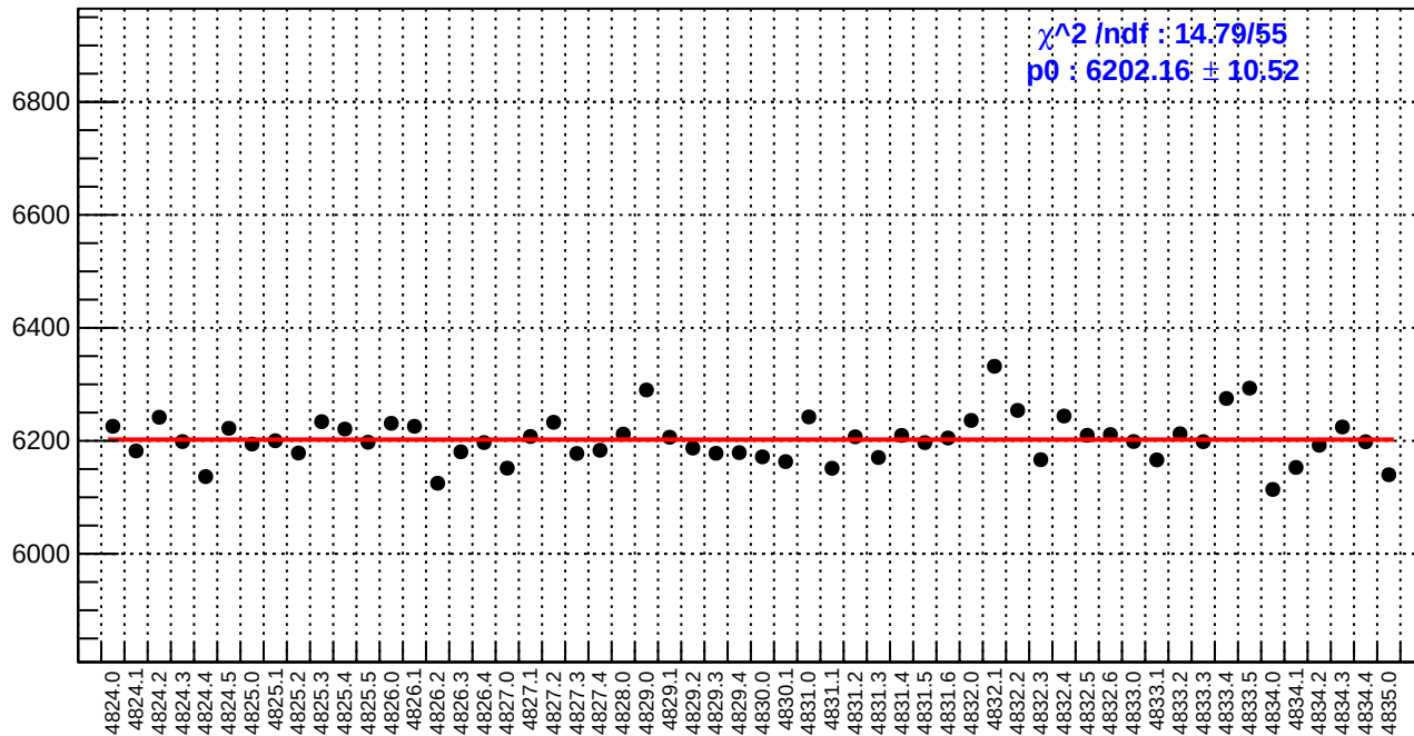
slug84: reg_asym_at1_avg.rms/ppm
