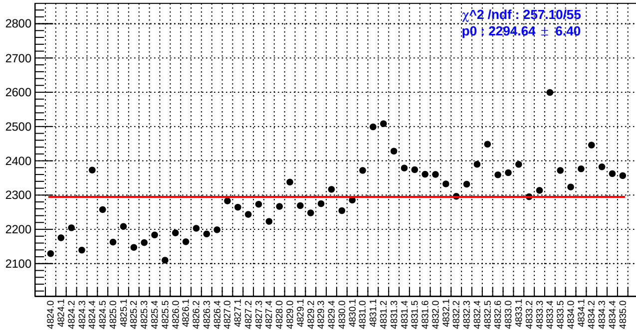
slug84: diff_bpm4eY.rms/nm
