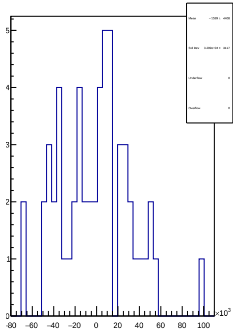
slug84: 1D Corr asym_sam4.mean/ppb-reg_asym_sam4.mean/ppb
