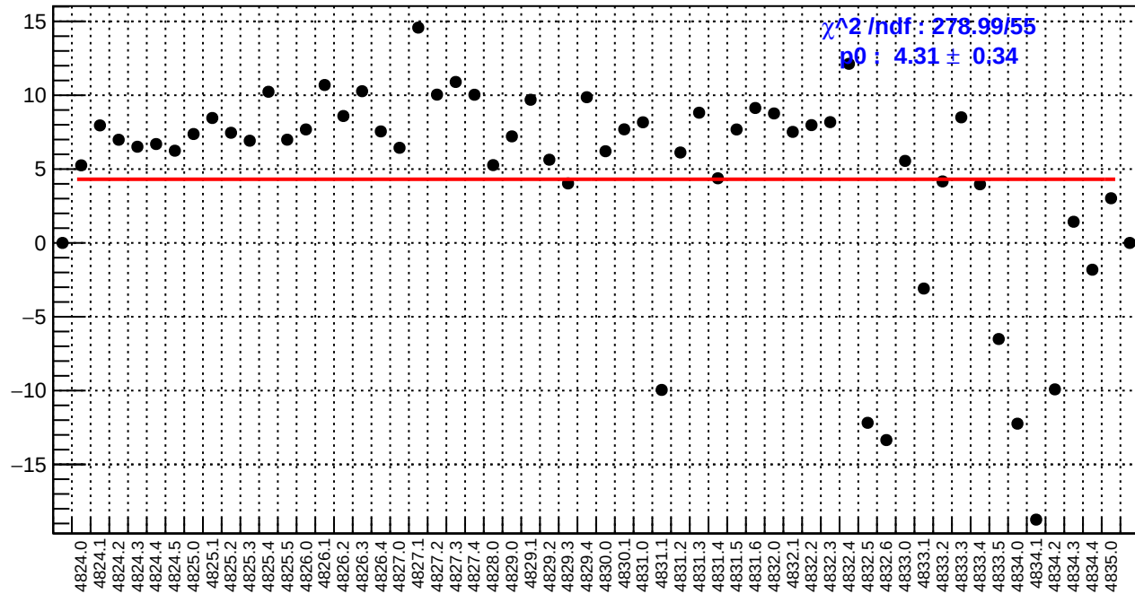
slug84: ds_avg_bpm4eY/(ppb/nm)
