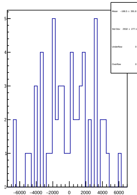
slug84: 1D Corr asym_atr1.mean/ppb-reg_asym_atr1.mean/ppb
