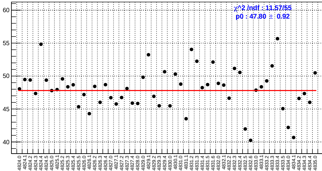
slug84: dsl_bpm4aX/(ppb/nm)
