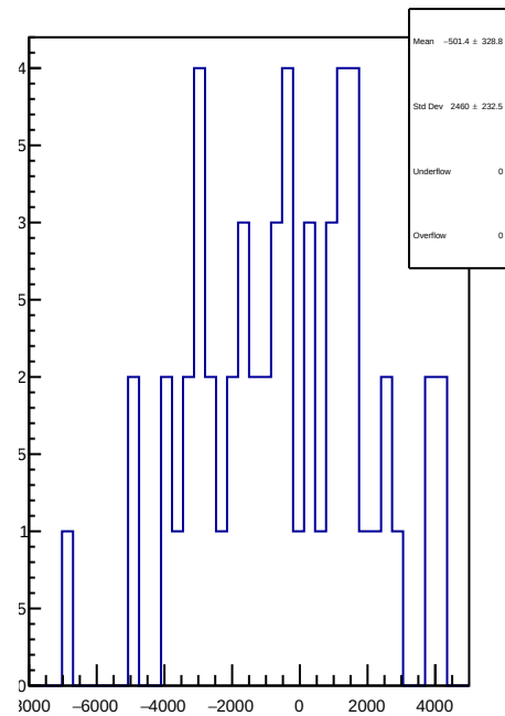
slug84: 1D Corr asym_atr1l2_avg.mean/ppb-reg_asym_atr1l2_avg.mean/ppb
