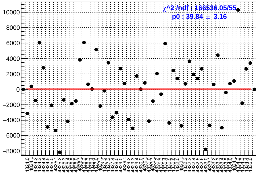
slug84: asym_us_dd.mean/ppb-reg_asym_us_dd.mean/ppb
