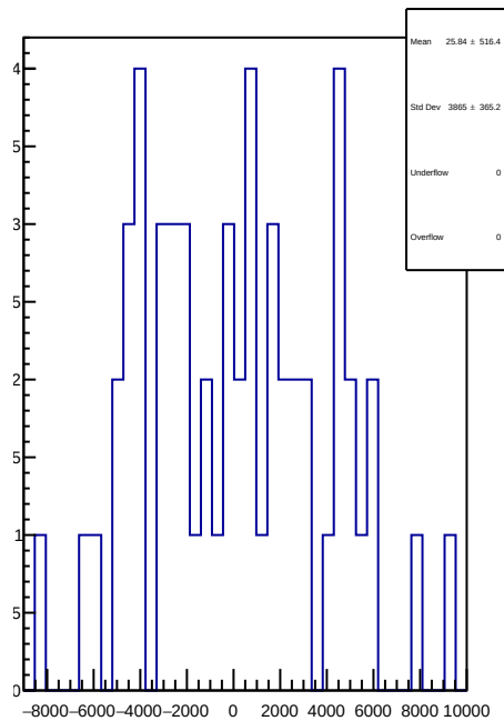
slug84: 1D Corr asym_atl1.mean/ppb-reg_asym_atl1.mean/ppb
