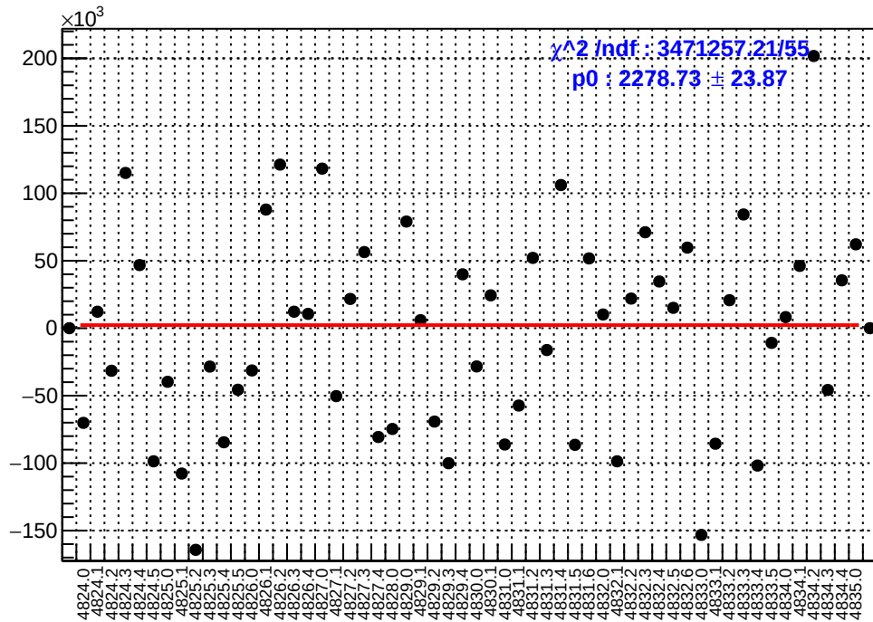
slug84: asym_sam3.mean/ppb-reg_asym_sam3.mean/ppb
