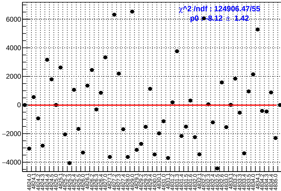
slug84: asym_at2_avg.mean/ppb-reg_asym_at2_avg.mean/ppb
