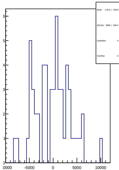
slug84: 1D Corr asym_us_dd.mean/ppb-reg_asym_us_dd.mean/ppb
