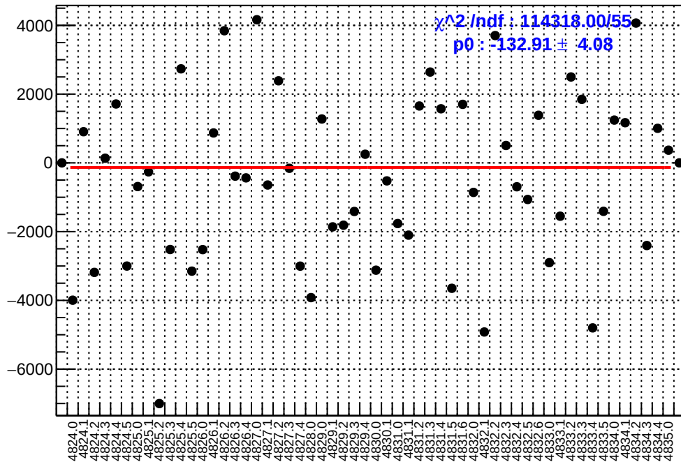
slug84: asym_atr1l2_avg.mean/ppb-reg_asym_atr1l2_avg.mean/ppb
