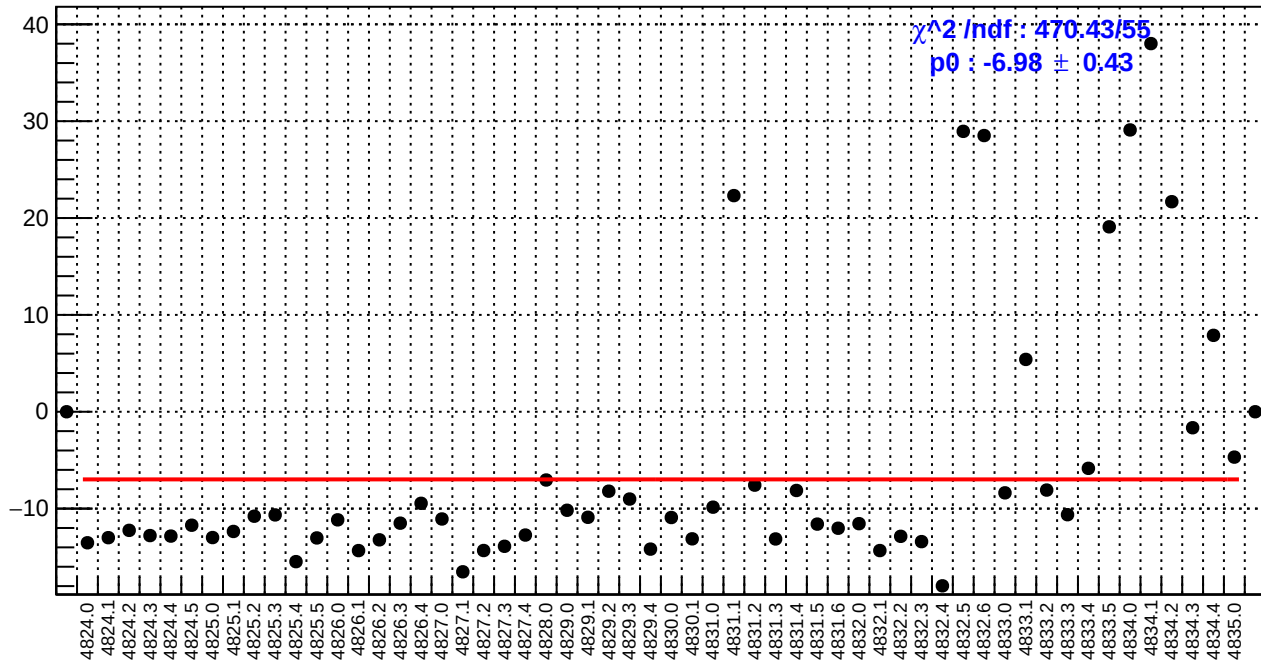
slug84: left_avg_bpm4aY/(ppb/nm)
