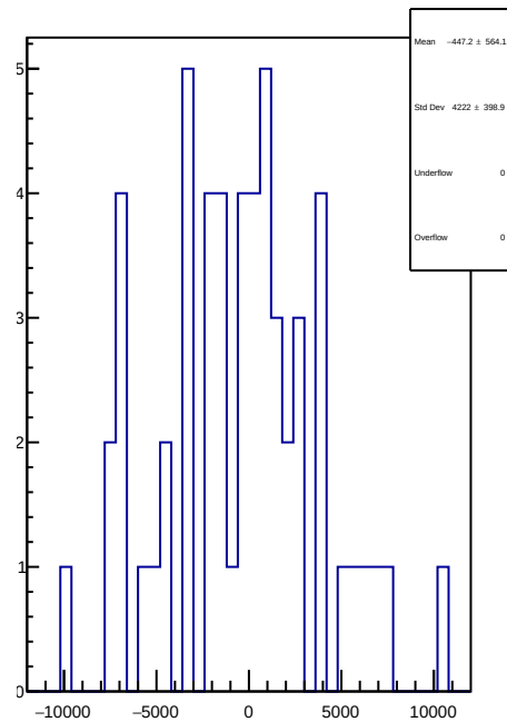
slug84: 1D Corr asym_right_avg.mean/ppb-reg_asym_right_avg.mean/ppb
