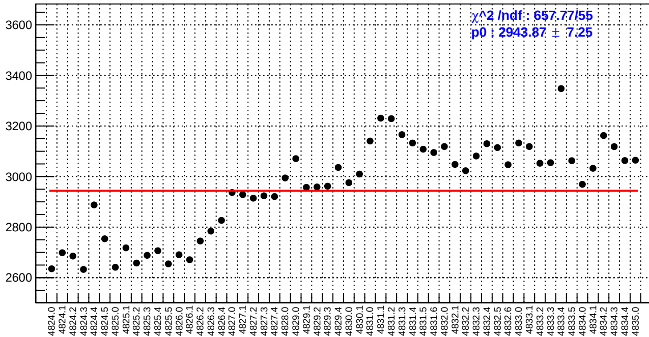
slug84: diff_bpm4aY.rms/nm
