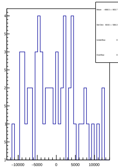
slug84: 1D Corr asym_left_avg.mean/ppb-reg_asym_left_avg.mean/ppb
