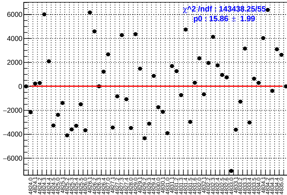
slug84: asym_at1_dd.mean/ppb-reg_asym_at1_dd.mean/ppb
