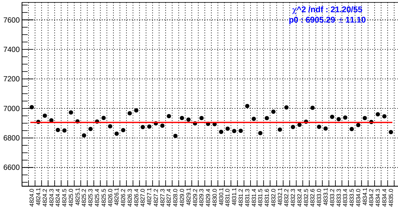
slug84: reg_asym_atr_avg.rms/ppm
