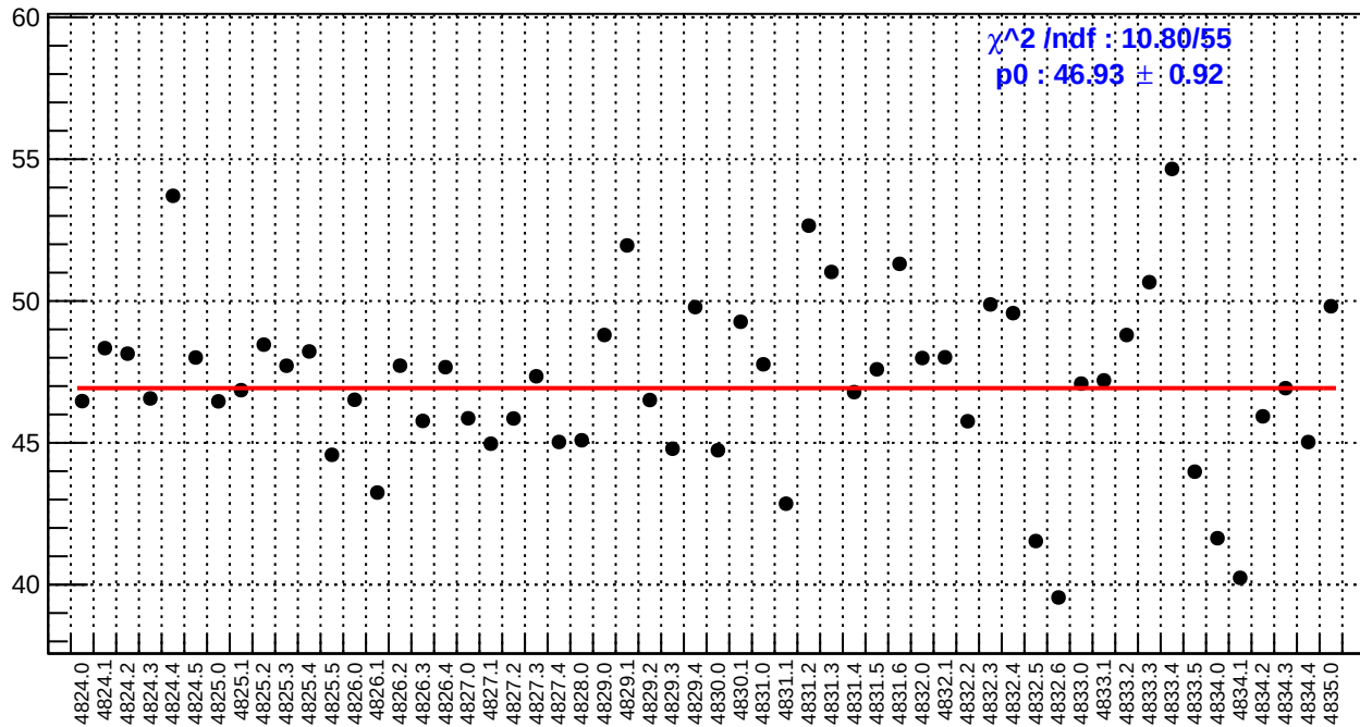
slug84: left_avg_bpm4aX/(ppb/nm)
