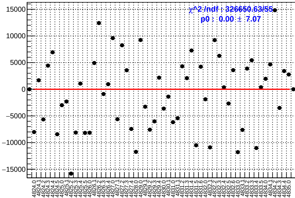
slug84: asym_atl2.mean/ppb-reg_asym_atl2.mean/ppb
