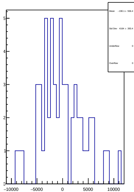
slug84: 1D Corr asym_atl1r2_dd.mean/ppb-reg_asym_atl1r2_dd.mean/ppb
