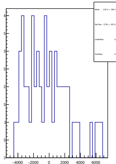
slug84: 1D Corr asym_at2_avg.mean/ppb-reg_asym_at2_avg.mean/ppb
