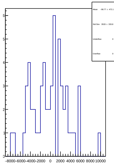
slug84: 1D Corr asym_ds_dd.mean/ppb-reg_asym_ds_dd.mean/ppb
