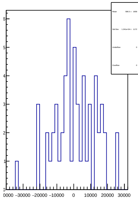
slug84: 1D Corr asym_sam8.mean/ppb-reg_asym_sam8.mean/ppb
