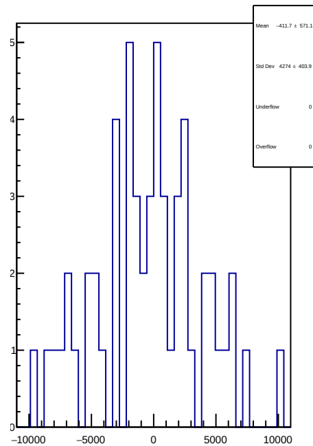
slug84: 1D Corr asym_usr.mean/ppb-reg_asym_usr.mean/ppb
