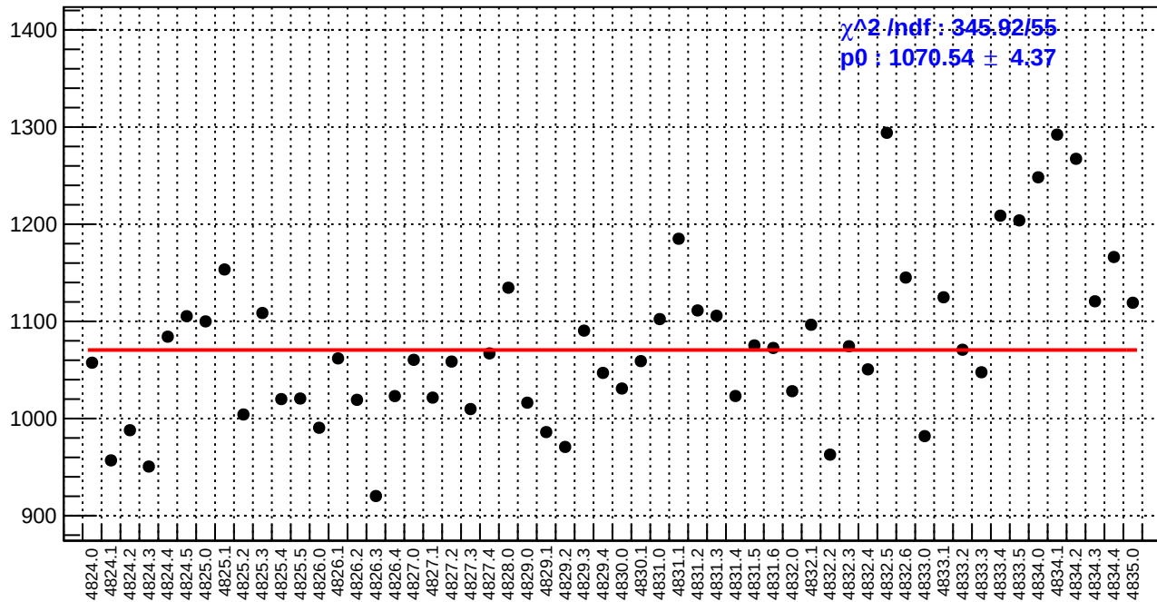
slug84: reg_asym_sam3.rms/ppm
