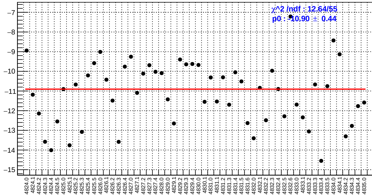
slug84: right_avg_bpm4aX/(ppb/nm)
