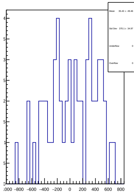
slug84: 1D Corr asym_right_dd.mean/ppb-reg_asym_right_dd.mean/ppb
