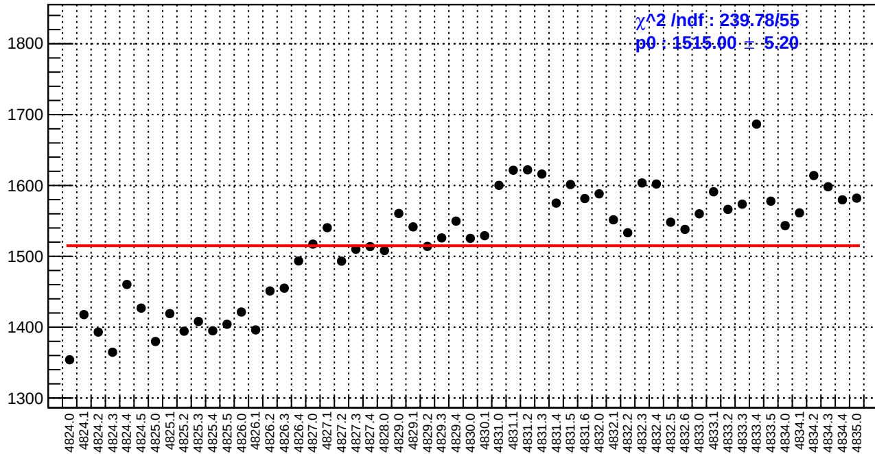
slug84: diff_bpm4aX.rms/nm
