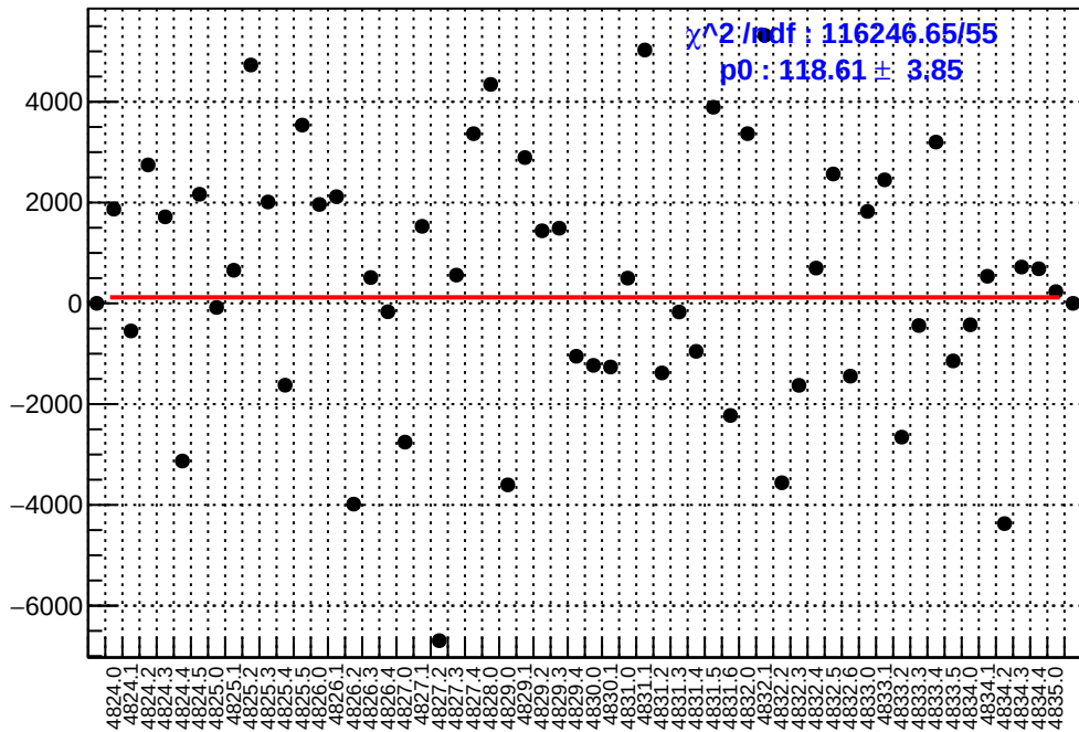
slug84: asym_atl_dd.mean/ppb-reg_asym_atl_dd.mean/ppb
