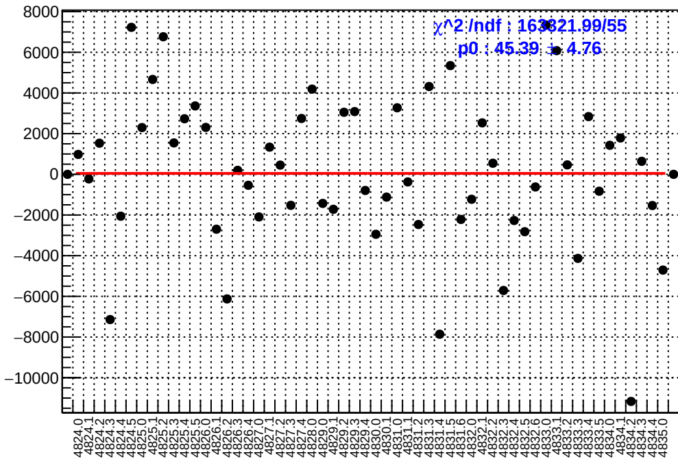
slug84: asym_atr_avg.mean/ppb-reg_asym_atr_avg.mean/ppb
