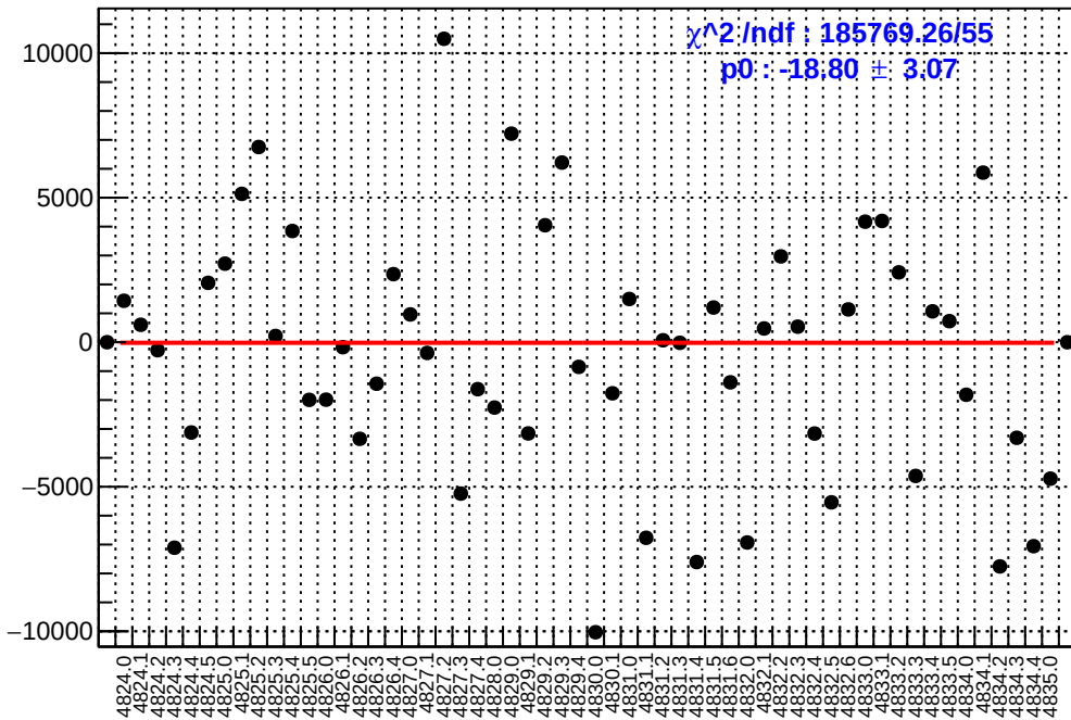
slug84: asym_right_avg.mean/ppb-reg_asym_right_avg.mean/ppb
