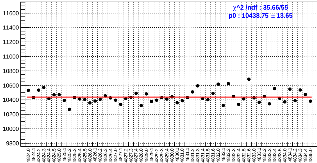
slug84: reg_asym_atr2.rms/ppm
