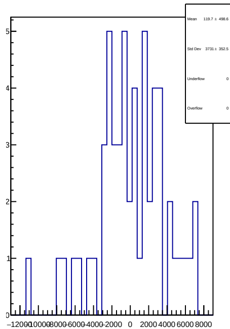
slug84: 1D Corr asym_atr_avg.mean/ppb-reg_asym_atr_avg.mean/ppb
