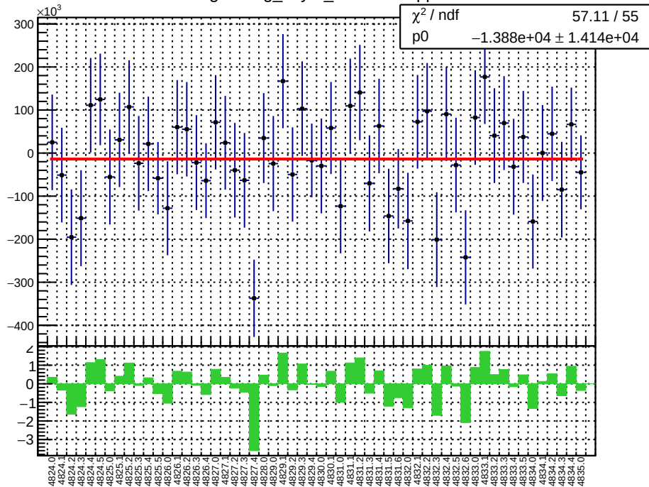
slug84: reg_asym_atr2.mean/ppb
