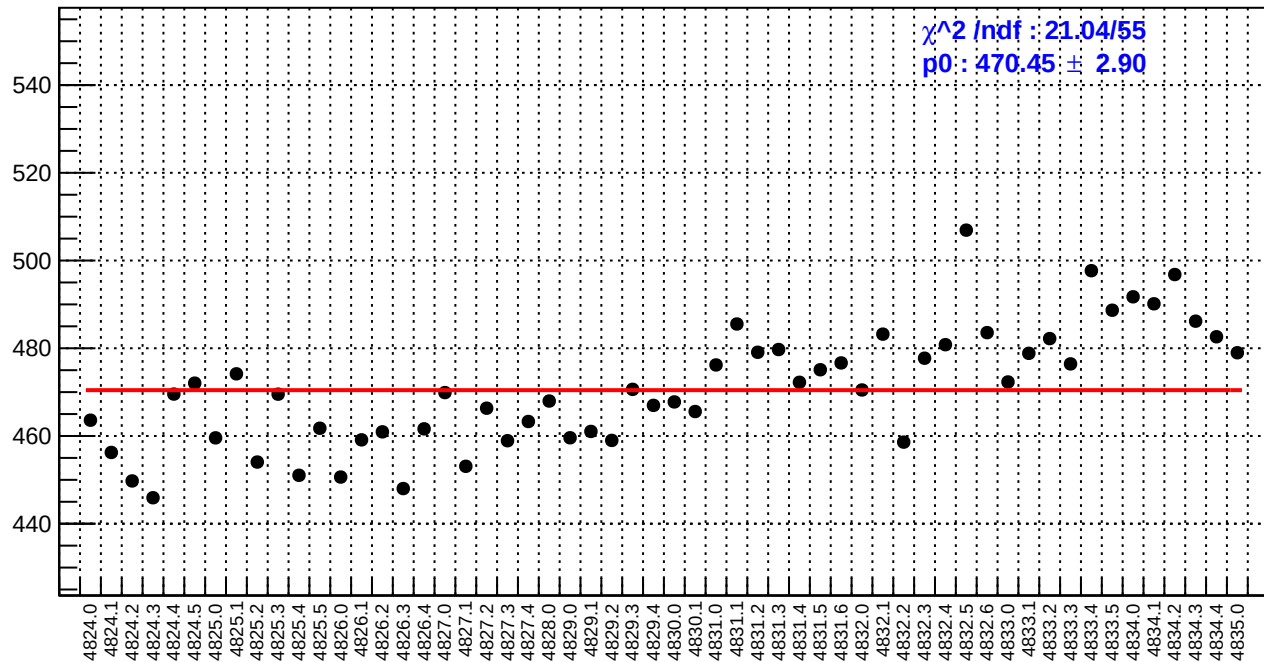
slug84: reg_asym_sam8.rms/ppm
