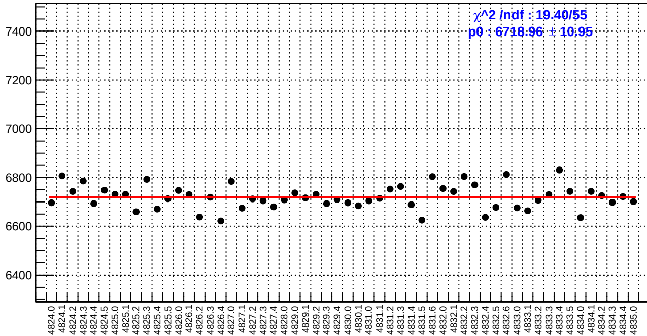
slug84: reg_asym_atl1r2_avg.rms/ppm
