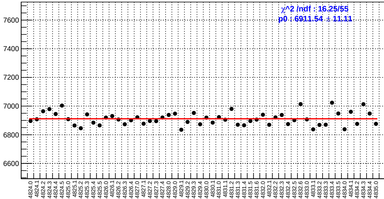
slug84: reg_asym_atr_dd.rms/ppm
