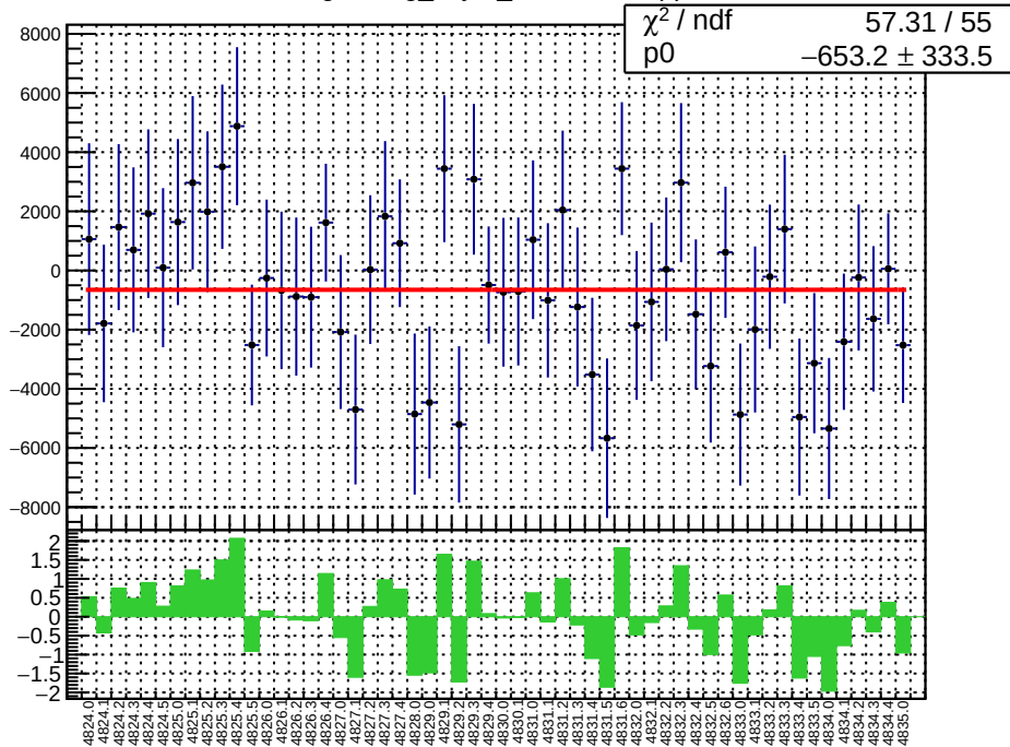
slug84: reg_asym_sam1.mean/ppb
