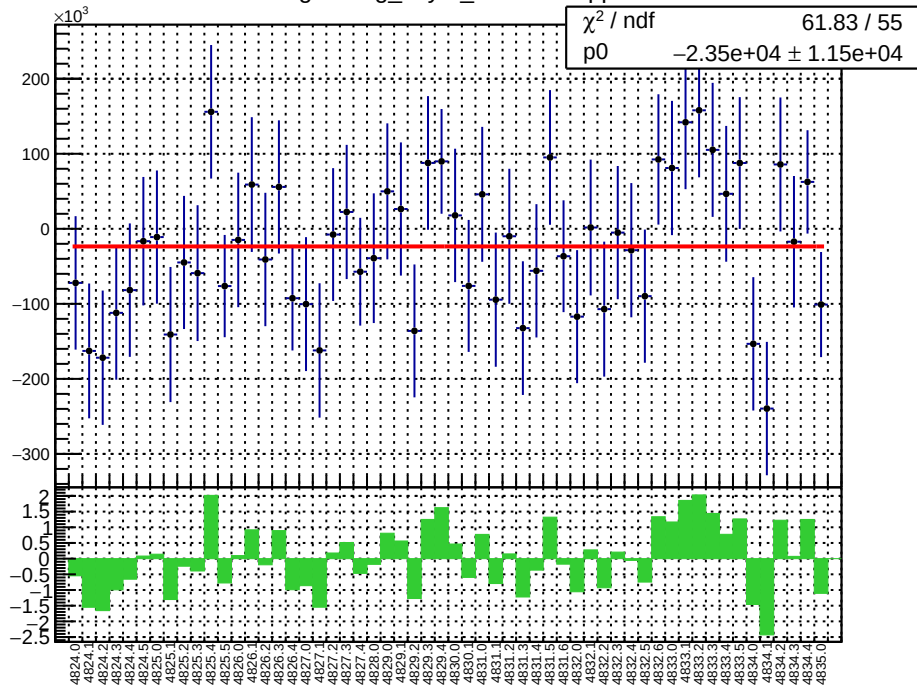
slug84: reg_asym_atl1.mean/ppb
