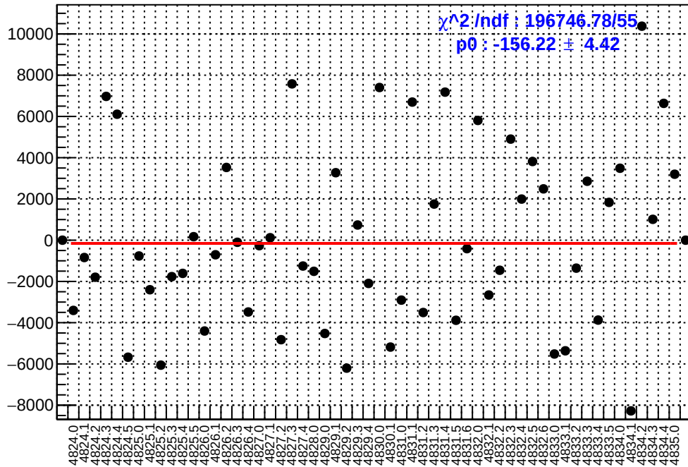
slug84: asym_sam5.mean/ppb-reg_asym_sam5.mean/ppb
