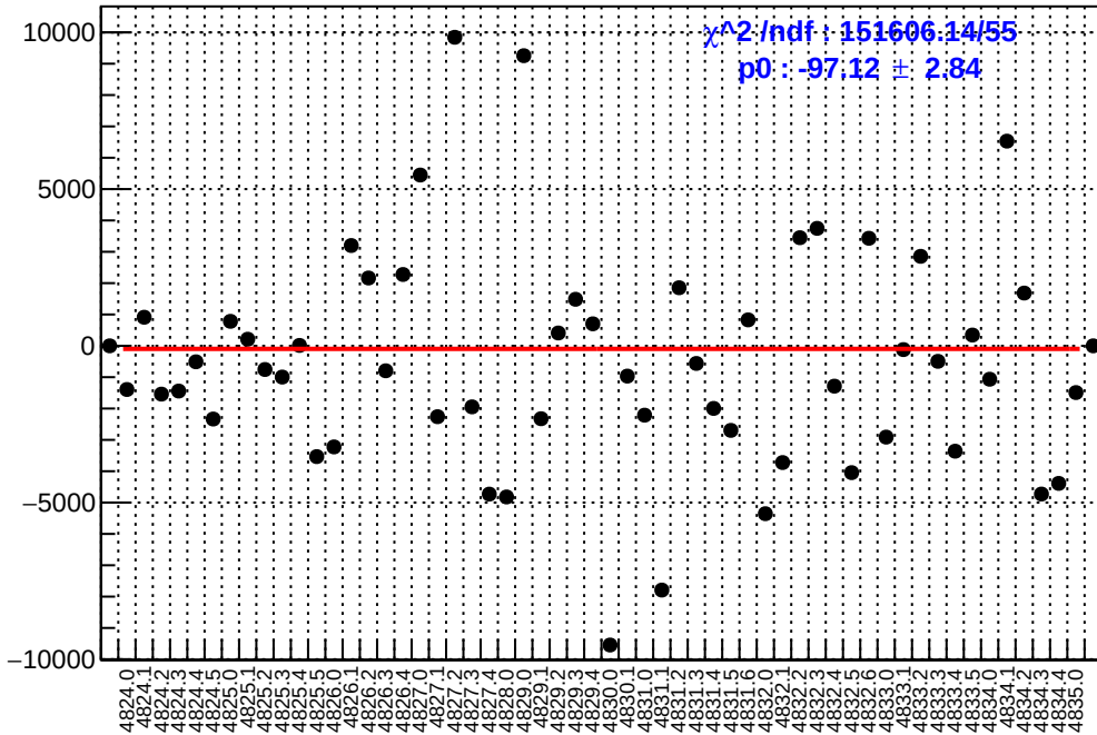
slug84: asym_us_avg.mean/ppb-reg_asym_us_avg.mean/ppb
