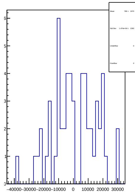
slug84: 1D Corr asym_sam7.mean/ppb-reg_asym_sam7.mean/ppb
