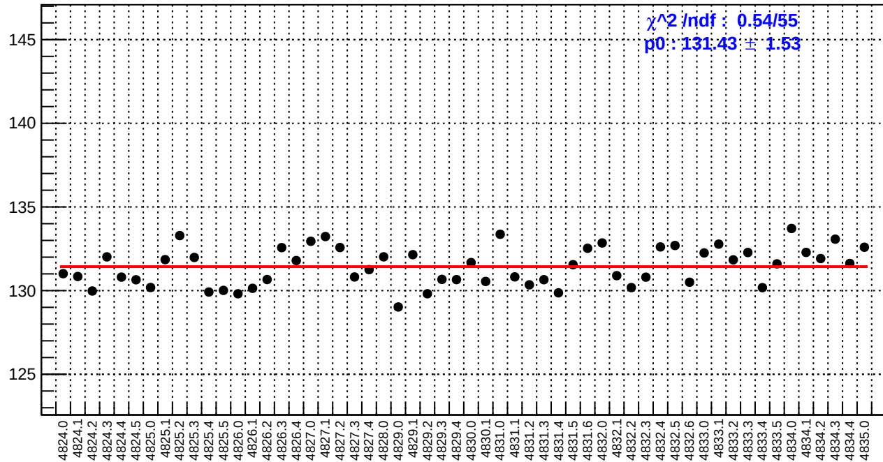
slug84: reg_asym_right_avg.rms/ppm
