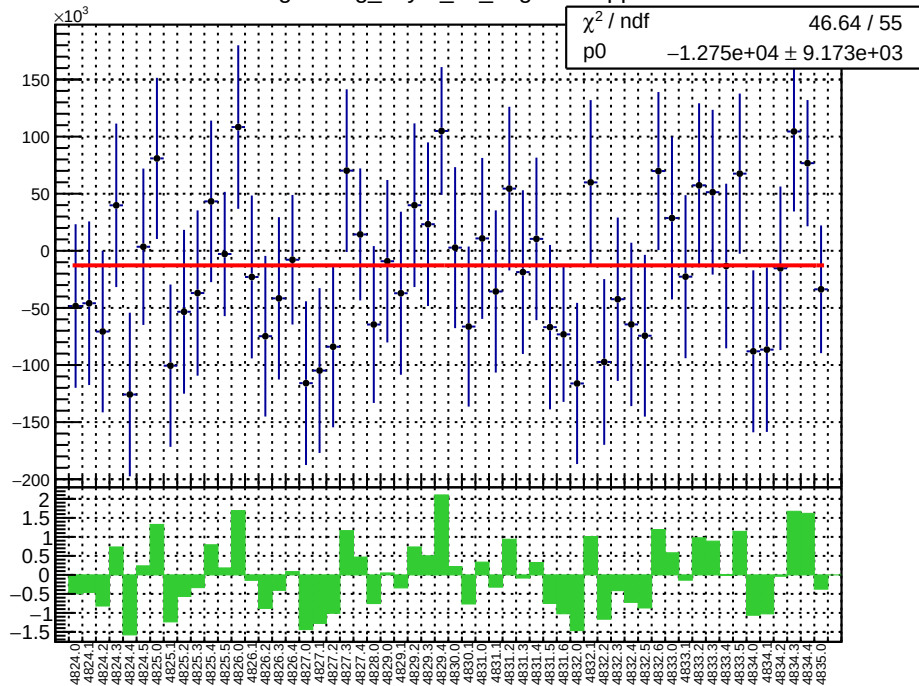
slug84: reg_asym_atl_avg.mean/ppb
