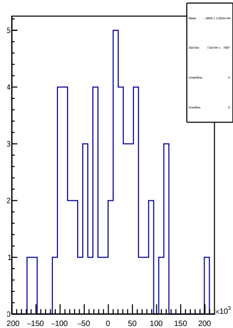
slug84: 1D Corr asym_sam3.mean/ppb-reg_asym_sam3.mean/ppb
