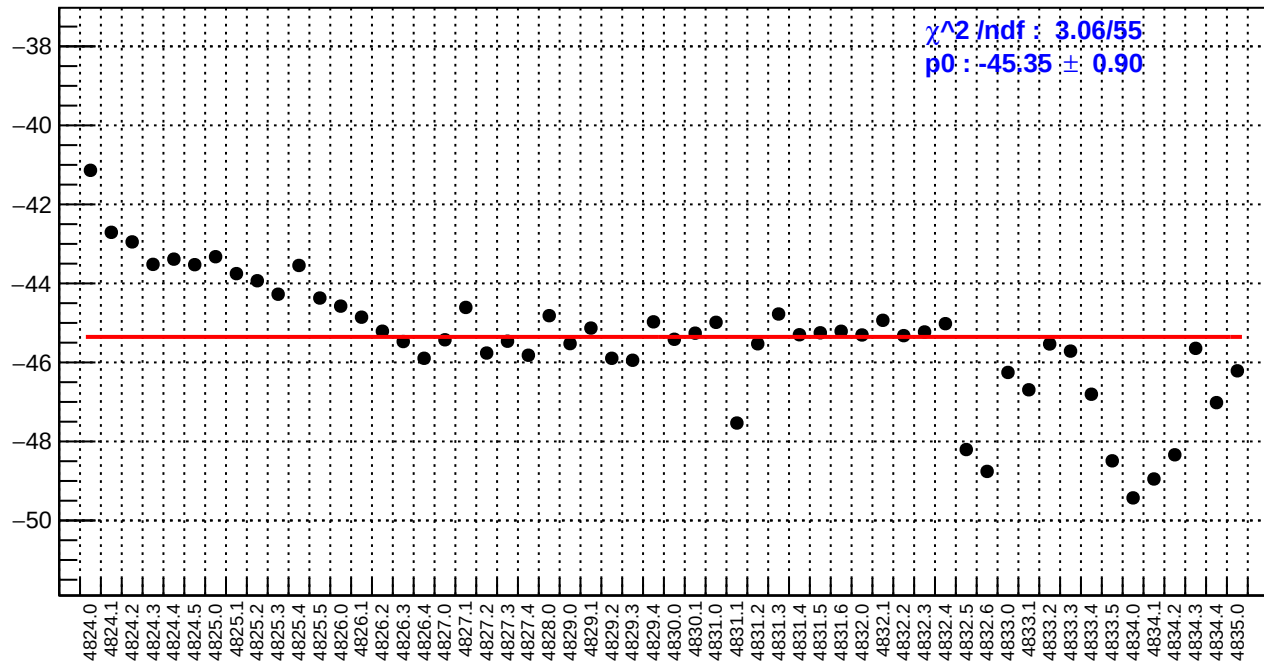
slug84: left_avg_bpm12X/(ppb/nm)
