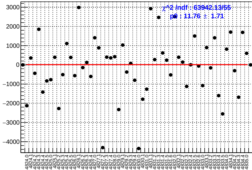
slug84: asym_at1_avg.mean/ppb-reg_asym_at1_avg.mean/ppb
