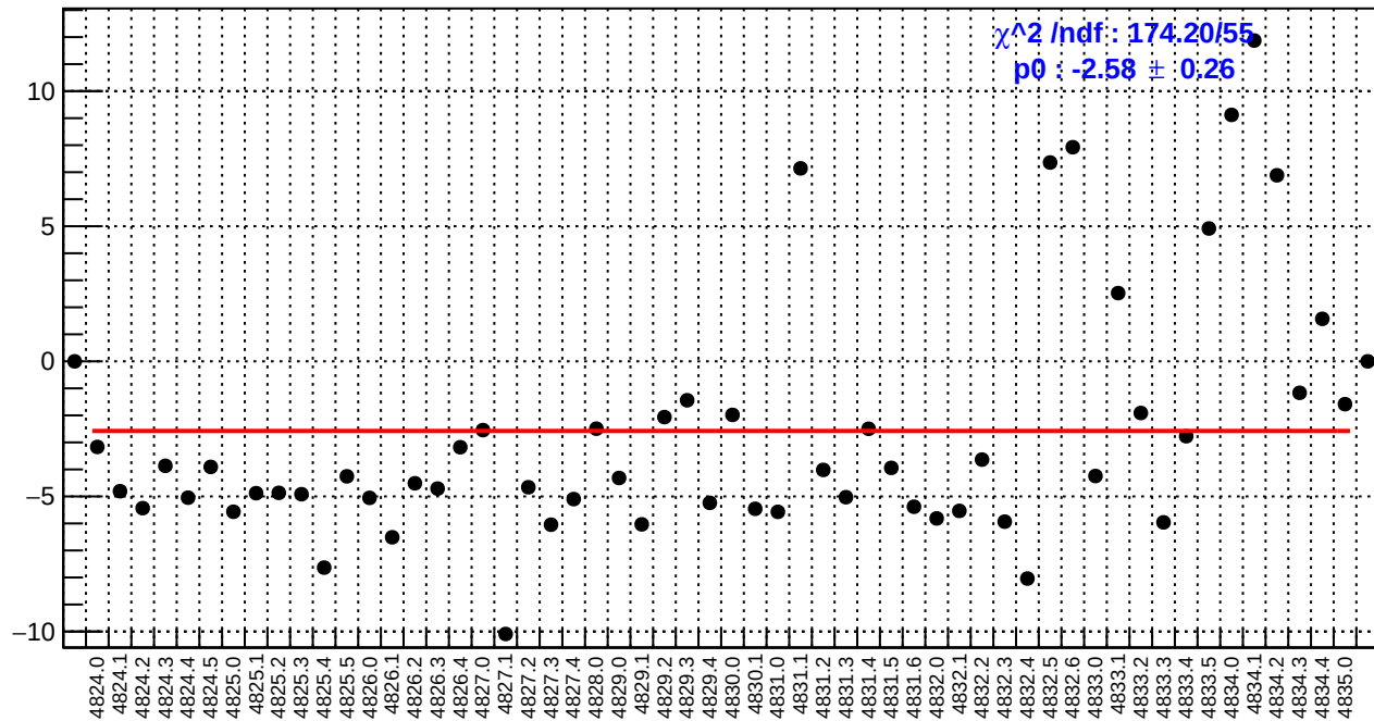
slug84: us_avg_bpm4aY/(ppb/nm)
