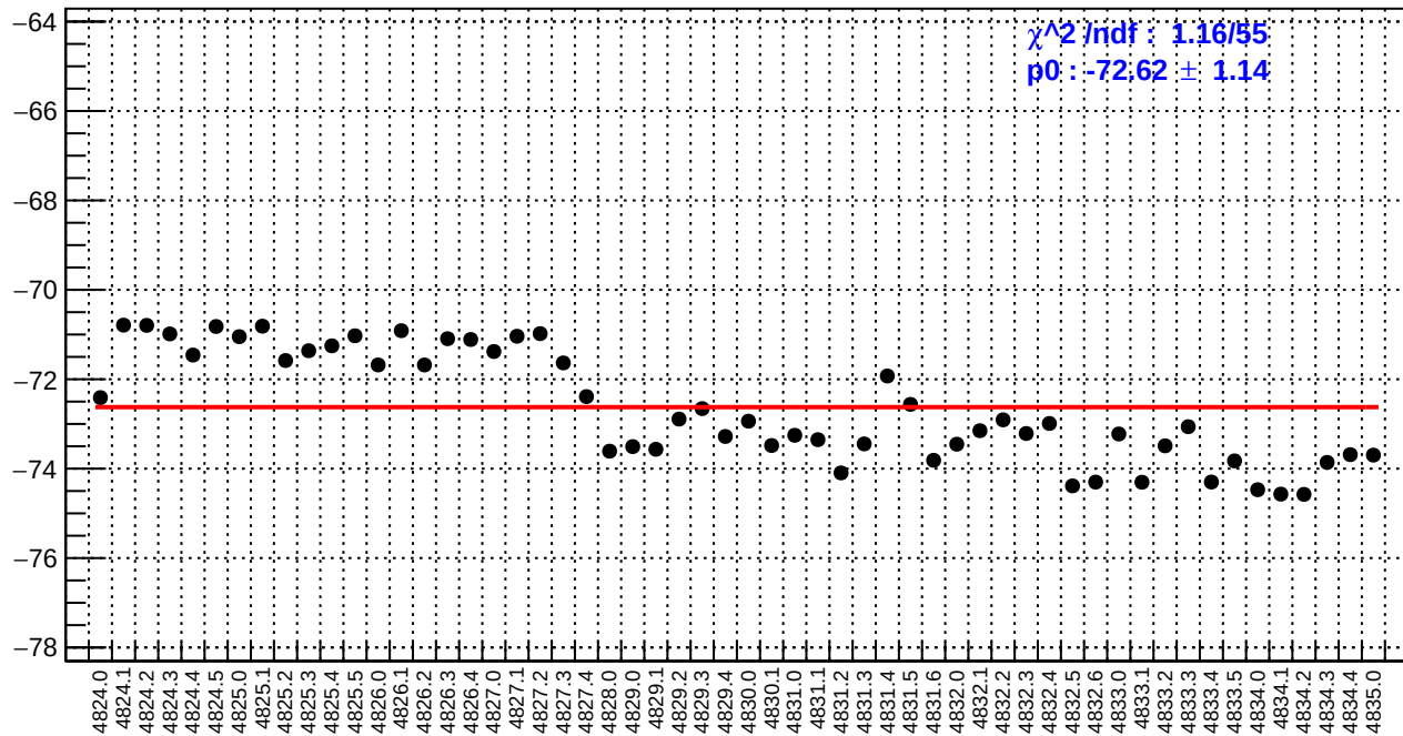
slug84: left_avg_bpm4eX/(ppb/nm)
