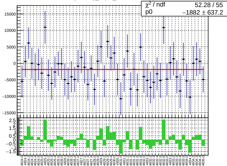
slug84: reg_asym_sam8.mean/ppb
