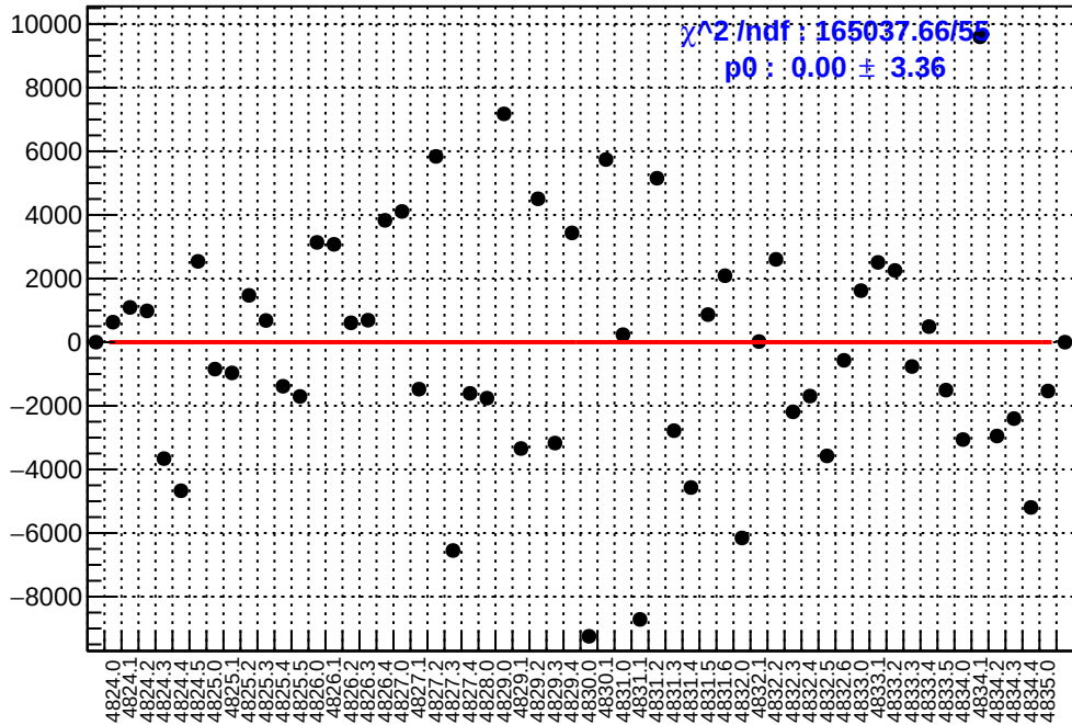
slug84: asym_sam1.mean/ppb-reg_asym_sam1.mean/ppb
