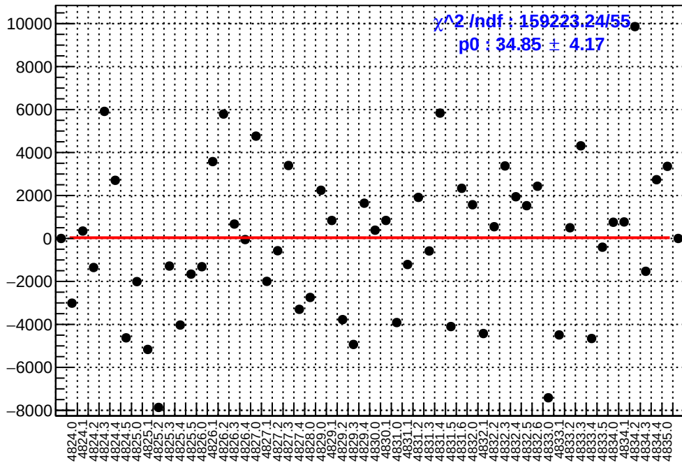
slug84: asym_ds_dd.mean/ppb-reg_asym_ds_dd.mean/ppb
