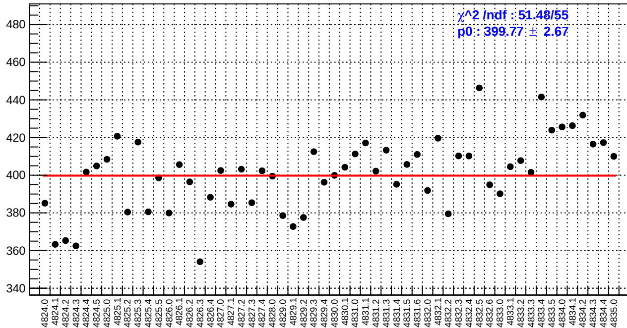
slug84: reg_asym_sam7.rms/ppm
