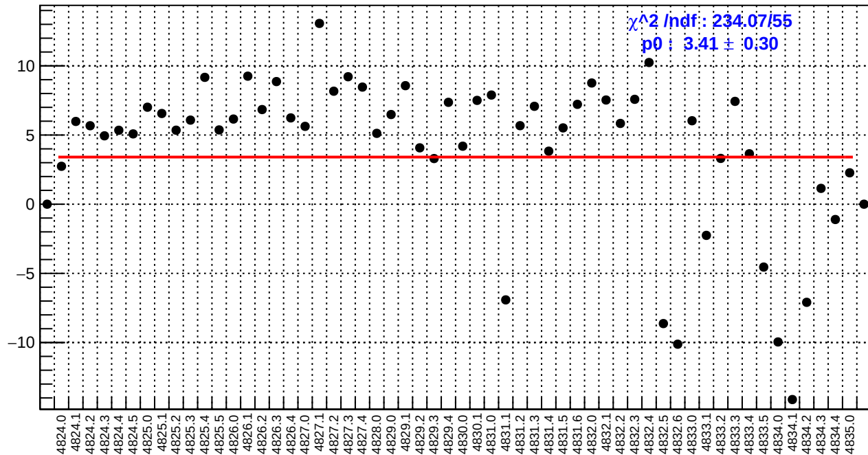
slug84: us_avg_bpm4eY/(ppb/nm)
