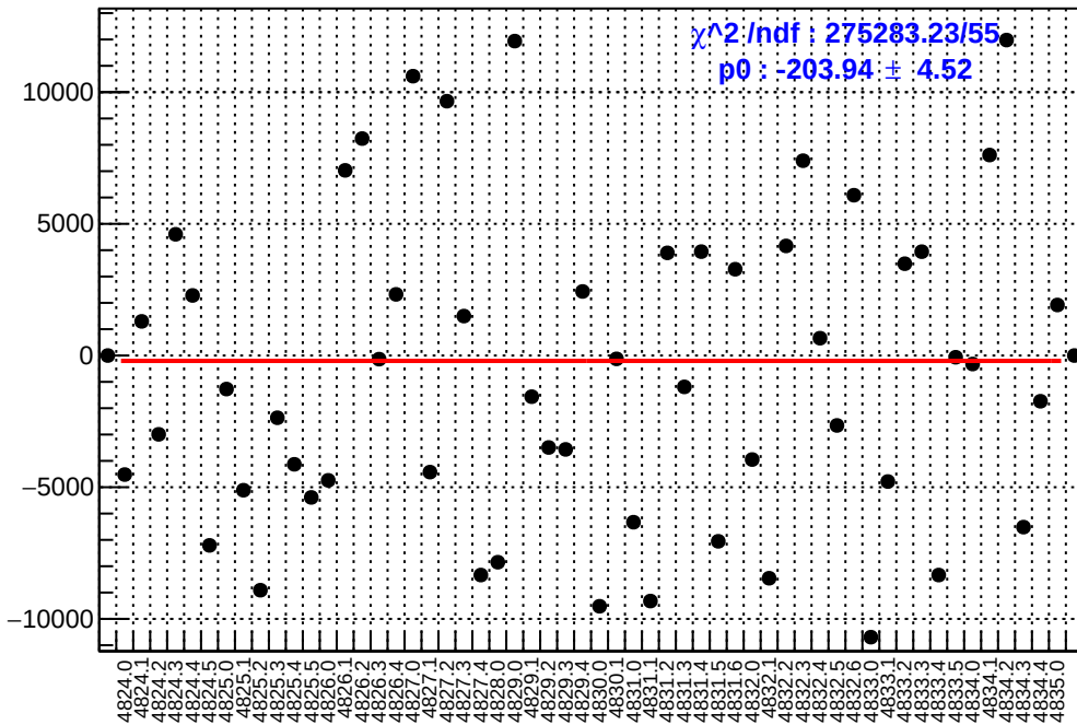
slug84: asym_usl.mean/ppb-reg_asym_usl.mean/ppb
