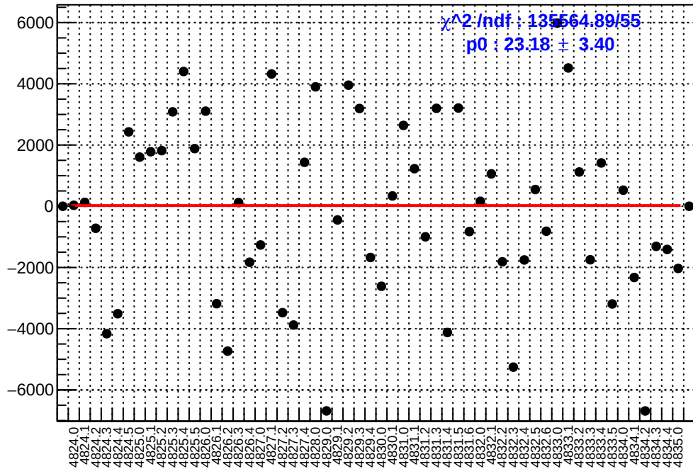
slug84: asym_atr1.mean/ppb-reg_asym_atr1.mean/ppb
