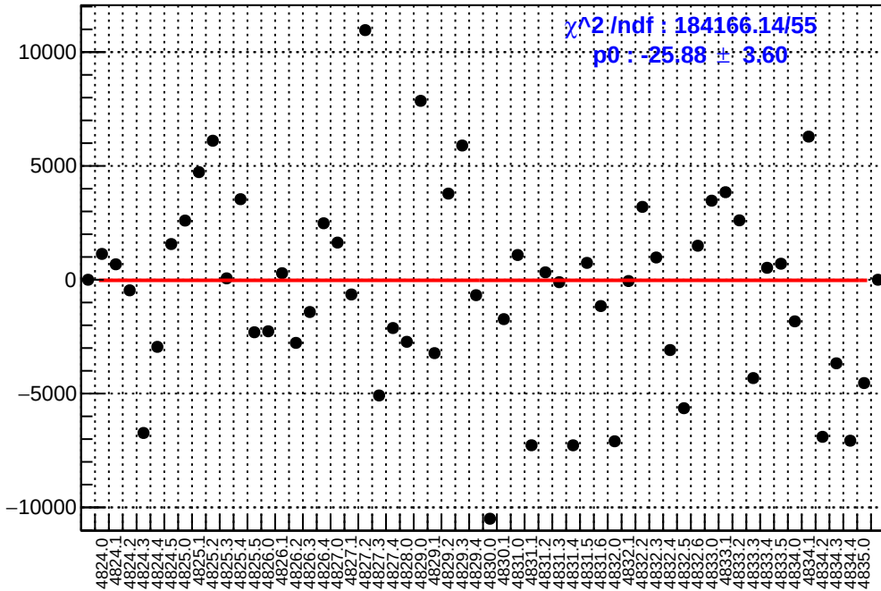
slug84: asym_dsr.mean/ppb-reg_asym_dsr.mean/ppb
