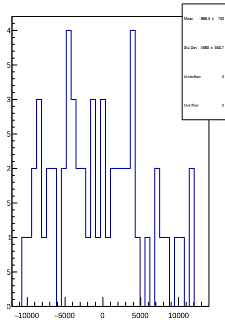
slug84: 1D Corr asym_usl.mean/ppb-reg_asym_usl.mean/ppb
