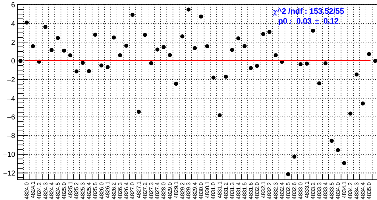
slug84: right_avg_bpm4aY/(ppb/nm)
