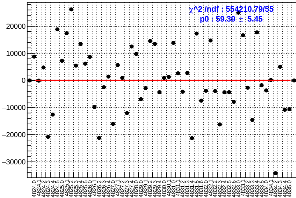
slug84: asym_sam8.mean/ppb-reg_asym_sam8.mean/ppb
