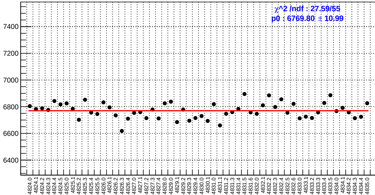
slug84: reg_asym_atl_dd.rms/ppm
