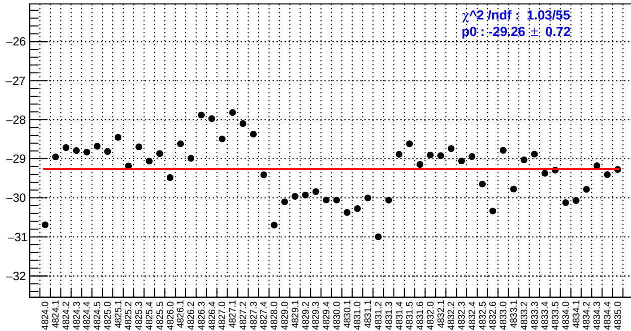
slug84: ds_avg_bpm4eX/(ppb/nm)
