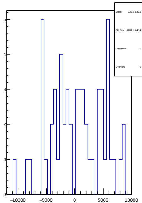
slug84: 1D Corr asym_atr1l2_dd.mean/ppb-reg_asym_atr1l2_dd.mean/ppb
