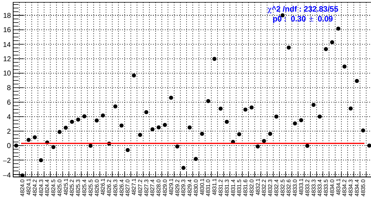
slug84: right_avg_bpm4eY/(ppb/nm)
