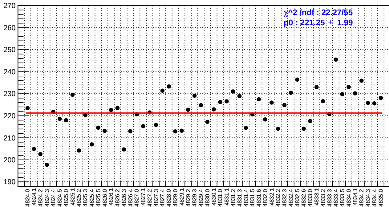
slug84: reg_asym_sam5.rms/ppm
