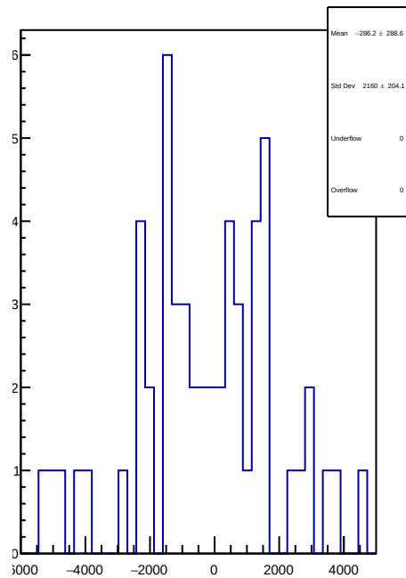
slug84: 1D Corr asym_atr_dd.mean/ppb-reg_asym_atr_dd.mean/ppb
