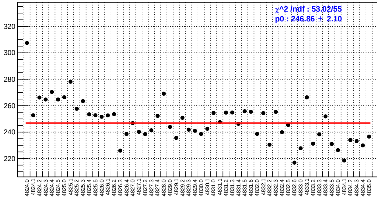
slug84: reg_asym_sam1.rms/ppm
