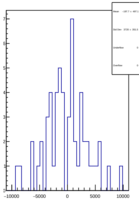
slug84: 1D Corr asym_sam1.mean/ppb-reg_asym_sam1.mean/ppb
