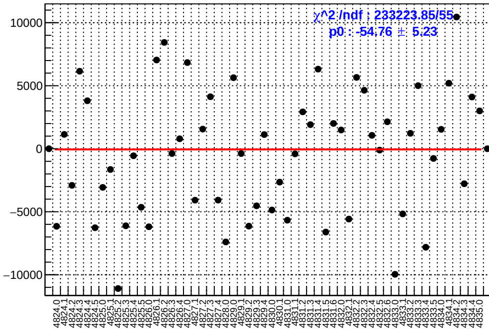
slug84: asym_atl_avg.mean/ppb-reg_asym_atl_avg.mean/ppb
