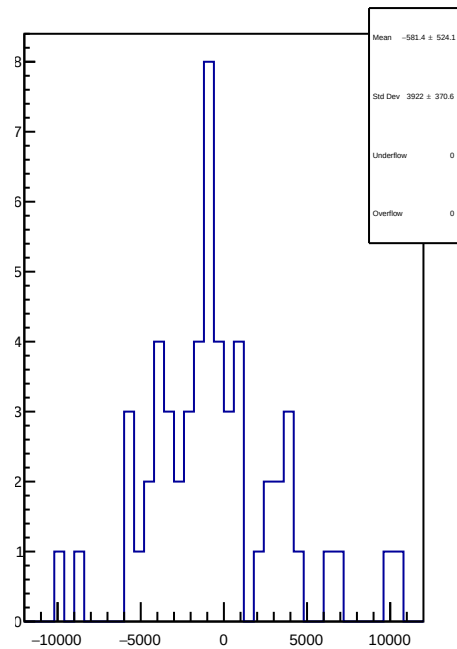
slug84: 1D Corr asym_ds_avg.mean/ppb-reg_asym_ds_avg.mean/ppb
