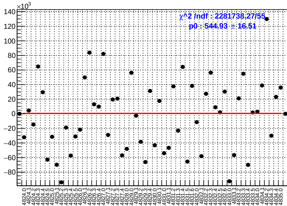
slug84: asym_sam2.mean/ppb-reg_asym_sam2.mean/ppb
