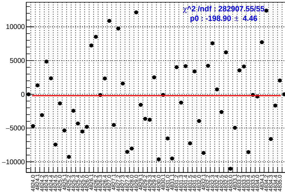
slug84: asym_left_avg.mean/ppb-reg_asym_left_avg.mean/ppb
