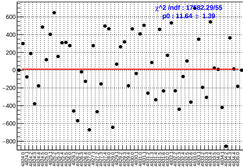
slug84: asym_right_dd.mean/ppb-reg_asym_right_dd.mean/ppb
