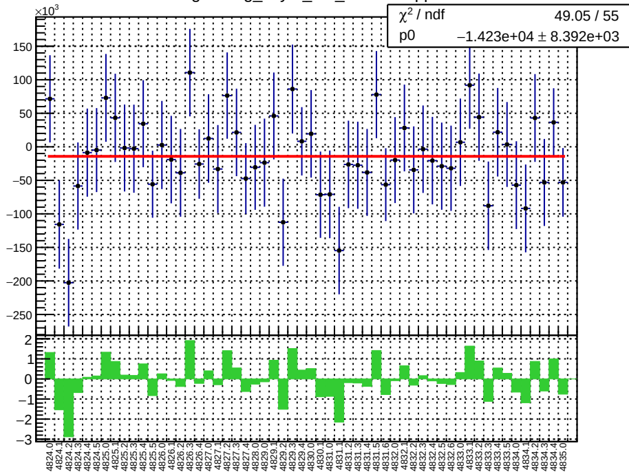
slug84: reg_asym_at1_dd.mean/ppb
