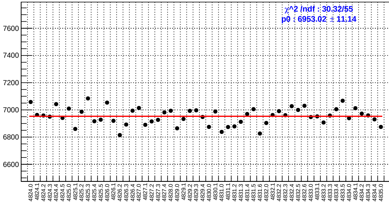
slug84: reg_asym_atr1l2_avg.rms/ppm
