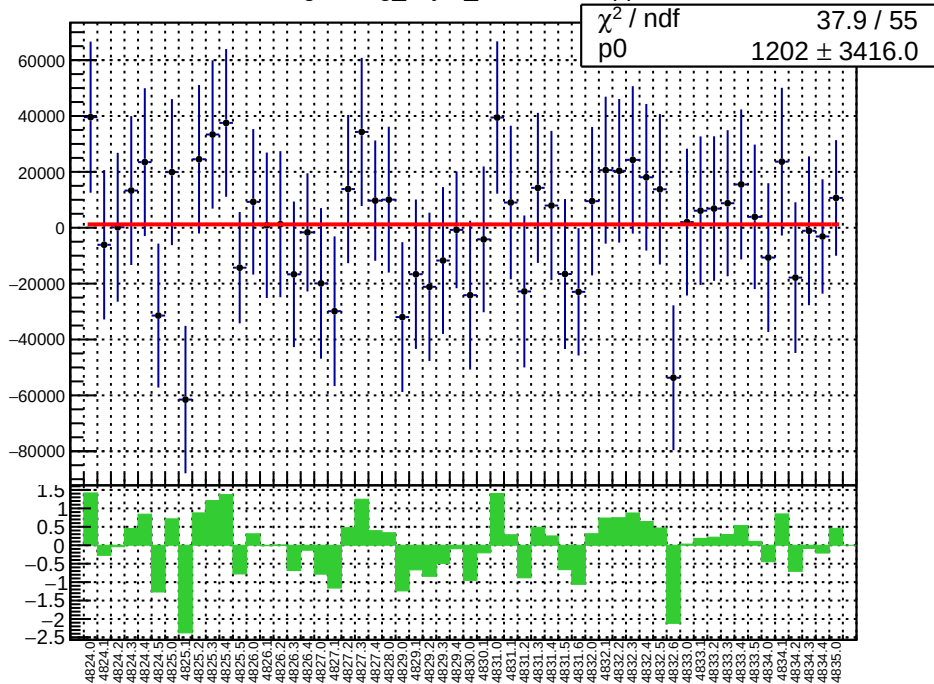
slug84: reg_asym_sam2.mean/ppb
