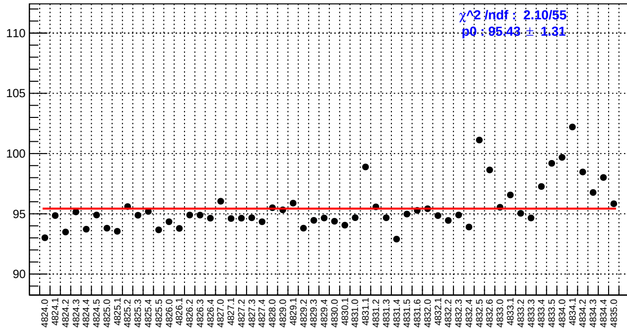
slug84: reg_asym_ds_dd.rms/ppm
