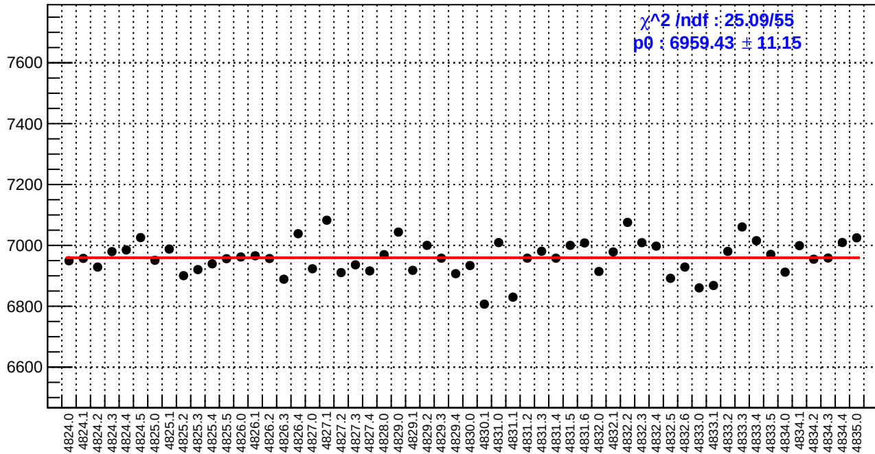
slug84: reg_asym_atr1l2_dd.rms/ppm
