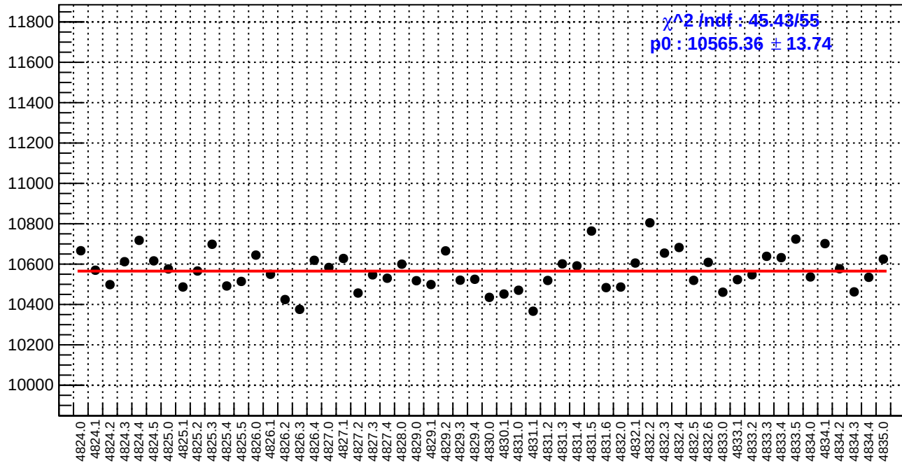
slug84: reg_asym_atl2.rms/ppm
