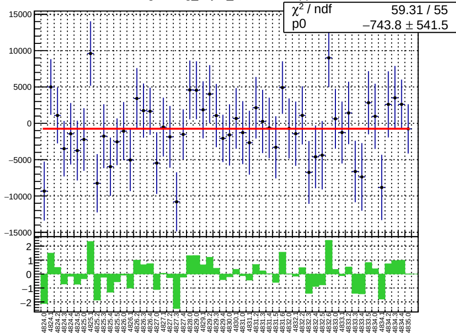
slug84: reg_asym_sam7.mean/ppb
