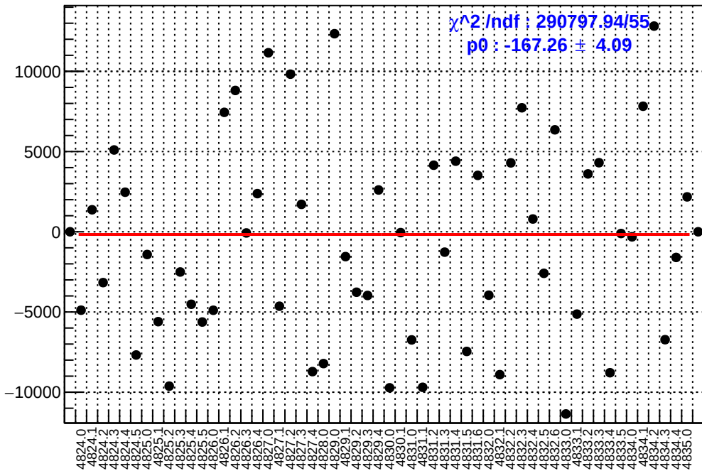
slug84: asym_dsl.mean/ppb-reg_asym_dsl.mean/ppb
