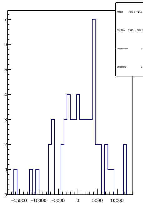
slug84: 1D Corr asym_atr2.mean/ppb-reg_asym_atr2.mean/ppb
