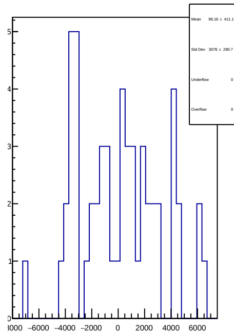
slug84: 1D Corr asym_at1_dd.mean/ppb-reg_asym_at1_dd.mean/ppb
