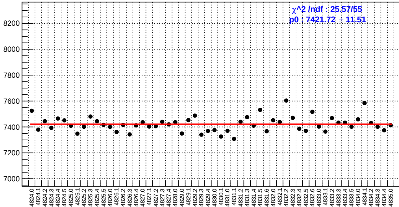
slug84: reg_asym_at2_avg.rms/ppm
