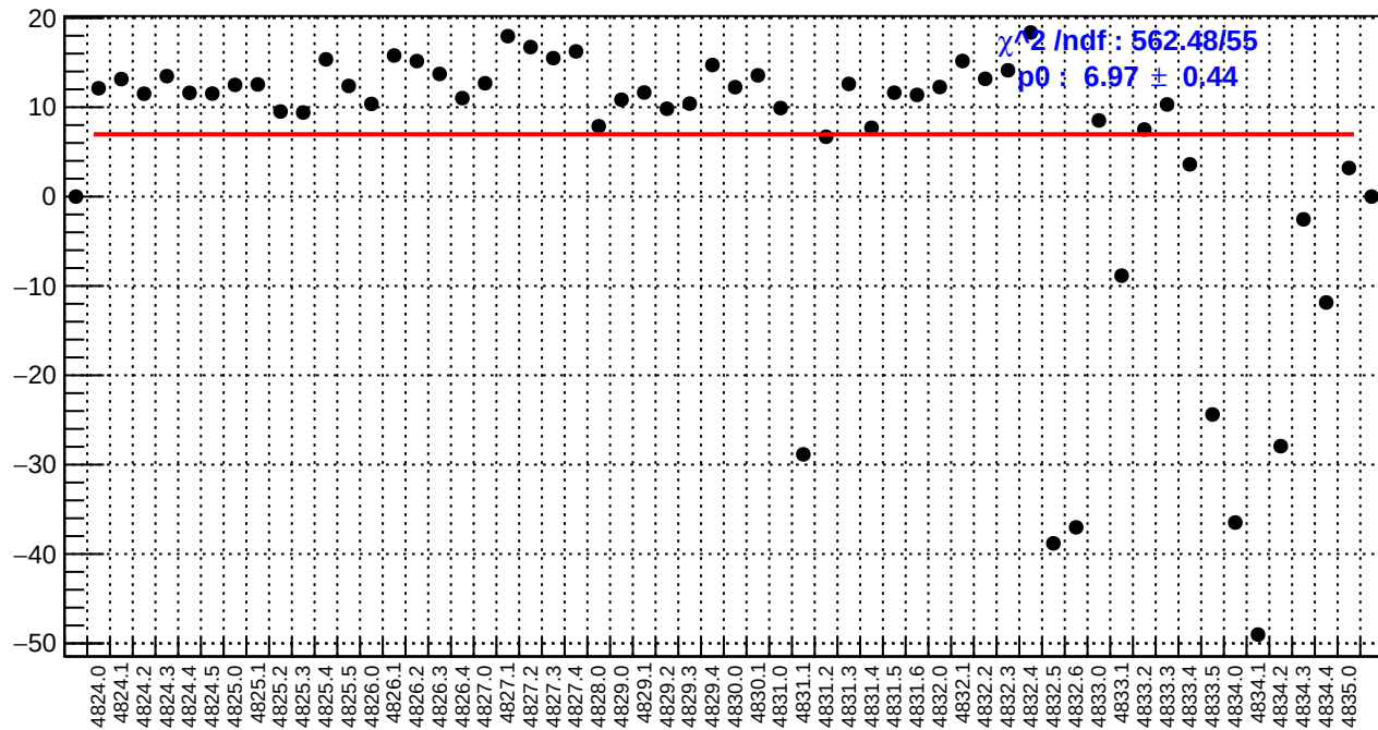
slug84: left_avg_bpm4eY/(ppb/nm)
