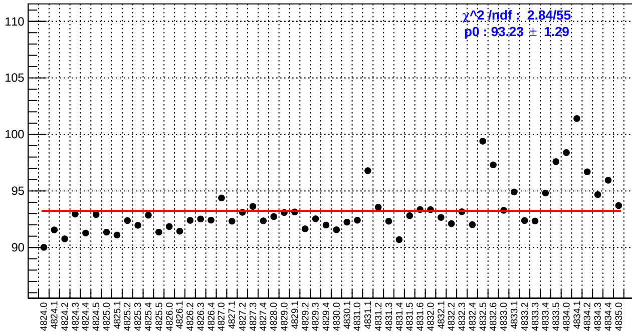
slug84: reg_asym_us_dd.rms/ppm
