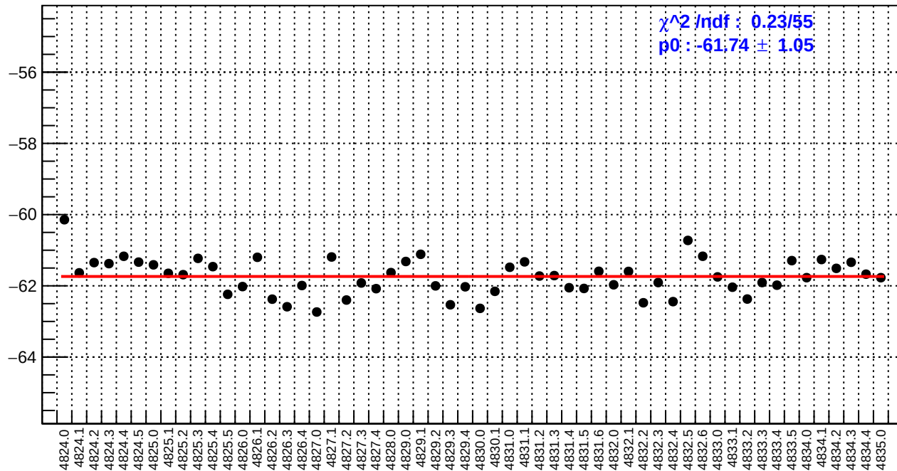
slug84: right_avg_bpm12X/(ppb/nm)
