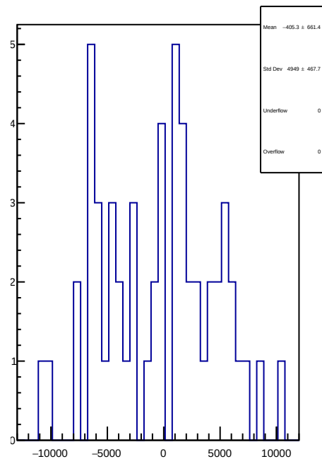
slug84: 1D Corr asym_atl_avg.mean/ppb-reg_asym_atl_avg.mean/ppb
