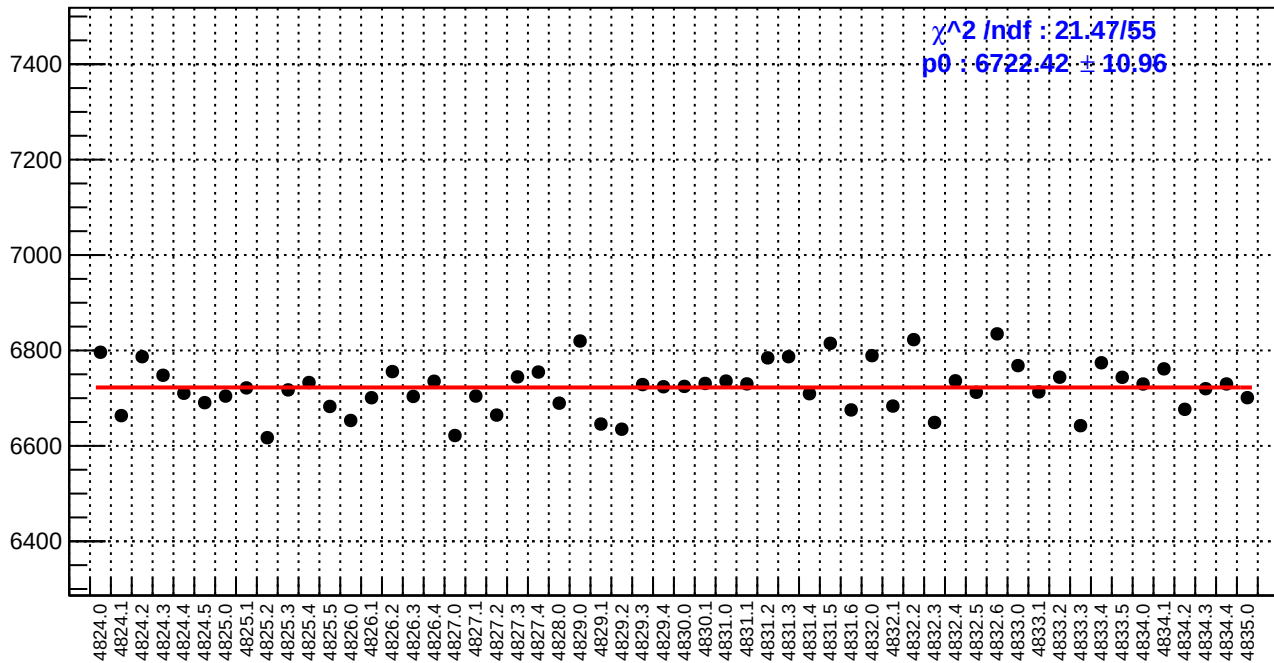
slug84: reg_asym_atl1r2_dd.rms/ppm
