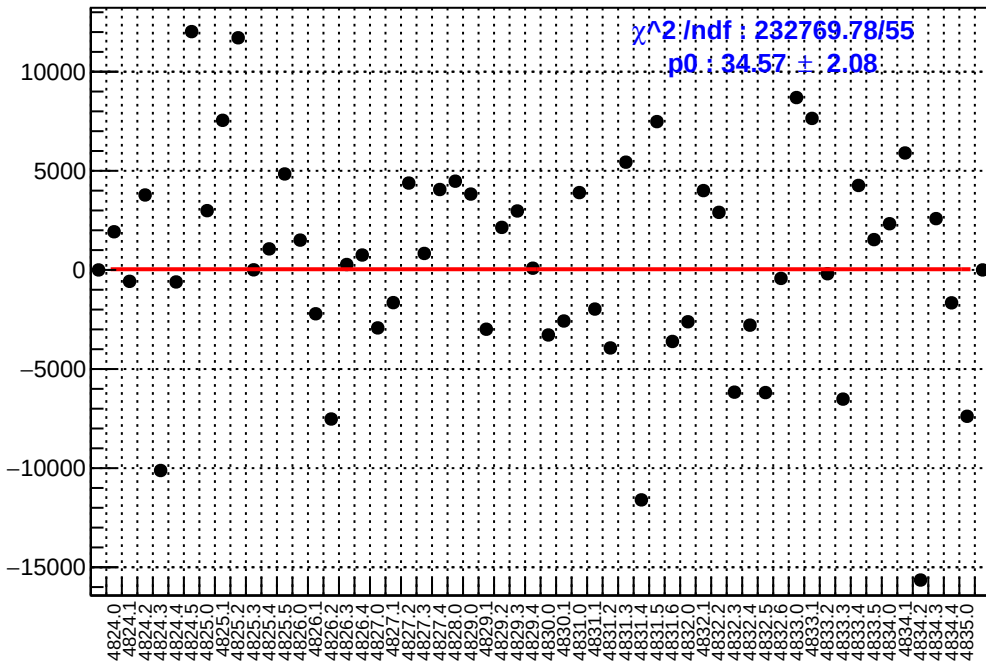
slug84: asym_atr2.mean/ppb-reg_asym_atr2.mean/ppb
