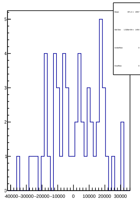
slug84: 1D Corr asym_sam6.mean/ppb-reg_asym_sam6.mean/ppb
