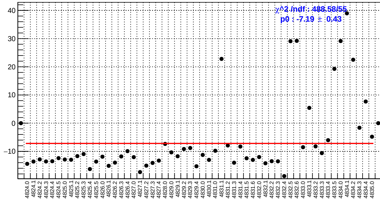
slug84: dsl_bpm4aY/(ppb/nm)
