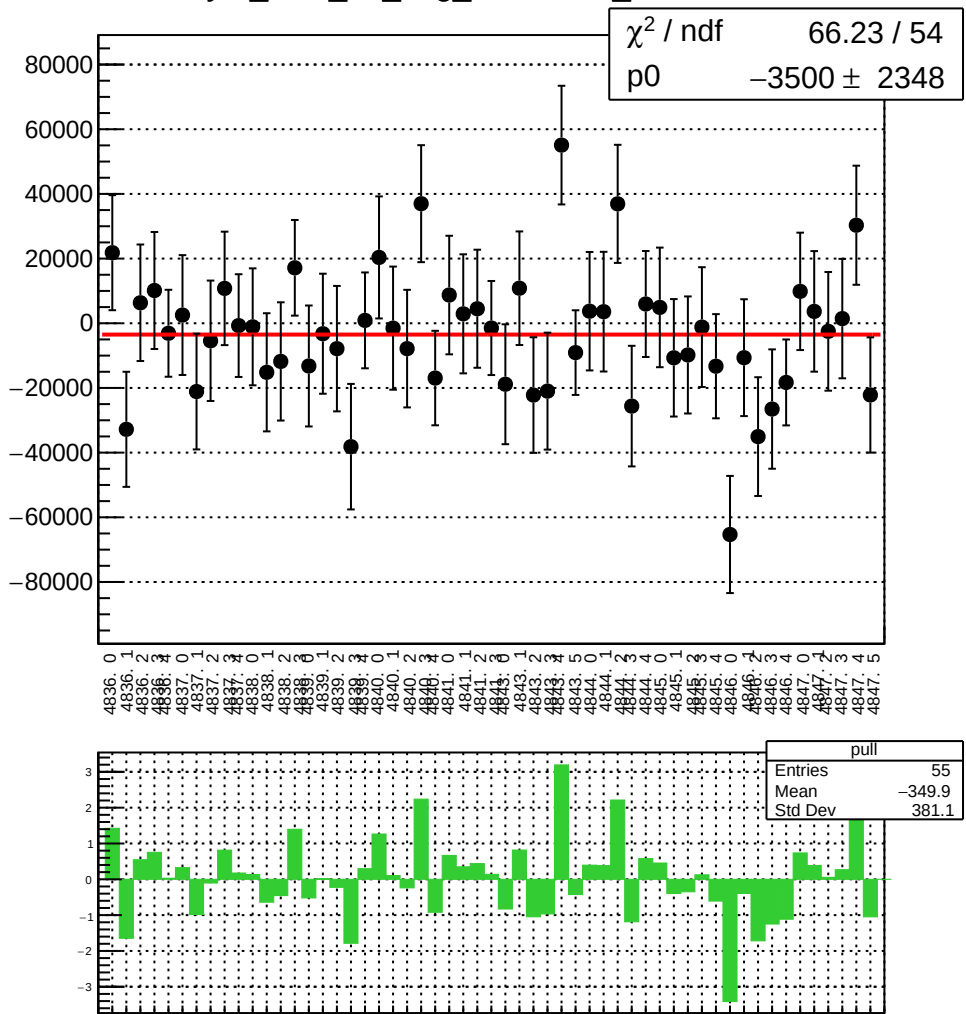
asym_sam_26_avg_correction_mean vs run
