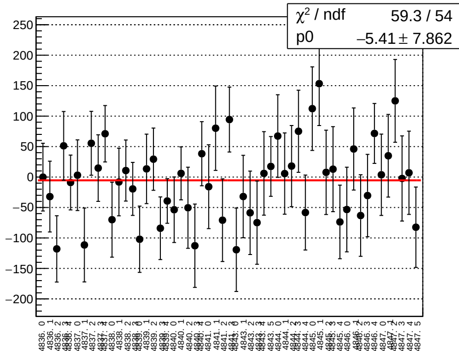
reg_asym_atl_dd_attr_dd_avg_diff_bpm4aY_slope vs un
