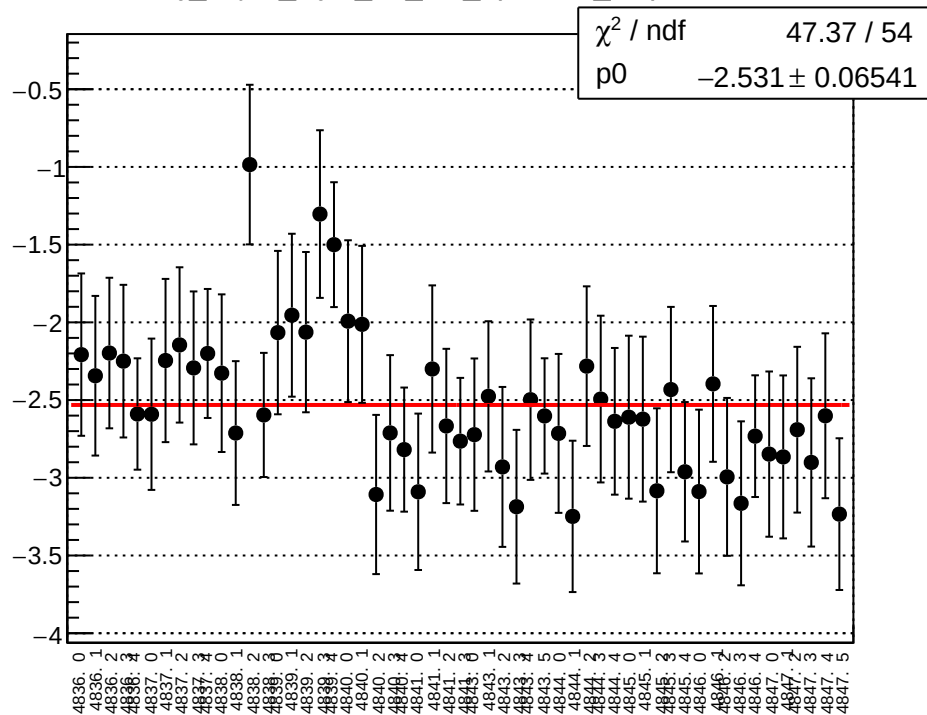
reg_asym_right_dd_diff_bpm4xX_slope vs run
