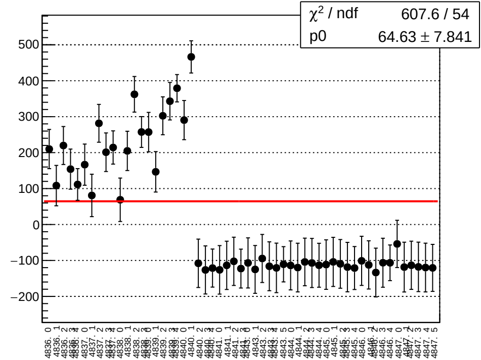
reg_asym_sam_37_dd_diff_bpm4aY_slope vs run
