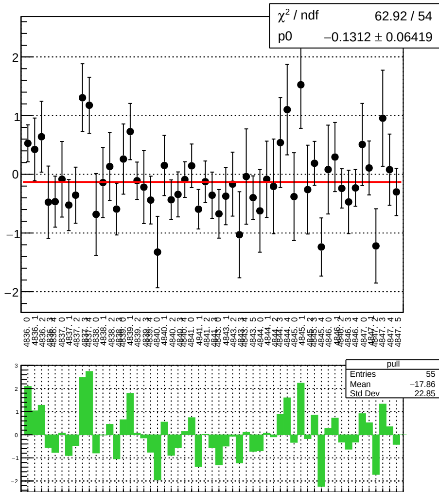
reg_bcm_cav4cQ_ds_dd_diff_bpm4eY_slope vs run
