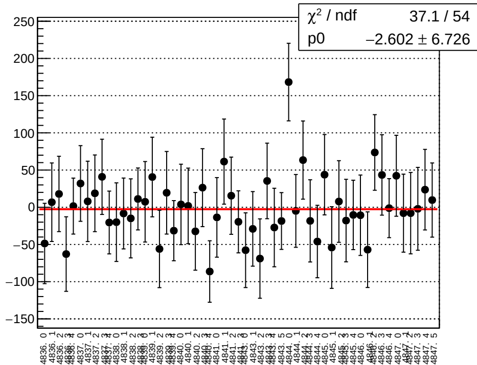
reg_asym_atl_dd_attr_dd_avg_diff_bpm4aX_slope vs run
