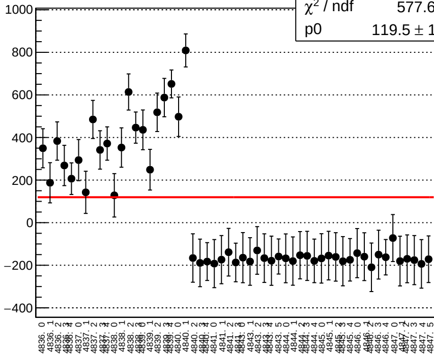
reg_asym_sam3_diff_bpm4aY_slope vs run
