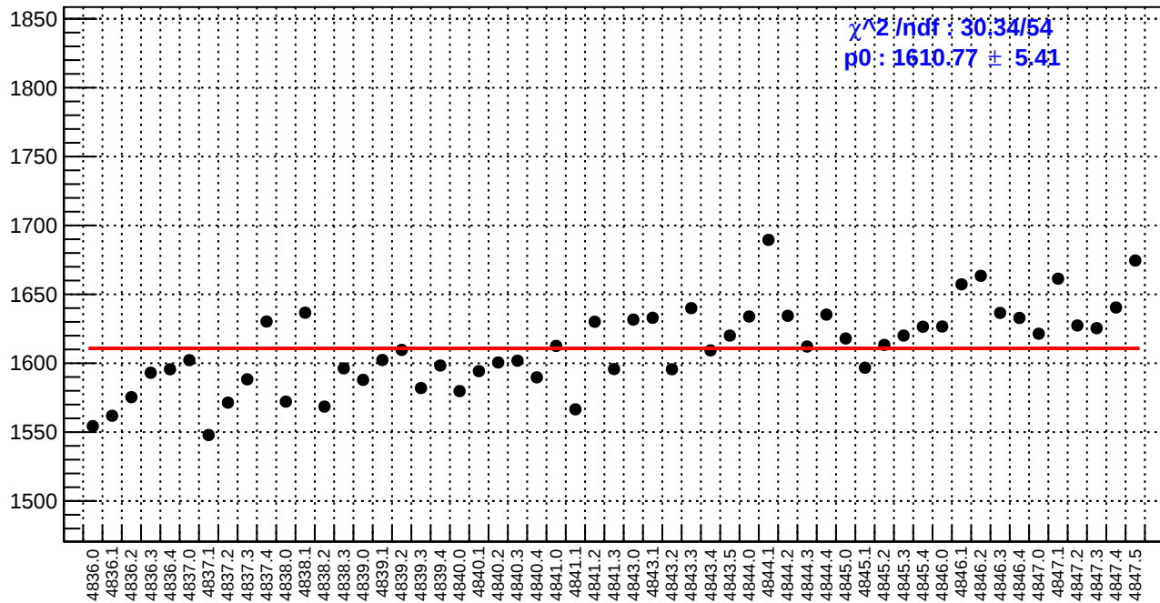
slug85: diff_bpm4aX.rms/nm
