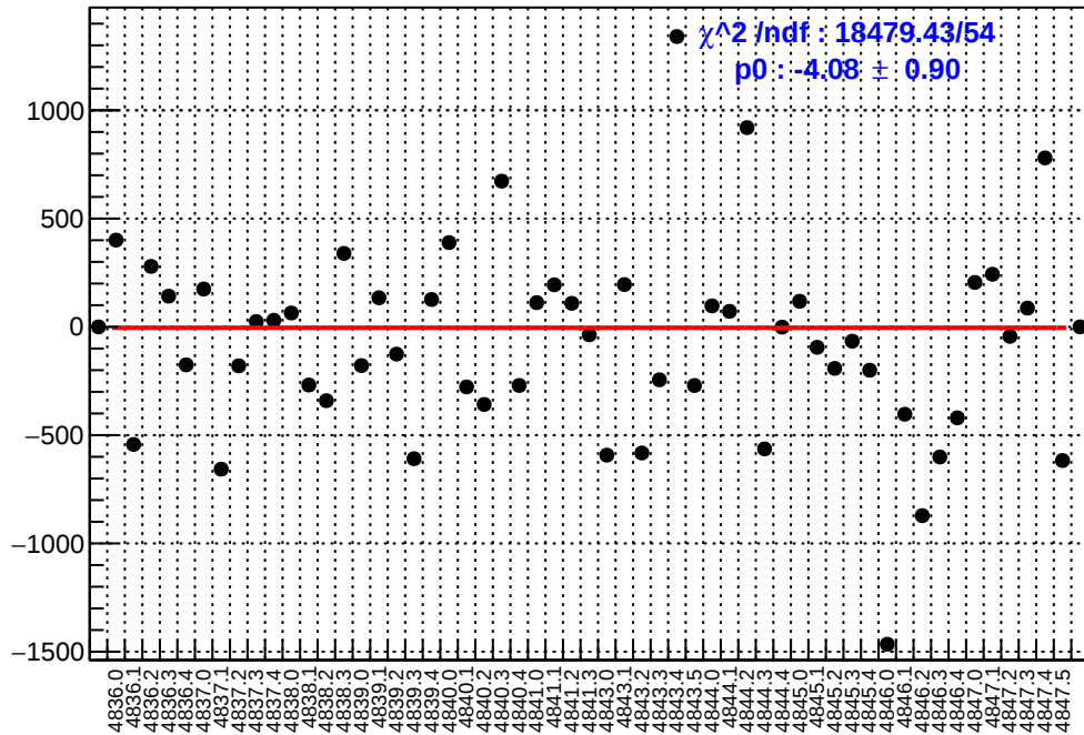
slug85: asym_right_dd.mean/ppb-reg_asym_right_dd.mean/ppb
