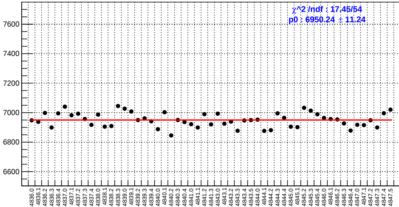
slug85: reg_asym_atr1l2_dd.rms/ppm
