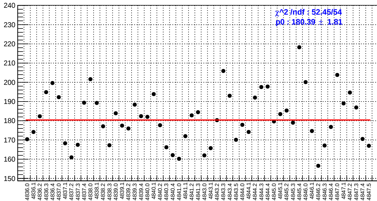
slug85: asym_bcm_an_ds.rms/ppm
