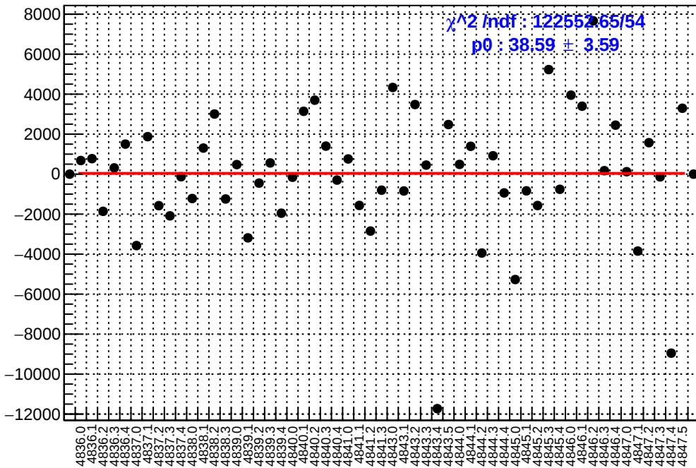
slug85: asym_at2_avg.mean/ppb-reg_asym_at2_avg.mean/ppb
