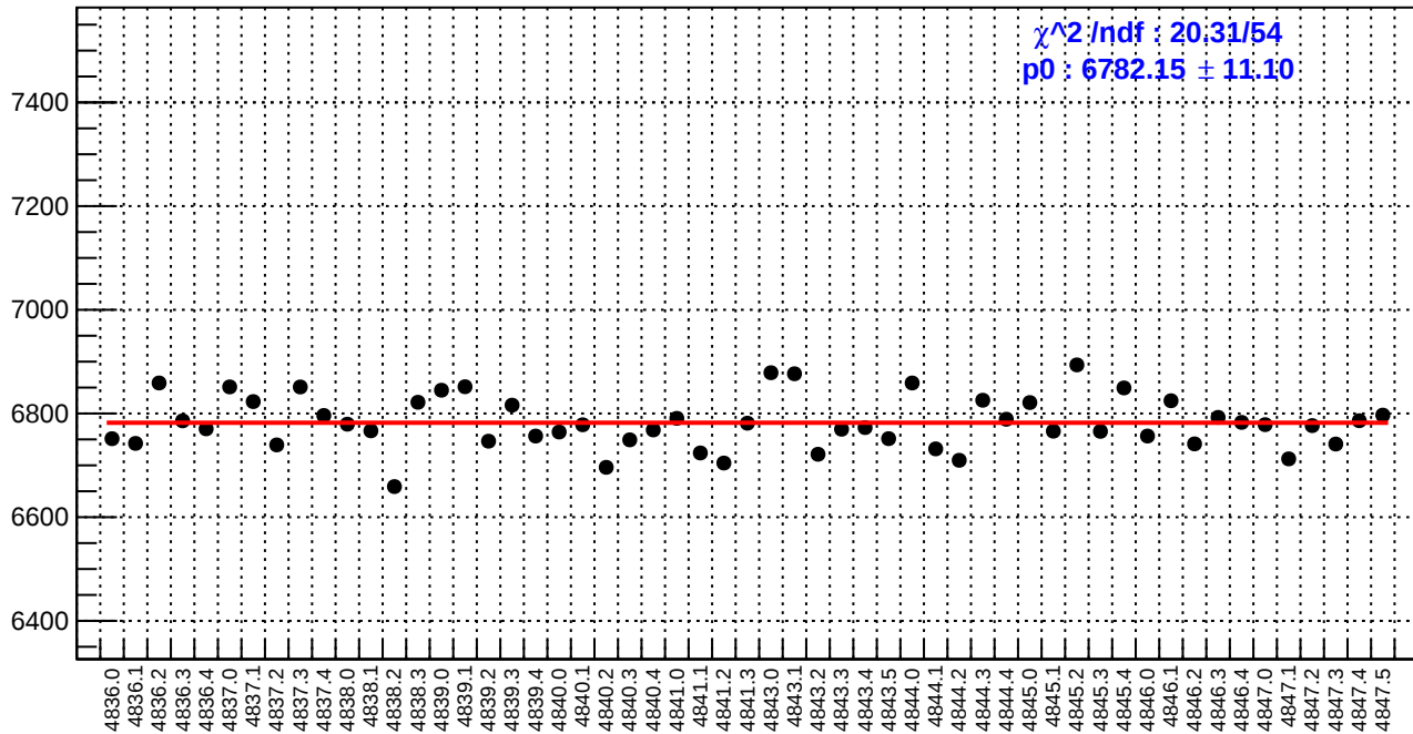
slug85: reg_asym_atl_avg.rms/ppm
