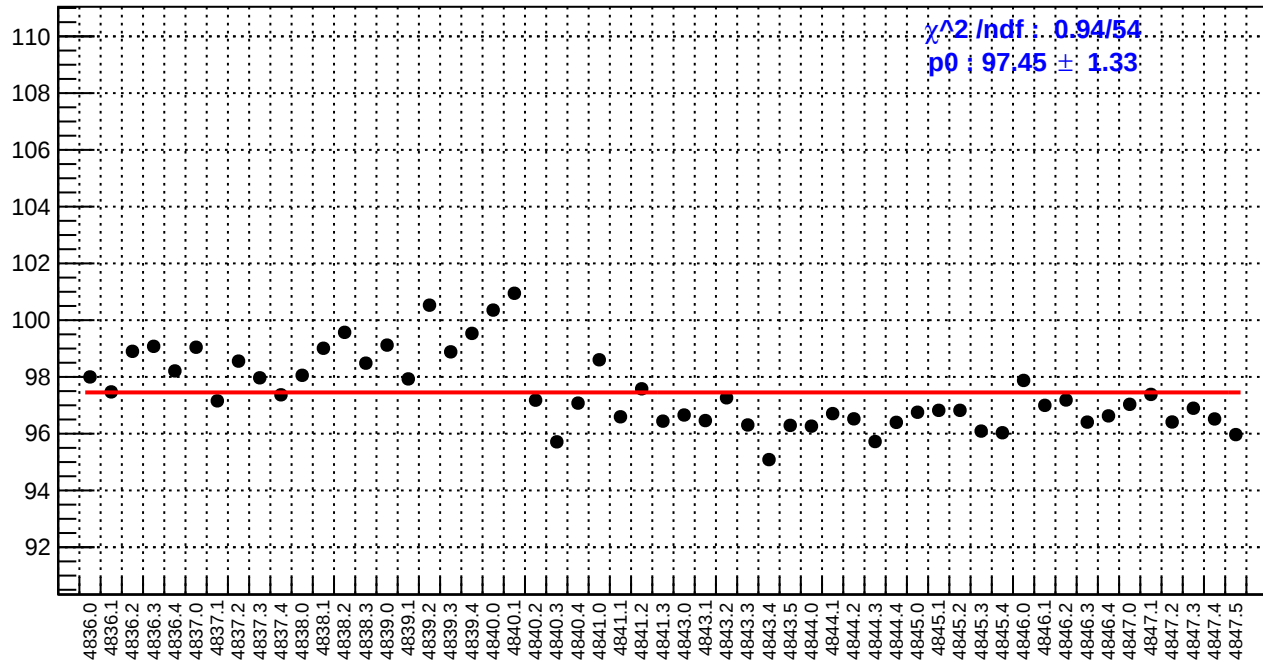
slug85: reg_asym_us_avg.rms/ppm
