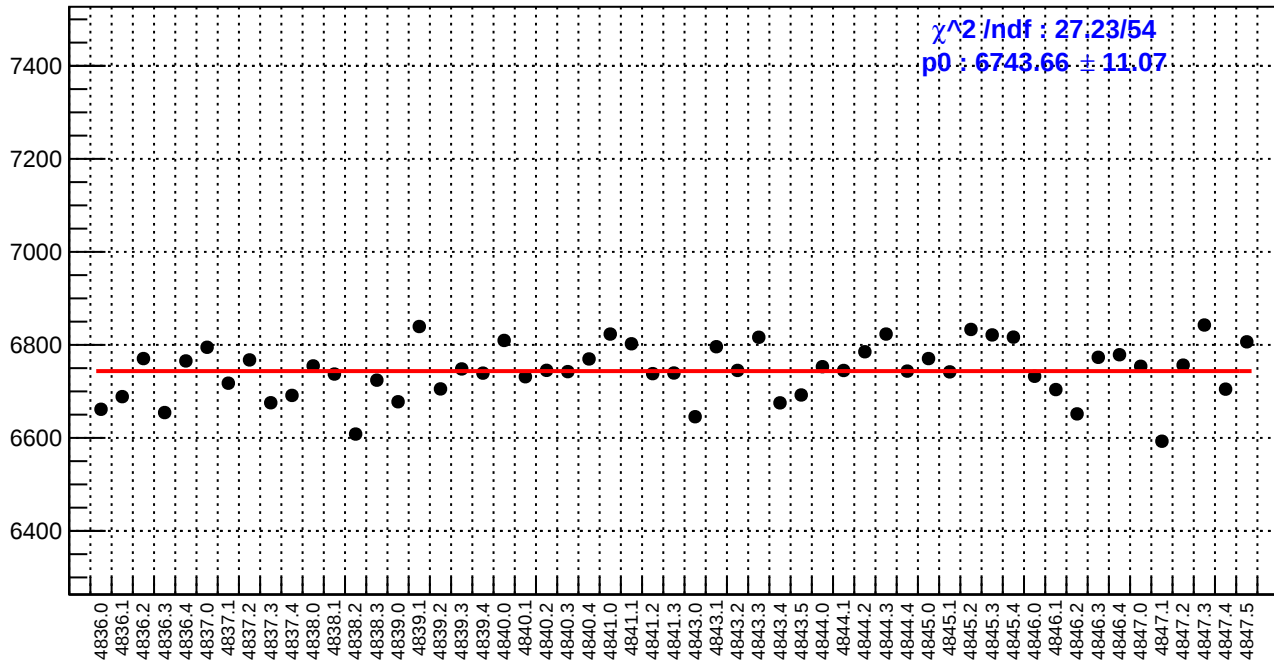
slug85: reg_asym_atl1r2_dd.rms/ppm
