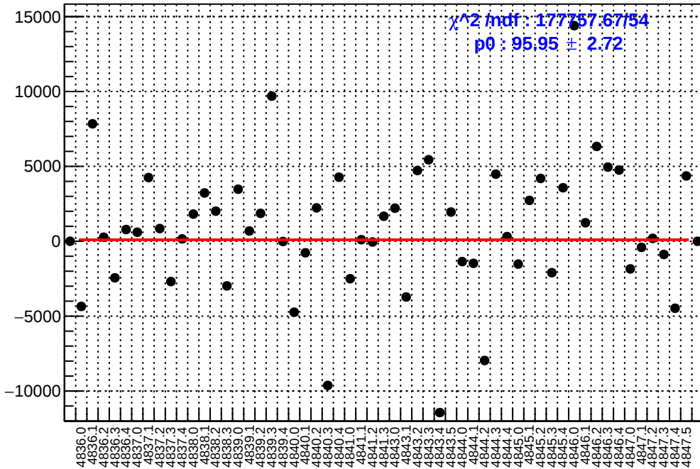
slug85: asym_us_dd.mean/ppb-reg_asym_us_dd.mean/ppb
