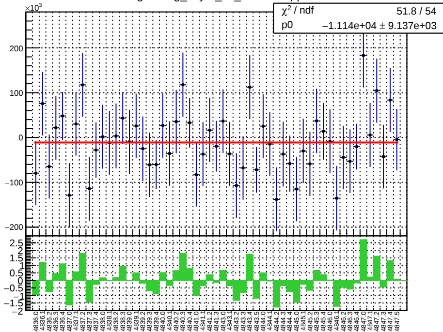
slug85: reg_asym_atl_dd.mean/ppb
