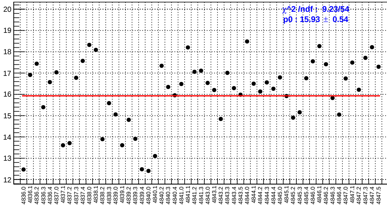
slug85: us_avg_bpm4aX/(ppb/nm)
