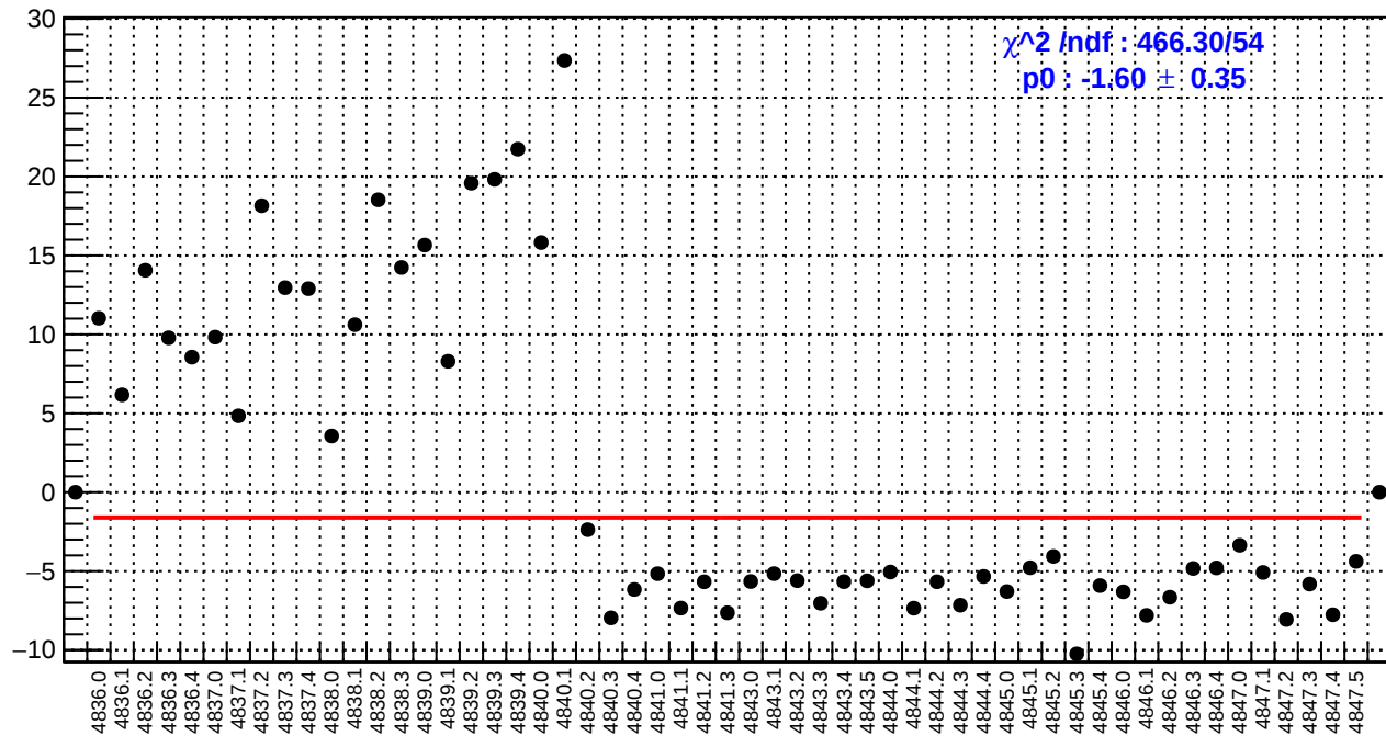
slug85: ds_avg_bpm4aY/(ppb/nm)
