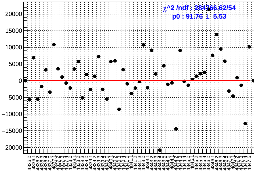
slug85: asym_usl.mean/ppb-reg_asym_usl.mean/ppb
