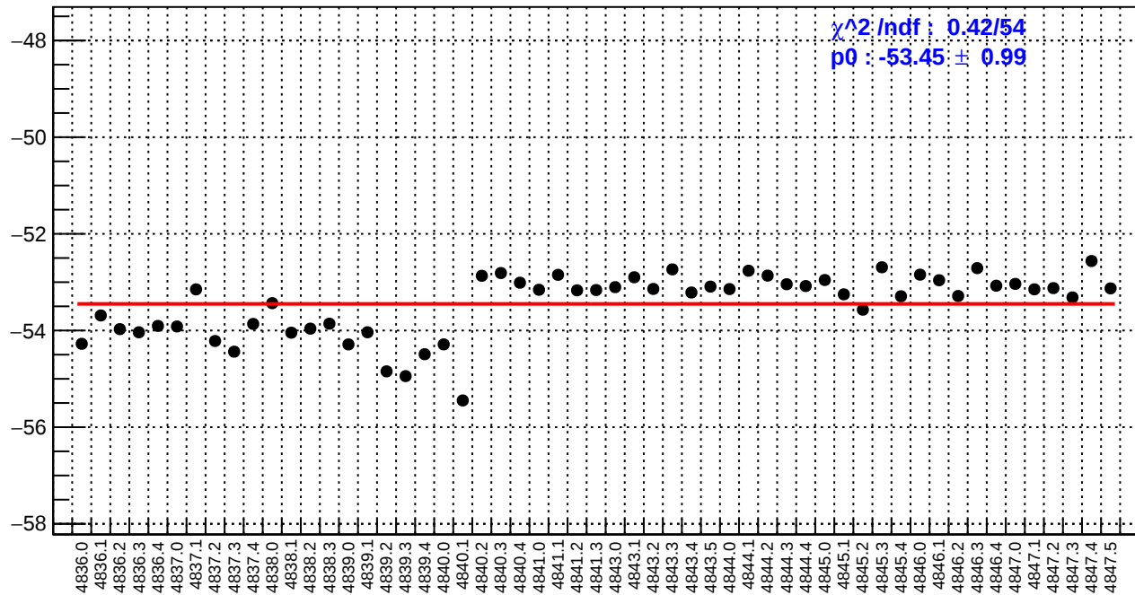
slug85: us_avg_bpm12X/(ppb/nm)
