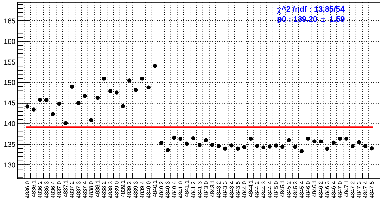
slug85: reg_asym_left_avg.rms/ppm
