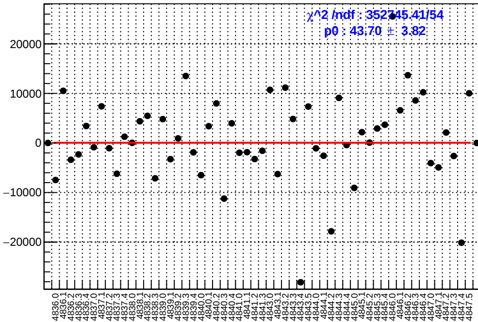
slug85: asym_atl2.mean/ppb-reg_asym_atl2.mean/ppb
