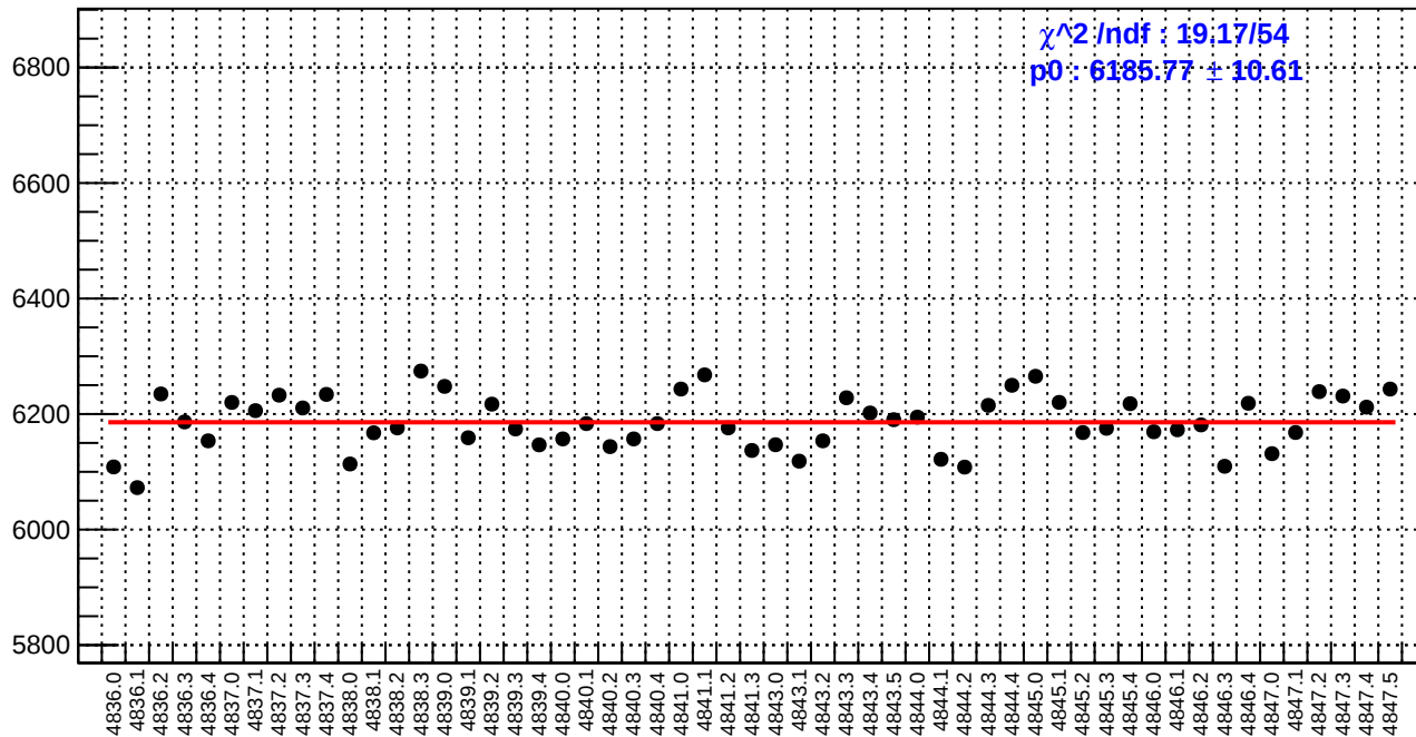
slug85: reg_asym_at1_avg.rms/ppm
