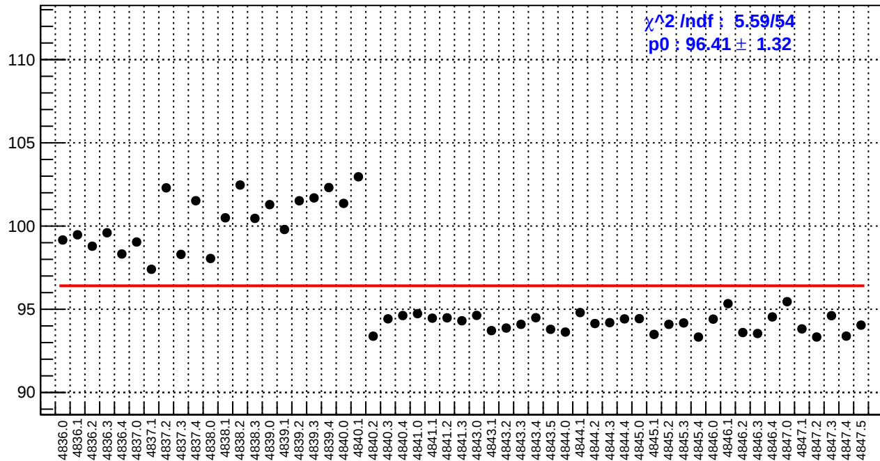
slug85: reg_asym_ds_dd.rms/ppm
