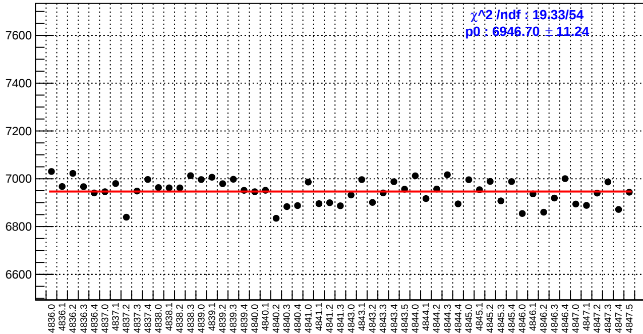
slug85: reg_asym_atr1l2_avg.rms/ppm
