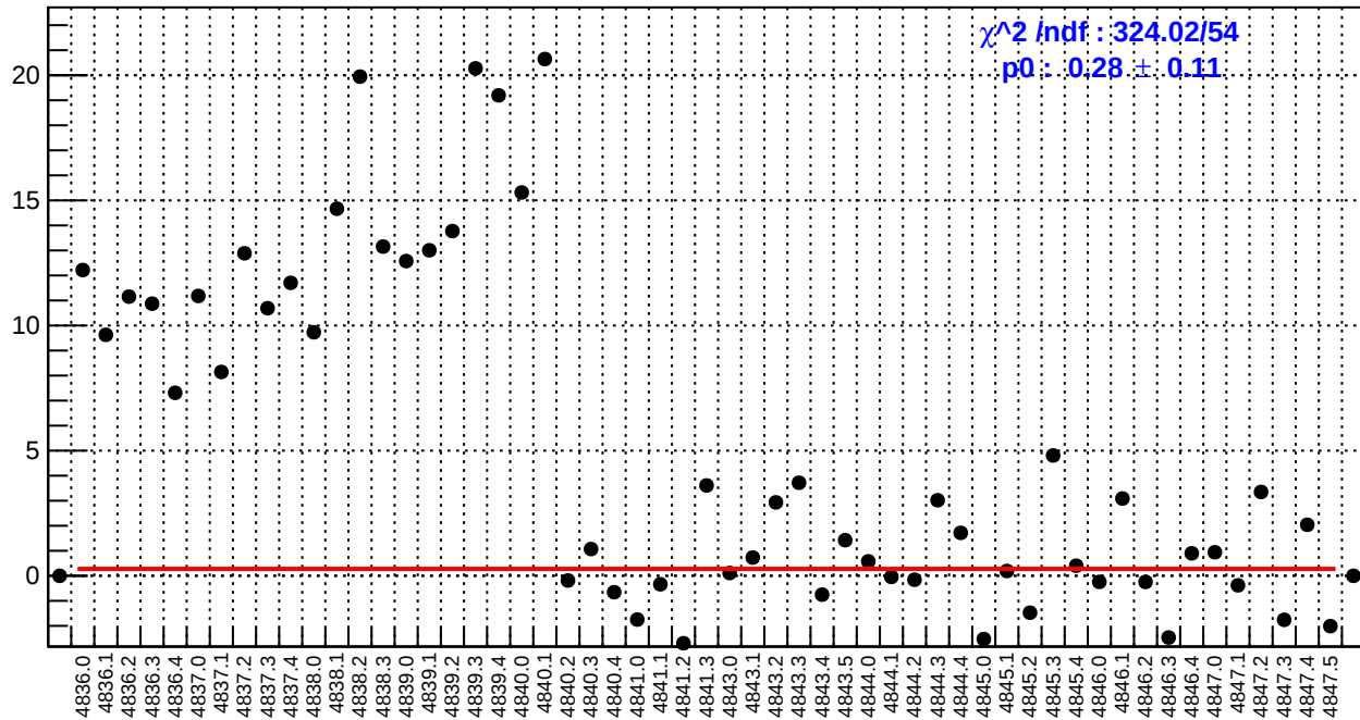
slug85: right_avg_bpm4eY/(ppb/nm)
