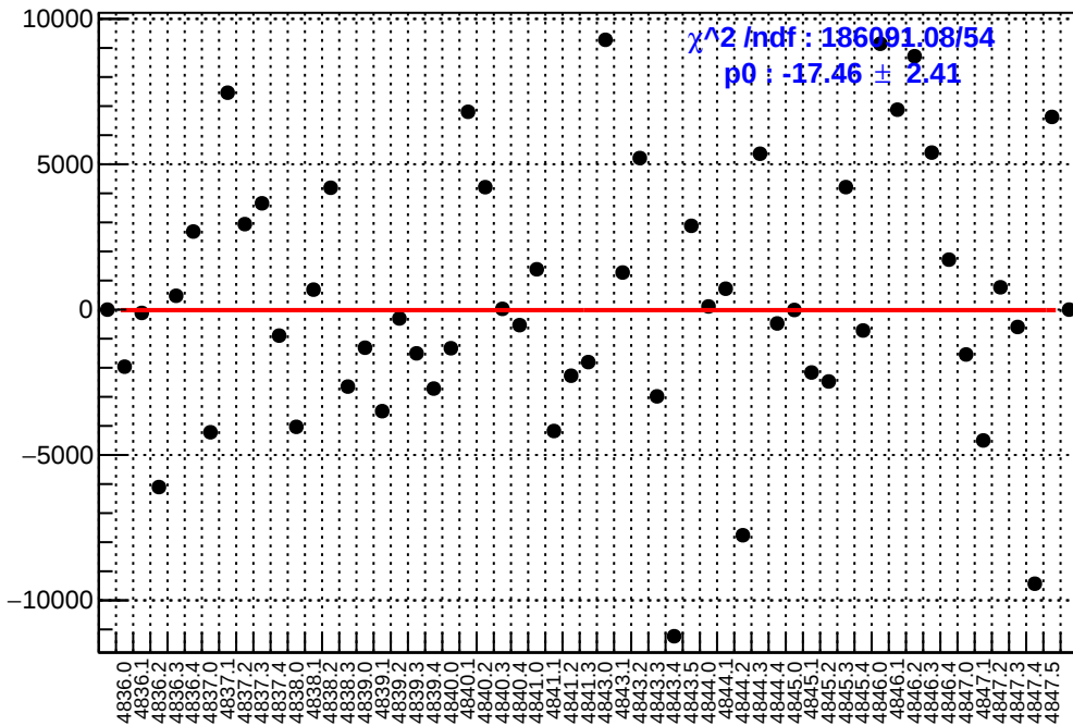
slug85: asym_ds_avg.mean/ppb-reg_asym_ds_avg.mean/ppb
