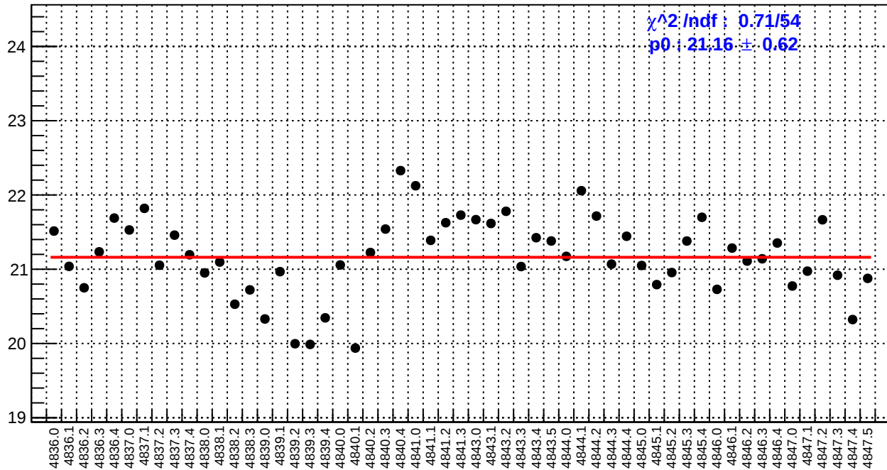
slug85: right_avg_bpm4eX/(ppb/nm)
