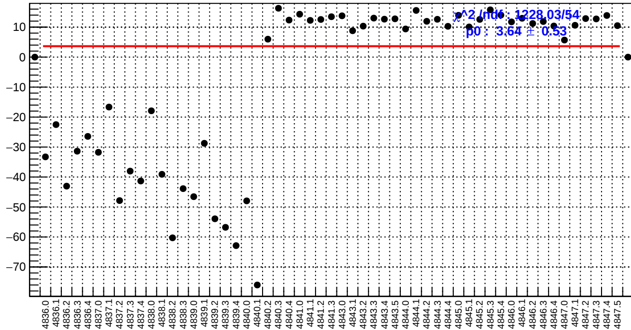
slug85: usl_bpm4eY/(ppb/nm)
