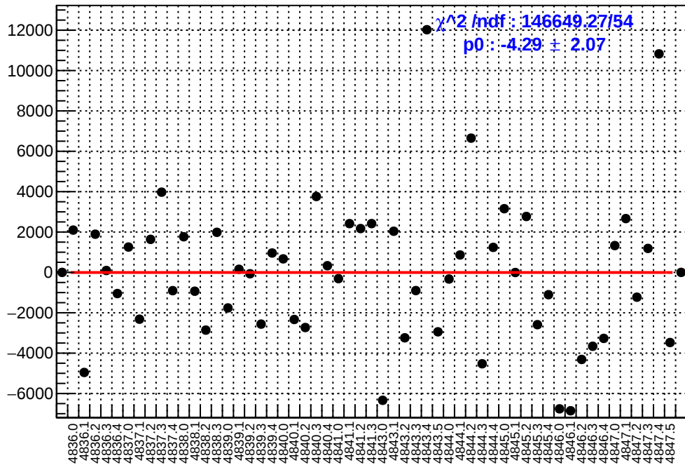
slug85: asym_atl_dd.mean/ppb-reg_asym_atl_dd.mean/ppb
