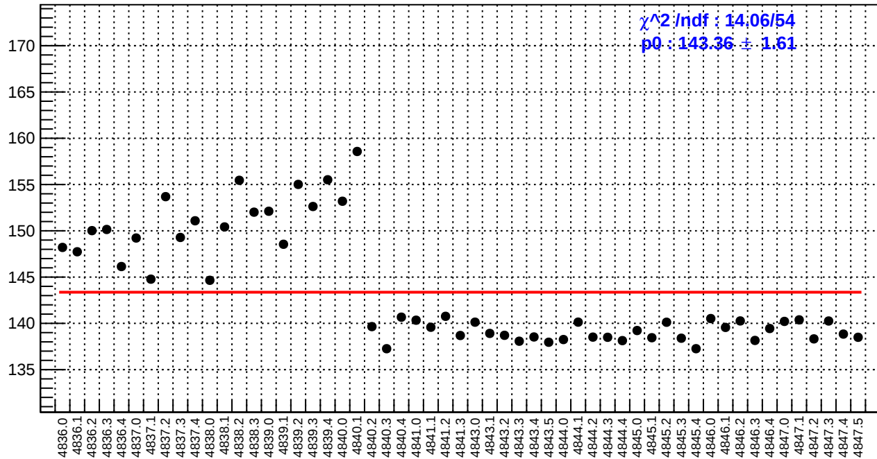
slug85: reg_asym_dsl.rms/ppm
