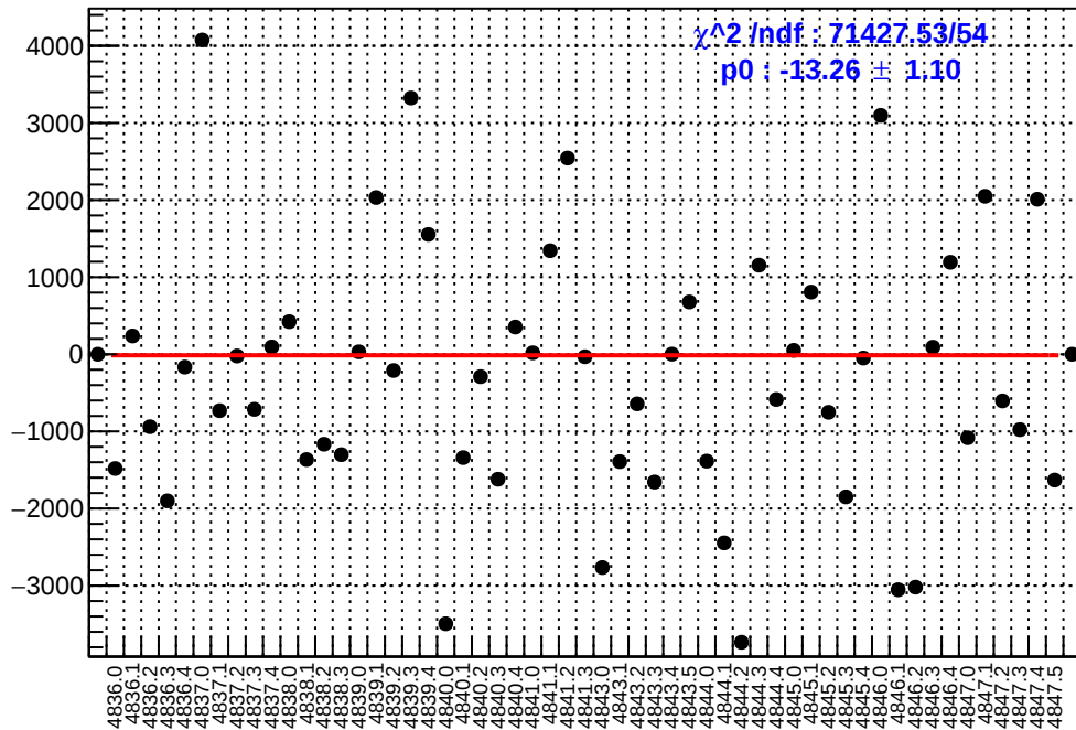
slug85: asym_atr_dd.mean/ppb-reg_asym_atr_dd.mean/ppb
