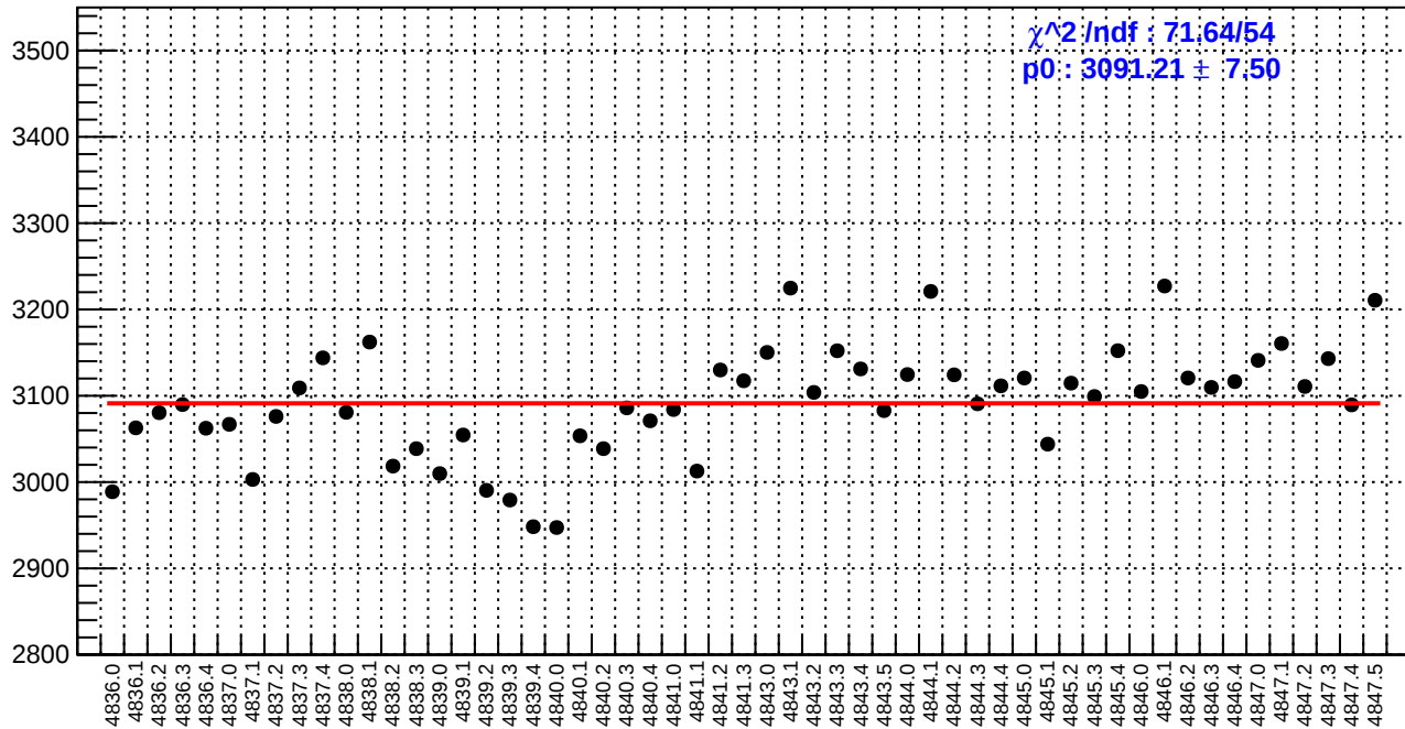
slug85: diff_bpm4aY.rms/nm
