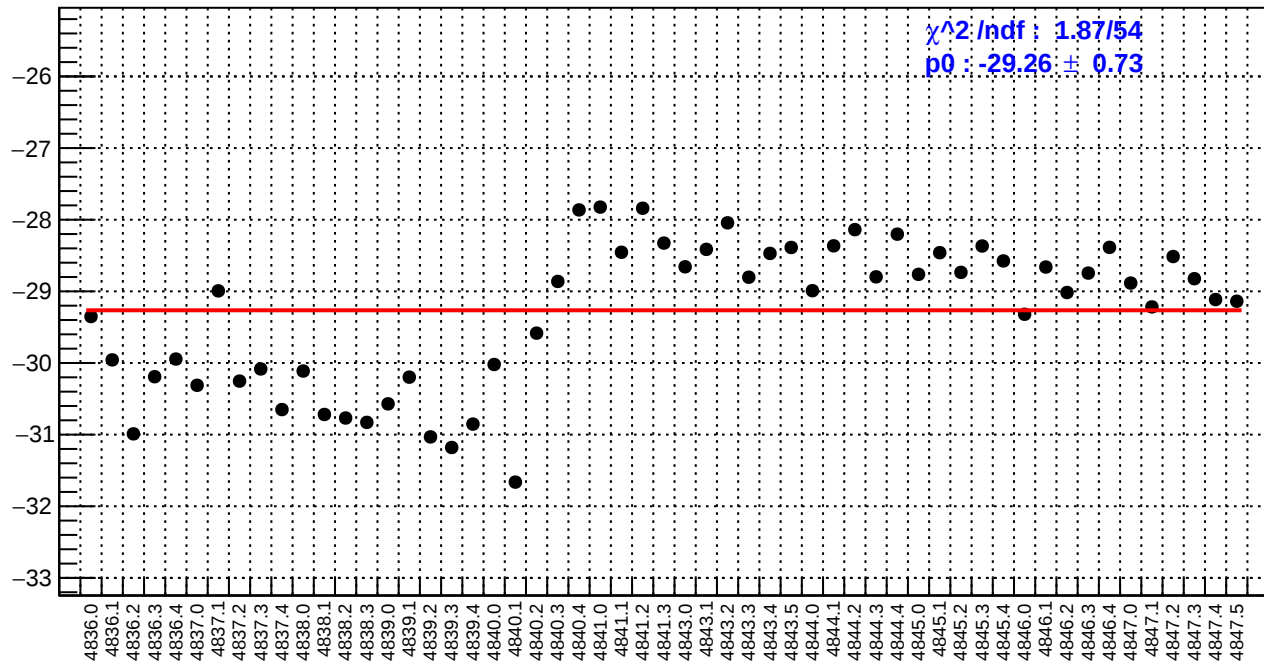
slug85: ds_avg_bpm4eX/(ppb/nm)
