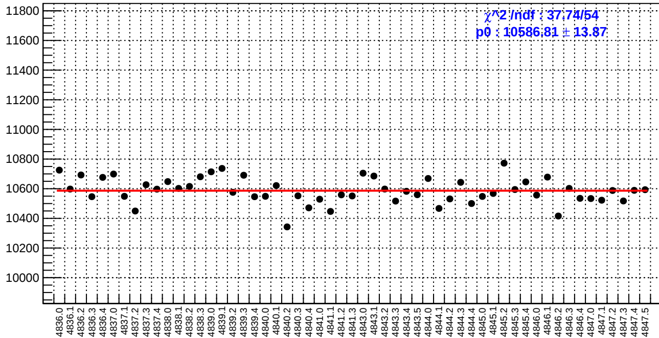
slug85: reg_asym_atl2.rms/ppm
