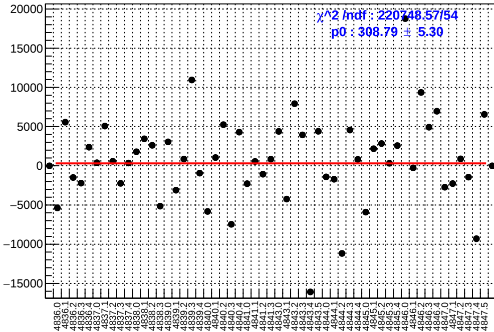
slug85: asym_atl_avg.mean/ppb-reg_asym_atl_avg.mean/ppb
