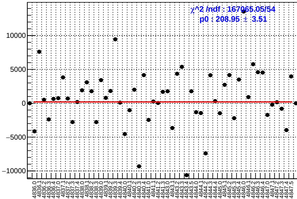
slug85: asym_ds_dd.mean/ppb-reg_asym_ds_dd.mean/ppb
