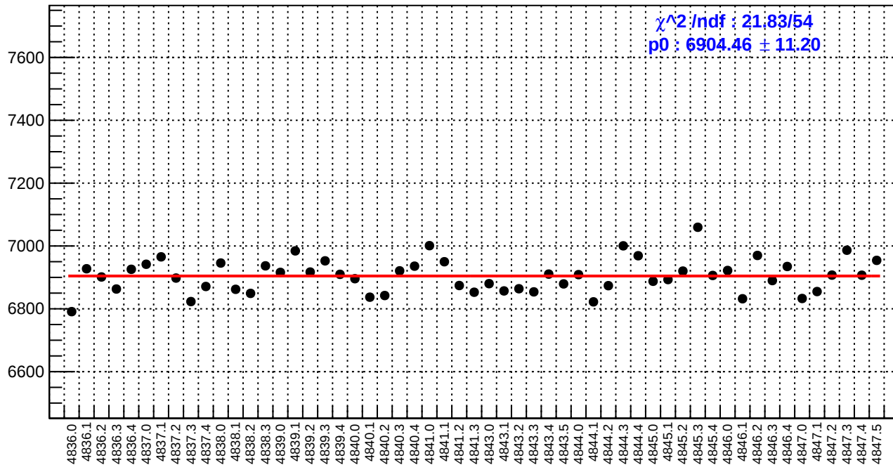
slug85: reg_asym_atr_dd.rms/ppm
