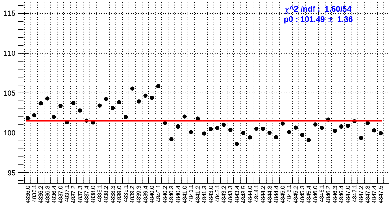
slug85: reg_asym_ds_avg.rms/ppm
