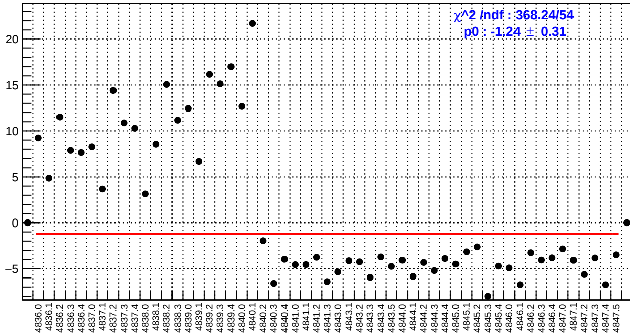
slug85: us_avg_bpm4aY/(ppb/nm)
