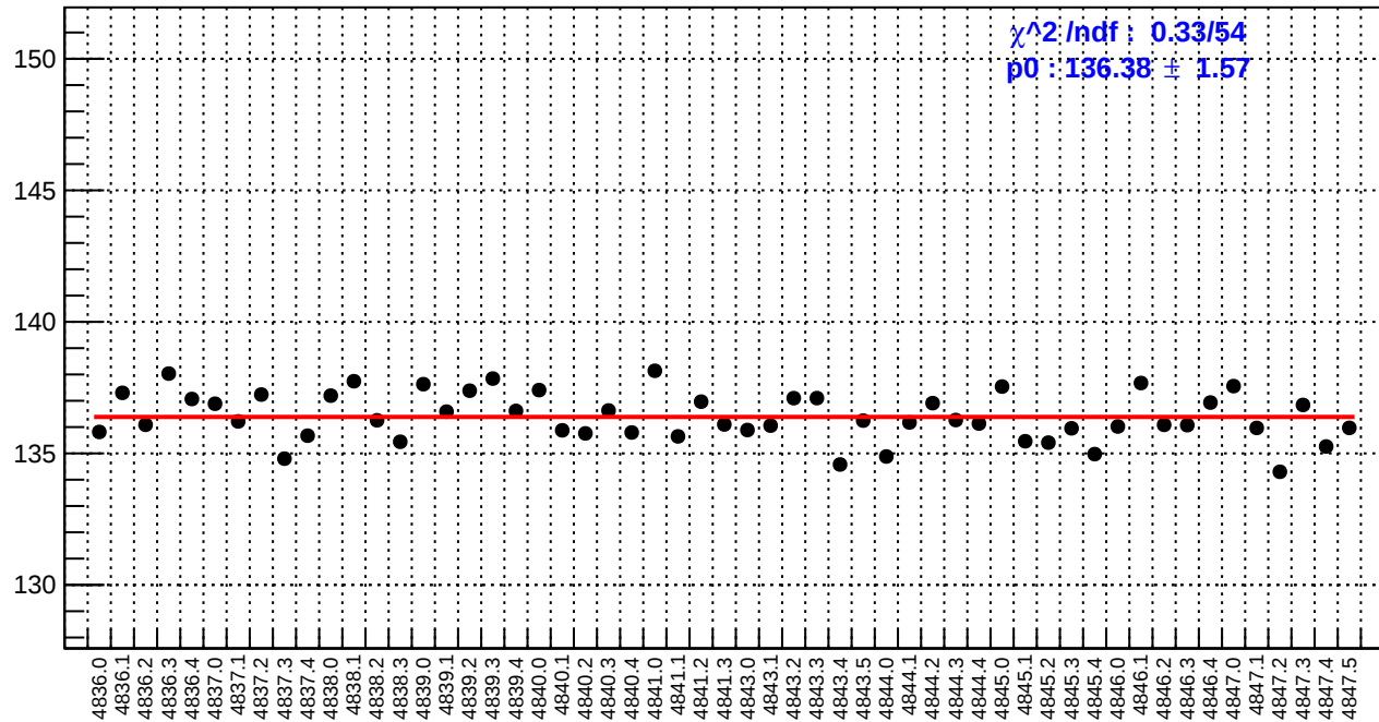
slug85: reg_asym_dsr.rms/ppm
