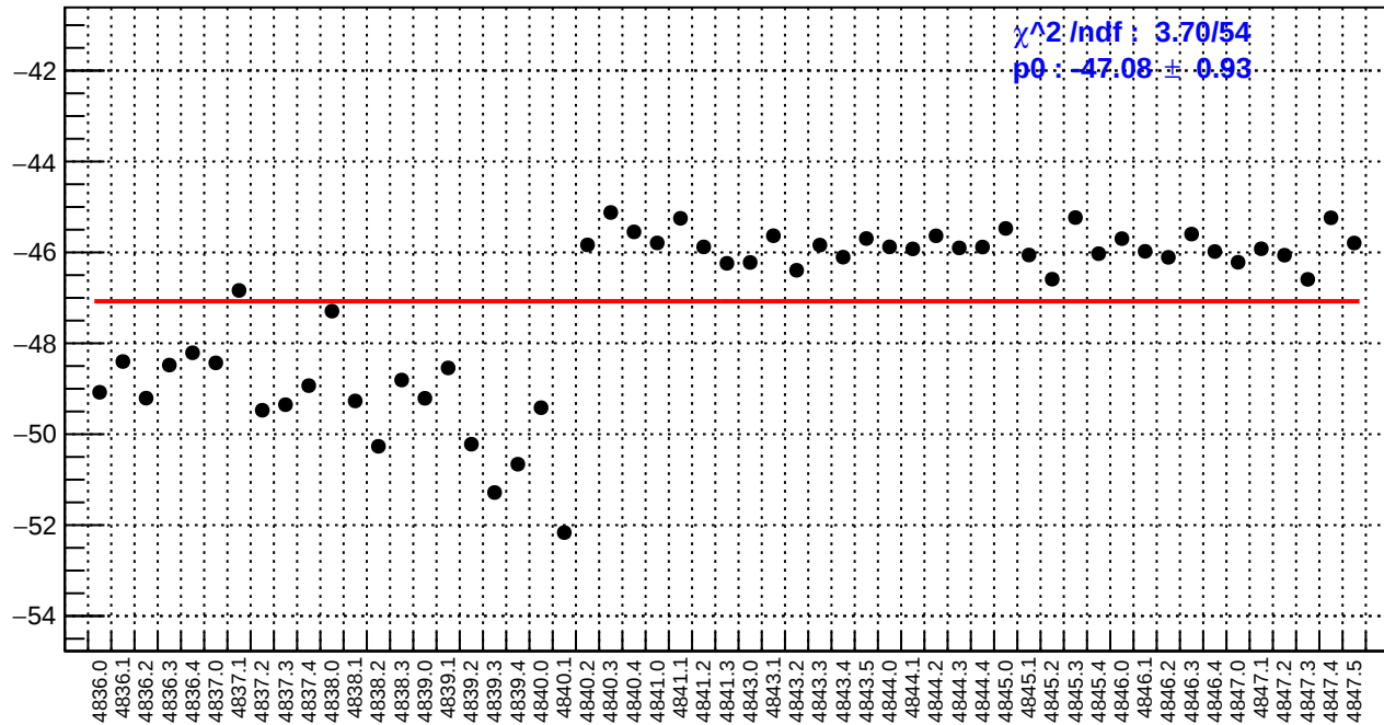
slug85: left_avg_bpm12X/(ppb/nm)
