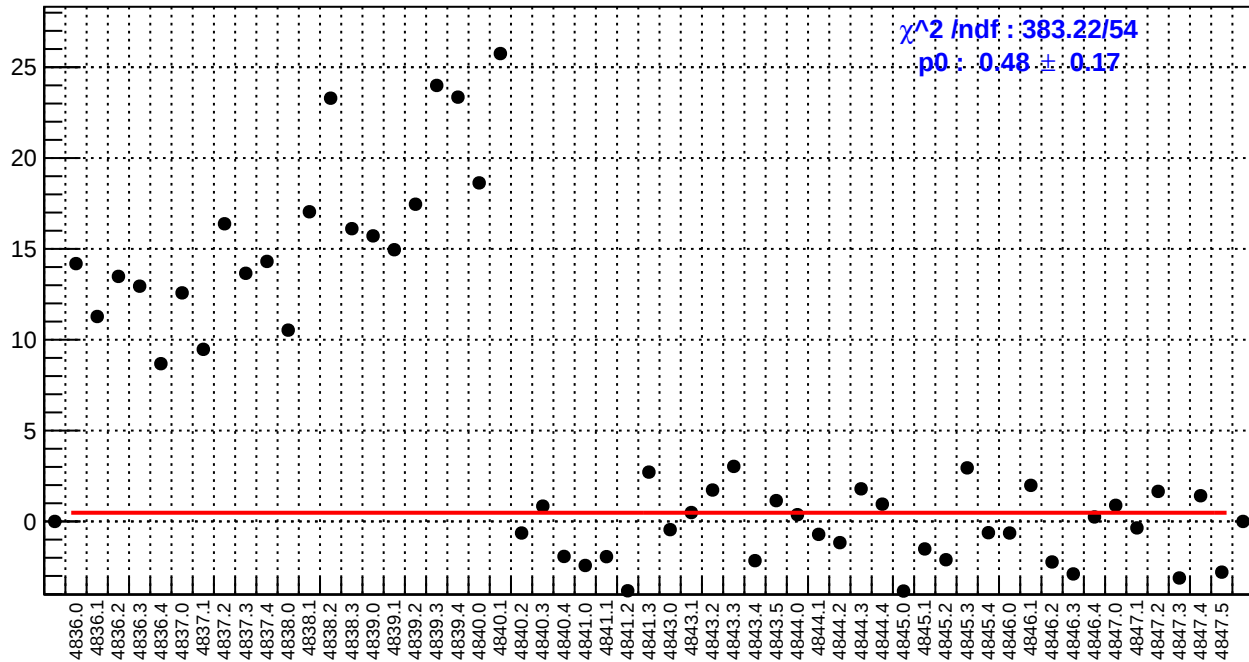
slug85: usr_bpm4eY/(ppb/nm)
