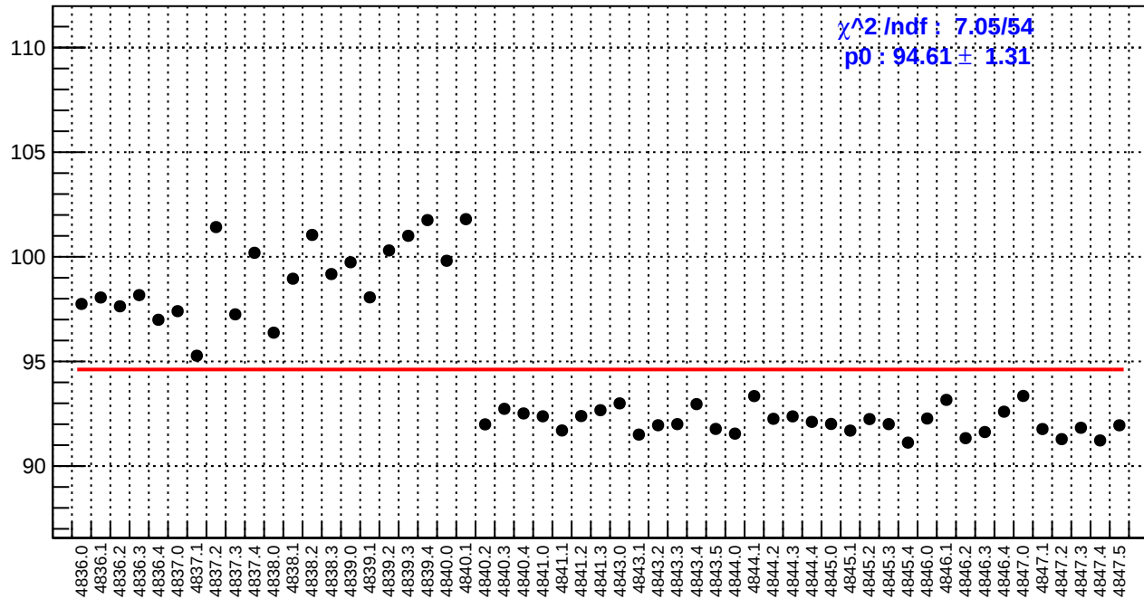
slug85: reg_asym_us_dd.rms/ppm
