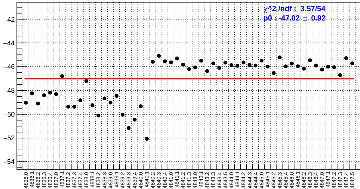
slug85: usl_bpm12X/(ppb/nm)
