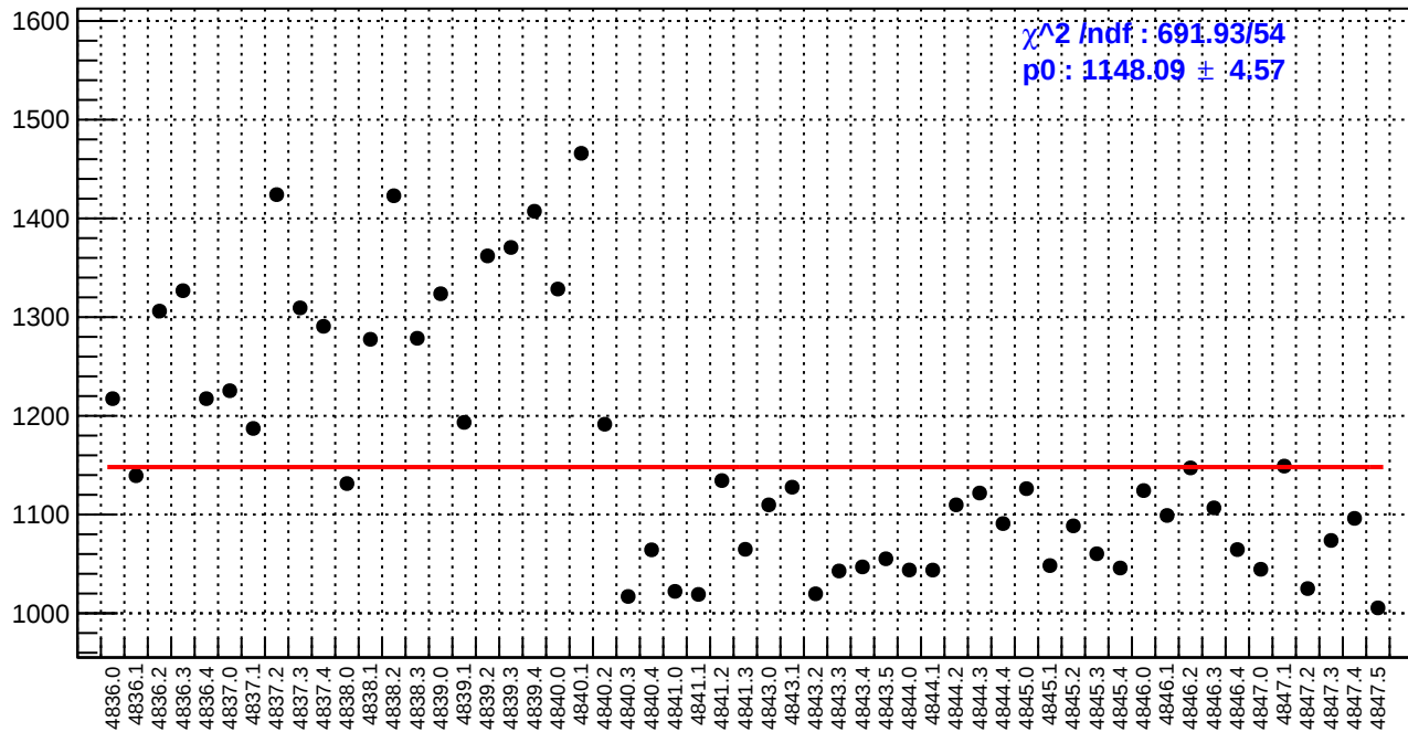
slug85: reg_asym_sam3.rms/ppm
