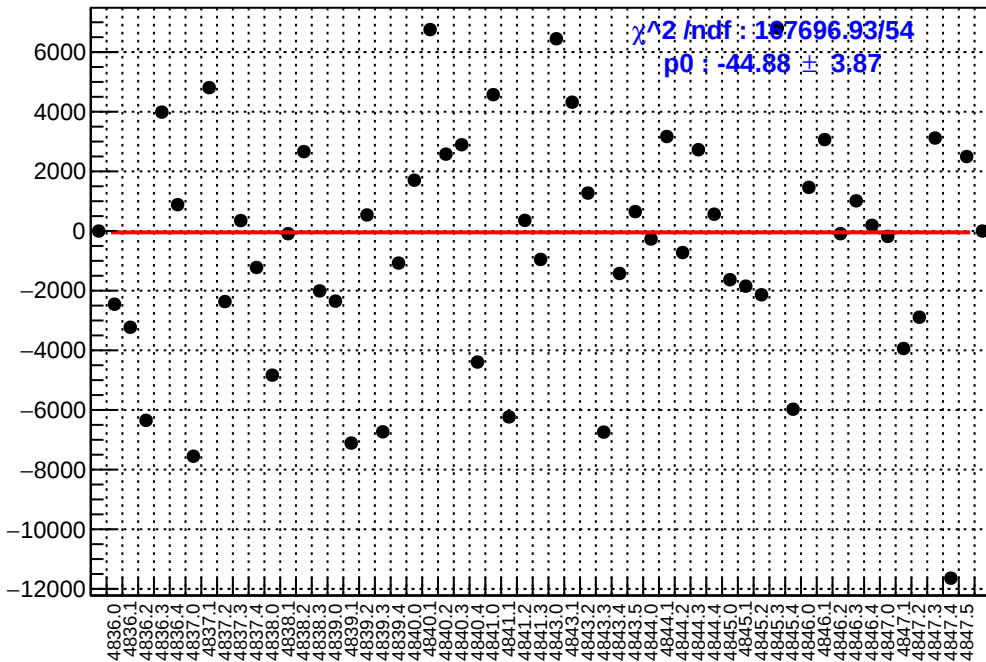
slug85: asym_sam1.mean/ppb-reg_asym_sam1.mean/ppb
