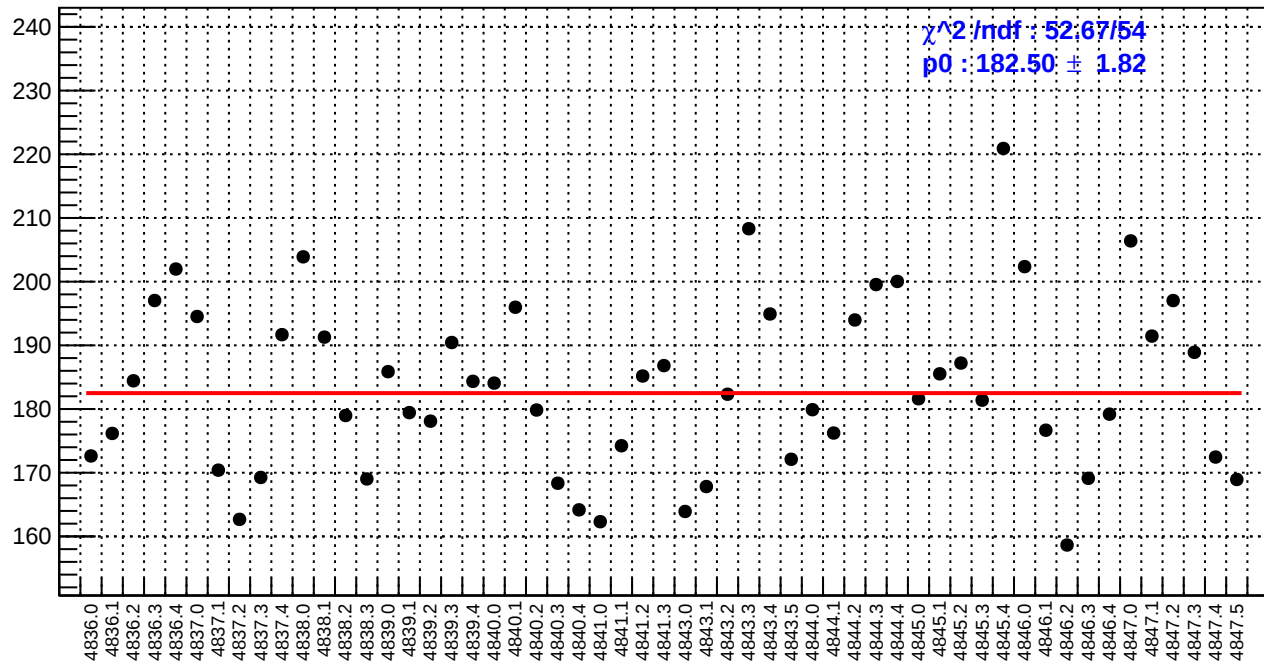
slug85: asym_bcm_an_ds3.rms/ppm
