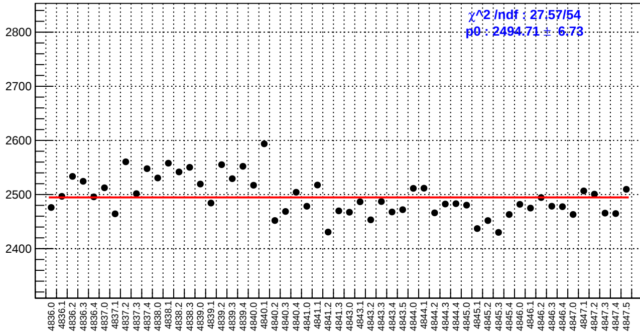
slug85: reg_asym_sam2.rms/ppm
