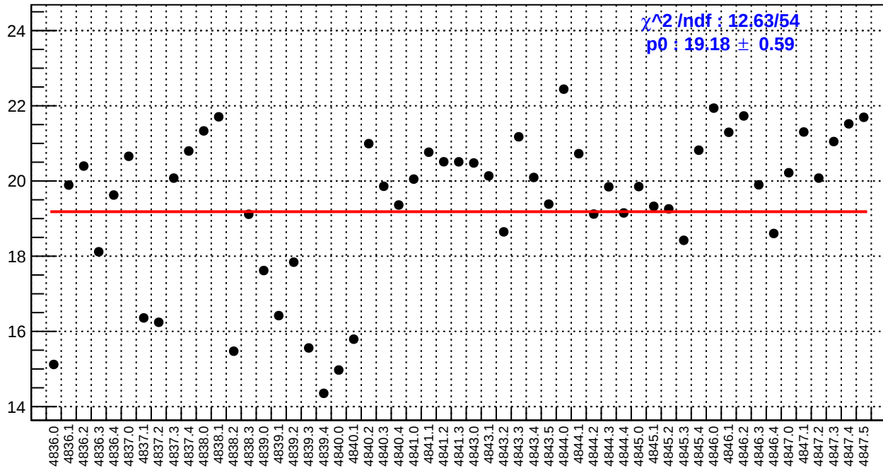
slug85: ds_avg_bpm4aX/(ppb/nm)
