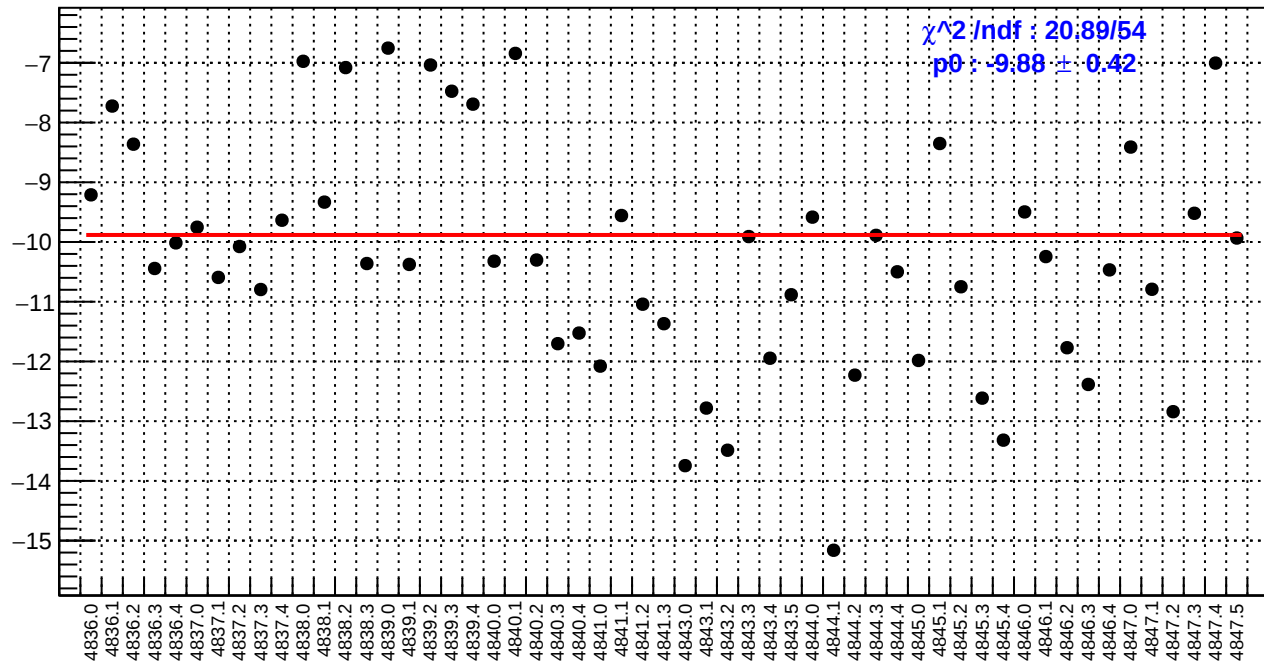
slug85: right_avg_bpm4aX/(ppb/nm)
