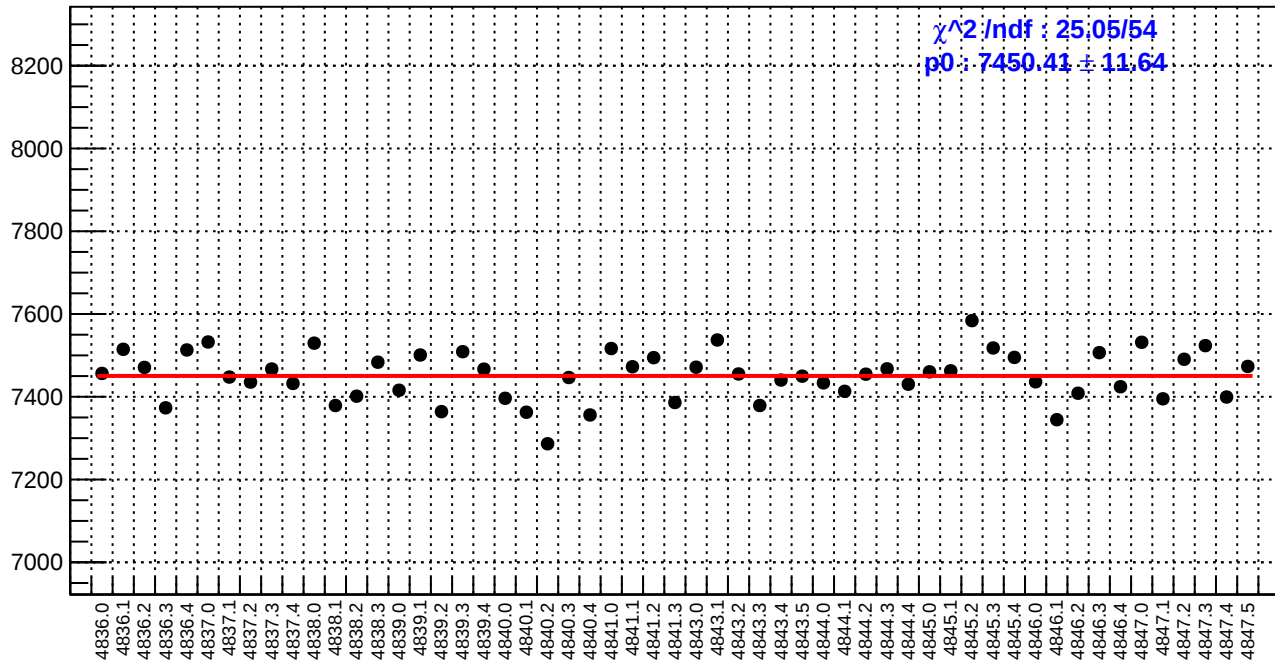
slug85: reg_asym_at2_avg.rms/ppm
