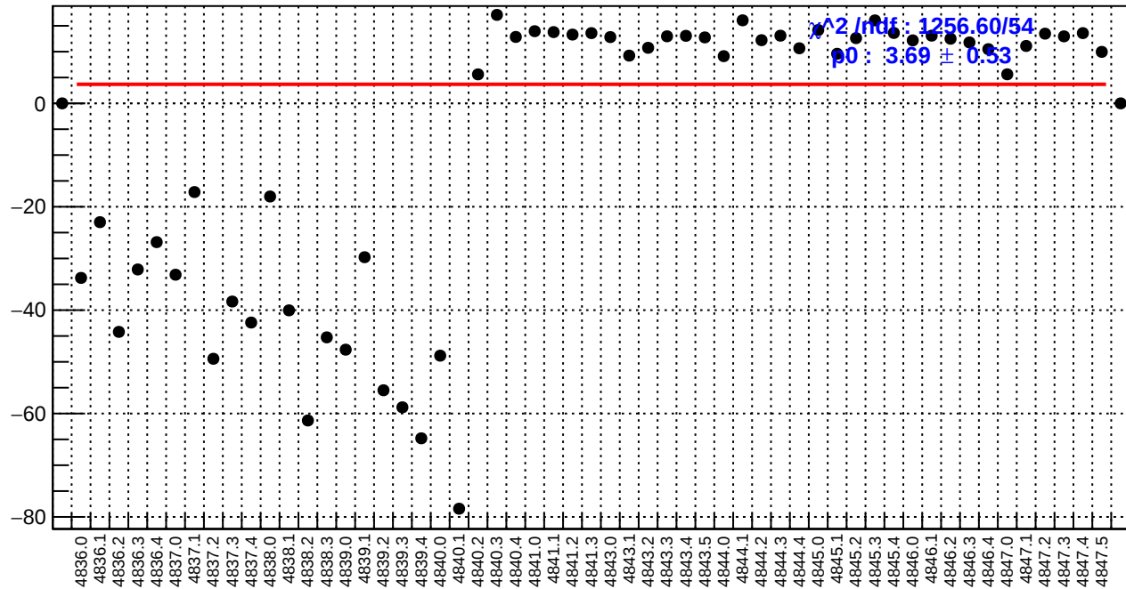
slug85: left_avg_bpm4eY/(ppb/nm)
