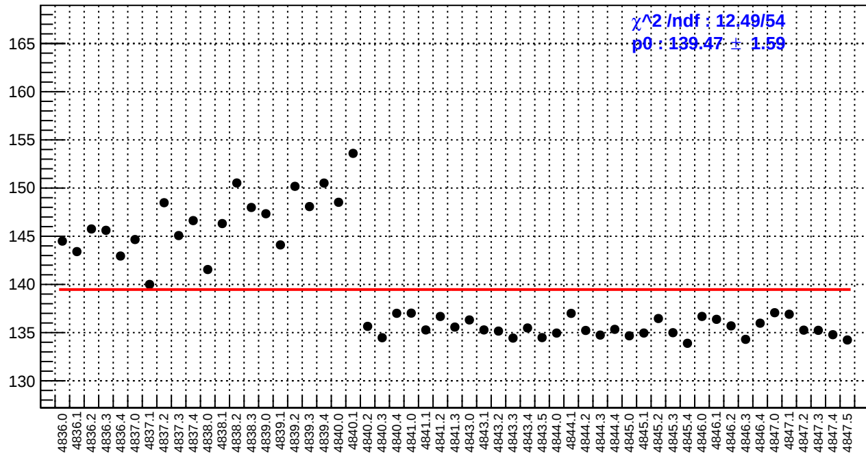
slug85: reg_asym_usl.rms/ppm
