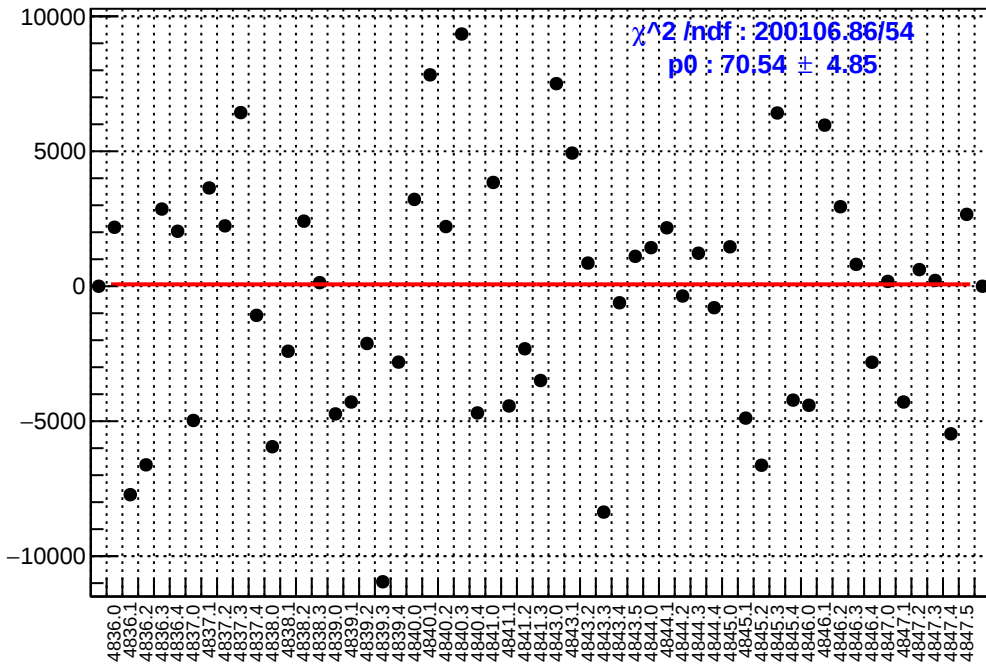
slug85: asym_dsr.mean/ppb-reg_asym_dsr.mean/ppb
