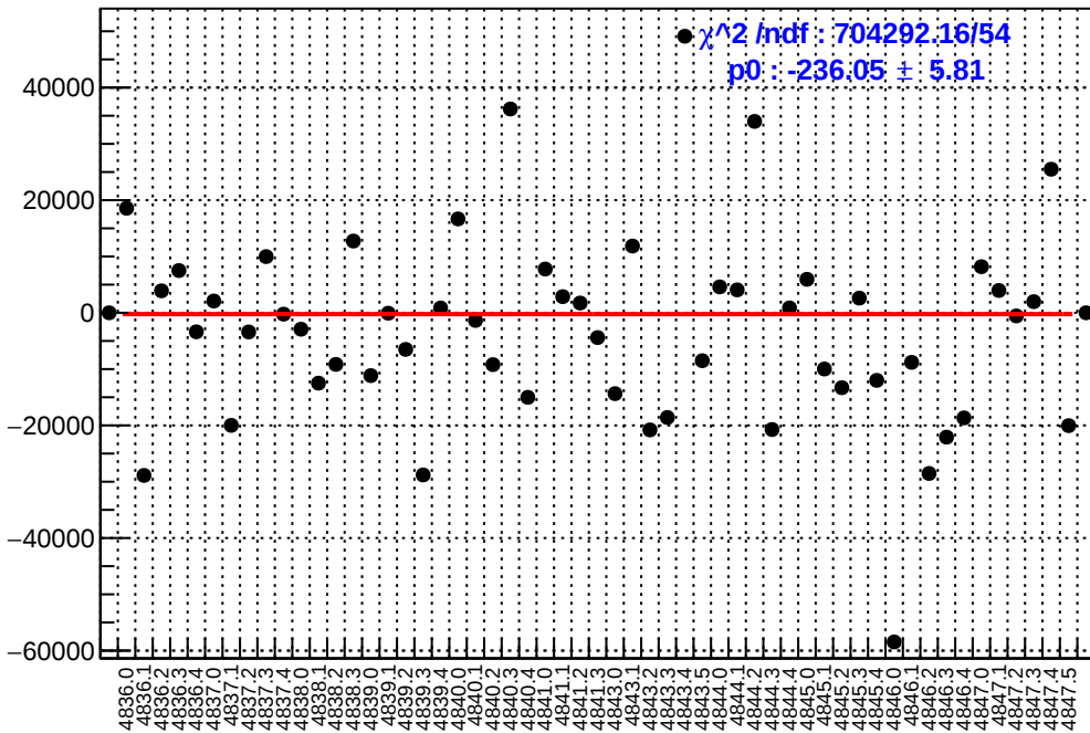
slug85: asym_sam7.mean/ppb-reg_asym_sam7.mean/ppb
