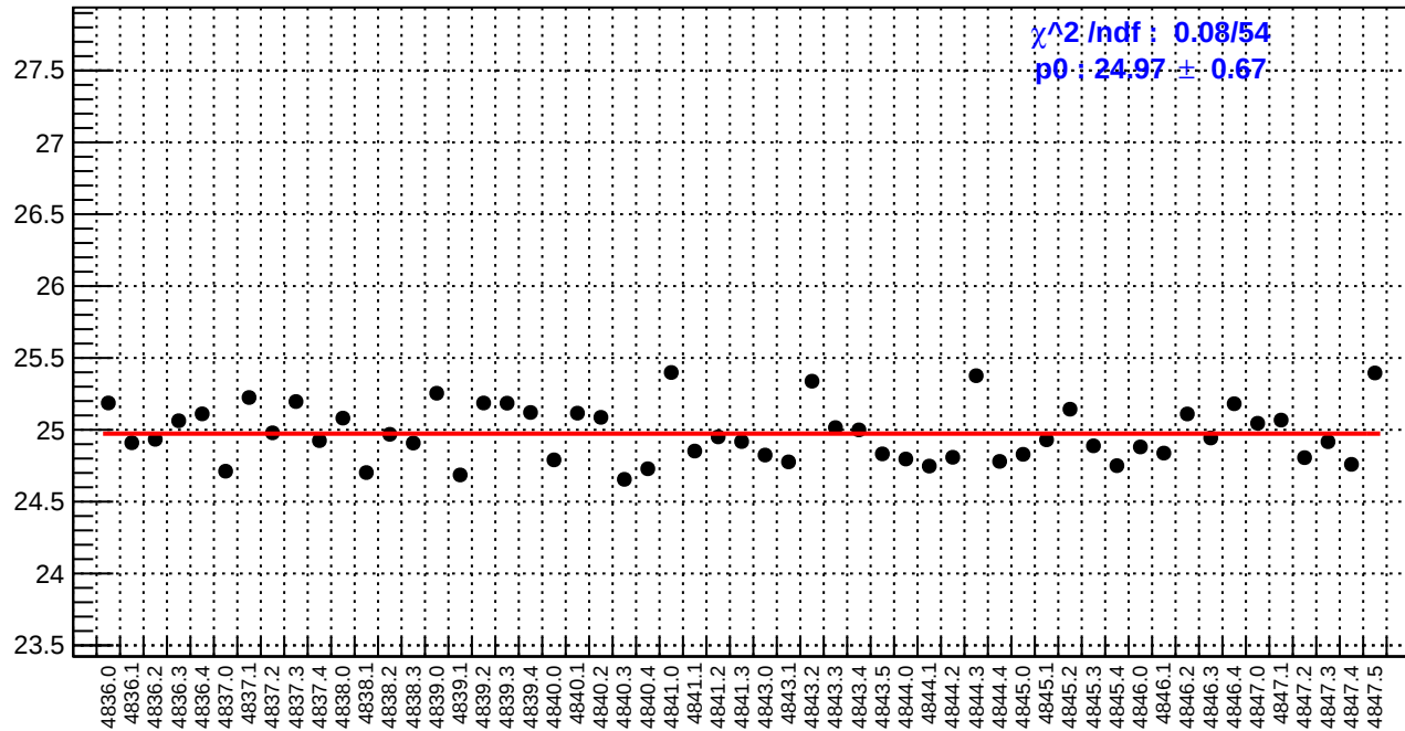
slug85: reg_asym_left_dd.rms/ppm
