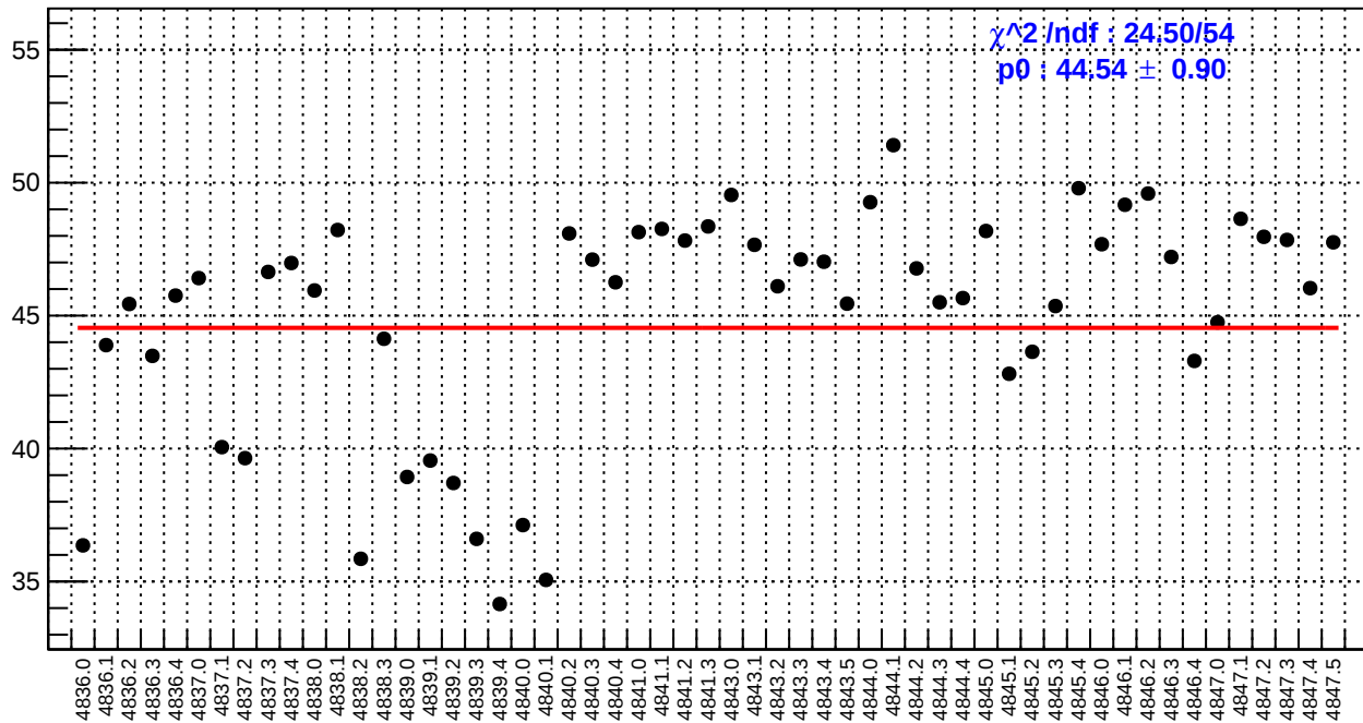
slug85: usl_bpm4aX/(ppb/nm)
