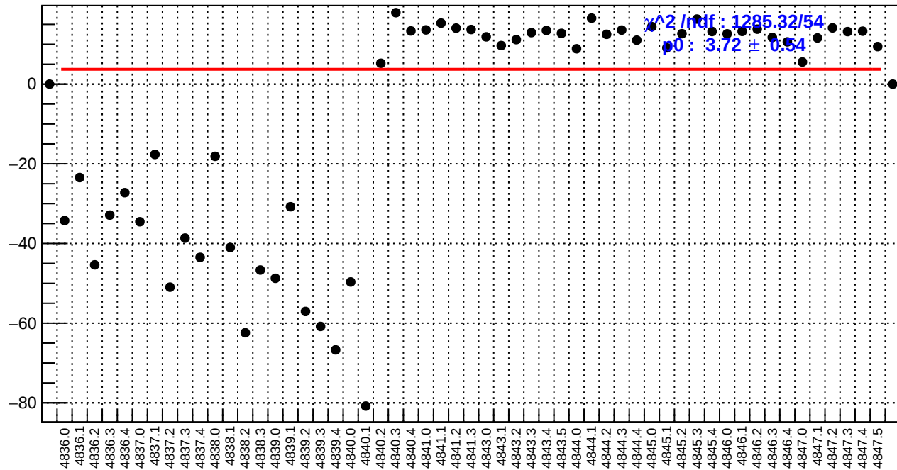
slug85: dsl_bpm4eY/(ppb/nm)
